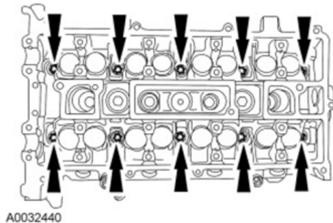
Fig. 345: Locating Cylinder Head Bolts Courtesy of FORD MOTOR CO.
