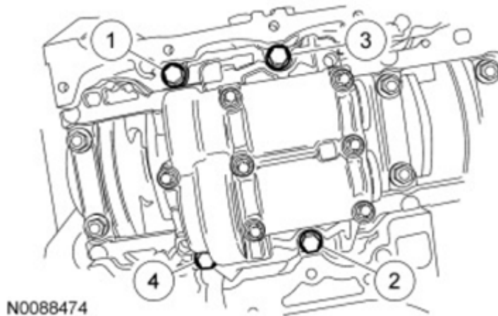
Fig. 16: Tightening Sequence Of Balancer Unit Bolts Courtesy of FORD MOTOR CO.
