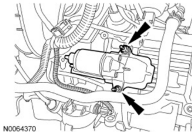
Fig. 274: Locating Starter Motor Stud Bolts Courtesy of FORD MOTOR CO.
