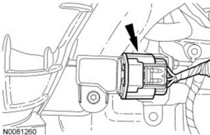
Fig. 301: Locating Manifold Absolute Pressure (MAP) Sensor Electrical Connector Courtesy of FORD MOTOR CO.
