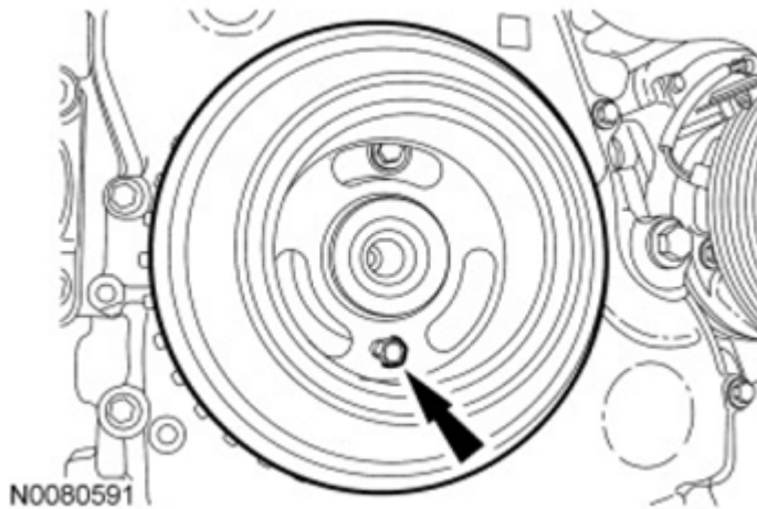
Fig. 33: View Of Crankshaft Pulley Alignment Bolt Courtesy of FORD MOTOR CO.
