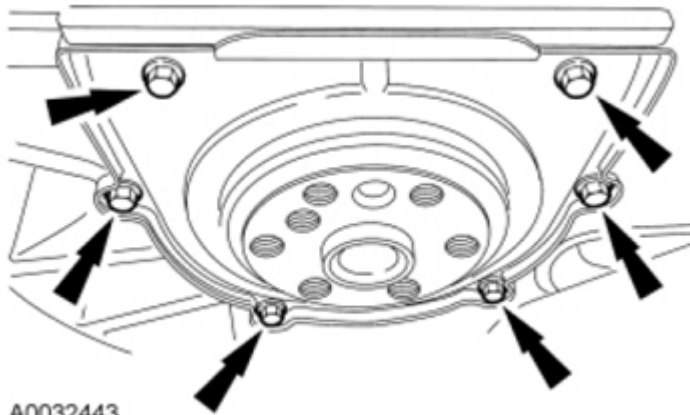
Fig. 348: Locating Rear Crankshaft Seal Bolts Courtesy of FORD MOTOR CO.
