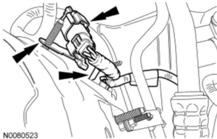
Fig. 259: Locating Generator Electrical Connector And Retainers Courtesy of FORD MOTOR CO.
