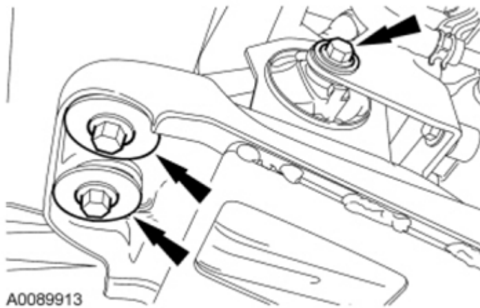
Fig. 566: Locating Front Roll Restrictor And Engine Support Crossmember Bolts Courtesy of FORD MOTOR CO.
