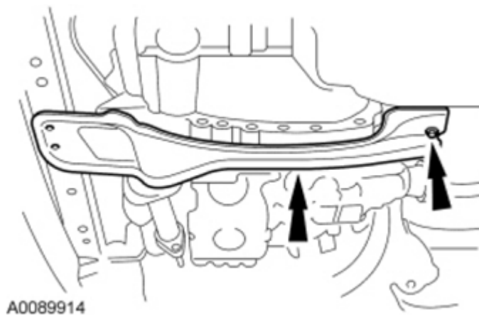
Fig. 263: Locating Engine Support Crossmember Rear Nut Courtesy of FORD MOTOR CO.
