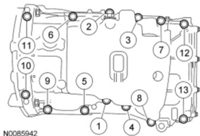
Fig. 176: Tightening Sequence Of Oil Pan Bolts Courtesy of FORD MOTOR CO.
