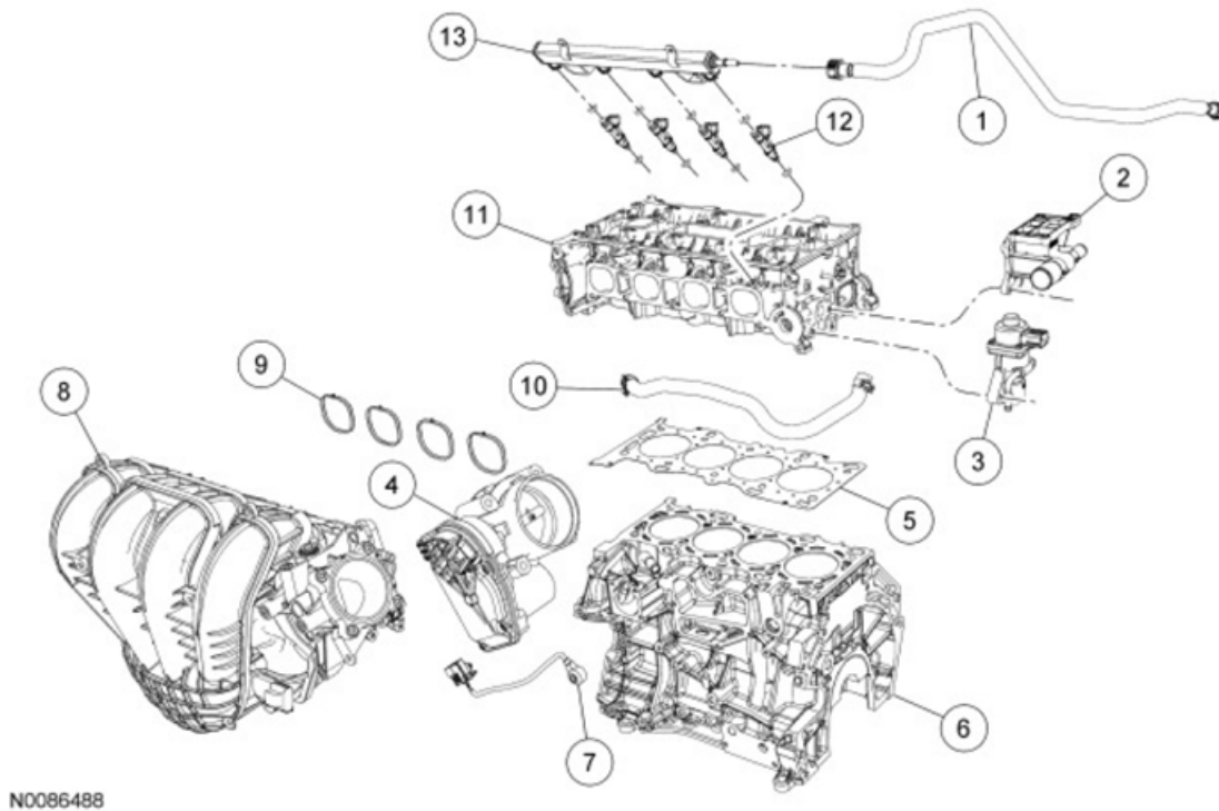
Fig. 373: Exploded View Of Intake Manifold Components Courtesy of FORD MOTOR CO.
