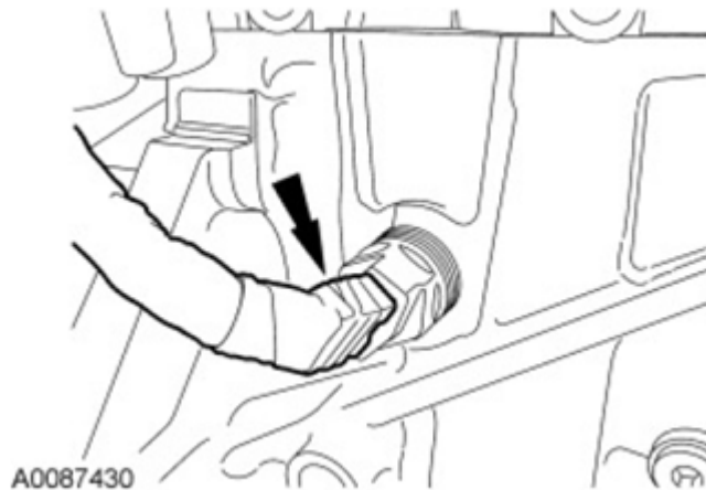
Fig. 250: Locating Block Heater Electrical Connector Courtesy of FORD MOTOR CO.
