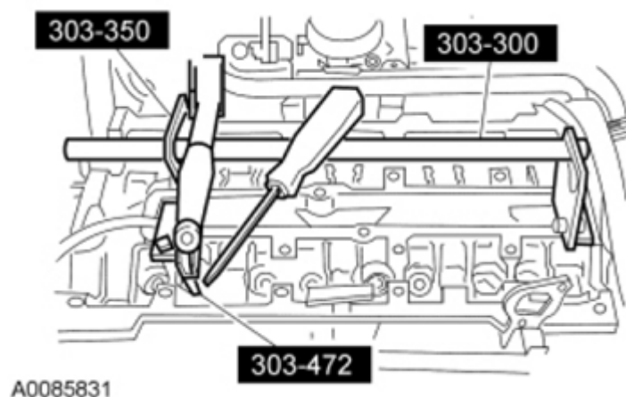
Fig. 140: Remove/Install Valve Spring Using Special Tools Courtesy of FORD MOTOR CO.
