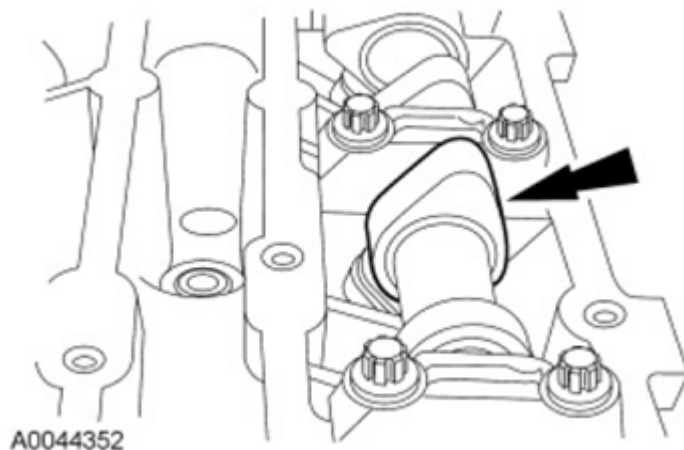
Fig. 123: View Of Camshaft Lobes Of No. 1 Cylinder Courtesy of FORD MOTOR CO.
