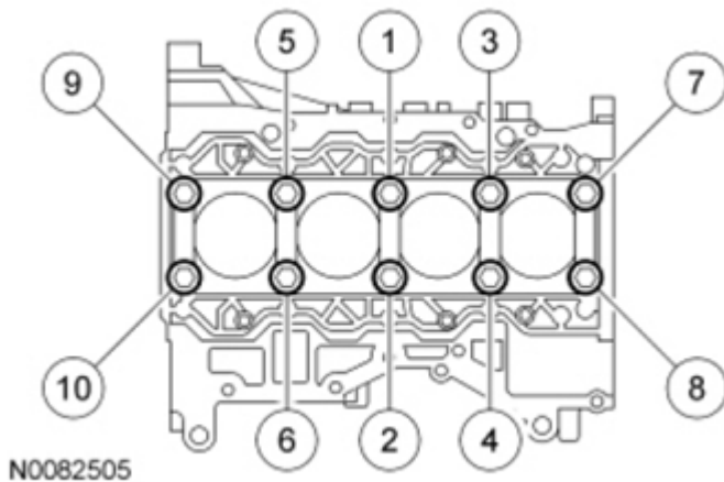
Fig. 388: Tightening Sequence Of Main Bearing Beam Bolts Courtesy of FORD MOTOR CO.
