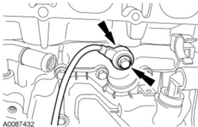
Fig. 318: Remove/Install KS With Bolt Courtesy of FORD MOTOR CO.
