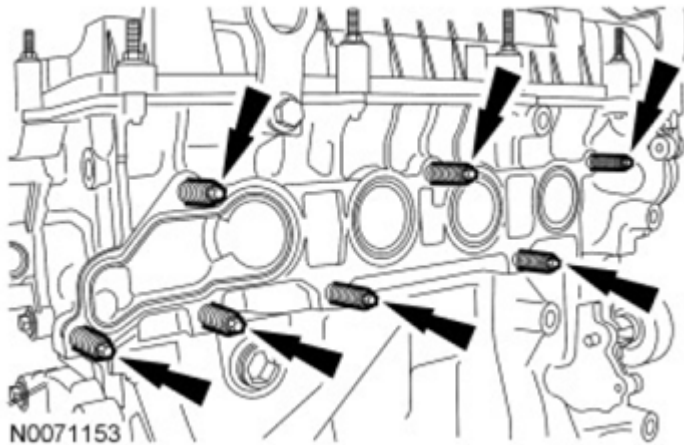
Fig. 486: View Of Exhaust Manifold Studs Courtesy of FORD MOTOR CO.
