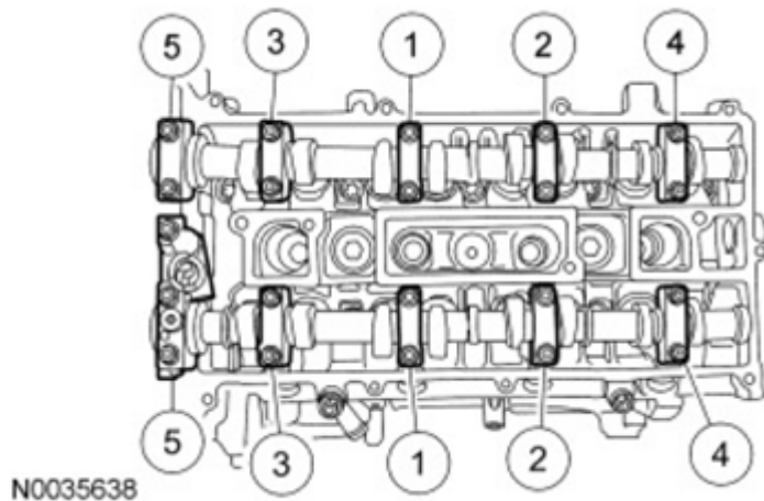
Fig. 153: Identifying Tightening Sequence Of Camshaft Bearing Cap Bolts Courtesy of FORD MOTOR CO.
