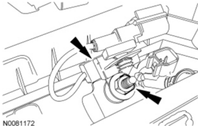
Fig. 310: Remove/Install Radio Capacitor And Nut Courtesy of FORD MOTOR CO.
