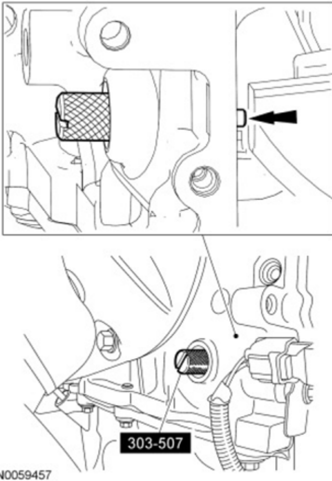
Fig. 87: View Of Crankshaft TDC Timing Peg Courtesy of FORD MOTOR CO.
