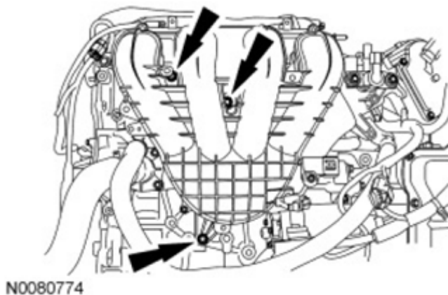
Fig. 312: Remove/Install Intake Manifold Bolts Courtesy of FORD MOTOR CO.
