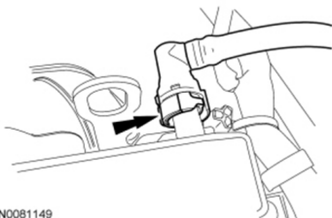
Fig. 299: Locating Crankcase Vent Hose Of Valve Cover Courtesy of FORD MOTOR CO.
