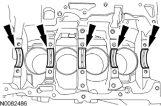
Fig. 360: View Of Main Bearings Of Cylinder Block Courtesy of FORD MOTOR CO.
