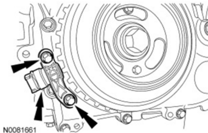
Fig. 63: Locating CKP Sensor Bolts Courtesy of FORD MOTOR CO.
