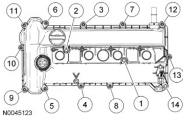
Fig. 25: Tightening Sequence Of Valve Cover Bolts Courtesy of FORD MOTOR CO.
