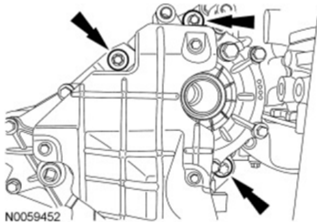
Fig. 233: Locating PTU And RH PTU Bolts Courtesy of FORD MOTOR CO.
