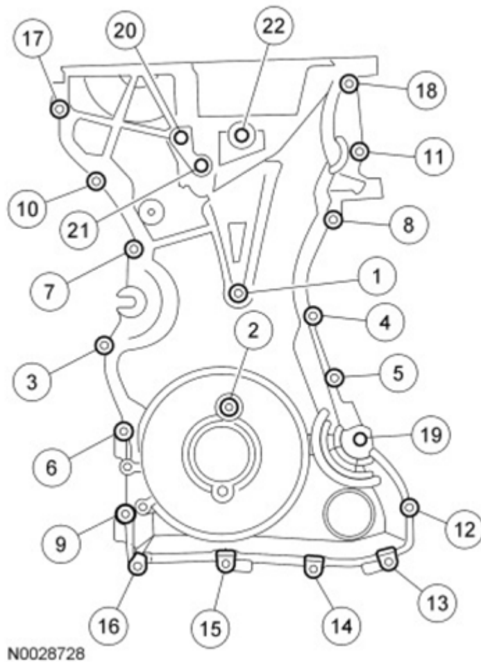
Fig. 429: Tightening Sequence Of Engine Front Cover Bolts Courtesy of FORD MOTOR CO.
