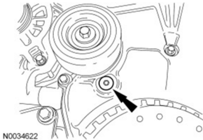
Fig. 136: Locating Lower Front Cover Timing Hole Plug Courtesy of FORD MOTOR CO.
