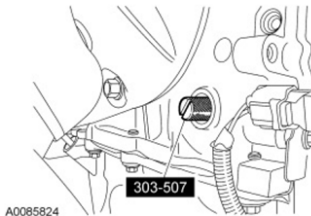
Fig. 437: View Of Crankshaft TDC Timing Peg Courtesy of FORD MOTOR CO.
