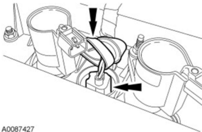
Fig. 466: Locating Cylinder Head Temperature Sensor Electrical Connector Courtesy of FORD MOTOR CO.
