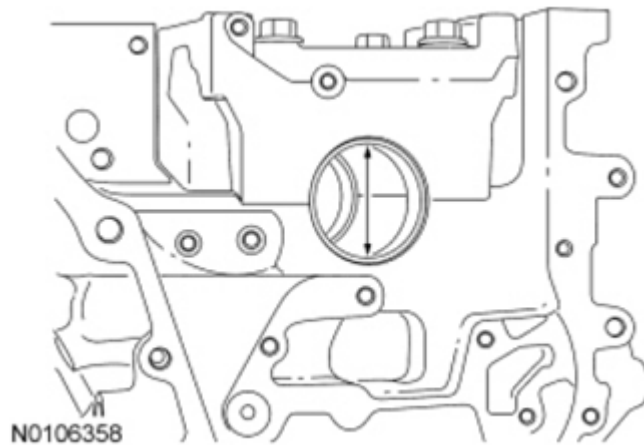
Fig. 378: Identifying Crankshaft Block Main Bearing Bore Diameter Courtesy of FORD MOTOR CO.
