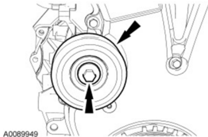
Fig. 288: Locating Accessory Drive Belt Idler Pulley And Bolt Courtesy of FORD MOTOR CO.
