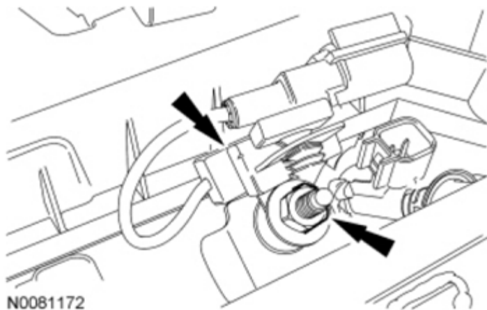
Fig. 462: Remove/Install Radio Capacitor And Nut Courtesy of FORD MOTOR CO.
