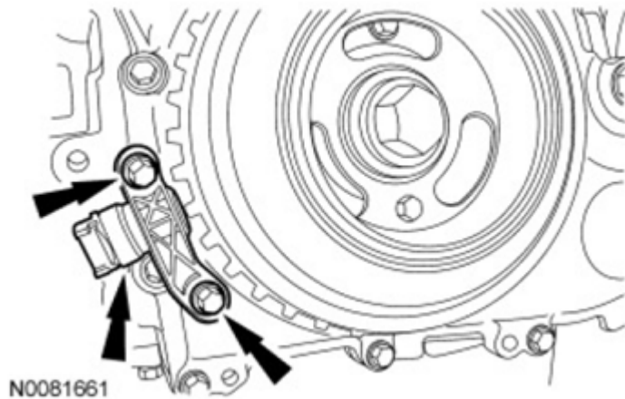
Fig. 442: Locating Crankshaft Position (CKP) Sensor And Bolts Courtesy of FORD MOTOR CO.
