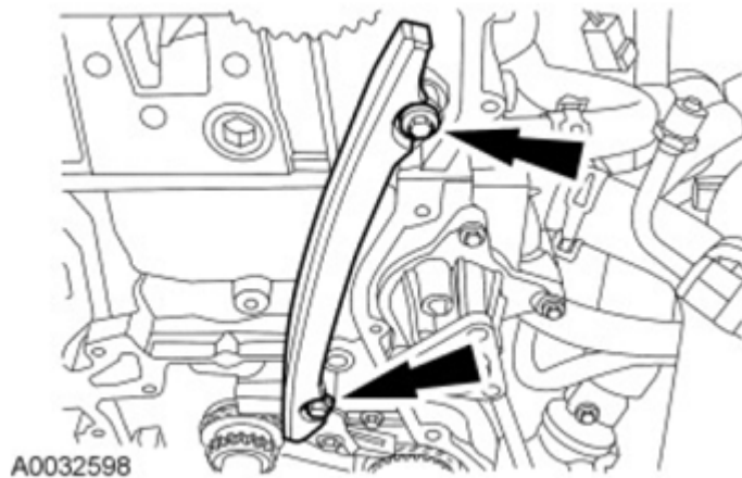
Fig. 336: Locating LH Timing Chain Guide Bolts Courtesy of FORD MOTOR CO.
