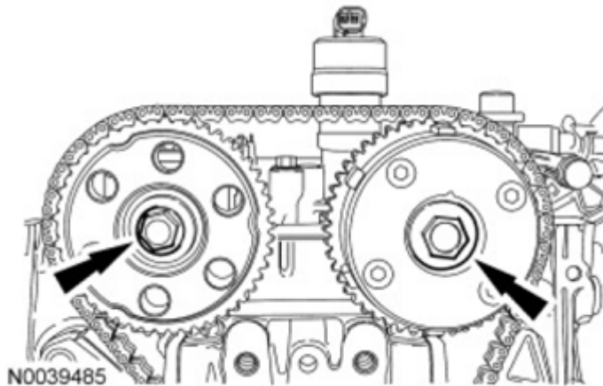
Fig. 427: View Of Camshaft Bolts Courtesy of FORD MOTOR CO.
