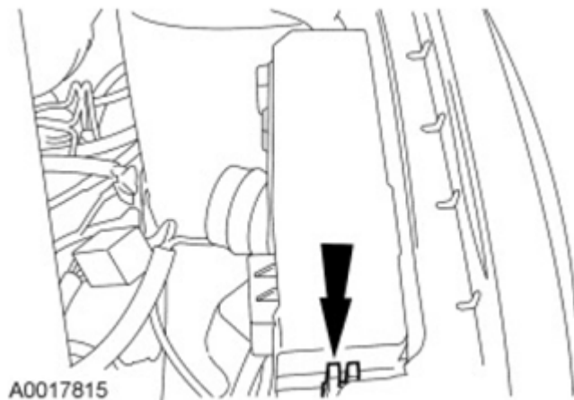
Fig. 541: Locating Power Distribution Box (PDB) Cover Courtesy of FORD MOTOR CO.
