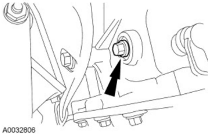
Fig. 137: Remove/Install Engine Plug Bolt Courtesy of FORD MOTOR CO.
