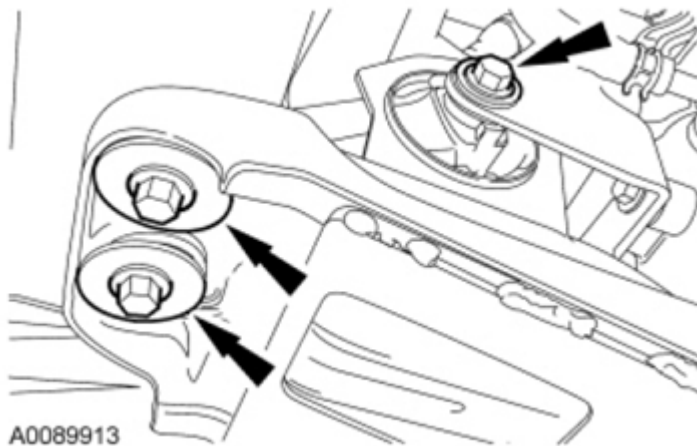
Fig. 262: Locating Front Roll Restrictor And Engine Support Crossmember Bolts Courtesy of FORD MOTOR CO.
