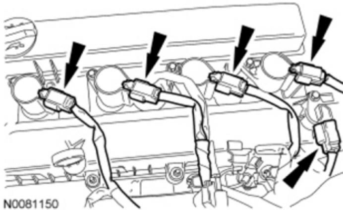
Fig. 467: View Of Coil-On-Plugs And Camshaft Position Sensor Electrical Connectors Courtesy of FORD MOTOR CO.
