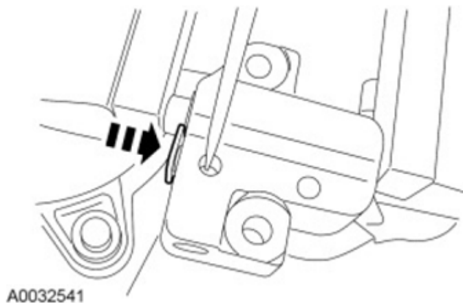
Fig. 79: Pushing Ratchet Arm Courtesy of FORD MOTOR CO.
