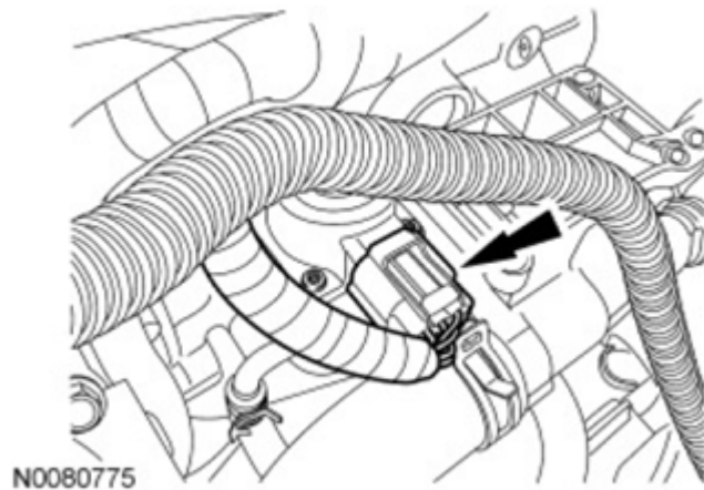
Fig. 469: Locating EGR Valve Electrical Connector Courtesy of FORD MOTOR CO.
