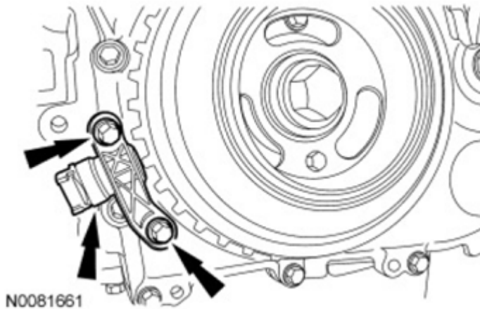
Fig. 324: Locating CKP Sensor With Bolts Courtesy of FORD MOTOR CO.
