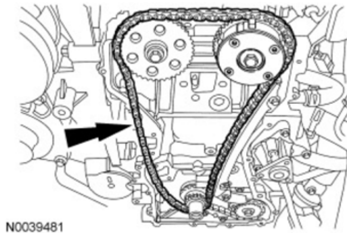
Fig. 75: View Of Timing Chain Courtesy of FORD MOTOR CO.
