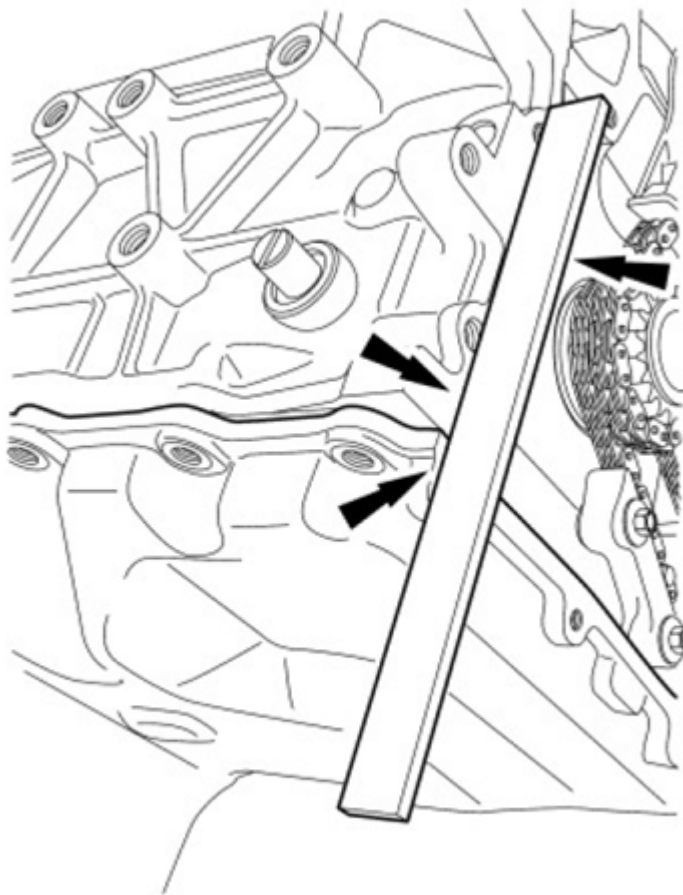
Fig. 404: Aligning Front Surface Of Oil Pan Courtesy of FORD MOTOR CO.
