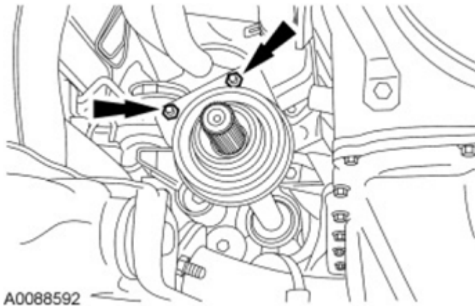
Fig. 183: Locating Intermediate Shaft Bearing Retainer Nuts Courtesy of FORD MOTOR CO.
