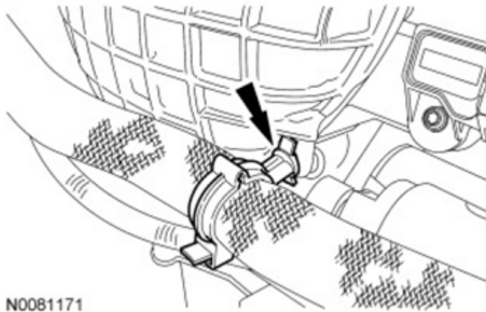
Fig. 479: Locating Coolant Tube Retainer Of Intake Manifold Courtesy of FORD MOTOR CO.
