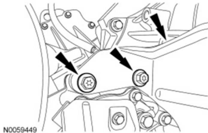
Fig. 514: Locating PTU Bracket-To-PTU Bolts And Bracket Courtesy of FORD MOTOR CO.
