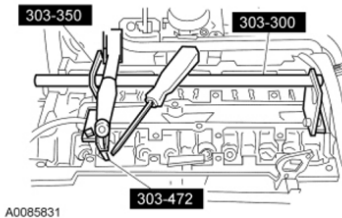
Fig. 141: Remove/Install Valve Spring Using Special Tools Courtesy of FORD MOTOR CO.
