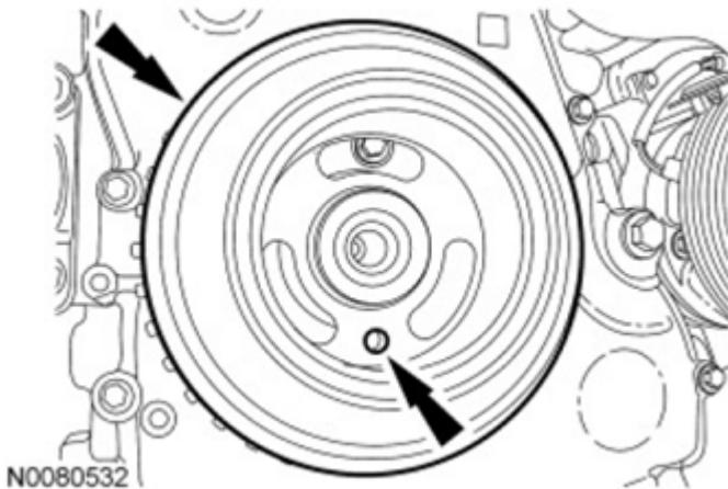
Fig. 431: Identifying Crankshaft Pulley And Hole Courtesy of FORD MOTOR CO.
