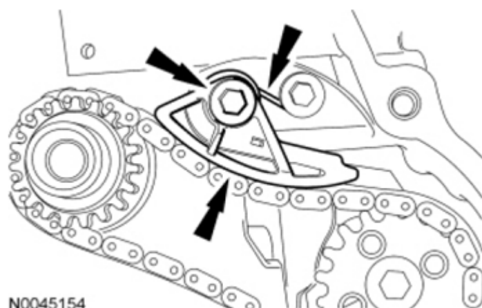
Fig. 416: Locating Oil Pump Drive Chain Tensioner And Shoulder Bolt Courtesy of FORD MOTOR CO.
