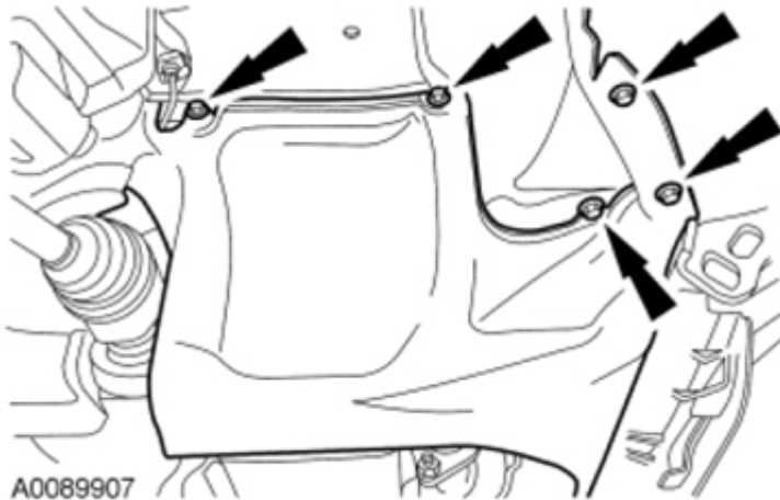
Fig. 3: Locating RH Splash Shield Bolts Courtesy of FORD MOTOR CO.
