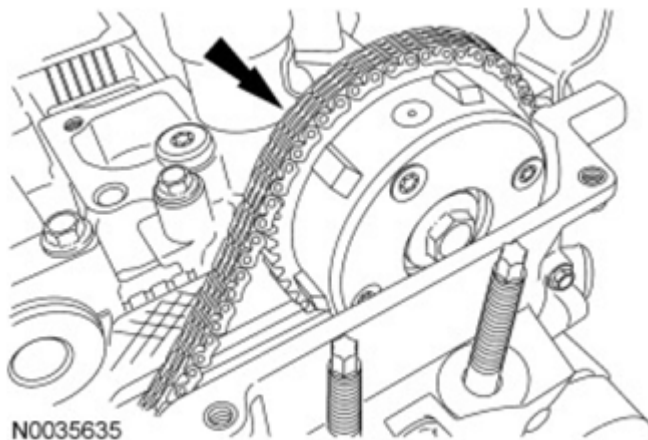
Fig. 102: Locating Timing Chain Of Intake Camshaft Drive Gear Courtesy of FORD MOTOR CO.
