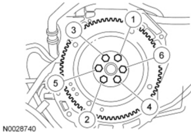
Fig. 494: Tightening Sequence Of Flexplate Bolts Courtesy of FORD MOTOR CO.
