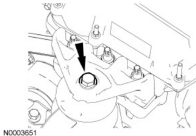
Fig. 223: Locating Engine Mount Bracket Bolt Courtesy of FORD MOTOR CO.
