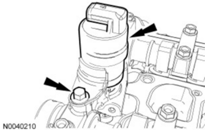
Fig. 412: Remove/Install VCT Solenoid And Bolt Courtesy of FORD MOTOR CO.
