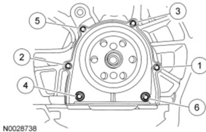
Fig. 402: Tightening Sequence Of Crankshaft Rear Oil Seal Bolts Courtesy of FORD MOTOR CO.
