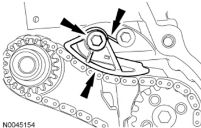
Fig. 173: Locating Oil Pump Drive Chain Tensioner And Shoulder Bolt Courtesy of FORD MOTOR CO.
