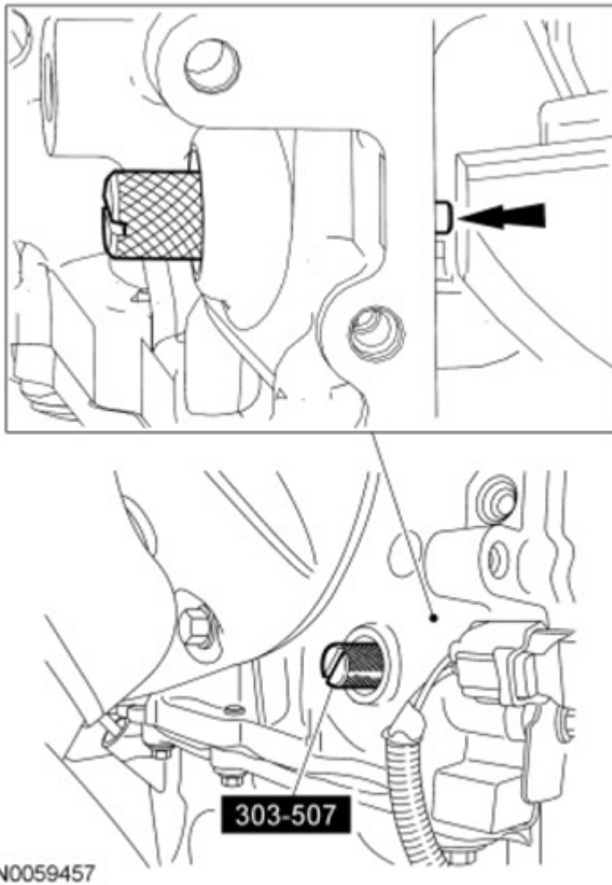
Fig. 10: View Of Crankshaft TDC Timing Peg Courtesy of FORD MOTOR CO.
