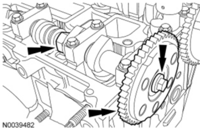
Fig. 337: View Of Exhaust Camshaft Sprocket With Bolt Courtesy of FORD MOTOR CO.
