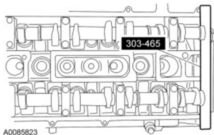
Fig. 440: View Of Camshaft Alignment Plate Courtesy of FORD MOTOR CO.
