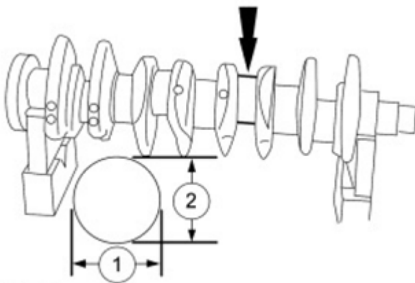
Fig. 381: Identifying Crankshaft Connecting Rod Bearing Journal Diameters Courtesy of FORD MOTOR CO.
