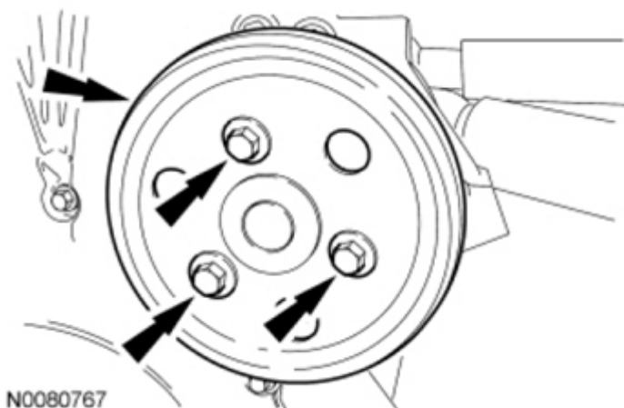
Fig. 482: Locating Coolant Pump Pulley And Bolts Courtesy of FORD MOTOR CO.
