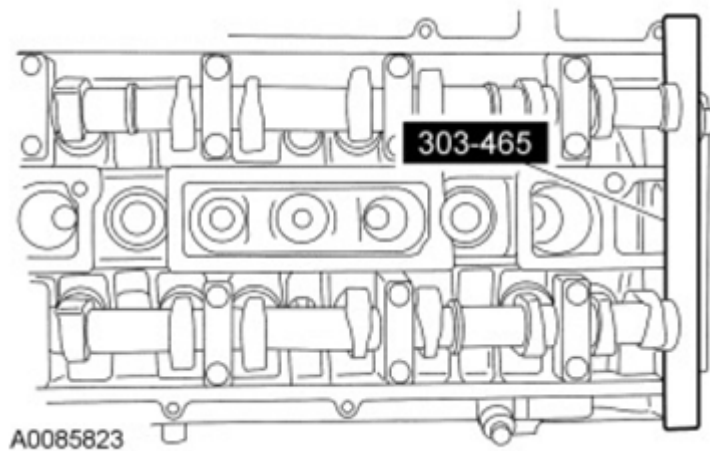
Fig. 154: View Of Camshaft Alignment Plate Courtesy of FORD MOTOR CO.
