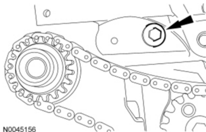
Fig. 415: Locating Oil Pump Drive Chain Tensioner Shoulder Bolt Courtesy of FORD MOTOR CO.
