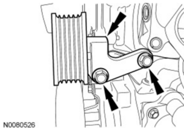
Fig. 289: Locating Accessory Drive Belt Idler Pulley And Bracket Bolts Courtesy of FORD MOTOR CO.
