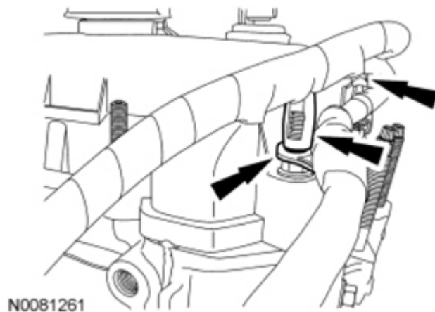
Fig. 298: Locating Wiring Harness Retainers Of RH Side Valve Cover Stud Bolt Courtesy of FORD MOTOR CO.
