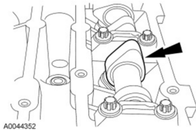
Fig. 96: View Of Camshaft Lobes Of No. 1 Cylinder Courtesy of FORD MOTOR CO.
