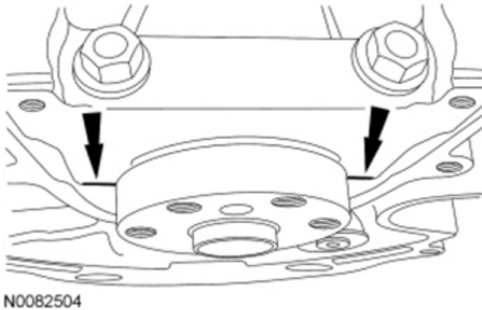
Fig. 387: Locating Main Bearing Beams Courtesy of FORD MOTOR CO.
