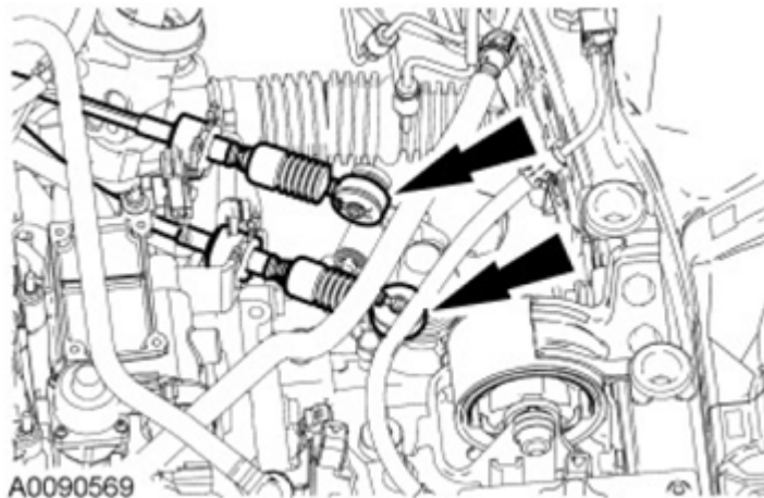
Fig. 248: Locating Shift Cables Courtesy of FORD MOTOR CO.
