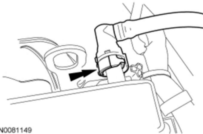
Fig. 473: Locating Crankcase Vent Hose Of Valve Cover Courtesy of FORD MOTOR CO.
