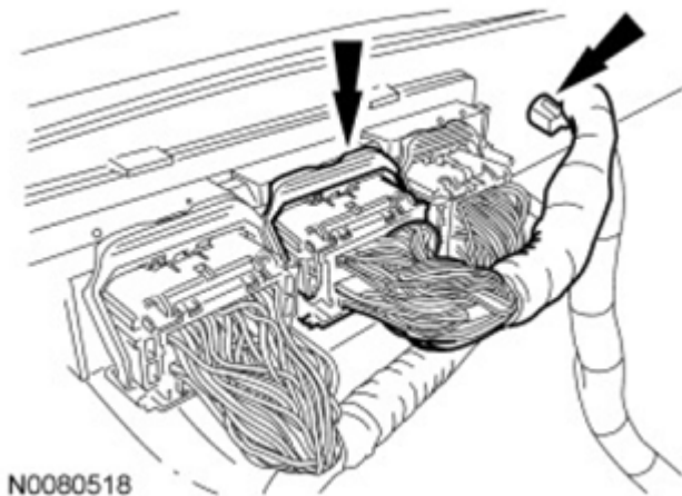
Fig. 257: Locating PCM Electrical Connector And Wire Harness Retainer Courtesy of FORD MOTOR CO.
