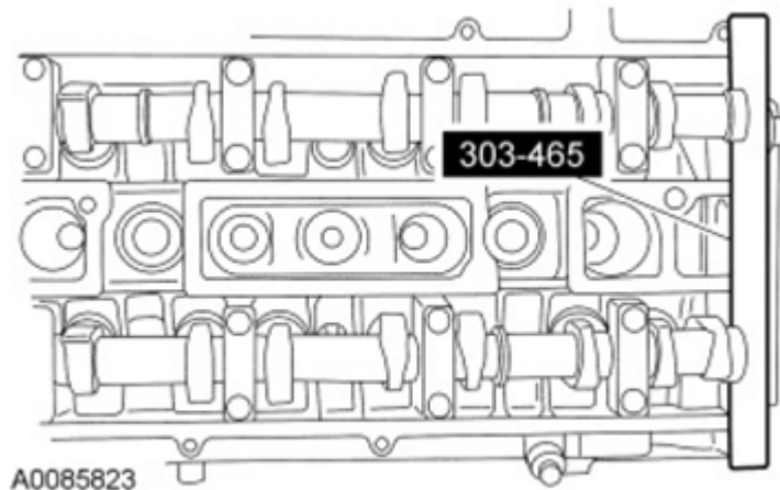
Fig. 42: View Of Camshaft Alignment Plate Courtesy of FORD MOTOR CO.
