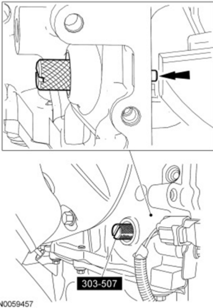
Fig. 11: View Of Crankshaft TDC Timing Peg Courtesy of FORD MOTOR CO.
