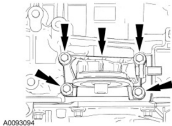
Fig. 295: Locating Oil Filter Adapter Bolts Courtesy of FORD MOTOR CO.
