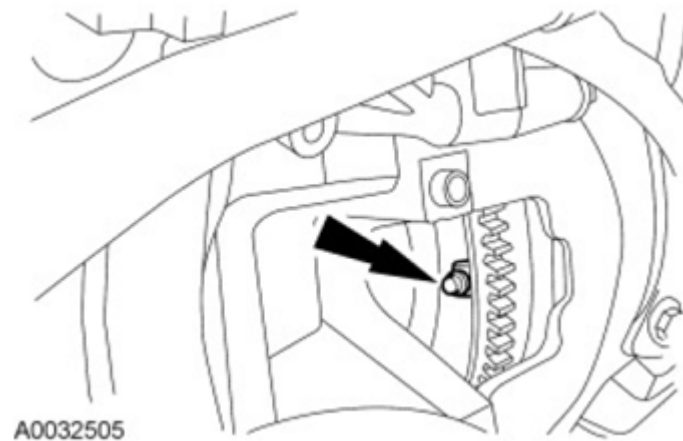
Fig. 236: Locating Torque Converter Nut Courtesy of FORD MOTOR CO.
