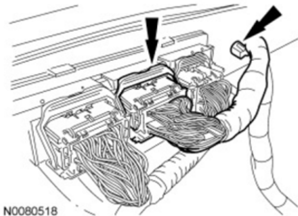
Fig. 208: Locating PCM Electrical Connector And Wire Harness Retainer Courtesy of FORD MOTOR CO.
