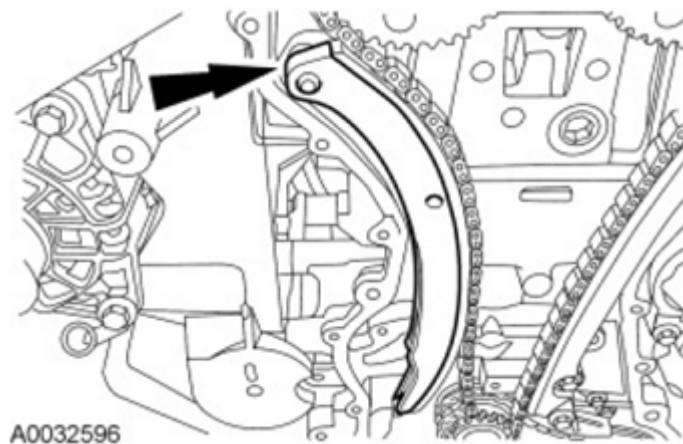
Fig. 421: Locating RH Timing Chain Guide Courtesy of FORD MOTOR CO.
