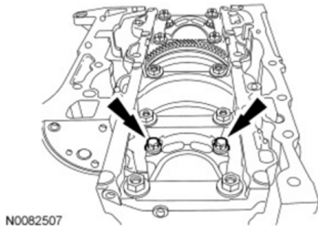
Fig. 391: Locating Connecting Rod Cap Bolts Courtesy of FORD MOTOR CO.
