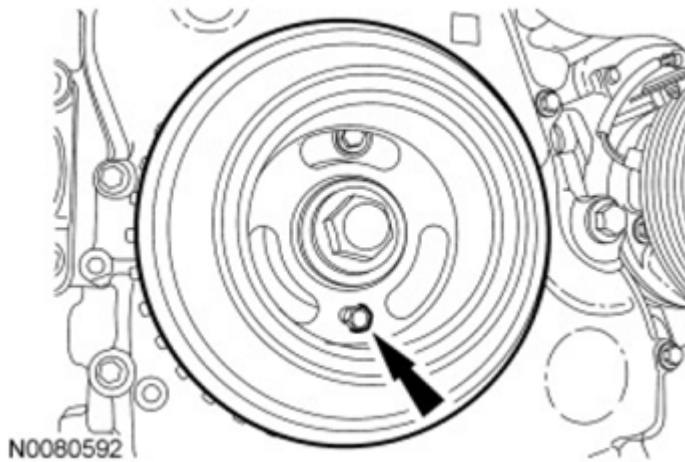
Fig. 65: View Of Crankshaft Pulley Alignment Bolt Courtesy of FORD MOTOR CO.
