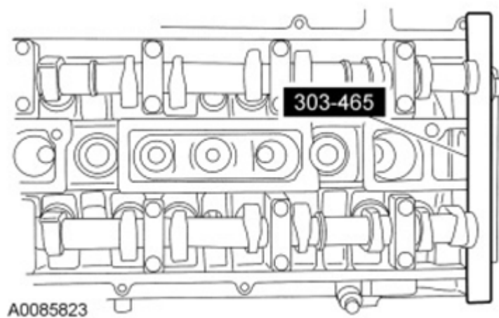
Fig. 37: View Of Camshaft Alignment Plate Courtesy of FORD MOTOR CO.
