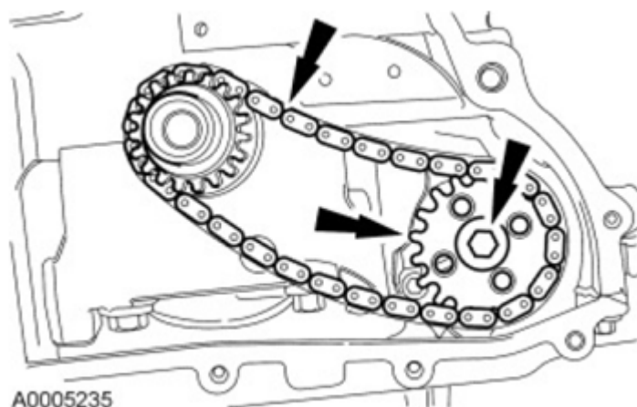
Fig. 414: Identifying Oil Pump Chain, Sprocket And Bolt Courtesy of FORD MOTOR CO.
