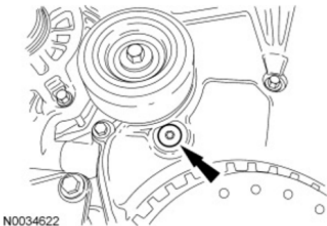
Fig. 109: Locating Lower Front Cover Timing Hole Plug Courtesy of FORD MOTOR CO.
