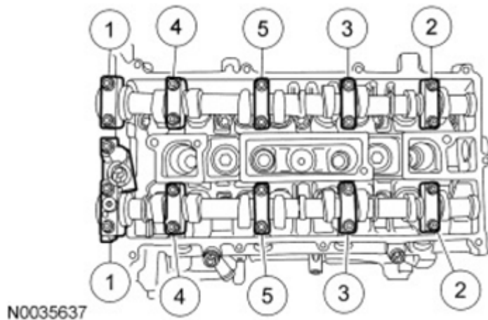
Fig. 149: Removing Sequence Of Camshaft Bearing Cap Bolts Courtesy of FORD MOTOR CO.
