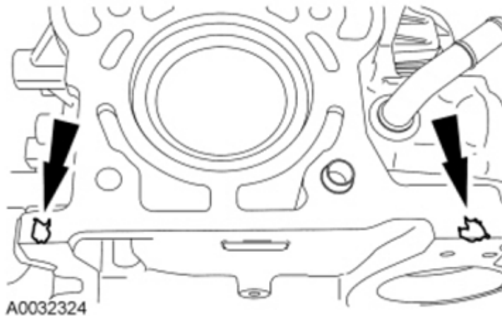
Fig. 150: Locating Silicone Gasket And Sealant Applying Areas Of Cylinder Block Courtesy of FORD MOTOR CO.
