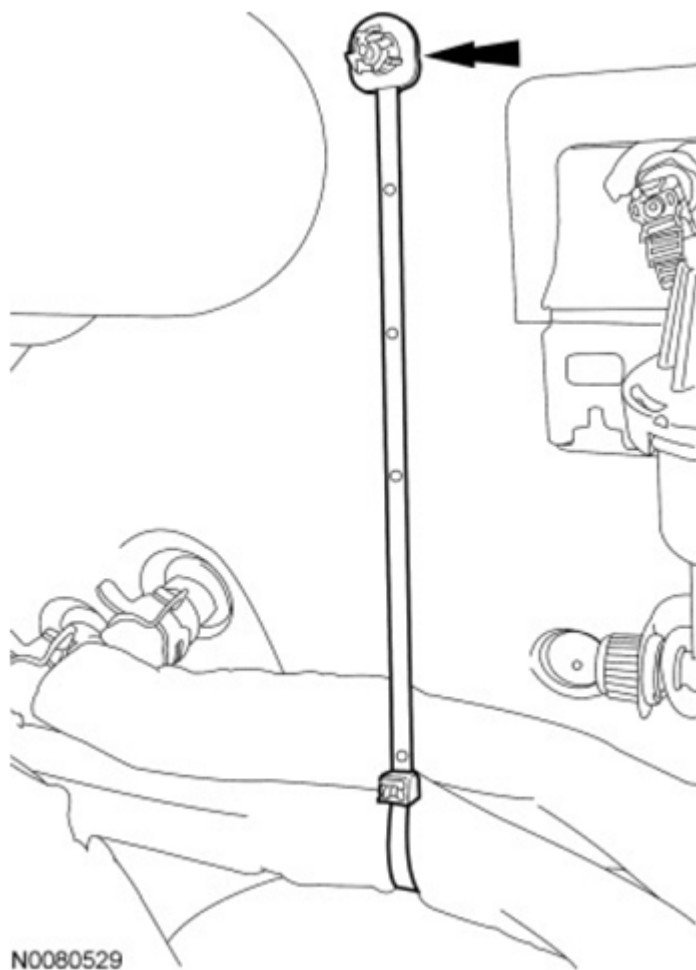
Fig. 203: Locating Heater Hose Support Strap Of Stud Courtesy of FORD MOTOR CO.
