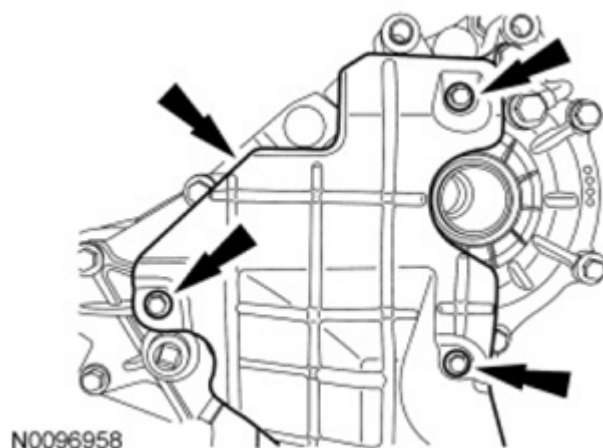
Fig. 501: Locating PTU Heat Shield Bolts Courtesy of FORD MOTOR CO.
