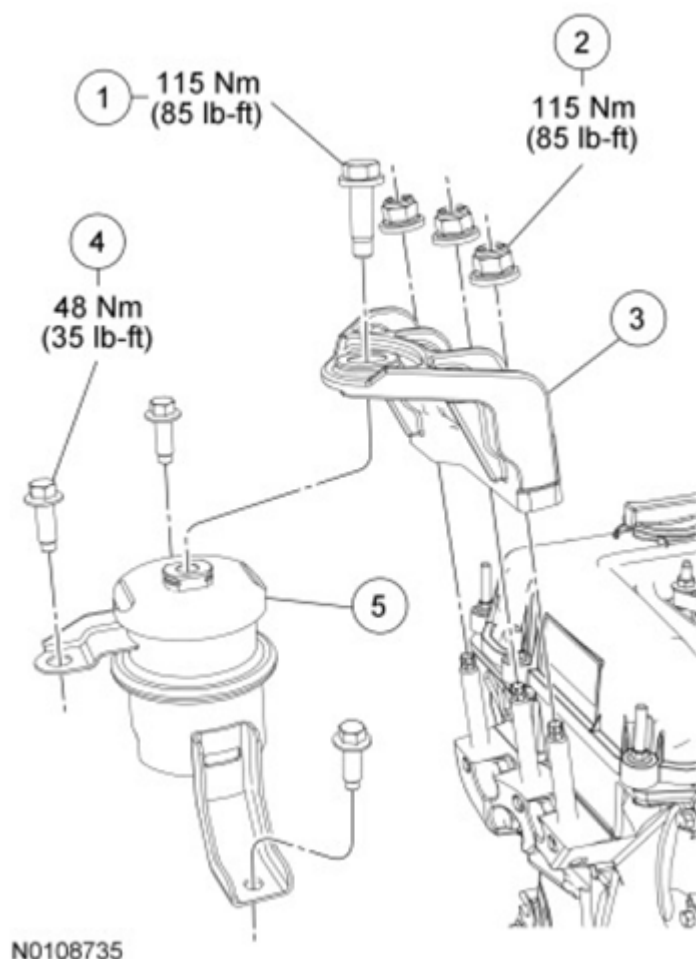
Fig. 179: Identifying Engine Mount With Torque Specifications Courtesy of FORD MOTOR CO.
