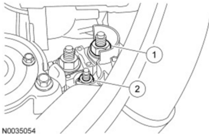
Fig. 272: Identifying Battery Cable And Starter Solenoid Terminal Nuts Courtesy of FORD MOTOR CO.
