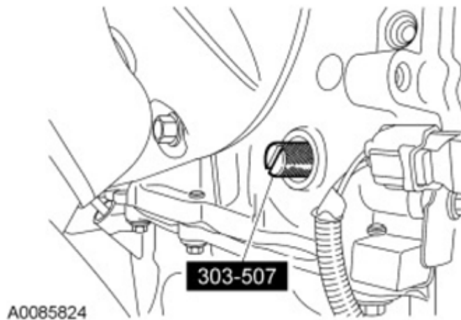
Fig. 44: View Of Crankshaft TDC Timing Peg Courtesy of FORD MOTOR CO.
