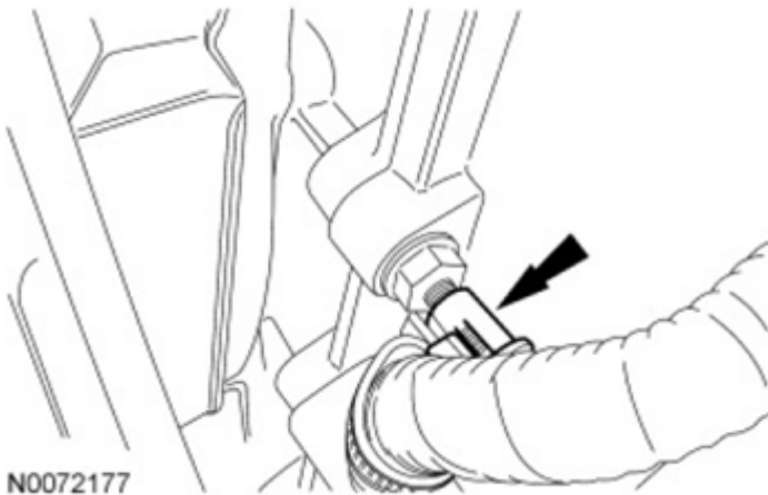
Fig. 545: Locating Wiring Harness Retainer Of Transaxle Stud Bolt Courtesy of FORD MOTOR CO.
