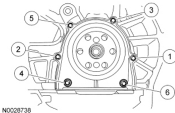
Fig. 52: Tightening Sequence Of Crankshaft Rear Oil Seal Bolts Courtesy of FORD MOTOR CO.
