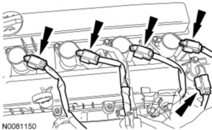
Fig. 305: View Of Coil-On-Plugs And Camshaft Position Sensor Electrical Connectors Courtesy of FORD MOTOR CO.
