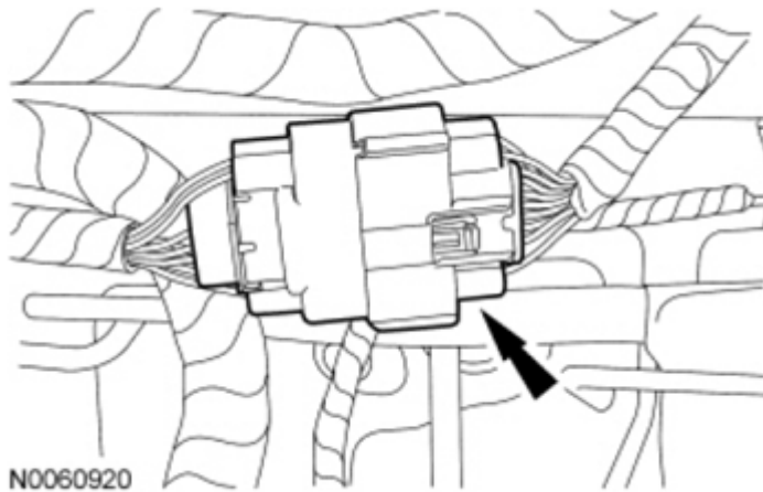
Fig. 570: Locating Engine Control Harness Electrical Connector Courtesy of FORD MOTOR CO.
