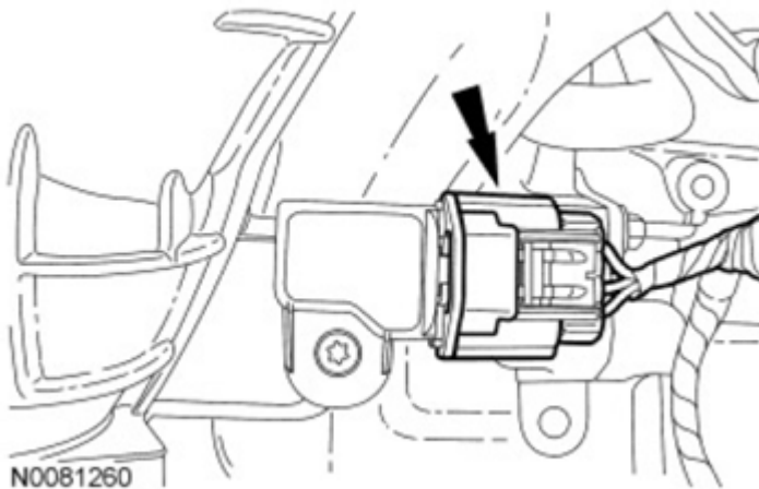
Fig. 471: Locating Manifold Absolute Pressure (MAP) Sensor Electrical Connector Courtesy of FORD MOTOR CO.
