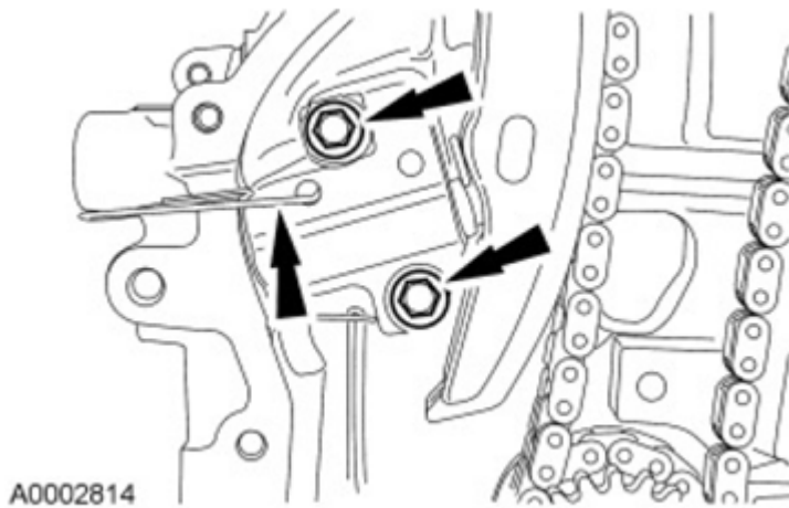
Fig. 81: Locating Timing Chain Tensioner Bolts Courtesy of FORD MOTOR CO.
