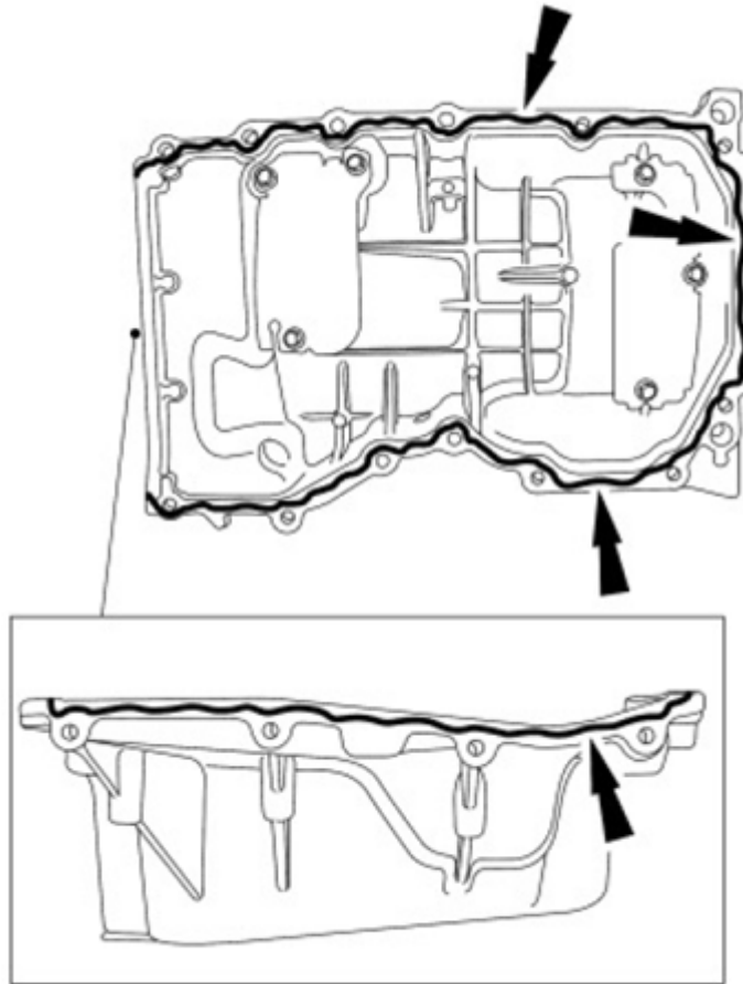
Fig. 166: Locating Gasket And Sealant Applying Area Of Oil Pan-To-Engine Block Courtesy of FORD MOTOR CO.
