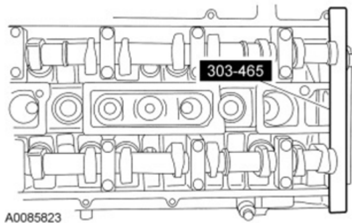
Fig. 132: View Of Camshaft Alignment Plate Courtesy of FORD MOTOR CO.
