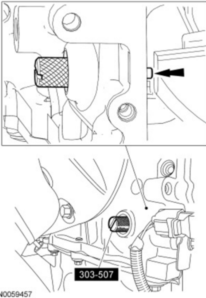
Fig. 351: View Of Crankshaft TDC Timing Peg Courtesy of FORD MOTOR CO.
