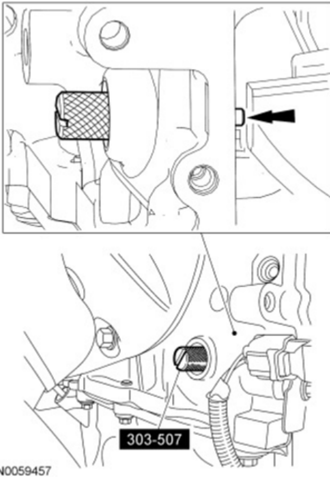
Fig. 328: View Of Crankshaft TDC Timing Peg Courtesy of FORD MOTOR CO.
