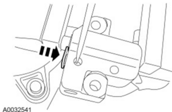
Fig. 424: Pushing Ratchet Arm Courtesy of FORD MOTOR CO.
