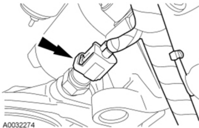
Fig. 478: Locating Engine Oil Pressure Switch Electrical Connector Courtesy of FORD MOTOR CO.
