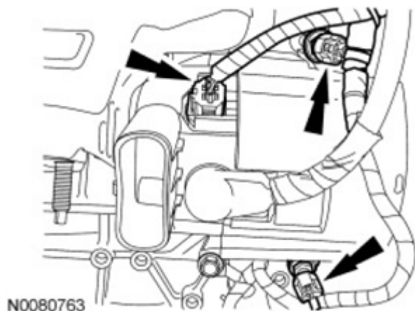
Fig. 492: Locating Generator Electrical Connection And Wiring Harness Retainers Courtesy of FORD MOTOR CO.
