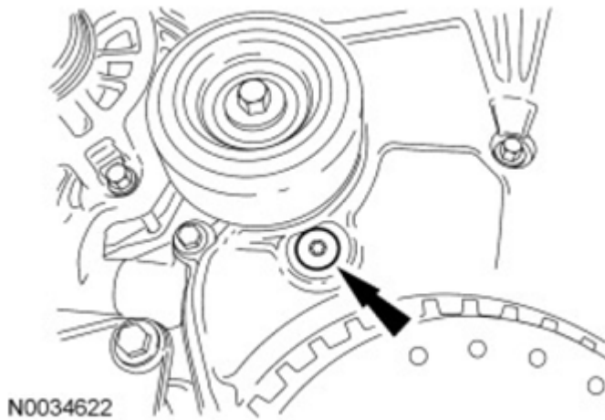
Fig. 116: Locating Lower Front Cover Timing Hole Plug Courtesy of FORD MOTOR CO.
