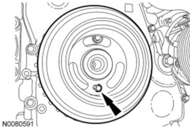
Fig. 432: View Of Crankshaft Pulley Alignment Bolt Courtesy of FORD MOTOR CO.
