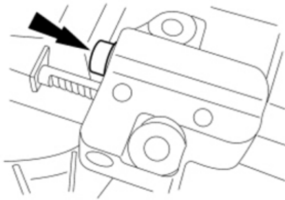
Fig. 422: Compressing Timing Chain Tensioner Plunger Courtesy of FORD MOTOR CO.
