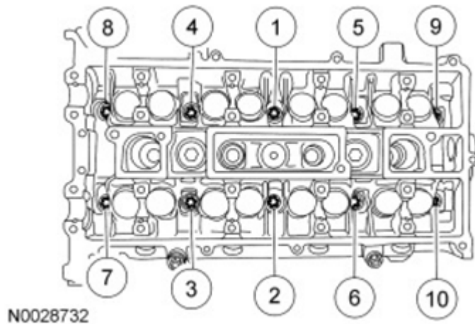
Fig. 151: Tightening Sequence Of Cylinder Head Bolts Courtesy of FORD MOTOR CO.
