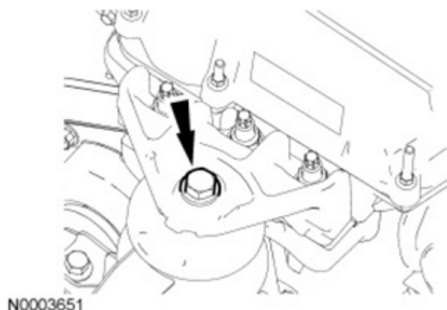
Fig. 512: Locating Engine Mount Bracket Bolt Courtesy of FORD MOTOR CO.
