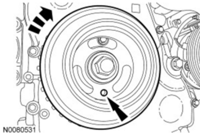
Fig. 325: Turning Crankshaft Pulley Courtesy of FORD MOTOR CO.
