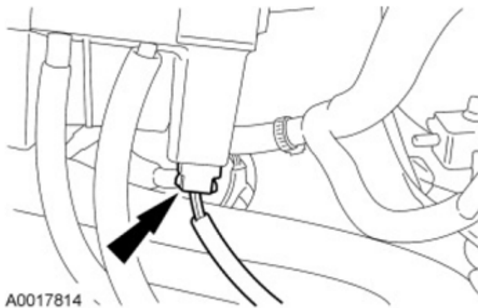
Fig. 539: Locating PDB Electrical Connector Courtesy of FORD MOTOR CO.
