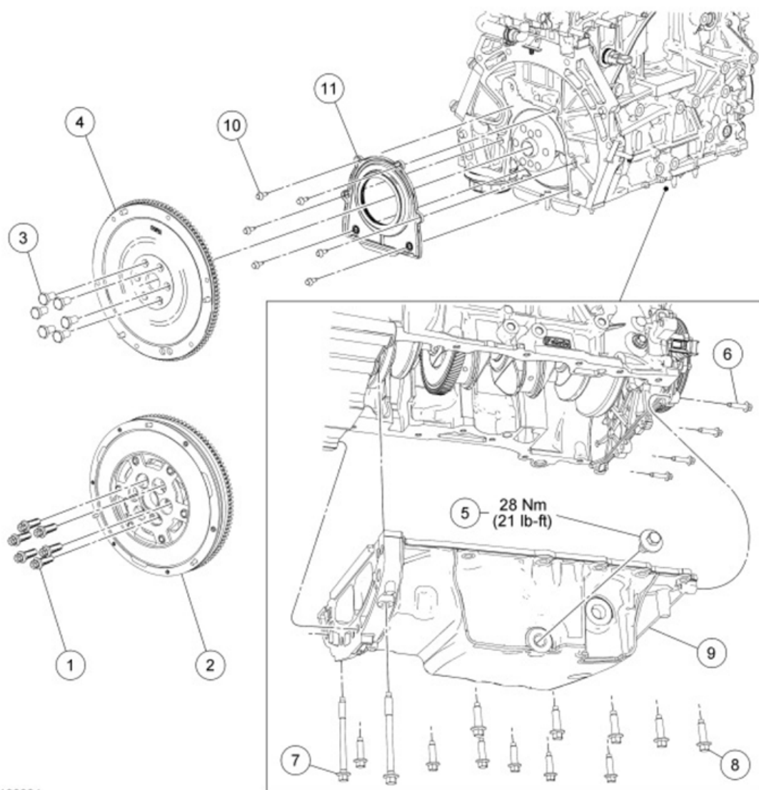
Fig. 48: Exploded View Of Lower End Components With Torque Specifications Courtesy of FORD MOTOR CO.
