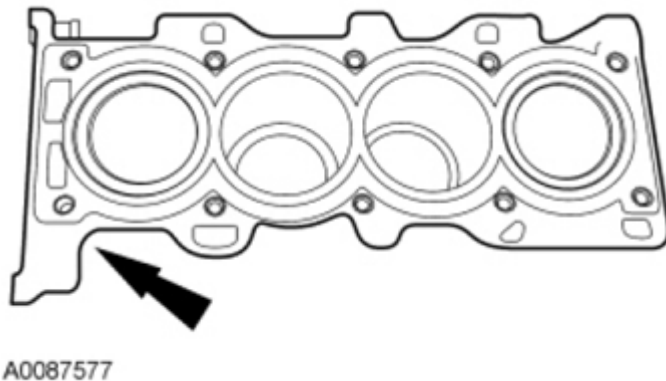
Fig. 408: View Of Head Gasket Courtesy of FORD MOTOR CO.
