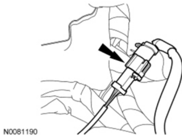
Fig. 489: Locating Heated Oxygen Sensor (HO2S) Electrical Connector Courtesy of FORD MOTOR CO.
