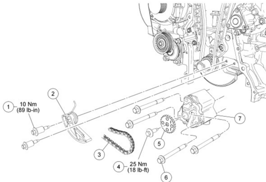
Fig. 159: Exploded View Of Engine Lubrication Components With Torque Specifications - (5 Of 5) Courtesy of FORD MOTOR CO.
