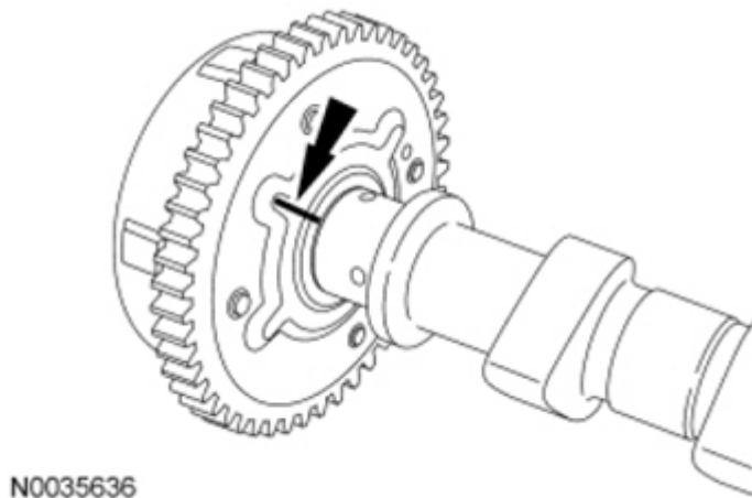
Fig. 125: View Of Sprocket And Camshaft Marking Courtesy of FORD MOTOR CO.
