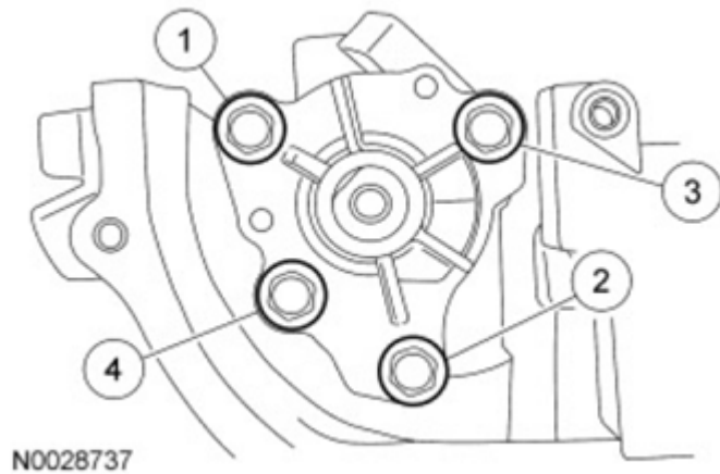
Fig. 399: Tightening Sequence Of Oil Pump Assembly Bolts Courtesy of FORD MOTOR CO.
