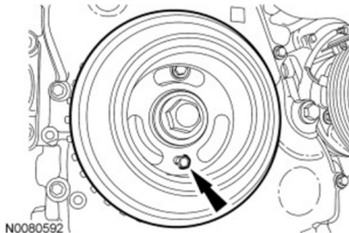
Fig. 43: View Of Crankshaft Pulley Alignment Bolt Courtesy of FORD MOTOR CO.
