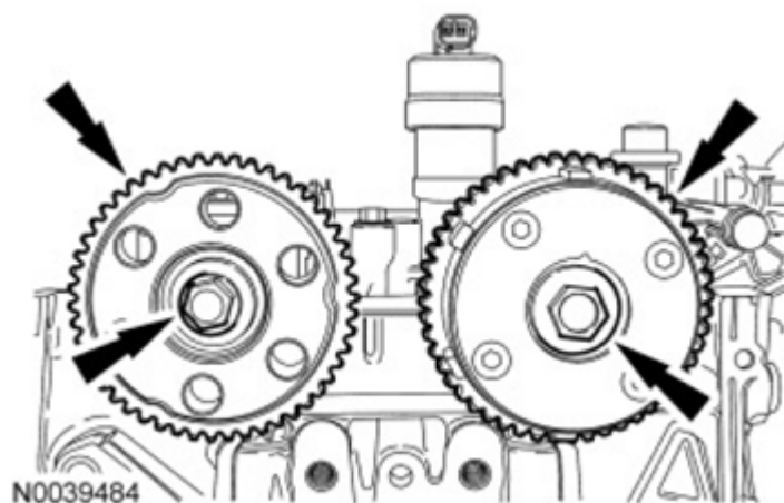
Fig. 73: View Of Camshaft Sprockets Bolts Courtesy of FORD MOTOR CO.
