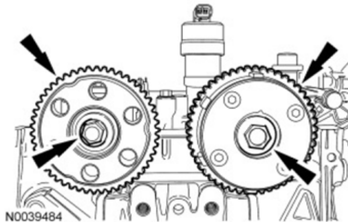
Fig. 418: View Of Camshaft Sprockets Bolts Courtesy of FORD MOTOR CO.
