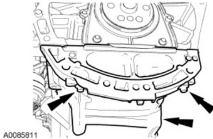
Fig. 403: Locating Oil Pan Bolts Courtesy of FORD MOTOR CO.
