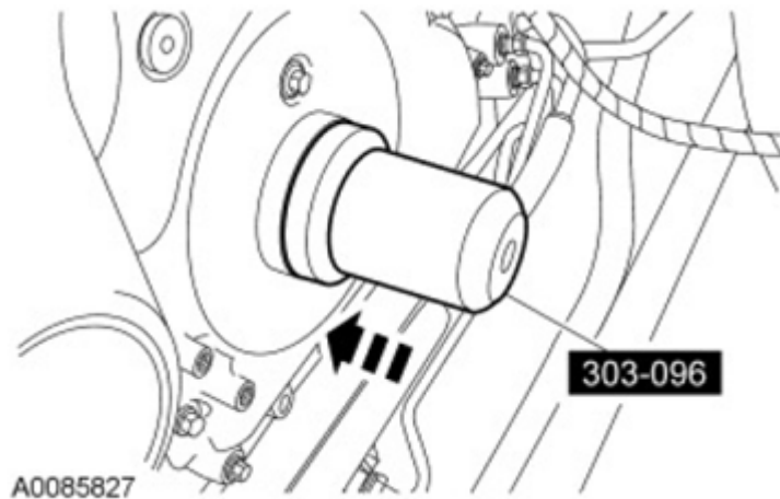
Fig. 47: Installing Crankshaft Front Oil Seal Using Camshaft Front Oil Seal Installer Courtesy of FORD MOTOR CO.
