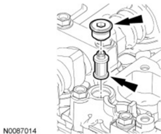
Fig. 411: View Of VCT System Oil Filter And Plug Courtesy of FORD MOTOR CO.
