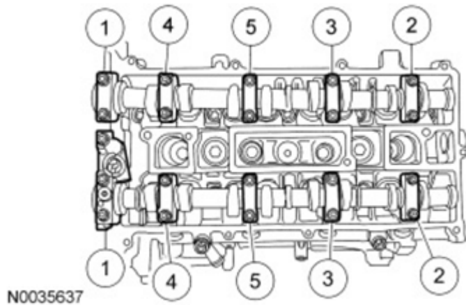
Fig. 97: Removing Sequence Of Camshaft Bearing Cap Bolts Courtesy of FORD MOTOR CO.
