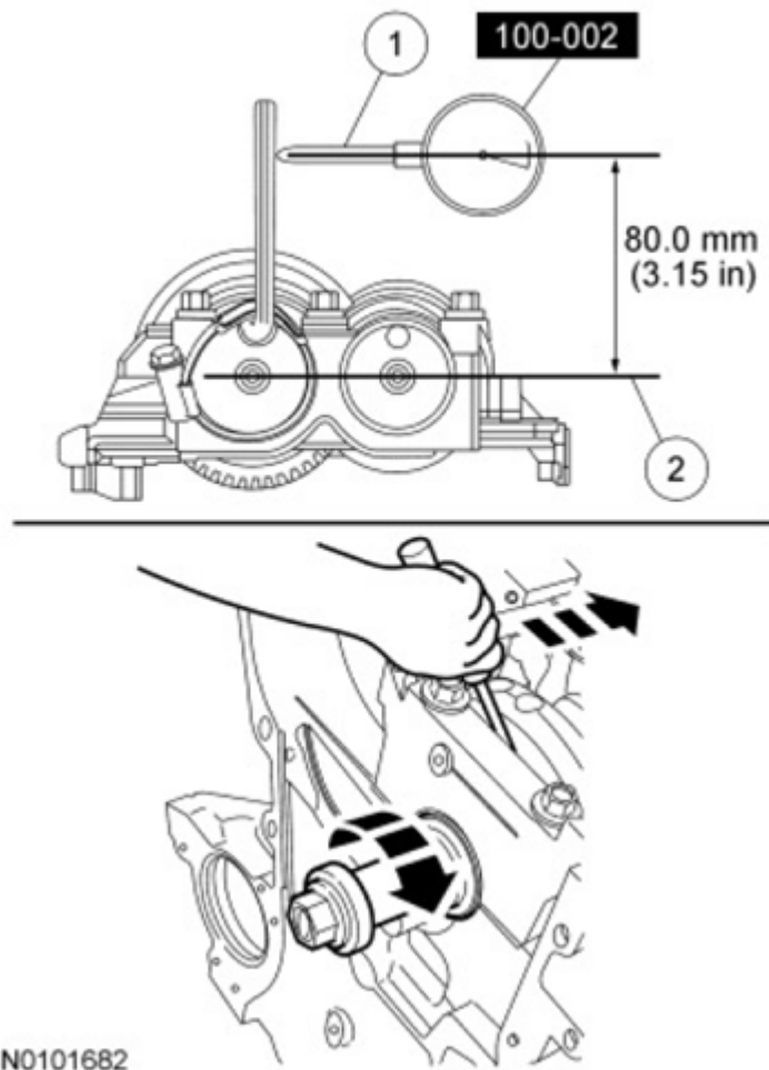
Fig. 17: Measuring Gear Backlash With Specifications Courtesy of FORD MOTOR CO.
