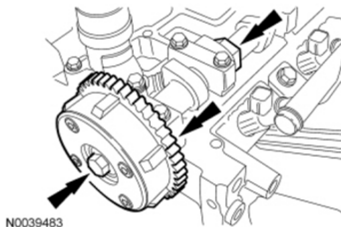
Fig. 72: View Of Camshaft Phaser, Sprocket With Bolts Courtesy of FORD MOTOR CO.
