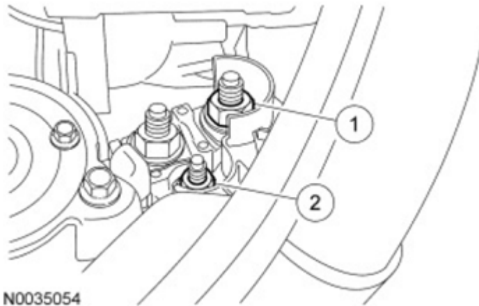
Fig. 557: Identifying Battery Cable And Starter Solenoid Terminal Nuts Courtesy of FORD MOTOR CO.
