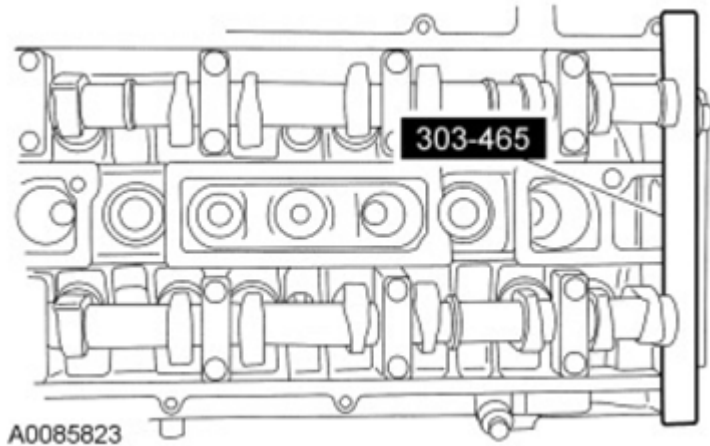
Fig. 128: View Of Camshaft Alignment Plate Courtesy of FORD MOTOR CO.
