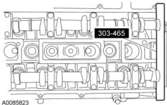
Fig. 41: View Of Camshaft Alignment Plate
