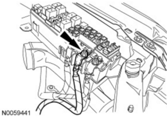
Fig. 587: Locating PDB Cable Nut Courtesy of FORD MOTOR CO.
