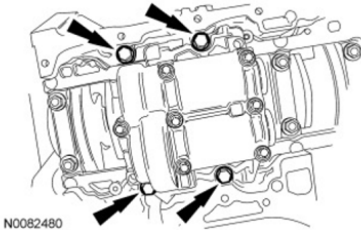
Fig. 7: Locating Balancer Unit Bolts
