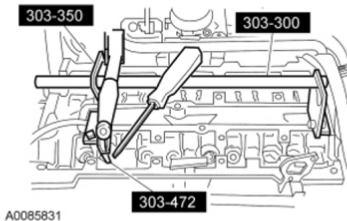
Fig. 145: Remove/Install Valve Spring Using Special Tools Courtesy of FORD MOTOR CO.
