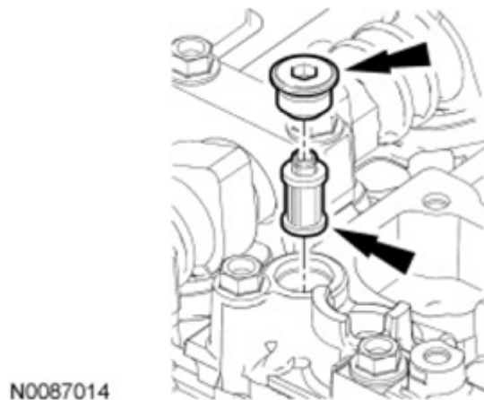
Fig. 343: View Of VCT System Oil Filter And Plug Courtesy of FORD MOTOR CO.
