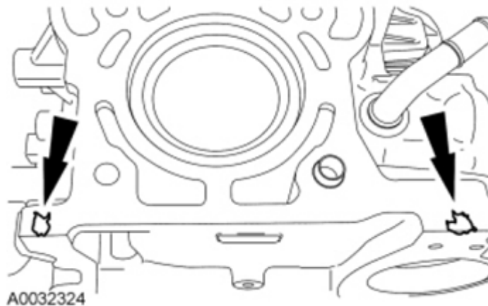
Fig. 407: Locating Silicone Gasket And Sealant Applying Areas Of Cylinder Block Courtesy of FORD MOTOR CO.
