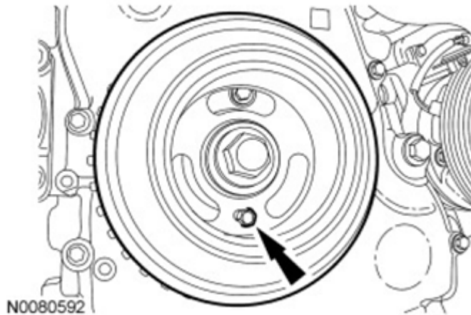
Fig. 106: View Of Crankshaft Pulley Alignment Bolt Courtesy of FORD MOTOR CO.
