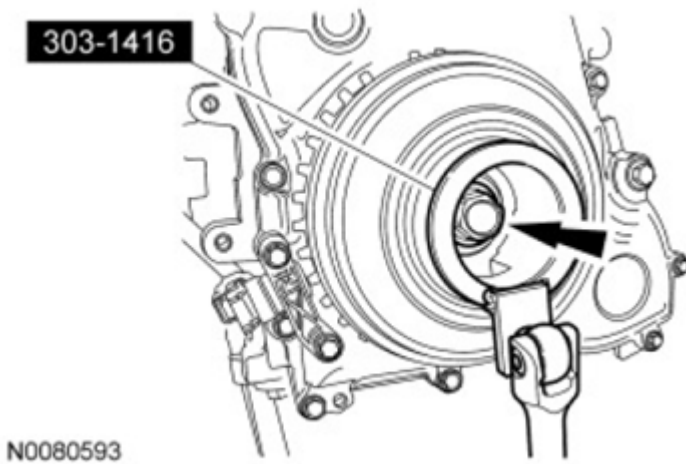
Fig. 34: Remove/Install Crankshaft Pulley Bolt Courtesy of FORD MOTOR CO.
