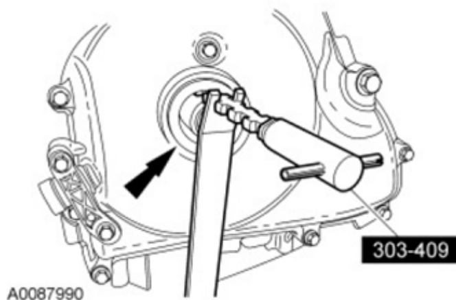
Fig. 330: Removing Crankshaft Front Oil Seal Courtesy of FORD MOTOR CO.
