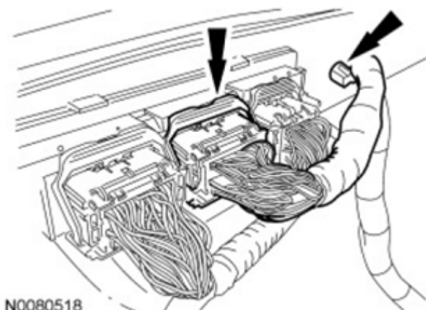
Fig. 526: Locating PCM Electrical Connector And Wire Harness Retainer Courtesy of FORD MOTOR CO.
