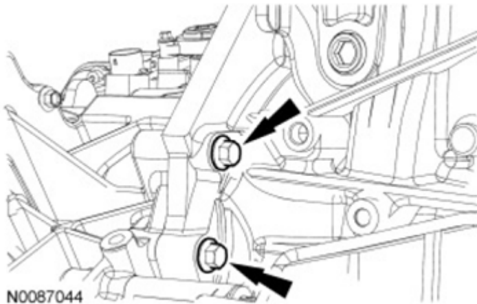
Fig. 163: Locating RH Engine-To-Bellhousing Bolts (All-Wheel Drive Vehicles) Courtesy of FORD MOTOR CO.
