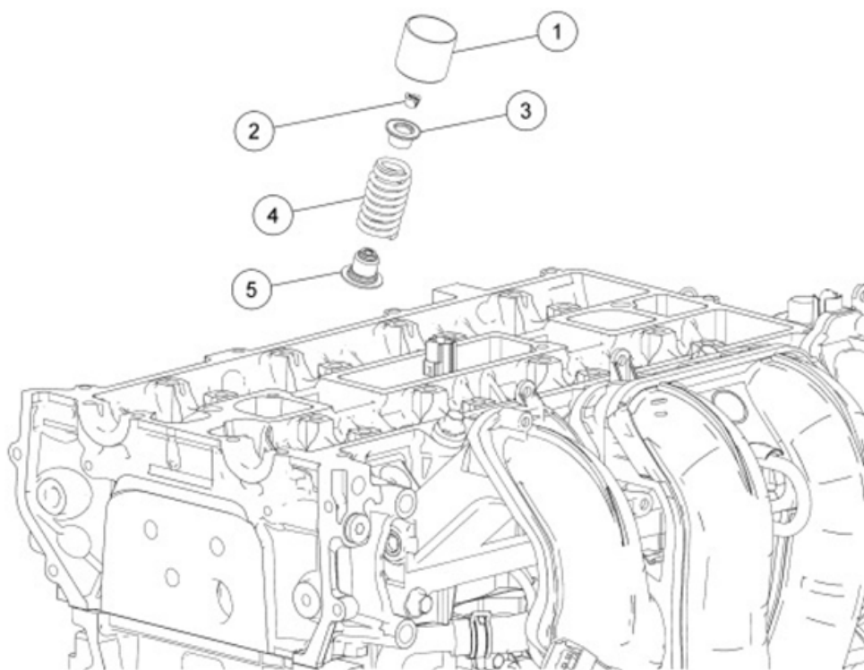
Fig. 138: Exploded View Of Valve Train Components Courtesy of FORD MOTOR CO.
