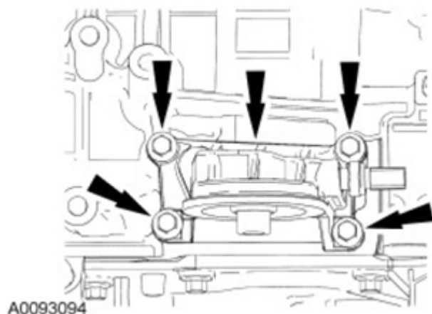
Fig. 477: Locating Oil Filter Adapter Bolts Courtesy of FORD MOTOR CO.
