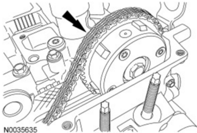
Fig. 122: Locating Timing Chain Of Intake Camshaft Drive Gear Courtesy of FORD MOTOR CO.
