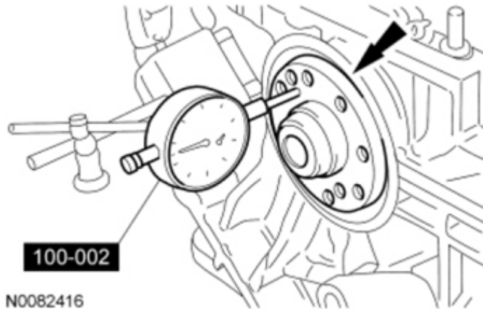
Fig. 389: Measuring Crankshaft End Play
