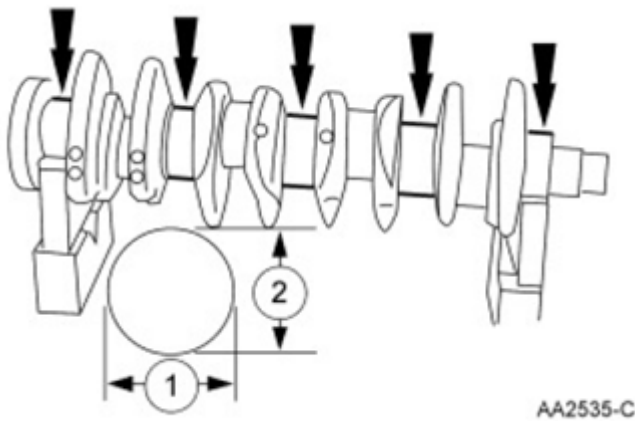
Fig. 375: Locating Crankshaft Main Bearing Journal Courtesy of FORD MOTOR CO.
