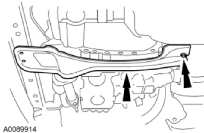
Fig. 565: Locating Engine Support Crossmember Rear Nut Courtesy of FORD MOTOR CO.
