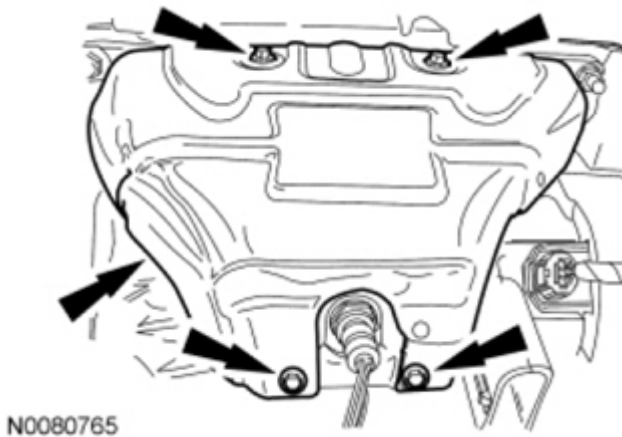
Fig. 284: Locating Exhaust Manifold Heat Shield With Bolts Courtesy of FORD MOTOR CO.
