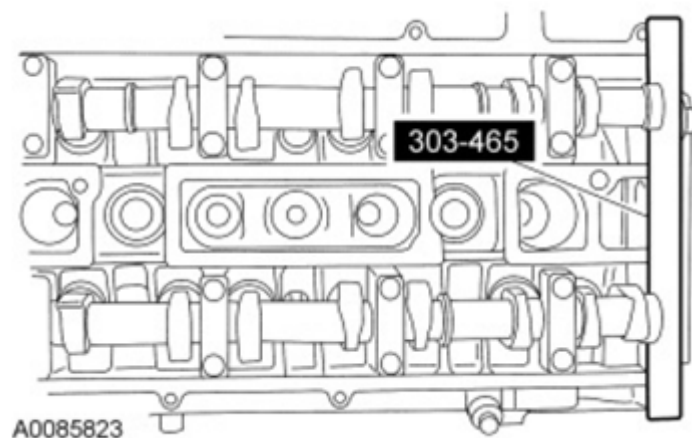
Fig. 417: View Of Camshaft Alignment Plate Courtesy of FORD MOTOR CO.
