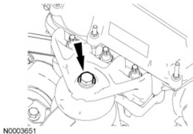
Fig. 268: Locating Engine Mount Bracket Bolt Courtesy of FORD MOTOR CO.
