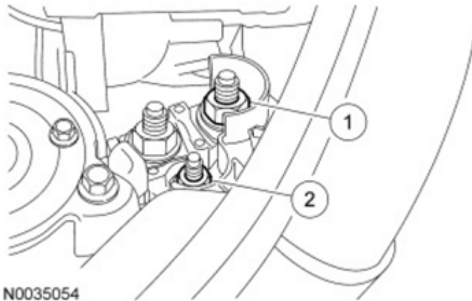
Fig. 227: Identifying Battery Cable And Starter Solenoid Terminal Nuts Courtesy of FORD MOTOR CO.
