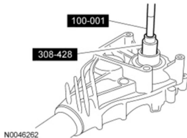
Fig. 235: Removing Intermediate Shaft Seal Courtesy of FORD MOTOR CO.
