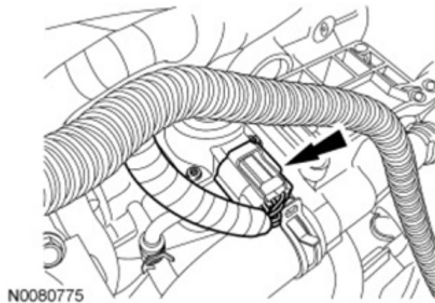
Fig. 303: Locating EGR Valve Electrical Connector Courtesy of FORD MOTOR CO.
