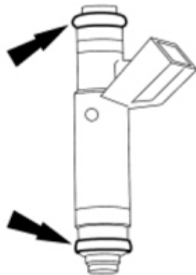
Fig. 460: Identifying Fuel Injector O-Rings Courtesy of FORD MOTOR CO.
