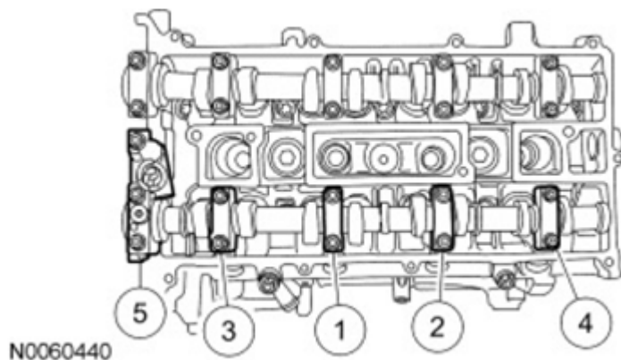
Fig. 127: Tightening Sequence Of Intake Camshaft Bearing Cap Bolts Courtesy of FORD MOTOR CO.
