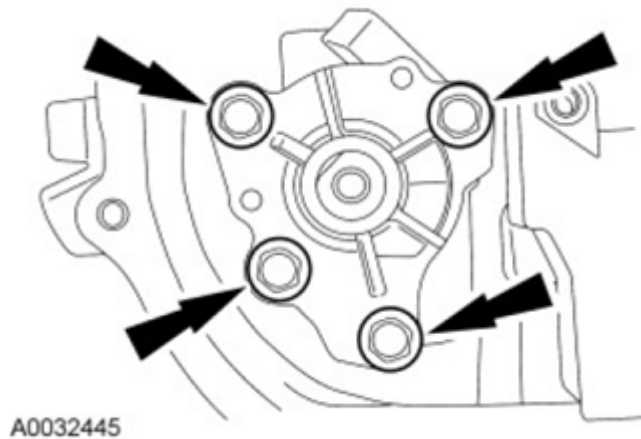
Fig. 350: Locating Oil Pump Bolts Courtesy of FORD MOTOR CO.
