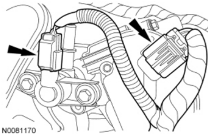
Fig. 302: Locating Evaporative Emission (EVAP) Canister Purge Valve Electrical Connectors Courtesy of FORD MOTOR CO.
