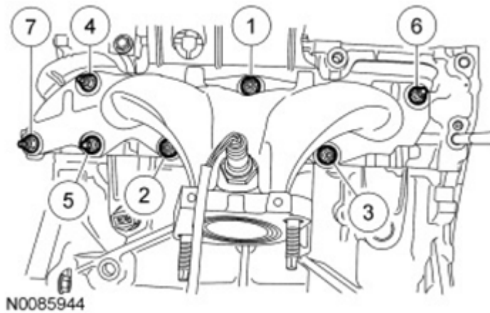
Fig. 487: Tightening Sequence Of Exhaust Manifold Gasket Nuts Courtesy of FORD MOTOR CO.
