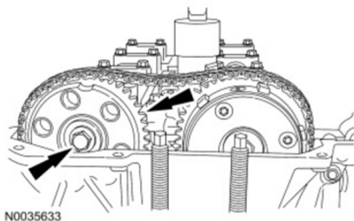
Fig. 130: Locating Exhaust Camshaft Bolt Courtesy of FORD MOTOR CO.
