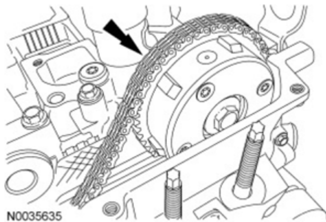
Fig. 95: Locating Timing Chain Of Intake Camshaft Drive Gear Courtesy of FORD MOTOR CO.
