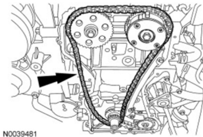
Fig. 335: View Of Timing Chain Courtesy of FORD MOTOR CO.
