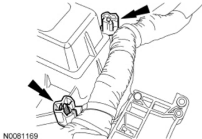
Fig. 472: Locating Wiring Harness Retainers Of LH Side Valve Cover Stud Bolts Courtesy of FORD MOTOR CO.
