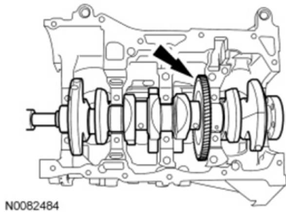
Fig. 385: View Of Crankshaft Courtesy of FORD MOTOR CO.
