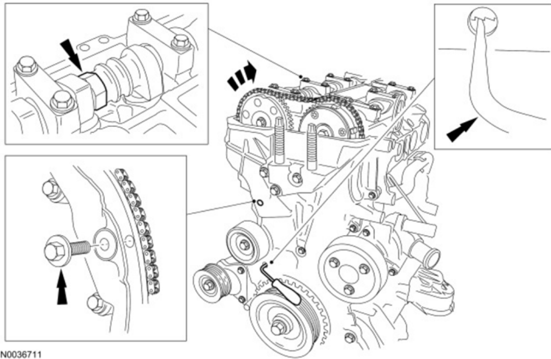
Fig. 119: Releasing Timing Chain Tensioner Ratchet Courtesy of FORD MOTOR CO.
