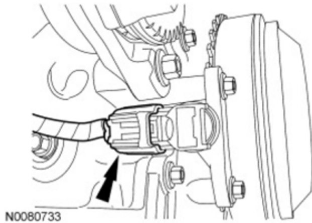
Fig. 493: Locating CKP Sensor Electrical Connector Courtesy of FORD MOTOR CO.
