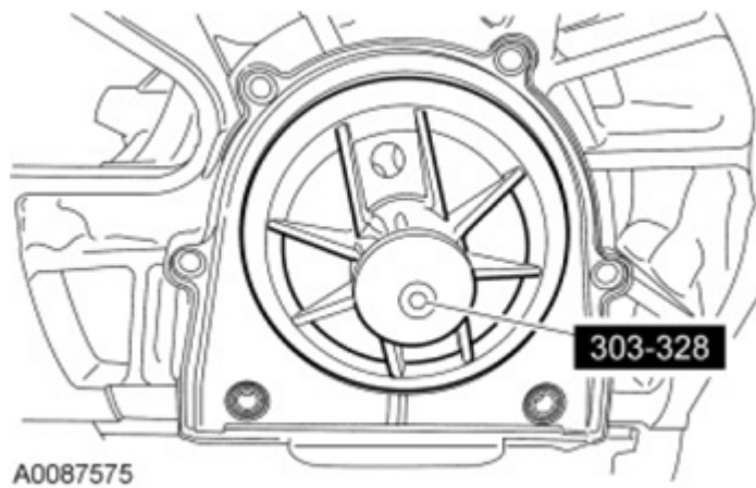
Fig. 401: Installing Crankshaft Rear Main Oil Seal Courtesy of FORD MOTOR CO.
