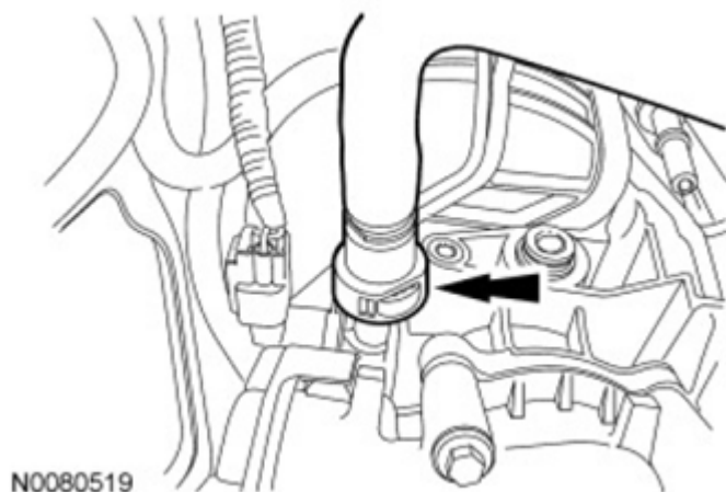
Fig. 206: Locating Fuel Vapor Return Tube Courtesy of FORD MOTOR CO.
