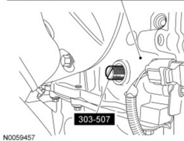
Fig. 438: View Of Crankshaft TDC Timing Peg Courtesy of FORD MOTOR CO.
