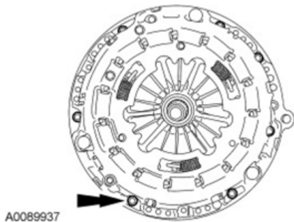
Fig. 276: Locating Clutch Pressure Plate Bolt Courtesy of FORD MOTOR CO.
