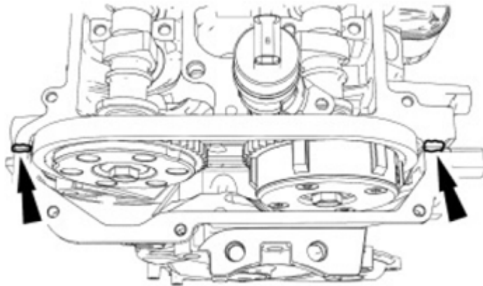
Fig. 447: Locating Silicone Gasket And Sealant Applying Locations Courtesy of FORD MOTOR CO.
