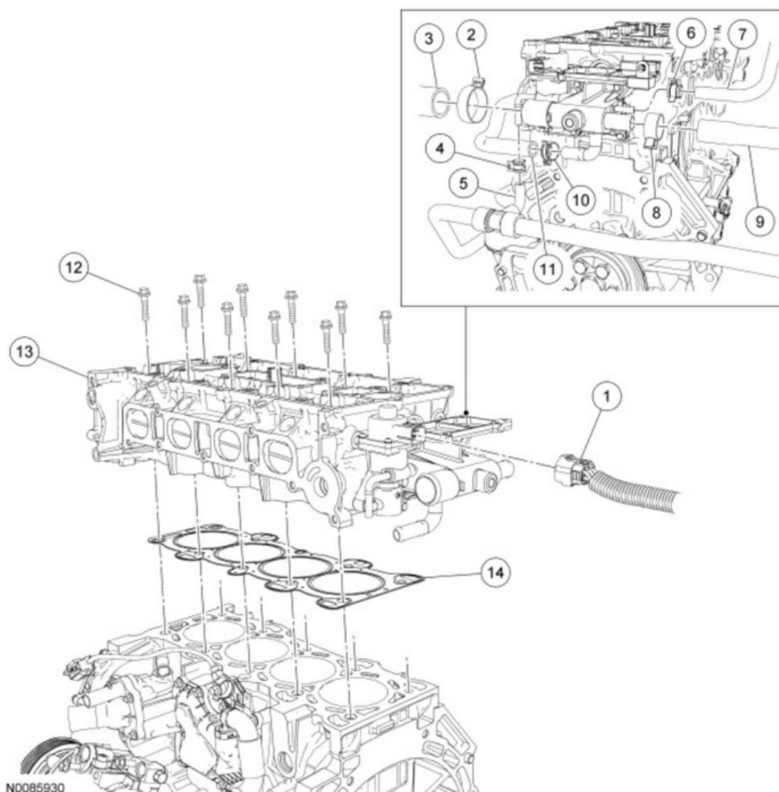
Fig. 146: Identifying Cylinder Head Components Courtesy of FORD MOTOR CO.
