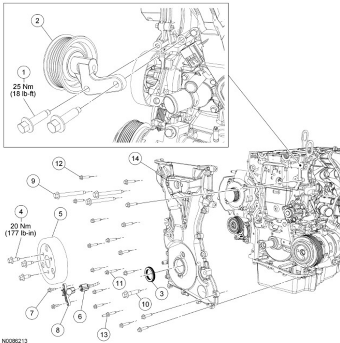
Fig. 56: Identifying Engine Front Cover Components With Torque Specifications Courtesy of FORD MOTOR CO.
