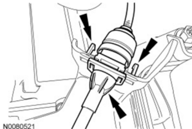
Fig. 535: View Of Transmission Shift Cable Tabs Courtesy of FORD MOTOR CO.
