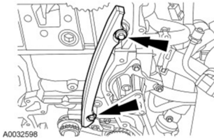
Fig. 419: Locating LH Timing Chain Guide Bolts Courtesy of FORD MOTOR CO.
