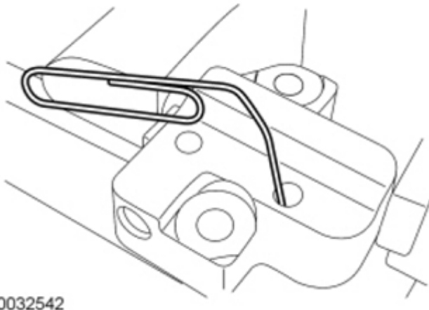
Fig. 80: Holding Ratchet Mechanism Courtesy of FORD MOTOR CO.
