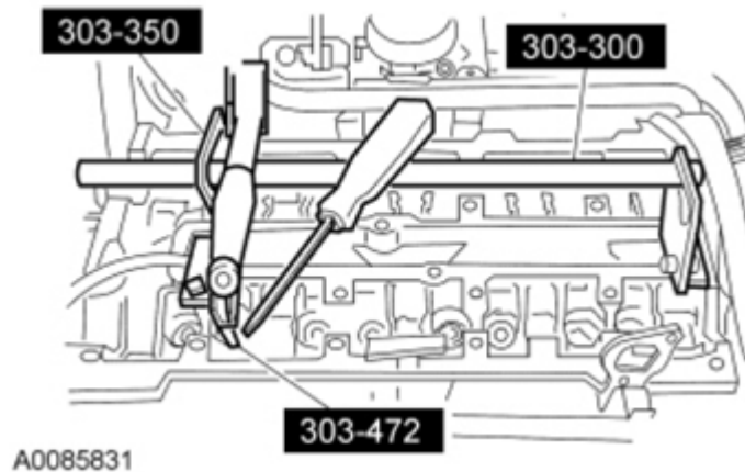
Fig. 363: Remove/Install Valve Spring Using Special Tools Courtesy of FORD MOTOR CO.
