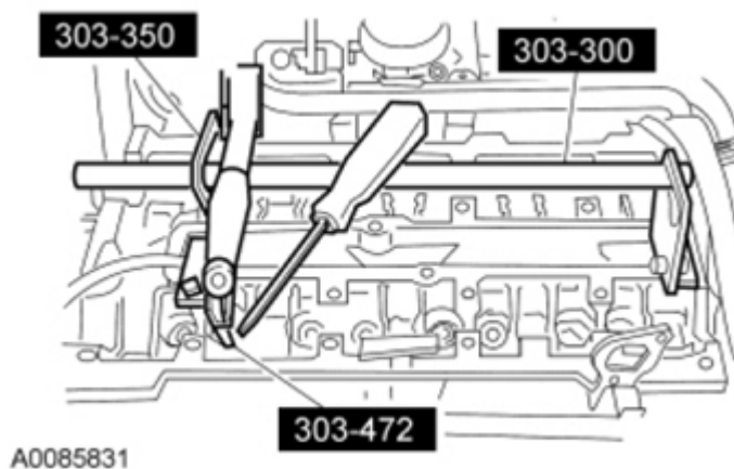
Fig. 366: Remove/Install Valve Spring Using Special Tools Courtesy of FORD MOTOR CO.
