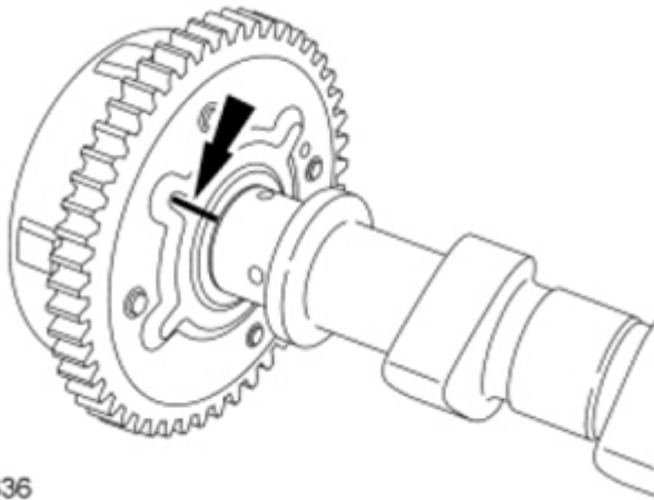
Fig. 126: View Of Sprocket And Camshaft Marking Courtesy of FORD MOTOR CO.
