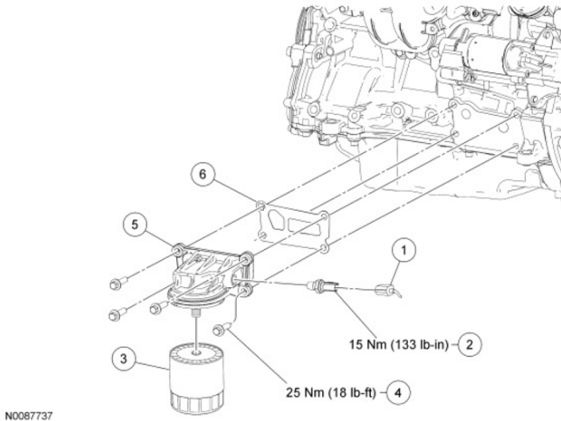
Fig. 155: Exploded View Of Engine Lubrication Components With Torque Specifications - (1 Of 5) Courtesy of FORD MOTOR CO.
