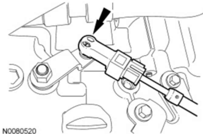
Fig. 198: View Of Shift Cable Of Transaxle Manual Lever Courtesy of FORD MOTOR CO.
