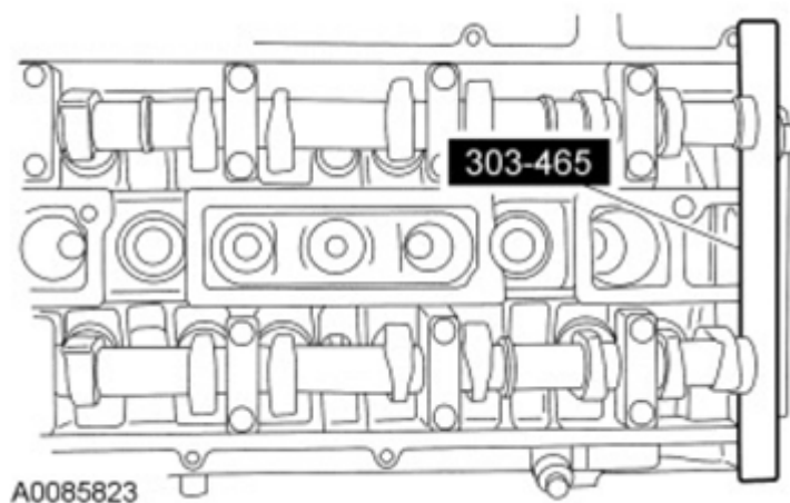
Fig. 28: View Of Camshaft Alignment Plate Courtesy of FORD MOTOR CO.
