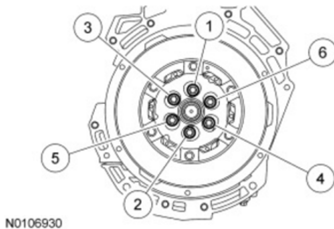
Fig. 50: Tightening Sequence Of Flywheel Bolts Courtesy of FORD MOTOR CO.
