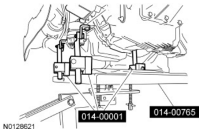
Fig. 499: Securing Engine And Transaxle Onto Powertrain Lift Courtesy of FORD MOTOR CO.
