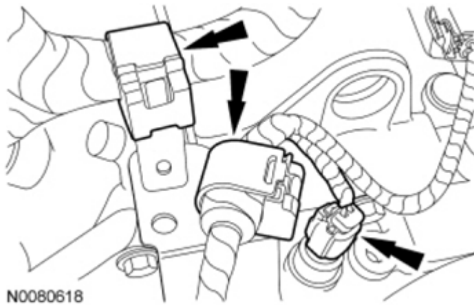
Fig. 581: Locating Reversing Lamp Indicator Switch Electrical Connector And Wiring Harness Retainers
