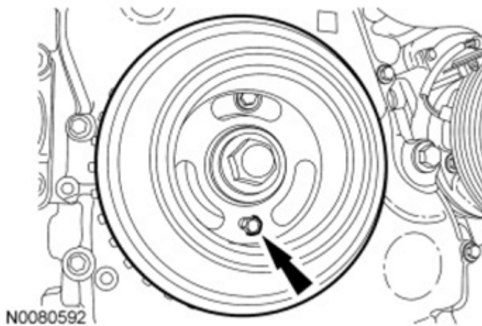
Fig. 35: View Of Crankshaft Pulley Alignment Bolt Courtesy of FORD MOTOR CO.
