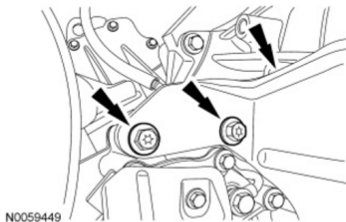
Fig. 220: Locating PTU Bracket-To-PTU Bolts And Bracket Courtesy of FORD MOTOR CO.
