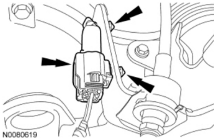
Fig. 582: Locating Vehicle Speed Sensor Electrical Connector And Pin-Type Retainers
