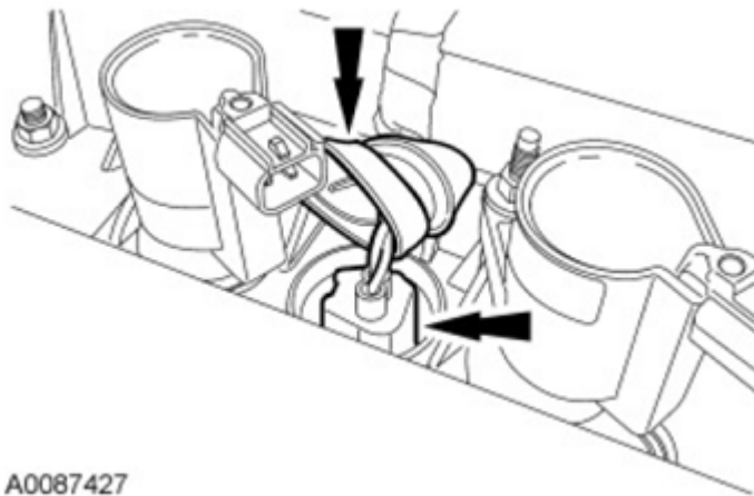
Fig. 306: Locating Cylinder Head Temperature Sensor Electrical Connector Courtesy of FORD MOTOR CO.
