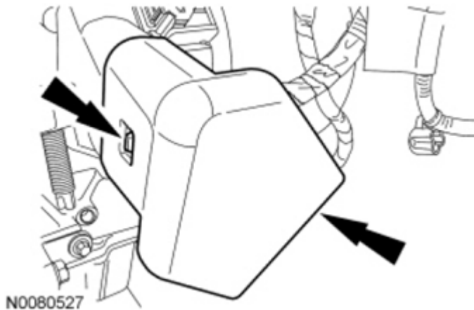
Fig. 549: Locating Locking Tab And Generator Air Duct Courtesy of FORD MOTOR CO.
