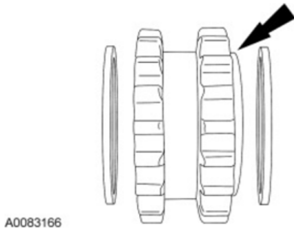
Fig. 413: View Of Crankshaft Sprocket Courtesy of FORD MOTOR CO.
