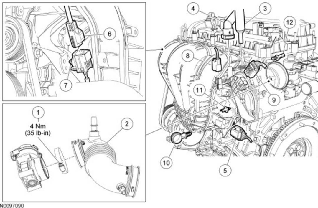
Fig. 18: Identifying Intake Manifold Components With Torque Specifications - (1 Of 2) Courtesy of FORD MOTOR CO.
