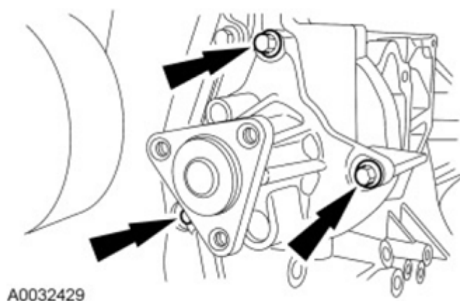
Fig. 481: Locating Coolant Pump Bolts Courtesy of FORD MOTOR CO.
