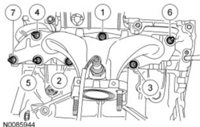
Fig. 178: Tightening Sequence Of Exhaust Manifold Gasket Nuts
