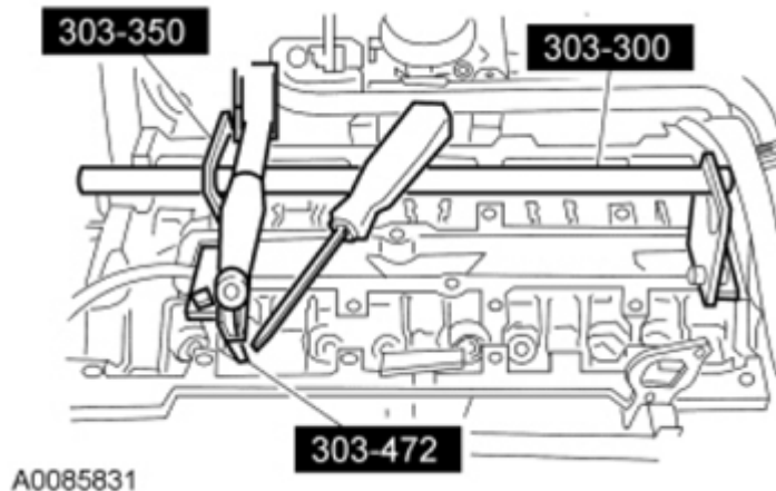
Fig. 139: Remove/Install Valve Spring Using Special Tools Courtesy of FORD MOTOR CO.
