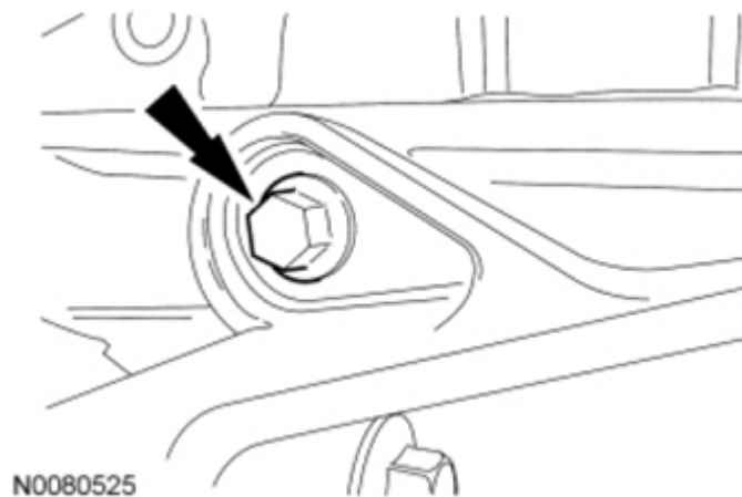
Fig. 515: Locating PTU Bracket-To-Engine Bolt Courtesy of FORD MOTOR CO.
