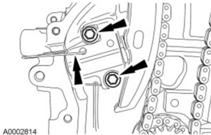
Fig. 426: Locating Timing Chain Tensioner Bolts Courtesy of FORD MOTOR CO.
