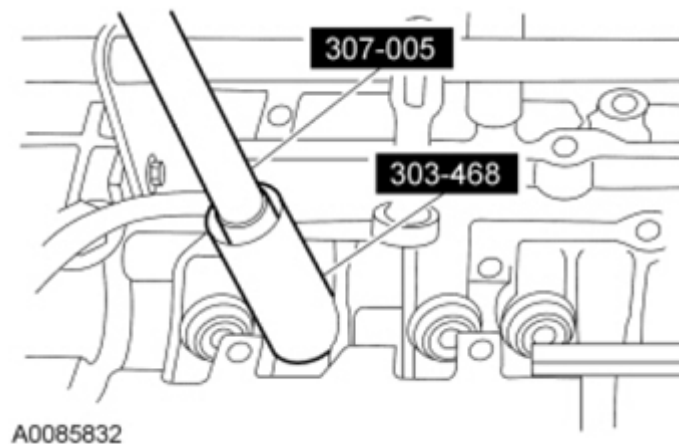
Fig. 364: Removing Valve Seal Courtesy of FORD MOTOR CO.
