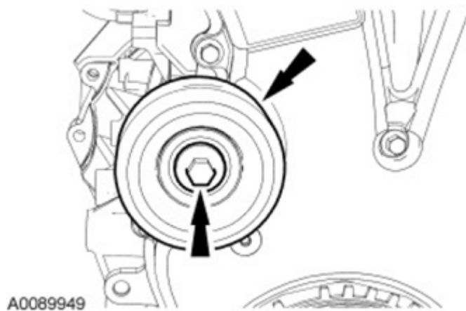
Fig. 484: Locating Accessory Drive Belt Idler Pulley And Bolt Courtesy of FORD MOTOR CO.
