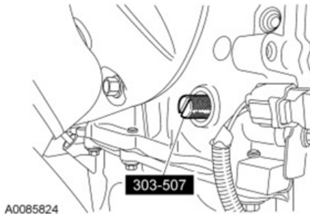
Fig. 107: View Of Crankshaft TDC Timing Peg Courtesy of FORD MOTOR CO.
