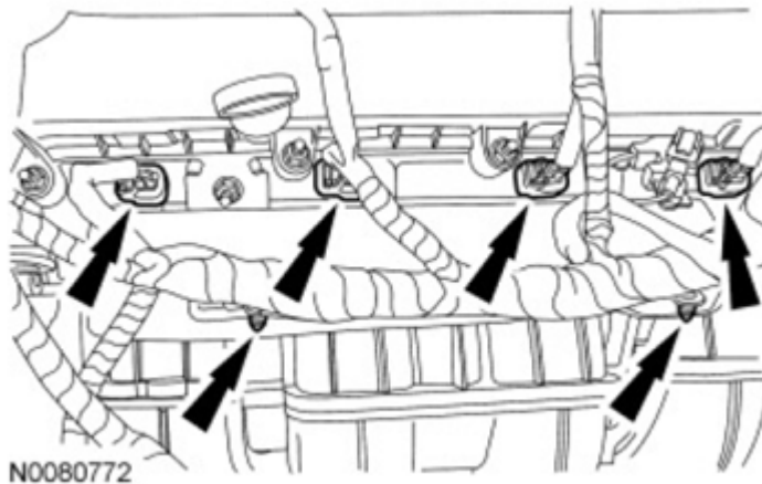
Fig. 308: Locating Fuel Injector Electrical Connectors And Retainers Courtesy of FORD MOTOR CO.
