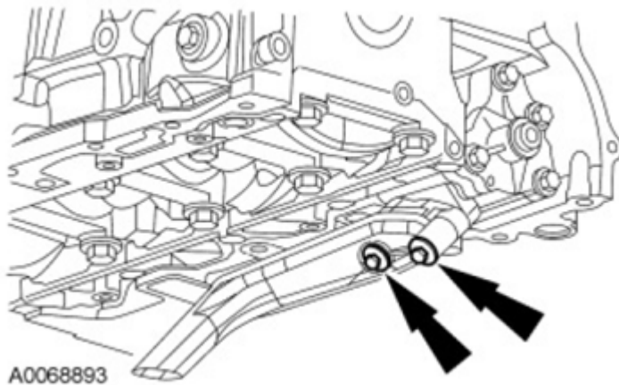
Fig. 349: Remove/Install Oil Pump Pickup Tube Bolts Courtesy of FORD MOTOR CO.
