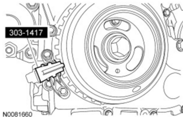
Fig. 64: Adjusting CKP Sensor Using Crankshaft Sensor Aligner Courtesy of FORD MOTOR CO.
