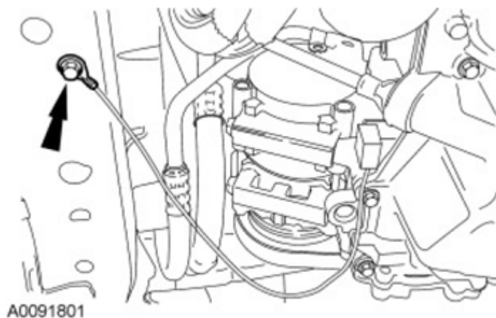
Fig. 239: Locating Ground Eyelet Bolts Courtesy of FORD MOTOR CO.
