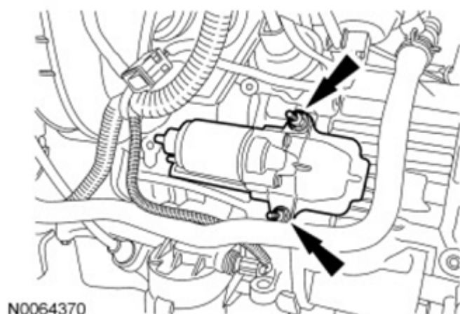
Fig. 555: Locating Starter Motor Stud Bolts Courtesy of FORD MOTOR CO.
