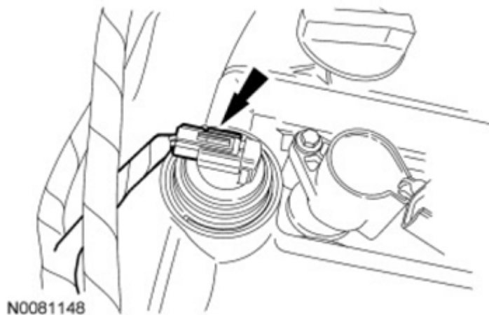
Fig. 297: Locating Variable Camshaft Timing (VCT) Electrical Connector Courtesy of FORD MOTOR CO.
