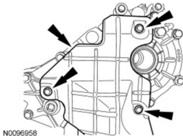
Fig. 234: Locating PTU Heat Shield Bolts Courtesy of FORD MOTOR CO.
