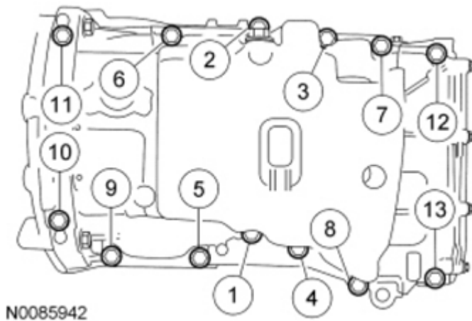
Fig. 55: Tightening Sequence Of Oil Pan Bolts Courtesy of FORD MOTOR CO.
