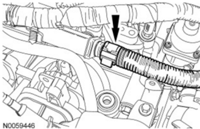
Fig. 572: Locating Fuel Supply Tube Quick Connect Coupling Courtesy of FORD MOTOR CO.
