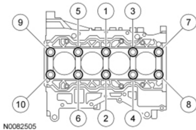
Fig. 377: Tightening Sequence Of Main Bearing Beam Bolts Courtesy of FORD MOTOR CO.
