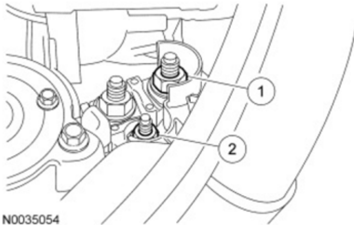
Fig. 508: Identifying Battery Cable And Starter Solenoid Terminal Nuts Courtesy of FORD MOTOR CO.
