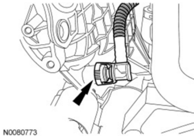
Fig. 458: Locating Crankcase Vent Oil Separator Tube Tab
