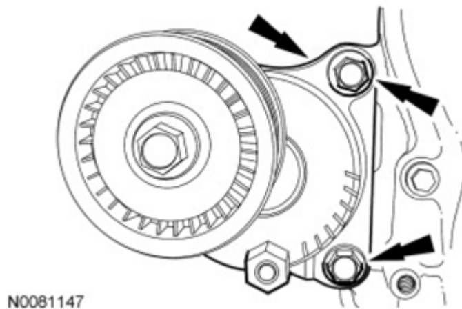
Fig. 287: Locating Accessory Drive Belt Tensioner And Bolts Courtesy of FORD MOTOR CO.
