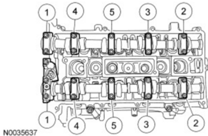
Fig. 344: Removing Sequence Of Camshaft Bearing Cap Bolts Courtesy of FORD MOTOR CO.
