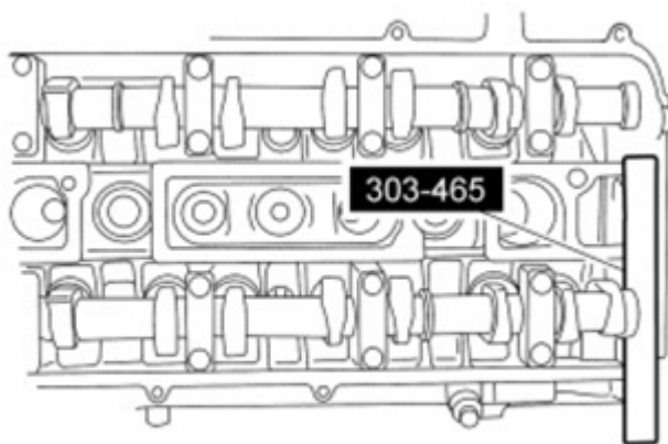
Fig. 94: View Of Camshaft Alignment Plate Courtesy of FORD MOTOR CO.
