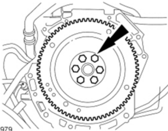
Fig. 278: Locating Flexplate Bolt Courtesy of FORD MOTOR CO.
