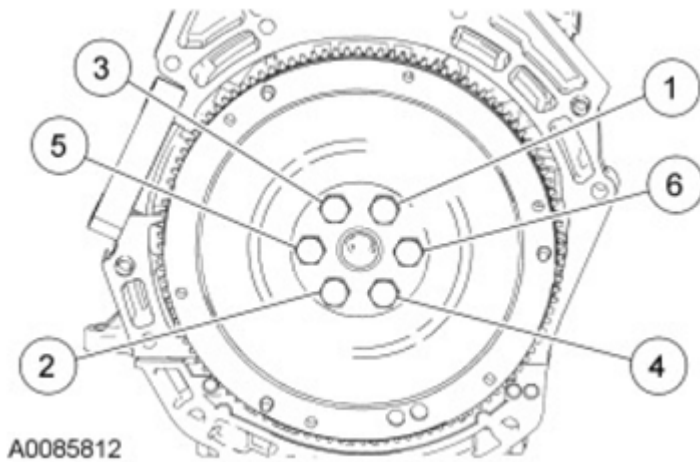
Fig. 49: Tightening Sequence Of Flexplate Bolts Courtesy of FORD MOTOR CO.
