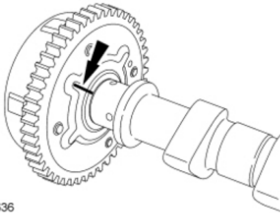
Fig. 99: View Of Sprocket And Camshaft Marking Courtesy of FORD MOTOR CO.
