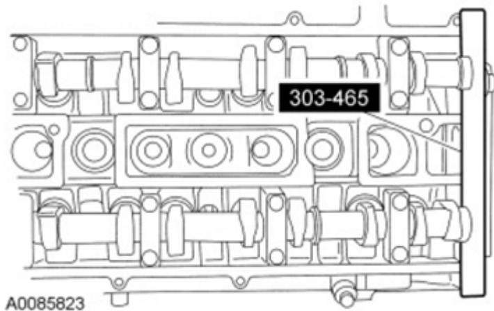
Fig. 112: View Of Camshaft Alignment Plate Courtesy of FORD MOTOR CO.
