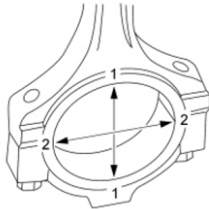
Fig. 380: Identifying Connecting Rod Large End Bore Dimensions Courtesy of FORD MOTOR CO.
