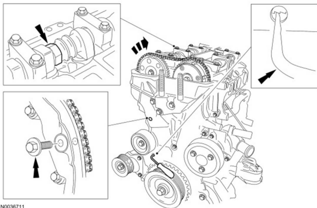
Fig. 92: Releasing Timing Chain Tensioner Ratchet Courtesy of FORD MOTOR CO.
