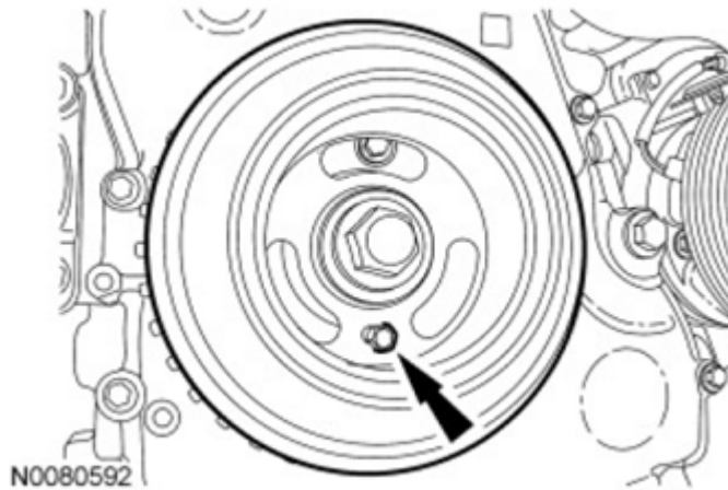
Fig. 434: View Of Crankshaft Pulley Alignment Bolt Courtesy of FORD MOTOR CO.
