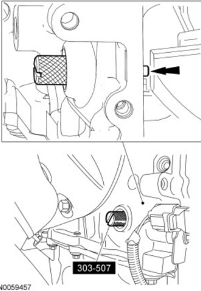
Fig. 398: View Of Crankshaft TDC Timing Peg Courtesy of FORD MOTOR CO.
