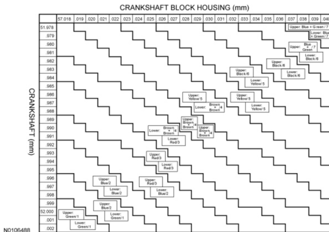
Fig. 379: Crankshaft Main Bearings Selection Chart Courtesy of FORD MOTOR CO.
