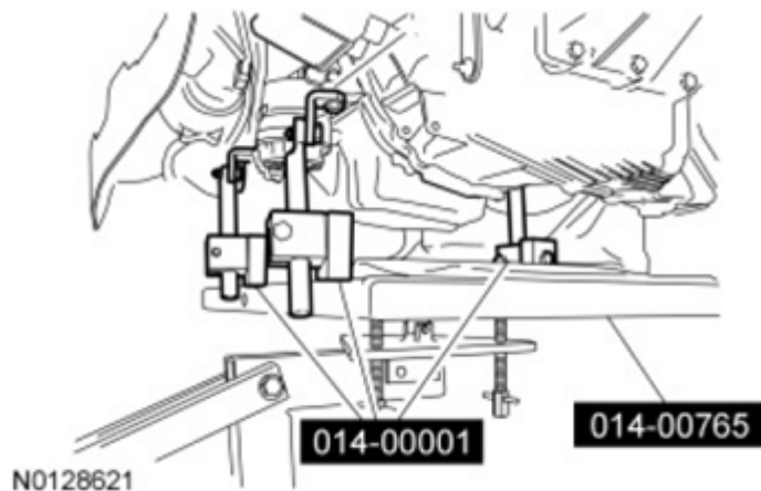
Fig. 222: Securing Engine And Transaxle Onto Powertrain Lift Courtesy of FORD MOTOR CO.
