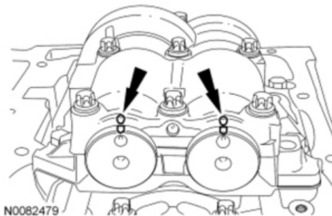
Fig. 352: Locating Balancer Unit Marks
