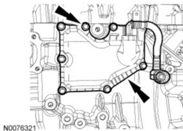
Fig. 319: Remove/Install Crankcase Vent Oil Separator Bolts Courtesy of FORD MOTOR CO.
