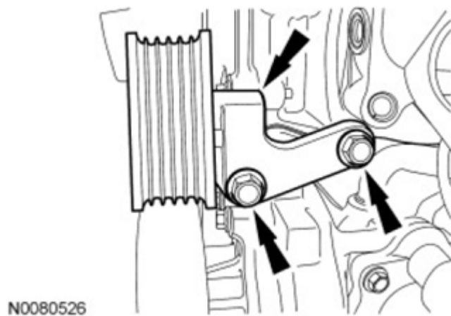
Fig. 483: Locating Accessory Drive Belt Idler Pulley And Bracket Bolts Courtesy of FORD MOTOR CO.
