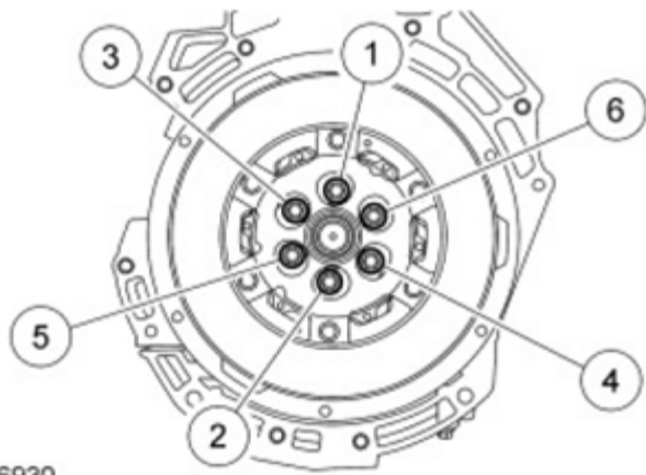
Fig. 495: Tightening Sequence Of Flywheel Bolts Courtesy of FORD MOTOR CO.
