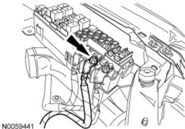
Fig. 241: Locating PDB Cable Nut Courtesy of FORD MOTOR CO.
