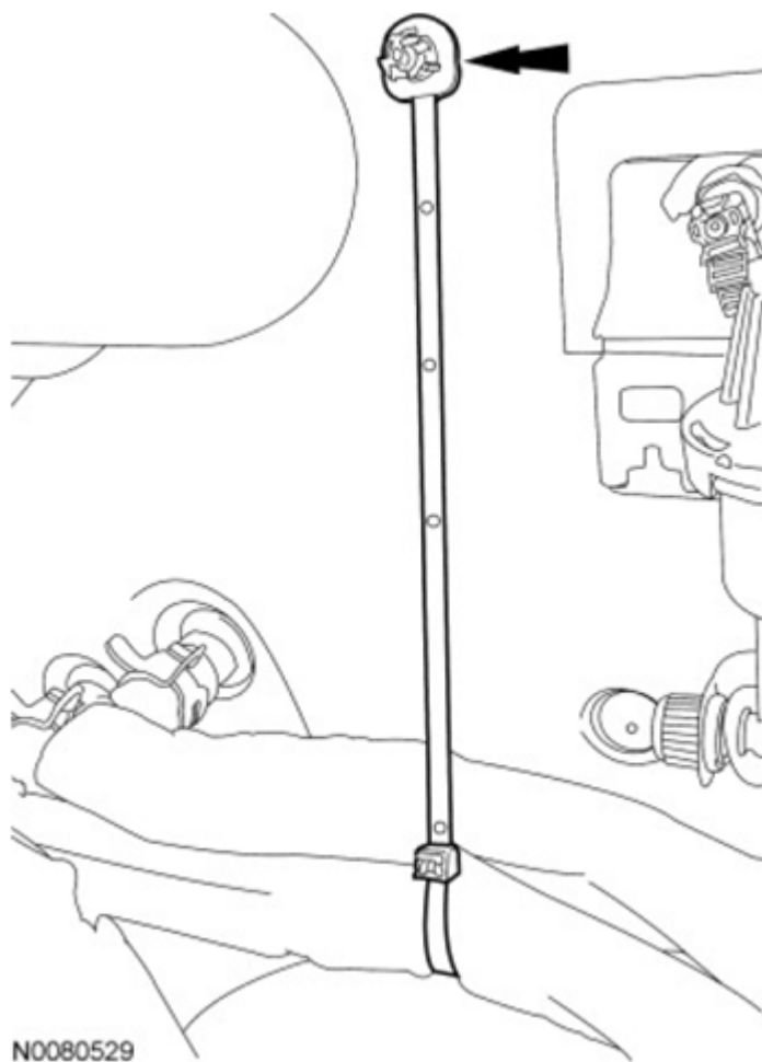
Fig. 252: Locating Heater Hose Support Strap Of Stud Courtesy of FORD MOTOR CO.
