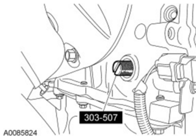
Fig. 38: View Of Crankshaft TDC Timing Peg Courtesy of FORD MOTOR CO.
