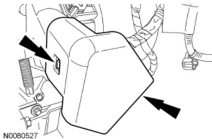
Fig. 238: Locating Locking Tab And Generator Air Duct Courtesy of FORD MOTOR CO.
