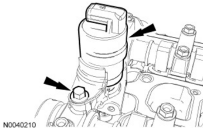
Fig. 342: Remove/Install VCT Solenoid And Bolt Courtesy of FORD MOTOR CO.
