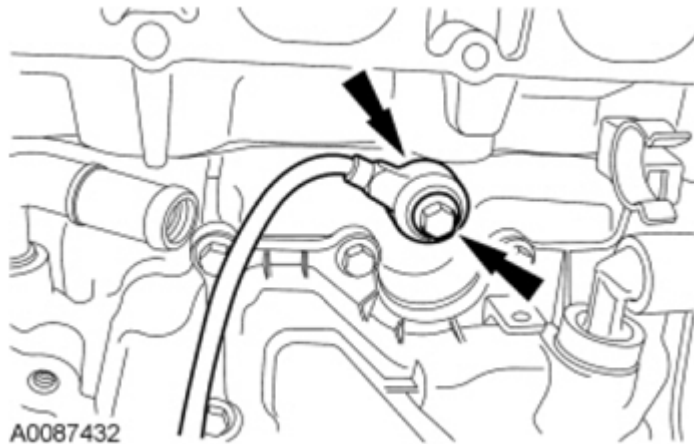
Fig. 453: Remove/Install KS With Bolt Courtesy of FORD MOTOR CO.
