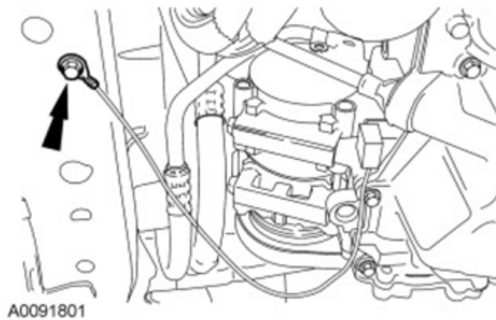
Fig. 187: Locating Ground Eyelet Bolts Courtesy of FORD MOTOR CO.
