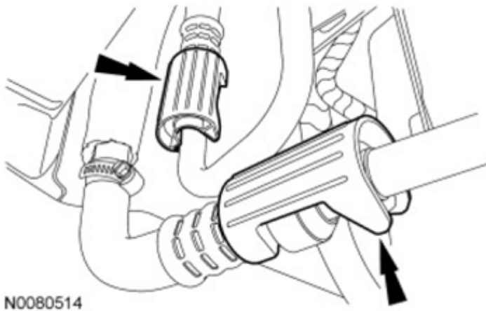
Fig. 543: Locating Secondary Latches Of Transaxle Fluid Cooler Tubes Courtesy of FORD MOTOR CO.
