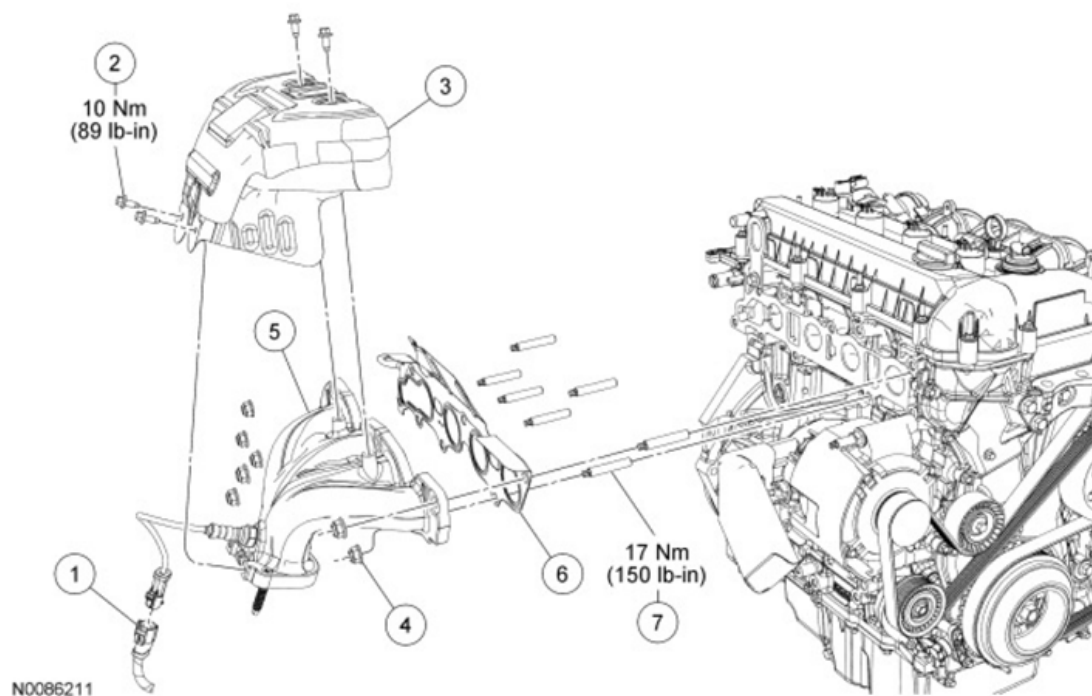
Fig. 177: Identifying Exhaust Manifold Components With Torque Specifications Courtesy of FORD MOTOR CO.
