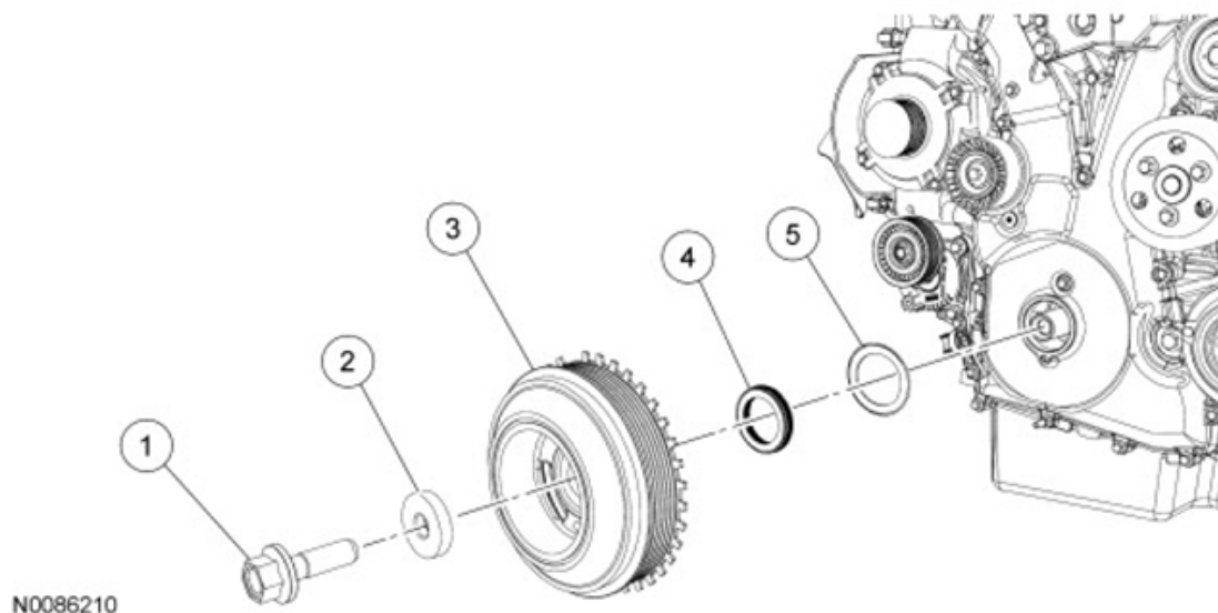
Fig. 26: Exploded View Of Lower End Components Courtesy of FORD MOTOR CO.
