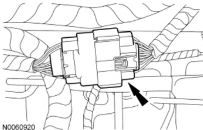
Fig. 525: Locating Engine Control Harness Electrical Connector Courtesy of FORD MOTOR CO.
