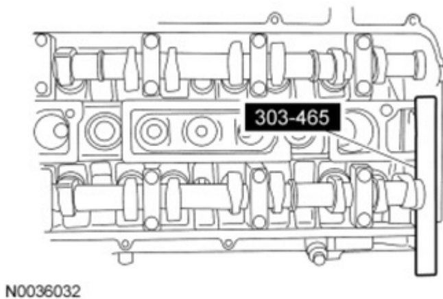
Fig. 91: View Of Camshaft Alignment Plate Courtesy of FORD MOTOR CO.
