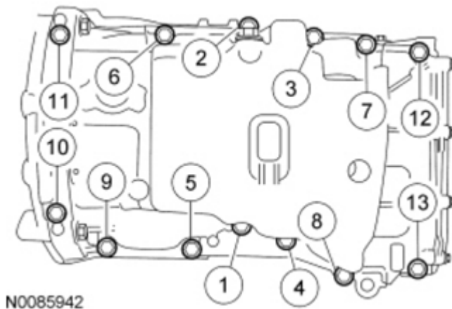
Fig. 168: Tightening Sequence Of Oil Pan Bolts Courtesy of FORD MOTOR CO.
