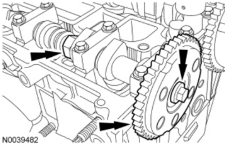
Fig. 71: View Of Exhaust Camshaft Sprocket With Bolt Courtesy of FORD MOTOR CO.
