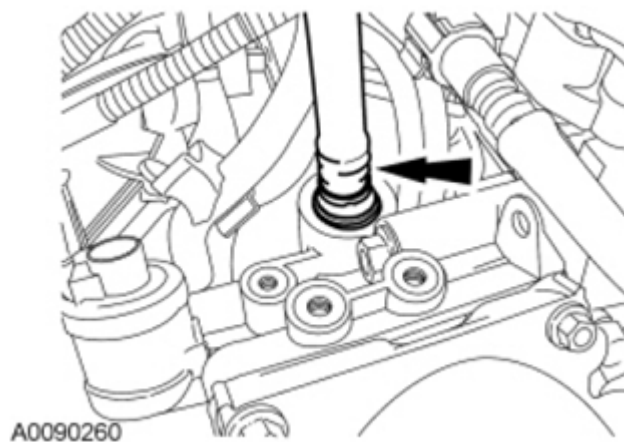
Fig. 529: Locating Vacuum Supply Tube Courtesy of FORD MOTOR CO.
