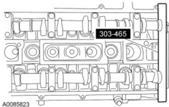
Fig. 441: View Of Camshaft Alignment Plate Courtesy of FORD MOTOR CO.
