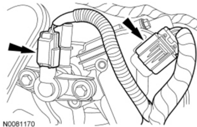
Fig. 470: Locating Evaporative Emission (EVAP) Canister Purge Valve Electrical Connectors Courtesy of FORD MOTOR CO.
