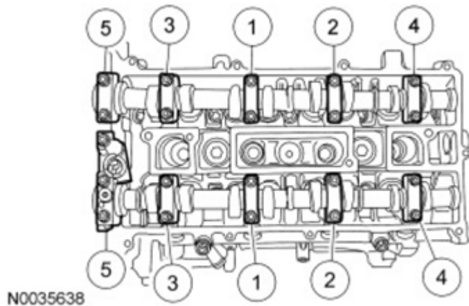
Fig. 410: Identifying Tightening Sequence Of Camshaft Bearing Cap Bolts Courtesy of FORD MOTOR CO.
