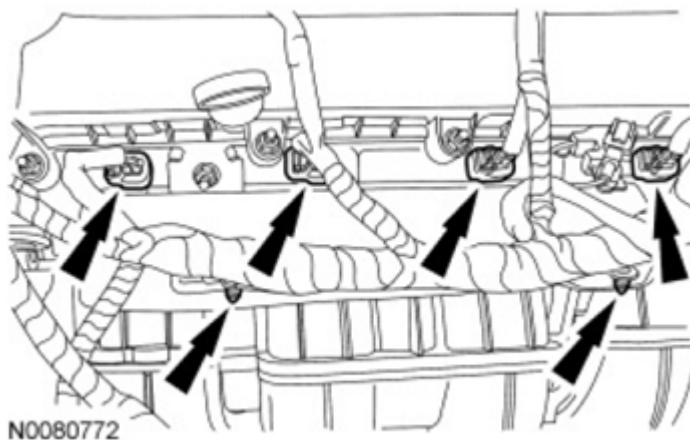
Fig. 464: Locating Fuel Injector Electrical Connectors And Retainers Courtesy of FORD MOTOR CO.
