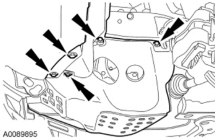
Fig. 165: Locating LH Splash Shield Retainers Courtesy of FORD MOTOR CO.
