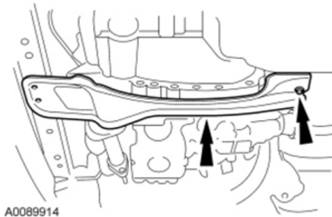
Fig. 214: Locating Engine Support Crossmember Rear Nut Courtesy of FORD MOTOR CO.
