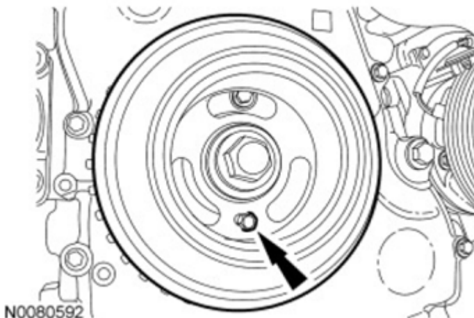
Fig. 62: View Of Crankshaft Pulley Alignment Bolt Courtesy of FORD MOTOR CO.
