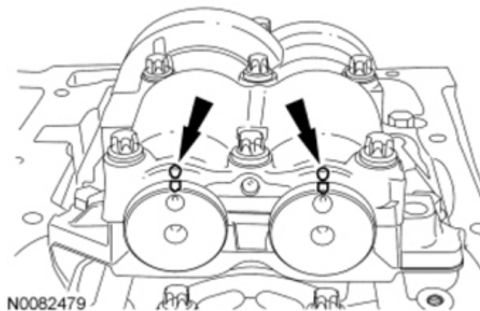
Fig. 393: Locating Balancer Unit Marks Courtesy of FORD MOTOR CO.
