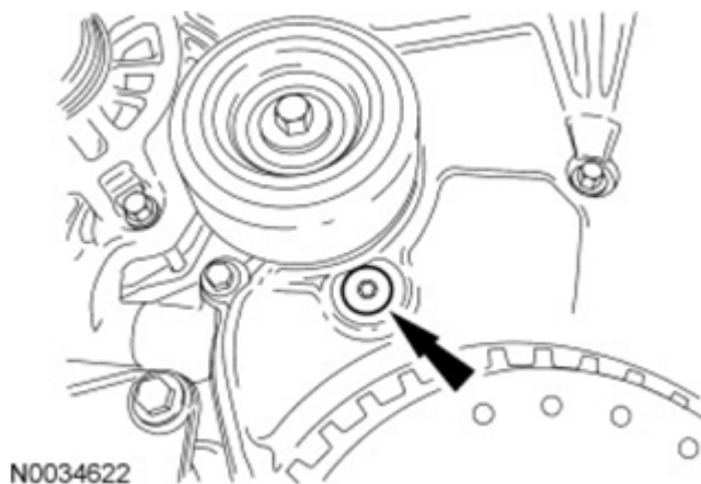
Fig. 89: Locating Lower Front Cover Timing Hole Plug Courtesy of FORD MOTOR CO.
