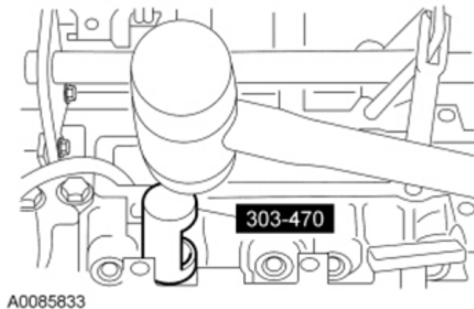
Fig. 144: Installing Valve Seal Courtesy of FORD MOTOR CO.
