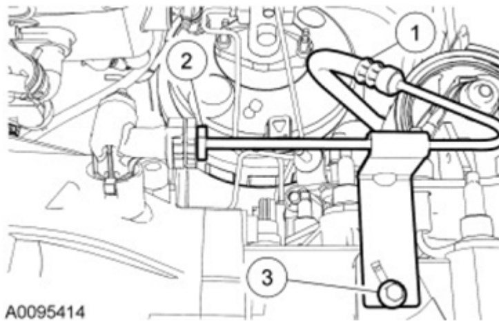
Fig. 583: Identifying Clutch Hydraulic Line And Bracket-To-Transaxle Bolt Courtesy of FORD MOTOR CO.
