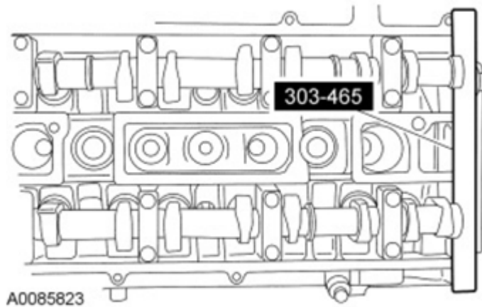
Fig. 101: View Of Camshaft Alignment Plate Courtesy of FORD MOTOR CO.
