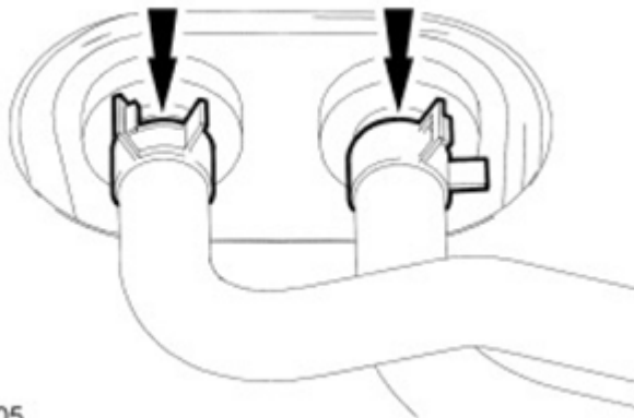
Fig. 530: Locating Heater Hoses Of Heater Core Courtesy of FORD MOTOR CO.
