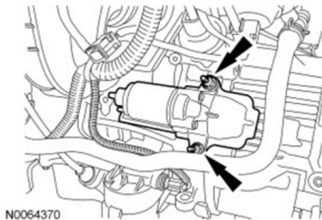
Fig. 506: Locating Starter Motor Stud Bolts Courtesy of FORD MOTOR CO.
