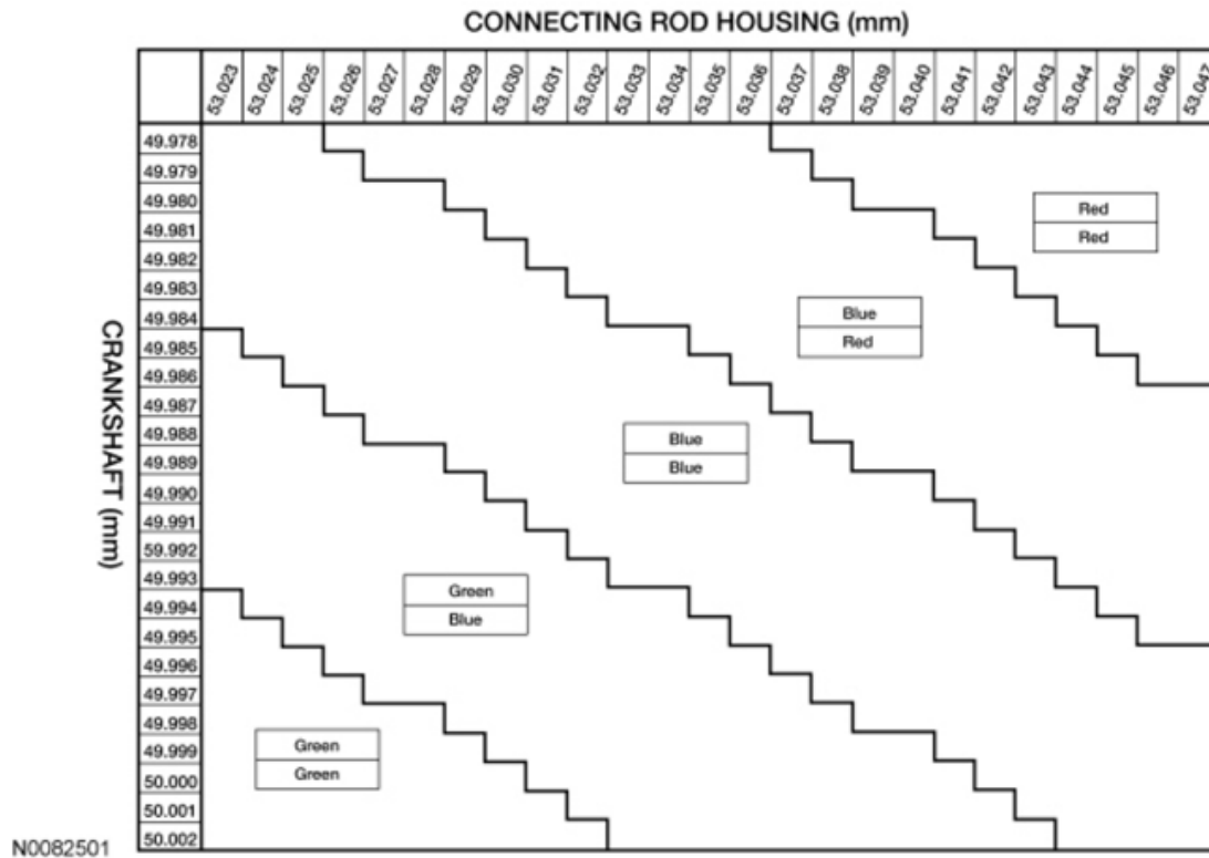
Fig. 382: Connecting Rod Bearings Selection Chart Courtesy of FORD MOTOR CO.
