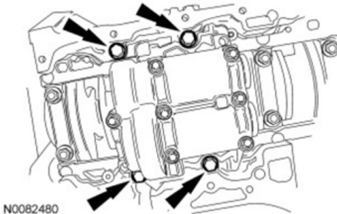
Fig. 353: Locating Balancer Unit Bolts Courtesy of FORD MOTOR CO.
