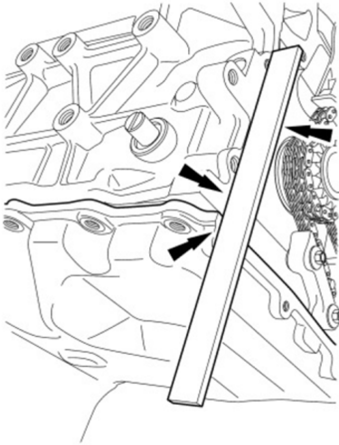
Fig. 175: Aligning Front Surface Of Oil Pan Courtesy of FORD MOTOR CO.
