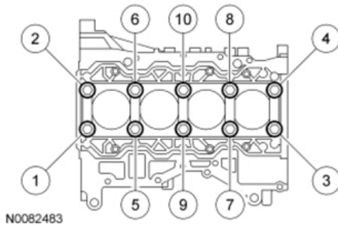
Fig. 357: Removing Order Of Main Bearing Beam Bolts Courtesy of FORD MOTOR CO.
