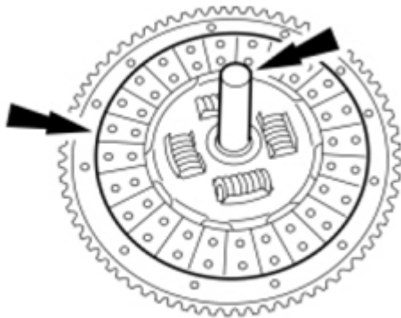
Fig. 497: Positioning Clutch Disc On Flywheel Courtesy of FORD MOTOR CO.
