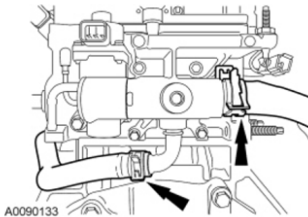
Fig. 454: Locating Coolant Hoses Courtesy of FORD MOTOR CO.
