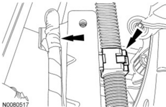
Fig. 537: Locating Battery Tray Bracket Wiring Harness Retainers Courtesy of FORD MOTOR CO.
