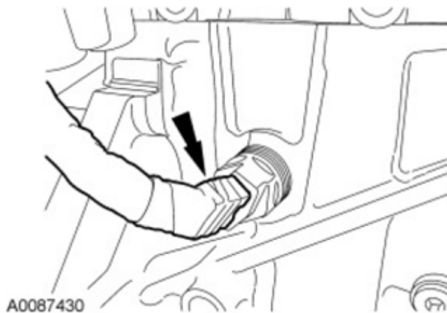
Fig. 578: Locating Block Heater Electrical Connector Courtesy of FORD MOTOR CO.
