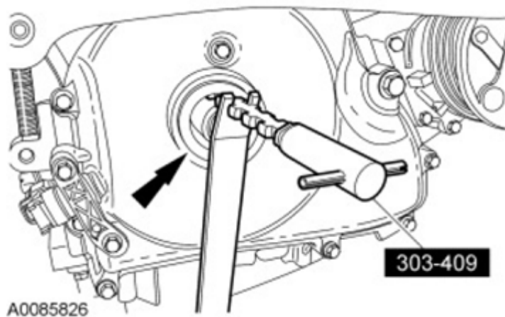
Fig. 57: Removing Crankshaft Front Oil Seal Using Oil Seal Remover Courtesy of FORD MOTOR CO.
