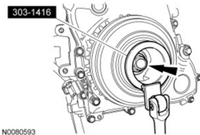
Fig. 433: Remove/Install Crankshaft Pulley Bolt Courtesy of FORD MOTOR CO.
