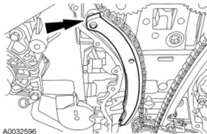
Fig. 334: Locating RH Timing Chain Guide Courtesy of FORD MOTOR CO.
