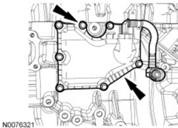
Fig. 452: Remove/Install Crankcase Vent Oil Separator Bolts Courtesy of FORD MOTOR CO.
