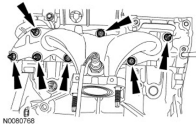
Fig. 285: Locating Exhaust Manifold Nuts Courtesy of FORD MOTOR CO.
