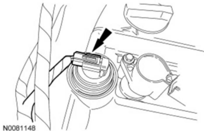
Fig. 475: Locating Variable Camshaft Timing (VCT) Electrical Connector Courtesy of FORD MOTOR CO.
