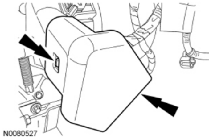
Fig. 590: Locating Locking Tab And Generator Air Duct Courtesy of FORD MOTOR CO.
