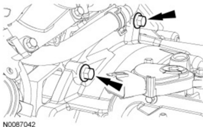
Fig. 162: Locating Upper Bellhousing-To-Engine Bolts Courtesy of FORD MOTOR CO.
