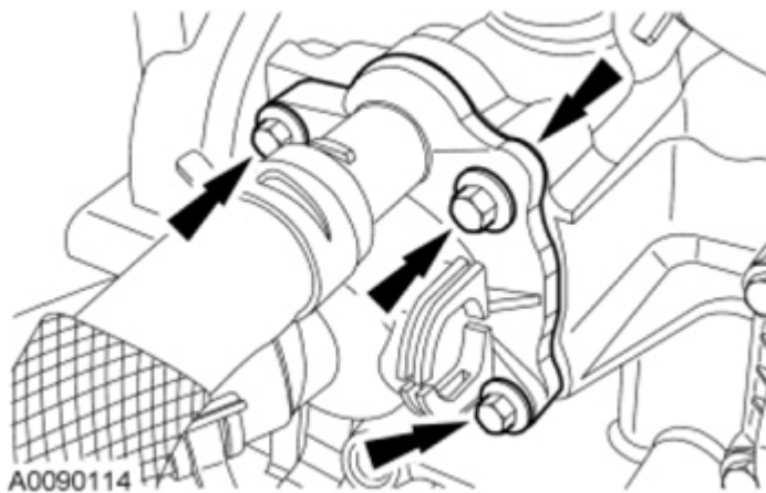
Fig. 480: Locating Thermostat Housing And Bolts Courtesy of FORD MOTOR CO.
