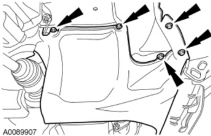
Fig. 161: Locating RH Splash Shield Bolts
