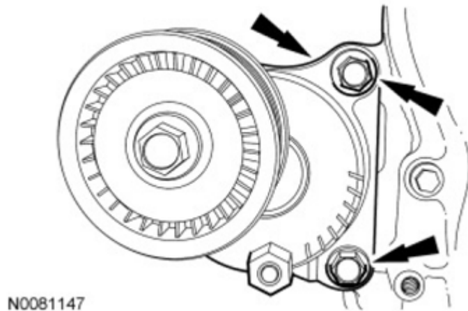
Fig. 485: Locating Accessory Drive Belt Tensioner And Bolts Courtesy of FORD MOTOR CO.
