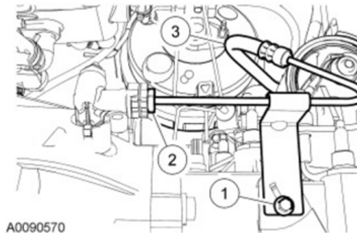
Fig. 245: Identifying Clutch Hydraulic Line And Bracket-To-Transaxle Bolt Courtesy of FORD MOTOR CO.
