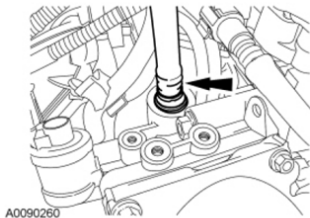
Fig. 574: Locating Vacuum Supply Tube Courtesy of FORD MOTOR CO.
