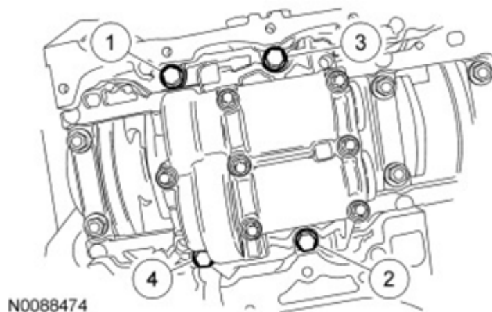
Fig. 9: Tightening Sequence Of Balancer Unit Bolts Courtesy of FORD MOTOR CO.
