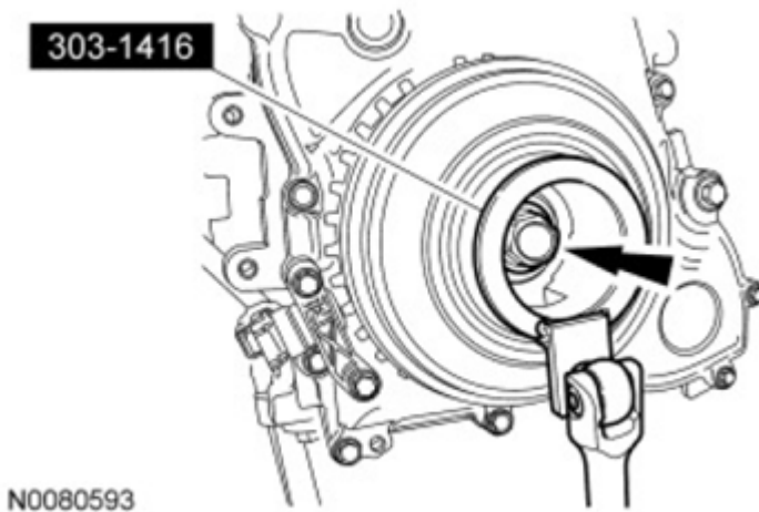
Fig. 31: Remove/Install Crankshaft Pulley Bolt Courtesy of FORD MOTOR CO.
