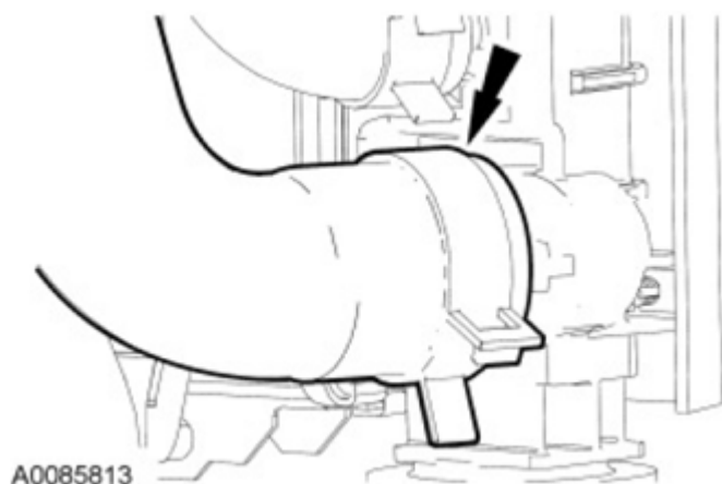
Fig. 522: Locating Lower Radiator Hose Courtesy of FORD MOTOR CO.
