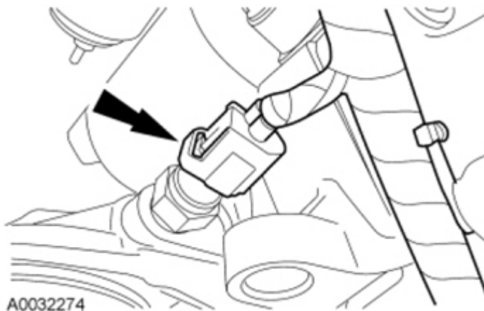
Fig. 294: Locating Engine Oil Pressure Switch Electrical Connector Courtesy of FORD MOTOR CO.
