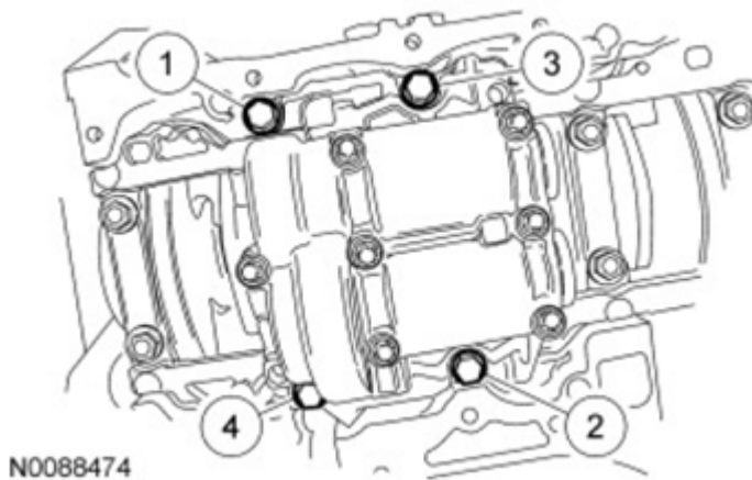
Fig. 394: Tightening Sequence Of Balancer Unit Bolts Courtesy of FORD MOTOR CO.
