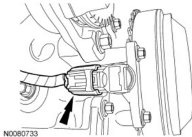
Fig. 279: Locating CKP Sensor Electrical Connector Courtesy of FORD MOTOR CO.
