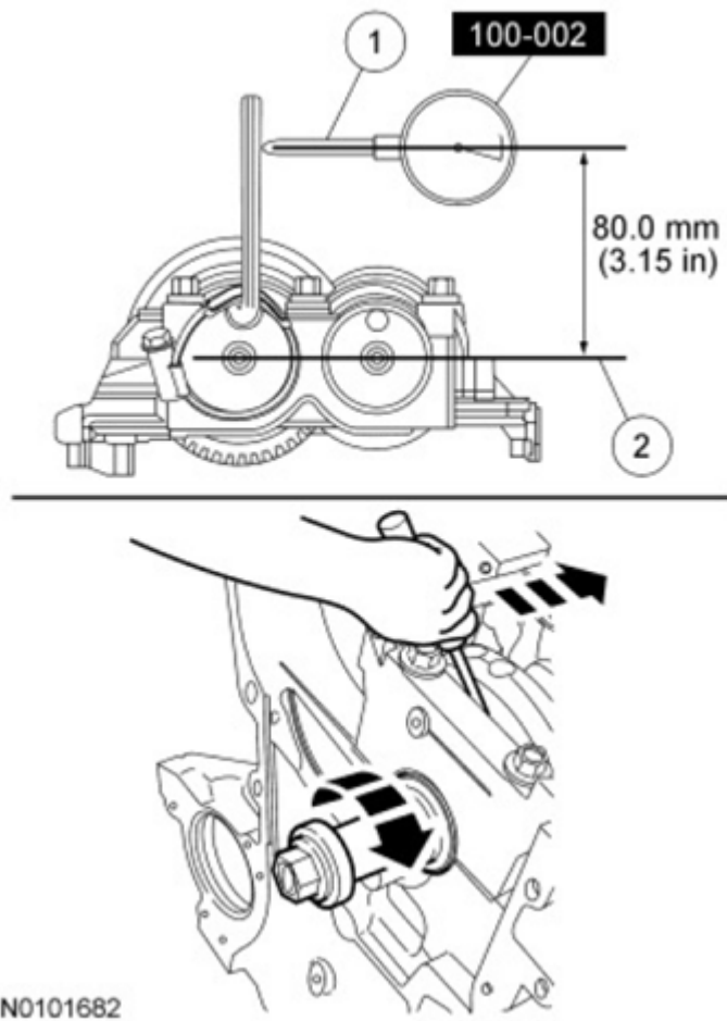
Fig. 397: Measuring Gear Backlash With Specifications Courtesy of FORD MOTOR CO.
