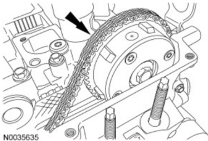
Fig. 129: Locating Timing Chain Of Intake Camshaft Drive Gear Courtesy of FORD MOTOR CO.
