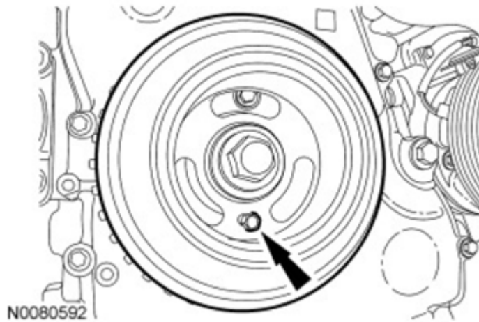
Fig. 115: View Of Crankshaft Pulley Alignment Bolt Courtesy of FORD MOTOR CO.
