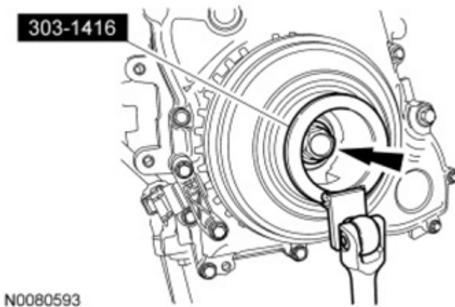
Fig. 329: Remove/Install Crankshaft Pulley Bolt Courtesy of FORD MOTOR CO.
