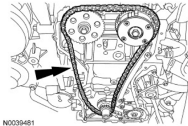
Fig. 420: View Of Timing Chain Courtesy of FORD MOTOR CO.
