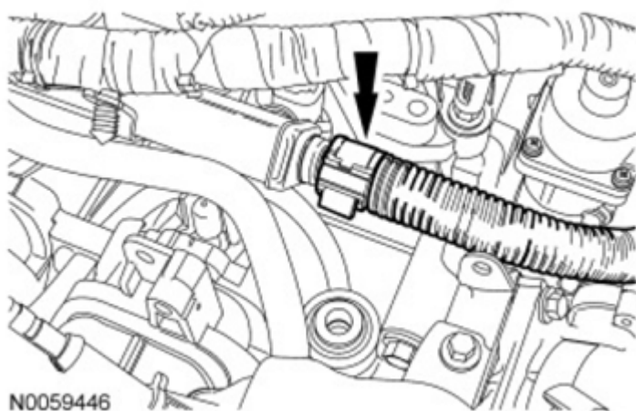
Fig. 527: Locating Fuel Supply Tube Quick Connect Coupling Courtesy of FORD MOTOR CO.
