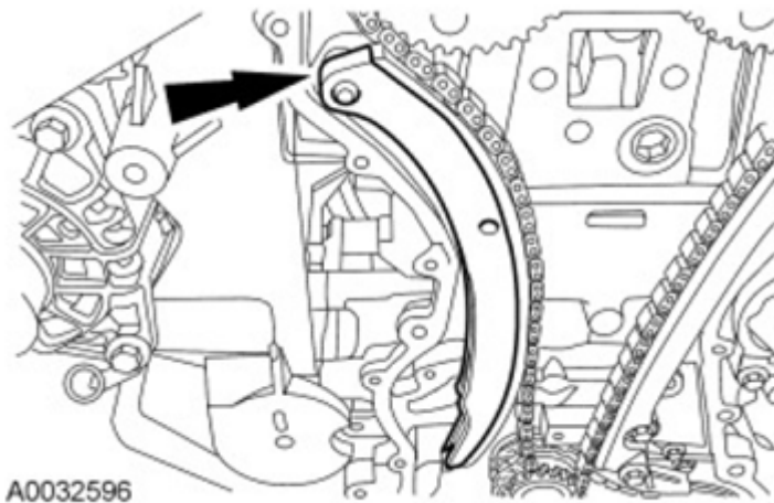
Fig. 68: Locating RH Timing Chain Guide Courtesy of FORD MOTOR CO.
