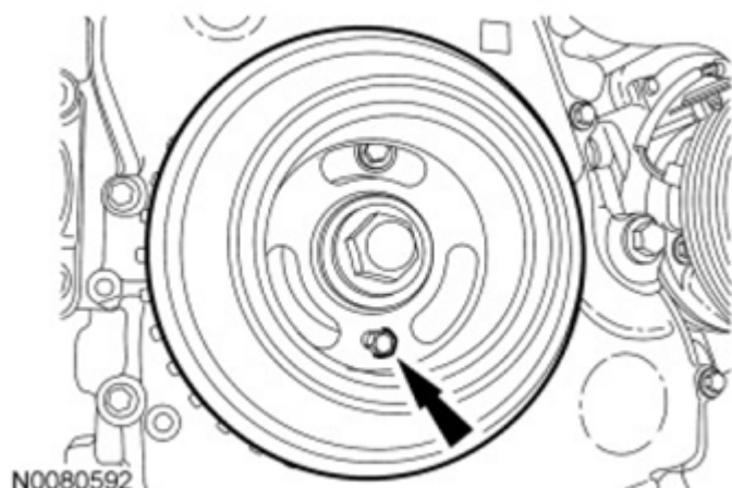
Fig. 439: View Of Crankshaft Pulley Alignment Bolt Courtesy of FORD MOTOR CO.
