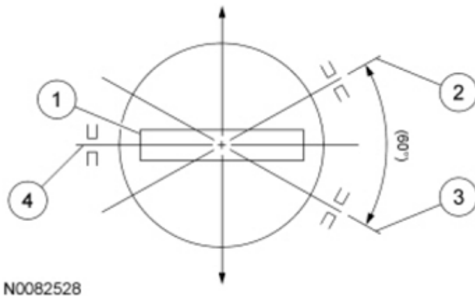
Fig. 368: Piston Rings Positioning Diagram Courtesy of FORD MOTOR CO.
