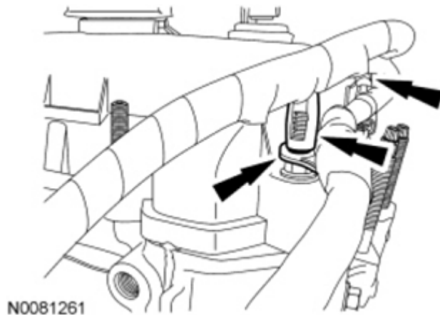
Fig. 474: Locating Wiring Harness Retainers Of RH Side Valve Cover Stud Bolt Courtesy of FORD MOTOR CO.
