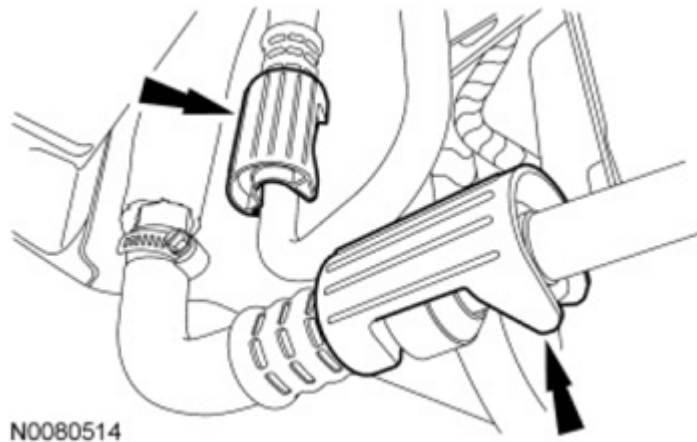
Fig. 191: Locating Secondary Latches Of Transaxle Fluid Cooler Tubes Courtesy of FORD MOTOR CO.
