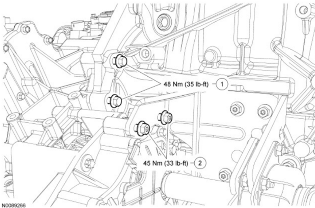
Fig. 157: Exploded View Of Engine Lubrication Components With Torque Specifications - (3 Of 5) Courtesy of FORD MOTOR CO.
