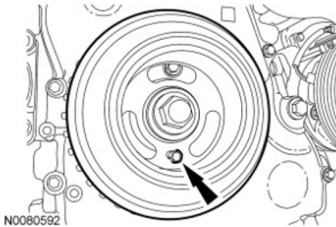
Fig. 40: View Of Crankshaft Pulley Alignment Bolt Courtesy of FORD MOTOR CO.
