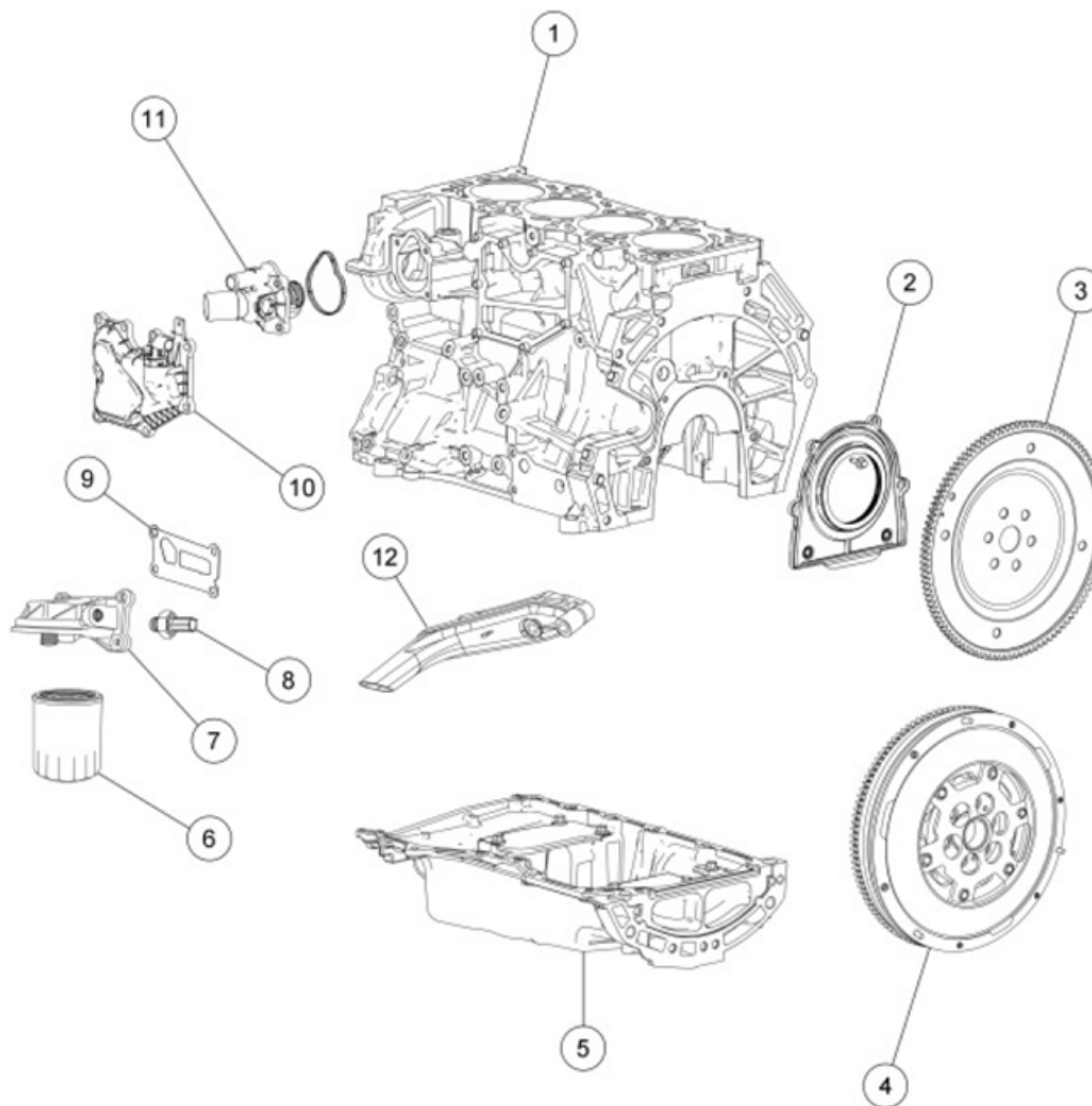
Fig. 369: Exploded View Of Lower Engine Block Components (View 1) Courtesy of FORD MOTOR CO.
