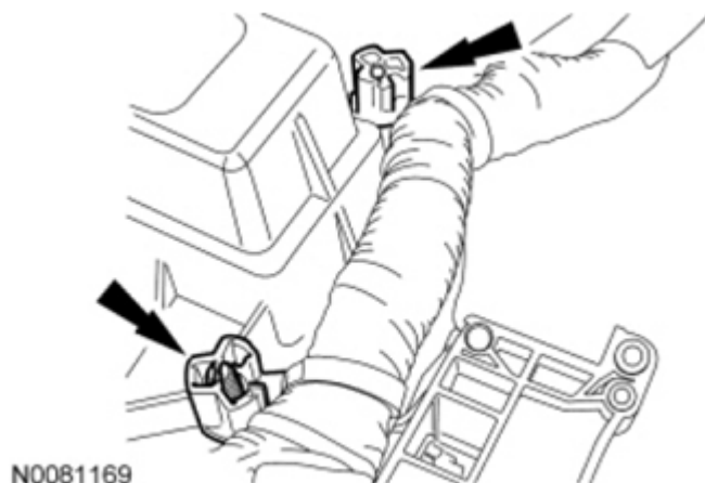
Fig. 300: Locating Wiring Harness Retainers Of LH Side Valve Cover Stud Bolts Courtesy of FORD MOTOR CO.
