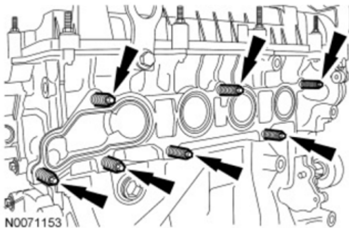
Fig. 286: View Of Exhaust Manifold Studs Courtesy of FORD MOTOR CO.
