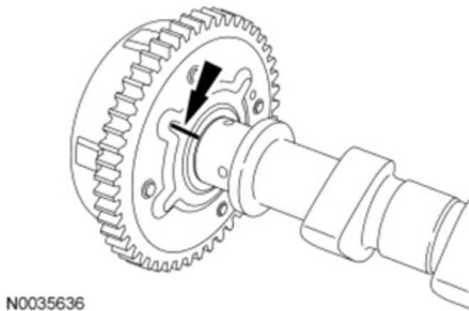
Fig. 98: View Of Sprocket And Camshaft Marking Courtesy of FORD MOTOR CO.
