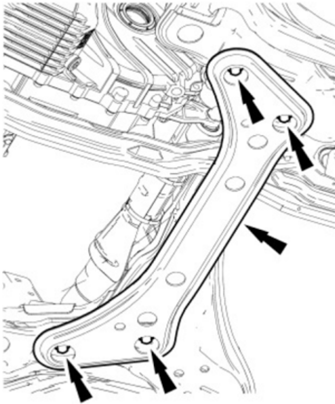
Fig. 591: Locating Lateral Support Crossmember Bolts Courtesy of FORD MOTOR CO.
