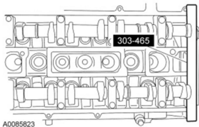
Fig. 85: View Of Camshaft Alignment Plate Courtesy of FORD MOTOR CO.
