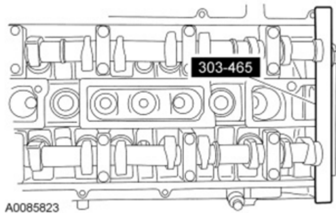
Fig. 436: View Of Camshaft Alignment Plate Courtesy of FORD MOTOR CO.
