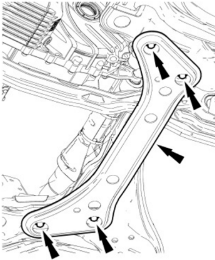
Fig. 552: Locating Lateral Support Crossmember Bolts Courtesy of FORD MOTOR CO.
