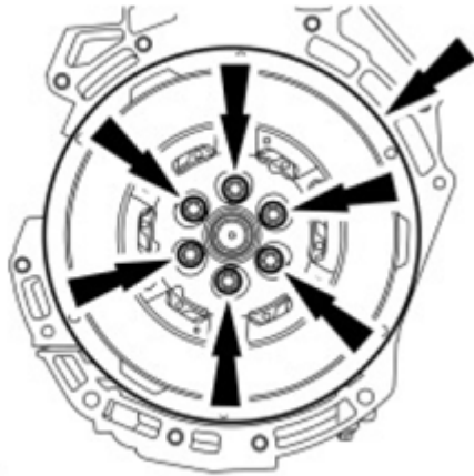
Fig. 277: Locating Flywheel Bolts Courtesy of FORD MOTOR CO.
