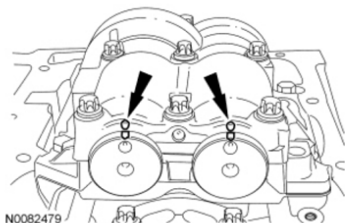
Fig. 8: Locating Balancer Unit Marks Courtesy of FORD MOTOR CO.
