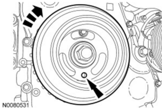
Fig. 84: Turning Crankshaft Pulley Courtesy of FORD MOTOR CO.
