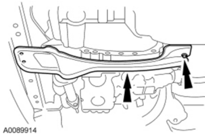
Fig. 520: Locating Engine Support Crossmember Rear Nut Courtesy of FORD MOTOR CO.
