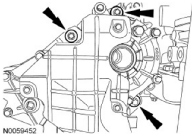
Fig. 502: Locating PTU And RH PTU Bolts Courtesy of FORD MOTOR CO.
