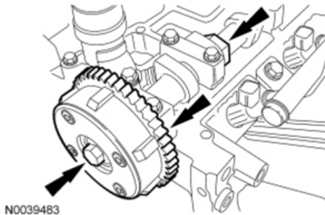
Fig. 338: View Of Camshaft Phaser And Sprocket Bolts Courtesy of FORD MOTOR CO.
