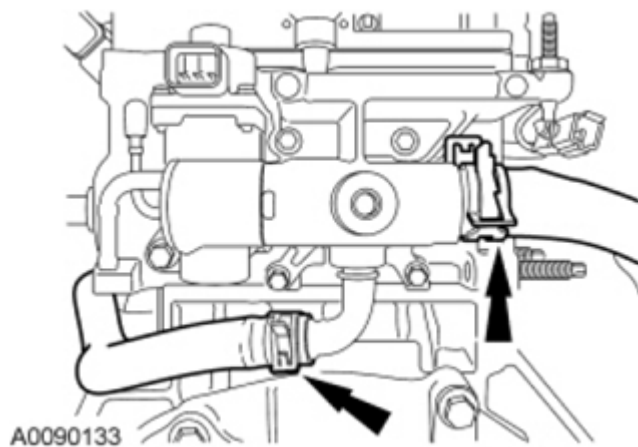
Fig. 317: Locating Coolant Hoses Courtesy of FORD MOTOR CO.
