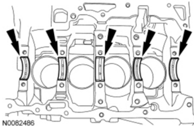
Fig. 383: View Of Main Bearings Of Cylinder Block Courtesy of FORD MOTOR CO.
