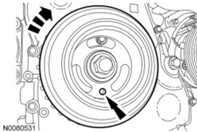
Fig. 27: Turning Crankshaft Pulley Courtesy of FORD MOTOR CO.
