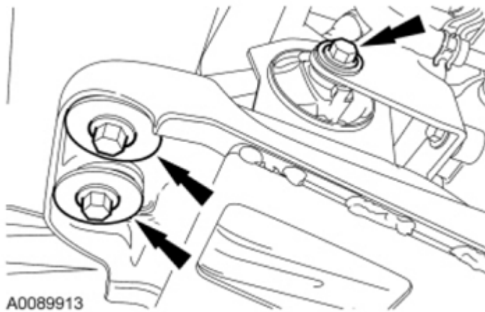
Fig. 521: Locating Front Roll Restrictor And Engine Support Crossmember Bolts Courtesy of FORD MOTOR CO.
