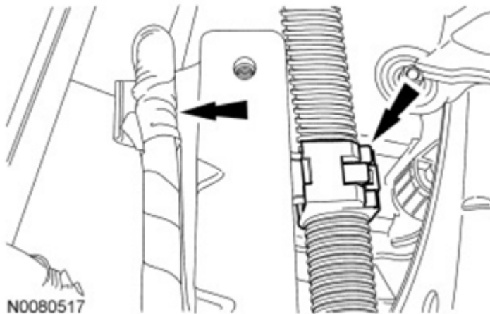
Fig. 197: Locating Battery Tray Bracket Wiring Harness Retainers Courtesy of FORD MOTOR CO.
