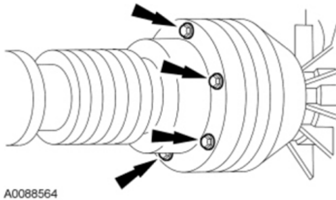
Fig. 548: Locating Driveshaft Bolts Courtesy of FORD MOTOR CO.
