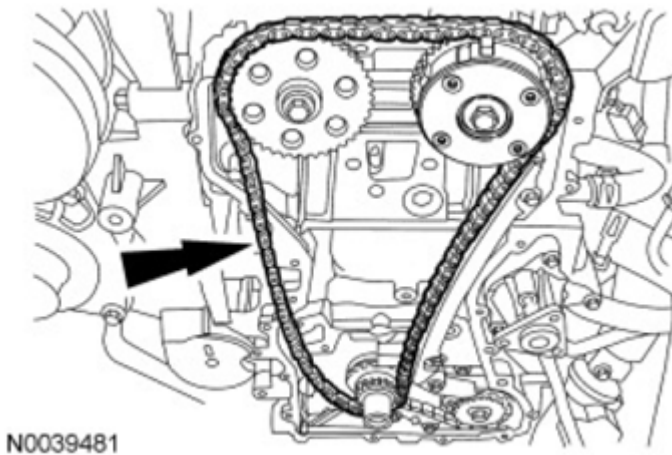
Fig. 69: View Of Timing Chain Courtesy of FORD MOTOR CO.
