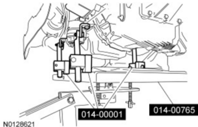
Fig. 267: Securing Engine And Transaxle Onto Powertrain Lift Courtesy of FORD MOTOR CO.
