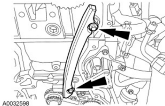
Fig. 74: Locating LH Timing Chain Guide Bolts Courtesy of FORD MOTOR CO.
