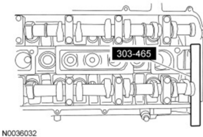
Fig. 118: View Of Camshaft Alignment Plate Courtesy of FORD MOTOR CO.
