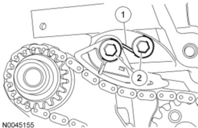
Fig. 170: Locating Oil Pump Drive Chain Tensioner And Shoulder Bolts Courtesy of FORD MOTOR CO.
