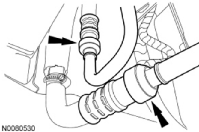
Fig. 542: Locating Transaxle Fluid Cooler Tubes Courtesy of FORD MOTOR CO.
