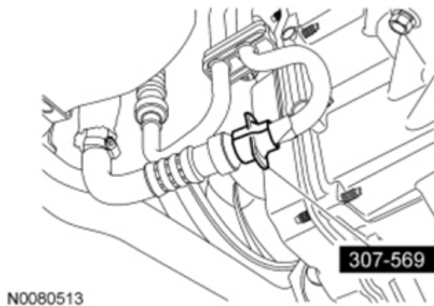
Fig. 192: Disconnecting Transaxle Fluid Cooler Tubes Courtesy of FORD MOTOR CO.
