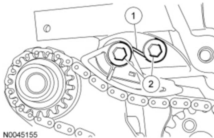
Fig. 339: Locating Oil Pump Drive Chain Tensioner And Shoulder Bolts Courtesy of FORD MOTOR CO.
