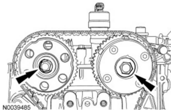
Fig. 82: View Of Camshaft Bolts Courtesy of FORD MOTOR CO.
