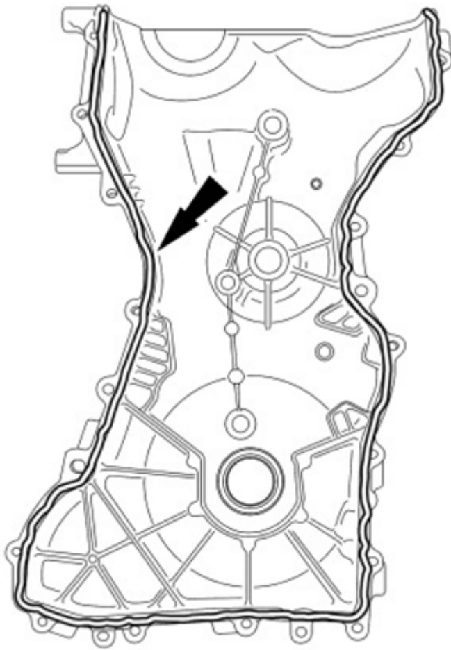
Fig. 59: Locating Silicone And Sealant Applying Areas Of Cylinder Head And Oil Pan Joint Courtesy of FORD MOTOR CO.
