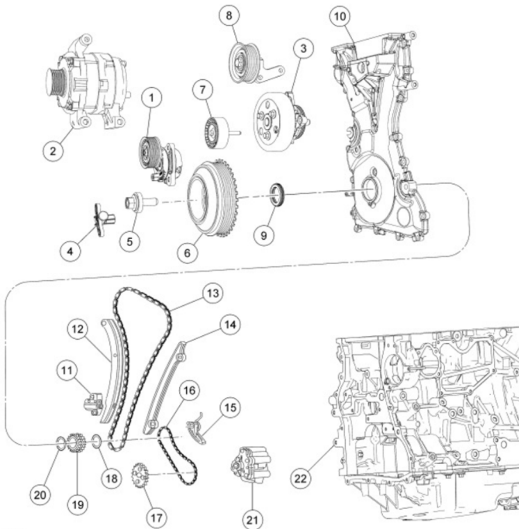
Fig. 371: Exploded View Of Front Engine Block Components Courtesy of FORD MOTOR CO.
