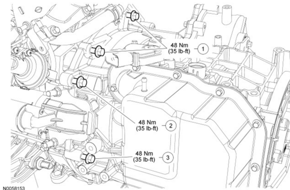
Fig. 156: Exploded View Of Engine Lubrication Components With Torque Specifications - (2 Of 5) Courtesy of FORD MOTOR CO.
