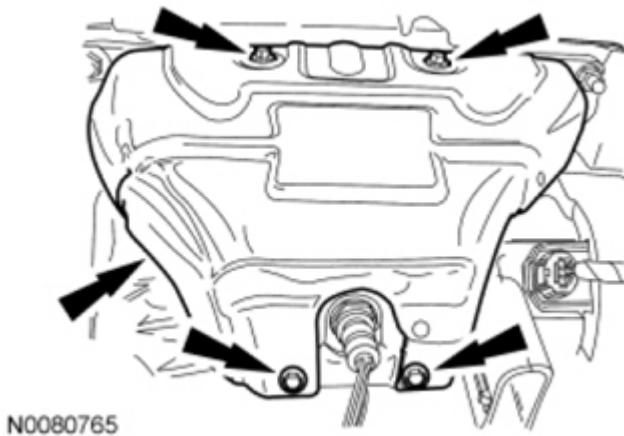
Fig. 488: Locating Exhaust Manifold Heat Shield With Bolts Courtesy of FORD MOTOR CO.
