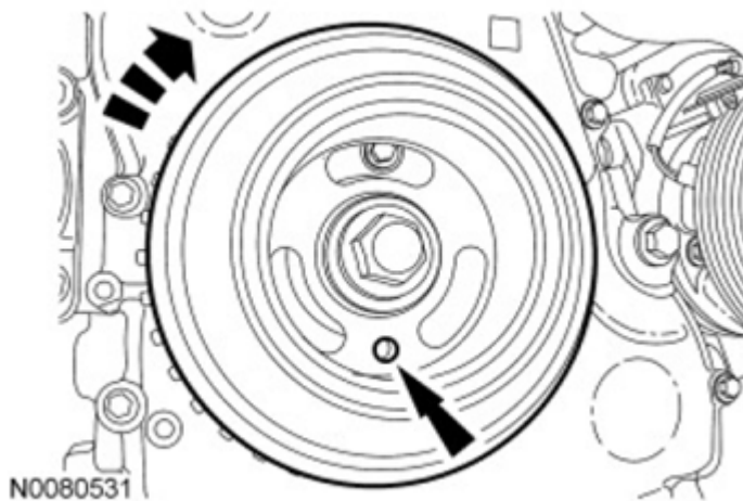
Fig. 111: Turning Crankshaft Pulley Courtesy of FORD MOTOR CO.
