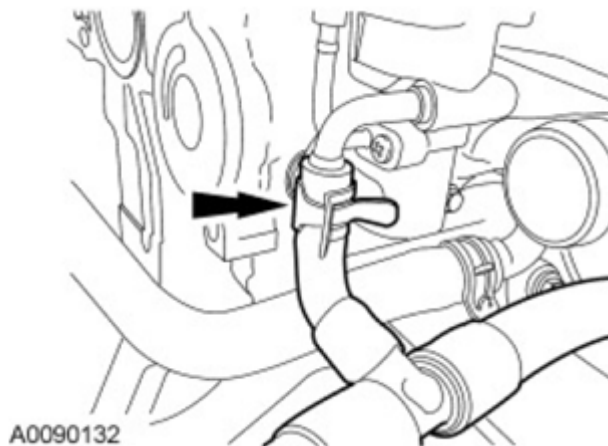
Fig. 316: Locating Coolant Hose Courtesy of FORD MOTOR CO.
