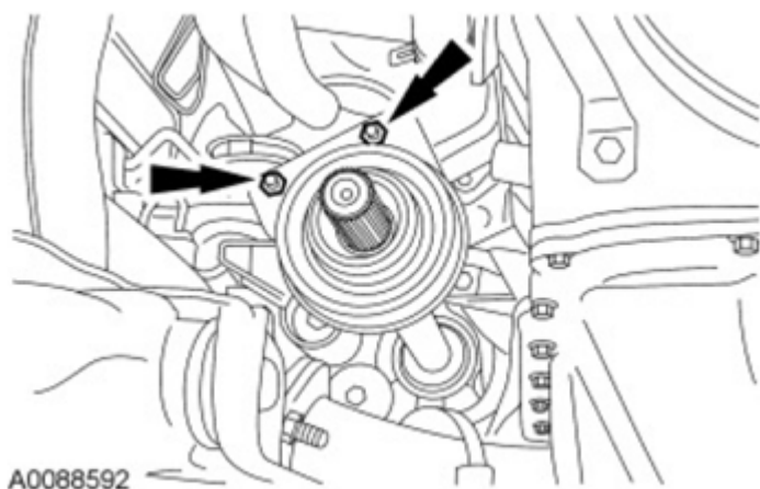
Fig. 551: Locating Intermediate Shaft Bearing Retainer Nuts Courtesy of FORD MOTOR CO.
