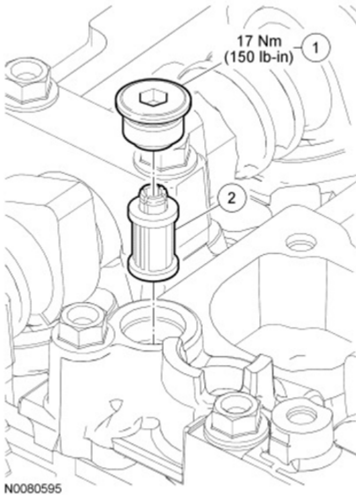
Fig. 83: Identifying Variable Camshaft Timing (VCT) System Oil Filter Components With Torque Specifications Courtesy of FORD MOTOR CO.
