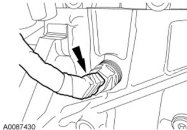
Fig. 201: Locating Block Heater Electrical Connector Courtesy of FORD MOTOR CO.
