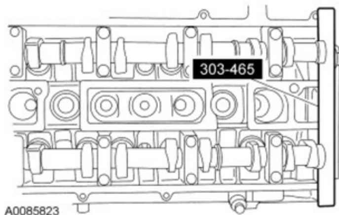
Fig. 326: View Of Camshaft Alignment Plate Courtesy of FORD MOTOR CO.
