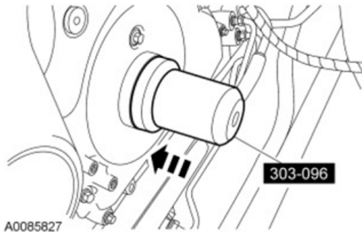
Fig. 61: Installing Crankshaft Front Oil Seal Using Camshaft Front Oil Seal Installer Courtesy of FORD MOTOR CO.
