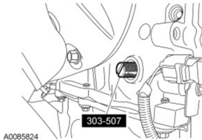
Fig. 36: View Of Crankshaft TDC Timing Peg Courtesy of FORD MOTOR CO.
