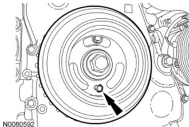
Fig. 88: View Of Crankshaft Pulley Alignment Bolt Courtesy of FORD MOTOR CO.
