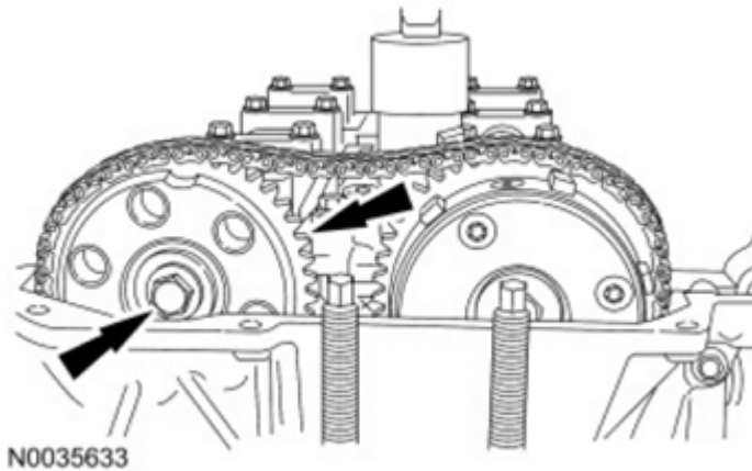
Fig. 103: Locating Exhaust Camshaft Bolt Courtesy of FORD MOTOR CO.
