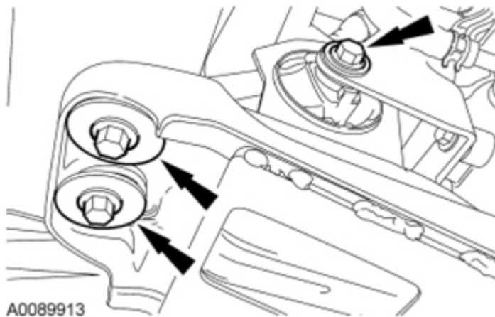
Fig. 213: Locating Front Roll Restrictor And Engine Support Crossmember Bolts Courtesy of FORD MOTOR CO.
