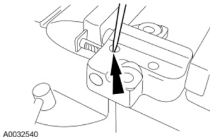
Fig. 78: Pushing Ratchet Mechanism Courtesy of FORD MOTOR CO.
