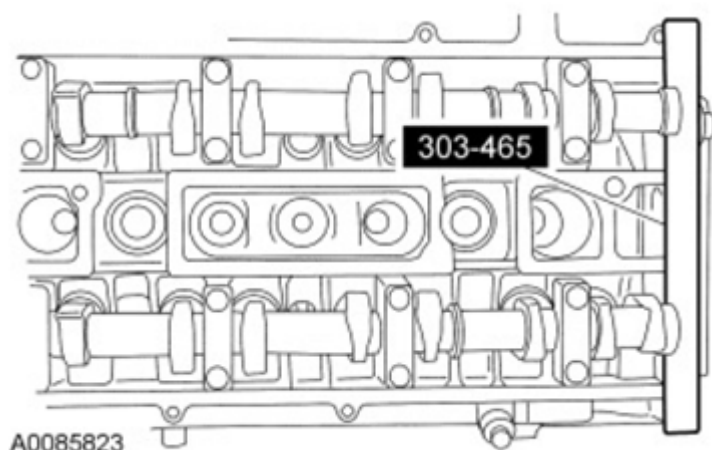
Fig. 147: View Of Camshaft Alignment Plate Courtesy of FORD MOTOR CO.
