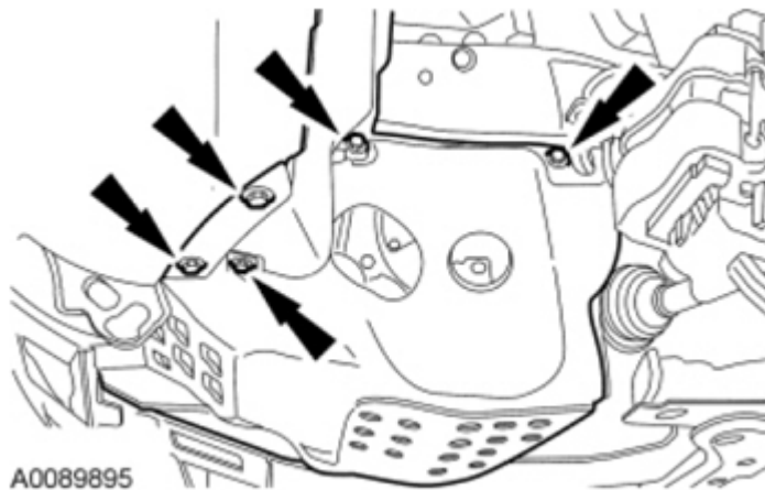
Fig. 169: Locating LH Splash Shield Retainers Courtesy of FORD MOTOR CO.
