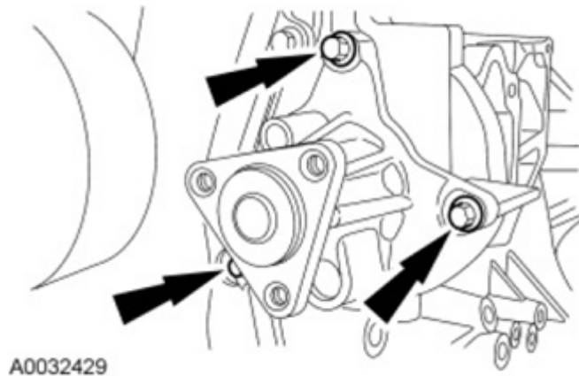
Fig. 291: Locating Coolant Pump Bolts Courtesy of FORD MOTOR CO.
