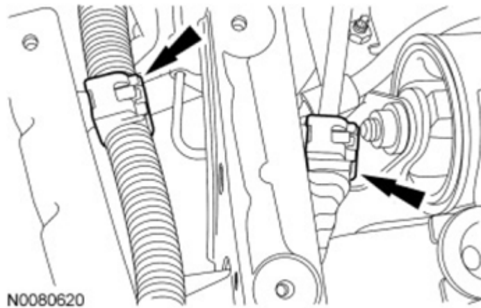
Fig. 584: Locating Wiring Harness Retainers Of Battery Tray Bracket Courtesy of FORD MOTOR CO.
