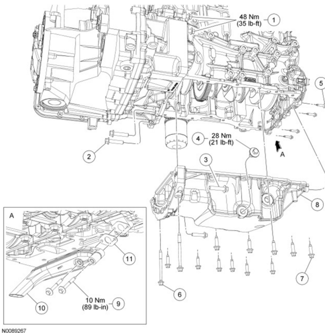
Fig. 158: Exploded View Of Engine Lubrication Components With Torque Specifications - (4 Of 5) Courtesy of FORD MOTOR CO.
