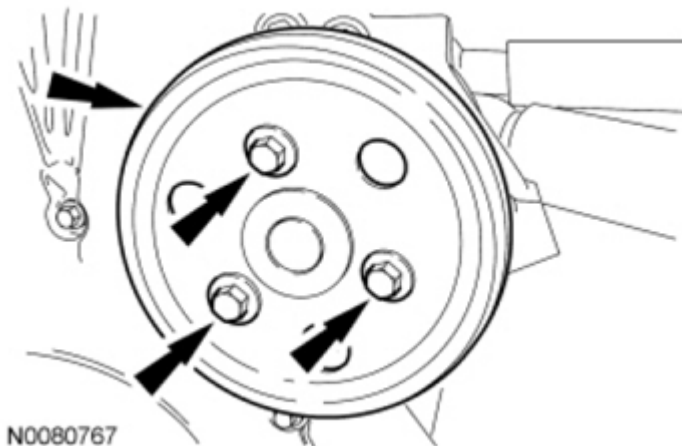
Fig. 290: Locating Coolant Pump Pulley And Bolts Courtesy of FORD MOTOR CO.
