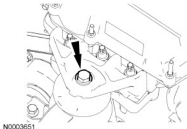
Fig. 561: Locating Engine Mount Bracket Bolt Courtesy of FORD MOTOR CO.
