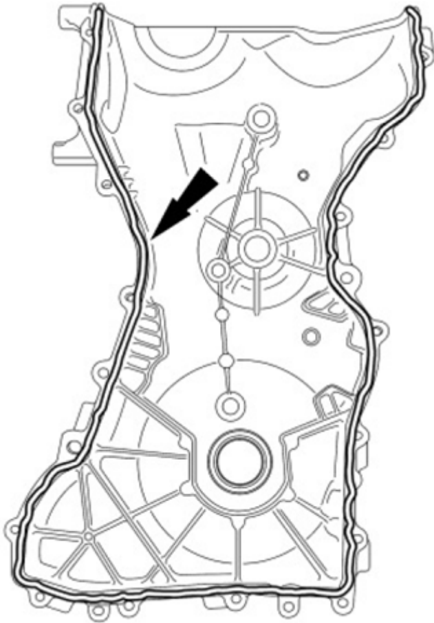
Fig. 428: Locating Silicone And Sealant Applying Areas Of Cylinder Head And Oil Pan Joint Courtesy of FORD MOTOR CO.
