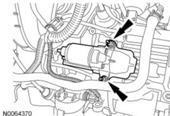
Fig. 229: Locating Starter Motor Stud Bolts Courtesy of FORD MOTOR CO.
