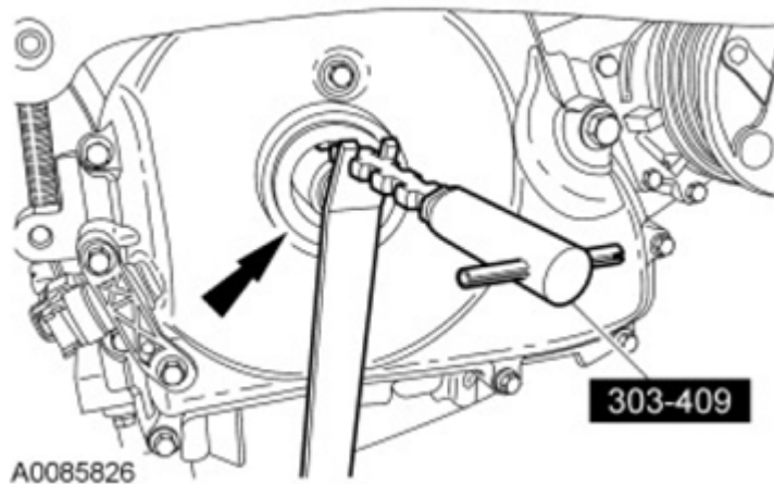
Fig. 46: Removing Crankshaft Front Oil Seal Using Oil Seal Remover Courtesy of FORD MOTOR CO.
