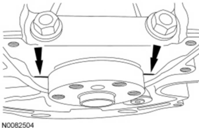
Fig. 376: Locating Main Bearing Beams Courtesy of FORD MOTOR CO.
