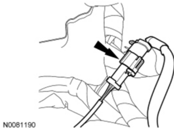
Fig. 283: Locating Heated Oxygen Sensor (HO2S) Electrical Connector Courtesy of FORD MOTOR CO.
