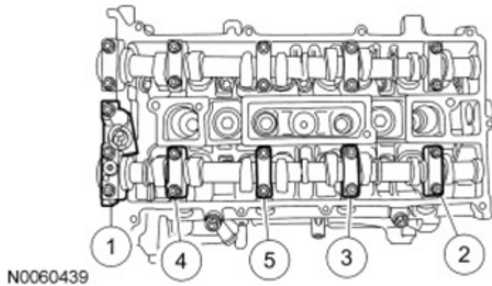
Fig. 124: Removing Order Of Intake Camshaft Bearing Cap Bolts Courtesy of FORD MOTOR CO.
