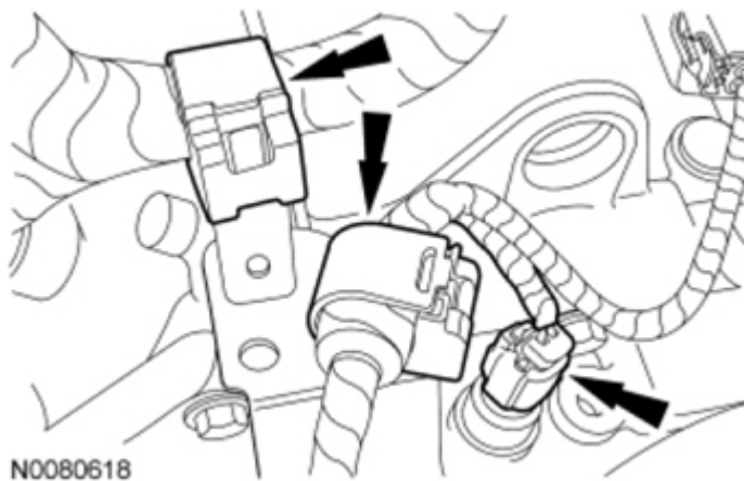
Fig. 247: Locating Reversing Lamp Indicator Switch Electrical Connector And Wiring Harness Retainers Courtesy of FORD MOTOR CO.
