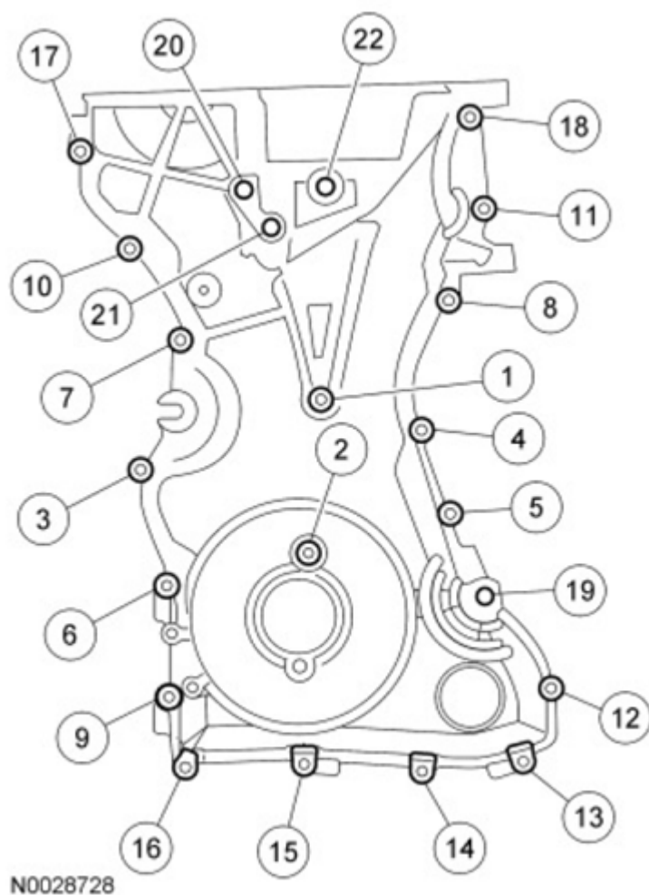
Fig. 60: Tightening Sequence Of Engine Front Cover Bolts Courtesy of FORD MOTOR CO.
