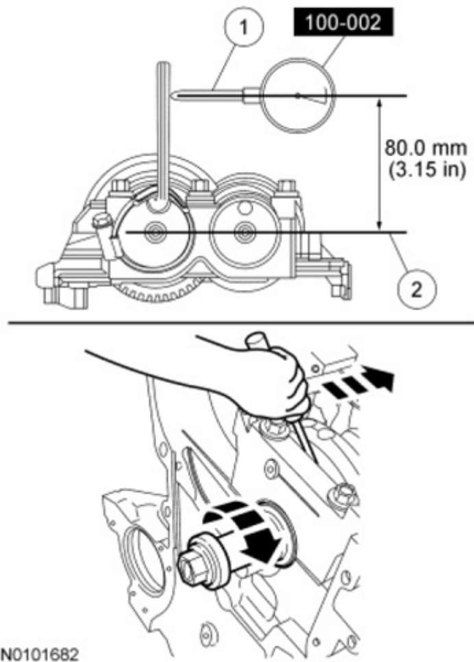
Fig. 12: Measuring Gear Backlash With Specifications Courtesy of FORD MOTOR CO.
