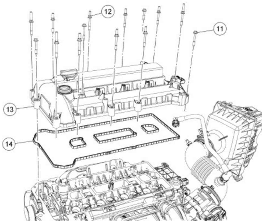
Fig. 23: Identifying Valve Cover Components - (2 Of 2)
