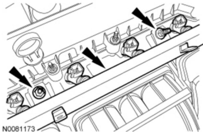
Fig. 311: Locating Fuel Injector With Stud Bolts Courtesy of FORD MOTOR CO.
