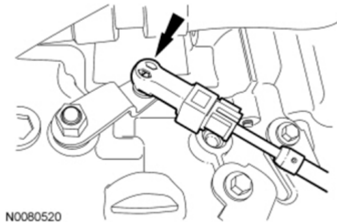
Fig. 536: View Of Shift Cable Of Transaxle Manual Lever Courtesy of FORD MOTOR CO.
