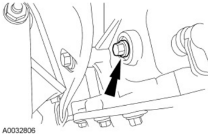
Fig. 110: Remove/Install Engine Plug Bolt Courtesy of FORD MOTOR CO.
