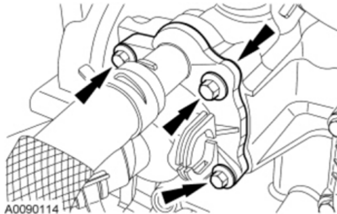
Fig. 292: Locating Thermostat Housing And Bolts Courtesy of FORD MOTOR CO.
