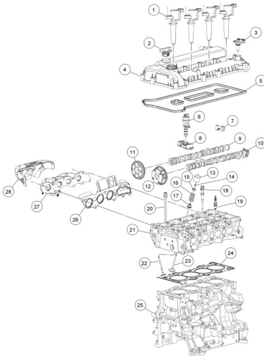
Fig. 372: Exploded View Of Cylinder Head Components Courtesy of FORD MOTOR CO.
