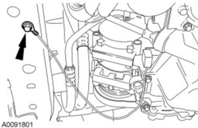
Fig. 547: Locating Ground Eyelet Bolts Courtesy of FORD MOTOR CO.
