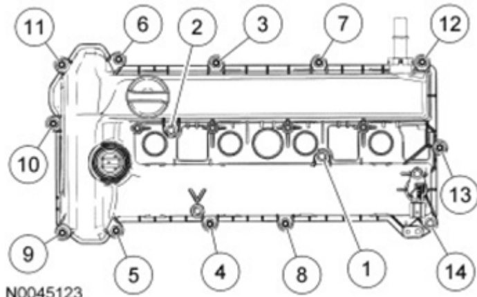
Fig. 448: Tightening Sequence Of Valve Cover Bolts Courtesy of FORD MOTOR CO.
