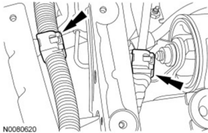
Fig. 244: Locating Wiring Harness Retainers Of Battery Tray Bracket Courtesy of FORD MOTOR CO.
