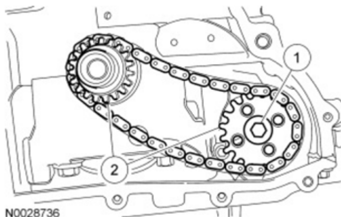
Fig. 340: Locating Oil Pump Chain And Sprockets Courtesy of FORD MOTOR CO.
