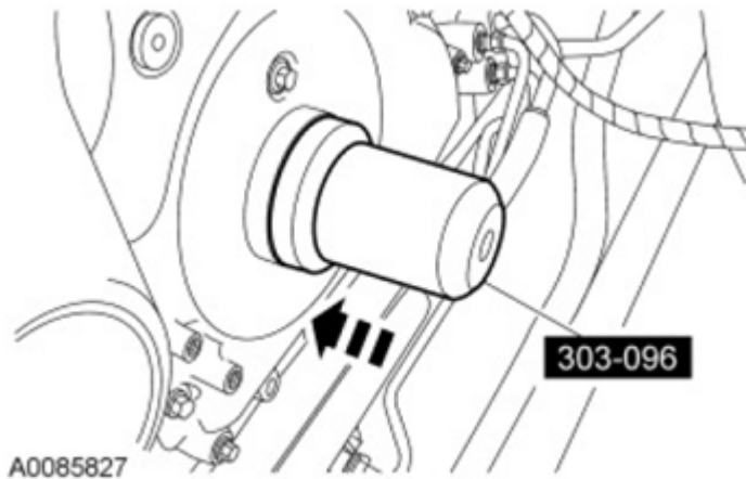
Fig. 430: Installing Crankshaft Front Oil Seal Using Camshaft Front Oil Seal Installer Courtesy of FORD MOTOR CO.
