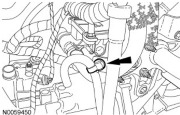
Fig. 504: Locating PTU Vent Hose Retainer Courtesy of FORD MOTOR CO.
