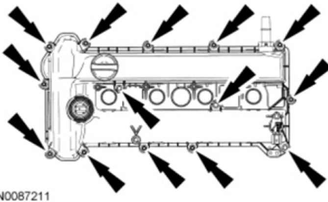
Fig. 323: Locating Valve Cover Retainers Courtesy of FORD MOTOR CO.
