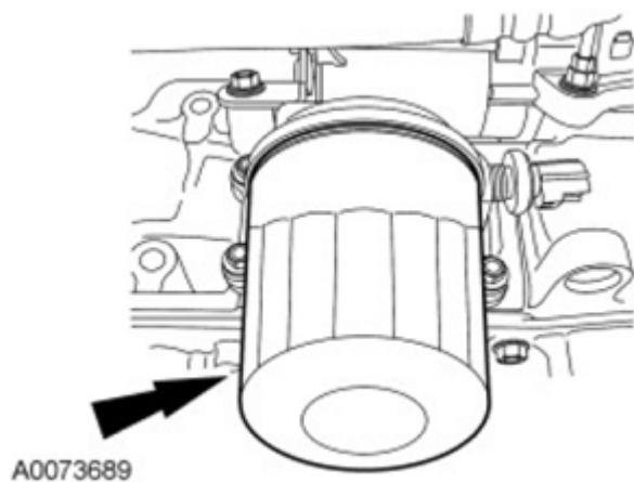
Fig. 562: Locating Engine Oil Filter Courtesy of FORD MOTOR CO.
