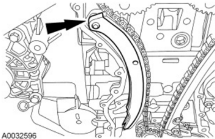
Fig. 76: Locating RH Timing Chain Guide Courtesy of FORD MOTOR CO.
