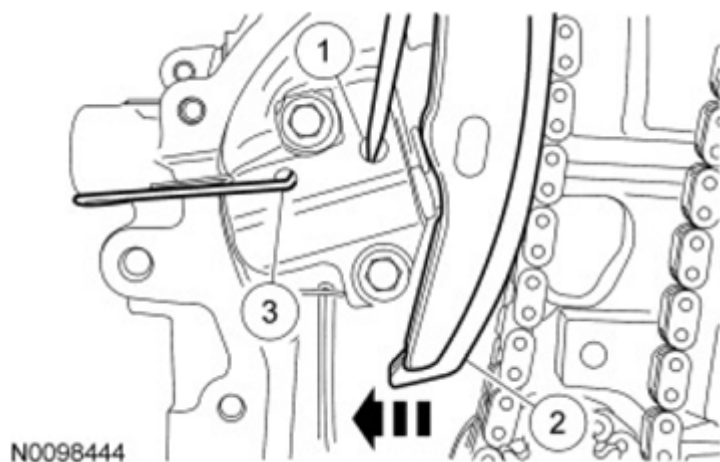
Fig. 66: Pushing Timing Chain Arm Courtesy of FORD MOTOR CO.
