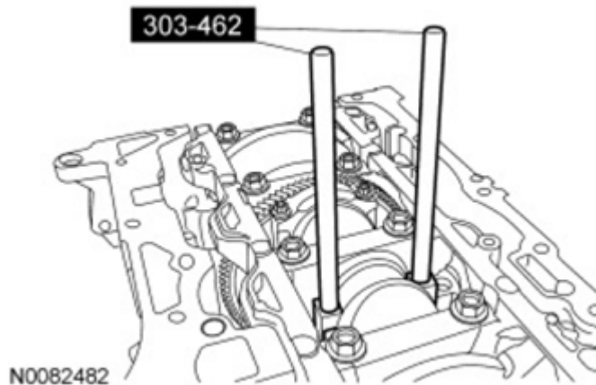
Fig. 356: Removing Piston/Rod Assembly Of Engine Block Courtesy of FORD MOTOR CO.
