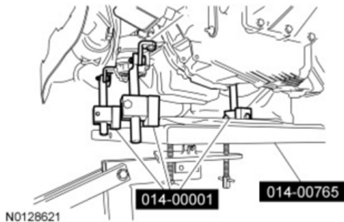
Fig. 553: Securing Engine And Transaxle Onto Powertrain Lift Courtesy of FORD MOTOR CO.
