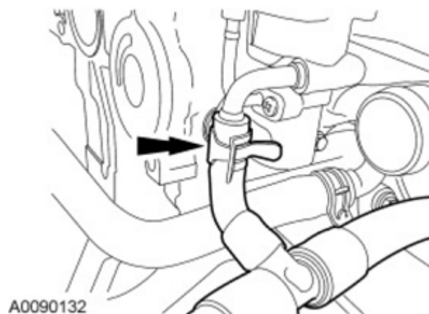
Fig. 455: Locating Coolant Hose Courtesy of FORD MOTOR CO.
