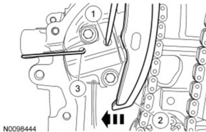
Fig. 332: Pushing Timing Chain Arm Courtesy of FORD MOTOR CO.
