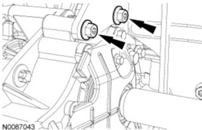
Fig. 164: Locating RH Engine Bracket-To-Power Transfer Unit (PTU) Bolts Courtesy of FORD MOTOR CO.
