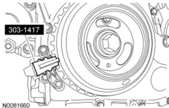
Fig. 443: Adjusting CKP Sensor Using Crankshaft Sensor Aligner Courtesy of FORD MOTOR CO.
