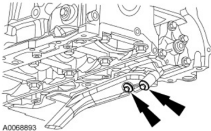
Fig. 400: Remove/Install Oil Pump Pickup Tube Bolts Courtesy of FORD MOTOR CO.
