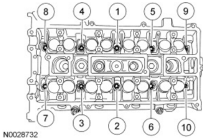
Fig. 409: Tightening Sequence Of Cylinder Head Bolts Courtesy of FORD MOTOR CO.
