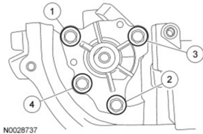
Fig. 171: Tightening Sequence Of Oil Pump Assembly Bolts Courtesy of FORD MOTOR CO.
