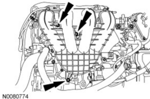
Fig. 459: Remove/Install Intake Manifold Bolts Courtesy of FORD MOTOR CO.
