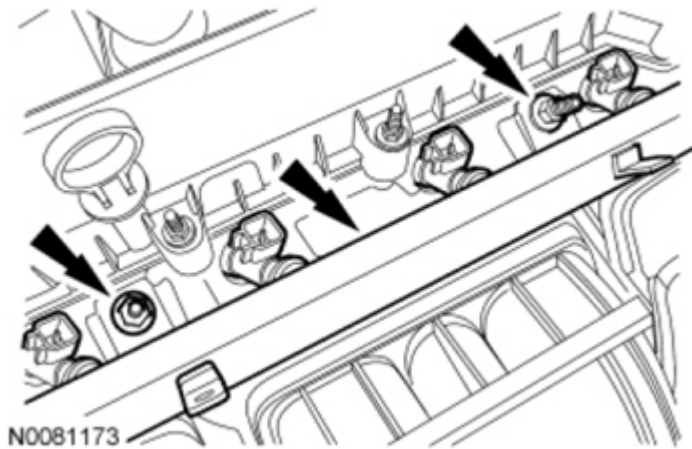
Fig. 461: Locating Fuel Injector Assembly Courtesy of FORD MOTOR CO.
