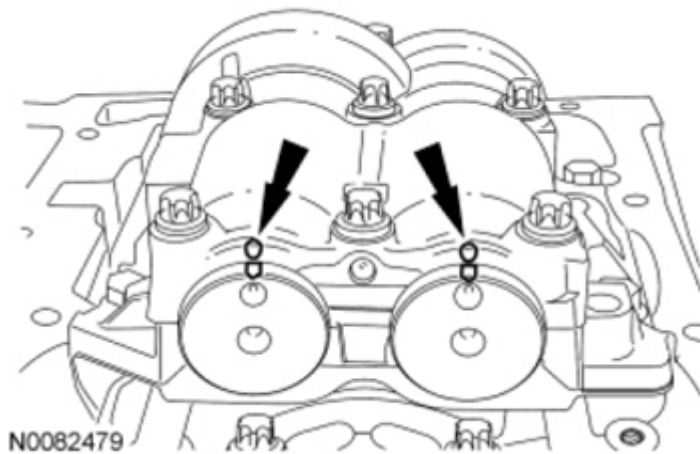
Fig. 15: Locating Balancer Unit Marks Courtesy of FORD MOTOR CO.
