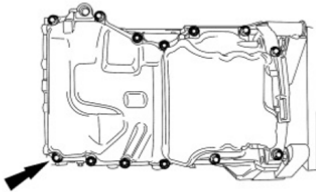
Fig. 347: Locating Oil Pan Bolt Courtesy of FORD MOTOR CO.
