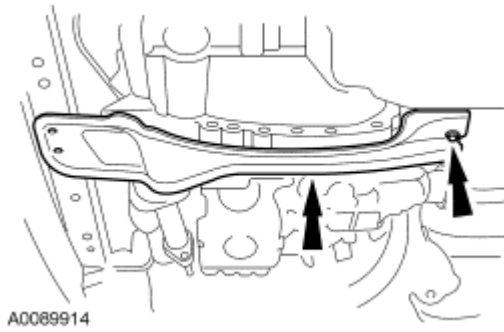
Fig. 416: Identifying Cross Brace And Rear Nut Courtesy of FORD MOTOR CO.
