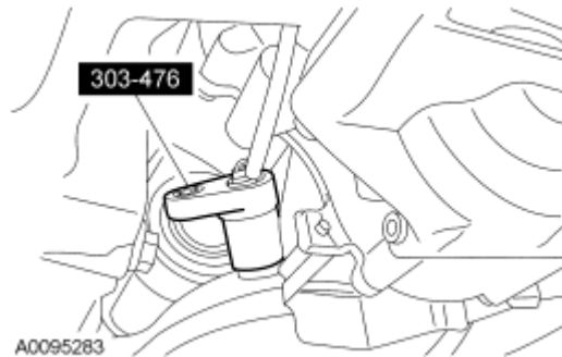
Fig. 217: Identifying Special Oxygen Sensor Tool Courtesy of FORD MOTOR CO.
