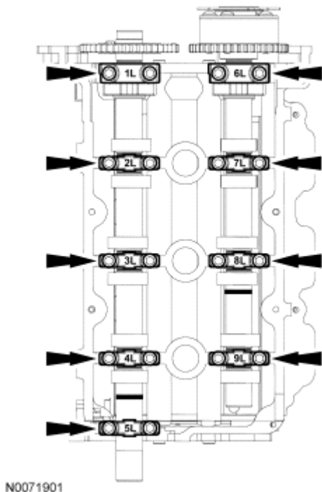
Fig. 255: Identifying Bearing Cap Position And Orientation Marks
