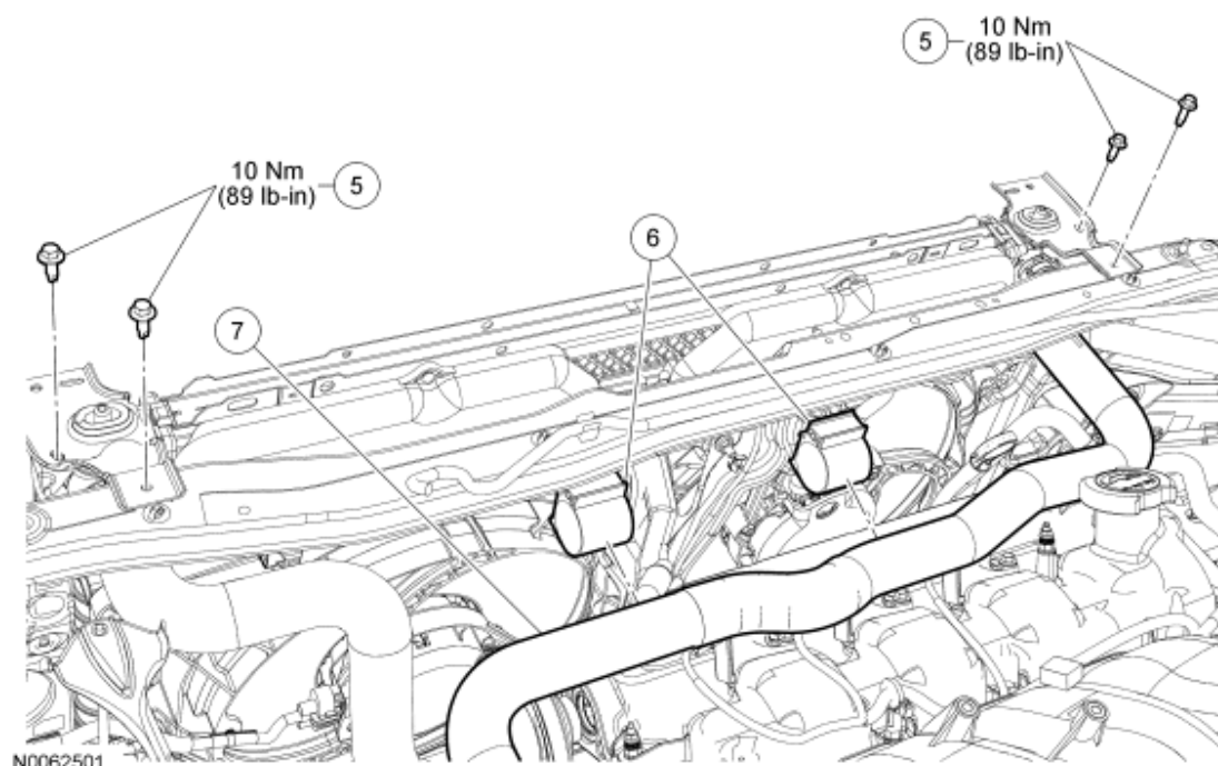
Fig. 104: Radiator Hose With Torque Specifications
