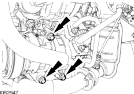
Fig. 420: Identifying Bolts Courtesy of FORD MOTOR CO.
