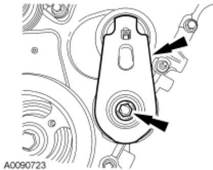
Fig. 304: Locating Belt Tensioner & Bolt Courtesy of FORD MOTOR CO.
