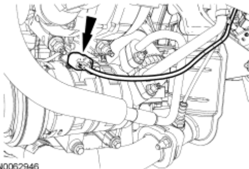
Fig. 421: Identifying Connector Courtesy of FORD MOTOR CO.
