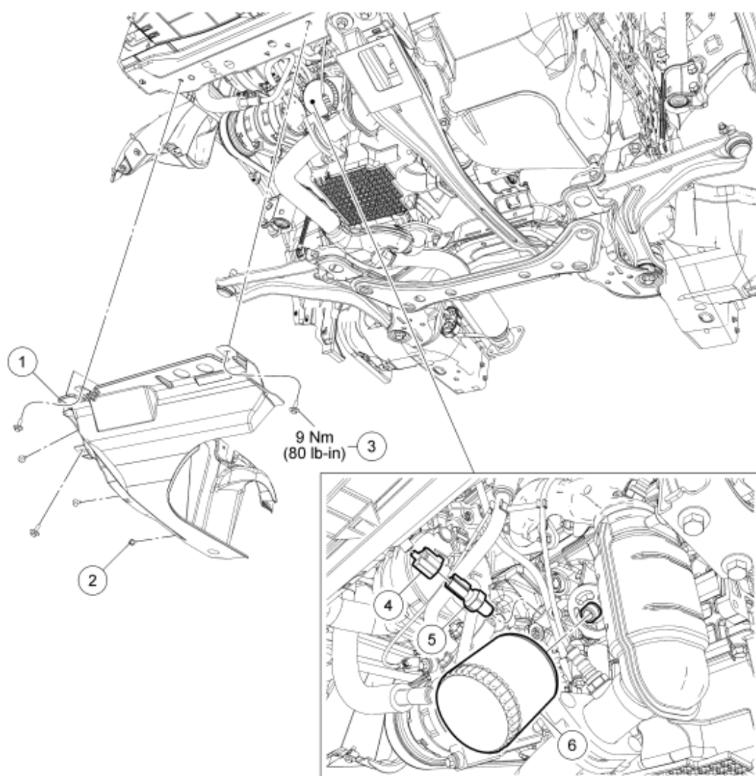
Fig. 102: Engine Oil Pressure (EOP) Switch With Torque Specification Courtesy of FORD MOTOR CO.
