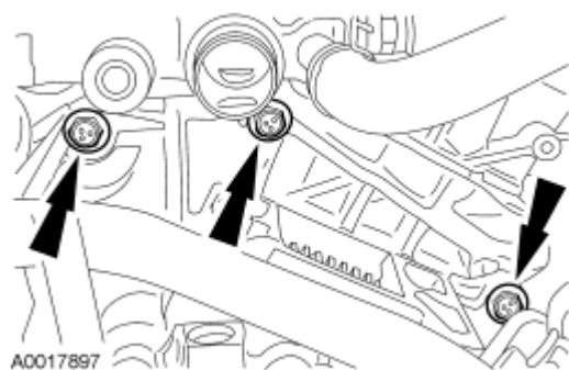
Fig. 182: Locating Transaxle-To-Engine Bolts Courtesy of FORD MOTOR CO.
