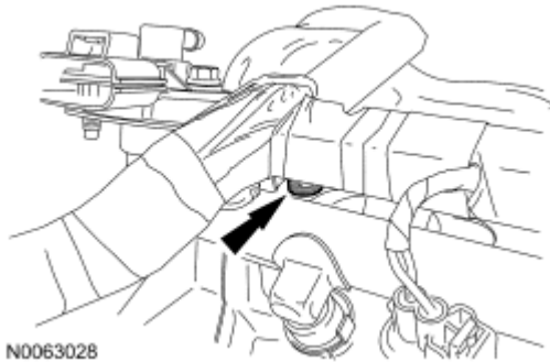
Fig. 337: Identifying Retainer Courtesy of FORD MOTOR CO.
