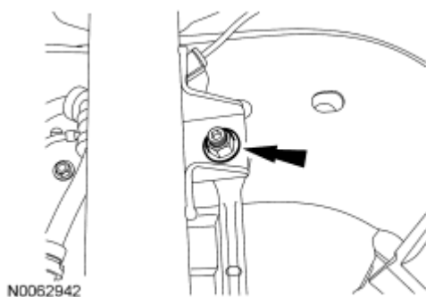
Fig. 429: Identifying Nut
