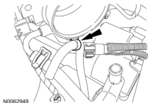
Fig. 136: Identifying Retainer Courtesy of FORD MOTOR CO.
