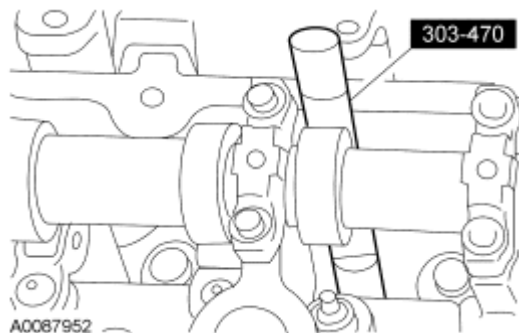
Fig. 84: Installing Valve Seal Courtesy of FORD MOTOR CO.
