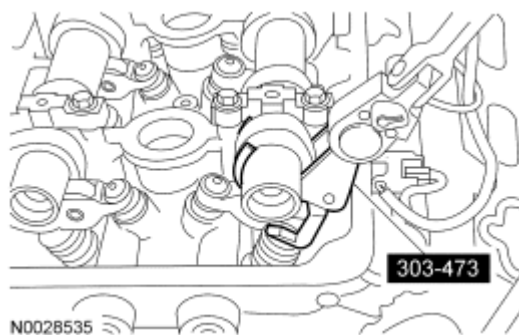
Fig. 81: Removing Roller Using Special Tool (303-473) Courtesy of FORD MOTOR CO.
