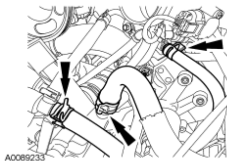
Fig. 135: Locating Heater Hoses & Throttle Body Coolant Hose Courtesy of FORD MOTOR CO.
