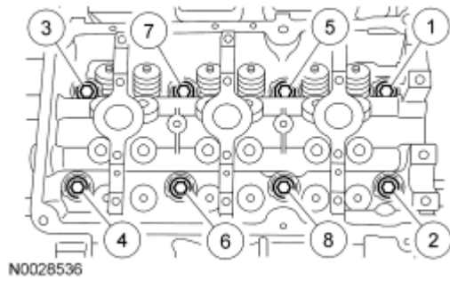
Fig. 87: Identifying Removing Sequence Of Cylinder Head Bolts Courtesy of FORD MOTOR CO.
