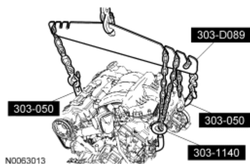
Fig. 181: Identifying Special Tools Courtesy of FORD MOTOR CO.
