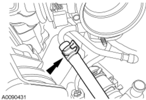
Fig. 347: Locating Throttle Body Coolant Hose Courtesy of FORD MOTOR CO.
