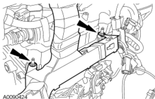
Fig. 191: Locating Engine Control Wiring Harness & Nuts Courtesy of FORD MOTOR CO.
