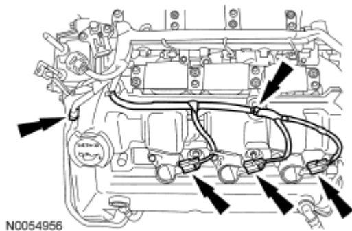
Fig. 200: Coil-On-Plug Electrical Connectors & Wiring Retainers Courtesy of FORD MOTOR CO.
