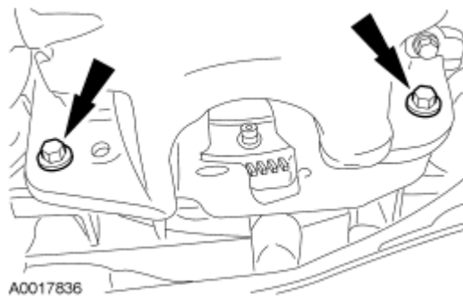
Fig. 385: Locating Oil Pan-To-Transaxle Bolts Courtesy of FORD MOTOR CO.
