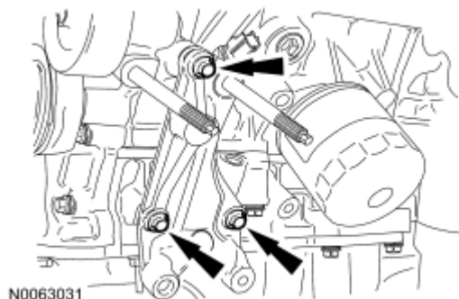
Fig. 214: Identifying Bolts Courtesy of FORD MOTOR CO.
