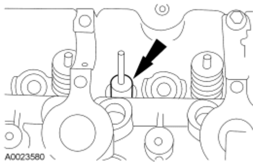
Fig. 83: Locating Valve Seal Courtesy of FORD MOTOR CO.
