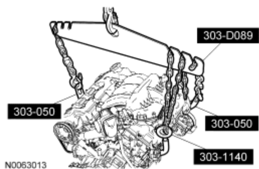
Fig. 360: Identifying Special Tools Courtesy of FORD MOTOR CO.
