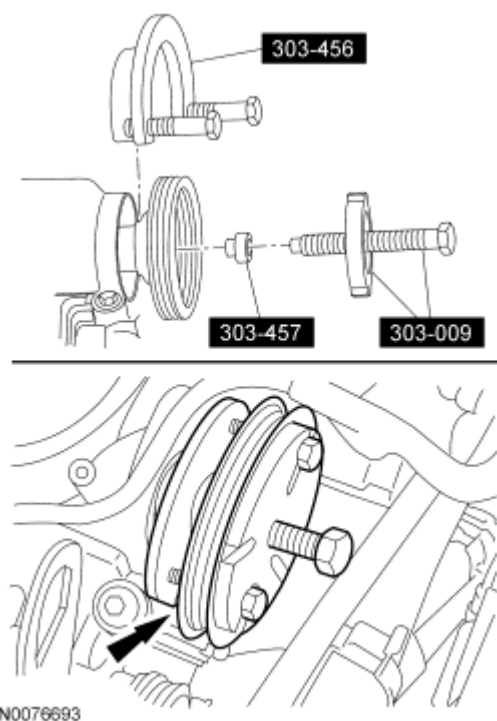
Fig. 64: Removing Coolant Pump Pulley Using Special Tools (303-009, 303-456, 303-457) Courtesy of FORD MOTOR CO.
