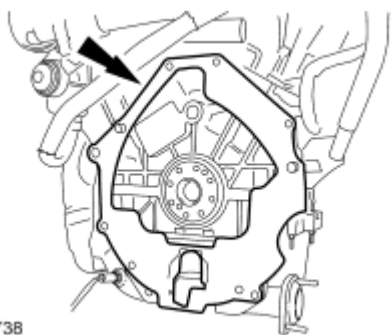
Fig. 358: Locating Engine-To-Transaxle Separator Plate Courtesy of FORD MOTOR CO.
