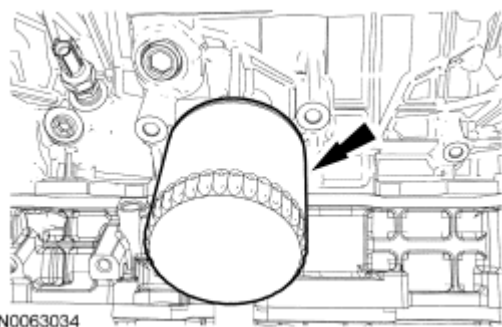
Fig. 321: Identifying Oil Filter Courtesy of FORD MOTOR CO.
