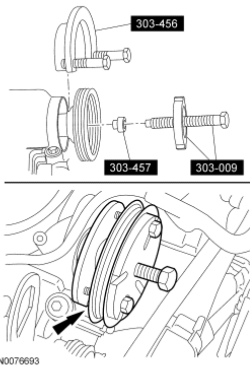
Fig. 222: Removing Coolant Pump Pulley Using Special Tools (303-009, 303-456, 303-457) Courtesy of FORD MOTOR CO.
