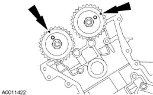
Fig. 292: Aligning Marks RH Camshafts Courtesy of FORD MOTOR CO.
