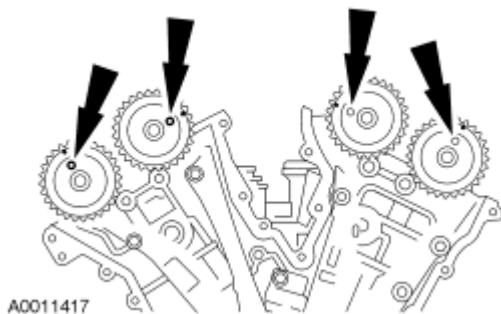
Fig. 274: Locating Camshafts Matching Marks Courtesy of FORD MOTOR CO.
