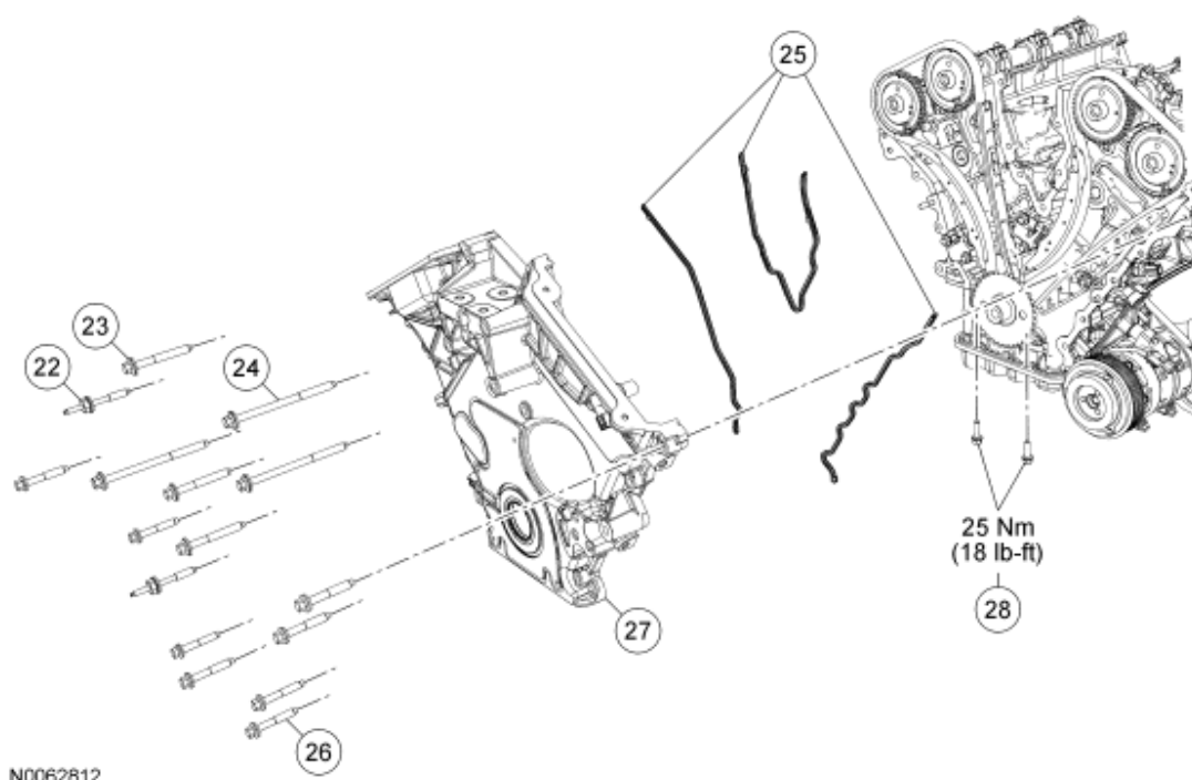
Fig. 28: Engine Front Cover Components With Torque Specification (4 Of 4) Courtesy of FORD MOTOR CO.
