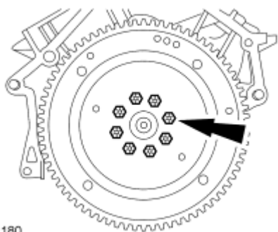
Fig. 359: Locating Flexplate & Bolts Courtesy of FORD MOTOR CO.
