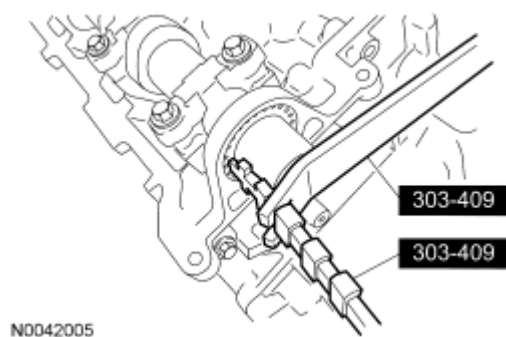
Fig. 65: Identifying Special Tools (303-409) Courtesy of FORD MOTOR CO.
