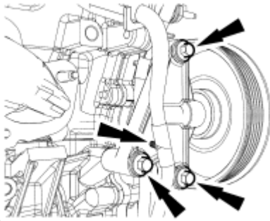
Fig. 419: Identifying Bolts Courtesy of FORD MOTOR CO.
