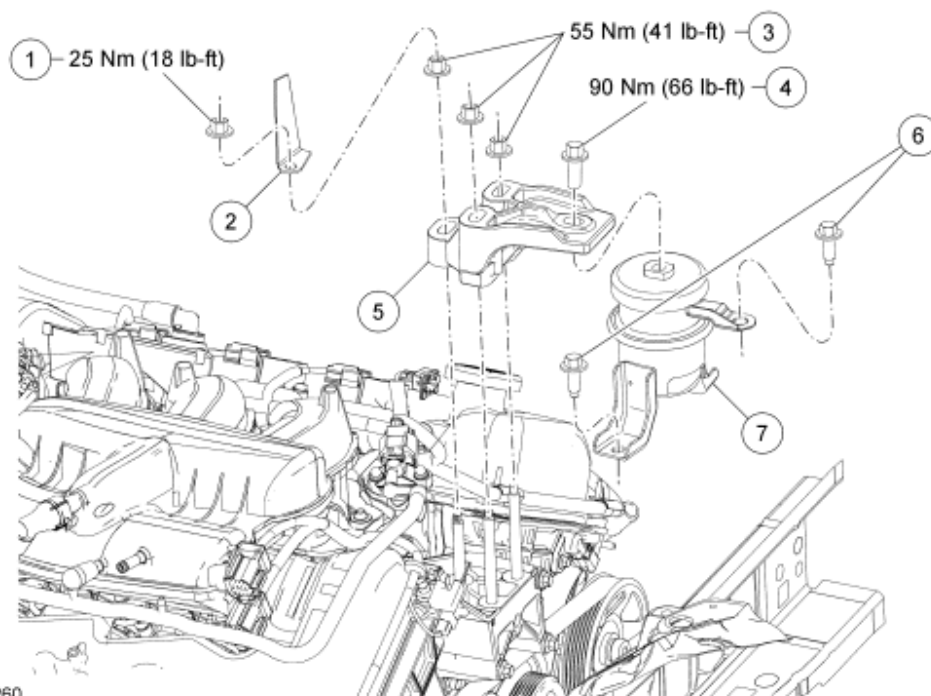
Fig. 99: Exploded View Of Engine Support Insulators (With Torque Specifications) Courtesy of FORD MOTOR CO.
