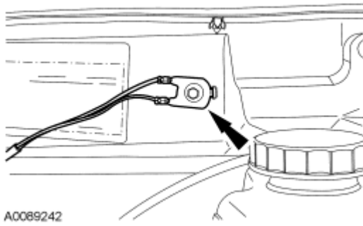
Fig. 353: Locating Ground Wire & Bolt Courtesy of FORD MOTOR CO.
