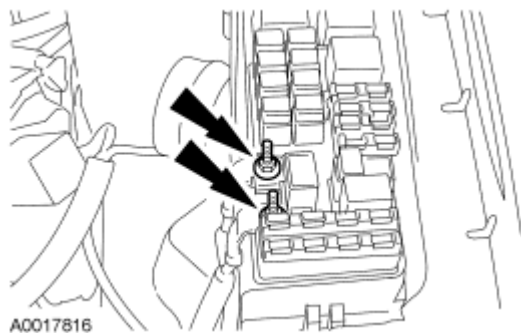
Fig. 351: Locating Cables & Nuts Courtesy of FORD MOTOR CO.
