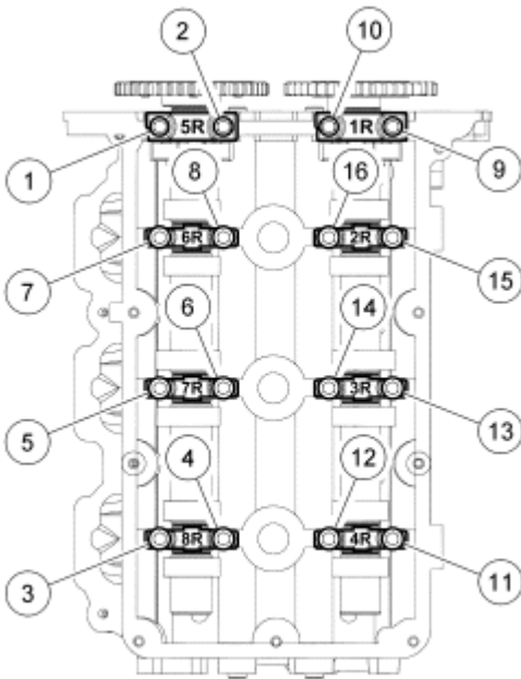
Fig. 76: Identifying Loosening Sequence Of Camshaft Bearing Bolts Courtesy of FORD MOTOR CO.
