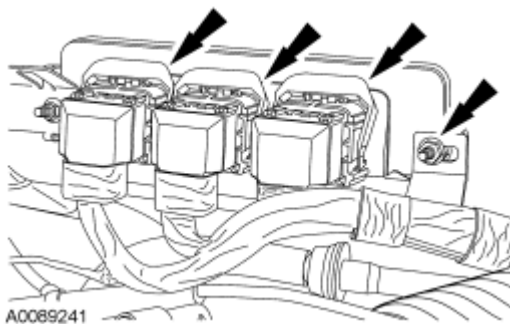
Fig. 128: Locating Powertrain Control Module (PCM) Electrical Connectors Courtesy of FORD MOTOR CO.
