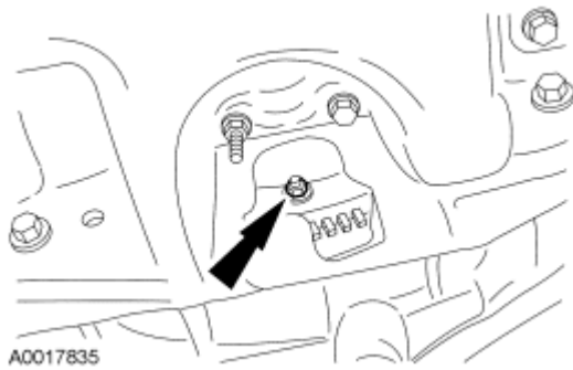
Fig. 139: Locating Torque Converter Nuts Courtesy of FORD MOTOR CO.
