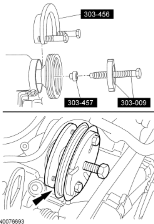
Fig. 220: Removing Coolant Pump Pulley Courtesy of FORD MOTOR CO.
