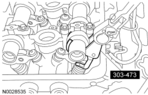
Fig. 79: Removing Roller Using Special Tool (303-473) Courtesy of FORD MOTOR CO.
