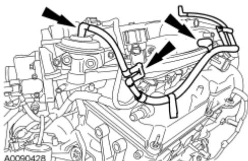
Fig. 312: Vacuum Tube Fittings At EGR Valve, EGR Vacuum Regulator & Intake Manifold Courtesy of FORD MOTOR CO.
