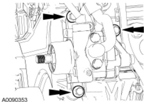
Fig. 372: Locating Power Steering Pump Bolts Courtesy of FORD MOTOR CO.
