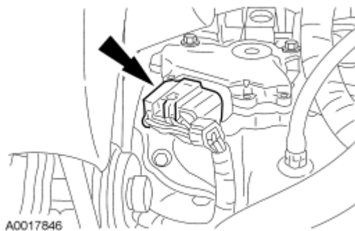
Fig. 147: Locating Transmission Range (TR) Sensor Electrical Connector Courtesy of FORD MOTOR CO.
