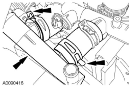
Fig. 192: Locating Coolant Tube Courtesy of FORD MOTOR CO.
