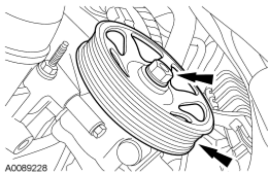
Fig. 373: Locating Power Steering Pump Pulley & Nut Courtesy of FORD MOTOR CO.
