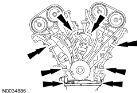
Fig. 28: Identifying Area For Applying Sealant Courtesy of FORD MOTOR CO.
