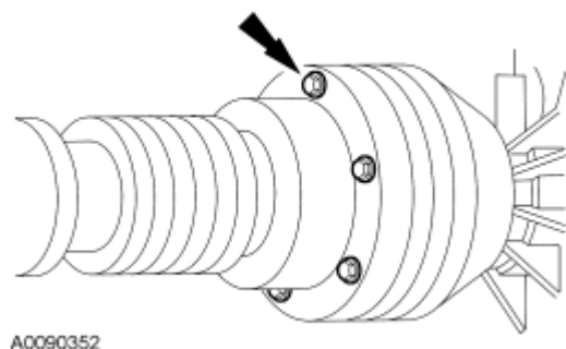
Fig. 377: Locating Driveshaft-To-Power Take Off Bolts & Washers Courtesy of FORD MOTOR CO.
