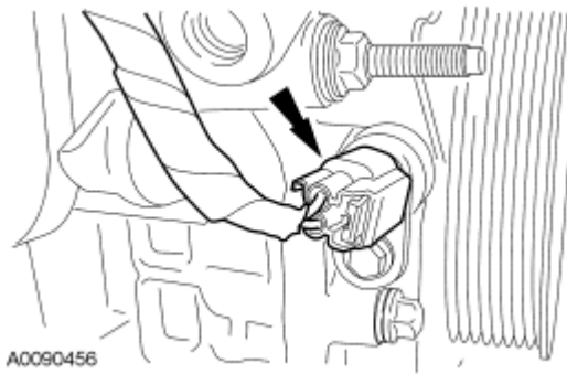
Fig. 304: Locating Crankshaft Position (CKP) Sensor Electrical Connector Courtesy of FORD MOTOR CO.
