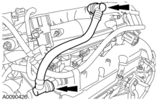
Fig. 165: Locating Positive Crankcase Ventilation (PCV) Tube Courtesy of FORD MOTOR CO.
