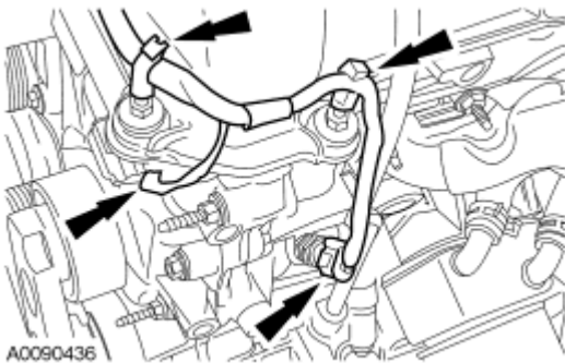
Fig. 305: Locating Camshaft Position Sensor (CMP) & Oil Pressure Sensor Electrical Connectors & Wiring Retainers Courtesy of FORD MOTOR CO.
