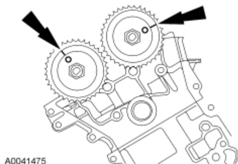
Fig. 212: Locating Camshafts Align Marks Courtesy of FORD MOTOR CO.
