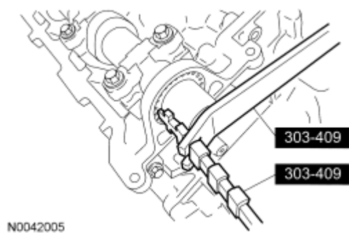
Fig. 63: Identifying Special Tools (303-409) Courtesy of FORD MOTOR CO.
