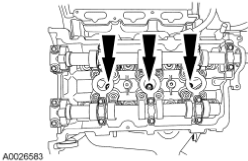
Fig. 59: Locating Spark Plugs Courtesy of FORD MOTOR CO.
