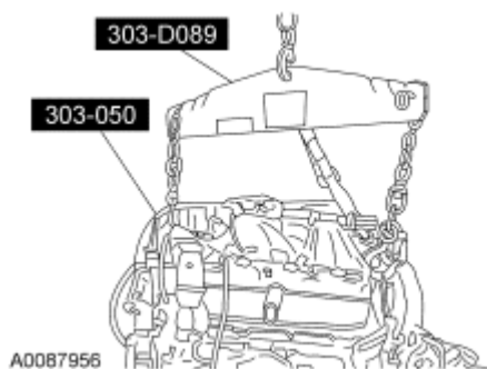
Fig. 320: Removing Engine From Engine Stand Courtesy of FORD MOTOR CO.
