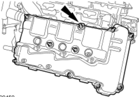
Fig. 180: Locating RH Valve Cover Bolts Courtesy of FORD MOTOR CO.
