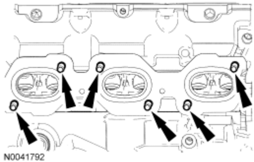
Fig. 152: Locating Exhaust Manifold Studs Courtesy of FORD MOTOR CO.
