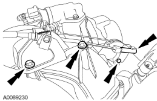
Fig. 365: Accelerator Cable, Speed Control Actuator Cable & Cable Bracket Bolts Courtesy of FORD MOTOR CO.
