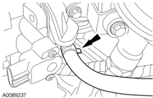
Fig. 125: Locating Vacuum Tube Retainer Courtesy of FORD MOTOR CO.
