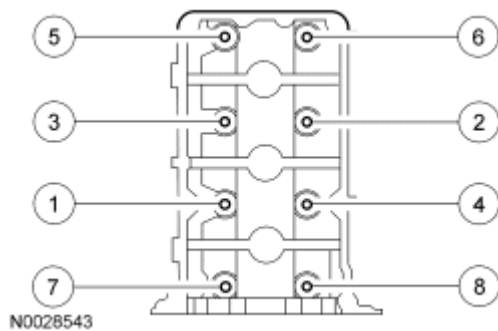
Fig. 239: Identifying Cylinder Heads Bolts Tightening Sequence Courtesy of FORD MOTOR CO.
