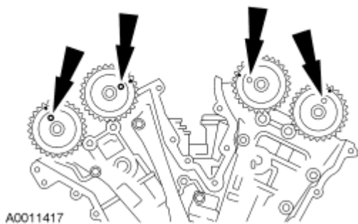
Fig. 242: Locating Camshafts Matching Marks Courtesy of FORD MOTOR CO.
