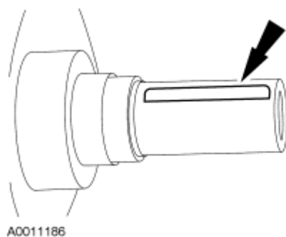
Fig. 230: Locating Crankshaft Key Courtesy of FORD MOTOR CO.
