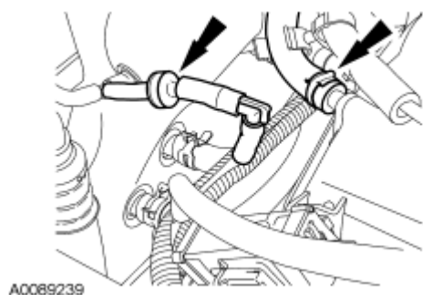
Fig. 356: Locating Brake Booster Vacuum Tube & Vacuum Reservoir Tube Courtesy of FORD MOTOR CO.
