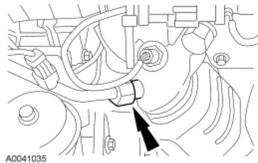
Fig. 367: Locating EGR Tube-To-RH Catalytic Converter Fitting Courtesy of FORD MOTOR CO.
