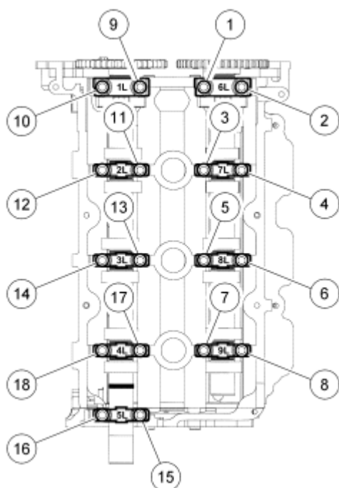
Fig. 245: Identifying Tightening Sequence Of Bolts Courtesy of FORD MOTOR CO.
