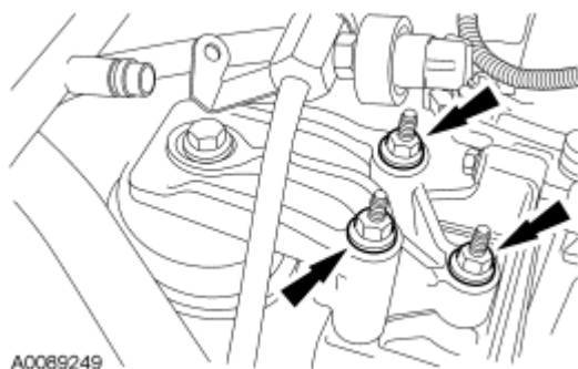
Fig. 336: Locating Front Engine Support Bolts & Nut Courtesy of FORD MOTOR CO.
