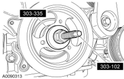
Fig. 18: Installing Crankshaft Pulley Using Special Tools (303-102, 303-335) Courtesy of FORD MOTOR CO.
