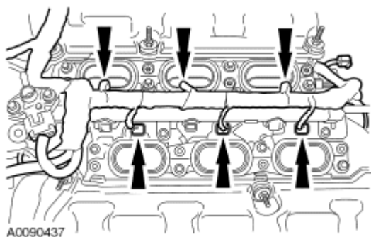
Fig. 302: Locating Fuel Injector Electrical Connectors Courtesy of FORD MOTOR CO.
