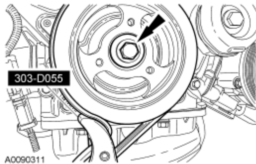
Fig. 19: Locating Special Tool (303-D055) And Crankshaft Pulley Bolt Courtesy of FORD MOTOR CO.
