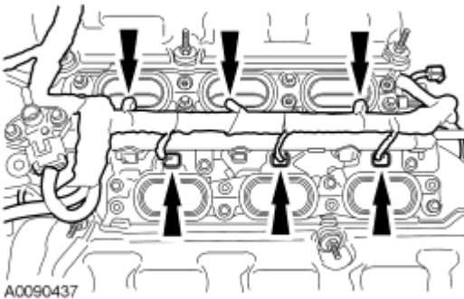
Fig. 176: Locating Fuel Injector Electrical Connectors Courtesy of FORD MOTOR CO.
