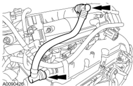
Fig. 313: Locating Positive Crankcase Ventilation (PCV) Tube Courtesy of FORD MOTOR CO.
