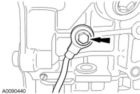
Fig. 276: Locating Knock Sensor (KS) & Bolt Courtesy of FORD MOTOR CO.
