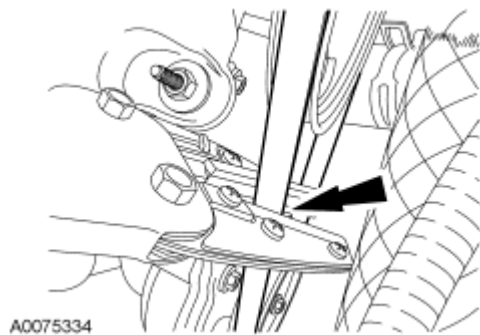
Fig. 189: Cutting Coolant Pump Belt Courtesy of FORD MOTOR CO.
