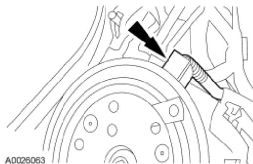
Fig. 106: Locating A/C Clutch Field Coil Electrical Connector Courtesy of FORD MOTOR CO.
