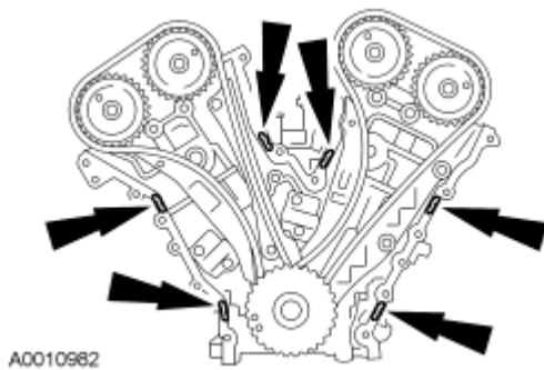
Fig. 268: Applying Sealant To Cylinder Block Courtesy of FORD MOTOR CO.
