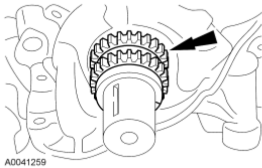
Fig. 44: Locating Crankshaft Sprockets With Timing Marks Out Courtesy of FORD MOTOR CO.
