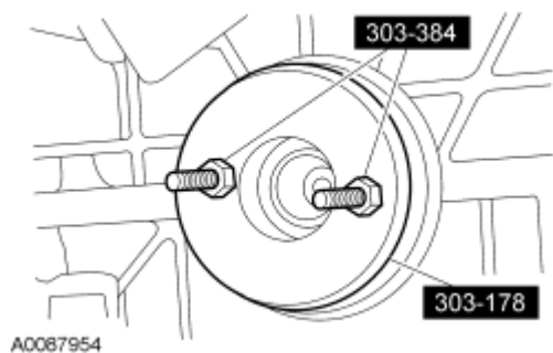
Fig. 321: Identifying Special Tools (303-384 And 303-178) Courtesy of FORD MOTOR CO.
