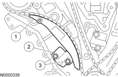
Fig. 55: Identifying Tensioner Arm, Tensioner And Bolts Courtesy of FORD MOTOR CO.
