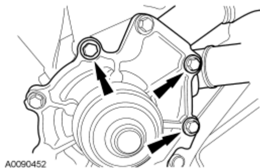
Fig. 191: Locating Coolant Pump & Bolts Courtesy of FORD MOTOR CO.
