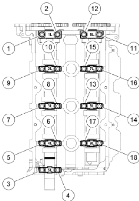
Fig. 66: Identifying Loosening Sequence Of Camshaft Bearing Thrust Caps Courtesy of FORD MOTOR CO.
