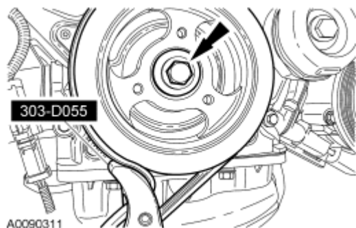
Fig. 15: Locating Special Tool (303-D055) And Crankshaft Pulley Bolt Courtesy of FORD MOTOR CO.
