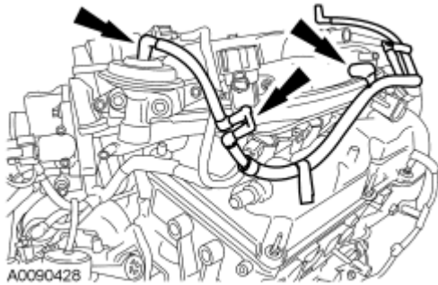
Fig. 166: Vacuum Tube Fittings At EGR Valve, EGR Vacuum Regulator & Intake Manifold Courtesy of FORD MOTOR CO.
