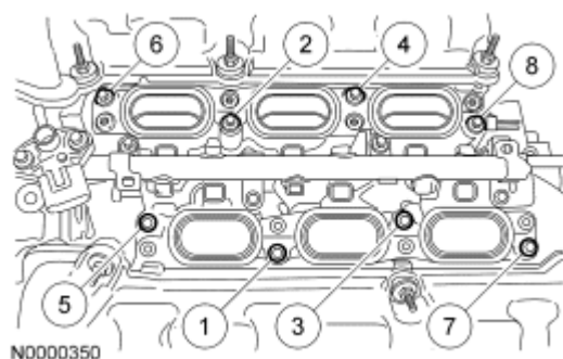
Fig. 301: Identifying Tightening Sequence Of Lower Intake Manifold Bolts Courtesy of FORD MOTOR CO.
