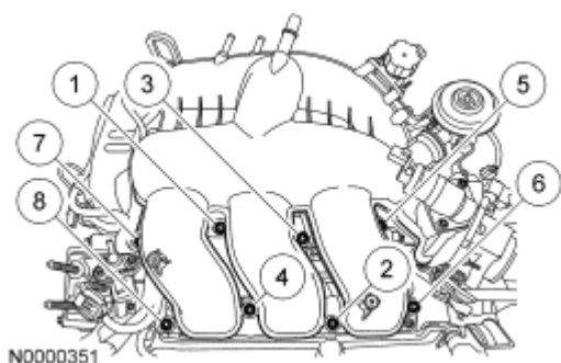
Fig. 310: Identifying Tightening Sequence Of Upper Intake Manifold Bolts Courtesy of FORD MOTOR CO.
