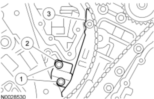
Fig. 41: Locating LH Timing Chain & Tensioner Arm
