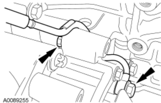
Fig. 326: Locating Pin-Type Retainer & Bolts Courtesy of FORD MOTOR CO.
