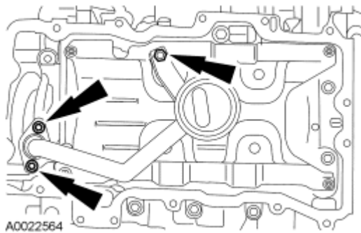
Fig. 94: Locating Oil Pump Screen & Pickup Tube Bolts Courtesy of FORD MOTOR CO.
