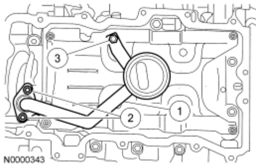
Fig. 280: Identifying Oil Pump Screen, Pickup Tube & Bolts Courtesy of FORD MOTOR CO.
