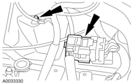
Fig. 133: Locating Ground Strap & Electrical Connector Courtesy of FORD MOTOR CO.
