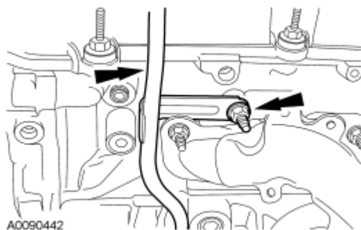
Fig. 194: Positioning Oil Level Indicator Tube Courtesy of FORD MOTOR CO.
