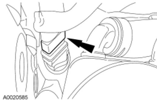
Fig. 348: Locating Engine Block Heater Electrical Connector Courtesy of FORD MOTOR CO.
