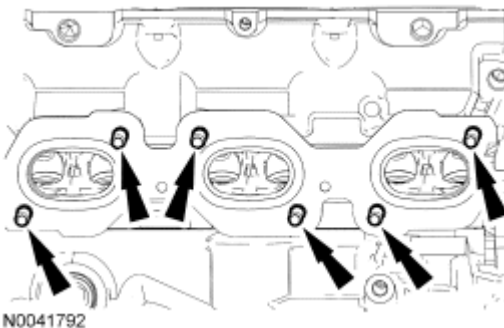
Fig. 184: Locating Exhaust Manifold Studs Courtesy of FORD MOTOR CO.
