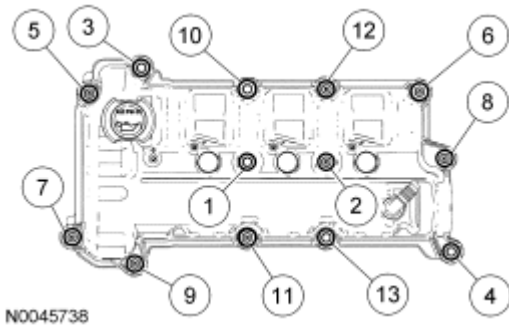
Fig. 10: Identifying Tightening Sequence Of Valve Cover Bolts & Studs Courtesy of FORD MOTOR CO.
