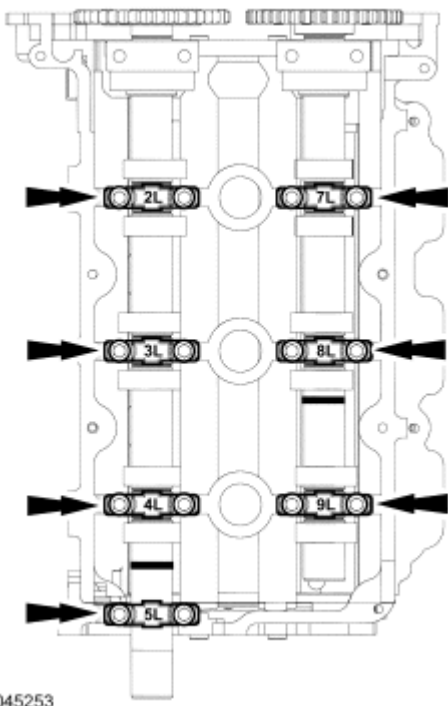
Fig. 68: Locating Camshaft Bearing Caps Installing Sequence Courtesy of FORD MOTOR CO.
