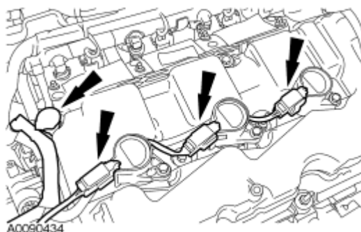
Fig. 170: Coil-On-Plug Electrical Connectors & Wiring Retainers Courtesy of FORD MOTOR CO.
