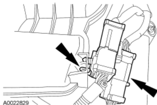
Fig. 319: Locating Engine Control Sensor Wiring Connectors Courtesy of FORD MOTOR CO.
