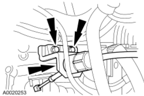
Fig. 360: Locating Gearshift Cable Bracket Bolts Courtesy of FORD MOTOR CO.
