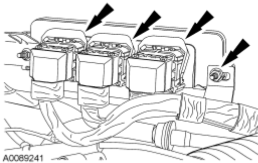
Fig. 354: Locating Powertrain Control Module (PCM) Electrical Connectors Courtesy of FORD MOTOR CO.
