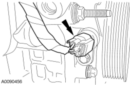
Fig. 174: Locating Crankshaft Position (CKP) Sensor Electrical Connector Courtesy of FORD MOTOR CO.
