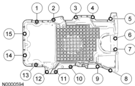
Fig. 343: Identifying Tightening Sequence Of Oil Pan-To-Engine Bolts And Stud Bolts Courtesy of FORD MOTOR CO.
