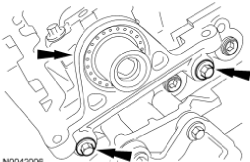
Fig. 249: Locating Camshaft Oil Seal Retainer And Bolts Courtesy of FORD MOTOR CO.
