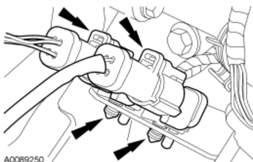
Fig. 334: Locating Heated Oxygen & Catalyst Monitor Sensor Electrical Connectors Courtesy of FORD MOTOR CO.
