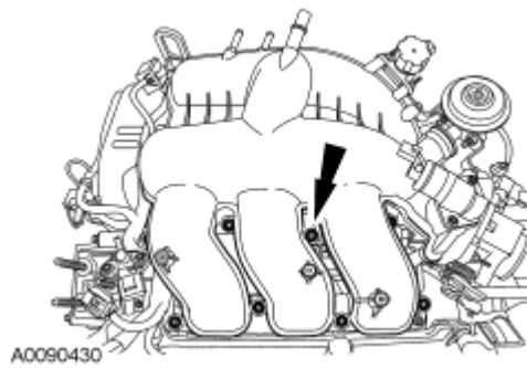
Fig. 168: Locating Upper Intake Manifold Bolts Courtesy of FORD MOTOR CO.
