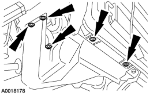
Fig. 27: Locating RH Lower Splash Shield Bolts Courtesy of FORD MOTOR CO.
