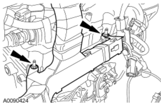
Fig. 315: Locating Engine Control Wiring Harness & Nuts Courtesy of FORD MOTOR CO.
