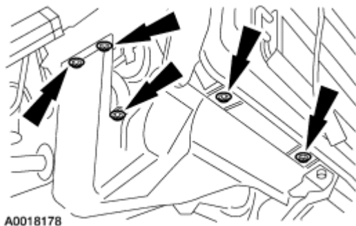
Fig. 30: Locating RH Lower Splash Shield Bolts Courtesy of FORD MOTOR CO.
