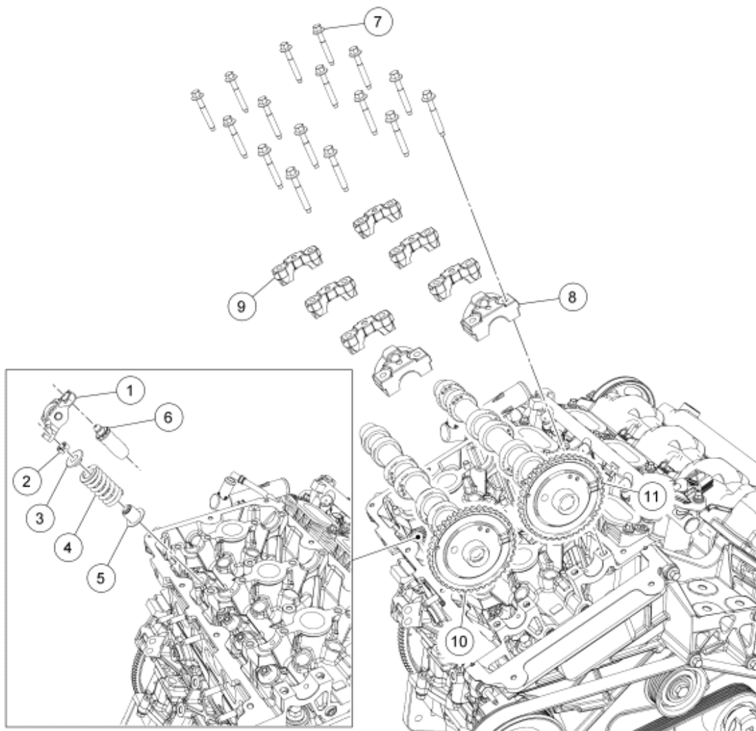
Fig. 61: Exploded View Of Right Valve Train Components (With Torque Specifications) Courtesy of FORD MOTOR CO.
