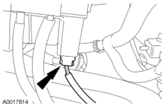
Fig. 132: Power Distribution Box Electrical Connector Courtesy of FORD MOTOR CO.
