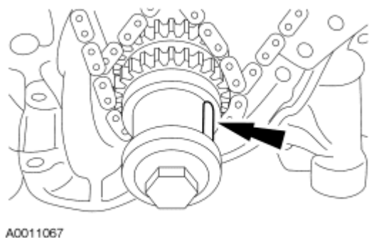
Fig. 211: Identifying Crankshaft Keyway Courtesy of FORD MOTOR CO.
