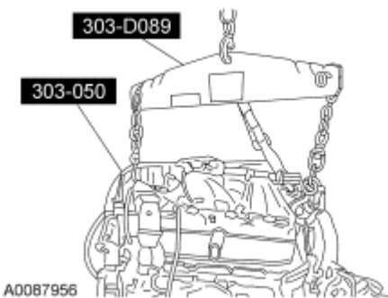
Fig. 156: Removing Engine From Universal Powertrain Lift Courtesy of FORD MOTOR CO.
