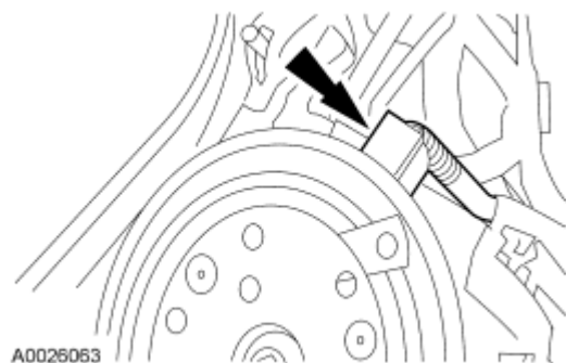
Fig. 375: Locating A/C Clutch Field Coil Electrical Connector Courtesy of FORD MOTOR CO.
