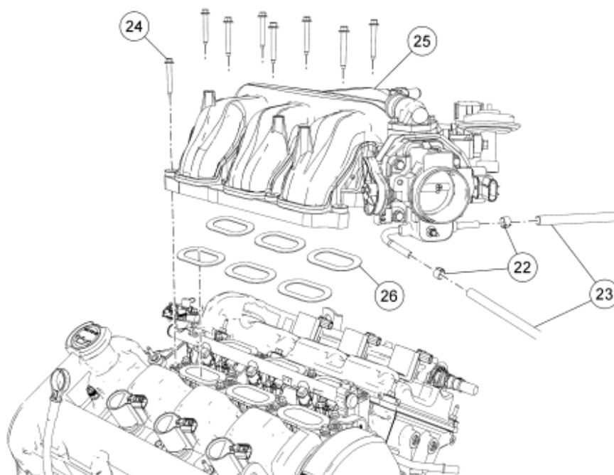
Fig. 4: Exploded View Of Upper Intake Manifold (3 Of 3) Courtesy of FORD MOTOR CO.
