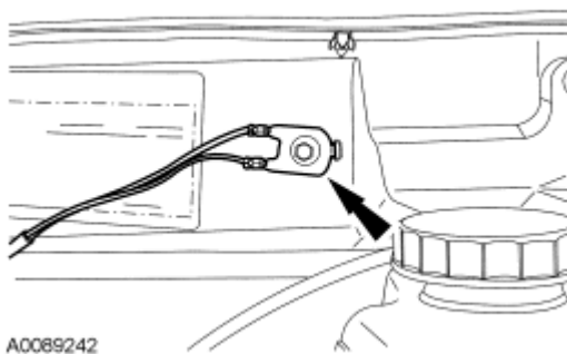
Fig. 129: Locating Ground Wire & Bolt Courtesy of FORD MOTOR CO.
