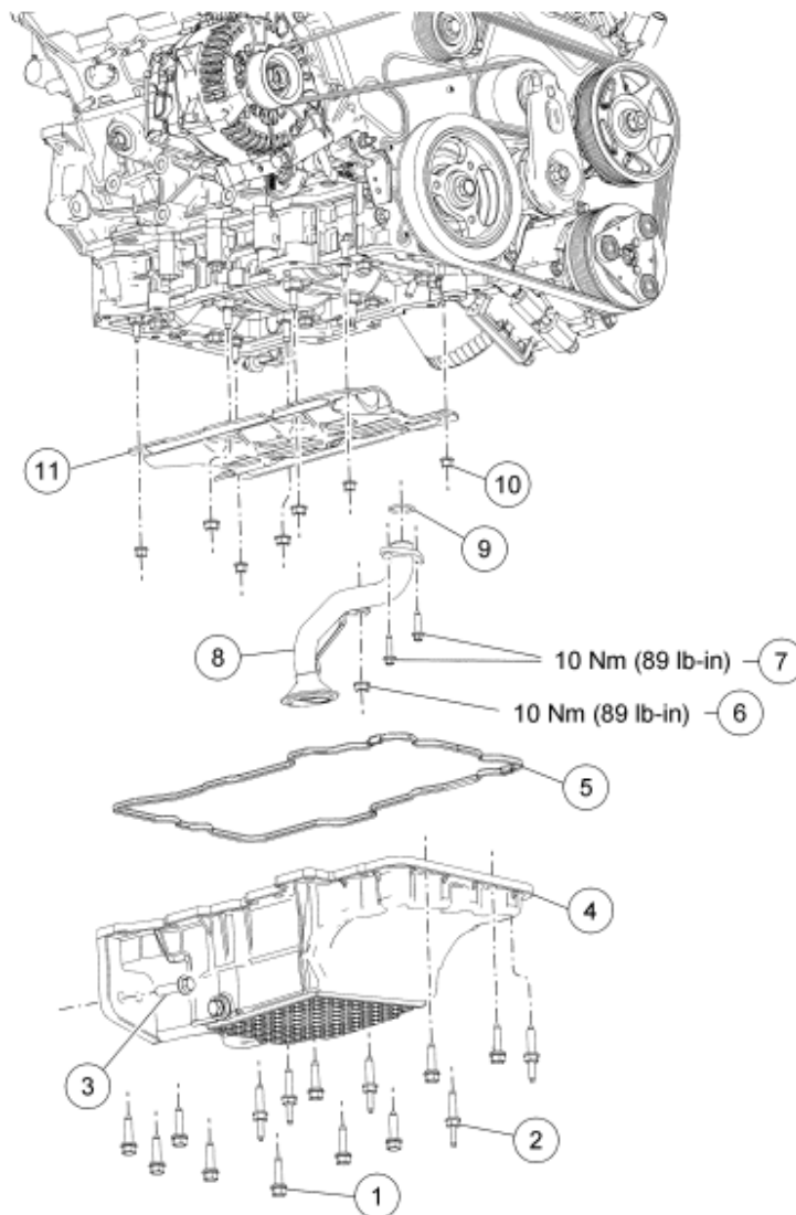
Fig. 90: Exploded View Of Oil Pan, Oil Pump Screen and Pickup Tube and Oil Pan Baffle (With Torque Specifications)
