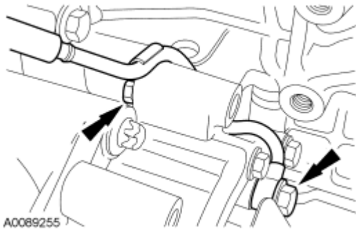
Fig. 154: Locating Pin-Type Retainer & Bolt Courtesy of FORD MOTOR CO.
