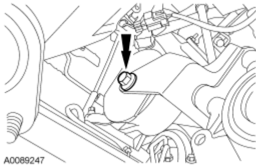
Fig. 339: Locating RH Transaxle Support Insulator Bolt Courtesy of FORD MOTOR CO.
