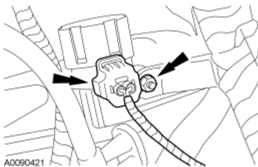
Fig. 161: Locating Exhaust Gas Recirculation (EGR) Vacuum Regulator Electrical Connector Courtesy of FORD MOTOR CO.
