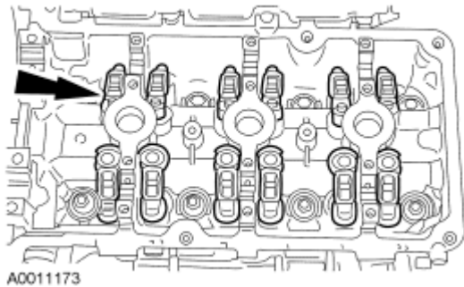
Fig. 241: Locating Camshaft Roller Followers Courtesy of FORD MOTOR CO.
