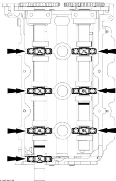
Fig. 243: Locating Camshaft Bearing Caps Installing Sequence Courtesy of FORD MOTOR CO.
