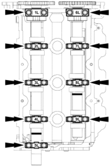
Fig. 223: Marking Camshaft Bearing Caps Courtesy of FORD MOTOR CO.
