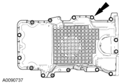
Fig. 341: Locating Oil Pan Gasket Bolts & Stud Bolts Courtesy of FORD MOTOR CO.
