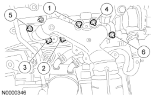
Fig. 293: Left Exhaust Manifold Nuts Tightening Sequence Courtesy of FORD MOTOR CO.
