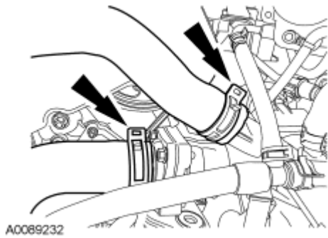
Fig. 118: Locating Hoses Courtesy of FORD MOTOR CO.
