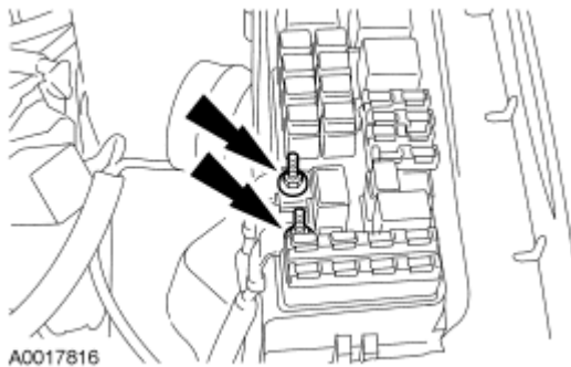
Fig. 131: Locating Cables & Nuts Courtesy of FORD MOTOR CO.
