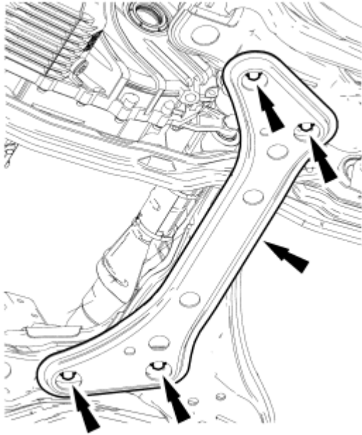
Fig. 371: Identifying Lateral Support Crossmember And Bolts Courtesy of FORD MOTOR CO.
