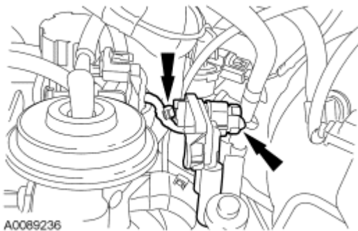
Fig. 123: Locating EGR Sensor Electrical Connector Courtesy of FORD MOTOR CO.
