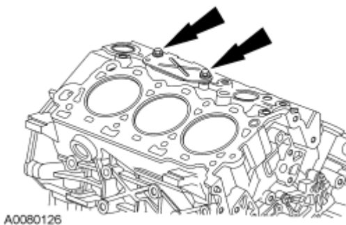
Fig. 238: Locating Oil Separator Cover Bolts
