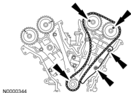
Fig. 259: Aligning Marks On Timing Chain With Marks On Camshaft And Crankshaft Sprockets Courtesy of FORD MOTOR CO.
