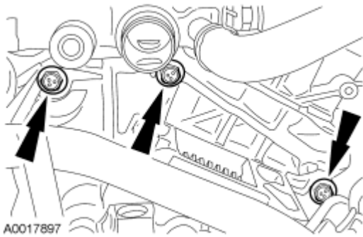
Fig. 155: Locating Transaxle-To-Engine Bolts Courtesy of FORD MOTOR CO.
