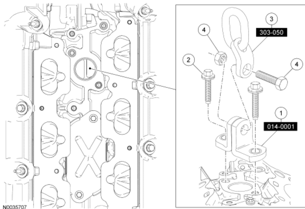
Fig. 100: Identifying Special Tools (303-050 And 014-0001) Courtesy of FORD MOTOR CO.
