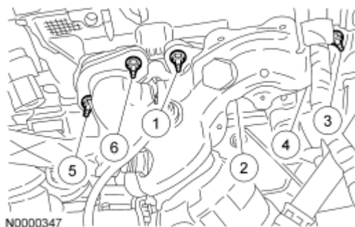
Fig. 329: Identifying Tightening Sequence Of RH Exhaust Manifold Nuts Courtesy of FORD MOTOR CO.
