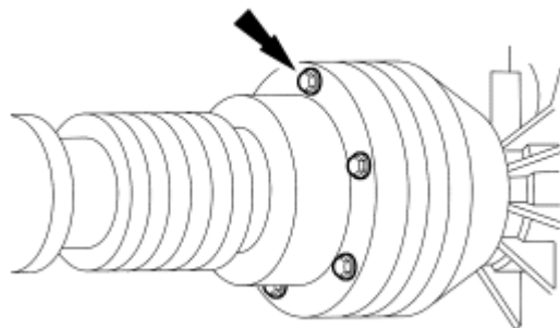
Fig. 104: Locating Driveshaft-To-Power Take Off Bolts & Washers Courtesy of FORD MOTOR CO.
