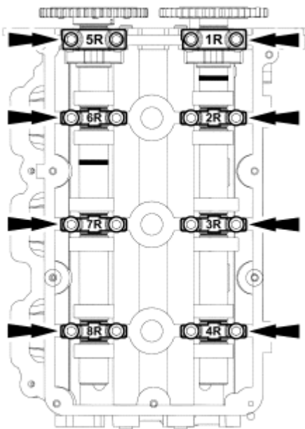
Fig. 225: Marking Camshaft Bearing Cap Positions Courtesy of FORD MOTOR CO.
