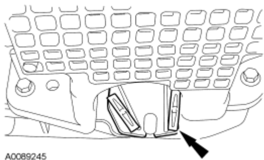
Fig. 345: Locating Torque Converter Inspection Cover Courtesy of FORD MOTOR CO.
