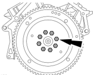
Fig. 322: Locating Flexplate & Bolts Courtesy of FORD MOTOR CO.
