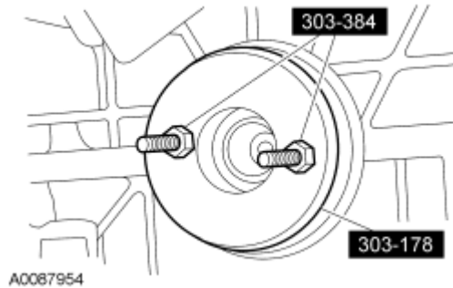
Fig. 23: Identifying Special Tools (303-384 And 303-178) Courtesy of FORD MOTOR CO.
