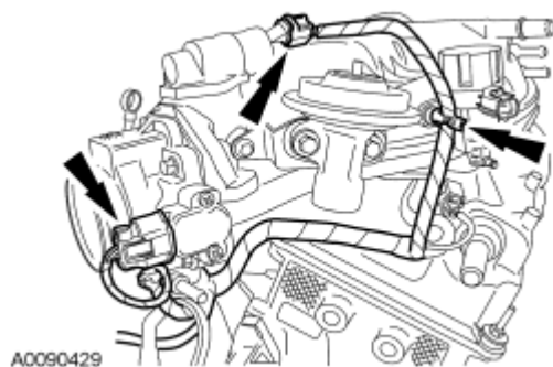
Fig. 314: Idle Air Control Valve & Throttle Position Sensor Electrical Connectors Courtesy of FORD MOTOR CO.
