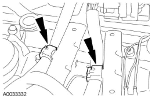
Fig. 349: Wiring Harness Retainers Courtesy of FORD MOTOR CO.
