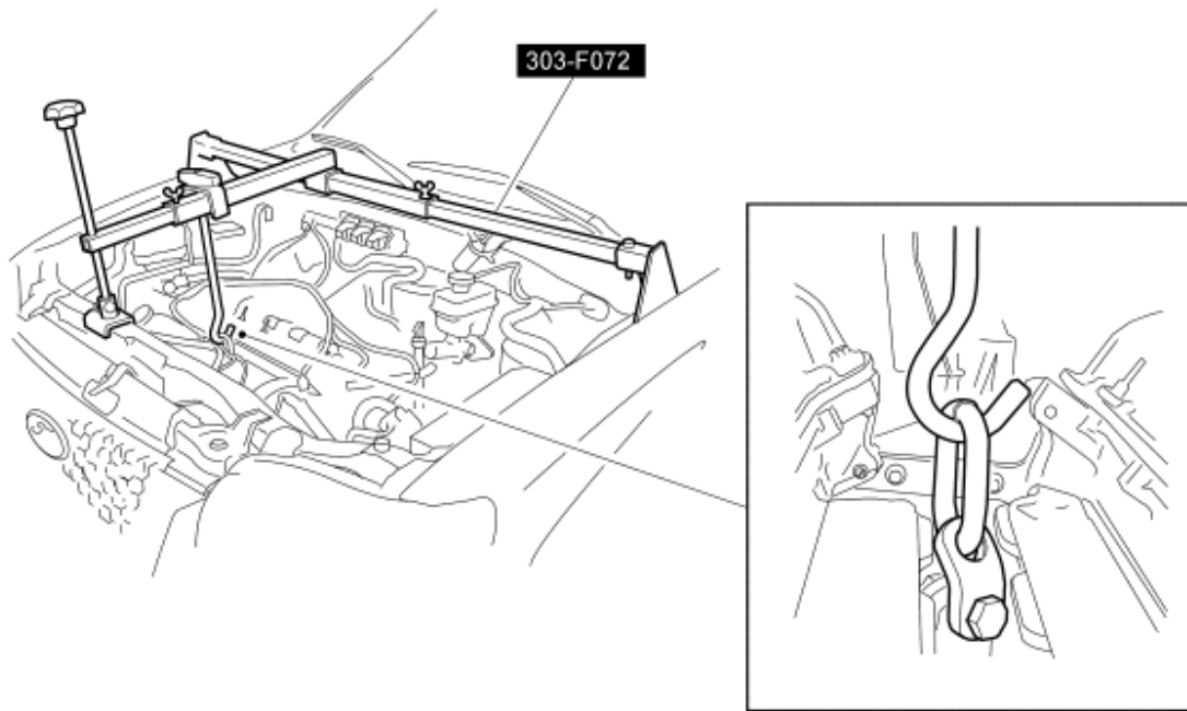
Fig. 101: Lifting Engine 12 mm (0.47 in) Courtesy of FORD MOTOR CO.
