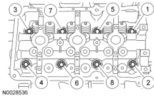
Fig. 84: Identifying Removing Sequence Of Cylinder Head Bolts Courtesy of FORD MOTOR CO.
