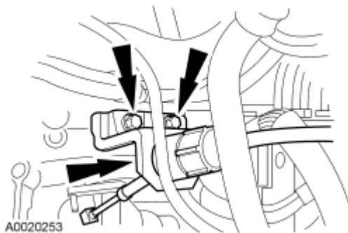
Fig. 122: Locating Gearshift Cable Bracket Bolts Courtesy of FORD MOTOR CO.
