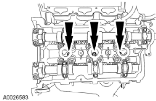
Fig. 33: Locating Spark Plugs Courtesy of FORD MOTOR CO.
