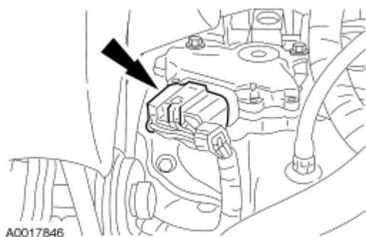
Fig. 333: Locating Transmission Range (TR) Sensor Electrical Connector Courtesy of FORD MOTOR CO.
