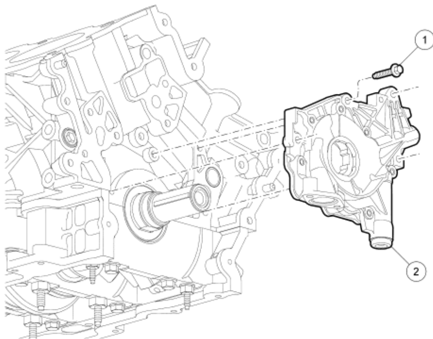
Fig. 91: Exploded View Of Oil Pump Courtesy of FORD MOTOR CO.
