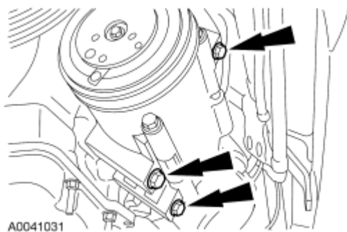
Fig. 374: Locating A/C Compressor & Bolts Courtesy of FORD MOTOR CO.
