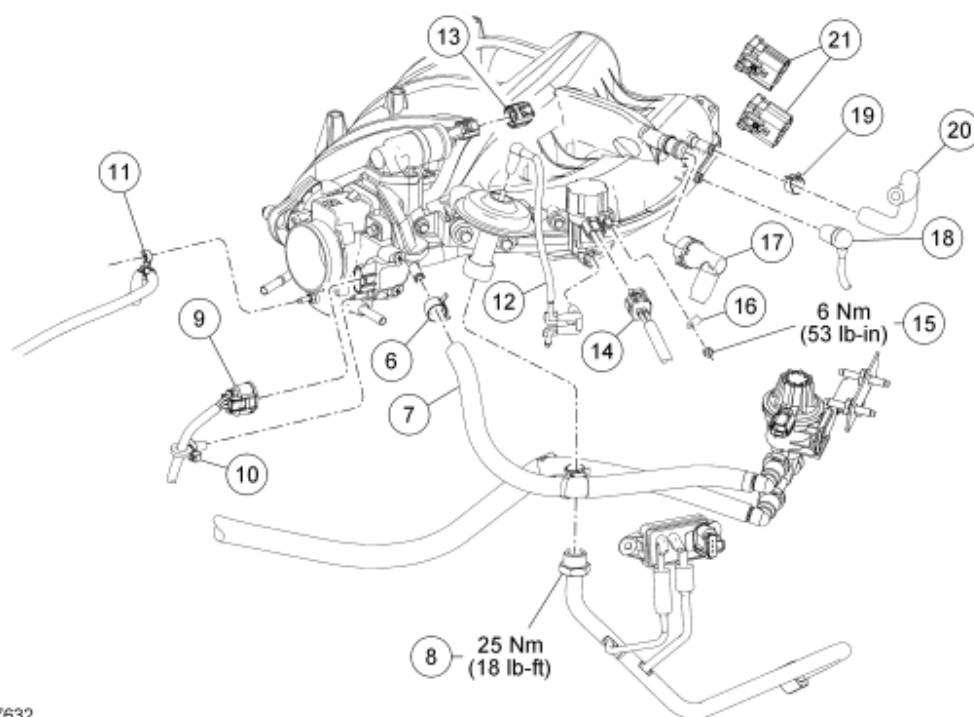
Fig. 3: Exploded View Of Upper Intake Manifold With Torque Specifications (2 Of 3) Courtesy of FORD MOTOR CO.
