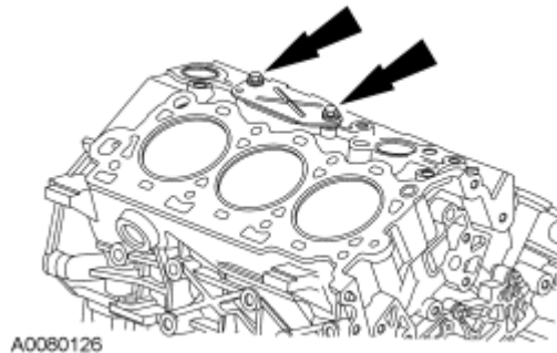
Fig. 229: Locating Oil Separator Cover Bolts Courtesy of FORD MOTOR CO.
