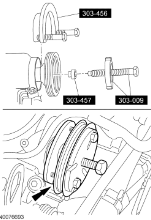
Fig. 62: Removing Coolant Pump Pulley Courtesy of FORD MOTOR CO.
