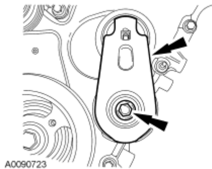
Fig. 270: Locating Belt Tensioner & Bolt Courtesy of FORD MOTOR CO.
