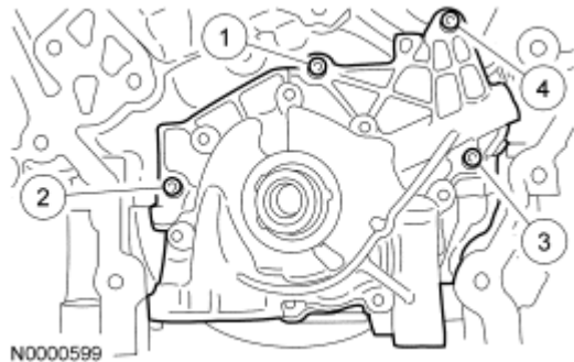
Fig. 97: Identifying Tightening Sequence Of Oil Pump Bolts Courtesy of FORD MOTOR CO.
