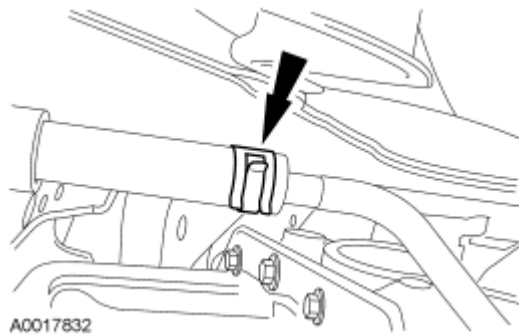
Fig. 113: Locating Transmission Cooler Tubes Courtesy of FORD MOTOR CO.
