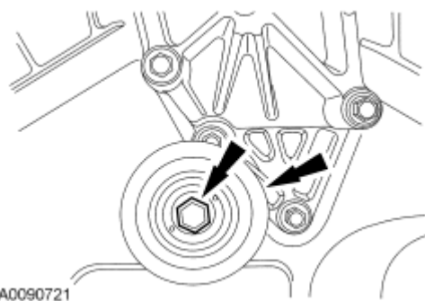
Fig. 204: Locating Idler Pulley & Bolt Courtesy of FORD MOTOR CO.
