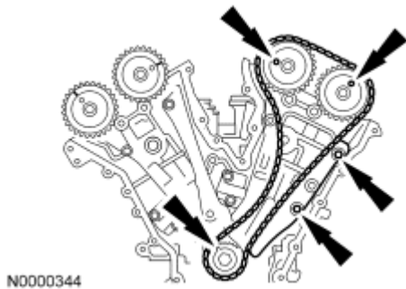
Fig. 50: Aligning Marks On Timing Chain With Marks On Camshaft And Crankshaft Sprockets Courtesy of FORD MOTOR CO.
