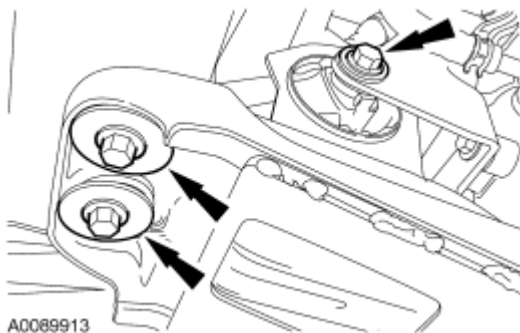
Fig. 111: Identifying Front Roll Restrictor Bolt & Bolts For Engine Support Crossmember Courtesy of FORD MOTOR CO.
