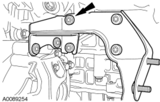
Fig. 153: Locating Half Shaft Support Bracket & Bolts Courtesy of FORD MOTOR CO.
