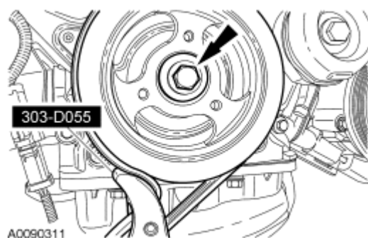
Fig. 201: Locating Special Tool (303-D055) And Crankshaft Pulley Bolt Courtesy of FORD MOTOR CO.
