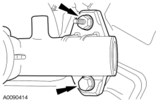
Fig. 193: Locating Coolant Bypass Tube Bolt & Nut Courtesy of FORD MOTOR CO.
