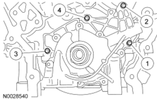
Fig. 96: Identifying Removing Sequence Of Oil Pump Bolts Courtesy of FORD MOTOR CO.
