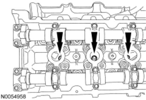
Fig. 209: Spark Plugs Courtesy of FORD MOTOR CO.
