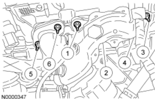
Fig. 86: Identifying Tightening Sequence Of RH Exhaust Manifold Nuts Courtesy of FORD MOTOR CO.
