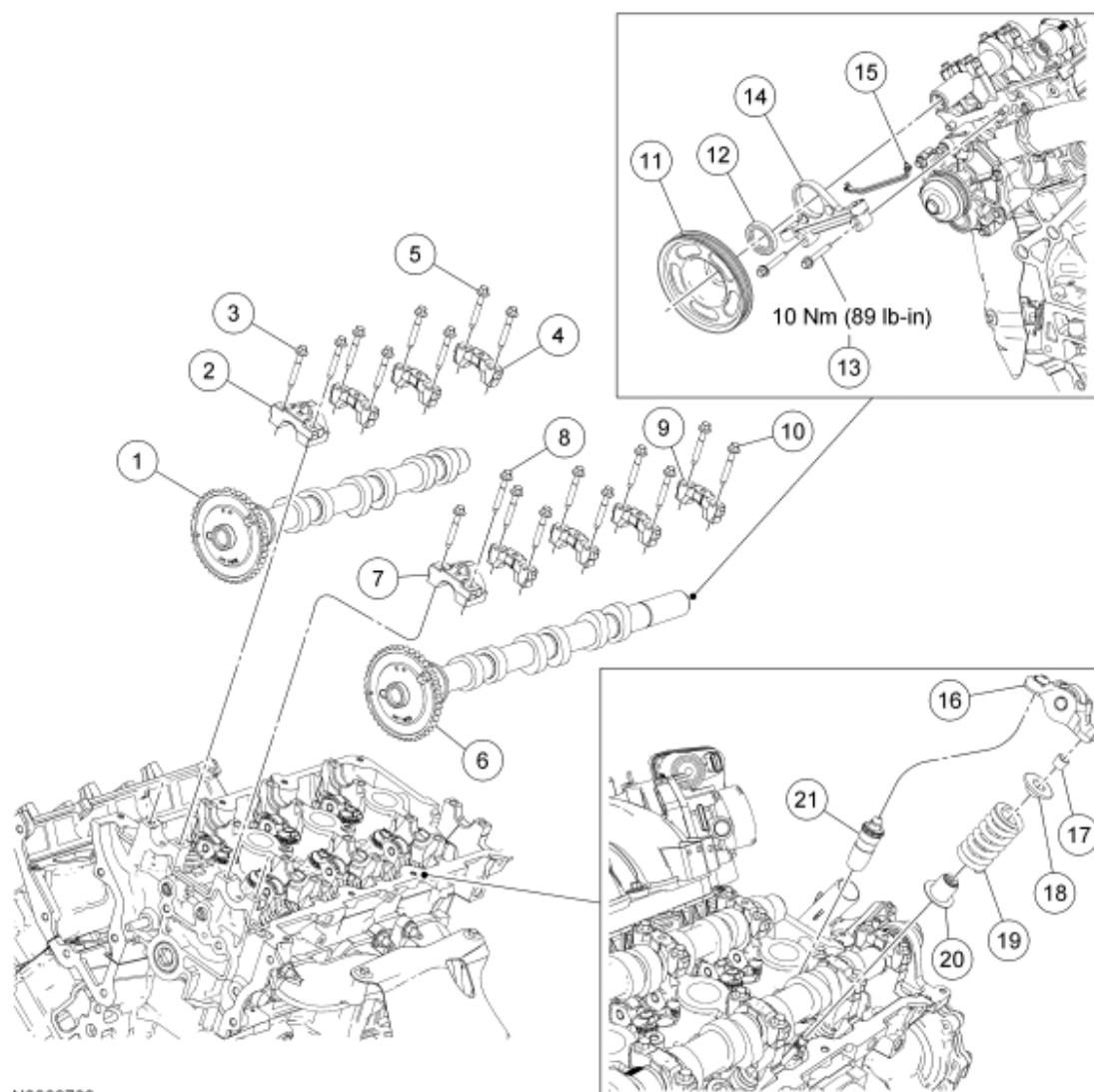
Fig. 60: Exploded View Of Left Valve Train Components (With Torque Specifications) Courtesy of FORD MOTOR CO.
