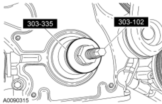
Fig. 21: Installing Crankshaft Seal Using Special Tools (303-335 And 303-102) Courtesy of FORD MOTOR CO.
