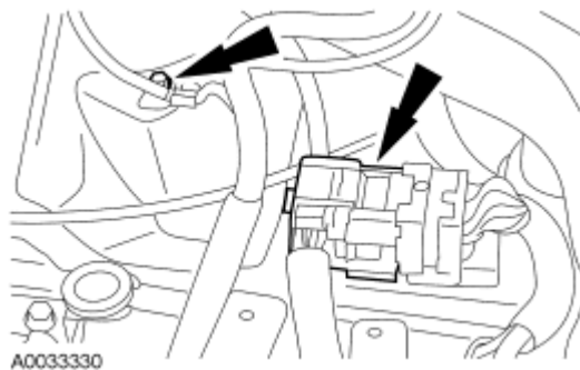
Fig. 350: Locating Ground Strap & Electrical Connector Courtesy of FORD MOTOR CO.
