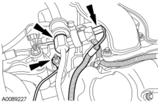
Fig. 379: Locating Power Steering Pressure (PSP) Switch Electrical Connector Courtesy of FORD MOTOR CO.
