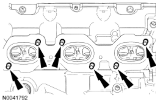
Fig. 187: Locating Exhaust Manifold Studs Courtesy of FORD MOTOR CO.
