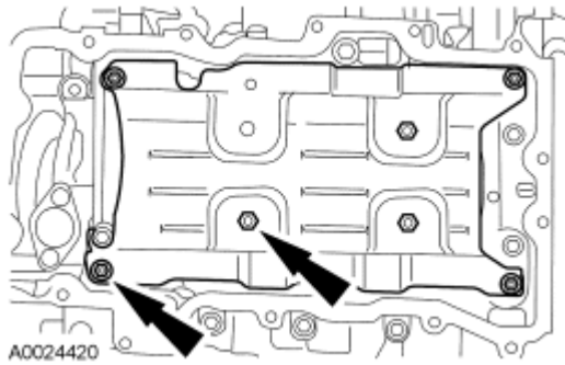
Fig. 198: Locating Oil Pan Baffle Nuts Courtesy of FORD MOTOR CO.
