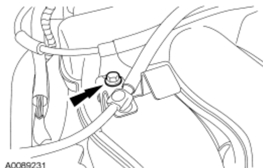
Fig. 364: Locating Cable Bracket Bolts (2 Of 2) Courtesy of FORD MOTOR CO.
