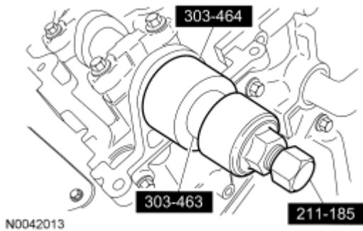
Fig. 72: Identifying Special Tools (303-463, 303-464 And 211-185) Courtesy of FORD MOTOR CO.
