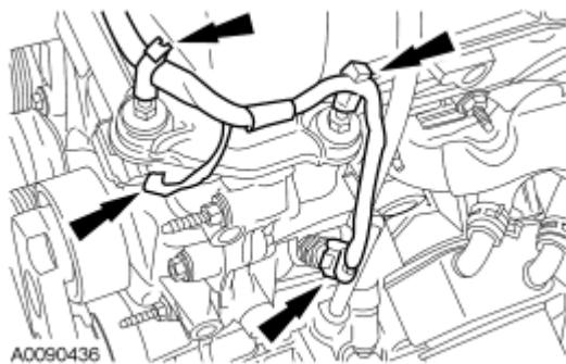
Fig. 173: Locating Camshaft Position Sensor (CMP) & Oil Pressure Sensor Electrical Connectors & Wiring Retainers Courtesy of FORD MOTOR CO.
