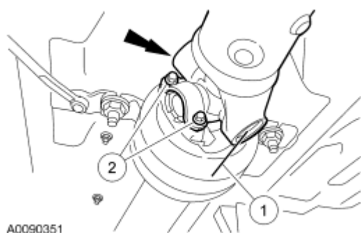
Fig. 376: Locating Straps & Bolts Courtesy of FORD MOTOR CO.
