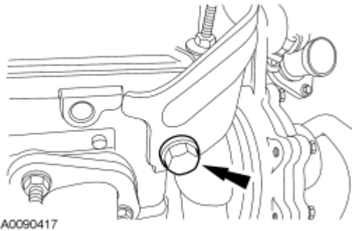
Fig. 297: Locating Lift Bracket & Bolt Courtesy of FORD MOTOR CO.
