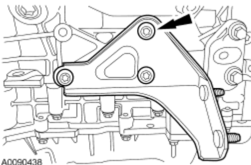
Fig. 185: Locating Halfshaft Support Bracket & Bolts Courtesy of FORD MOTOR CO.
