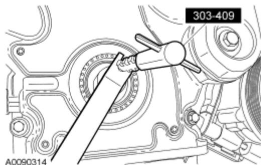
Fig. 20: Removing Crankshaft Front Seal Using Special Tool (303-409) Courtesy of FORD MOTOR CO.
