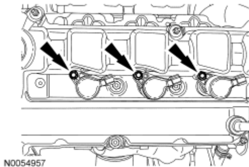
Fig. 178: Coil-On-Plug Bolts Courtesy of FORD MOTOR CO.
