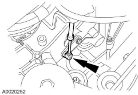
Fig. 121: Locating Shift Cable End At Manual Lever Courtesy of FORD MOTOR CO.
