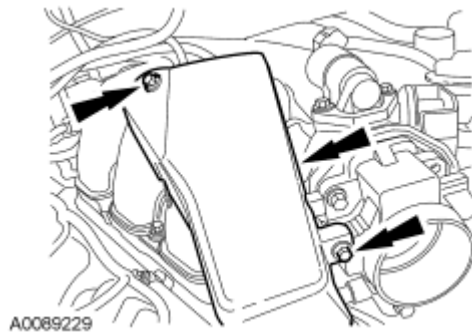
Fig. 115: Locating Accelerator Cable Snow Shield Bolts Courtesy of FORD MOTOR CO.
