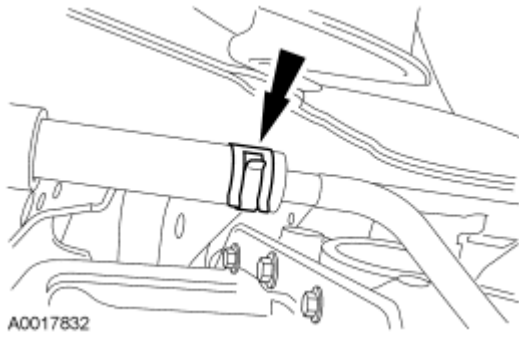
Fig. 368: Locating Transmission Cooler Tubes Courtesy of FORD MOTOR CO.
