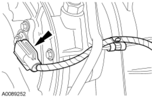
Fig. 330: Locating Turbine Speed Sensor (TSS) Electrical Connector Courtesy of FORD MOTOR CO.
