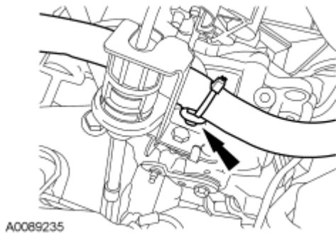
Fig. 361: Locating Pin-Type Retainer Courtesy of FORD MOTOR CO.
