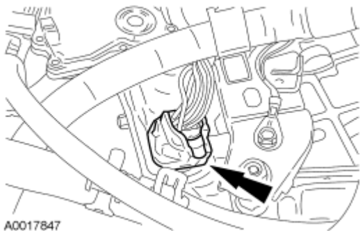
Fig. 332: Locating Transaxle Wiring Harness Electronic Control Switch Electrical Connector Courtesy of FORD MOTOR CO.
