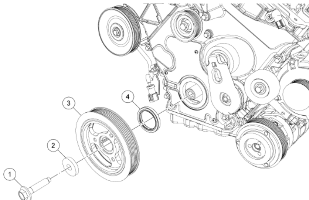
Fig. 13: Exploded View Of Crankshaft Pulley and Front Seal Courtesy of FORD MOTOR CO.
