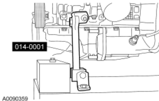
Fig. 141: Securing Engine & Transaxle To Powertrain Lift Using Special Tool (014-0001) Courtesy of FORD MOTOR CO.
