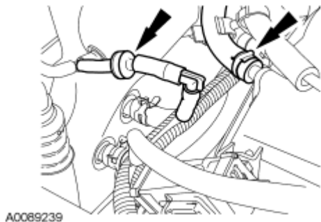
Fig. 126: Locating Brake Booster Vacuum Tube & Vacuum Reservoir Tube Courtesy of FORD MOTOR CO.
