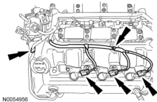
Fig. 172: Coil-On-Plug Electrical Connectors & Wiring Retainers Courtesy of FORD MOTOR CO.
