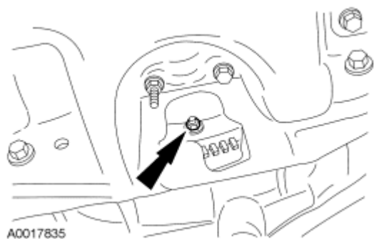
Fig. 344: Locating Torque Converter Nuts Courtesy of FORD MOTOR CO.
