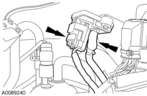
Fig. 127: Locating Manifold Absolute Pressure (MAP) Sensor Vacuum Tube & Electrical Connector Courtesy of FORD MOTOR CO.
