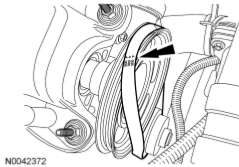
Fig. 287: Locating Coolant Pump Belt On Coolant Pump Pulley Courtesy of FORD MOTOR CO.
