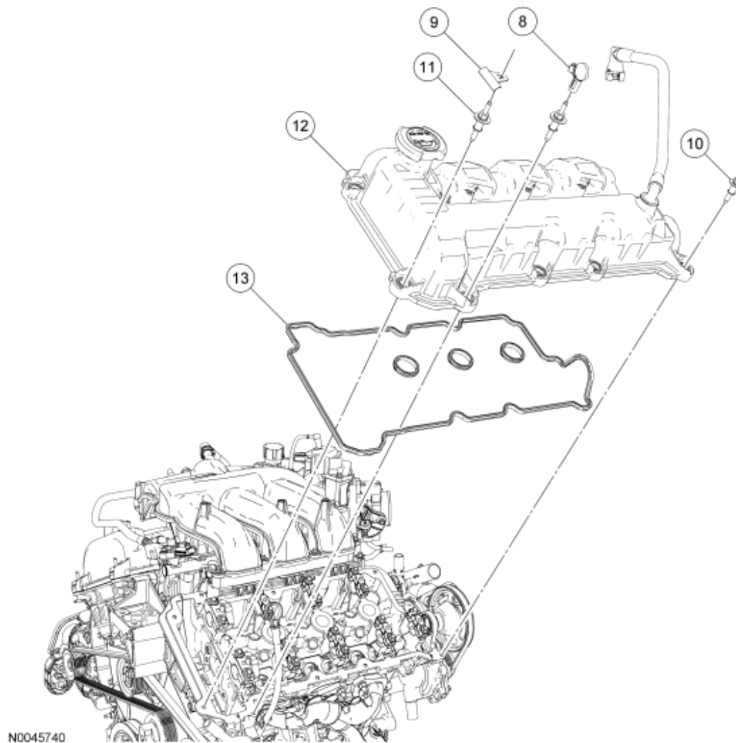
Fig. 9: Exploded View Of Left Valve Cover - 2 Of 2 (With Torque Specifications) Courtesy of FORD MOTOR CO.
