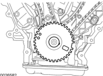
Fig. 207: Identifying Ignition Pulse Wheel Courtesy of FORD MOTOR CO.
