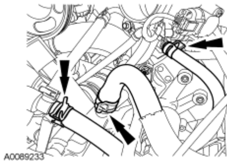
Fig. 119: Locating Heater Hoses & Throttle Body Coolant Hose Courtesy of FORD MOTOR CO.
