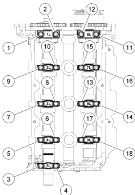
Fig. 224: Camshaft Bearing Cap Bolts Loosening Sequence Courtesy of FORD MOTOR CO.
