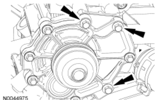
Fig. 87: Locating Coolant Pump And Bolts Courtesy of FORD MOTOR CO.
