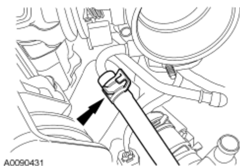
Fig. 311: Locating Throttle Body Coolant Hose Courtesy of FORD MOTOR CO.
