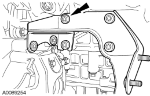
Fig. 327: Locating Half Shaft Support Bracket & Bolts Courtesy of FORD MOTOR CO.
