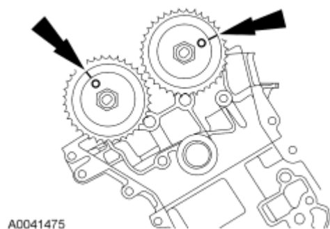
Fig. 36: Locating Camshafts Align Marks Courtesy of FORD MOTOR CO.
