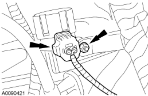
Fig. 317: Locating Exhaust Gas Recirculation (EGR) Vacuum Regulator Electrical Connector Courtesy of FORD MOTOR CO.
