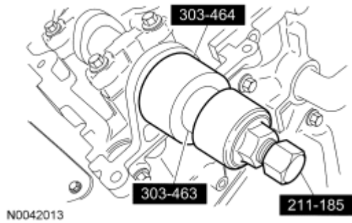
Fig. 250: Identifying Special Tools (303-463, 303-464 And 211-185) Courtesy of FORD MOTOR CO.
