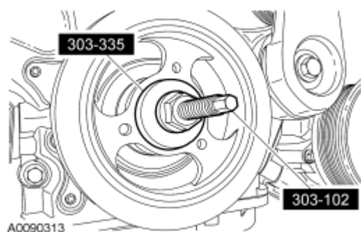
Fig. 274: Installing Crankshaft Pulley Using Special Tools (303-102, 303-335) Courtesy of FORD MOTOR CO.
