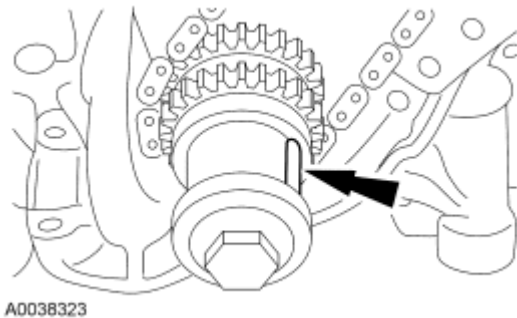
Fig. 261: Locating Crankshaft Keyway Courtesy of FORD MOTOR CO.
