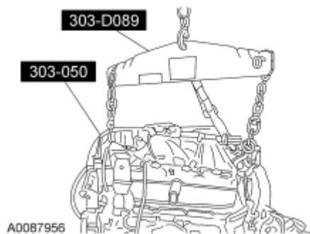
Fig. 323: Aligning Engine With Transaxle Courtesy of FORD MOTOR CO.
