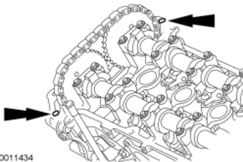
Fig. 295: Applying Silicone Gasket And Sealant At Cylinder Head To Front Cover Mating Surface
