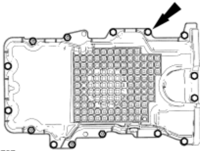
Fig. 195: Locating Oil Pan Gasket Bolts & Stud Bolts Courtesy of FORD MOTOR CO.
