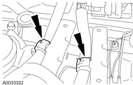
Fig. 134: Wiring Harness Retainers Courtesy of FORD MOTOR CO.
