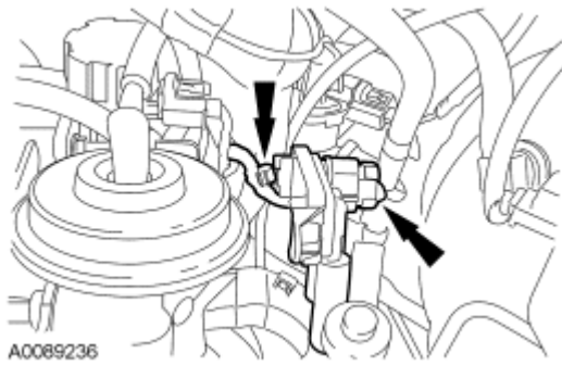
Fig. 359: Locating EGR Sensor Electrical Connector Courtesy of FORD MOTOR CO.
