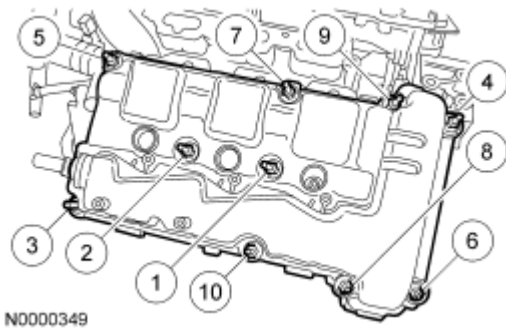
Fig. 12: Identifying Tightening Sequence Of Valve Cover Stud Bolts Courtesy of FORD MOTOR CO.
