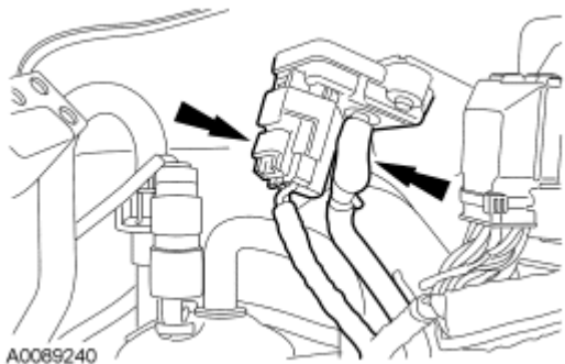
Fig. 355: Locating Manifold Absolute Pressure (MAP) Sensor Vacuum Tube & Electrical Connector Courtesy of FORD MOTOR CO.
