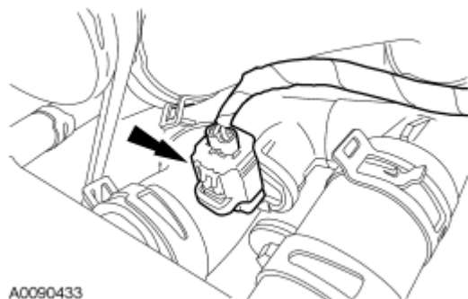
Fig. 309: Locating Engine Coolant Temperature (ECT) Sensor Electrical Connector Courtesy of FORD MOTOR CO.
