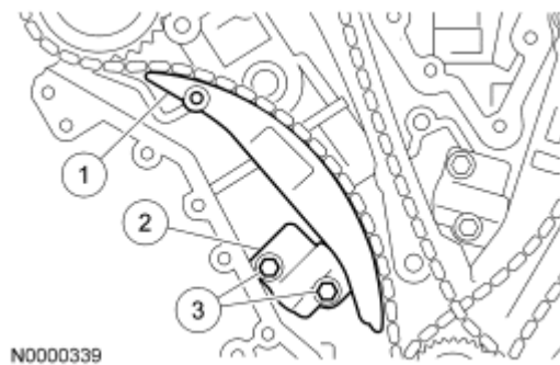
Fig. 264: Identifying Tensioner Arm, Tensioner And Bolts Courtesy of FORD MOTOR CO.
