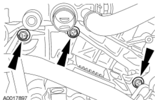
Fig. 324: Locating Transaxle-To-Engine Bolts
