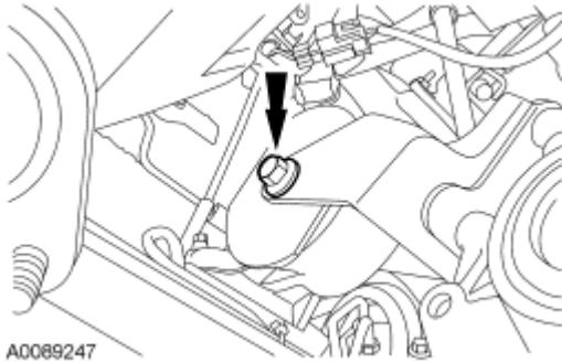
Fig. 142: Locating RH Transaxle Support Insulator Bolt Courtesy of FORD MOTOR CO.
