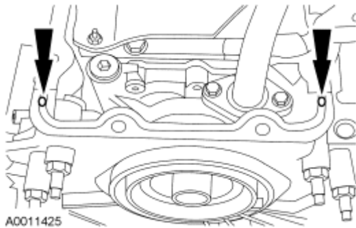
Fig. 340: Applying Silicone Gasket And Sealant To Front Cover-To-Cylinder Block Courtesy of FORD MOTOR CO.
