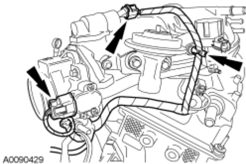
Fig. 164: Idle Air Control Valve & Throttle Position Sensor Electrical Connectors Courtesy of FORD MOTOR CO.
