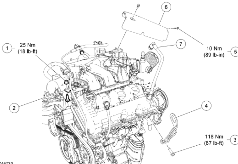
Fig. 8: Exploded View Of Left Valve Cover - 1 Of 2 (With Torque Specifications) Courtesy of FORD MOTOR CO.
