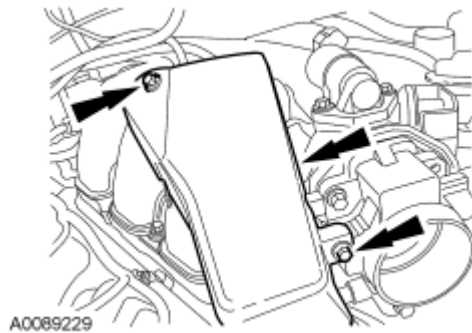
Fig. 366: Locating Accelerator Cable Snow Shield Bolts Courtesy of FORD MOTOR CO.
