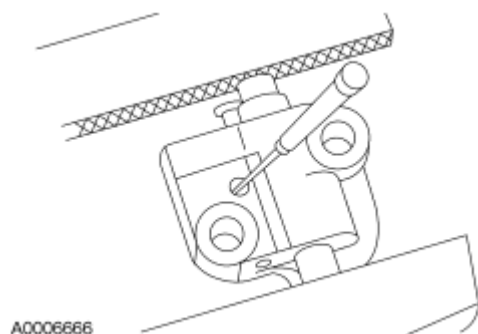
Fig. 256: Holding Chain Tensioner Ratchet Lock Mechanism Away From Ratchet Stem Courtesy of FORD MOTOR CO.
