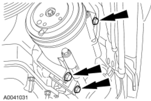
Fig. 107: Locating A/C Compressor & Bolts Courtesy of FORD MOTOR CO.
