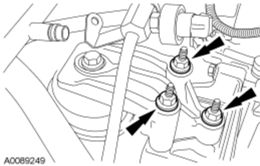
Fig. 145: Locating Front Engine Support Bolts & Nut Courtesy of FORD MOTOR CO.
