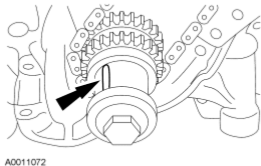
Fig. 215: Positioning Crankcase Key Way In 11 O'Clock Position Courtesy of FORD MOTOR CO.
