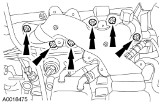
Fig. 186: Locating LH Exhaust Manifold & Gasket Courtesy of FORD MOTOR CO.
