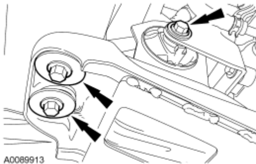
Fig. 370: Identifying Front Roll Restrictor Bolt & Bolts For Engine Support Crossmember Courtesy of FORD MOTOR CO.
