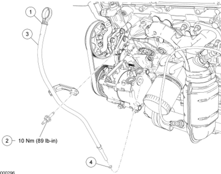
Fig. 98: Exploded View Of Oil Level Indicator & Tube (With Torque Specifications) Courtesy of FORD MOTOR CO.
