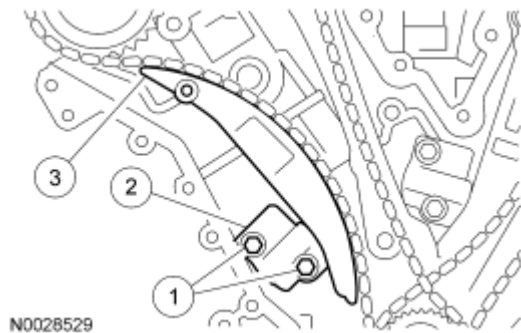
Fig. 213: Identifying RH Timing Chain Tensioner Arm & Bolts Courtesy of FORD MOTOR CO.
