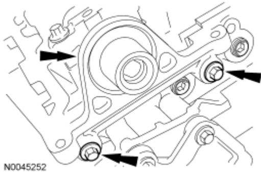
Fig. 64: Locating Camshaft Oil Seal Retainer & Bolts Courtesy of FORD MOTOR CO.
