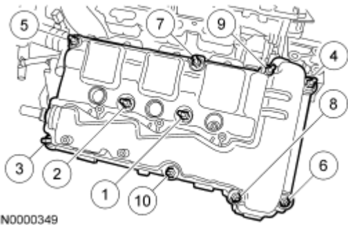
Fig. 298: Identifying Tightening Sequence Of Valve Cover Stud Bolts Courtesy of FORD MOTOR CO.
