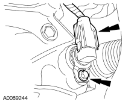
Fig. 346: Locating Output Shaft Speed (OSS) Sensor Electrical Connector Courtesy of FORD MOTOR CO.
