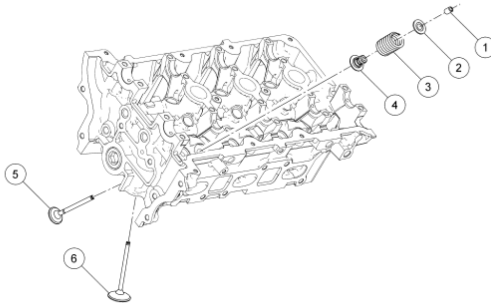
Fig. 231: Exploded View Of Valve Components Courtesy of FORD MOTOR CO.
