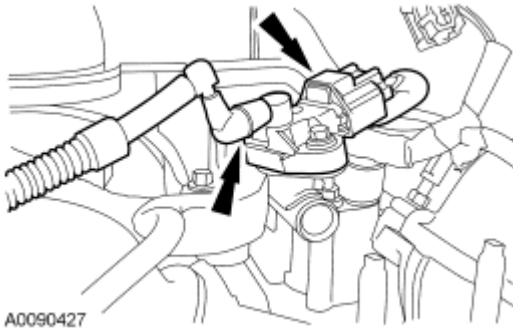
Fig. 175: Locating Fuel Rail Pressure & Temperature Sensor Electrical Connector Courtesy of FORD MOTOR CO.
