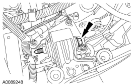
Fig. 337: Locating Transaxle Mount Bolt Courtesy of FORD MOTOR CO.
