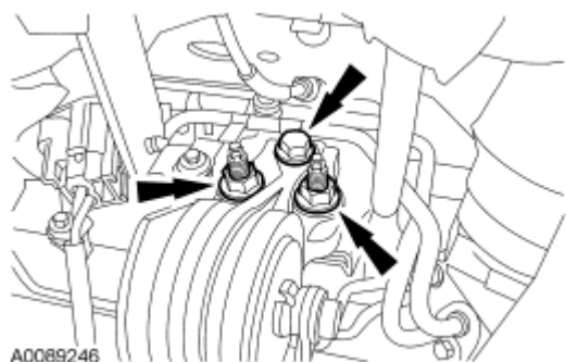
Fig. 338: Locating Transaxle Support Insulator Bolt & Nuts Courtesy of FORD MOTOR CO.
