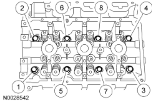
Fig. 228: Identifying Cylinder Heads Bolts Loosening Sequence Courtesy of FORD MOTOR CO.
