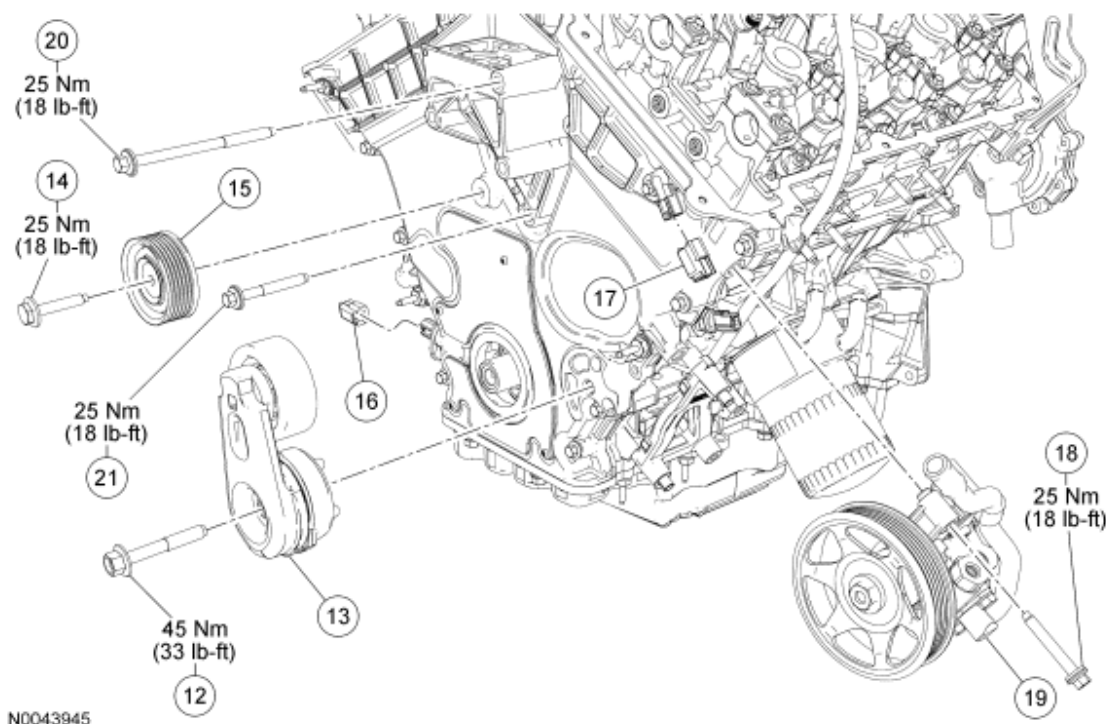
Fig. 25: Exploded View Of Engine Front Cover Components - 2 Of 3 (With Torque Specifications) Courtesy of FORD MOTOR CO.
