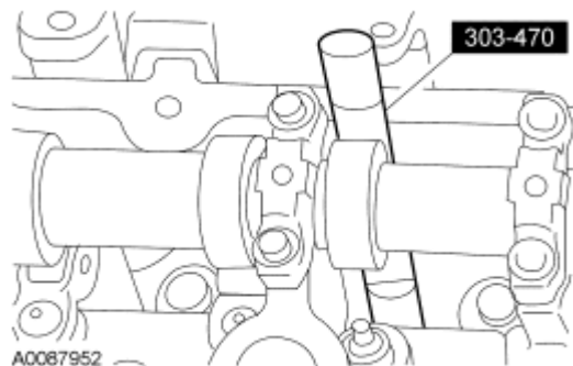
Fig. 82: Installing Valve Seal Courtesy of FORD MOTOR CO.
