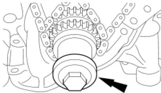
Fig. 266: Identifying Damper Bolt Courtesy of FORD MOTOR CO.
