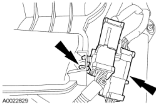
Fig. 159: Locating Engine Control Sensor Wiring Connectors Courtesy of FORD MOTOR CO.
