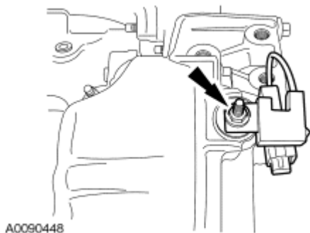
Fig. 179: Locating Radio Interference Capacitor Nut Courtesy of FORD MOTOR CO.
