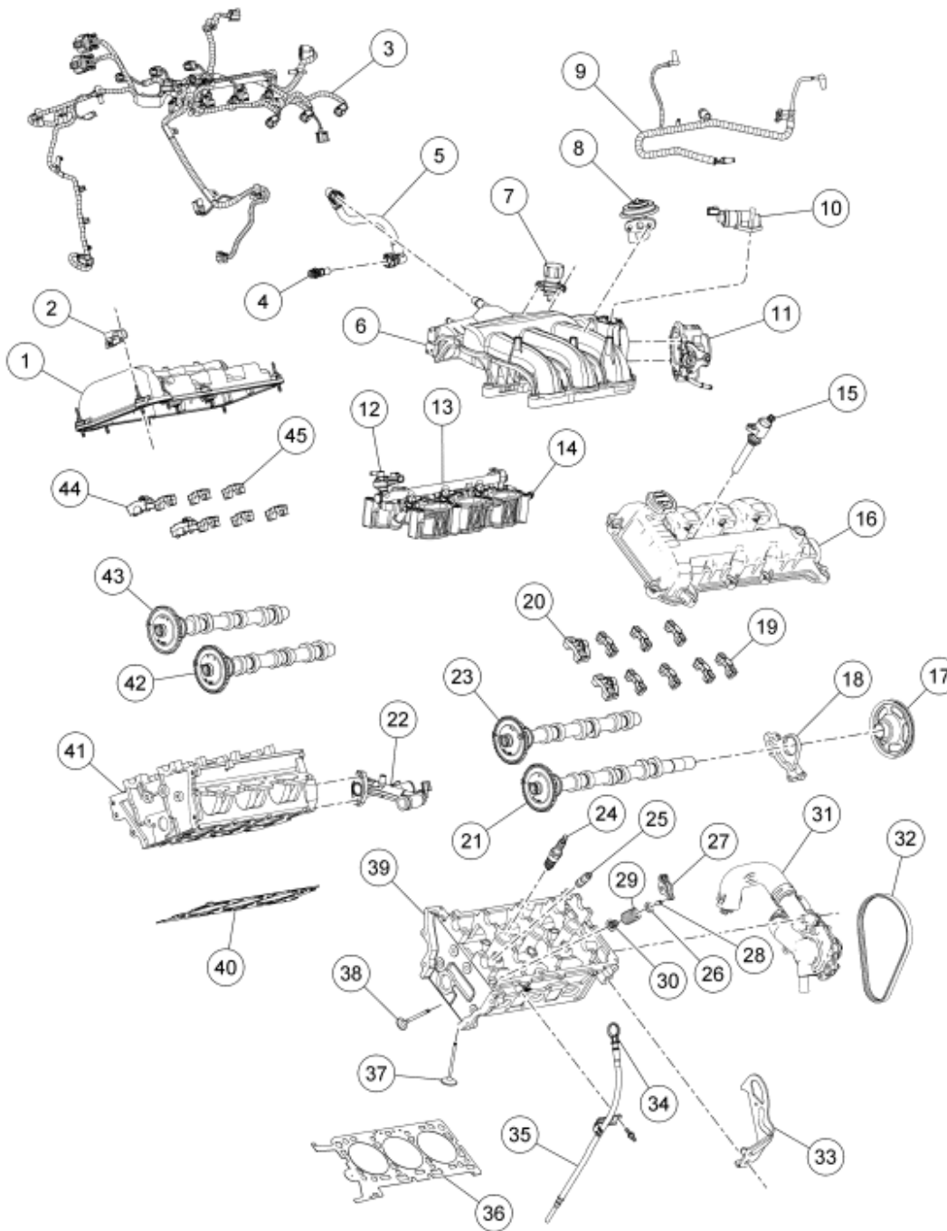
Fig. 236: Exploded View Of Engine (2 Of 2) Courtesy of FORD MOTOR CO.
