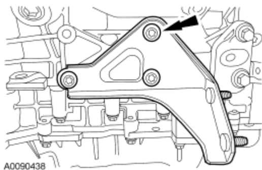
Fig. 289: Locating Halfshaft Support Bracket & Bolts Courtesy of FORD MOTOR CO.
