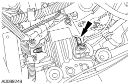
Fig. 144: Locating Transaxle Mount Bolt Courtesy of FORD MOTOR CO.
