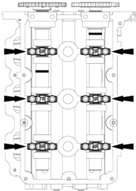
Fig. 246: Locating Camshaft Bearing Caps Installing Sequence Courtesy of FORD MOTOR CO.
