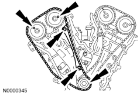
Fig. 54: Aligning Marks On Timing Chain With Marks On Camshaft And Crankshaft Sprockets Courtesy of FORD MOTOR CO.
