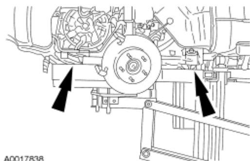
Fig. 335: Positioning Powertrain Into Vehicle Courtesy of FORD MOTOR CO.
