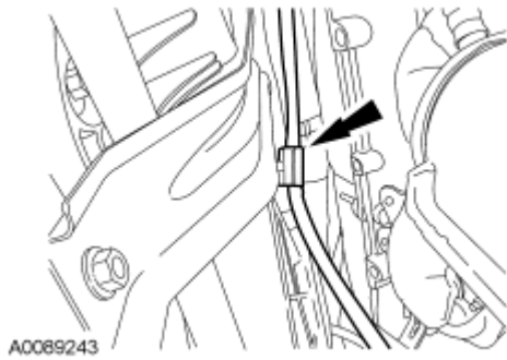
Fig. 136: Locating Heated Oxygen Sensor (HO2S) Wiring Retainer Courtesy of FORD MOTOR CO.
