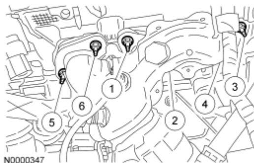
Fig. 291: Right Exhaust Manifold Nuts Tightening Sequence Courtesy of FORD MOTOR CO.
