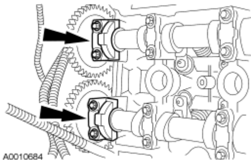
Fig. 244: Locating Camshaft Bearing Thrust Caps Courtesy of FORD MOTOR CO.
