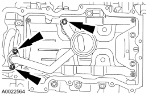
Fig. 196: Locating Oil Pump Screen & Pickup Tube Bolts Courtesy of FORD MOTOR CO.
