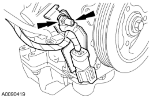
Fig. 318: Locating Heated Oxygen Sensor (HO2S) Electrical Connector Bracket Courtesy of FORD MOTOR CO.
