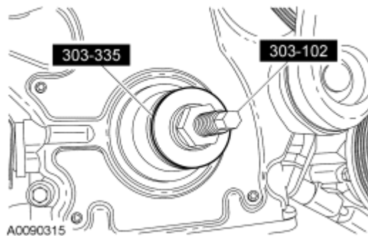
Fig. 272: Installing Crankshaft Seal Using Special Tools (303-335 And 303-102) Courtesy of FORD MOTOR CO.
