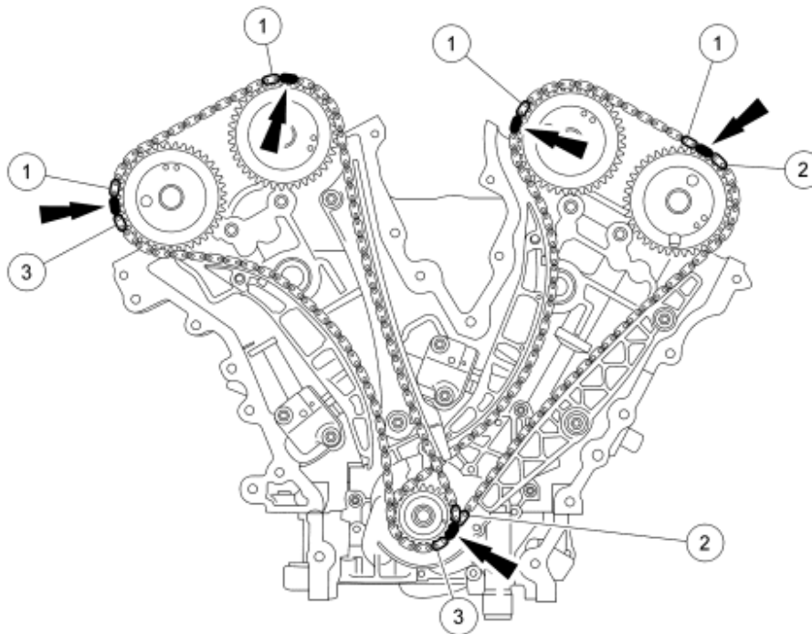
Fig. 265: Checking Chain Links Timing Marks Courtesy of FORD MOTOR CO.
