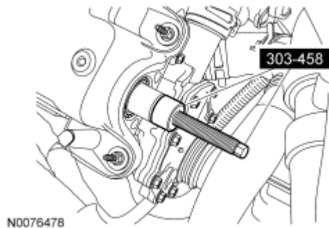
Fig. 251: Installing Special Tool On Camshaft Courtesy of FORD MOTOR CO.
