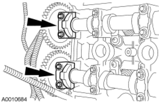
Fig. 247: Locating Camshaft Bearing Thrust Caps Courtesy of FORD MOTOR CO.
