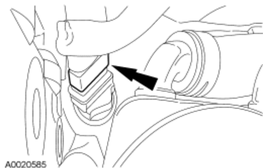
Fig. 135: Locating Engine Block Heater Electrical Connector Courtesy of FORD MOTOR CO.
