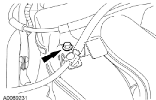
Fig. 117: Cable Bracket Courtesy of FORD MOTOR CO.
