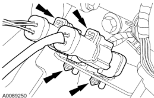
Fig. 146: Locating Heated Oxygen & Catalyst Monitor Sensor Electrical Connectors Courtesy of FORD MOTOR CO.
