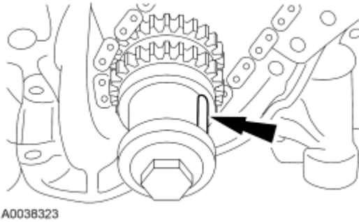
Fig. 52: Locating Crankshaft Keyway Courtesy of FORD MOTOR CO.
