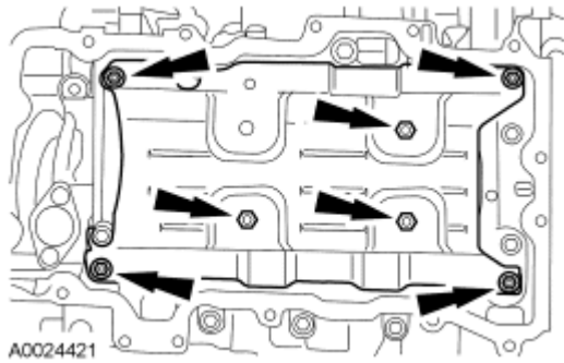
Fig. 278: Locating Oil Pan Baffle And Nuts Courtesy of FORD MOTOR CO.
