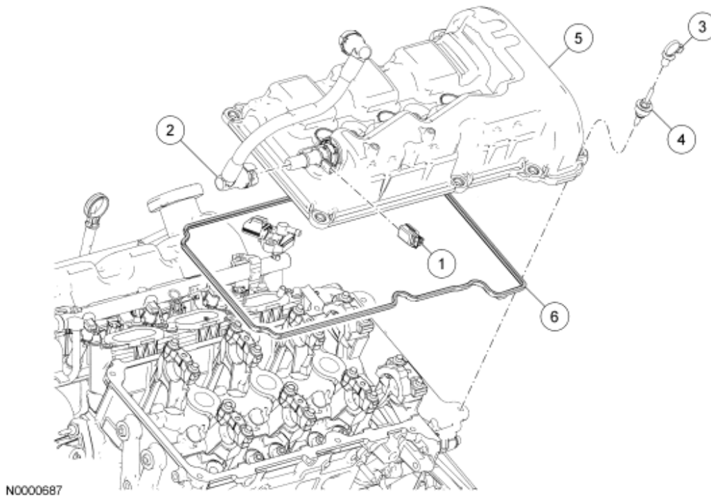
Fig. 11: Exploded View Of Right Valve Cover Courtesy of FORD MOTOR CO.
