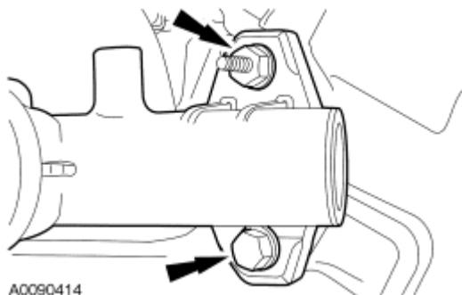
Fig. 283: Locating Coolant Bypass Tube Bolts Courtesy of FORD MOTOR CO.
