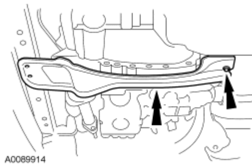
Fig. 112: Identifying Cross Brace And Rear Nut Courtesy of FORD MOTOR CO.
