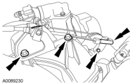
Fig. 116: Accelerator Cable, Speed Control Actuator Cable & Cable Bracket Bolts Courtesy of FORD MOTOR CO.
