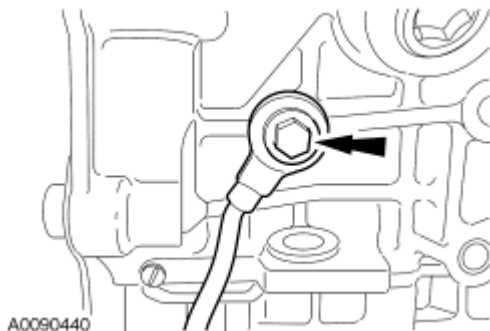
Fig. 200: Locating Knock Sensor (KS) & Bolt Courtesy of FORD MOTOR CO.
