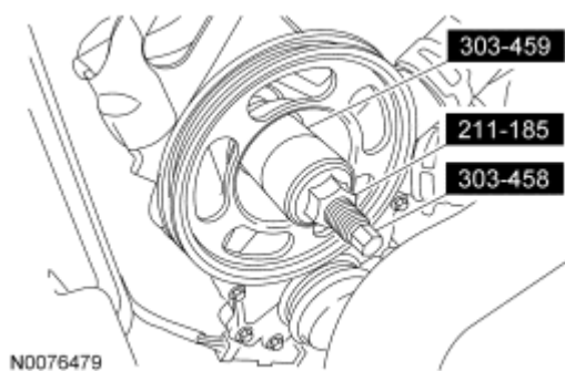
Fig. 252: Installing Coolant Pump Pulley Courtesy of FORD MOTOR CO.
