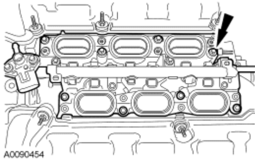
Fig. 177: Locating Lower Intake Manifold Bolts Courtesy of FORD MOTOR CO.
