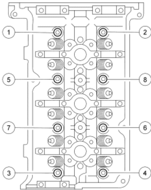
Fig. 88: Identifying Loosening Sequence Of Cylinder Head Bolts Courtesy of FORD MOTOR CO.
