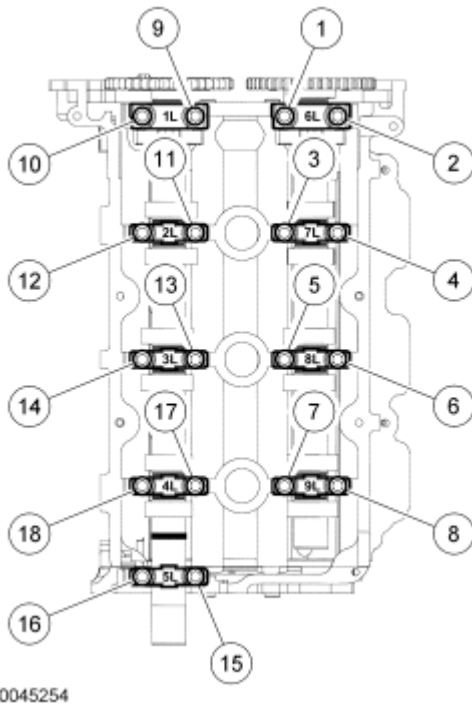
Fig. 70: Identifying Tightening Sequence Of Bolts Courtesy of FORD MOTOR CO.
