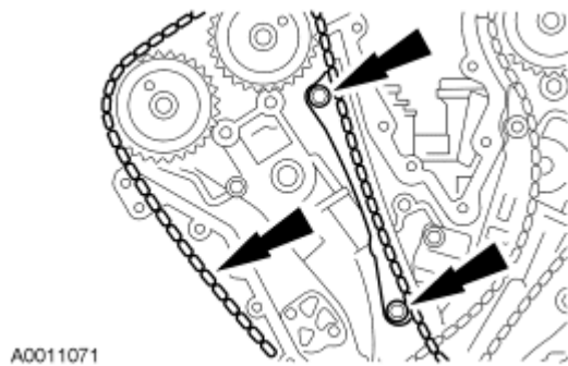
Fig. 214: Locating Timing Chain Guide & Bolts Courtesy of FORD MOTOR CO.
