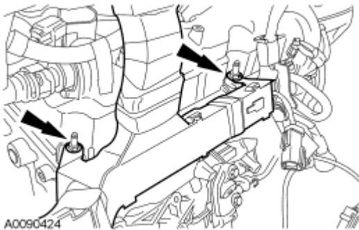
Fig. 163: Locating Engine Control Wiring Harness & Nuts Courtesy of FORD MOTOR CO.
