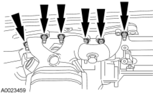
Fig. 183: Locating Gasket & Nuts Courtesy of FORD MOTOR CO.
