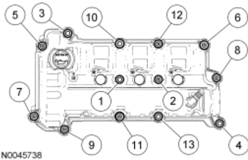
Fig. 296: Identifying Tightening Sequence Of Valve Cover Bolts & Studs Courtesy of FORD MOTOR CO.
