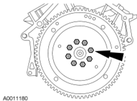
Fig. 157: Locating Flexplate & Bolts Courtesy of FORD MOTOR CO.
