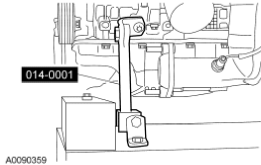
Fig. 325: Securing Engine & Transaxle To Powertrain Lift Using Special Tool (014-0001) Courtesy of FORD MOTOR CO.
