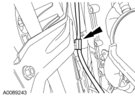
Fig. 347: Locating Heated Oxygen Sensor (HO2S) Wiring Retainer Courtesy of FORD MOTOR CO.
