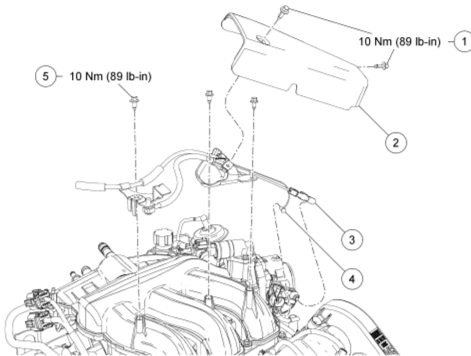
Fig. 2: Exploded View Of Upper Intake Manifold With Torque Specifications (1 Of 3) Courtesy of FORD MOTOR CO.
