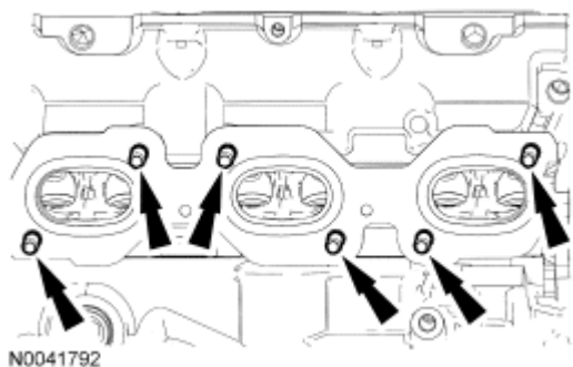
Fig. 290: Locating Exhaust Manifold Studs Courtesy of FORD MOTOR CO.
