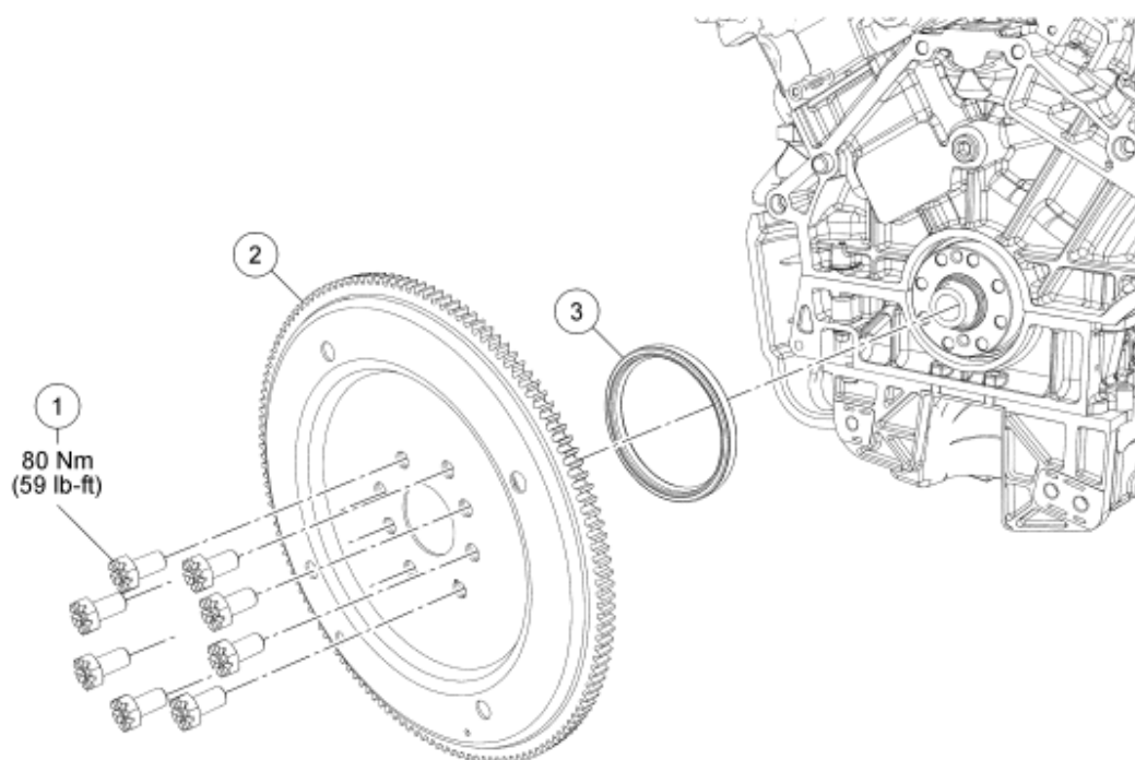
Fig. 14: Exploded View Of Flexplate and Rear Seal Courtesy of FORD MOTOR CO.
