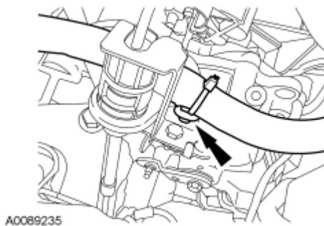
Fig. 120: Locating Pin-Type Retainer Courtesy of FORD MOTOR CO.
