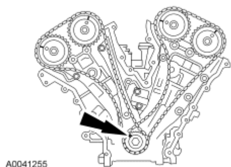
Fig. 210: Identifying Crankshaft Keyway In 11 O'Clock Position Courtesy of FORD MOTOR CO.
