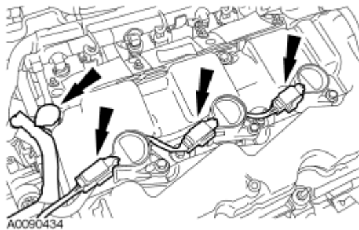
Fig. 308: Locating Coil-On-Plug Electrical Connectors & Wiring Retainers Courtesy of FORD MOTOR CO.
