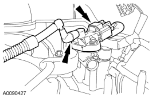
Fig. 303: Locating Fuel Rail Pressure & Temperature Sensor Electrical Connector Courtesy of FORD MOTOR CO.
