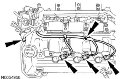
Fig. 306: Coil-On-Plug Electrical Connectors & Wiring Retainers Courtesy of FORD MOTOR CO.
