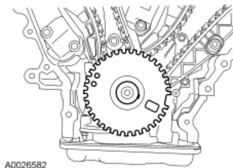
Fig. 31: Identifying Ignition Pulse Wheel Courtesy of FORD MOTOR CO.
