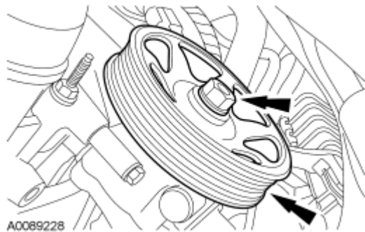
Fig. 108: Locating Power Steering Pump Pulley & Nut Courtesy of FORD MOTOR CO.
