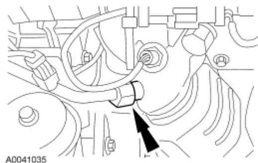
Fig. 114: Locating EGR Tube-To-RH Catalytic Converter Fitting Courtesy of FORD MOTOR CO.
