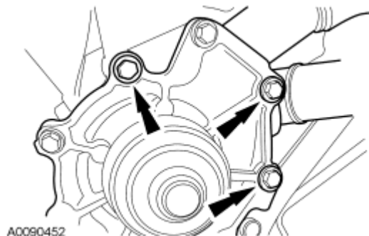
Fig. 285: Locating Coolant Pump & Bolts Courtesy of FORD MOTOR CO.
