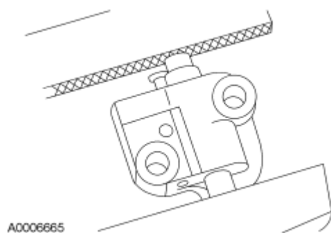
Fig. 255: Identifying Chain Tensioner In Soft-Jawed Vise Courtesy of FORD MOTOR CO.
