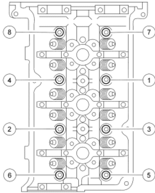
Fig. 89: Identifying Tightening Sequence Of Cylinder Head Bolts Courtesy of FORD MOTOR CO.
