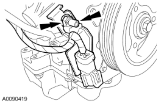
Fig. 160: Locating Heated Oxygen Sensor (HO2S) Electrical Connector Bracket Courtesy of FORD MOTOR CO.
