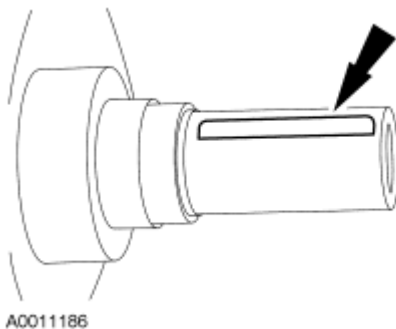
Fig. 237: Locating Crankshaft Key Courtesy of FORD MOTOR CO.
