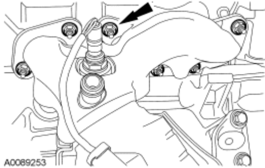
Fig. 151: Locating Nuts & Gasket Courtesy of FORD MOTOR CO.
