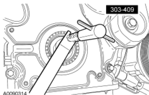
Fig. 203: Removing Crankshaft Front Seal Using Special Tool (303-409) Courtesy of FORD MOTOR CO.
