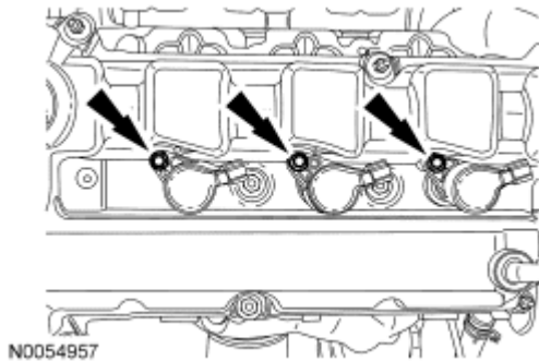
Fig. 300: Coil-On-Plug Bolts Courtesy of FORD MOTOR CO.
