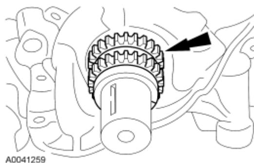
Fig. 254: Locating Crankshaft Sprockets With Timing Marks Out Courtesy of FORD MOTOR CO.
