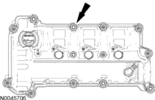
Fig. 182: Locating LH Valve Cover Bolts Courtesy of FORD MOTOR CO.
