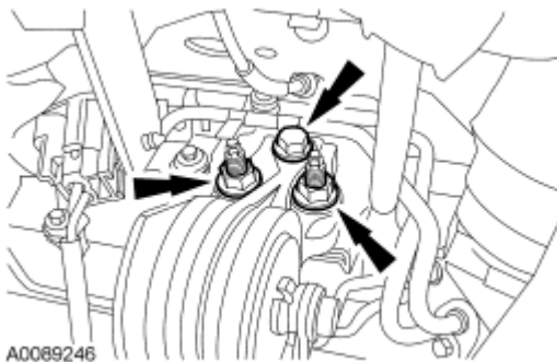
Fig. 143: Locating Transaxle Support Insulator Bolt & Nuts Courtesy of FORD MOTOR CO.
