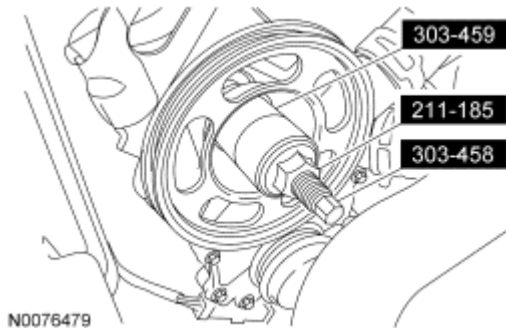
Fig. 74: Installing Coolant Pump Pulley Courtesy of FORD MOTOR CO.
