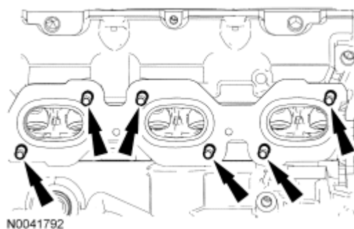
Fig. 407: Locating Exhaust Manifold Studs Courtesy of FORD MOTOR CO.
