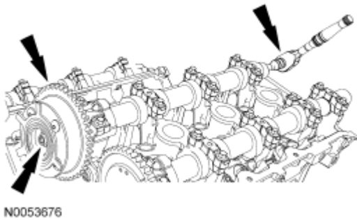
Fig. 323: Locating VCT Actuator And Bolt Courtesy of FORD MOTOR CO.
