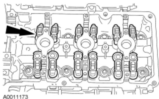
Fig. 330: Locating Camshaft Roller Followers Courtesy of FORD MOTOR CO.
