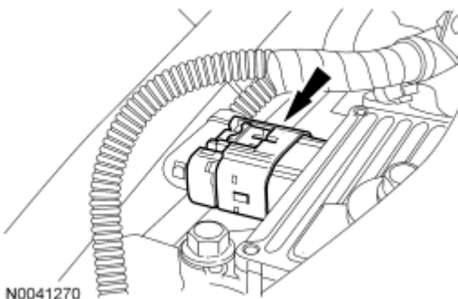
Fig. 472: Locating Transmission Control Module (TCM) Electrical Connector Courtesy of FORD MOTOR CO.
