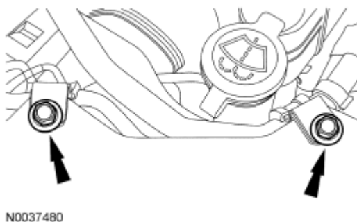
Fig. 178: Locating A/C Tube Bracket Bolts Courtesy of FORD MOTOR CO.
