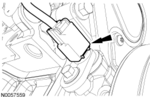
Fig. 254: Identifying Crankshaft Position (CKP) Sensor Electrical Connector Courtesy of FORD MOTOR CO.
