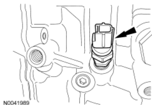
Fig. 289: Locating EOP Switch Courtesy of FORD MOTOR CO.
