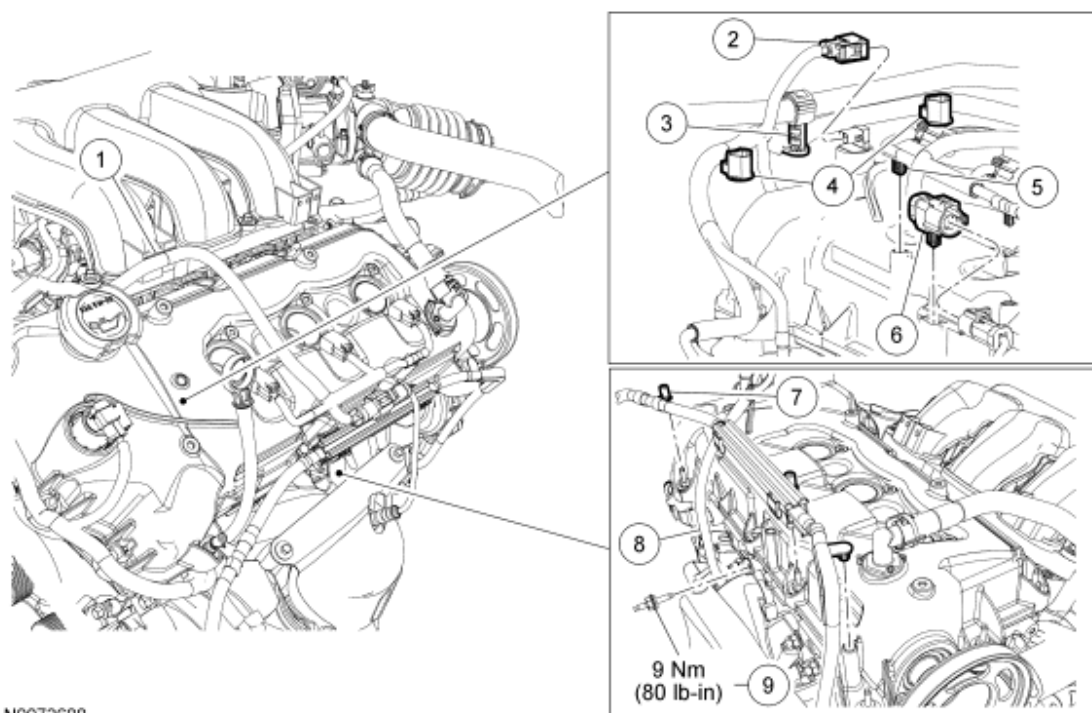
Fig. 7: Exploded View Of LH Valve Cover With Torque Specification (1 Of 2) Courtesy of FORD MOTOR CO.
