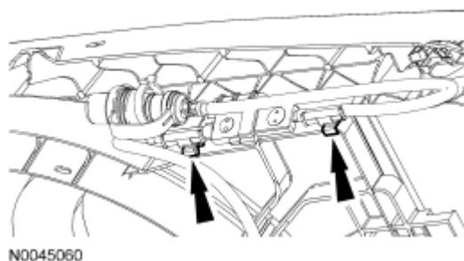
Fig. 173: Locating Block Heater Cable Retaining Clips Courtesy of FORD MOTOR CO.
