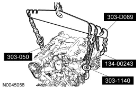
Fig. 456: Identifying Special Tools (134-00243, 303-050, 303-1140, 303-D089) Courtesy of FORD MOTOR CO.
