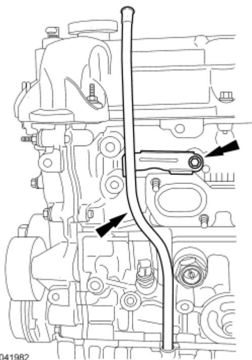
Fig. 405: Locating Oil Level Indicator Tube And Bolt Courtesy of FORD MOTOR CO.
