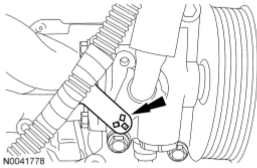
Fig. 426: Locating Wiring Harness Retainer Courtesy of FORD MOTOR CO.
