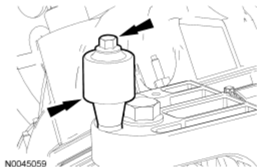
Fig. 489: Locating Damper And Bolt Courtesy of FORD MOTOR CO.
