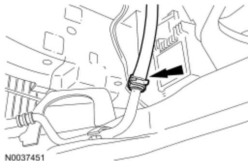
Fig. 541: Locating Power Steering Cooler Tube Courtesy of FORD MOTOR CO.
