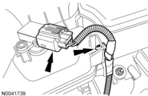
Fig. 447: Locating Manifold Actual Pressure Sensor Electrical Connector And Pin-Type Retainer Courtesy of FORD MOTOR CO.
