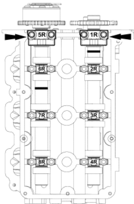
Fig. 348: Locating Camshaft Bearing Thrust Caps Courtesy of FORD MOTOR CO.
