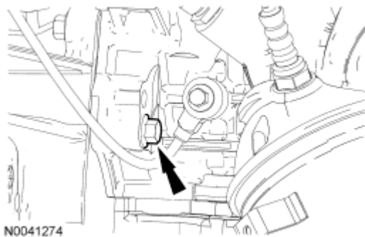
Fig. 224: Locating Engine-To-Transaxle Bolt Courtesy of FORD MOTOR CO.
