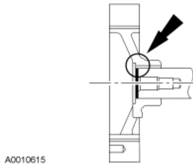
Fig. 379: Applying Silicone Gasket And Sealant Courtesy of FORD MOTOR CO.
