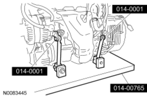
Fig. 476: Installing Engine Lifting Bracket Set & Powertrain Lift To Engine Courtesy of FORD MOTOR CO.
