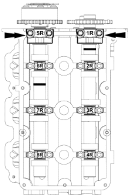
Fig. 93: Locating Camshaft Bearing Thrust Caps Courtesy of FORD MOTOR CO.
