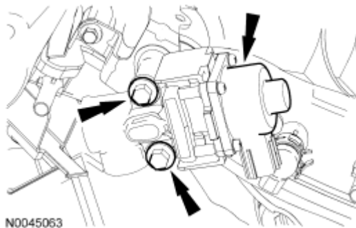
Fig. 480: Locating EGR Valve And Bolts Courtesy of FORD MOTOR CO.
