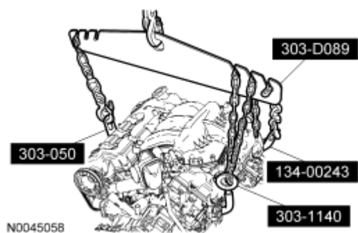
Fig. 452: Identifying Special Tools (134-00243, 303-050, 303-1140, 303-D089) Courtesy of FORD MOTOR CO.
