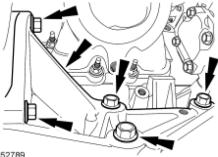
Fig. 494: Identifying PTU Support Bracket Bolts Courtesy of FORD MOTOR CO.
