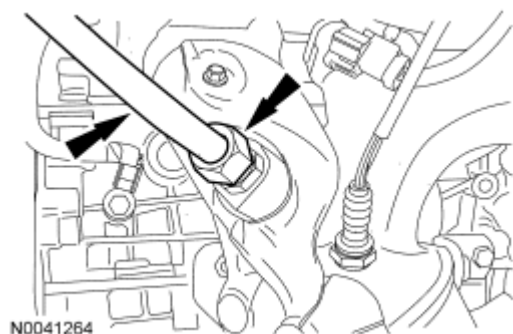
Fig. 212: Locating EGR Tube-To-Catalytic Converter Nut And EGR Tube Courtesy of FORD MOTOR CO.
