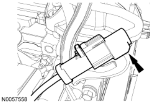
Fig. 427: Identifying RH Catalyst Monitor Sensor Electrical Connector Courtesy of FORD MOTOR CO.
