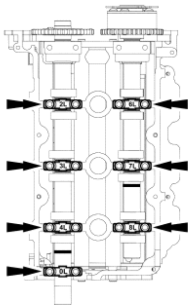
Fig. 352: Loosely Installing Bolts Courtesy of FORD MOTOR CO.
