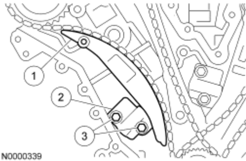
Fig. 60: Identifying Tensioner Arm, Tensioner And Bolts Courtesy of FORD MOTOR CO.
