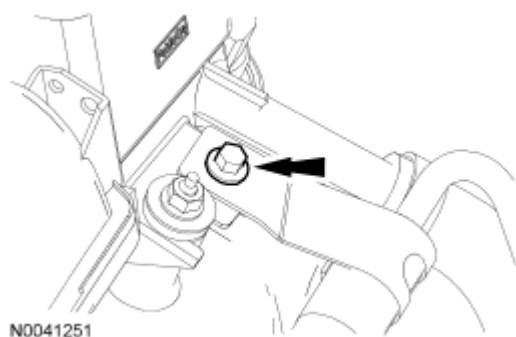
Fig. 206: Locating Power Steering Pressure Hose Bracket-To-Power Steering Reservoir Bolt Courtesy of FORD MOTOR CO.
