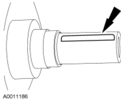
Fig. 322: Locating Crankshaft Key Courtesy of FORD MOTOR CO.
