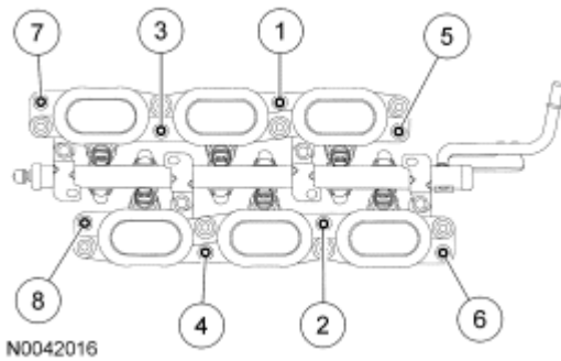
Fig. 407: Identifying Tightening Sequence Of Lower Intake Manifold Bolts Courtesy of FORD MOTOR CO.
