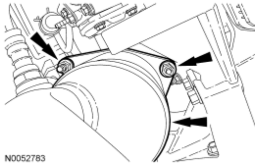
Fig. 193: Locating RH Catalytic Converter Nuts Courtesy of FORD MOTOR CO.
