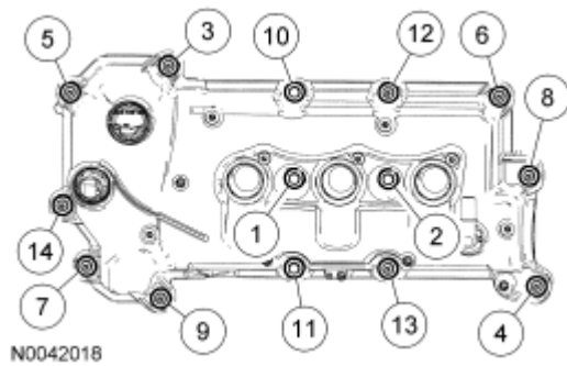
Fig. 10: Identifying Tightening Sequence Of Valve Cover Bolts Courtesy of FORD MOTOR CO.
