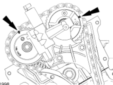
Fig. 37: Locating RH Camshafts In Neutral Position Courtesy of FORD MOTOR CO.
