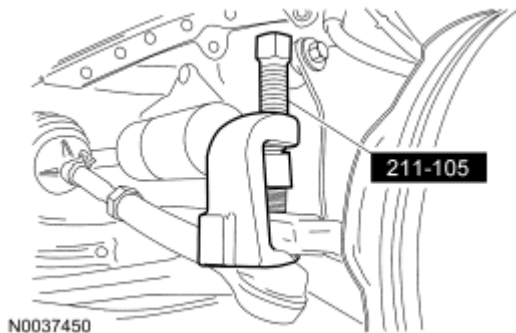
Fig. 146: Separating Tie-Rod Ends From Wheel Knuckles Using Special Tool (211-105) Courtesy of FORD MOTOR CO.
