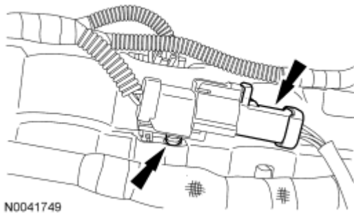
Fig. 472: Locating LH Heated Oxygen Sensor Electrical Connector And Pin-Type Retainer Courtesy of FORD MOTOR CO.
