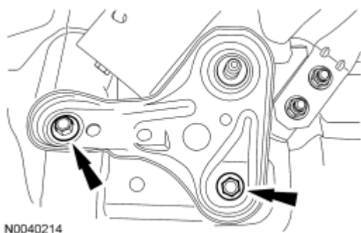
Fig. 542: Locating Subframe Brackets Bolts Courtesy of FORD MOTOR CO.
