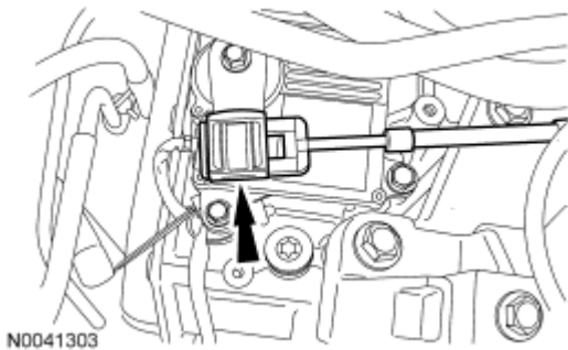
Fig. 167: Locating Transaxle Control Cable To Transaxle Selector Lever Courtesy of FORD MOTOR CO.
