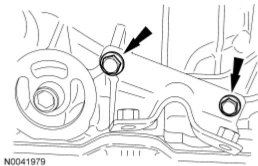
Fig. 281: Locating LH Catalytic Converter Bracket Bolts Courtesy of FORD MOTOR CO.
