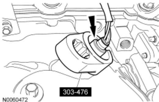
Fig. 189: Identifying RH HO2S & Special Tool (303-476) Courtesy of FORD MOTOR CO.
