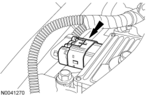
Fig. 223: Locating Transmission Control Module (TCM) Electrical Connector Courtesy of FORD MOTOR CO.
