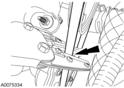
Fig. 285: Locating Coolant Pump Belt Courtesy of FORD MOTOR CO.
