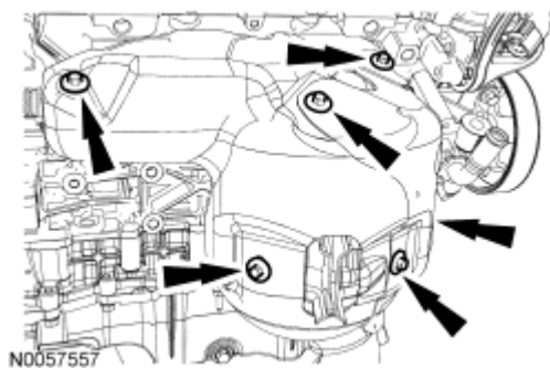
Fig. 190: Locating RH Exhaust Heat Shield Bolts - Outboard Half Courtesy of FORD MOTOR CO.
