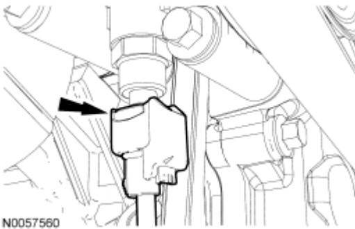
Fig. 258: Identifying Power Steering Pressure (PSP) Switch Electrical Connector Courtesy of FORD MOTOR CO.
