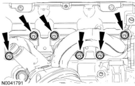
Fig. 274: Locating RH Catalytic Converter Nuts Courtesy of FORD MOTOR CO.
