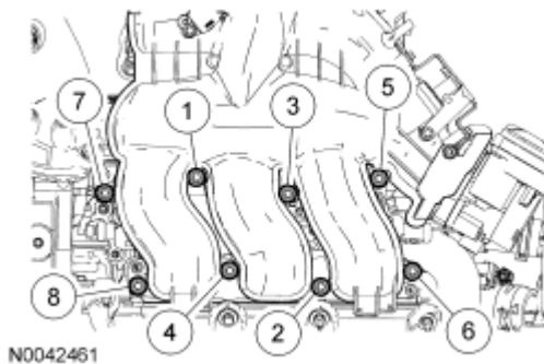
Fig. 446: Identifying Tightening Sequence Of Upper Intake Manifold Bolts Courtesy of FORD MOTOR CO.
