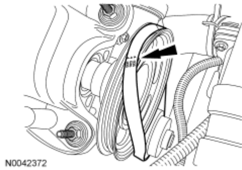
Fig. 402: Locating Coolant Pump Belt On Coolant Pump Pulley Courtesy of FORD MOTOR CO.
