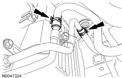
Fig. 539: Locating Transaxle Cooler Hoses Clamps Courtesy of FORD MOTOR CO.
