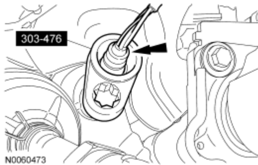
Fig. 187: Identifying RH Catalyst Monitor Sensor & Special Tool (303-476) Courtesy of FORD MOTOR CO.
