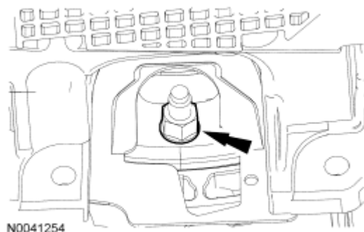
Fig. 495: Locating Torque Converter Nuts Courtesy of FORD MOTOR CO.
