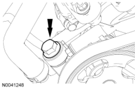
Fig. 209: Locating Banjo Bolt Courtesy of FORD MOTOR CO.
