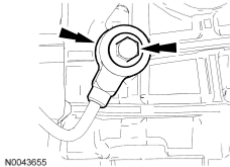
Fig. 398: Locating Knock Sensor (KS) And Bolt Courtesy of FORD MOTOR CO.
