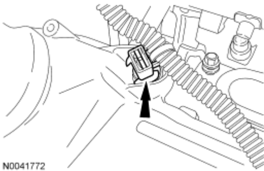
Fig. 437: Locating Wiring Harness Retainer Courtesy of FORD MOTOR CO.
