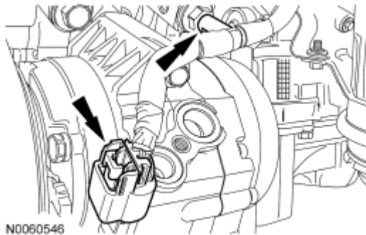
Fig. 445: Identifying A/C Compressor Electrical Connector & Wiring Harness Retainer Courtesy of FORD MOTOR CO.
