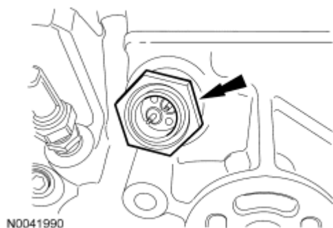
Fig. 293: Locating Block Heater Courtesy of FORD MOTOR CO.
