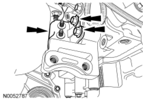
Fig. 192: Locating RH Exhaust Heat Shield Bracket Bolts Courtesy of FORD MOTOR CO.
