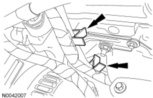
Fig. 242: Locating Block Heater Wiring Harness Retainers Courtesy of FORD MOTOR CO.
