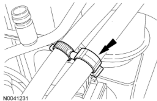
Fig. 176: Locating Coolant Hose Retaining Clip Courtesy of FORD MOTOR CO.
