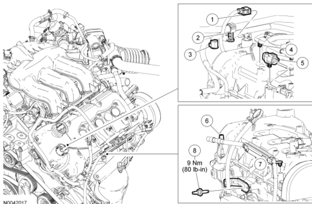
Fig. 7: Exploded View Of Valve Cover With Torque Specification - LH (1 Of 2) Courtesy of FORD MOTOR CO.
