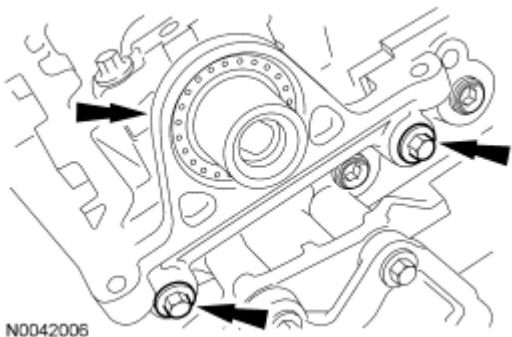
Fig. 359: Locating Camshaft Oil Seal Retainer And Bolts Courtesy of FORD MOTOR CO.
