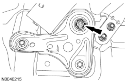
Fig. 543: Locating Subframe Nuts Courtesy of FORD MOTOR CO.
