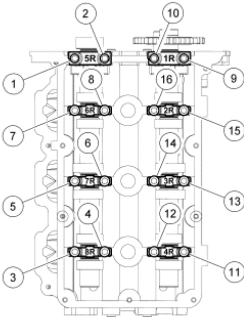
Fig. 332: Identifying Loosening Sequence Of Camshaft Bearing Bolts Courtesy of FORD MOTOR CO.
