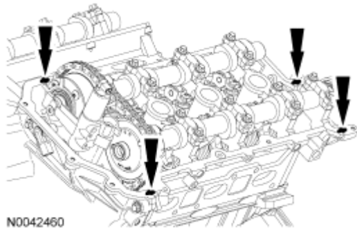
Fig. 390: Locating Silicone Gasket Sealant Courtesy of FORD MOTOR CO.
