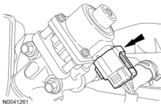
Fig. 211: Locating Exhaust Gas Recirculation Valve Electrical Connector Courtesy of FORD MOTOR CO.
