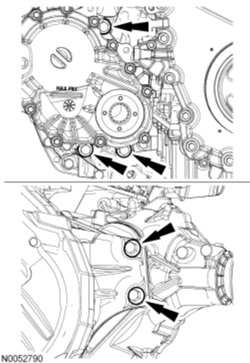
Fig. 196: Locating PTU Bolts Courtesy of FORD MOTOR CO.
