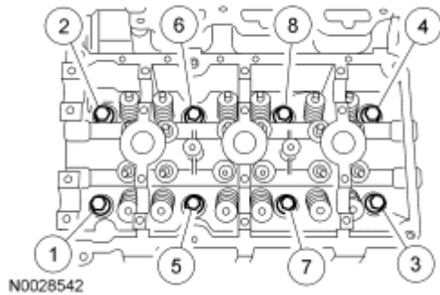
Fig. 334: Identifying Loosening Sequence Of Cylinder Heads Bolts Courtesy of FORD MOTOR CO.
