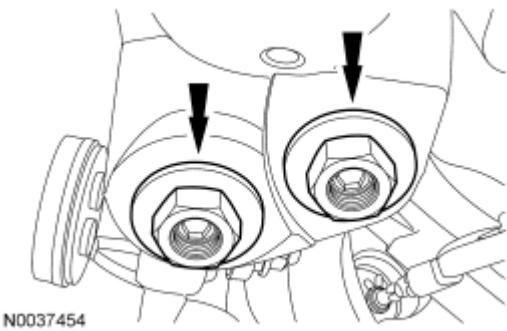
Fig. 148: Locating Lower Ball Joint Nuts Courtesy of FORD MOTOR CO.
