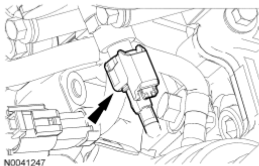
Fig. 183: Locating Power Steering Pressure (PSP) Switch Electrical Connector Courtesy of FORD MOTOR CO.
