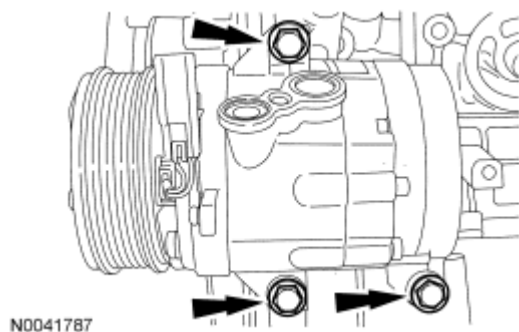
Fig. 272: Locating A/C Compressor Bolts Courtesy of FORD MOTOR CO.
