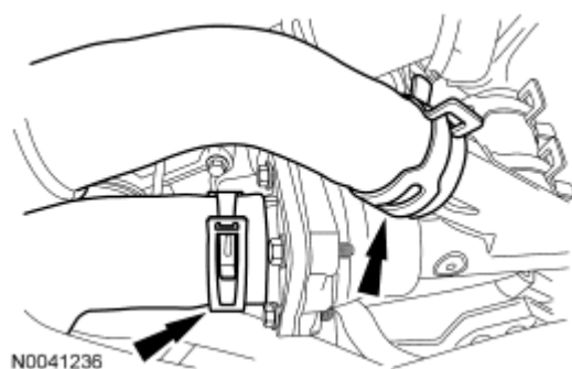
Fig. 529: Locating Upper And Lower Radiator Hoses From Thermostat Housing Courtesy of FORD MOTOR CO.
