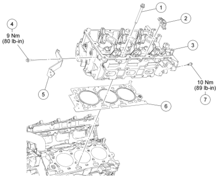
Fig. 105: Exploded View Of Cylinder Head With Torque Specifications - RH
