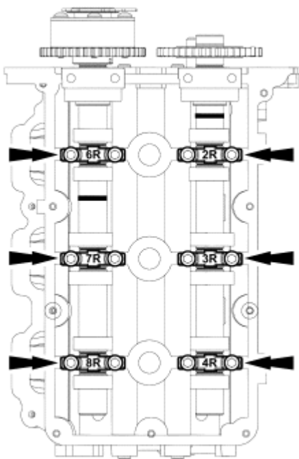
Fig. 350: Locating Camshaft Bearing Caps Courtesy of FORD MOTOR CO.
