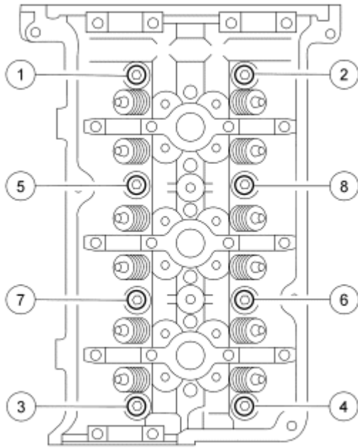
Fig. 110: Identifying Loosening Sequence Of Cylinder Head Bolts Courtesy of FORD MOTOR CO.
