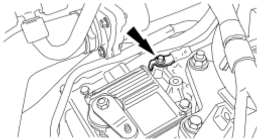
Fig. 221: Identifying Ground Wire Bolt Courtesy of FORD MOTOR CO.
