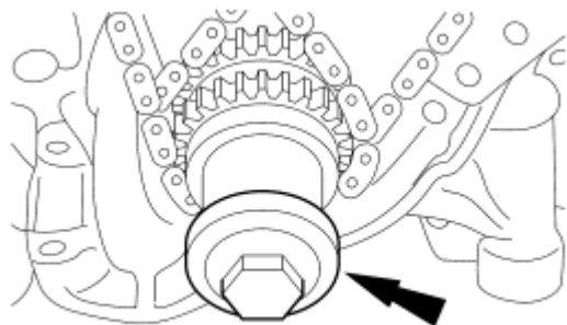
Fig. 377: Identifying Damper Bolt Courtesy of FORD MOTOR CO.
