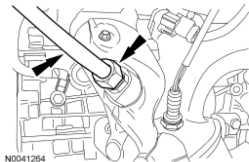
Fig. 214: Locating EGR Tube-To-Catalytic Converter Nut And EGR Tube Courtesy of FORD MOTOR CO.
