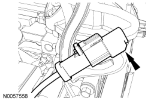
Fig. 431: Identifying RH Catalyst Monitor Sensor Electrical Connector Courtesy of FORD MOTOR CO.
