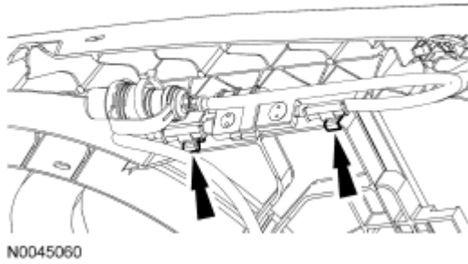
Fig. 172: Locating Block Heater Cable Retaining Clips Courtesy of FORD MOTOR CO.
