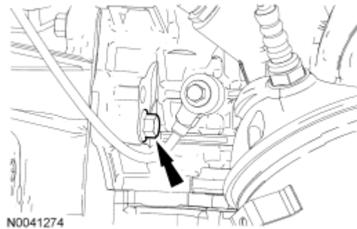
Fig. 464: Locating Engine-To-Transaxle Bolt Courtesy of FORD MOTOR CO.
