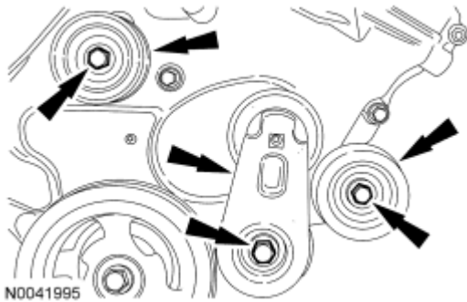
Fig. 385: Locating Accessory Drive Belt Tensioner And Idler Pulleys Courtesy of FORD MOTOR CO.
