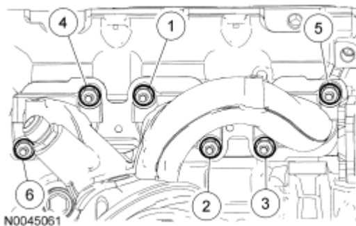
Fig. 413: Identifying Tightening Sequence Of RH Catalytic Converter Nuts
