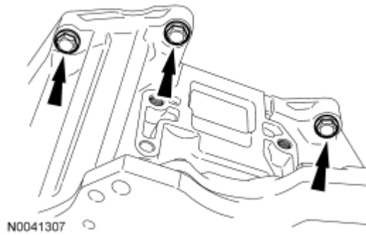
Fig. 463: Locating Transaxle-To-Engine Bolts Courtesy of FORD MOTOR CO.
