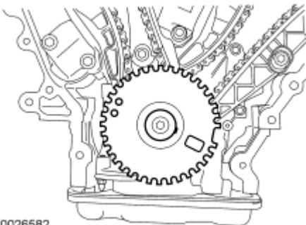
Fig. 306: Identifying Ignition Pulse Wheel Courtesy of FORD MOTOR CO.
