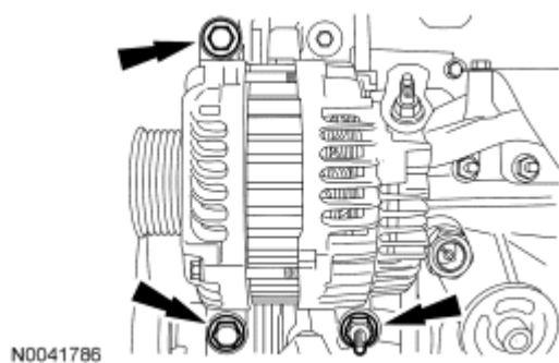
Fig. 416: Locating Generator Bolts Courtesy of FORD MOTOR CO.
