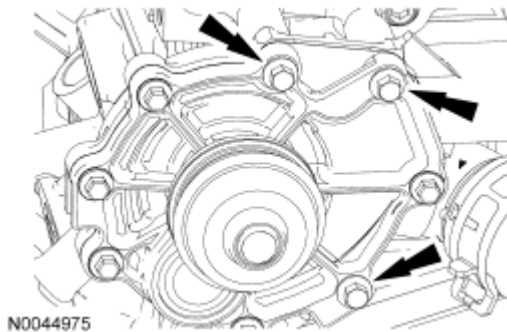
Fig. 109: Locating Coolant Pump Bolts Courtesy of FORD MOTOR CO.
