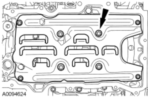
Fig. 300: Locating Oil Pan Baffle Nuts Courtesy of FORD MOTOR CO.
