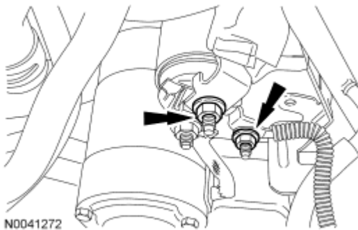
Fig. 475: Locating Starter Motor Wiring Nuts Courtesy of FORD MOTOR CO.
