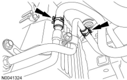
Fig. 155: Locating Transaxle Cooler Hoses Clamps Courtesy of FORD MOTOR CO.
