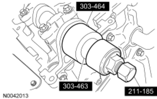
Fig. 360: Identifying Special Tools (303-463, 303-464 And 211-185) Courtesy of FORD MOTOR CO.
