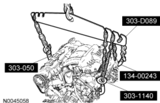
Fig. 220: Identifying Special Tools (134-00243, 303-050, 303-1140, 303-D089) Courtesy of FORD MOTOR CO.
