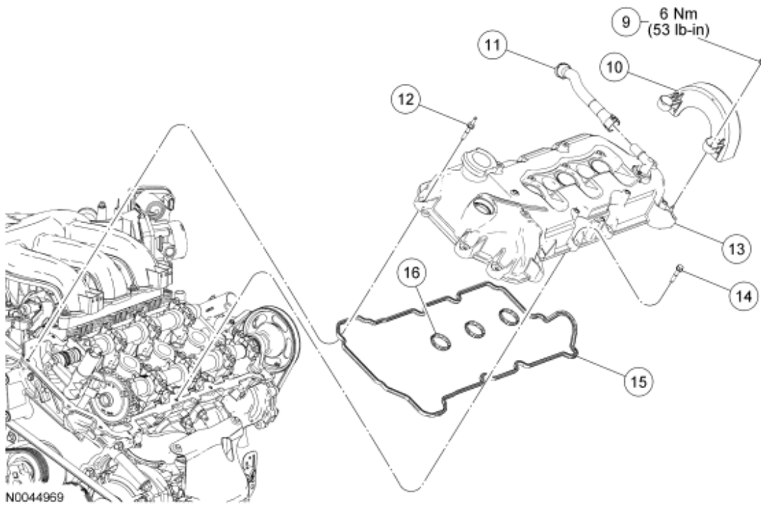
Fig. 8: Exploded View Of Valve Cover With Torque Specification - LH (2 Of 2) Courtesy of FORD MOTOR CO.
