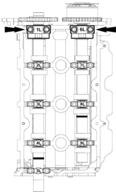
Fig. 356: Locating Camshaft Bearing Thrust Caps Courtesy of FORD MOTOR CO.
