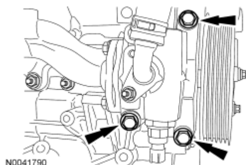
Fig. 419: Locating Power Steering Pump Bolts Courtesy of FORD MOTOR CO.
