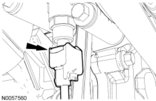
Fig. 428: Identifying Power Steering Pressure (PSP) Switch Electrical Connector Courtesy of FORD MOTOR CO.
