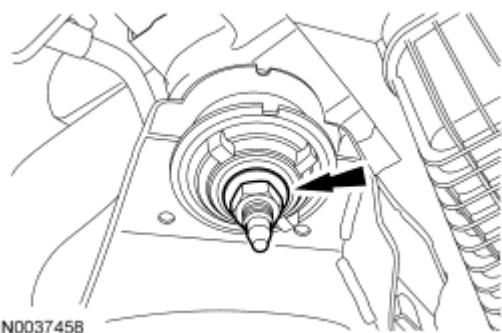
Fig. 541: Locating Front Subframe Nut Courtesy of FORD MOTOR CO.
