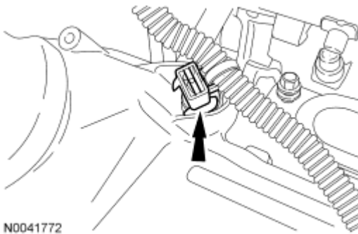
Fig. 249: Locating Wiring Harness Retainer Courtesy of FORD MOTOR CO.
