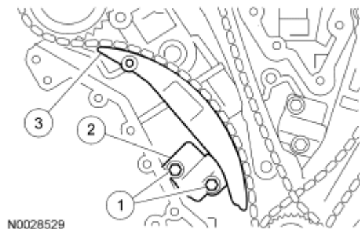
Fig. 312: Identifying RH Timing Chain Tensioner Arm & Bolts Courtesy of FORD MOTOR CO.
