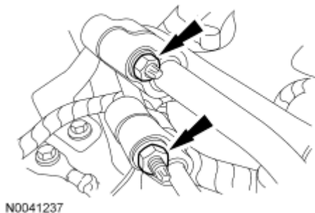
Fig. 517: Locating A/C Tubes And Nuts Courtesy of FORD MOTOR CO.
