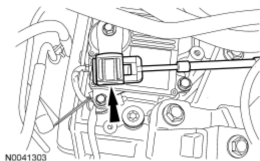
Fig. 528: Locating Transaxle Control Cable To Transaxle Selector Lever Courtesy of FORD MOTOR CO.
