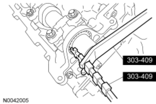
Fig. 69: Identifying Special Tools (303-409) Courtesy of FORD MOTOR CO.
