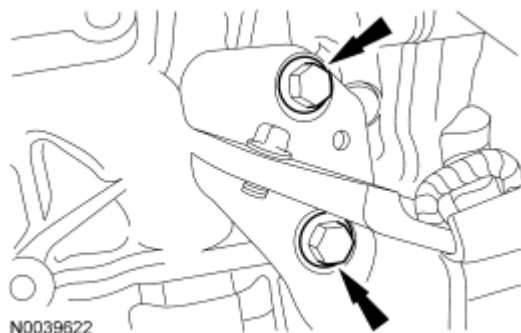
Fig. 509: Locating RH Halfshaft Carrier Bearing Bracket Bolts Courtesy of FORD MOTOR CO.
