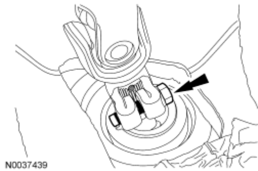
Fig. 560: Locating Steering Intermediate Shaft Bolt Courtesy of FORD MOTOR CO.
