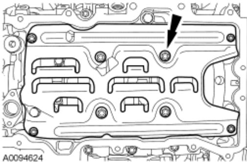
Fig. 386: Locating Oil Pan Baffle Nuts Courtesy of FORD MOTOR CO.
