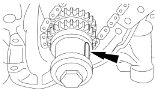
Fig. 371: Locating Crankshaft Keyway Courtesy of FORD MOTOR CO.
