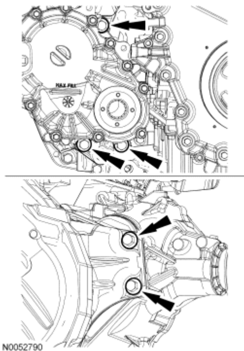
Fig. 497: Locating PTU Bolts Courtesy of FORD MOTOR CO.
