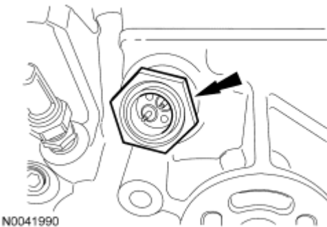
Fig. 396: Locating Block Heater Courtesy of FORD MOTOR CO.
