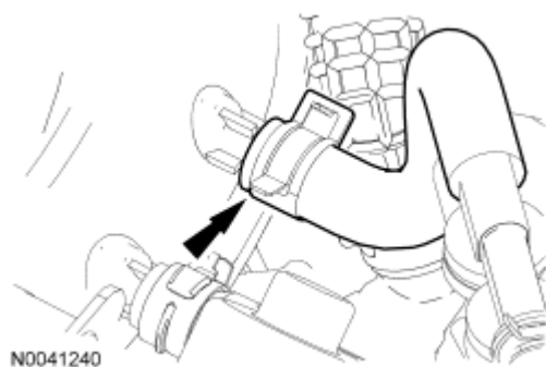
Fig. 524: Locating Vacuum Hose From Intake Manifold Courtesy of FORD MOTOR CO.
