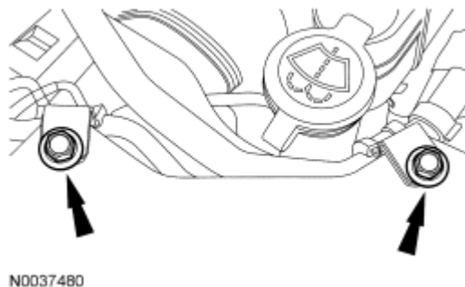
Fig. 177: Locating A/C Tube Bracket Bolts Courtesy of FORD MOTOR CO.
