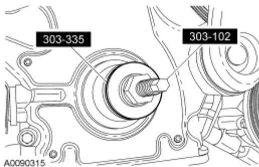
Fig. 381: Installing Crankshaft Seal Using Special Tools (303-335 And 303-102) Courtesy of FORD MOTOR CO.
