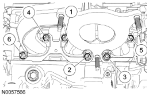
Fig. 412: Identifying Tightening Sequence RH Exhaust Manifold Nuts Courtesy of FORD MOTOR CO.
