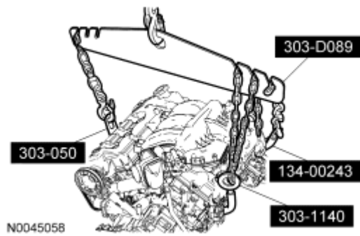
Fig. 460: Identifying Special Tools (134-00243, 303-050, 303-1140, 303-D089) Courtesy of FORD MOTOR CO.
