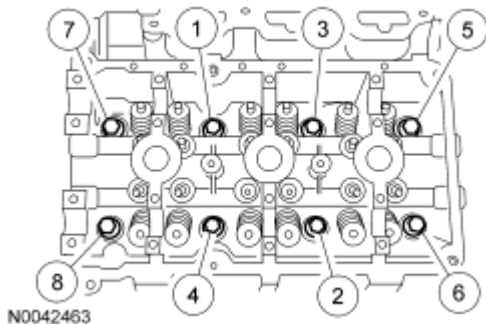
Fig. 343: Identifying Tightening Sequence Of Cylinder Head Bolts Courtesy of FORD MOTOR CO.
