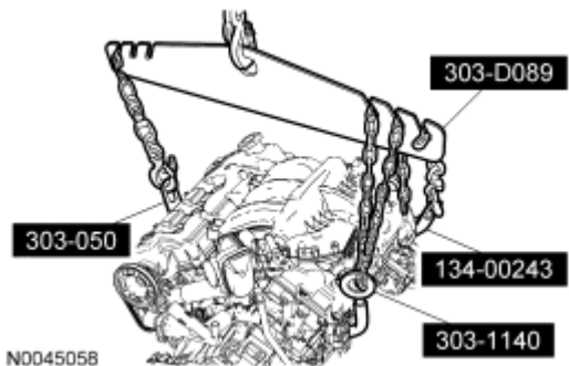
Fig. 479: Identifying Special Tools (134-00243, 303-050, 303-1140, 303-D089) Courtesy of FORD MOTOR CO.
