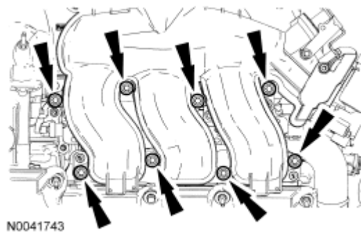
Fig. 239: Locating Upper Intake Manifold Bolts Courtesy of FORD MOTOR CO.
