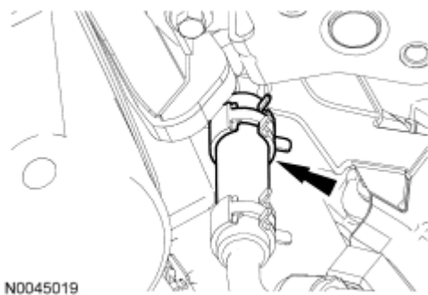
Fig. 530: Locating Evaporative Emissions (EVAP) Hose Courtesy of FORD MOTOR CO.
