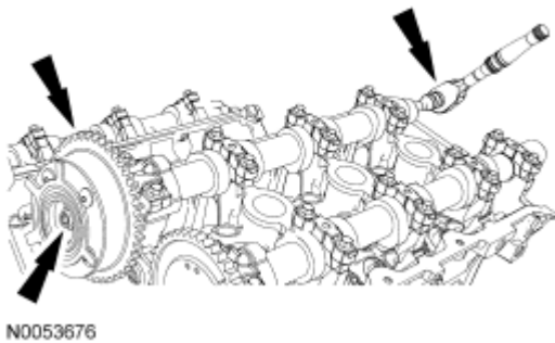
Fig. 358: Locating VCT Actuator And Bolt Courtesy of FORD MOTOR CO.
