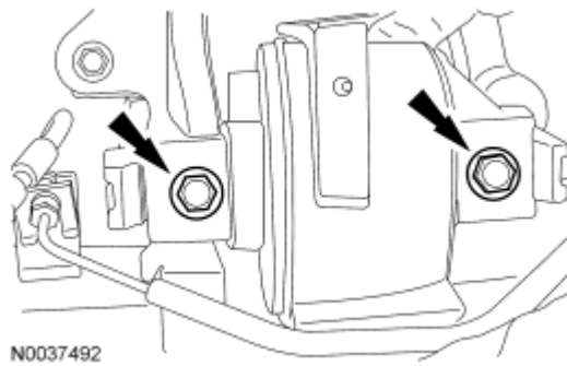
Fig. 201: Locating Transaxle Mount Bolts Courtesy of FORD MOTOR CO.
