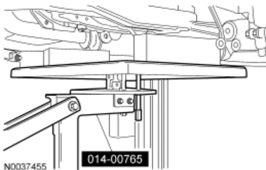
Fig. 540: Positioning Special Tool (014-00765) Under Subframe Assembly Courtesy of FORD MOTOR CO.
