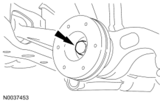
Fig. 150: Locating Lower Control Arms Through Bolt Courtesy of FORD MOTOR CO.
