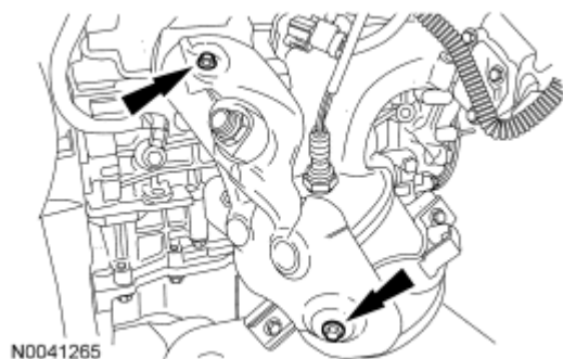
Fig. 215: Locating Heat Shield Bolts Courtesy of FORD MOTOR CO.
