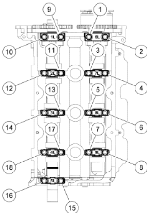
Fig. 357: Identifying Tightening Sequence Camshaft Bearing Cap Bolts
