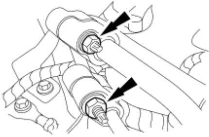
Fig. 178: Locating A/C Tubes And Nuts Courtesy of FORD MOTOR CO.
