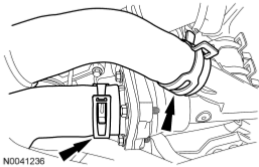
Fig. 166: Locating Upper And Lower Radiator Hoses From Thermostat Housing Courtesy of FORD MOTOR CO.
