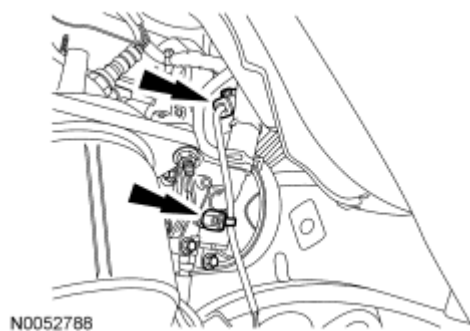
Fig. 507: Locating RH Catalyst Monitor Sensor Electrical Connector & Wiring Retainer Courtesy of FORD MOTOR CO.
