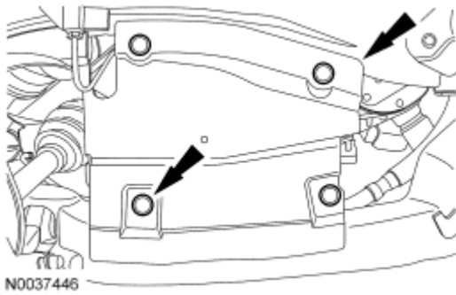
Fig. 552: Locating Splash Shield Pin-Type Retainers Courtesy of FORD MOTOR CO.
