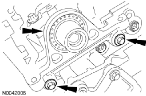
Fig. 324: Locating Camshaft Oil Seal Retainer And Bolts Courtesy of FORD MOTOR CO.
