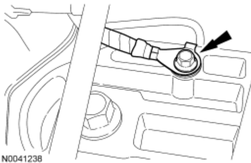
Fig. 179: Locating Ground Wire And Bolt Courtesy of FORD MOTOR CO.
