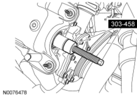
Fig. 400: Installing Special Tool (303-458) On Camshaft Courtesy of FORD MOTOR CO.
