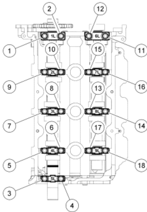
Fig. 74: Identifying Loosening Sequence Of Camshaft Bearing Bolts Courtesy of FORD MOTOR CO.
