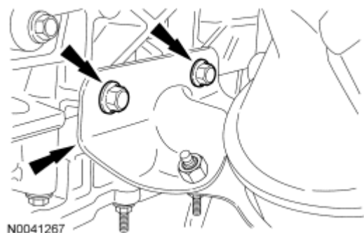
Fig. 217: Locating Catalytic Converter Bracket Assembly Bolts Courtesy of FORD MOTOR CO.
