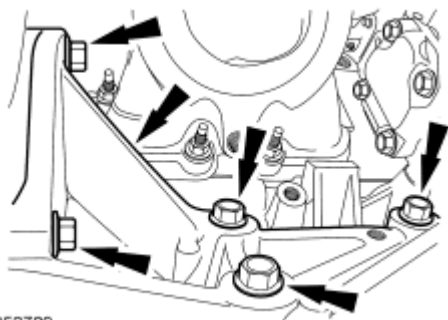
Fig. 195: Identifying PTU Support Bracket Bolts Courtesy of FORD MOTOR CO.
