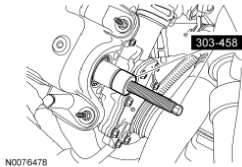
Fig. 83: Installing Special Tool (303-458) On Camshaft Courtesy of FORD MOTOR CO.
