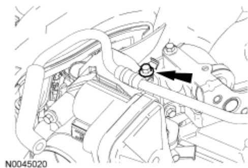
Fig. 525: Locating Vacuum Tube Bracket Bolt Courtesy of FORD MOTOR CO.
