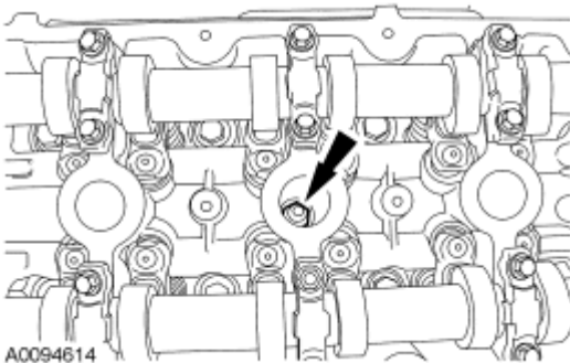
Fig. 389: Locating Spark Plugs Courtesy of FORD MOTOR CO.
