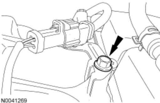
Fig. 222: Locating Catalyst Monitor Sensor (CMS) Electrical Connector Bracket Bolt Courtesy of FORD MOTOR CO.
