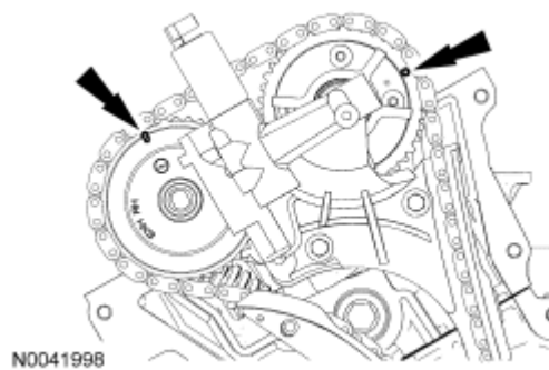
Fig. 311: Locating RH Camshafts In Neutral Position Courtesy of FORD MOTOR CO.
