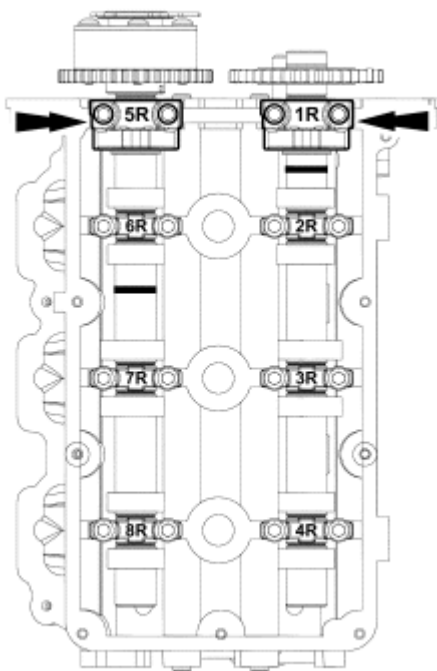
Fig. 351: Locating Camshaft Bearing Thrust Caps Courtesy of FORD MOTOR CO.
