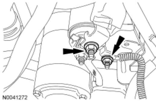
Fig. 224: Locating Starter Motor Wiring Nuts Courtesy of FORD MOTOR CO.
