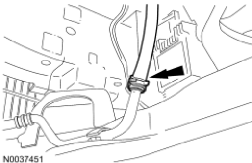
Fig. 138: Locating Power Steering Cooler Tube Courtesy of FORD MOTOR CO.
