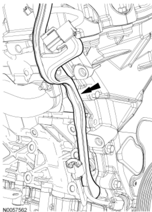
Fig. 417: Identifying Wiring Harness To Cylinder Block Courtesy of FORD MOTOR CO.
