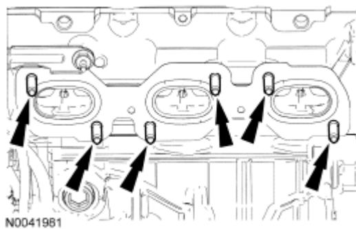
Fig. 280: Locating LH Catalytic Converter Studs Courtesy of FORD MOTOR CO.
