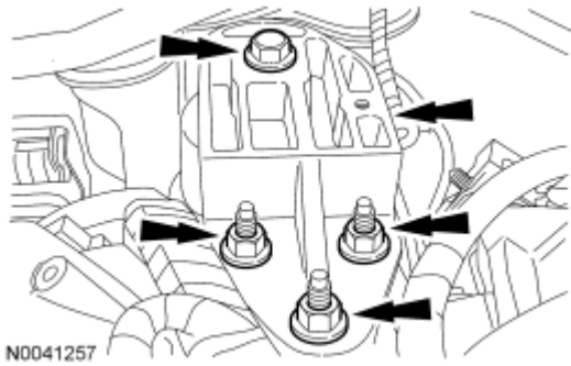
Fig. 203: Locating Engine Mount Bracket, Bolt And Nuts Courtesy of FORD MOTOR CO.
