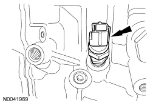
Fig. 292: Locating EOP Switch Courtesy of FORD MOTOR CO.
