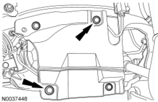
Fig. 137: Locating LH Splash Shield And Pin-Type Retainers Courtesy of FORD MOTOR CO.
