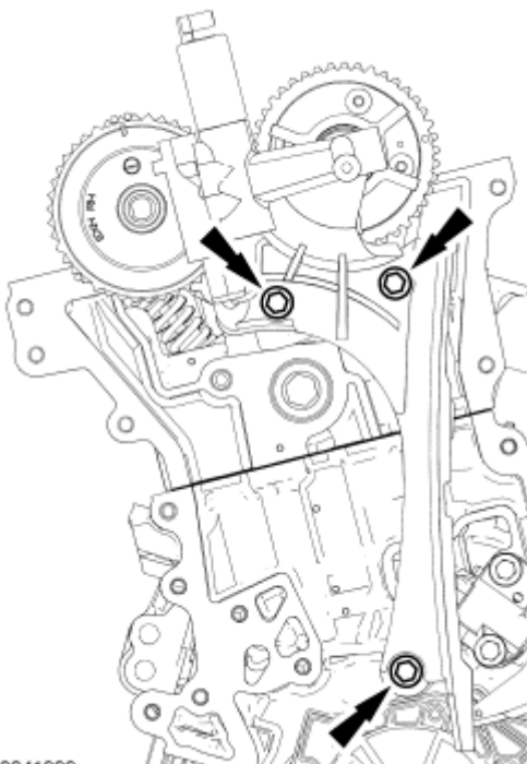
Fig. 314: Locating RH VCT Assembly Bolts
