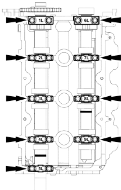
Fig. 327: Marking Camshaft Bearing Cap Position & Orientation Courtesy of FORD MOTOR CO.
