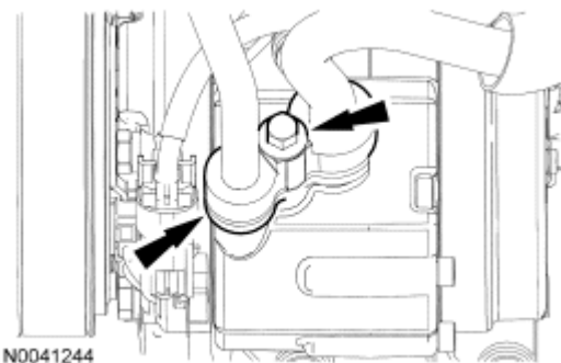
Fig. 180: Locating A/C Manifold And Bolt Courtesy of FORD MOTOR CO.
