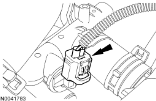
Fig. 423: Locating Electronic Coolant Temperature Sensor Electrical Connector Courtesy of FORD MOTOR CO.
