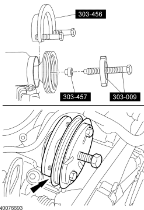
Fig. 289: Removing Coolant Pump Pulley Using Special Tools (303-009, 303-456, 303-457) Courtesy of FORD MOTOR CO.
