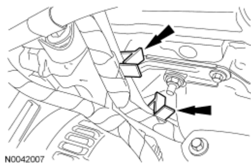
Fig. 443: Locating Block Heater Wiring Harness Retainers Courtesy of FORD MOTOR CO.
