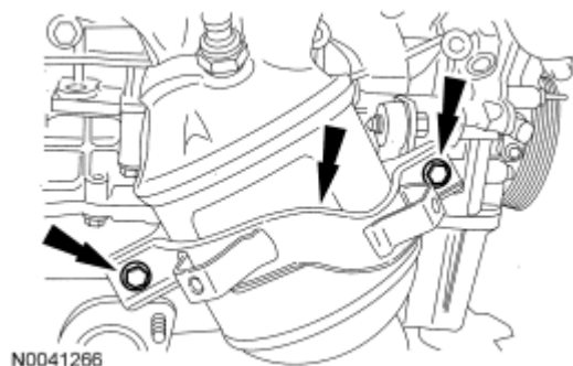
Fig. 216: Locating Catalytic Converter Bracket And Bolts Courtesy of FORD MOTOR CO.
