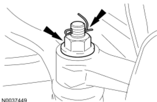
Fig. 549: Locating Tie-Rod Ends Nuts And Cotter Pin Courtesy of FORD MOTOR CO.
