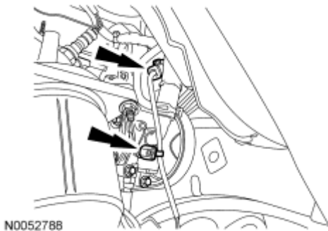
Fig. 186: Locating RH Catalyst Monitor Sensor Electrical Connector & Wiring Retainer Courtesy of FORD MOTOR CO.
