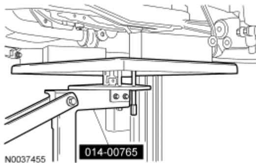
Fig. 151: Positioning Special Tool (014-00765) Under Subframe Assembly Courtesy of FORD MOTOR CO.
