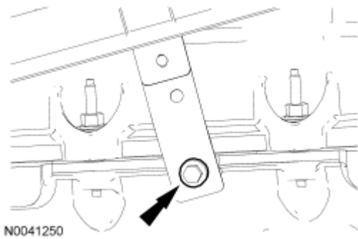
Fig. 207: Locating PSP Hose Bracket To Cylinder Head Bolt Courtesy of FORD MOTOR CO.
