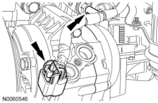
Fig. 240: Identifying A/C Compressor Electrical Connector & Wiring Harness Retainer Courtesy of FORD MOTOR CO.
