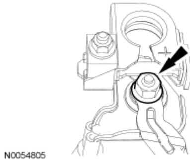
Fig. 158: Locating Power Feed To Battery Terminal And Nut Courtesy of FORD MOTOR CO.
