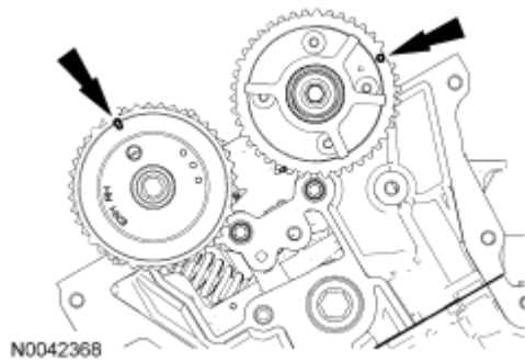
Fig. 329: Locating RH Camshafts Position Courtesy of FORD MOTOR CO.
