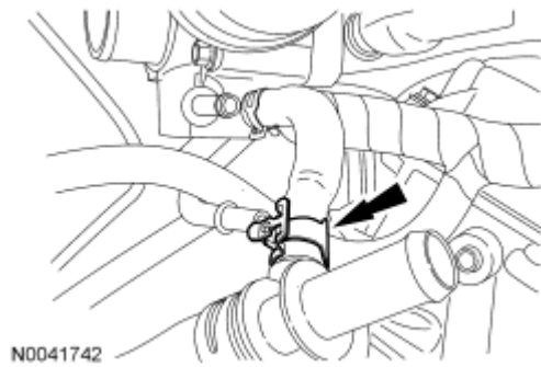
Fig. 447: Locating Throttle Body Coolant Hose Courtesy of FORD MOTOR CO.
