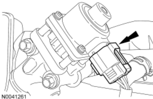
Fig. 486: Locating Exhaust Gas Recirculation Valve Electrical Connector Courtesy of FORD MOTOR CO.
