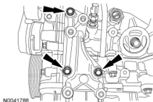
Fig. 273: Locating A/C Compressor Bracket Bolts Courtesy of FORD MOTOR CO.
