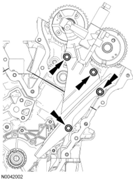
Fig. 368: Identifying LH VCT Assembly Bolts Courtesy of FORD MOTOR CO.
