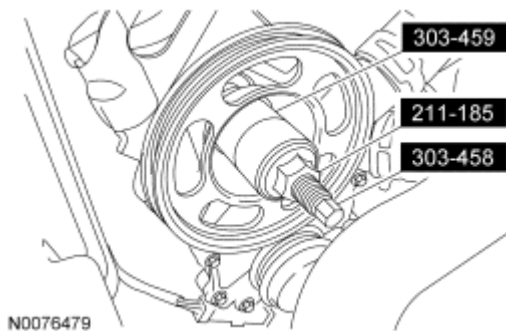
Fig. 401: Installing Coolant Pump Pulley Using Special Tools (211-185, 303-458, 303-459) Courtesy of FORD MOTOR CO.
