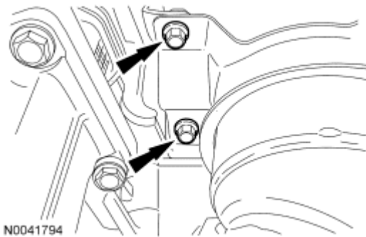
Fig. 278: Locating LH Catalytic Converter Bracket Bolts Courtesy of FORD MOTOR CO.
