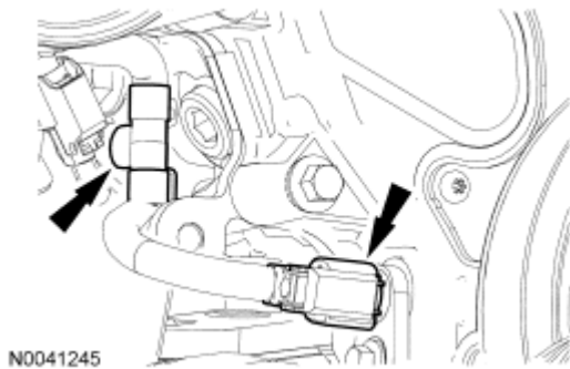
Fig. 182: Locating Crankshaft Position Sensor Electrical Connector And Pin-Type Retainer Courtesy of FORD MOTOR CO.
