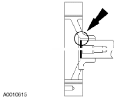
Fig. 382: Applying Silicone Gasket And Sealant Courtesy of FORD MOTOR CO.
