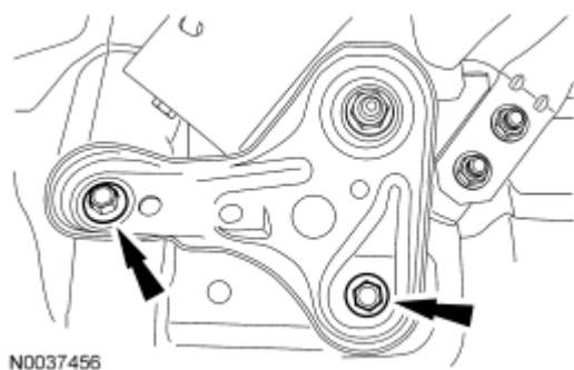
Fig. 152: Locating Subframe Bracket-To-Body Bolts Courtesy of FORD MOTOR CO.
