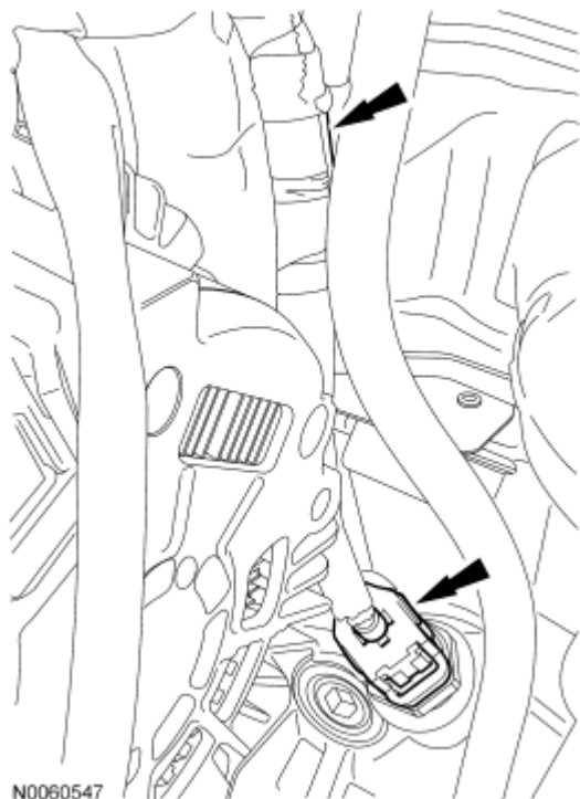
Fig. 442: Identifying Engine Oil Pressure (EOP) Switch Electrical Connector & Wiring Harness Retainer Courtesy of FORD MOTOR CO.
