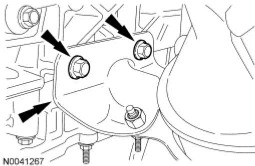
Fig. 481: Locating Catalytic Converter Bracket Assembly Bolts Courtesy of FORD MOTOR CO.
