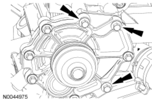
Fig. 399: Locating Coolant Pump Bolts Courtesy of FORD MOTOR CO.
