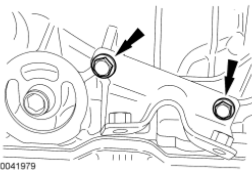
Fig. 410: Locating LH Catalytic Converter Bracket Bolts Courtesy of FORD MOTOR CO.
