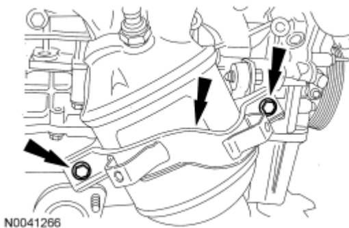
Fig. 482: Locating Catalytic Converter Bracket And Bolts Courtesy of FORD MOTOR CO.
