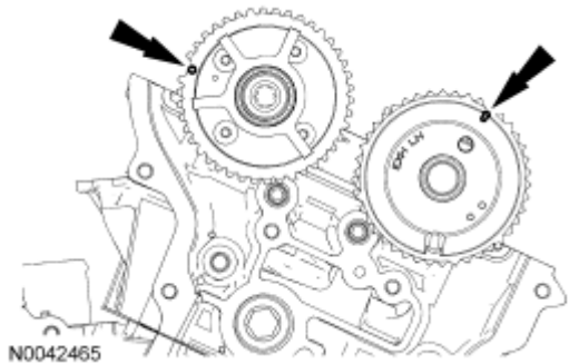
Fig. 325: Locating Camshafts In Neutral Position Courtesy of FORD MOTOR CO.
