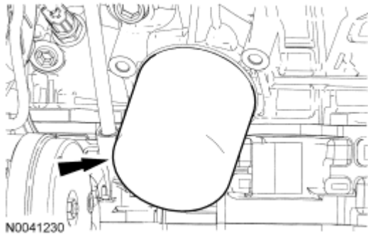
Fig. 538: Locating Engine Oil Filter Courtesy of FORD MOTOR CO.
