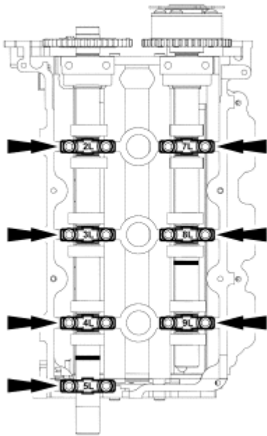
Fig. 355: Locating Camshaft Bearing Caps Courtesy of FORD MOTOR CO.
