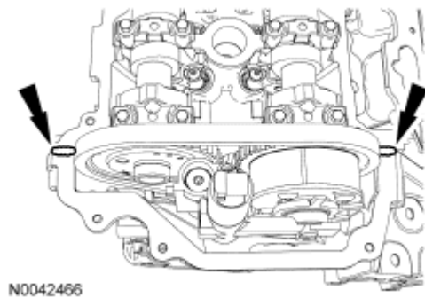
Fig. 393: Locating Silicone Gasket Sealant Courtesy of FORD MOTOR CO.
