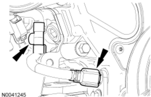
Fig. 512: Locating Crankshaft Position Sensor Electrical Connector And Pin-Type Retainer Courtesy of FORD MOTOR CO.
