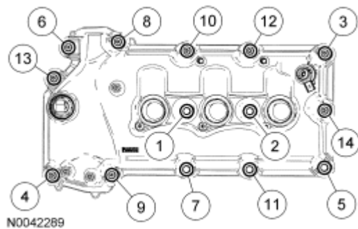
Fig. 394: Identifying Tightening Sequence Of Valve Cover Bolts Courtesy of FORD MOTOR CO.
