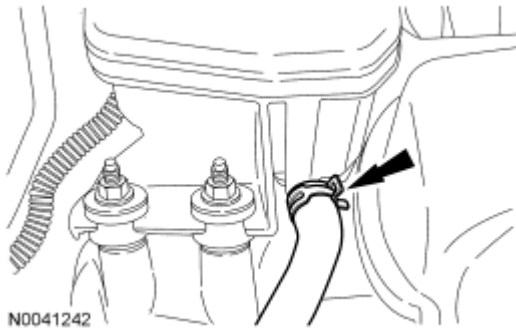
Fig. 173: Locating Power Steering Hose From Power Steering Reservoir Courtesy of FORD MOTOR CO.
