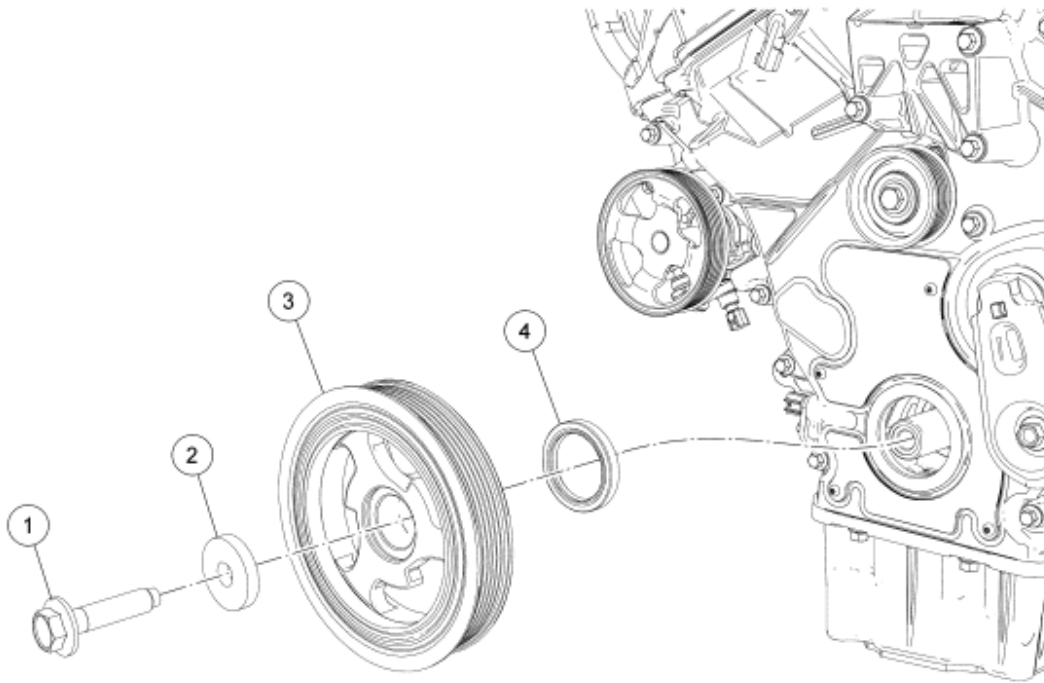
Fig. 17: Exploded View Of Crankshaft Pulley & Crankshaft Front Seal Courtesy of FORD MOTOR CO.
