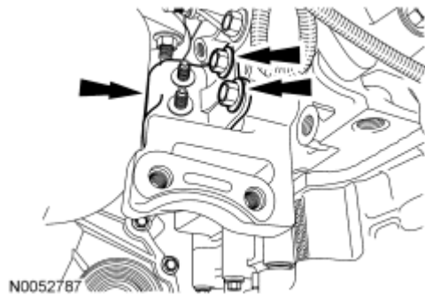
Fig. 501: Locating RH Exhaust Heat Shield Bracket Bolts Courtesy of FORD MOTOR CO.
