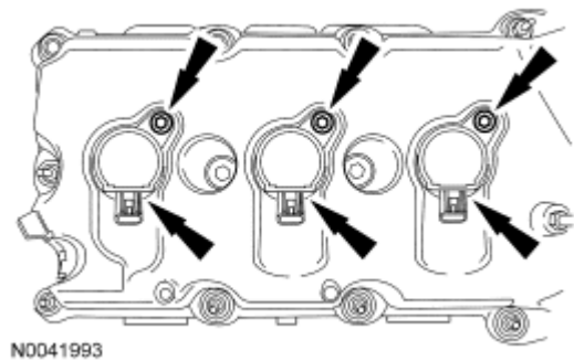
Fig. 296: Locating RH Coil-On-Plug Assemblies And Bolts Courtesy of FORD MOTOR CO.
