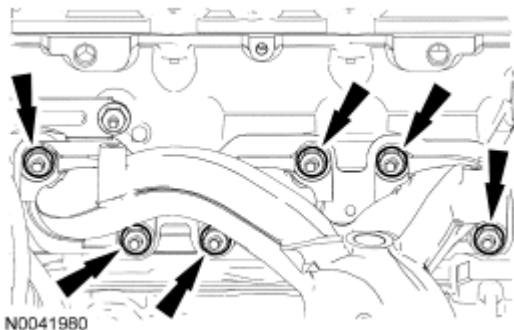
Fig. 279: Locating LH Catalytic Converter Nuts Courtesy of FORD MOTOR CO.
