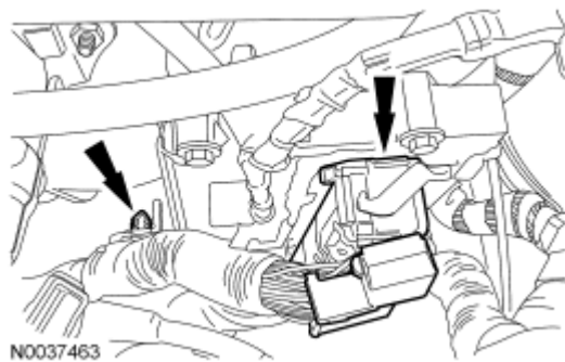
Fig. 534: Locating Powertrain Control Module (PCM) Electrical Connector And Pin-Type Retainer Courtesy of FORD MOTOR CO.
