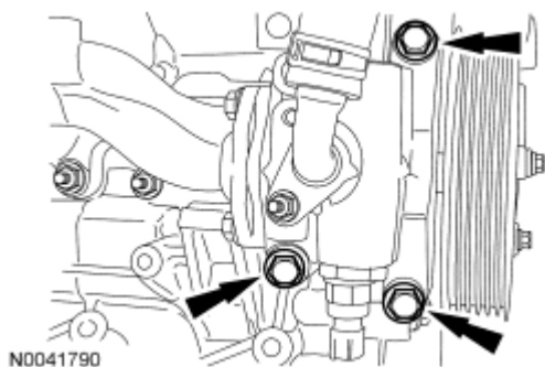
Fig. 268: Locating Power Steering Pump Bolts Courtesy of FORD MOTOR CO.
