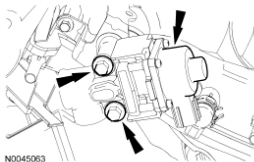
Fig. 484: Locating EGR Valve And Bolts Courtesy of FORD MOTOR CO.
