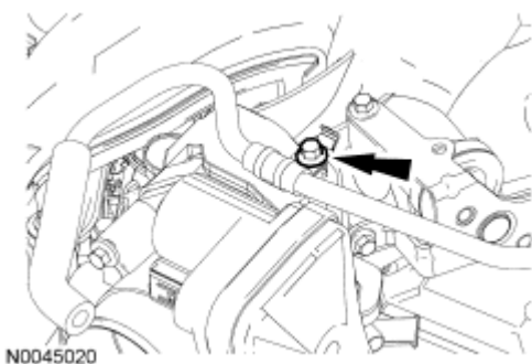
Fig. 170: Locating Vacuum Tube Bracket Bolt Courtesy of FORD MOTOR CO.
