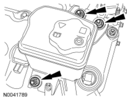
Fig. 420: Locating Power Steering Reservoir Nuts Courtesy of FORD MOTOR CO.
