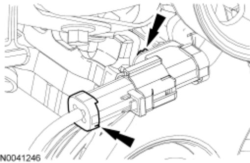
Fig. 510: Locating CMS Electrical Connector And Pin-Type Retainer Courtesy of FORD MOTOR CO.
