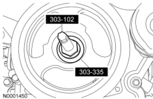
Fig. 21: Installing Crankshaft Pulley Using Special Tools (303-102) & (303-335) Courtesy of FORD MOTOR CO.
