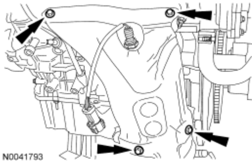
Fig. 277: Locating Heat Shield Bolts Courtesy of FORD MOTOR CO.
