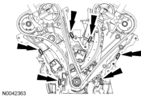
Fig. 379: Locating Silicone Gasket And Sealant On Cylinder Block Courtesy of FORD MOTOR CO.
