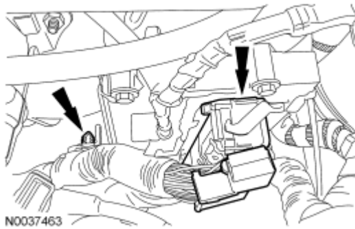
Fig. 161: Locating Powertrain Control Module (PCM) Electrical Connector And Pin-Type Retainer Courtesy of FORD MOTOR CO.
