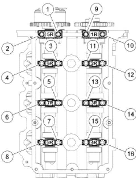
Fig. 94: Identifying Tightening Sequence Of Camshaft Bearing Cap Bolts
