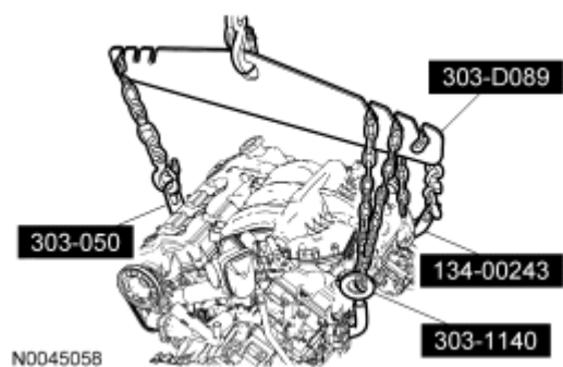
Fig. 230: Identifying Special Tools (134-00243, 303-050, 303-1140, 303-D089) Courtesy of FORD MOTOR CO.
