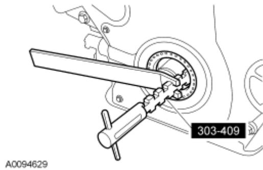
Fig. 304: Identifying Special Tools (303-409) And Crankshaft Front Seal Courtesy of FORD MOTOR CO.
