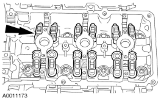
Fig. 333: Locating Camshaft Roller Followers Courtesy of FORD MOTOR CO.
