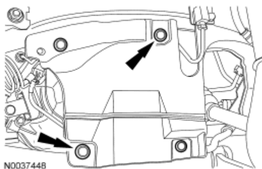
Fig. 550: Locating LH Splash Shield And Pin-Type Retainers Courtesy of FORD MOTOR CO.
