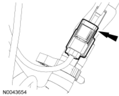
Fig. 424: Locating Knock Sensor Electrical Connector Courtesy of FORD MOTOR CO.
