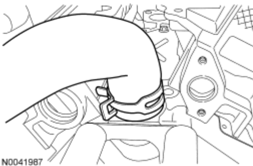
Fig. 404: Locating Coolant Pump Hose From Cylinder Block Outlet Courtesy of FORD MOTOR CO.
