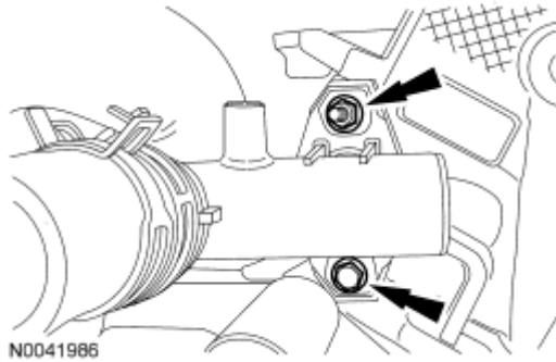
Fig. 405: Locating Bolt, Stud Bolt And Coolant Bypass Courtesy of FORD MOTOR CO.
