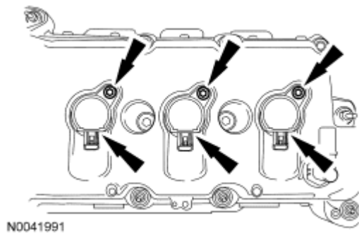
Fig. 392: Locating LH Coil-On-Plug Assemblies And Bolts Courtesy of FORD MOTOR CO.
