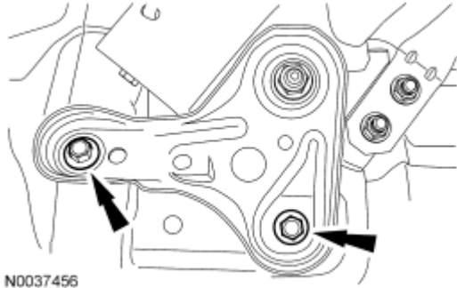
Fig. 544: Locating Subframe Bracket-To-Body Bolts Courtesy of FORD MOTOR CO.
