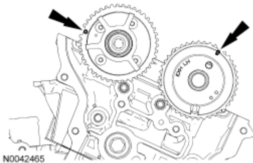
Fig. 354: Locating Camshafts In Neutral Position Courtesy of FORD MOTOR CO.
