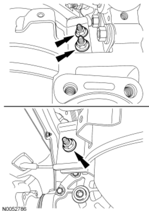
Fig. 191: Locating RH Exhaust Heat Shield Bracket Nuts - Inboard Half Courtesy of FORD MOTOR CO.
