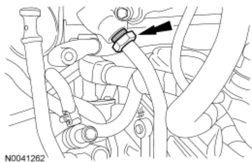
Fig. 212: Locating EGR Tube-To-EGR Valve Nut Courtesy of FORD MOTOR CO.
