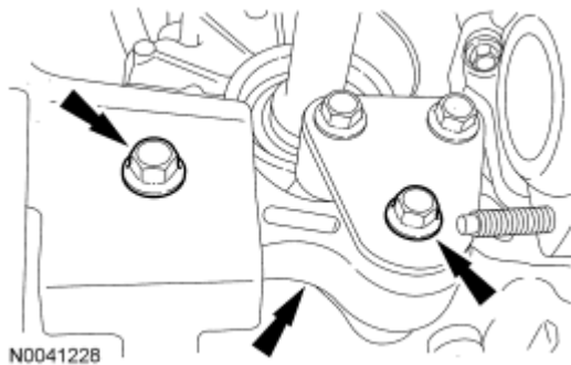
Fig. 144: Identifying Engine Roll Restrictor And Bolts Courtesy of FORD MOTOR CO.
