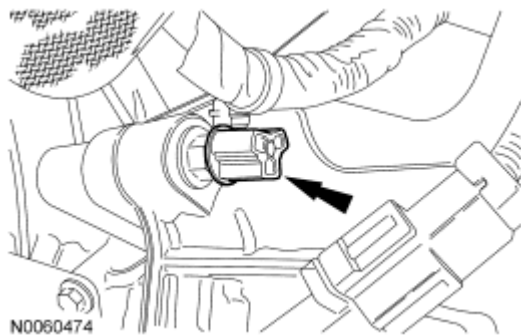
Fig. 462: Locating Wiring Harness Retainer From Stud Bolt Courtesy of FORD MOTOR CO.
