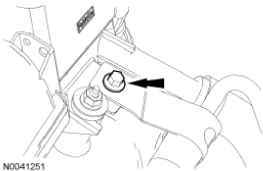
Fig. 208: Locating Power Steering Pressure Hose Bracket-To-Power Steering Reservoir Bolt Courtesy of FORD MOTOR CO.
