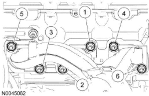
Fig. 469: Identifying Tightening Sequence Of LH Catalytic Converter Nuts Courtesy of FORD MOTOR CO.
