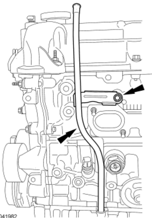
Fig. 282: Locating Oil Level Indicator Tube And Bolt Courtesy of FORD MOTOR CO.
