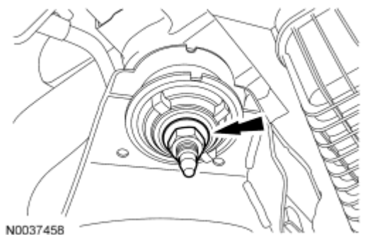
Fig. 154: Locating Front Subframe Nut
