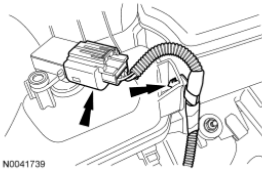
Fig. 234: Locating Manifold Actual Pressure Sensor Electrical Connector And Pin-Type Retainer Courtesy of FORD MOTOR CO.
