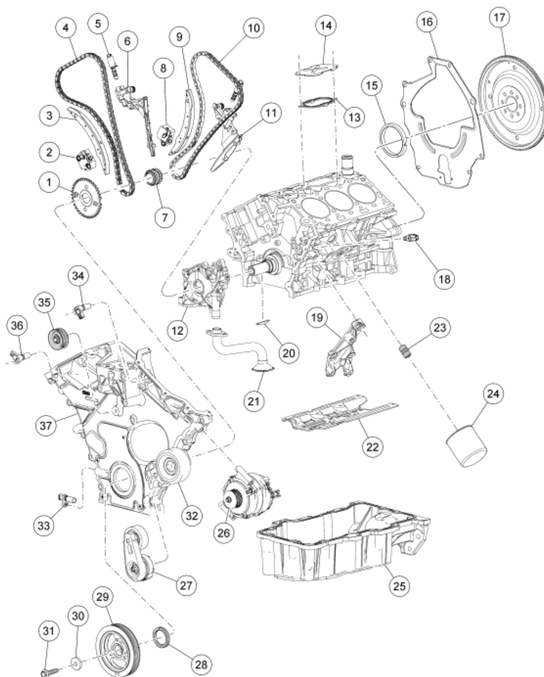
Fig. 340: Exploded View Of Engine Assembly (1 Of 2)
