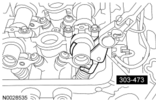
Fig. 100: Removing Roller Using Special Tool (303-473) Courtesy of FORD MOTOR CO.
