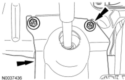
Fig. 132: Locating Steering Joint Cover And Nuts Courtesy of FORD MOTOR CO.
