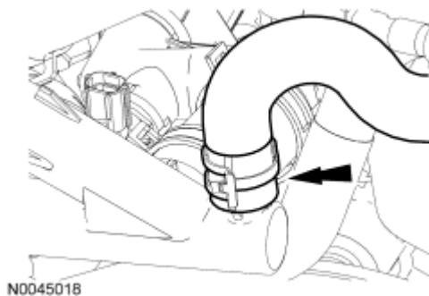
Fig. 162: Locating Heater Hose From Thermostat Housing Courtesy of FORD MOTOR CO.
