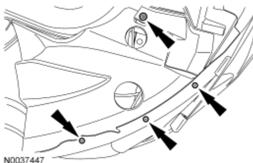
Fig. 551: Locating LH Fender Splash Shield Screws Courtesy of FORD MOTOR CO.
