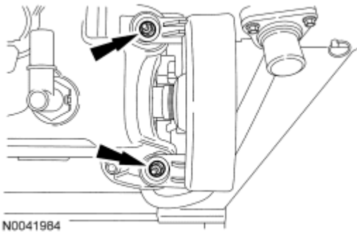
Fig. 284: Locating Coolant Pump Drive Pulley Cover Nuts Courtesy of FORD MOTOR CO.
