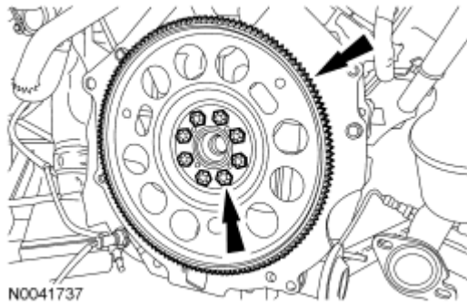
Fig. 231: Locating Flexplate And Bolts Courtesy of FORD MOTOR CO.
