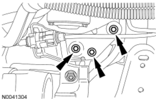
Fig. 168: Locating Transaxle Control Cable Bracket Bolts Courtesy of FORD MOTOR CO.
