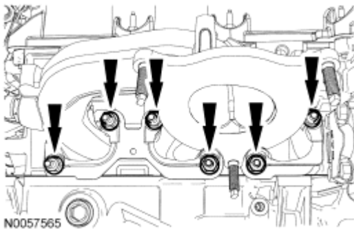
Fig. 275: Identifying RH Exhaust Manifold Nuts Courtesy of FORD MOTOR CO.
