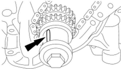
Fig. 315: Positioning Crankcase Key Way In 11 O'Clock Position Courtesy of FORD MOTOR CO.
