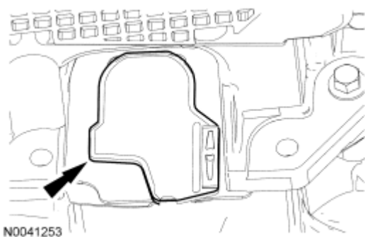
Fig. 197: Locating Torque Converter Nut Access Plug Courtesy of FORD MOTOR CO.
