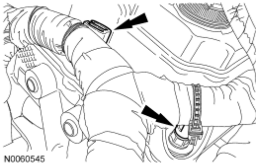
Fig. 256: Identifying Wiring Harness Retainers Courtesy of FORD MOTOR CO.
