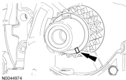
Fig. 362: Locating Timing Marks On Crankshaft Sprockets Courtesy of FORD MOTOR CO.
