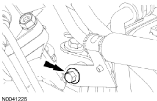
Fig. 141: Locating Power Steering Pressure (PSP) Hose Bracket Bolt
