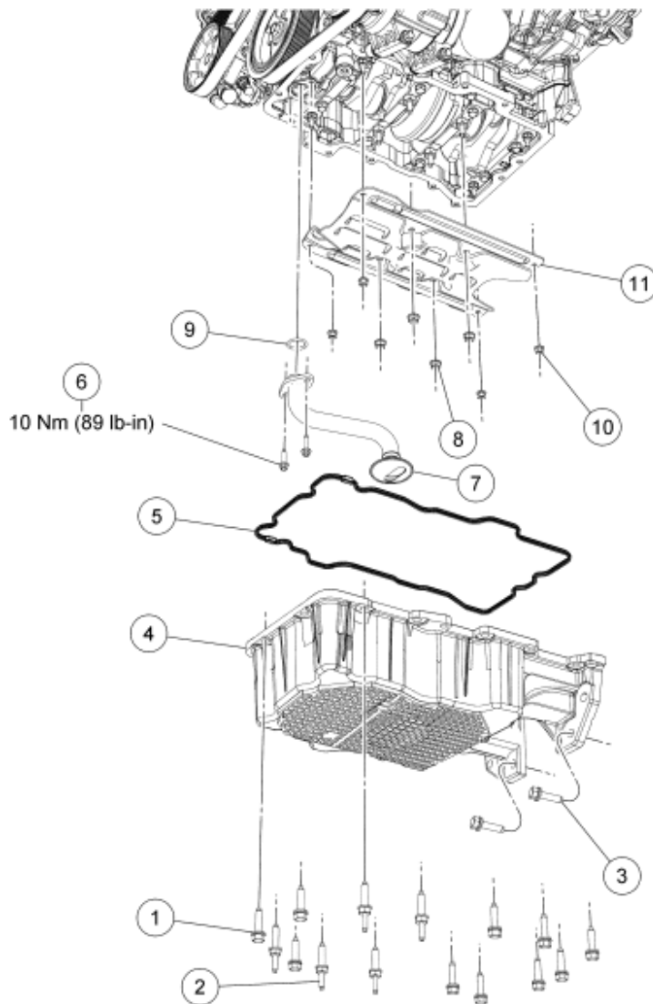
Fig. 112: Exploded View Of Oil Pan, Oil Pump Screen, Pickup Tube & Oil Pan Baffle With Torque Specification
