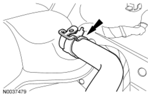
Fig. 175: Locating Coolant Hose To Degas Bottle Courtesy of FORD MOTOR CO.
