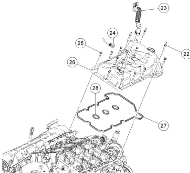
Fig. 14: Exploded View Of Valve Cover - RH (4 Of 4) Courtesy of FORD MOTOR CO.
