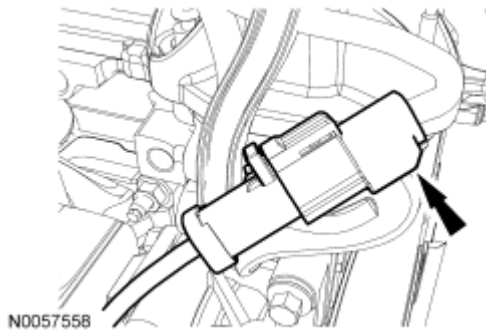
Fig. 255: Identifying RH Catalyst Monitor Sensor Electrical Connector Courtesy of FORD MOTOR CO.
