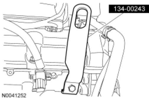
Fig. 454: Identifying Special Tools (134-00243) Courtesy of FORD MOTOR CO.
