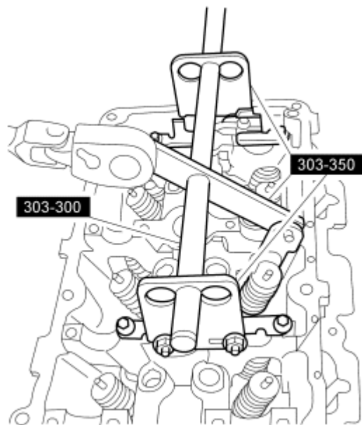
Fig. 339: Identifying Special Tools (303-300 And 303-350) Courtesy of FORD MOTOR CO.
