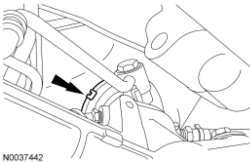
Fig. 140: Locating Steering Gear-To-Dash Seal Clips Courtesy of FORD MOTOR CO.
