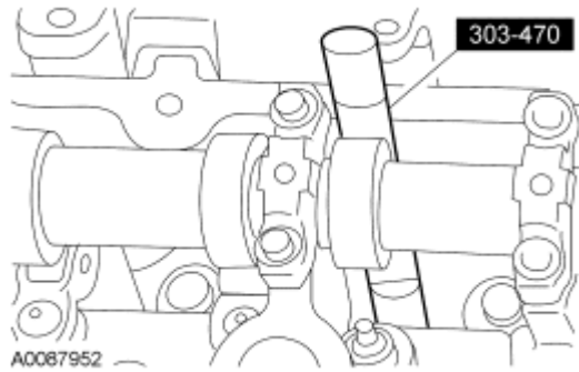
Fig. 103: Identifying Special Tool (303-470) Courtesy of FORD MOTOR CO.
