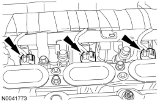
Fig. 436: Locating Fuel Injector Electrical Connectors Courtesy of FORD MOTOR CO.
