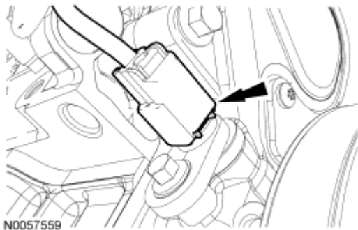
Fig. 429: Identifying Crankshaft Position (CKP) Sensor Electrical Connector Courtesy of FORD MOTOR CO.
