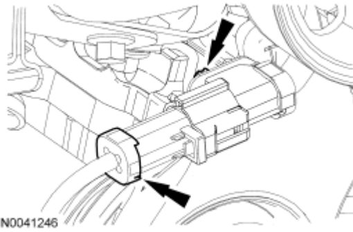
Fig. 184: Locating CMS Electrical Connector And Pin-Type Retainer Courtesy of FORD MOTOR CO.
