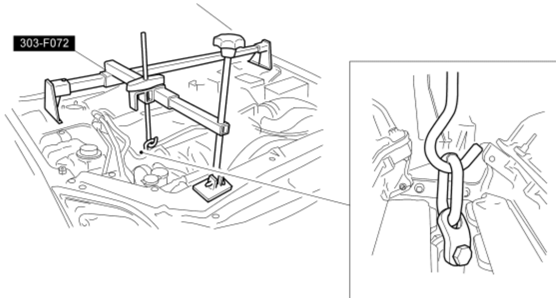
Fig. 131: Identifying Special Tools (303-F072) Courtesy of FORD MOTOR CO.
