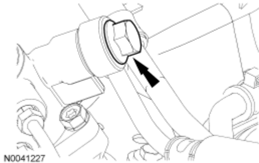
Fig. 142: Locating PSP Hose Banjo Bolt Courtesy of FORD MOTOR CO.
