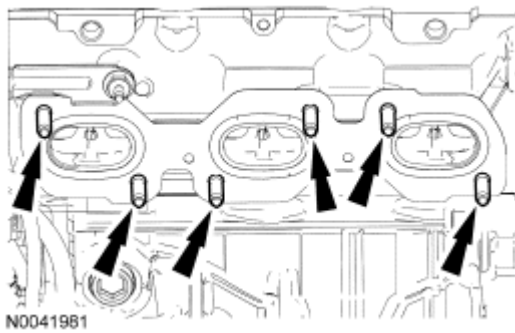
Fig. 468: Locating LH Catalytic Converter Studs Courtesy of FORD MOTOR CO.
