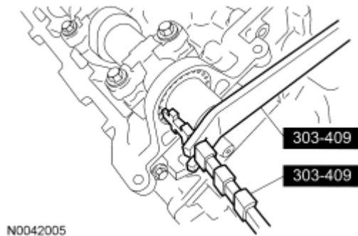
Fig. 323: Identifying Special Tools (303-409) Courtesy of FORD MOTOR CO.
