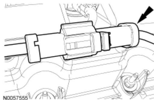
Fig. 426: Identifying RH HO2S Electrical Connector Courtesy of FORD MOTOR CO.
