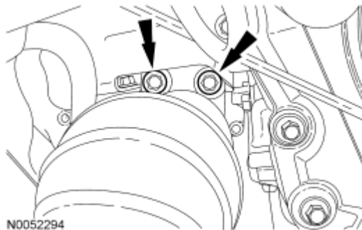
Fig. 194: Locating RH Halfshaft Bearing Support Bracket Bolts Courtesy of FORD MOTOR CO.
