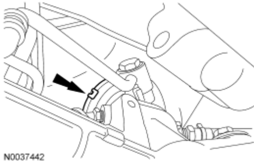
Fig. 558: Locating Steering Gear-To-Dash Seal Clips Courtesy of FORD MOTOR CO.
