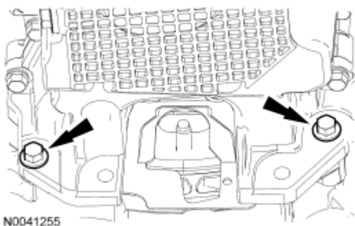
Fig. 199: Locating Oil Pan-To-Transaxle Bolts Courtesy of FORD MOTOR CO.
