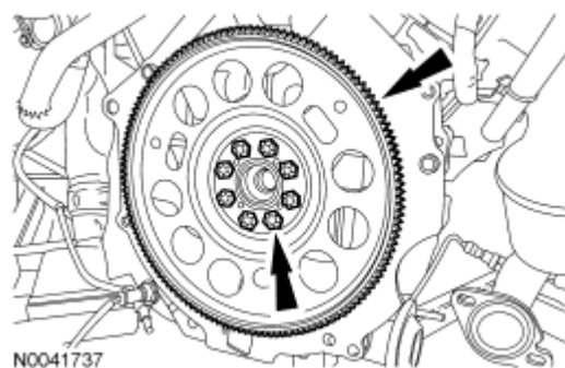
Fig. 459: Locating Flexplate And Bolts Courtesy of FORD MOTOR CO.
