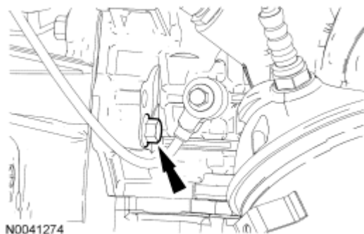
Fig. 226: Locating Engine-To-Transaxle Bolt Courtesy of FORD MOTOR CO.
