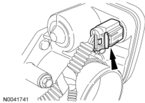
Fig. 237: Locating Electronic Throttle Body Electrical Connector Courtesy of FORD MOTOR CO.
