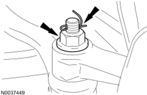
Fig. 145: Locating Tie-Rod Ends Nuts And Cotter Pin Courtesy of FORD MOTOR CO.
