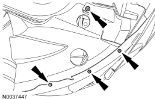
Fig. 136: Locating LH Fender Splash Shield Screws Courtesy of FORD MOTOR CO.
