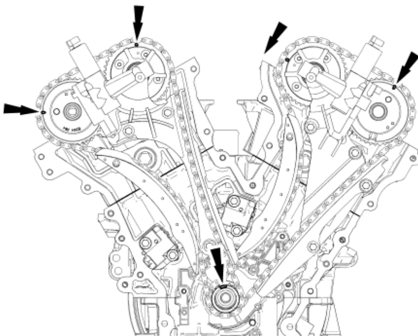
Fig. 309: Locating Keyways Position Courtesy of FORD MOTOR CO.
