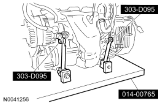
Fig. 200: Identifying Special Tools (303-D095, 014-00765) Courtesy of FORD MOTOR CO.
