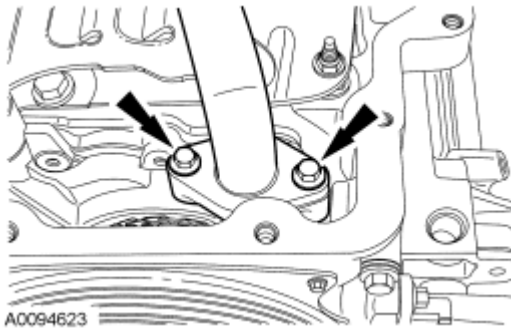
Fig. 388: Locating Oil Pump Screen And Pickup Tube Bolts Courtesy of FORD MOTOR CO.
