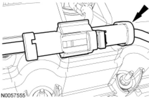
Fig. 505: Identifying RH HO2S Electrical Connector Courtesy of FORD MOTOR CO.
