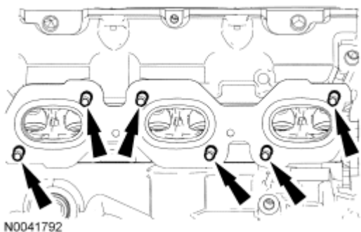
Fig. 276: Locating Exhaust Manifold Studs Courtesy of FORD MOTOR CO.
