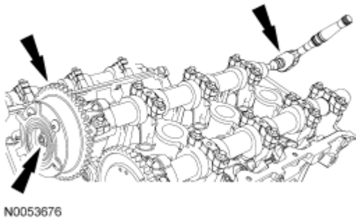
Fig. 326: Locating VCT Actuator And Bolt Courtesy of FORD MOTOR CO.
