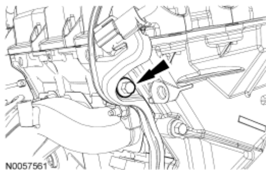
Fig. 418: Identifying Wiring Harness Retainer Bolt Courtesy of FORD MOTOR CO.
