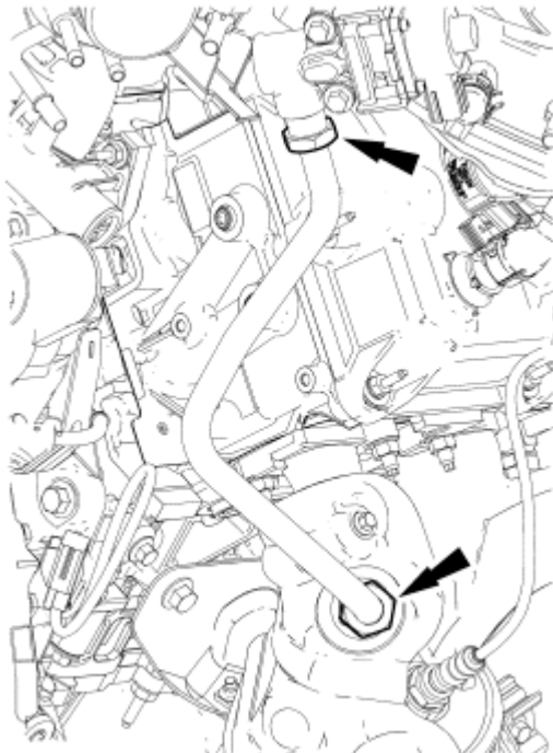
Fig. 485: Locating EGR Tube And Nuts Courtesy of FORD MOTOR CO.
