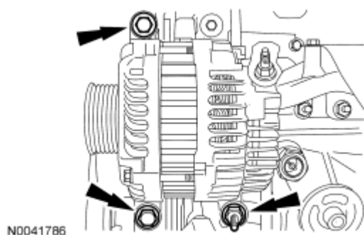
Fig. 271: Locating Generator Bolts Courtesy of FORD MOTOR CO.
