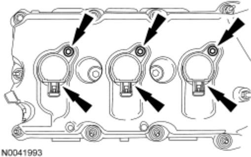
Fig. 395: Locating RH Coil-On-Plug Assemblies And Bolts Courtesy of FORD MOTOR CO.
