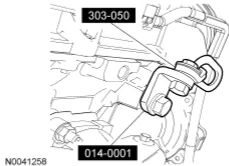
Fig. 204: Identifying Special Tools (303-050 And 014-0001) Courtesy of FORD MOTOR CO.
