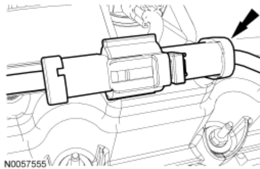
Fig. 188: Identifying RH HO2S Electrical Connector Courtesy of FORD MOTOR CO.
