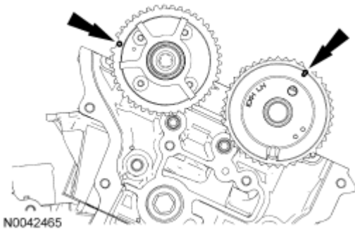
Fig. 76: Locating Camshafts In Neutral Position Courtesy of FORD MOTOR CO.
