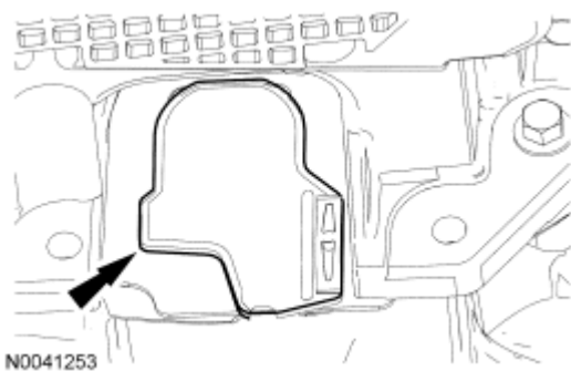
Fig. 496: Locating Torque Converter Nut Access Plug Courtesy of FORD MOTOR CO.
