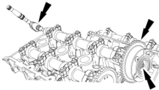
Fig. 353: Locating VCT Actuator And Bolt Courtesy of FORD MOTOR CO.
