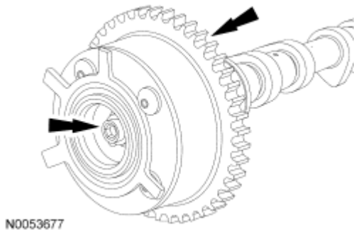
Fig. 348: Locating VCT Actuator Onto Intake Camshaft Courtesy of FORD MOTOR CO.
