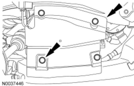
Fig. 135: Locating Splash Shield Pin-Type Retainers Courtesy of FORD MOTOR CO.
