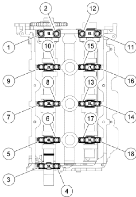
Fig. 328: Identifying Loosening Sequence Of Camshaft Bearing Bolts Courtesy of FORD MOTOR CO.
