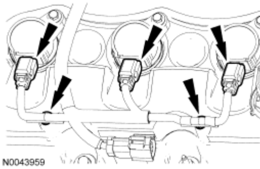
Fig. 248: Locating LH Coil-On-Plug Electrical Connectors Courtesy of FORD MOTOR CO.
