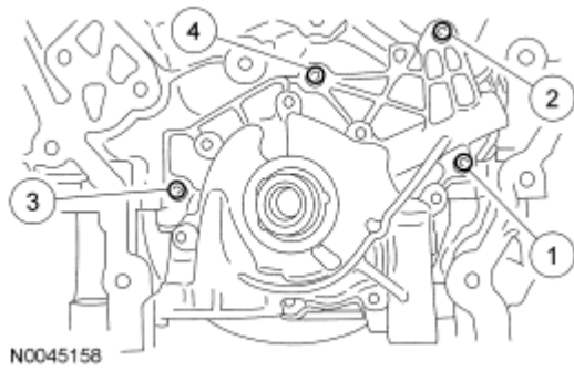
Fig. 321: Identifying Removal Sequence Of Oil Pump Bolts Courtesy of FORD MOTOR CO.
