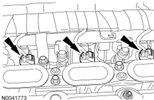
Fig. 250: Locating Fuel Injector Electrical Connectors Courtesy of FORD MOTOR CO.
