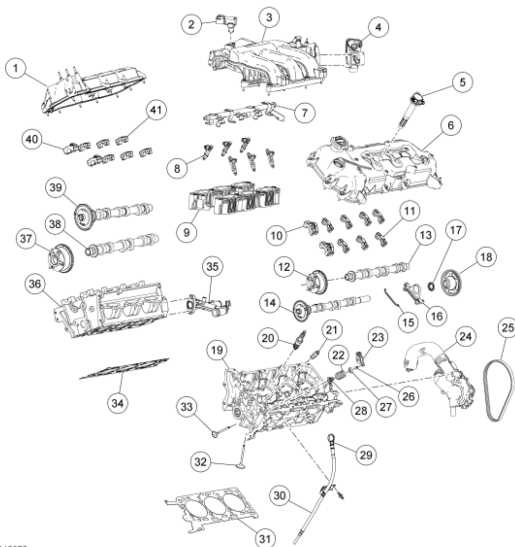
Fig. 341: Exploded View Of Engine Assembly (2 Of 2) Courtesy of FORD MOTOR CO.
