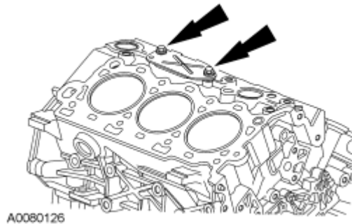
Fig. 335: Locating Oil Separator Cover Bolts Courtesy of FORD MOTOR CO.
