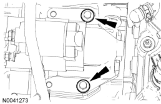
Fig. 225: Locating Starter Motor Bolts Courtesy of FORD MOTOR CO.
