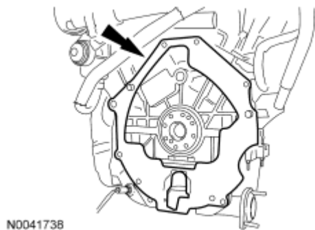
Fig. 458: Locating Engine-To-Transaxle Separator Plate Courtesy of FORD MOTOR CO.
