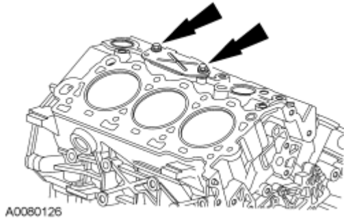
Fig. 342: Locating Oil Separator Cover Bolts Courtesy of FORD MOTOR CO.
