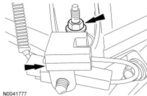
Fig. 432: Locating Radio Frequency Interference Capacitor And Nut Courtesy of FORD MOTOR CO.
