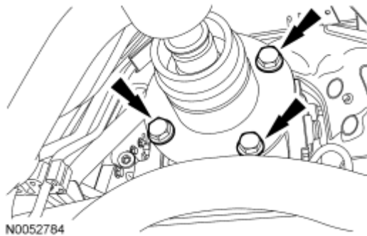
Fig. 559: Identifying Drive Shaft Bolts Courtesy of FORD MOTOR CO.
