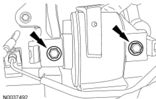
Fig. 494: Locating Transaxle Mount Bolts Courtesy of FORD MOTOR CO.
