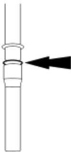
Fig. 408: Locating O-Ring On Oil Level Indicator Tube Courtesy of FORD MOTOR CO.
