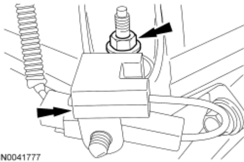
Fig. 254: Locating Radio Frequency Interference Capacitor And Nut Courtesy of FORD MOTOR CO.
