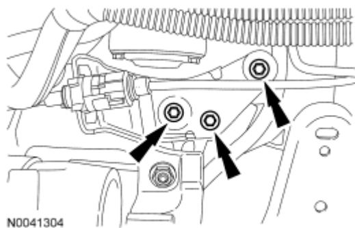
Fig. 527: Locating Transaxle Control Cable Bracket Bolts Courtesy of FORD MOTOR CO.
