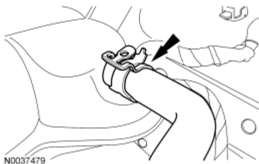
Fig. 520: Locating Coolant Hose To Degas Bottle Courtesy of FORD MOTOR CO.
