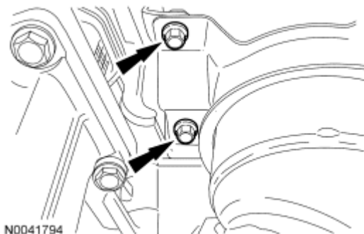
Fig. 470: Locating LH Catalytic Converter Bracket Bolts Courtesy of FORD MOTOR CO.
