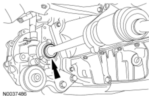
Fig. 508: Locating RH Halfshaft Courtesy of FORD MOTOR CO.
