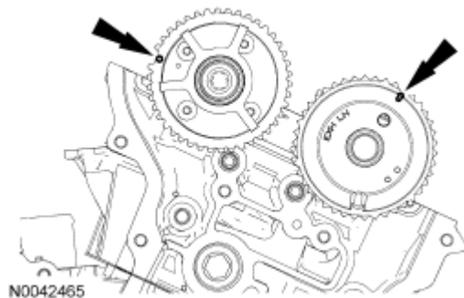
Fig. 367: Locating Camshafts In Neutral Position Courtesy of FORD MOTOR CO.
