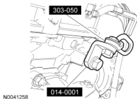
Fig. 455: Identifying Special Tools (303-050 And 014-0001) Courtesy of FORD MOTOR CO.
