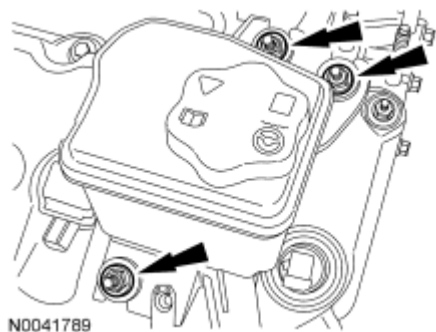
Fig. 267: Locating Power Steering Reservoir Nuts Courtesy of FORD MOTOR CO.
