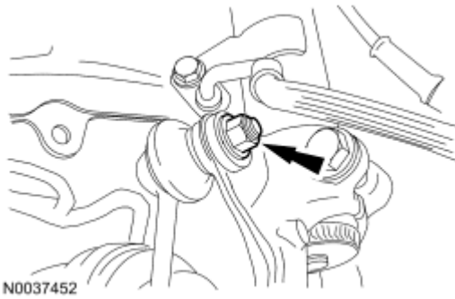
Fig. 147: Locating Stabilizer Bar Links Nut Courtesy of FORD MOTOR CO.
