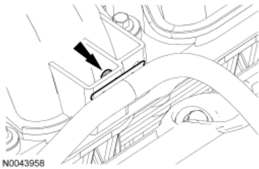
Fig. 235: Locating Wiring Harness Pin-Type Retainer Courtesy of FORD MOTOR CO.
