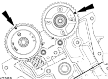
Fig. 372: Locating RH Camshafts Position Courtesy of FORD MOTOR CO.
