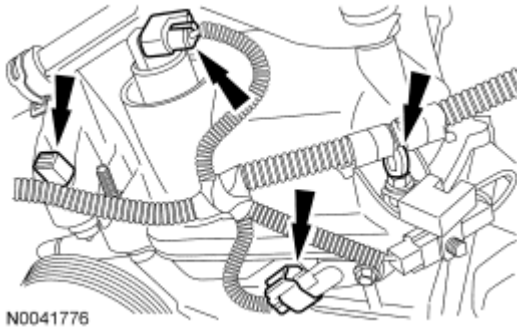
Fig. 433: Locating RH VCT Solenoid And LH Camshaft Position Sensor Electrical Connectors Courtesy of FORD MOTOR CO.
