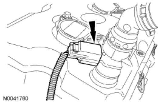
Fig. 425: Locating Positive Crankcase Ventilation Valve Electrical Connector Courtesy of FORD MOTOR CO.
