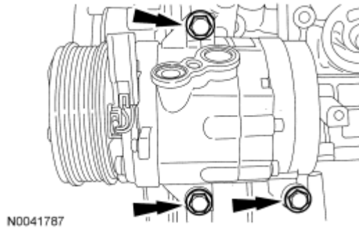
Fig. 415: Locating A/C Compressor Bolts Courtesy of FORD MOTOR CO.
