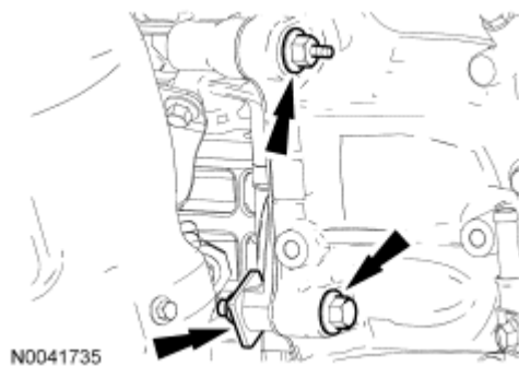
Fig. 229: Locating Transaxle-To-Engine Stud Bolt, Bolt And Nut Courtesy of FORD MOTOR CO.
