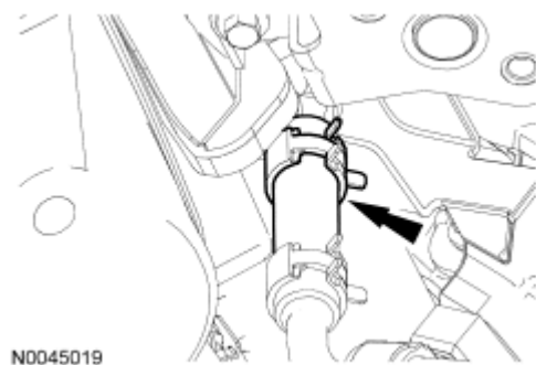
Fig. 165: Locating Evaporative Emissions (EVAP) Hose Courtesy of FORD MOTOR CO.
