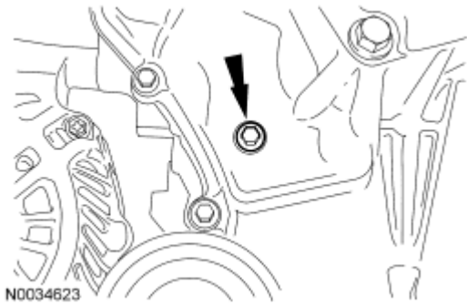
Fig. 119: Locating Upper Front Cover Timing Hole Plug Courtesy of FORD MOTOR CO.
