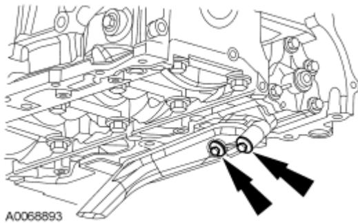
Fig. 463: Locating Oil Pump Pickup Tube Bolts Courtesy of FORD MOTOR CO.
