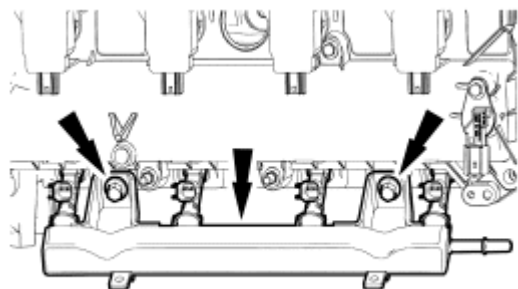
Fig. 515: Locating Fuel Rail And Injector Assembly Bolts Courtesy of FORD MOTOR CO.
