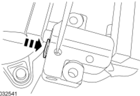
Fig. 486: Pushing Ratchet Arm Back Into Tensioner Housing Courtesy of FORD MOTOR CO.
