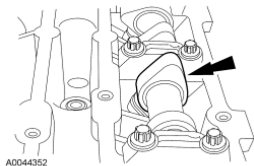
Fig. 406: Locating Camshaft Lobe Courtesy of FORD MOTOR CO.
