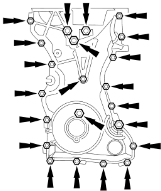
Fig. 397: Locating Engine Front Cover Bolts Courtesy of FORD MOTOR CO.
