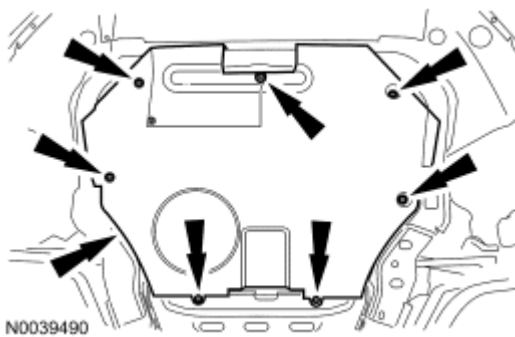
Fig. 181: Locating Splash Shield Bolts Courtesy of FORD MOTOR CO.
