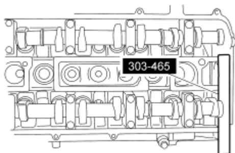
Fig. 135: Identifying Special Tool (303-465) In Slots On Rear Of Camshafts Courtesy of FORD MOTOR CO.
