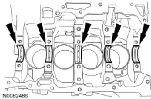
Fig. 424: Locating Main Bearings
