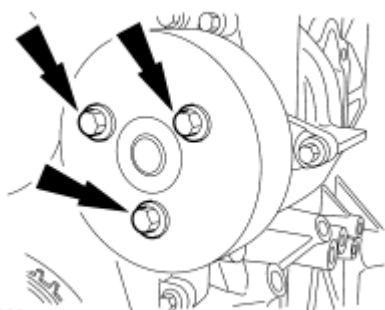
Fig. 340: Locating Coolant Pump Pulley Bolts Courtesy of FORD MOTOR CO.
