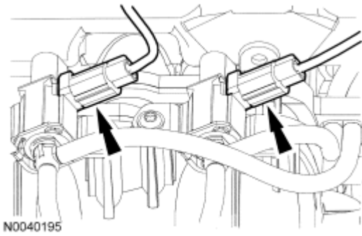
Fig. 367: Locating Swirl Control Valve Electrical Connectors Courtesy of FORD MOTOR CO.
