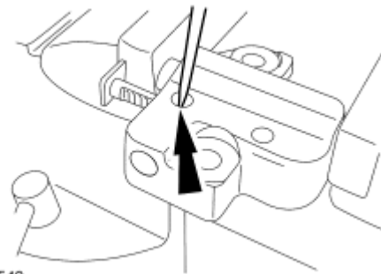
Fig. 485: Using A Small Pick To Push Back And Hold Ratchet Mechanism Courtesy of FORD MOTOR CO.
