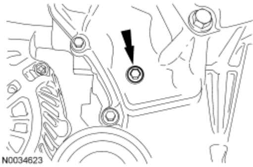
Fig. 118: Locating Upper Front Cover Timing Hole Plug Courtesy of FORD MOTOR CO.
