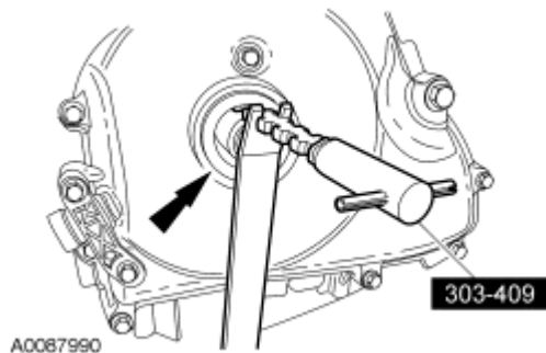
Fig. 394: Removing Crankshaft Front Oil Seal Using Special Tool (303-409) Courtesy of FORD MOTOR CO.
