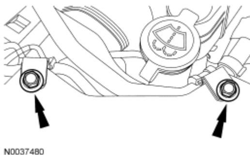
Fig. 303: Locating A/C Tube Bracket Bolts Courtesy of FORD MOTOR CO.
