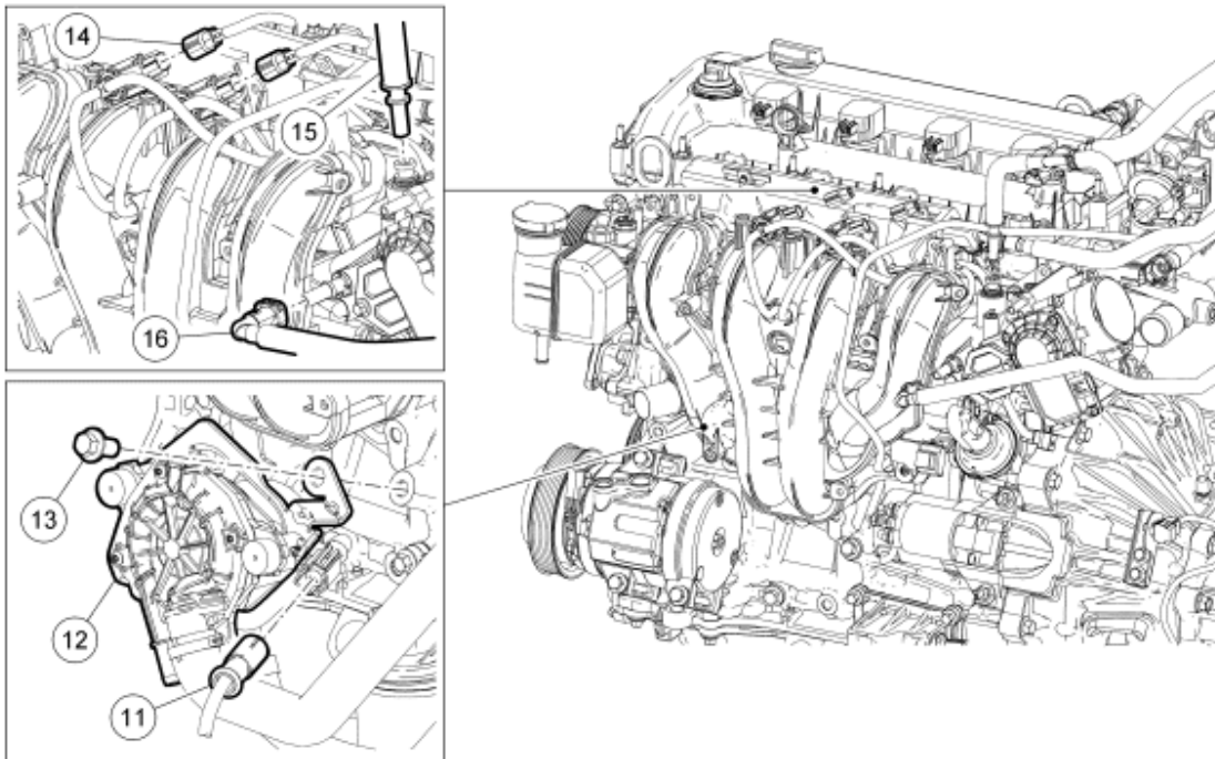
Fig. 16: Exploded View Of Intake Manifold (2 Of 4) Courtesy of FORD MOTOR CO.
