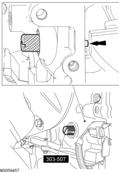
Fig. 414: Installing Crankshaft TDC Timing Peg
