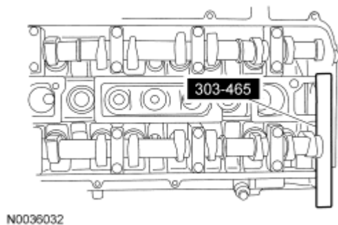
Fig. 101: Identifying Special Tool (303-465) In Slots On Rear Of Camshafts Courtesy of FORD MOTOR CO.
