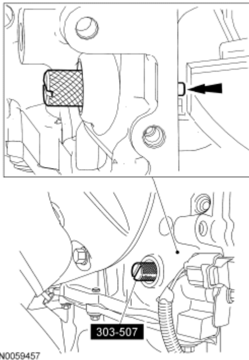
Fig. 417: Installing Crankshaft TDC Timing Peg
