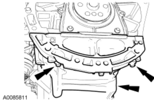
Fig. 193: Identifying Rear Oil Pan Bolts Courtesy of FORD MOTOR CO.
