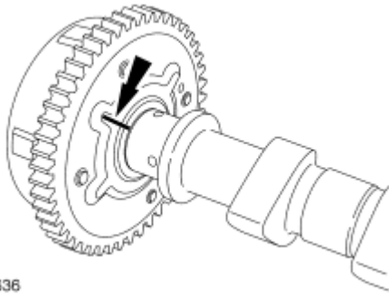
Fig. 109: Locating Marks On Camshaft Phaser Courtesy of FORD MOTOR CO.
