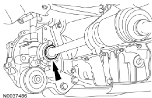
Fig. 244: Locating RH Halfshaft Into Transaxle Courtesy of FORD MOTOR CO.
