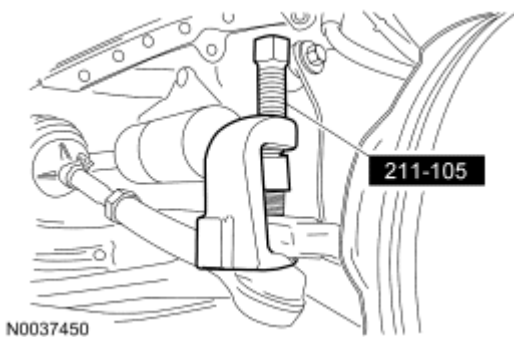
Fig. 210: Separating Tie-Rod Ends From Wheel Knuckles Using Special Tool (211-105) Courtesy of FORD MOTOR CO.
