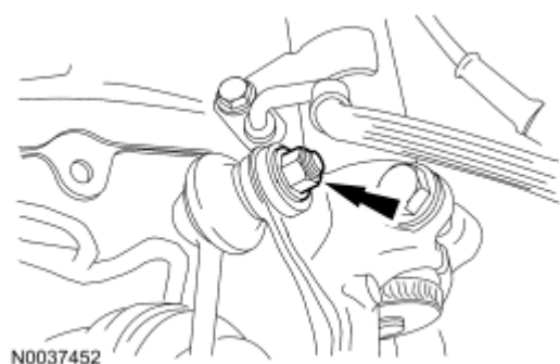
Fig. 212: Locating Sway Bar Links And Nuts Courtesy of FORD MOTOR CO.
