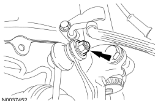
Fig. 626: Locating Sway Bar Links And Nuts
