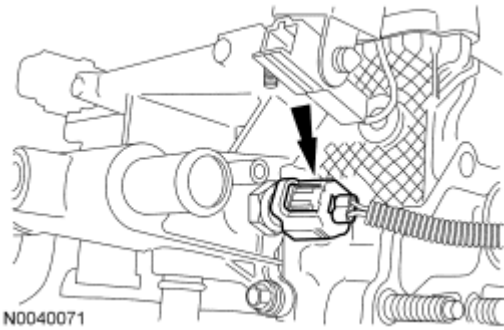
Fig. 539: Locating Coolant Temperature Sender Electrical Connector Courtesy of FORD MOTOR CO.
