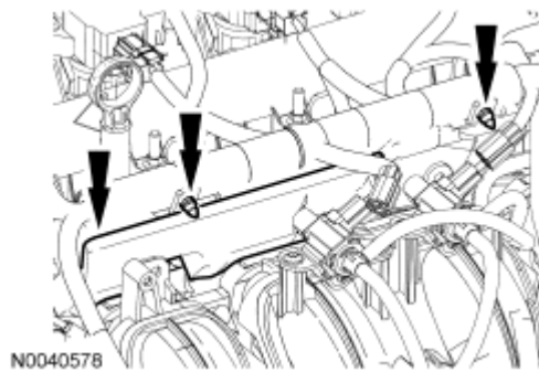
Fig. 21: Locating Fuel Rail Insulator Retainers Courtesy of FORD MOTOR CO.
