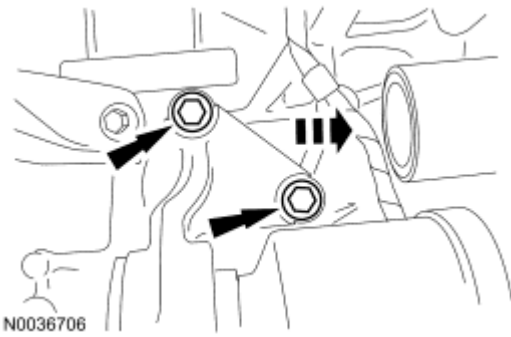
Fig. 125: Locating Half Shaft Carrier Bracket Bolts And Sliding Rh Halfshaft Out Of Transaxle Courtesy of FORD MOTOR CO.
