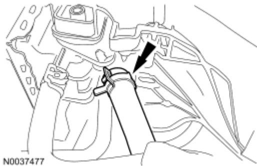
Fig. 300: Locating Power Steering Cooler Tube Courtesy of FORD MOTOR CO.
