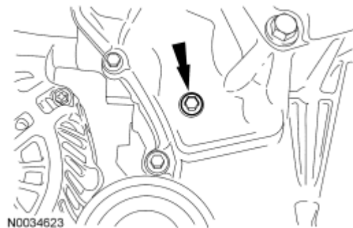
Fig. 100: Locating Upper Front Cover Timing Hole Plug Courtesy of FORD MOTOR CO.
