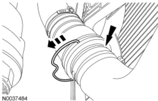
Fig. 307: Removing Retaining Clip And Locating Lower Radiator Hose Courtesy of FORD MOTOR CO.
