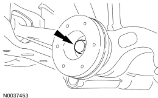
Fig. 279: Locating Lower Control Arms Through Bolt Courtesy of FORD MOTOR CO.
