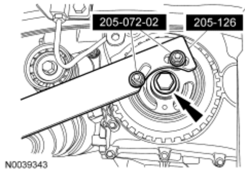
Fig. 393: Locating Crankshaft Pulley Bolt And Special Tools (205-126, 205-072-02) Courtesy of FORD MOTOR CO.
