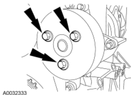
Fig. 338: Locating Coolant Pump Pulley Bolts Courtesy of FORD MOTOR CO.
