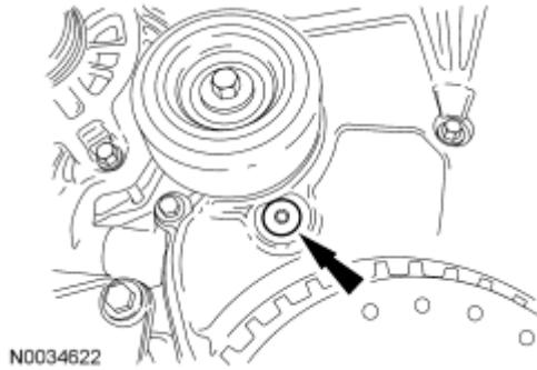
Fig. 99: Locating Lower Front Cover Timing Hole Plug Courtesy of FORD MOTOR CO.
