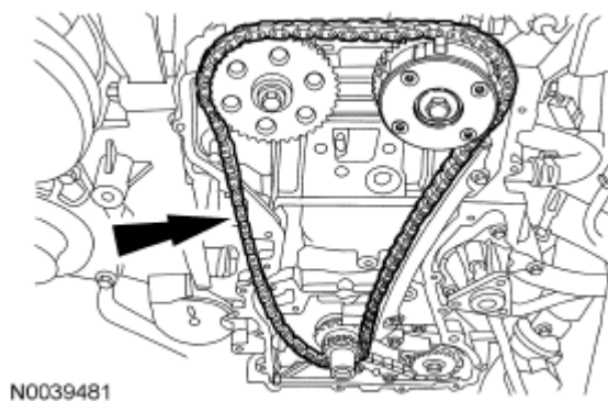
Fig. 479: Locating Timing Chain
