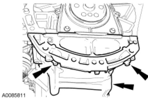
Fig. 463: Identifying Rear Oil Pan Bolts Courtesy of FORD MOTOR CO.
