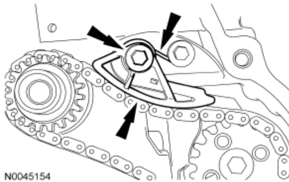
Fig. 190: Locating Oil Pump Chain Tensioner And Bolt Courtesy of FORD MOTOR CO.
