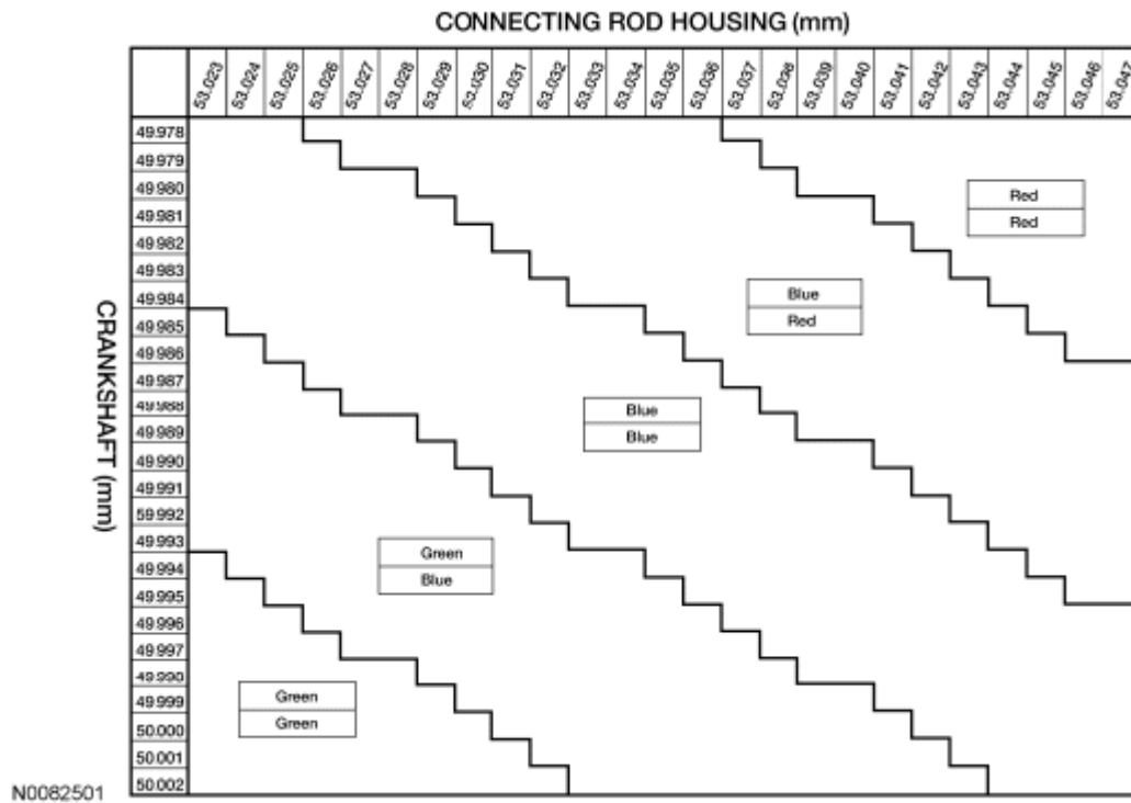
Fig. 441: Connecting Rod Bearings Chart
