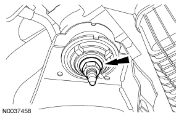
Fig. 618: Locating Front Subframe Nuts Courtesy of FORD MOTOR CO.
