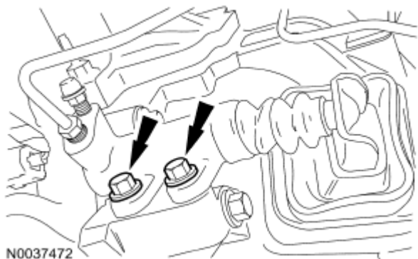
Fig. 296: Locating Clutch Slave Cylinder Bolts Courtesy of FORD MOTOR CO.
