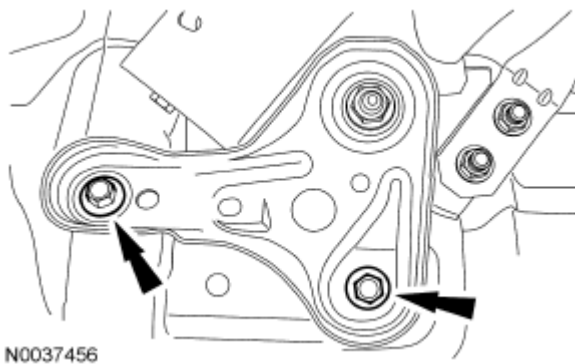
Fig. 679: Locating Subframe Bracket-To-Body Bolts Courtesy of FORD MOTOR CO.
