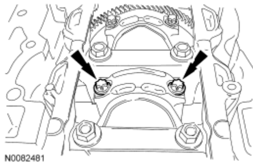
Fig. 416: Locating Connecting Rod Cap Bolts
