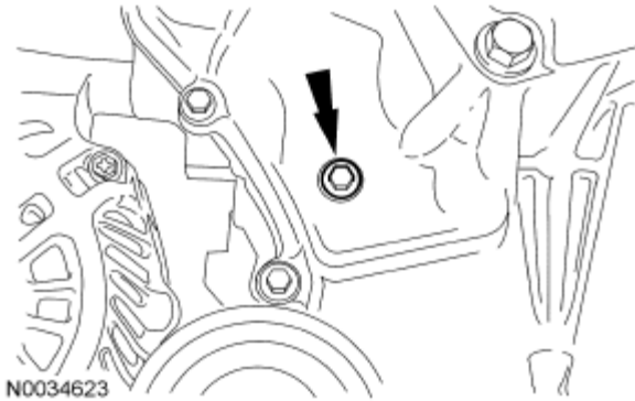
Fig. 148: Locating Upper Timing Hole Plug Courtesy of FORD MOTOR CO.
