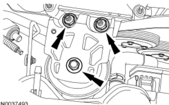
Fig. 646: Locating Engine Mount Bracket Nuts And Bolt Courtesy of FORD MOTOR CO.
