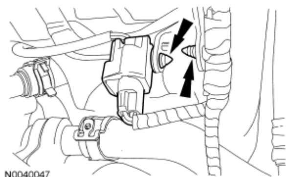
Fig. 563: Locating KS Electrical Connector And Harness Pin-Type Retainers Courtesy of FORD MOTOR CO.
