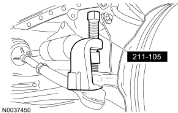
Fig. 272: Locating Special Tool Courtesy of FORD MOTOR CO.
