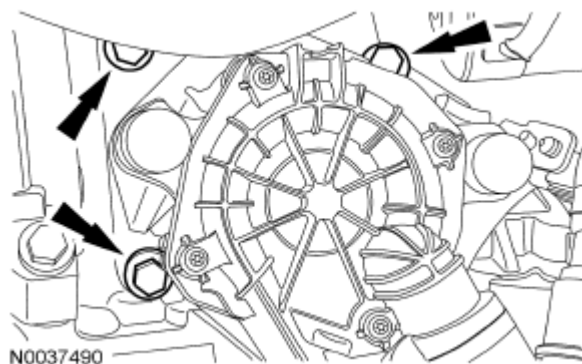
Fig. 588: Locating AIR Pump Bolts Courtesy of FORD MOTOR CO.
