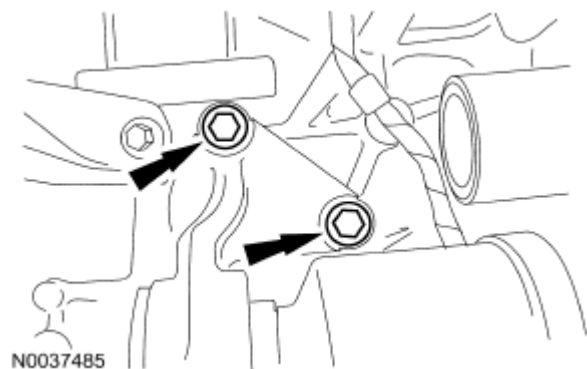
Fig. 307: Locating RH Halfshaft Carrier Bearing Bracket Bolts Courtesy of FORD MOTOR CO.
