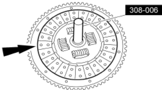
Fig. 574: Locating Special Tool And Clutch Disc Courtesy of FORD MOTOR CO.
