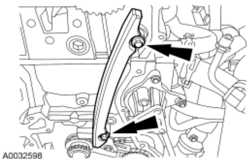
Fig. 398: Identifying Bolts And LH Timing Chain Guide Courtesy of FORD MOTOR CO.
