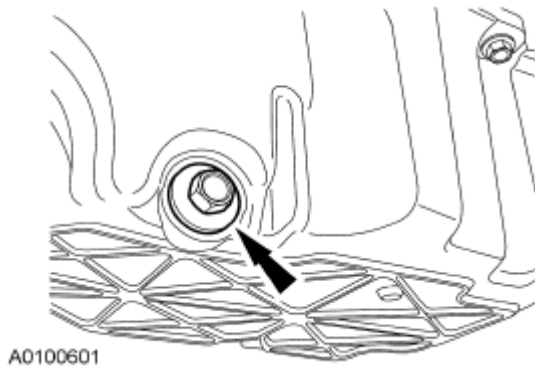
Fig. 282: Locating Drain Plug Courtesy of FORD MOTOR CO.
