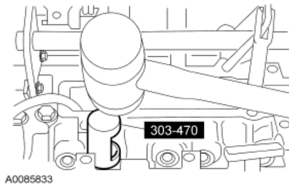
Fig. 426: Installing Valve Seals Courtesy of FORD MOTOR CO.
