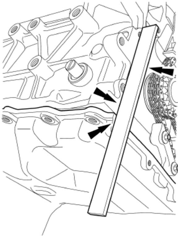
Fig. 192: Aligning Front Surface Of Oil Pan Flush With Front Surface Of Engine Block Using Suitable Straightedge Courtesy of FORD MOTOR CO.
