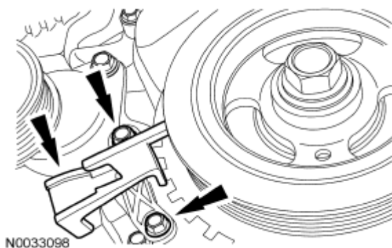
Fig. 76: Locating CKP Sensor Bolts And Alignment Tool Courtesy of FORD MOTOR CO.
