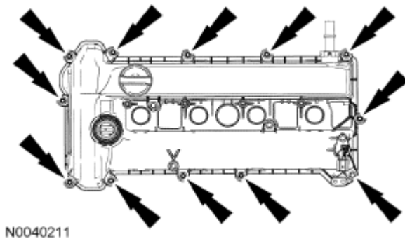
Fig. 386: Locating Valve Cover Retainers Courtesy of FORD MOTOR CO.
