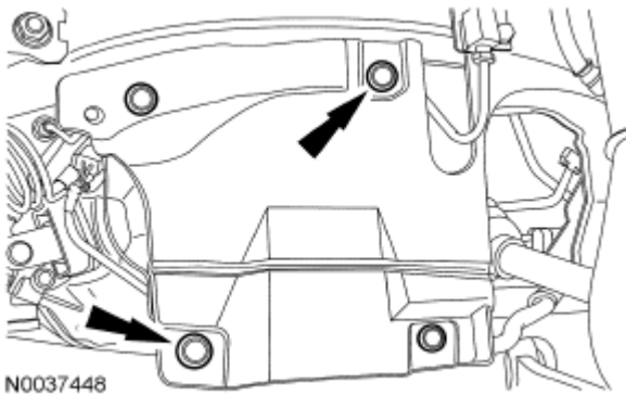
Fig. 206: Locating Pin-Type Retainers And LH Splash Shield Courtesy of FORD MOTOR CO.
