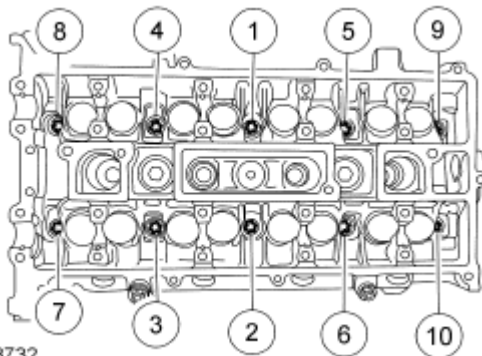
Fig. 469: Identifying Tightening Sequence Of Cylinder Head Bolts Courtesy of FORD MOTOR CO.
