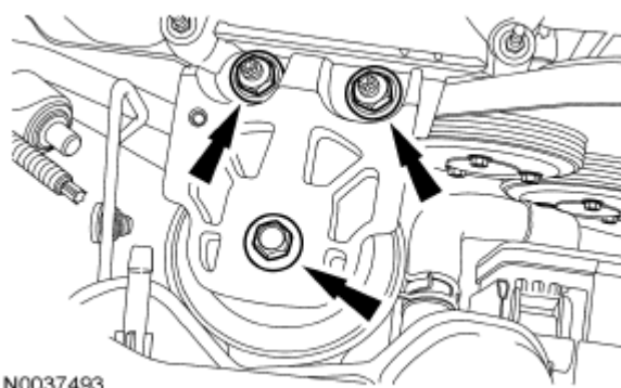
Fig. 587: Locating Engine Mount Bracket Nuts And Bolt Courtesy of FORD MOTOR CO.
