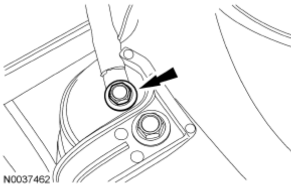
Fig. 613: Locating Ground Wire Bolt
