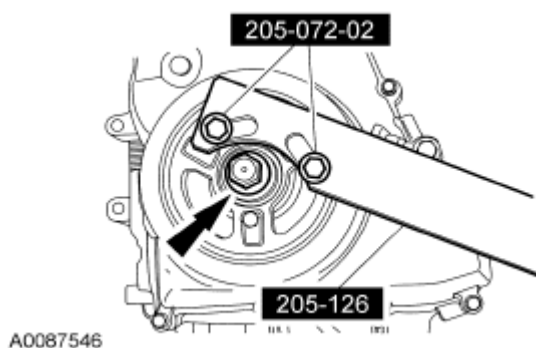
Fig. 493: Locating Crankshaft Pulley Bolt And Special Tools Courtesy of FORD MOTOR CO.
