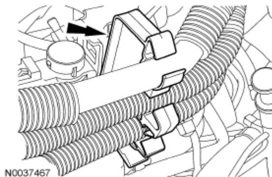
Fig. 291: Locating EVAP Tube Bundle Retaining Clip Courtesy of FORD MOTOR CO.
