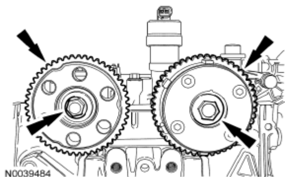
Fig. 85: Locating Camshaft Sprocket And Bolt Courtesy of FORD MOTOR CO.
