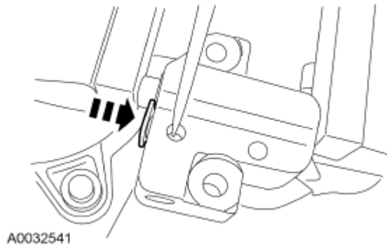
Fig. 483: Pushing Ratchet Arm Back Into Tensioner Housing Courtesy of FORD MOTOR CO.
