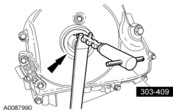
Fig. 393: Locating Special Tool And Crankshaft Front Oil Seal Courtesy of FORD MOTOR CO.
