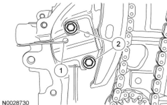
Fig. 79: Identifying Timing Chain Tensioner Bolts And Paper Clip Courtesy of FORD MOTOR CO.
