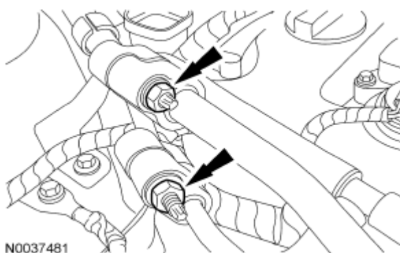
Fig. 655: Locating A/C Tubes Nuts Courtesy of FORD MOTOR CO.
