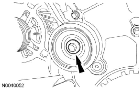
Fig. 555: Locating Accessory Drive Belt Idler Pulley Courtesy of FORD MOTOR CO.
