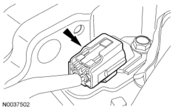
Fig. 578: Locating Turbine Shaft Speed (TSS) Sensor Electrical Connector Courtesy of FORD MOTOR CO.
