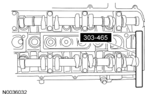
Fig. 131: Identifying Special Tool Courtesy of FORD MOTOR CO.
