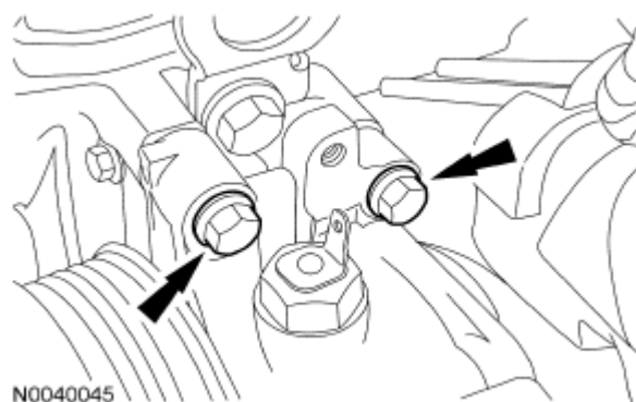
Fig. 565: Locating Upper Power Steering Pump Bolts Courtesy of FORD MOTOR CO.
