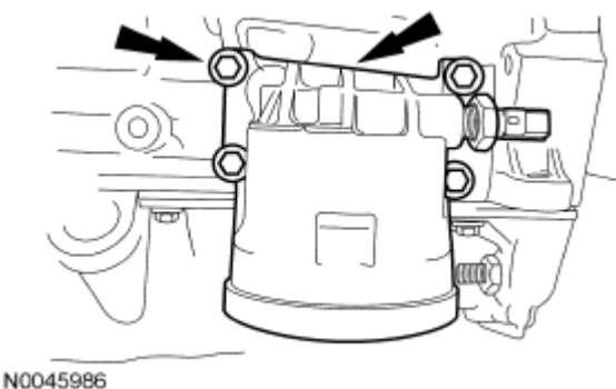
Fig. 375: Locating Oil Filter Adapter And Bolts Courtesy of FORD MOTOR CO.
