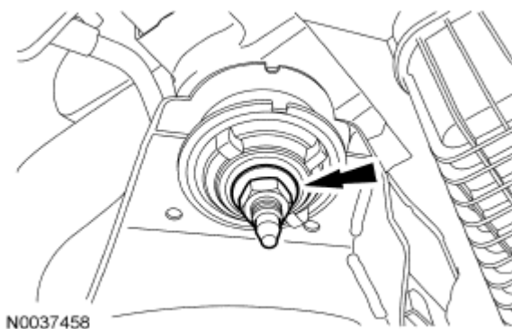
Fig. 217: Locating Front Subframe Nuts Courtesy of FORD MOTOR CO.
