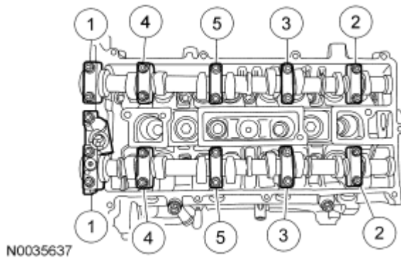
Fig. 107: Identifying Loosening Sequence Of Camshaft Bearing Cap Bolts Courtesy of FORD MOTOR CO.
