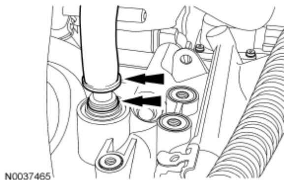
Fig. 610: Locating Locking Ring And Brake Booster Vacuum Supply Tube Courtesy of FORD MOTOR CO.
