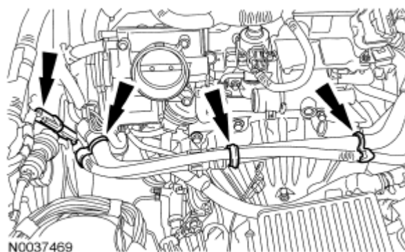
Fig. 229: Locating Heater Hose Retaining Clips Courtesy of FORD MOTOR CO.
