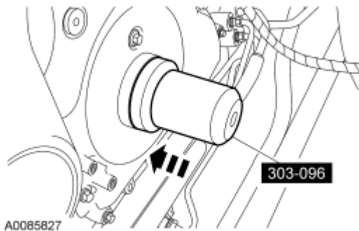
Fig. 489: Installing Crankshaft Front Oil Seal Using Special Tool Courtesy of FORD MOTOR CO.
