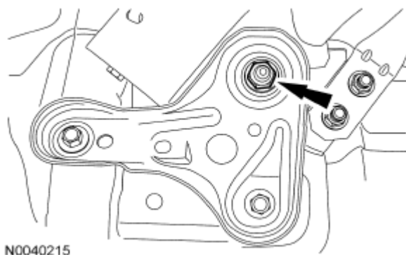
Fig. 620: Locating Subframe Nuts Courtesy of FORD MOTOR CO.
