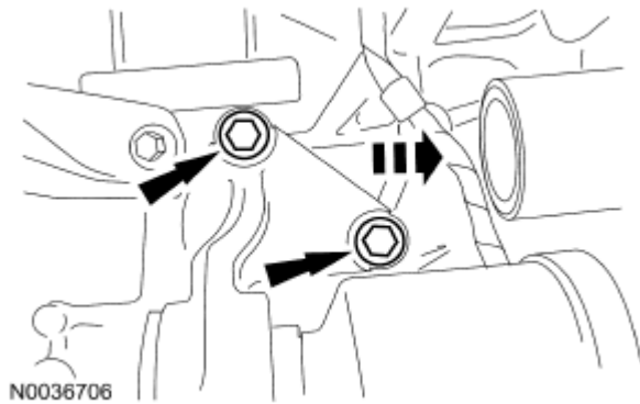
Fig. 125: Locating Halfshaft Carrier Bracket Bolts And Sliding Out Of Transaxle Courtesy of FORD MOTOR CO.
