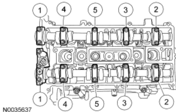
Fig. 167: Identifying Loosening Sequence Of Camshaft Bearing Cap Bolts Courtesy of FORD MOTOR CO.
