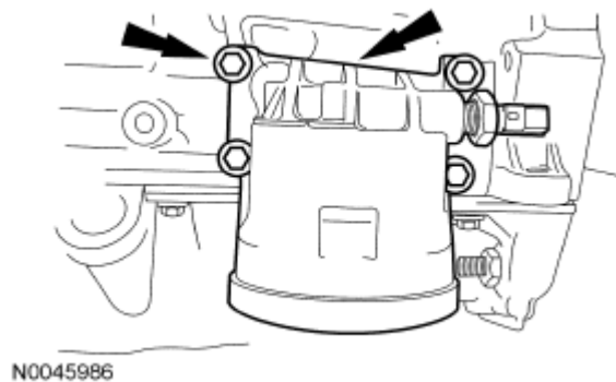
Fig. 520: Locating Oil Filter Adapter Bolts Courtesy of FORD MOTOR CO.
