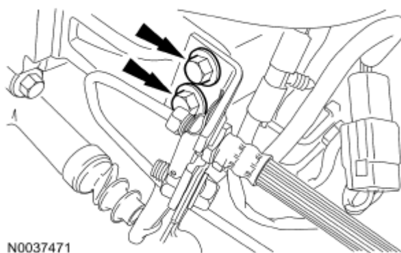
Fig. 662: Locating Clutch Tube Bracket Bolts Courtesy of FORD MOTOR CO.
