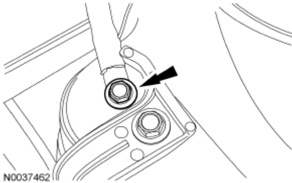
Fig. 671: Installing Ground Wire And Bolt Courtesy of FORD MOTOR CO.
