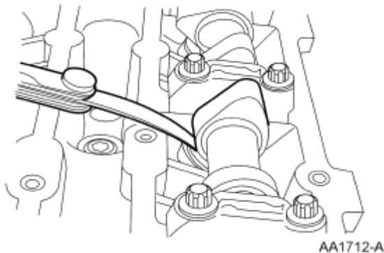
Fig. 1: Measuring Valve Clearance Courtesy of FORD MOTOR CO.
