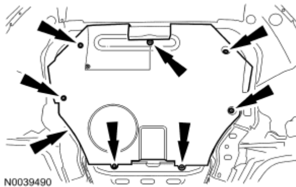
Fig. 181: Locating Underbody Cover Screws Courtesy of FORD MOTOR CO.
