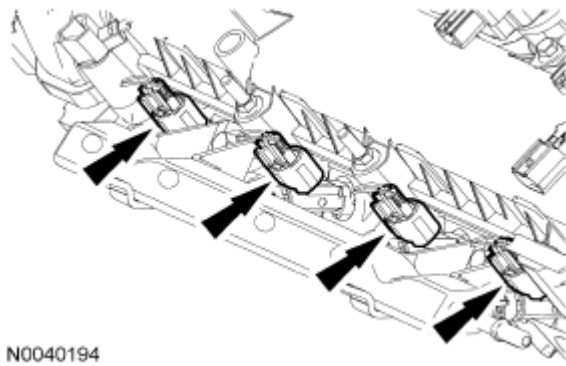
Fig. 514: Locating Fuel Injector Electrical Connectors Courtesy of FORD MOTOR CO.
