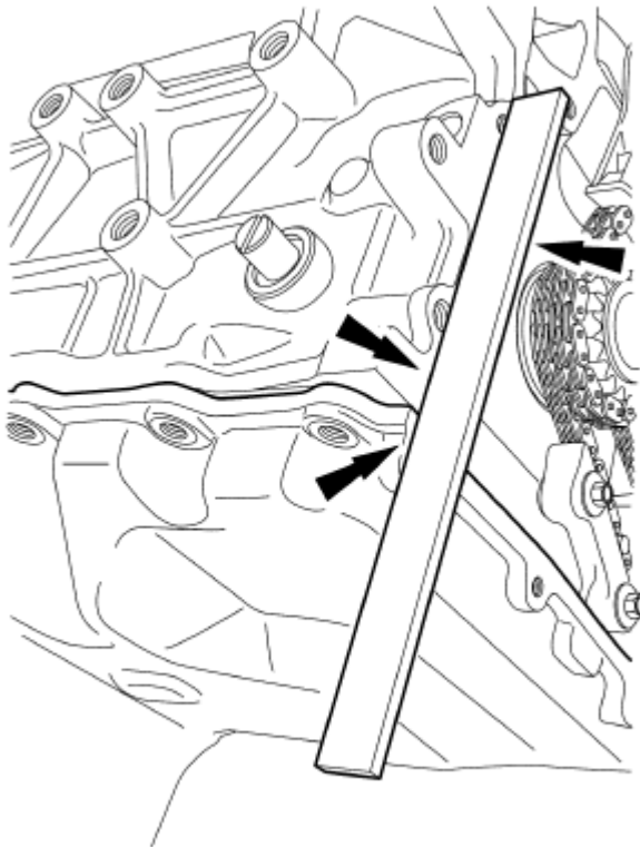
Fig. 464: Using Suitable Straight Edge To Align Front Surface Of Oil Pan Flush With Front Surface Of Engine Block
