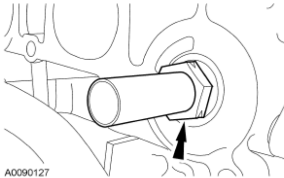
Fig. 526: Locating EGR Tube Courtesy of FORD MOTOR CO.
