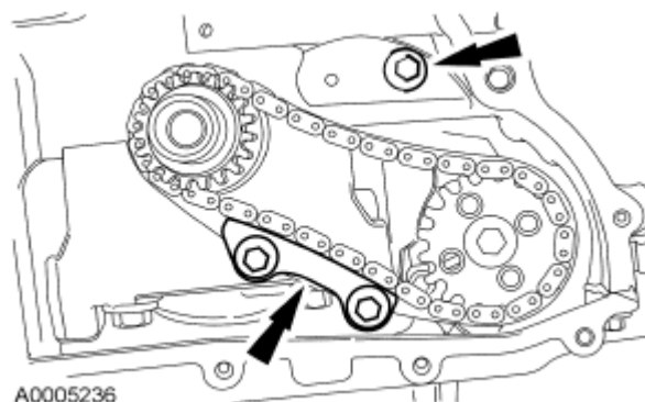
Fig. 189: Identifying Oil Pump Chain Guide And Shoulder Bolts Courtesy of FORD MOTOR CO.
