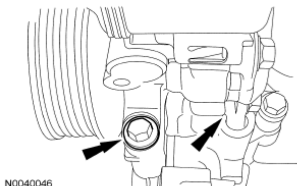
Fig. 564: Locating Power Steering Pump And Lower Bolt Courtesy of FORD MOTOR CO.
