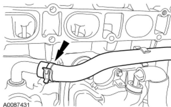
Fig. 524: Locating Bypass Hose To Cylinder Block Nipple Courtesy of FORD MOTOR CO.
