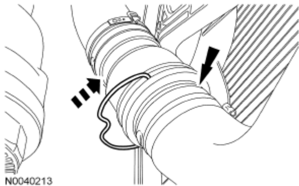
Fig. 652: Identifying Lower Radiator Hose And Installing Retaining Clip Courtesy of FORD MOTOR CO.
