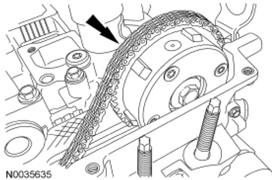
Fig. 135: Locating Timing Chain Courtesy of FORD MOTOR CO.
