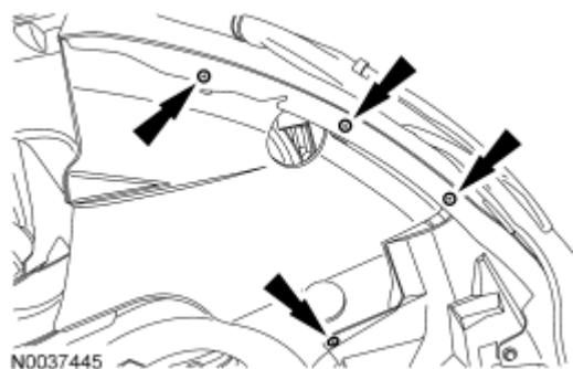
Fig. 688: Locating RH Fender Splash Shield Screws Courtesy of FORD MOTOR CO.
