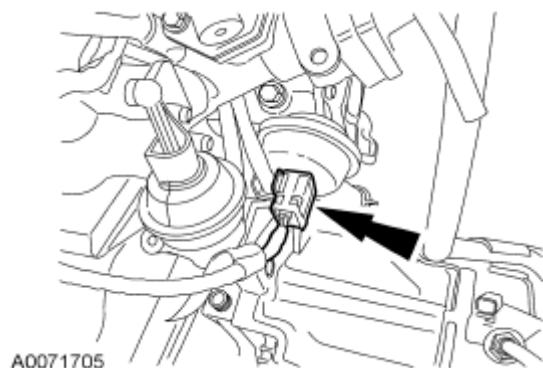
Fig. 532: Locating Intake Manifold Runner Control (IMRC) Actuator Electrical Connector Courtesy of FORD MOTOR CO.
