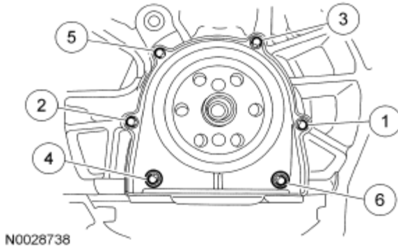
Fig. 462: Identifying Tightening Sequence Of Crankshaft Rear Main Oil Seal Bolts Courtesy of FORD MOTOR CO.
