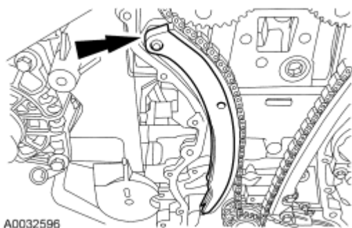
Fig. 396: Locating RH Timing Chain Guide Courtesy of FORD MOTOR CO.
