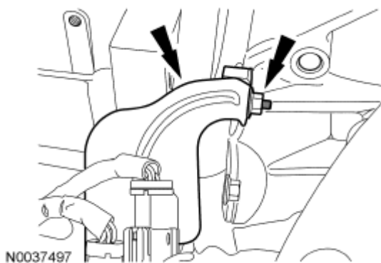
Fig. 641: Locating Engine Wiring Harness Bracket And Nut Courtesy of FORD MOTOR CO.
