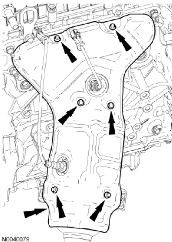
Fig. 542: Locating Heat Shield Screws Courtesy of FORD MOTOR CO.
