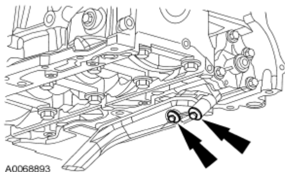
Fig. 460: Locating Oil Pump Pickup Tube Bolts Courtesy of FORD MOTOR CO.
