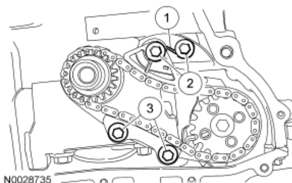
Fig. 401: Locating Tensioner Shoulder Bolts, Tensioner Spring And Guide Courtesy of FORD MOTOR CO.
