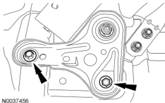
Fig. 621: Locating Subframe Bracket-To-Body Bolts Courtesy of FORD MOTOR CO.
