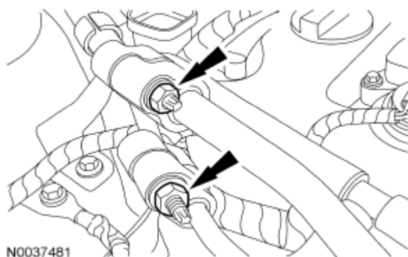
Fig. 237: Locating A/C Tubes Nuts Courtesy of FORD MOTOR CO.
