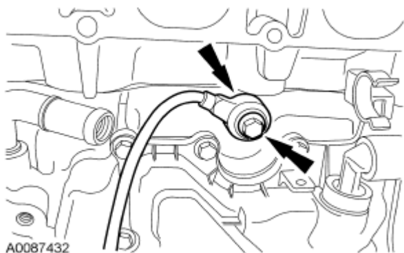
Fig. 373: Locating KS And Bolt Courtesy of FORD MOTOR CO.
