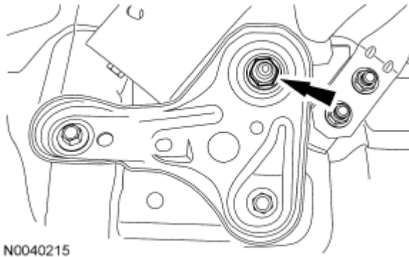
Fig. 678: Locating Subframe Nut Courtesy of FORD MOTOR CO.
