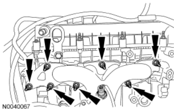
Fig. 355: Locating Nuts, Catalytic Converter, Gasket And Studs Courtesy of FORD MOTOR CO.
