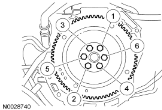
Fig. 570: Identifying Tightening Sequence Of Flexplate Bolts Courtesy of FORD MOTOR CO.
