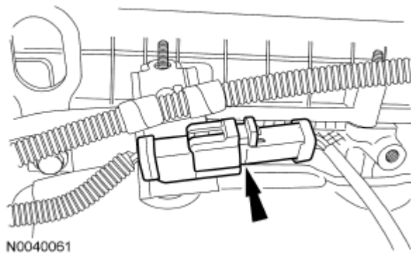
Fig. 350: Locating Heated Oxygen Sensor (HO2S) Electrical Connector Courtesy of FORD MOTOR CO.
