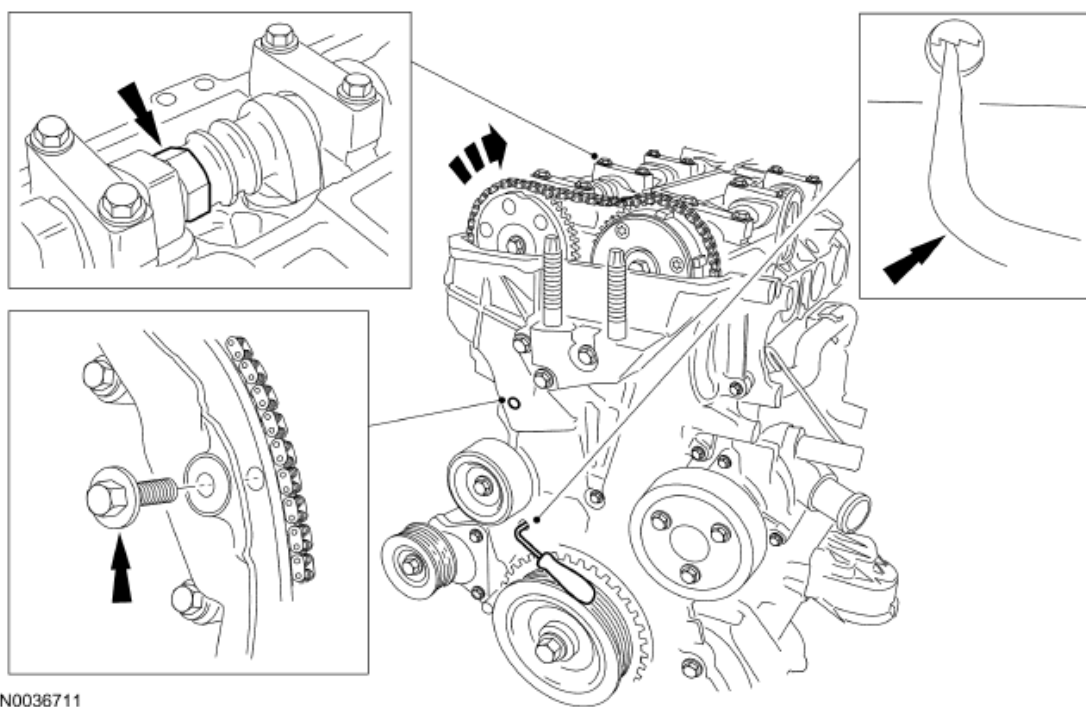
Fig. 102: Identifying Small Pick Tool And Timing Chain Tensioner Ratchet Courtesy of FORD MOTOR CO.
