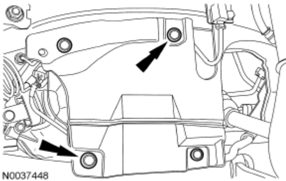
Fig. 270: Locating LH Splash Shield And Pin-Type Retainers Courtesy of FORD MOTOR CO.
