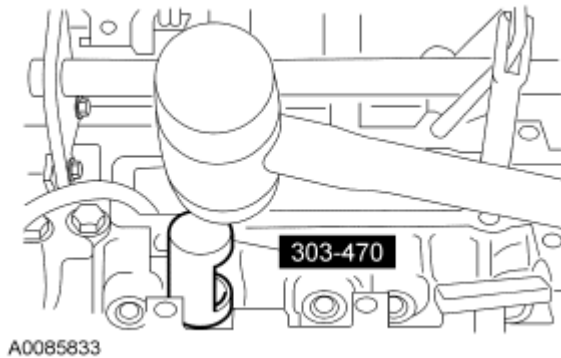
Fig. 158: Installing Valve Seal Courtesy of FORD MOTOR CO.
