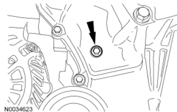
Fig. 100: Locating Upper Timing Hole Plug Courtesy of FORD MOTOR CO.
