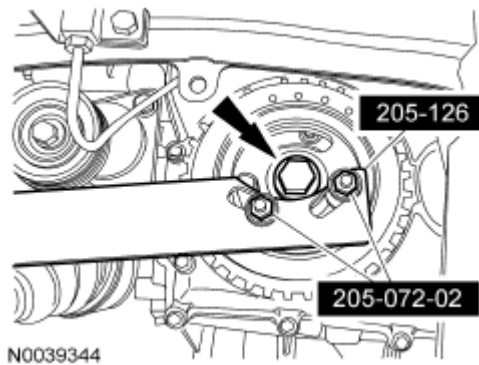
Fig. 43: Identifying Special Tools And Crankshaft Pulley Bolt Courtesy of FORD MOTOR CO.
