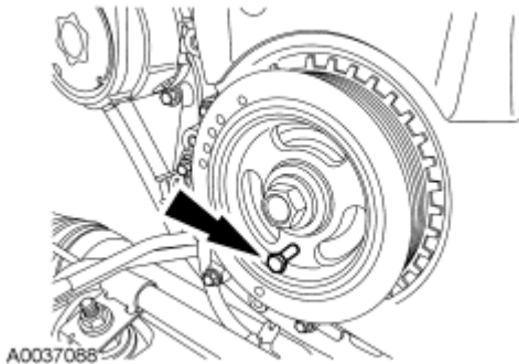
Fig. 504: Installing Bolt Through Crankshaft Pulley And Thread It Into Front Cover Courtesy of FORD MOTOR CO.
