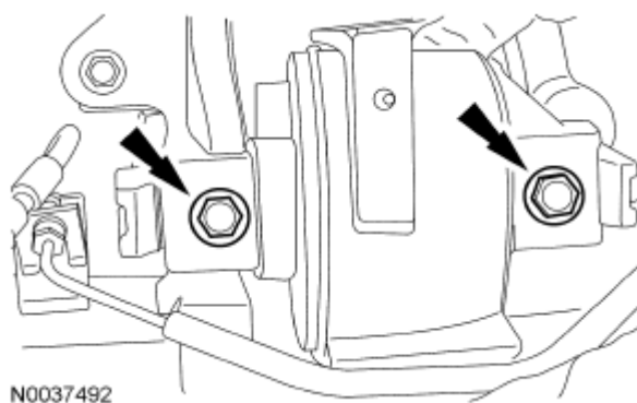
Fig. 645: Locating Transaxle Mount Bolts Courtesy of FORD MOTOR CO.
