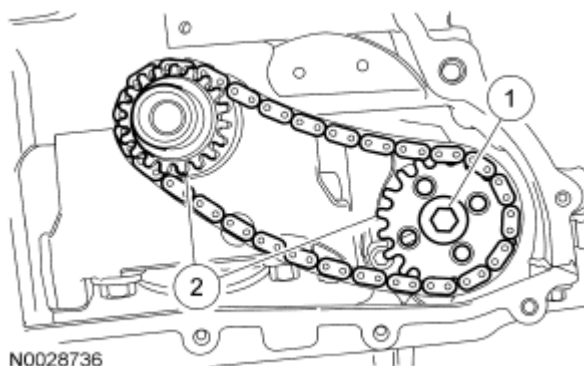
Fig. 402: Locating Sprockets And Bolt Courtesy of FORD MOTOR CO.
