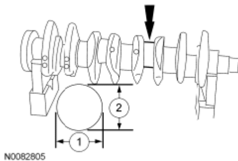
Fig. 440: Identifying Measuring Directions Of Crankshaft Connecting Rod Bearing Journal Diameters
