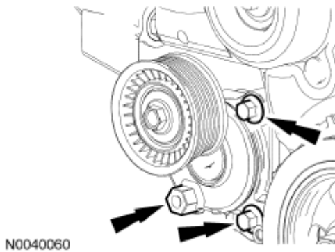
Fig. 567: Locating Accessory Drive Belt Tensioner Bolts Courtesy of FORD MOTOR CO.
