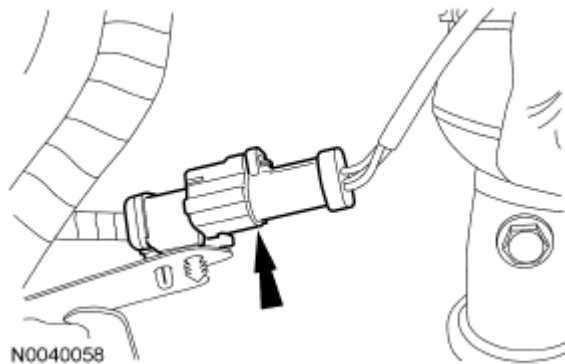
Fig. 349: Locating CMS Electrical Connector Courtesy of FORD MOTOR CO.
