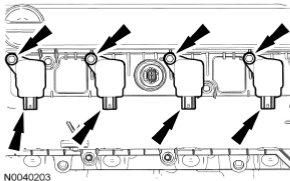
Fig. 384: Locating Coil-On-Plug Assemblies And Bolts Courtesy of FORD MOTOR CO.
