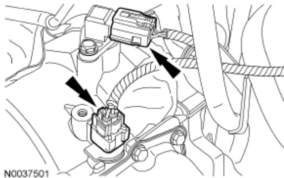
Fig. 256: Locating Transaxle Control Electrical Connectors
