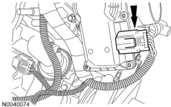
Fig. 529: Locating Electronic Throttle Body Electrical Connector Courtesy of FORD MOTOR CO.
