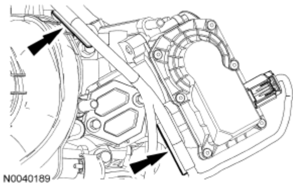
Fig. 530: Locating Wiring Harness Pin-Type Retainers Courtesy of FORD MOTOR CO.
