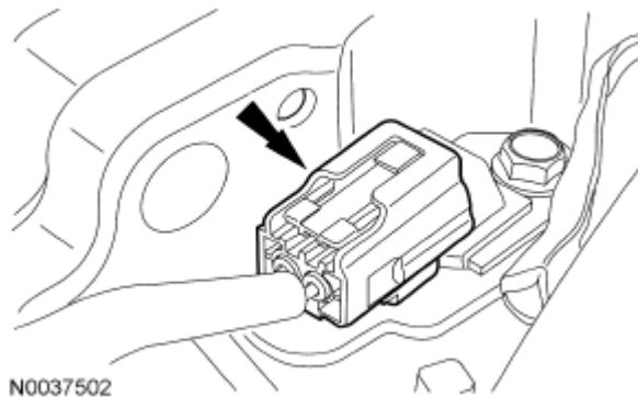
Fig. 257: Locating Turbine Shaft Speed (TSS) Sensor Electrical Connector
