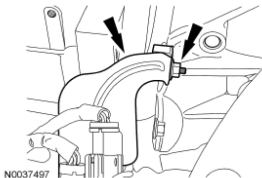
Fig. 317: Locating Engine Wiring Harness Bracket And Nut Courtesy of FORD MOTOR CO.
