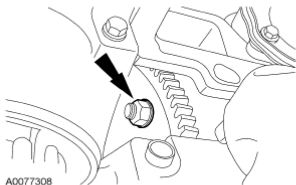
Fig. 252: Locating Torque Converter Nuts Courtesy of FORD MOTOR CO.
