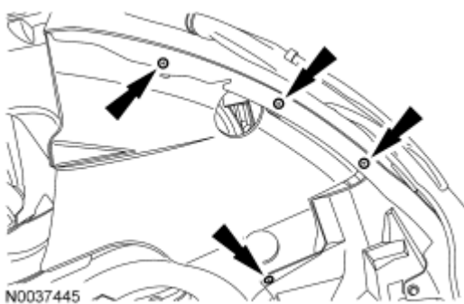
Fig. 203: Locating RH Fender Splash Shield Screws
