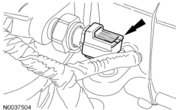
Fig. 259: Locating Transaxle Pressure Switch Electrical Connector Courtesy of FORD MOTOR CO.
