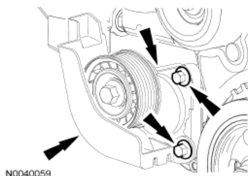
Fig. 326: Locating Pin-Type Retainer, Bolts, Shield And Tensioner Courtesy of FORD MOTOR CO.
