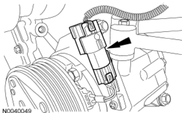
Fig. 560: Locating A/C Compressor Electrical Connector Courtesy of FORD MOTOR CO.
