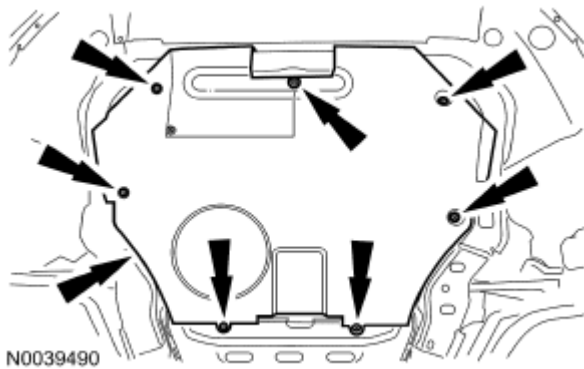
Fig. 264: Locating Underbody Cover Screws Courtesy of FORD MOTOR CO.
