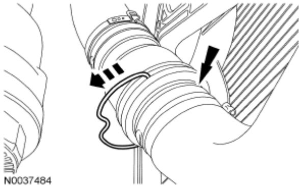
Fig. 240: Removing Retaining Clip And Identifying Lower Radiator Hose Courtesy of FORD MOTOR CO.
