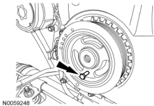
Fig. 491: Locating Bolt Courtesy of FORD MOTOR CO.
