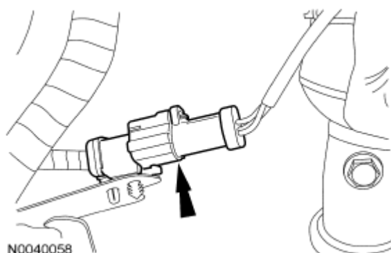
Fig. 546: Locating CMS Electrical Connector Courtesy of FORD MOTOR CO.
