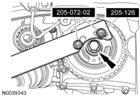
Fig. 39: Locating Crankshaft Pulley Bolt And Special Tool Courtesy of FORD MOTOR CO.
