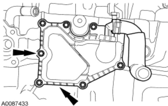
Fig. 374: Locating Crankcase Vent Oil Separator And Bolts Courtesy of FORD MOTOR CO.
