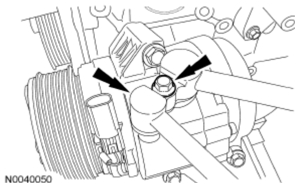
Fig. 335: Locating A/C Manifold And Bolt Courtesy of FORD MOTOR CO.
