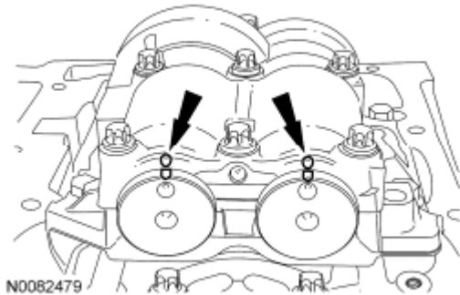
Fig. 452: Locating Balancer Unit And Shafts Reference Mark
