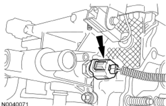
Fig. 359: Locating Coolant Temperature Sender Electrical Connector Courtesy of FORD MOTOR CO.
