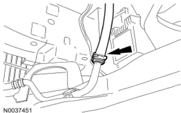
Fig. 273: Locating Power Steering Cooler Tube Courtesy of FORD MOTOR CO.
