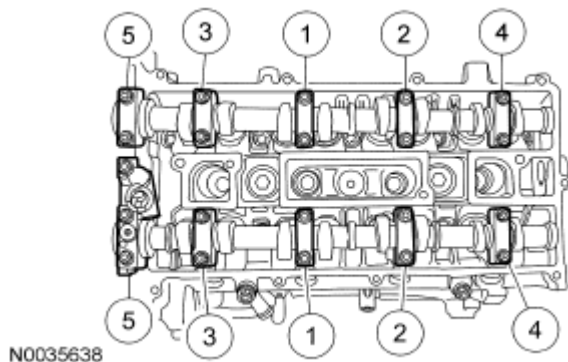
Fig. 172: Identifying Tightening Sequence Of Camshaft Bearing Caps Courtesy of FORD MOTOR CO.
