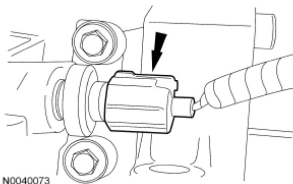
Fig. 361: Locating Oil Pressure Sender Electrical Connector Courtesy of FORD MOTOR CO.
