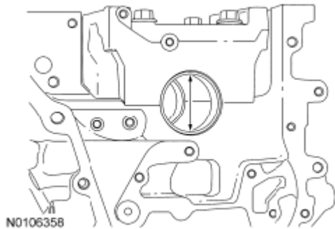
Fig. 437: Identifying Crankshaft Block Main Bearing Bore Diameter
