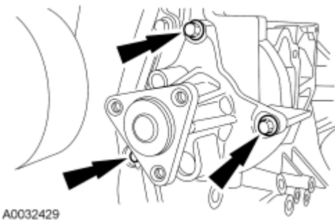
Fig. 556: Locating Coolant Pump Bolts Courtesy of FORD MOTOR CO.
