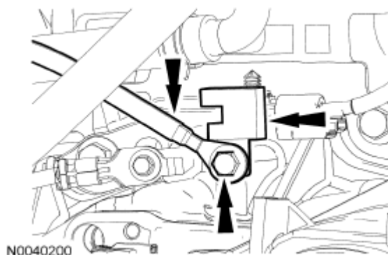
Fig. 658: Locating Radio Frequency Interference Capacitor, Ground Wire And Bolt Courtesy of FORD MOTOR CO.
