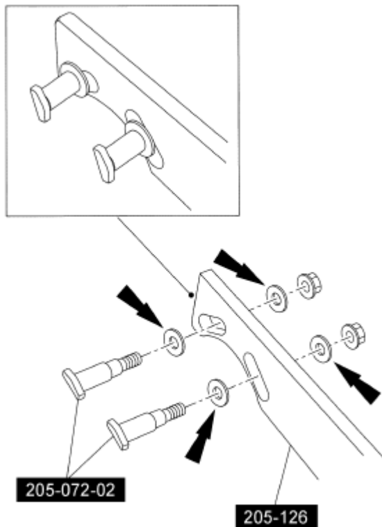
Fig. 38: Locating Special Tools And Hardened Washers Courtesy of FORD MOTOR CO.
