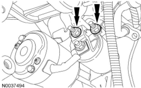
Fig. 585: Locating Starter Wire Nuts Courtesy of FORD MOTOR CO.
