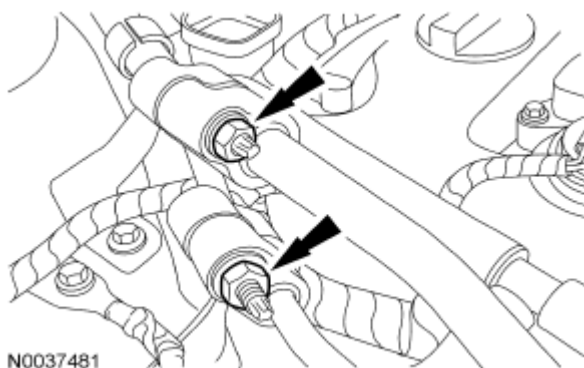
Fig. 598: Locating A/C Tubes Nuts Courtesy of FORD MOTOR CO.
