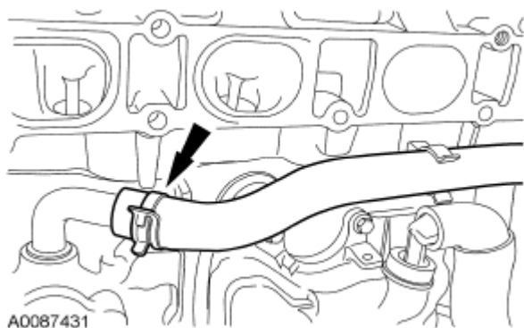
Fig. 371: Locating Bypass Hose From Cylinder Block Nipple Courtesy of FORD MOTOR CO.
