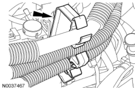
Fig. 666: Locating Evaporative Emissions (EVAP) Tube Bundle Retaining Clip Courtesy of FORD MOTOR CO.
