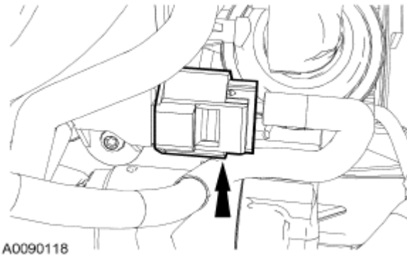
Fig. 362: Locating Manifold Actual Pressure (MAP) Sensor Electrical Connector Courtesy of FORD MOTOR CO.
