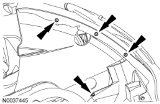
Fig. 630: Locating RH Fender Splash Shield Screws Courtesy of FORD MOTOR CO.
