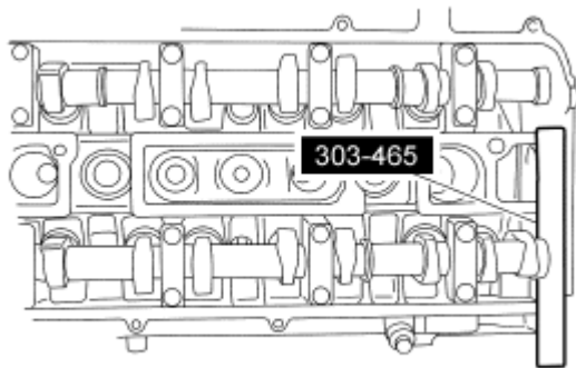
Fig. 104: Locating Special Tool Courtesy of FORD MOTOR CO.
