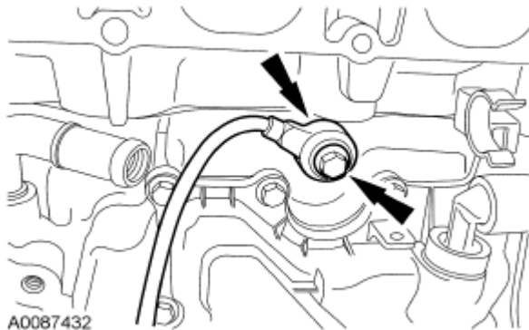
Fig. 522: Locating Knock Sensor Bolts Courtesy of FORD MOTOR CO.
