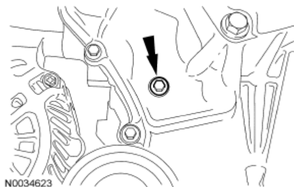
Fig. 130: Locating Upper Timing Hole Plug Courtesy of FORD MOTOR CO.
