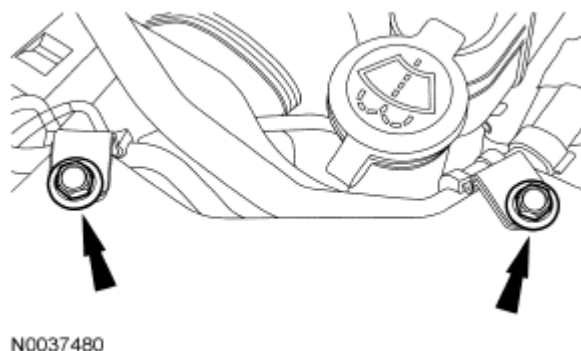
Fig. 301: Locating A/C Tube Bracket Bolts Courtesy of FORD MOTOR CO.
