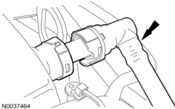
Fig. 288: Locating Crankcase Vent Tube Courtesy of FORD MOTOR CO.
