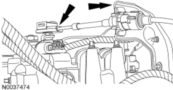
Fig. 231: Locating Transaxle Control Cable From Control Lever Courtesy of FORD MOTOR CO.
