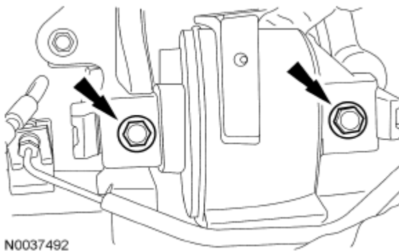
Fig. 586: Locating Transaxle Mount Bolts Courtesy of FORD MOTOR CO.
