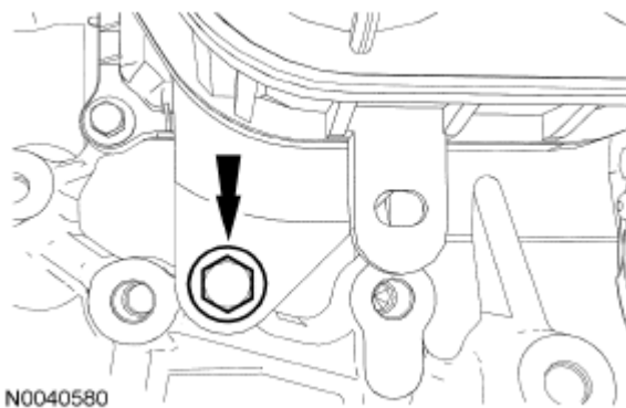
Fig. 24: Locating Intake Manifold Lower Bolt Courtesy of FORD MOTOR CO.
