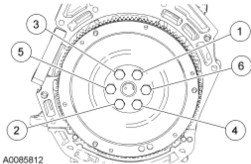
Fig. 571: Identifying Flexplate Bolts Tightening Sequence Courtesy of FORD MOTOR CO.
