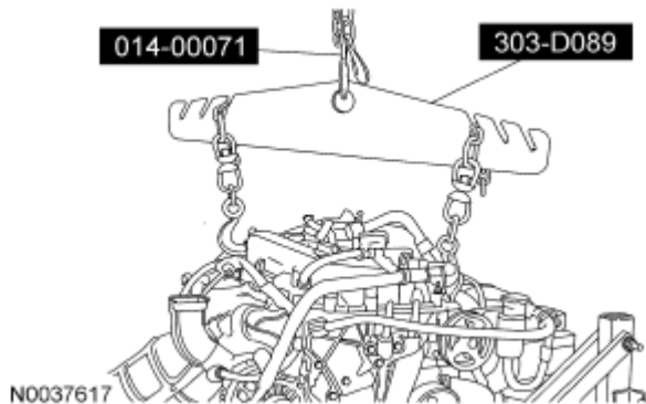
Fig. 320: Identifying Special Tools Courtesy of FORD MOTOR CO.
