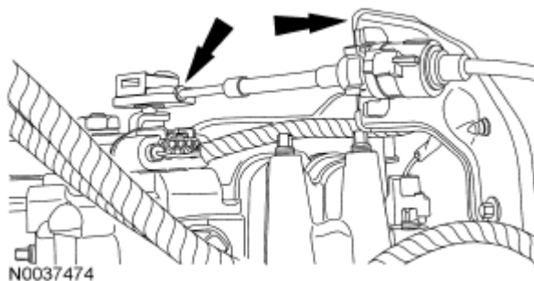
Fig. 604: Locating Transaxle Control Cable Courtesy of FORD MOTOR CO.
