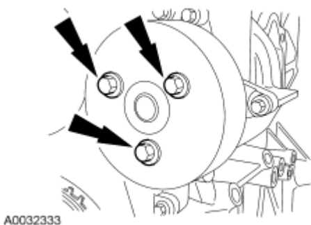
Fig. 337: Locating Coolant Pump Pulley Bolts Courtesy of FORD MOTOR CO.
