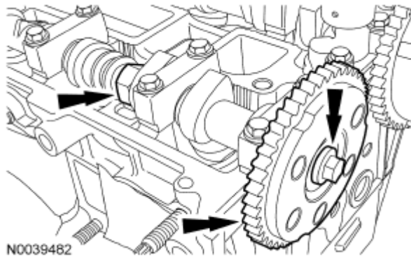
Fig. 399: Locating Bolt And Exhaust Camshaft Sprocket Courtesy of FORD MOTOR CO.
