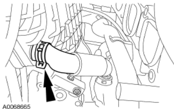
Fig. 368: Locating Positive Crankcase Ventilation (PCV) Hose Courtesy of FORD MOTOR CO.
