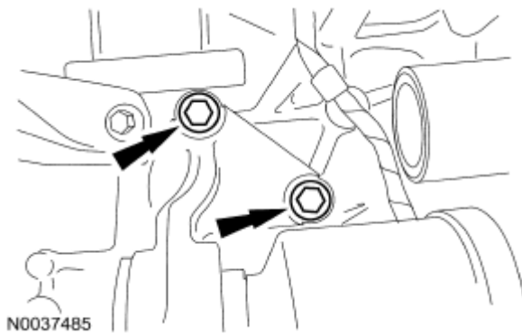
Fig. 650: Locating RH Halfshaft Carrier Bearing Bracket Bolts Courtesy of FORD MOTOR CO.
