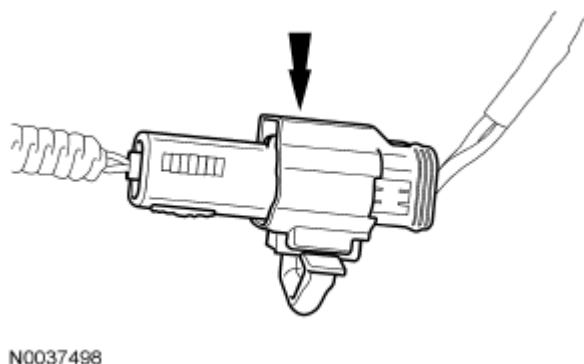
Fig. 318: Locating Backup Lamp Electrical Connector Courtesy of FORD MOTOR CO.
