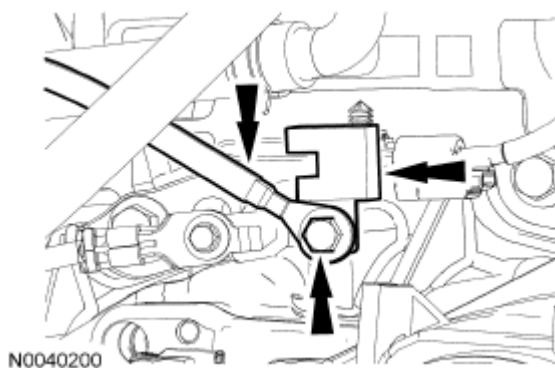
Fig. 299: Locating Bolt, Radio Frequency Interference Capacitor And Ground Wire Courtesy of FORD MOTOR CO.
