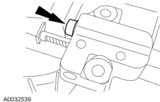
Fig. 481: Locating Timing Chain Tensioner Plunger Courtesy of FORD MOTOR CO.
