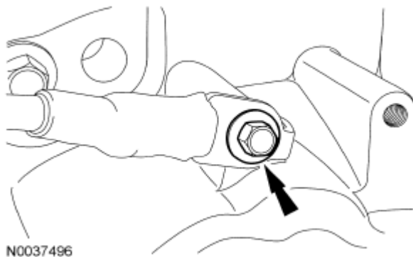
Fig. 642: Locating Ground Wire Bolt Courtesy of FORD MOTOR CO.
