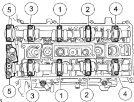
Fig. 110: Identifying Tightening Sequence Of Camshaft Bearing Cap Bolts Courtesy of FORD MOTOR CO.
