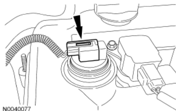
Fig. 518: Locating VCT Solenoid Electrical Connector Courtesy of FORD MOTOR CO.
