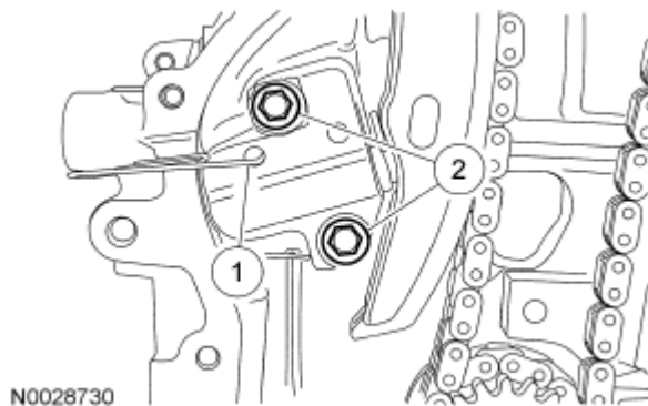
Fig. 395: Locating Timing Chain Tensioner Bolts And Paper Clip Courtesy of FORD MOTOR CO.
