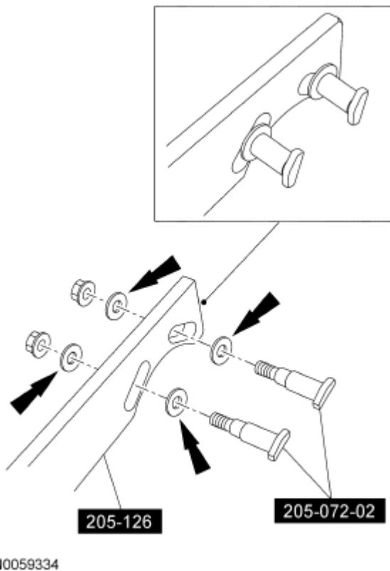
Fig. 42: Locating Special Tools And Hardened Washers Courtesy of FORD MOTOR CO.
