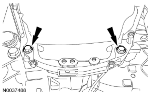
Fig. 590: Locating Oil Pan-To-Bellhousing Bolts Courtesy of FORD MOTOR CO.
