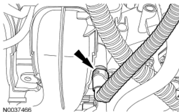
Fig. 609: Locating EVAP Tube Courtesy of FORD MOTOR CO.
