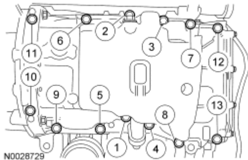
Fig. 65: Identifying Tightening Sequence Of Oil Pan Bolts Courtesy of FORD MOTOR CO.
