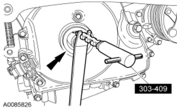
Fig. 56: Locating Special Tool And Crankshaft Front Oil Seal Courtesy of FORD MOTOR CO.
