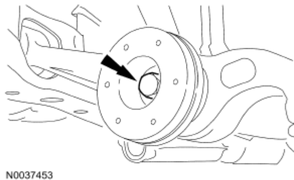
Fig. 213: Locating Lower Control Arms Through Bolt Courtesy of FORD MOTOR CO.
