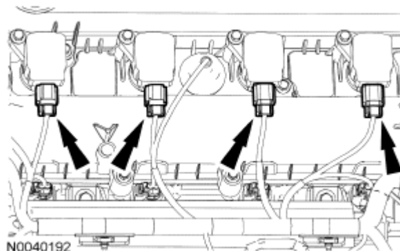
Fig. 378: Locating Coil-On-Plug Electrical Connectors Courtesy of FORD MOTOR CO.
