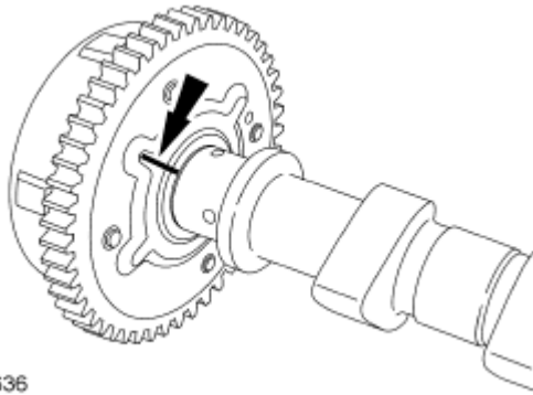
Fig. 109: Locating Mark On Sprocket Courtesy of FORD MOTOR CO.
