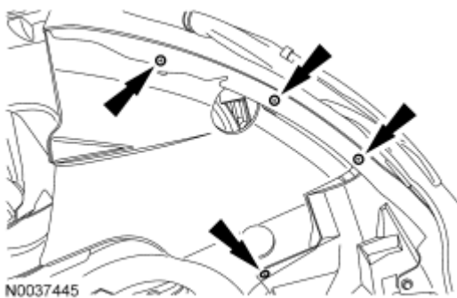
Fig. 267: Locating RH Fender Splash Shield Screws
