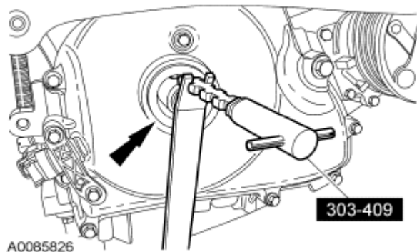
Fig. 69: Locating Crankshaft Front Oil Seal And Special Tool Courtesy of FORD MOTOR CO.
