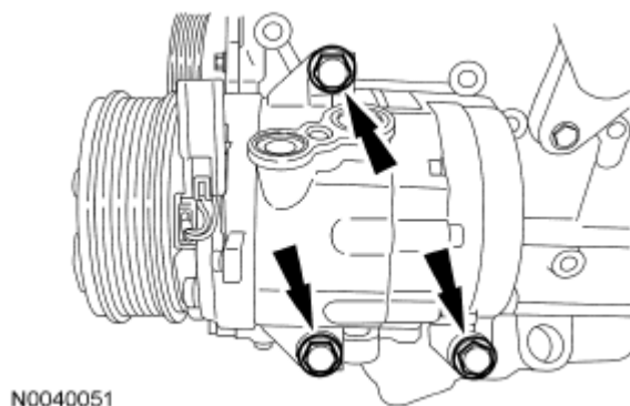
Fig. 558: Locating A/C Compressor Bolts Courtesy of FORD MOTOR CO.
