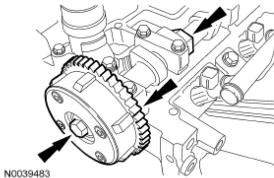
Fig. 400: Locating Intake Camshaft Phaser And Sprocket Bolt Courtesy of FORD MOTOR CO.
