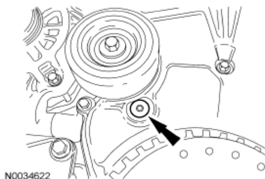
Fig. 119: Locating Lower Front Cover Timing Hole Plug Courtesy of FORD MOTOR CO.
