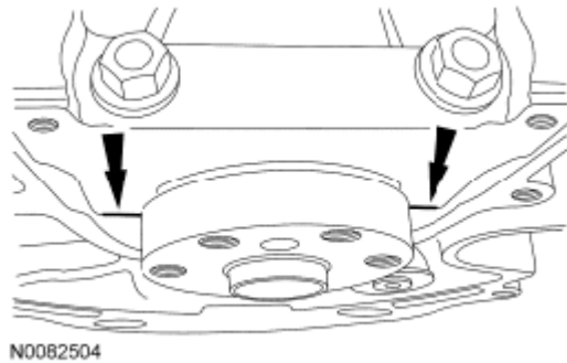
Fig. 435: Locating Main Bearing Beam
