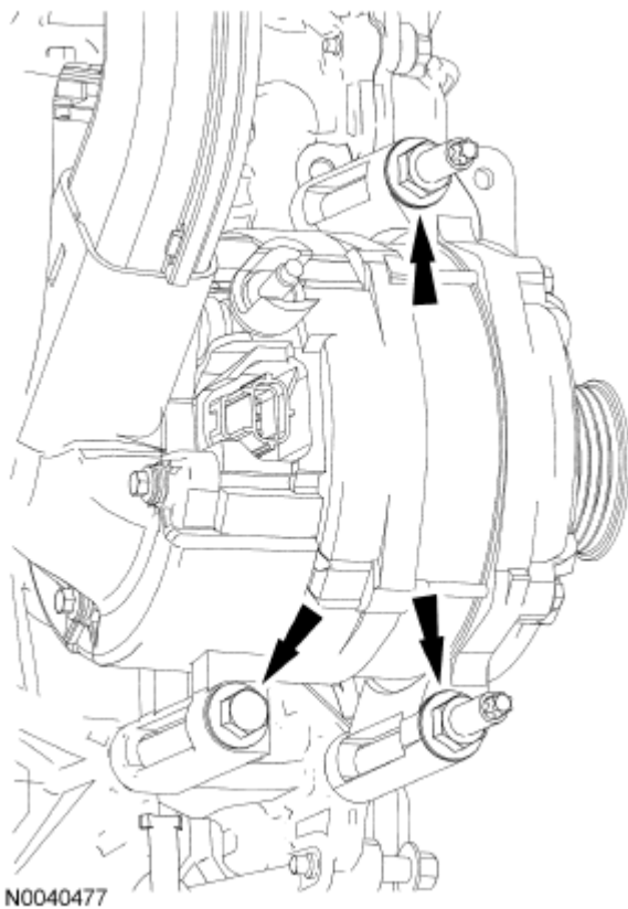
Fig. 344: Locating Bolt, Stud Bolts And Generator Courtesy of FORD MOTOR CO.
