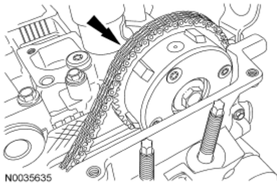
Fig. 142: Locating Timing Chain Courtesy of FORD MOTOR CO.
