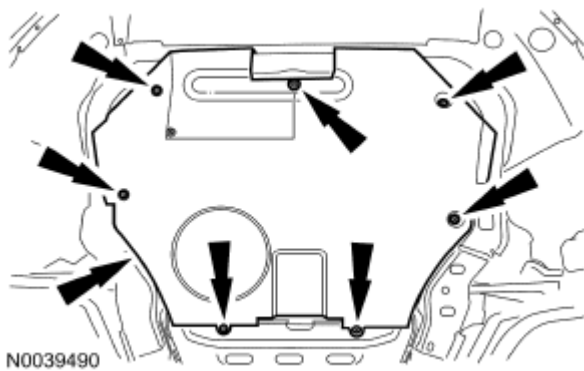
Fig. 200: Locating Underbody Cover Screws Courtesy of FORD MOTOR CO.
