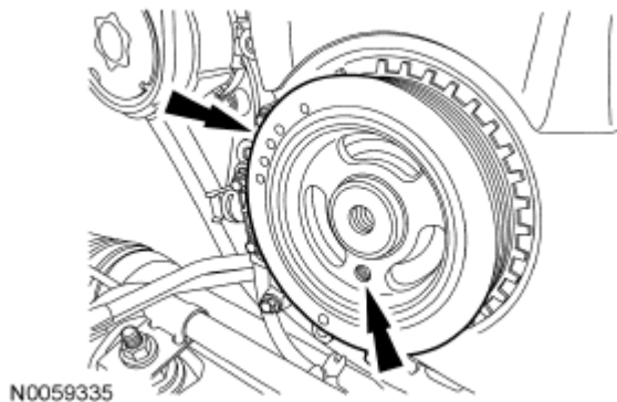
Fig. 40: Locating Holes In Crankshaft Pulley Courtesy of FORD MOTOR CO.
