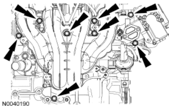
Fig. 367: Locating Intake Manifold Bolts Courtesy of FORD MOTOR CO.
