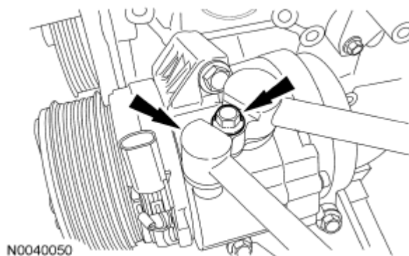
Fig. 559: Locating A/C Manifold And Bolt Courtesy of FORD MOTOR CO.
