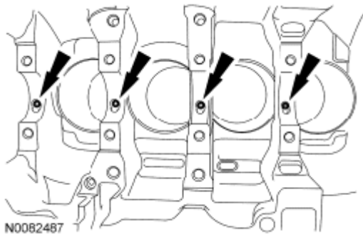
Fig. 422: Locating Oil Squirters
