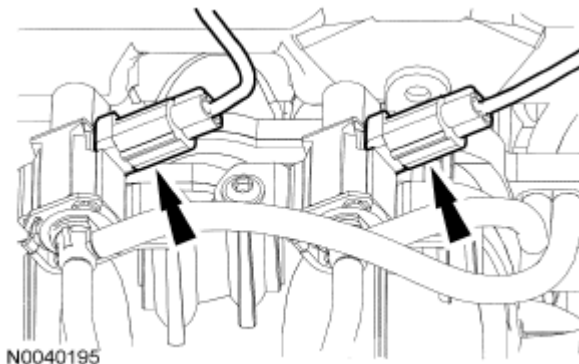
Fig. 364: Locating Swirl Control Valve Electrical Connectors Courtesy of FORD MOTOR CO.
