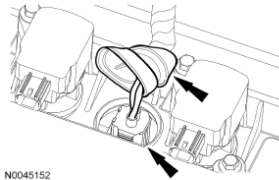
Fig. 516: Locating Cylinder Head Temperature (CHT) Sensor Electrical Connector And Boot Courtesy of FORD MOTOR CO.
