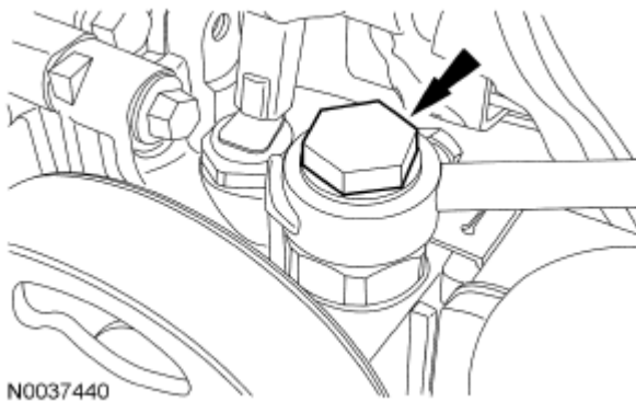
Fig. 693: Locating Power Steering Pump Bolt Courtesy of FORD MOTOR CO.
