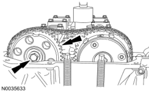
Fig. 143: Locating Exhaust Camshaft Drive Gear Bolt Courtesy of FORD MOTOR CO.
