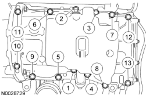
Fig. 465: Identifying Tightening Sequence Of Oil Pan Bolts
