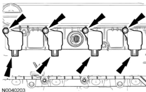
Fig. 510: Locating Coil-On-Plug Assemblies And Bolts Courtesy of FORD MOTOR CO.
