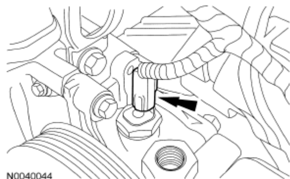
Fig. 328: Locating Power Steering Pressure (PSP) Switch Electrical Connector Courtesy of FORD MOTOR CO.
