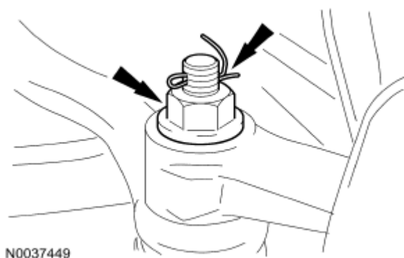
Fig. 626: Locating Tie-Rod Ends Nuts And Cotter Pin Courtesy of FORD MOTOR CO.
