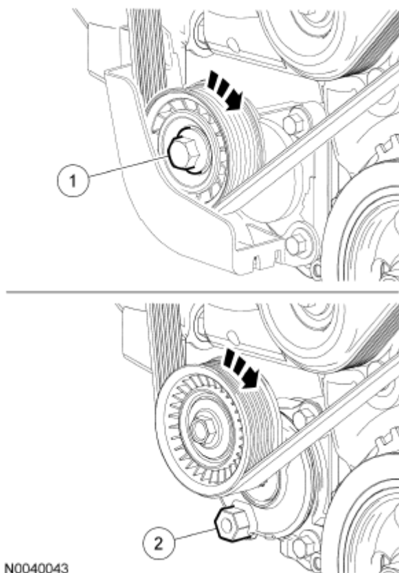
Fig. 325: Using Pulley Bolt To Rotate Tensioner And Using Hex Feature To Rotate Tensioner Courtesy of FORD MOTOR CO.
