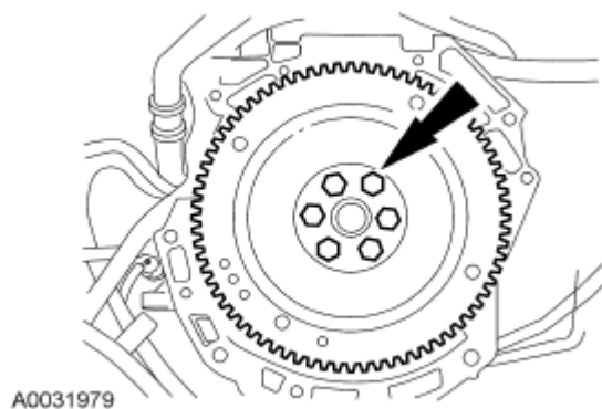
Fig. 324: Locating Flexplate Bolts Courtesy of FORD MOTOR CO.
