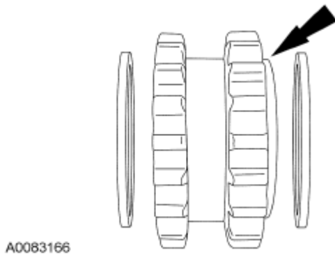
Fig. 472: Locating Crankshaft Sprocket, Crankshaft Sprocket Diamond Washers, Oil Pump Chain And Oil Pump Sprocket Courtesy of FORD MOTOR CO.
