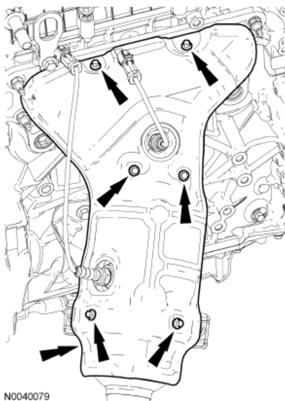
Fig. 353: Locating Heat Shield And Screws Courtesy of FORD MOTOR CO.
