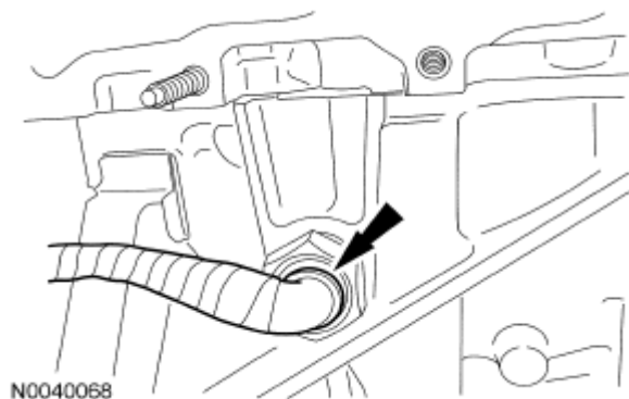
Fig. 539: Locating Block Heater Electrical Connector
