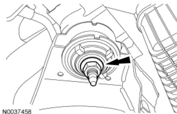
Fig. 676: Locating Front Subframe Nuts Courtesy of FORD MOTOR CO.
