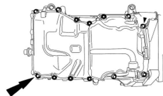
Fig. 408: Locating Oil Pan Bolts Courtesy of FORD MOTOR CO.
