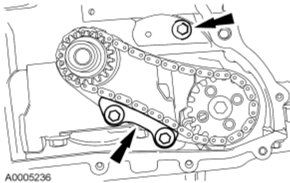
Fig. 474: Locating Oil Pump Chain Guide And Shoulder Bolts Courtesy of FORD MOTOR CO.
