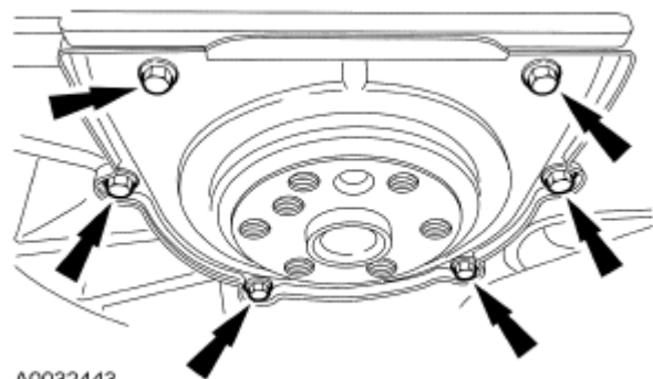
Fig. 409: Locating Rear Crankshaft Seal Bolts Courtesy of FORD MOTOR CO.
