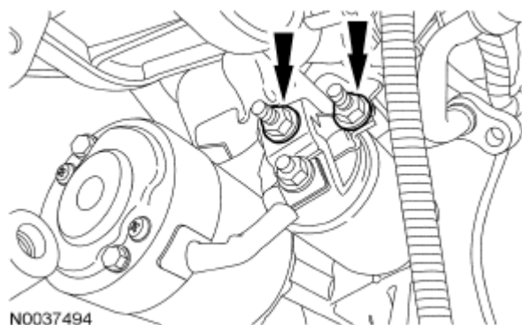
Fig. 314: Locating Starter Wires Nuts Courtesy of FORD MOTOR CO.
