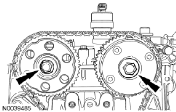
Fig. 90: Locating Camshaft Sprocket Bolts Courtesy of FORD MOTOR CO.
