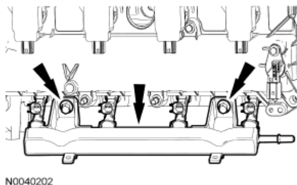
Fig. 383: Locating Fuel Rail And Bolts Courtesy of FORD MOTOR CO.
