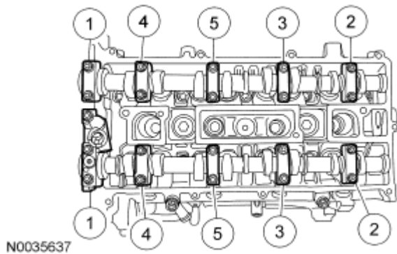
Fig. 405: Identifying Loosening Sequence Of Camshaft Bearing Caps Bolts Courtesy of FORD MOTOR CO.
