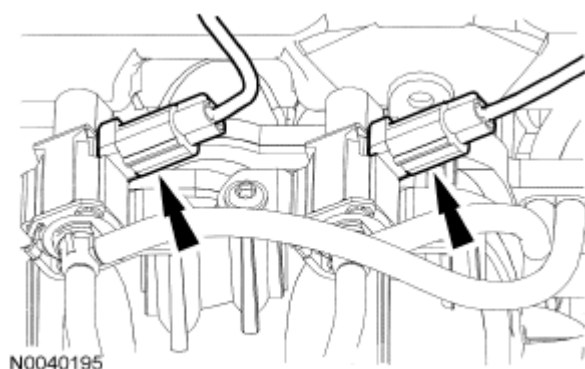
Fig. 531: Locating Swirl Control Valve Electrical Connectors Courtesy of FORD MOTOR CO.
