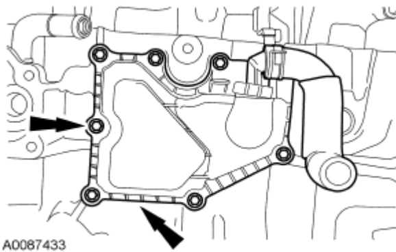
Fig. 521: Locating Crankcase Vent Oil Separator And Bolts Courtesy of FORD MOTOR CO.
