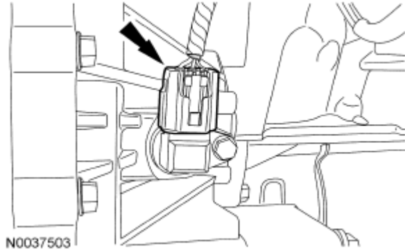
Fig. 258: Locating Output Shaft Speed (OSS) Sensor Electrical Connector Courtesy of FORD MOTOR CO.
