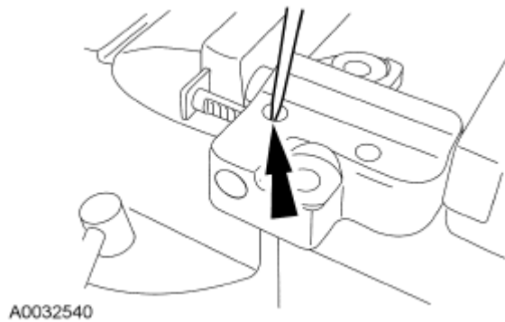
Fig. 482: Using Small Pick To Push Back Courtesy of FORD MOTOR CO.
