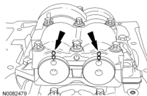
Fig. 413: Locating Balancer Unit And Shafts Reference Mark
