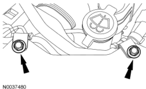
Fig. 236: Locating A/C Tube Bracket Bolts Courtesy of FORD MOTOR CO.
