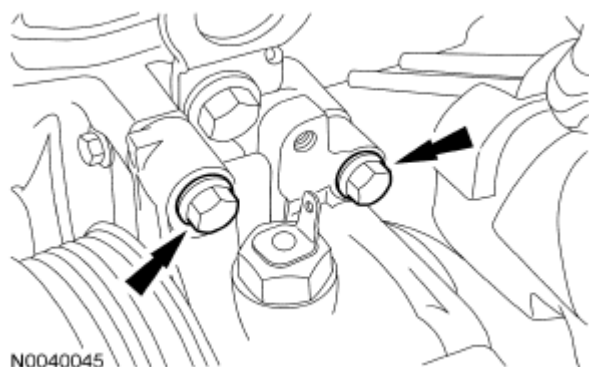
Fig. 329: Locating Upper Power Steering Pump Bolts Courtesy of FORD MOTOR CO.
