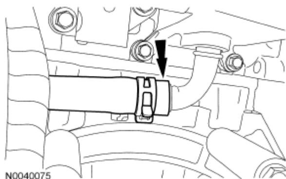
Fig. 523: Locating Bypass Hose To Coolant Outlet Courtesy of FORD MOTOR CO.
