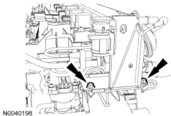
Fig. 348: Locating AIR Valve Bolts Courtesy of FORD MOTOR CO.
