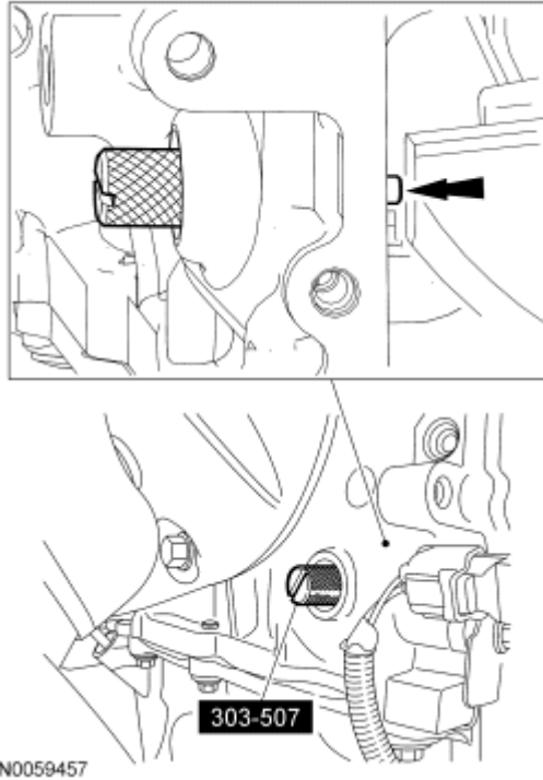
Fig. 458: Identifying Special Tool (303-507)
