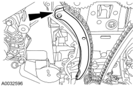
Fig. 480: Locating RH Timing Chain Guide Courtesy of FORD MOTOR CO.
