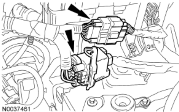
Fig. 672: Locating Engine Wiring Harness Electrical Connectors Courtesy of FORD MOTOR CO.
