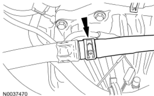
Fig. 663: Locating Heater Hose Inline Connector Courtesy of FORD MOTOR CO.
