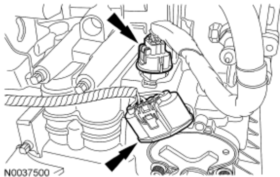
Fig. 580: Locating Transmission Range (TR) Sensor And Primary Control Solenoid Electrical Connectors Courtesy of FORD MOTOR CO.
