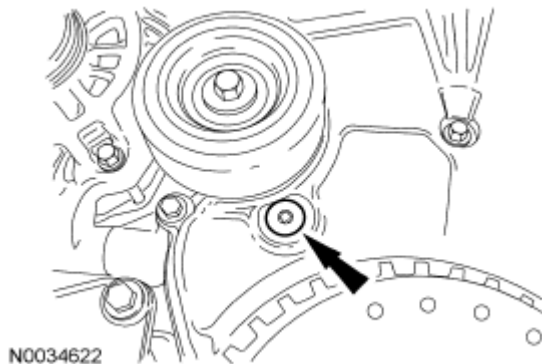
Fig. 149: Locating Lower Timing Hole Plug Courtesy of FORD MOTOR CO.
