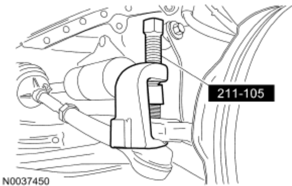
Fig. 208: Identifying Special Tool Courtesy of FORD MOTOR CO.
