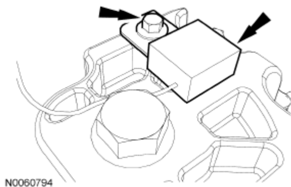
Fig. 239: Locating Radio Frequency Interference Capacitor Bolt Courtesy of FORD MOTOR CO.
