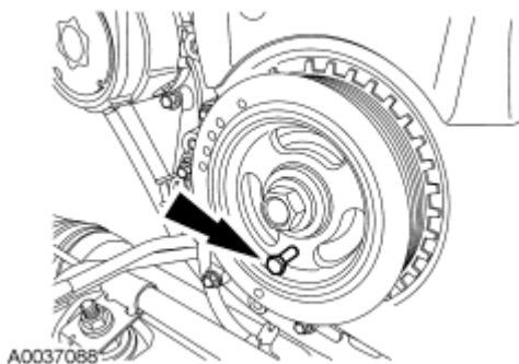
Fig. 499: Installing Bolt Through Crankshaft Pulley And Thread It Into Front Cover Courtesy of FORD MOTOR CO.
