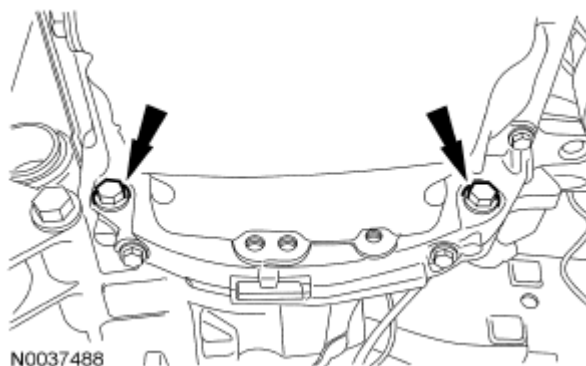
Fig. 647: Locating Oil Pan-To-Bellhousing Bolts Courtesy of FORD MOTOR CO.
