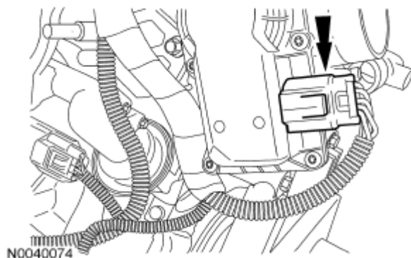
Fig. 366: Locating Electronic Throttle Body Electrical Connector Courtesy of FORD MOTOR CO.
