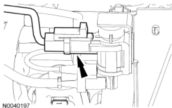
Fig. 548: Locating AIR Valve Electrical Connector Courtesy of FORD MOTOR CO.
