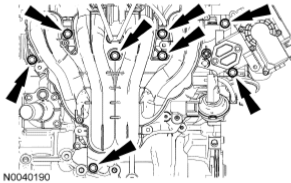
Fig. 528: Locating Intake Manifold Bolts Courtesy of FORD MOTOR CO.
