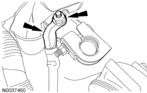
Fig. 673: Locating Battery Cable And Nut Courtesy of FORD MOTOR CO.
