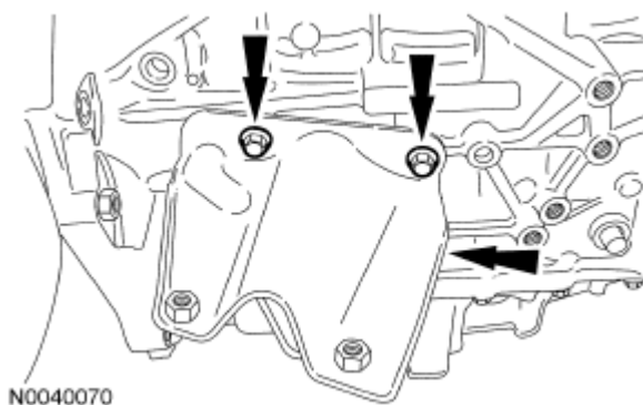
Fig. 537: Locating Catalytic Converter Bracket Bolts Courtesy of FORD MOTOR CO.
