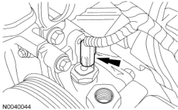
Fig. 566: Locating Power Steering Pressure (PSP) Switch Electrical Connector Courtesy of FORD MOTOR CO.
