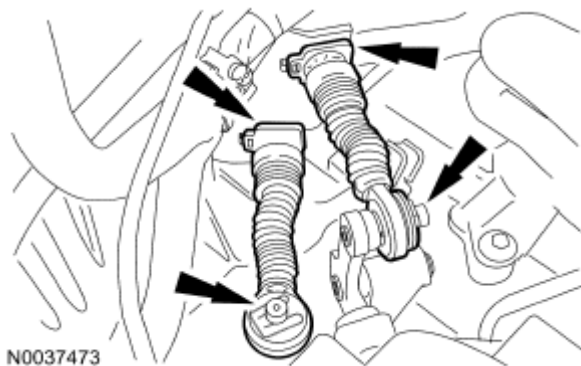
Fig. 660: Locating Transaxle Control Cables To Bracket Courtesy of FORD MOTOR CO.
