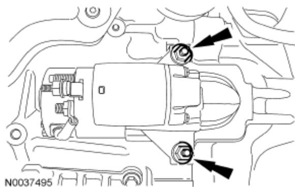
Fig. 251: Locating Starter Stud Bolts Courtesy of FORD MOTOR CO.
