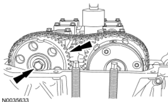
Fig. 113: Locating Timing Chain Gear And Bolt Courtesy of FORD MOTOR CO.
