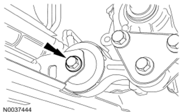
Fig. 266: Locating Engine Roll Restrictor Bolt
