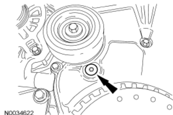
Fig. 99: Locating Lower Timing Hole Plug Courtesy of FORD MOTOR CO.
