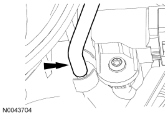
Fig. 549: Locating AIR Valve Vacuum Supply Tube Courtesy of FORD MOTOR CO.
