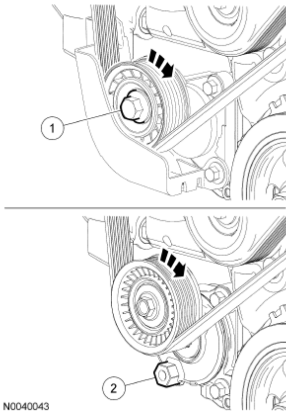
Fig. 569: Using Pulley Bolt And Hex Feature To Rotate Tensioner Courtesy of FORD MOTOR CO.
