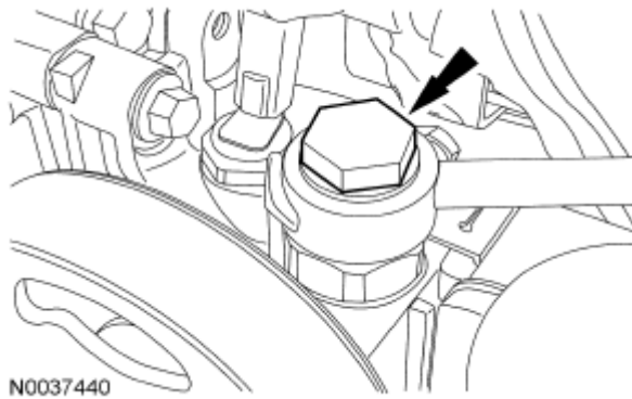
Fig. 199: Locating Bolt Courtesy of FORD MOTOR CO.
