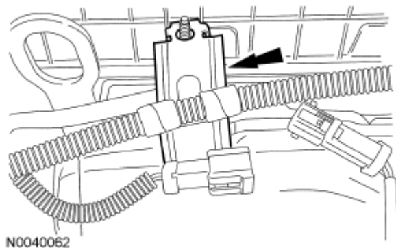
Fig. 351: Locating Wiring Harness Bracket
