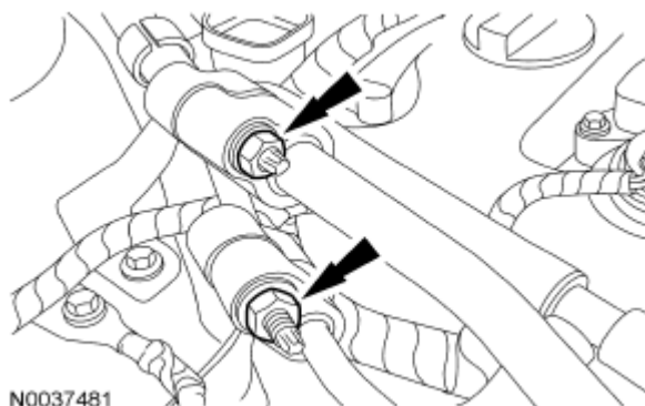
Fig. 302: Locating A/C Tubes Nuts Courtesy of FORD MOTOR CO.
