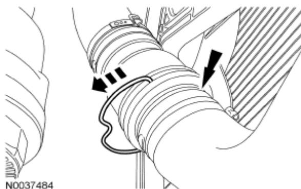
Fig. 305: Removing Retaining Clip And Locating Lower Radiator Hose Courtesy of FORD MOTOR CO.
