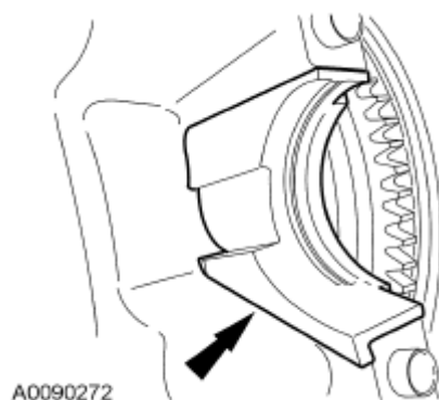
Fig. 322: Locating Starter Motor Isolator Courtesy of FORD MOTOR CO.
