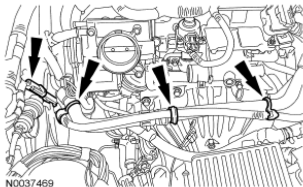
Fig. 664: Locating Block Heater Electrical Connector Harness Retaining Clips Courtesy of FORD MOTOR CO.
