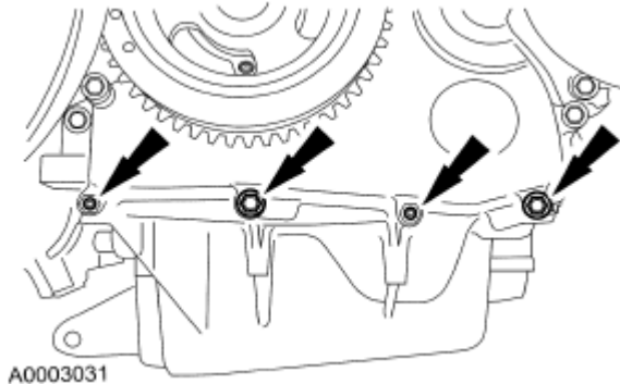
Fig. 64: Locating Oil Pan Bolts Courtesy of FORD MOTOR CO.
