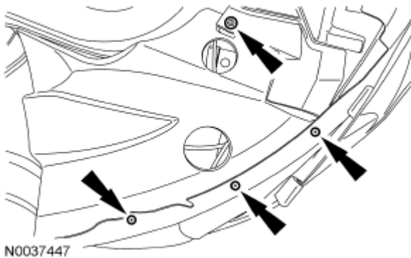
Fig. 205: Locating LH Fender Splash Shield Screws Courtesy of FORD MOTOR CO.
