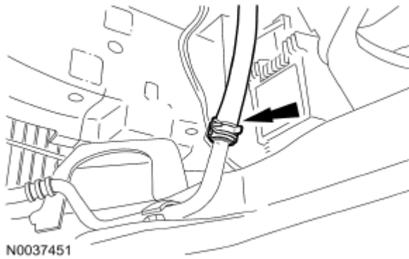
Fig. 625: Locating Power Steering Cooler Tube Courtesy of FORD MOTOR CO.
