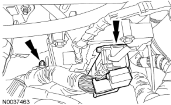
Fig. 287: Locating Powertrain Control Module (PCM) Electrical Connector And Pin-Type Retainer Courtesy of FORD MOTOR CO.
