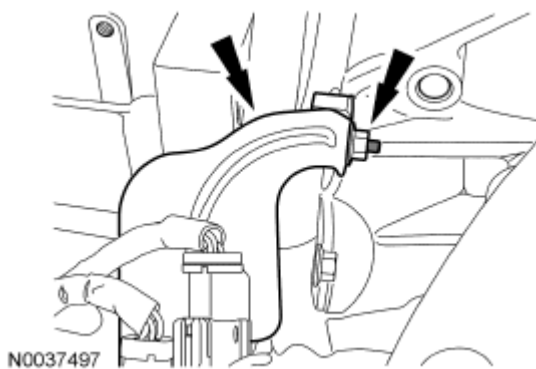
Fig. 581: Locating Engine Wiring Harness Bracket And Nut Courtesy of FORD MOTOR CO.
