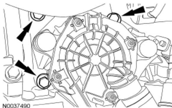
Fig. 246: Locating AIR Pump Bolts Courtesy of FORD MOTOR CO.
