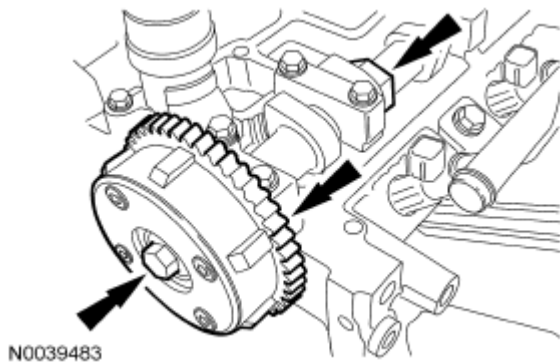
Fig. 84: Locating Bolt, Camshaft Phaser And Sprocket Courtesy of FORD MOTOR CO.
