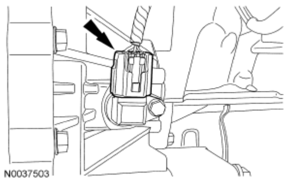
Fig. 577: Locating Output Shaft Speed (OSS) Sensor Electrical Connector Courtesy of FORD MOTOR CO.
