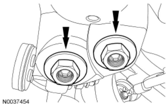
Fig. 211: Locating Lower Ball Joint Nuts Courtesy of FORD MOTOR CO.
