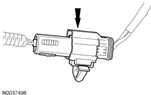
Fig. 640: Locating Backup Lamp Electrical Connector Courtesy of FORD MOTOR CO.
