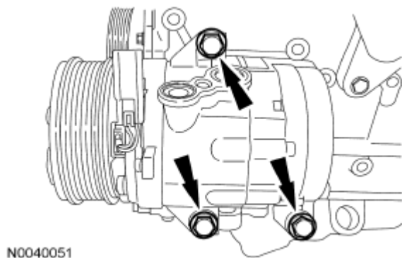
Fig. 336: Locating A/C Compressor And Bolts Courtesy of FORD MOTOR CO.
