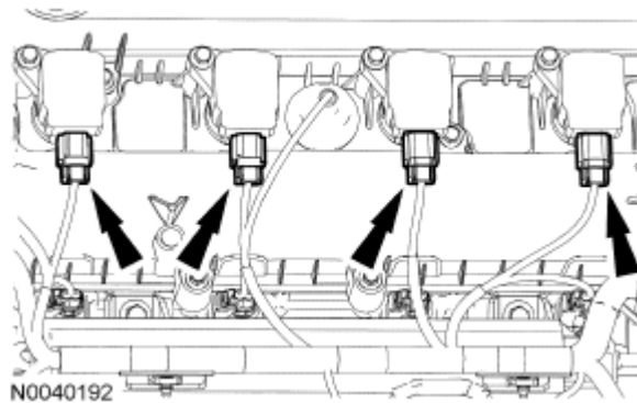
Fig. 517: Locating Coil-On-Plug Electrical Connectors Courtesy of FORD MOTOR CO.
