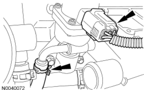
Fig. 535: Locating Exhaust Gas Recirculation (EGR) Coolant Hose And Electrical Connector Courtesy of FORD MOTOR CO.
