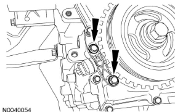
Fig. 341: Locating CKP Sensor Bolts Courtesy of FORD MOTOR CO.
