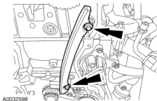
Fig. 478: Identifying Bolts And LH Timing Chain Guide Courtesy of FORD MOTOR CO.
