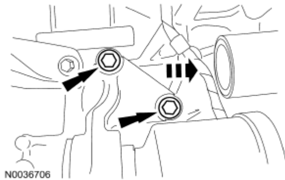
Fig. 95: Removing Halfshaft Carrier Bracket Bolts And Sliding Halfshaft Out Of Transaxle Courtesy of FORD MOTOR CO.
