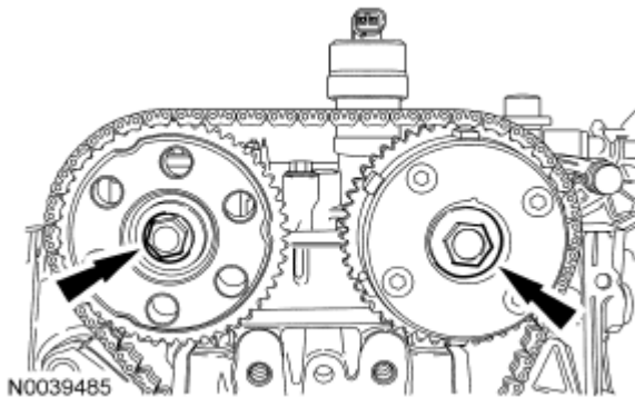
Fig. 486: Identifying Camshafts Sprocket Bolts Courtesy of FORD MOTOR CO.
