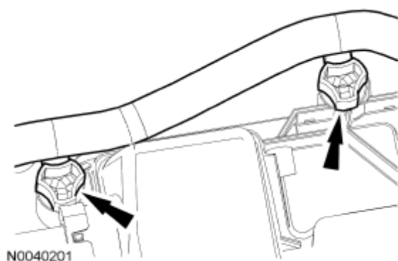
Fig. 382: Locating Wiring Harness Retainers Courtesy of FORD MOTOR CO.
