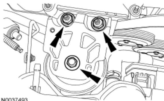
Fig. 249: Locating Engine Mount Bracket Bolt And Nuts Courtesy of FORD MOTOR CO.
