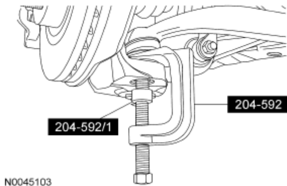
Fig. 276: Identifying Special Tools Courtesy of FORD MOTOR CO.
