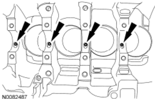
Fig. 433: Locating Oil Squirters
