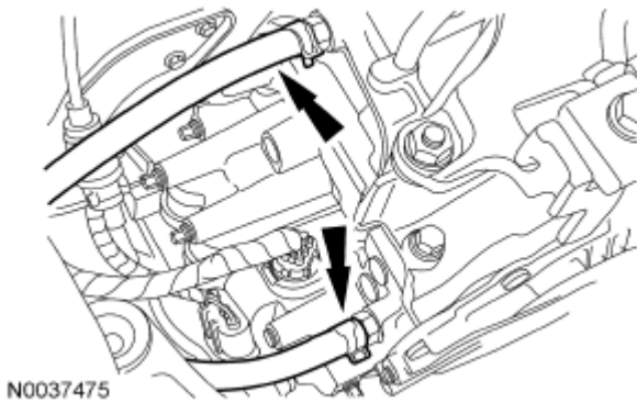
Fig. 232: Locating Transaxle Cooler Tubes Courtesy of FORD MOTOR CO.
