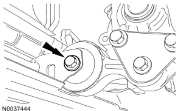
Fig. 689: Locating Engine Roll Restrictor Bolt Courtesy of FORD MOTOR CO.
