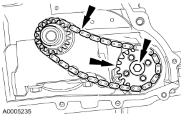
Fig. 473: Locating Oil Pump Chain, Sprocket And Bolt Courtesy of FORD MOTOR CO.
