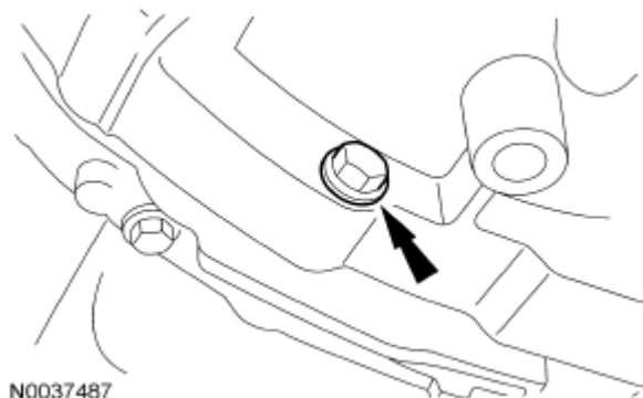
Fig. 243: Locating Bellhousing-To-Oil Pan Bolt Courtesy of FORD MOTOR CO.
