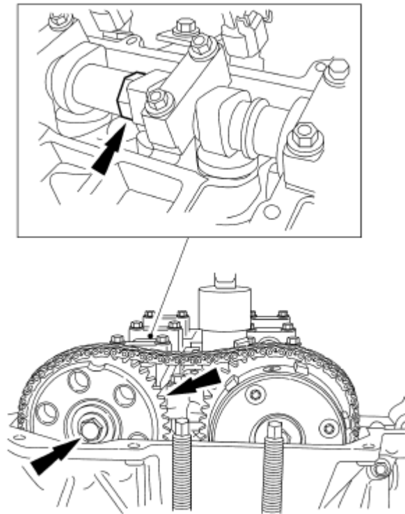
Fig. 133: Identifying Exhaust Camshaft Drive Gear Bolt Courtesy of FORD MOTOR CO.
