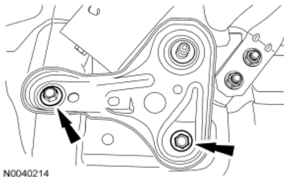
Fig. 619: Locating Subframe Brackets Bolts Courtesy of FORD MOTOR CO.
