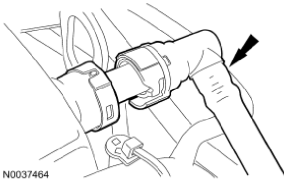
Fig. 224: Locating Crankcase Vent Tube Courtesy of FORD MOTOR CO.
