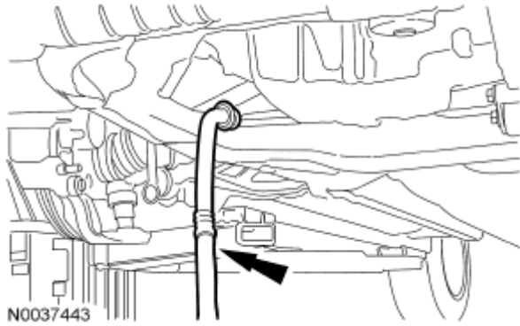
Fig. 632: Locating Power Steering Pressure (PSP) Tube Courtesy of FORD MOTOR CO.
