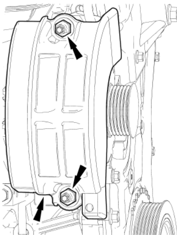
Fig. 553: Locating Generator Splash Shield And Nuts Courtesy of FORD MOTOR CO.
