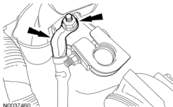
Fig. 220: Locating Battery Cable And Nut Courtesy of FORD MOTOR CO.
