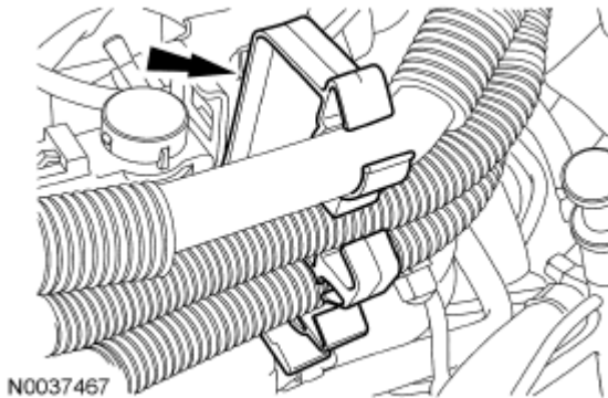
Fig. 227: Locating Retaining Clip Courtesy of FORD MOTOR CO.
