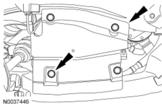
Fig. 687: Locating Splash Shield Pin-Type Retainers Courtesy of FORD MOTOR CO.
