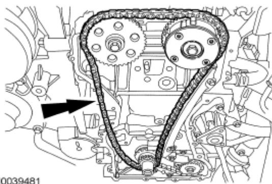
Fig. 81: Locating Timing Chain Courtesy of FORD MOTOR CO.
