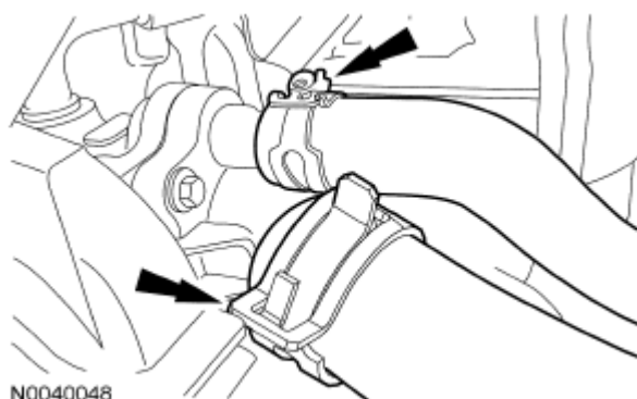
Fig. 332: Locating Lower Radiator And Heater Hoses From Thermostat Housing Courtesy of FORD MOTOR CO.
