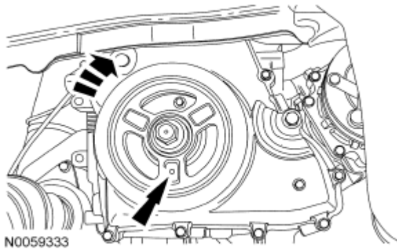
Fig. 93: Identifying Crankshaft Pulley Bolt Turning Crankshaft Clockwise Courtesy of FORD MOTOR CO.
