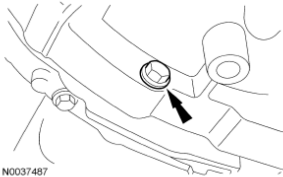
Fig. 309: Locating Bellhousing-To-Oil Pan Bolt Courtesy of FORD MOTOR CO.
