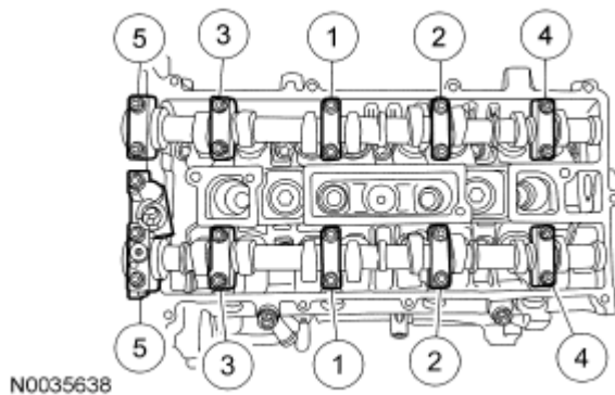
Fig. 470: Identifying Tightening Sequence Of Camshaft Bearing Cap Bolts Courtesy of FORD MOTOR CO.
