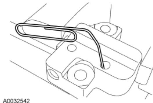
Fig. 484: Identifying Paper Clip Into Hole In Tensioner Housing Courtesy of FORD MOTOR CO.
