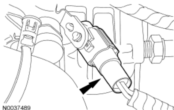
Fig. 245: Locating AIR Pump Electrical Connector Courtesy of FORD MOTOR CO.
