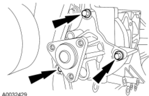
Fig. 338: Locating Coolant Pump Bolts Courtesy of FORD MOTOR CO.
