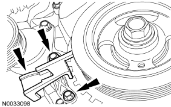
Fig. 503: Locating CKP Sensor Bolts And Alignment Tool Courtesy of FORD MOTOR CO.
