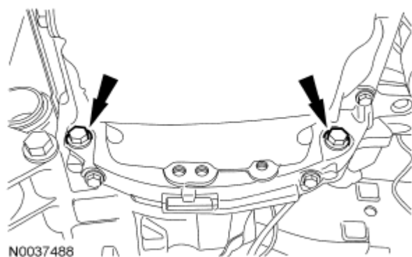
Fig. 244: Locating Oil Pan-To-Bellhousing Bolts Courtesy of FORD MOTOR CO.
