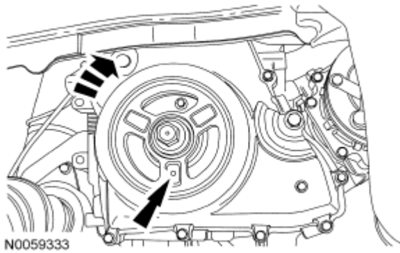
Fig. 387: Using Crankshaft Pulley Bolt To Turn Crankshaft Clockwise Courtesy of FORD MOTOR CO.
