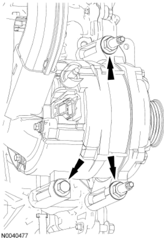
Fig. 551: Locating Generator Bolt And Stud Bolts Courtesy of FORD MOTOR CO.
