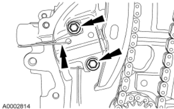
Fig. 485: Locating Timing Chain Tensioner Bolts And Paper Clip Courtesy of FORD MOTOR CO.
