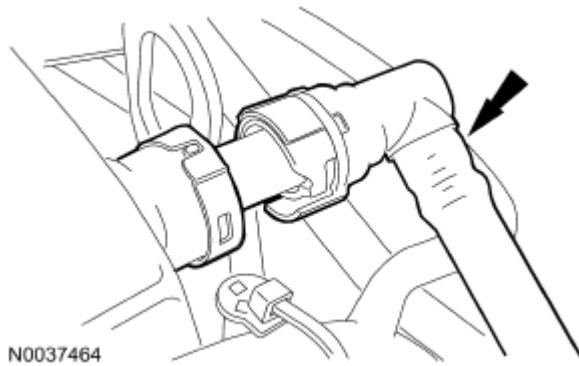
Fig. 611: Locating Crankcase Vent Tube Courtesy of FORD MOTOR CO.
