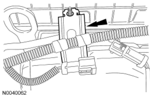
Fig. 544: Locating Wiring Harness Bracket Courtesy of FORD MOTOR CO.
