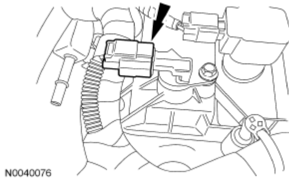
Fig. 376: Locating Camshaft Position (CMP) Sensor Electrical Connector Courtesy of FORD MOTOR CO.
