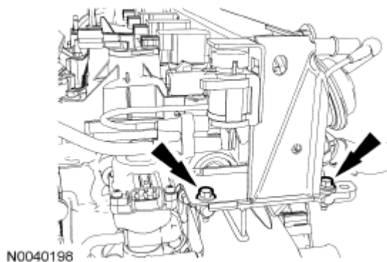
Fig. 547: Locating Pump Assembly Bolts Courtesy of FORD MOTOR CO.
