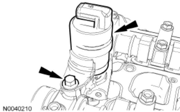
Fig. 404: Locating VCT Solenoid And Bolt Courtesy of FORD MOTOR CO.
