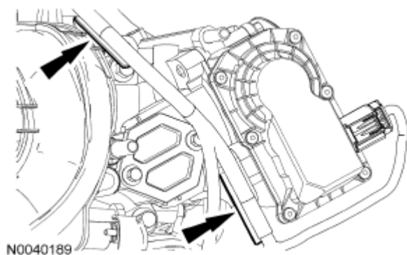
Fig. 365: Locating Wiring Harness Pin-Type Retainers From Intake Manifold Courtesy of FORD MOTOR CO.
