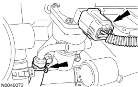
Fig. 360: Locating Exhaust Gas Recirculation (EGR) Coolant Hose And Electrical Connector Courtesy of FORD MOTOR CO.
