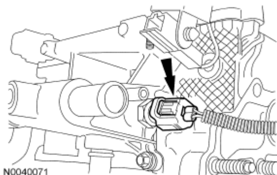
Fig. 536: Locating Coolant Temperature Sender Electrical Connector Courtesy of FORD MOTOR CO.
