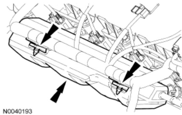
Fig. 515: Locating Pin-Type Harness Retainers And Fuel Supply Rail Insulator Courtesy of FORD MOTOR CO.
