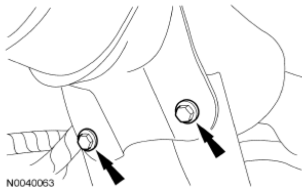
Fig. 354: Locating Catalytic Converter Bracket Bolts Courtesy of FORD MOTOR CO.
