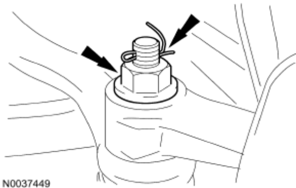
Fig. 207: Locating Tie-Rod Ends Cotter Pins And Nuts Courtesy of FORD MOTOR CO.
