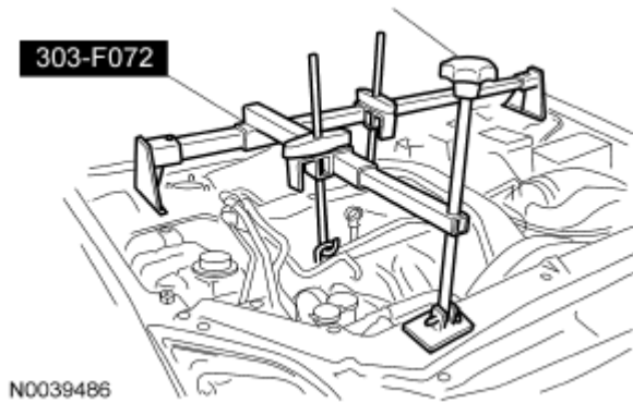
Fig. 195: Identifying Special Tool Courtesy of FORD MOTOR CO.
