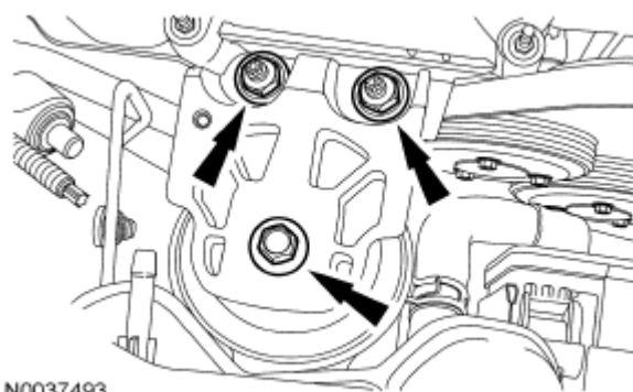
Fig. 313: Locating Motor Mount Bracket Bolt And Nuts Courtesy of FORD MOTOR CO.
