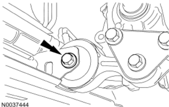
Fig. 631: Locating Engine Roll Restrictor Bolt Courtesy of FORD MOTOR CO.
