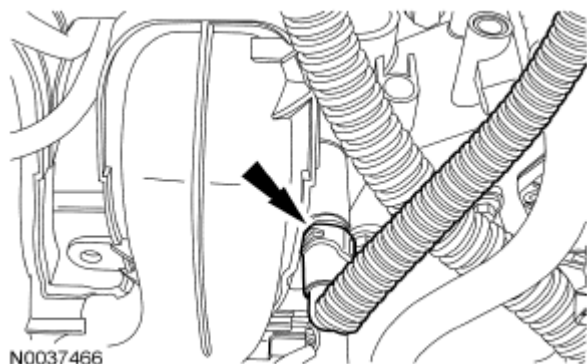
Fig. 290: Locating Evaporative Emissions (EVAP) Tube Courtesy of FORD MOTOR CO.
