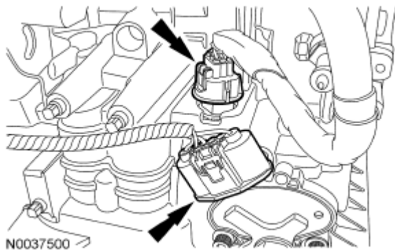
Fig. 255: Locating Transmission Range (TR) Sensor And Primary Control Solenoid Electrical Connectors
