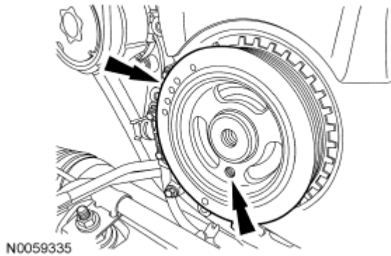
Fig. 490: Locating Hole In Pulley Courtesy of FORD MOTOR CO.
