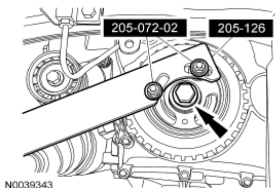
Fig. 392: Locating Crankshaft Pulley Bolt And Special Tools Courtesy of FORD MOTOR CO.
