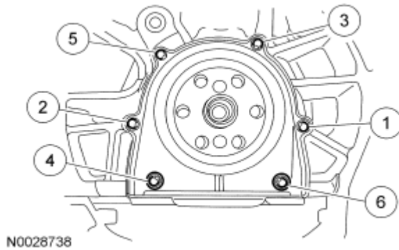
Fig. 62: Identifying Tightening Sequence Of Crankshaft Rear Oil Seal Retainer Plate Bolts Courtesy of FORD MOTOR CO.
