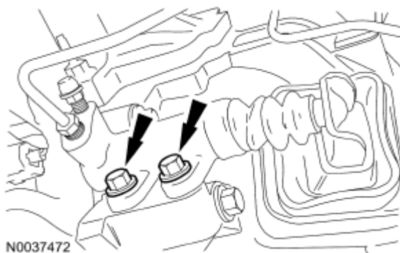
Fig. 661: Locating Clutch Slave Cylinder And Bolts Courtesy of FORD MOTOR CO.
