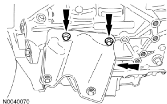
Fig. 358: Locating Catalytic Converter Bracket And Bolts Courtesy of FORD MOTOR CO.
