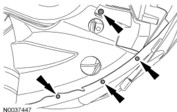
Fig. 628: Locating LH Fender Splash Shield Screws Courtesy of FORD MOTOR CO.
