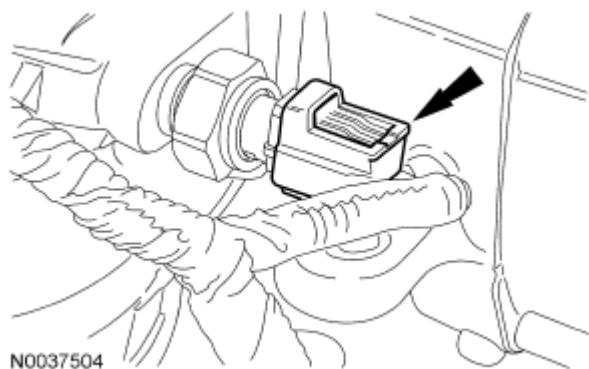
Fig. 576: Locating Transaxle Pressure Switch Electrical Connector Courtesy of FORD MOTOR CO.
