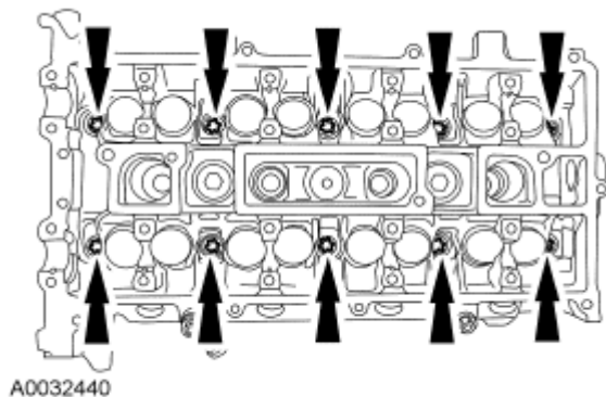
Fig. 406: Locating Cylinder Head Bolts Courtesy of FORD MOTOR CO.
