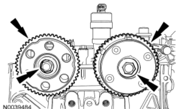
Fig. 477: Locating Camshaft Sprockets And Bolts Courtesy of FORD MOTOR CO.
