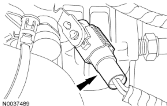
Fig. 589: Locating AIR Pump Electrical Connector
