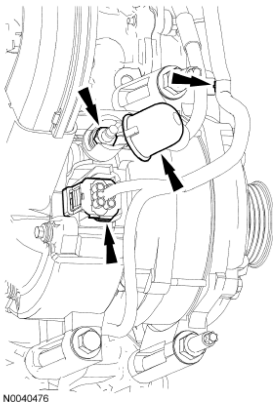
Fig. 552: Locating Pin-Type Retainer, Generator Electrical Connections And Install Nut Courtesy of FORD MOTOR CO.
