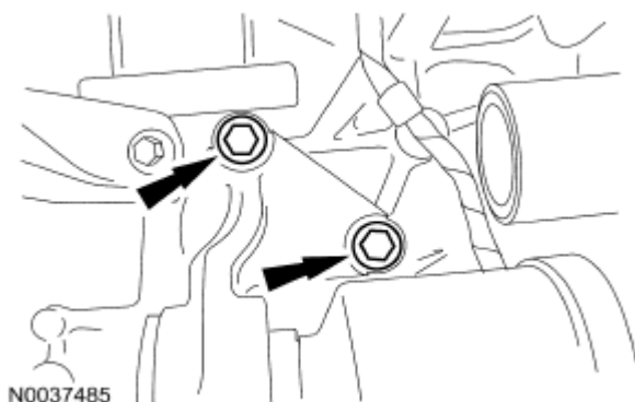
Fig. 593: Locating RH Halfshaft Carrier Bearing Bracket Bolts Courtesy of FORD MOTOR CO.
