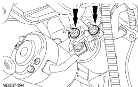
Fig. 644: Locating Starter Wire Nuts Courtesy of FORD MOTOR CO.
