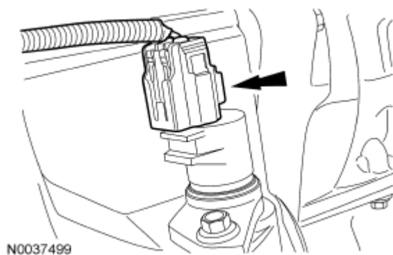
Fig. 639: Locating Vehicle Speed Sensor (VSS) Electrical Connector Courtesy of FORD MOTOR CO.
