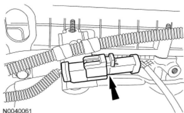
Fig. 545: Locating Heated Oxygen Sensor (HO2S) Electrical Connector Courtesy of FORD MOTOR CO.
