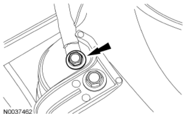
Fig. 286: Locating Bolt And Ground Wire Courtesy of FORD MOTOR CO.
