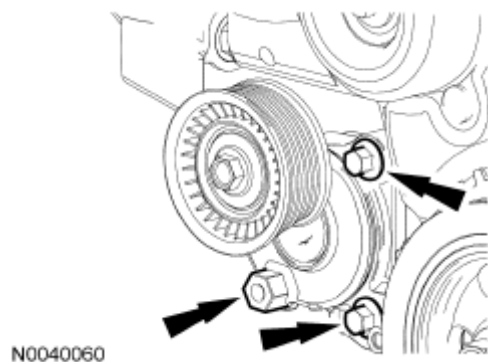
Fig. 327: Locating Tensioner And Bolts Courtesy of FORD MOTOR CO.
