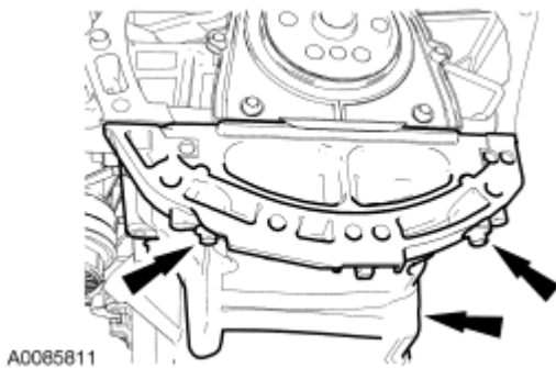
Fig. 191: Identifying Rear Oil Pan Bolts Courtesy of FORD MOTOR CO.
