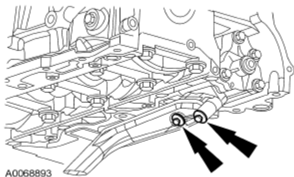
Fig. 410: Locating Oil Pump Pickup Tube Bolts Courtesy of FORD MOTOR CO.
