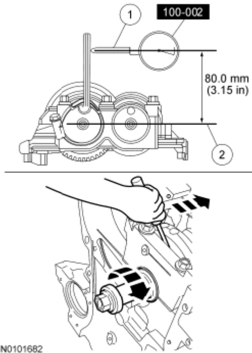
Fig. 456: Measuring Gear Backlash
