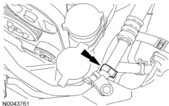
Fig. 300: Locating Coolant Vent Hose Retaining Clip Courtesy of FORD MOTOR CO.
