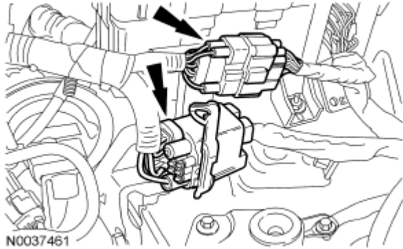
Fig. 614: Locating Engine Wiring Harness Electrical Connectors Courtesy of FORD MOTOR CO.
