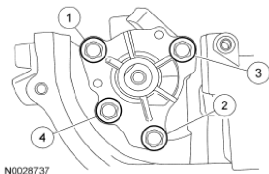
Fig. 188: Identifying Tightening Sequence Of Oil Pump Assembly Bolts Courtesy of FORD MOTOR CO.
