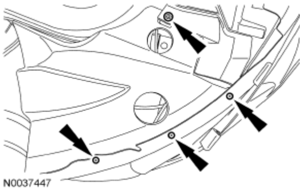
Fig. 269: Locating LH Fender Splash Shield And Screws Courtesy of FORD MOTOR CO.
