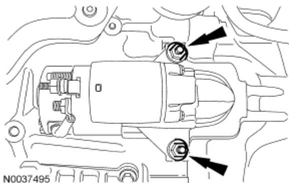
Fig. 643: Locating Starter Stud Bolts Courtesy of FORD MOTOR CO.
