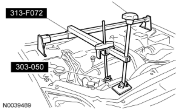
Fig. 174: Identifying Special Tool Courtesy of FORD MOTOR CO.
