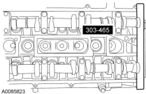
Fig. 388: Identifying Special Camshaft Tool (303-465) Courtesy of FORD MOTOR CO.
