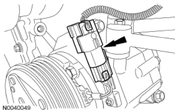
Fig. 334: Locating A/C Compressor Electrical Connector Courtesy of FORD MOTOR CO.
