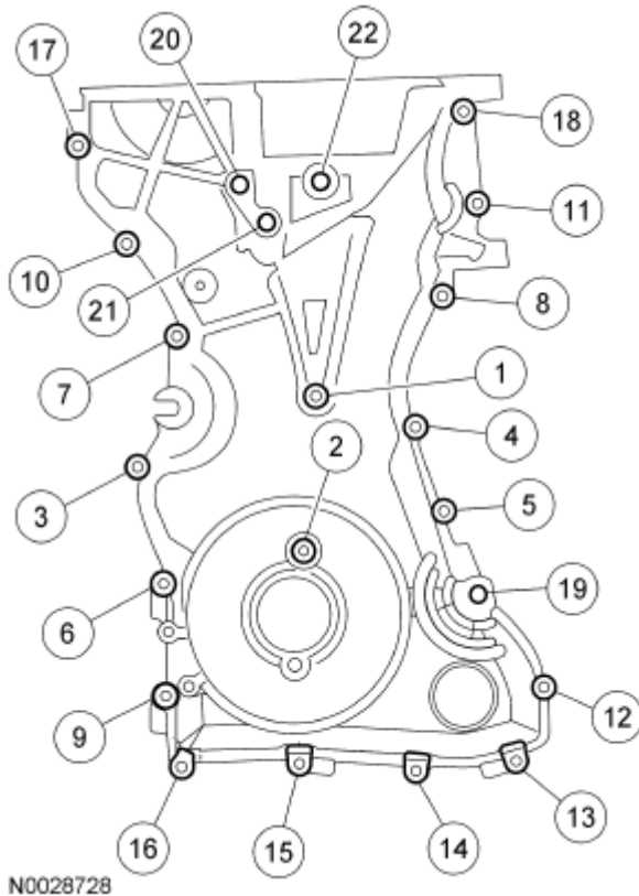
Fig. 488: Identifying Tightening Sequence Of Engine Front Cover Bolts Courtesy of FORD MOTOR CO.
