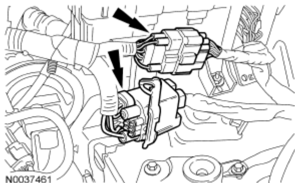
Fig. 221: Locating Electrical Connectors Courtesy of FORD MOTOR CO.
