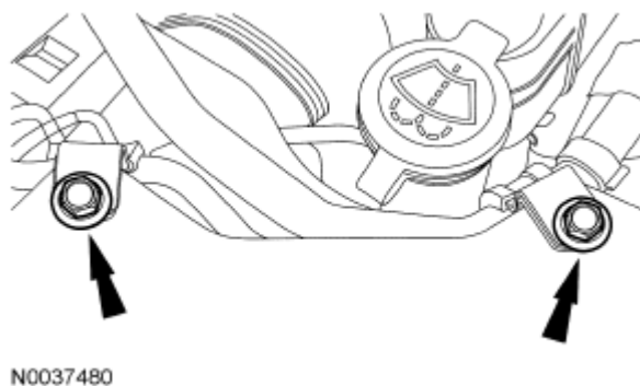
Fig. 599: Locating A/C Tube Bracket Bolts Courtesy of FORD MOTOR CO.
