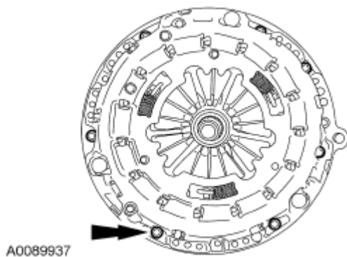
Fig. 321: Locating Clutch Pressure Plate Bolts Courtesy of FORD MOTOR CO.
