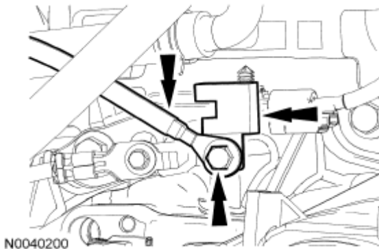
Fig. 233: Locating Bolt, Radio Frequency Interference Capacitor And Ground Wire Courtesy of FORD MOTOR CO.
