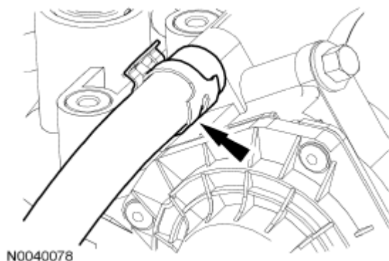
Fig. 333: Locating Coolant Hose Courtesy of FORD MOTOR CO.
