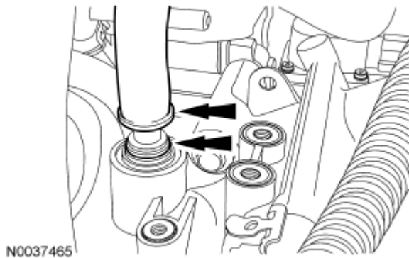
Fig. 668: Locating Brake Booster Vacuum Supply Tube Courtesy of FORD MOTOR CO.
