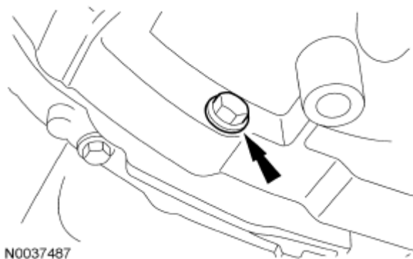
Fig. 591: Locating Bellhousing-To-Oil Pan Bolt Courtesy of FORD MOTOR CO.
