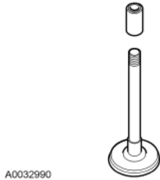
Fig. 157: Identifying Valve Stem Seal Installation Sleeve Courtesy of FORD MOTOR CO.
