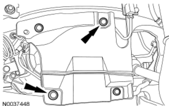
Fig. 685: Locating LH Splash Shield Pin-Type Retainers Courtesy of FORD MOTOR CO.
