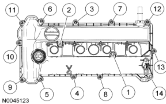
Fig. 508: Identifying Tightening Sequence Of Valve Cover Bolts Courtesy of FORD MOTOR CO.
