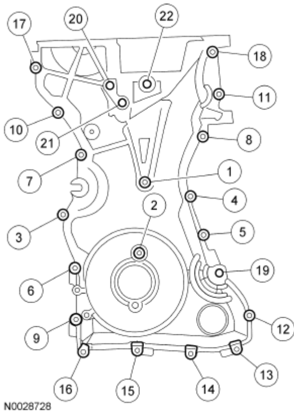
Fig. 72: Identifying Tightening Sequence Of Engine Front Cover Bolts Courtesy of FORD MOTOR CO.
