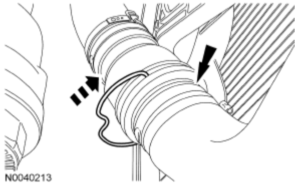
Fig. 595: Identifying Lower Radiator Hose And Installing Retaining Clip Courtesy of FORD MOTOR CO.
