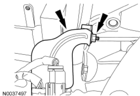
Fig. 254: Locating Engine Wiring Harness Bracket And Nut Courtesy of FORD MOTOR CO.
