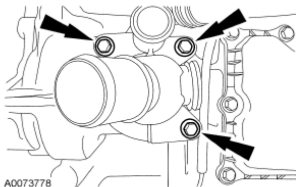
Fig. 370: Locating Thermostat Housing Bolts Courtesy of FORD MOTOR CO.
