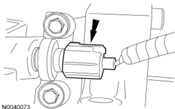
Fig. 534: Locating Oil Pressure Sender Electrical Connector Courtesy of FORD MOTOR CO.
