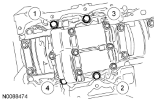
Fig. 453: Identifying Balancer Unit Bolts Tightening Sequence
