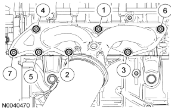
Fig. 540: Identifying Catalytic Converter Nuts Tightening Sequence Courtesy of FORD MOTOR CO.
