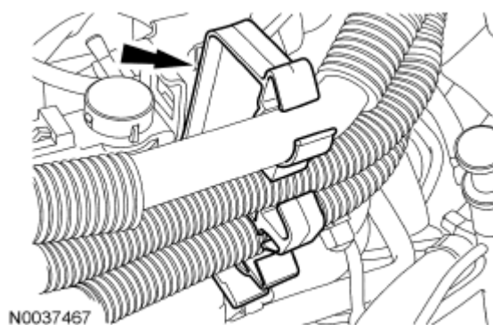
Fig. 608: Locating Evaporative Emissions (EVAP) Tube Bundle Retaining Clip Courtesy of FORD MOTOR CO.
