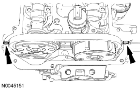
Fig. 507: Applying Silicone Gasket And Sealant Courtesy of FORD MOTOR CO.
