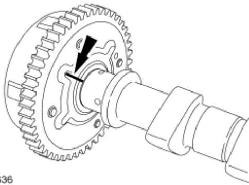
Fig. 139: Locating Marks On Camshaft Phaser Courtesy of FORD MOTOR CO.
