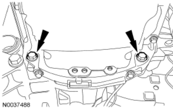
Fig. 310: Locating Oil Pan-To-Bellhousing Bolts Courtesy of FORD MOTOR CO.
