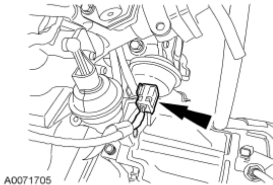
Fig. 363: Locating Intake Manifold Runner Control (IMRC) Actuator Electrical Connector Courtesy of FORD MOTOR CO.
