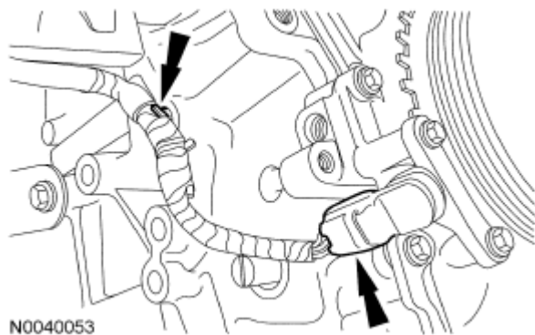
Fig. 554: Locating CKP Sensor Electrical Connector And Harness Pin-Type Retainer Courtesy of FORD MOTOR CO.
