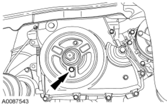
Fig. 44: Locating Bolt Courtesy of FORD MOTOR CO.
