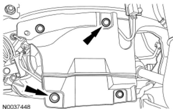
Fig. 627: Locating LH Splash Shield Pin-Type Retainers Courtesy of FORD MOTOR CO.
