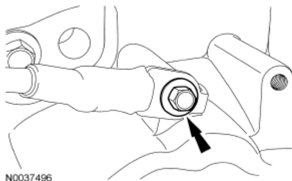
Fig. 316: Locating Ground Wire Bolt Courtesy of FORD MOTOR CO.
