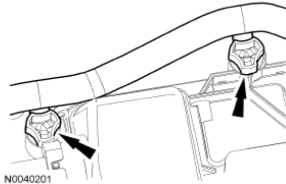
Fig. 513: Locating Wiring Harness Retainers Courtesy of FORD MOTOR CO.
