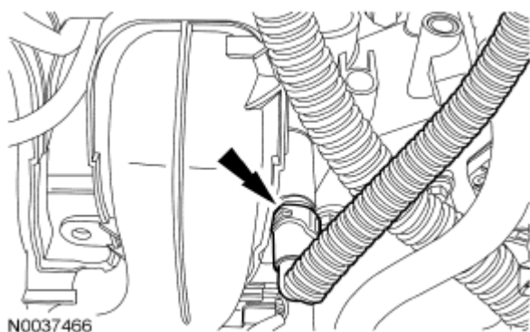
Fig. 667: Locating EVAP Tube Courtesy of FORD MOTOR CO.
