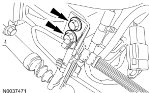
Fig. 295: Locating Clutch Tube Bracket Bolts Courtesy of FORD MOTOR CO.
