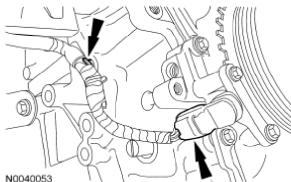
Fig. 340: Locating Crankshaft Position (CKP) Sensor Electrical Connector And Harness Pin-Type Retainer
