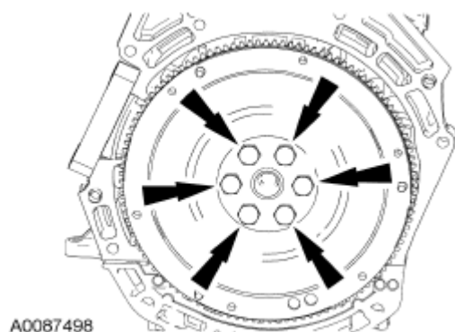
Fig. 323: Locating Flywheel Bolts Courtesy of FORD MOTOR CO.
