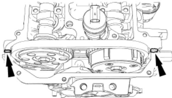
Fig. 28: Identifying Silicone Gasket Sealant Locations Courtesy of FORD MOTOR CO.
