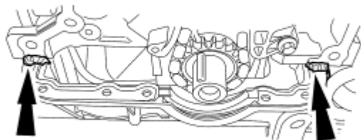
Fig. 69: Locating Engine Block Mating Surfaces Sealant Areas Courtesy of FORD MOTOR CO.
