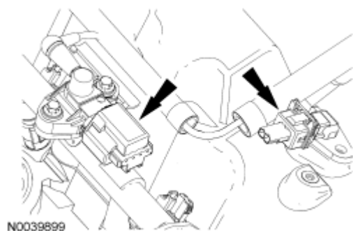
Fig. 192: Locating Fuel Rail Pressure & Temperature Sensor And Camshaft Position (CMP) Sensor Electrical Connector Courtesy of FORD MOTOR CO.
