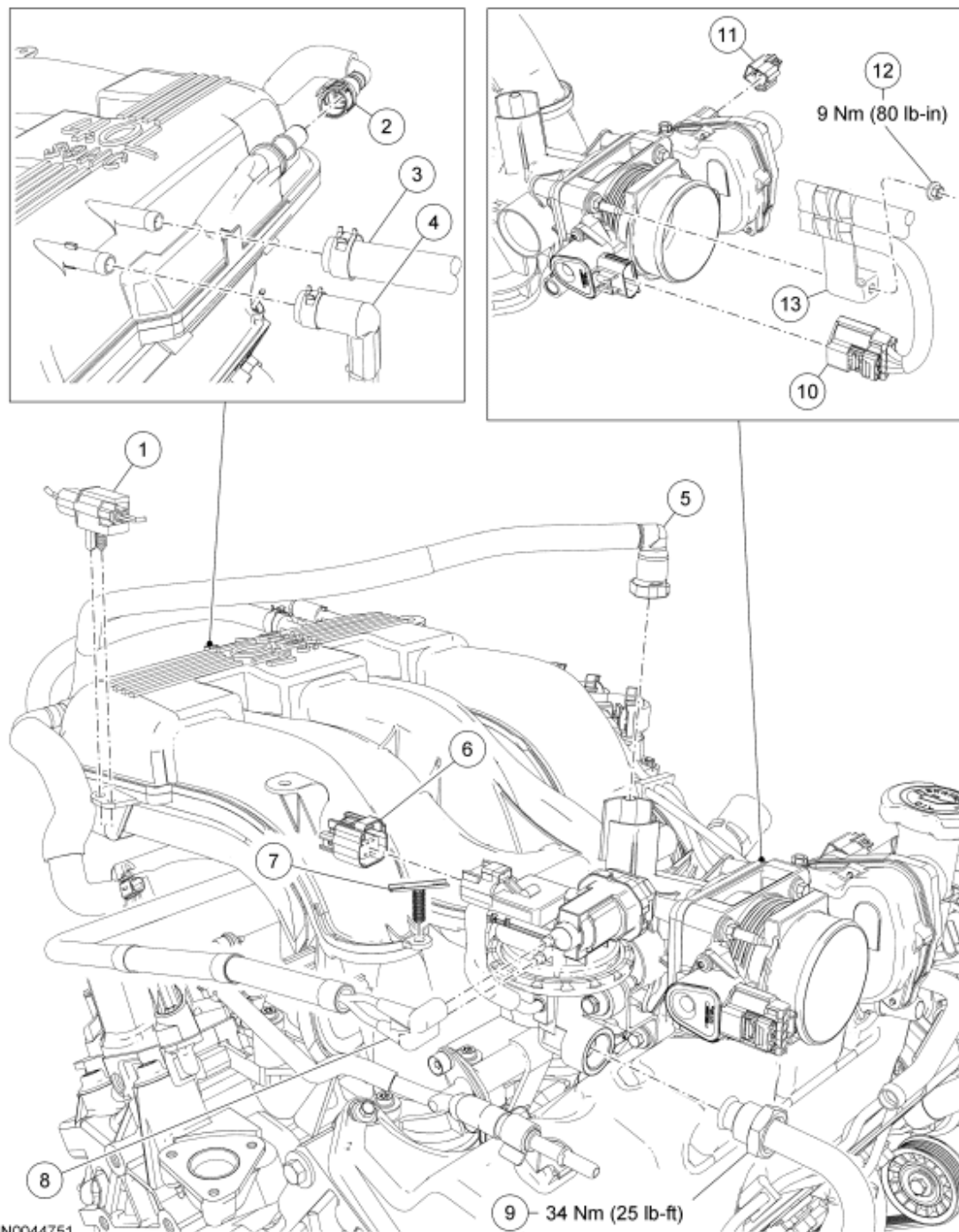
Fig. 30: Intake Manifold Connections With Torque Specifications
