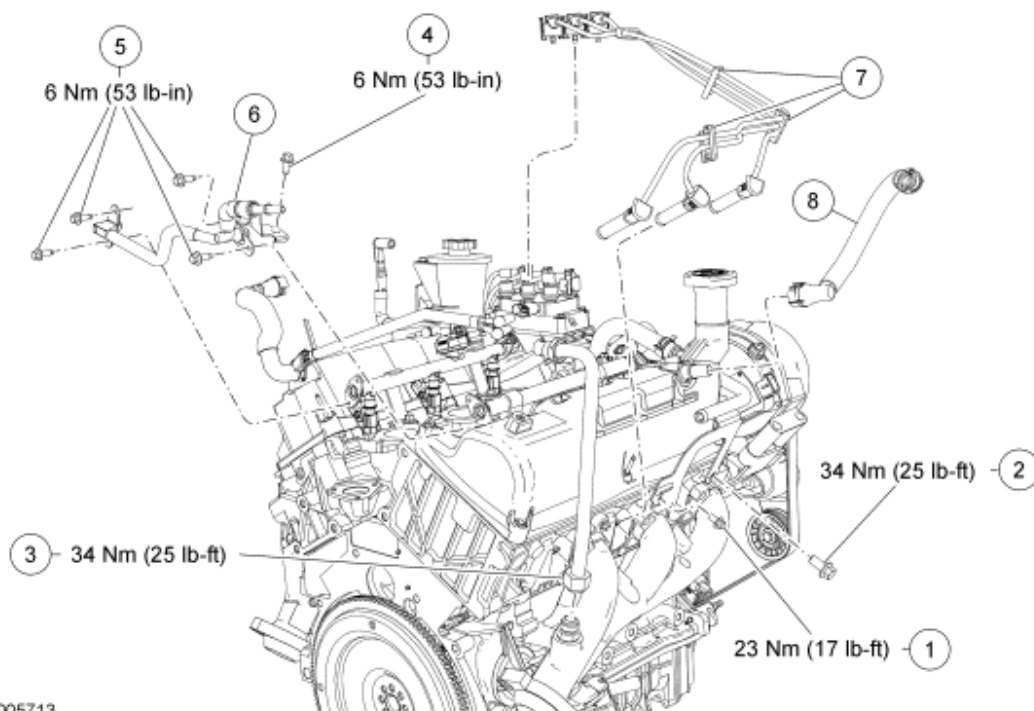
Fig. 32: Heater Hose Tube, Spark Plug Wires, Fuel Supply Tube and Crankcase Ventilation Tube With Torque Specifications Courtesy of FORD MOTOR CO.
