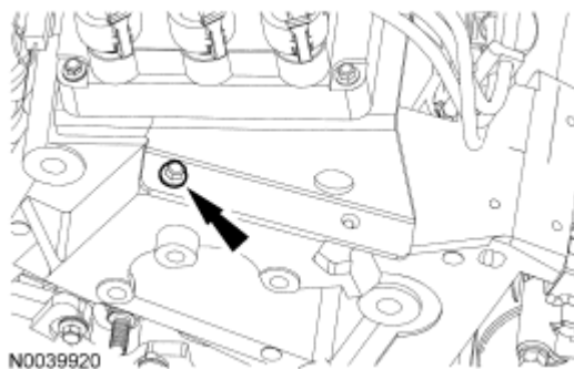
Fig. 169: Identifying Bolt
