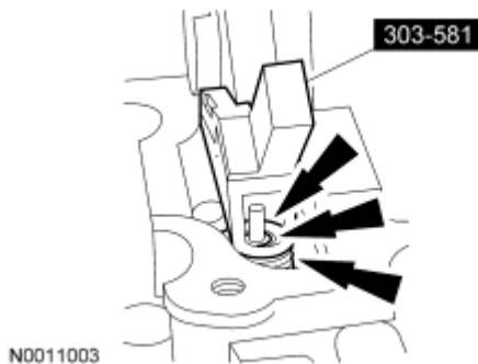
Fig. 264: Removing Valve Spring Retainer Keys, Valve Spring Retainers & Valve Springs Using Special Tool (303-581) Courtesy of FORD MOTOR CO.
