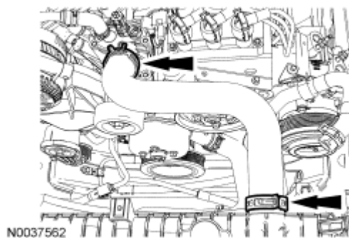
Fig. 426: Locating Upper Radiator Hose Clamps Courtesy of FORD MOTOR CO.
