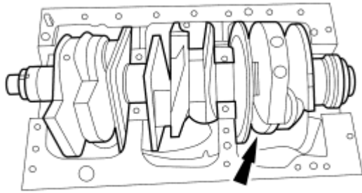
Fig. 277: Locating Crankshaft Main Bearings Courtesy of FORD MOTOR CO.
