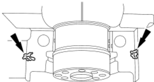
Fig. 278: Apply Silicone Gasket & Sealant To Rear Main Bearing Cap Courtesy of FORD MOTOR CO.
