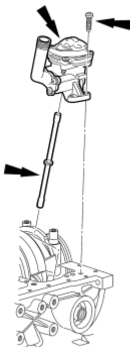
Fig. 293: Locating Oil Pump Intermediate Shaft, Oil Pump And Bolt Courtesy of FORD MOTOR CO.
