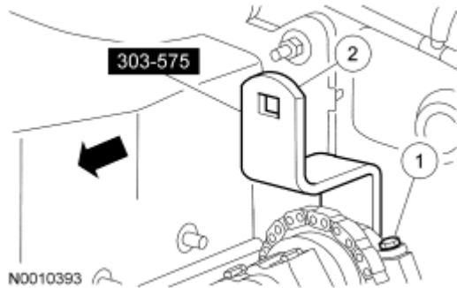
Fig. 13: Identifying Special Tool (303-575) & Clamp Bolt Courtesy of FORD MOTOR CO.
