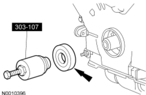
Fig. 37: Locating Special Tool And Crankshaft Front Oil Seal Courtesy of FORD MOTOR CO.
