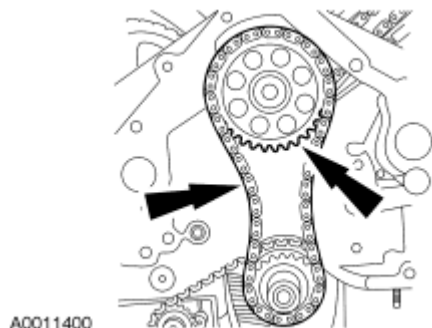
Fig. 76: Locating Jackshaft Chain And Sprockets Courtesy of FORD MOTOR CO.
