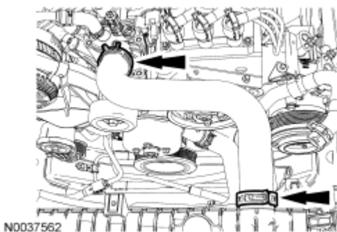
Fig. 144: Locating Upper Radiator Hose Clamps Courtesy of FORD MOTOR CO.
