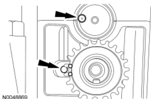
Fig. 290: Locating Timing Marks Courtesy of FORD MOTOR CO.
