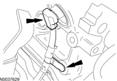
Fig. 162: Locating Block Heater Electrical Connector And Wiring Harness Retainer Courtesy of FORD MOTOR CO.
