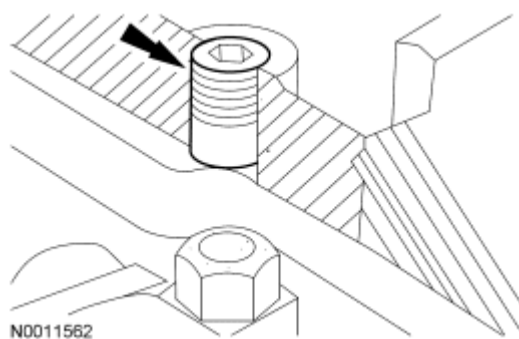
Fig. 311: Locating Cylinder Block Cradle Boss Screw Courtesy of FORD MOTOR CO.
