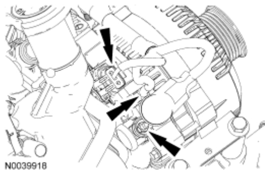
Fig. 172: Identifying Generator Electrical Connectors And Wire Harness Retainer Courtesy of FORD MOTOR CO.
