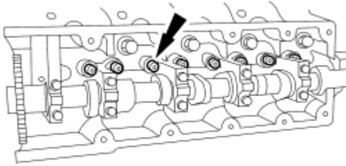
Fig. 263: Locating Hydraulic Lash Adjusters Courtesy of FORD MOTOR CO.
