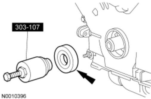
Fig. 226: Locating Special Tool And Crankshaft Front Oil Seal Courtesy of FORD MOTOR CO.
