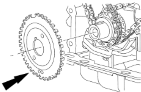
Fig. 511: View Of Crankshaft Sensor Ring At Crankshaft Courtesy of FORD MOTOR CO.
