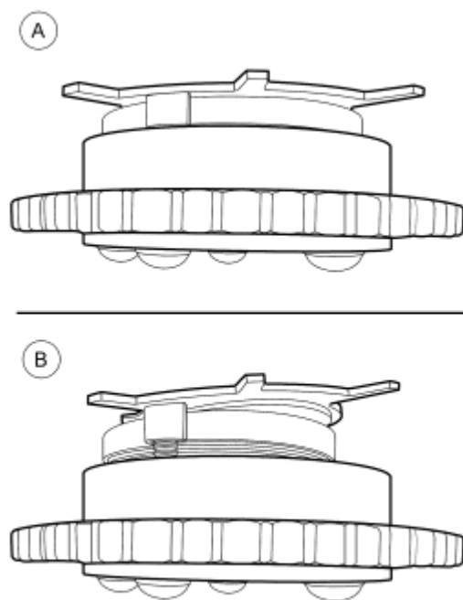
Fig. 133: Inspecting Camshaft Phaser And Sprocket For Squareness Courtesy of FORD MOTOR CO.
