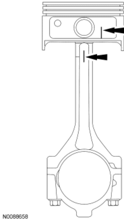
Fig. 344: Marking Piston & Connecting Rod On Same Side For Assembly Reference Courtesy of FORD MOTOR CO.
