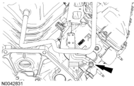
Fig. 490: Locating Heater Supply Tube Stud Bolt Courtesy of FORD MOTOR CO.
