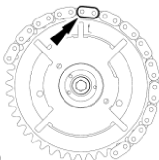
Fig. 379: Positioning LH Timing Chain On Camshaft Sprocket Courtesy of FORD MOTOR CO.
