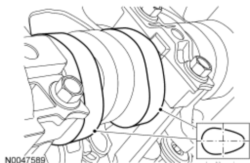
Fig. 103: Checking Position Of No. 5 Cylinder Intake And Exhaust Camshaft Lobes Courtesy of FORD MOTOR CO.
