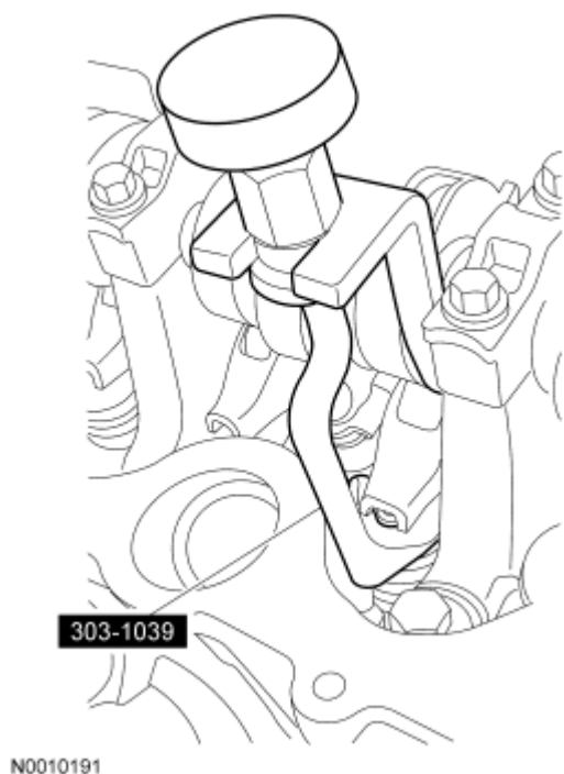
Fig. 104: Compressing Spring Using Special Tool Courtesy of FORD MOTOR CO.
