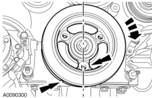
Fig. 114: Positioning Crankshaft Damper Spoke At 6 O'clock Position And Timing Mark Indentation At 7 O'clock Position
