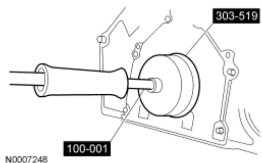
Fig. 21: Removing Crankshaft Rear Seal Courtesy of FORD MOTOR CO.
