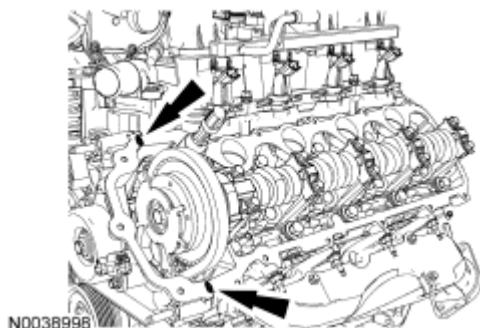
Fig. 524: Locating Silicone Gasket And Sealant Area Courtesy of FORD MOTOR CO.
