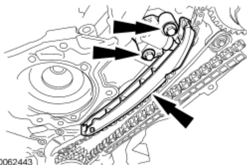
Fig. 380: Identifying LH Timing Chain Tensioner & Tensioner Arm Courtesy of FORD MOTOR CO.
