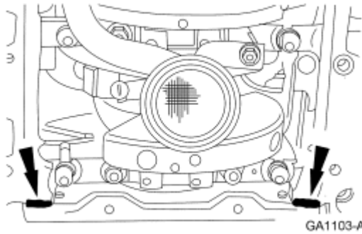
Fig. 448: Applying Silicone Gasket And Sealant Courtesy of FORD MOTOR CO.
