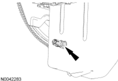
Fig. 209: Locating Oil Temperature Sensor Courtesy of FORD MOTOR CO.
