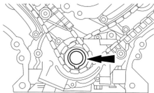
Fig. 327: Crankshaft Positioned With Keyway At 6 O'clock Position Courtesy of FORD MOTOR CO.
