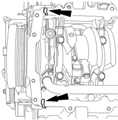
Fig. 161: Applying Silicone Gasket And Sealant At Engine Front Cover-To-Cylinder Block Sealing Surface Courtesy of FORD MOTOR CO.
