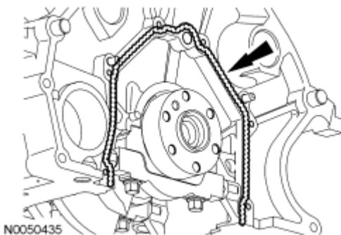
Fig. 25: Applying Bead Of Gasket Maker To Rear Crankshaft Seal Retainer Courtesy of FORD MOTOR CO.
