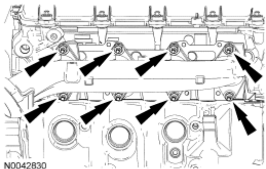
Fig. 305: Locating RH Exhaust Manifold Nuts Courtesy of FORD MOTOR CO.
