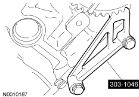
Fig. 62: Identifying Special Sprocket Phase Tool Courtesy of FORD MOTOR CO.
