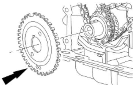
Fig. 78: View Of Crankshaft Sensor Ring At Crankshaft Courtesy of FORD MOTOR CO.
