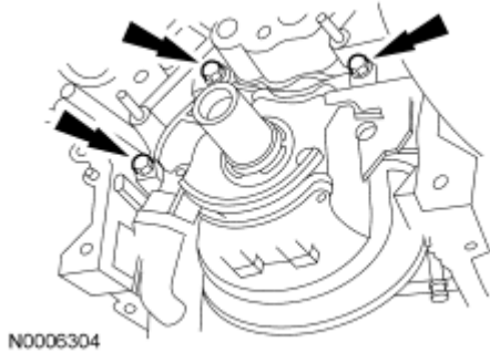
Fig. 172: Locating Oil Pump Bolts Courtesy of FORD MOTOR CO.
