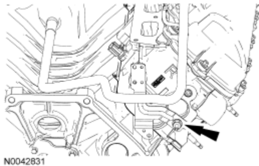
Fig. 427: Locating Heater Supply Tube Stud Bolt Courtesy of FORD MOTOR CO.
