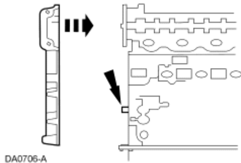
Fig. 399: Installing Engine Front Cover Gasket
