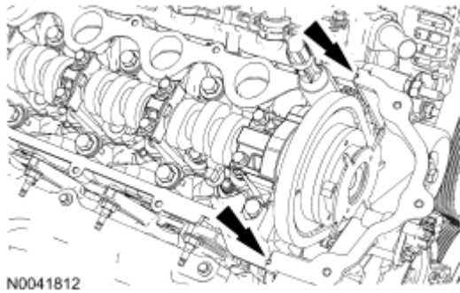
Fig. 532: Locating Silicone Gasket And Sealant Area Courtesy of FORD MOTOR CO.
