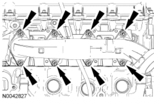
Fig. 264: Locating LH Exhaust Manifold Nuts Courtesy of FORD MOTOR CO.
