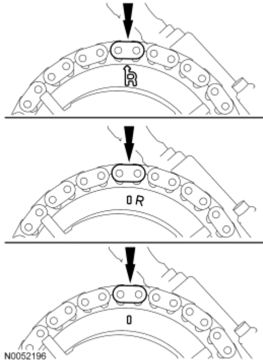
Fig. 517: Locating Camshaft Sprocket Timing Mark Aligned With Copper Chain Link Courtesy of FORD MOTOR CO.
