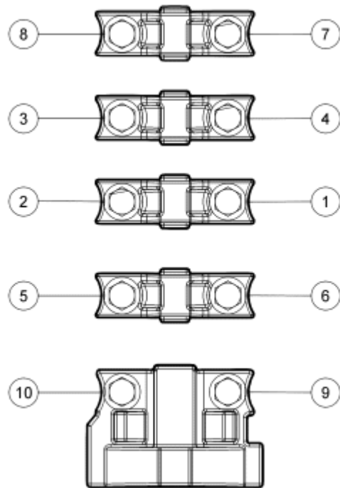
Fig. 60: Identifying Camshaft Bearing Cap Bolt Loosening/Tightening Sequence Courtesy of FORD MOTOR CO.
