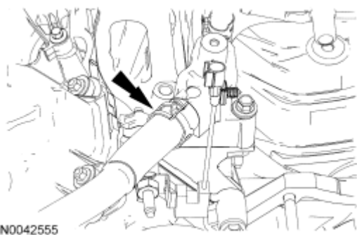
Fig. 192: Locating Heater Hose Clamp Courtesy of FORD MOTOR CO.
