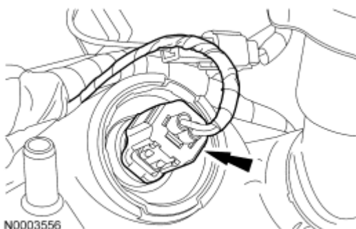
Fig. 551: Locating Camshaft Timing (VCT) Solenoid Electrical Connectors Courtesy of FORD MOTOR CO.
