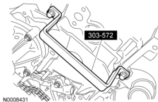
Fig. 374: Identifying Special Tool Onto Cylinder Head Courtesy of FORD MOTOR CO.
