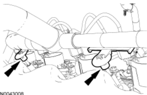
Fig. 290: Locating RH Valve Cover Studs Courtesy of FORD MOTOR CO.
