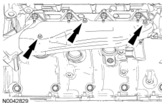
Fig. 304: Identifying RH Exhaust Manifold Heat Shield Bolts Courtesy of FORD MOTOR CO.
