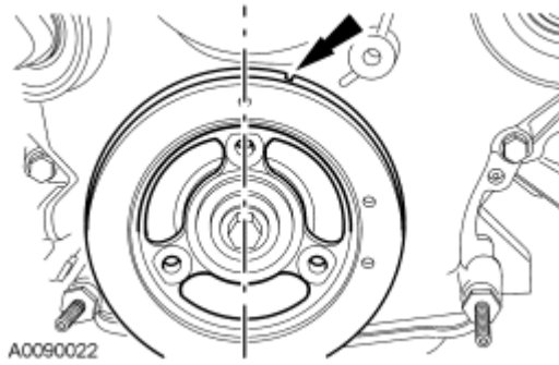
Fig. 103: Locating Crankshaft Damper Spoke Timing Mark Courtesy of FORD MOTOR CO.
