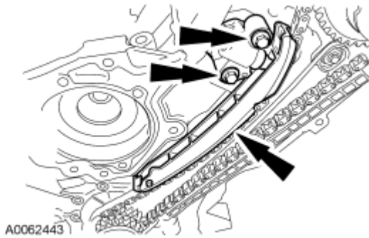
Fig. 252: Identifying LH Timing Chain Tensioner & Tensioner Arm Courtesy of FORD MOTOR CO.
