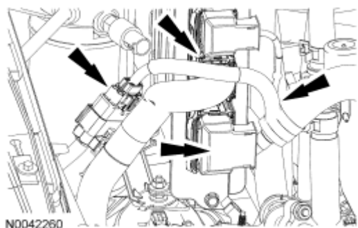
Fig. 197: Locating Wiring Harness Pin-Type Retainer, Powertrain Control Module (PCM) Electrical Connectors & In-Line Electrical Connector Courtesy of FORD MOTOR CO.
