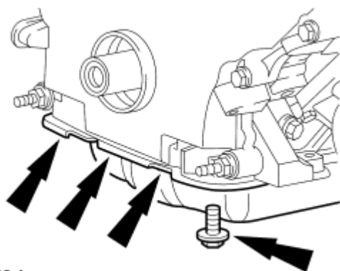
Fig. 241: Identifying Front Oil Pan Bolts Courtesy of FORD MOTOR CO.
