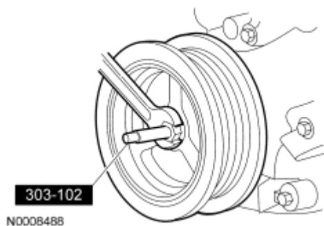
Fig. 530: Installing Crankshaft Pulley Using Special Tool Courtesy of FORD MOTOR CO.
