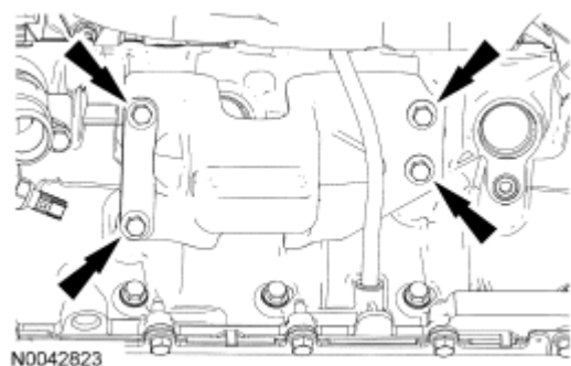
Fig. 298: Locating LH Engine Support Insulator Bracket Bolts Courtesy of FORD MOTOR CO.
