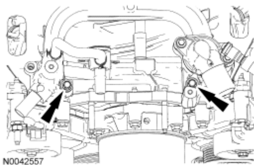
Fig. 194: Locating PCV Fitting Hose Assembly Bolts Courtesy of FORD MOTOR CO.
