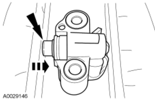
Fig. 508: Compressing Tensioner Plunger Courtesy of FORD MOTOR CO.
