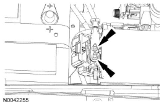
Fig. 185: Locating Wiring Harness Terminals Nuts Courtesy of FORD MOTOR CO.
