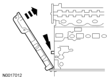
Fig. 524: Installing Engine Front Cover Gasket On Engine Front Cover Courtesy of FORD MOTOR CO.
