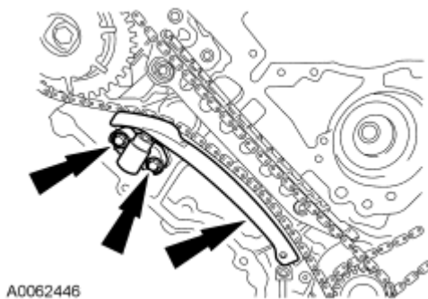
Fig. 253: Identifying RH Timing Chain Tensioner, Tensioner Arm And Bolts Courtesy of FORD MOTOR CO.
