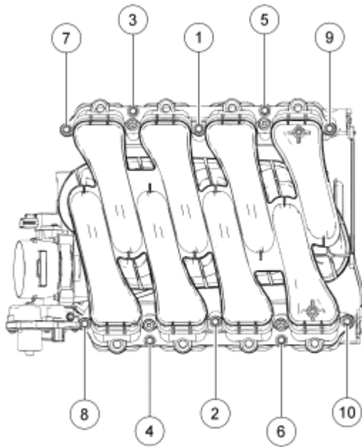
Fig. 2: Identifying Tightening Sequence Of Intake Manifold Bolts Courtesy of FORD MOTOR CO.
