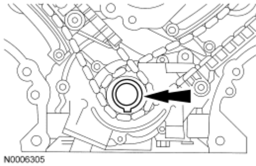
Fig. 251: Crankshaft Positioned With Keyway At 6 O'clock Position Courtesy of FORD MOTOR CO.
