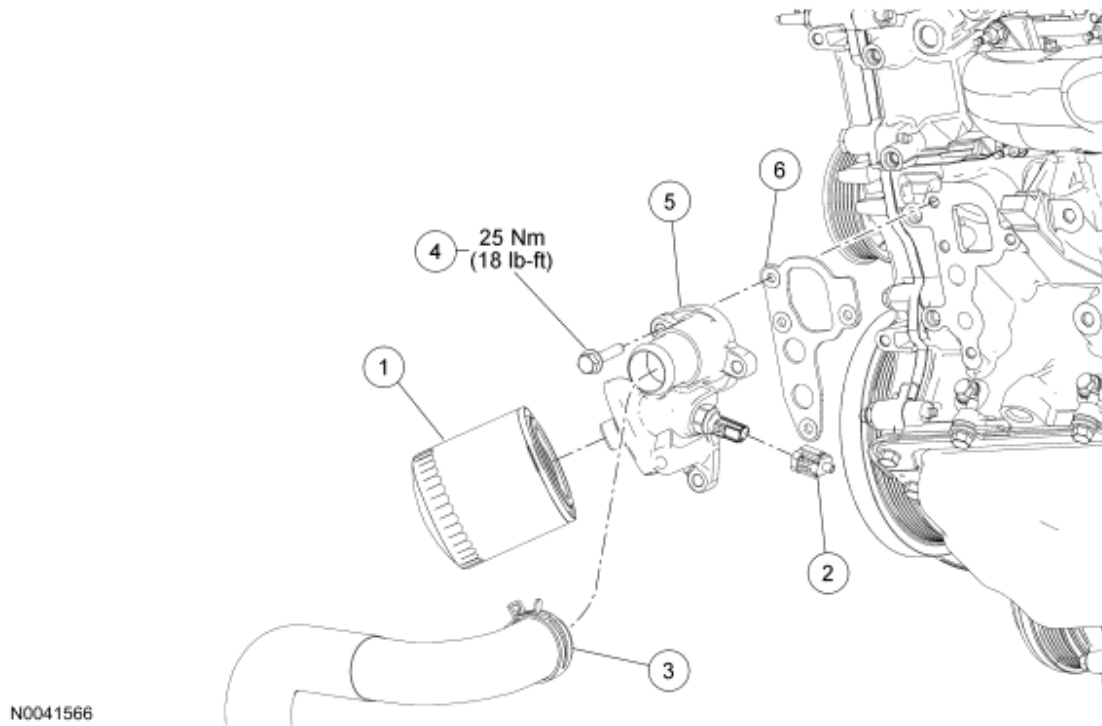
Fig. 174: Exploded View Of Oil Filter Adapter With Torque Specification Courtesy of FORD MOTOR CO.
