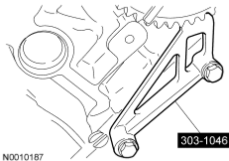
Fig. 379: Identifying Special Sprocket Phase Tool Courtesy of FORD MOTOR CO.
