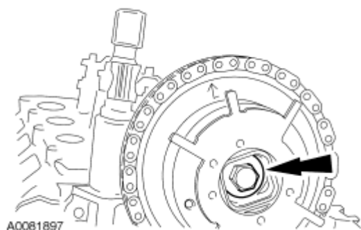
Fig. 378: Identifying Camshaft Phase And Sprocket Assembly Bolt Courtesy of FORD MOTOR CO.
