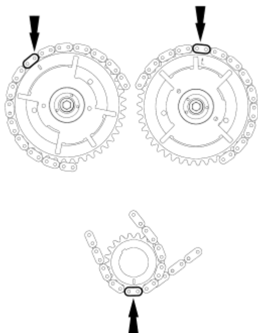
Fig. 520: Verifying Correct Alignment Of All Timing Marks Courtesy of FORD MOTOR CO.
