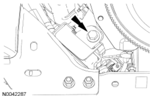
Fig. 457: Locating LH Engine Support Insulator Through-Bolt
