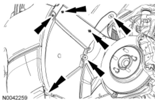
Fig. 200: Locating Inner Fender Splash Shield Pushpins And Screws Courtesy of FORD MOTOR CO.
