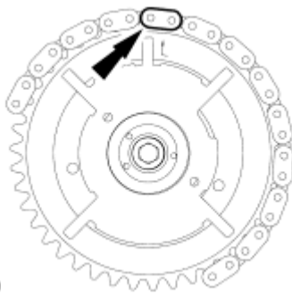
Fig. 388: Positioning LH Timing Chain On Camshaft Sprocket Courtesy of FORD MOTOR CO.
