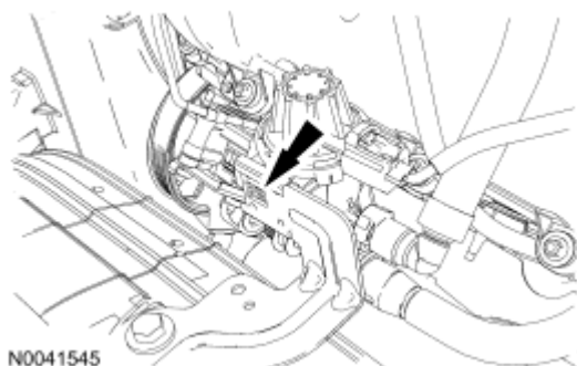
Fig. 149: Locating EVAP Canister Purge Valve To Bracket Courtesy of FORD MOTOR CO.
