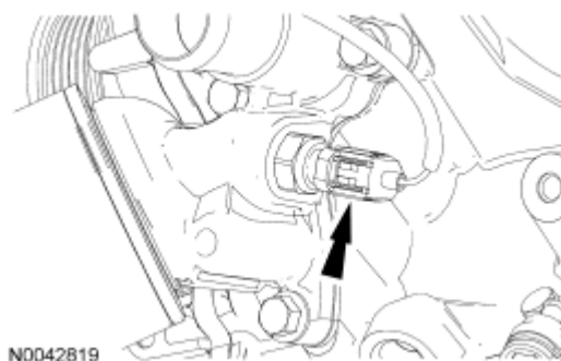
Fig. 548: Locating Oil Pressure Sensor Electrical Connector Courtesy of FORD MOTOR CO.
