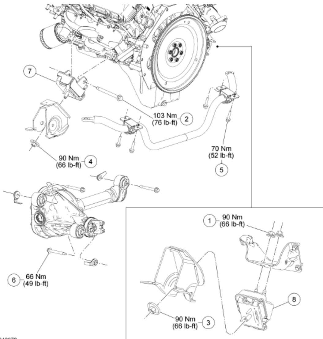
Fig. 176: Exploded View Of Engine Support Insulators With Torque Specifications Courtesy of FORD MOTOR CO.
