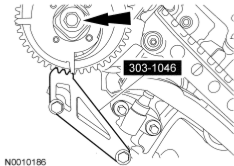
Fig. 332: Identifying VCT Phase Sprocket Bolt And Holder Tool Courtesy of FORD MOTOR CO.
