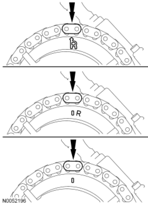
Fig. 392: Locating Camshaft Sprocket Timing Mark Aligned With Copper Chain Link
