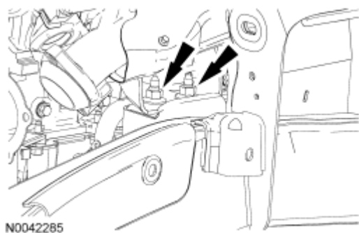
Fig. 459: Locating RH Engine Support Insulator Nuts Courtesy of FORD MOTOR CO.
