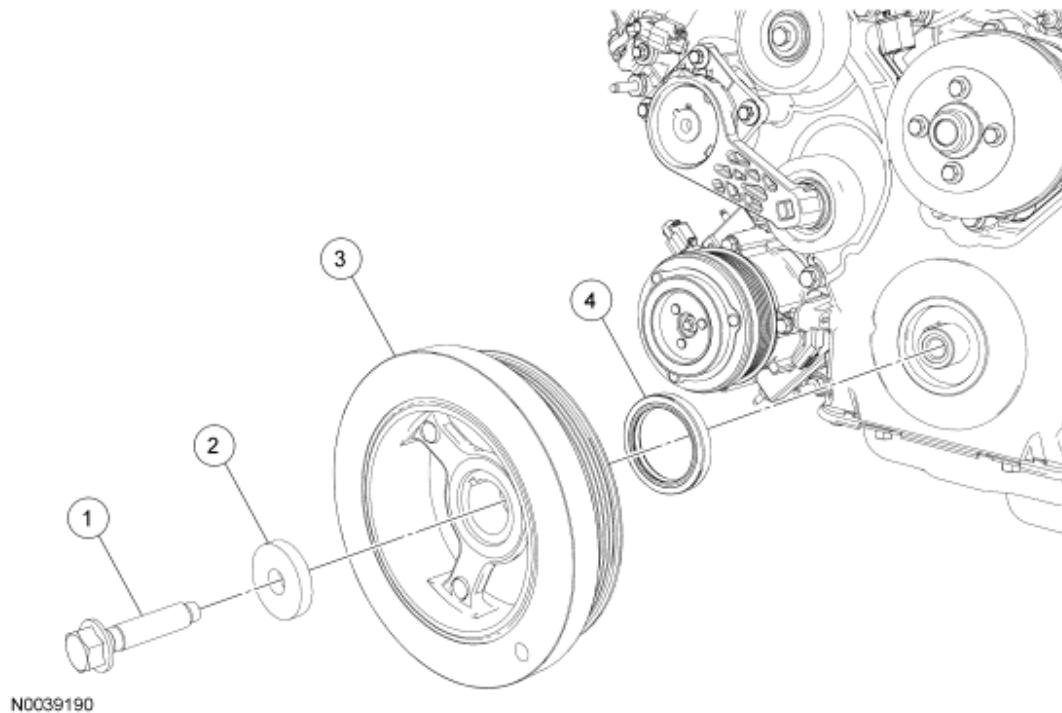
Fig. 10: Exploded View Of Crankshaft Pulley & Crankshaft Front Seal - Lower End Components Courtesy of FORD MOTOR CO.
