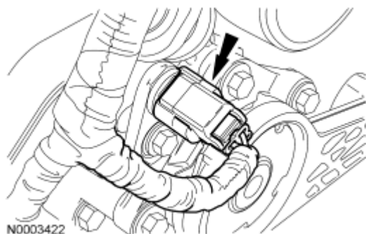
Fig. 552: Identifying RH CMP Sensor Electrical Connector Courtesy of FORD MOTOR CO.
