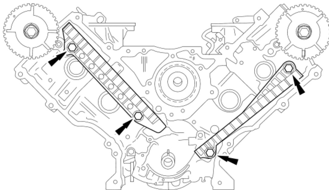
Fig. 386: Identifying Timing Chain Guides Courtesy of FORD MOTOR CO.
