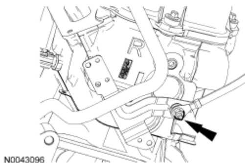
Fig. 501: Locating Ground Strap Nut Courtesy of FORD MOTOR CO.
