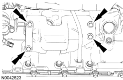
Fig. 423: Locating LH Engine Support Insulator Bracket Bolts Courtesy of FORD MOTOR CO.
