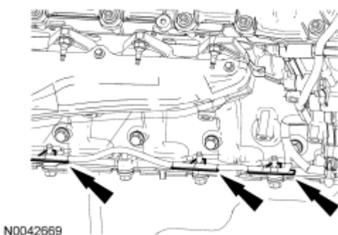
Fig. 157: Locating Oil Pan Wiring Harness Retainers Courtesy of FORD MOTOR CO.
