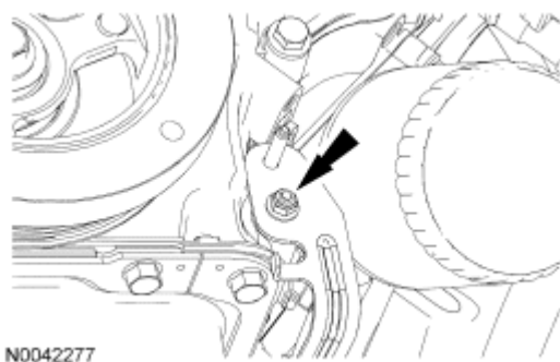
Fig. 202: Locating Battery Cable Bracket Nut Courtesy of FORD MOTOR CO.
