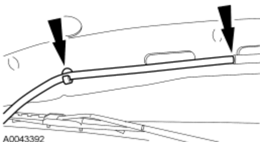
Fig. 488: Locating Windshield Washer Hose And Retainer Courtesy of FORD MOTOR CO.
