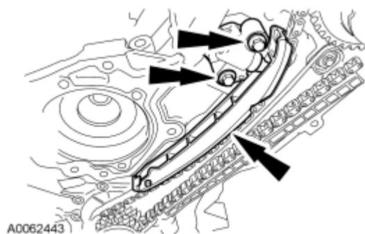
Fig. 328: Identifying LH Timing Chain Tensioner & Tensioner Arm Courtesy of FORD MOTOR CO.
