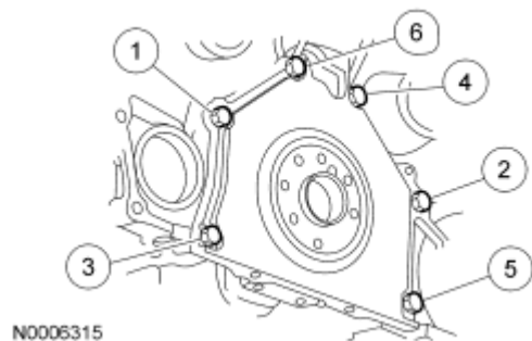
Fig. 447: Identifying Crankshaft Rear Seal Retainer Plate Bolts Tightening Sequence Courtesy of FORD MOTOR CO.
