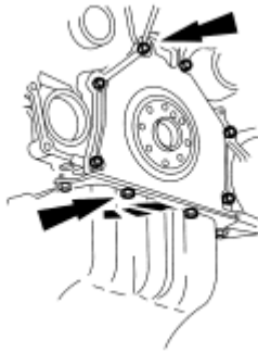
Fig. 276: Identifying Crankshaft Rear Seal Retainer Plate Bolts Courtesy of FORD MOTOR CO.
