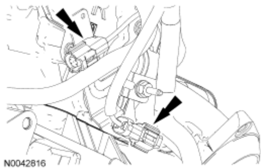
Fig. 428: Locating Electrical Connector Retainers And Engine Wiring Harness Courtesy of FORD MOTOR CO.
