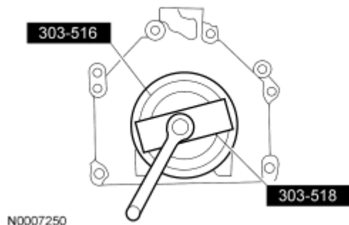
Fig. 21: Using Special Tools To Install New Crankshaft Rear Seal Courtesy of FORD MOTOR CO.
