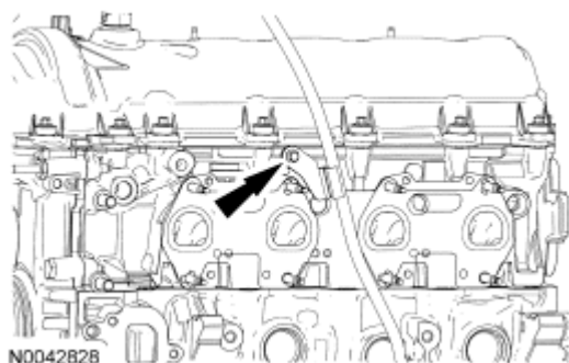
Fig. 302: Locating Oil Level Indicator Tube Bolt Courtesy of FORD MOTOR CO.
