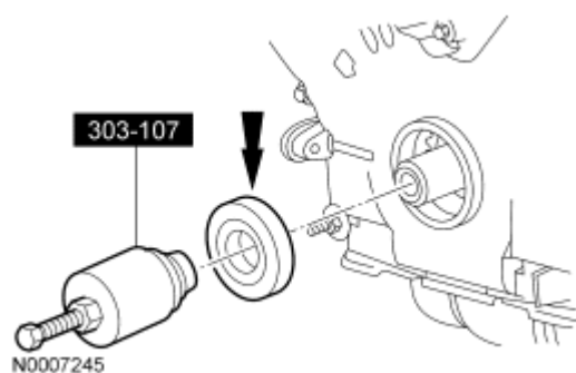
Fig. 240: Removing Crankshaft Front Seal Using Special Tool Courtesy of FORD MOTOR CO.
