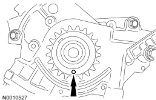
Fig. 381: Locating Crankshaft Sprocket Timing Mark Courtesy of FORD MOTOR CO.
