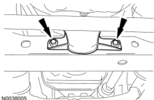
Fig. 158: Locating Oil Drain Splash Shield Bolts Courtesy of FORD MOTOR CO.
