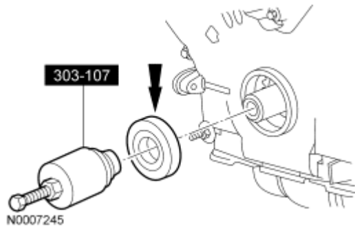
Fig. 14: Removing Crankshaft Front Seal Using Special Tool (303-107) Courtesy of FORD MOTOR CO.
