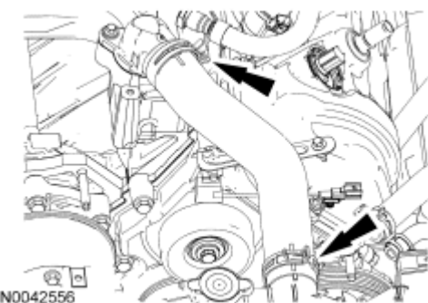
Fig. 193: Locating Upper Radiator Hose Clamps Courtesy of FORD MOTOR CO.
