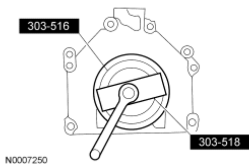
Fig. 452: Using Special Tools To Install New Crankshaft Rear Seal Courtesy of FORD MOTOR CO.
