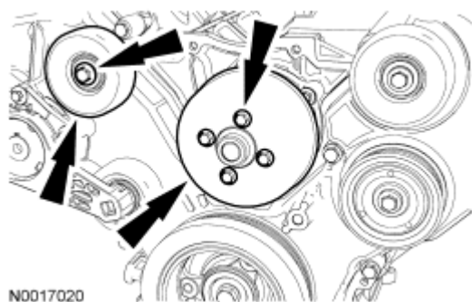
Fig. 238: Locating Accessory Drive Belt Idler Pulley And Bolts Courtesy of FORD MOTOR CO.
