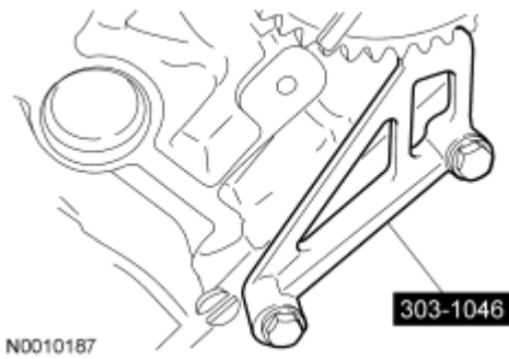
Fig. 257: Identifying Special Sprocket Phase Tool Courtesy of FORD MOTOR CO.
