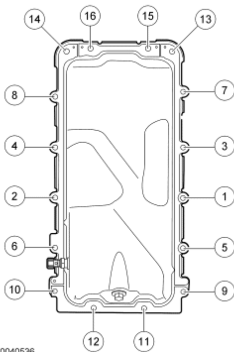
Fig. 451: Identifying Tightening Sequence Of Bolts Courtesy of FORD MOTOR CO.
