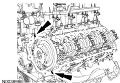
Fig. 5: Locating Silicone Gasket And Sealant Area Courtesy of FORD MOTOR CO.
