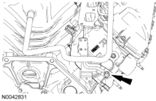
Fig. 269: Locating Heater Supply Tube Stud Bolt Courtesy of FORD MOTOR CO.
