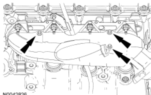
Fig. 421: Locating LH Exhaust Manifold Heat Shield Bolts Courtesy of FORD MOTOR CO.
