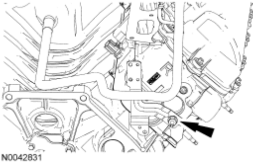
Fig. 294: Locating Heater Supply Tube Stud Bolt Courtesy of FORD MOTOR CO.
