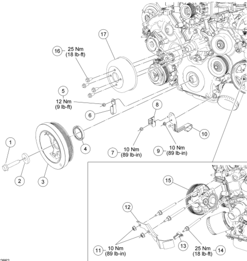
Fig. 29: Exploded View Of Engine Front Cover With Torque Specifications (1 Of 2) Courtesy of FORD MOTOR CO.
