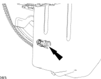
Fig. 462: Locating Oil Temperature Sensor Courtesy of FORD MOTOR CO.
