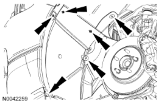
Fig. 471: Locating Inner Fender Splash Shield Pushpins And Screws Courtesy of FORD MOTOR CO.
