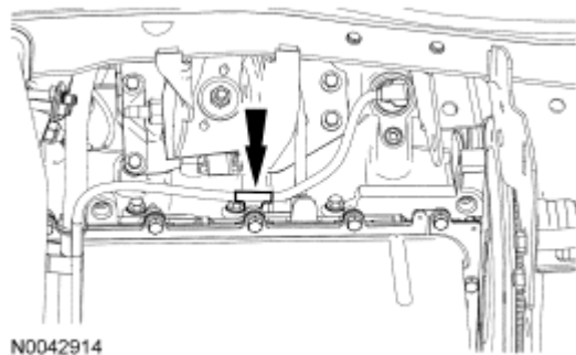
Fig. 163: Locating Block Heater Wiring Harness Retainer Courtesy of FORD MOTOR CO.
