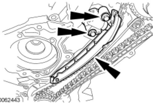
Fig. 389: Identifying LH Timing Chain Tensioner & Tensioner Arm Courtesy of FORD MOTOR CO.
