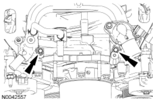
Fig. 477: Locating PCV Fitting Hose Assembly Bolts Courtesy of FORD MOTOR CO.
