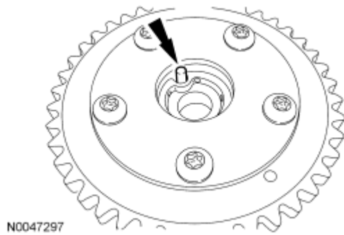
Fig. 126: Inspecting Rear Of Camshaft Phase And Sprocket Courtesy of FORD MOTOR CO.
