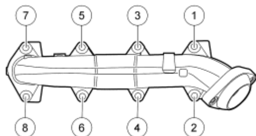
Fig. 420: Identifying Tightening Sequence Of Exhaust Manifold Nuts Courtesy of FORD MOTOR CO.
