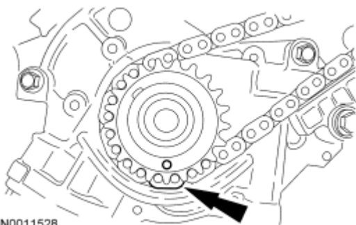
Fig. 387: Aligning Crankshaft Sprocket Timing Mark And LH Timing Chain Link Courtesy of FORD MOTOR CO.
