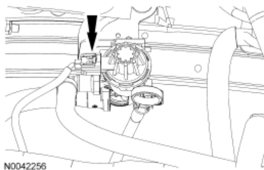
Fig. 195: Locating Evaporative Emission (EVAP) Canister Purge Valve Electrical Connector Courtesy of FORD MOTOR CO.
