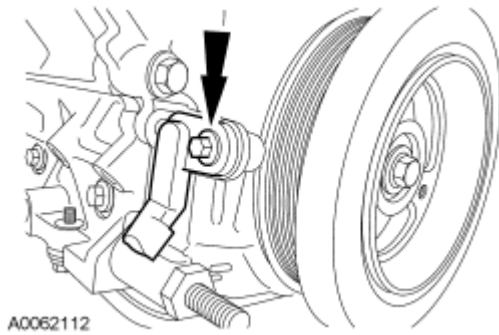
Fig. 409: Locating Crankshaft Position (CKP) Sensor Bolt Courtesy of FORD MOTOR CO.
