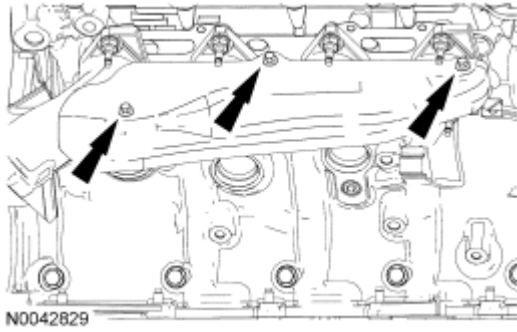
Fig. 417: Identifying RH Exhaust Manifold Heat Shield Bolts Courtesy of FORD MOTOR CO.
