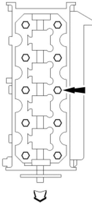
Fig. 340: Identifying Cylinder Head Gasket And Bolts Courtesy of FORD MOTOR CO.
