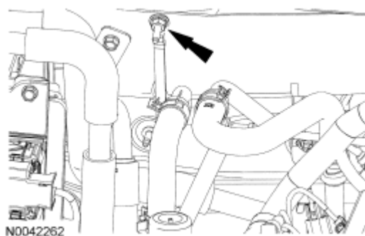
Fig. 199: Locating Ground Wire And Nut Courtesy of FORD MOTOR CO.
