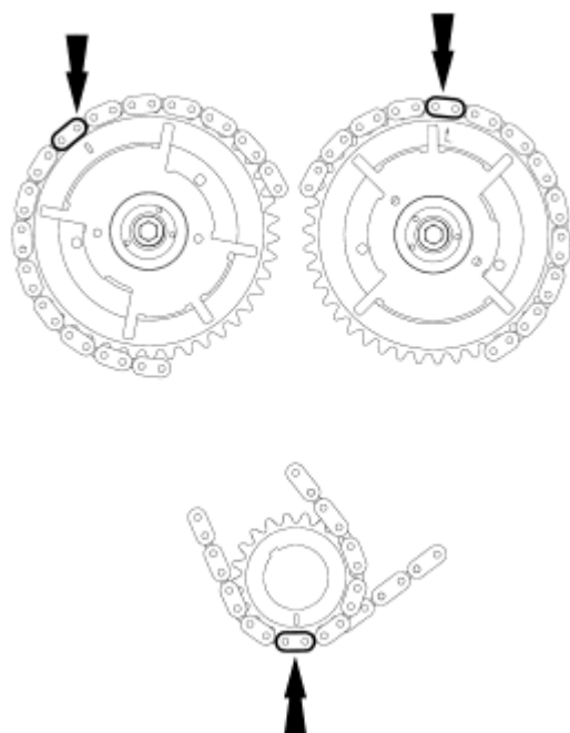
Fig. 395: Verifying Correct Alignment Of All Timing Marks Courtesy of FORD MOTOR CO.
