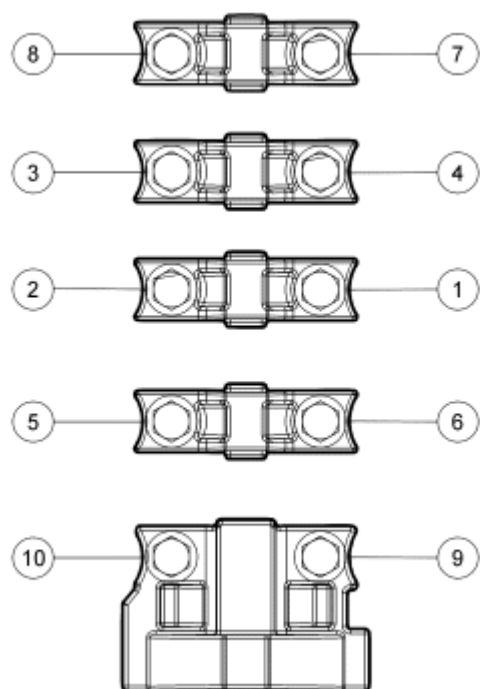
Fig. 377: Identifying Camshaft Bearing Cap Bolt Loosening/Tightening Sequence Courtesy of FORD MOTOR CO.
