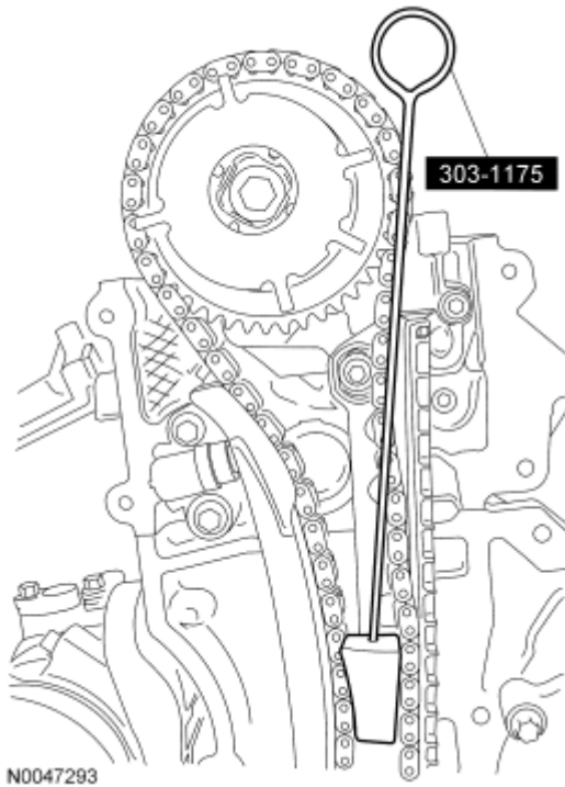
Fig. 110: Installing Special Tool (303-1175) In RH Timing Chain Courtesy of FORD MOTOR CO.
