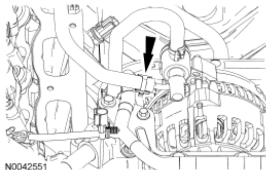
Fig. 188: Locating Heated PCV Fitting Coolant Hose Courtesy of FORD MOTOR CO.
