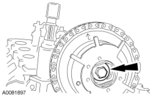
Fig. 92: Identifying Camshaft Phase And Sprocket Assembly Bolt Courtesy of FORD MOTOR CO.
