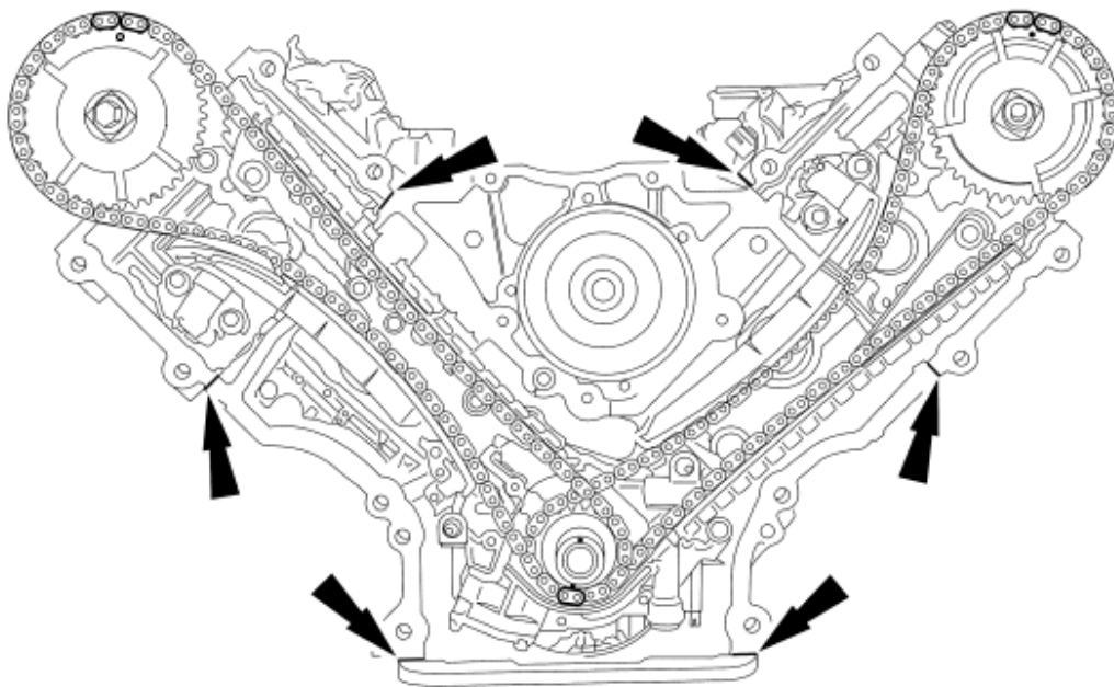
Fig. 34: Applying Bead Of Silicone Gasket And Sealant Along Cylinder Head-To-Cylinder Block Surface And Oil Pan-To-Cylinder Block Surface
