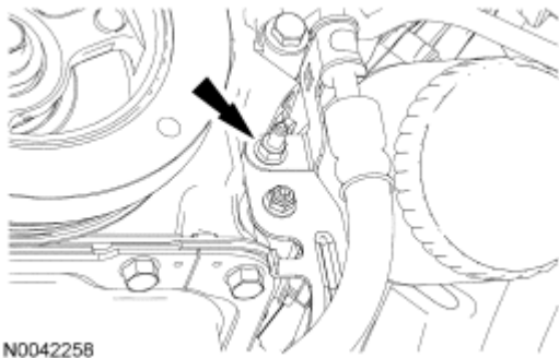
Fig. 470: Locating Power Steering Pressure (PSP) Hose Bracket Nut Courtesy of FORD MOTOR CO.
