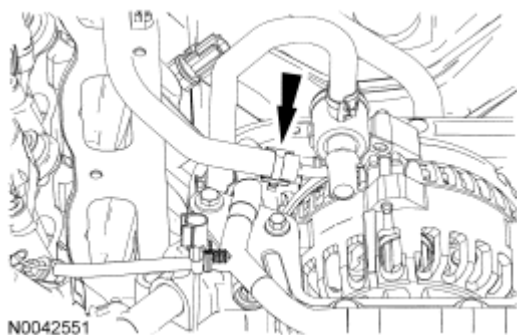
Fig. 483: Locating Heated PCV Fitting Coolant Hose Courtesy of FORD MOTOR CO.
