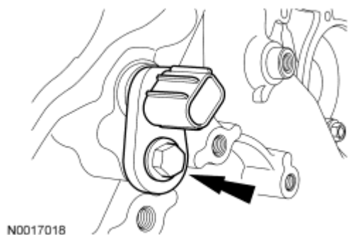
Fig. 308: Locating RH CMP Sensor And Bolt Courtesy of FORD MOTOR CO.
