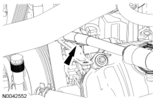
Fig. 482: Locating Wiring Harness Retainer From Cooling Fan Wiring Harness Bracket Courtesy of FORD MOTOR CO.
