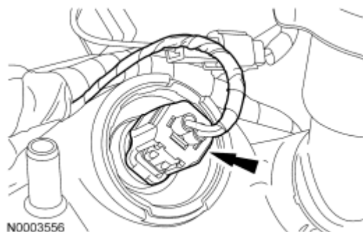
Fig. 281: Locating Camshaft Timing (VCT) Solenoid Electrical Connectors Courtesy of FORD MOTOR CO.
