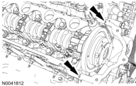
Fig. 412: Locating Silicone Gasket And Sealant Area Courtesy of FORD MOTOR CO.
