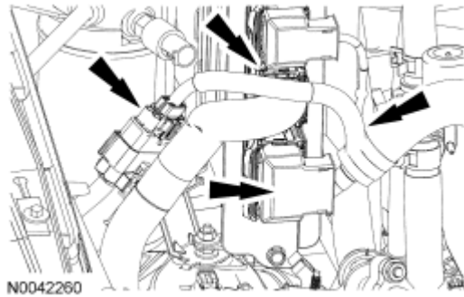
Fig. 474: Locating Wiring Harness Pin-Type Retainer, Powertrain Control Module (PCM) Electrical Connectors And In-Line Electrical Connector Courtesy of FORD MOTOR CO.
