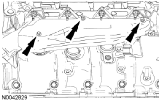
Fig. 266: Identifying RH Exhaust Manifold Heat Shield Bolts Courtesy of FORD MOTOR CO.
