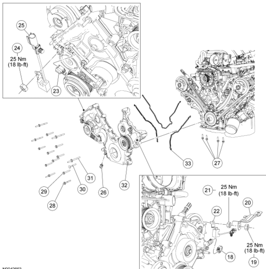
Fig. 30: Exploded View Of Engine Front Cover With Torque Specifications (2 Of 2) Courtesy of FORD MOTOR CO.
