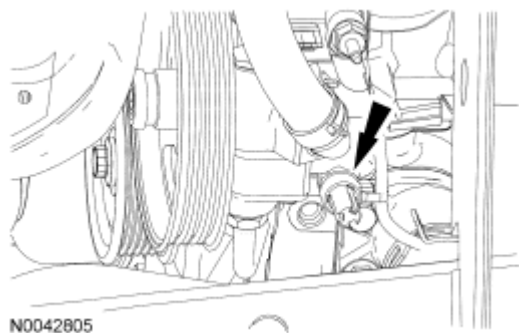
Fig. 204: Locating Power Steering Pump Wiring Harness Retainer Courtesy of FORD MOTOR CO.
