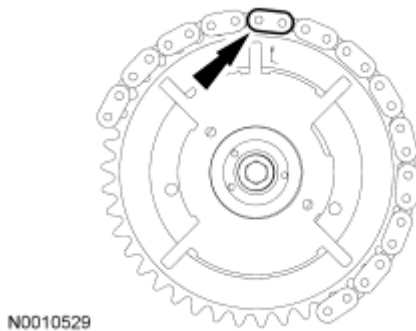
Fig. 513: Positioning LH Timing Chain On Camshaft Sprocket Courtesy of FORD MOTOR CO.
