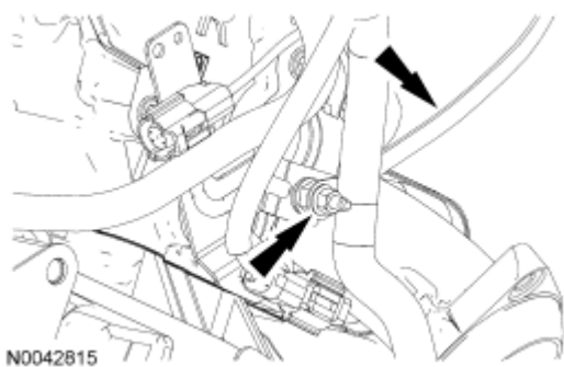
Fig. 292: Locating Ground Strap Nut Courtesy of FORD MOTOR CO.
