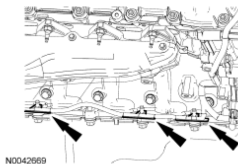
Fig. 217: Locating Oil Pan Wiring Harness Retainers Courtesy of FORD MOTOR CO.
