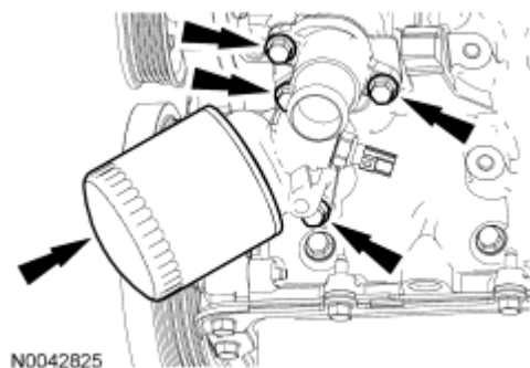
Fig. 299: Locating Bolts And Oil Filter Adapter Courtesy of FORD MOTOR CO.
