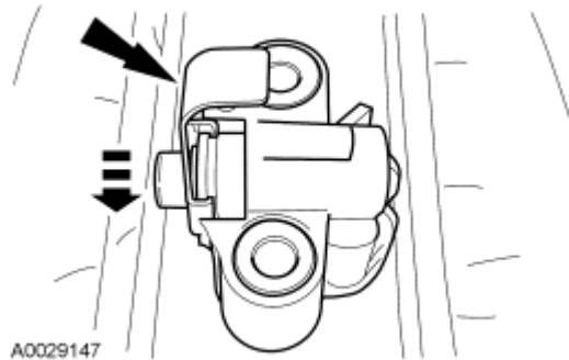
Fig. 384: Identifying Retaining Clip on Tensioner Courtesy of FORD MOTOR CO.
