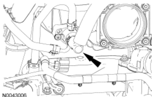
Fig. 177: Locating Positive Crankcase Ventilation (PCV) Valve Hose Courtesy of FORD MOTOR CO.
