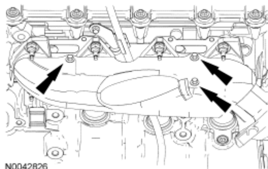
Fig. 494: Locating LH Exhaust Manifold Heat Shield Bolts Courtesy of FORD MOTOR CO.
