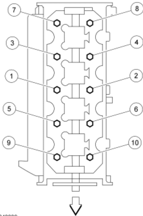
Fig. 495: Identifying RH Cylinder Head Bolts Tightening Sequence Courtesy of FORD MOTOR CO.
