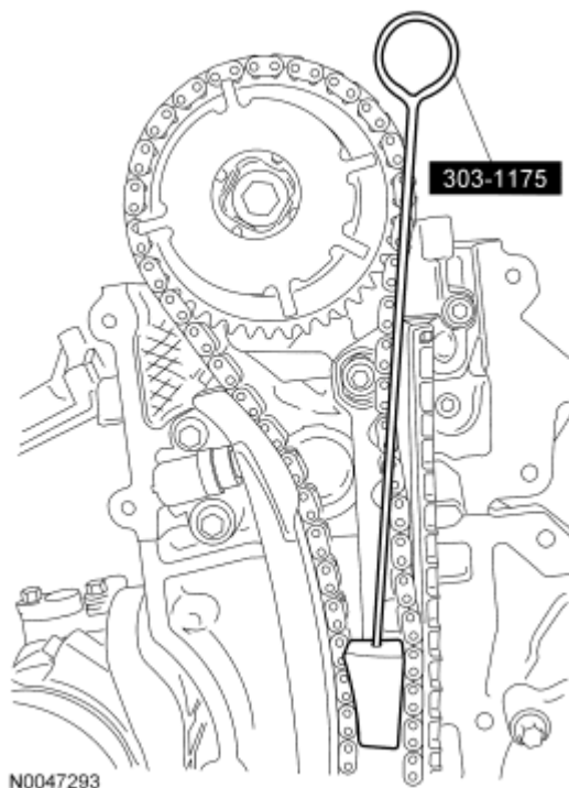
Fig. 118: Installing Special Tool (303-1175) In RH Timing Chain Courtesy of FORD MOTOR CO.
