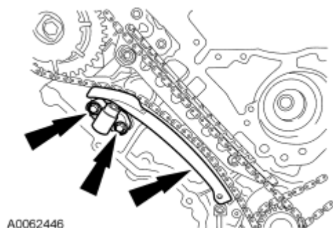
Fig. 51: Identifying RH Timing Chain Tensioner, Tensioner Arm And Bolts Courtesy of FORD MOTOR CO.
