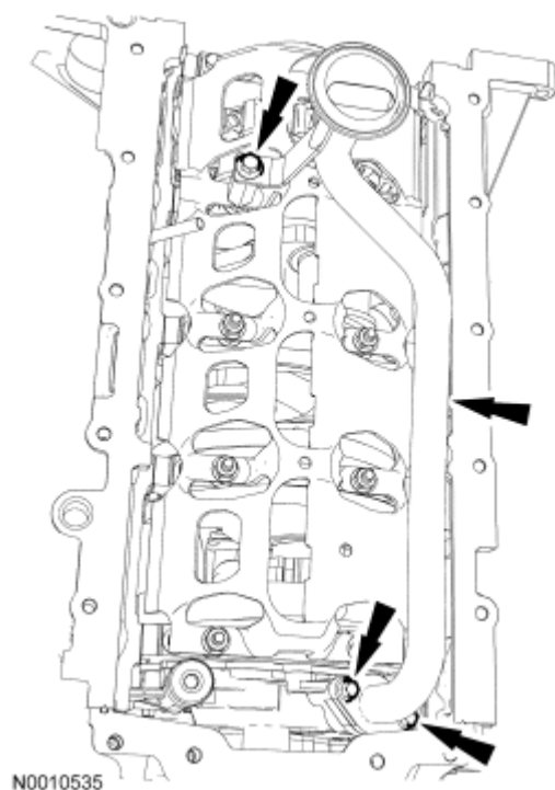
Fig. 173: Locating Oil Pump Screen And Pickup Tube And Bolt Courtesy of FORD MOTOR CO.
