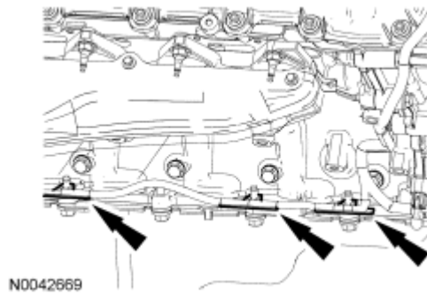
Fig. 278: Locating Oil Pan Wiring Harness Retainers Courtesy of FORD MOTOR CO.
