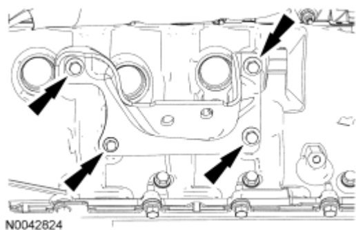
Fig. 303: Locating RH Engine Support Insulator Bracket Bolts Courtesy of FORD MOTOR CO.
