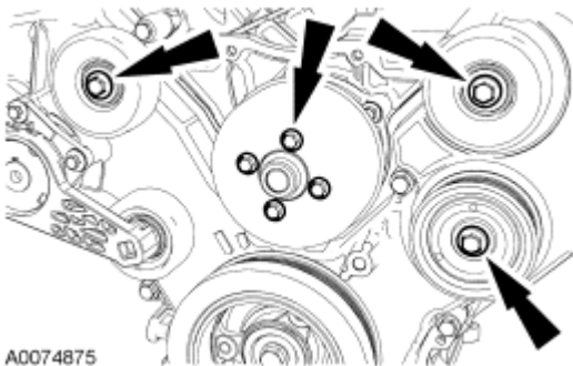
Fig. 408: Locating Coolant Pump Pulley And Accessory Drive Belt Idler Pulley Bolts Courtesy of FORD MOTOR CO.
