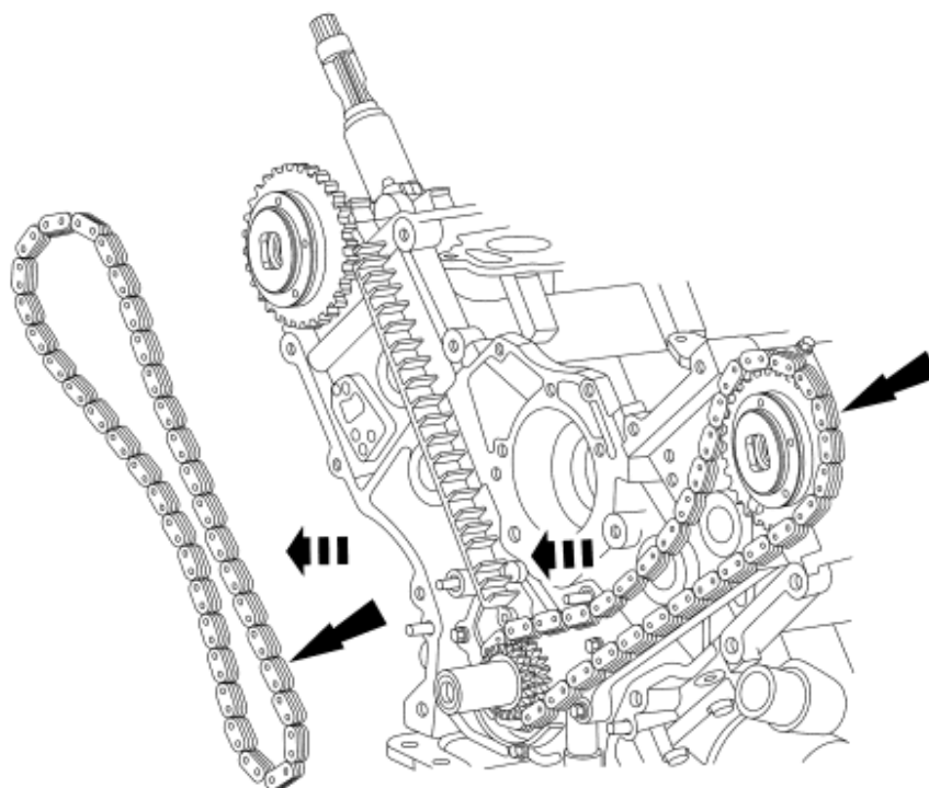
Fig. 254: Identifying RH/LH Timing Chains Courtesy of FORD MOTOR CO.
