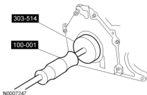
Fig. 274: Removing Crankshaft Rear Oil Seal Slinger Courtesy of FORD MOTOR CO.
