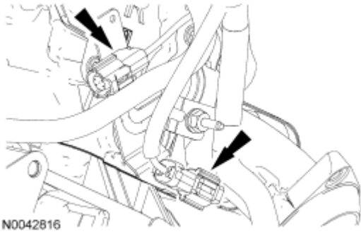
Fig. 293: Locating Electrical Connector Retainers And Engine Wiring Harness Courtesy of FORD MOTOR CO.
