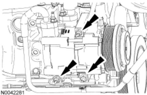
Fig. 208: Locating A/C Compressor Stud Bolt And Nut Courtesy of FORD MOTOR CO.
