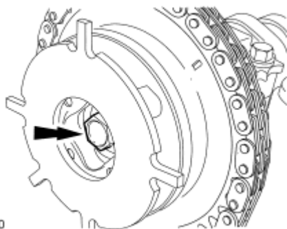
Fig. 114: Identifying Camshaft Phase And Sprocket Assembly Bolt Courtesy of FORD MOTOR CO.
