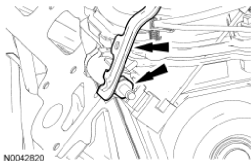
Fig. 435: Locating Cooling Fan Wiring Harness Bracket Nut Courtesy of FORD MOTOR CO.
