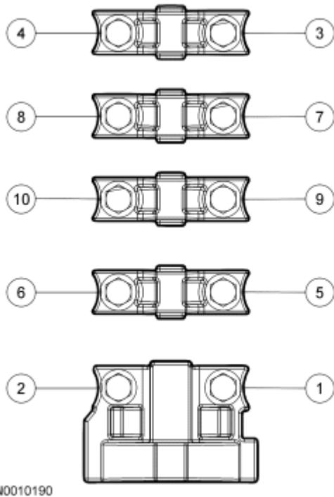
Fig. 258: Identifying Camshaft Bearing Caps Loosening/Tightening Sequence Courtesy of FORD MOTOR CO.
