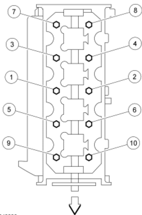
Fig. 373: Identifying RH Cylinder Head Bolts Tightening Sequence Courtesy of FORD MOTOR CO.
