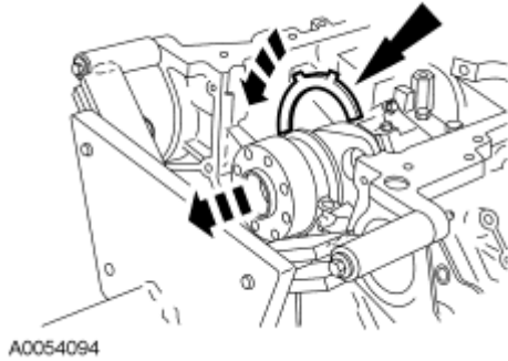
Fig. 358: Locating Crankshaft Upper Thrust Washer At Back Of Upper Main Bearing Courtesy of FORD MOTOR CO.
