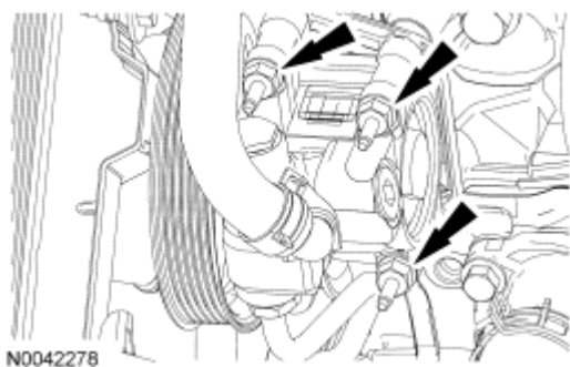
Fig. 466: Locating Power Steering Pump Stud Bolts Courtesy of FORD MOTOR CO.
