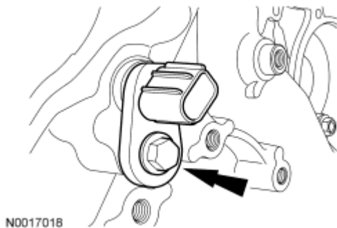
Fig. 411: Locating RH CMP Sensor And Bolt Courtesy of FORD MOTOR CO.
