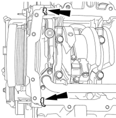
Fig. 449: Applying Silicone Gasket And Sealant At Engine Front Cover-To-Cylinder Block Sealing Surface Courtesy of FORD MOTOR CO.
