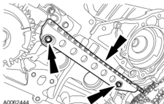
Fig. 255: Identifying Timing Chain Guide And Mounting Bolts Courtesy of FORD MOTOR CO.
