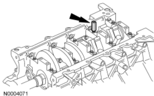
Fig. 369: Locating Pickup Tube Spacer Courtesy of FORD MOTOR CO.
