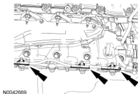
Fig. 554: Locating Oil Pan Wiring Harness Retainers Courtesy of FORD MOTOR CO.
