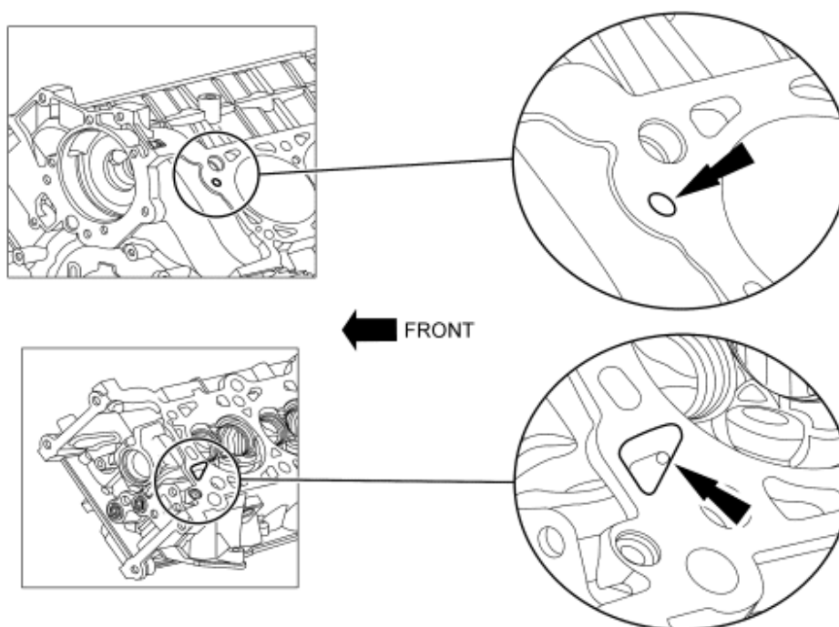
Fig. 341: Identifying Cylinder Head/Cylinder Block Oil Pressure Feed Areas Courtesy of FORD MOTOR CO.
