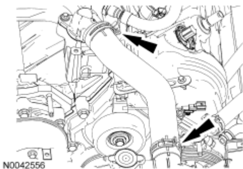
Fig. 478: Locating Upper Radiator Hose Clamps Courtesy of FORD MOTOR CO.
