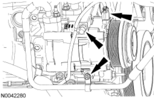
Fig. 207: Locating A/C Hose Bracket And A/C Clutch Electrical Connector Courtesy of FORD MOTOR CO.
