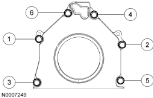
Fig. 26: Tightening Sequence Of Crankshaft Rear Seal Retainer Plate Bolts Courtesy of FORD MOTOR CO.
