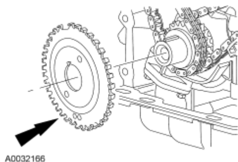
Fig. 320: View Of Crankshaft Sensor Ring At Crankshaft Courtesy of FORD MOTOR CO.
