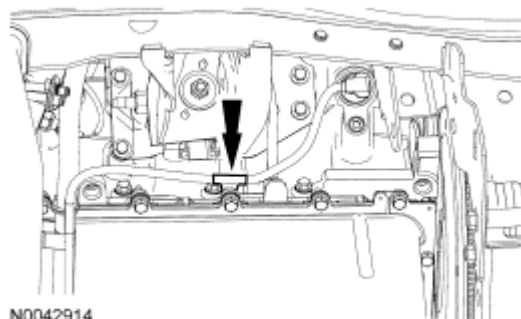
Fig. 159: Locating Block Heater Wiring Harness Retainer Courtesy of FORD MOTOR CO.
