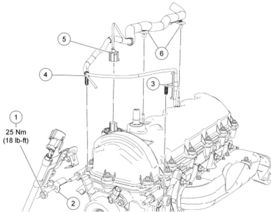
Fig. 3: Exploded View Of Valve Cover With Torque Specification - LH (1 Of 2) Courtesy of FORD MOTOR CO.
