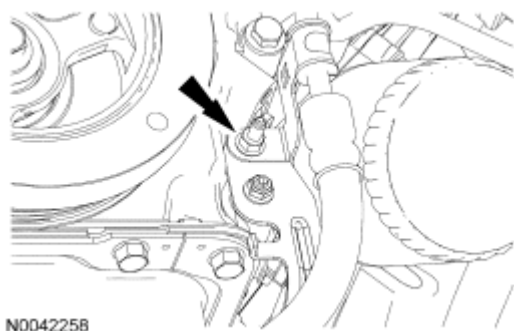
Fig. 167: Locating Power Steering Pressure (PSP) Hose Bracket Nut Courtesy of FORD MOTOR CO.
