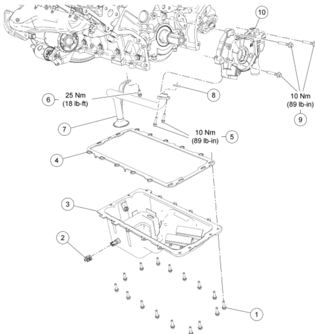
Fig. 154: Exploded View Of Engine Lubrication Components With Torque Specifications Courtesy of FORD MOTOR CO.
