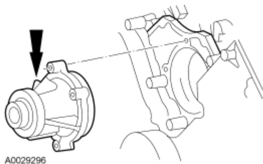
Fig. 405: Identifying Coolant Pump Courtesy of FORD MOTOR CO.
