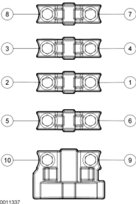
Fig. 117: Identifying Camshaft Bearing Cap Bolt Loosening/Tightening Sequence
