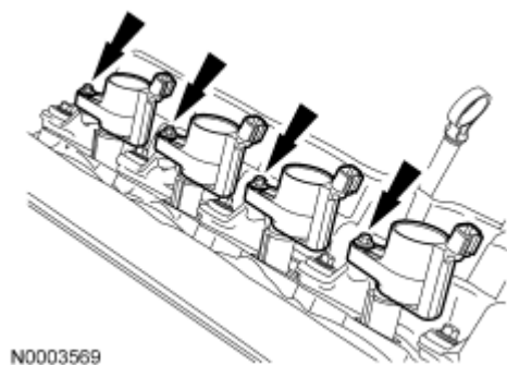
Fig. 234: Identifying Ignition Coils And Bolts Courtesy of FORD MOTOR CO.
