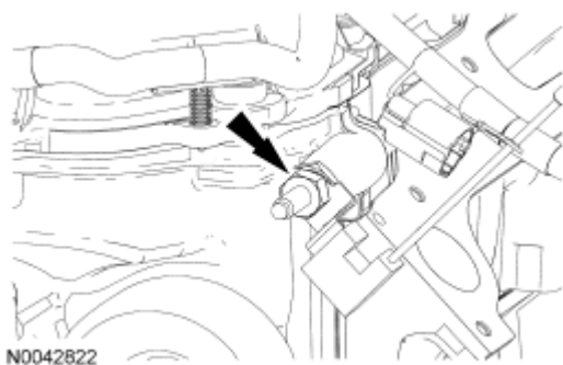
Fig. 549: Locating RH Radio Ignition Interference Capacitor Nut Courtesy of FORD MOTOR CO.
