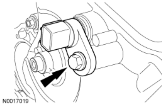
Fig. 410: Locating LH Camshaft Position (CMP) Sensor And Bolt Courtesy of FORD MOTOR CO.
