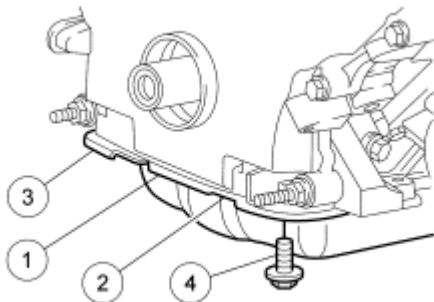
Fig. 526: Identifying Tightening Sequence Of Front Oil Pan Bolts Courtesy of FORD MOTOR CO.
