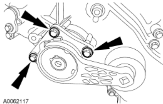
Fig. 312: Identifying Accessory Drive Belt Tensioner Bolts Courtesy of FORD MOTOR CO.
