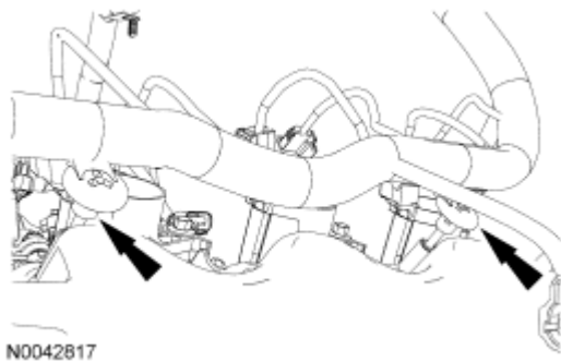
Fig. 544: Locating LH Valve Cover Studs Courtesy of FORD MOTOR CO.
