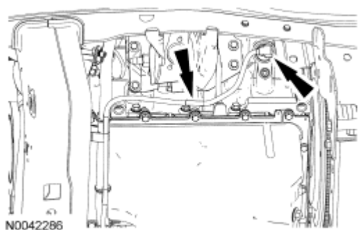
Fig. 458: Locating Block Heater Wiring Harness Retainers And Block Heater Electrical Connector
