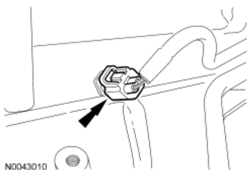
Fig. 230: Locating Cylinder Head Temperature (CHT) Sensor Electrical Connector Courtesy of FORD MOTOR CO.
