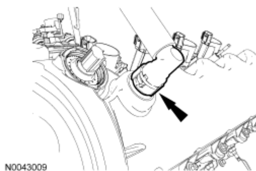
Fig. 233: Locating Positive Crankcase Ventilation (PCV) Hose Courtesy of FORD MOTOR CO.
