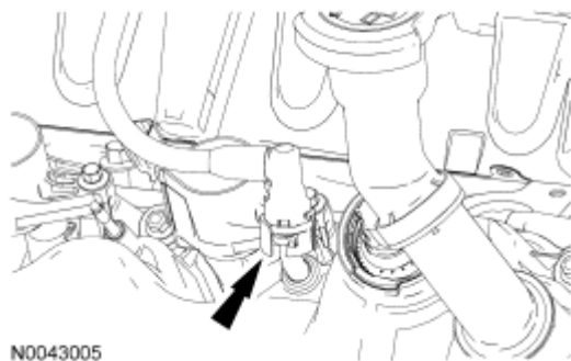
Fig. 539: Locating Breather Tube Connector Retaining Clip Courtesy of FORD MOTOR CO.
