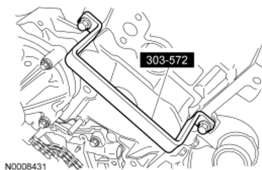
Fig. 334: Identifying Special Tool Onto Cylinder Head Courtesy of FORD MOTOR CO.
