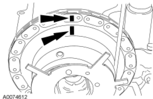
Fig. 94: Identifying Scribe Marks Of Camshaft Phase And Chain Courtesy of FORD MOTOR CO.
