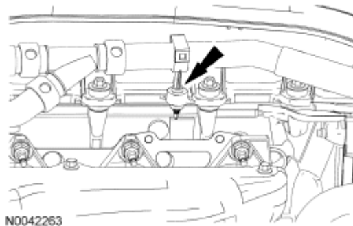
Fig. 475: Locating Heater Hose Retainer Courtesy of FORD MOTOR CO.
