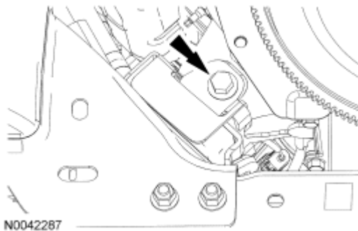
Fig. 214: Locating LH Engine Support Insulator Through-Bolt Courtesy of FORD MOTOR CO.
