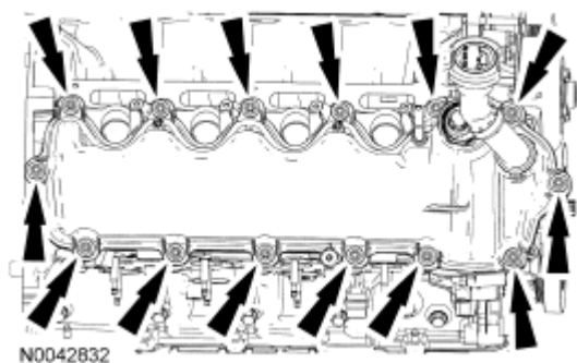
Fig. 237: Locating RH Valve Cover Bolts Courtesy of FORD MOTOR CO.
