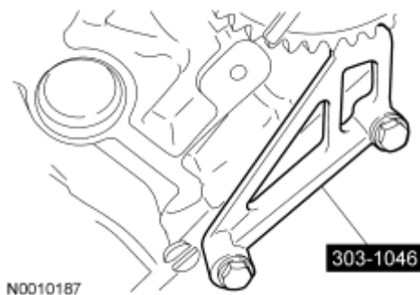
Fig. 504: Identifying Special Sprocket Phase Tool Courtesy of FORD MOTOR CO.
