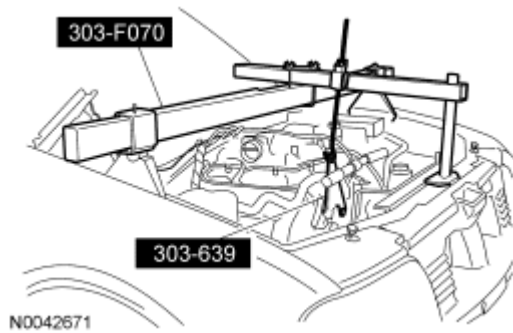
Fig. 181: Identifying Special Tools (303-639) & (303-F070) Courtesy of FORD MOTOR CO.
