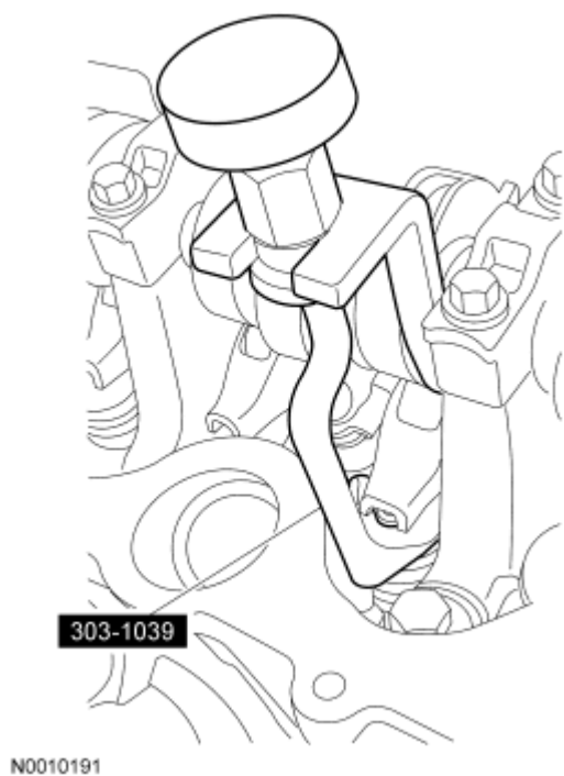
Fig. 99: Compressing Spring Using Special Tool Courtesy of FORD MOTOR CO.
