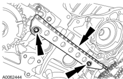
Fig. 331: Identifying Timing Chain Guide And Mounting Bolts Courtesy of FORD MOTOR CO.
