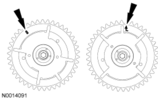
Fig. 507: Rotating Camshaft Sprockets To Position RH Camshaft Sprocket Timing Mark Courtesy of FORD MOTOR CO.
