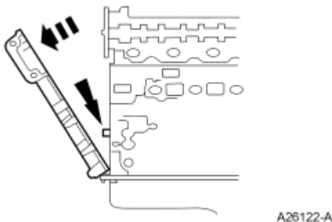
Fig. 33: Removing Engine Front Cover From Front Cover-To-Cylinder Block Dowel Courtesy of FORD MOTOR CO.
