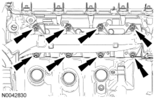
Fig. 267: Locating RH Exhaust Manifold Nuts Courtesy of FORD MOTOR CO.
