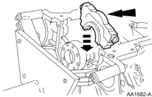
Fig. 359: Locating Rear Main Bearing Cap Courtesy of FORD MOTOR CO.
