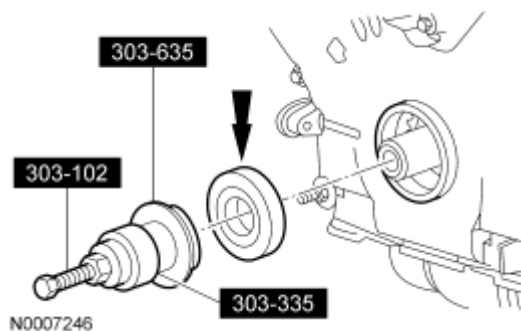
Fig. 402: Installing Crankshaft Front Seal Using Special Tools Courtesy of FORD MOTOR CO.
