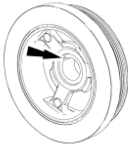
Fig. 12: Applying Silicone Gasket And Sealant To Woodruff Key Slot In Crankshaft Pulley Courtesy of FORD MOTOR CO.
