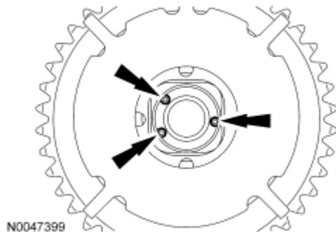
Fig. 125: Inspecting Front Of Camshaft Phase And Sprocket For Missing Or Damaged Roll Pins Courtesy of FORD MOTOR CO.
