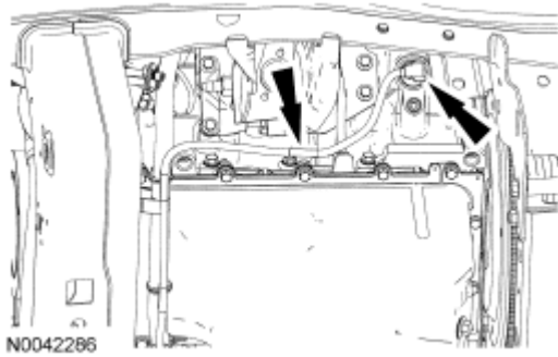
Fig. 213: Locating Block Heater Wiring Harness Retainers And Block Heater Electrical Connector Courtesy of FORD MOTOR CO.
