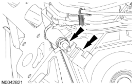
Fig. 434: Locating LH Radio Interference Capacitor And Nuts Courtesy of FORD MOTOR CO.
