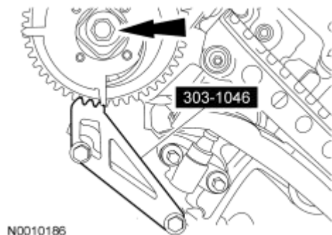
Fig. 256: Identifying VCT Phase Sprocket Bolt And Holder Tool Courtesy of FORD MOTOR CO.
