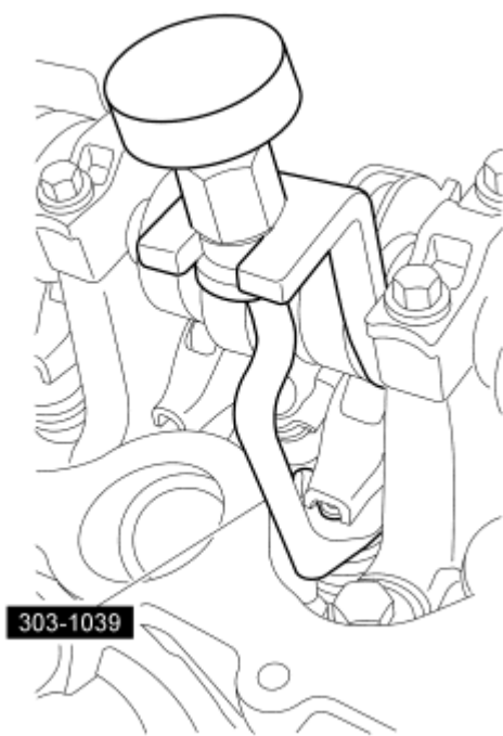
Fig. 326: Compressing Spring Using Special Tool Courtesy of FORD MOTOR CO.
