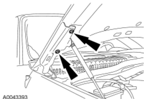
Fig. 184: Locating Hood Hinge Bolts Courtesy of FORD MOTOR CO.
