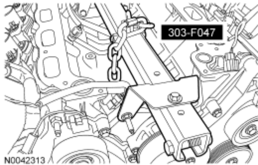
Fig. 277: Identifying Special Tool (303-F047) Courtesy of FORD MOTOR CO.
