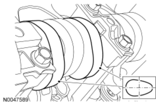
Fig. 98: Checking Position Of No. 5 Cylinder Intake And Exhaust Camshaft Lobes Courtesy of FORD MOTOR CO.
