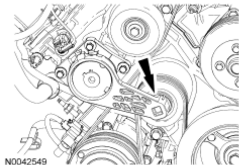
Fig. 186: Locating Accessory Drive Belt Tensioner Courtesy of FORD MOTOR CO.
