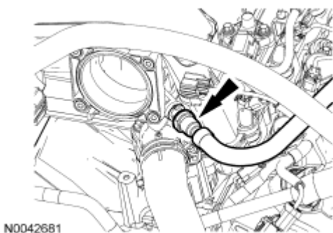
Fig. 179: Locating Evaporative Emission (EVAP) Hose Courtesy of FORD MOTOR CO.
