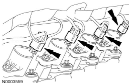
Fig. 289: Locating Ignition Coil Electrical Connectors Courtesy of FORD MOTOR CO.
