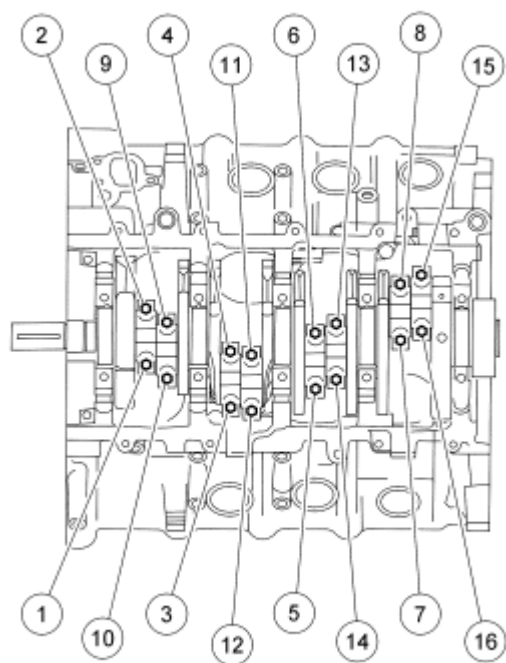
Fig. 367: Identifying Main Bearing Caps Bolts Tightening Sequence Courtesy of FORD MOTOR CO.
