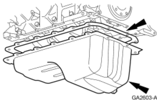
Fig. 450: Positioning New Oil Pan Gasket And Oil Pan Courtesy of FORD MOTOR CO.
