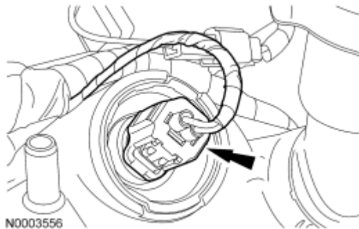
Fig. 220: Locating Camshaft Timing (VCT) Solenoid Electrical Connectors Courtesy of FORD MOTOR CO.
