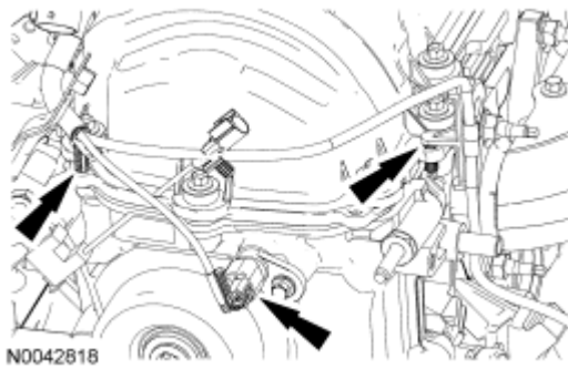
Fig. 285: Locating LH Camshaft Position Sensor And Attach Wiring Harness Retainers Courtesy of FORD MOTOR CO.
