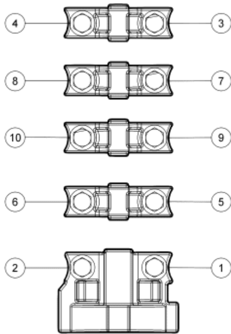
Fig. 338: Identifying Camshaft Bearing Caps Loosening/Tightening Sequence
