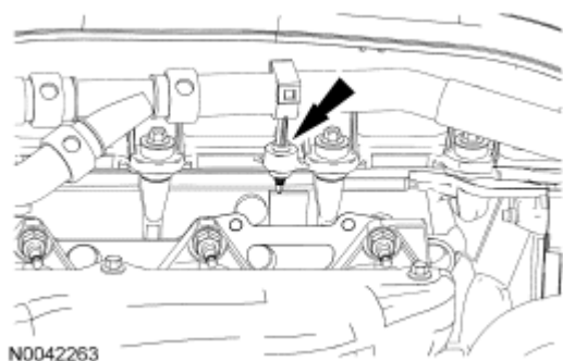
Fig. 196: Locating Heater Hose Retainer Courtesy of FORD MOTOR CO.
