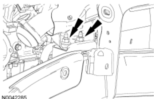
Fig. 212: Locating RH Engine Support Insulator Nuts Courtesy of FORD MOTOR CO.
