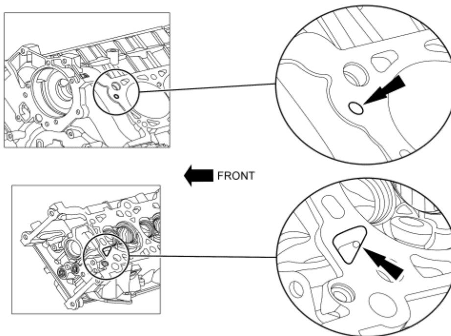
Fig. 271: Identifying Cylinder Head/Cylinder Block Oil Pressure Feed Areas Courtesy of FORD MOTOR CO.
