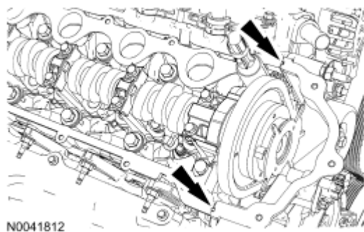
Fig. 8: Locating Silicone Gasket And Sealant Area Courtesy of FORD MOTOR CO.
