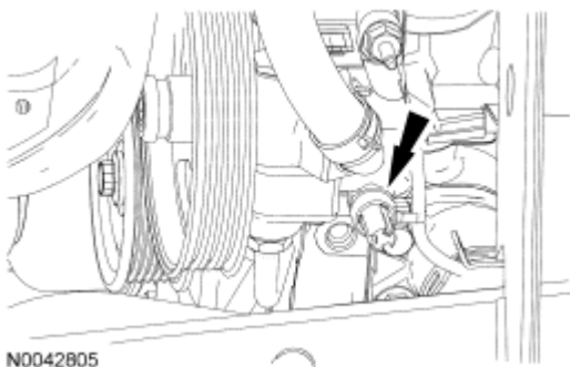
Fig. 467: Locating Power Steering Pump Wiring Harness Retainer Courtesy of FORD MOTOR CO.
