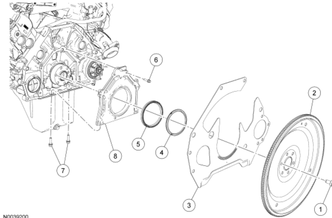
Fig. 17: Exploded View Of Flexplate Or Flywheel & Crankshaft Rear Seal Courtesy of FORD MOTOR CO.
