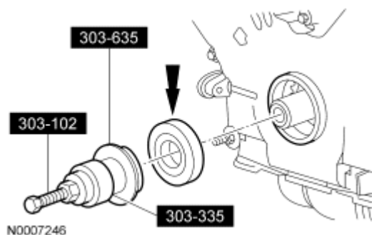
Fig. 528: Installing Crankshaft Front Seal Using Special Tools Courtesy of FORD MOTOR CO.
