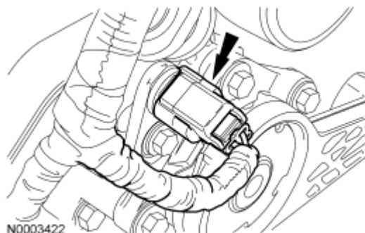
Fig. 280: Identifying RH CMP Sensor Electrical Connector Courtesy of FORD MOTOR CO.
