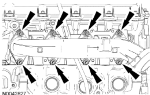
Fig. 301: Locating LH Exhaust Manifold Nuts Courtesy of FORD MOTOR CO.
