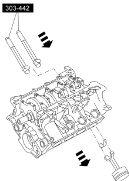
Fig. 345: Pushing Piston Through Top Of Cylinder Block Courtesy of FORD MOTOR CO.
