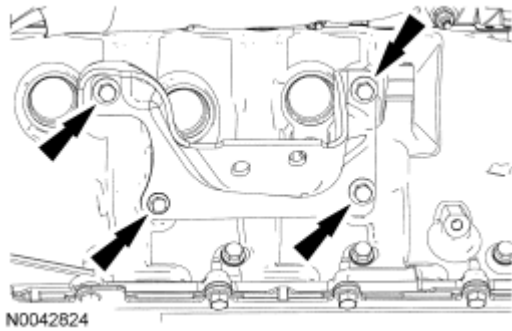
Fig. 418: Locating RH Engine Support Insulator Bracket Bolts Courtesy of FORD MOTOR CO.
