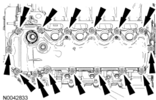
Fig. 307: Locating LH Valve Cover Bolts Courtesy of FORD MOTOR CO.
