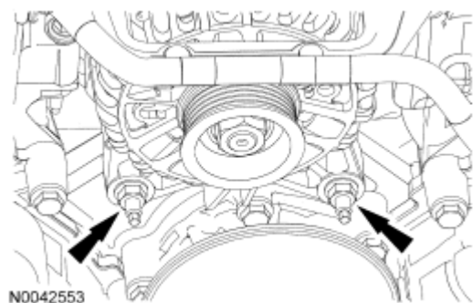
Fig. 190: Locating Nuts Courtesy of FORD MOTOR CO.
