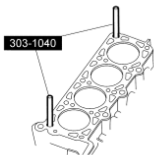
Fig. 489: Positioning Cylinder Head Gaskets And Cylinder Heads Over Dowels Courtesy of FORD MOTOR CO.
