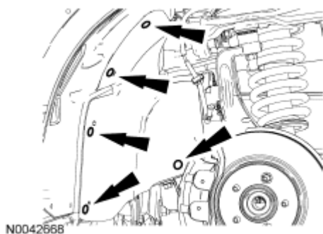
Fig. 460: Locating Pushpins And Splash Shield Courtesy of FORD MOTOR CO.
