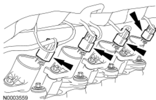
Fig. 228: Locating Ignition Coil Electrical Connectors Courtesy of FORD MOTOR CO.
