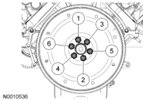
Fig. 18: Identifying Flexplate Bolts Tightening Sequence Courtesy of FORD MOTOR CO.
