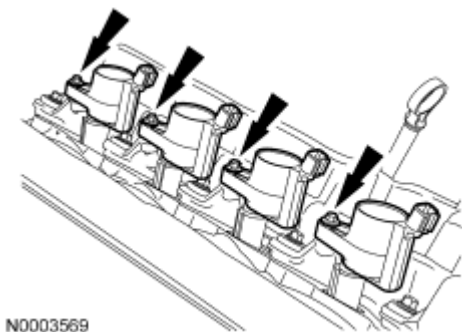
Fig. 424: Identifying Ignition Coils And Bolts Courtesy of FORD MOTOR CO.
