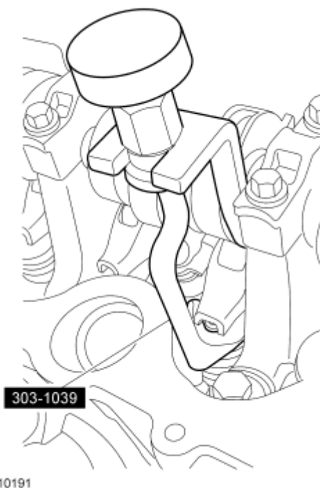
Fig. 522: Compressing Spring Using Special Tool Courtesy of FORD MOTOR CO.
