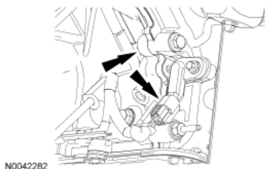
Fig. 553: Locating Crankshaft Position Sensor Electrical Connector And Wiring Harness Retainer Courtesy of FORD MOTOR CO.
