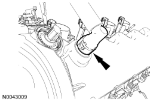
Fig. 296: Locating Positive Crankcase Ventilation (PCV) Hose Courtesy of FORD MOTOR CO.
