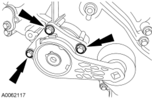
Fig. 407: Identifying Accessory Drive Belt Tensioner Bolts Courtesy of FORD MOTOR CO.
