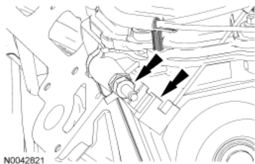
Fig. 287: Locating LH Radio Interference Capacitor And Nuts Courtesy of FORD MOTOR CO.
