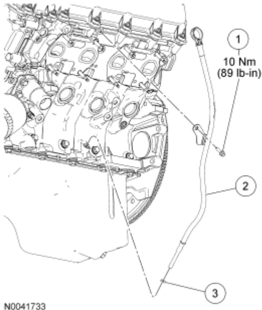
Fig. 175: Exploded View Of Oil Level Indicator & Tube With Torque Specification Courtesy of FORD MOTOR CO.
