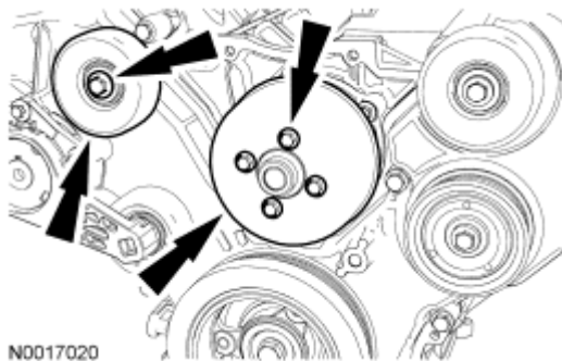
Fig. 531: Locating Accessory Drive Belt Idler Pulley And Bolts Courtesy of FORD MOTOR CO.
