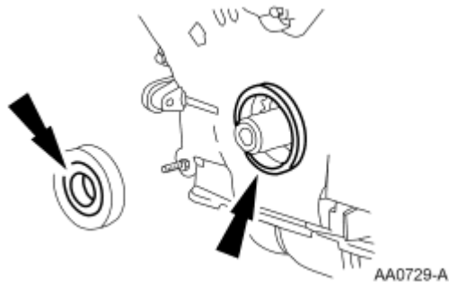
Fig. 15: Lubricating Engine Front Cover And Crankshaft Front Seal Inner Lip With Clean Engine Oil Courtesy of FORD MOTOR CO.
