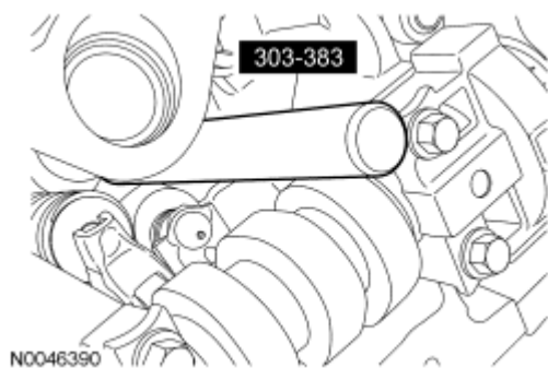
Fig. 351: Installing Valve Seal Using Special Tool Courtesy of FORD MOTOR CO.
