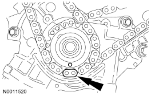
Fig. 391: Aligning Crankshaft Sprocket Timing Mark And RH Timing Chain Link Courtesy of FORD MOTOR CO.
