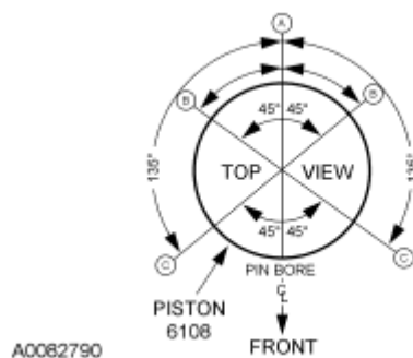
Fig. 364: Identifying Piston Ring Gaps Positioning Courtesy of FORD MOTOR CO.
