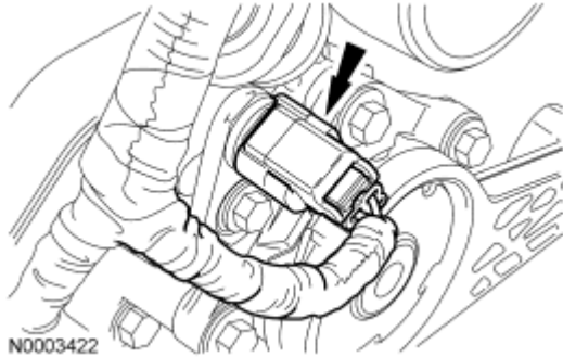
Fig. 219: Identifying RH CMP Sensor Electrical Connector Courtesy of FORD MOTOR CO.
