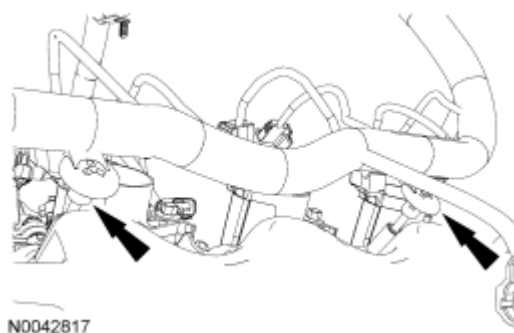
Fig. 227: Locating LH Valve Cover Studs Courtesy of FORD MOTOR CO.
