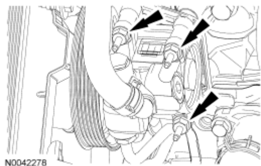
Fig. 205: Locating Power Steering Pump Stud Bolts Courtesy of FORD MOTOR CO.
