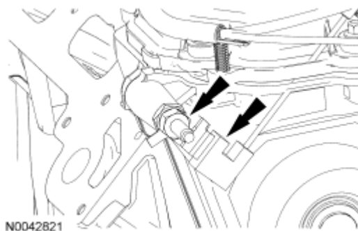
Fig. 226: Locating LH Radio Interference Capacitor And Nuts Courtesy of FORD MOTOR CO.
