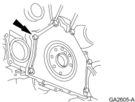
Fig. 446: Locating Crankshaft Rear Seal Retainer Plate Bolts Courtesy of FORD MOTOR CO.
