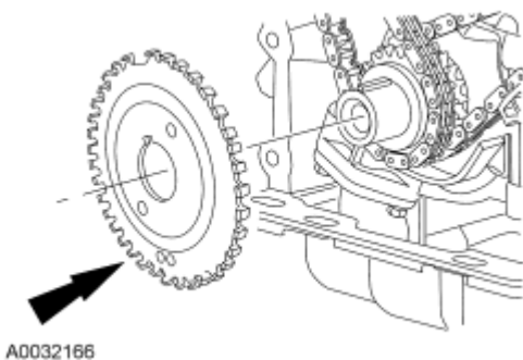
Fig. 396: View Of Crankshaft Sensor Ring At Crankshaft Courtesy of FORD MOTOR CO.
