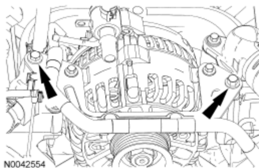
Fig. 480: Locating Alternator Bracket And Wiring Harness Bolts Courtesy of FORD MOTOR CO.
