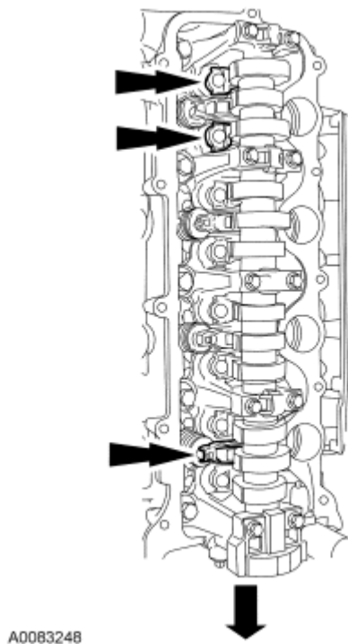
Fig. 107: Identifying RH Cylinder Head Camshaft Roller Followers And Bolts Courtesy of FORD MOTOR CO.
