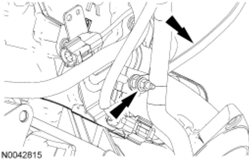
Fig. 429: Locating Ground Strap Nut Courtesy of FORD MOTOR CO.
