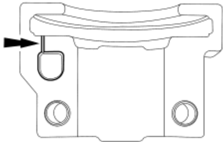
Fig. 259: Identifying Camshaft Front Thrust Bearing Cap Oil Metering Groove Courtesy of FORD MOTOR CO.
