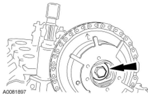
Fig. 61: Identifying Camshaft Phase And Sprocket Assembly Bolt Courtesy of FORD MOTOR CO.
