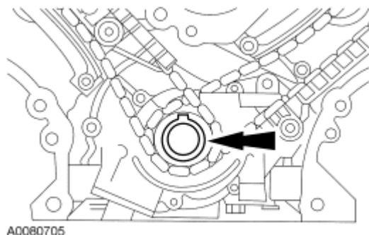
Fig. 245: Positioning Crankshaft Keyway At 12 O'Clock Position Courtesy of FORD MOTOR CO.
