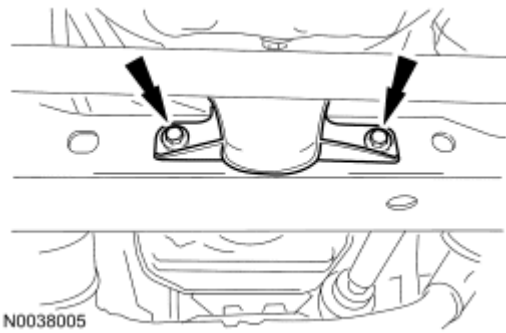
Fig. 164: Locating Oil Drain Splash Shield Bolts Courtesy of FORD MOTOR CO.
