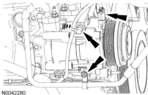
Fig. 464: Locating A/C Hose Bracket And A/C Clutch Electrical Connector Courtesy of FORD MOTOR CO.
