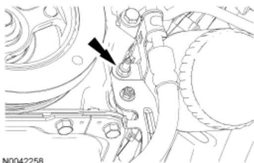
Fig. 201: Locating Power Steering Pressure (PSP) Hose Bracket Nut Courtesy of FORD MOTOR CO.
