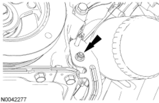
Fig. 469: Locating Battery Cable Bracket Nut Courtesy of FORD MOTOR CO.
