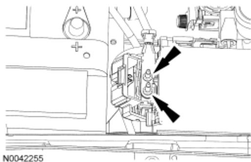
Fig. 486: Locating Wiring Harness Terminals Nuts Courtesy of FORD MOTOR CO.
