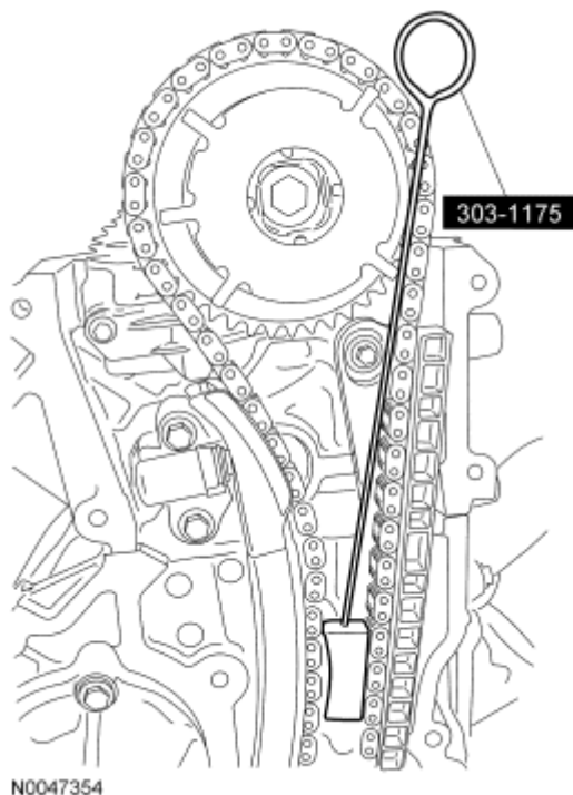
Fig. 88: Identifying Special Tool (303-1175)
