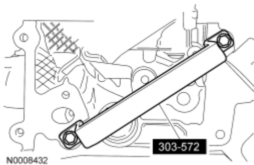
Fig. 265: Identifying Special Tool On Cylinder Head Courtesy of FORD MOTOR CO.
