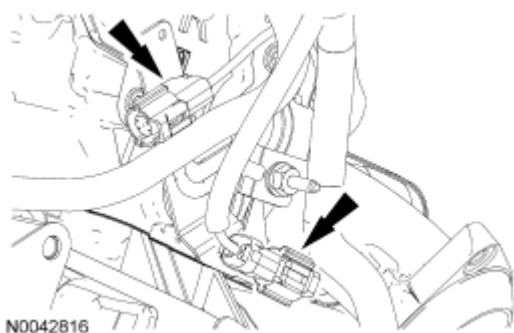
Fig. 540: Locating Electrical Connector Retainers And Engine Wiring Harness Courtesy of FORD MOTOR CO.
