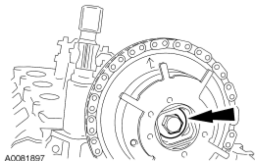
Fig. 93: Identifying Camshaft Phase And Sprocket Assembly Bolt Courtesy of FORD MOTOR CO.
