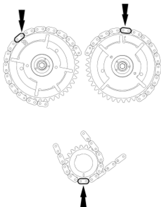
Fig. 77: Verify Correct Alignment Of All Timing Marks Courtesy of FORD MOTOR CO.
