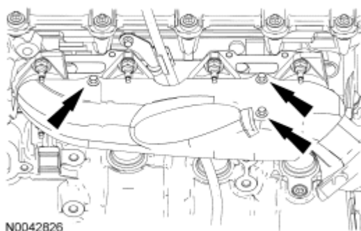
Fig. 300: Locating LH Exhaust Manifold Heat Shield Bolts Courtesy of FORD MOTOR CO.
