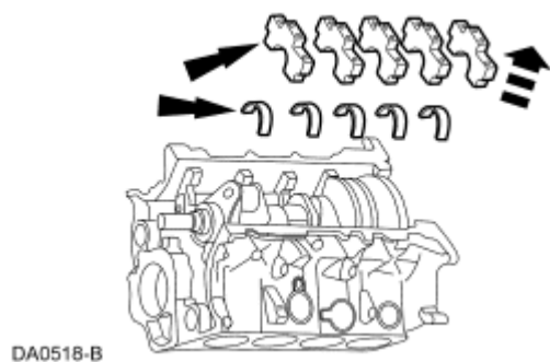
Fig. 347: Locating Main Bearing Caps, Lower Crankshaft Main Bearings And Lower Thrust Washer Courtesy of FORD MOTOR CO.
