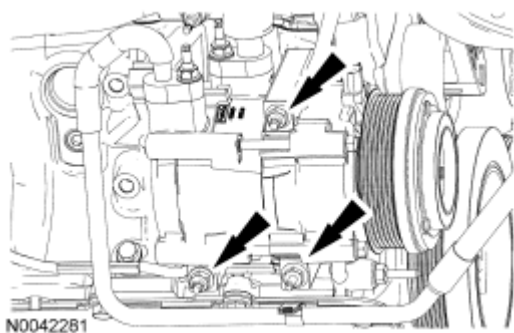
Fig. 463: Locating A/C Compressor Stud Bolt And Nut Courtesy of FORD MOTOR CO.
