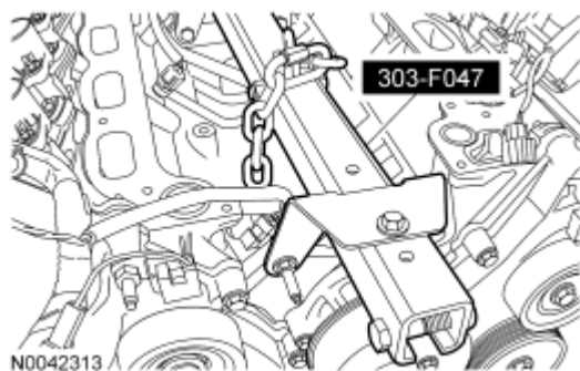
Fig. 555: Identifying Special Tool (303-F047) Courtesy of FORD MOTOR CO.
