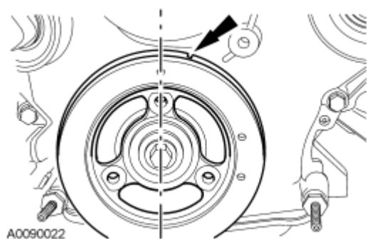
Fig. 81: Locating Crankshaft Damper Spoke Timing Mark Courtesy of FORD MOTOR CO.
