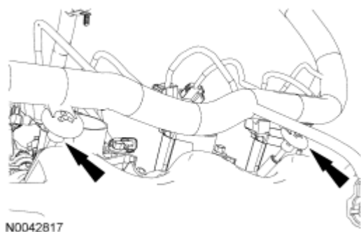
Fig. 288: Locating LH Valve Cover Studs Courtesy of FORD MOTOR CO.
