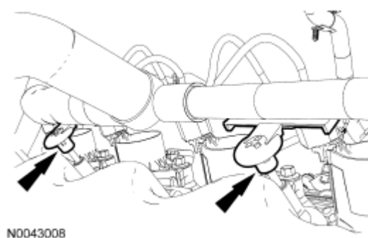
Fig. 229: Locating RH Valve Cover Studs Courtesy of FORD MOTOR CO.
