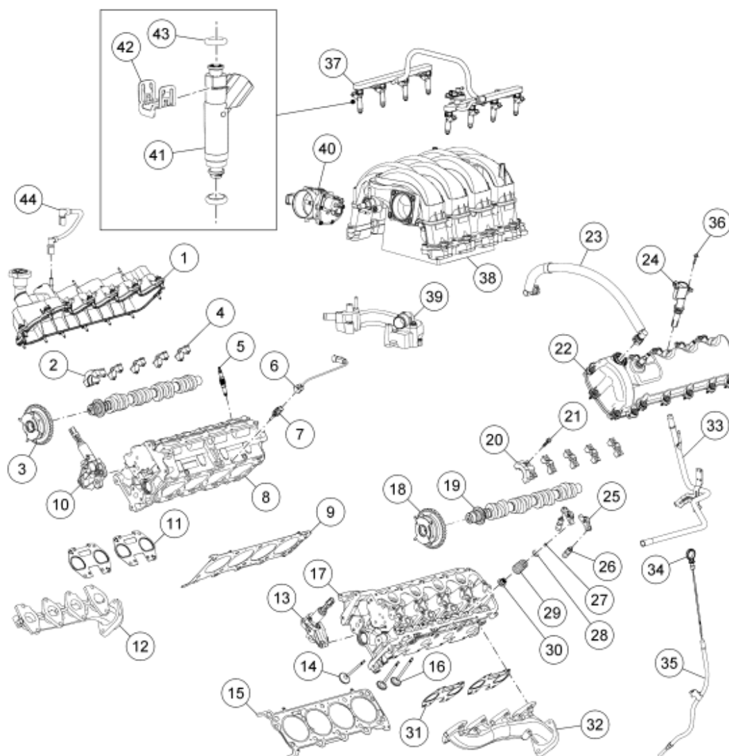
Fig. 355: Exploded View Of Engine - Upper End Courtesy of FORD MOTOR CO.
