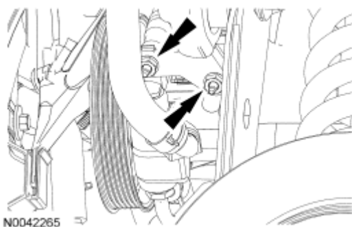
Fig. 203: Locating Wiring Harness Bracket Nuts Courtesy of FORD MOTOR CO.
