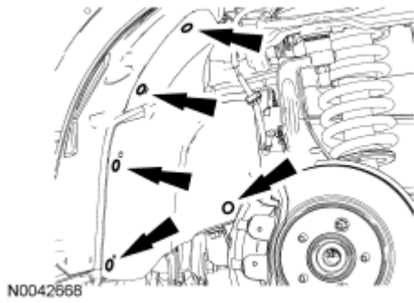
Fig. 151: Locating Pushpins And Splash Shield Courtesy of FORD MOTOR CO.
