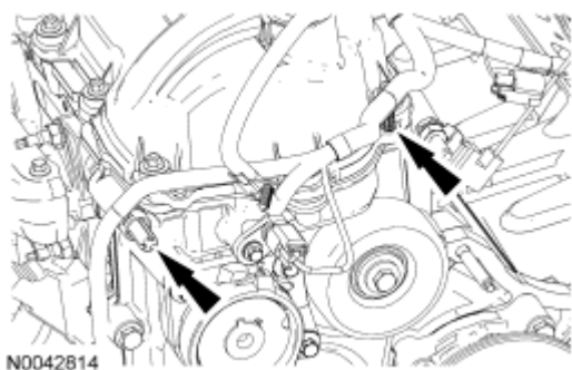
Fig. 550: Locating Wiring Harness Retainers Courtesy of FORD MOTOR CO.
