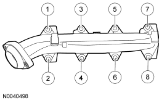
Fig. 152: Identifying Tightening Sequence Of Exhaust Manifold-To-Catalytic Converter Nuts Courtesy of FORD MOTOR CO.
