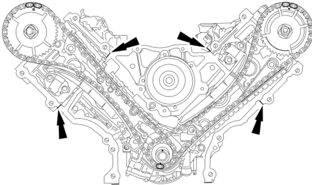
Fig. 398: Applying Bead Of Silicone Gasket And Sealant Along Cylinder Head-To-Cylinder Block Surface
