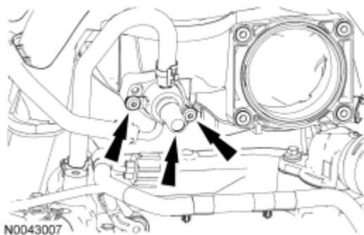
Fig. 178: Locating Heated PCV Fitting Bolts Courtesy of FORD MOTOR CO.
