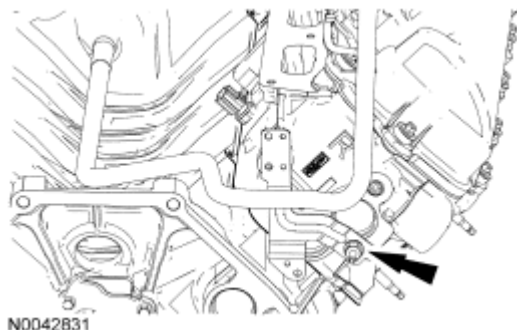
Fig. 500: Locating Heater Supply Tube Stud Bolt Courtesy of FORD MOTOR CO.
