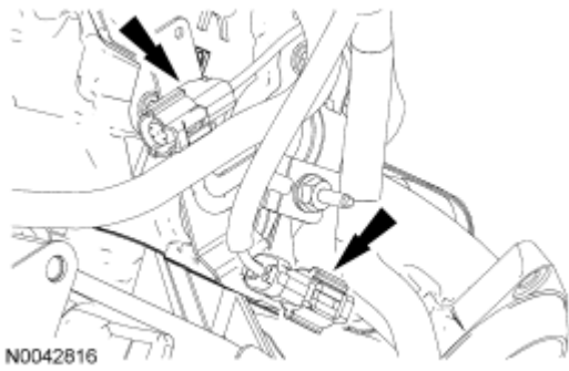
Fig. 231: Locating Electrical Connector Retainers And Engine Wiring Harness Courtesy of FORD MOTOR CO.
