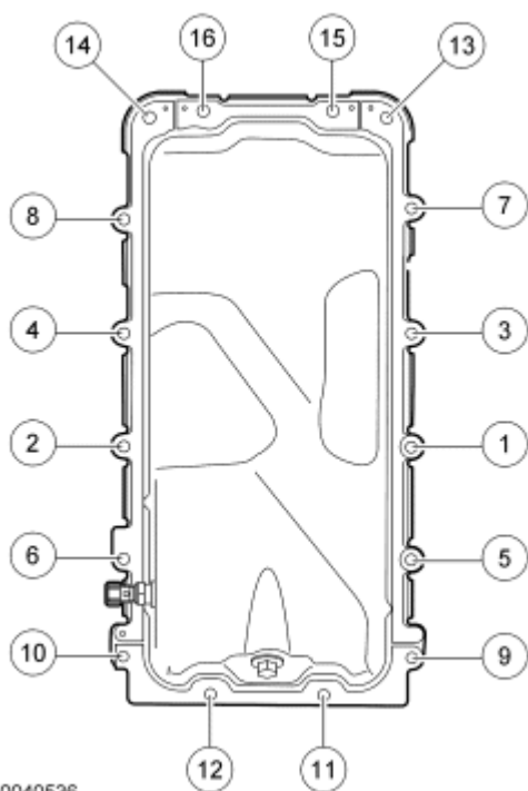
Fig. 162: Identifying Tightening Sequence Of Bolts Courtesy of FORD MOTOR CO.
