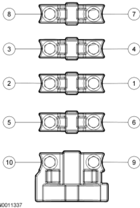
Fig. 502: Identifying Camshaft Bearing Cap Bolt Loosening/Tightening Sequence Courtesy of FORD MOTOR CO.
