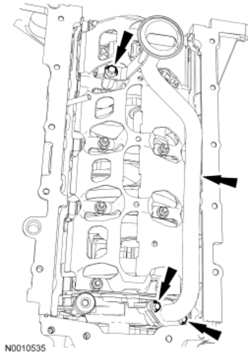
Fig. 169: Locating Oil Pump Screen And Pickup Tube And Bolt Courtesy of FORD MOTOR CO.
