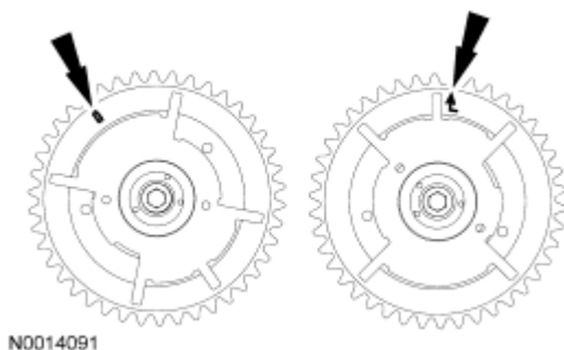
Fig. 382: Rotating Camshaft Sprockets To Position RH Camshaft Sprocket Timing Mark Courtesy of FORD MOTOR CO.
