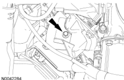
Fig. 210: Locating RH Engine Support Insulator Bracket Bolt Courtesy of FORD MOTOR CO.
