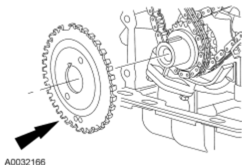
Fig. 244: View Of Crankshaft Sensor Ring At Crankshaft Courtesy of FORD MOTOR CO.
