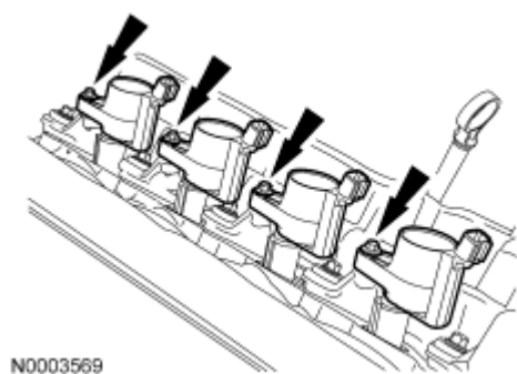
Fig. 297: Identifying Ignition Coils And Bolts Courtesy of FORD MOTOR CO.
