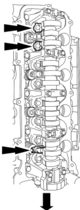
Fig. 323: Identifying RH Cylinder Head Camshaft Roller Followers And Bolts Courtesy of FORD MOTOR CO.
