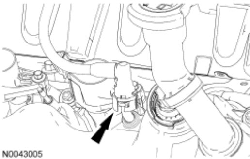
Fig. 232: Locating Breather Tube Connector Retaining Clip Courtesy of FORD MOTOR CO.
