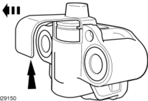
Fig. 390: View Of Retaining Clip And Timing Chain Tensioner Courtesy of FORD MOTOR CO.
