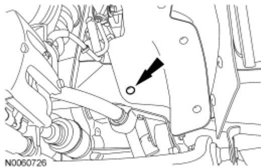
Fig. 147: Locating Push Pin Courtesy of FORD MOTOR CO.
