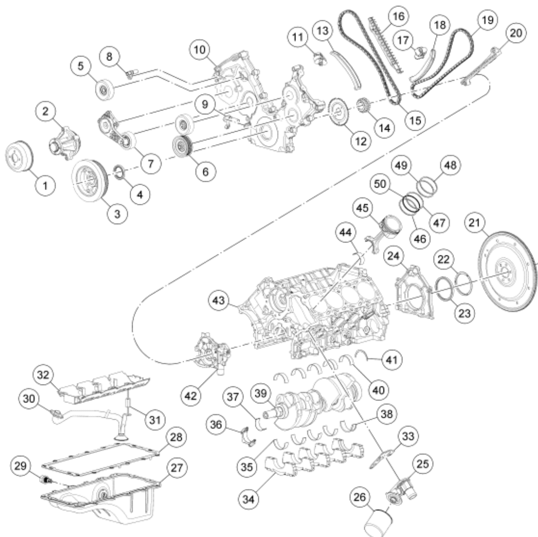
Fig. 356: Exploded View Of Engine - Lower End Courtesy of FORD MOTOR CO.
