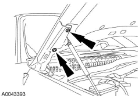
Fig. 487: Locating Hood Hinge Bolts Courtesy of FORD MOTOR CO.
