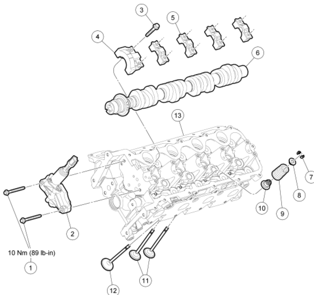
Fig. 349: Exploded View Of Cylinder Head With Torque Specification Courtesy of FORD MOTOR CO.
