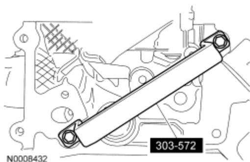
Fig. 335: Identifying Special Tool On Cylinder Head Courtesy of FORD MOTOR CO.
