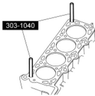
Fig. 371: Positioning Cylinder Head Gaskets And Cylinder Heads Over Dowels Courtesy of FORD MOTOR CO.
