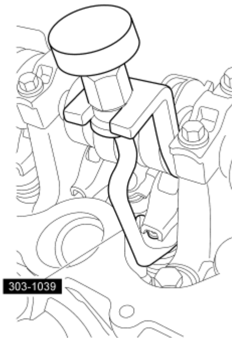
Fig. 250: Compressing Spring Using Special Tool Courtesy of FORD MOTOR CO.
