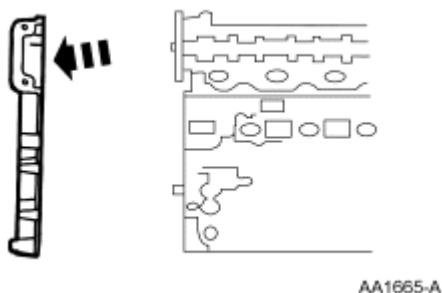
Fig. 243: Removing Engine Front Cover From Cylinder Block Courtesy of FORD MOTOR CO.
