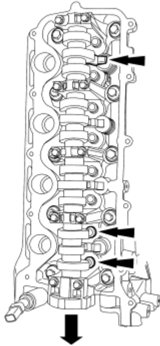
Fig. 85: Locating LH Cylinder Head Camshaft Roller Followers And Bolts Courtesy of FORD MOTOR CO.
