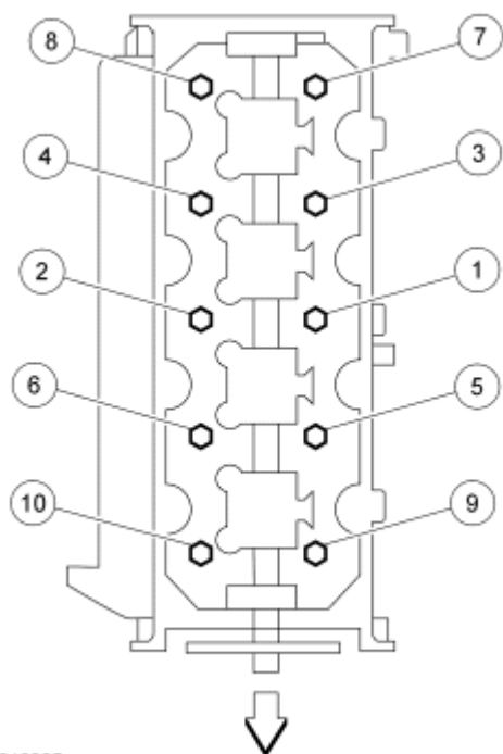
Fig. 372: Identifying Cylinder Head Bolt Tightening Sequence Courtesy of FORD MOTOR CO.
