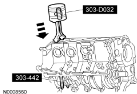
Fig. 365: Using Special Tools To Install Piston And Connecting Rod Assembly Courtesy of FORD MOTOR CO.
