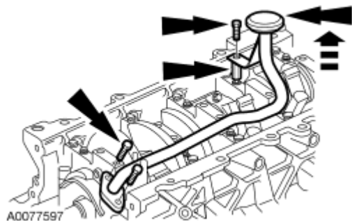
Fig. 342: Identifying Oil Pump Screen And Pickup Tube And Spacer Courtesy of FORD MOTOR CO.
