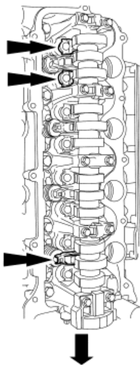
Fig. 247: Identifying RH Cylinder Head Camshaft Roller Followers And Bolts Courtesy of FORD MOTOR CO.
