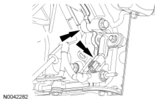
Fig. 218: Locating Crankshaft Position Sensor Electrical Connector And Wiring Harness Retainer Courtesy of FORD MOTOR CO.
