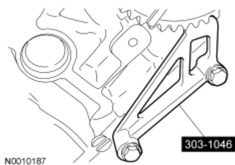
Fig. 333: Identifying Special Sprocket Phase Tool Courtesy of FORD MOTOR CO.
