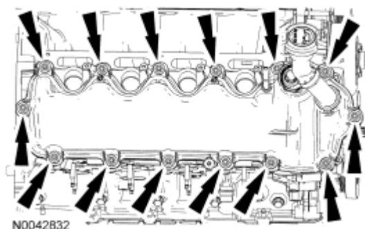
Fig. 306: Locating RH Valve Cover Bolts Courtesy of FORD MOTOR CO.
