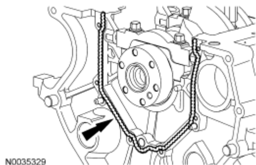
Fig. 445: Applying Bead Of Gasket Maker To Rear Crankshaft Seal Retainer Mating Surface On Engine Block Courtesy of FORD MOTOR CO.
