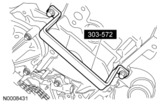
Fig. 262: Identifying Special Tool Onto Cylinder Head Courtesy of FORD MOTOR CO.
