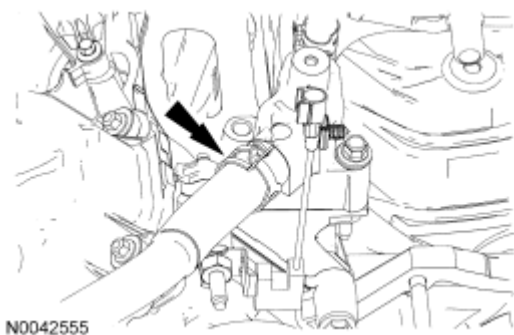
Fig. 479: Locating Heater Hose Clamp Courtesy of FORD MOTOR CO.
