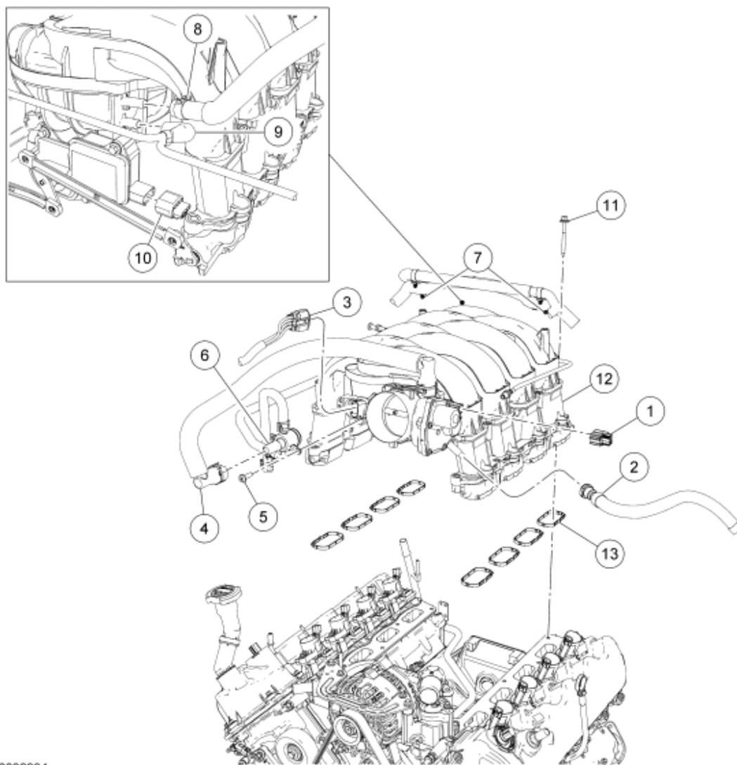
Fig. 1: Exploded View Of Intake Manifold
