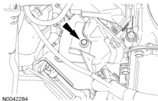
Fig. 461: Locating RH Engine Support Insulator Bracket Bolt Courtesy of FORD MOTOR CO.
