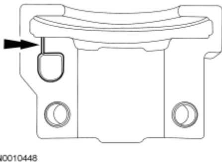
Fig. 57: Identifying Camshaft Front Thrust Bearing Cap Oil Metering Groove
