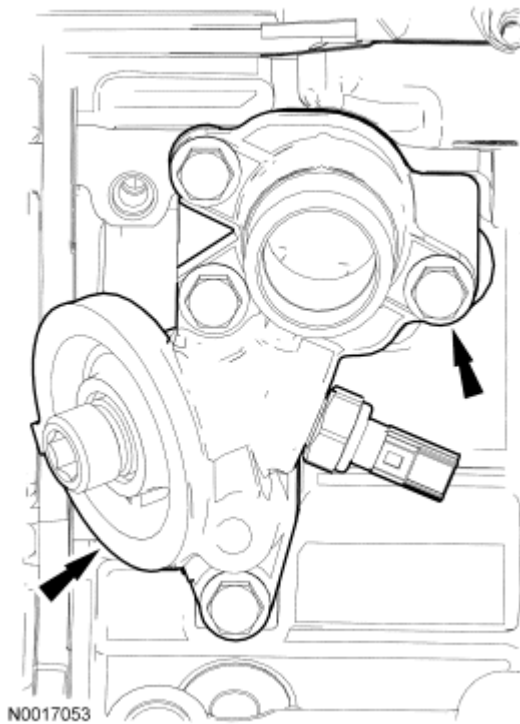
Fig. 422: Locating Oil Filter Adapter And Bolts Courtesy of FORD MOTOR CO.
