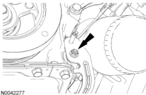
Fig. 166: Locating Battery Cable Bracket Nut Courtesy of FORD MOTOR CO.
