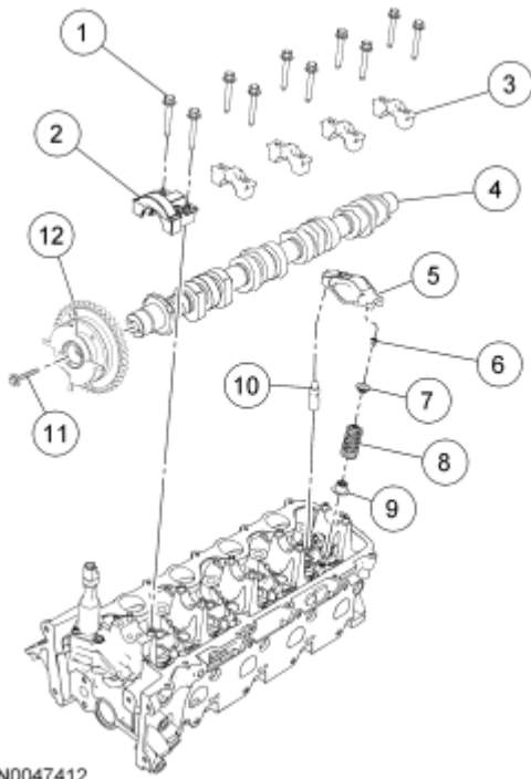
Fig. 80: Exploded View Of Valve Train Components Courtesy of FORD MOTOR CO.
