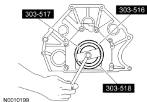
Fig. 453: Installing Crankshaft Rear Oil Slinger Using Special Tools Courtesy of FORD MOTOR CO.
