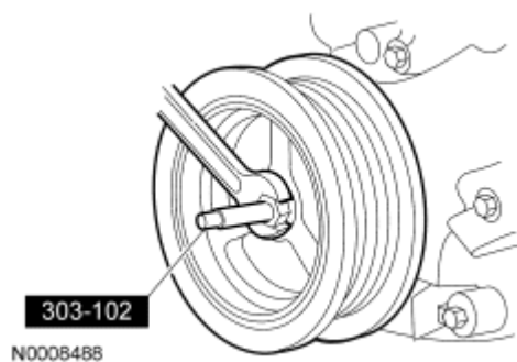
Fig. 404: Installing Crankshaft Pulley Using Special Tool Courtesy of FORD MOTOR CO.
