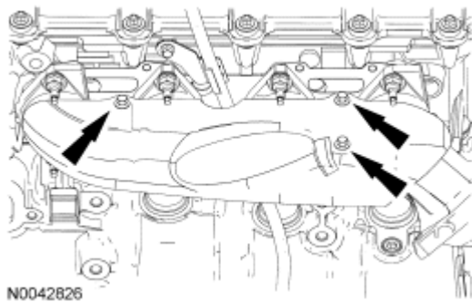
Fig. 263: Locating LH Exhaust Manifold Heat Shield Bolts Courtesy of FORD MOTOR CO.
