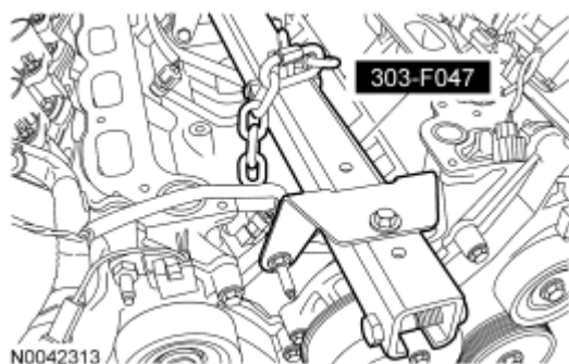
Fig. 216: Identifying Special Tool (303-F047) Courtesy of FORD MOTOR CO.
