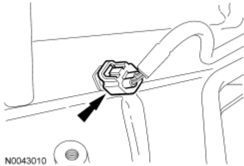
Fig. 430: Locating Cylinder Head Temperature (CHT) Sensor Electrical Connector Courtesy of FORD MOTOR CO.
