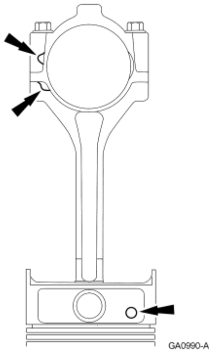
Fig. 354: Positioning Connecting Rod In Piston Courtesy of FORD MOTOR CO.
