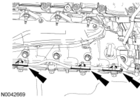
Fig. 165: Locating Oil Pan Wiring Harness Retainers Courtesy of FORD MOTOR CO.
