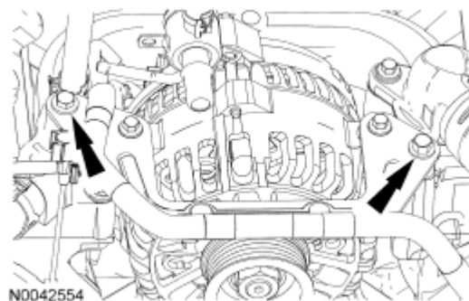
Fig. 191: Locating Alternator Bracket And Wiring Harness Bolts Courtesy of FORD MOTOR CO.
