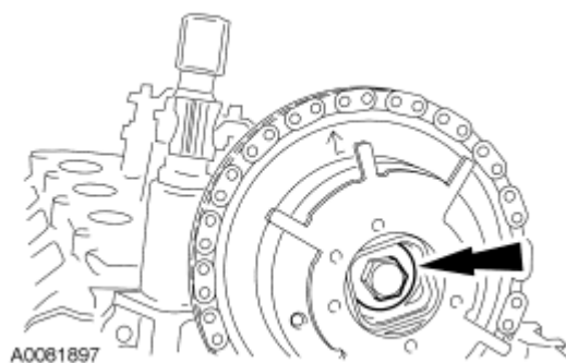
Fig. 102: Identifying Camshaft Phase And Sprocket Assembly Bolt Courtesy of FORD MOTOR CO.
