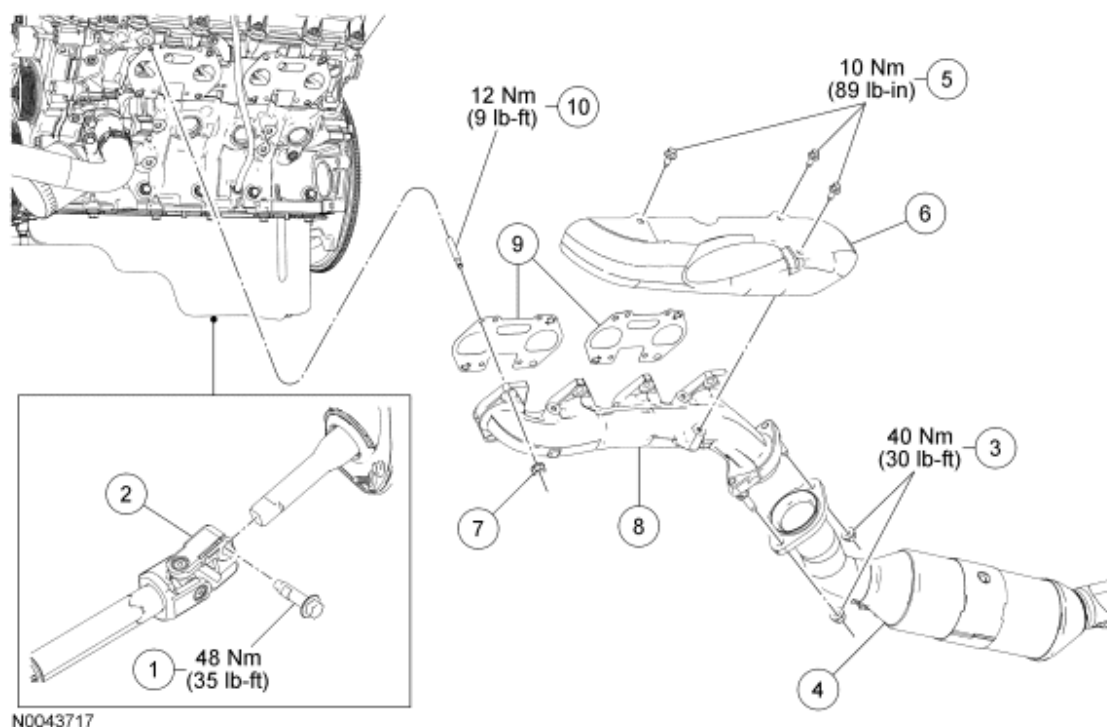
Fig. 140: Exploded View Of Exhaust Manifold With Torque Specifications - LH Courtesy of FORD MOTOR CO.
