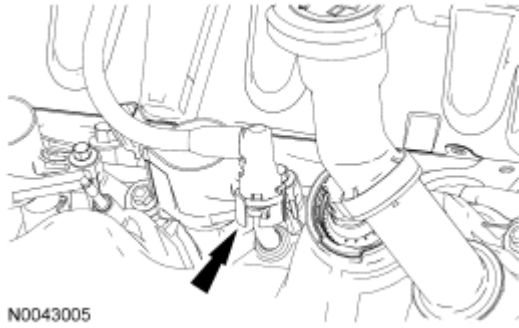
Fig. 426: Locating Breather Tube Connector Retaining Clip Courtesy of FORD MOTOR CO.
