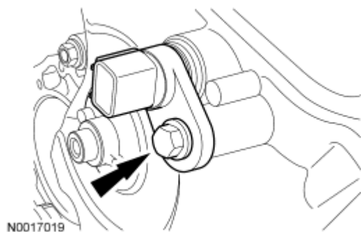
Fig. 309: Locating LH Camshaft Position (CMP) Sensor And Bolt Courtesy of FORD MOTOR CO.
