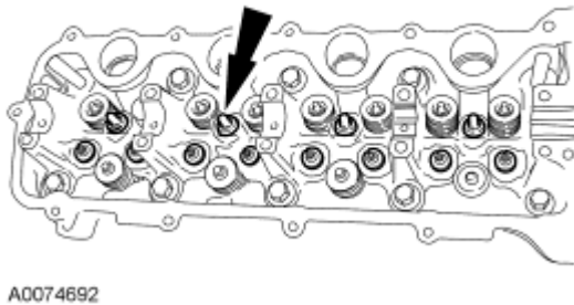
Fig. 492: Identifying Hydraulic Lash Adjusters Courtesy of FORD MOTOR CO.
