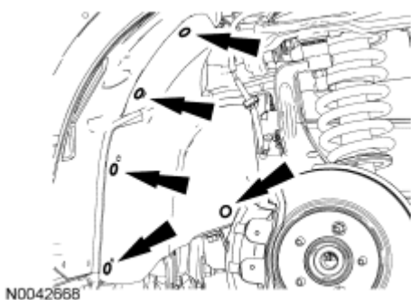
Fig. 180: Locating Pushpins And Splash Shield Courtesy of FORD MOTOR CO.
