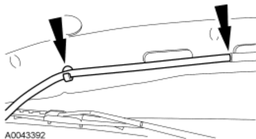
Fig. 183: Locating Windshield Washer Hose And Retainer Courtesy of FORD MOTOR CO.
