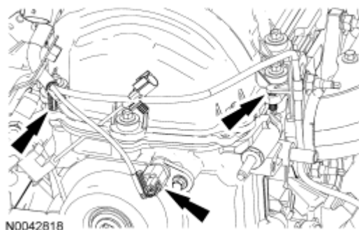
Fig. 436: Locating LH Camshaft Position Sensor And Attach Wiring Harness Retainers Courtesy of FORD MOTOR CO.
