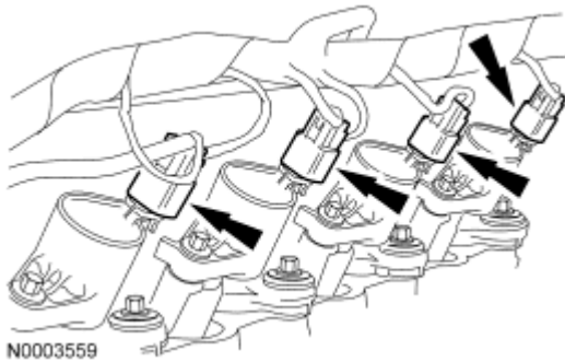
Fig. 543: Locating Ignition Coil Electrical Connectors Courtesy of FORD MOTOR CO.
