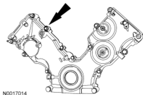
Fig. 242: Locating Engine Front Cover Fasteners Courtesy of FORD MOTOR CO.
