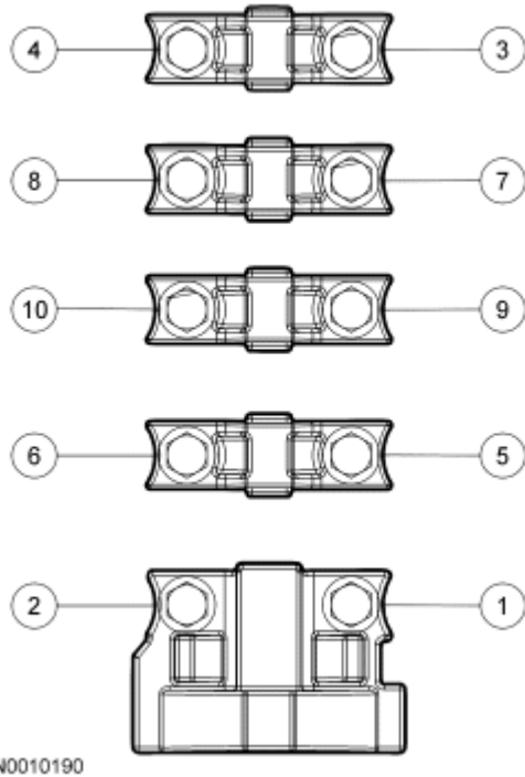
Fig. 336: Identifying Camshaft Bearing Caps Loosening/Tightening Sequence Courtesy of FORD MOTOR CO.
