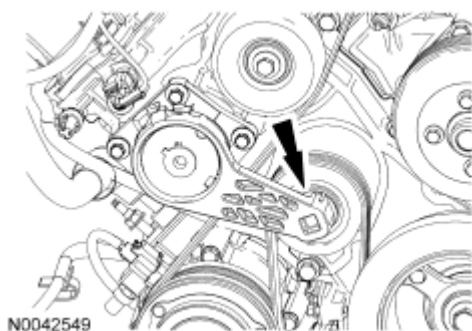
Fig. 485: Locating Accessory Drive Belt Tensioner Courtesy of FORD MOTOR CO.
