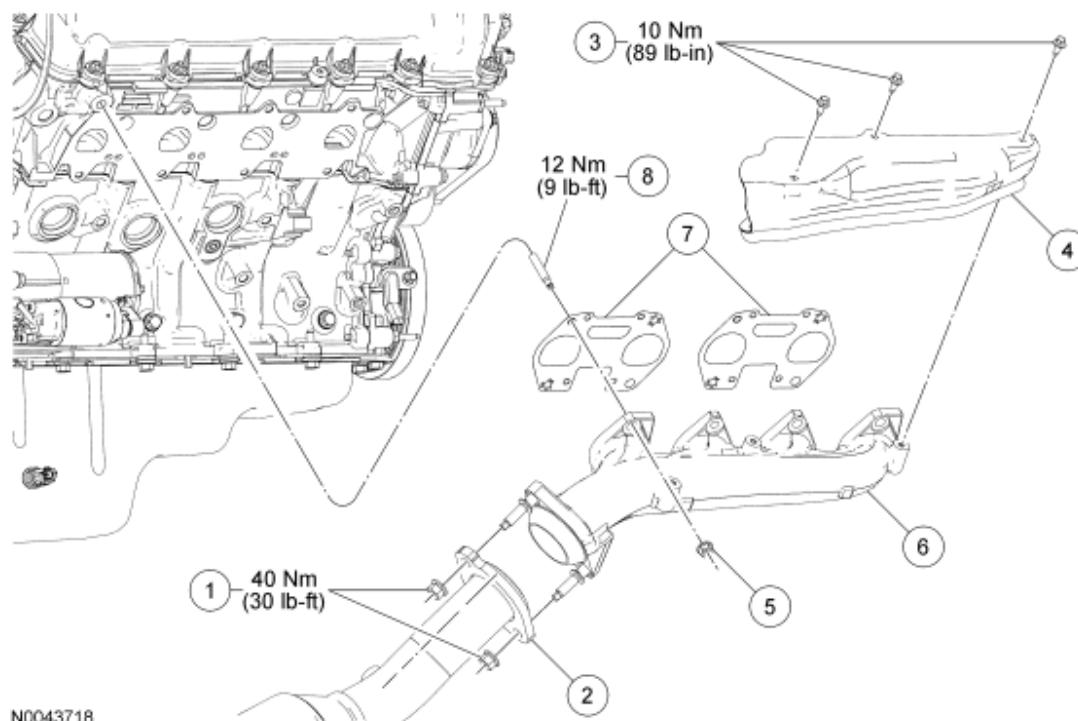
Fig. 150: Exploded View Of Exhaust Manifold With Torque Specifications - RH Courtesy of FORD MOTOR CO.
