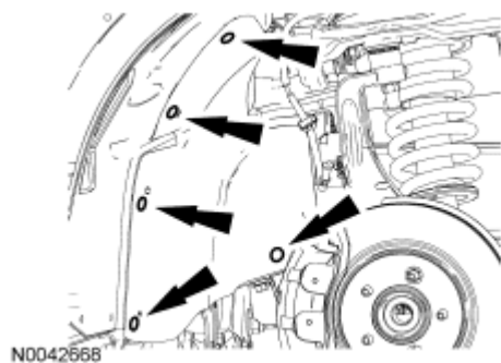
Fig. 153: Locating Pushpins And Splash Shield Courtesy of FORD MOTOR CO.
