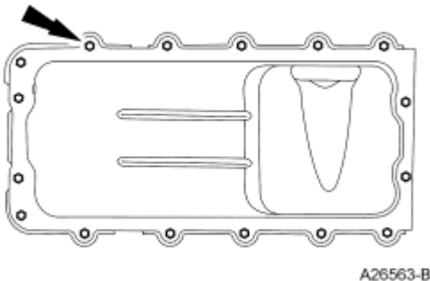
Fig. 317: Locating Oil Pan And Oil Pan Gasket Bolts Courtesy of FORD MOTOR CO.
