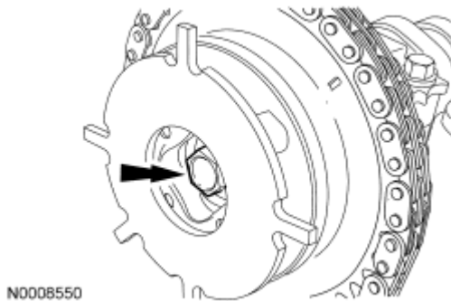
Fig. 124: Identifying Camshaft Phase And Sprocket Assembly Bolt Courtesy of FORD MOTOR CO.
