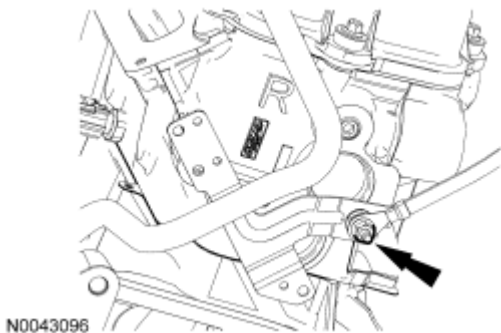
Fig. 268: Locating Ground Strap Nut Courtesy of FORD MOTOR CO.
