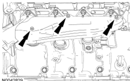
Fig. 499: Identifying RH Exhaust Manifold Heat Shield Bolts
