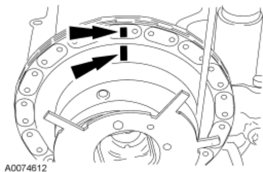
Fig. 128: Identifying Scribe Marks Of Camshaft Phase And Chain Courtesy of FORD MOTOR CO.
