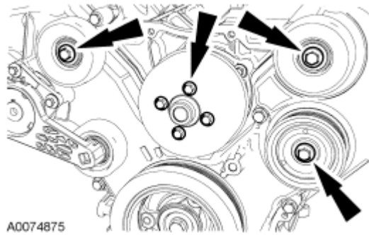
Fig. 311: Locating Coolant Pump Pulley And Accessory Drive Belt Idler Pulley Bolts Courtesy of FORD MOTOR CO.
