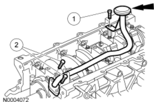
Fig. 370: Locating Oil Pump Screen And Pickup Tube Courtesy of FORD MOTOR CO.
