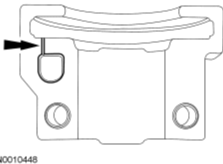
Fig. 337: Identifying Camshaft Front Thrust Bearing Cap Oil Metering Groove Courtesy of FORD MOTOR CO.
