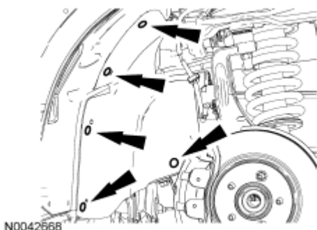
Fig. 211: Locating Pushpins And Splash Shield Courtesy of FORD MOTOR CO.
