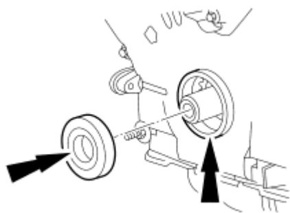
Fig. 527: Locating Crankshaft Front Seal Courtesy of FORD MOTOR CO.
