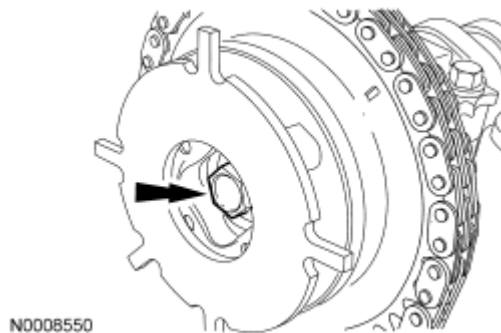
Fig. 115: Identifying Camshaft Phase And Sprocket Assembly Bolt Courtesy of FORD MOTOR CO.
