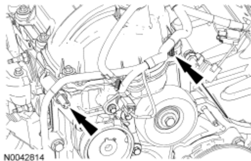
Fig. 221: Locating Wiring Harness Retainers
