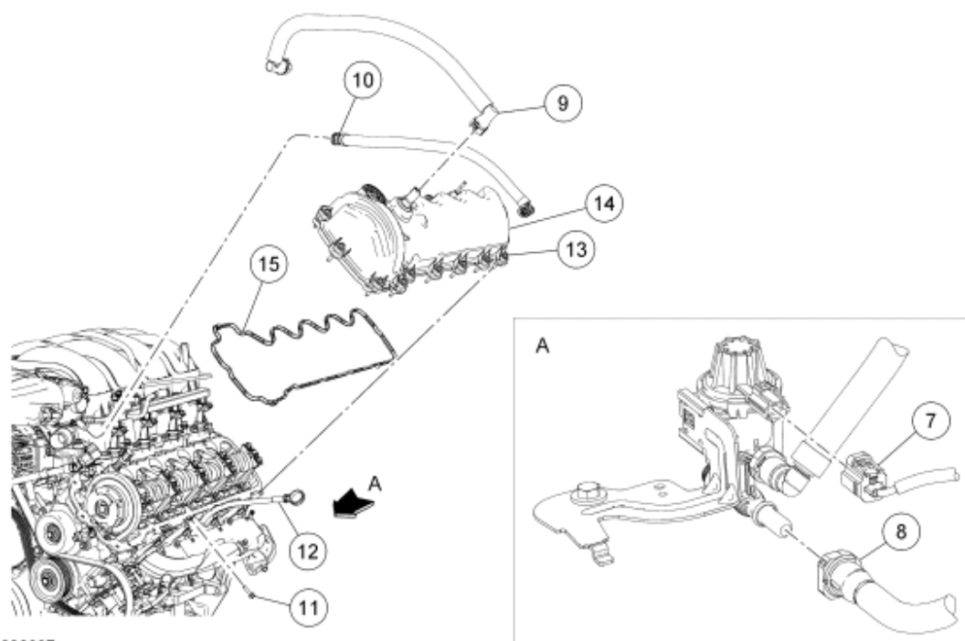
Fig. 4: Exploded View Of Valve Cover - LH (2 Of 2) Courtesy of FORD MOTOR CO.
