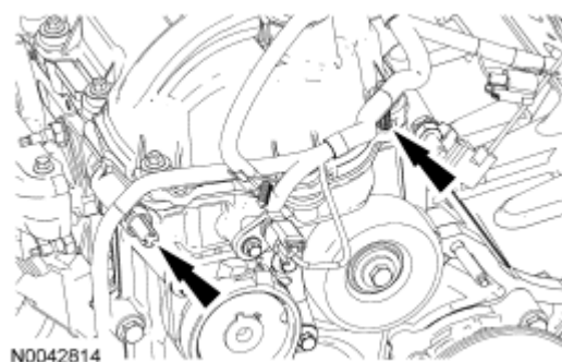
Fig. 282: Locating Wiring Harness Retainers Courtesy of FORD MOTOR CO.
