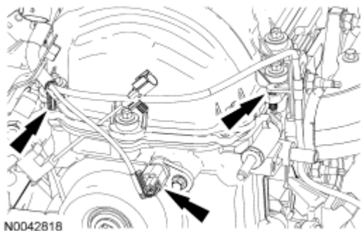
Fig. 224: Locating LH Camshaft Position Sensor And Attach Wiring Harness Retainers Courtesy of FORD MOTOR CO.
