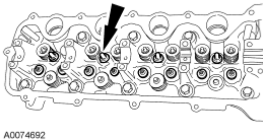
Fig. 376: Identifying Hydraulic Lash Adjusters Courtesy of FORD MOTOR CO.
