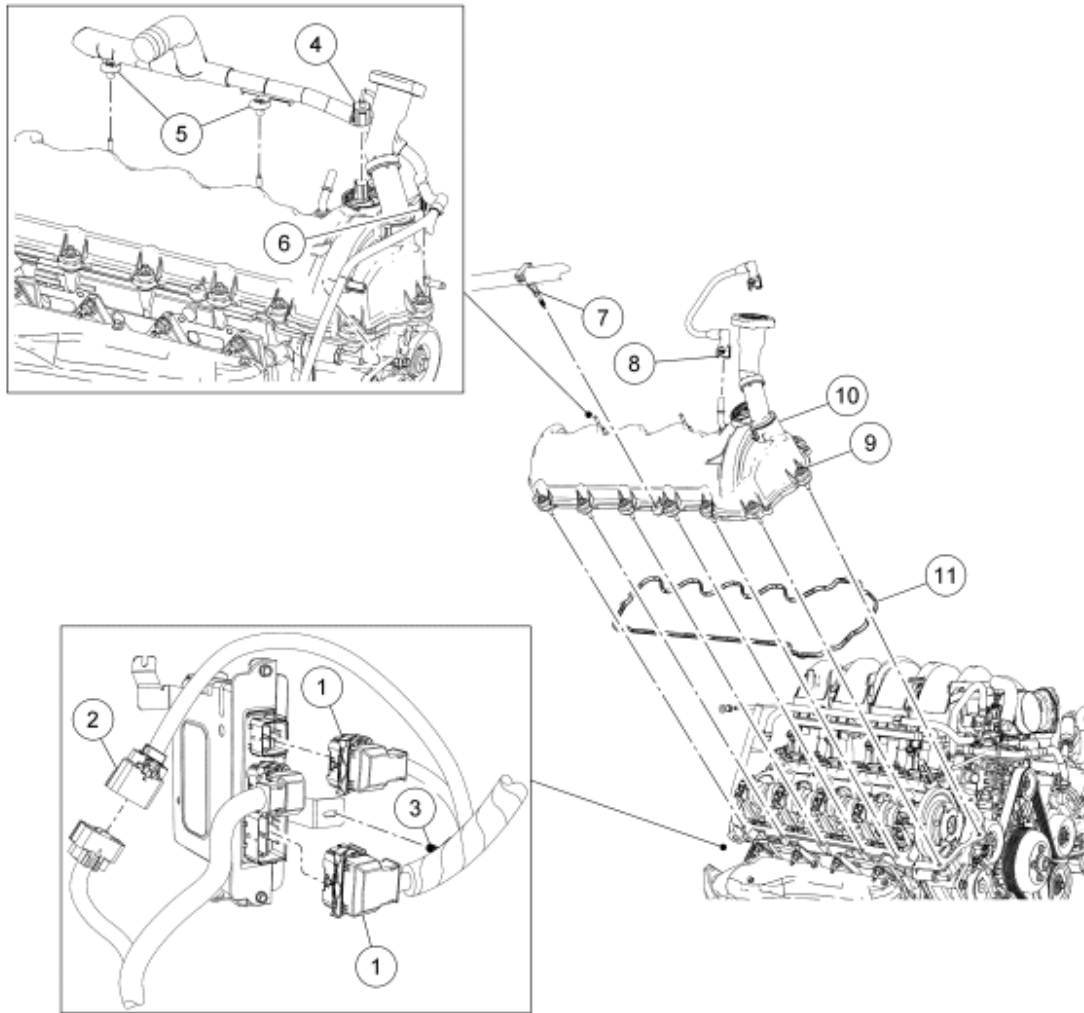
Fig. 7: Exploded View Of Valve Cover - RH Courtesy of FORD MOTOR CO.
