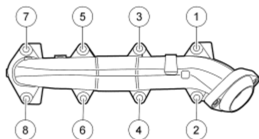
Fig. 493: Identifying Tightening Sequence Of Exhaust Manifold Nuts Courtesy of FORD MOTOR CO.
