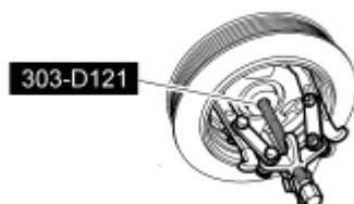
Fig. 239: Removing Crankshaft Pulley Using Special Tool (303-D121) Courtesy of FORD MOTOR CO.
