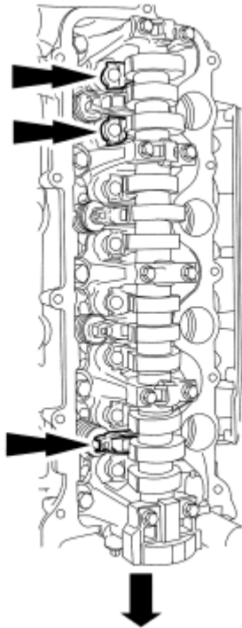
Fig. 45: Identifying RH Cylinder Head Camshaft Roller Followers And Bolts
