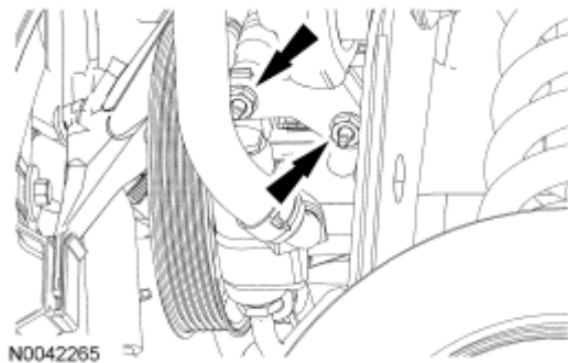
Fig. 142: Locating Wiring Harness Bracket Nuts Courtesy of FORD MOTOR CO.
