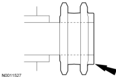
Fig. 380: Identifying Crankshaft Sprocket Courtesy of FORD MOTOR CO.
