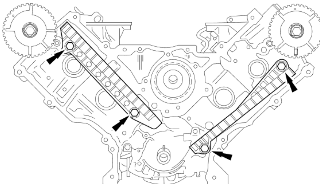
Fig. 511: Identifying Timing Chain Guides Courtesy of FORD MOTOR CO.
