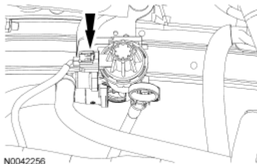
Fig. 476: Locating Evaporative Emission (EVAP) Canister Purge Valve Electrical Connector Courtesy of FORD MOTOR CO.
