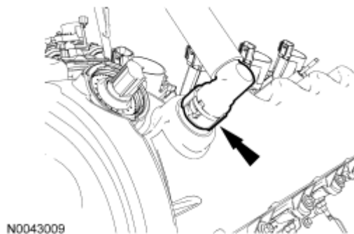
Fig. 538: Locating Positive Crankcase Ventilation (PCV) Hose Courtesy of FORD MOTOR CO.
