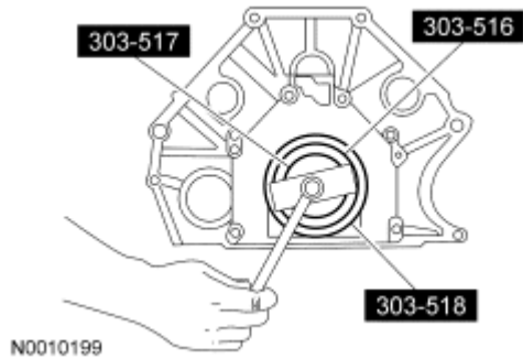
Fig. 28: Installing Crankshaft Rear Oil Slinger Using Special Tools Courtesy of FORD MOTOR CO.
