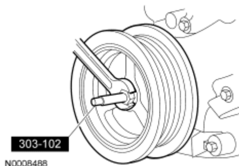
Fig. 13: Installing Crankshaft Pulley Using Special Tool
