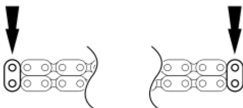
Fig. 510: Identifying Timing Chain Copper Links Courtesy of FORD MOTOR CO.
