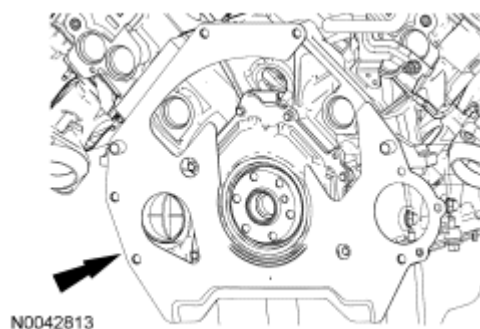
Fig. 454: Locating Spacer Plate Courtesy of FORD MOTOR CO.
