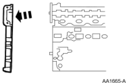
Fig. 319: Removing Engine Front Cover From Cylinder Block Courtesy of FORD MOTOR CO.
