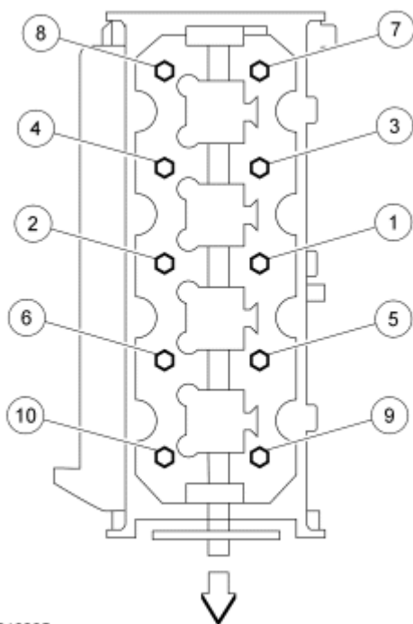
Fig. 490: Identifying Cylinder Head Bolt Tightening Sequence Courtesy of FORD MOTOR CO.
