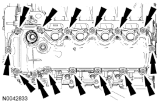
Fig. 236: Locating LH Valve Cover Bolts Courtesy of FORD MOTOR CO.
