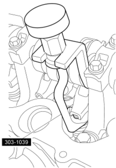
Fig. 79: Compressing Spring Using Special Tool Courtesy of FORD MOTOR CO.
