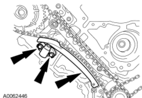
Fig. 329: Identifying RH Timing Chain Tensioner, Tensioner Arm And Bolts Courtesy of FORD MOTOR CO.
