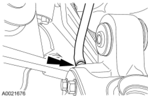
Fig. 182: Disconnecting Vent Hose From Differential Housing Vent Tube Courtesy of FORD MOTOR CO.
