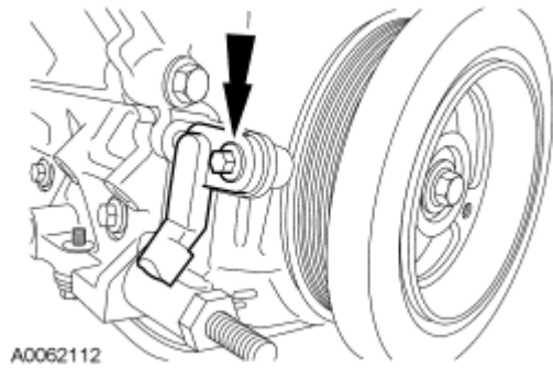
Fig. 310: Locating Crankshaft Position (CKP) Sensor Bolt Courtesy of FORD MOTOR CO.
