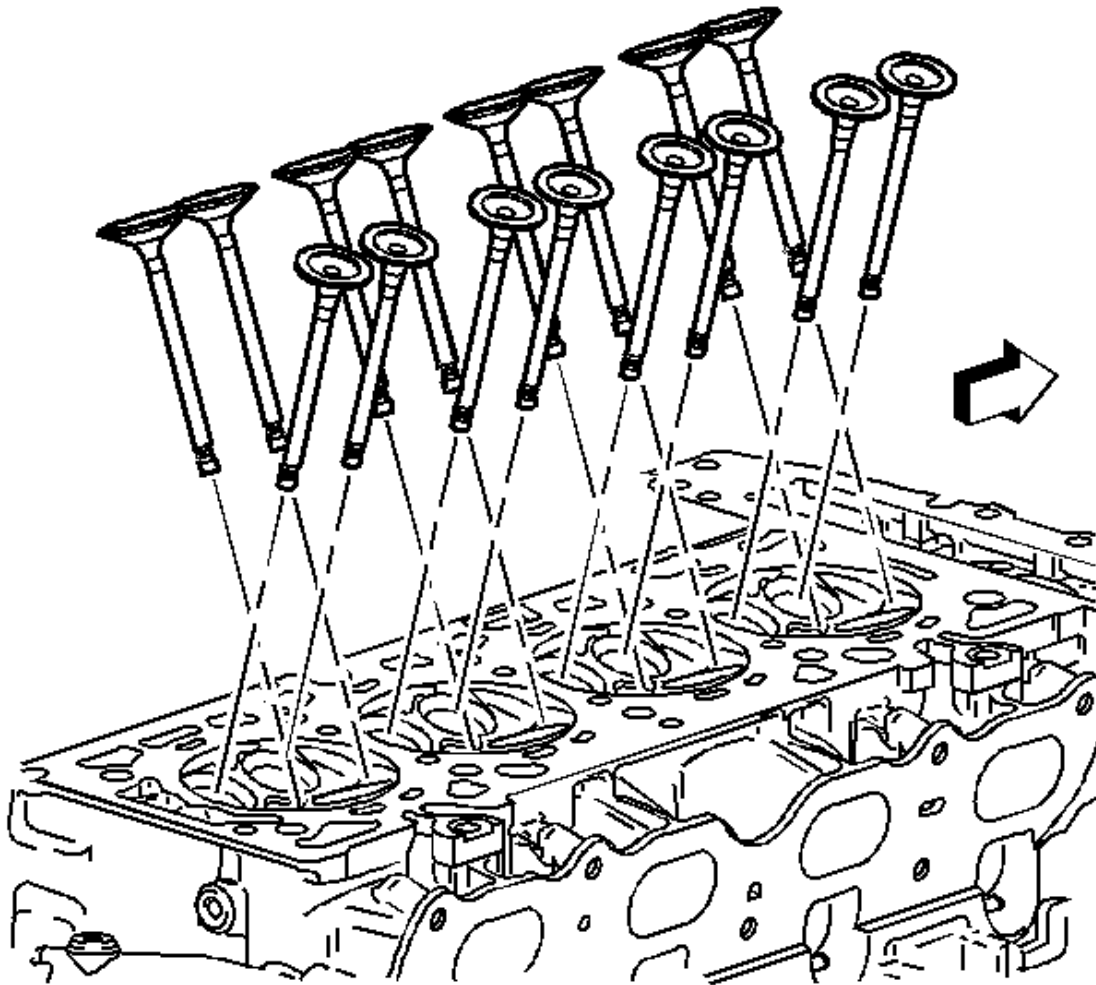
Fig. 359: Identifying Engine Valves Courtesy of GENERAL MOTORS CORP.
