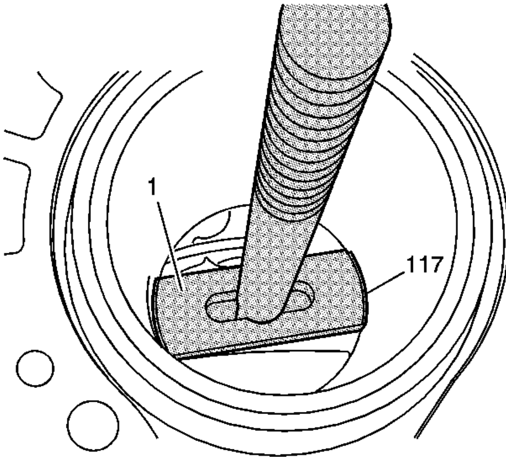
Fig. 293: View Of Cylinder Bore Liner Puller Courtesy of GENERAL MOTORS CORP.
