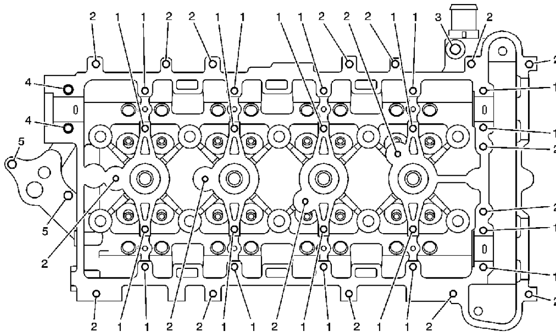
Fig. 12: Identifying Bolt Size & Locations On Cylinder Head - Top Courtesy of GENERAL MOTORS CORP.
