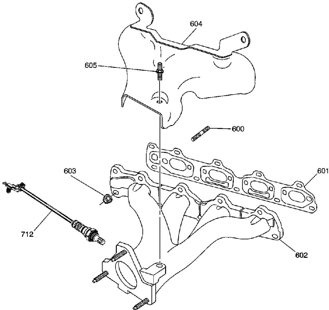
Fig. 20: Exhaust Manifold & Components
