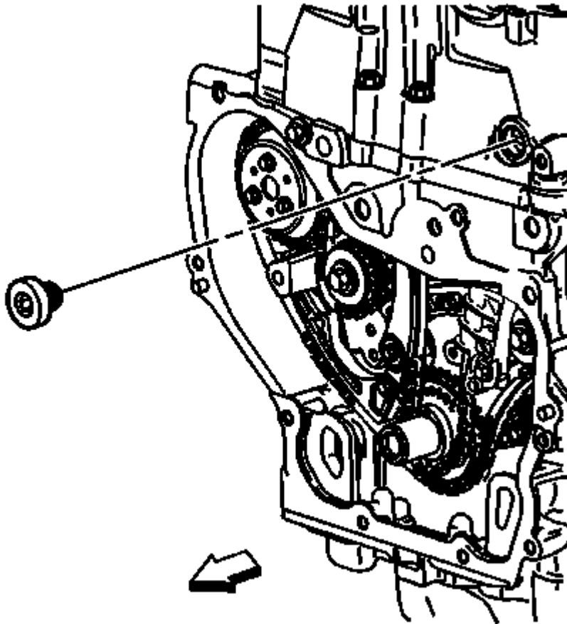
Fig. 246: View Of Fixed Timing Chain Guide Access Plug Courtesy of GENERAL MOTORS CORP.
