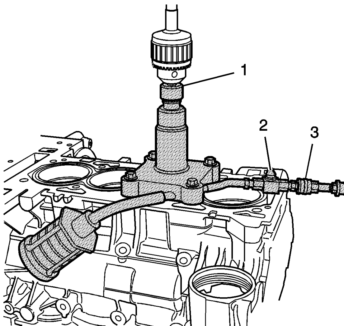
Fig. 312: View Of Drive Adapter Courtesy of GENERAL MOTORS CORP.
