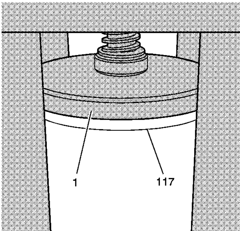
Fig. 300: View Of Installation Arbor Courtesy of GENERAL MOTORS CORP.
