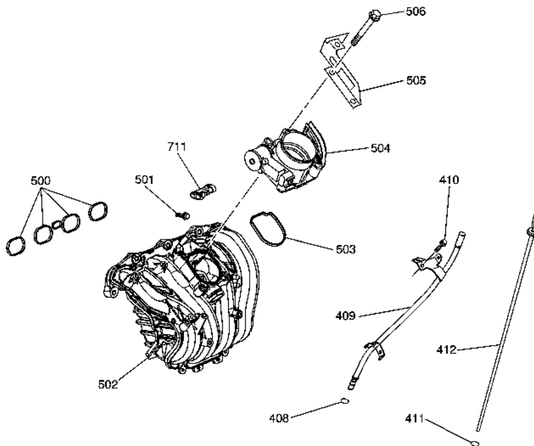
Fig. 19: Intake Manifold & Components Courtesy of GENERAL MOTORS CORP.
