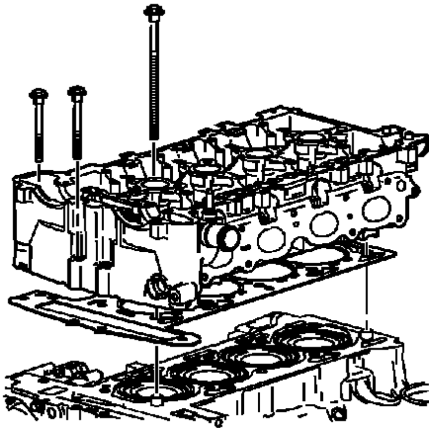
Fig. 421: View Of Cylinder Head And Gasket Courtesy of GENERAL MOTORS CORP.
