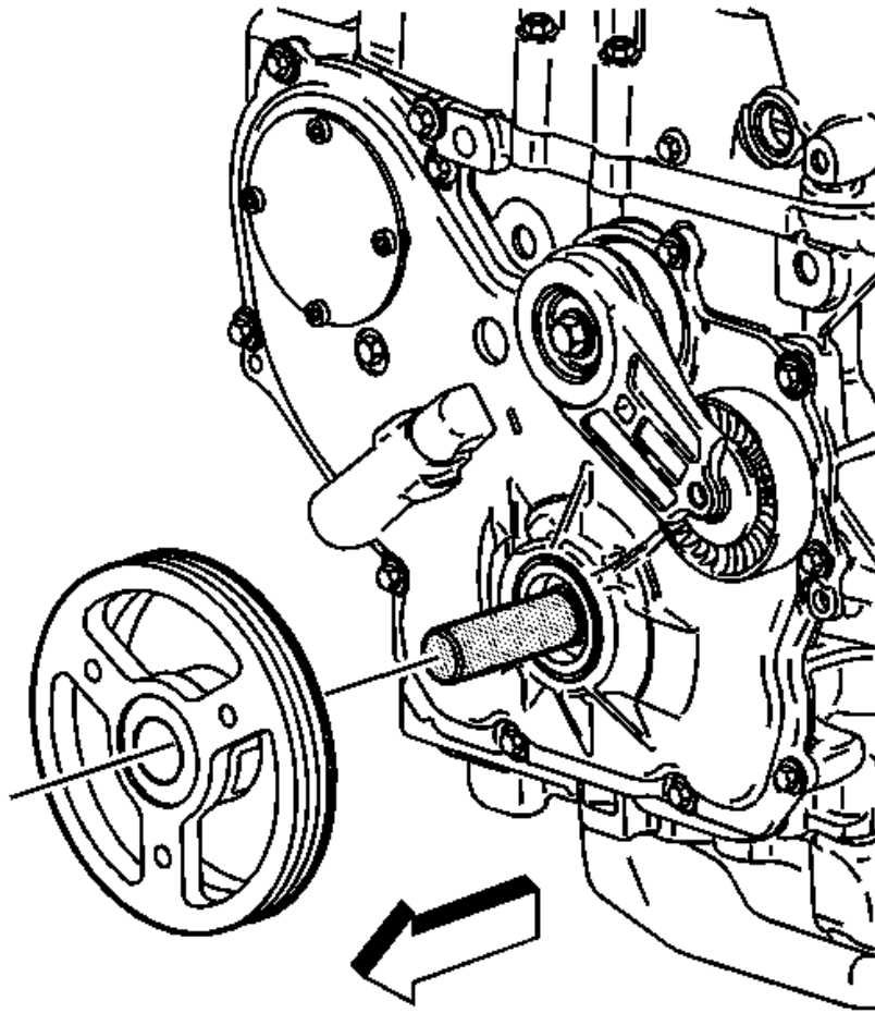
Fig. 234: View Of Crankshaft Balancer Courtesy of GENERAL MOTORS CORP.
