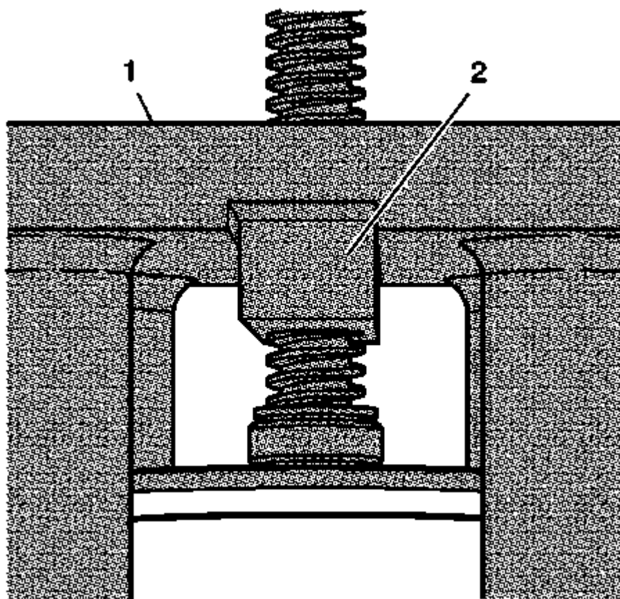
Fig. 301: View Of Pusher Block Courtesy of GENERAL MOTORS CORP.
