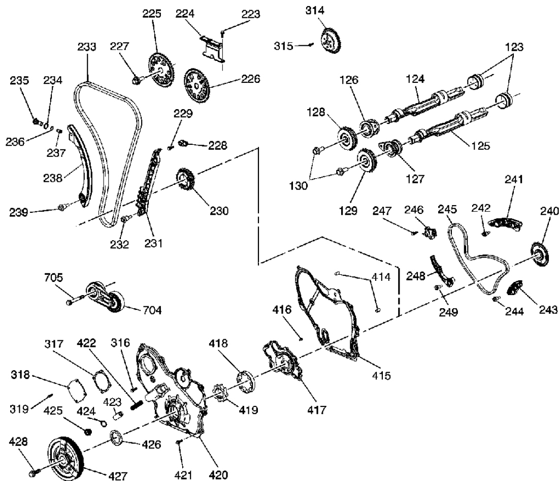
Fig. 22: Timing Chain & Components Courtesy of GENERAL MOTORS CORP.
