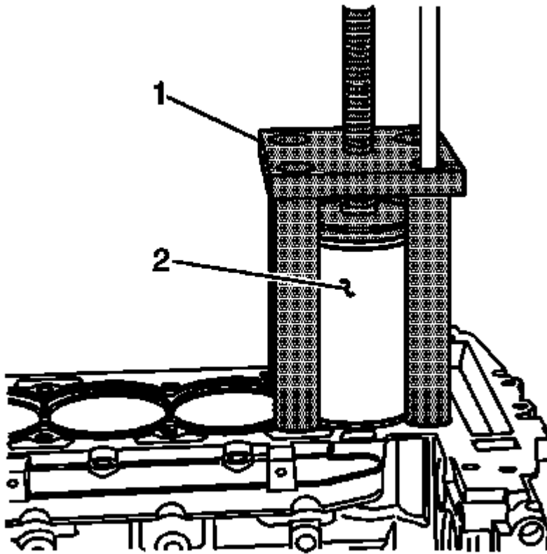
Fig. 158: View Of Cylinder Bore Sleeve Installer Courtesy of GENERAL MOTORS CORP.
