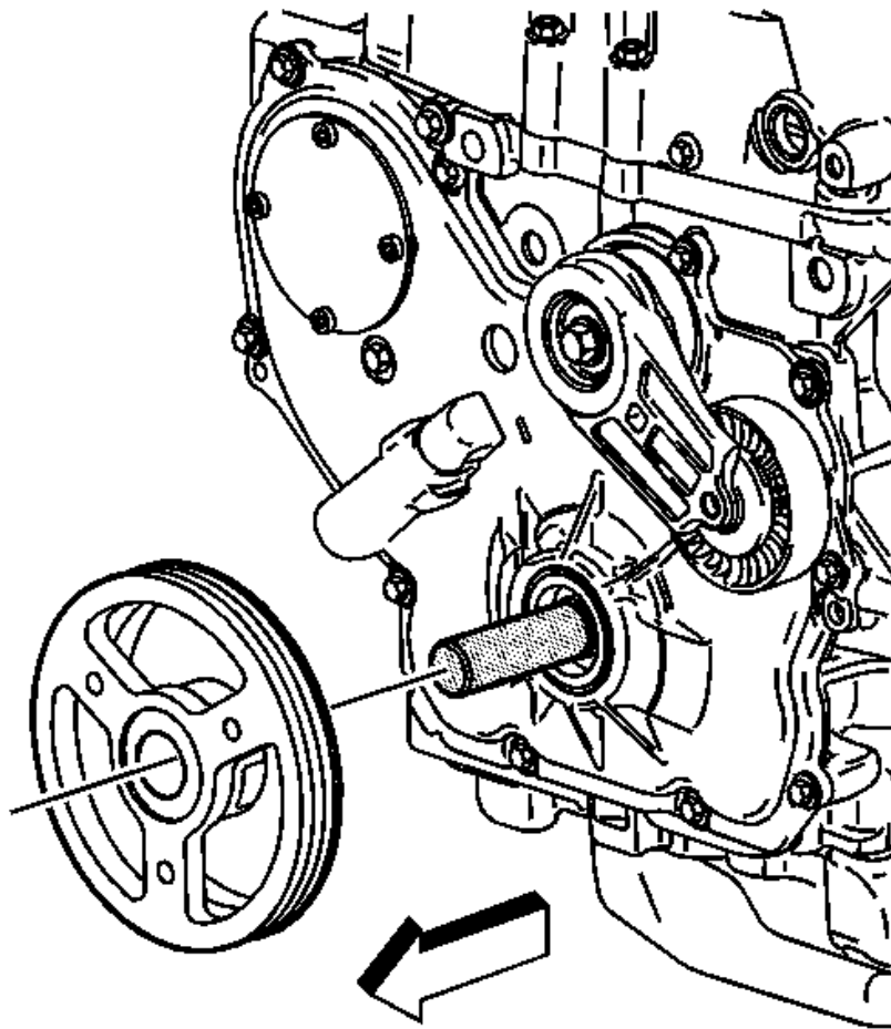
Fig. 483: View Of Crankshaft Balancer Courtesy of GENERAL MOTORS CORP.
