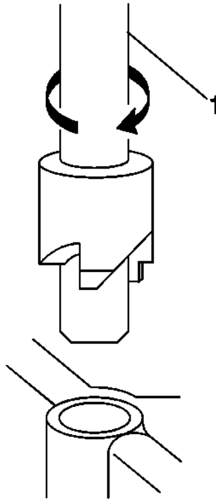
Fig. 376: View Of Counterbore Drill Courtesy of GENERAL MOTORS CORP.
