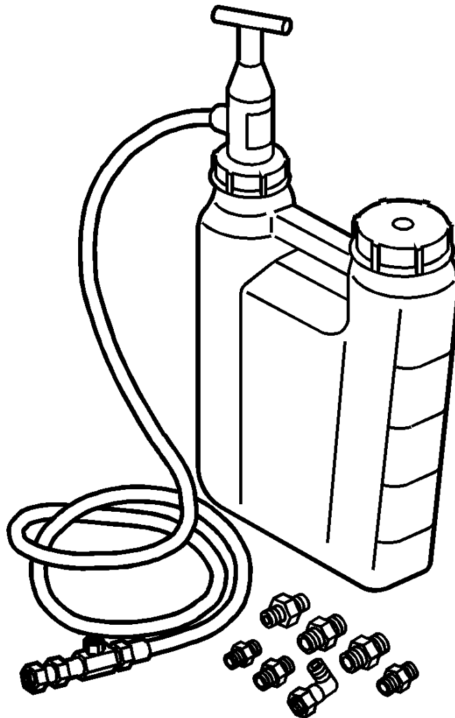
Fig. 494: Identifying Engine Preluber J 45299 Courtesy of GENERAL MOTORS CORP.
