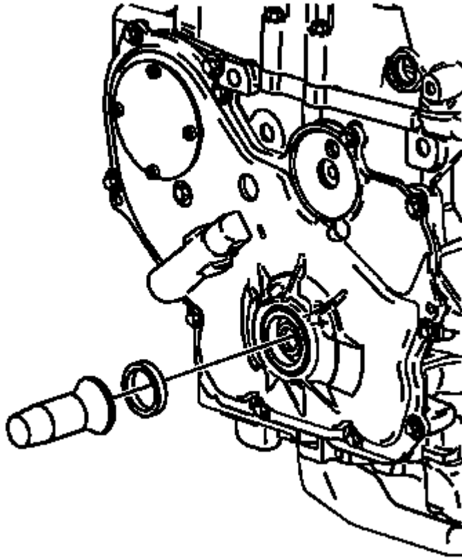
Fig. 57: Installing Crankshaft Front Oil Seal Courtesy of GENERAL MOTORS CORP.
