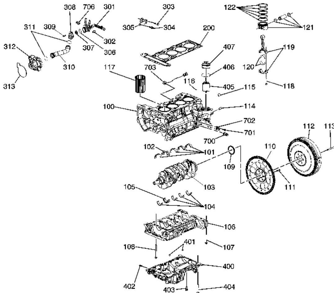
Fig. 21: Engine Block & Components Courtesy of GENERAL MOTORS CORP.
