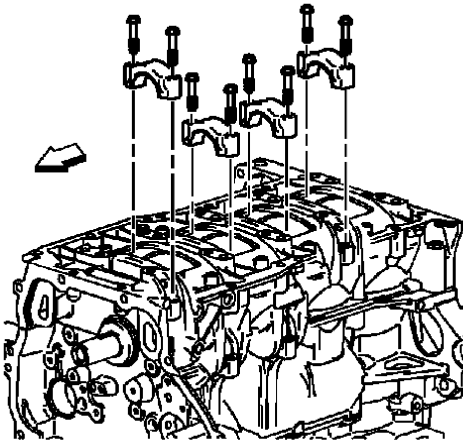
Fig. 274: View Of Connecting Rod Nuts And Caps Courtesy of GENERAL MOTORS CORP.
