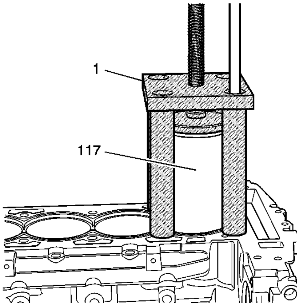
Fig. 298: Installing Cylinder Bore Sleeve Puller Attachment Bolts Courtesy of GENERAL MOTORS CORP.
