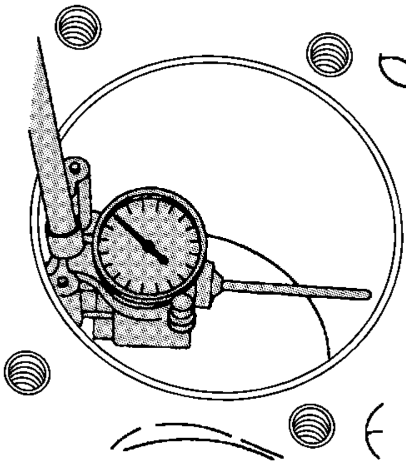
Fig. 335: Measuring Cylinder Bore Courtesy of GENERAL MOTORS CORP.
