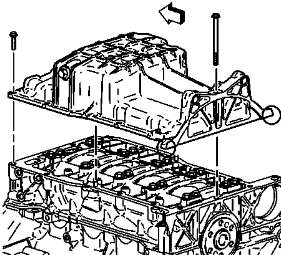
Fig. 273: View Of Oil Pan
