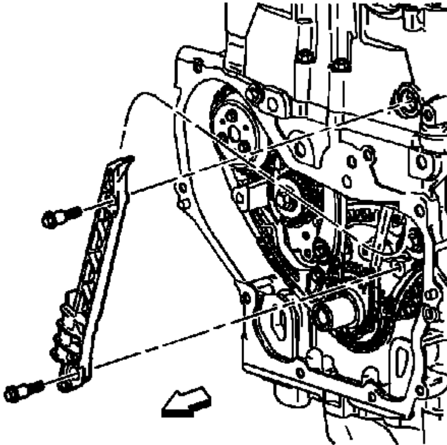
Fig. 456: View Of Fixed Timing Chain Guide Courtesy of GENERAL MOTORS CORP.
