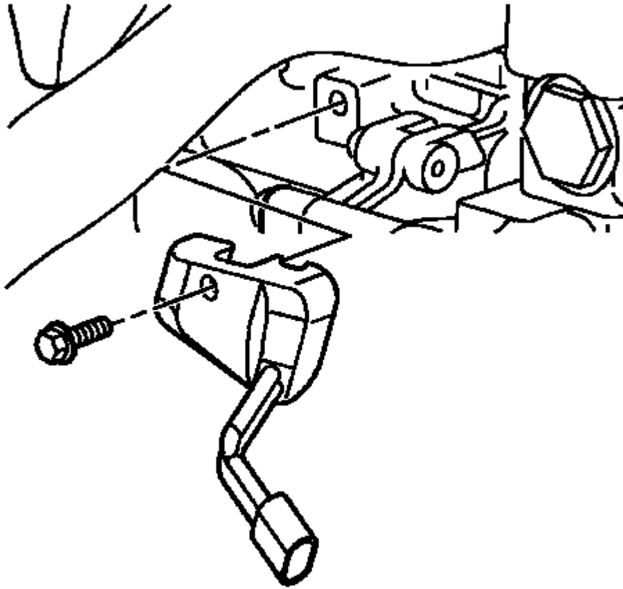
Fig. 489: View Of Block Heater Courtesy of GENERAL MOTORS CORP.
