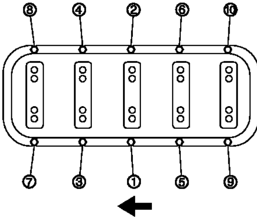
Fig. 416: Lower Crankcase Perimeter Bolt Tightening Sequence Courtesy of GENERAL MOTORS CORP.
