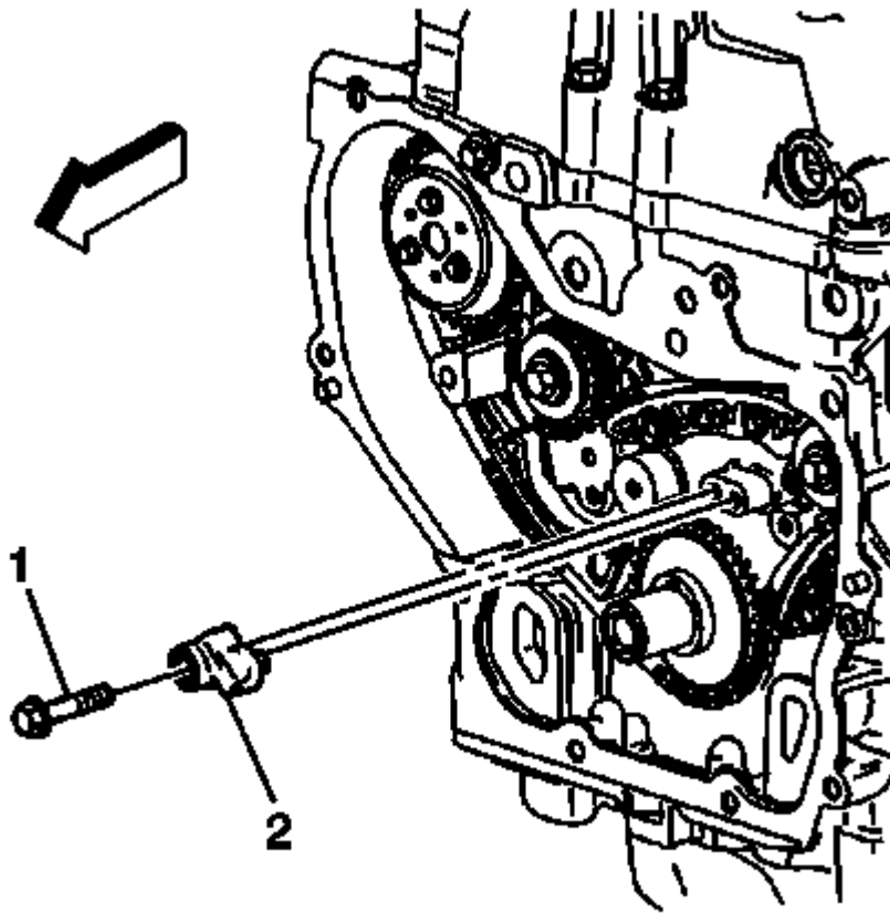
Fig. 463: View Of Oil Nozzle & Bolt Courtesy of GENERAL MOTORS CORP.
