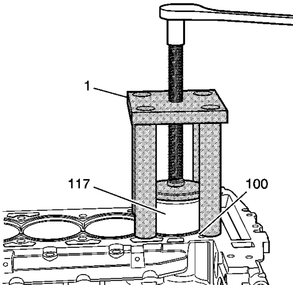
Fig. 302: Installing Cylinder Bore Sleeve Into Engine Block Using Tool Courtesy of GENERAL MOTORS CORP.
