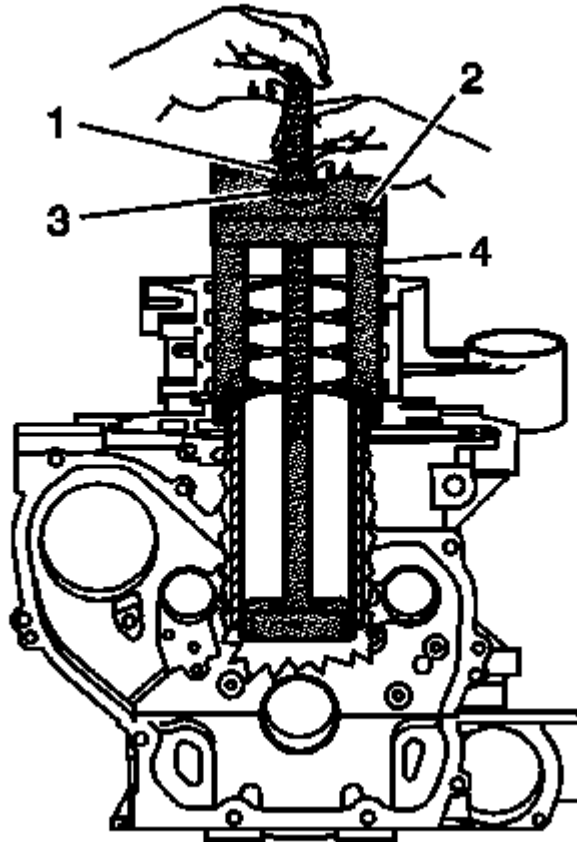
Fig. 294: Aligning Cylinder Bore Sleeve Puller Courtesy of GENERAL MOTORS CORP.
