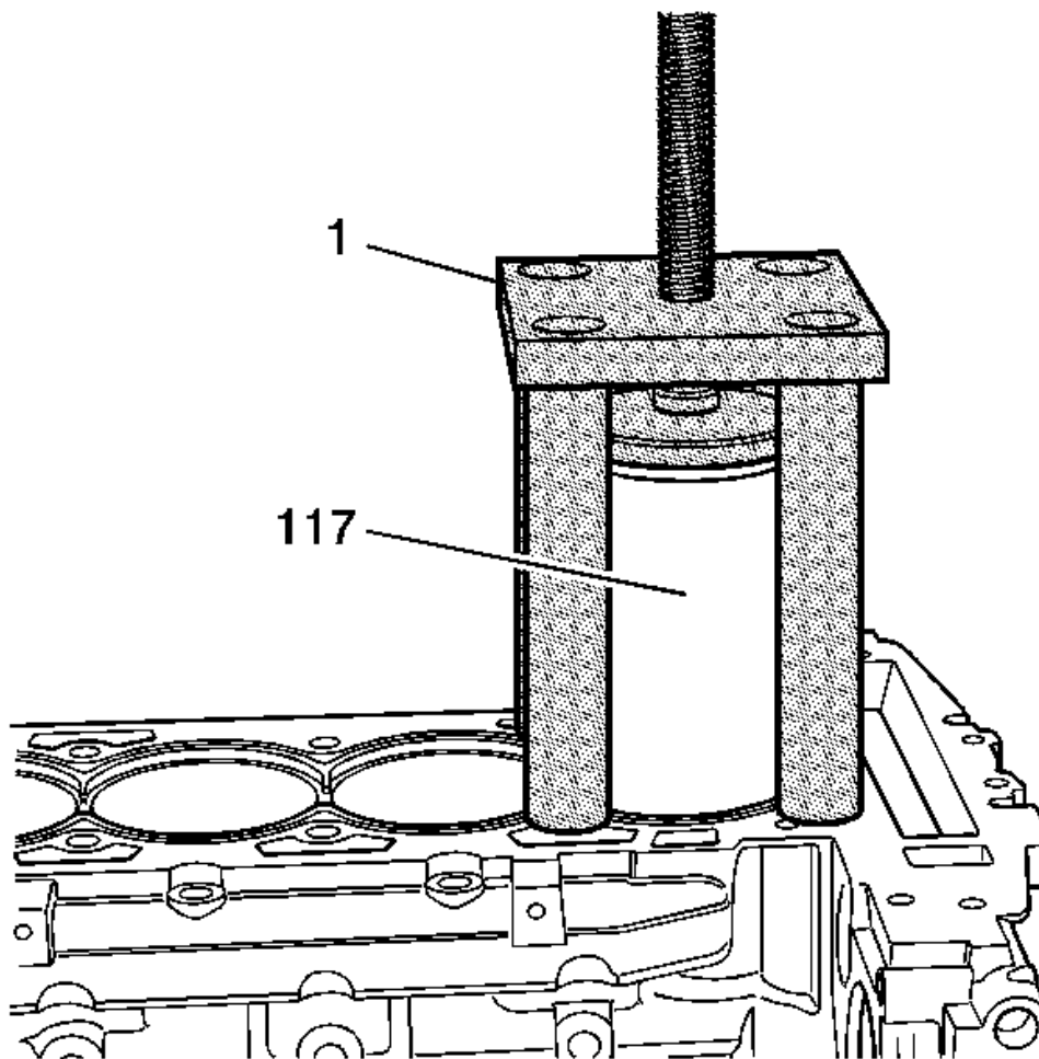
Fig. 297: View Of Cylinder Bore Sleeve Fixture Courtesy of GENERAL MOTORS CORP.
