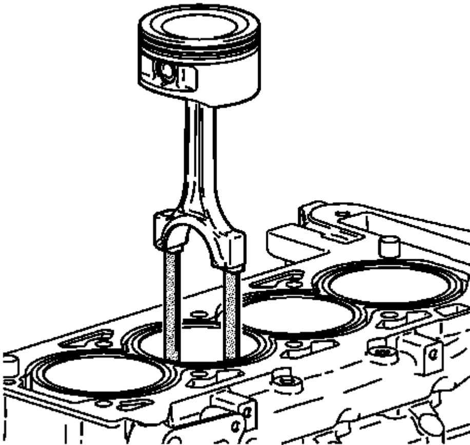
Fig. 275: J-43966-1 Installed Into Connecting Rod Bolt Holes Courtesy of GENERAL MOTORS CORP.
