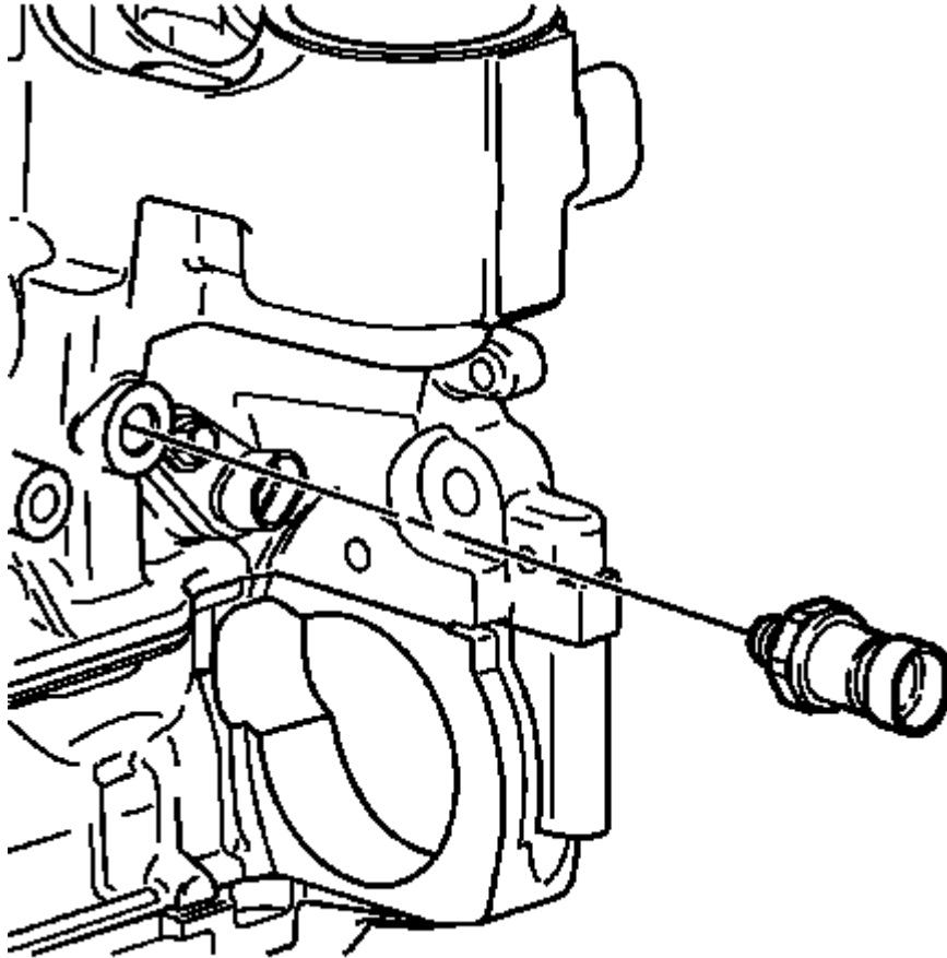
Fig. 493: View Of Engine Oil Pressure Sensor Courtesy of GENERAL MOTORS CORP.
