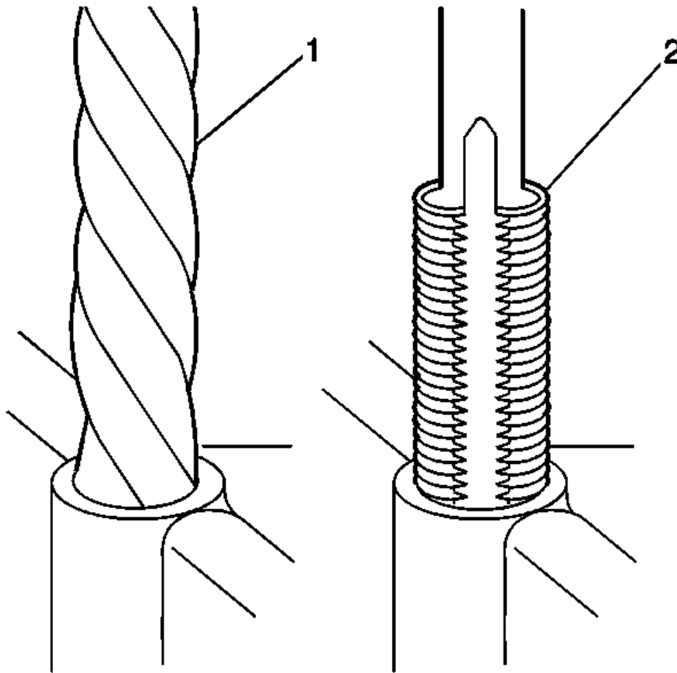
Fig. 375: Drilling & Tapping Threads Courtesy of GENERAL MOTORS CORP.
