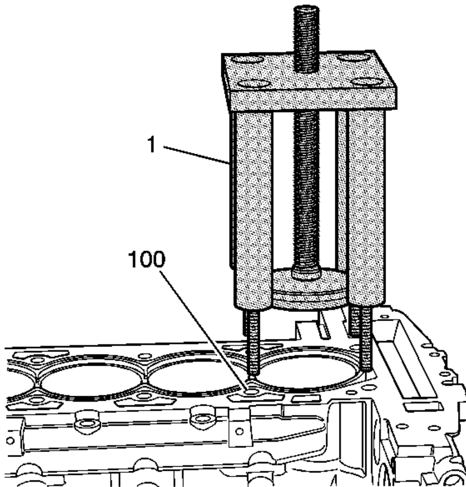
Fig. 304: View Of Service Tool Assembly Courtesy of GENERAL MOTORS CORP.
