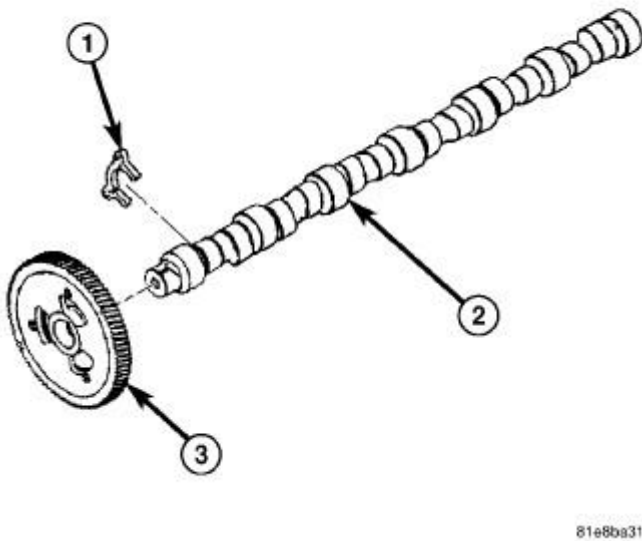
Fig. 131: Camshaft, Gear & Thrust Plate Courtesy of CHRYSLER GROUP, LLC
