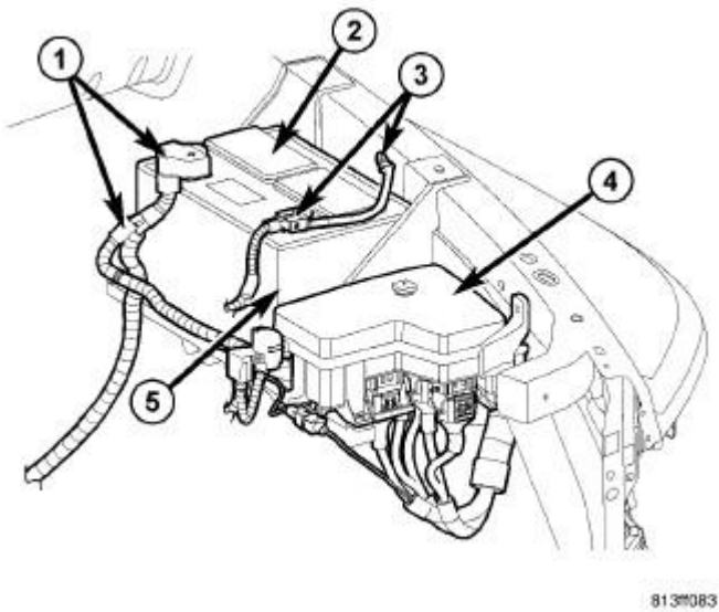
Fig. 173: Battery Cables
