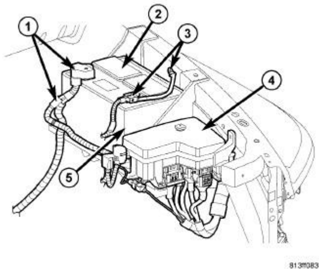
Fig. 181: Battery Cables Courtesy of CHRYSLER GROUP, LLC
