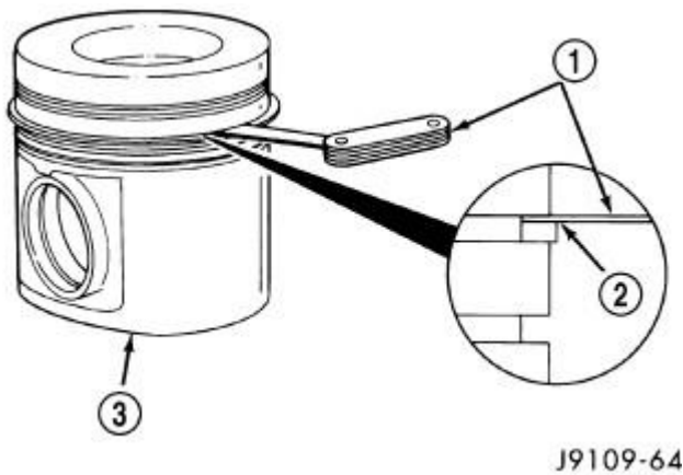
Fig. 163: Intermediate And Oil Ring To Piston Groove Clearances Courtesy of CHRYSLER GROUP, LLC
