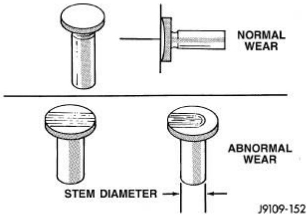
Fig. 188: Tappet Inspection
