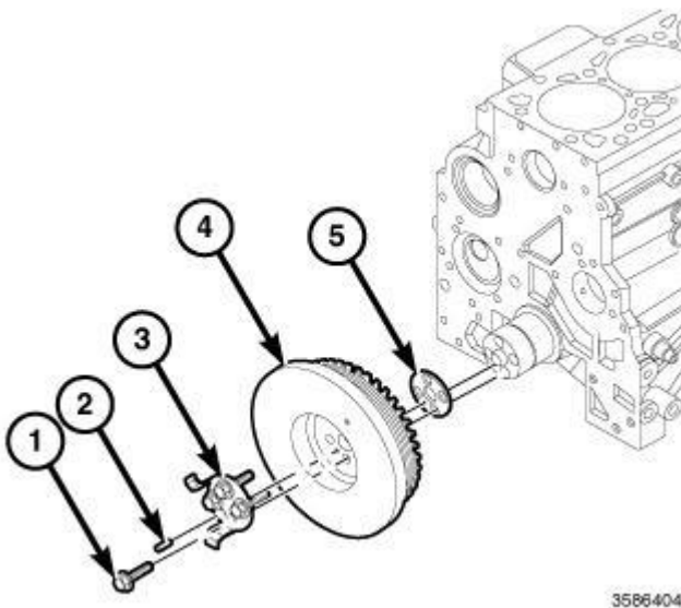
Fig. 145: Crankshaft Damper (High Output Engine) Courtesy of CHRYSLER GROUP, LLC
