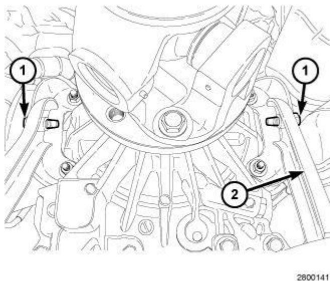
Fig. 217: Transmission Side Support Bracket & Bolts - AS68RC A/T Courtesy of CHRYSLER GROUP, LLC
