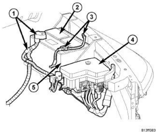
Fig. 226: Battery Cables
