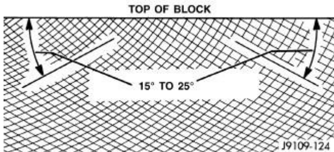
Fig. 113: Crosshatch Pattern Of Repaired Sleeve(s)
