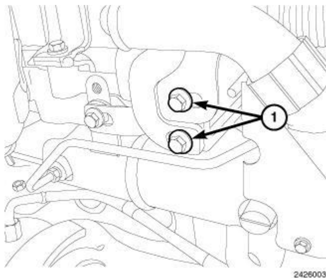
Fig. 235: Identifying Bracket Bolts Courtesy of CHRYSLER LLC
