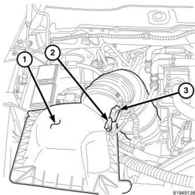
Fig. 262: Housing - Air Cleaner Courtesy of CHRYSLER LLC
