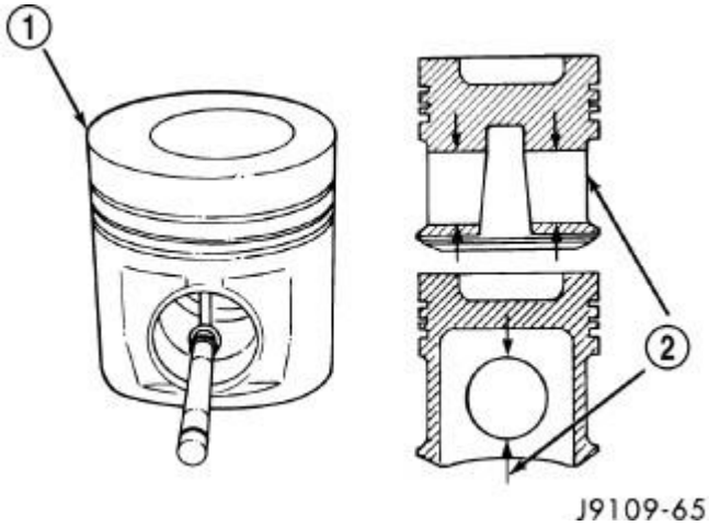
Fig. 164: Piston Pin Bore Courtesy of CHRYSLER LLC
