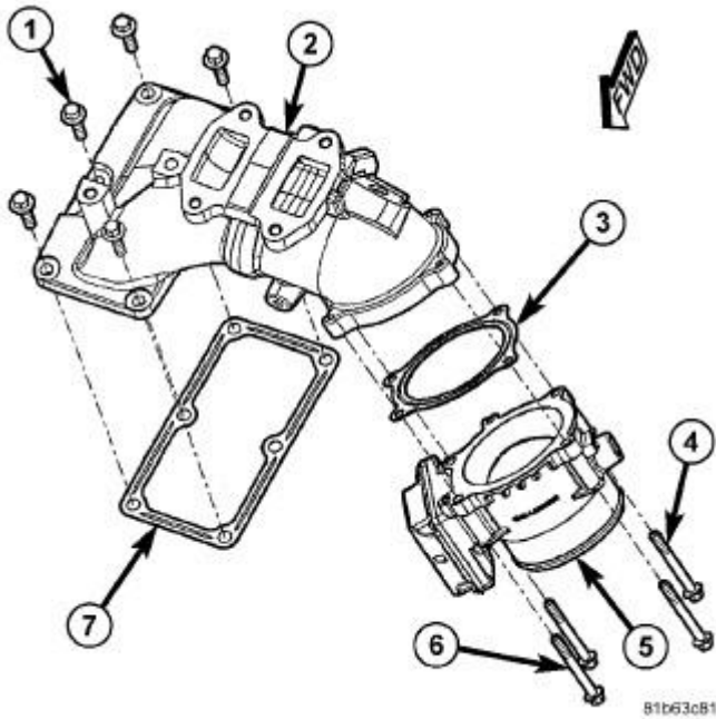
Fig. 295: EGR Air Flow Control Valve Location Courtesy of CHRYSLER LLC
