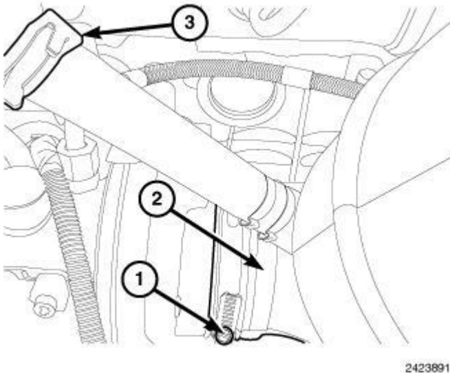
Fig. 41: Identifying Clamp, Outlet Tube & Breather Hose Courtesy of CHRYSLER LLC
