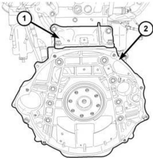
Fig. 24: Flywheel Housing And Collar Courtesy of CHRYSLER LLC
