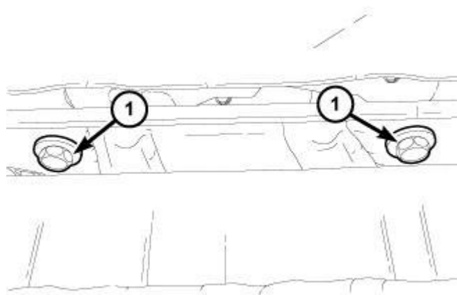
Fig. 216: Identifying Transmission Mount Support Bracket Bolts - AS68RC A/T Courtesy of CHRYSLER LLC
