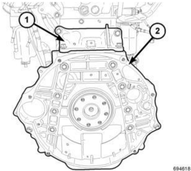
Fig. 13: Flywheel Housing And Collar Courtesy of CHRYSLER LLC
