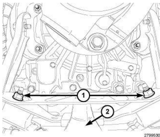
Fig. 208: Identifying Rear Transmission Mount & Nuts - AS68RC A/T Courtesy of CHRYSLER LLC
