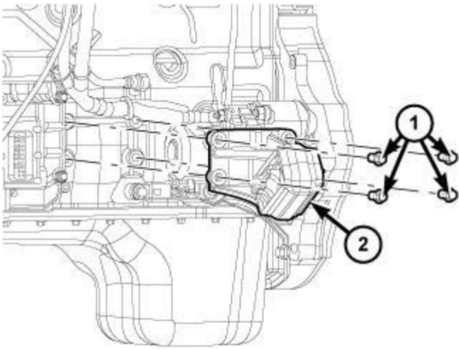
Fig. 204: LH Engine Mount Courtesy of CHRYSLER LLC
