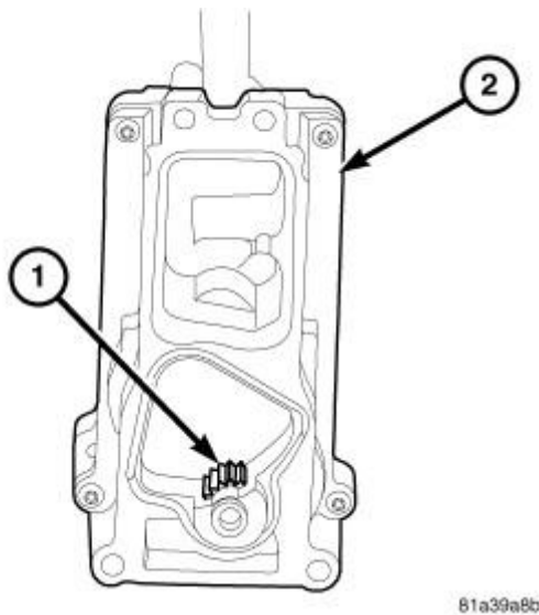
Fig. 311: Identifying Turbocharger Actuator Alignment Courtesy of CHRYSLER LLC
