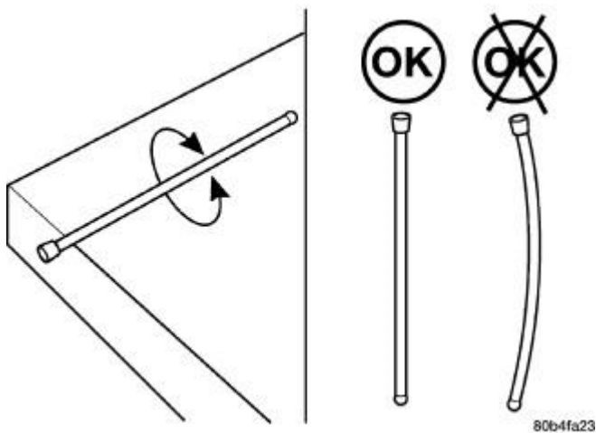
Fig. 85: Inspecting Push Rod For Flatness Courtesy of CHRYSLER LLC
