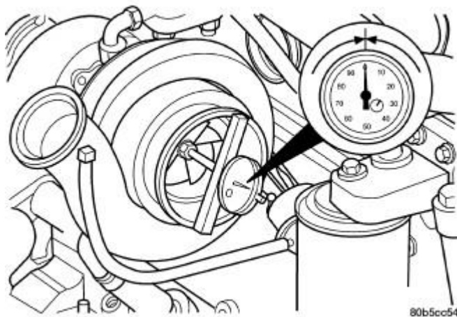
Fig. 331: Measure Turbocharger Axial End Play Courtesy of CHRYSLER LLC
