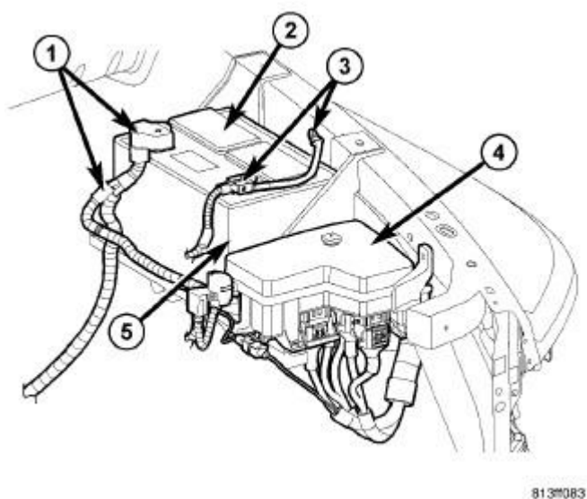
Fig. 256: Locating Battery System Components (Typical) Courtesy of CHRYSLER LLC
