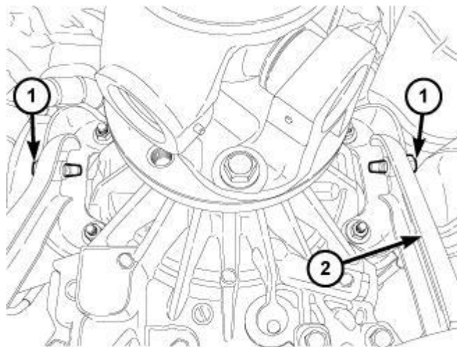
Fig. 217: Identifying Transmission Support Bracket & Bolts - AS68RC A/T Courtesy of CHRYSLER LLC
