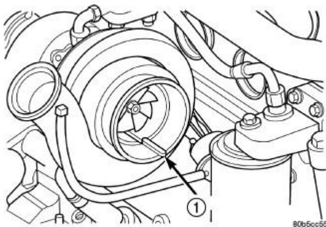
Fig. 332: Measure Turbocharger Bearing Radial Clearance Courtesy of CHRYSLER LLC
