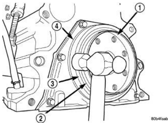
Fig. 150: Installing Seal Using Alignment Tool And Hammer Courtesy of CHRYSLER LLC
