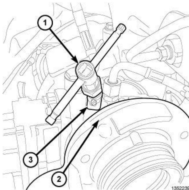
Fig. 303: Removing/Installing Tap
