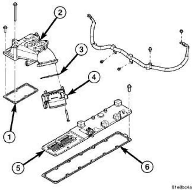
Fig. 294: Intake Air Heater Assembly Courtesy of CHRYSLER LLC
