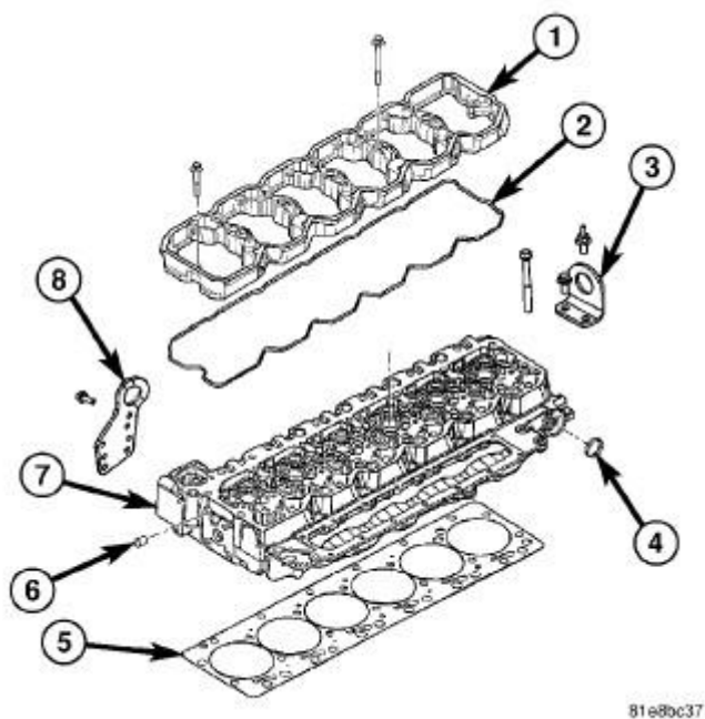
Fig. 62: Cylinder Head And Gasket Courtesy of CHRYSLER LLC
