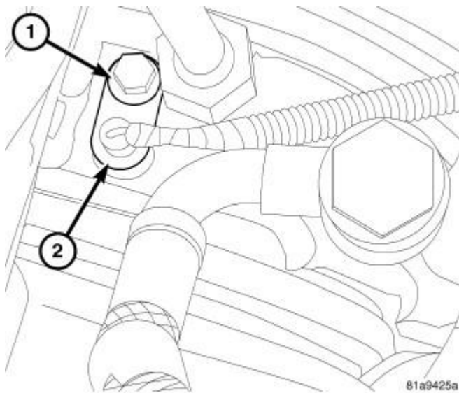
Fig. 320: Identifying Turbocharger Speed Sensor Courtesy of CHRYSLER LLC
