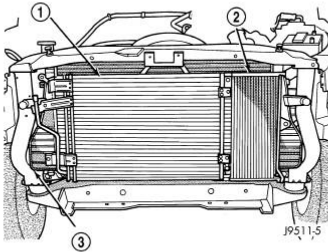
Fig. 362: Condenser And Transmission Auxiliary Cooler Courtesy of CHRYSLER LLC
