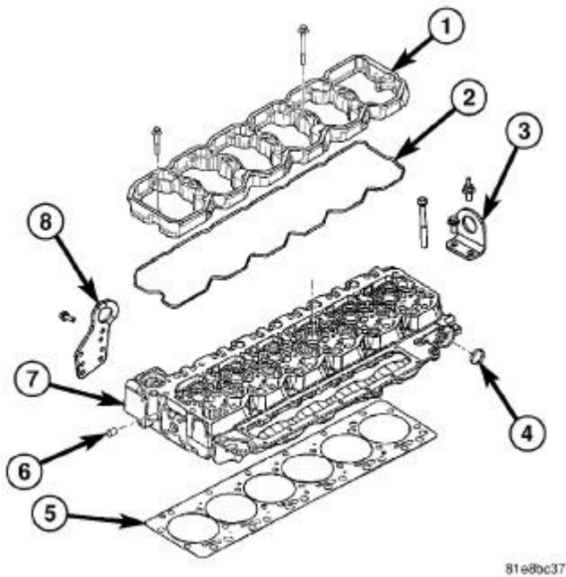
Fig. 70: Cylinder Head And Gasket Courtesy of CHRYSLER LLC
