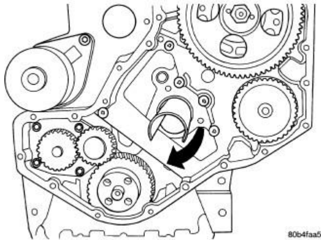
Fig. 194: Rotate Trough One Half Turn (180 Degrees) So Open Side Faces Down Courtesy of CHRYSLER LLC
