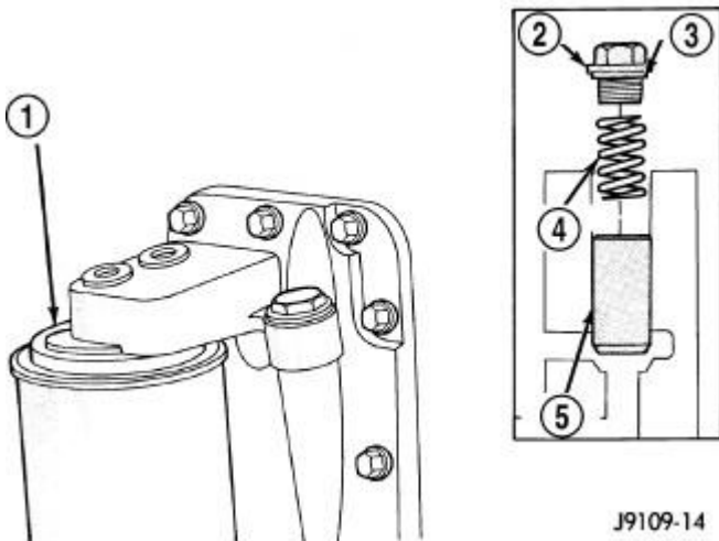
Fig. 287: Oil Pressure Regulator Courtesy of CHRYSLER LLC
