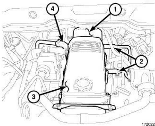
Fig. 14: Cylinder Head Cover Components Courtesy of CHRYSLER LLC
