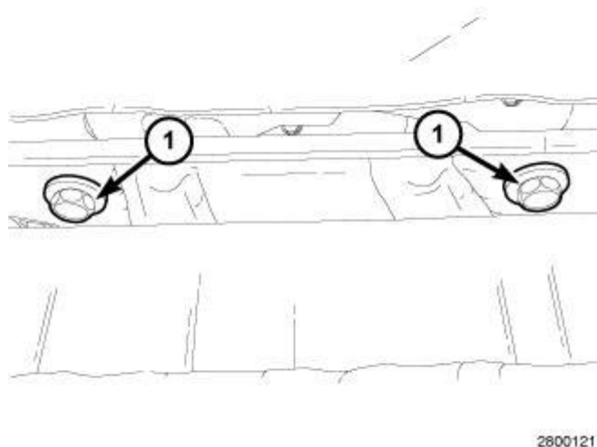
Fig. 209: Identifying Transmission Mount Support Bracket Bolts - AS68RC A/T Courtesy of CHRYSLER LLC
