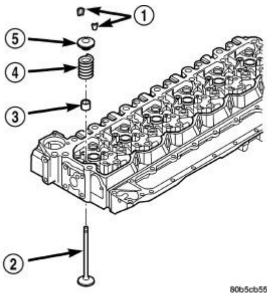
Fig. 100: Valve Spring, Seal, And Retainers Courtesy of CHRYSLER LLC
