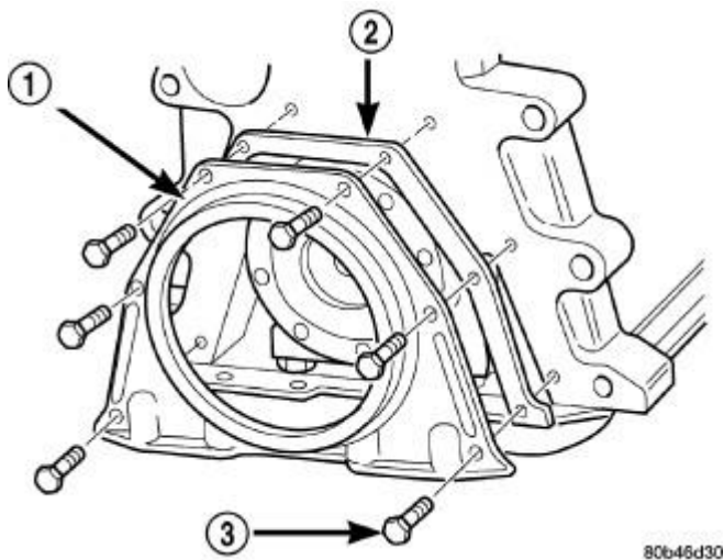
Fig. 149: Crankshaft Rear Seal Retainer And Gasket Courtesy of CHRYSLER LLC
