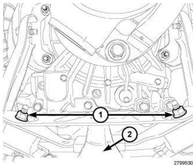
Fig. 218: Identifying Rear Transmission Mount & Nuts - AS68RC A/T Courtesy of CHRYSLER LLC
