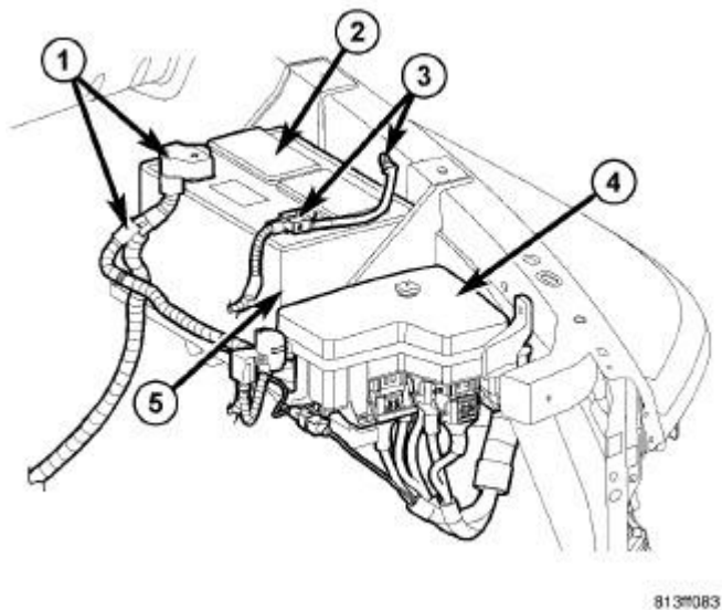
Fig. 253: Locating Battery System Components (Typical) Courtesy of CHRYSLER LLC
