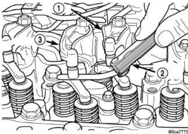
Fig. 104: Measuring Valve Lash Courtesy of CHRYSLER LLC
