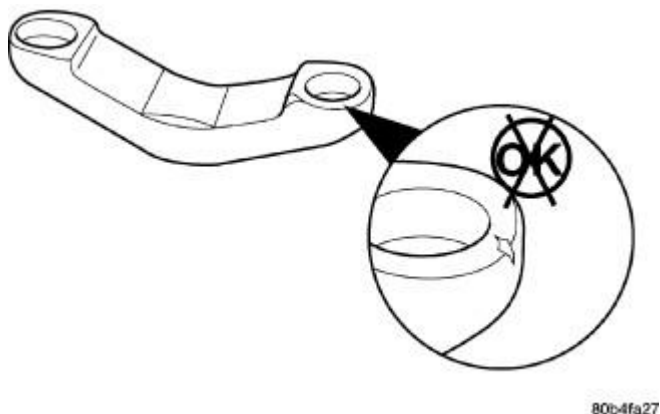
Fig. 56: Inspecting Crosshead For Cracks
