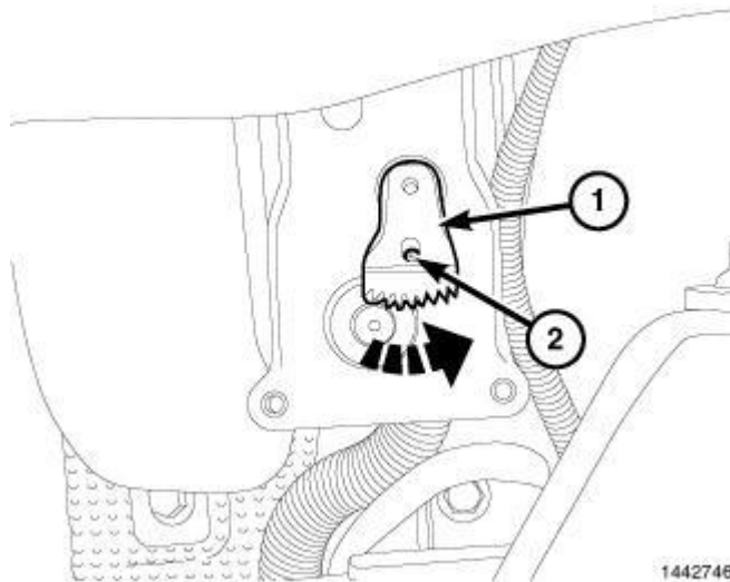
Fig. 324: Selector Gear - Forward Courtesy of CHRYSLER LLC
