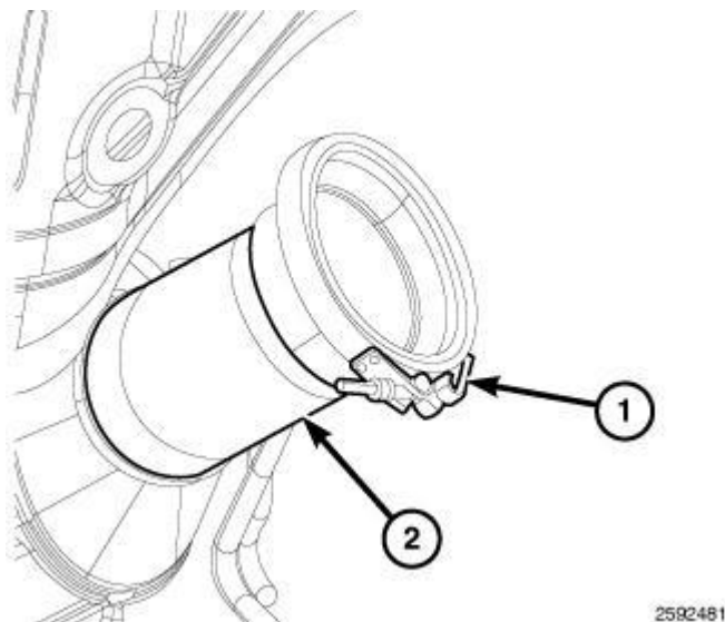
Fig. 334: Turbocharger Exhaust Outlet V-clamp Courtesy of CHRYSLER LLC
