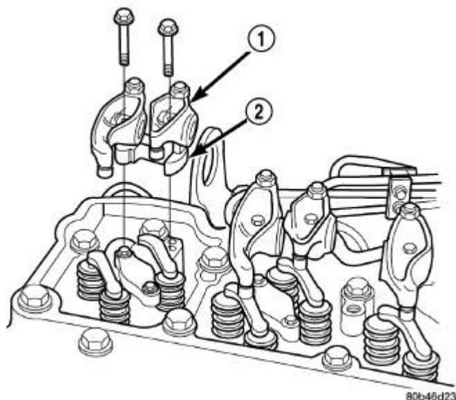
Fig. 16: Rocker Arms And Pedestal Removal
