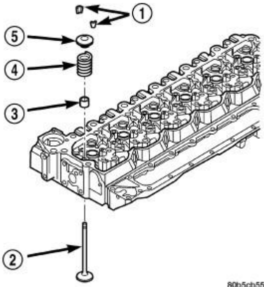
Fig. 92: Valve Spring, Seal, And Retainers Courtesy of CHRYSLER LLC
