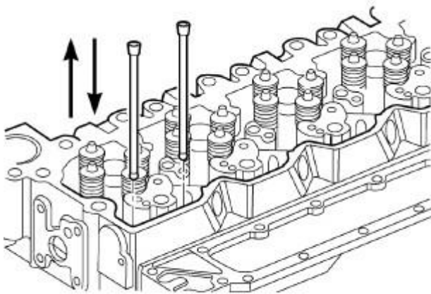
Fig. 60: Push Rod Removal/Installation Courtesy of CHRYSLER LLC
