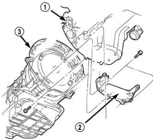
Fig. 170: Transmission Collar Courtesy of CHRYSLER LLC
