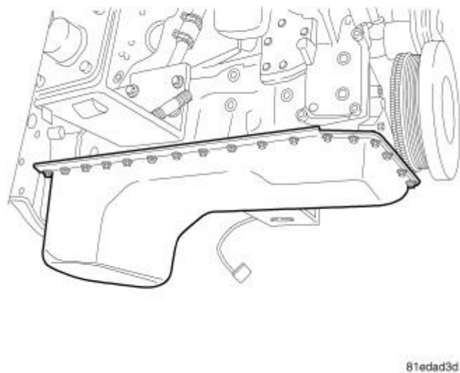
Fig. 30: Identifying Oil Pan Courtesy of CHRYSLER LLC
