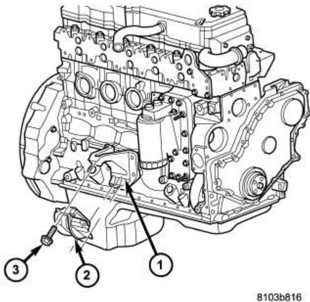
Fig. 261: RH Insulator Courtesy of CHRYSLER LLC
