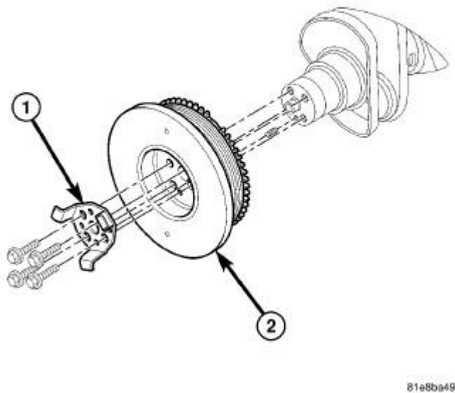
Fig. 180: Crankshaft Damper (Non-High Output Engine) Courtesy of CHRYSLER LLC
