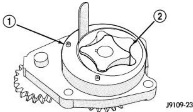
Fig. 283: Measuring Gerotor Planetary To Body Bore Clearance Courtesy of CHRYSLER LLC
