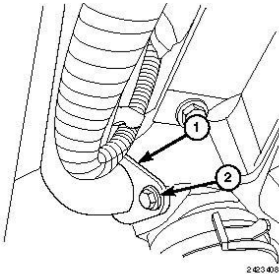
Fig. 242: Installing Front Coolant Tube Bolt Courtesy of CHRYSLER LLC
