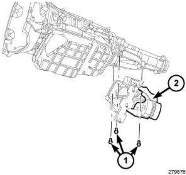
Fig. 214: Identifying Rear Transmission Mount & Bolts - 68RFE A/T, 4X2 Crew & Mega Cab Models
