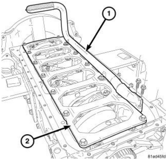
Fig. 352: Identifying Oil Pickup Tube
