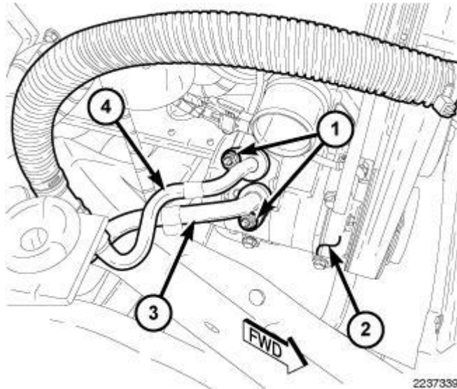
Fig. 26: Identifying Nuts, A/C Suction Line, A/C Discharge Line & A/C Compressor Courtesy of CHRYSLER LLC
