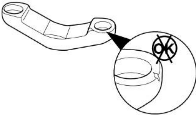
Fig. 86: Inspecting Crosshead For Cracks Courtesy of CHRYSLER LLC
