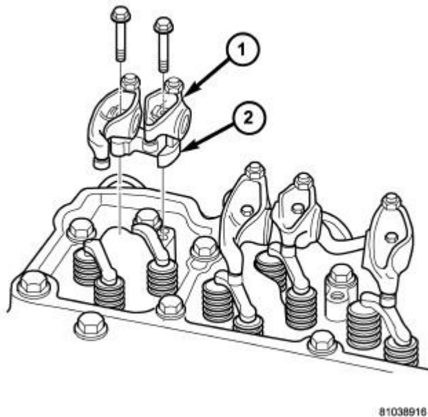
Fig. 61: Identifying Rocker Arm & Pedestal Courtesy of CHRYSLER LLC
