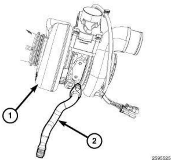
Fig. 318: Turbocharger & Drain Tube Courtesy of CHRYSLER LLC
