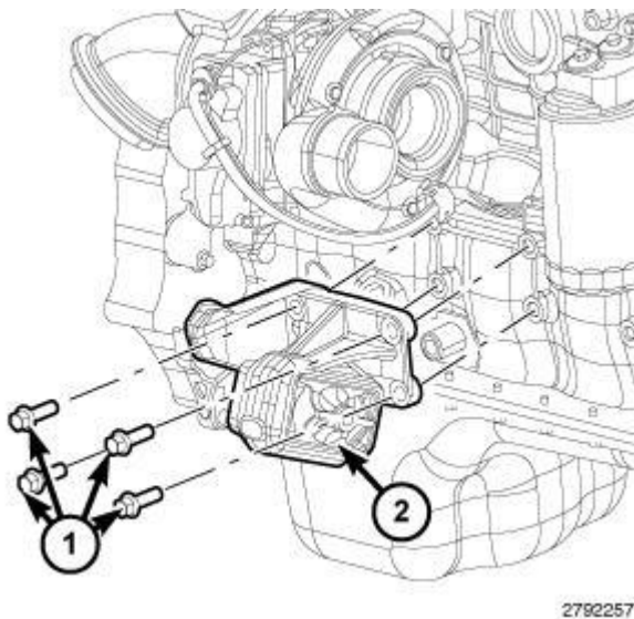
Fig. 199: RH Engine Mount Courtesy of CHRYSLER LLC
