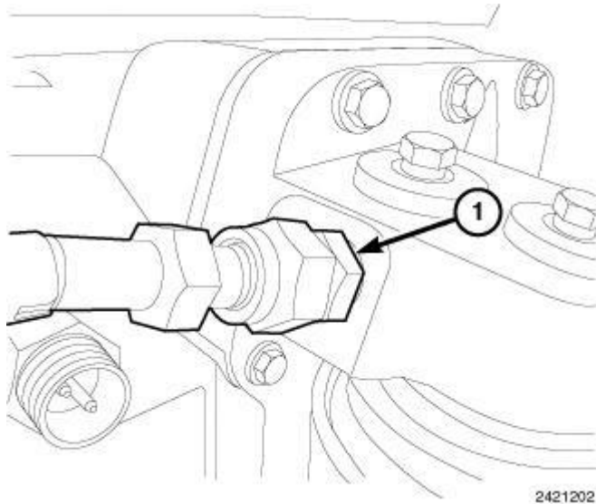
Fig. 241: Turbocharger Oil Supply Line Courtesy of CHRYSLER LLC
