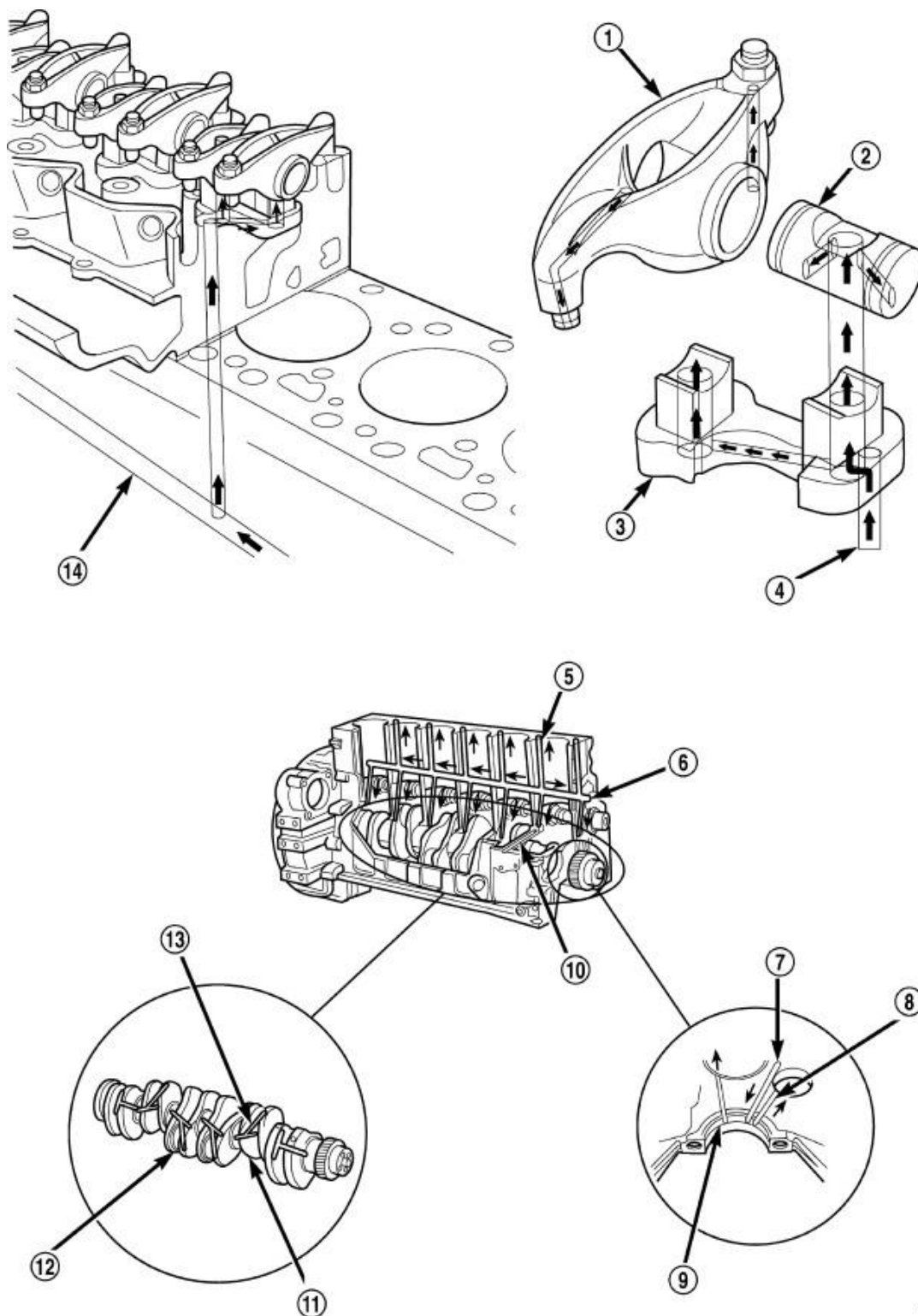
Fig. 225: Lubrication System Circulation (2 Of 2) Courtesy of CHRYSLER LLC
