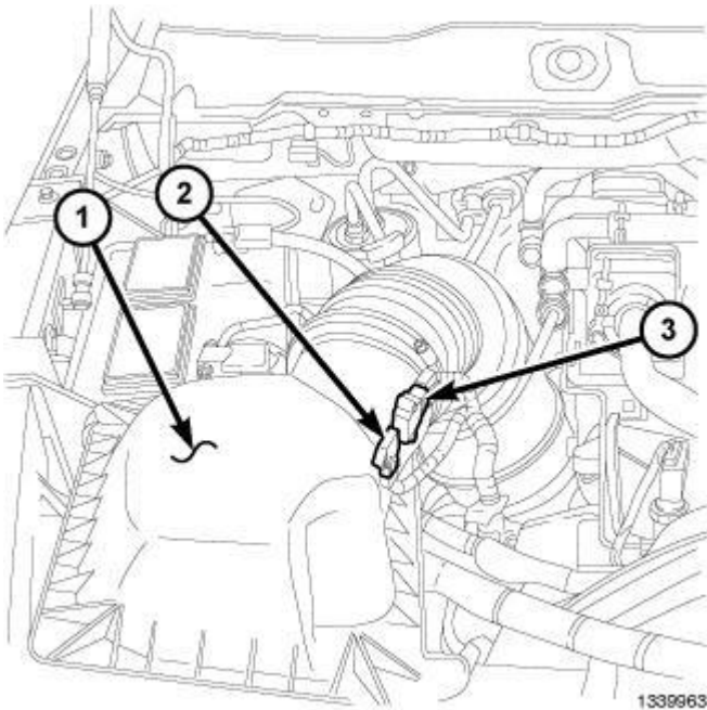
Fig. 298: Identifying Air Filter Housing Cover & Mass Air Flow (MAF) Sensor Courtesy of CHRYSLER LLC
