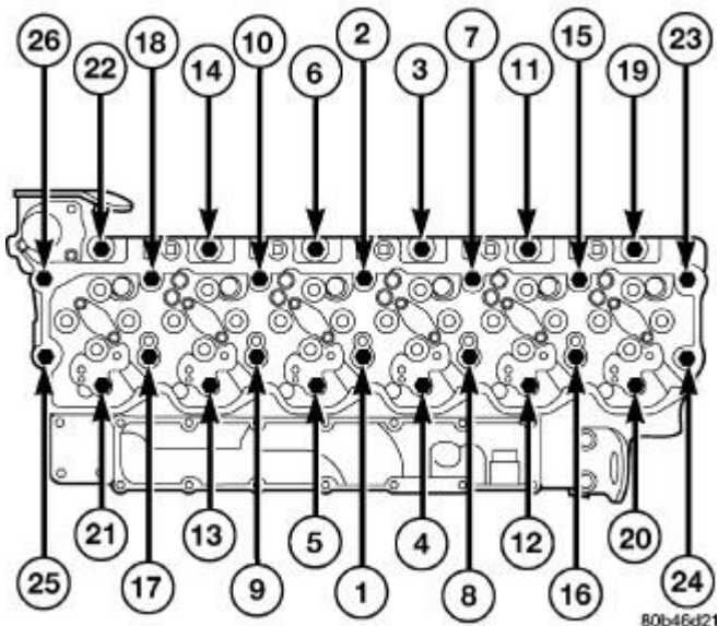
Fig. 59: Cylinder Head Bolt Torque Sequence
