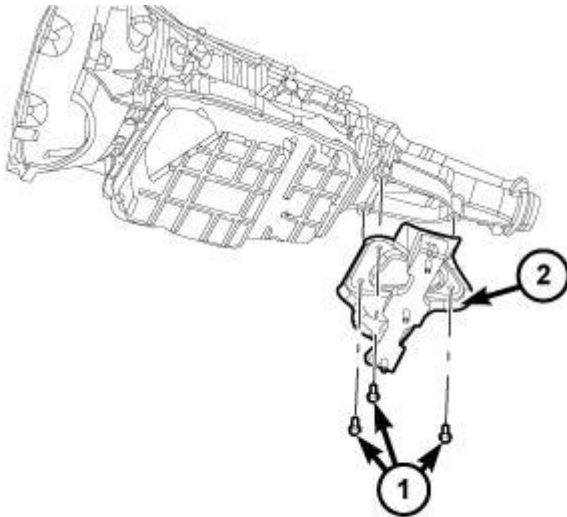
Fig. 213: Identifying Rear Transmission Mount & Bolts - 68RFE A/T - 4X2 Regular Cab Models Courtesy of CHRYSLER LLC
