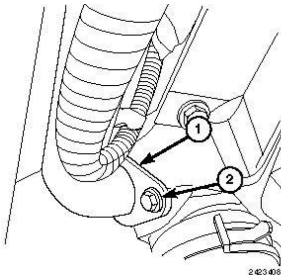
Fig. 234: Installing Front Coolant Tube Bolt Courtesy of CHRYSLER LLC
