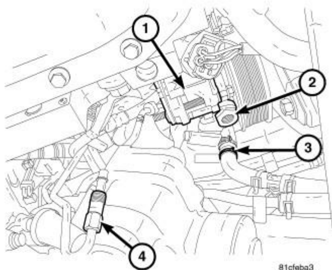
Fig. 342: Identifying Power Steering Pump, Pressure Line & Return Hose Courtesy of CHRYSLER LLC
