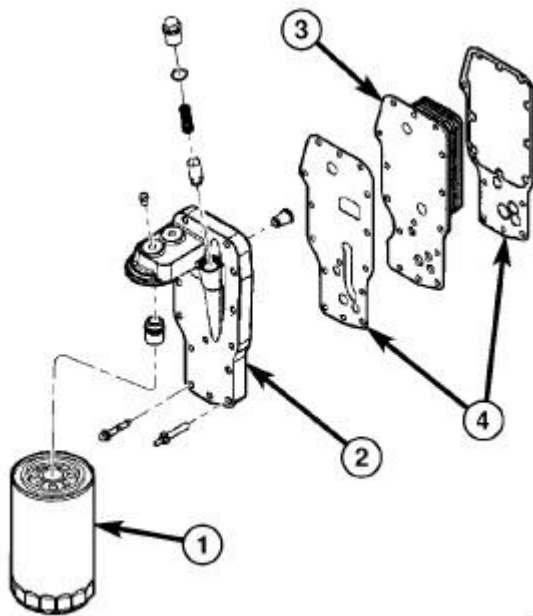
Fig. 239: Identifying Oil Filter And Cooler Courtesy of CHRYSLER LLC
