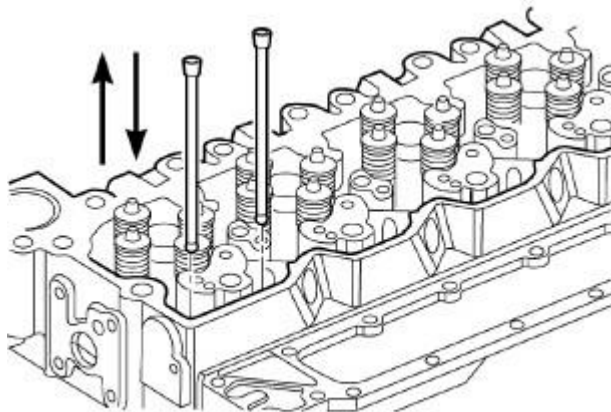
Fig. 52: Push Rod Removal/Installation Courtesy of CHRYSLER LLC
