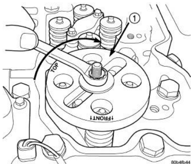
Fig. 102: Compressing Valve Springs With Tool 8319 Courtesy of CHRYSLER LLC
