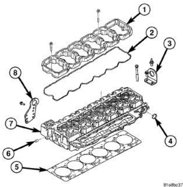
Fig. 45: Cylinder Head And Gasket Courtesy of CHRYSLER LLC
