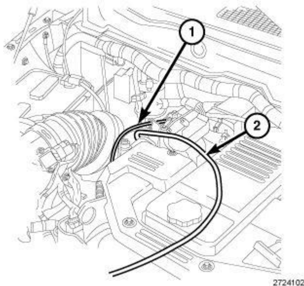
Fig. 306: Cleaning Tool Hose Courtesy of CHRYSLER LLC
