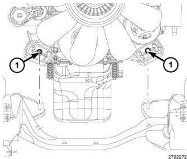
Fig. 206: Frame Mounts Courtesy of CHRYSLER LLC
