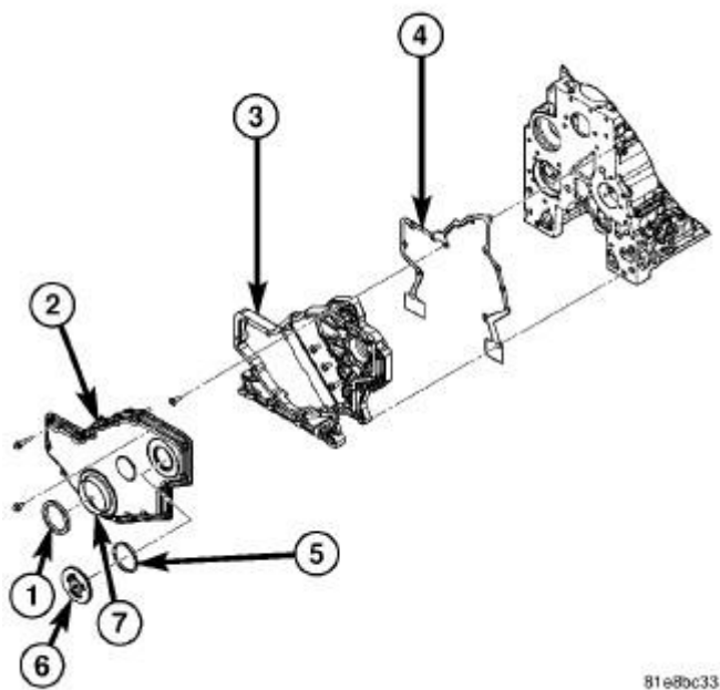
Fig. 137: Front Cover Courtesy of CHRYSLER LLC
