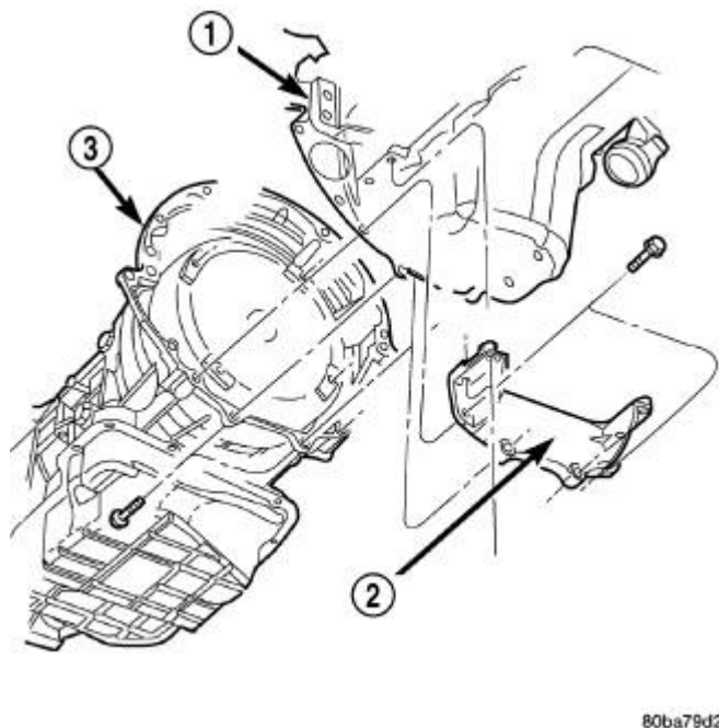
Fig. 160: Transmission Collar Courtesy of CHRYSLER LLC
