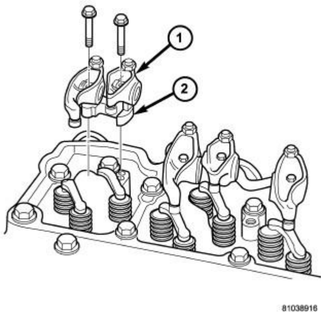
Fig. 80: Identifying Rocker Arm & Pedestal
