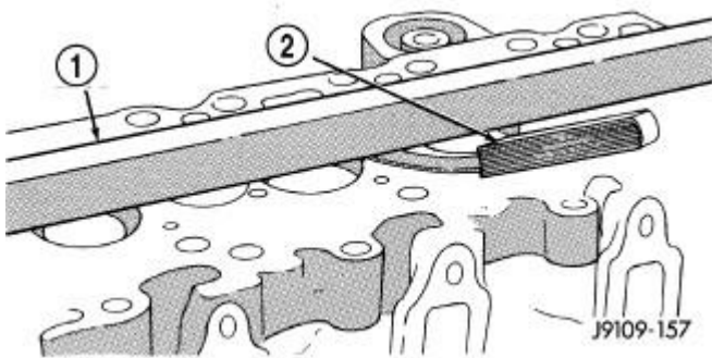
Fig. 54: Inspecting Cylinder Head Combustion Deck Face For Warpage Courtesy of CHRYSLER LLC
