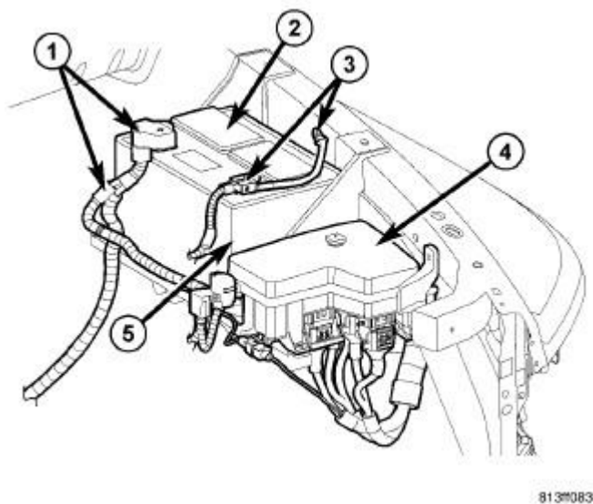
Fig. 226: Locating Battery System Components (Typical) Courtesy of CHRYSLER LLC
