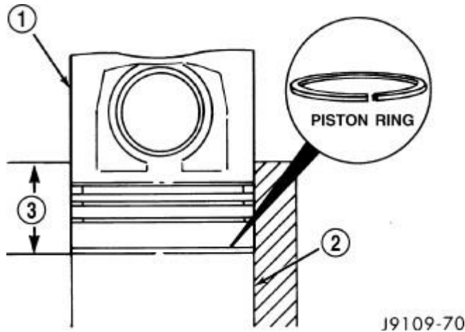
Fig. 152: Position Of Ring In Cylinder Bore Courtesy of CHRYSLER LLC
