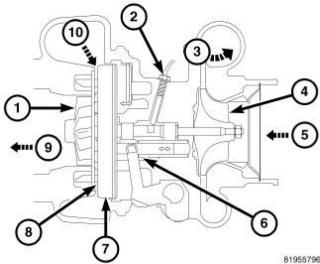
Fig. 322: 6.7L Turbocharger Courtesy of CHRYSLER LLC
