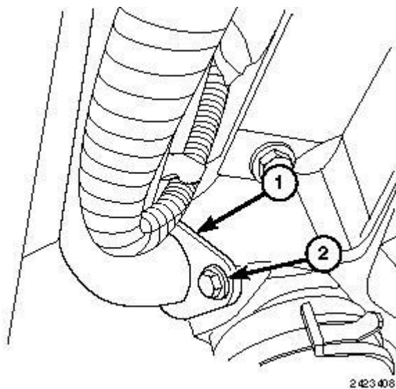
Fig. 237: Installing Front Coolant Tube Bolt
