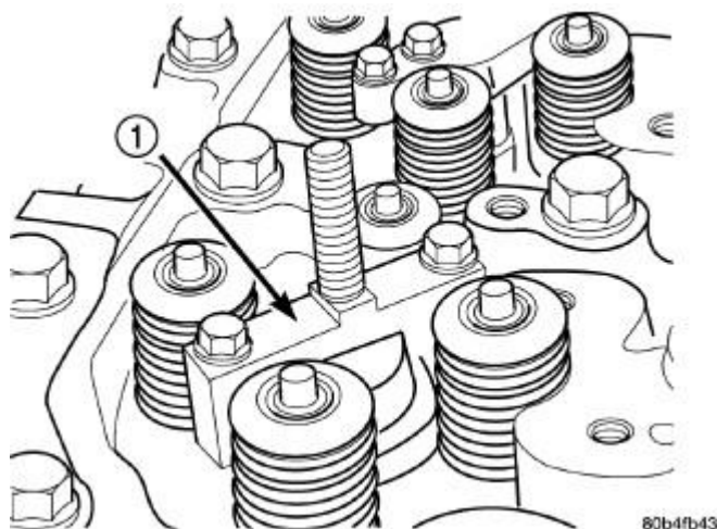
Fig. 101: Spring Compressor Mounting Base-Part of Tool 8319 Courtesy of CHRYSLER LLC
