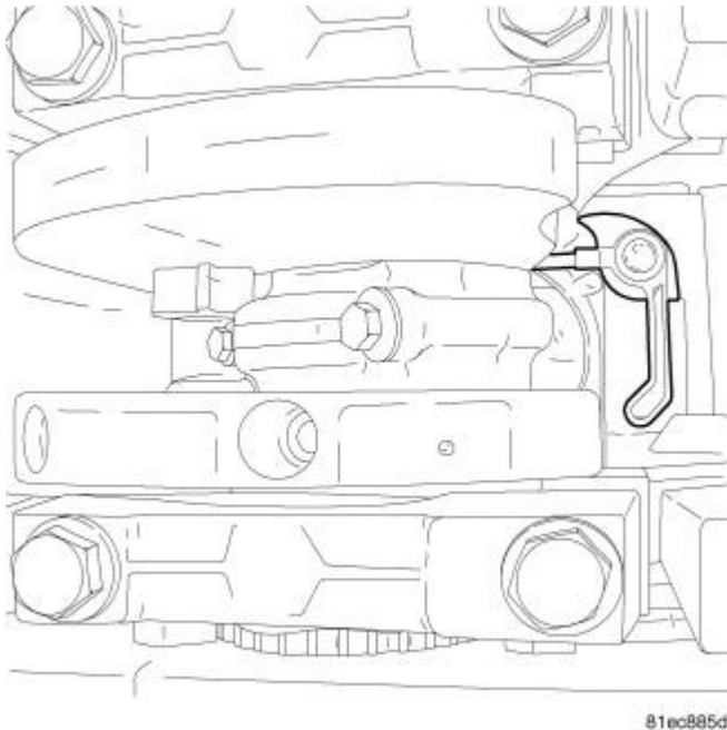
Fig. 169: Identifying Oil Jet Courtesy of CHRYSLER LLC
