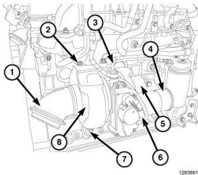
Fig. 336: Identifying Turbocharger Components Courtesy of CHRYSLER LLC
