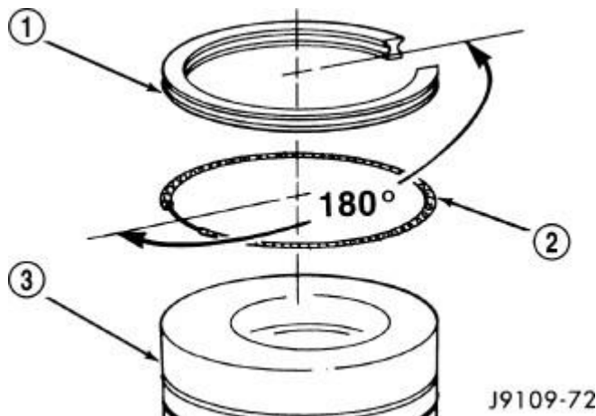
Fig. 153: Oil Control Ring/Expander Location In Groove
