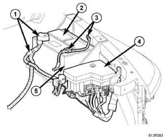
Fig. 263: Locating Battery System Components (Typical) Courtesy of CHRYSLER LLC
