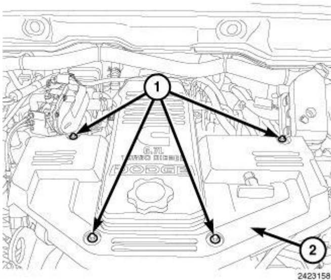
Fig. 6: Engine Cover Bolts Courtesy of CHRYSLER LLC
