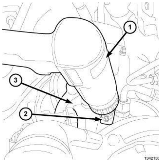
Fig. 302: Drilling Hole Through Turbocharger Center Housing Courtesy of CHRYSLER LLC
