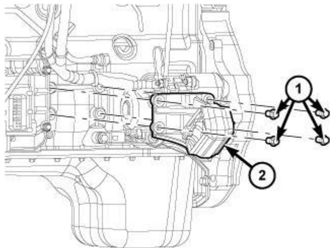
Fig. 200: LH Engine Mount Courtesy of CHRYSLER LLC
