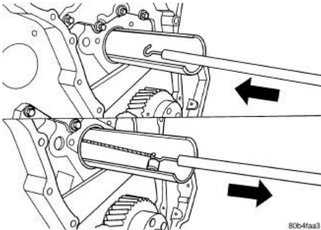
Fig. 191: Retrieve Tappet Installation Tool Through Cam Bore Courtesy of CHRYSLER LLC
