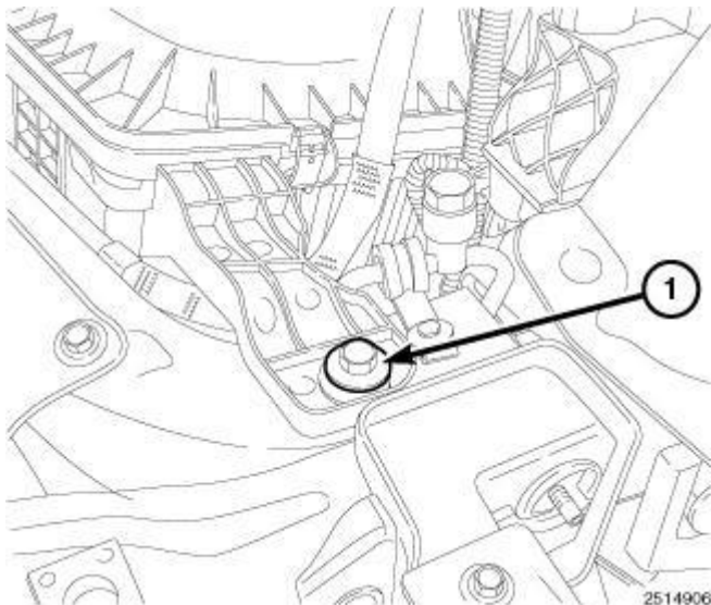
Fig. 39: Identifying Intake Air Housing Bolt Courtesy of CHRYSLER LLC
