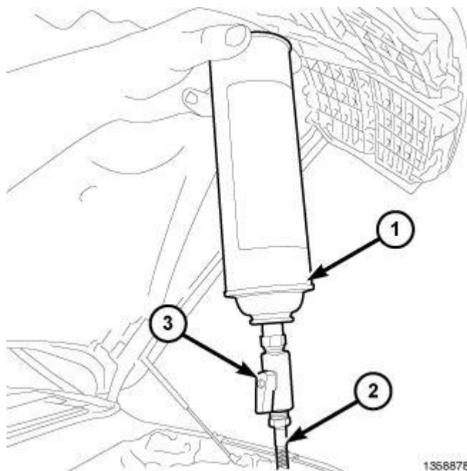
Fig. 307: Identifying Turbocharger Cleaner Can, Handle & Hose Courtesy of CHRYSLER LLC
