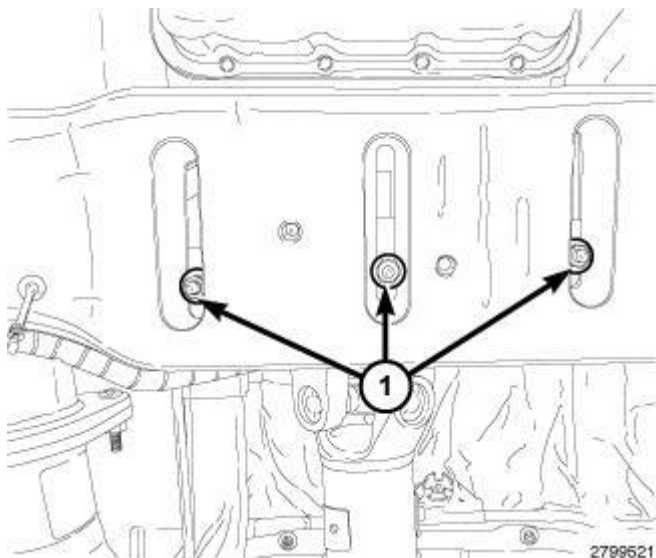
Fig. 207: Identifying Rear Transmission Mount To Crossmember Nuts - AS68RC A/T Courtesy of CHRYSLER LLC
