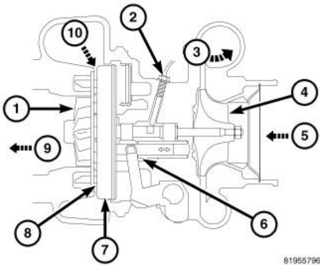
Fig. 321: 6.7L Turbocharger Courtesy of CHRYSLER LLC
