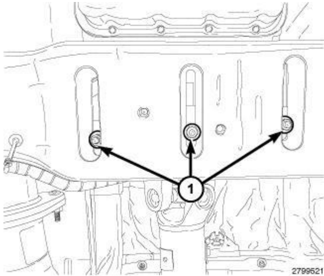
Fig. 219: Identifying Rear Transmission Mount To Crossmember Nuts - AS68RC A/T Courtesy of CHRYSLER LLC
