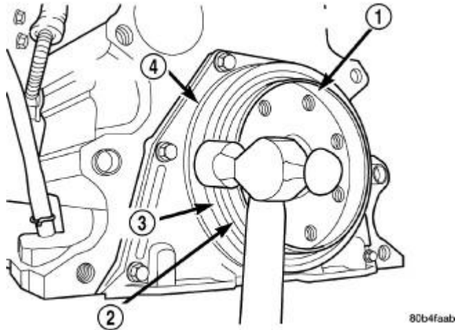
Fig. 183: Seal Installation Using Alignment Tool And Hammer Courtesy of CHRYSLER LLC
