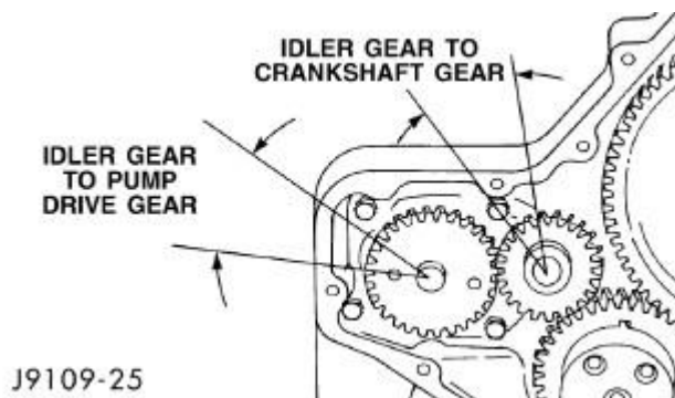
Fig. 286: Idler Gear To Pump Drive Gear And Crankshaft Gear Backlash Courtesy of CHRYSLER LLC
