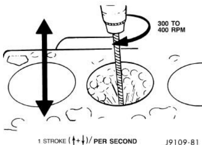
Fig. 112: De-Glazing Drill Speed And Vertical Speed
