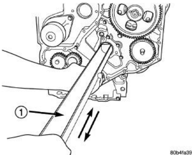
Fig. 189: Inserting The Trough Courtesy of CHRYSLER LLC
