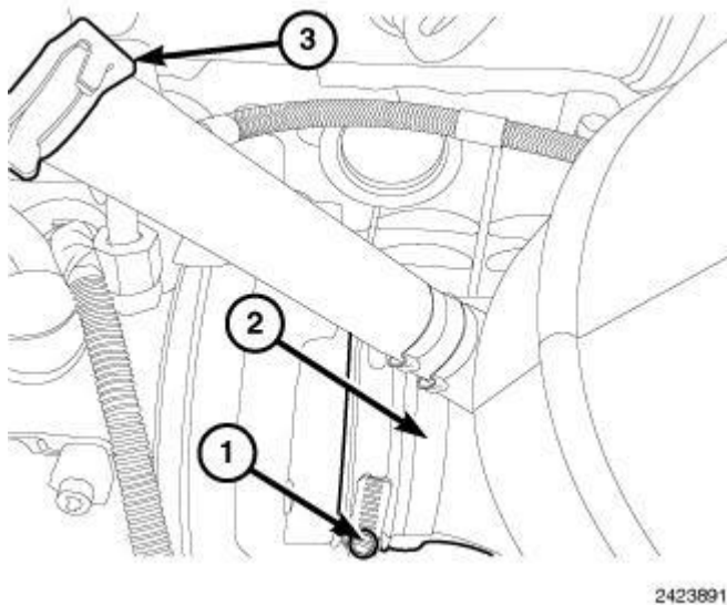
Fig. 44: Identifying Clamp, Outlet Tube & Breather Hose Courtesy of CHRYSLER LLC
