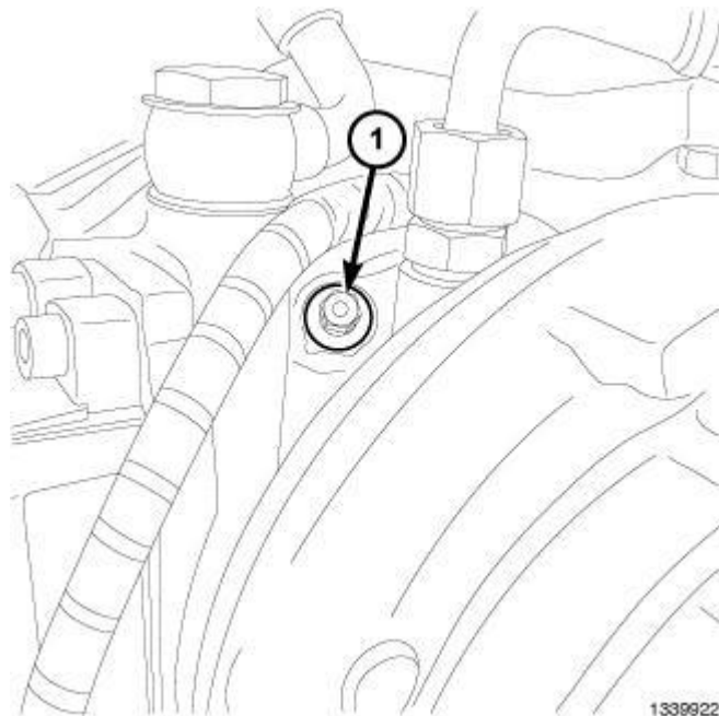
Fig. 309: Installing Turbocharger Cleaning Port Plug Courtesy of CHRYSLER LLC
