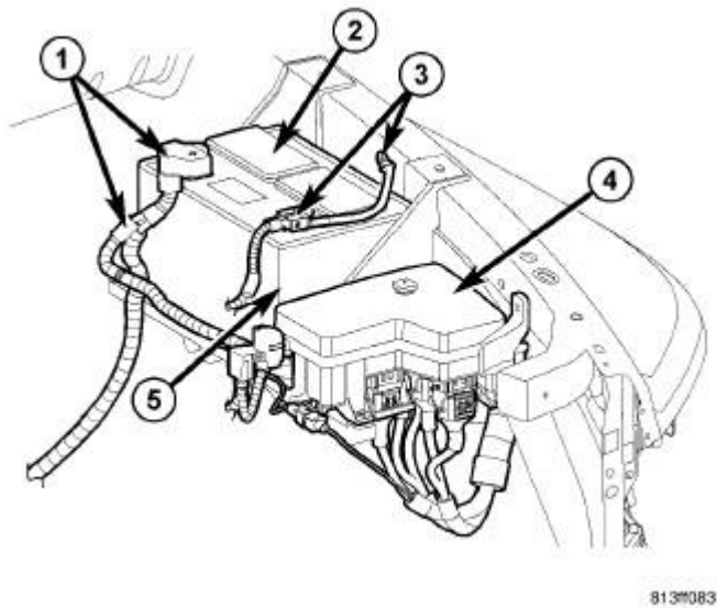
Fig. 181: Locating Battery System Components (Typical) Courtesy of CHRYSLER LLC
