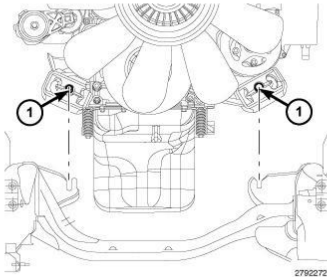
Fig. 203: Frame Mounts Courtesy of CHRYSLER LLC
