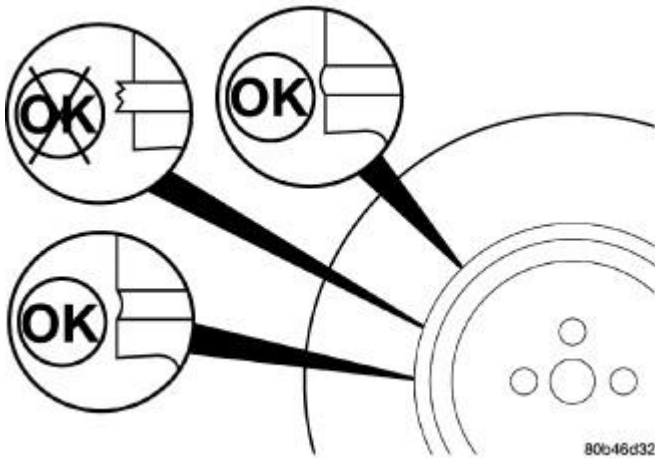
Fig. 146: Inspect Damper Rubber Member Courtesy of CHRYSLER LLC
