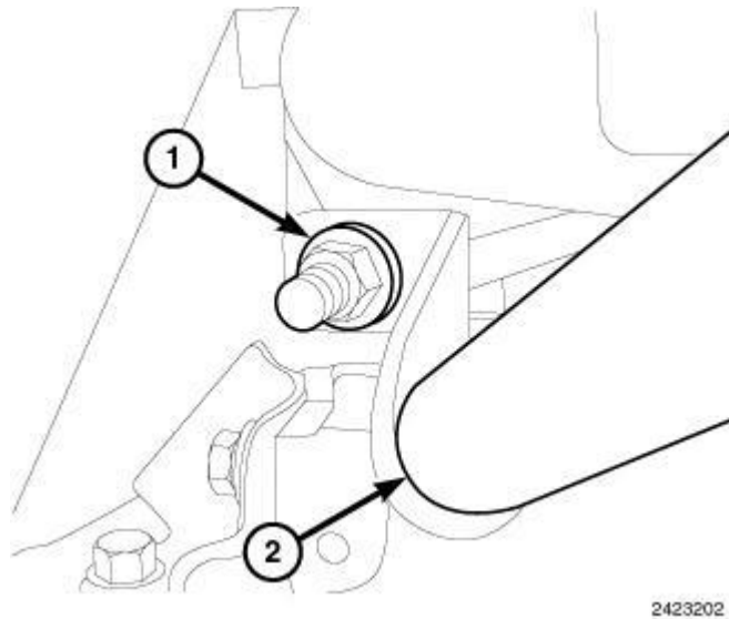
Fig. 246: Installing Coolant Outlet Tube Bracket Nut Courtesy of CHRYSLER LLC
