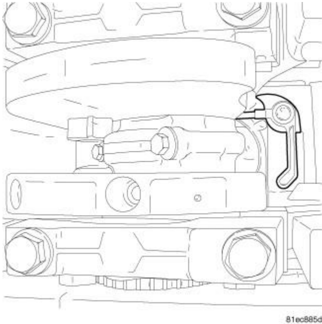
Fig. 162: Identifying Oil Jet Courtesy of CHRYSLER LLC
