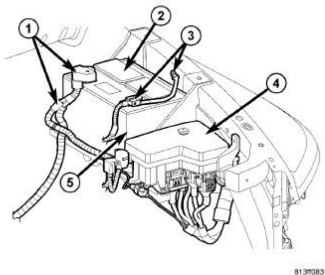
Fig. 173: Locating Battery System Components (Typical) Courtesy of CHRYSLER LLC
