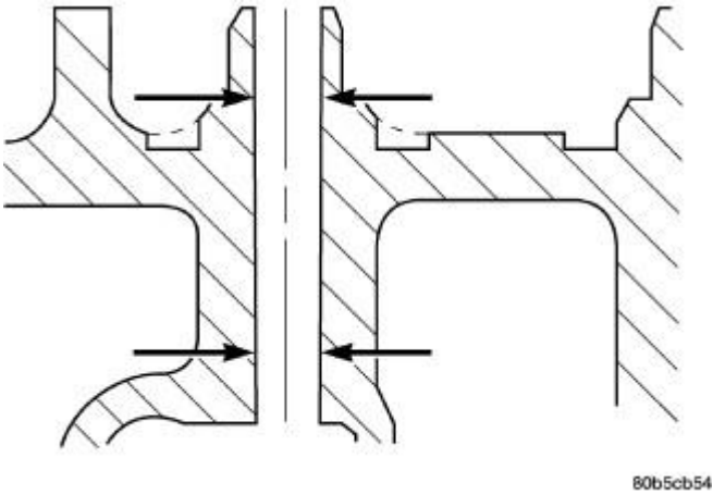
Fig. 95: Measure Valve Guide Bore Courtesy of CHRYSLER LLC
