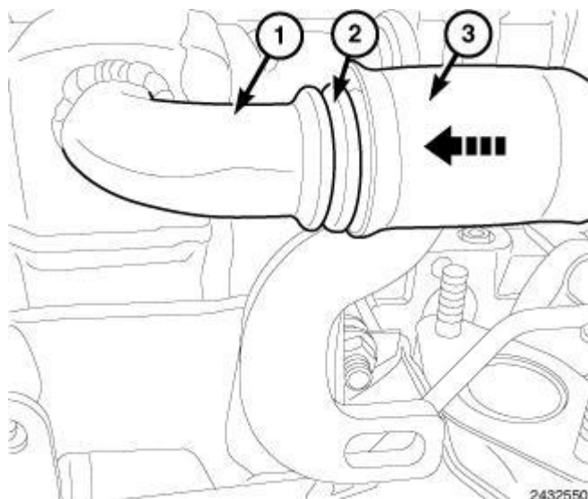
Fig. 243: Installing EGR Cooler, O-ring & Forward Coolant Tube Courtesy of CHRYSLER LLC
