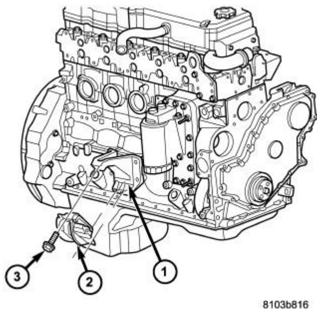
Fig. 67: RH Insulator Courtesy of CHRYSLER LLC
