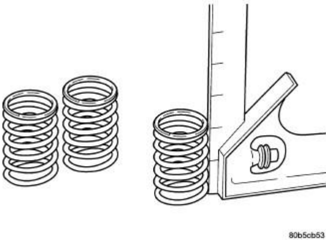
Fig. 97: Measure Valve Spring Free Length And Max. Inclination Courtesy of CHRYSLER LLC
