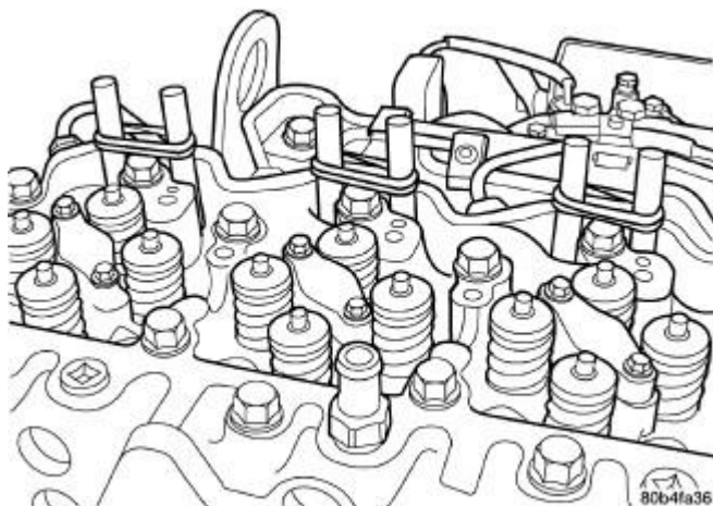
Fig. 125: Use Wooden Dowel Rods To Secure Tappets In Place Courtesy of CHRYSLER LLC
