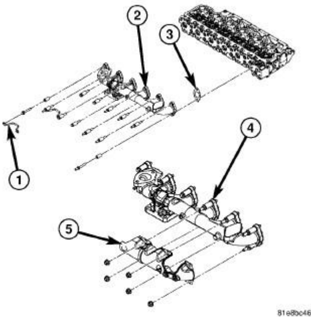
Fig. 66: Cylinder Head And Exhaust Manifold Courtesy of CHRYSLER LLC
