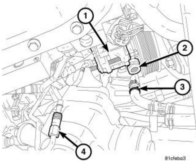
Fig. 10: Identifying Power Steering Pump, Pressure Line & Return Hose Courtesy of CHRYSLER LLC
