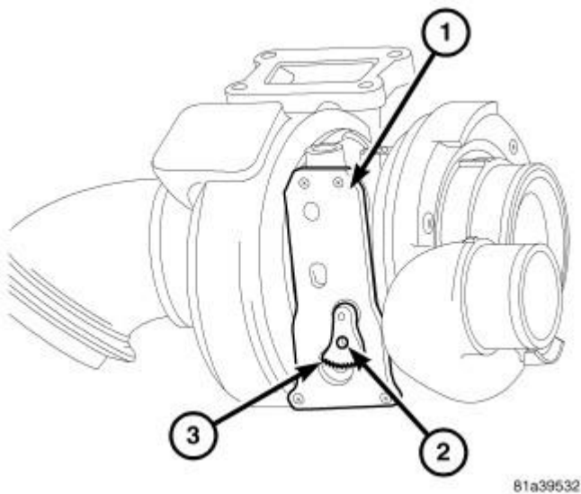
Fig. 323: Identifying Sector Gear Checks Courtesy of CHRYSLER LLC
