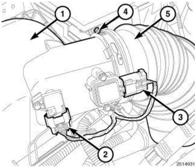
Fig. 42: Installing MAF Sensor, TBAP Sensor, Intake Air Tube, Air Cleaner Body & Clamp Courtesy of CHRYSLER LLC
