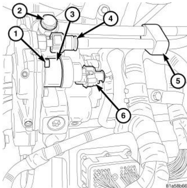
Fig. 348: Fuel Injection Pump - Rear View Courtesy of CHRYSLER LLC
