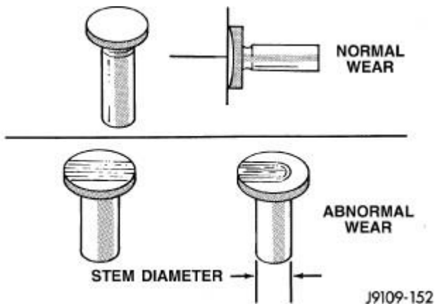
Fig. 188: Tappet Inspection Courtesy of CHRYSLER LLC
