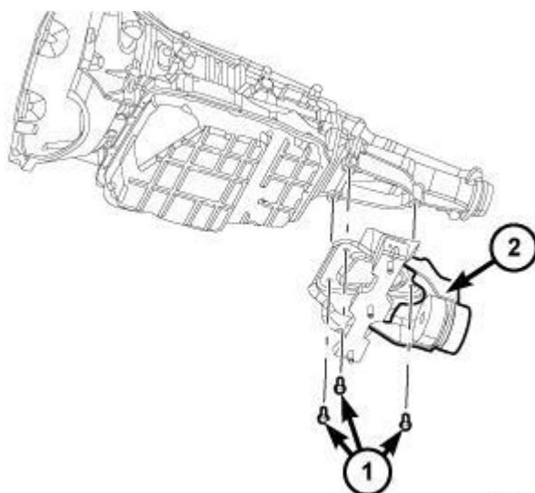
Fig. 223: Identifying Rear Transmission Mount & Bolts - 68RFE A/T, 4X2 Crew & Mega Cab Models Courtesy of CHRYSLER LLC
