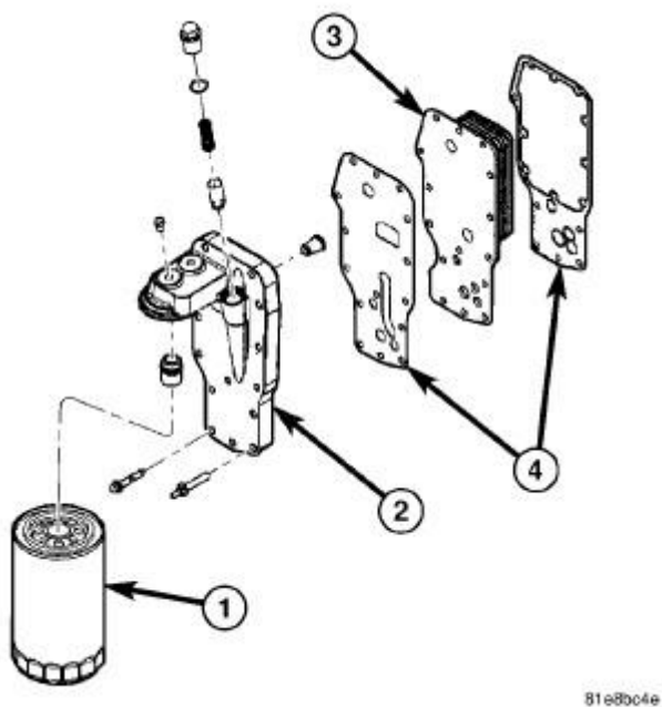
Fig. 254: Identifying Oil Filter And Cooler
