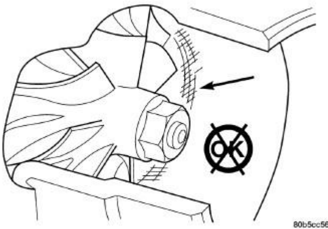
Fig. 330: Inspect Compressor Housing For Impeller Rubbing Condition Courtesy of CHRYSLER LLC
