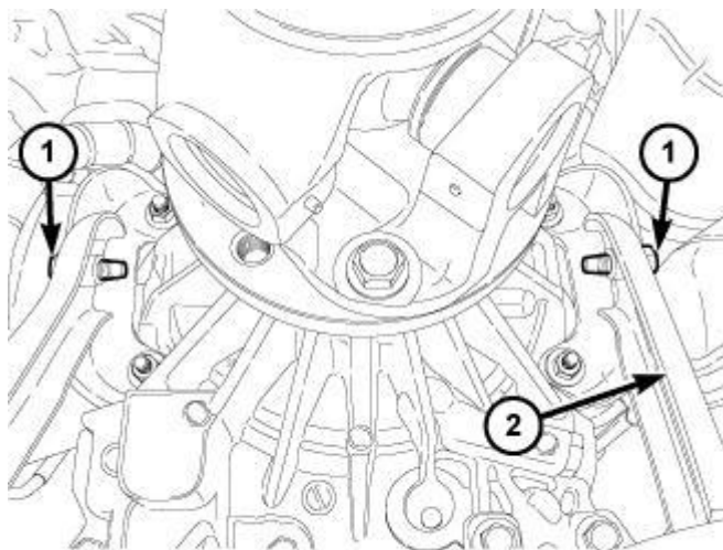
Fig. 215: Identifying Transmission Support Bracket & Bolts - AS68RC A/T Courtesy of CHRYSLER LLC
