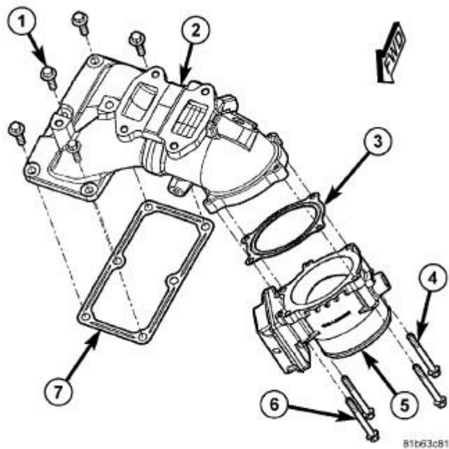
Fig. 293: EGR Air Flow Control Valve Location Courtesy of CHRYSLER LLC
