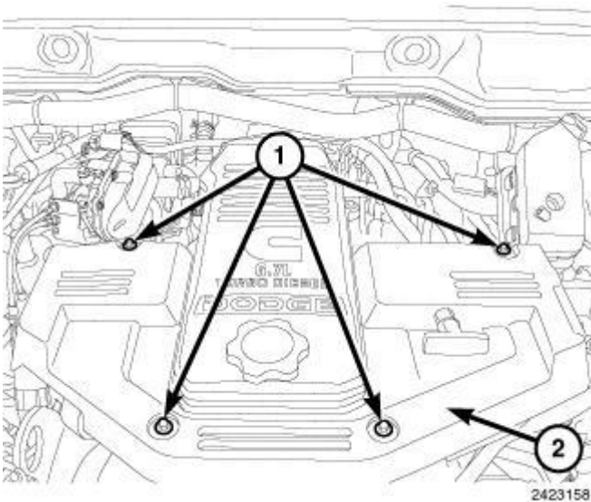
Fig. 71: Engine Cover Bolts Courtesy of CHRYSLER LLC
