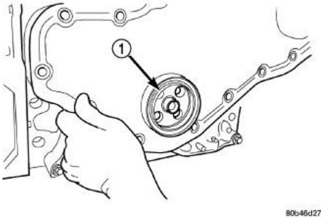
Fig. 178: Installing Front Cover With Seal Pilot Courtesy of CHRYSLER LLC
