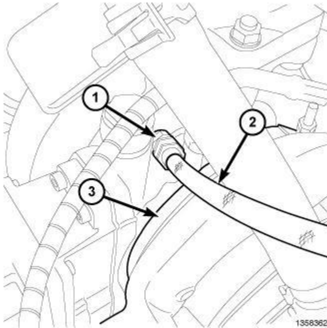
Fig. 308: Removing Nozzle, Cleaning Tool Hose & Turbocharger Courtesy of CHRYSLER LLC
