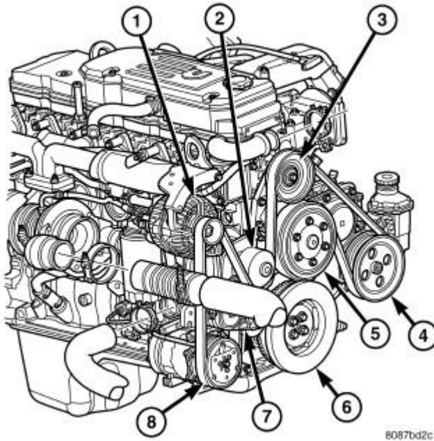
Fig. 361: Accessory Drive Belt Courtesy of CHRYSLER LLC
