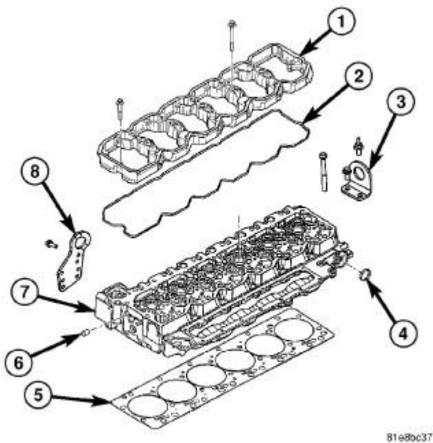
Fig. 158: Cylinder Head And Gasket Courtesy of CHRYSLER LLC
