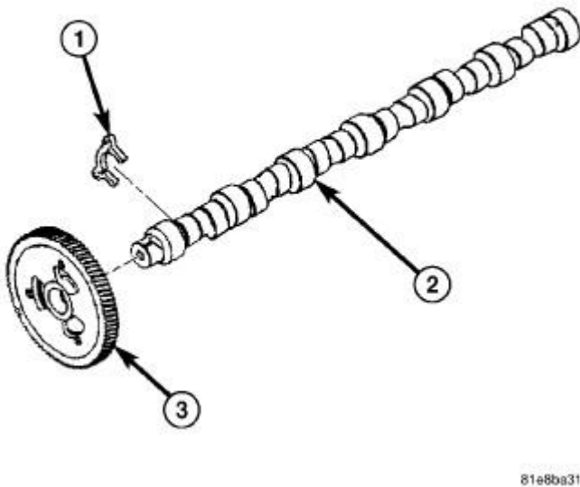
Fig. 133: Camshaft And Thrust Bearing Courtesy of CHRYSLER LLC
