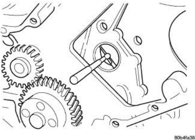
Fig. 129: Measuring Camshaft Bore Courtesy of CHRYSLER LLC
