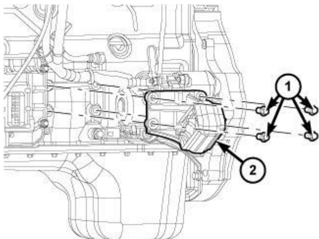
Fig. 201: LH Engine Mount Courtesy of CHRYSLER LLC
