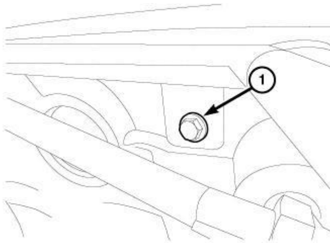
Fig. 232: Installing Coolant Outlet Tube Bracket Bolt Courtesy of CHRYSLER LLC
