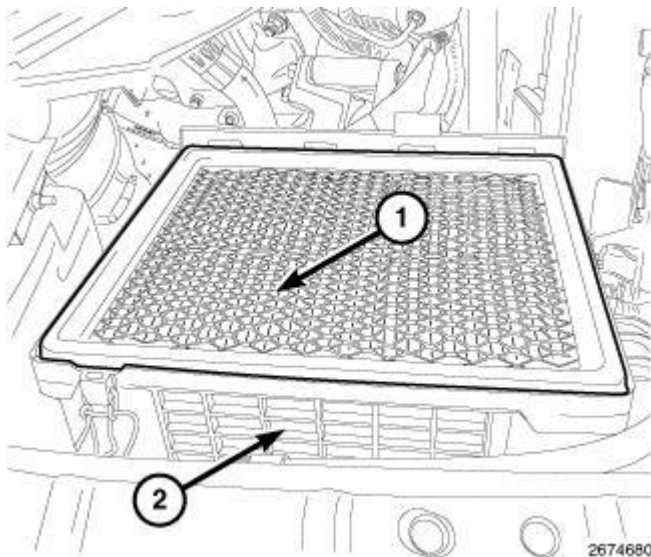
Fig. 35: Identifying Air Cleaner Housing & Air Cleaner Filter Courtesy of CHRYSLER LLC
