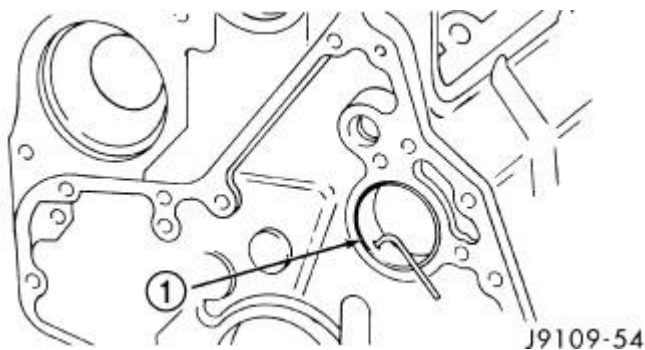
Fig. 132: Oil Hole Alignment Courtesy of CHRYSLER LLC
