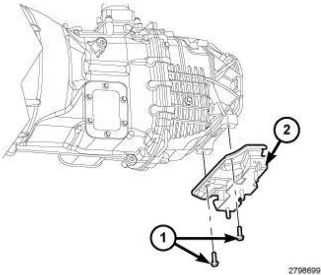
Fig. 220: Identifying Rear Transmission Mount & Bolts (M/T) Courtesy of CHRYSLER LLC
