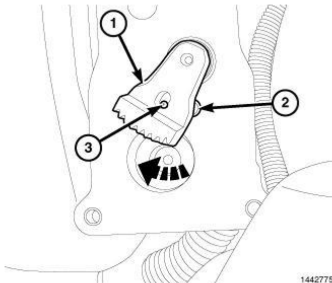
Fig. 325: Selector Gear - Rearward Position
