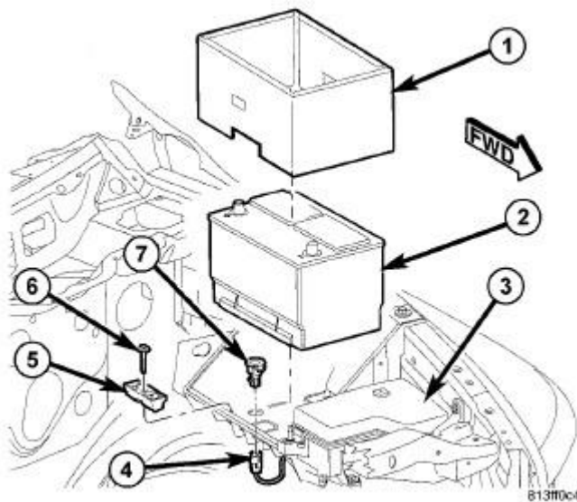
Fig. 69: Removing/installing Battery & Components Courtesy of CHRYSLER LLC
