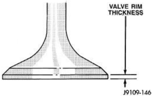
Fig. 96: Measure Valve Margin (Rim Thickness) Courtesy of CHRYSLER LLC
