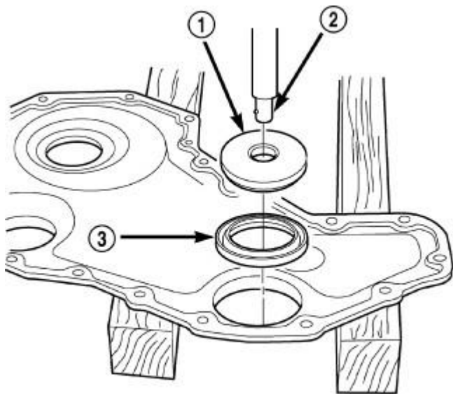
Fig. 356: Installing Seal Into Cover With Tool 8281 Courtesy of CHRYSLER LLC
