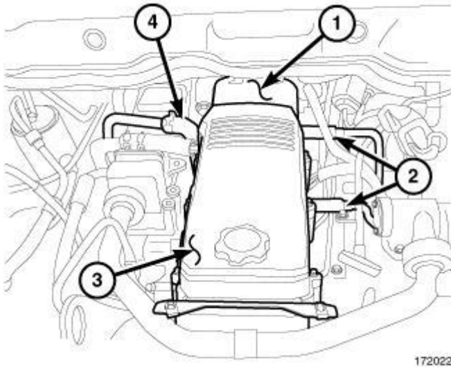
Fig. 23: Cylinder Head Cover Components Courtesy of CHRYSLER LLC
