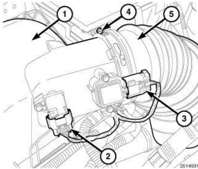
Fig. 40: Installing MAF Sensor, TBAP Sensor, Intake Air Tube, Air Cleaner Body & Clamp Courtesy of CHRYSLER LLC
