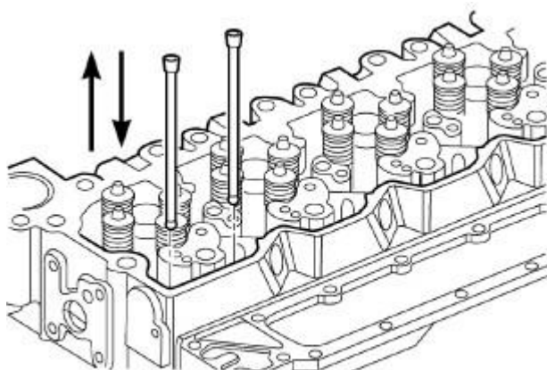
Fig. 124: Push Rod Removal/Installation Courtesy of CHRYSLER LLC
