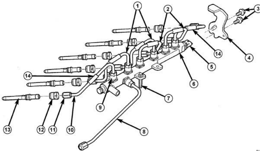
Fig. 50: Fuel Lines At Rail Courtesy of CHRYSLER LLC
