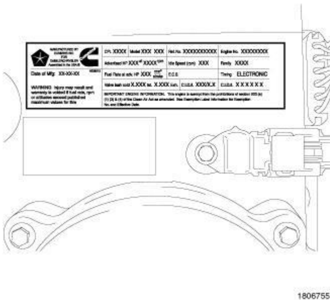
Fig. 33: Engine Data Plate Details Courtesy of CHRYSLER LLC
