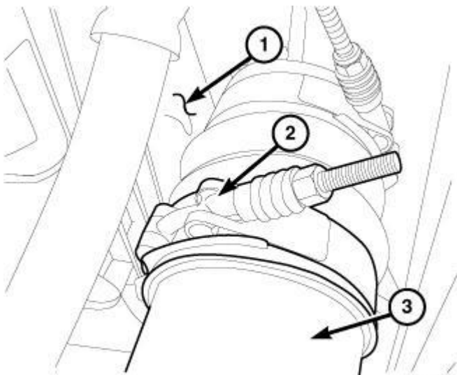
Fig. 248: Identifying Clamp, Charge Inlet Tube & Charge Air Cooler (CAC) Courtesy of CHRYSLER LLC
