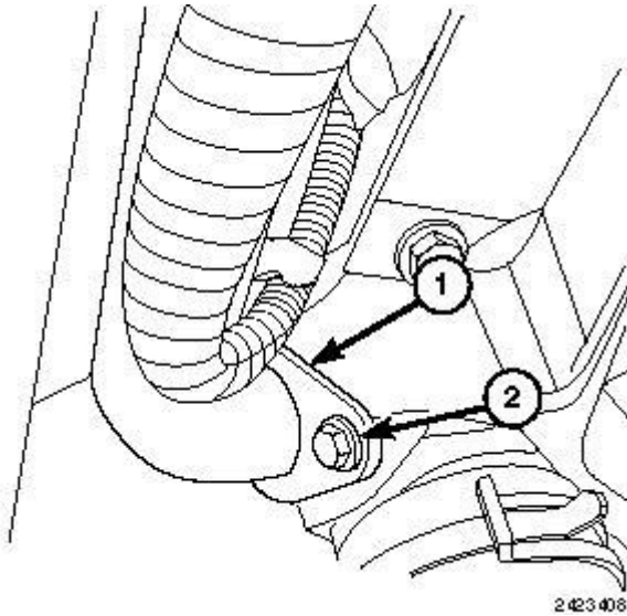
Fig. 245: Installing Front Coolant Tube Bolt Courtesy of CHRYSLER LLC
