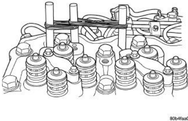
Fig. 185: Secure Dowel/Tappet To Adjacent Cylinder Courtesy of CHRYSLER LLC
