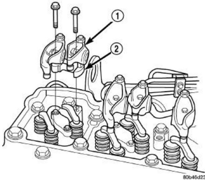
Fig. 21: Rocker Arms And Pedestal Removal Courtesy of CHRYSLER LLC
