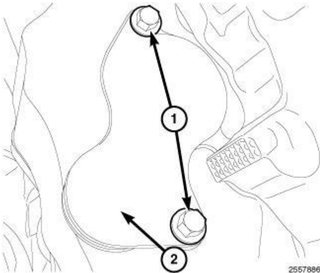
Fig. 105: Identifying Bolts & Bell Housing Access Cover Courtesy of CHRYSLER LLC
