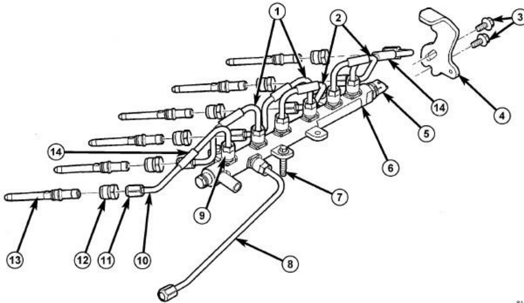
Fig. 20: Fuel Lines At Rail Courtesy of CHRYSLER LLC
