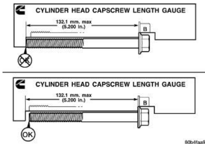
Fig. 55: Head Bolt Stretch Gauge Courtesy of CHRYSLER LLC
