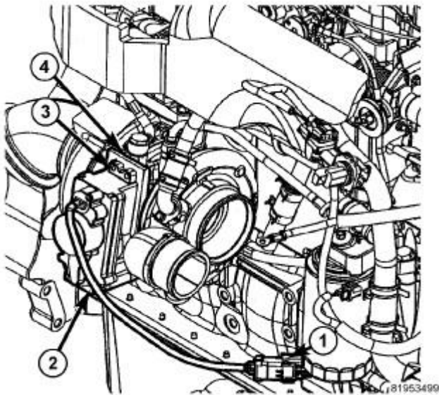
Fig. 310: 6.7L Turbocharger Actuator Courtesy of CHRYSLER LLC
