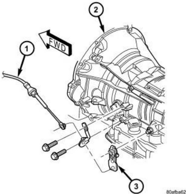
Fig. 269: Gearshift Cable at Transmission - RFE Courtesy of CHRYSLER LLC
