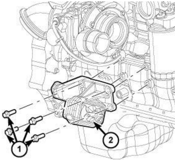
Fig. 202: RH Engine Mount Courtesy of CHRYSLER LLC
