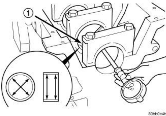
Fig. 118: Identifying Main Bearing Bore Diameter Courtesy of CHRYSLER LLC
