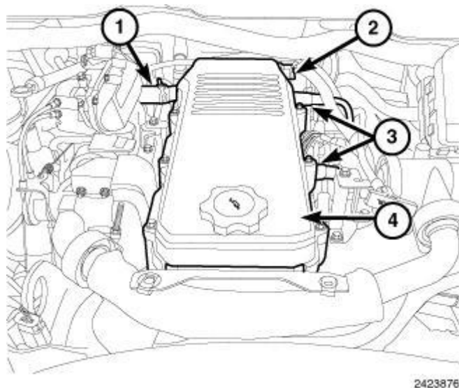
Fig. 77: Identifying CCV Tube, Crankcase Pressure Sensor Connector, CCV Oil Drains & Close Crankcase Ventilation (CCV) Cover Courtesy of CHRYSLER LLC
