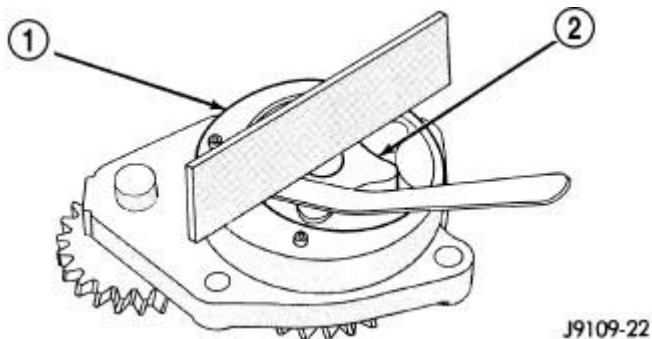
Fig. 282: Measuring Gerotor To Port Plate Clearance Courtesy of CHRYSLER LLC
