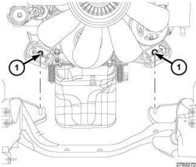
Fig. 195: Frame Mounts Courtesy of CHRYSLER LLC
