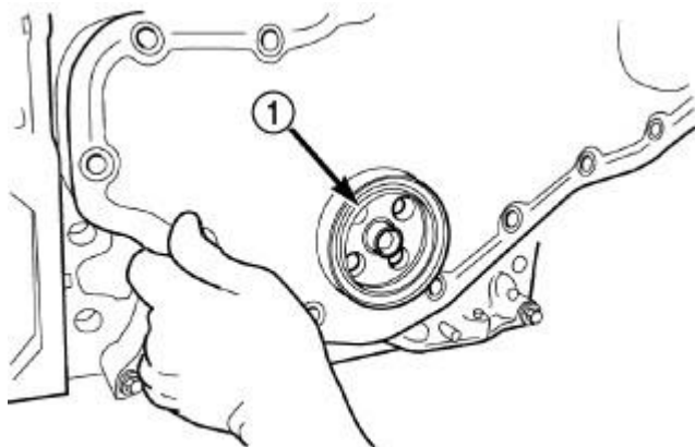
Fig. 357: Installing Front Cover With Seal Pilot Courtesy of CHRYSLER LLC
