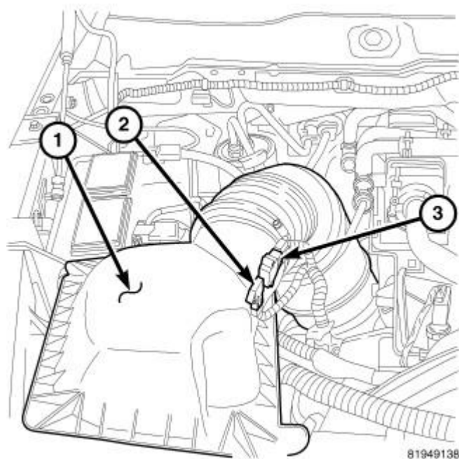
Fig. 252: Housing - Air Cleaner Courtesy of CHRYSLER LLC
