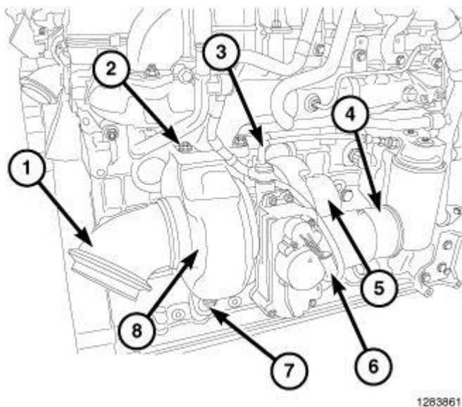
Fig. 326: Identifying Turbocharger Components Courtesy of CHRYSLER LLC
