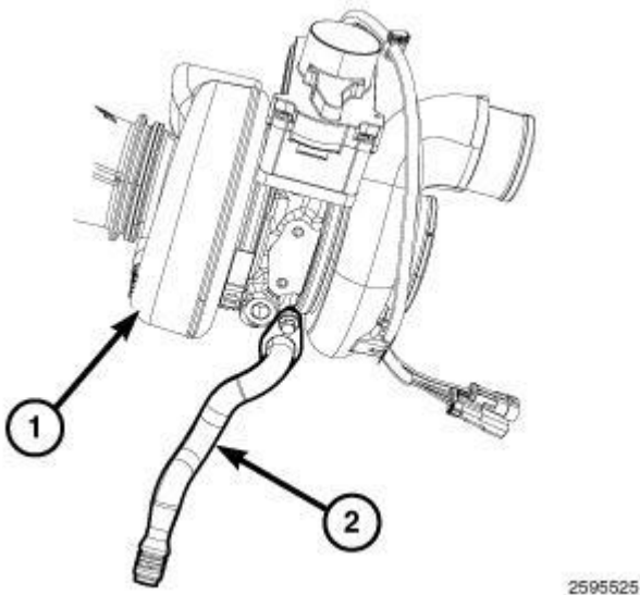
Fig. 329: Turbocharger & Drain Tube Courtesy of CHRYSLER LLC
