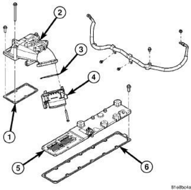
Fig. 49: Intake Air Heater Assembly Courtesy of CHRYSLER LLC
