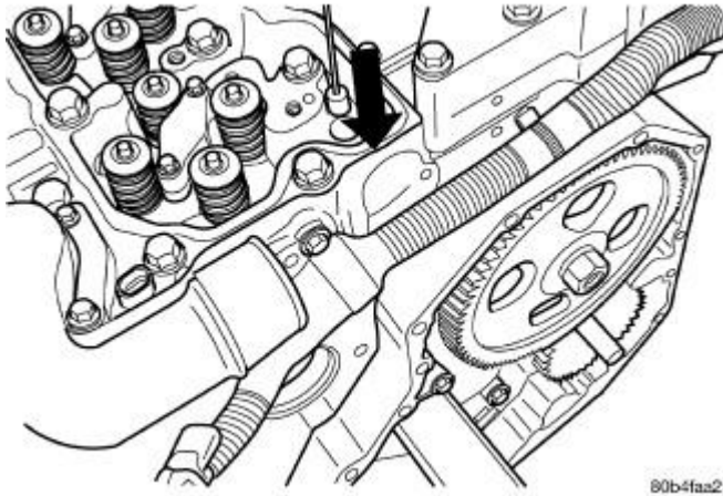
Fig. 190: Insert Installation Tool Through Push Rod Hole Courtesy of CHRYSLER LLC
