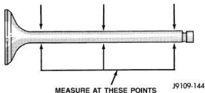
Fig. 94: Measure Valve Stem Diameter Courtesy of CHRYSLER LLC
