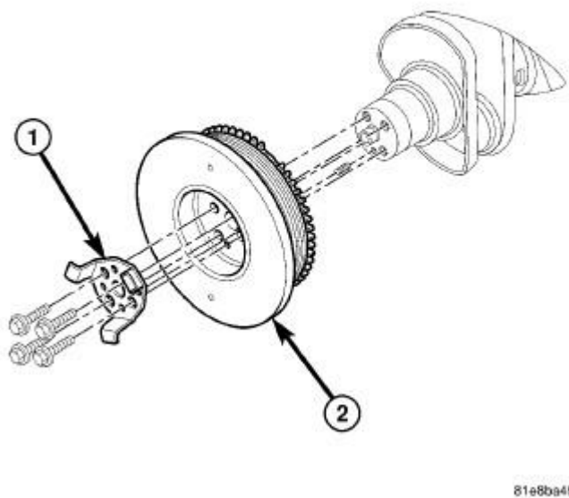
Fig. 138: Crankshaft Damper (Non-High Output Engine) Courtesy of CHRYSLER LLC
