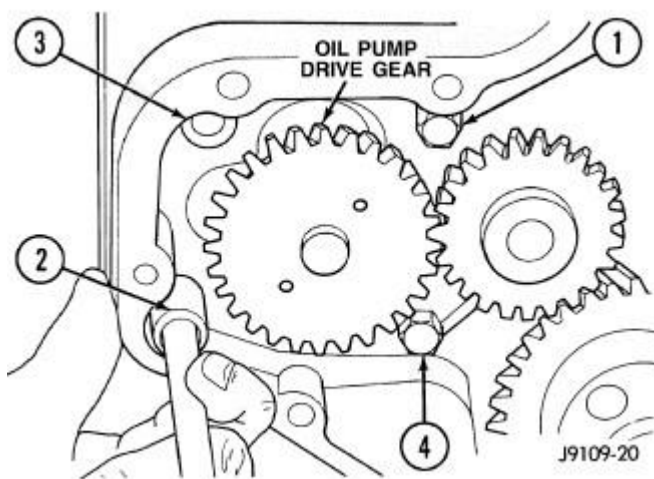
Fig. 285: Oil Pump Mounting Bolt Torque Sequence Courtesy of CHRYSLER LLC
