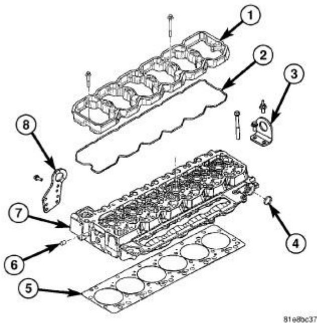
Fig. 53: Cylinder Head And Gasket Courtesy of CHRYSLER LLC
