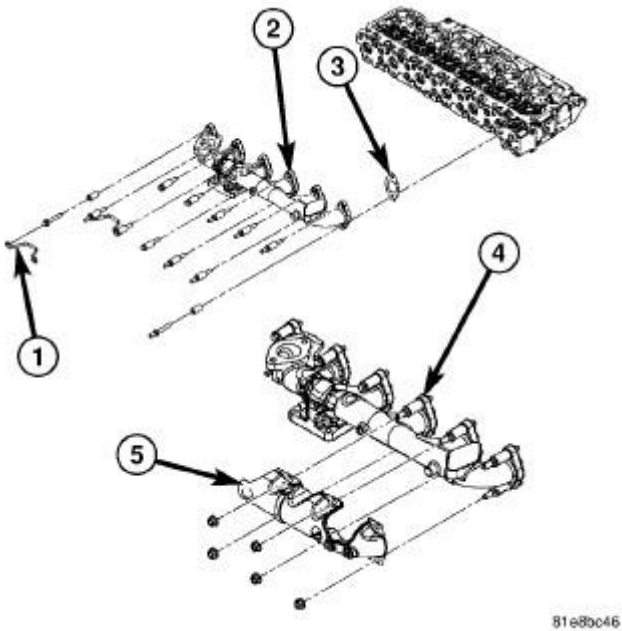
Fig. 47: Cylinder Head And Exhaust Manifold Courtesy of CHRYSLER LLC
