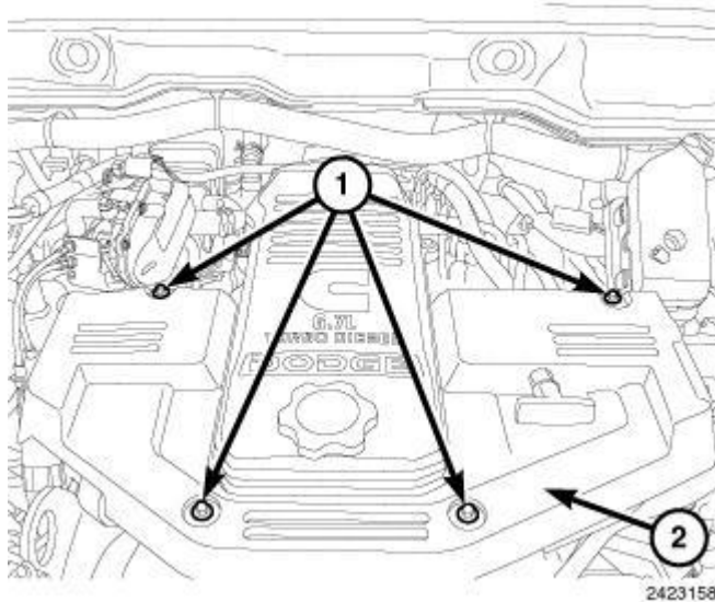
Fig. 31: Engine Cover Bolts Courtesy of CHRYSLER LLC
