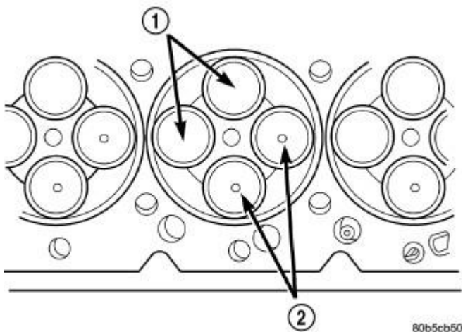
Fig. 99: Valve Identification Courtesy of CHRYSLER LLC
