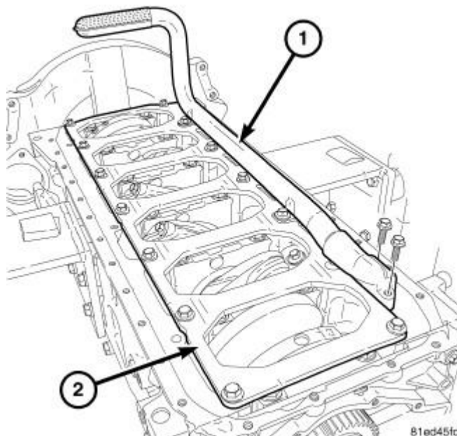
Fig. 171: Identifying Oil Pickup Tube
