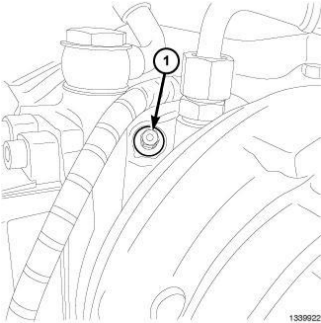
Fig. 297: Installing Turbocharger Cleaning Port Plug Courtesy of CHRYSLER LLC
