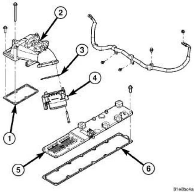
Fig. 64: Intake Air Heater Assembly Courtesy of CHRYSLER LLC
