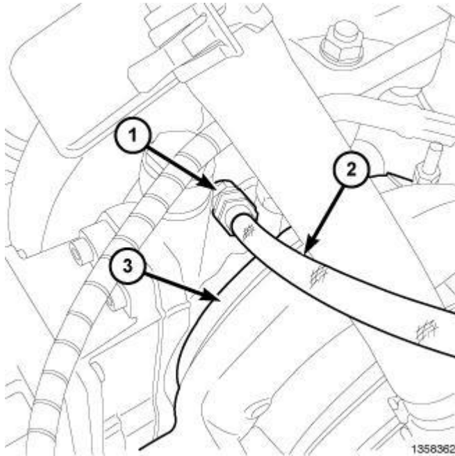
Fig. 305: Removing Nozzle, Cleaning Tool Hose & Turbocharger Courtesy of CHRYSLER LLC
