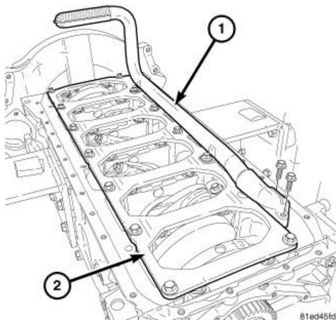
Fig. 351: Identifying Oil Pickup Tube
