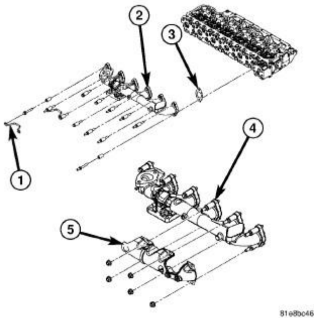
Fig. 290: Cylinder Head And Exhaust Manifold Courtesy of CHRYSLER LLC
