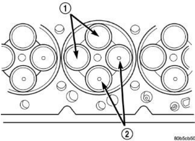
Fig. 89: Valve Identification Courtesy of CHRYSLER LLC
