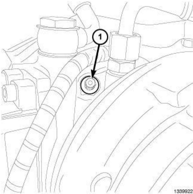
Fig. 304: Installing Turbocharger Cleaning Port Plug Courtesy of CHRYSLER LLC
