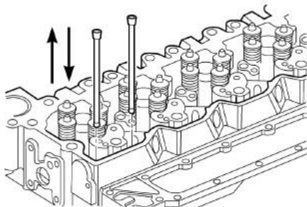
Fig. 81: Push Rod Removal/Installation
