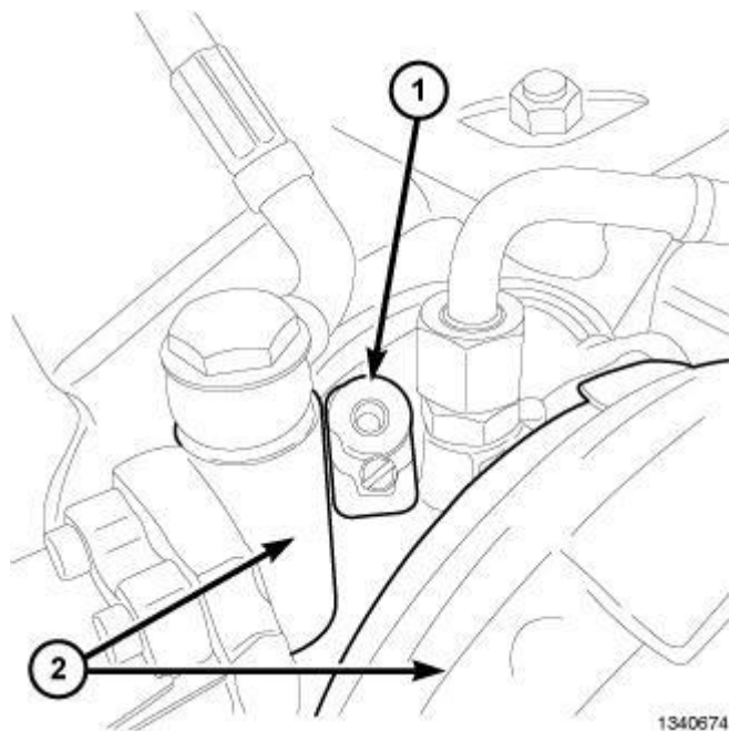
Fig. 301: Drill/Tap Guide Courtesy of CHRYSLER LLC
