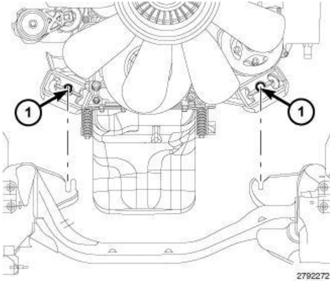
Fig. 198: Frame Mounts Courtesy of CHRYSLER LLC
