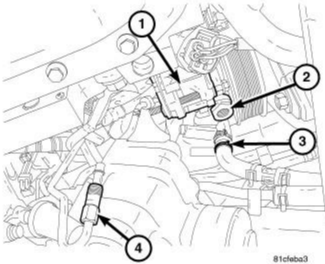
Fig. 139: Identifying Power Steering Pump, Pressure Line & Return Hose Courtesy of CHRYSLER LLC
