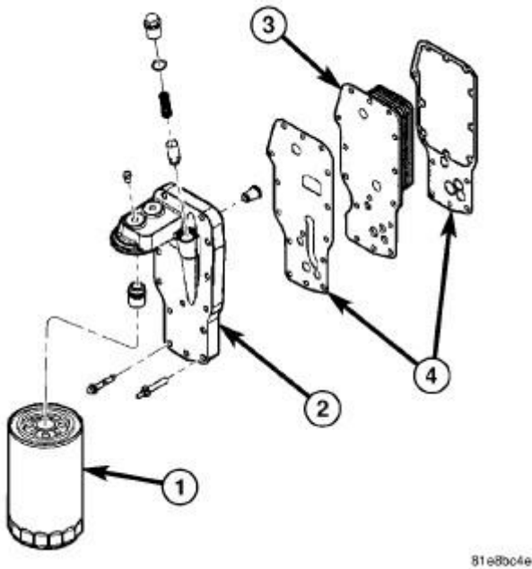
Fig. 255: Identifying Oil Filter And Cooler Courtesy of CHRYSLER LLC
