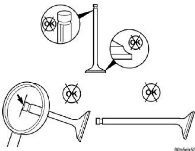
Fig. 93: Visually Inspect Valves For Abnormal Wear Courtesy of CHRYSLER LLC
