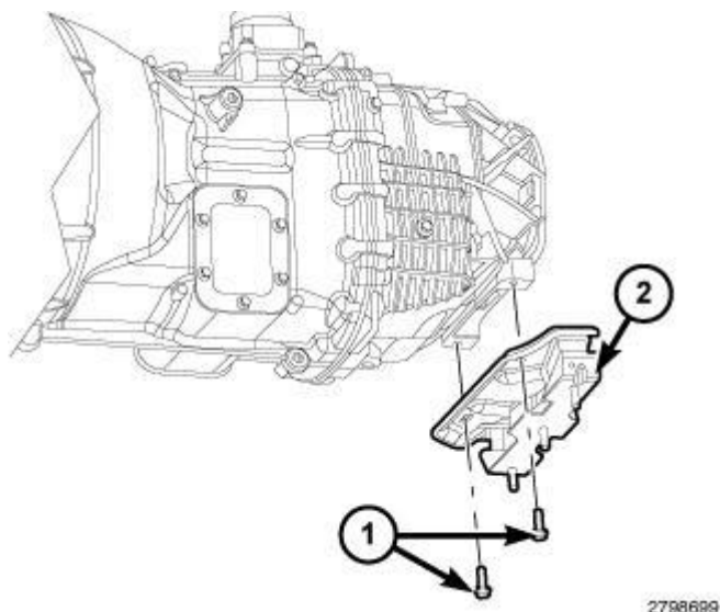
Fig. 211: Identifying Rear Transmission Mount & Bolts (M/T)
