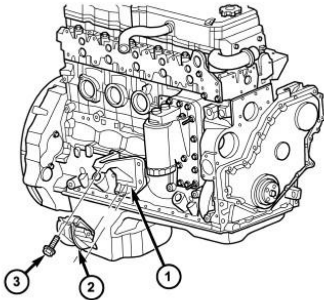
Fig. 258: RH Insulator Courtesy of CHRYSLER LLC
