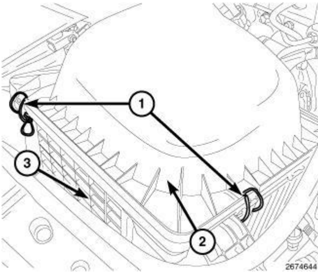
Fig. 34: Installing Air Cleaner Housing & Clips Courtesy of CHRYSLER LLC
