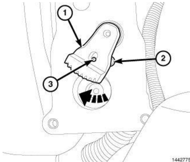
Fig. 313: Selector Gear - Rearward Position Courtesy of CHRYSLER LLC
