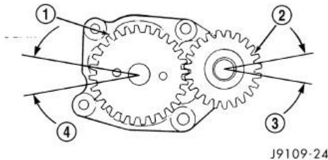
Fig. 284: Measure Gear Backlash Courtesy of CHRYSLER LLC
