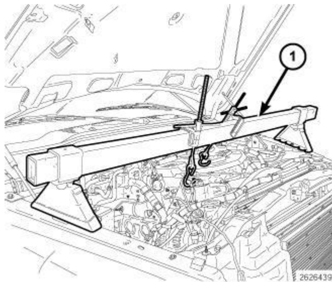
Fig. 327: Engine Support Fixture Tool 8534B Courtesy of CHRYSLER LLC
