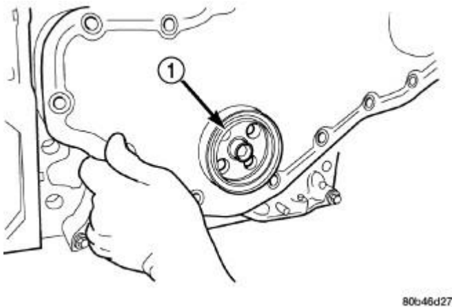
Fig. 340: Installing Front Cover With Seal Pilot
