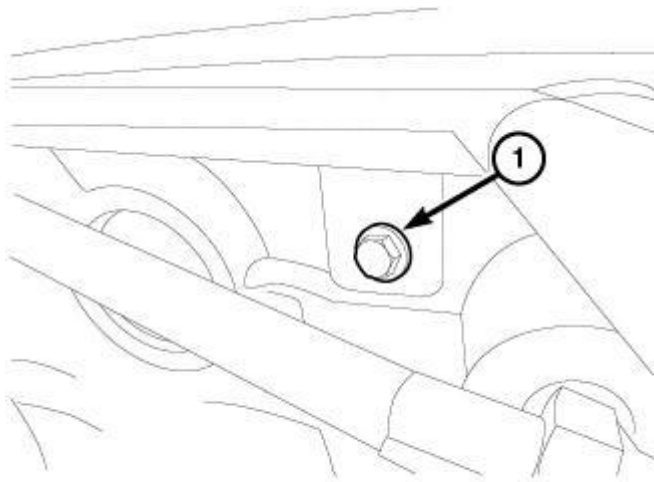
Fig. 247: Installing Coolant Outlet Tube Bracket Bolt Courtesy of CHRYSLER LLC
