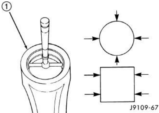
Fig. 166: Connecting Rod Pin Bore Courtesy of CHRYSLER LLC
