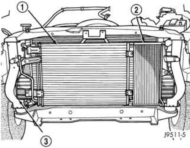
Fig. 343: Condenser And Transmission Auxiliary Cooler Courtesy of CHRYSLER LLC
