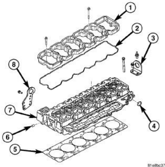
Fig. 172: Cylinder Head And Gasket Courtesy of CHRYSLER LLC
