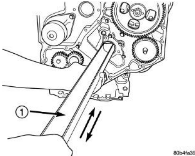
Fig. 184: Inserting The Trough Courtesy of CHRYSLER LLC
