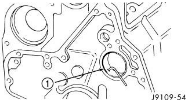
Fig. 114: Oil Hole Alignment Courtesy of CHRYSLER LLC
