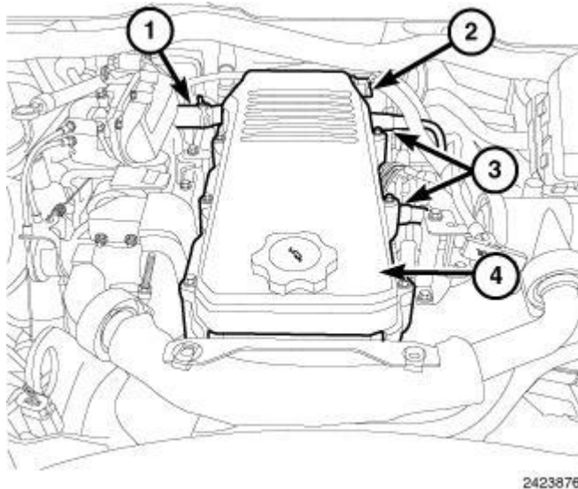
Fig. 72: Identifying CCV Tube, Crankcase Pressure Sensor Connector, CCV Oil Drains & Close Crankcase Ventilation (CCV) Cover Courtesy of CHRYSLER LLC
