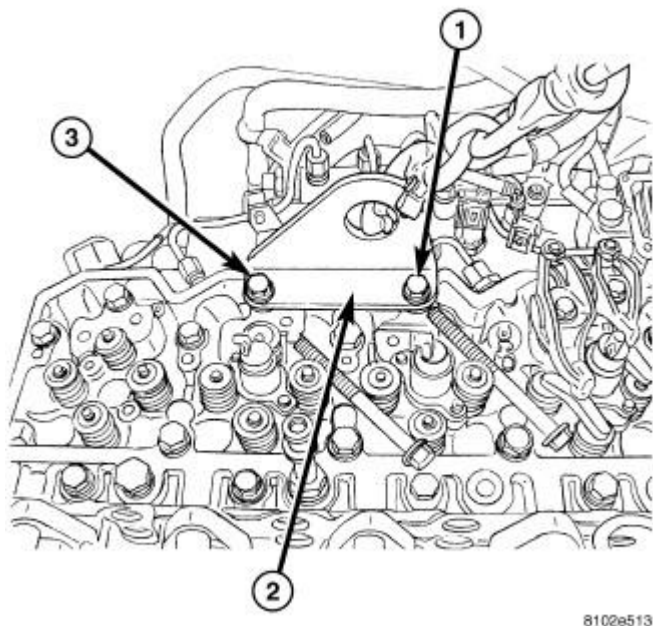
Fig. 17: Engine Lift Bracket Courtesy of CHRYSLER LLC
