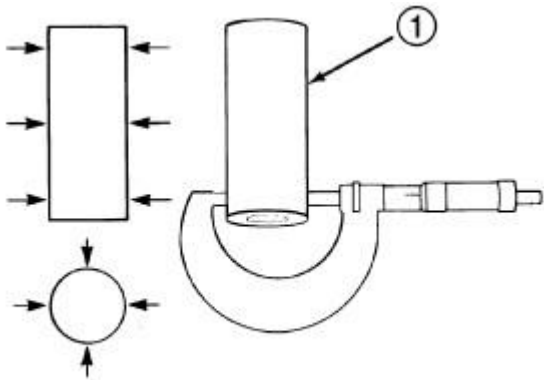
Fig. 165: Piston Pin Diameter Courtesy of CHRYSLER LLC
