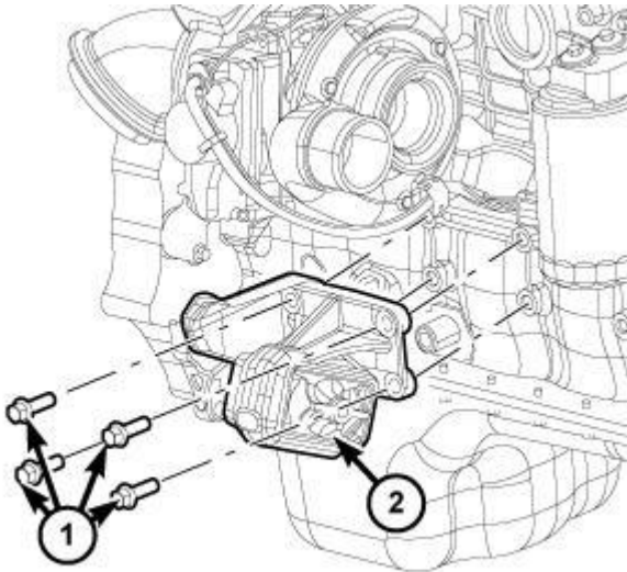
Fig. 196: RH Engine Mount Courtesy of CHRYSLER LLC
