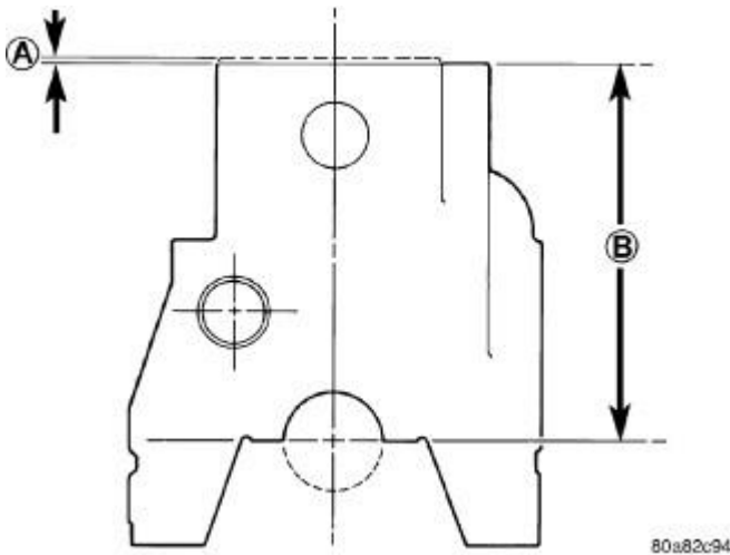
Fig. 110: Refacing Dimensions Of The Cylinder Block Courtesy of CHRYSLER LLC
