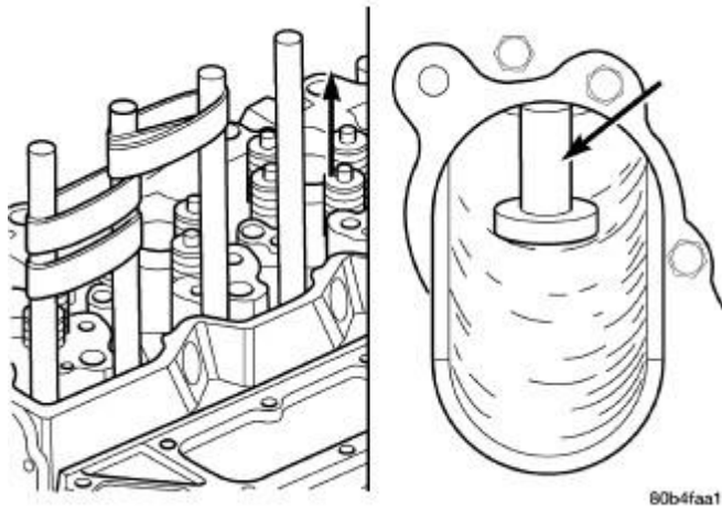
Fig. 186: Lift Dowel Rod To Disengage From Tappet Courtesy of CHRYSLER LLC
