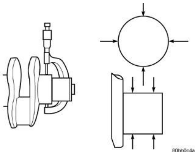
Fig. 119: Crankshaft Main Journal Diameter Courtesy of CHRYSLER LLC
