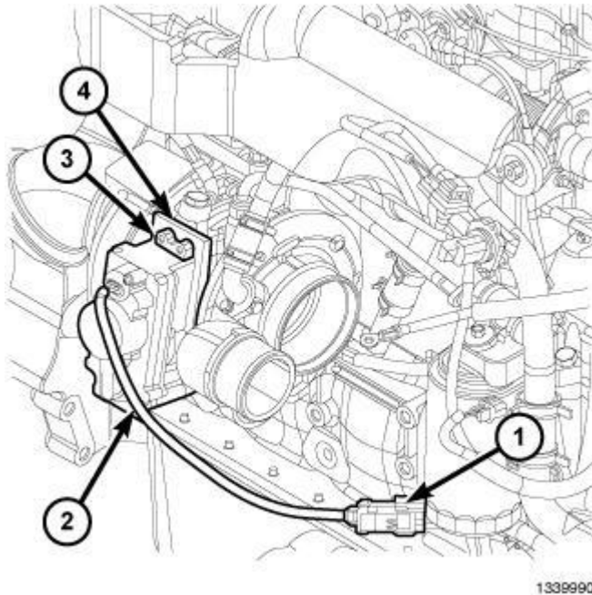
Fig. 299: Turbocharger Actuator Electrical Connector Courtesy of CHRYSLER LLC
