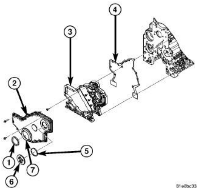
Fig. 349: Front Cover Courtesy of CHRYSLER LLC
