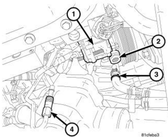
Fig. 27: Identifying Power Steering Pump, Pressure Line & Return Hose Courtesy of CHRYSLER LLC
