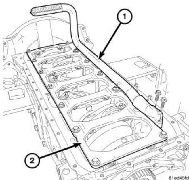
Fig. 159: Identifying Oil Pickup Tube Courtesy of CHRYSLER LLC
