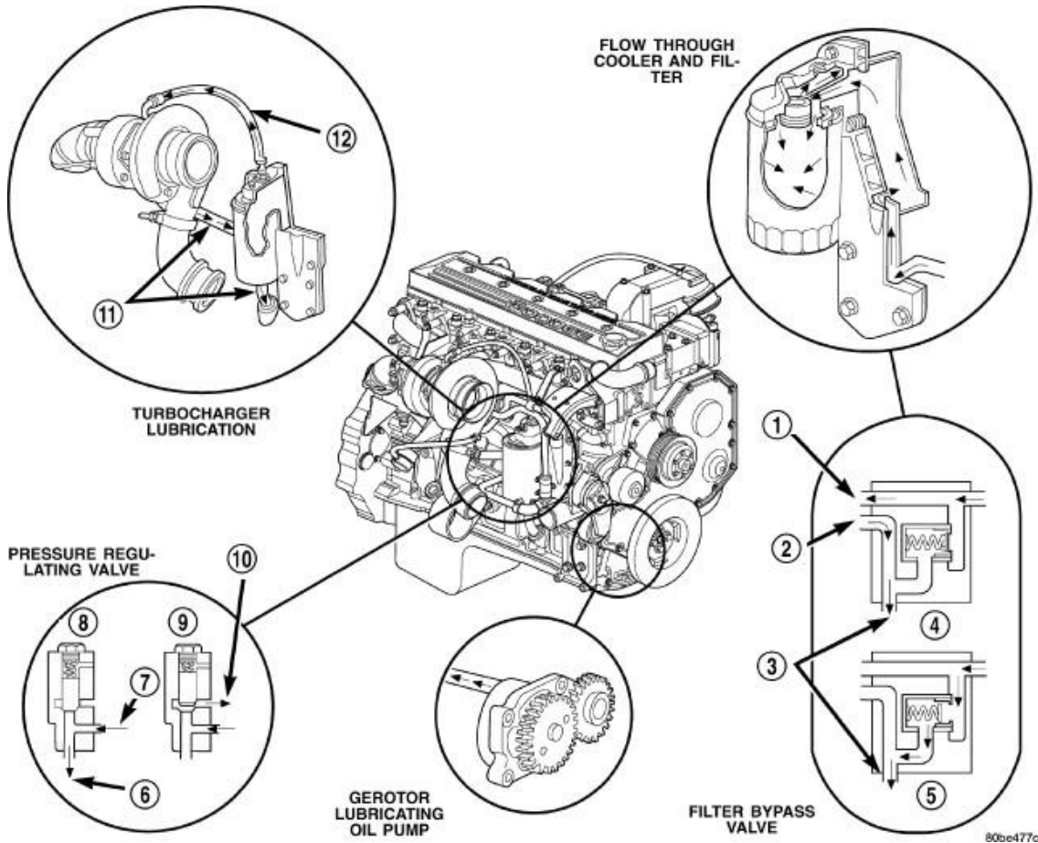
Fig. 224: Lubrication System Circulation (1 Of 2) Courtesy of CHRYSLER LLC
