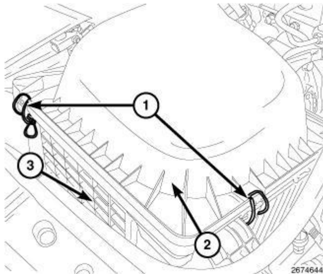
Fig. 38: Installing Air Cleaner Housing & Clips Courtesy of CHRYSLER LLC
