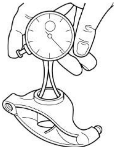
Fig. 82: Measuring Rocker Arm Bore Courtesy of CHRYSLER LLC
