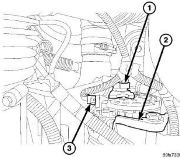
Fig. 228: Diesel Generator Connectors Courtesy of CHRYSLER LLC
