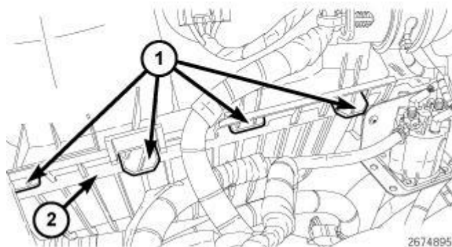
Fig. 37: Identifying Air Cleaner Cover Alignment Tabs & Housing Slots Courtesy of CHRYSLER LLC
