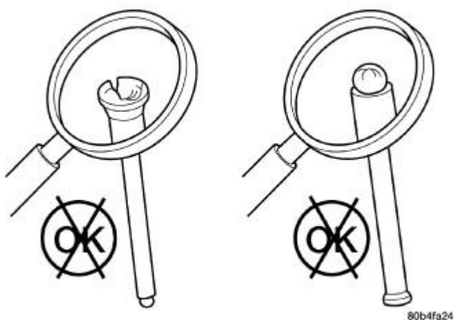
Fig. 84: Inspecting Push Rod For Cracks Courtesy of CHRYSLER LLC
