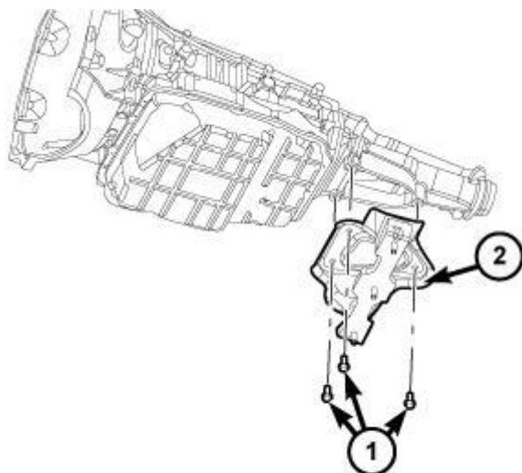
Fig. 222: Identifying Rear Transmission Mount & Bolts - 68RFE A/T - 4X2 Regular Cab Models Courtesy of CHRYSLER LLC
