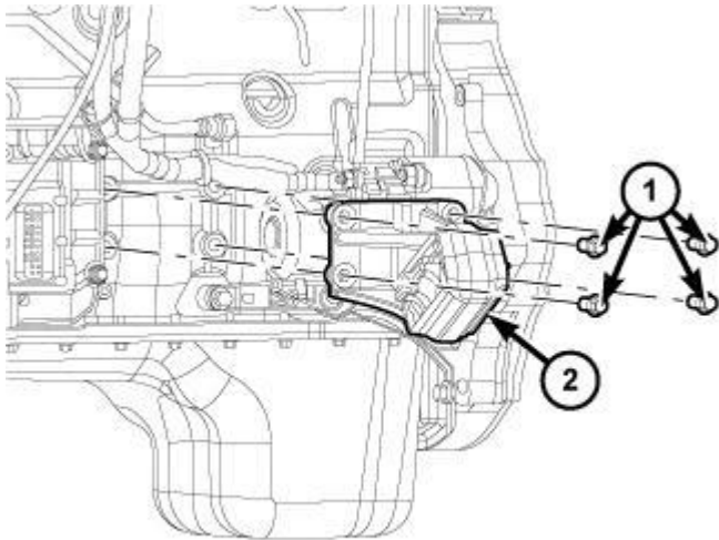
Fig. 197: LH Engine Mount Courtesy of CHRYSLER LLC
