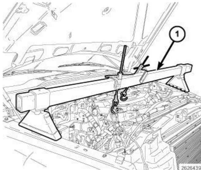
Fig. 335: Engine Support Fixture Tool 8534B Courtesy of CHRYSLER LLC
