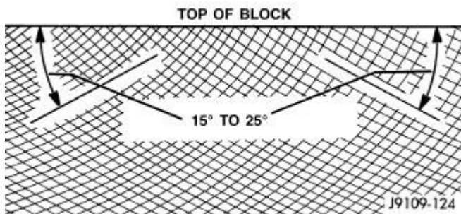
Fig. 111: Cylinder Bore Crosshatch Pattern
