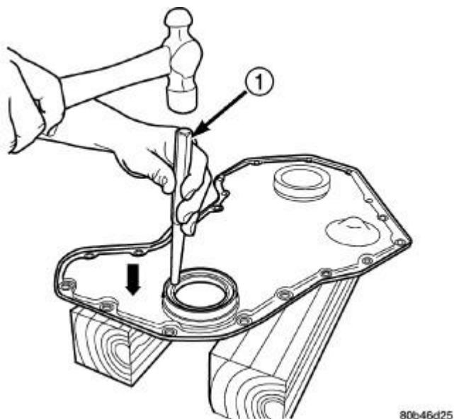
Fig. 176: Removing Seal From Cover Courtesy of CHRYSLER LLC
