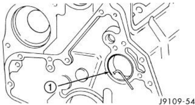
Fig. 130: Oil Hole Alignment Courtesy of CHRYSLER LLC
