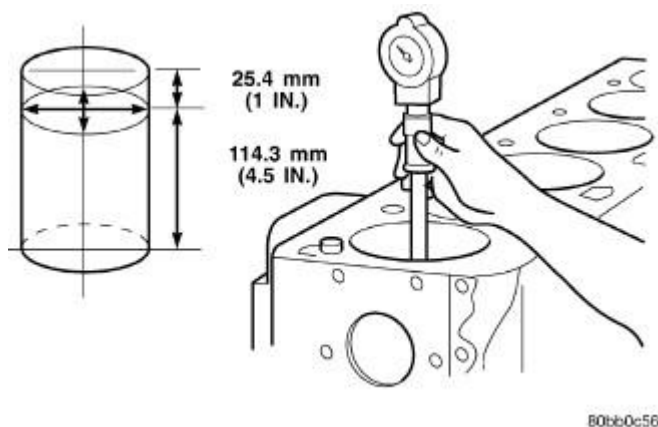
Fig. 116: Cylinder Bore Diameter Courtesy of CHRYSLER LLC
