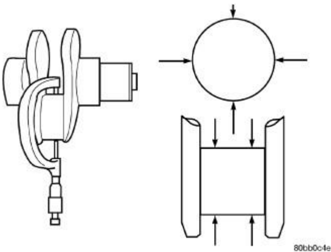
Fig. 117: Connecting Rod Journal Diameter Limits Courtesy of CHRYSLER LLC
