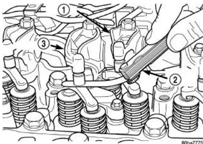
Fig. 103: Measuring Valve Lash Courtesy of CHRYSLER LLC
