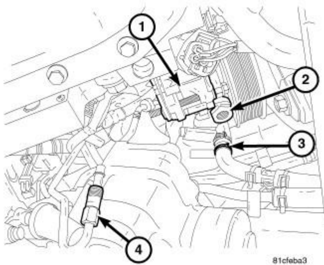
Fig. 179: Identifying Power Steering Pump, Pressure Line & Return Hose Courtesy of CHRYSLER LLC
