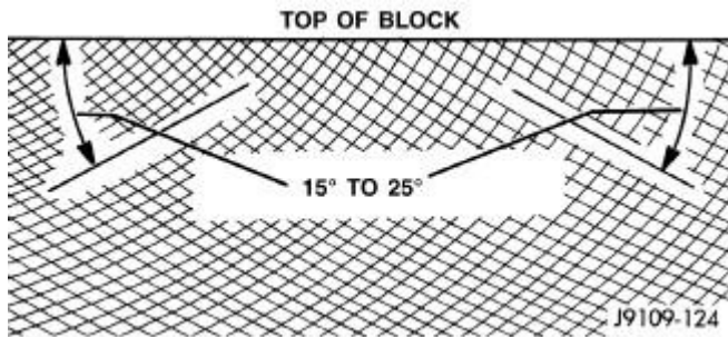
Fig. 111: Cylinder Bore Crosshatch Pattern Courtesy of CHRYSLER GROUP, LLC
