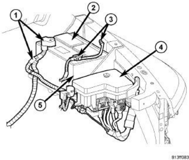
Fig. 226: Battery Cables
