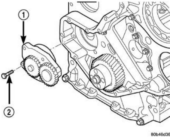
Fig. 279: Oil Pump & Bolts Courtesy of CHRYSLER GROUP, LLC
