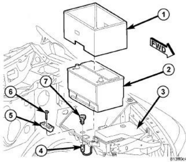
Fig. 69: Battery & Components Courtesy of CHRYSLER GROUP, LLC
