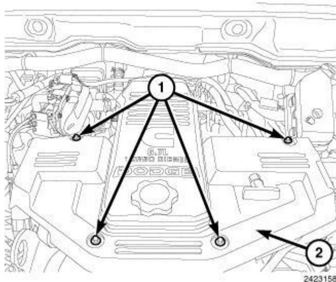
Fig. 31: Engine Cover & Bolts
