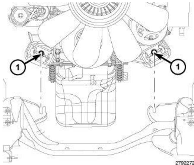
Fig. 203: Frame Mount Fasteners
