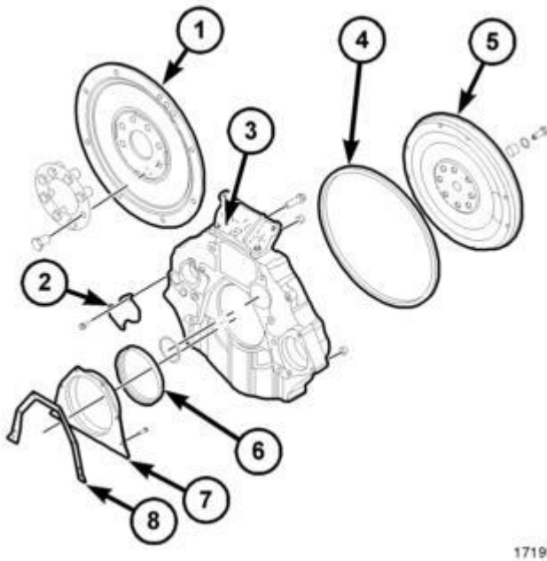
Fig. 18: Flywheel Housing, Adapter Plates & Rear Oil Seal Courtesy of CHRYSLER GROUP, LLC
