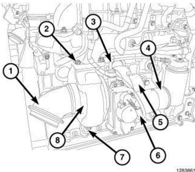
Fig. 326: Turbocharger Components Courtesy of CHRYSLER GROUP, LLC
