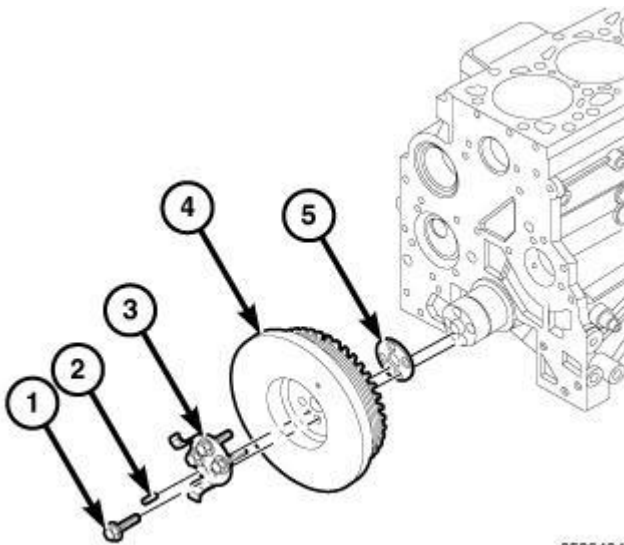
Fig. 148: Crankshaft Damper (High Output Engine)
