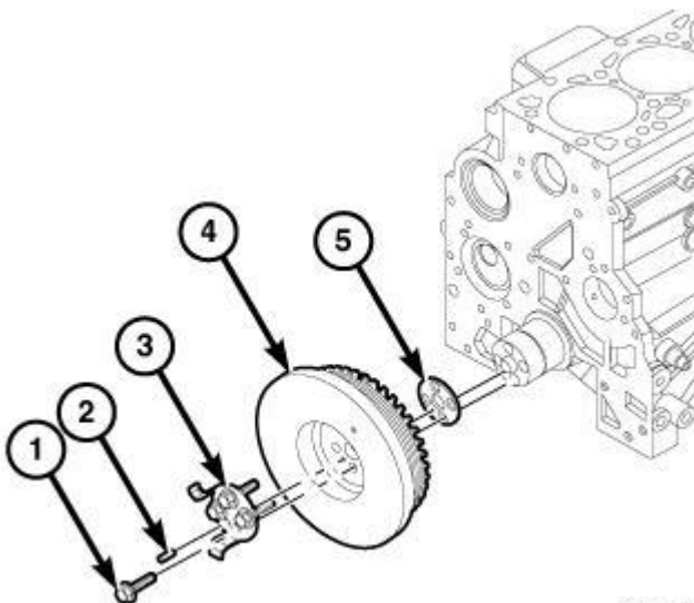
Fig. 145: Crankshaft Damper (High Output Engine)
