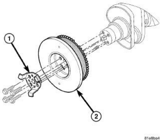
Fig. 122: Crankshaft Damper (Non-High Output Engine)
