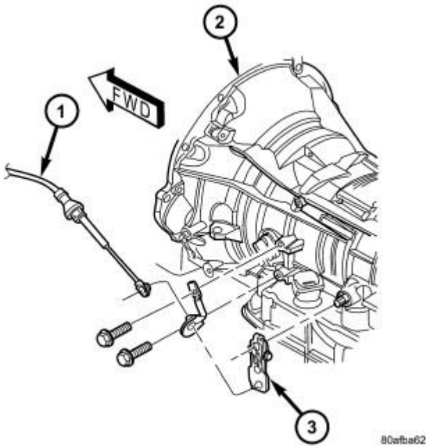
Fig. 269: Gearshift Cable, RFE Transmission & Manual Lever Courtesy of CHRYSLER GROUP, LLC
