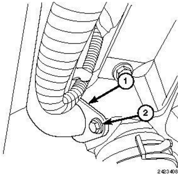
Fig. 237: Front Coolant Tube & Bolt
