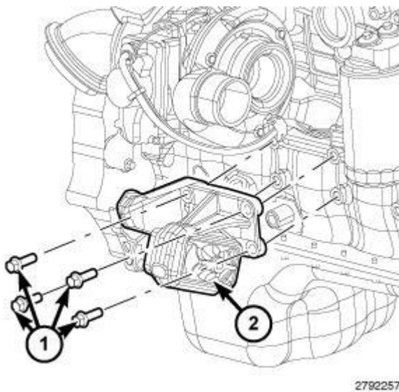
Fig. 199: RH Engine Mount & Bolts
