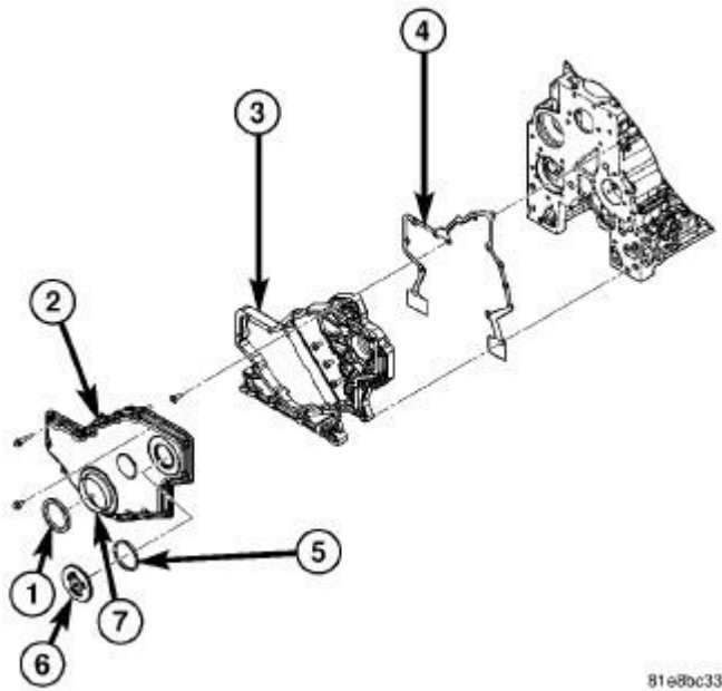
Fig. 123: Front Cover Assembly Components
