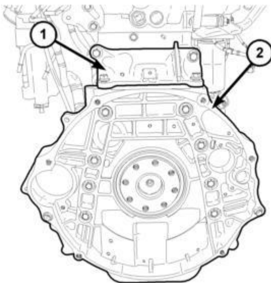
Fig. 24: Flywheel Housing & Collar Courtesy of CHRYSLER GROUP, LLC
