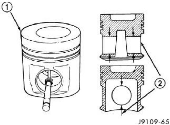
Fig. 164: Piston & Pin Bore
