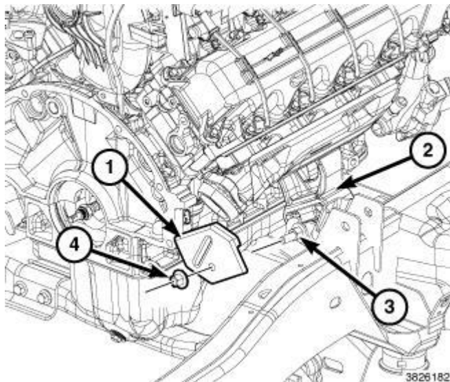
Fig. 248: Engine Mount, Heat Shield & Fasteners
