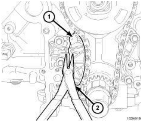
Fig. 336: Retracting Tensioner Shoe Using Pliers Courtesy of CHRYSLER GROUP, LLC
