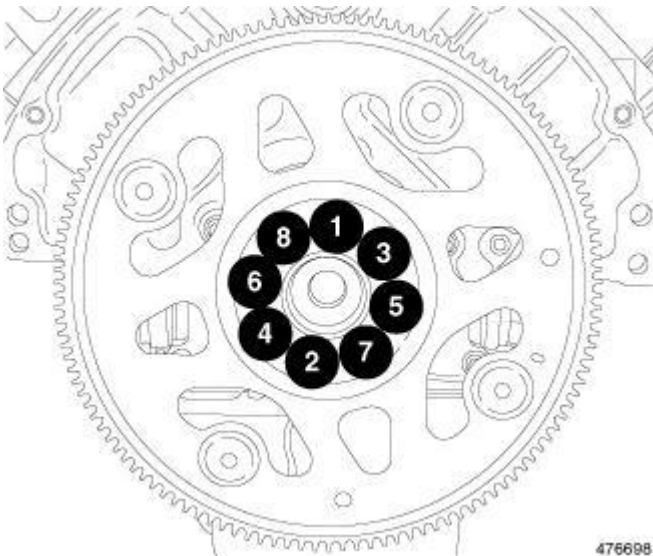
Fig. 183: Flexplate Retaining Bolt Removal & Tightening Sequence Courtesy of CHRYSLER GROUP, LLC
