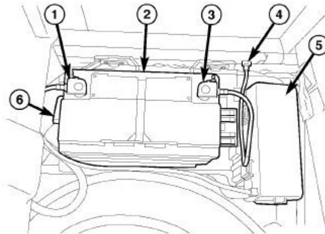
Fig. 218: Battery System Components & PDC Cover
