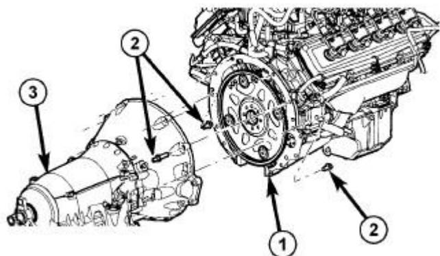
Fig. 16: Remove/Install Transmission To Engine Bolts Courtesy of CHRYSLER GROUP, LLC
