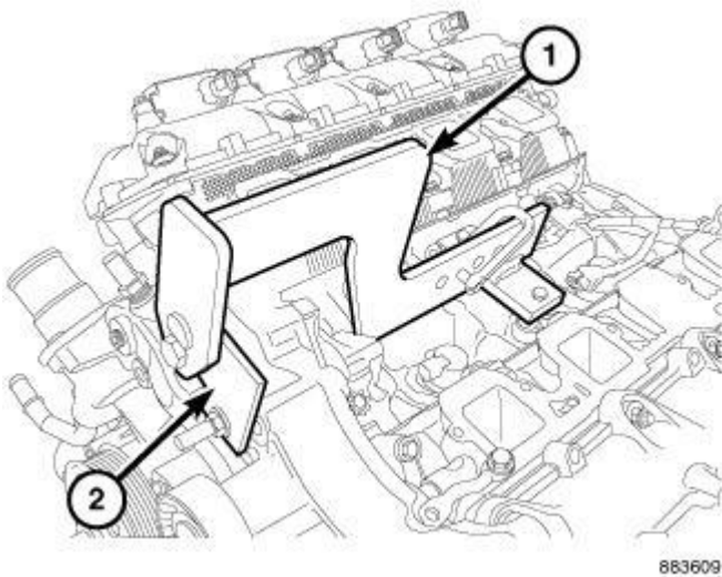
Fig. 19: Engine Lift Fixture & Adapter Courtesy of CHRYSLER GROUP, LLC
