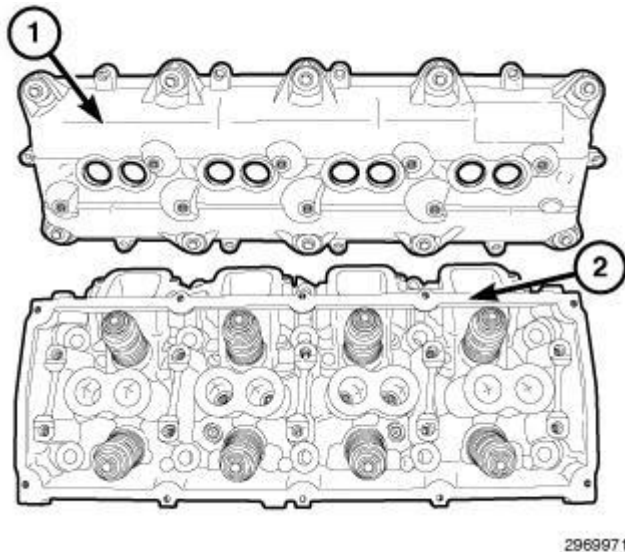
Fig. 83: Cylinder Head & Cover Courtesy of CHRYSLER GROUP, LLC
