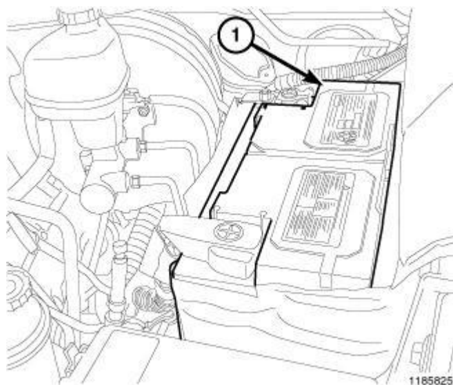
Fig. 332: Negative Battery Cable Courtesy of CHRYSLER GROUP, LLC
