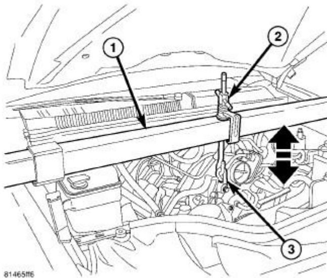
Fig. 285: Engine Support Tool Courtesy of CHRYSLER GROUP, LLC
