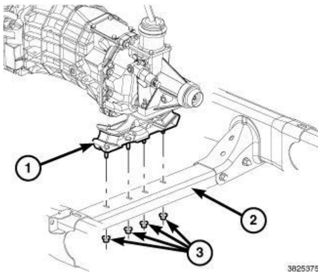
Fig. 229: Transmission Mount, Crossmember & Nuts
