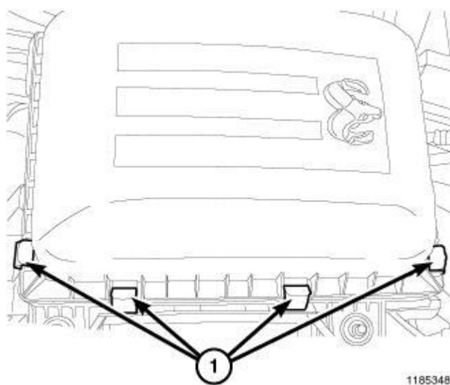
Fig. 55: Air Cleaner Body Cover Retaining Clamps Courtesy of CHRYSLER GROUP, LLC
