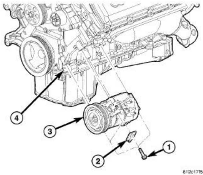
Fig. 34: A/C Compressor & Fasteners Courtesy of CHRYSLER GROUP, LLC
