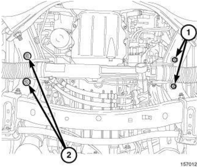
Fig. 203: Engine Mount Nuts Courtesy of CHRYSLER GROUP, LLC
