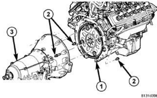
Fig. 22: Remove/Install Transmission To Engine Bolts
