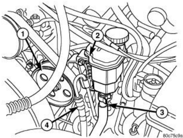
Fig. 31: Power Steering Pulley, Reservoir & Hoses
