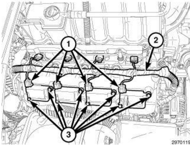
Fig. 81: Ignition Coil Electrical Connectors, Harness & Bolts Courtesy of CHRYSLER GROUP, LLC
