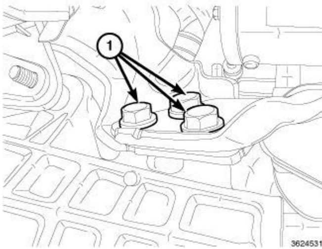
Fig. 257: Engine Bracket Bolts Courtesy of CHRYSLER GROUP, LLC
