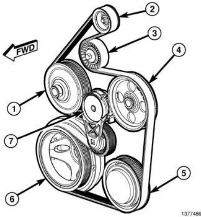
Fig. 36: Accessory Drive Belt Routing, Tensioner & Pulleys Courtesy of CHRYSLER GROUP, LLC
