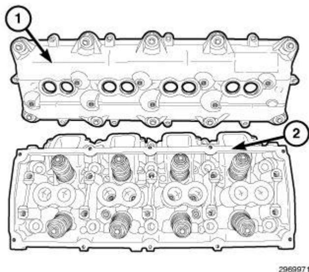
Fig. 84: Cylinder Head & Cover
