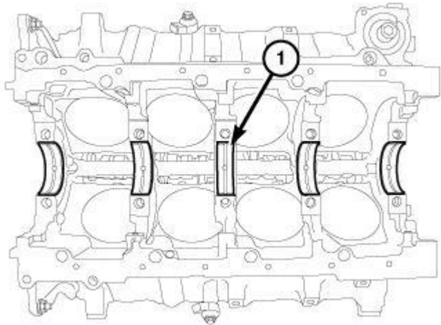
Fig. 167: Main Bearings
