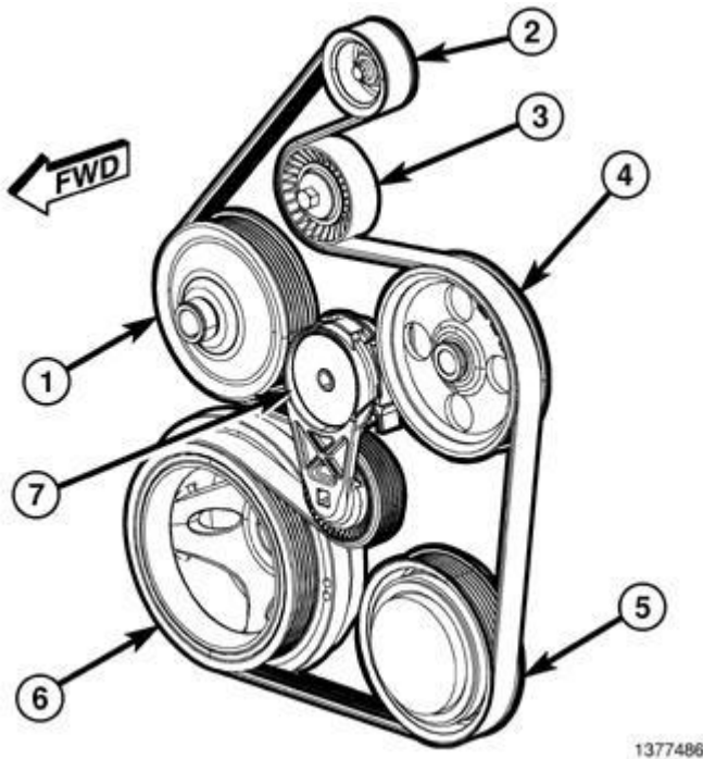
Fig. 5: Accessory Drive Belt Routing, Tensioner & Pulleys Courtesy of CHRYSLER GROUP, LLC
