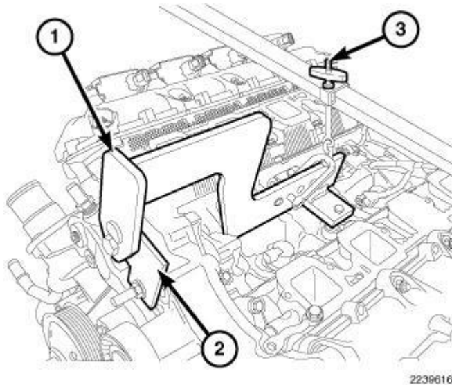
Fig. 205: Engine Lift Fixture & Adapter Courtesy of CHRYSLER GROUP, LLC
