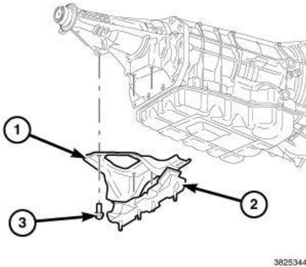
Fig. 227: Transmission Mounting Bracket, Insulator & Bolts Courtesy of CHRYSLER GROUP, LLC
