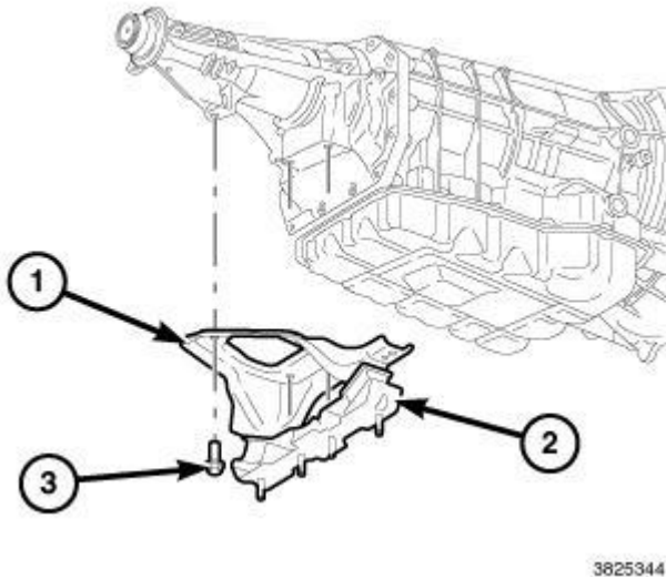
Fig. 228: Transmission Mounting Bracket, Insulator & Bolts Courtesy of CHRYSLER GROUP, LLC
