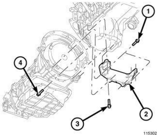
Fig. 278: Structural Cover
