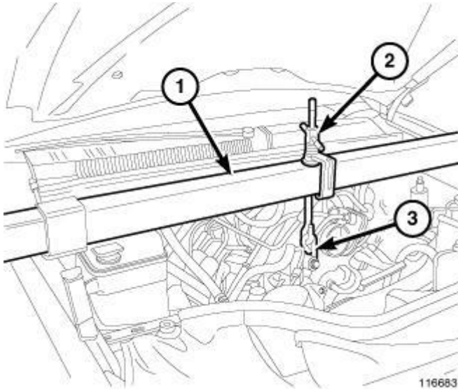
Fig. 233: Engine Support Tool Courtesy of CHRYSLER GROUP, LLC
