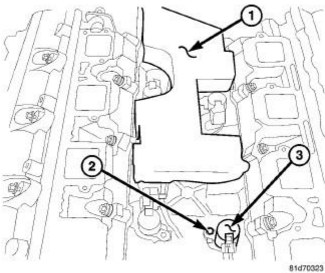
Fig. 222: Intake Manifold Foam Insulator Pad, MDS Solenoids & Bolts Courtesy of CHRYSLER GROUP, LLC
