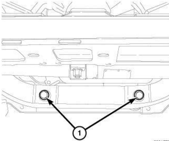
Fig. 152: Steering Rack To Frame Mounting Bolts Courtesy of CHRYSLER GROUP, LLC
