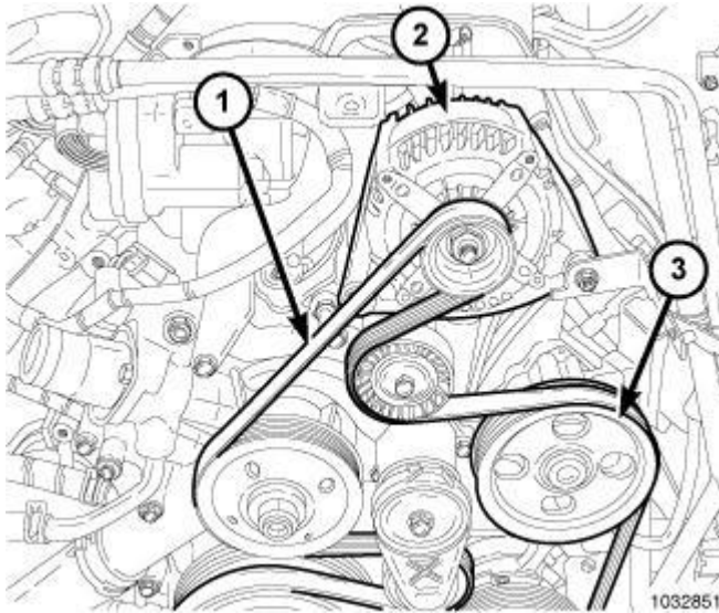
Fig. 181: Accessory Drive Belt Routing, Generator & Power Steering Pump Courtesy of CHRYSLER GROUP, LLC
