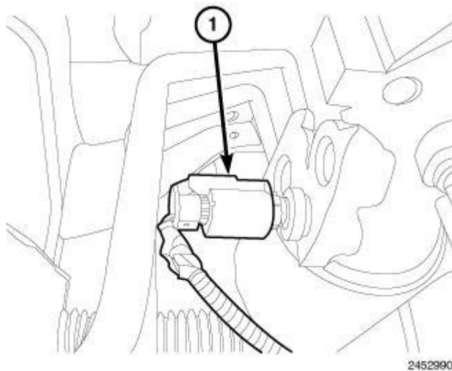
Fig. 298: Oil Temperature Sensor Electrical Connector Courtesy of CHRYSLER GROUP, LLC
