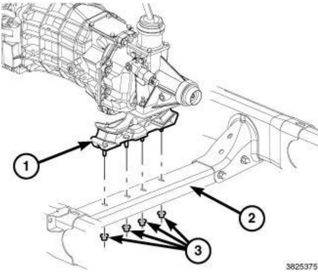
Fig. 226: Transmission Mount, Crossmember & Nuts Courtesy of CHRYSLER GROUP, LLC
