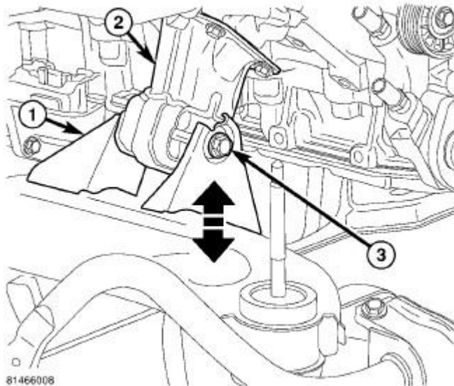
Fig. 311: Engine Mount & Bolt
