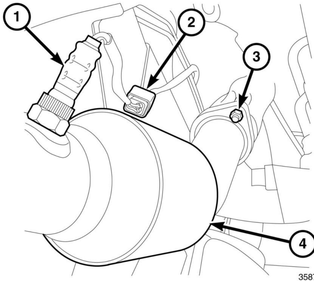
Fig. 312: Oxygen Sensor, Oxygen Sensor Connector, Ball Flange Nut & LH Catalytic Converter Courtesy of CHRYSLER GROUP, LLC
