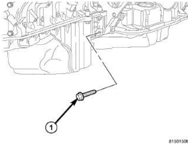
Fig. 15: Oil Pan To Transmission Bolts Courtesy of CHRYSLER GROUP, LLC
