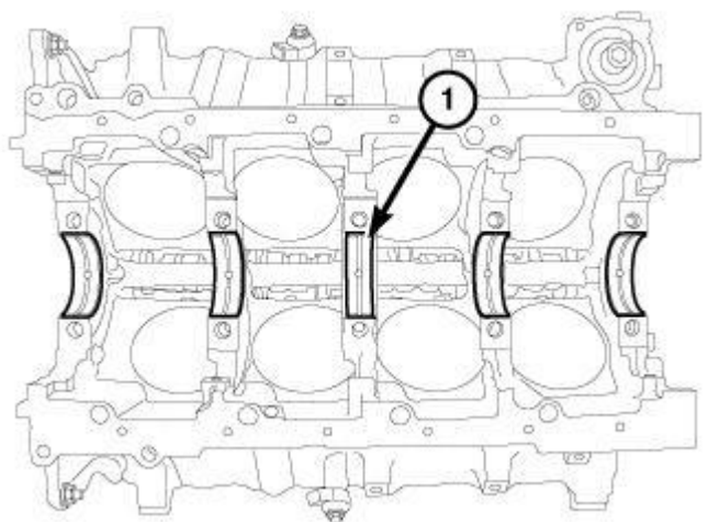
Fig. 167: Main Bearings
