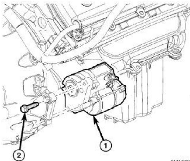
Fig. 27: Starter & Fasteners
