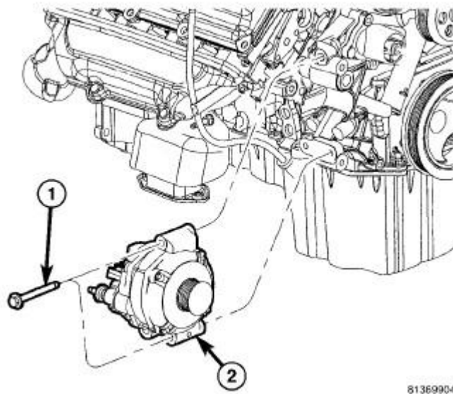
Fig. 33: Generator & Fasteners Courtesy of CHRYSLER GROUP, LLC
