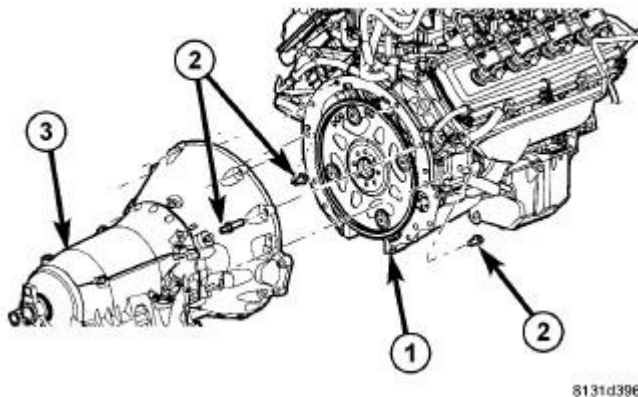
Fig. 16: Remove/Install Transmission To Engine Bolts Courtesy of CHRYSLER GROUP, LLC
