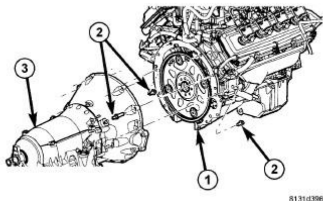
Fig. 20: Remove/Install Transmission To Engine Bolts Courtesy of CHRYSLER GROUP, LLC
