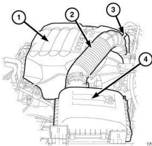
Fig. 49: Engine Cover, Clean Air Hose, Intake Air Temperature (IAT) Sensor Electrical Connector & Air Cleaner Housing Courtesy of CHRYSLER GROUP, LLC
