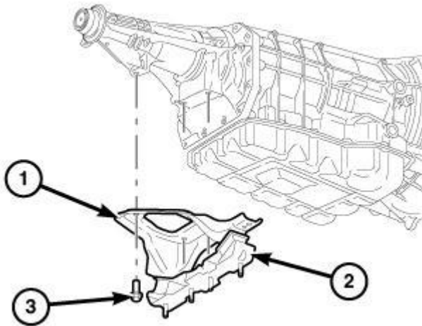
Fig. 227: Transmission Mounting Bracket, Insulator & Bolts Courtesy of CHRYSLER GROUP, LLC
