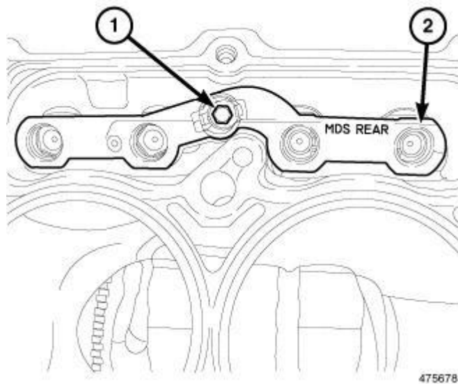
Fig. 147: Rear MDS Lifter Assembly Courtesy of CHRYSLER GROUP, LLC
