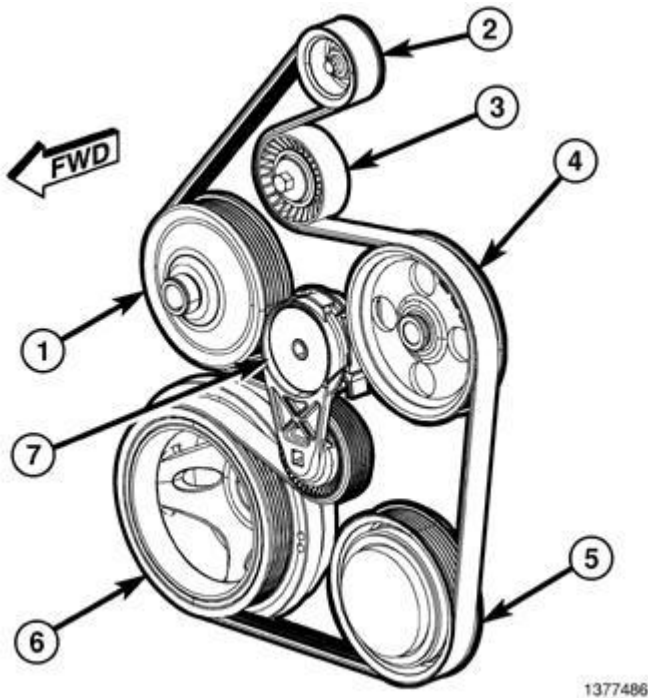
Fig. 5: Accessory Drive Belt Routing, Tensioner & Pulleys Courtesy of CHRYSLER GROUP, LLC
