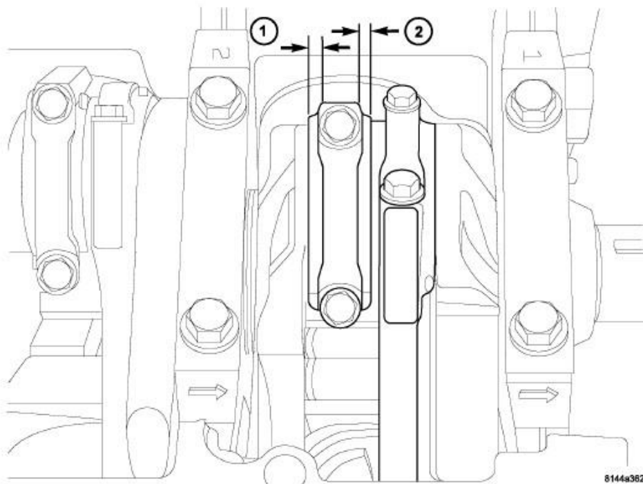
Fig. 212: Identifying Connecting Rod Proper Installation
