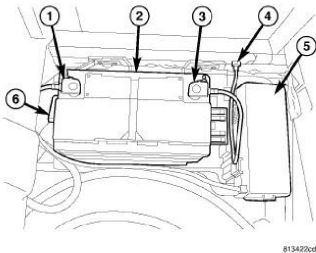
Fig. 200: Battery System Components & PDC Cover Courtesy of CHRYSLER GROUP, LLC
