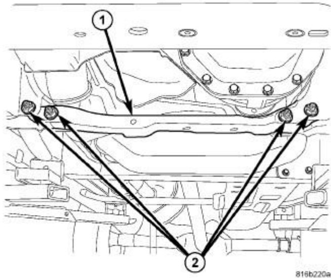
Fig. 258: Suspension Crossmember & Bolts
