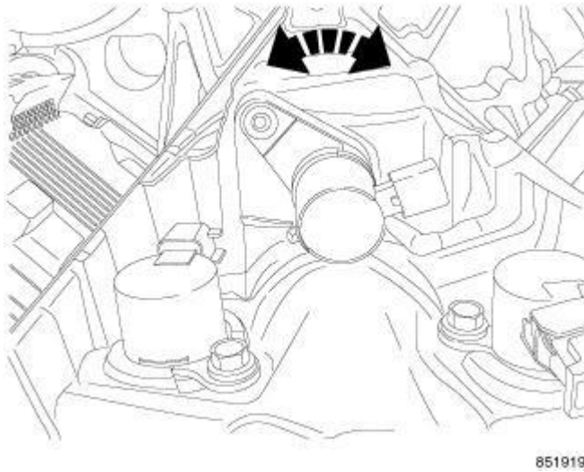
Fig. 274: Removing/Installing OCV Courtesy of CHRYSLER GROUP, LLC
