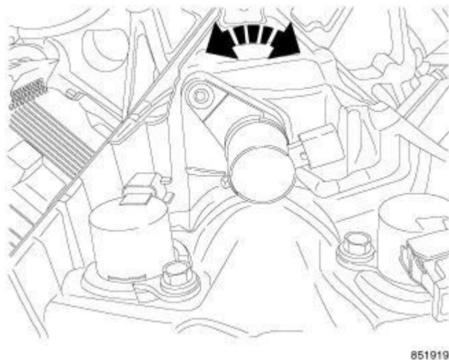
Fig. 274: Removing/Installing OCV
