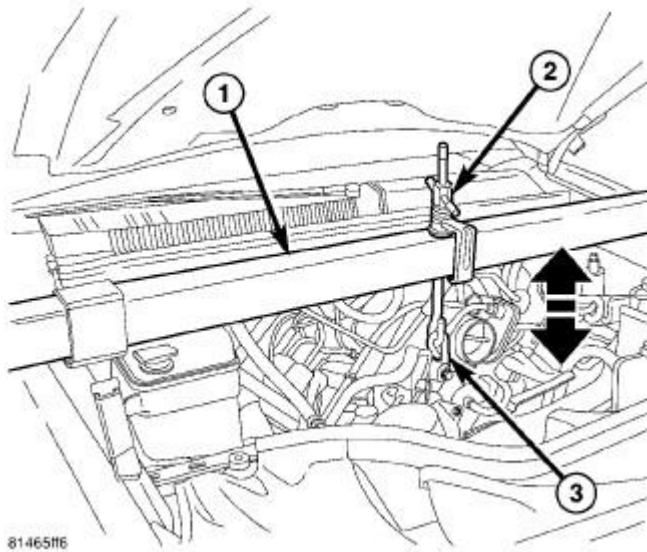
Fig. 279: Engine Support Tool
