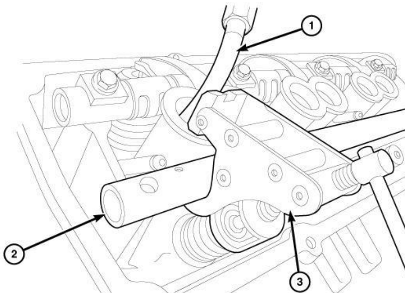
Fig. 114: Valve Spring Compressor Courtesy of CHRYSLER GROUP, LLC
