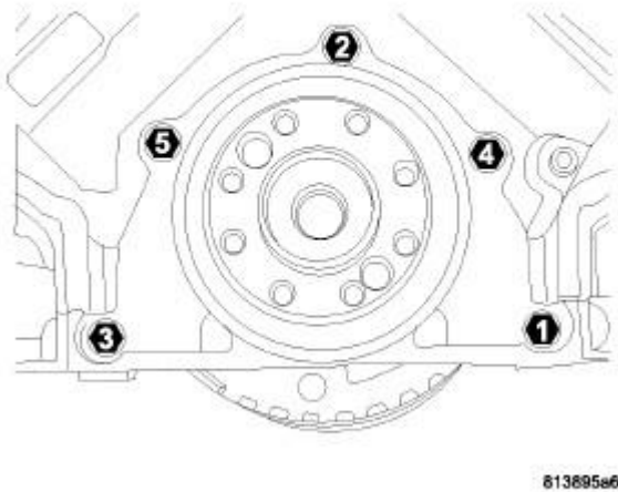
Fig. 191: Rear Seal Retainer Removal/Tightening Sequence Courtesy of CHRYSLER GROUP, LLC
