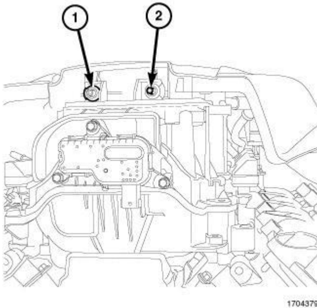
Fig. 318: Engine Cover Pegs & Grommets
