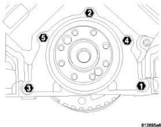
Fig. 192: Rear Seal Retainer Removal/Tightening Sequence
