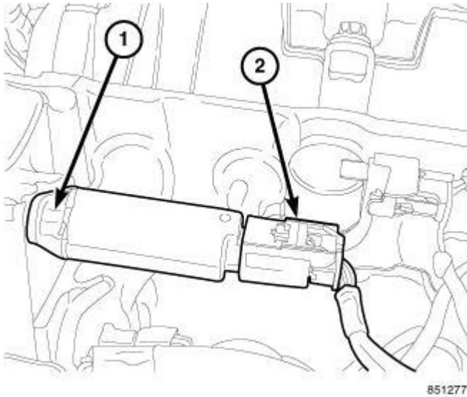
Fig. 275: Oil Control Valve Courtesy of CHRYSLER GROUP, LLC
