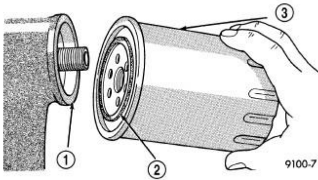
Fig. 276: Installing Engine Oil Filter Courtesy of CHRYSLER GROUP, LLC
