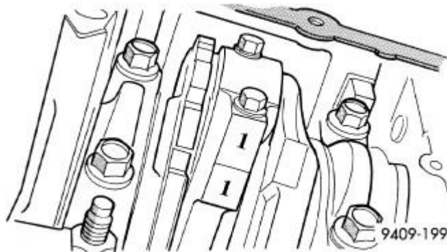
Fig. 163: Mark On Connecting Rod & Bearing Cap Courtesy of CHRYSLER GROUP, LLC
