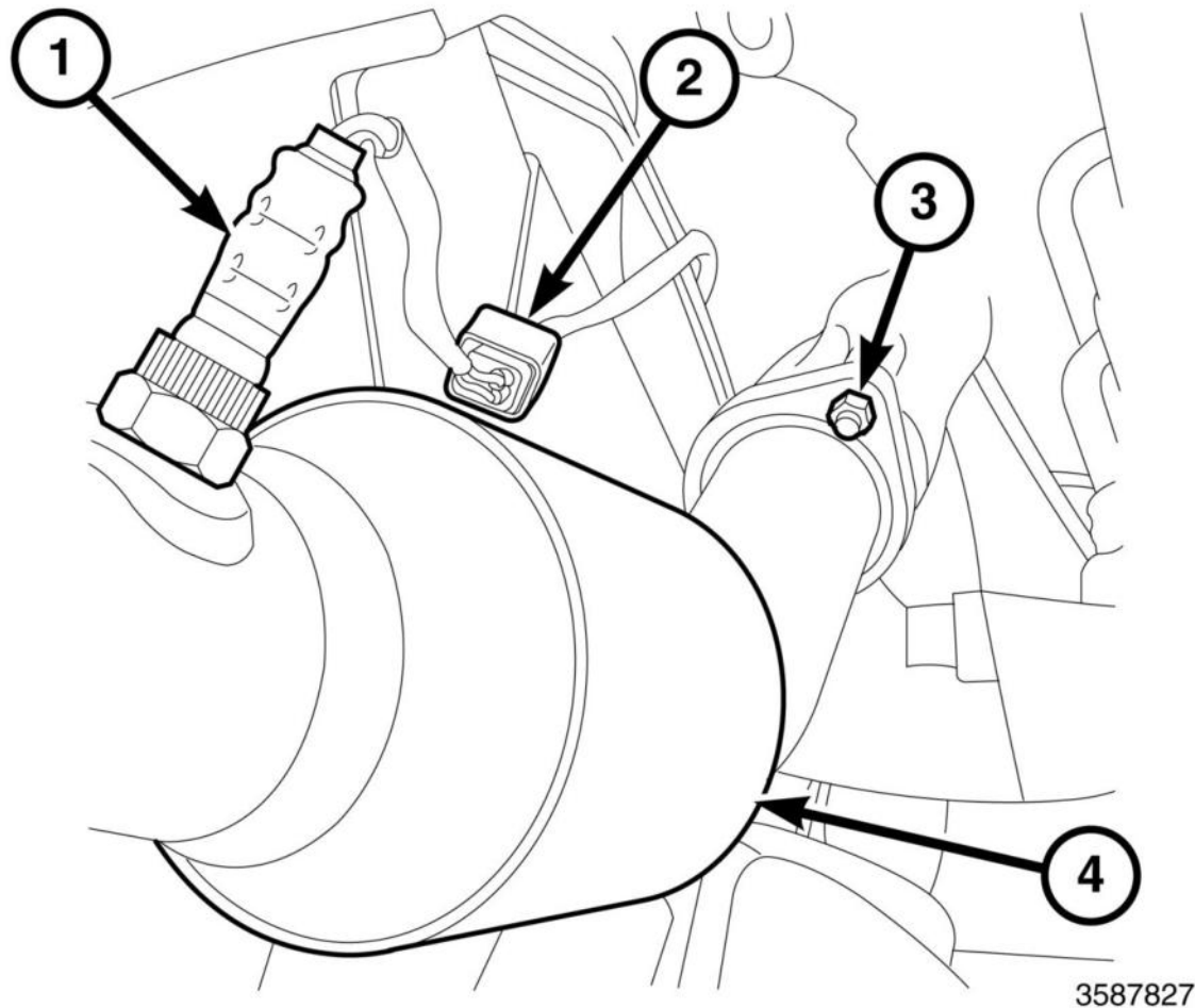
Fig. 302: Oxygen Sensor, Oxygen Sensor Connector, Ball Flange Nut & LH Catalytic Converter Courtesy of CHRYSLER GROUP, LLC
