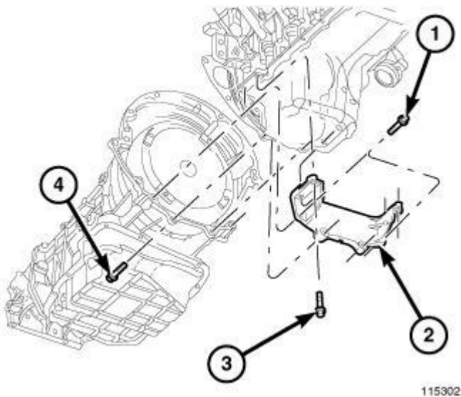
Fig. 155: Structural Cover
