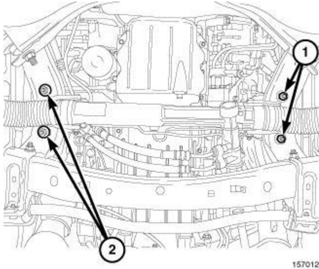
Fig. 203: Engine Mount Nuts
