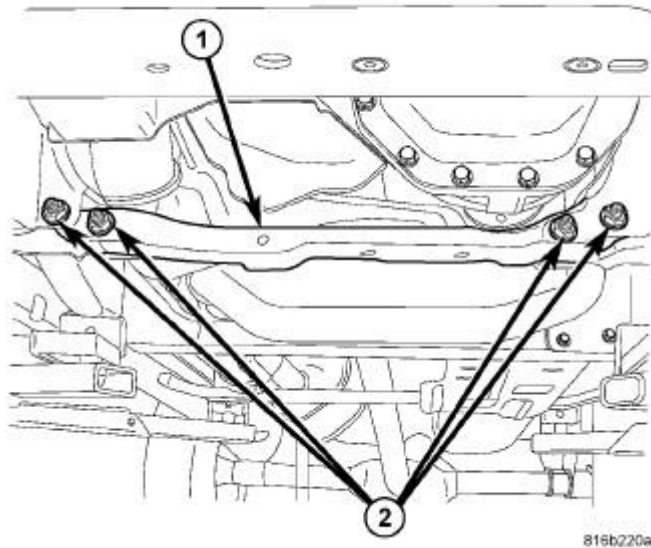
Fig. 269: Suspension Crossmember & Bolts Courtesy of CHRYSLER GROUP, LLC
