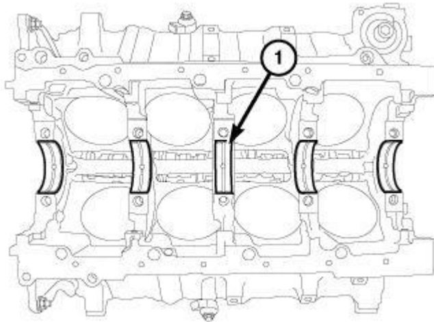
Fig. 167: Main Bearings
