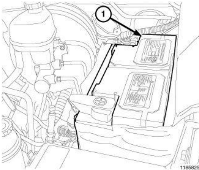
Fig. 4: Battery
