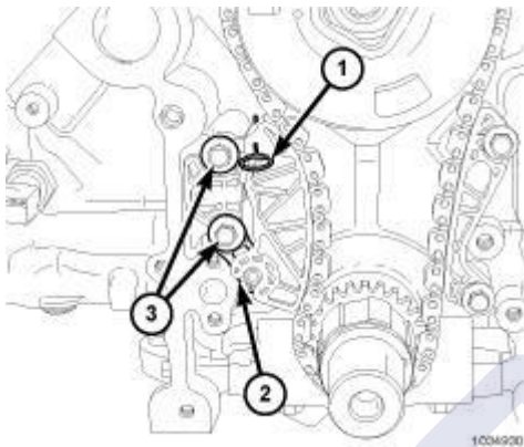
Fig. 351: Timing Chain Tensioner Pin & Bolts
