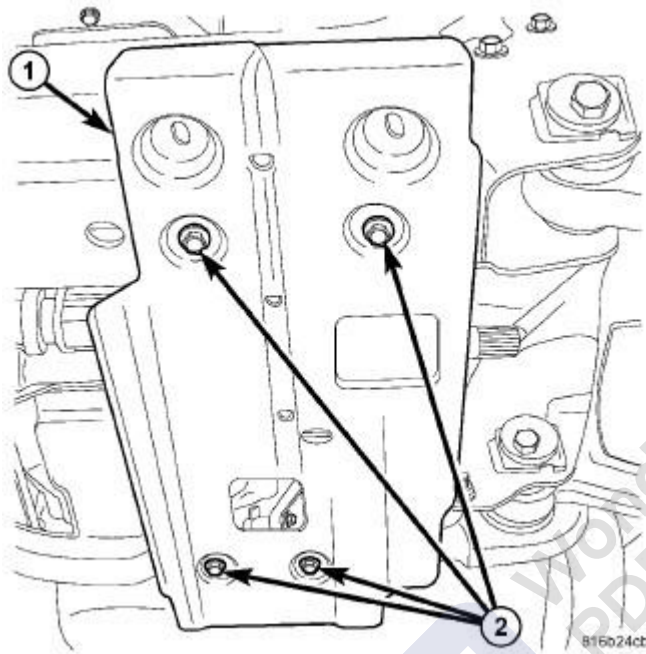
Fig. 233: Skid Plate And Bolts Courtesy of CHRYSLER GROUP, LLC
