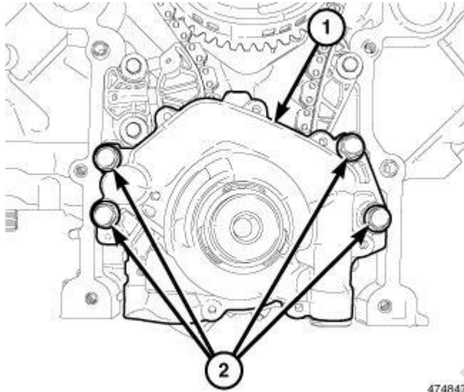
Fig. 175: Oil Pump Retaining Bolts
