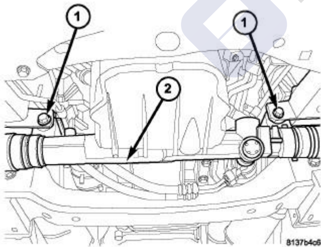
Fig. 205: Gear Mounting Bolts & Steering Gear
