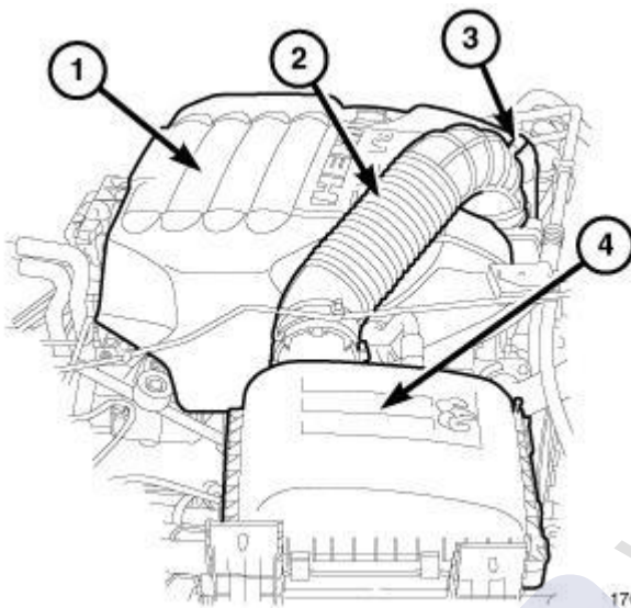
Fig. 366: Engine Cover, Clean Air Hose, Intake Air Temperature (IAT) Sensor Electrical Connector & Air Cleaner Housing
