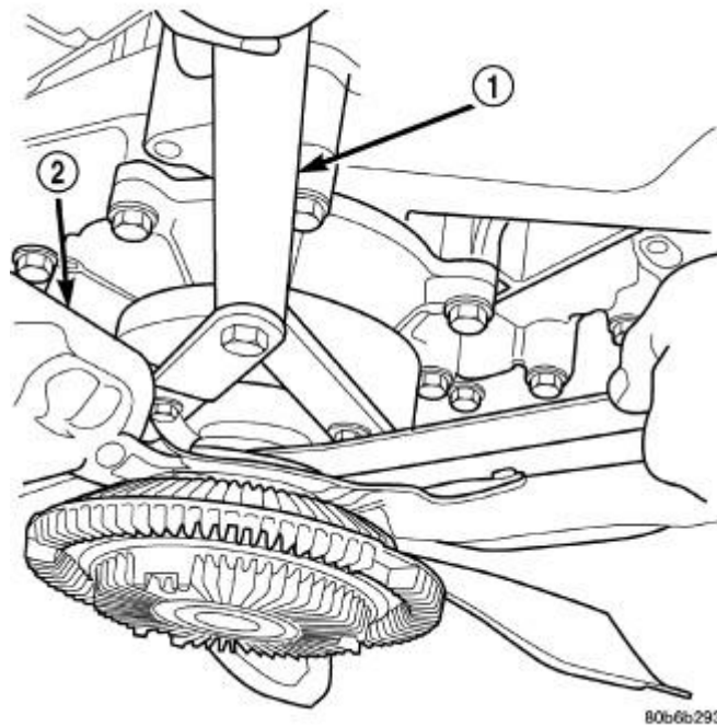
Fig. 367: Using Special Tool 6958 Spanner Wrench Courtesy of CHRYSLER GROUP, LLC
