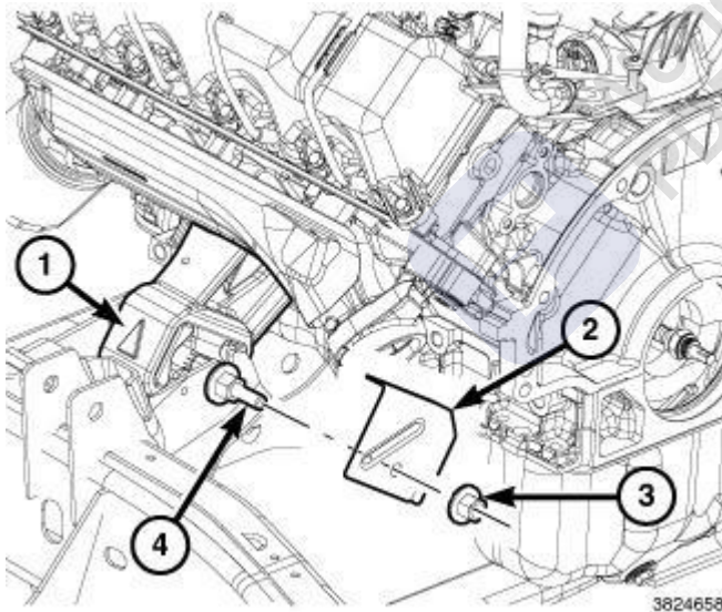
Fig. 237: Engine Mount, Heat Shield & Fasteners
