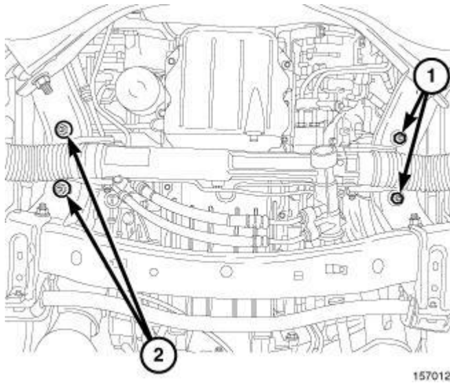
Fig. 216: Engine Mount Nuts
