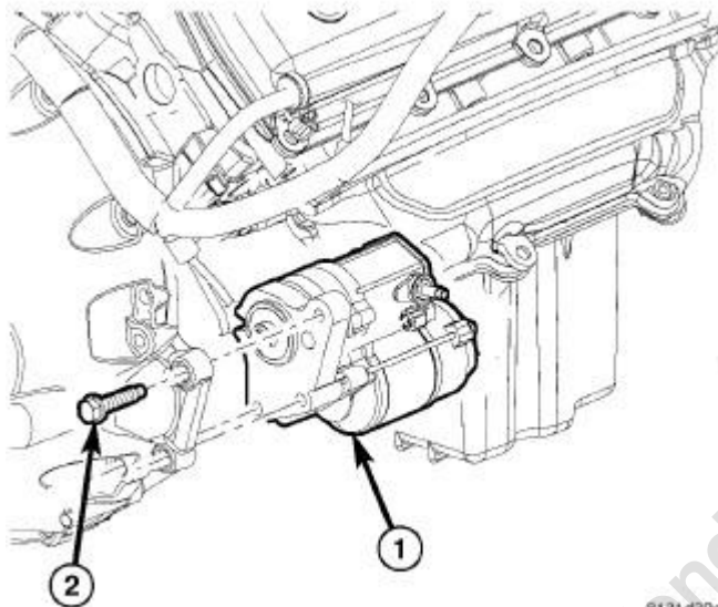
Fig. 27: Starter & Fasteners
