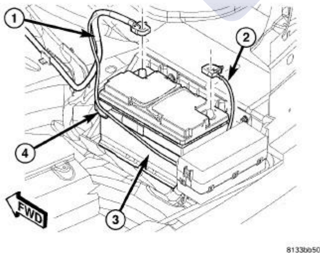
Fig. 60: Disconnecting/Connecting Battery Cables
