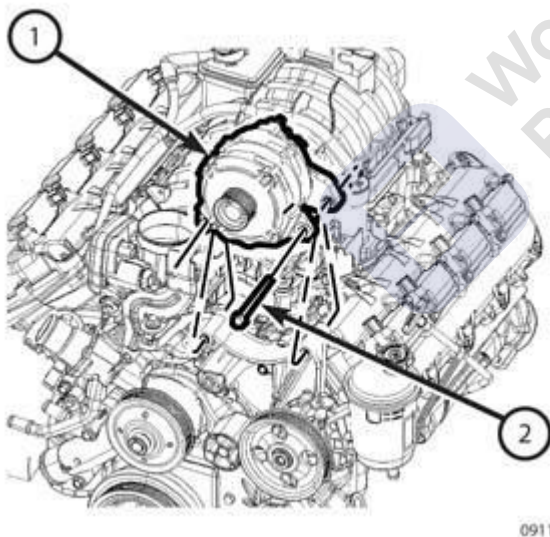
Fig. 388: Remove/Install Generator Courtesy of CHRYSLER GROUP, LLC
