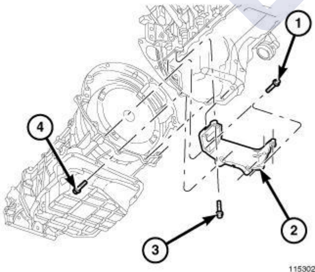
Fig. 155: Structural Cover
