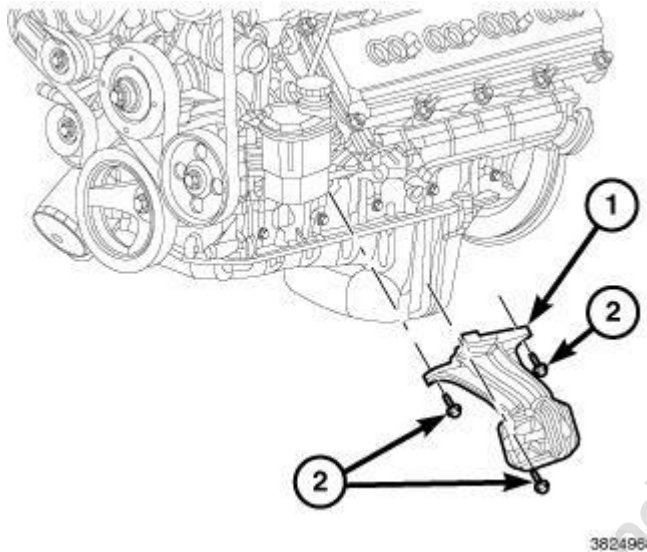
Fig. 231: Engine Mount & Bolts
