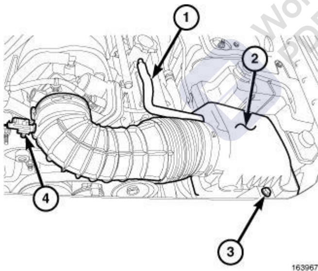
Fig. 217: Makeup Air Hose, Air Cleaner Housing, Retaining Bolt & Intake Air Temperature Sensor
