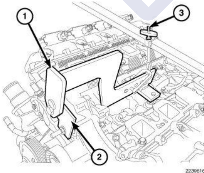
Fig. 214: Engine Lift Fixture & Adapter
