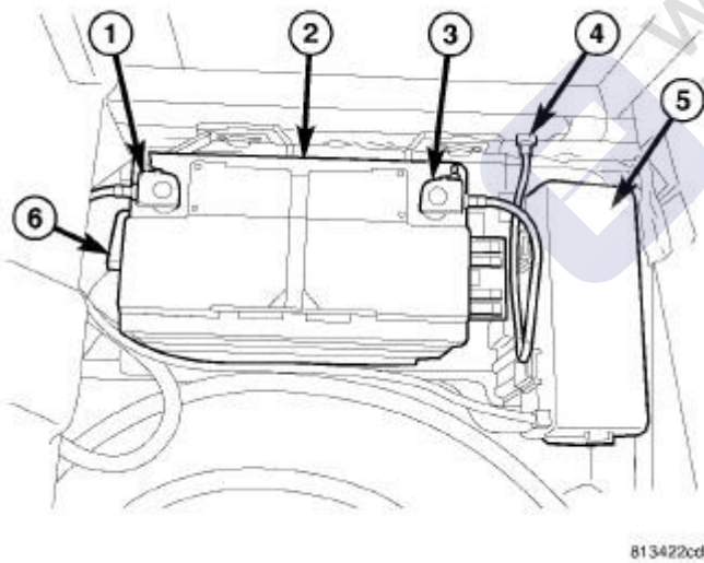
Fig. 201: Battery System Components & PDC Cover Courtesy of CHRYSLER GROUP, LLC
