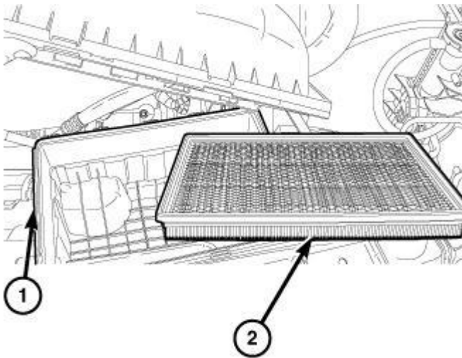
Fig. 54: Air Cleaner Body & Air Filter Element
