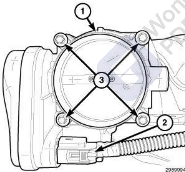
Fig. 342: Throttle Body, Connector & Bolts Courtesy of CHRYSLER GROUP, LLC
