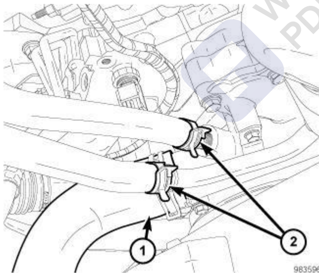
Fig. 8: Lower Radiator Hose & Heater Hoses
