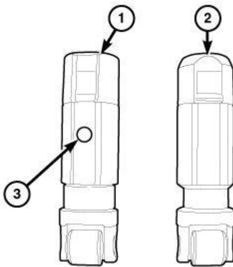
Fig. 185: MDS Lifter
