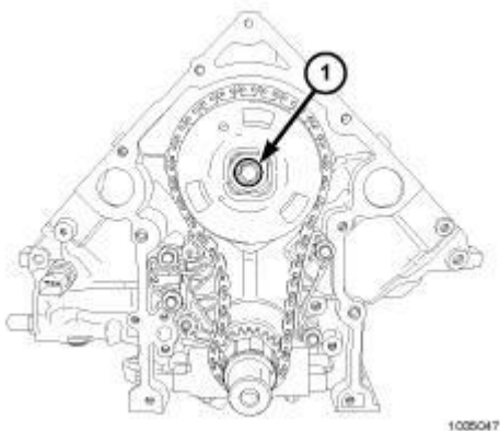
Fig. 352: Camshaft Phaser Retaining Bolt
