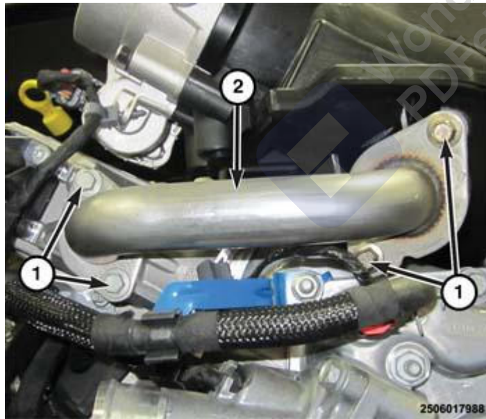
Fig. 333: Removing/Installing EGR Crossover Tube Courtesy of CHRYSLER GROUP, LLC
