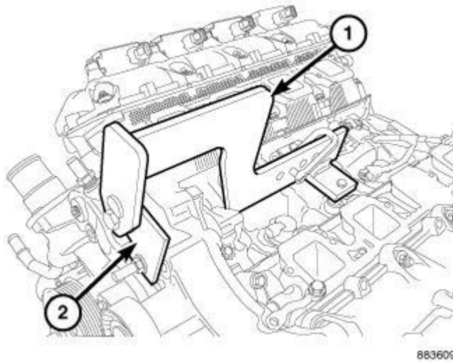
Fig. 29: Engine Lift Fixture & Adapter Courtesy of CHRYSLER GROUP, LLC
