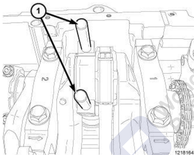
Fig. 208: Connecting Rod Guides Courtesy of CHRYSLER GROUP, LLC
