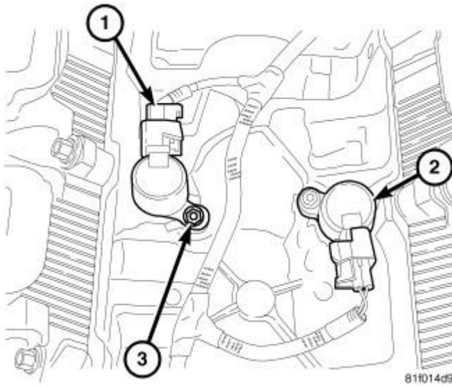
Fig. 224: MDS Solenoid Connector
