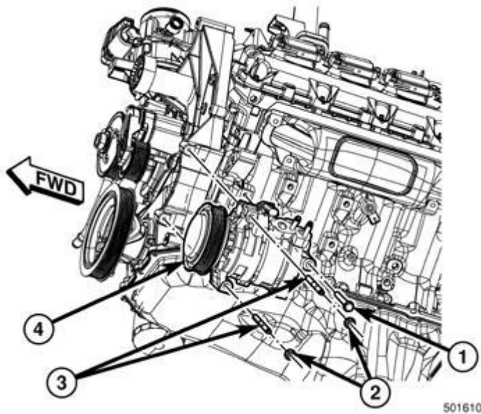
Fig. 7: A/C Compressor & Fasteners
