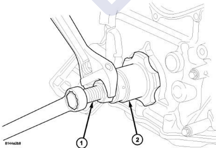
Fig. 222: Front Seal Installation
