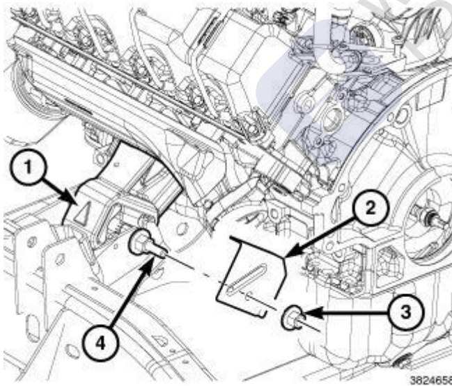
Fig. 230: Engine Mount, Heat Shield & Fasteners
