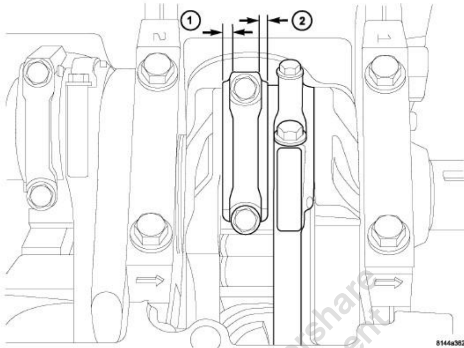
Fig. 213: Identifying Connecting Rod Proper Installation
