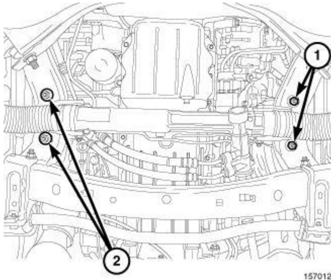
Fig. 204: Engine Mount Nuts
