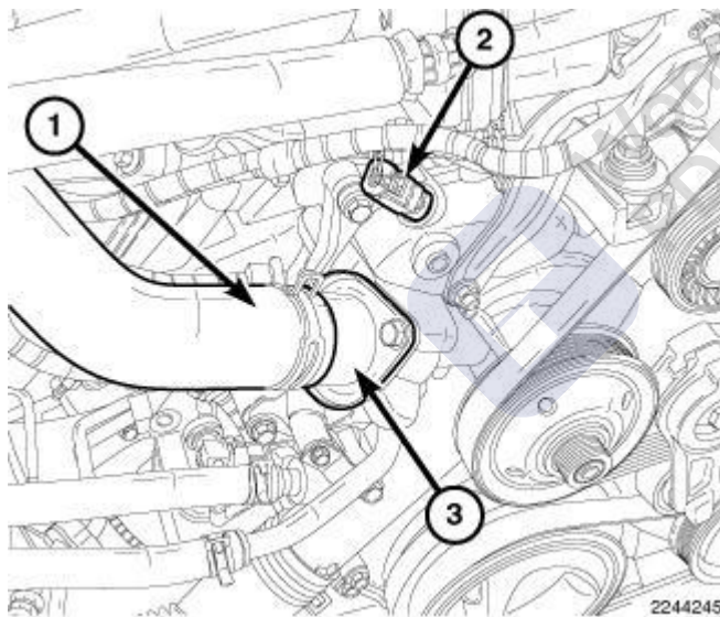
Fig. 390: Engine Coolant Temperature (ECT) Sensor & Thermostat
