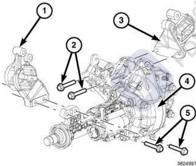
Fig. 266: Engine Mounts, Front Axle & Bolts
