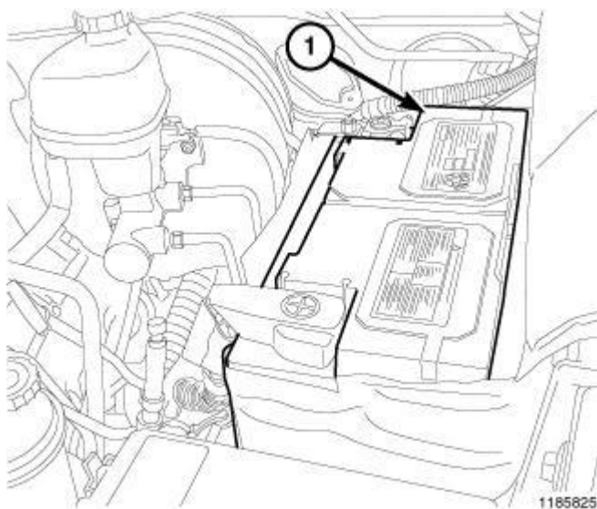
Fig. 104: Battery
