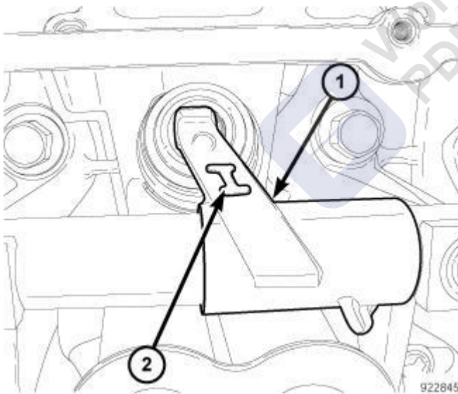
Fig. 95: Intake Rocker Arm Marking Courtesy of CHRYSLER GROUP, LLC
