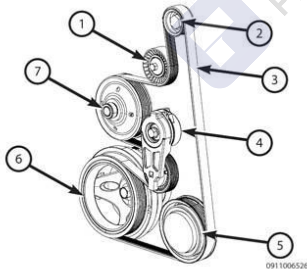
Fig. 368: Belt Routing (5.7L Engine) Courtesy of CHRYSLER GROUP, LLC
