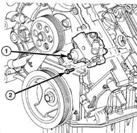
Fig. 73: Power Steering Pump & Bolts Courtesy of CHRYSLER GROUP, LLC
