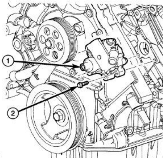
Fig. 64: Power Steering Pump & Bolts Courtesy of CHRYSLER GROUP, LLC
