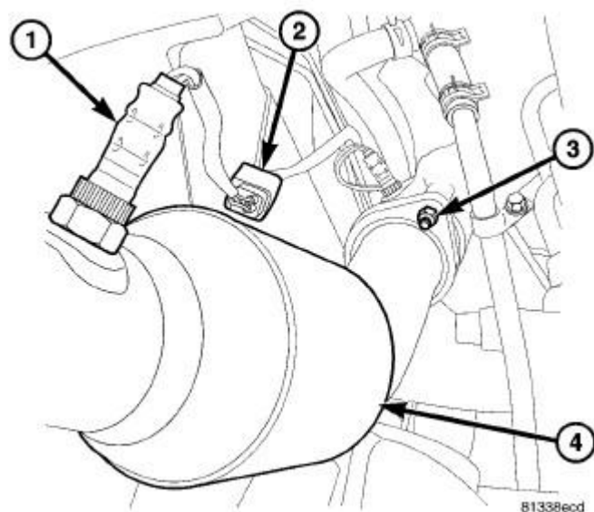
Fig. 11: Oxygen Sensor, Oxygen Sensor Connector, Ball Flange Nut & LH Catalytic Converter Courtesy of CHRYSLER GROUP, LLC
