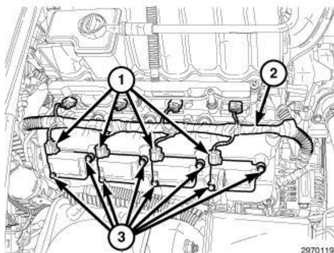
Fig. 81: Ignition Coil Electrical Connectors, Harness & Bolts Courtesy of CHRYSLER GROUP, LLC
