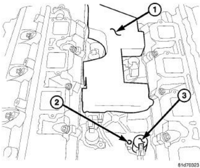
Fig. 224: Intake Manifold Foam Insulator Pad, MDS Solenoids & Bolts Courtesy of CHRYSLER GROUP, LLC
