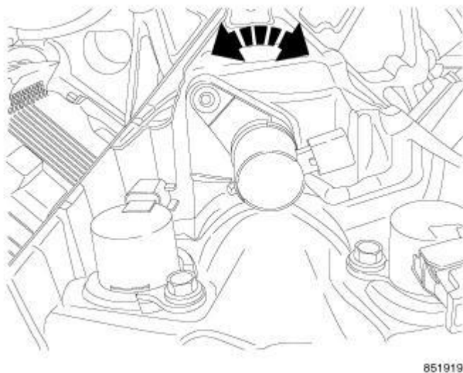
Fig. 297: Removing/Installing OCV
