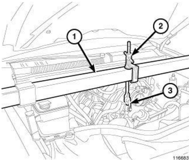
Fig. 243: Engine Support Tool Courtesy of CHRYSLER GROUP, LLC
