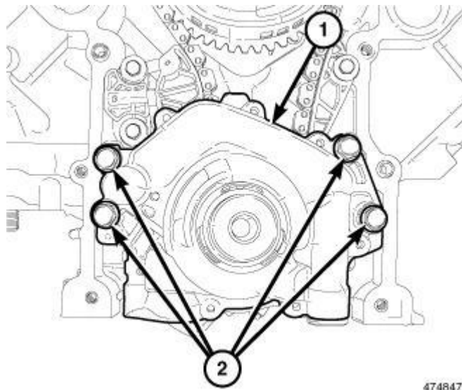
Fig. 161: Oil Pump Retaining Bolts Courtesy of CHRYSLER GROUP, LLC
