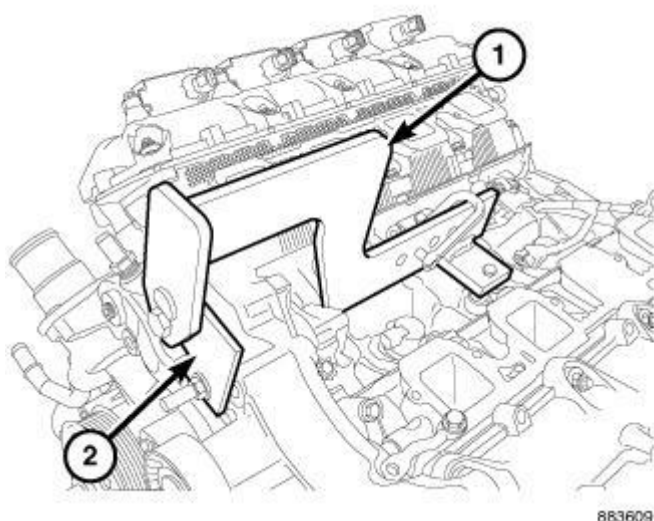
Fig. 19: Engine Lift Fixture & Adapter Courtesy of CHRYSLER GROUP, LLC
