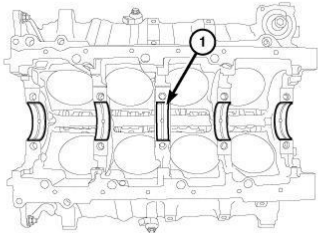
Fig. 167: Main Bearings
