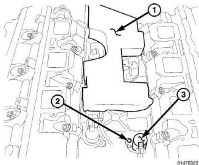
Fig. 227: Intake Manifold Foam Insulator Pad, MDS Solenoids & Bolts Courtesy of CHRYSLER GROUP, LLC
