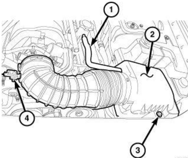
Fig. 204: Makeup Air Hose, Air Cleaner Housing, Retaining Bolt & Intake Air Temperature Sensor
