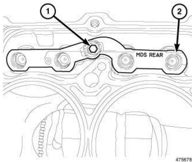
Fig. 188: Rear MDS Lifter Assembly Courtesy of CHRYSLER GROUP, LLC
