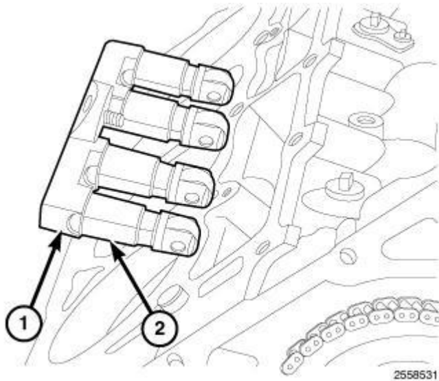
Fig. 191: Hydraulic Lifters/Tappets & Retainer/Guide Holder Courtesy of CHRYSLER GROUP, LLC
