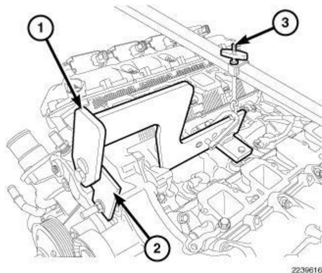
Fig. 207: Engine Lift Fixture & Adapter Courtesy of CHRYSLER GROUP, LLC
