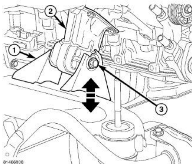
Fig. 311: Engine Mount & Bolt Courtesy of CHRYSLER GROUP, LLC
