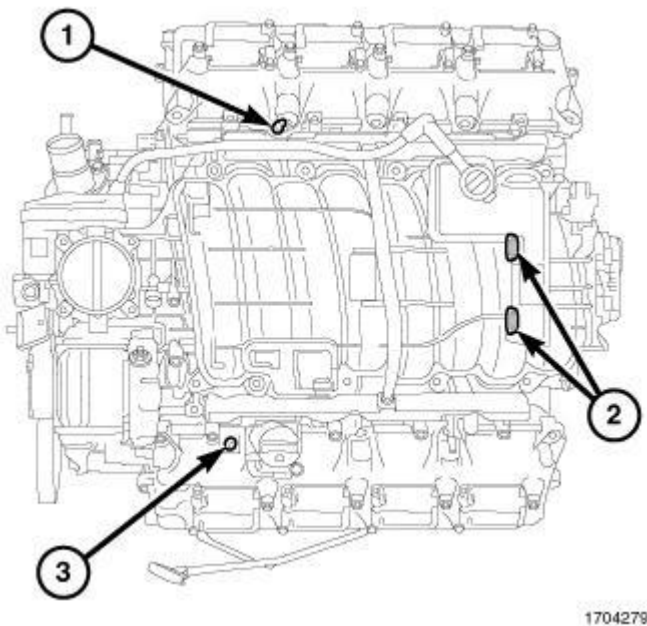
Fig. 40: Engine Cover Mounts
