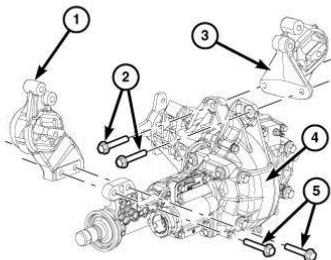
Fig. 256: Engine Mounts, Front Axle & Bolts Courtesy of CHRYSLER GROUP, LLC
