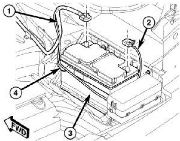
Fig. 78: Battery & Cables
