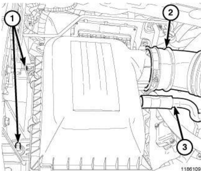
Fig. 57: Clean Air Tube To Air Cleaner Housing, Make Up Air Hose & Grommets
