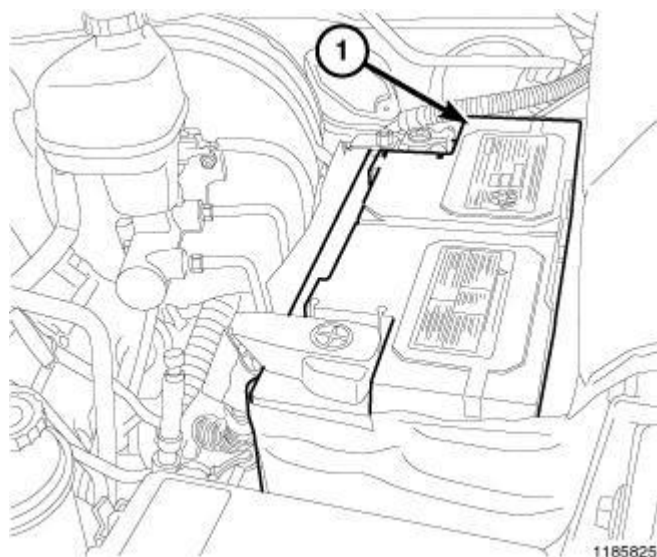
Fig. 332: Battery Courtesy of CHRYSLER GROUP, LLC
