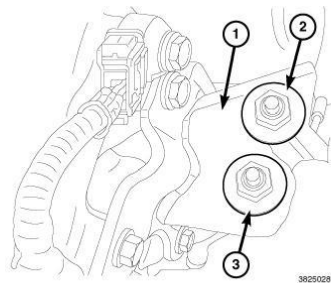
Fig. 249: Upper Engine Bracket, Mount & Bolts - Right Courtesy of CHRYSLER GROUP, LLC
