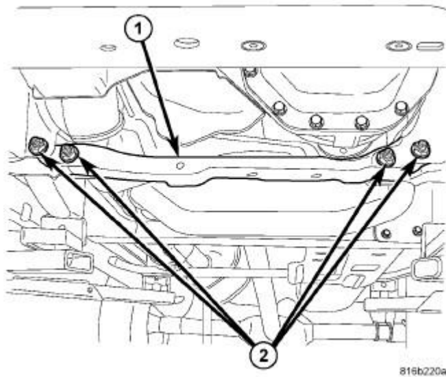
Fig. 235: Suspension Crossmember & Bolts Courtesy of CHRYSLER GROUP, LLC
