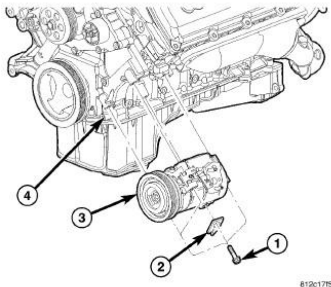
Fig. 34: A/C Compressor & Fasteners
