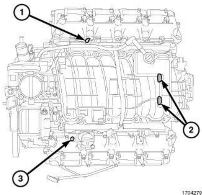
Fig. 45: Engine Cover Mounts
