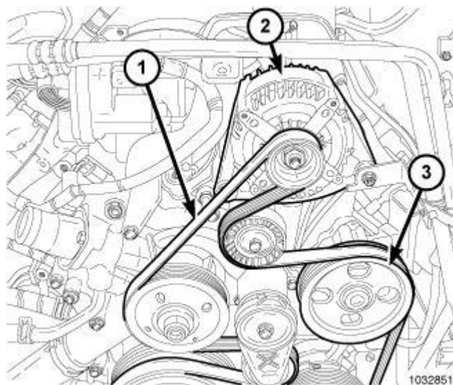
Fig. 181: Accessory Drive Belt Routing Courtesy of CHRYSLER GROUP, LLC
