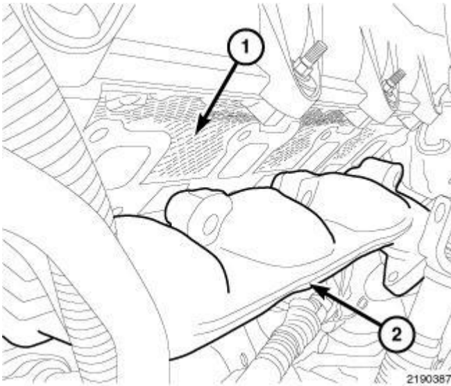
Fig. 307: Locating Exhaust Manifold & Gasket Courtesy of CHRYSLER GROUP, LLC
