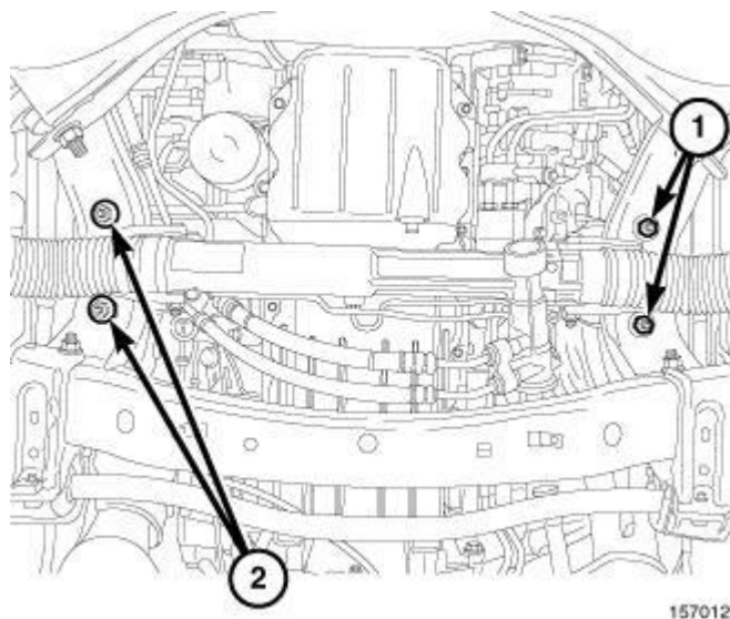
Fig. 217: Engine Mount Nuts
