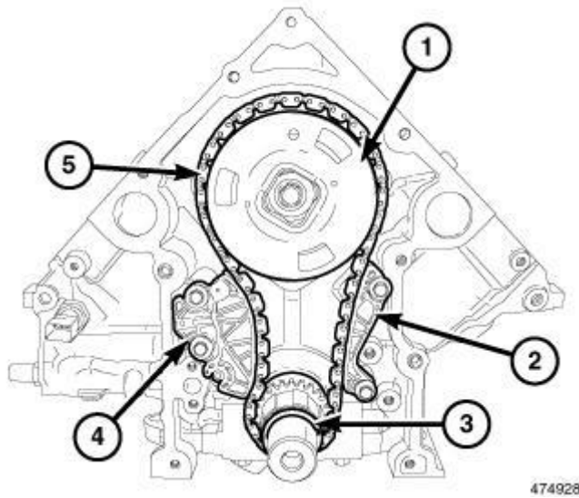
Fig. 136: Timing Chain, Sprockets, Timing Chain Tensioner & Guide Courtesy of CHRYSLER GROUP, LLC
