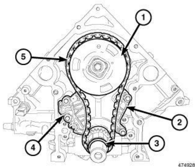
Fig. 162: Timing Chain, Sprockets, Timing Chain Tensioner & Guide Courtesy of CHRYSLER GROUP, LLC
