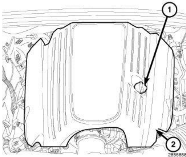
Fig. 80: Oil Fill Cap & Engine Cover
