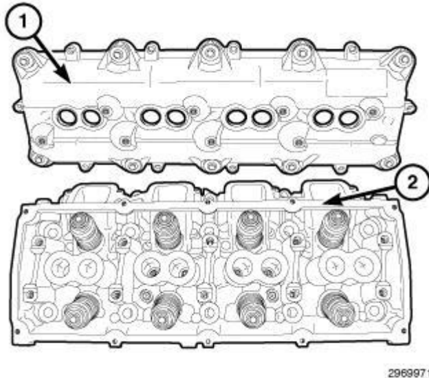
Fig. 83: Cylinder Head & Cover Courtesy of CHRYSLER GROUP, LLC
