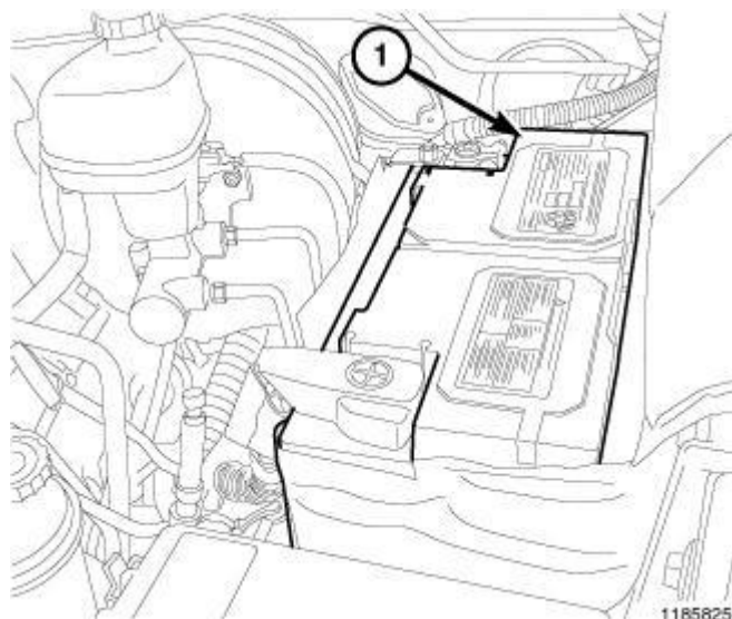
Fig. 4: Battery
