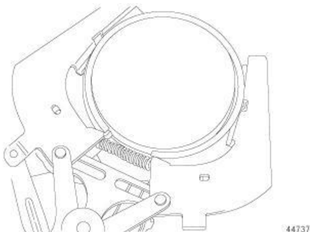
Fig. 198: Installing Upper & Intermediate Rings Courtesy of CHRYSLER GROUP, LLC
