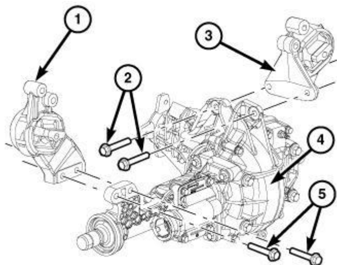
Fig. 267: Engine Mounts, Front Axle & Bolts Courtesy of CHRYSLER GROUP, LLC
