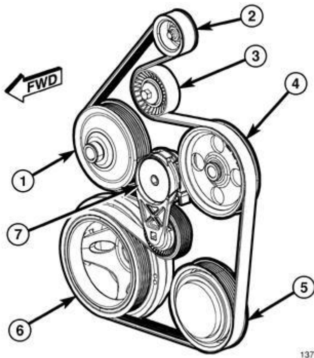
Fig. 36: Accessory Drive Belt Routing, Tensioner & Pulleys Courtesy of CHRYSLER GROUP, LLC
