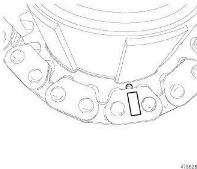
Fig. 343: Aligning Timing Chain & Crankshaft Sprocket Marks Courtesy of CHRYSLER GROUP, LLC
