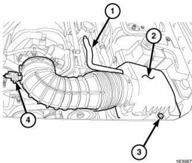
Fig. 218: Makeup Air Hose, Air Cleaner Housing, Retaining Bolt & Intake Air Temperature Sensor
