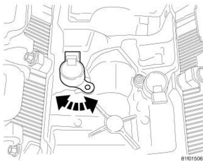
Fig. 226: MDS Solenoid Removal Courtesy of CHRYSLER GROUP, LLC
