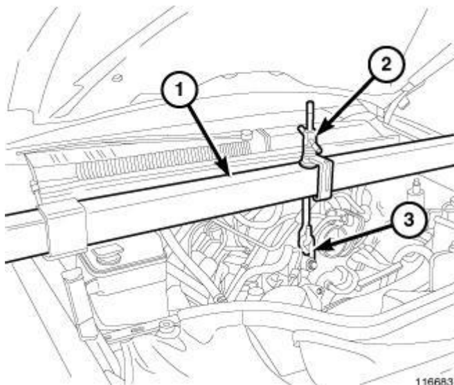
Fig. 230: Engine Support Tool Courtesy of CHRYSLER GROUP, LLC
