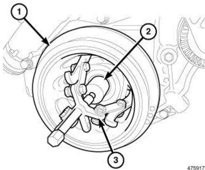
Fig. 221: Removing Vibration Damper Courtesy of CHRYSLER GROUP, LLC
