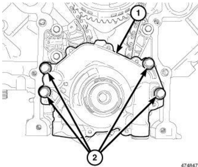
Fig. 283: Oil Pump Retaining Bolts
