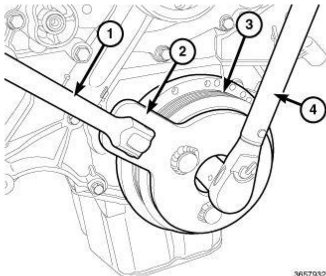
Fig. 180: Installing Vibration Damper Courtesy of CHRYSLER GROUP, LLC
