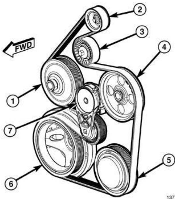
Fig. 63: Accessory Drive Belt Routing, Tensioner & Pulleys Courtesy of CHRYSLER GROUP, LLC
