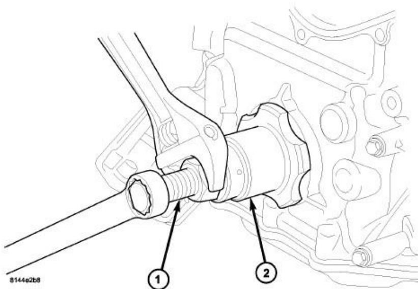
Fig. 223: Front Seal Installation
