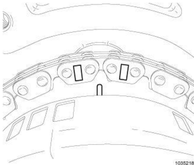
Fig. 342: Aligning Timing Chain & Camshaft Phaser Marks Courtesy of CHRYSLER GROUP, LLC
