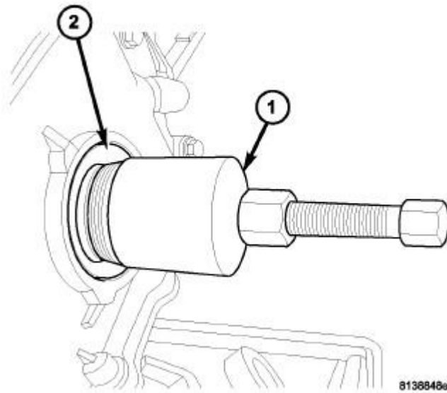
Fig. 222: Front Crankshaft Seal Removal Courtesy of CHRYSLER GROUP, LLC
