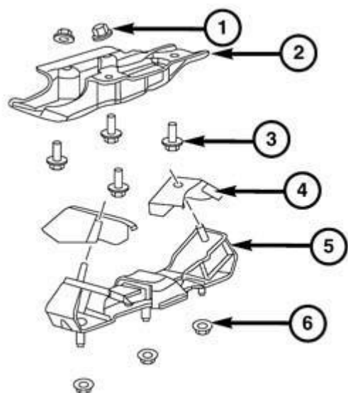
Fig. 228: Transmission Mount Nuts, Upper Mount Bracket, Bolts, Heat Shields, Mount & Lower Nuts Courtesy of CHRYSLER GROUP, LLC
