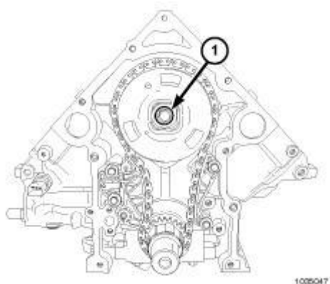
Fig. 338: Camshaft Phaser Retaining Bolt Courtesy of CHRYSLER GROUP, LLC
