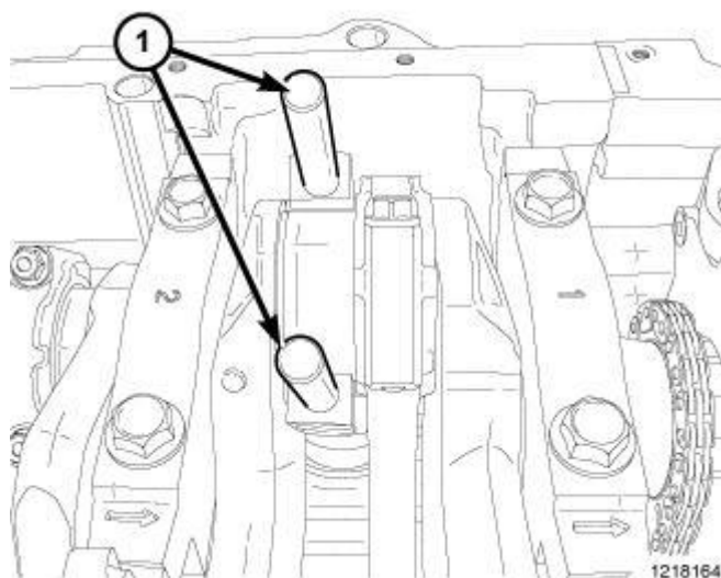
Fig. 211: Connecting Rod Guides Courtesy of CHRYSLER GROUP, LLC
