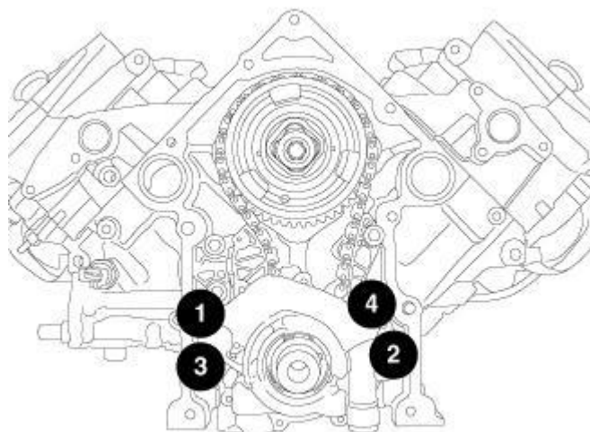
Fig. 350: Oil Pump Retaining Bolt Tightening Sequence Courtesy of CHRYSLER GROUP, LLC
