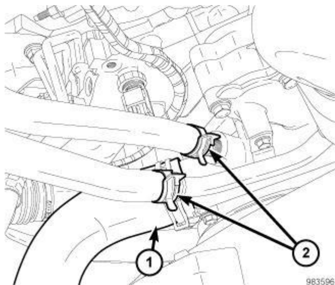
Fig. 62: Lower Radiator Hose & Heater Hoses Courtesy of CHRYSLER GROUP, LLC
