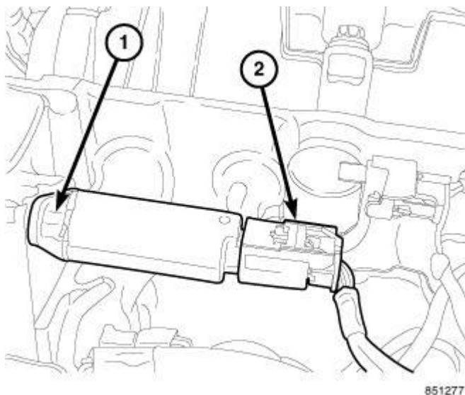
Fig. 298: Oil Control Valve
