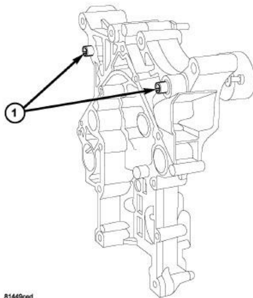
Fig. 353: Front Cover Slide Bushings Courtesy of CHRYSLER GROUP, LLC
