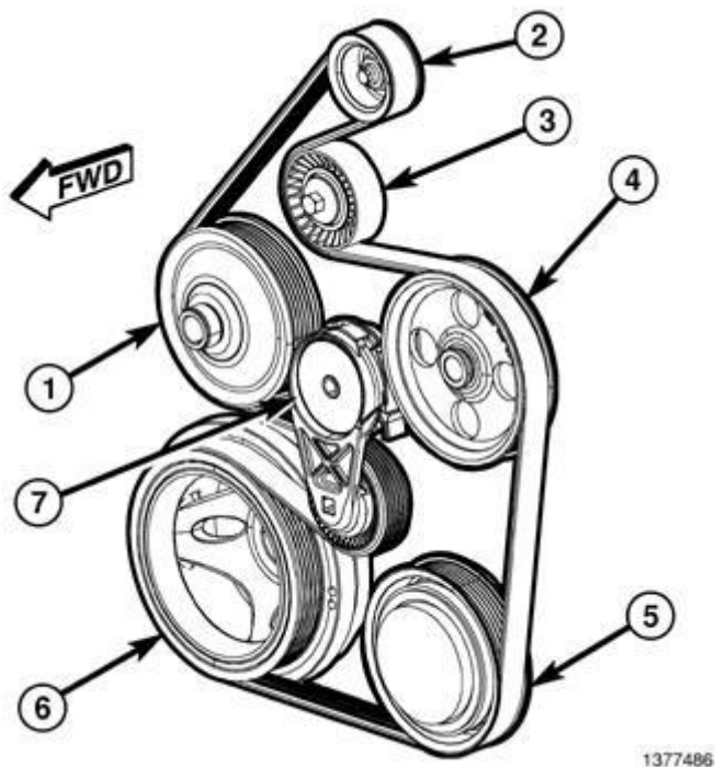
Fig. 5: Accessory Drive Belt Routing, Tensioner & Pulleys
