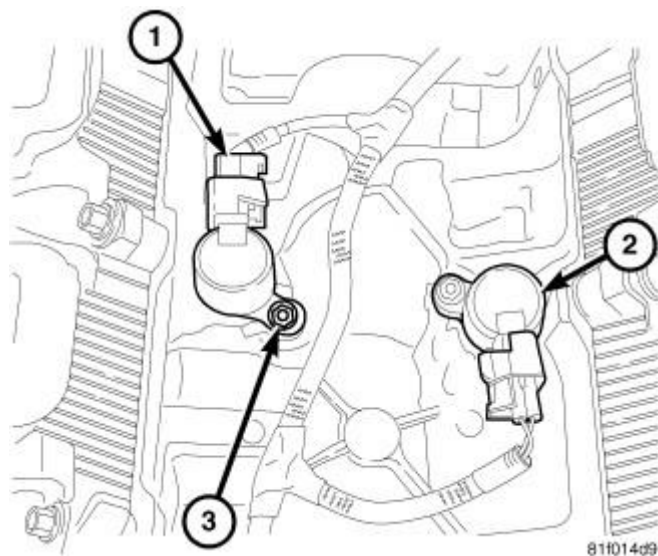
Fig. 225: MDS Solenoid Connector Courtesy of CHRYSLER GROUP, LLC
