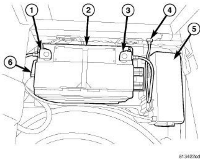
Fig. 202: Battery System Components & PDC Cover Courtesy of CHRYSLER GROUP, LLC
