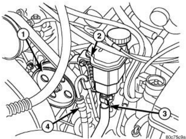
Fig. 31: Power Steering Pulley, Reservoir & Hoses Courtesy of CHRYSLER GROUP, LLC
