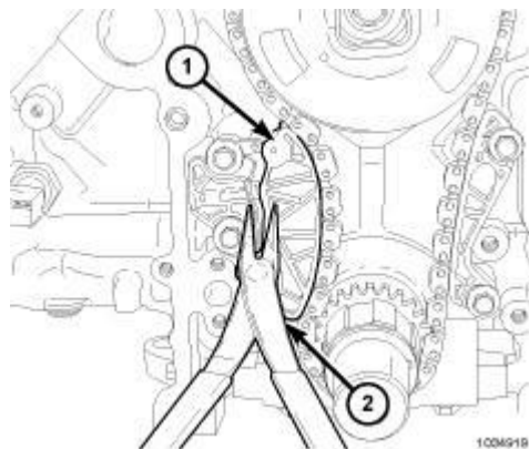
Fig. 336: Chain Tensioner Arm Courtesy of CHRYSLER GROUP, LLC
