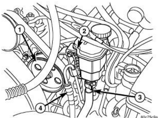
Fig. 9: Power Steering Pulley, Reservoir & Hoses Courtesy of CHRYSLER GROUP, LLC
