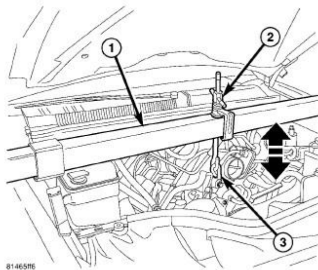
Fig. 282: Engine Support Tool Courtesy of CHRYSLER GROUP, LLC
