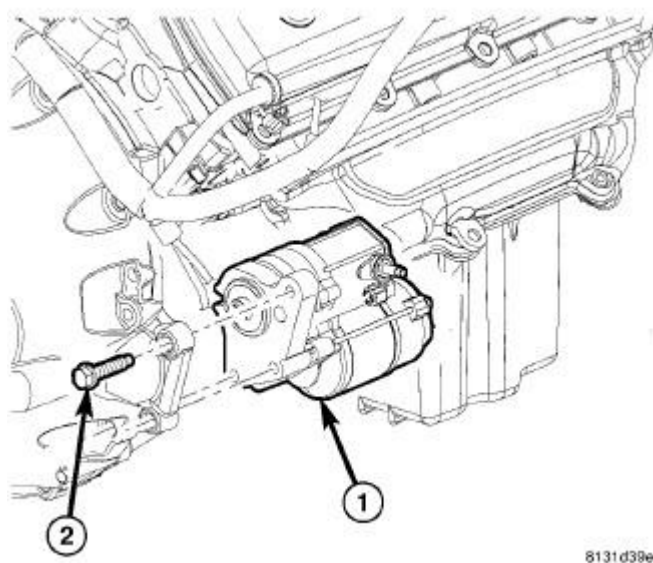
Fig. 12: Starter & Fasteners
