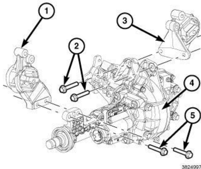
Fig. 236: Engine Mounts, Front Axle & Bolts Courtesy of CHRYSLER GROUP, LLC
