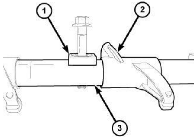
Fig. 96: Retainers, Rocker Arm & Rocker Shaft Courtesy of CHRYSLER GROUP, LLC
