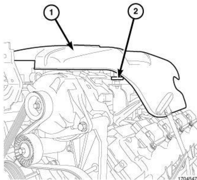
Fig. 317: Engine Cover & Grommets Courtesy of CHRYSLER GROUP, LLC
