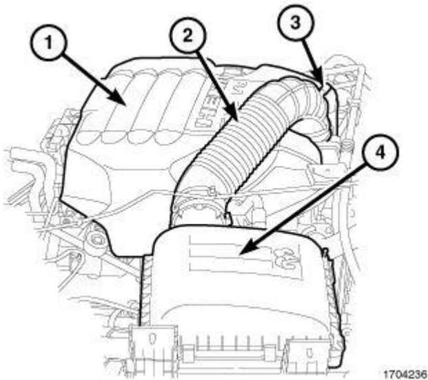
Fig. 3: Engine Cover, Clean Air Hose, Intake Air Temperature (IAT) Sensor Electrical Connector & Air Cleaner Housing
