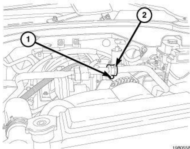
Fig. 328: A/C Line P-Clip & Retaining Bolt
