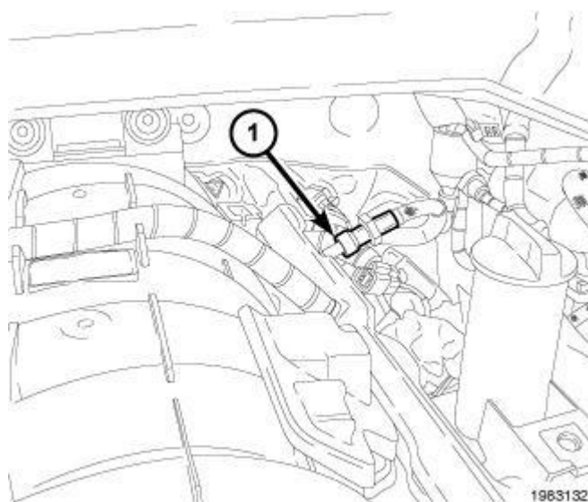
Fig. 320: Fuel Supply Line Quick Connect Fitting At Fuel Rail
