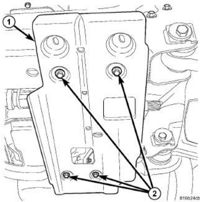
Fig. 234: Skid Plate & Bolts
