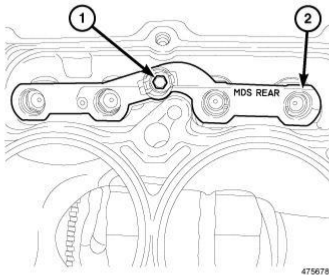
Fig. 192: Rear MDS Lifter Assembly Courtesy of CHRYSLER GROUP, LLC
