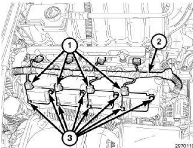
Fig. 87: Ignition Coil Electrical Connectors, Harness & Bolts Courtesy of CHRYSLER GROUP, LLC
