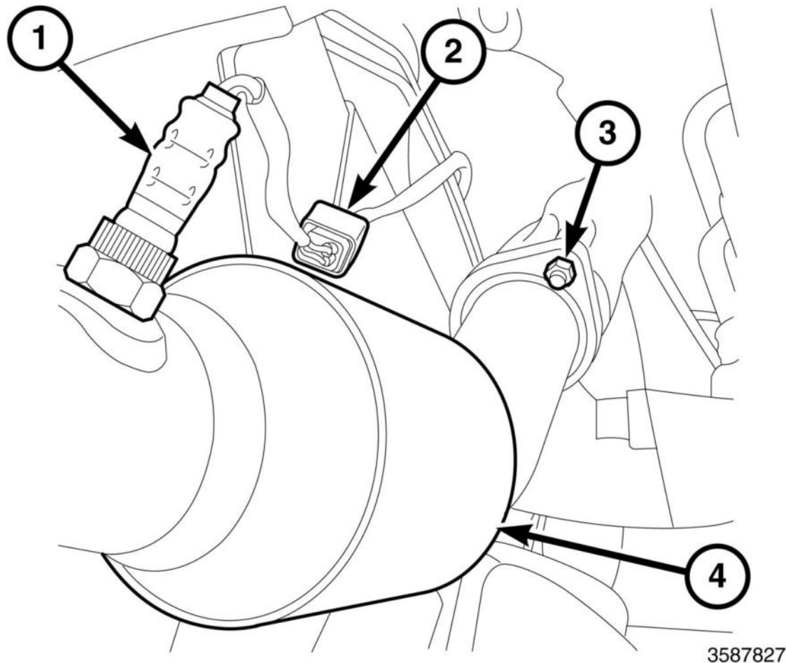
Fig. 312: Oxygen Sensor, Oxygen Sensor Connector, Ball Flange Nut & LH Catalytic Converter Courtesy of CHRYSLER GROUP, LLC
