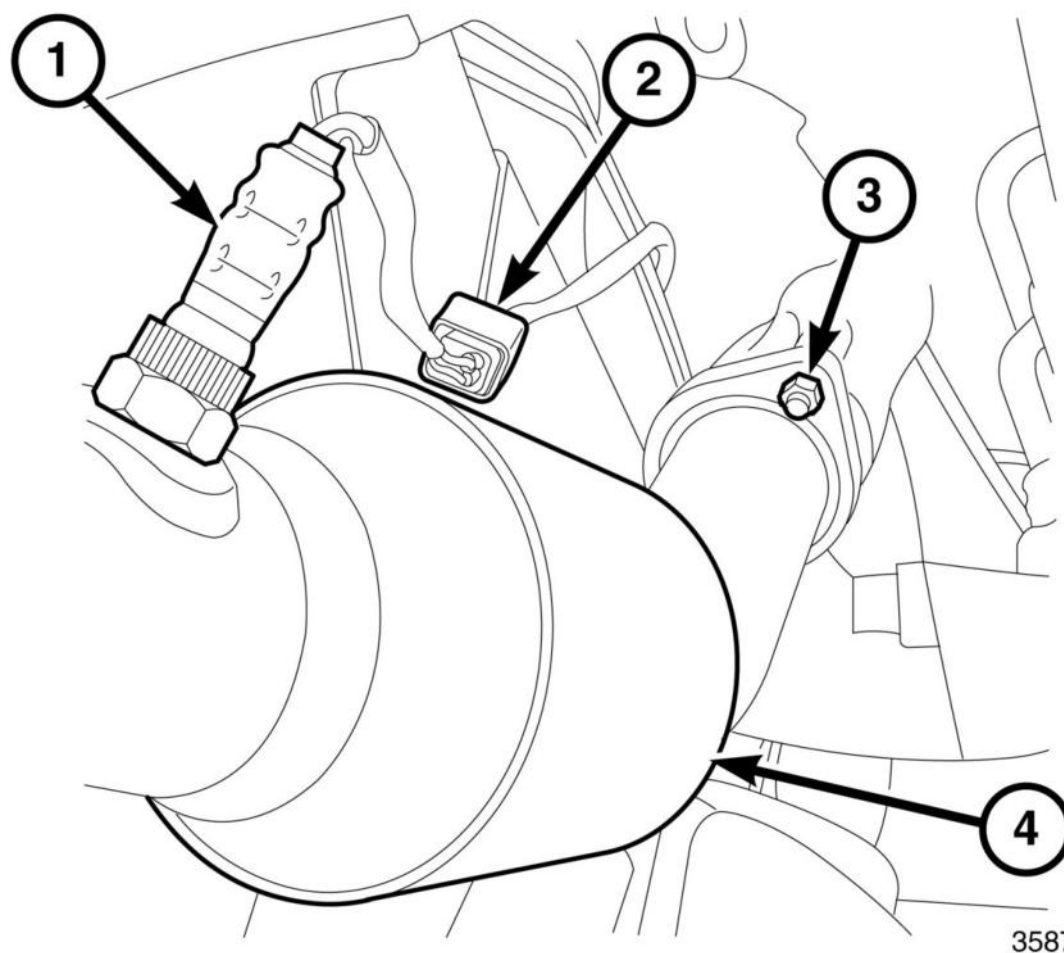
Fig. 302: Oxygen Sensor, Oxygen Sensor Connector, Ball Flange Nut & LH Catalytic Converter Courtesy of CHRYSLER GROUP, LLC
