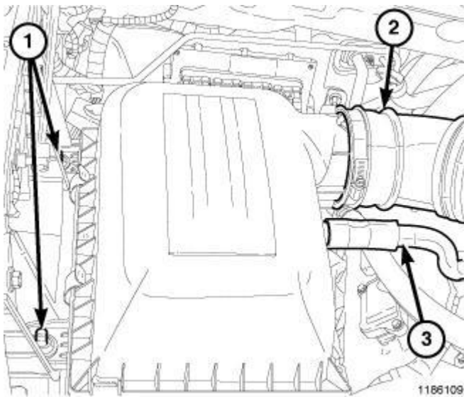
Fig. 56: Clean Air Tube To Air Cleaner Housing, Make Up Air Hose & Grommets Courtesy of CHRYSLER GROUP, LLC
