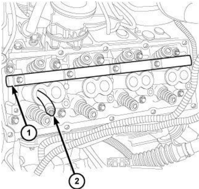
Fig. 110: Rocker Arm Valve Spring Compressor Shaft & Air Hose Courtesy of CHRYSLER GROUP, LLC
