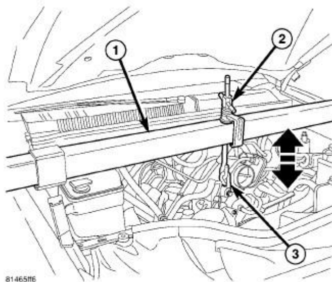
Fig. 252: Engine Support Tool
