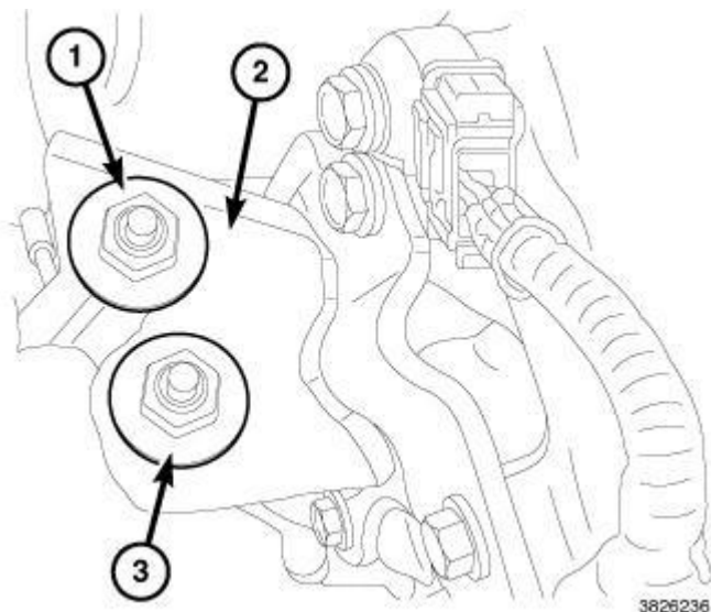
Fig. 253: Upper Engine Bracket, Mount & Bolts - Left Courtesy of CHRYSLER GROUP, LLC
