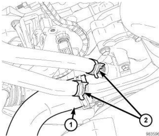
Fig. 386: Lower Radiator Hose & Heater Hoses Courtesy of CHRYSLER GROUP, LLC
