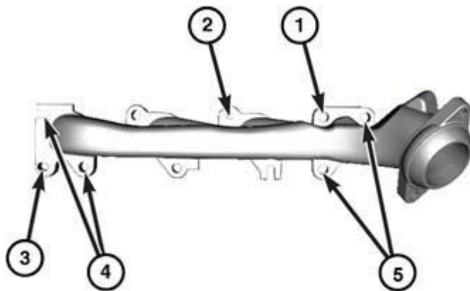
Fig. 314: Locating Exhaust Manifold Bolts & Washers Placement Locations
