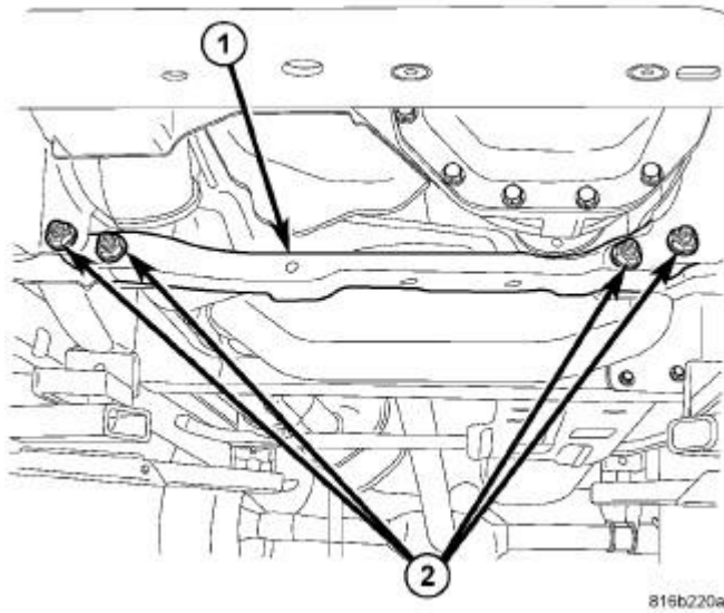
Fig. 234: Suspension Crossmember & Bolts Courtesy of CHRYSLER GROUP, LLC
