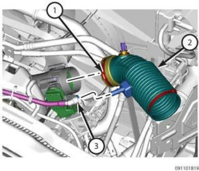
Fig. 323: Clamp, Air Intake Tube & Breather Hose Courtesy of CHRYSLER GROUP, LLC
