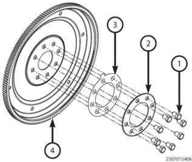
Fig. 181: Bolts, Clamp Ring, Shim & Flex Plate Courtesy of CHRYSLER GROUP, LLC
