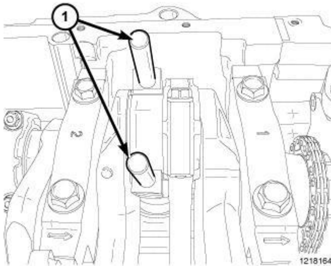
Fig. 208: Connecting Rod Guides
