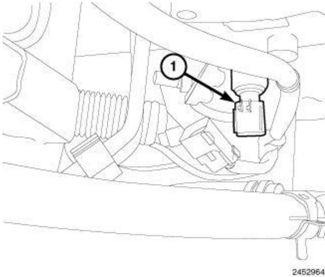
Fig. 290: Oil Pressure Sensor
