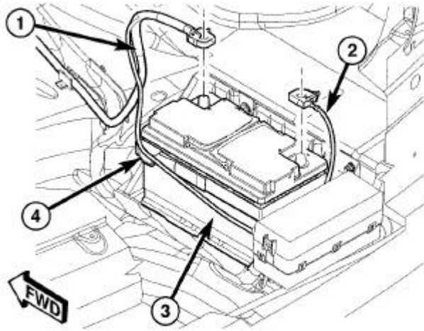
Fig. 78: Disconnecting/Connecting Battery Cables Courtesy of CHRYSLER GROUP, LLC
