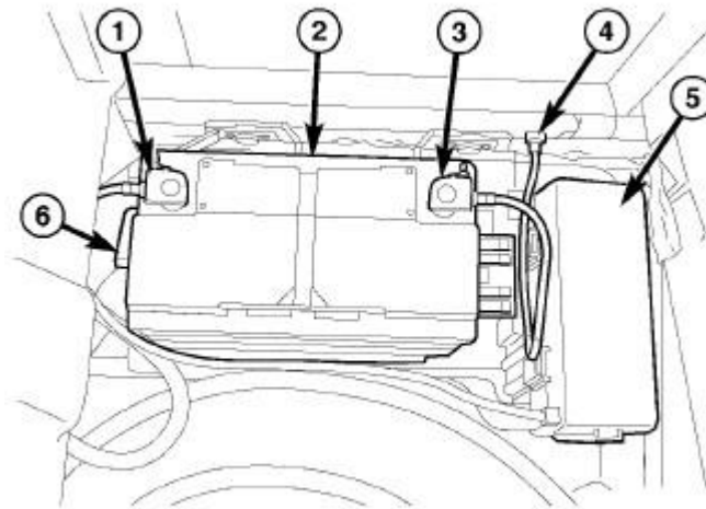
Fig. 219: Battery System Components & PDC Cover
