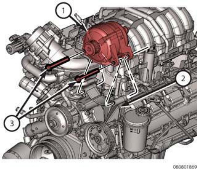
Fig. 340: Generator, Bolts & Connector Courtesy of CHRYSLER GROUP, LLC
