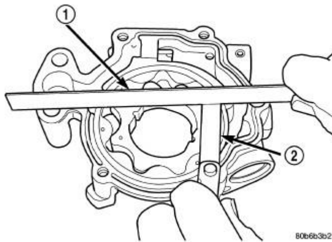
Fig. 286: Measuring Clearance Over Rotors Courtesy of CHRYSLER GROUP, LLC
