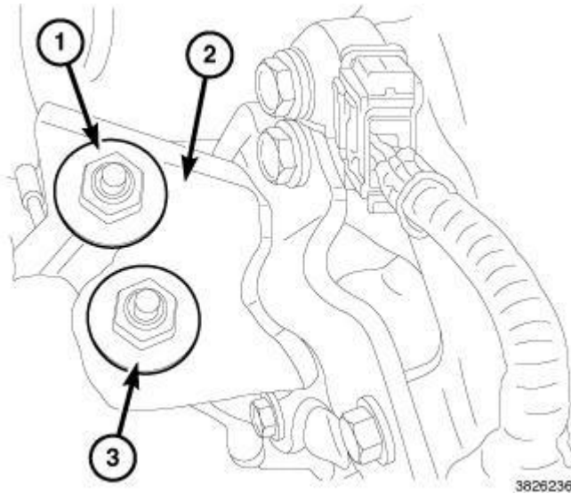
Fig. 238: Upper Engine Bracket, Mount & Bolts - Left Courtesy of CHRYSLER GROUP, LLC
