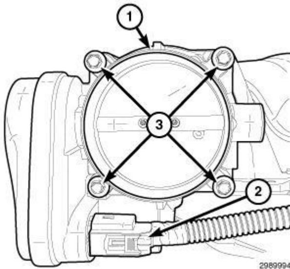
Fig. 342: Throttle Body, Connector & Bolts Courtesy of CHRYSLER GROUP, LLC
