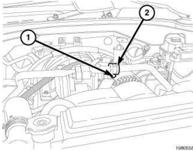
Fig. 391: A/C Line P-Clip & Retaining Bolt Courtesy of CHRYSLER GROUP, LLC
