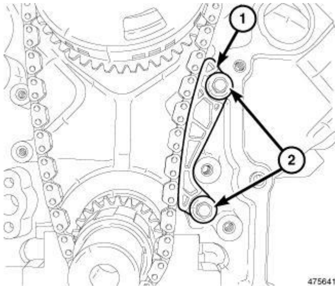
Fig. 359: Timing Chain Guide & Bolts Courtesy of CHRYSLER GROUP, LLC
