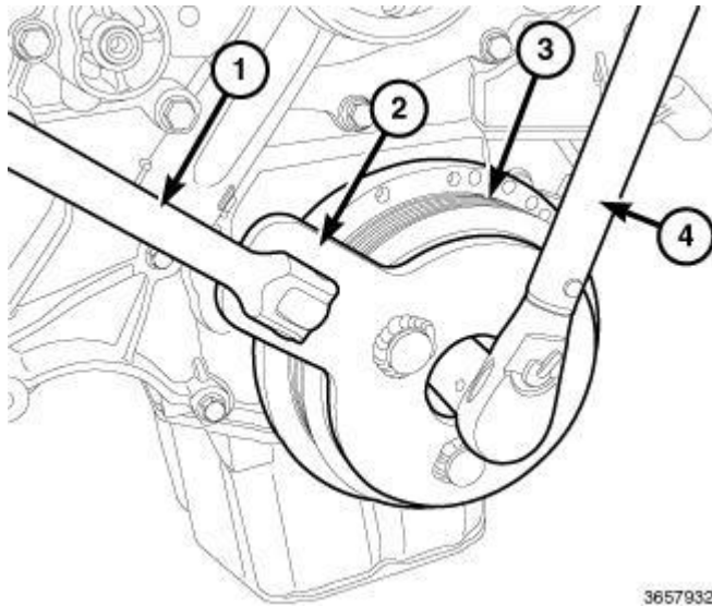
Fig. 385: Installing Vibration Damper Courtesy of CHRYSLER GROUP, LLC
