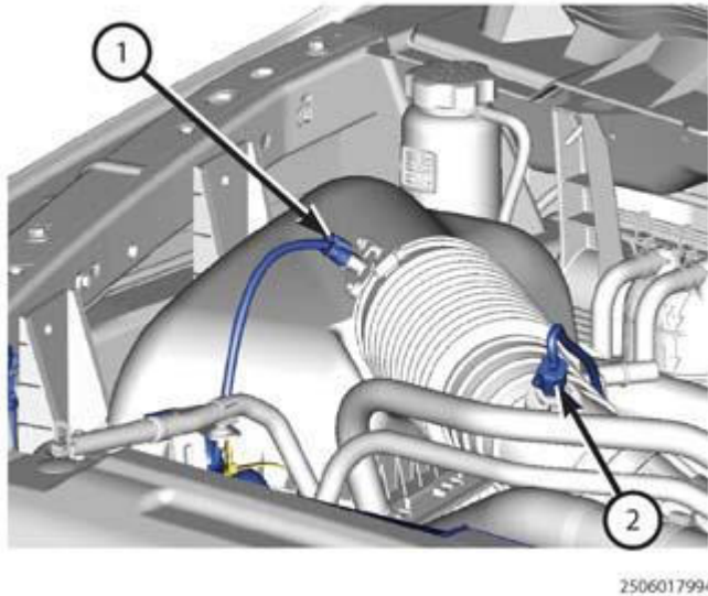
Fig. 345: Temperature Sensor Courtesy of CHRYSLER GROUP, LLC
