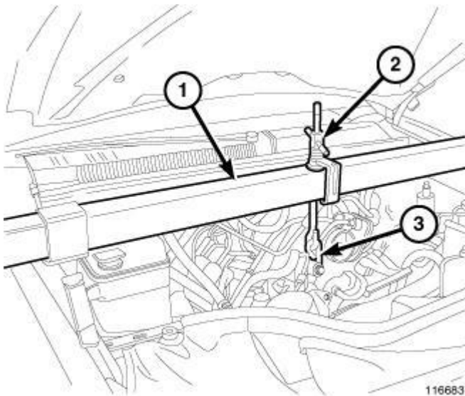
Fig. 239: Engine Support Tool Courtesy of CHRYSLER GROUP, LLC
