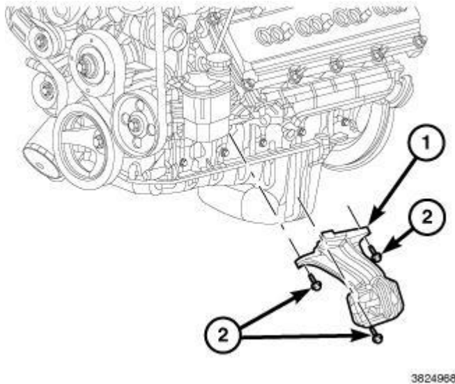
Fig. 231: Engine Mount & Bolts Courtesy of CHRYSLER GROUP, LLC
