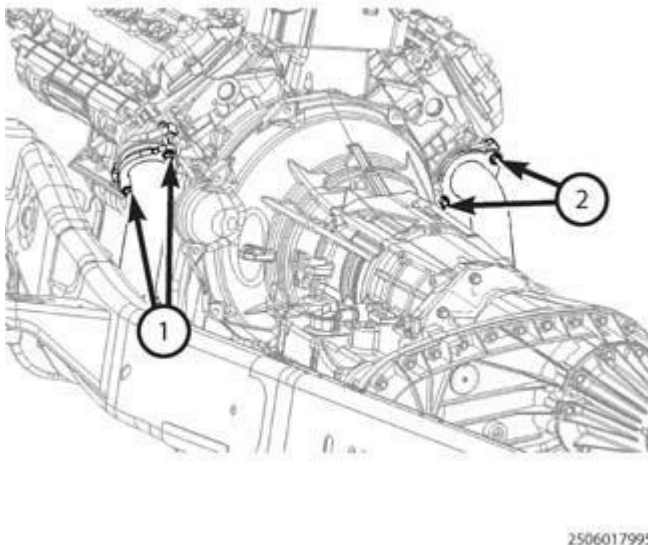
Fig. 310: Retaining Bolts & Nuts Courtesy of CHRYSLER GROUP, LLC
