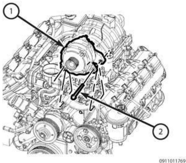
Fig. 388: Remove/Install Generator Courtesy of CHRYSLER GROUP, LLC
