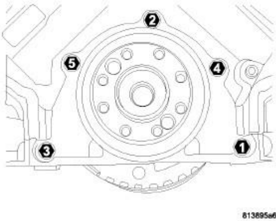
Fig. 192: Rear Seal Retainer Torque Sequence Courtesy of CHRYSLER GROUP, LLC
