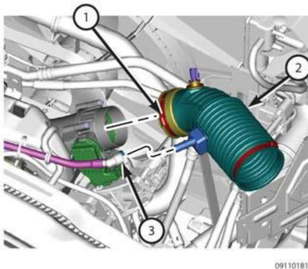
Fig. 344: Clamp, Air Intake Tube & Breather Hose Courtesy of CHRYSLER GROUP, LLC
