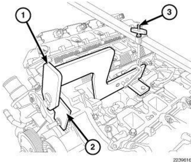
Fig. 214: Engine Lift Fixture & Adapter Courtesy of CHRYSLER GROUP, LLC
