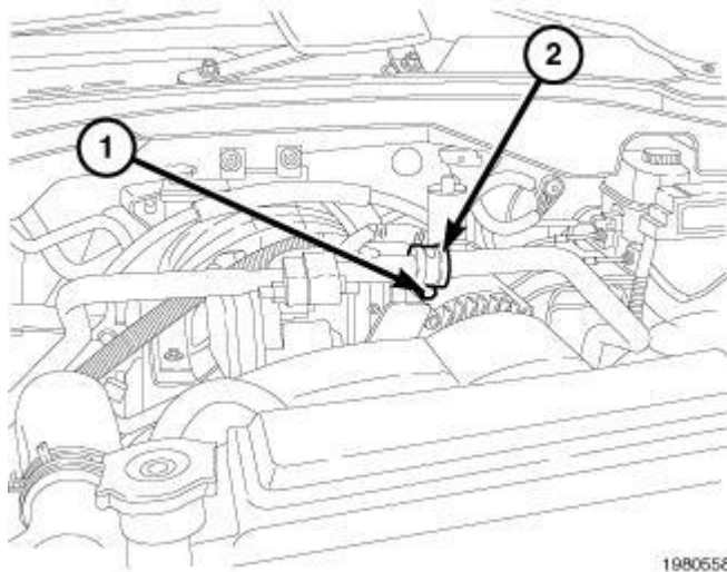
Fig. 370: A/C Line P-Clip & Retaining Bolt Courtesy of CHRYSLER GROUP, LLC
