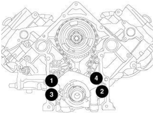
Fig. 364: Oil Pump Retaining Bolt Tightening Sequence Courtesy of CHRYSLER GROUP, LLC
