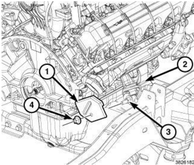
Fig. 247: Engine Mount, Heat Shield & Fasteners Courtesy of CHRYSLER GROUP, LLC
