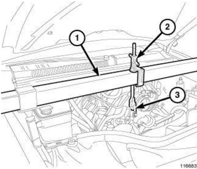
Fig. 229: Engine Support Tool Courtesy of CHRYSLER GROUP, LLC
