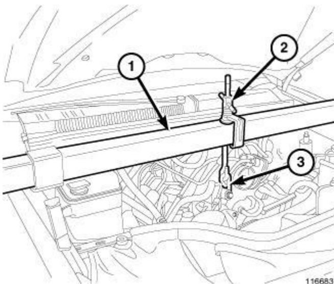
Fig. 232: Engine Support Tool
