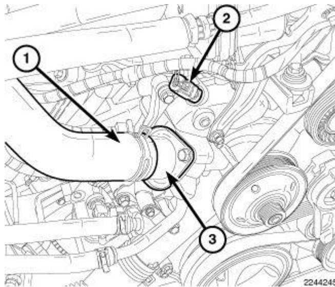
Fig. 390: Engine Coolant Temperature (ECT) Sensor & Thermostat Courtesy of CHRYSLER GROUP, LLC
