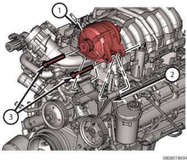
Fig. 329: Generator, Bolts & Connector Courtesy of CHRYSLER GROUP, LLC
