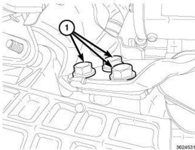
Fig. 246: Pinion Nose Mounting Bolts Courtesy of CHRYSLER GROUP, LLC
