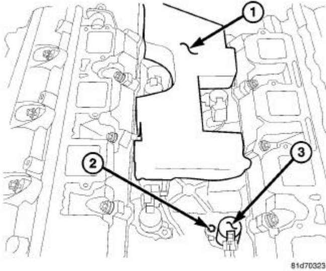
Fig. 226: Intake Manifold Foam Insulator Pad, MDS Solenoids & Bolts Courtesy of CHRYSLER GROUP, LLC
