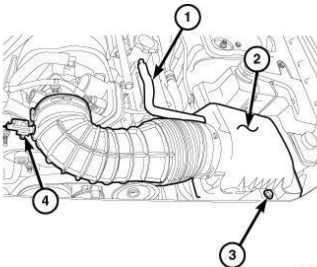
Fig. 203: Makeup Air Hose, Air Cleaner Housing, Retaining Bolt & Intake Air Temperature Sensor
