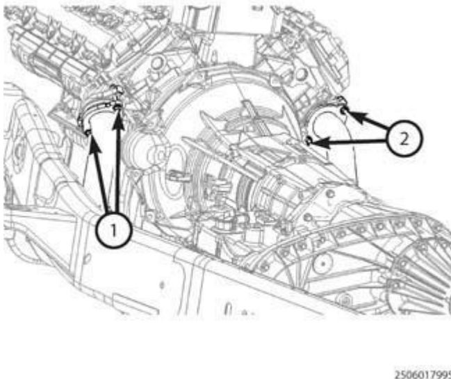
Fig. 319: Retaining Bolts & Nuts Courtesy of CHRYSLER GROUP, LLC
