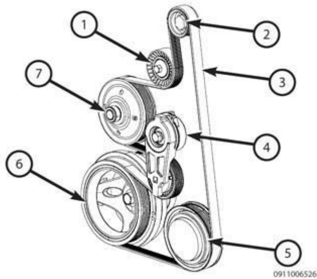
Fig. 389: Belt Routing (5.7L Engine) Courtesy of CHRYSLER GROUP, LLC
