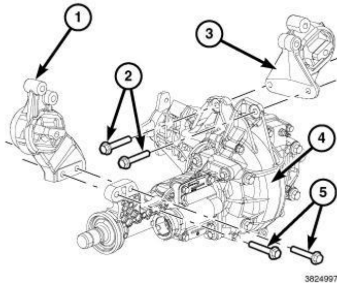
Fig. 235: Engine Mounts, Front Axle & Bolts Courtesy of CHRYSLER GROUP, LLC
