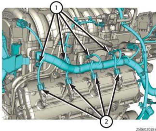
Fig. 337: Fuel Injector Electrical Connectors Courtesy of CHRYSLER GROUP, LLC
