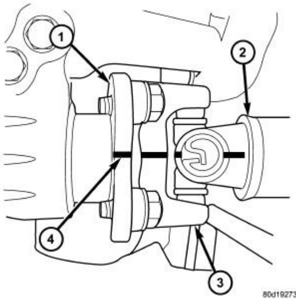
Fig. 377: Propeller Shaft & Pinion Flange. Reference Mark Courtesy of CHRYSLER GROUP, LLC
