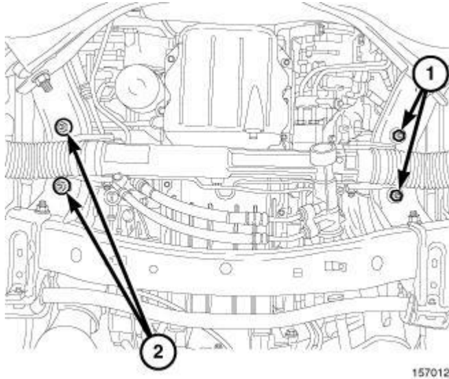
Fig. 204: Engine Mount Nuts Courtesy of CHRYSLER GROUP, LLC
