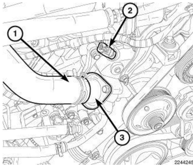
Fig. 372: Engine Coolant Temperature (ECT) Sensor & Thermostat Courtesy of CHRYSLER GROUP, LLC
