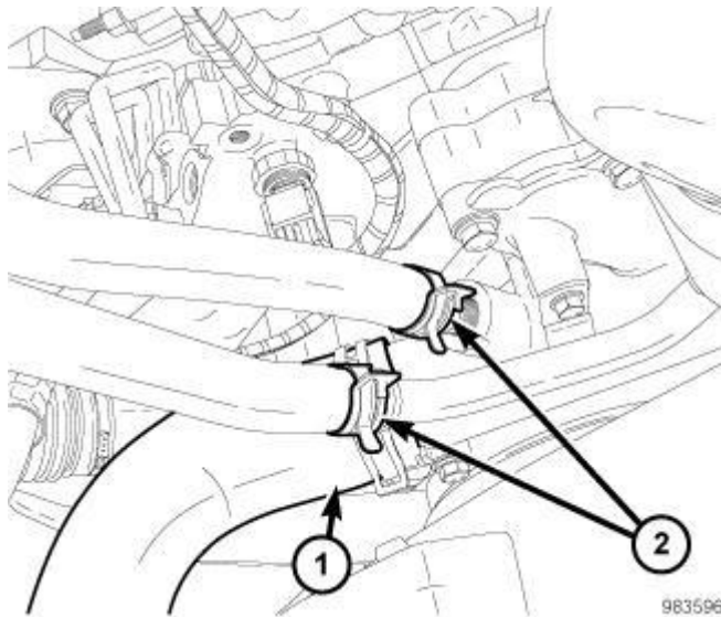
Fig. 373: Lower Radiator Hose & Heater Hoses Courtesy of CHRYSLER GROUP, LLC
