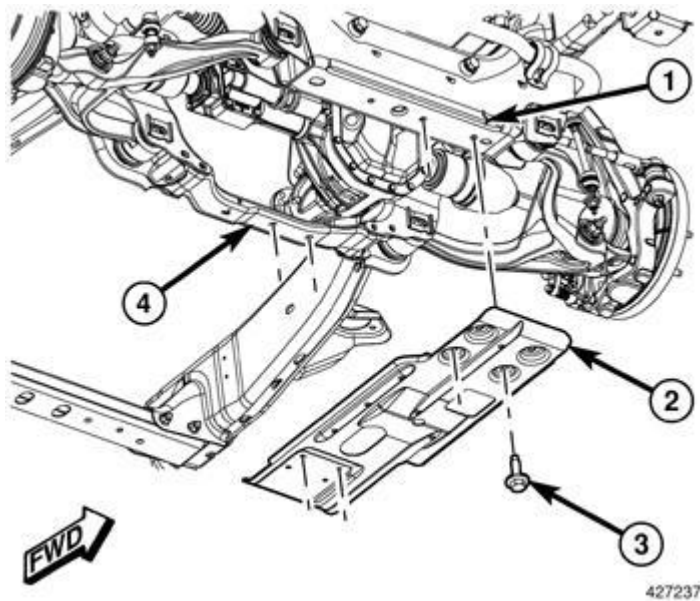
Fig. 375: Removing/Installing Front Skid Plate Courtesy of CHRYSLER GROUP, LLC
