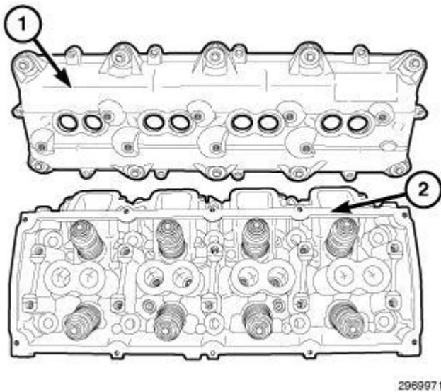
Fig. 84: Cylinder Head & Cover
