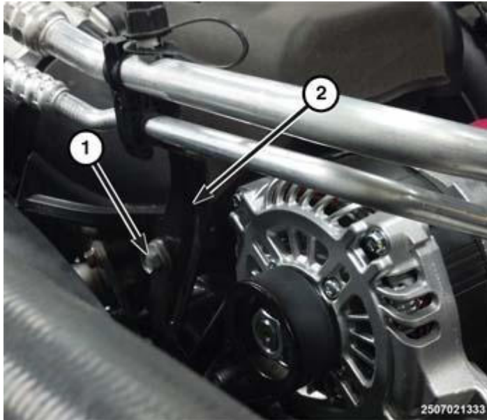
Fig. 341: A/C Line Support Bracket Courtesy of CHRYSLER GROUP, LLC
