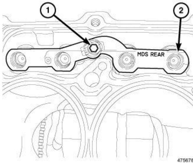
Fig. 191: Rear MDS Lifter Assembly Courtesy of CHRYSLER GROUP, LLC
