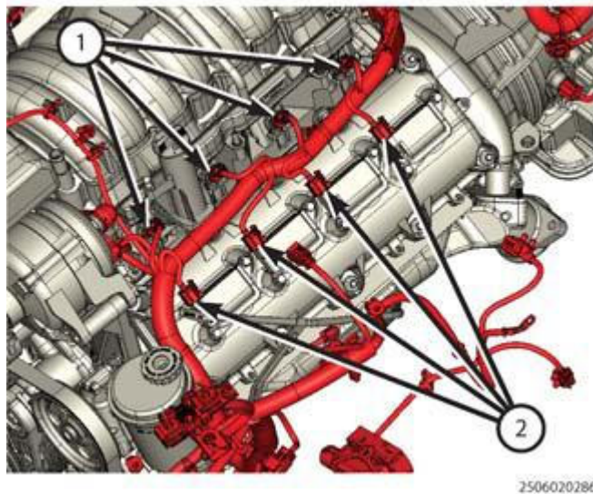
Fig. 327: Injectors Harness Connectors & Ignition Coil Harness Connectors Courtesy of CHRYSLER GROUP, LLC
