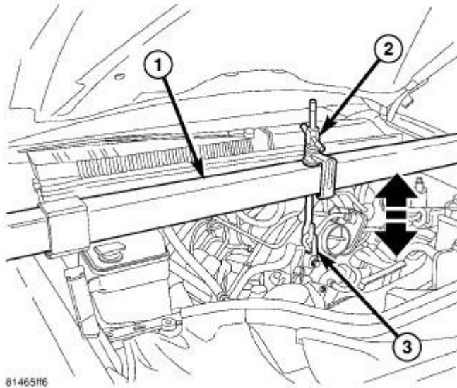
Fig. 251: Engine Support Tool
