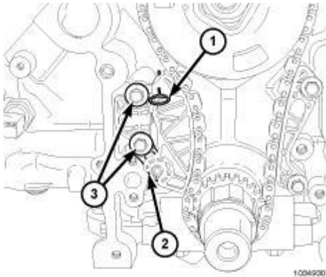
Fig. 351: Timing Chain Tensioner Pin & Bolts Courtesy of CHRYSLER GROUP, LLC
