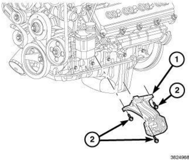
Fig. 249: Engine Mount & Bolts Courtesy of CHRYSLER GROUP, LLC
