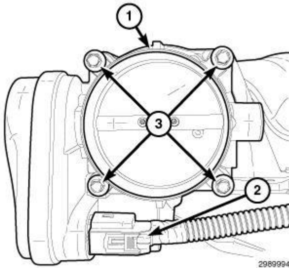
Fig. 330: Throttle Body, Connector & Bolts Courtesy of CHRYSLER GROUP, LLC
