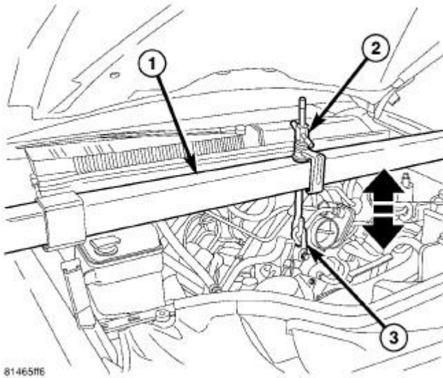
Fig. 274: Engine Support Tool Courtesy of CHRYSLER GROUP, LLC
