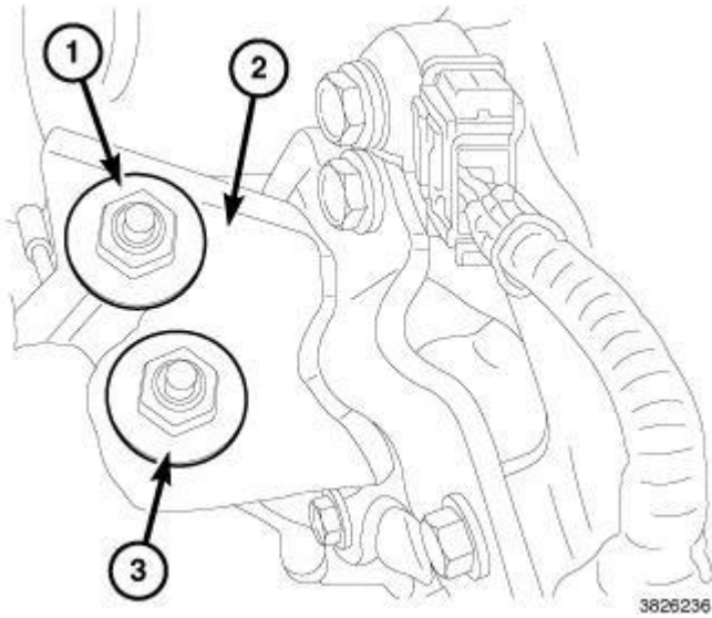
Fig. 252: Upper Engine Bracket, Mount & Bolts - Left Courtesy of CHRYSLER GROUP, LLC
