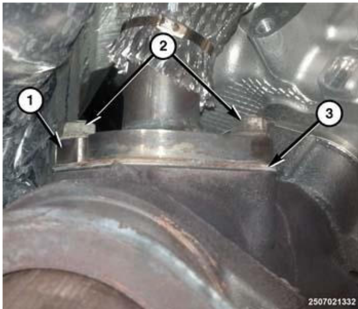
Fig. 303: Remove/Install Inlet Tube Courtesy of CHRYSLER GROUP, LLC
