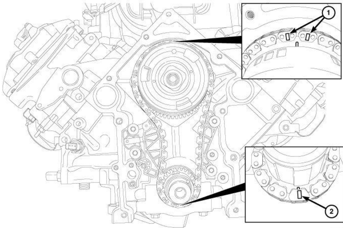
Fig. 361: Aligning Timing Marks With Timing Chain Sprockets Courtesy of CHRYSLER GROUP, LLC
