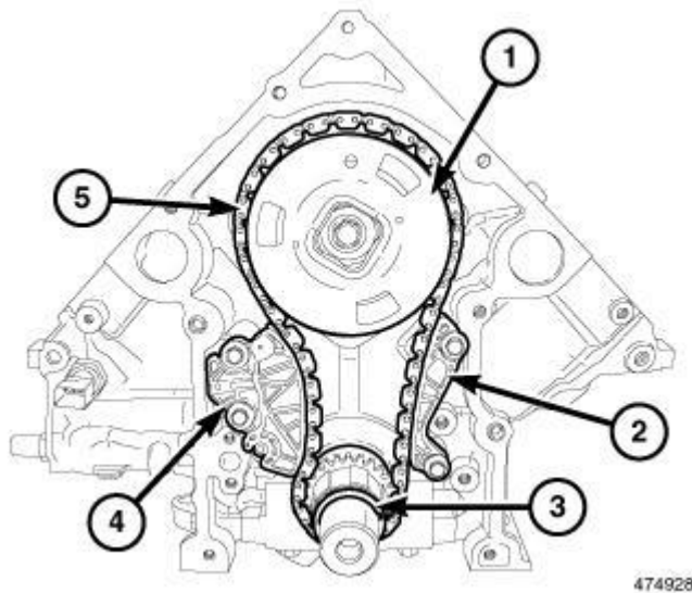
Fig. 162: Timing Chain, Sprockets, Timing Chain Tensioner & Guide
