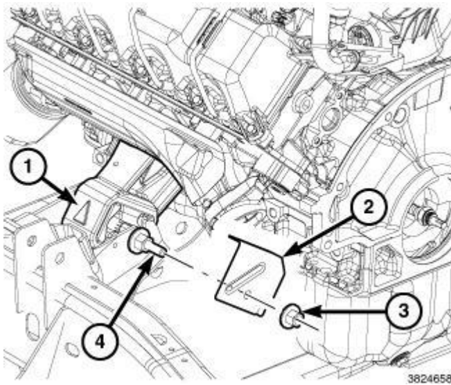
Fig. 250: Engine Mount, Heat Shield & Fasteners Courtesy of CHRYSLER GROUP, LLC
