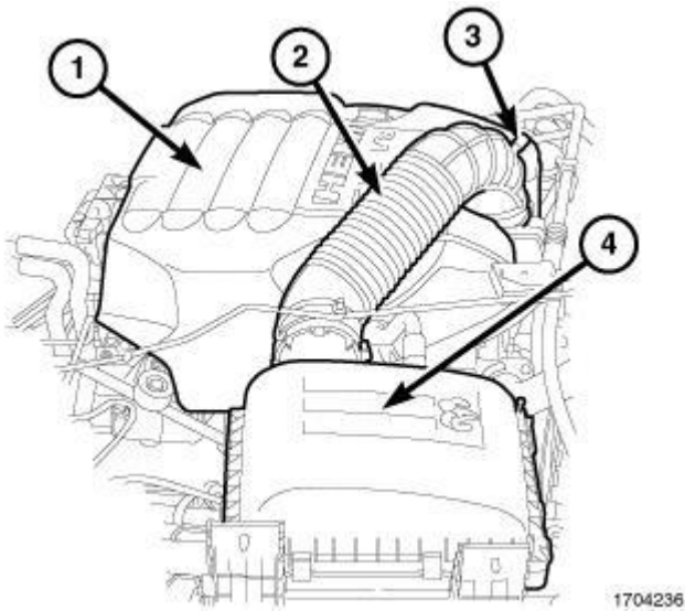
Fig. 366: Engine Cover, Clean Air Hose, Intake Air Temperature (IAT) Sensor Electrical Connector & Air Cleaner Housing
