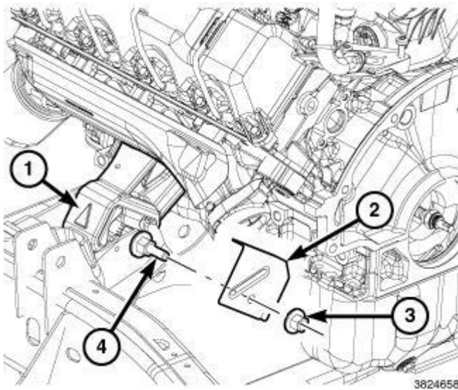
Fig. 230: Engine Mount, Heat Shield & Fasteners Courtesy of CHRYSLER GROUP, LLC
