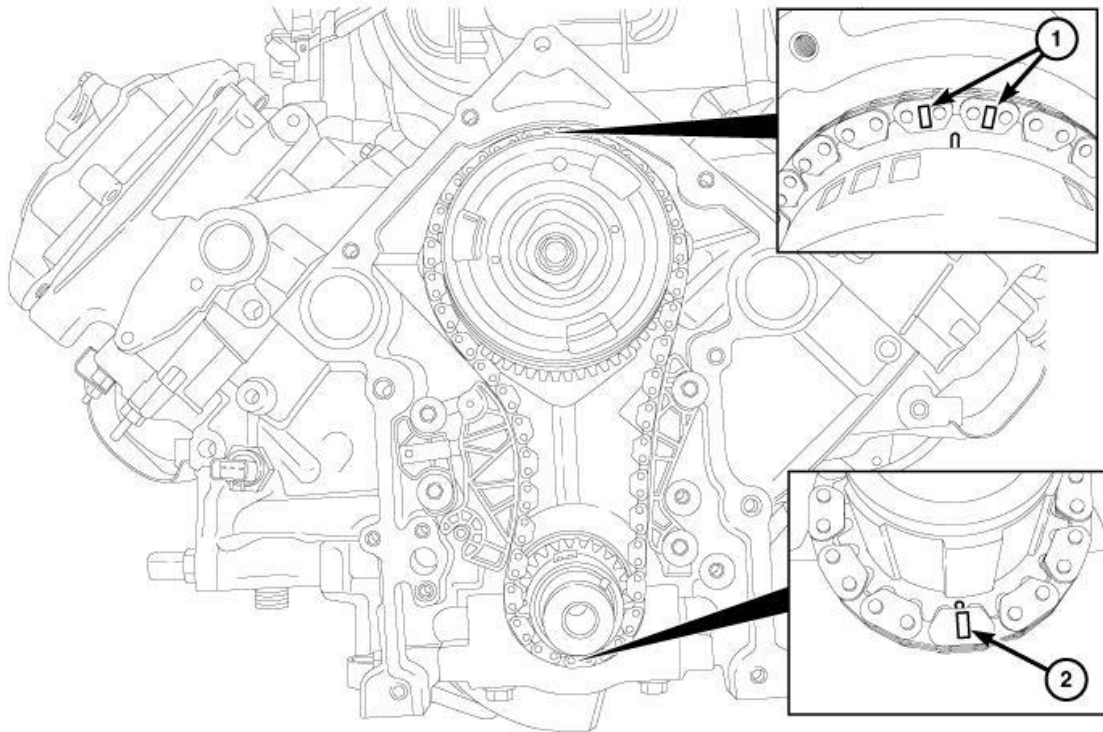
Fig. 349: Aligning Timing Marks With Timing Chain Sprockets Courtesy of CHRYSLER GROUP, LLC
