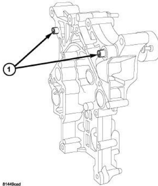
Fig. 347: Front Cover Slide Bushings Courtesy of CHRYSLER GROUP, LLC
