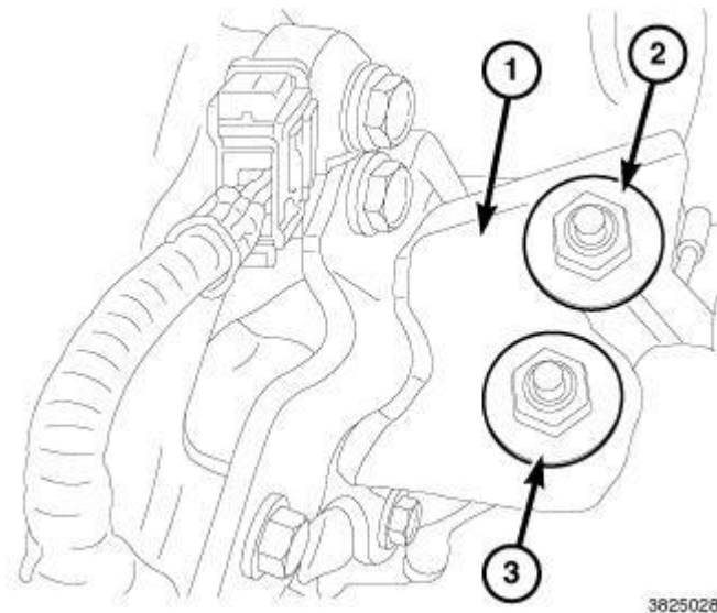
Fig. 248: Upper Engine Bracket, Mount & Bolts - Right Courtesy of CHRYSLER GROUP, LLC
