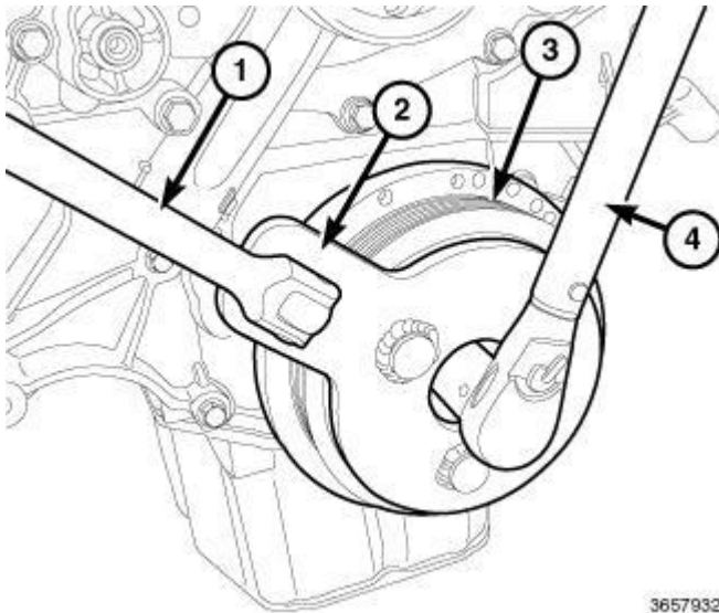
Fig. 179: Installing Vibration Damper Courtesy of CHRYSLER GROUP, LLC
