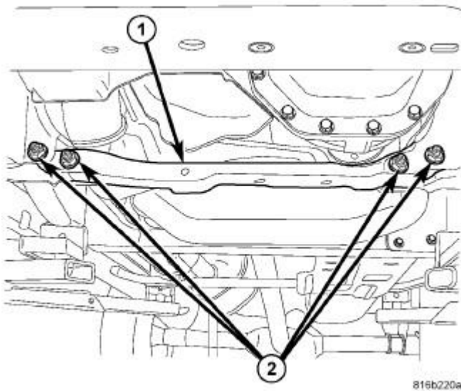
Fig. 244: Suspension Crossmember & Bolts Courtesy of CHRYSLER GROUP, LLC
