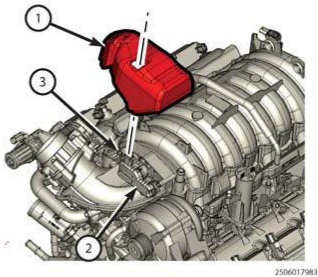
Fig. 332: Short Runner Valve Components Courtesy of CHRYSLER GROUP, LLC
