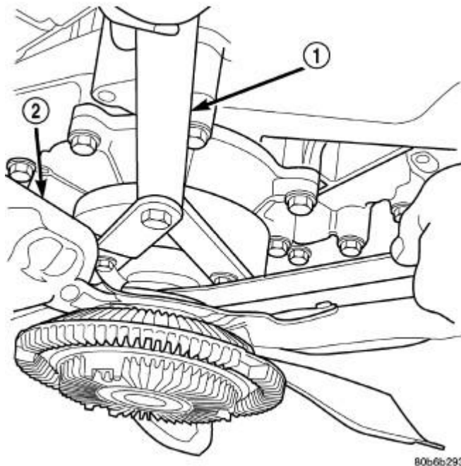
Fig. 392: Using Special Tool 6958 Spanner Wrench Courtesy of CHRYSLER GROUP, LLC
