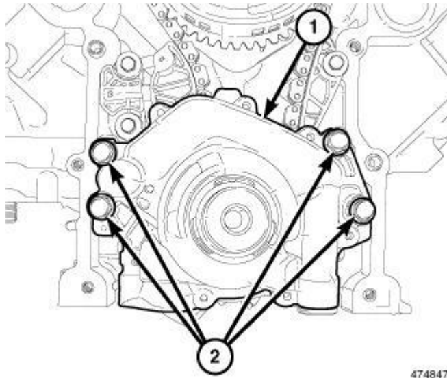
Fig. 161: Oil Pump Retaining Bolts
