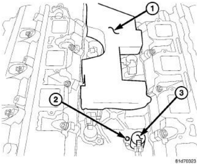
Fig. 223: Intake Manifold Foam Insulator Pad, MDS Solenoids & Bolts Courtesy of CHRYSLER GROUP, LLC
