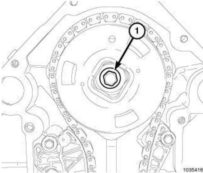
Fig. 362: Camshaft Phaser Retaining Bolt Courtesy of CHRYSLER GROUP, LLC
