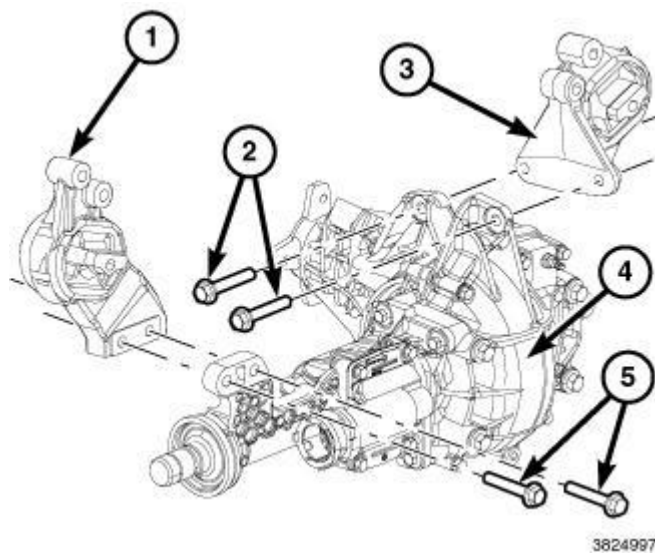
Fig. 387: Engine Mounts, Front Axle & Bolts Courtesy of CHRYSLER GROUP, LLC
