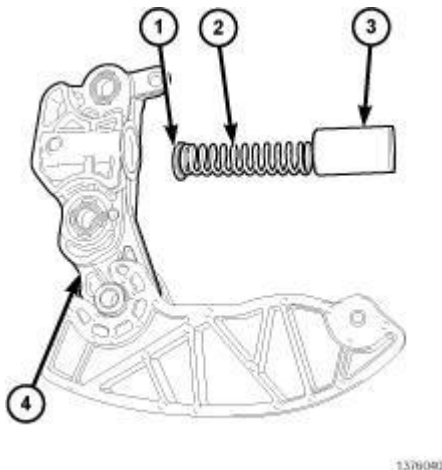
Fig. 394: Tensioner Body, Washer, Spring & Plunger Courtesy of CHRYSLER GROUP, LLC
