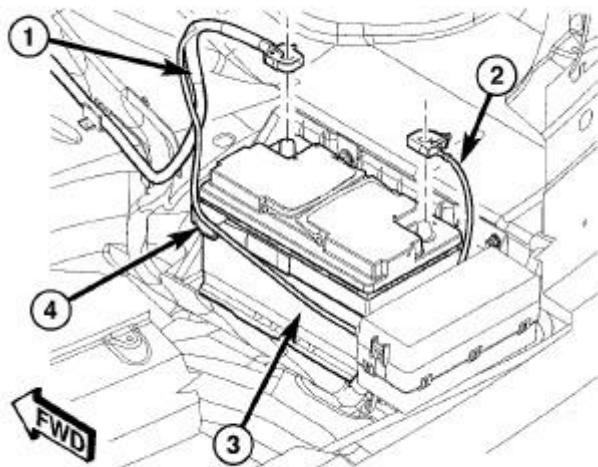
Fig. 60: Disconnecting/Connecting Battery Cables
