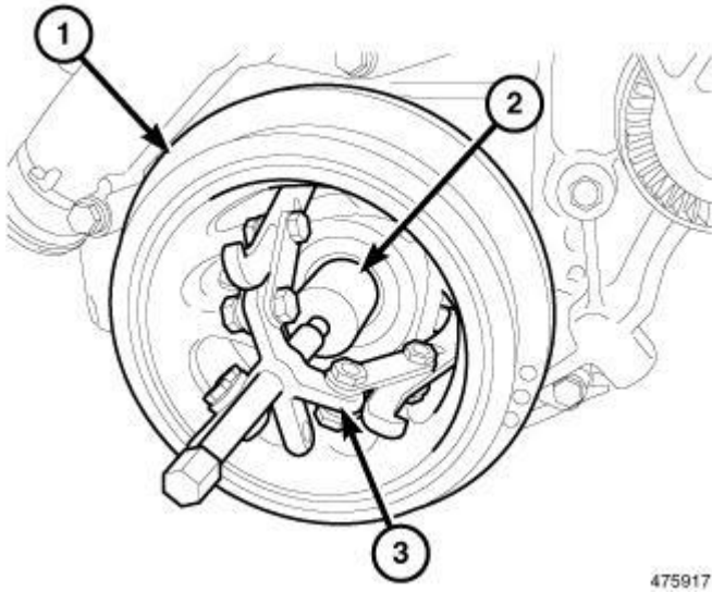
Fig. 220: Removing Vibration Damper Courtesy of CHRYSLER GROUP, LLC
