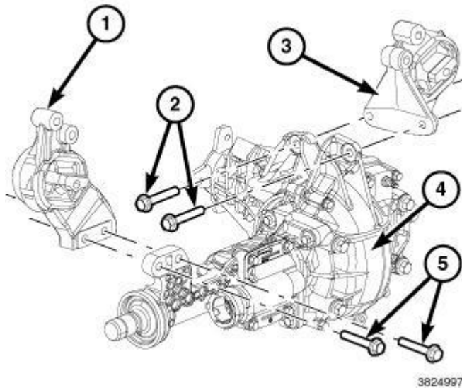
Fig. 245: Engine Mounts, Front Axle & Bolts Courtesy of CHRYSLER GROUP, LLC
