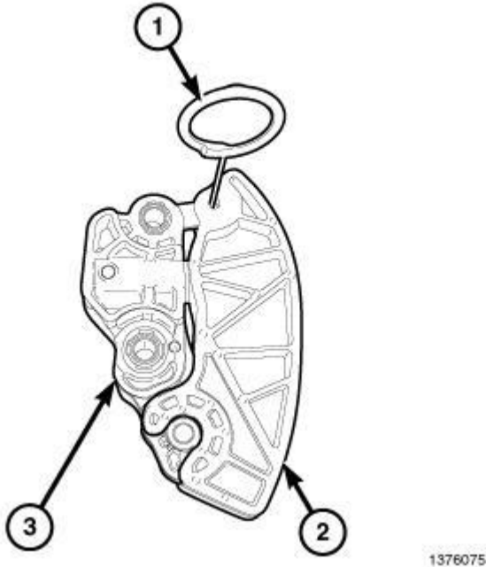
Fig. 395: Tensioner Pin, Guide Shoe & Tensioner Body Courtesy of CHRYSLER GROUP, LLC
