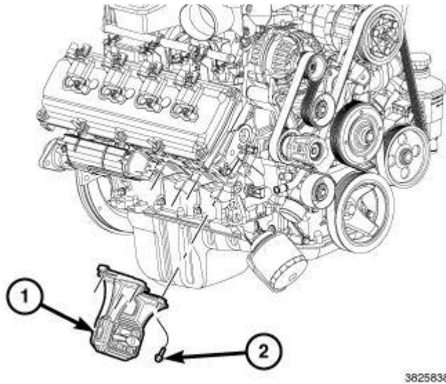
Fig. 241: Engine Mount & Bolts Courtesy of CHRYSLER GROUP, LLC
