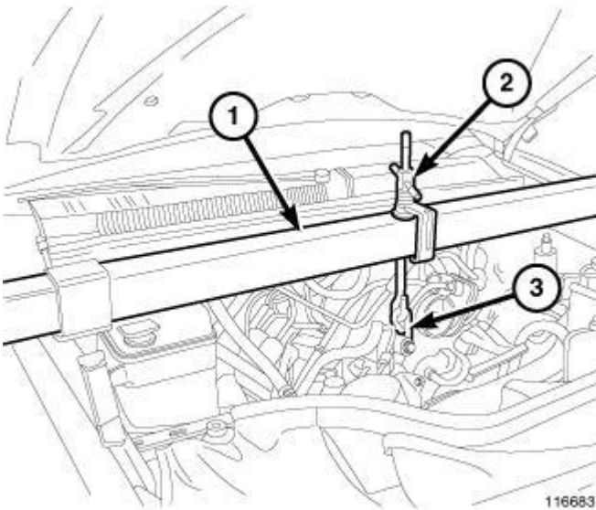
Fig. 242: Engine Support Tool Courtesy of CHRYSLER GROUP, LLC
