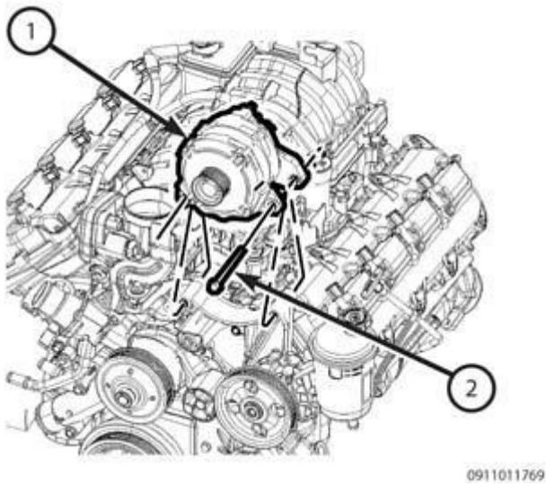
Fig. 371: Remove/Install Generator Courtesy of CHRYSLER GROUP, LLC
