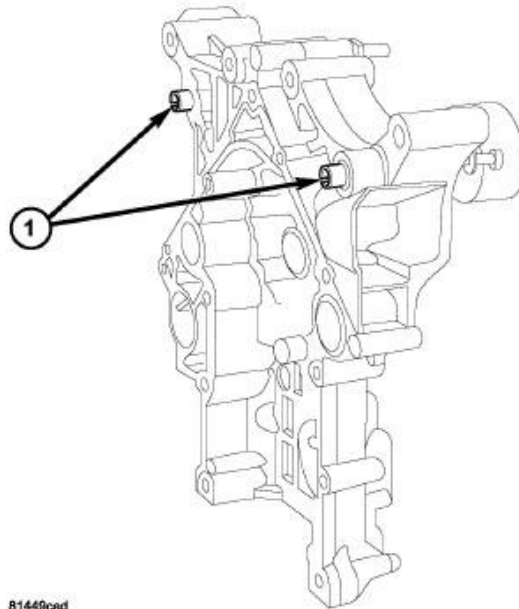
Fig. 365: Front Cover Slide Bushings Courtesy of CHRYSLER GROUP, LLC
