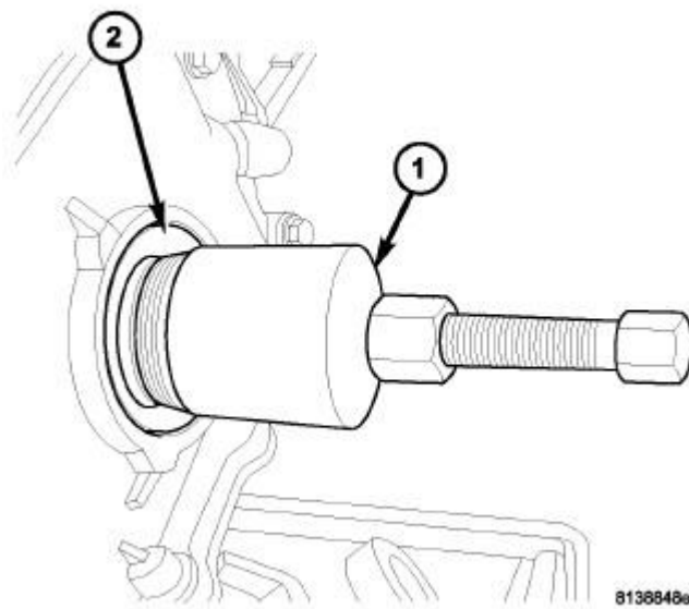
Fig. 222: Front Crankshaft Seal Removal Courtesy of CHRYSLER GROUP, LLC
