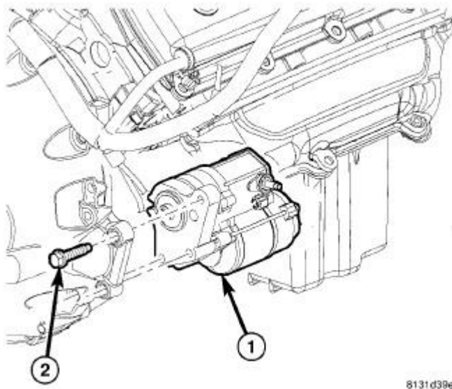
Fig. 12: Starter & Fasteners
