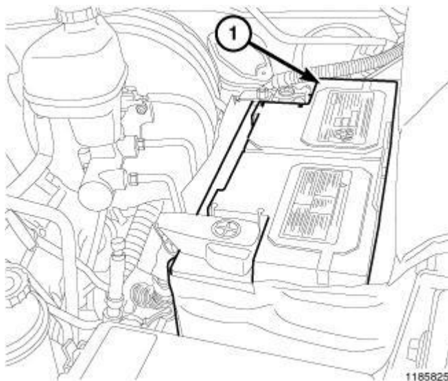
Fig. 300: Battery
