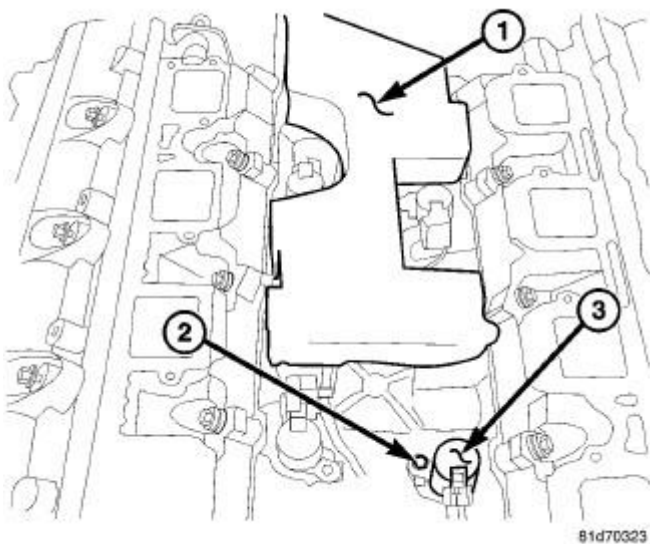
Fig. 224: Intake Manifold Foam Insulator Pad, MDS Solenoids & Bolts Courtesy of CHRYSLER GROUP, LLC
