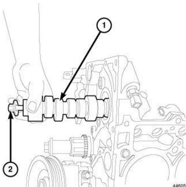
Fig. 140: Removing/Installing Camshaft
