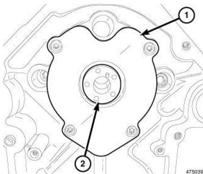
Fig. 141: Camshaft Thrust Plate
