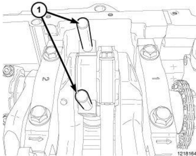
Fig. 209: Connecting Rod Guides
