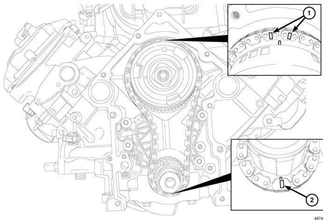
Fig. 347: Aligning Timing Marks With Timing Chain Sprockets
