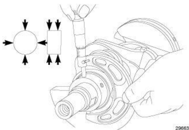
Fig. 128: Measuring Main Bearing Journal Diameter Courtesy of CHRYSLER GROUP, LLC
