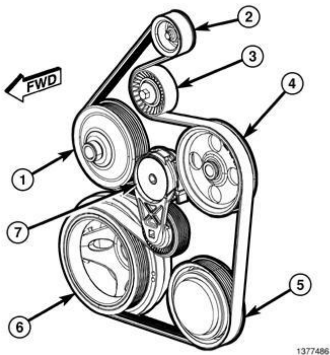
Fig. 63: Accessory Drive Belt Routing, Tensioner & Pulleys Courtesy of CHRYSLER GROUP, LLC
