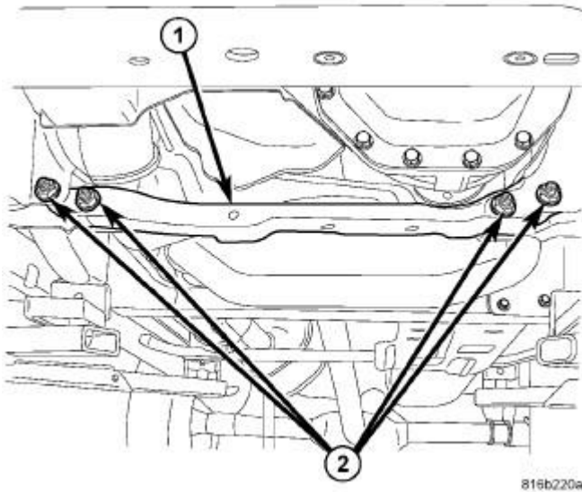
Fig. 243: Suspension Crossmember & Bolts
