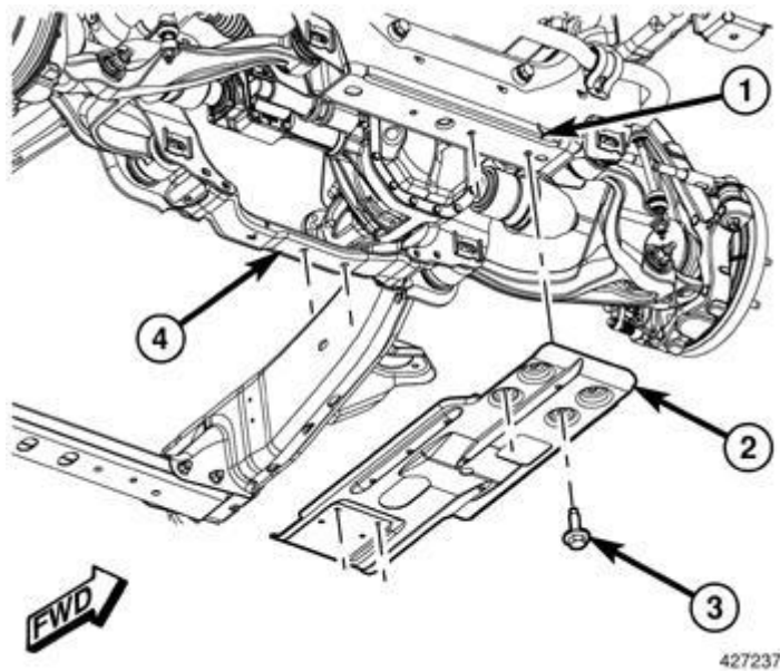
Fig. 257: Removing/Installing Front Skid Plate Courtesy of CHRYSLER GROUP, LLC
