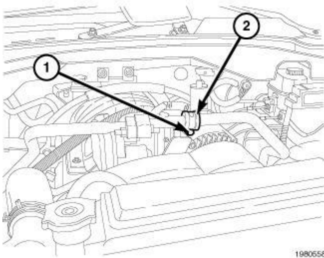
Fig. 319: A/C Line P-Clip & Retaining Bolt Courtesy of CHRYSLER GROUP, LLC
