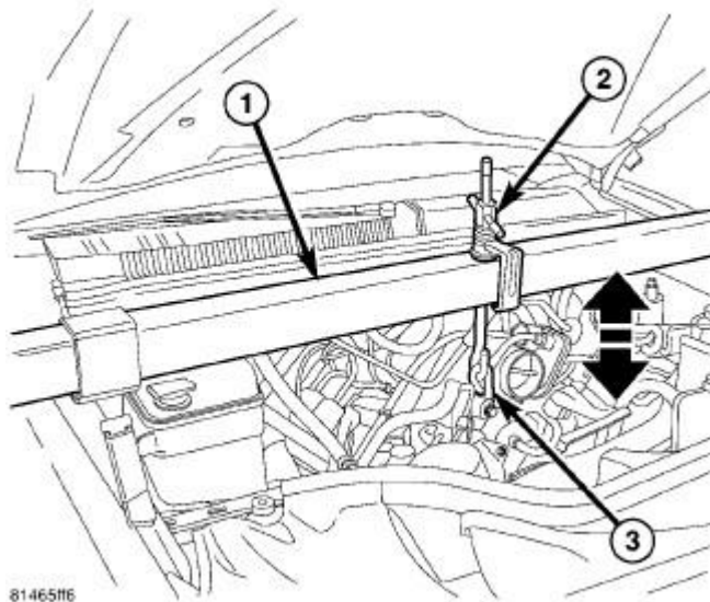
Fig. 269: Engine Support Tool Courtesy of CHRYSLER GROUP, LLC
