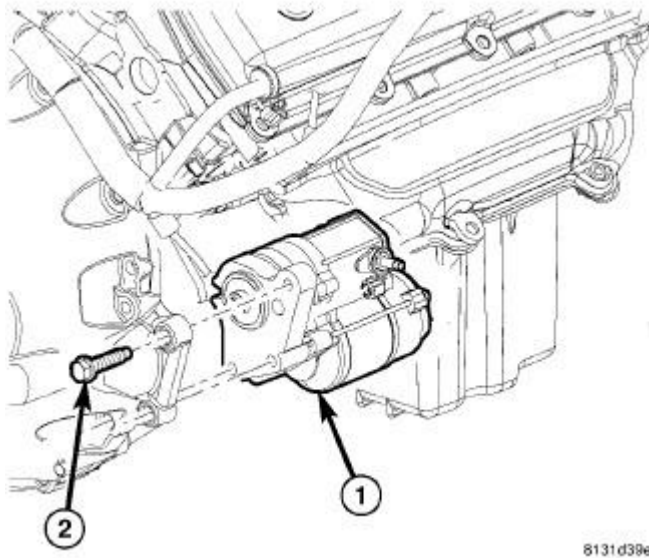
Fig. 27: Starter & Fasteners Courtesy of CHRYSLER GROUP, LLC
