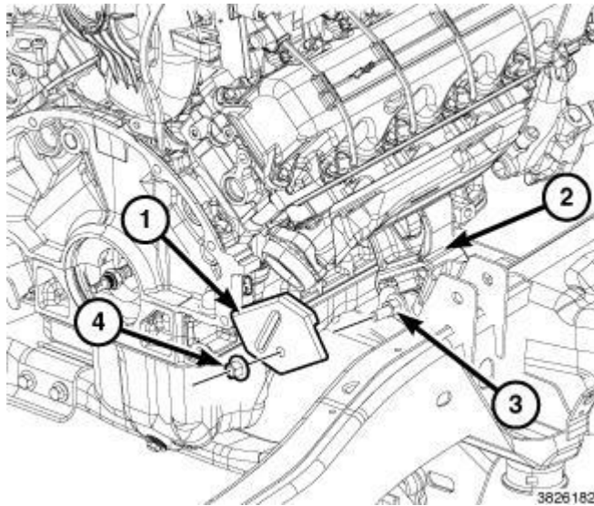
Fig. 246: Engine Mount, Heat Shield & Fasteners Courtesy of CHRYSLER GROUP, LLC
