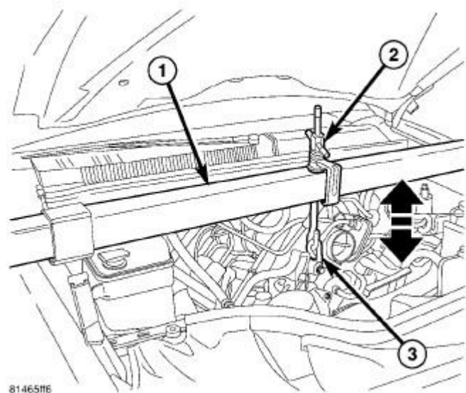
Fig. 299: Engine Support Tool
