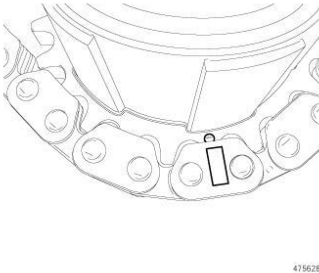
Fig. 341: Aligning Timing Chain & Crankshaft Sprocket Marks Courtesy of CHRYSLER GROUP, LLC
