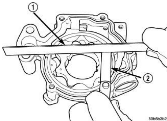
Fig. 287: Measuring Clearance Over Rotors Courtesy of CHRYSLER GROUP, LLC
