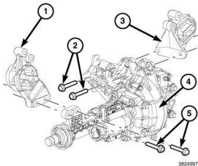
Fig. 244: Engine Mounts, Front Axle & Bolts Courtesy of CHRYSLER GROUP, LLC
