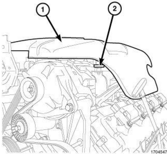
Fig. 328: Engine Cover & Grommets Courtesy of CHRYSLER GROUP, LLC
