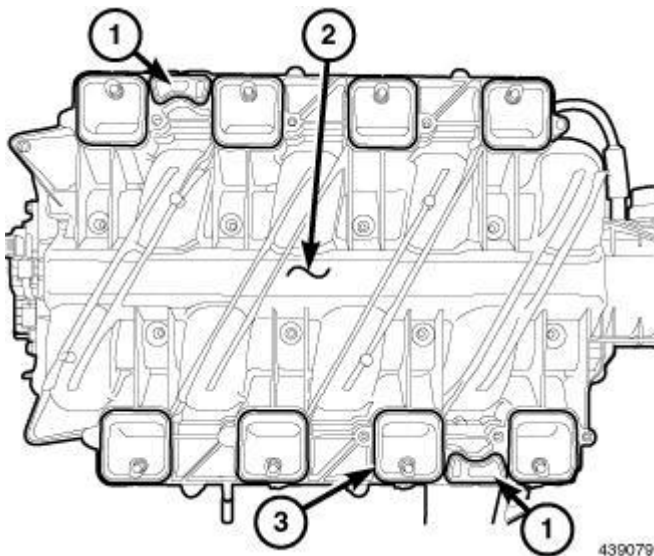
Fig. 322: Intake Manifold & PCV Seals Courtesy of CHRYSLER GROUP, LLC
