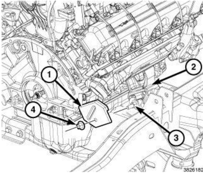
Fig. 263: Engine Mount, Heat Shield & Fasteners Courtesy of CHRYSLER GROUP, LLC
