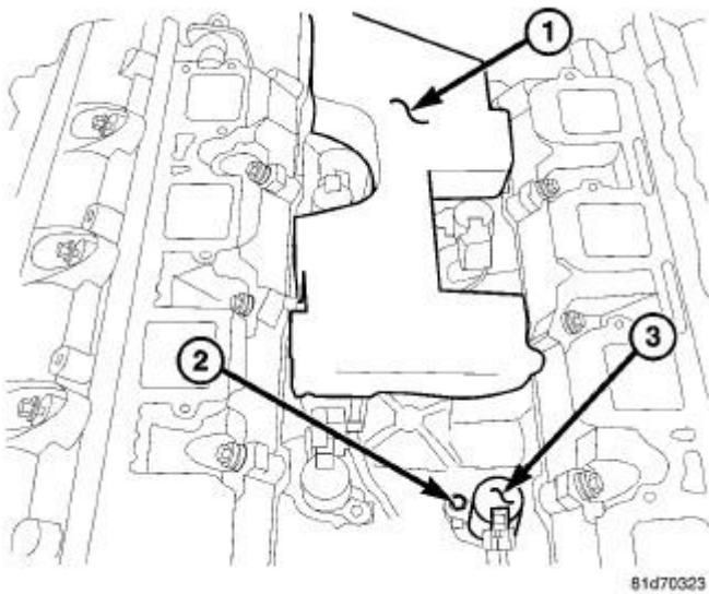
Fig. 222: Intake Manifold Foam Insulator Pad, MDS Solenoids & Bolts Courtesy of CHRYSLER GROUP, LLC
