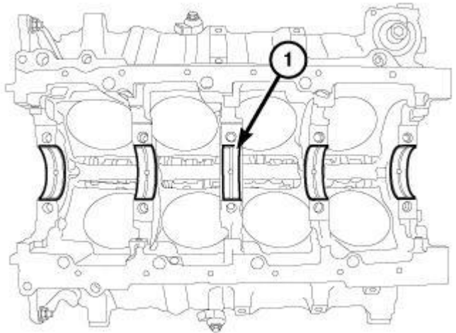
Fig. 167: Main Bearings
