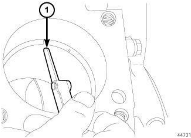
Fig. 193: Checking Piston Ring End Gap Using Feeler Gauge Courtesy of CHRYSLER GROUP, LLC
