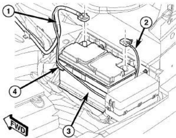
Fig. 60: Battery & Cables
