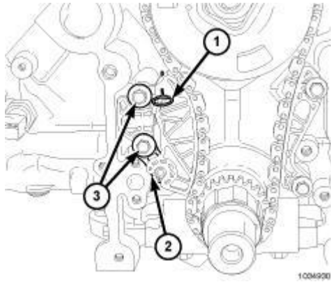
Fig. 344: Timing Chain Tensioner Pin & Bolts Courtesy of CHRYSLER GROUP, LLC
