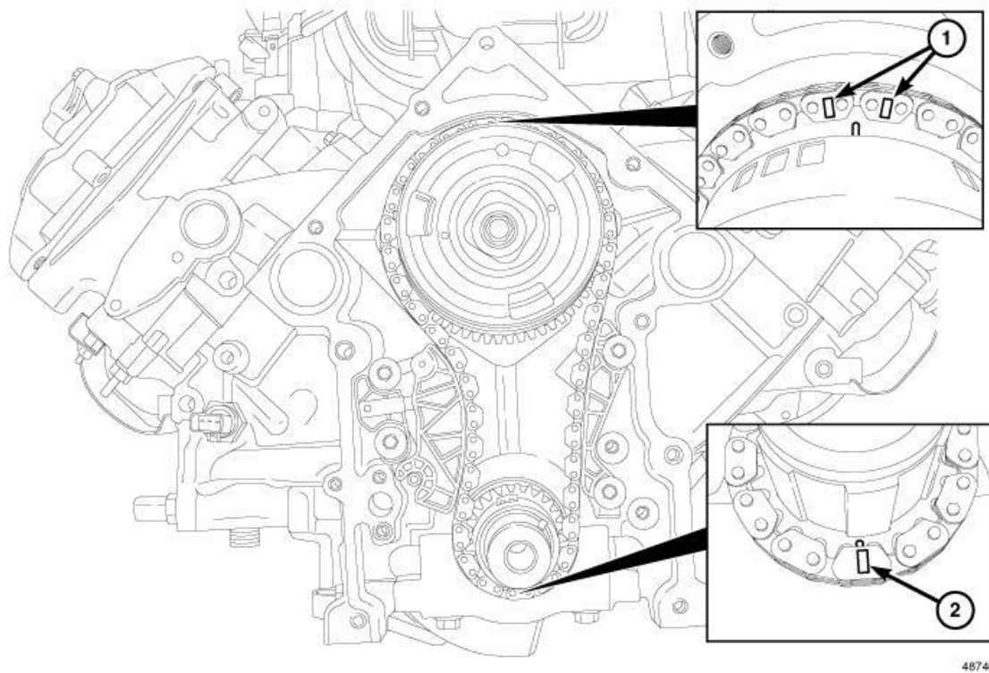
Fig. 345: Aligning Timing Marks With Timing Chain Sprockets Courtesy of CHRYSLER GROUP, LLC
