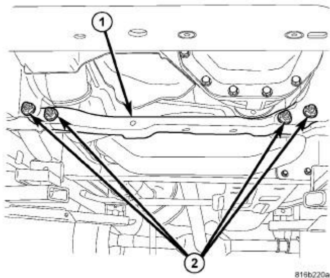
Fig. 233: Suspension Crossmember & Bolts Courtesy of CHRYSLER GROUP, LLC
