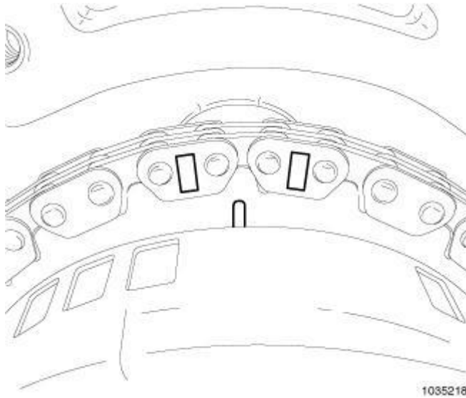
Fig. 340: Aligning Timing Chain & Camshaft Phaser Marks Courtesy of CHRYSLER GROUP, LLC
