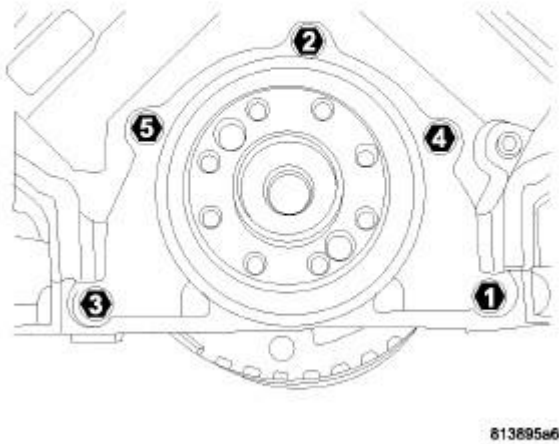
Fig. 192: Rear Seal Retainer Torque Sequence Courtesy of CHRYSLER GROUP, LLC
