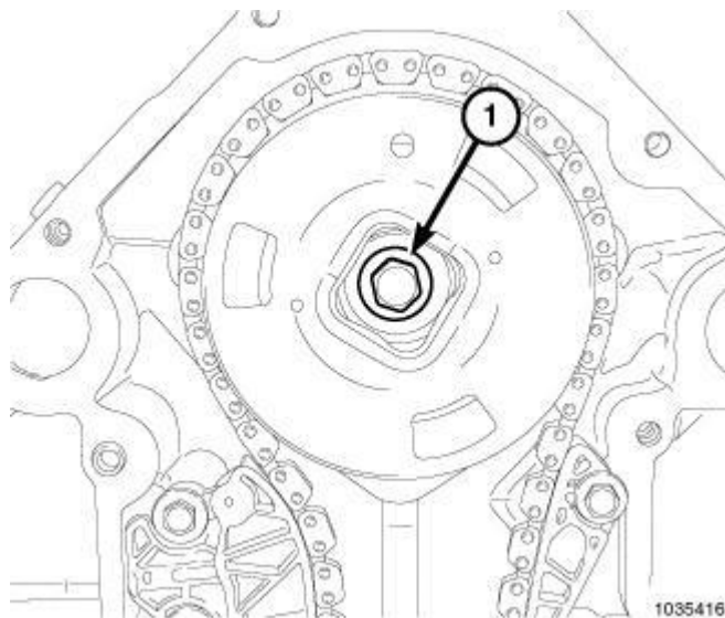
Fig. 346: Camshaft Phaser Retaining Bolt Courtesy of CHRYSLER GROUP, LLC
