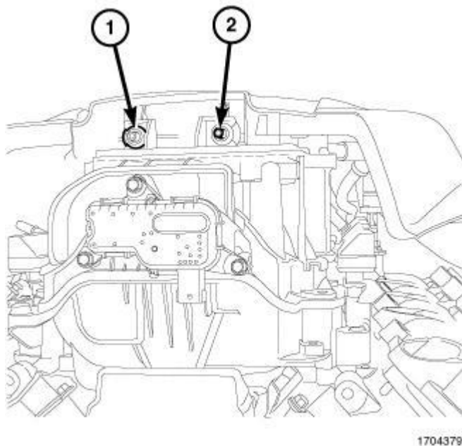
Fig. 316: Engine Cover Pegs & Grommets Courtesy of CHRYSLER GROUP, LLC
