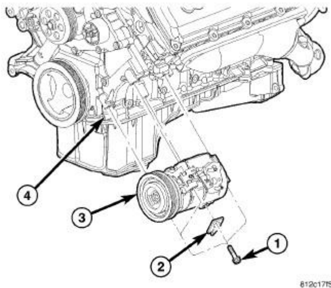
Fig. 34: A/C Compressor & Fasteners
