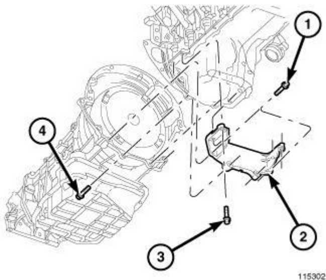
Fig. 276: Structural Cover
