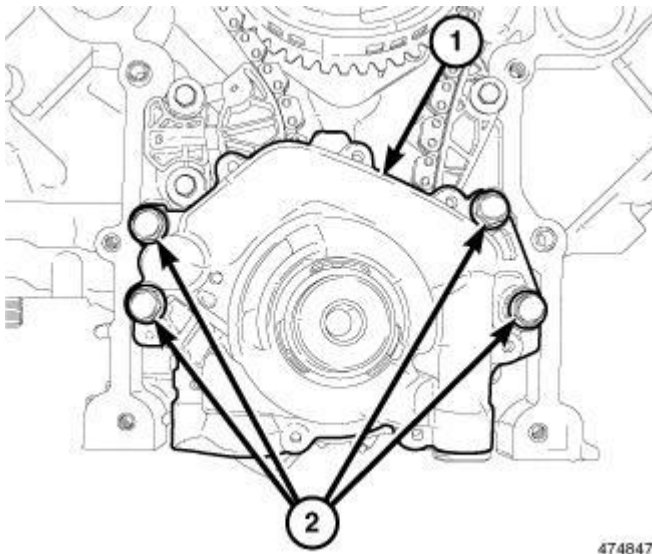
Fig. 284: Oil Pump Retaining Bolts
