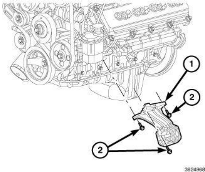
Fig. 230: Engine Mount & Bolts Courtesy of CHRYSLER GROUP, LLC
