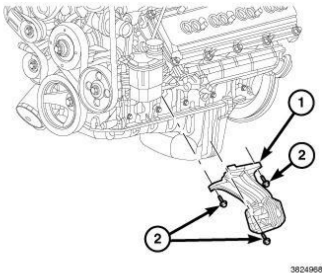
Fig. 248: Engine Mount & Bolts Courtesy of CHRYSLER GROUP, LLC
