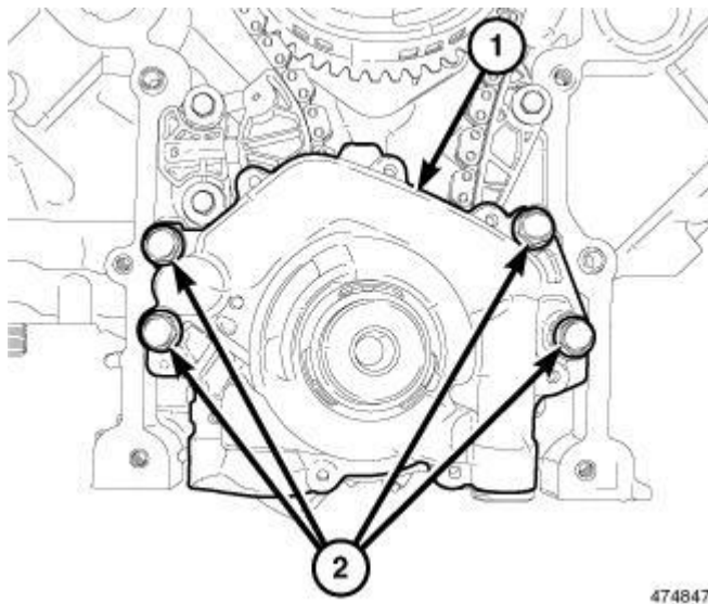
Fig. 332: Oil Pump Retaining Bolts Courtesy of CHRYSLER GROUP, LLC
