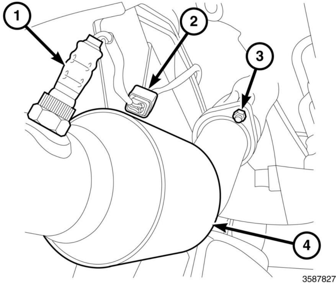
Fig. 310: Oxygen Sensor, Oxygen Sensor Connector, Ball Flange Nut & LH Catalytic Converter Courtesy of CHRYSLER GROUP, LLC
