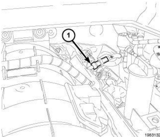
Fig. 318: Fuel Supply Line Quick Connect Fitting At Fuel Rail Courtesy of CHRYSLER GROUP, LLC
