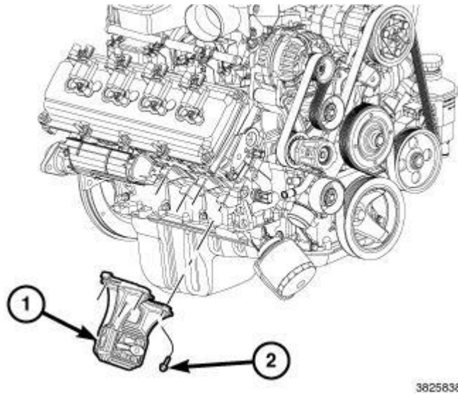
Fig. 240: Engine Mount & Bolts Courtesy of CHRYSLER GROUP, LLC
