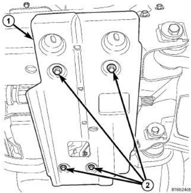
Fig. 242: Skid Plate & Bolts
