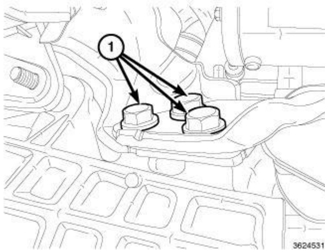
Fig. 266: Pinion Nose Mounting Bolts Courtesy of CHRYSLER GROUP, LLC
