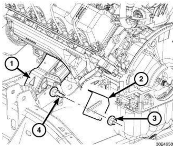
Fig. 249: Engine Mount, Heat Shield & Fasteners Courtesy of CHRYSLER GROUP, LLC
