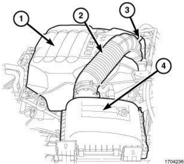
Fig. 311: Engine Cover, Clean Air Hose, Intake Air Temperature (IAT) Sensor Electrical Connector & Air Cleaner Housing Courtesy of CHRYSLER GROUP, LLC
