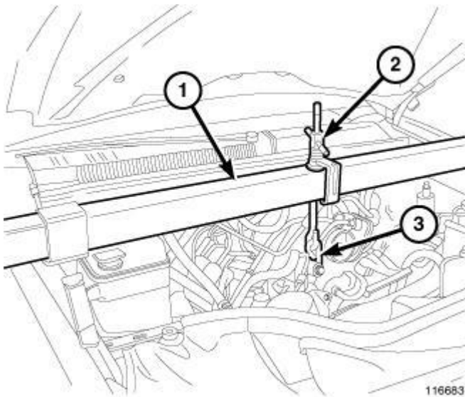
Fig. 241: Engine Support Tool Courtesy of CHRYSLER GROUP, LLC
