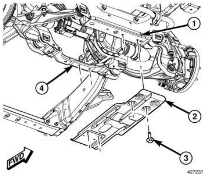
Fig. 268: Removing/Installing Front Skid Plate Courtesy of CHRYSLER GROUP, LLC
