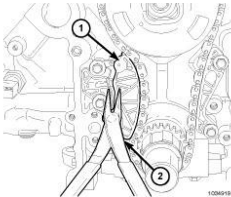
Fig. 334: Retracting Tensioner Shoe Using Pliers Courtesy of CHRYSLER GROUP, LLC
