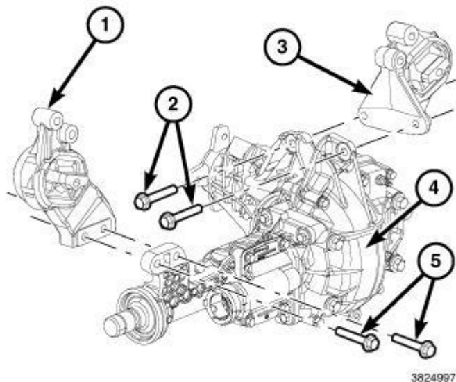
Fig. 234: Engine Mounts, Front Axle & Bolts Courtesy of CHRYSLER GROUP, LLC
