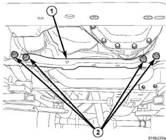
Fig. 256: Suspension Crossmember & Bolts Courtesy of CHRYSLER GROUP, LLC
