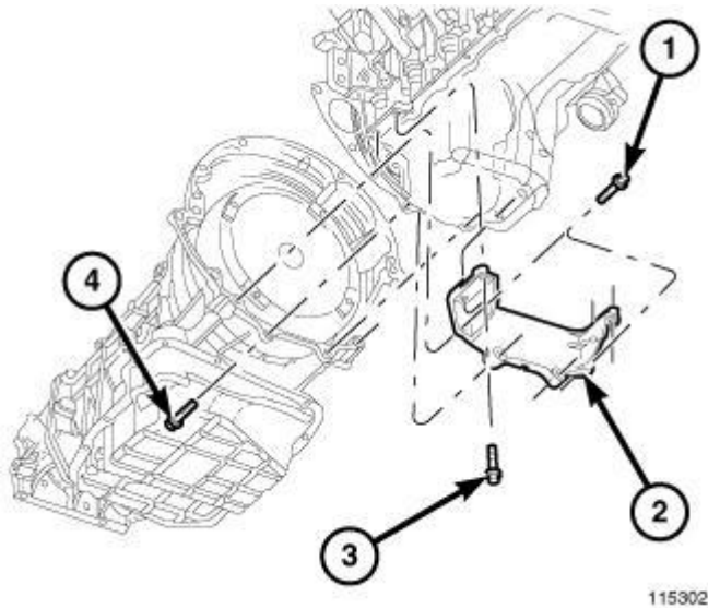
Fig. 282: Structural Cover Courtesy of CHRYSLER GROUP, LLC
