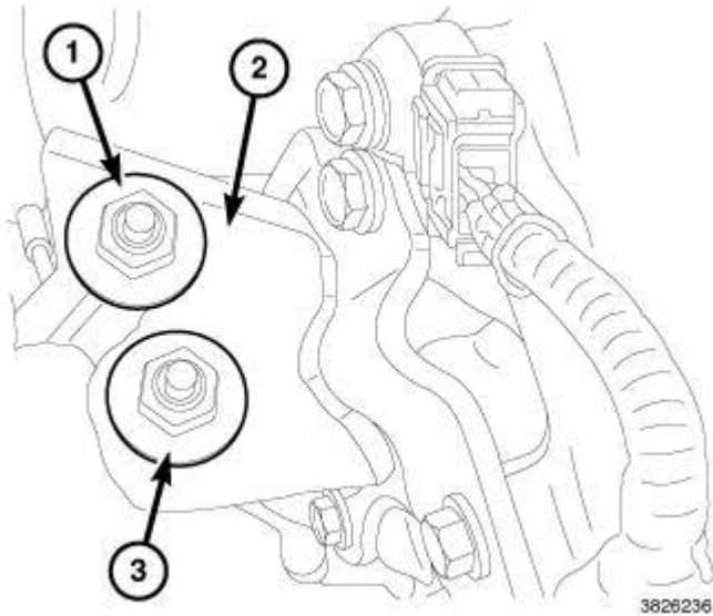
Fig. 251: Upper Engine Bracket, Mount & Bolts - Left Courtesy of CHRYSLER GROUP, LLC
