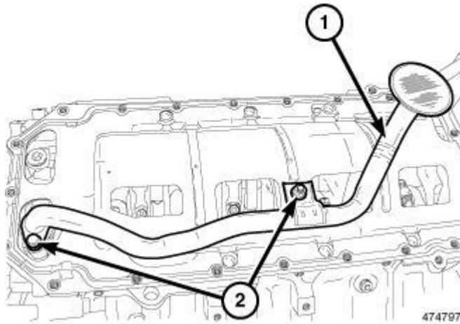
Fig. 177: Oil Pick Up Tube
