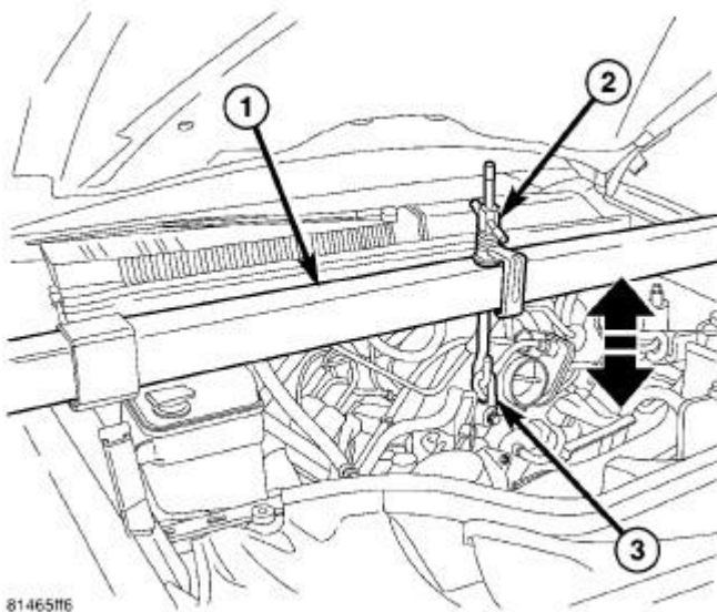
Fig. 275: Engine Support Tool
