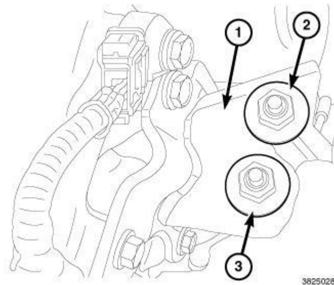
Fig. 247: Upper Engine Bracket, Mount & Bolts - Right Courtesy of CHRYSLER GROUP, LLC
