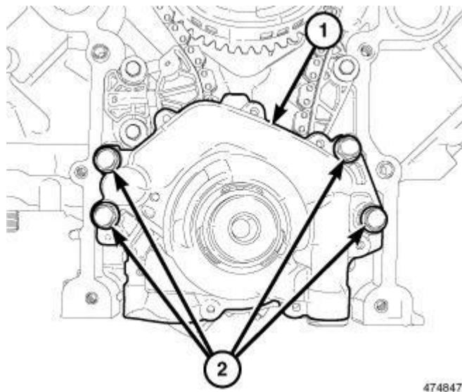
Fig. 347: Oil Pump Retaining Bolts Courtesy of CHRYSLER GROUP, LLC
