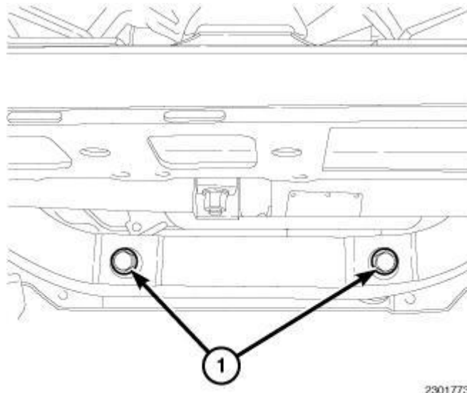
Fig. 152: Steering Rack To Frame Mounting Bolts Courtesy of CHRYSLER GROUP, LLC
