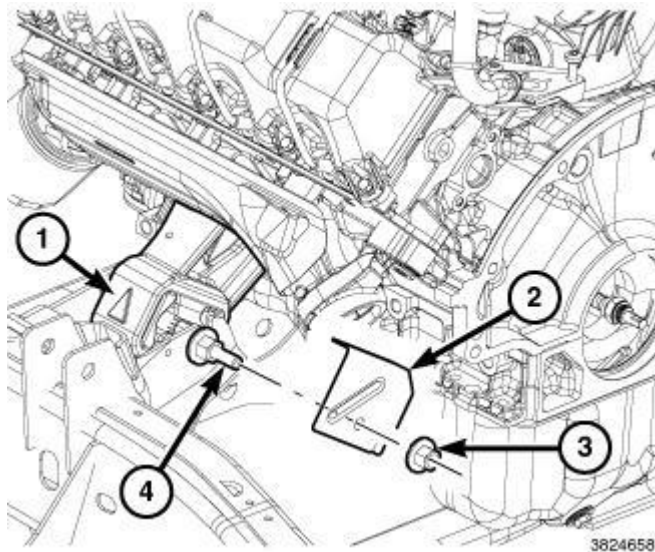
Fig. 236: Engine Mount, Heat Shield & Fasteners Courtesy of CHRYSLER GROUP, LLC
