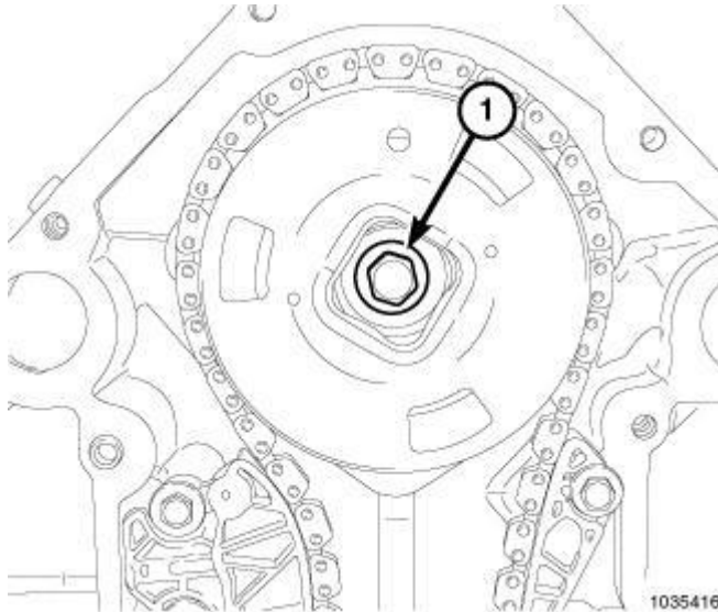
Fig. 342: Camshaft Phaser Retaining Bolt Courtesy of CHRYSLER GROUP, LLC
