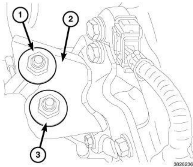
Fig. 237: Upper Engine Bracket, Mount & Bolts - Left Courtesy of CHRYSLER GROUP, LLC
