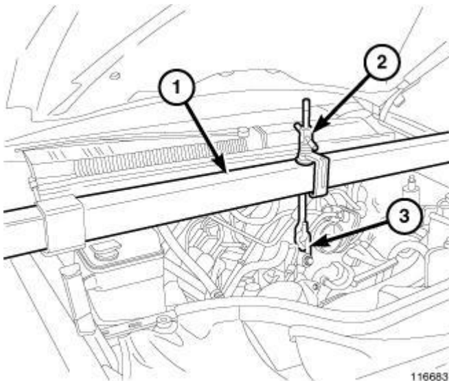
Fig. 238: Engine Support Tool Courtesy of CHRYSLER GROUP, LLC
