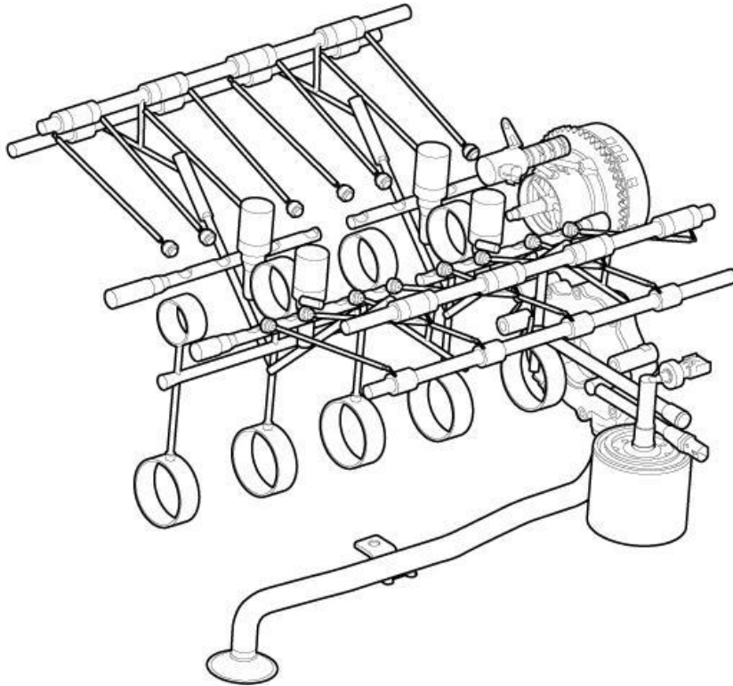
Fig. 270: 5.7L MDS Lubrication System Courtesy of CHRYSLER GROUP, LLC
