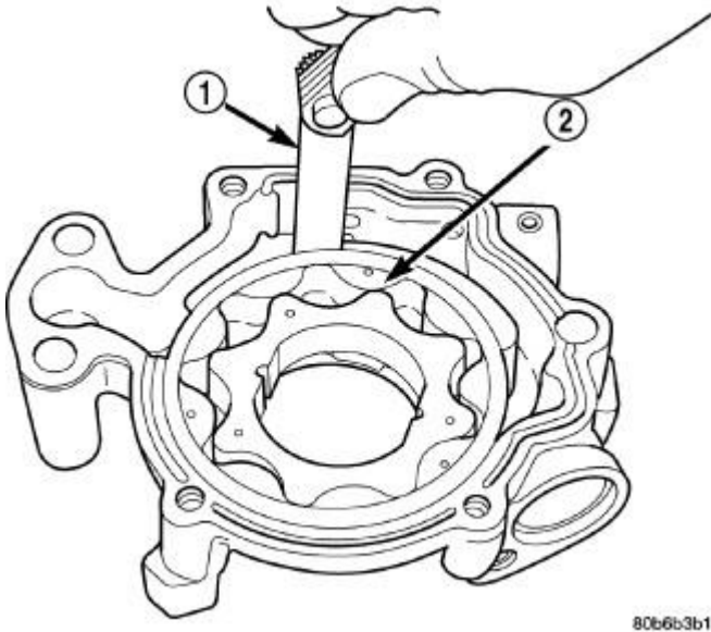
Fig. 285: Measuring Clearance Between Outer Rotor & Body Of Oil Pump Courtesy of CHRYSLER GROUP, LLC
