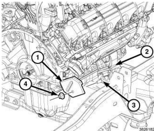
Fig. 260: Engine Mount, Heat Shield & Fasteners Courtesy of CHRYSLER GROUP, LLC
