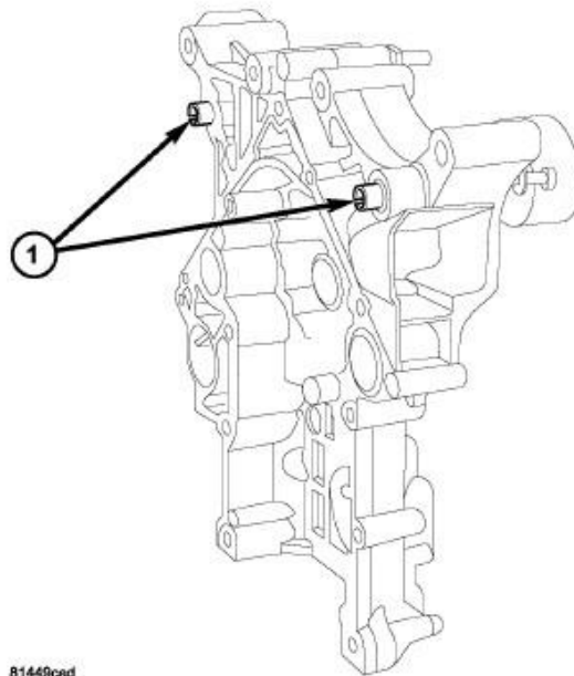
Fig. 349: Front Cover Slide Bushings Courtesy of CHRYSLER GROUP, LLC
