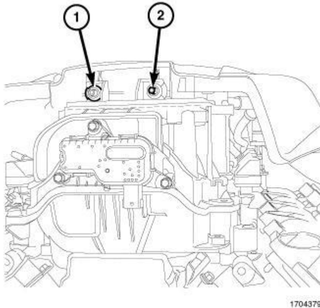
Fig. 327: Engine Cover Pegs & Grommets Courtesy of CHRYSLER GROUP, LLC
