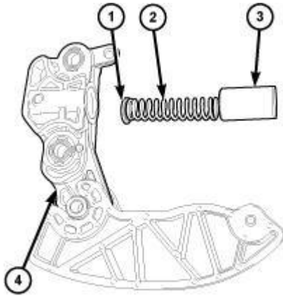
Fig. 354: Tensioner Body, Washer, Spring & Plunger Courtesy of CHRYSLER GROUP, LLC
