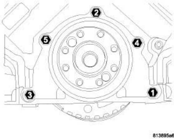
Fig. 191: Rear Seal Retainer Torque Sequence Courtesy of CHRYSLER GROUP, LLC
