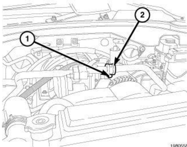
Fig. 326: A/C Line P-Clip & Retaining Bolt
