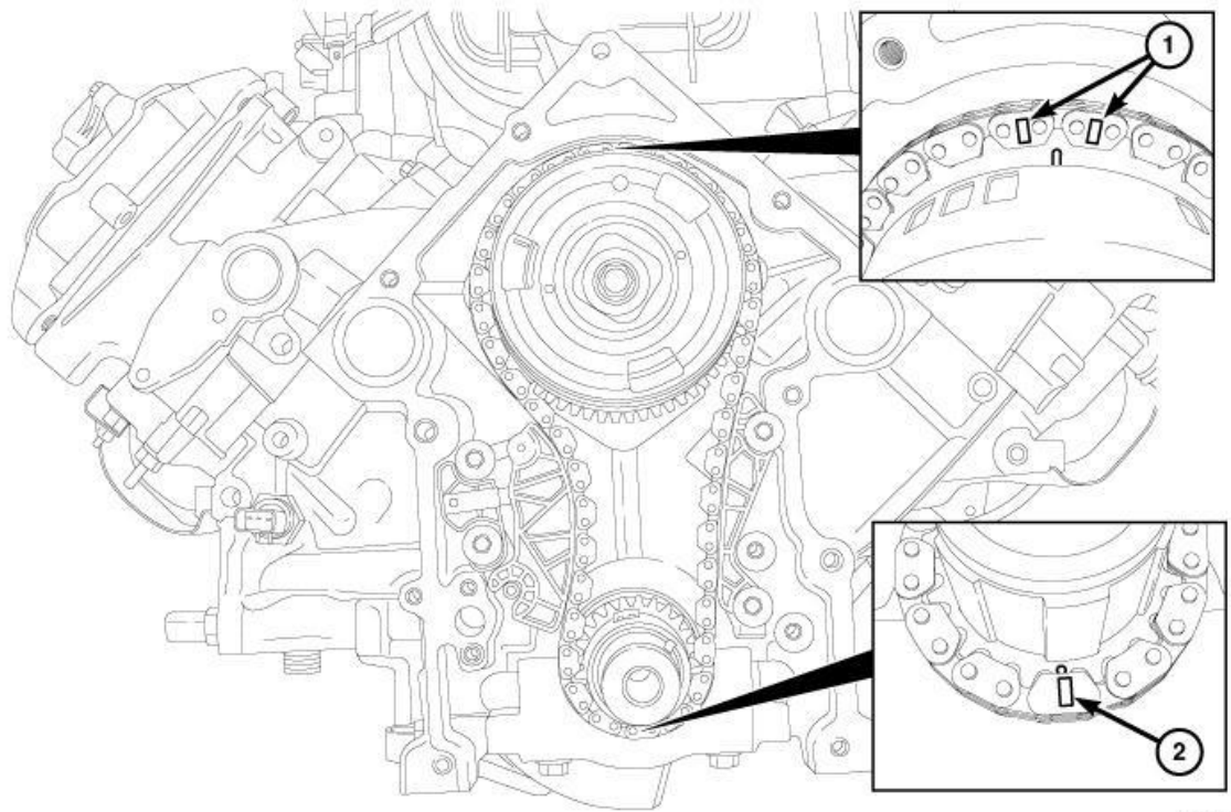
Fig. 333: Aligning Timing Marks With Timing Chain Sprockets Courtesy of CHRYSLER GROUP, LLC
