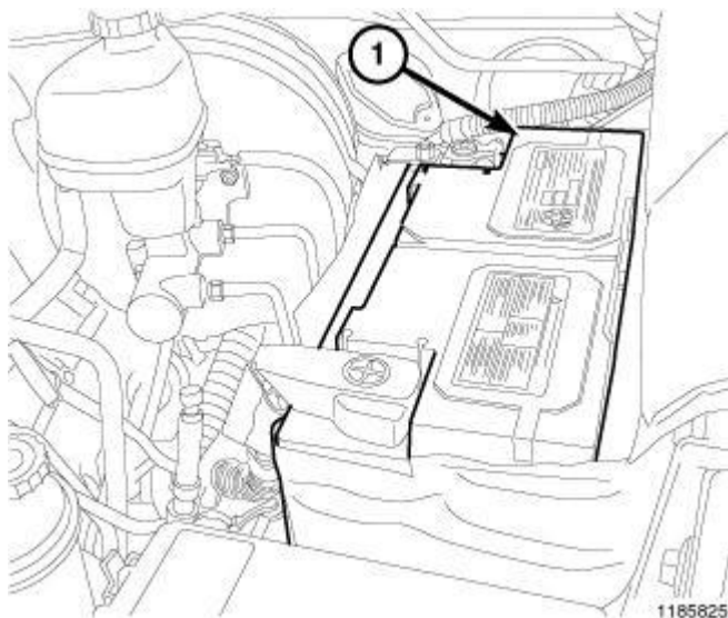
Fig. 312: Battery Courtesy of CHRYSLER GROUP, LLC
