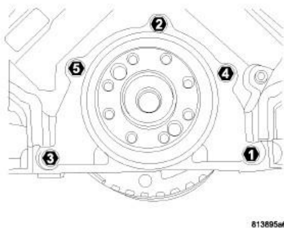
Fig. 176: Rear Seal Retainer Torque Sequence
