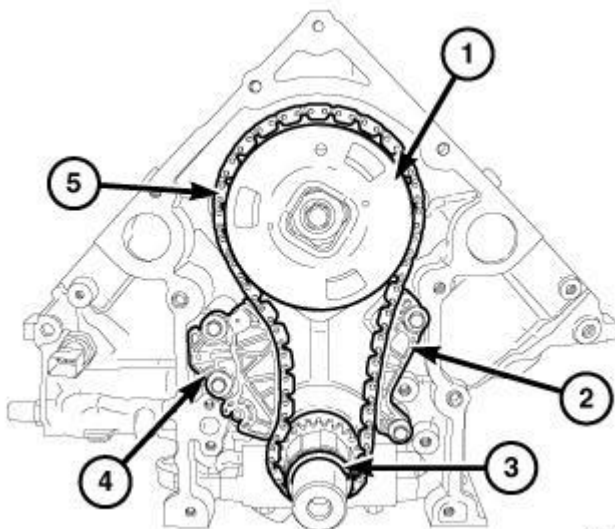
Fig. 174: Timing Chain, Sprockets, Timing Chain Tensioner & Guide Courtesy of CHRYSLER GROUP, LLC
