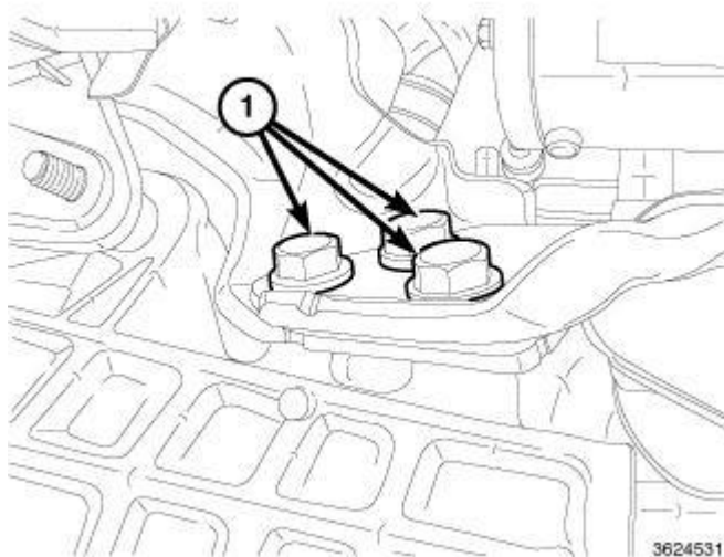
Fig. 255: Pinion Nose Mounting Bolts Courtesy of CHRYSLER GROUP, LLC
