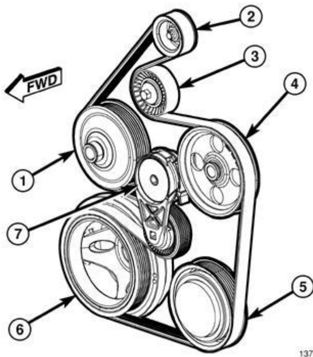
Fig. 5: Accessory Drive Belt Routing, Tensioner & Pulleys
