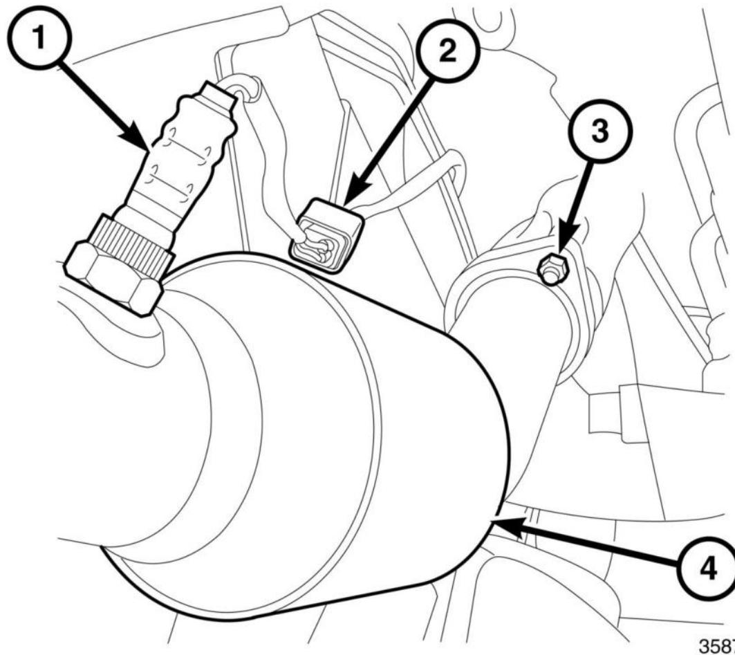
Fig. 300: Oxygen Sensor, Oxygen Sensor Connector, Ball Flange Nut & LH Catalytic Converter Courtesy of CHRYSLER GROUP, LLC
