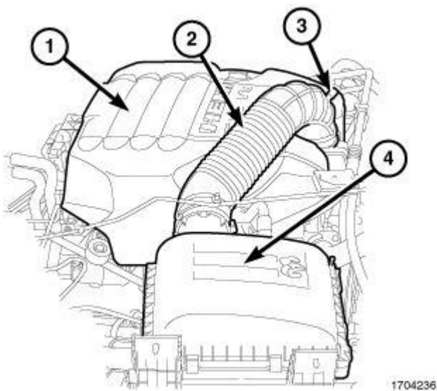
Fig. 297: Engine Cover, Clean Air Hose, Intake Air Temperature (IAT) Sensor Electrical Connector & Air Cleaner Housing
