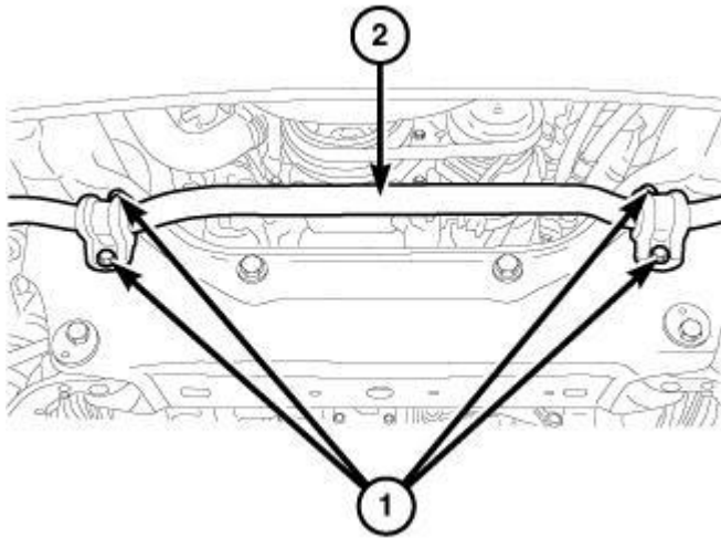
Fig. 264: Stabilizer Bar & Bolts Courtesy of CHRYSLER GROUP, LLC
