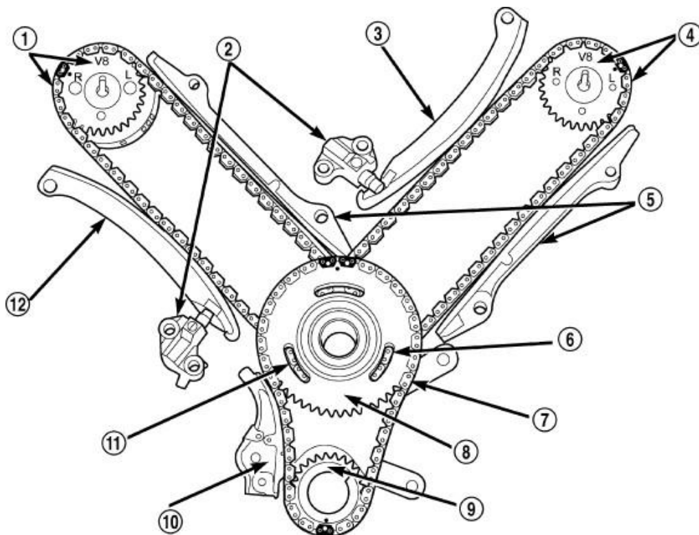
Fig. 199: Timing Drive System
