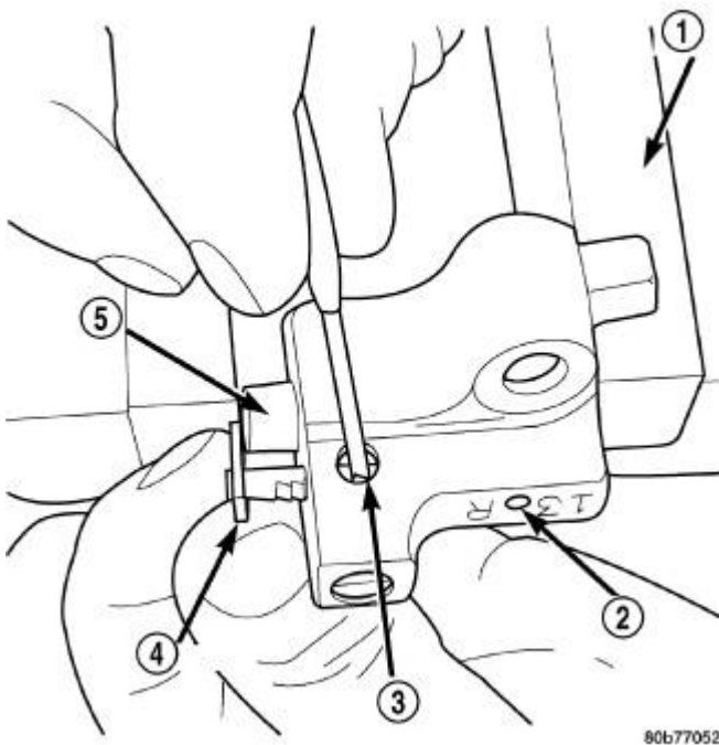
Fig. 210: Resetting Secondary Chain Tensioners Courtesy of CHRYSLER GROUP, LLC
