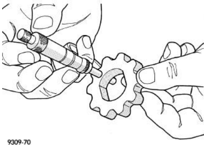
Fig. 173: Measuring Inner Rotor Thickness Courtesy of CHRYSLER GROUP, LLC
