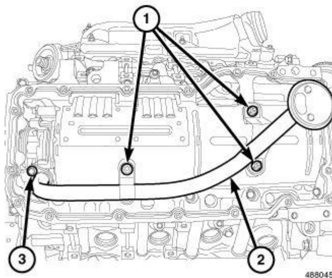
Fig. 178: Identifying Oil Pickup Tube Courtesy of CHRYSLER GROUP, LLC
