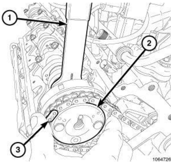
Fig. 67: Installing Camshaft Holder Onto Camshaft Courtesy of CHRYSLER GROUP, LLC
