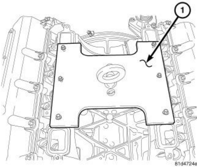
Fig. 16: Engine Lift Bracket 10101 Courtesy of CHRYSLER GROUP, LLC
