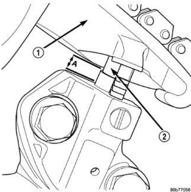
Fig. 189: Measuring Secondary Timing Chains For Wear Courtesy of CHRYSLER GROUP, LLC
