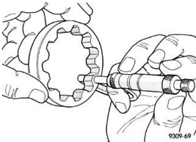
Fig. 172: Measuring Outer Rotor Thickness Courtesy of CHRYSLER GROUP, LLC
