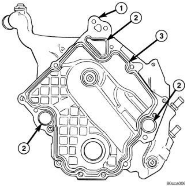
Fig. 218: Timing Chain Cover, Water Passage O-Ring & Engine RTV Sealer Courtesy of CHRYSLER GROUP, LLC
