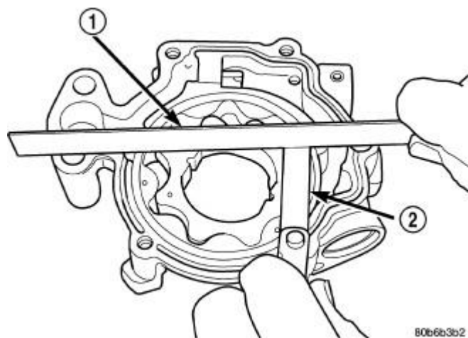
Fig. 176: Measuring Clearance Over Rotors Courtesy of CHRYSLER GROUP, LLC
