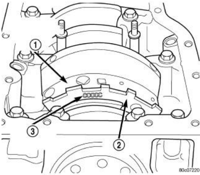
Fig. 121: Main Bearing Markings on Target Wheel Courtesy of CHRYSLER GROUP, LLC
