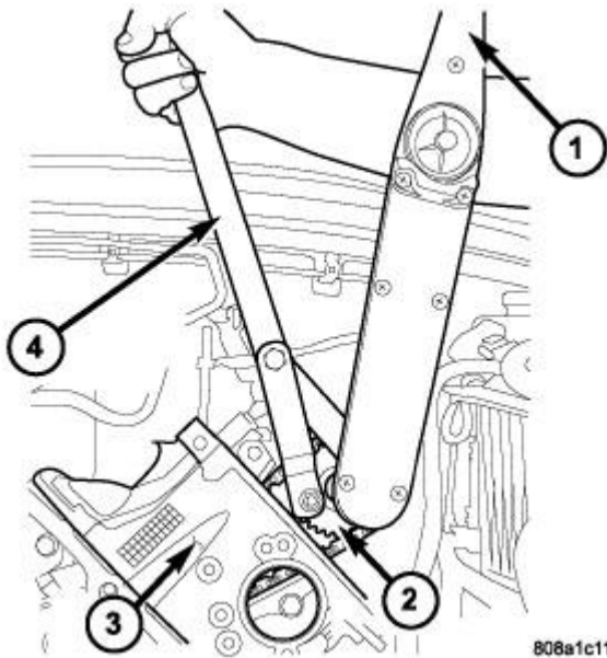
Fig. 71: Tightening Left Side Camshaft Sprocket Bolt Courtesy of CHRYSLER GROUP, LLC
