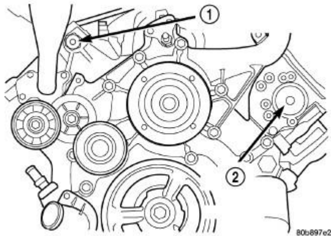
Fig. 43: Cylinder Head Access Plugs Courtesy of CHRYSLER GROUP, LLC
