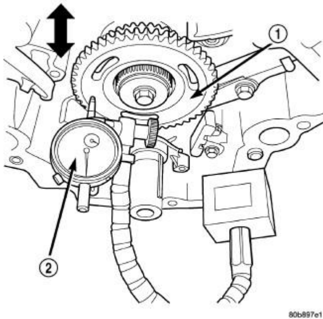
Fig. 215: Measuring Idler Gear End Play Courtesy of CHRYSLER GROUP, LLC
