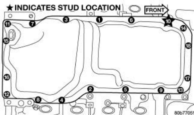
Fig. 133: Oil Pan Removal/Tightening Sequence Courtesy of CHRYSLER GROUP, LLC
