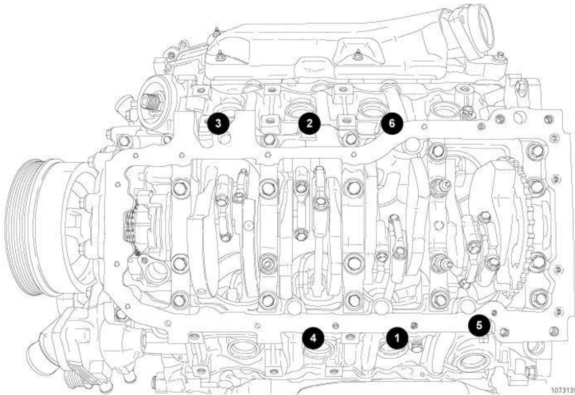
Fig. 132: Tightening Bedplate Bolts (4 Of 4) Courtesy of CHRYSLER GROUP, LLC
