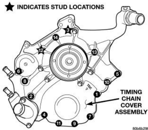
Fig. 204: Identifying Removal & Installation Sequence Of Timing Cover Bolts Courtesy of CHRYSLER GROUP, LLC
