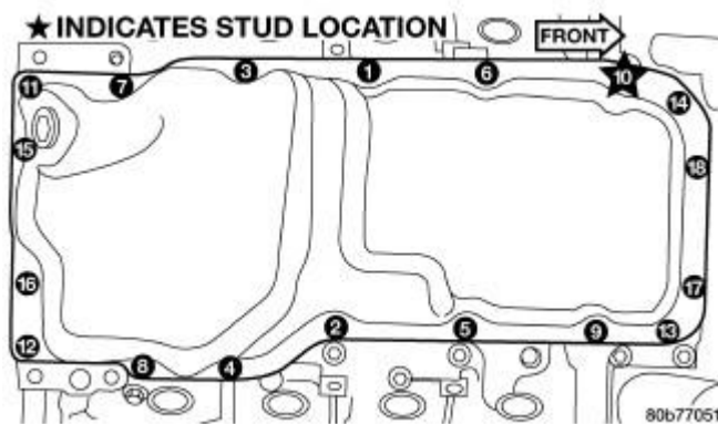
Fig. 169: Oil Pan Bolt Removal/Tightening Sequence Courtesy of CHRYSLER GROUP, LLC
