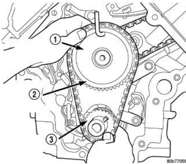
Fig. 212: Installing Idler Gear, Primary and Secondary Timing Chains Courtesy of CHRYSLER GROUP, LLC
