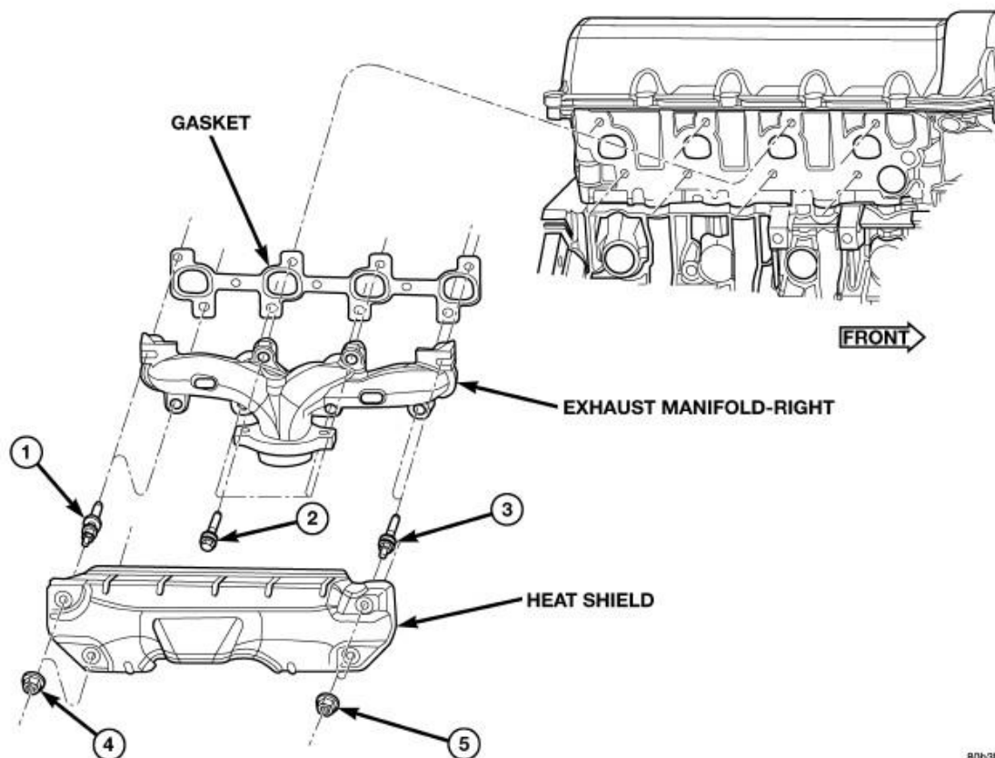
Fig. 183: Exhaust Manifold-Right Courtesy of CHRYSLER GROUP, LLC
