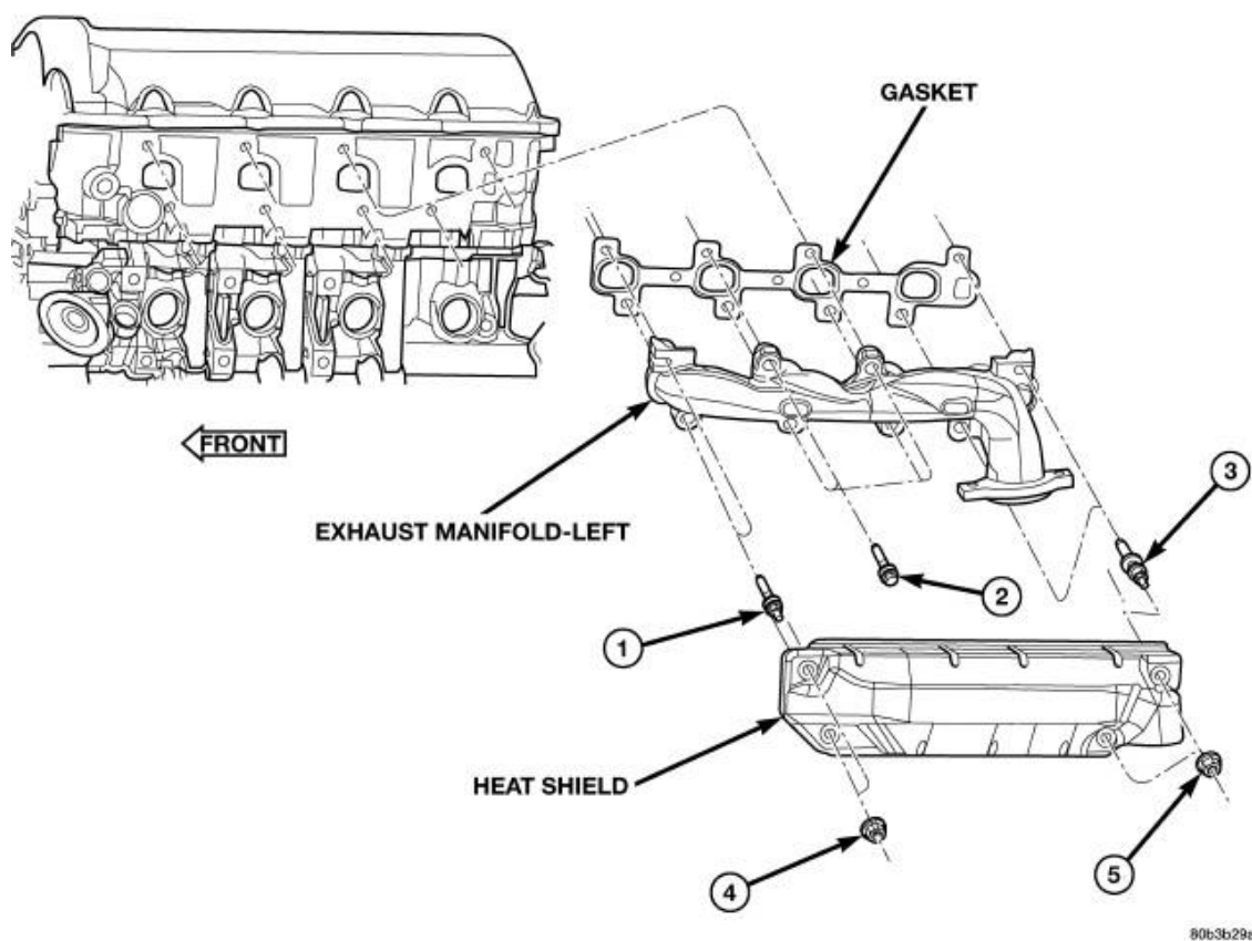
Fig. 184: Exhaust Manifold-Left
