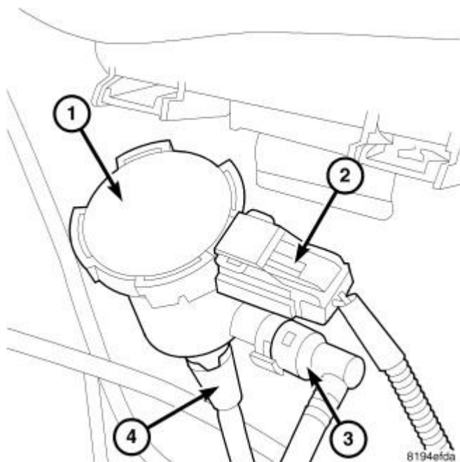
Fig. 98: Locating EVAP Canister Purge Solenoid
