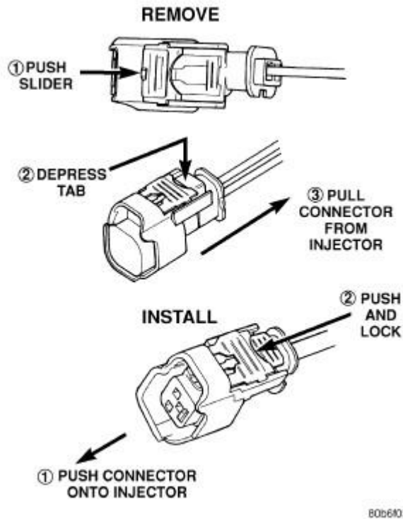
Fig. 99: Removing/Installing Injector Connector Courtesy of CHRYSLER GROUP, LLC
