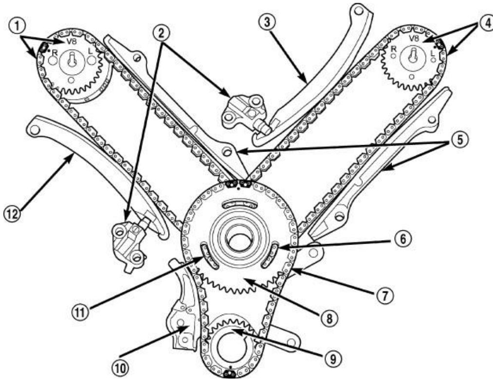
Fig. 188: Timing Drive System
