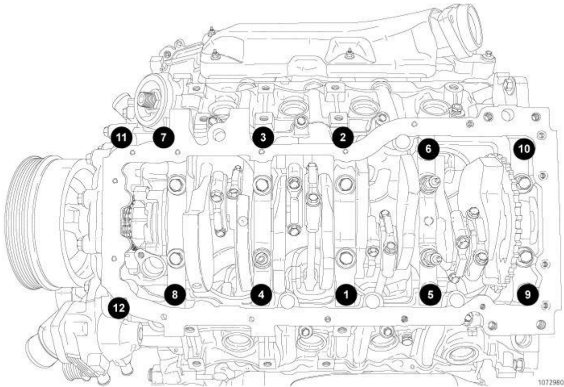
Fig. 130: Tightening Bedplate Bolts (2 Of 4) Courtesy of CHRYSLER GROUP, LLC
