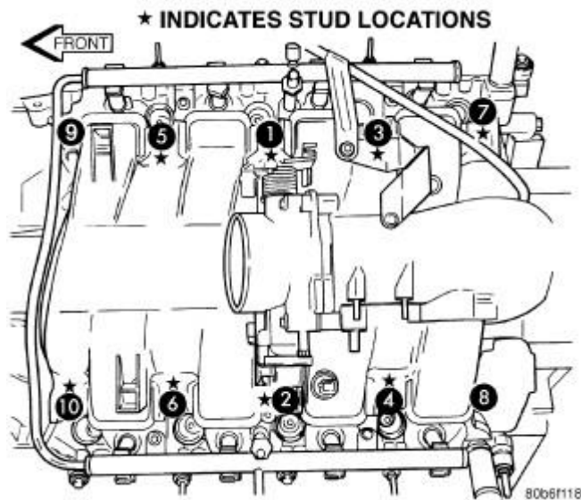
Fig. 60: Identifying Removal & Installation Sequence Of Intake Manifold Retaining Fasteners Courtesy of CHRYSLER GROUP, LLC
