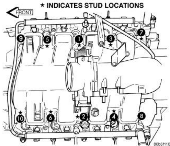
Fig. 31: Identifying Removal & Installation Sequence Of Intake Manifold Retaining Fasteners Courtesy of CHRYSLER GROUP, LLC
