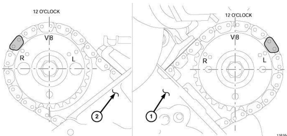
Fig. 201: Camshaft Sprocket V8 Marks Courtesy of CHRYSLER GROUP, LLC
