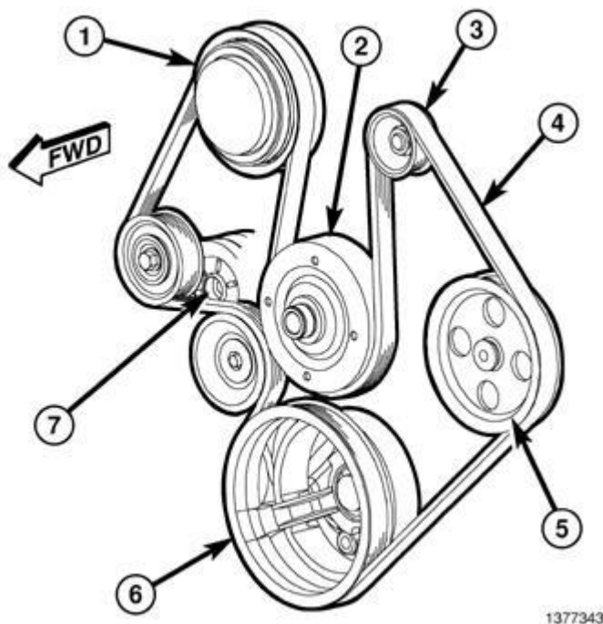
Fig. 90: Belt Routing (3.7L/4.7L Engine) Courtesy of CHRYSLER GROUP, LLC
