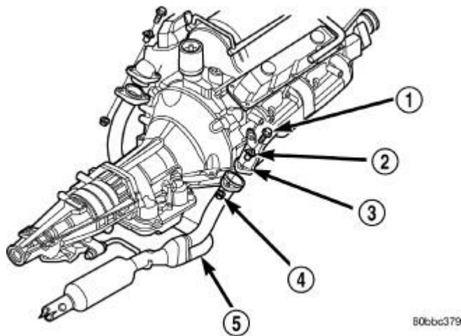
Fig. 24: Exhaust Pipe To Manifold Connection - Typical Courtesy of CHRYSLER GROUP, LLC
