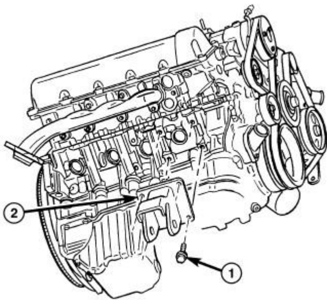
Fig. 161: Engine Mount Support Bracket Courtesy of CHRYSLER GROUP, LLC
