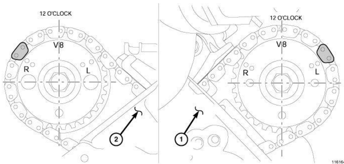
Fig. 49: Camshaft Sprocket V8 Marks Courtesy of CHRYSLER GROUP, LLC
