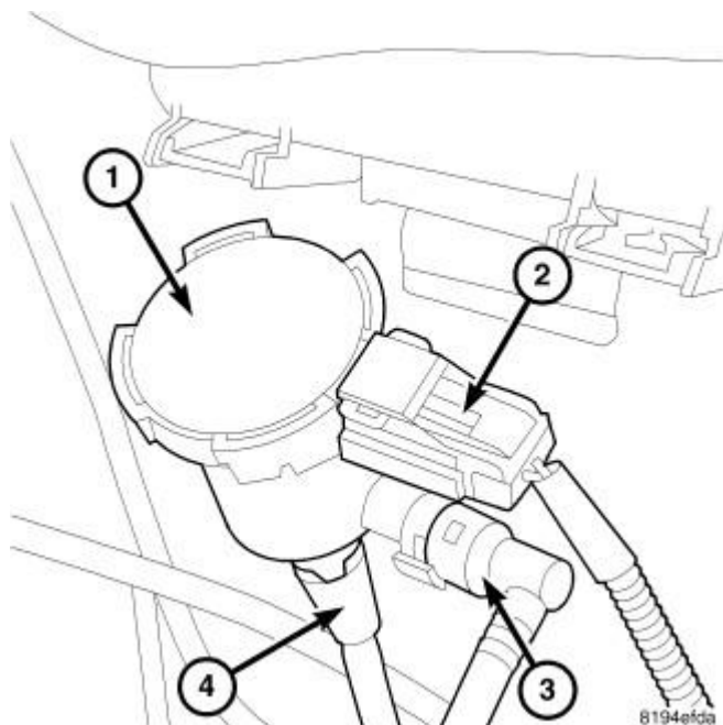
Fig. 93: Locating EVAP Canister Purge Solenoid Courtesy of CHRYSLER GROUP, LLC
