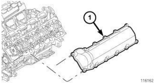
Fig. 95: Cylinder Head Cover - Left Courtesy of CHRYSLER GROUP, LLC
