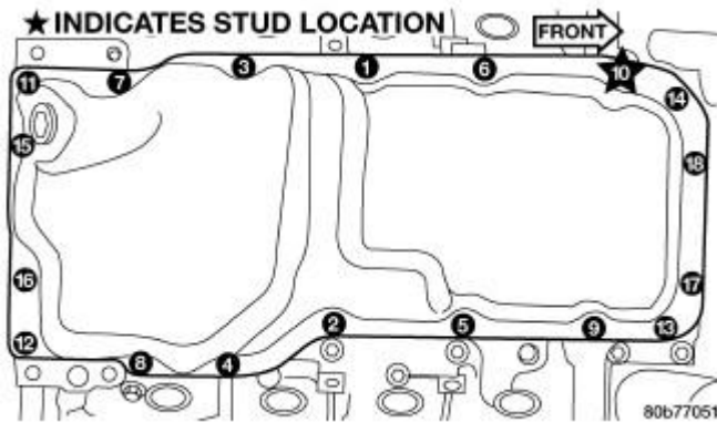
Fig. 170: Oil Pan Bolt Removal/Tightening Sequence
