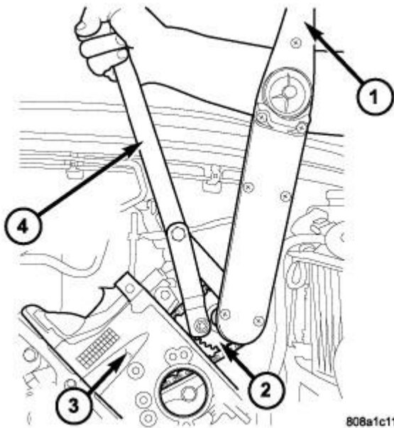
Fig. 86: Tightening Left Side Camshaft Sprocket Bolt Courtesy of CHRYSLER GROUP, LLC
