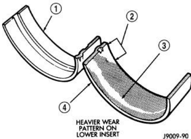
Fig. 122: Main Bearing Wear Patterns Courtesy of CHRYSLER GROUP, LLC
