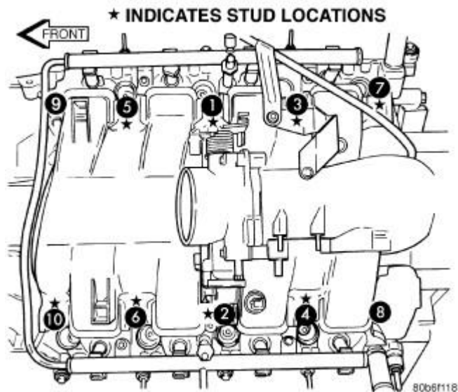
Fig. 186: Identifying Removal & Installation Sequence Of Intake Manifold Retaining Fasteners Courtesy of CHRYSLER GROUP, LLC
