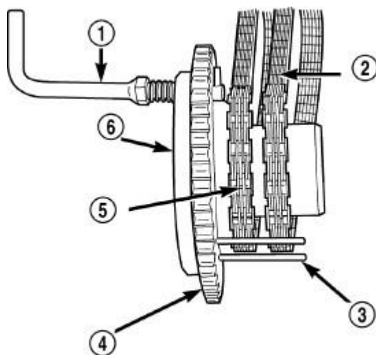
Fig. 58: Secondary Camshaft Chain Holder 8429 Courtesy of CHRYSLER GROUP, LLC
