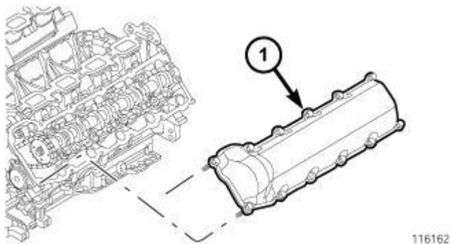
Fig. 199: Cylinder Head Cover - Left Courtesy of CHRYSLER GROUP, LLC
