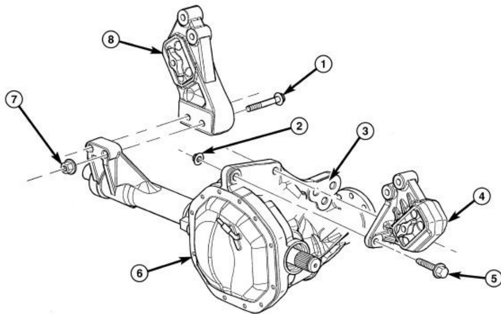
Fig. 160: Engine Insulator Mounts - 4X4 Courtesy of CHRYSLER GROUP, LLC
