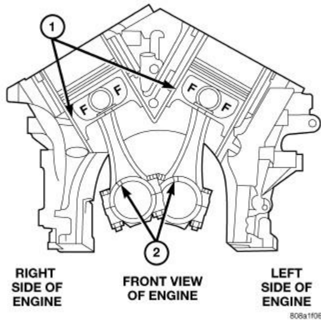
Fig. 152: Identifying Proper Connecting Rod Installation Courtesy of CHRYSLER GROUP, LLC
