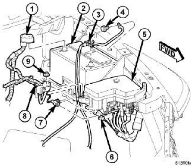
Fig. 198: Removing/Installing Battery Cables Courtesy of CHRYSLER GROUP, LLC
