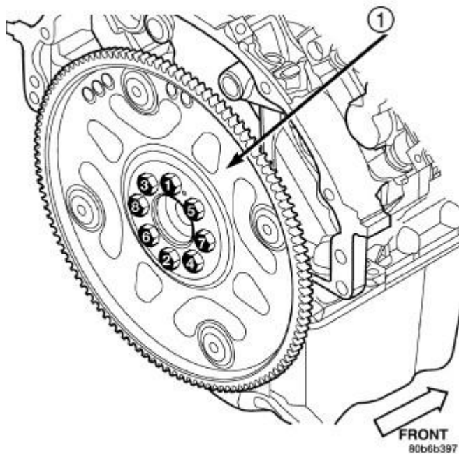
Fig. 141: Flexplate Removal/Tightening Sequence Courtesy of CHRYSLER GROUP, LLC
