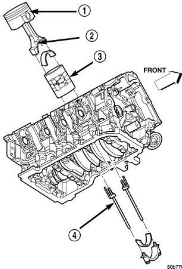
Fig. 117: Identifying Piston Ring Compressor And Guide Pins Special Tool 8507 Courtesy of CHRYSLER GROUP, LLC
