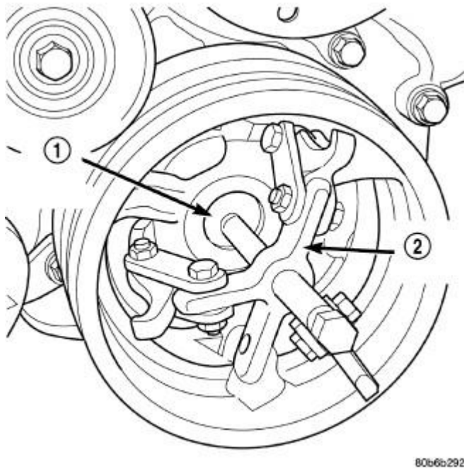
Fig. 203: Removing Crankshaft Damper Courtesy of CHRYSLER GROUP, LLC
