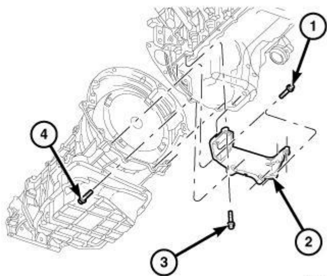
Fig. 7: Structural Cover Torque Sequence Courtesy of CHRYSLER GROUP, LLC
