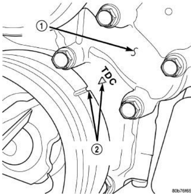
Fig. 40: Engine Top Dead Center (TDC) Indicator Mark Courtesy of CHRYSLER GROUP, LLC
