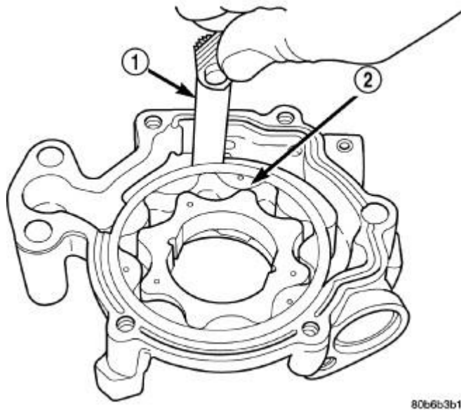
Fig. 174: Measuring Outer Rotor Clearance Courtesy of CHRYSLER GROUP, LLC
