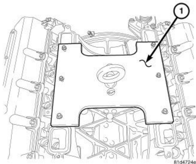
Fig. 13: Engine Lift Bracket 10101 Courtesy of CHRYSLER GROUP, LLC
