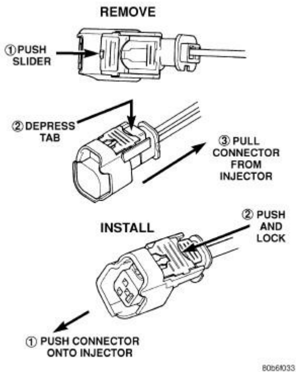
Fig. 94: Removing/Installing Injector Connector Courtesy of CHRYSLER GROUP, LLC
