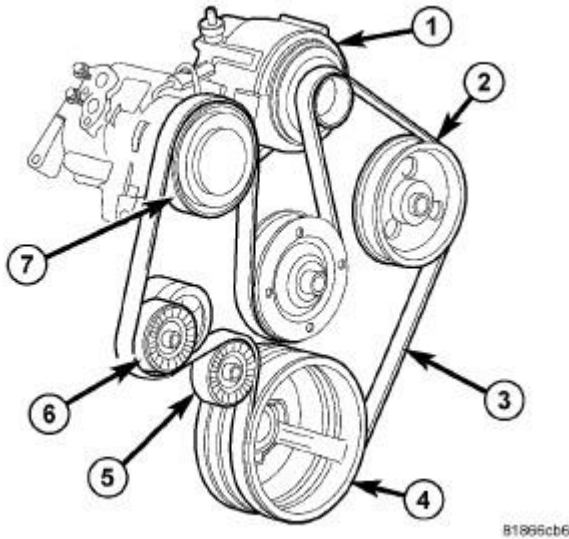
Fig. 135: Accessory Drive Belt Routing 3.7L/4.7L Courtesy of CHRYSLER GROUP, LLC
