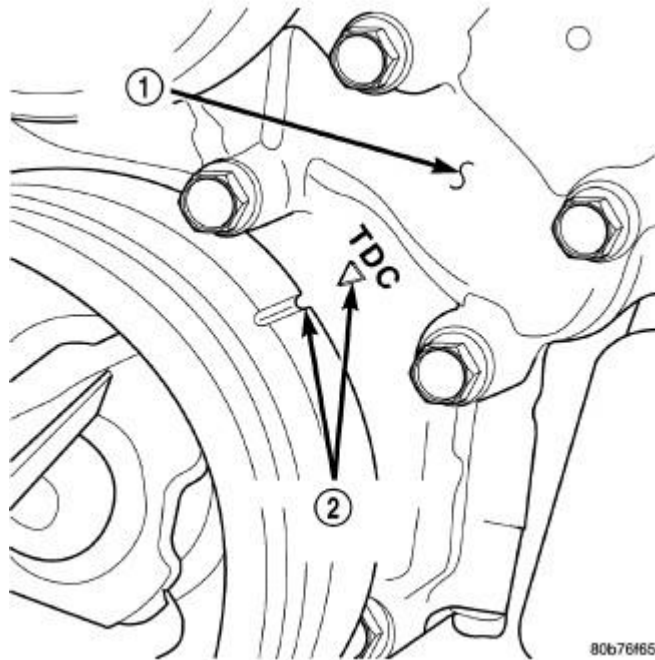
Fig. 33: Engine Top Dead Center (TDC) Indicator Mark Courtesy of CHRYSLER GROUP, LLC
