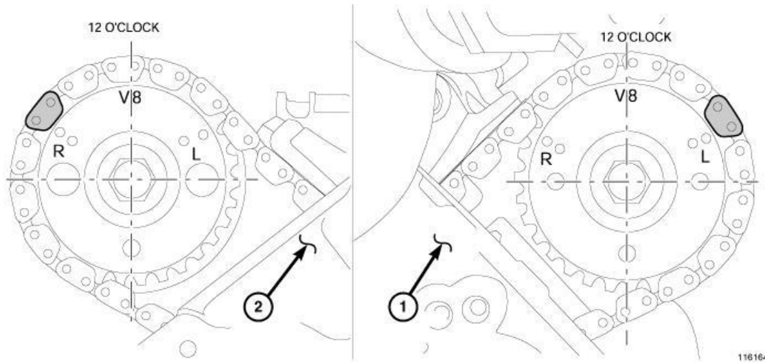
Fig. 191: Camshaft Sprocket V8 Marks Courtesy of CHRYSLER GROUP, LLC
