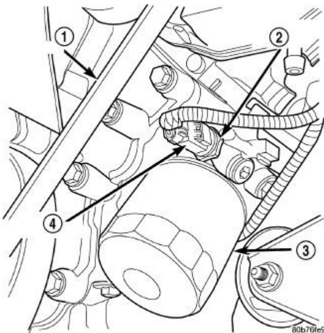
Fig. 180: Identifying Engine Oil Pressure Sensor Courtesy of CHRYSLER GROUP, LLC
