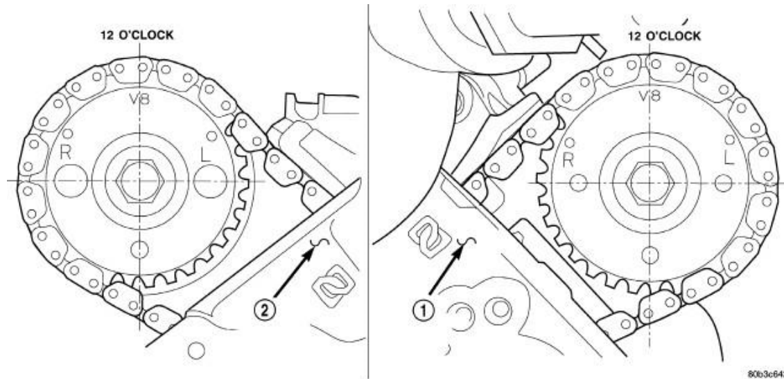
Fig. 36: Camshaft Sprocket V8 Marks Courtesy of CHRYSLER GROUP, LLC
