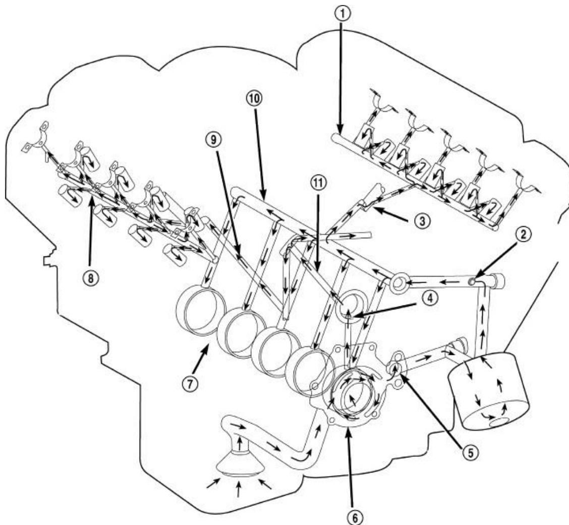
Fig. 164: Engine Oil Lubrication System Courtesy of CHRYSLER GROUP, LLC
