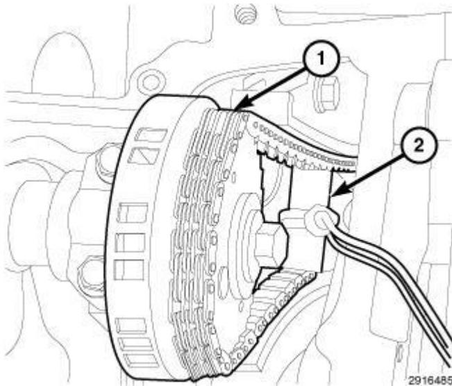
Fig. 63: Positioning Locking Wedge Between Timing Chain Courtesy of CHRYSLER GROUP, LLC
