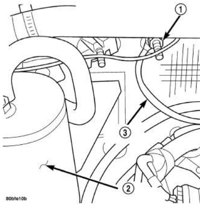
Fig. 17: Body Ground Strap-Right Side Removal / Installation
