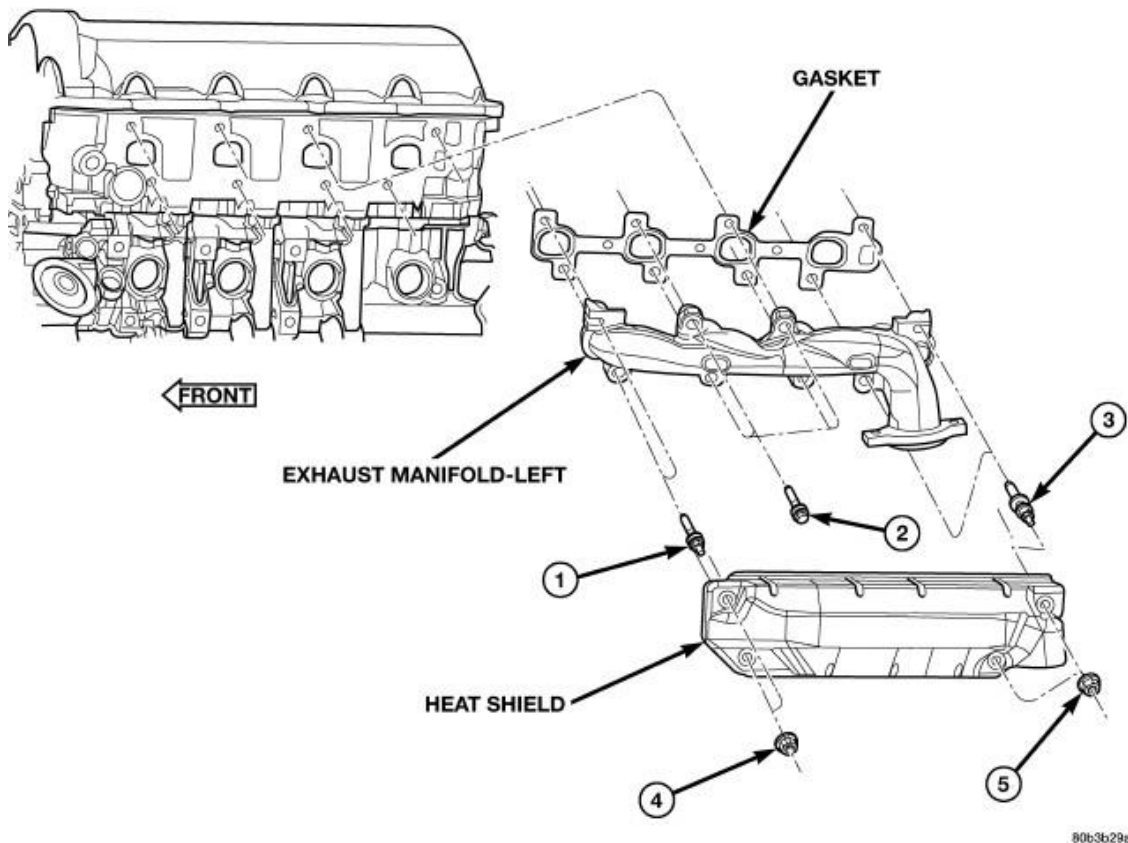
Fig. 182: Exhaust Manifold-Left Courtesy of CHRYSLER GROUP, LLC
