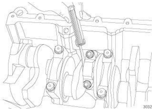
Fig. 120: Checking Connecting Rod Side Clearance - Typical Courtesy of CHRYSLER GROUP, LLC
