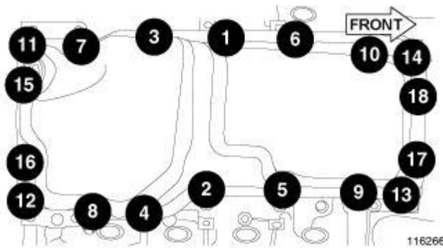
Fig. 125: Oil Pan Removal/Tightening Sequence Courtesy of CHRYSLER GROUP, LLC
