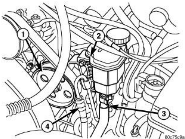
Fig. 101: Power Steering Pump Courtesy of CHRYSLER GROUP, LLC
