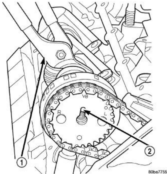
Fig. 208: Holding Right Camshaft With Pliers Courtesy of CHRYSLER GROUP, LLC
