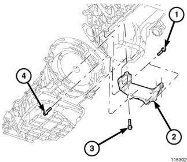
Fig. 123: Structural Cover Torque Sequence
