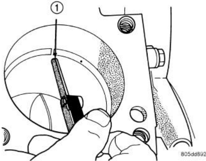
Fig. 143: Ring End Gap Measurement - Typical Courtesy of CHRYSLER GROUP, LLC
