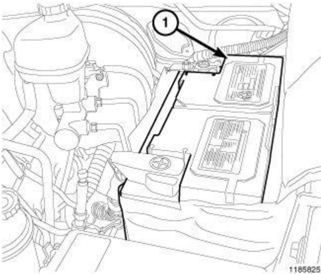
Fig. 134: Battery
