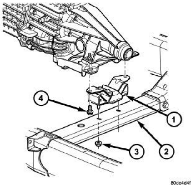
Fig. 159: Transmission Mount, Crossmember & Fasteners Courtesy of CHRYSLER GROUP, LLC
