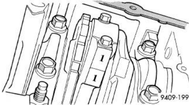
Fig. 150: Identifying Mark On Connecting Rod And Bearing Cap Courtesy of CHRYSLER GROUP, LLC
