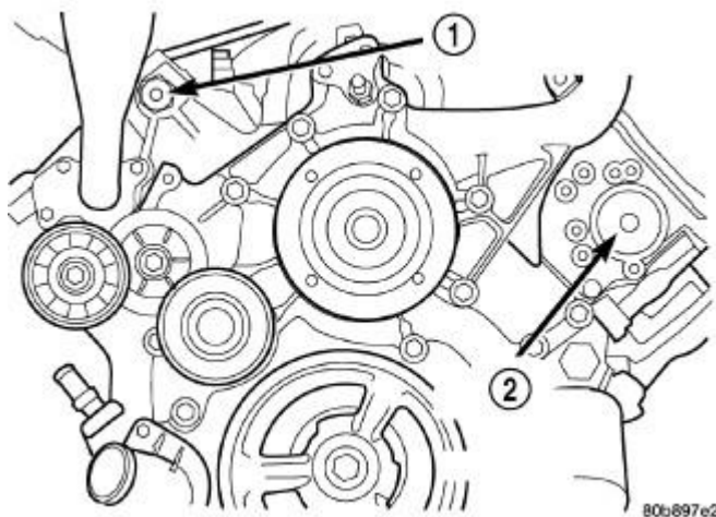
Fig. 57: Cylinder Head Access Plugs Courtesy of CHRYSLER GROUP, LLC
