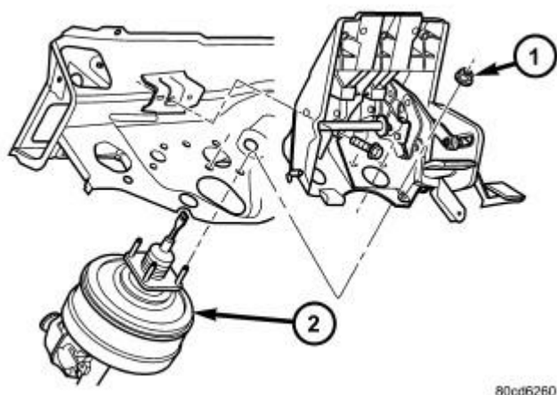
Fig. 89: Power Brake Booster & Mounting Nut Courtesy of CHRYSLER GROUP, LLC
