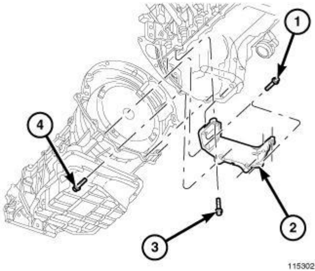
Fig. 124: Structural Cover Torque Sequence Courtesy of CHRYSLER GROUP, LLC
