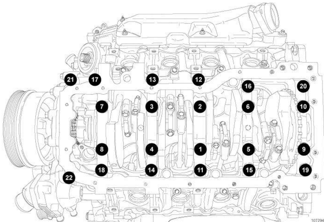
Fig. 129: Tightening Bedplate Bolts (1 Of 4)
