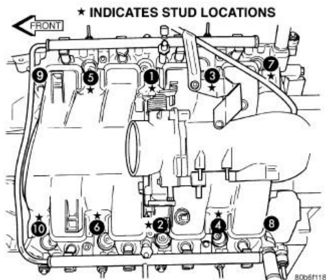
Fig. 187: Identifying Removal & Installation Sequence Of Intake Manifold Retaining Fasteners Courtesy of CHRYSLER GROUP, LLC
