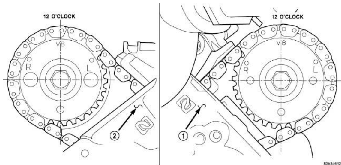
Fig. 34: Camshaft Sprocket V8 Marks Courtesy of CHRYSLER GROUP, LLC
