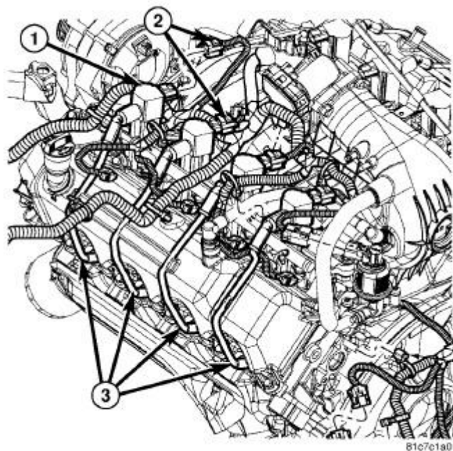
Fig. 92: Ignition Coils & Spark Plug Wires
