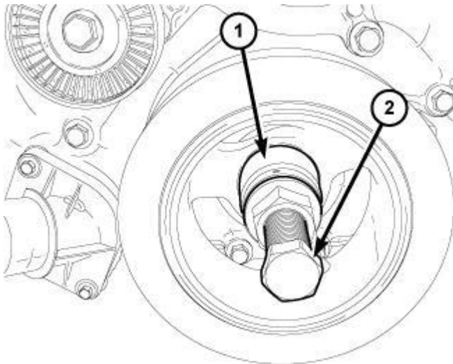
Fig. 139: Pressing Damper Onto Crankshaft Courtesy of CHRYSLER GROUP, LLC
