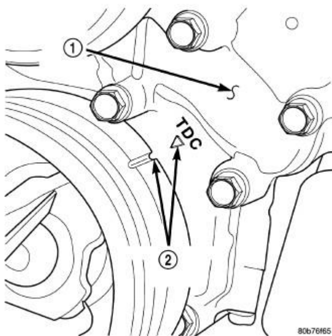
Fig. 200: Engine Top Dead Center (TDC) Indicator Mark Courtesy of CHRYSLER GROUP, LLC
