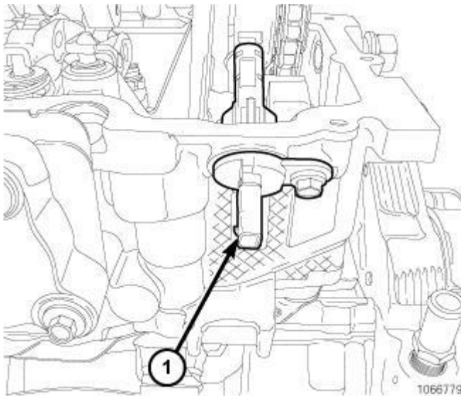
Fig. 65: Identifying Camshaft Position Sensor Courtesy of CHRYSLER GROUP, LLC
