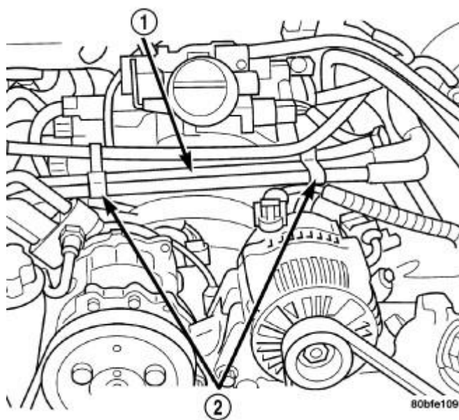
Fig. 12: Installing Heater Hoses And Tubes Courtesy of CHRYSLER GROUP, LLC
