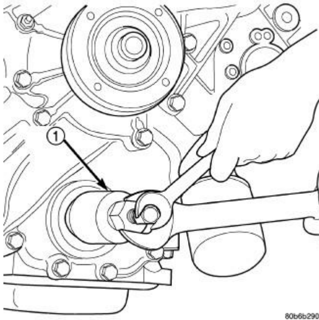
Fig. 154: Crankshaft Front Seal Removal Courtesy of CHRYSLER GROUP, LLC
