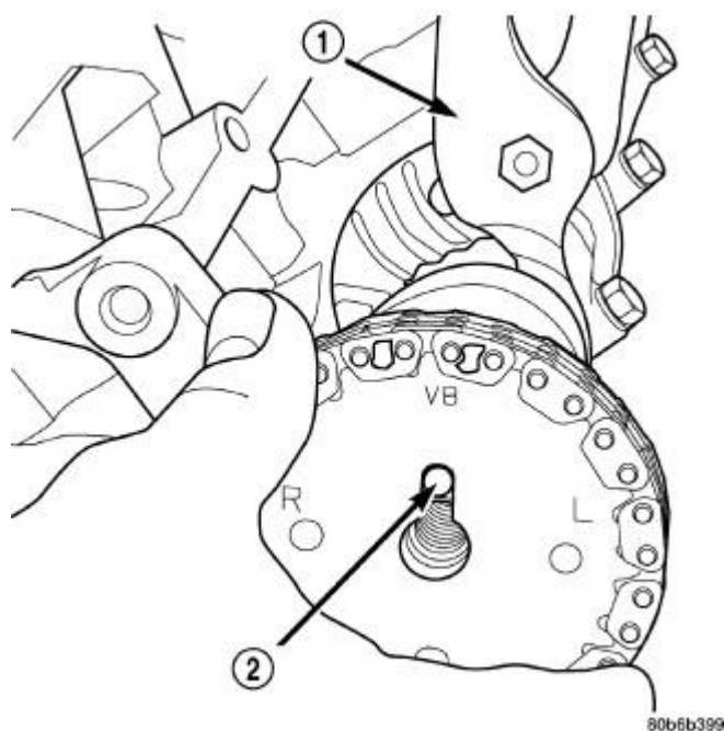
Fig. 193: Camshaft Sprocket Installation Courtesy of CHRYSLER GROUP, LLC
