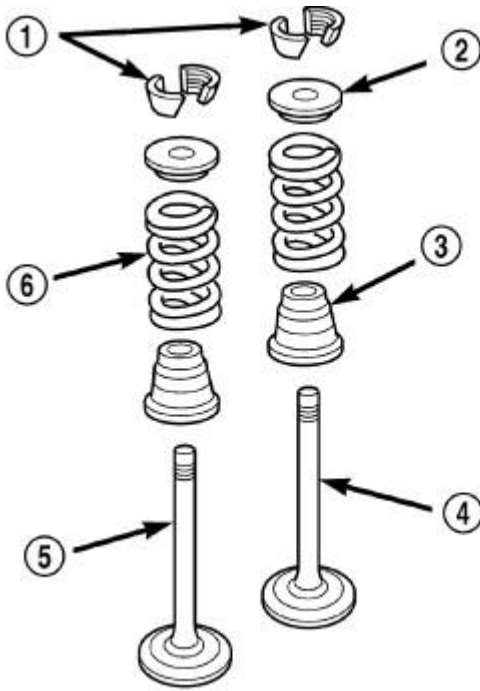
Fig. 110: Valve Assembly Configuration Courtesy of CHRYSLER GROUP, LLC
