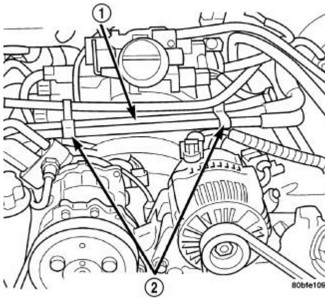
Fig. 185: Installing Heater Hoses And Tubes Courtesy of CHRYSLER GROUP, LLC
