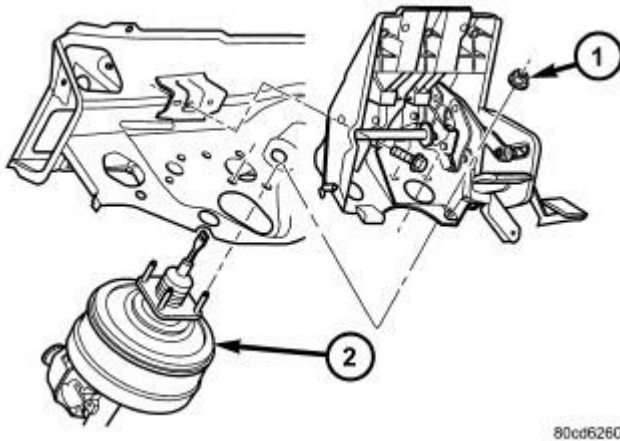
Fig. 103: Power Brake Booster & Mounting Nut Courtesy of CHRYSLER GROUP, LLC
