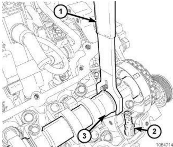
Fig. 66: Removing/Installing Cam Sensor And Camshaft Sprocket Bolt Using Spanner Wrench Courtesy of CHRYSLER GROUP, LLC
