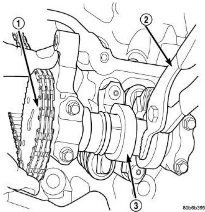
Fig. 207: Holding Camshaft With Adjustable Pliers Courtesy of CHRYSLER GROUP, LLC
