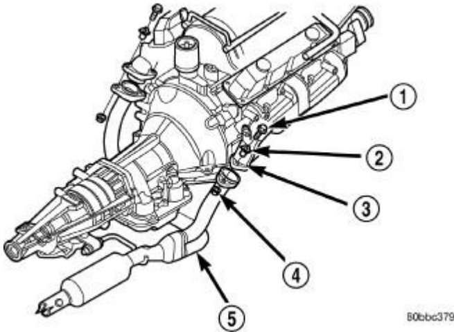
Fig. 5: Exhaust Pipe To Manifold Connection - Typical Courtesy of CHRYSLER GROUP, LLC
