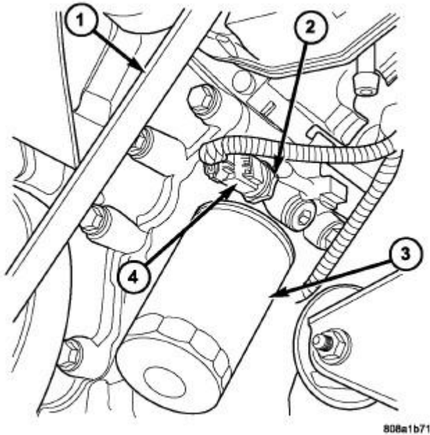
Fig. 165: Belt, Oil Pressure Sensor, Oil Filter & Connector Courtesy of CHRYSLER GROUP, LLC
