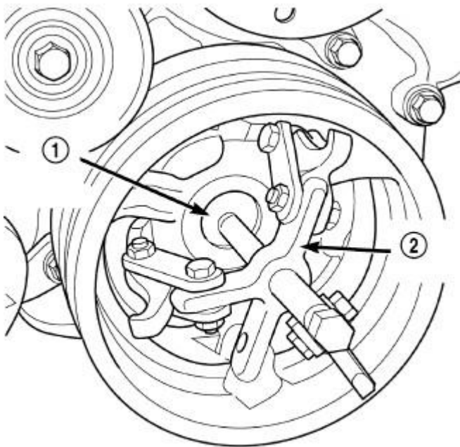
Fig. 153: Removing Crankshaft Damper Courtesy of CHRYSLER GROUP, LLC
