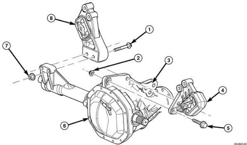
Fig. 163: Engine Insulator Mounts - 4X4 Courtesy of CHRYSLER GROUP, LLC
