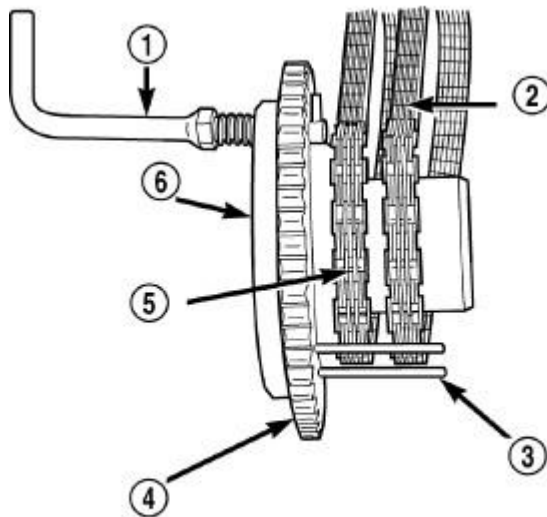
Fig. 211: Installing Secondary Timing Chains on Idler Sprocket Courtesy of CHRYSLER GROUP, LLC
