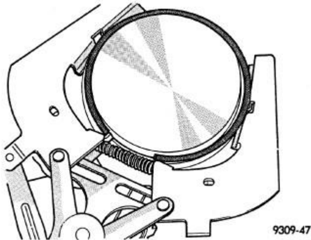
Fig. 146: Removing/Installing Upper & Intermediate Rings Courtesy of CHRYSLER GROUP, LLC
