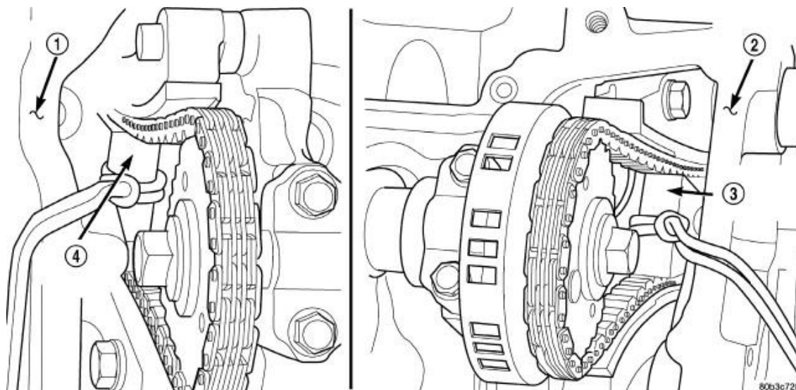
Fig. 196: Securing Timing Chain Tensioners Using Timing Chain Wedge
