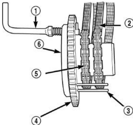
Fig. 51: Installing Secondary Timing Chains on Idler Sprocket Courtesy of CHRYSLER GROUP, LLC
