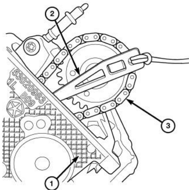
Fig. 161: Securing Timing Chain Tensioner Using Timing Chain Wedge Courtesy of CHRYSLER GROUP, LLC
