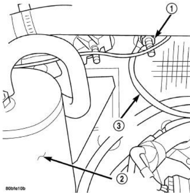
Fig. 10: Removal/Installation Body Ground Strap-Right Side
