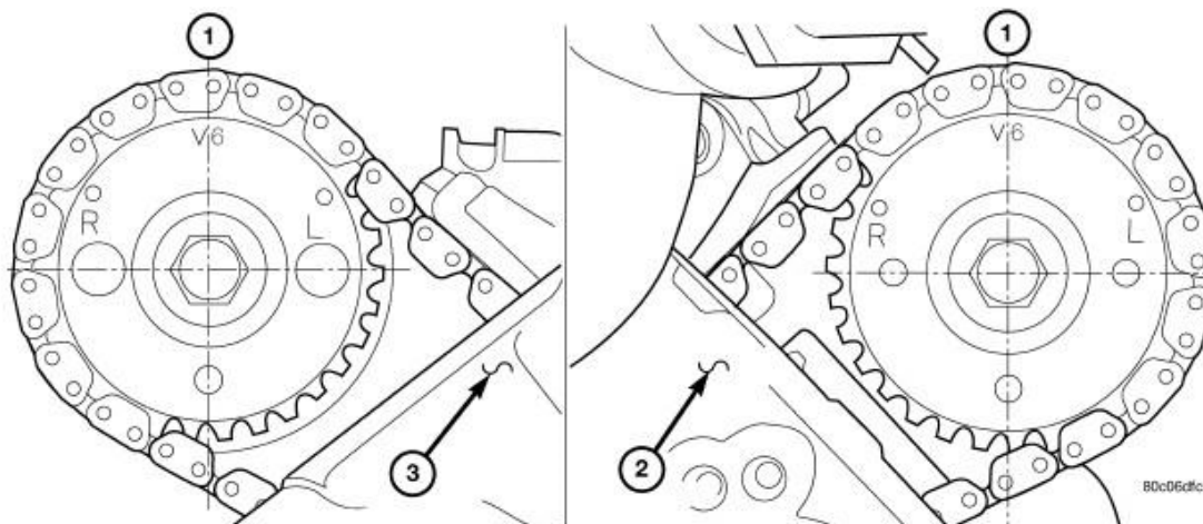
Fig. 61: Camshaft Sprocket V6 Timing Marks Courtesy of CHRYSLER GROUP, LLC
