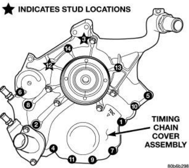
Fig. 179: Timing Chain Cover Assembly Removal/Tightening Sequence Courtesy of CHRYSLER GROUP, LLC
