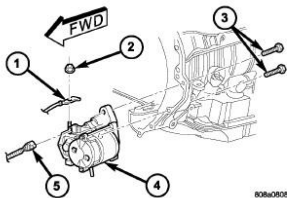
Fig. 9: Remove/Install Starter Motor Courtesy of CHRYSLER GROUP, LLC
