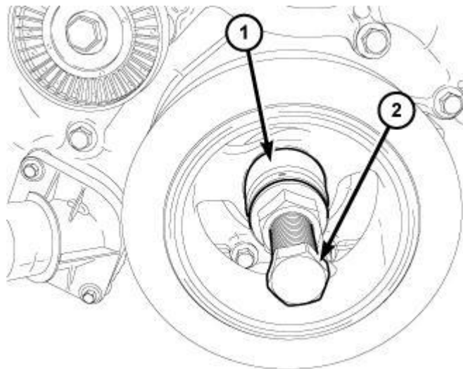
Fig. 88: Pressing Damper Onto Crankshaft Courtesy of CHRYSLER GROUP, LLC
