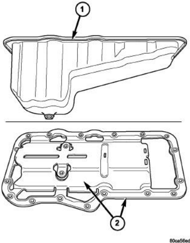
Fig. 128: Oil Pan & Gasket
