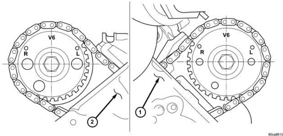
Fig. 163: Camshaft Sprocket V6 Timing Marks Courtesy of CHRYSLER GROUP, LLC
