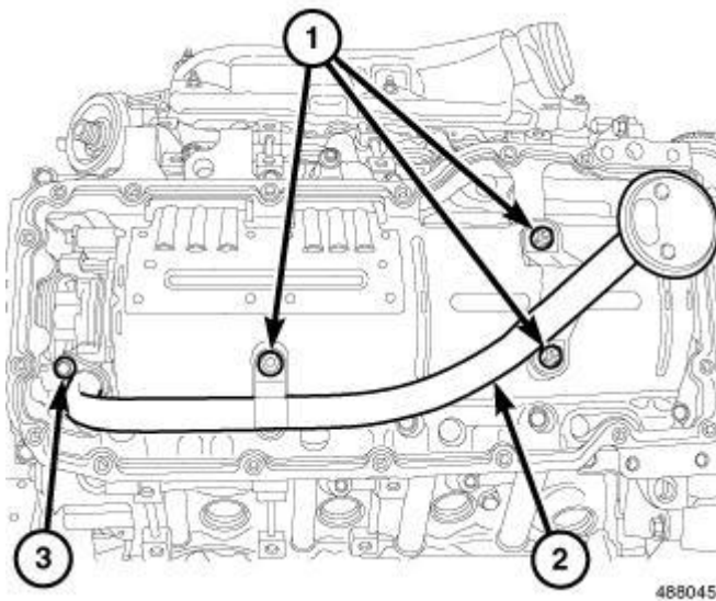
Fig. 138: Oil Pickup Tube & Fasteners Courtesy of CHRYSLER GROUP, LLC
