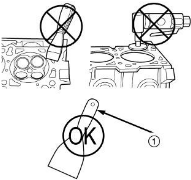
Fig. 55: Proper Tool Usage For Surface Preparation
