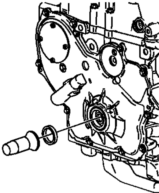
Fig. 60: Installing Crankshaft Front Oil Seal Courtesy of GENERAL MOTORS COMPANY
