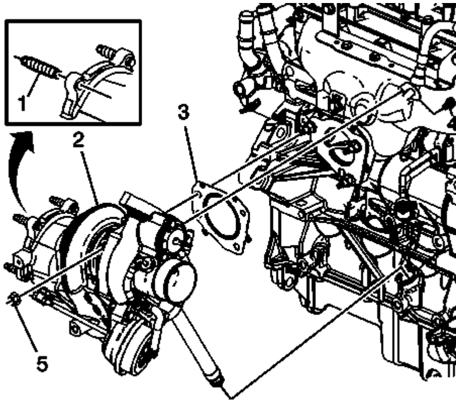
Fig. 31: Turbocharger Assembly
