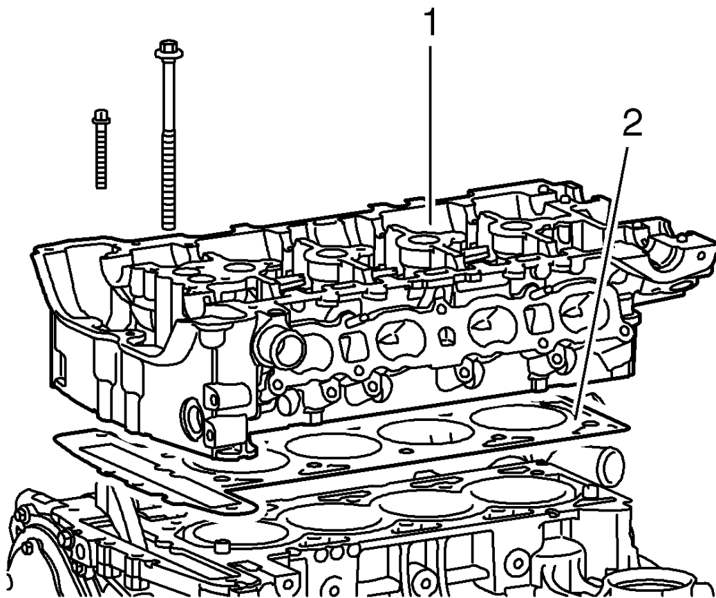
Fig. 149: Cylinder Head And Gasket
