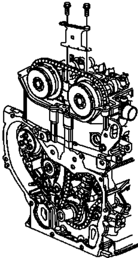
Fig. 66: View Of Upper Timing Chain Guide Bolts And Guide Courtesy of GENERAL MOTORS COMPANY
