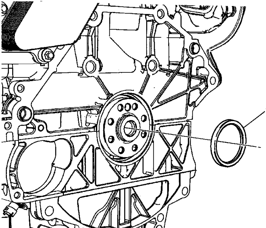
Fig. 156: Crankshaft Rear Oil Seal Courtesy of GENERAL MOTORS COMPANY
