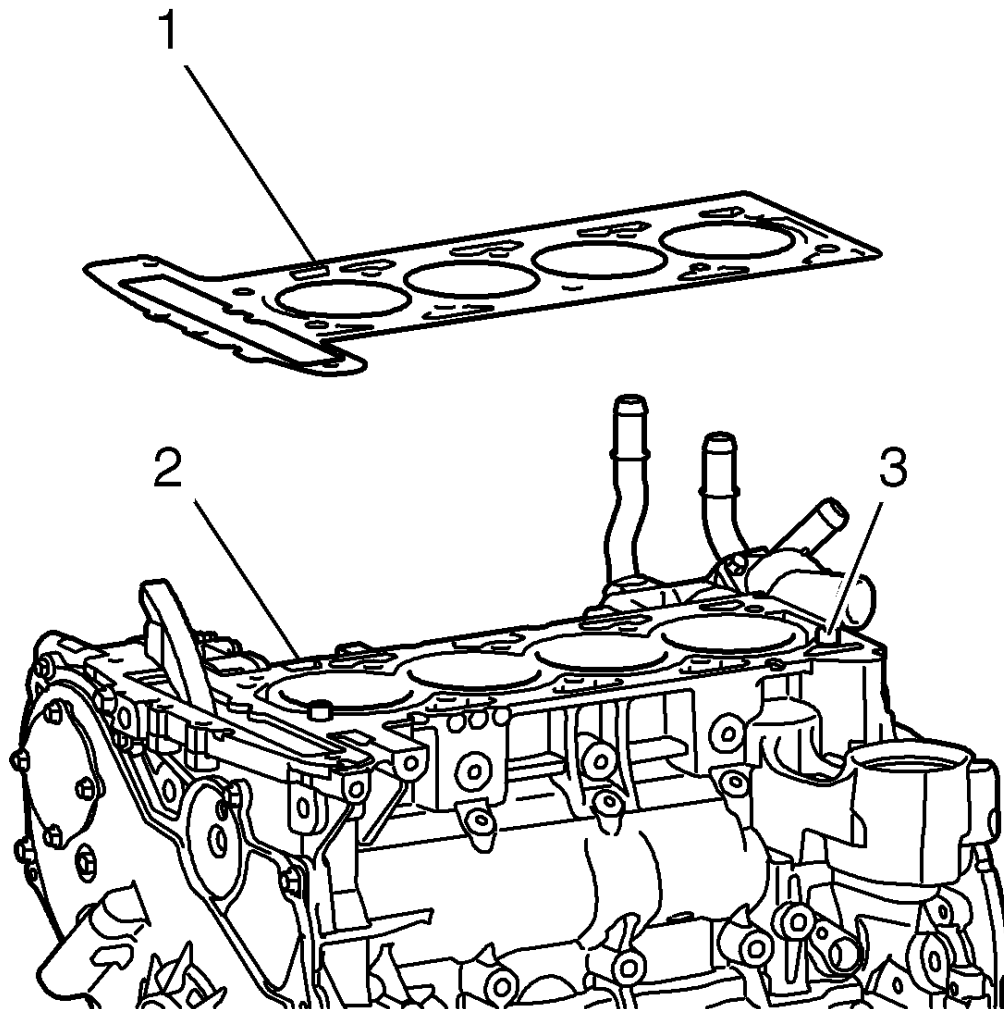
Fig. 150: Cylinder Head Gasket And Lock Pin Courtesy of GENERAL MOTORS COMPANY
