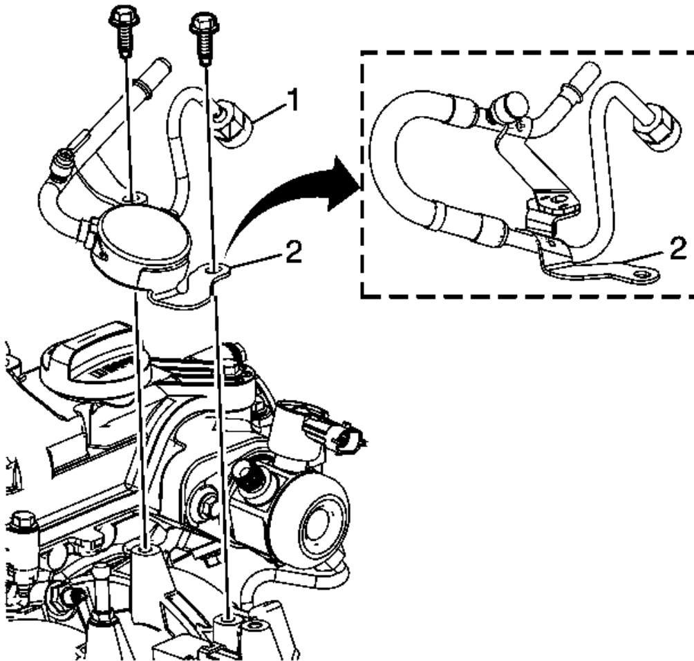
Fig. 45: Fuel Feed Line And Fuel Feed Line Tube Nut Courtesy of GENERAL MOTORS COMPANY
