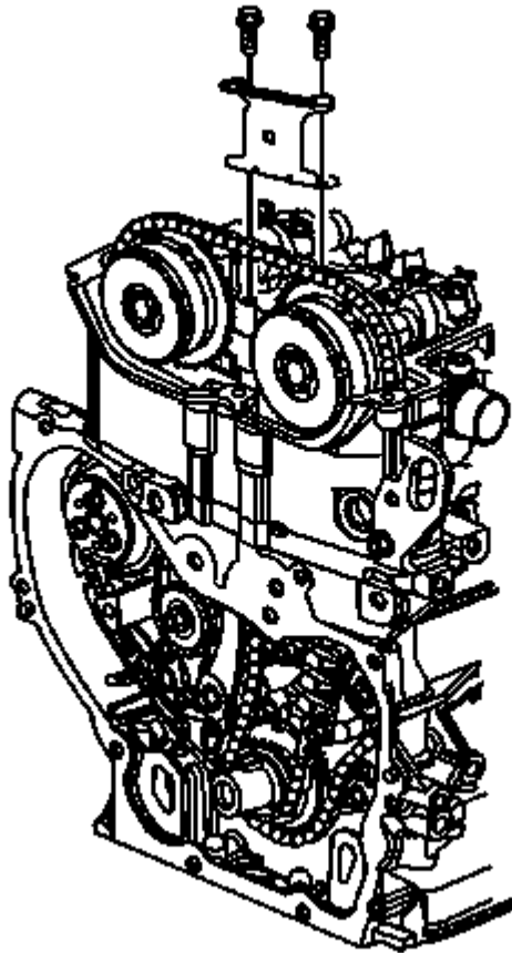
Fig. 128: View Of Upper Timing Chain Guide Bolts And Guide Courtesy of GENERAL MOTORS COMPANY
