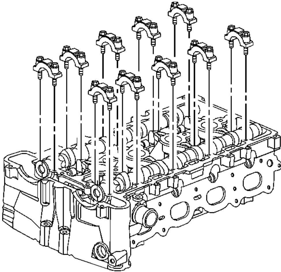
Fig. 111: Camshaft Bearing Caps
