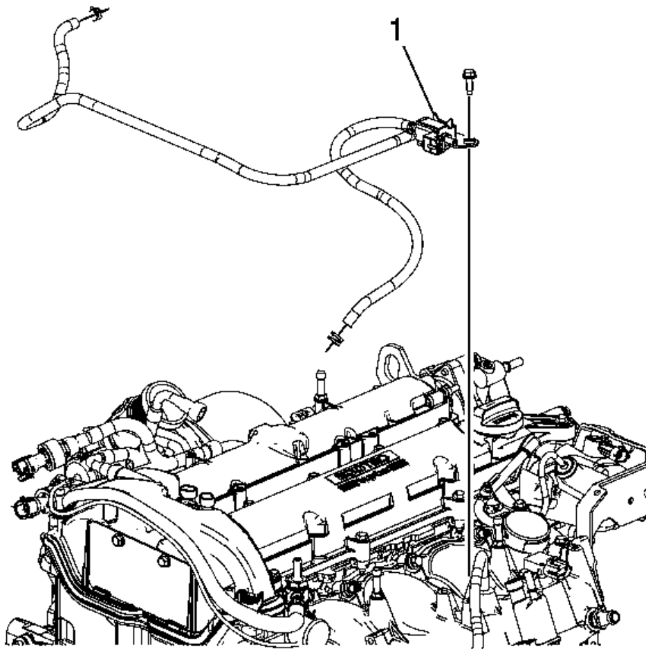
Fig. 53: Charger AIR Bypass Valve Solenoid Courtesy of GENERAL MOTORS COMPANY
