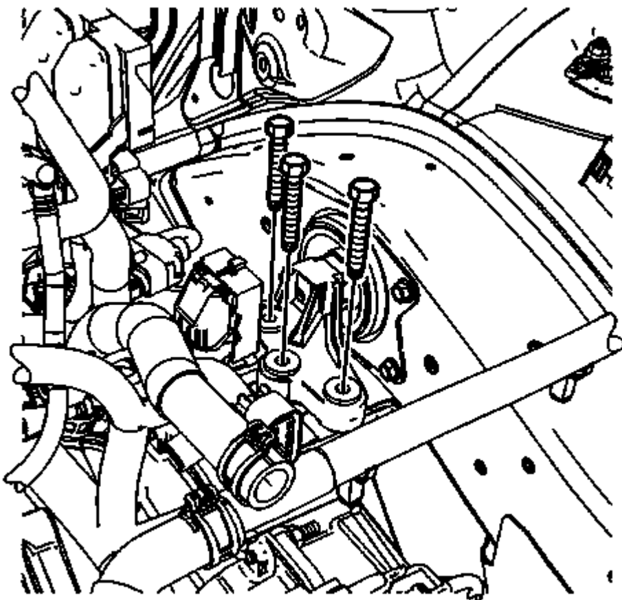
Fig. 170: Transaxle Mount To Transaxle Bolts Courtesy of GENERAL MOTORS COMPANY
