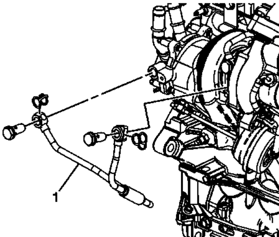
Fig. 28: Turbocharger Coolant Return Pipe Courtesy of GENERAL MOTORS COMPANY
