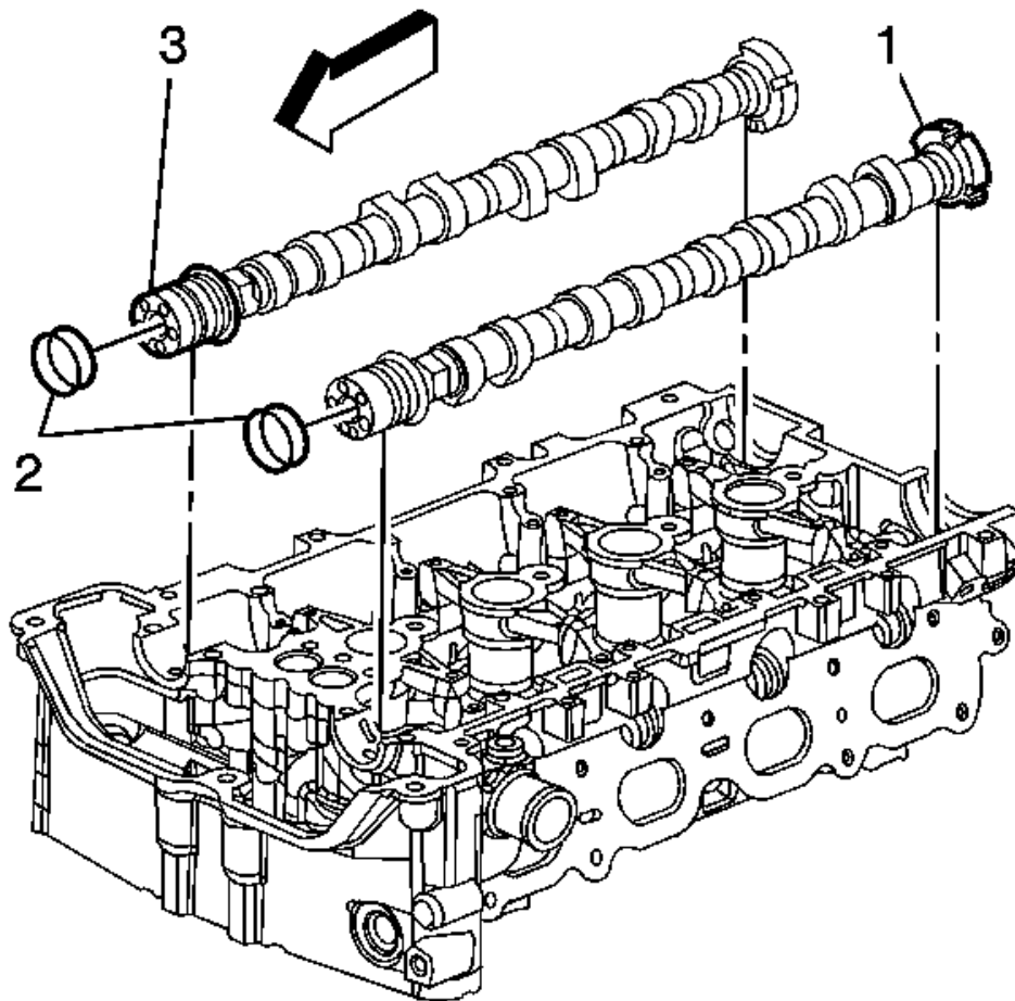
Fig. 112: Intake/Exhaust Camshaft Courtesy of GENERAL MOTORS COMPANY
