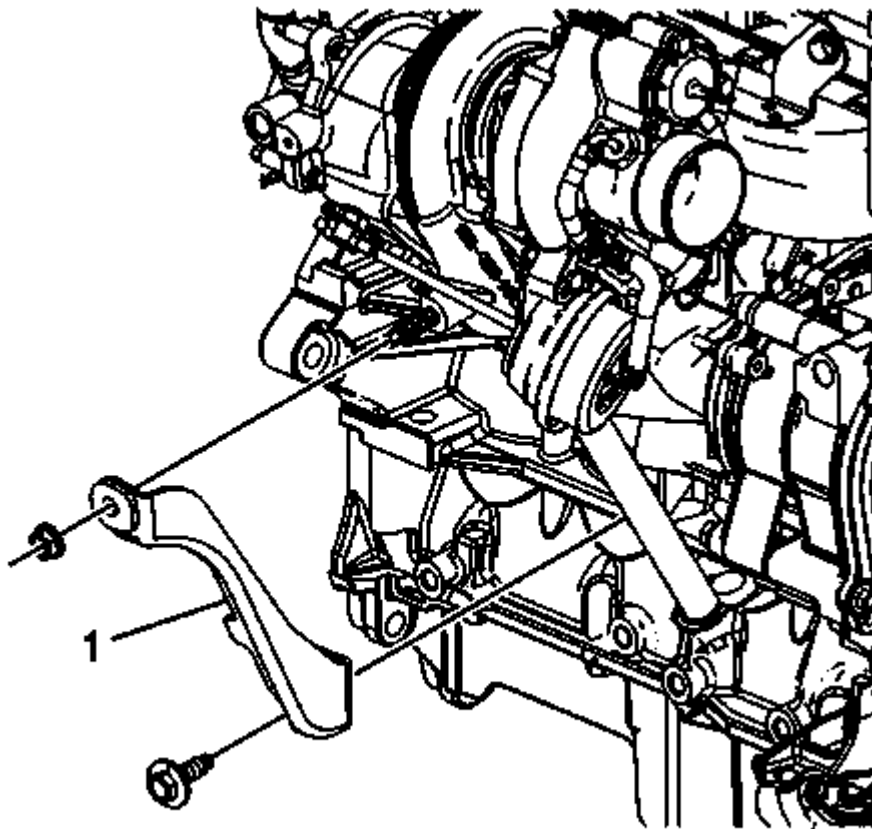
Fig. 30: Turbocharger Brace
