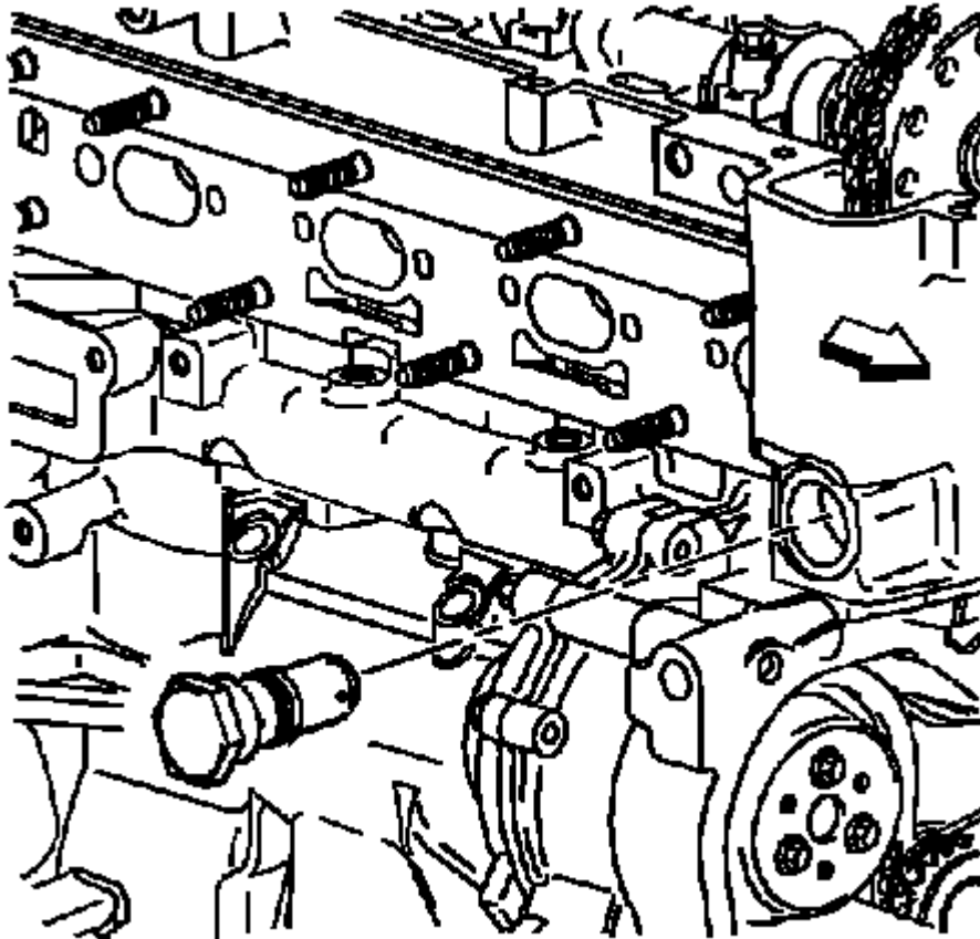
Fig. 106: Identifying Timing Chain Tensioner Courtesy of GENERAL MOTORS COMPANY
