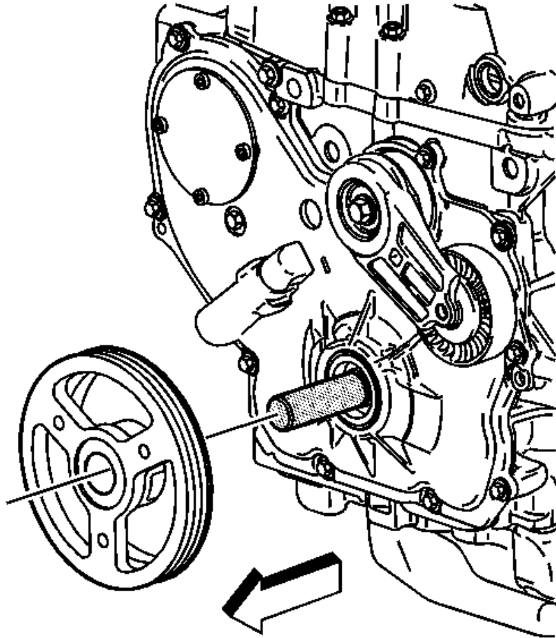
Fig. 56: View Of Crankshaft Balancer Courtesy of GENERAL MOTORS COMPANY
