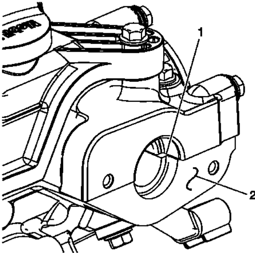
Fig. 116: Identifying Fuel Pump Roller Lifter Orifice Courtesy of GENERAL MOTORS COMPANY
