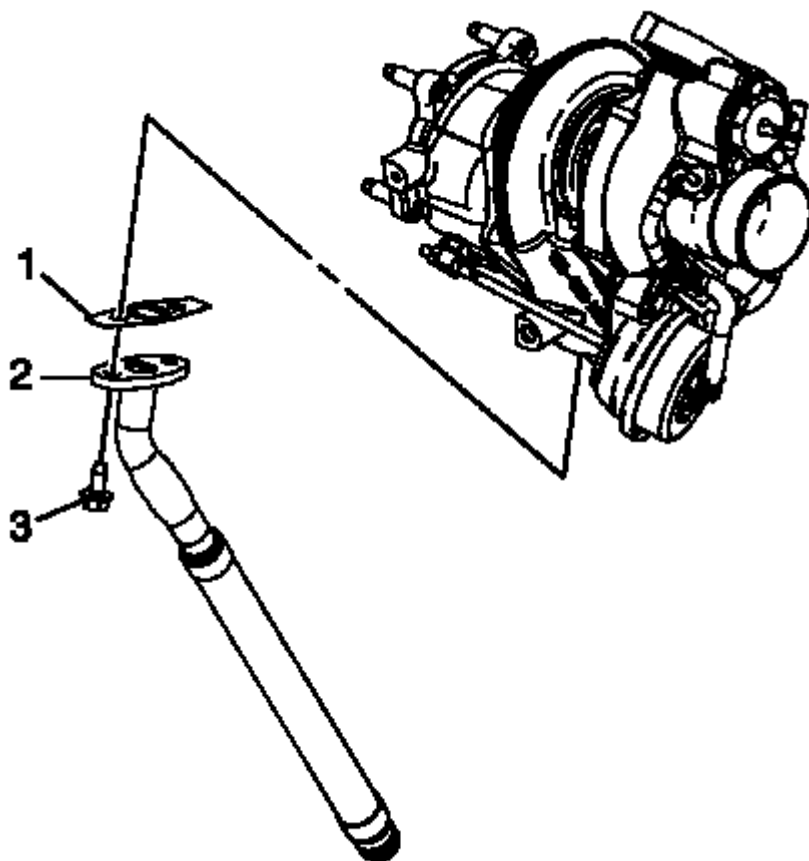
Fig. 33: Turbocharger Oil Return Pipe Courtesy of GENERAL MOTORS COMPANY
