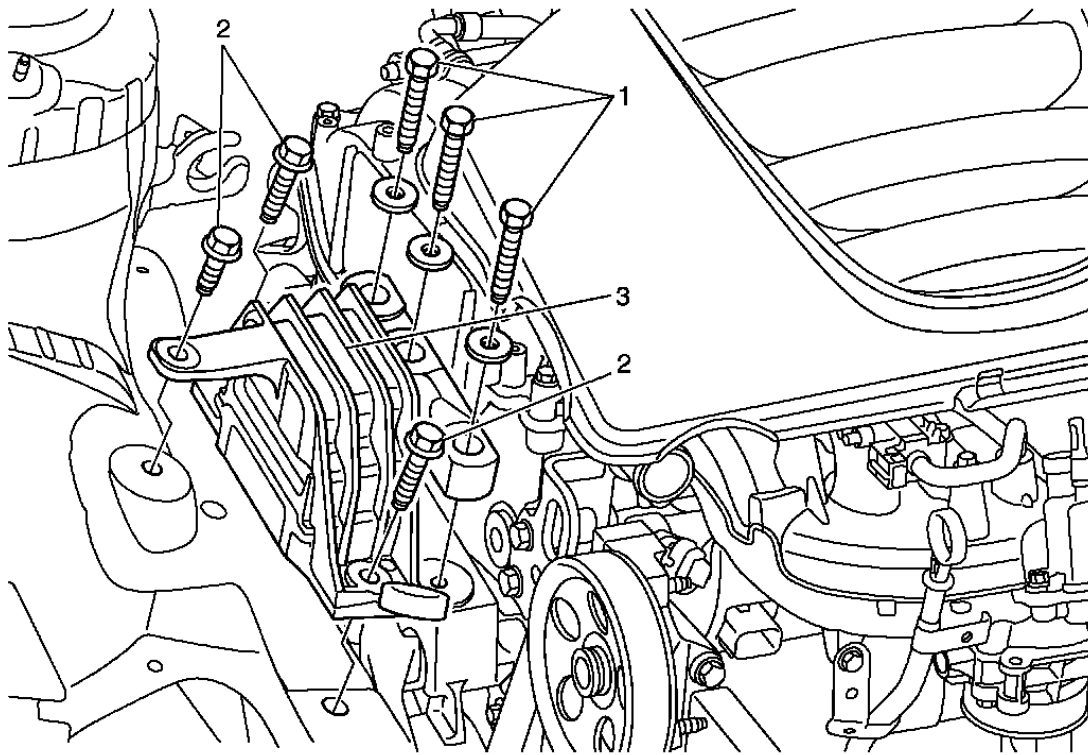
Fig. 25: Engine Mount
