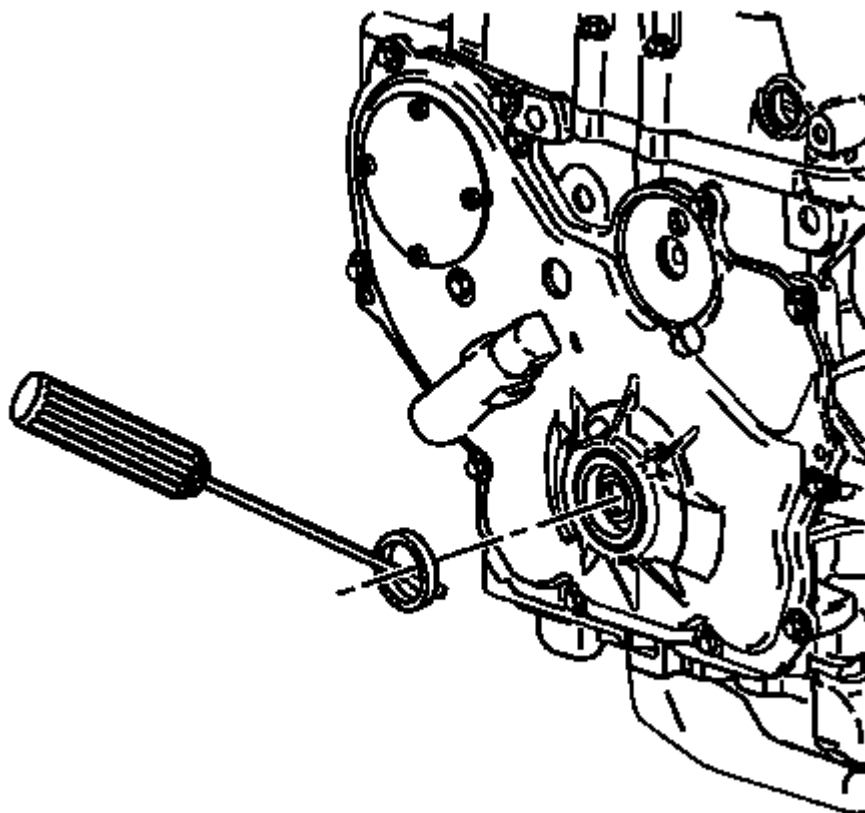
Fig. 59: Removing Crankshaft Front Oil Seal Courtesy of GENERAL MOTORS COMPANY
