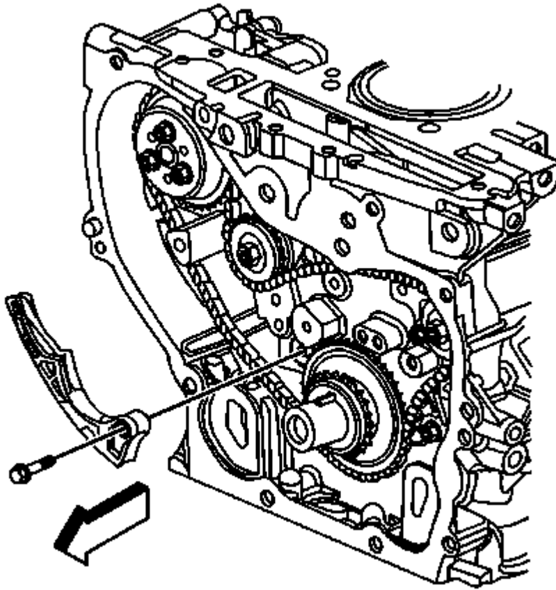
Fig. 75: Adjustable Balance Shaft Chain Guide Courtesy of GENERAL MOTORS COMPANY
