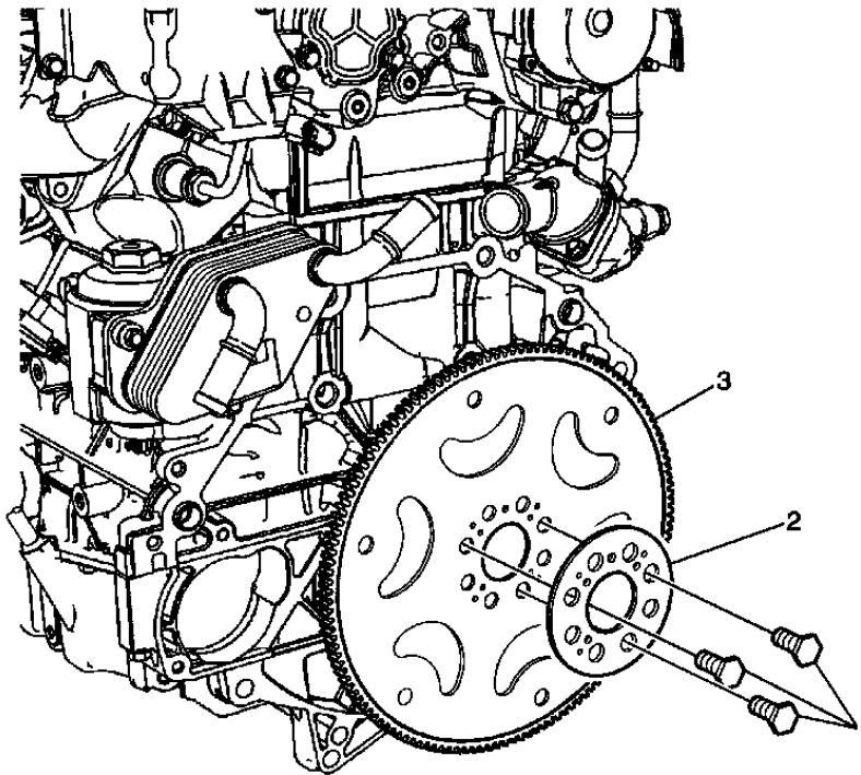
Fig. 157: Engine Flywheel
