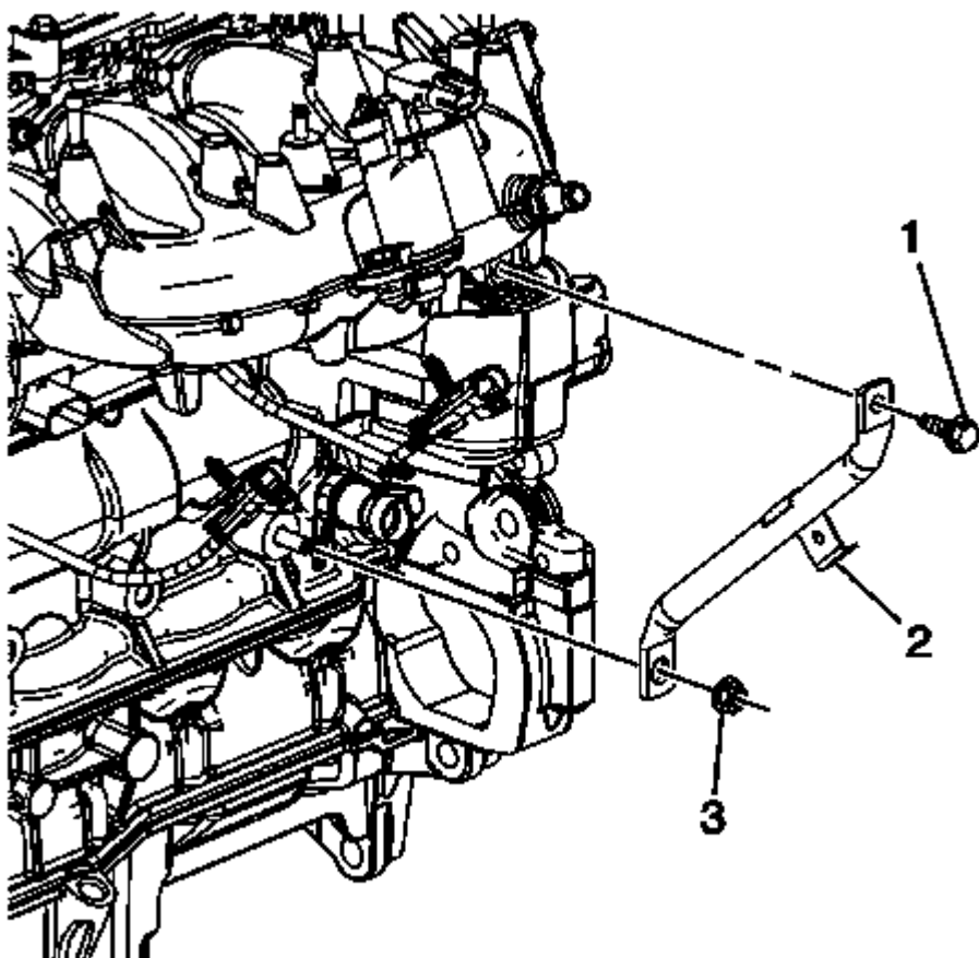
Fig. 46: Intake Manifold Brace
