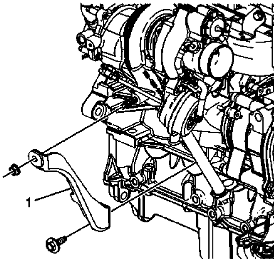
Fig. 35: Turbocharger Brace
