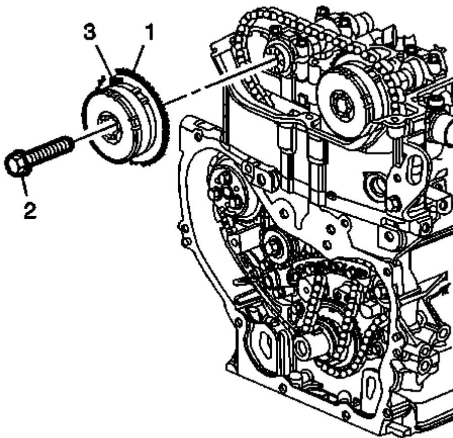
Fig. 142: Exhaust Camshaft Sprocket Courtesy of GENERAL MOTORS COMPANY
