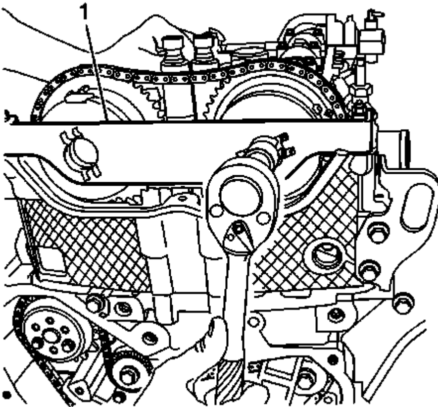
Fig. 127: Loosening/Tightening Camshaft Actuator Retainer Bolts Courtesy of GENERAL MOTORS COMPANY
