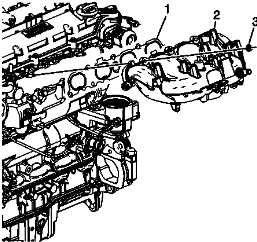
Fig. 47: Intake Manifold, Intake Manifold Bolts And Intake Manifold Gasket Courtesy of GENERAL MOTORS COMPANY
