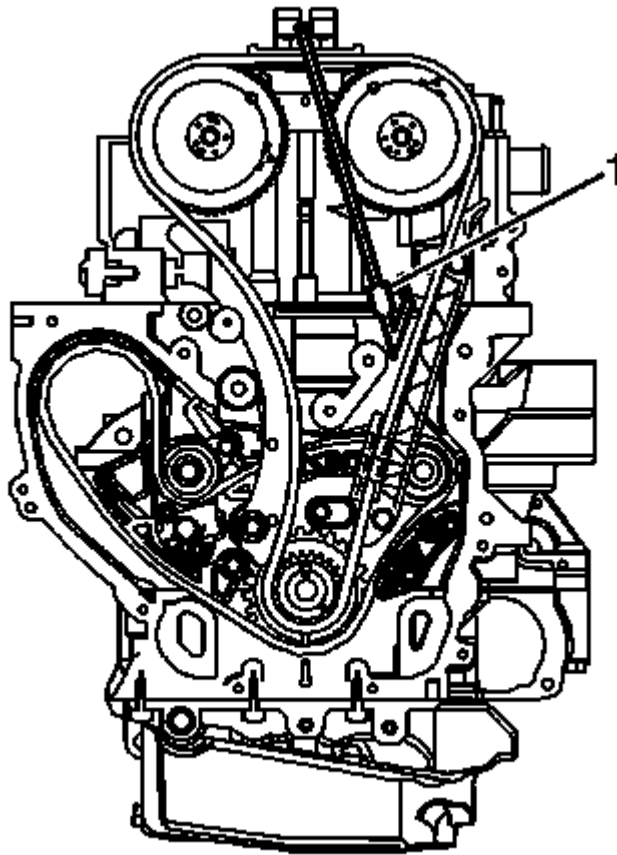
Fig. 130: View Of Timing Chain & Chain Retention Tool Courtesy of GENERAL MOTORS COMPANY
