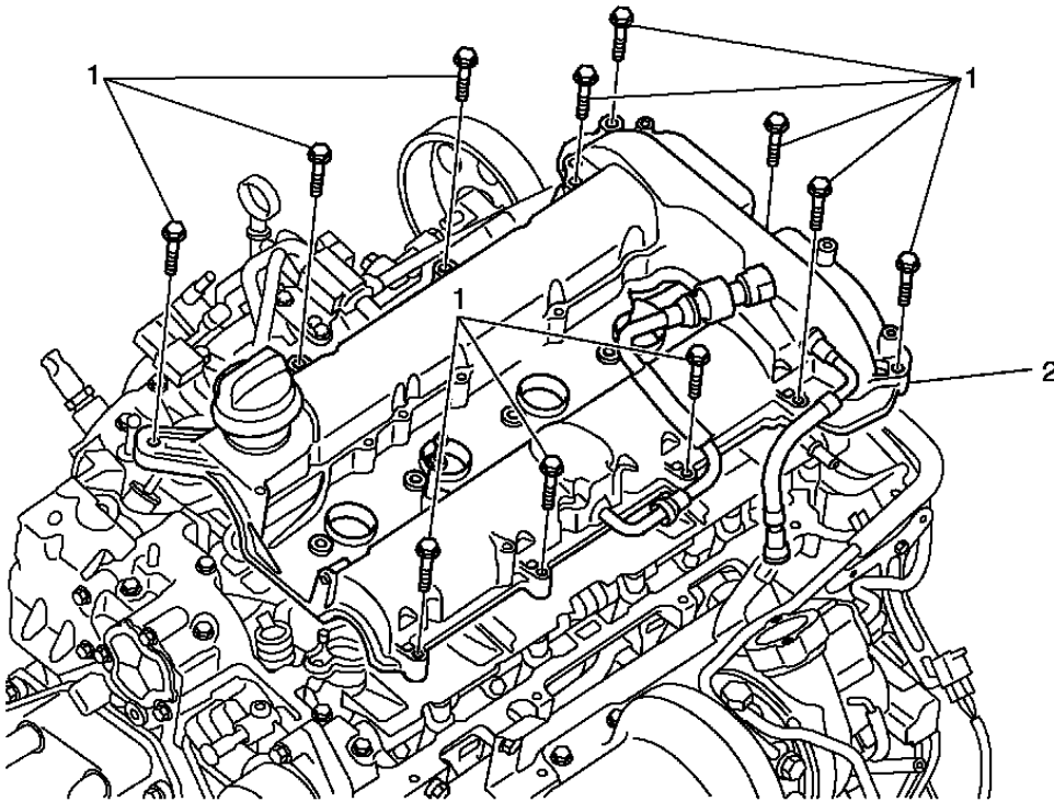
Fig. 102: Camshaft Cover
