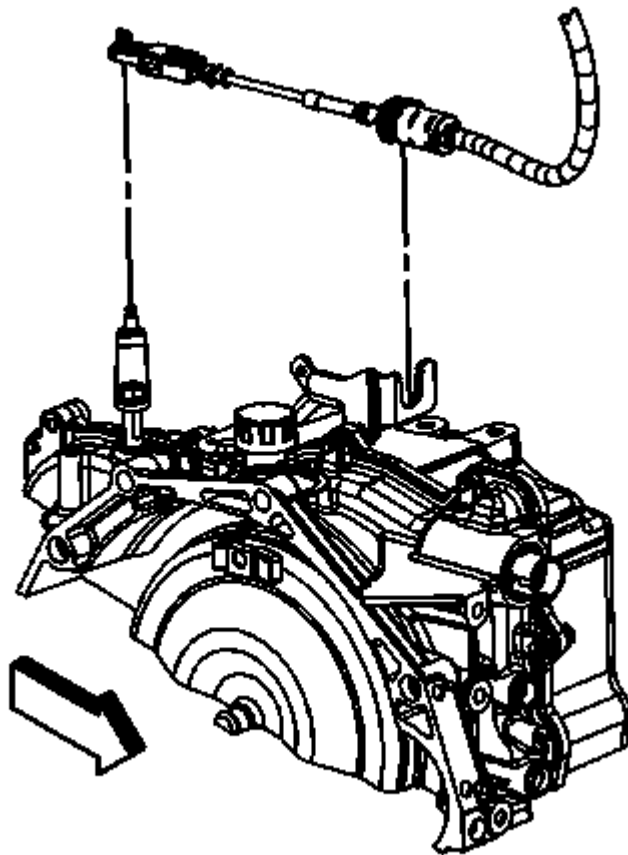
Fig. 174: Transaxle Shift Cable And Range Select Lever Courtesy of GENERAL MOTORS COMPANY
