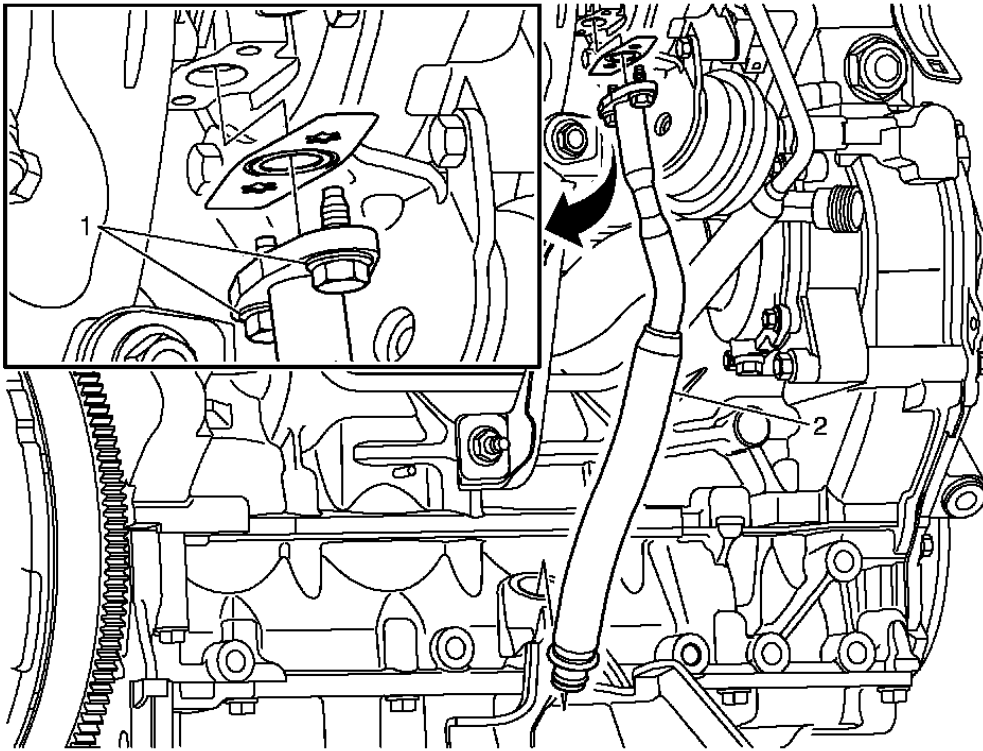
Fig. 41: Turbocharger Oil Return Pipe Courtesy of GENERAL MOTORS COMPANY
