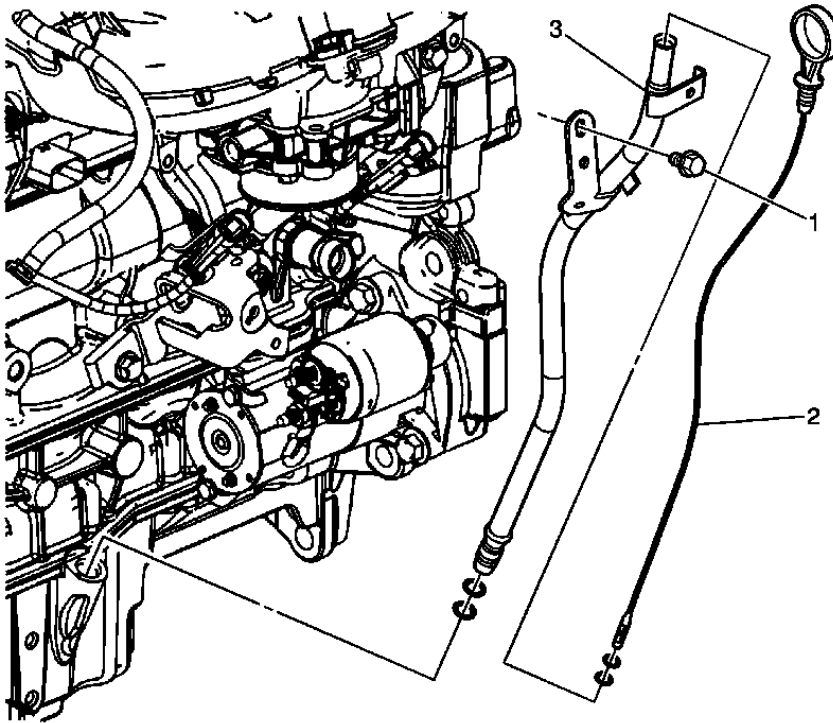
Fig. 26: Oil Level Indicator Tube Courtesy of GENERAL MOTORS COMPANY
