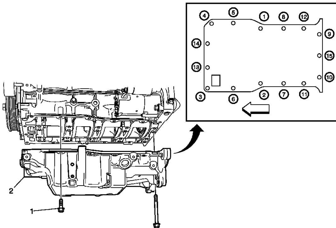
Fig. 155: Engine Oil Pan
