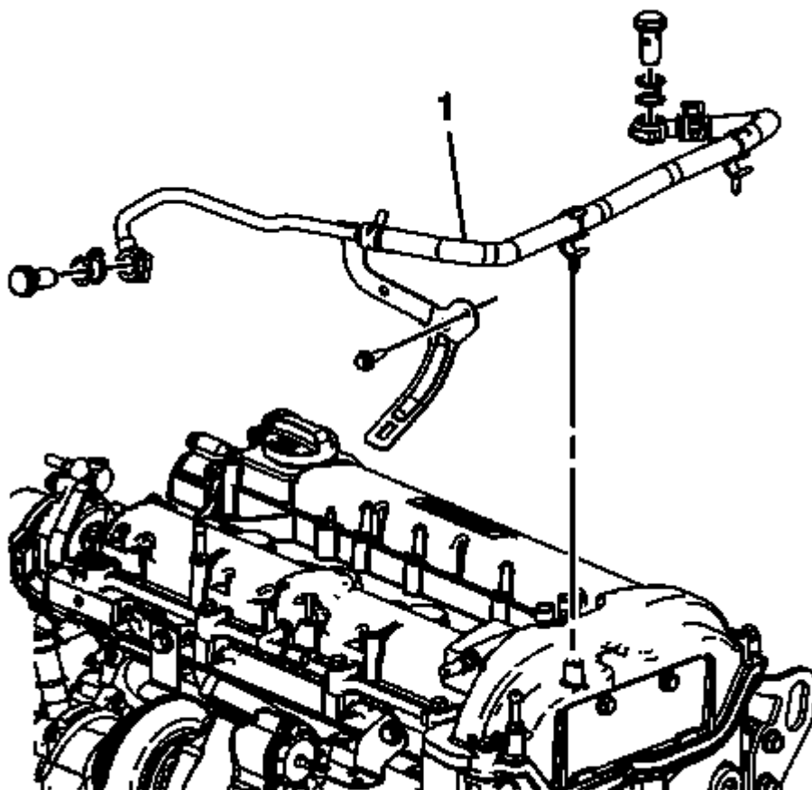
Fig. 29: Turbocharger Coolant Feed Pipe Courtesy of GENERAL MOTORS COMPANY
