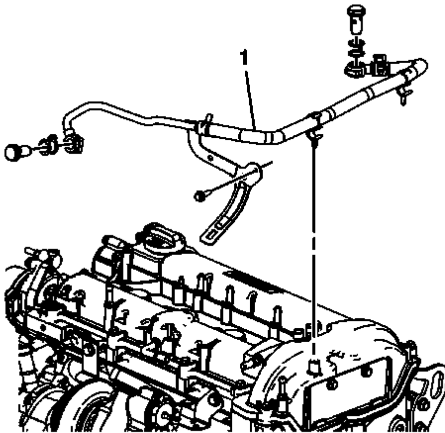
Fig. 36: Turbocharger Coolant Feed Pipe Courtesy of GENERAL MOTORS COMPANY
