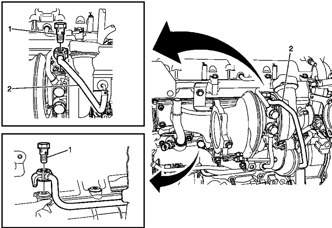
Fig. 40: Turbocharger Oil Feed Pipe Courtesy of GENERAL MOTORS COMPANY
