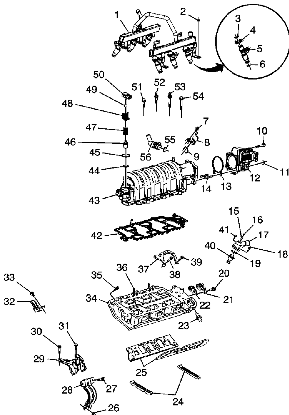
Fig. 4: Identifying Engine Block & Components Courtesy of GENERAL MOTORS CORP.
