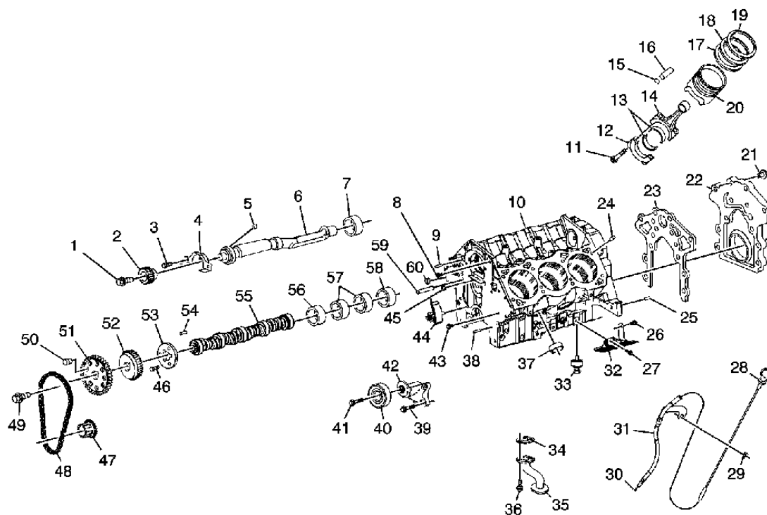
Fig. 2: Exploded View Of Upper Intake Manifold & Components Courtesy of GENERAL MOTORS CORP.
