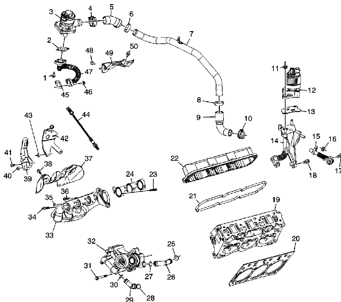
Fig. 8: View Of Engine Oil Fill Cap Courtesy of GENERAL MOTORS CORP.
