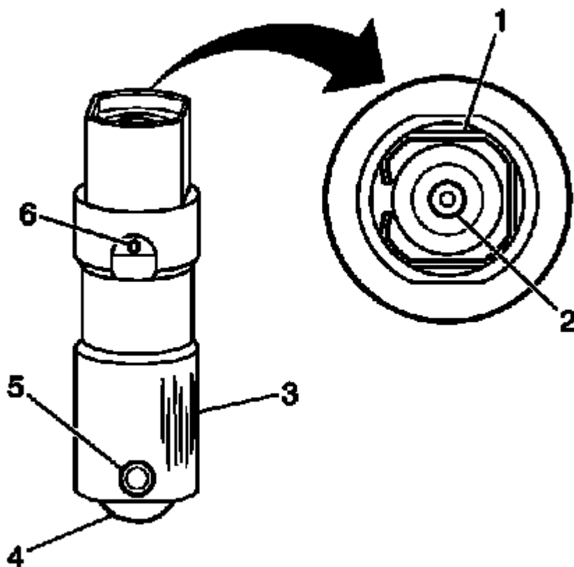
Fig. 372: View Of Valve Lifter Guides Courtesy of GENERAL MOTORS CORP.
