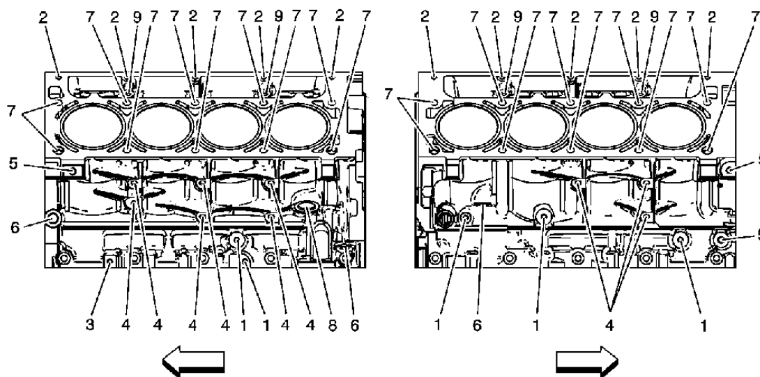
Fig. 494: View Of Right Valve Rocker Arm Cover Courtesy of GENERAL MOTORS CORP.
