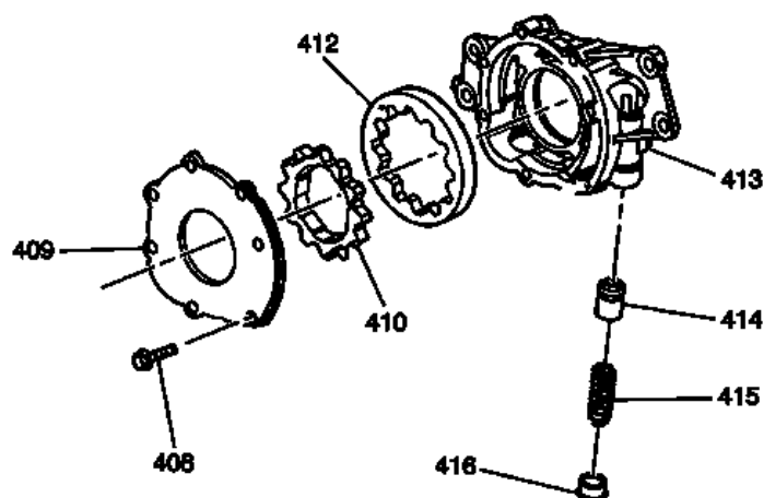
Fig. 504: Identifying Oil Filter Adapter & Heat Shield Courtesy of GENERAL MOTORS CORP.
