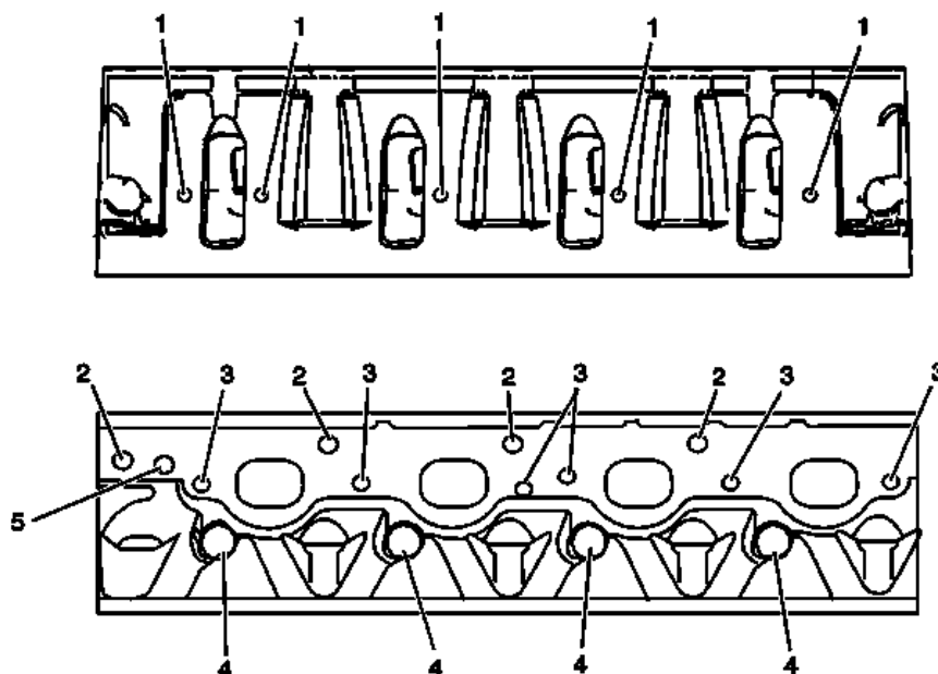
Fig. 497: Identifying Ignition Coil Assembly Bolts And Nuts Courtesy of GENERAL MOTORS CORP.
