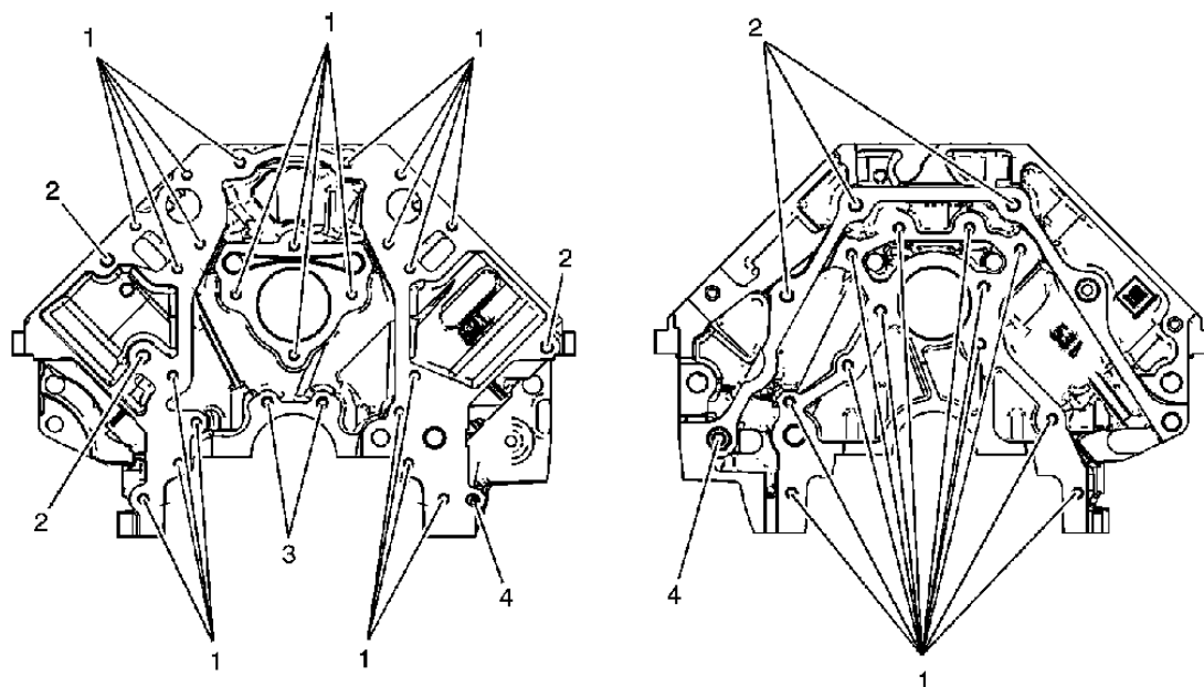
Fig. 493: Locating Positive Crankcase Ventilation (PCV) Tube Courtesy of GENERAL MOTORS CORP.
