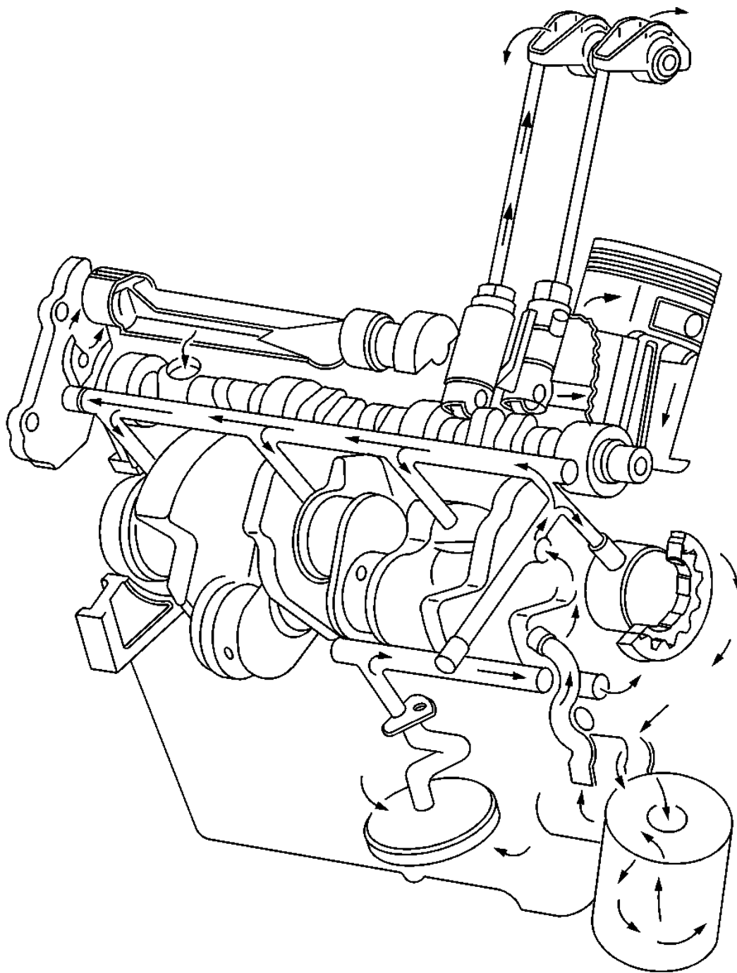
Fig. 491: Identifying Cylinder Head To Lower Intake Manifold Joint Courtesy of GENERAL MOTORS CORP.
