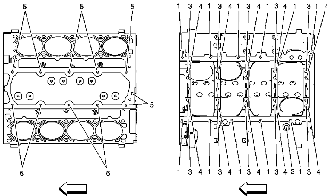
Fig. 495: Identifying Cylinder Head To Lower Intake Manifold Joint Courtesy of GENERAL MOTORS CORP.
