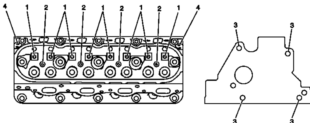
Fig. 496: Identifying Fresh Air Tube & Valve Rocker Arm Cover Courtesy of GENERAL MOTORS CORP.
