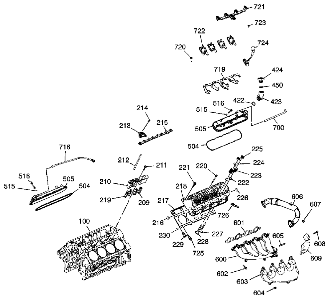
Fig. 499: Identifying Left Exhaust Manifold, Gasket & Bolts Courtesy of GENERAL MOTORS CORP.
