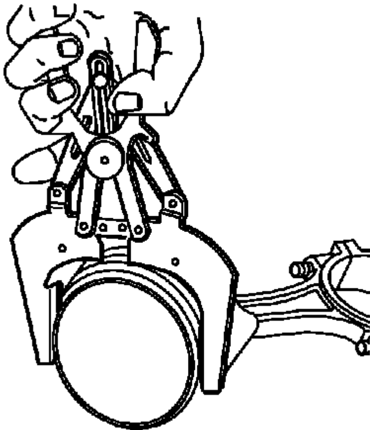
Fig. 356: View Of Connecting Rod Courtesy of GENERAL MOTORS CORP.
