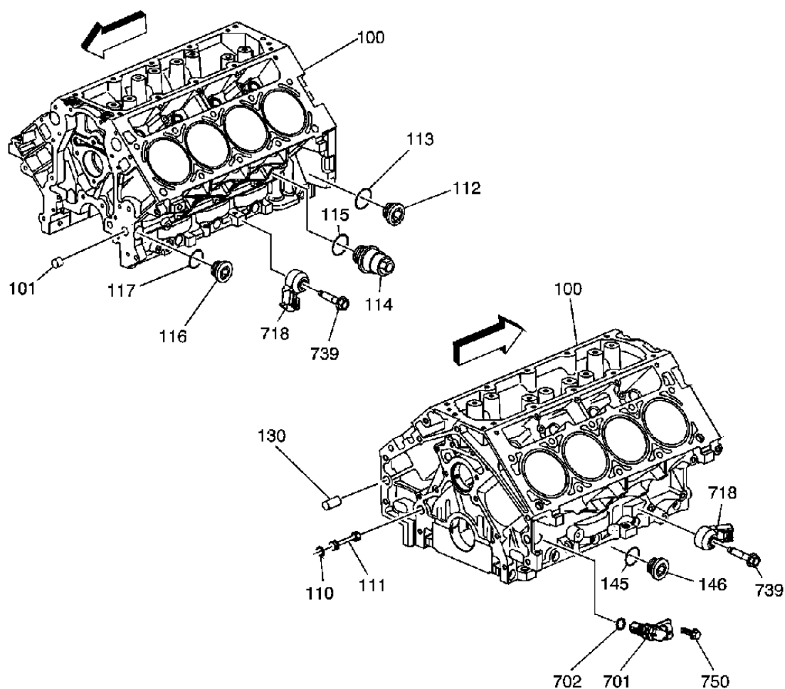
Fig. 503: Locating Oil Filter Bypass Hole & Bypass Valve Courtesy of GENERAL MOTORS CORP.
