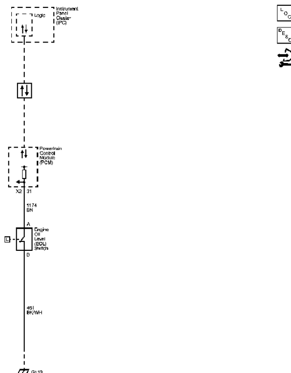
Fig. 1: Engine Oil Level Switch Wiring Schematic Courtesy of GENERAL MOTORS CORP.
