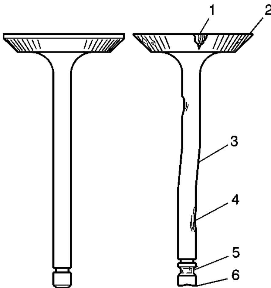
Fig. 381: View Of Valve Components Courtesy of GENERAL MOTORS CORP.
