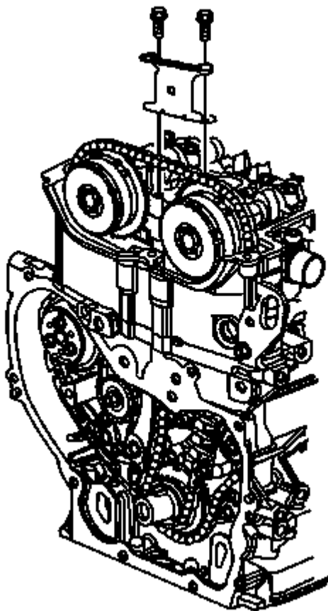
Fig. 114: Upper Timing Chain Guide And Bolts Courtesy of GENERAL MOTORS CORP.
