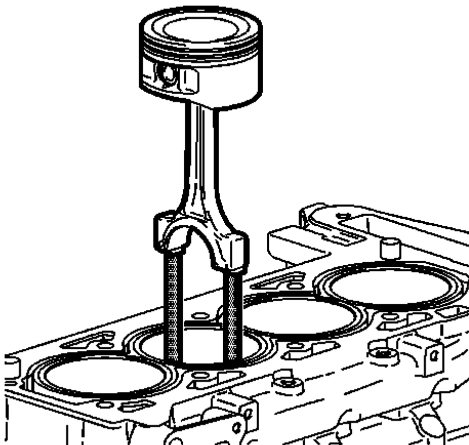
Fig. 177: Connecting Rod And Piston Courtesy of GENERAL MOTORS CORP.
