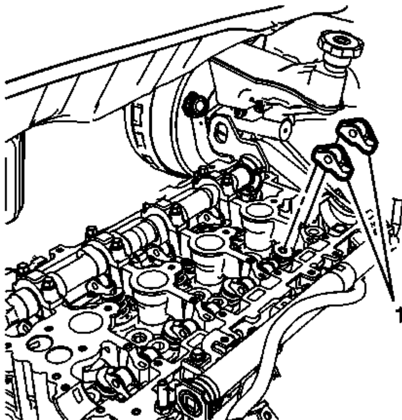
Fig. 134: Camshaft Roller Followers Courtesy of GENERAL MOTORS CORP.
