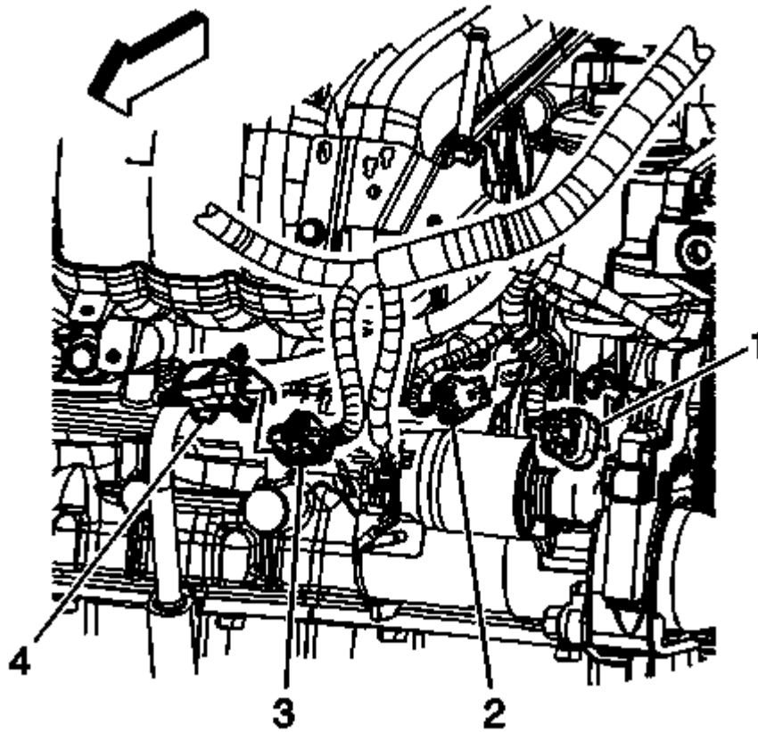
Fig. 4: Starter And Engine Electrical Connectors Courtesy of GENERAL MOTORS CORP.
