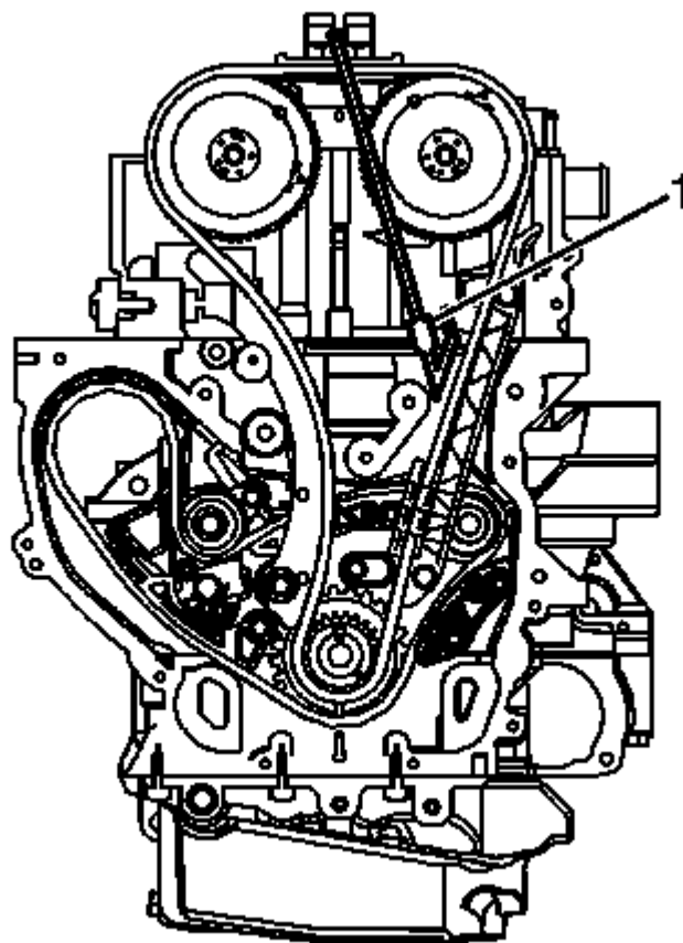
Fig. 162: Timing Chain & Chain Retention Tool Courtesy of GENERAL MOTORS CORP.
