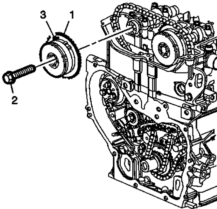
Fig. 148: Exhaust Camshaft Actuator Courtesy of GENERAL MOTORS CORP.
