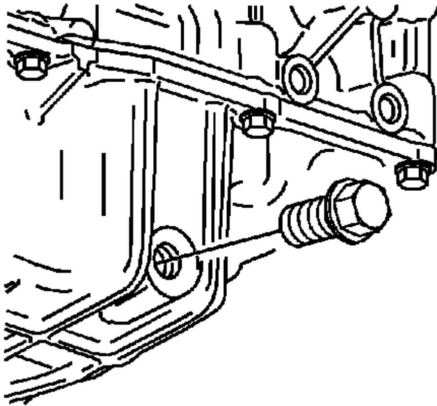
Fig. 169: Oil Pan Drain Plug
