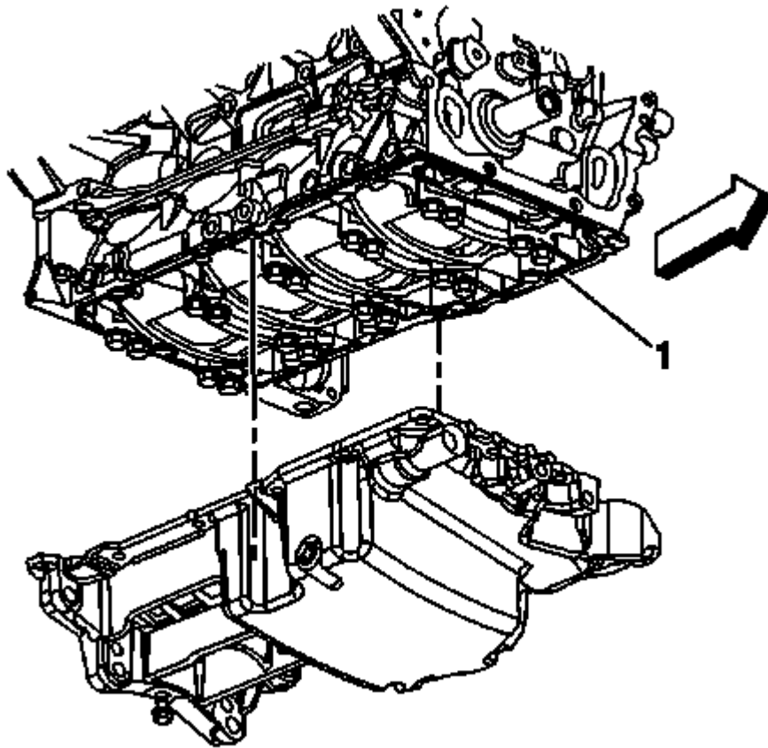
Fig. 171: Oil Pan
