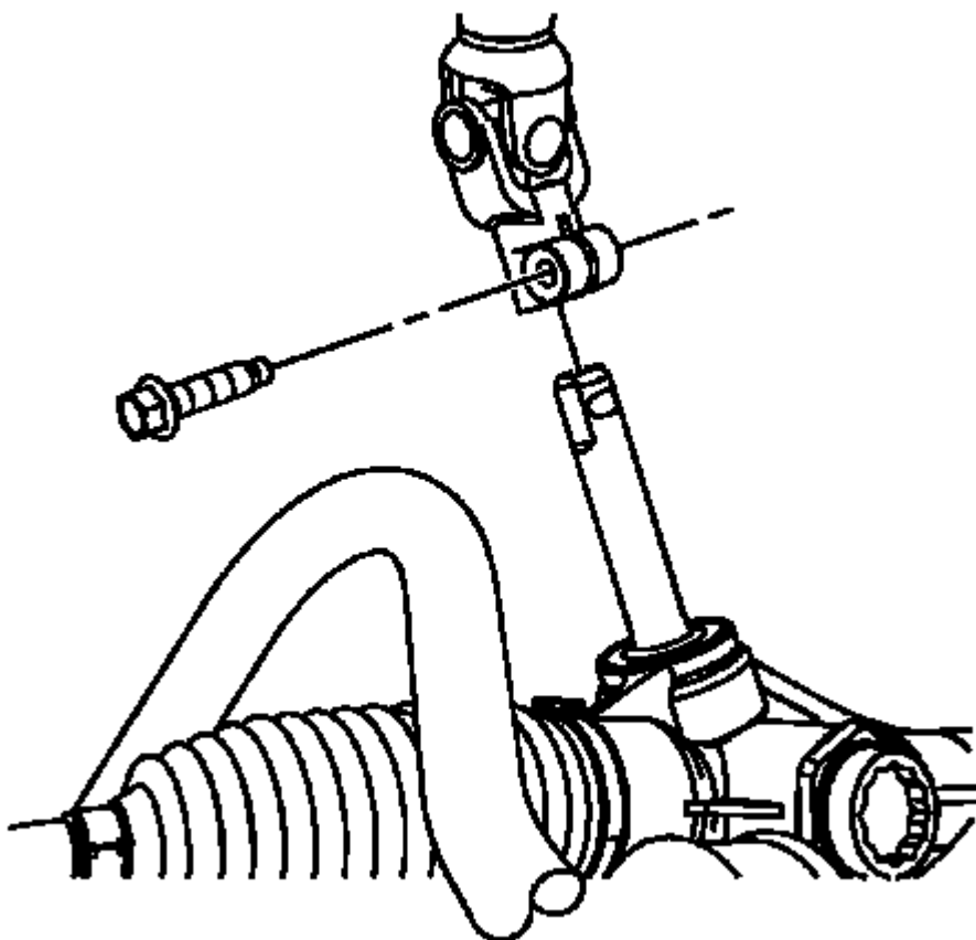
Fig. 189: Intermediate Shaft To Steering Gear Pinch Bolt Courtesy of GENERAL MOTORS CORP.
