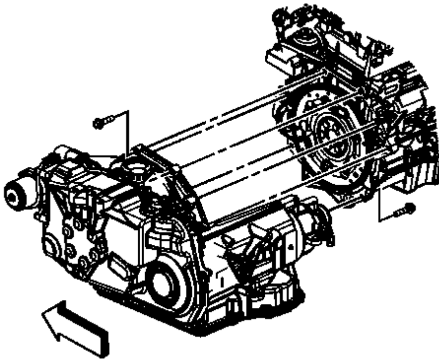
Fig. 196: Transaxle To Engine Bolts Courtesy of GENERAL MOTORS CORP.
