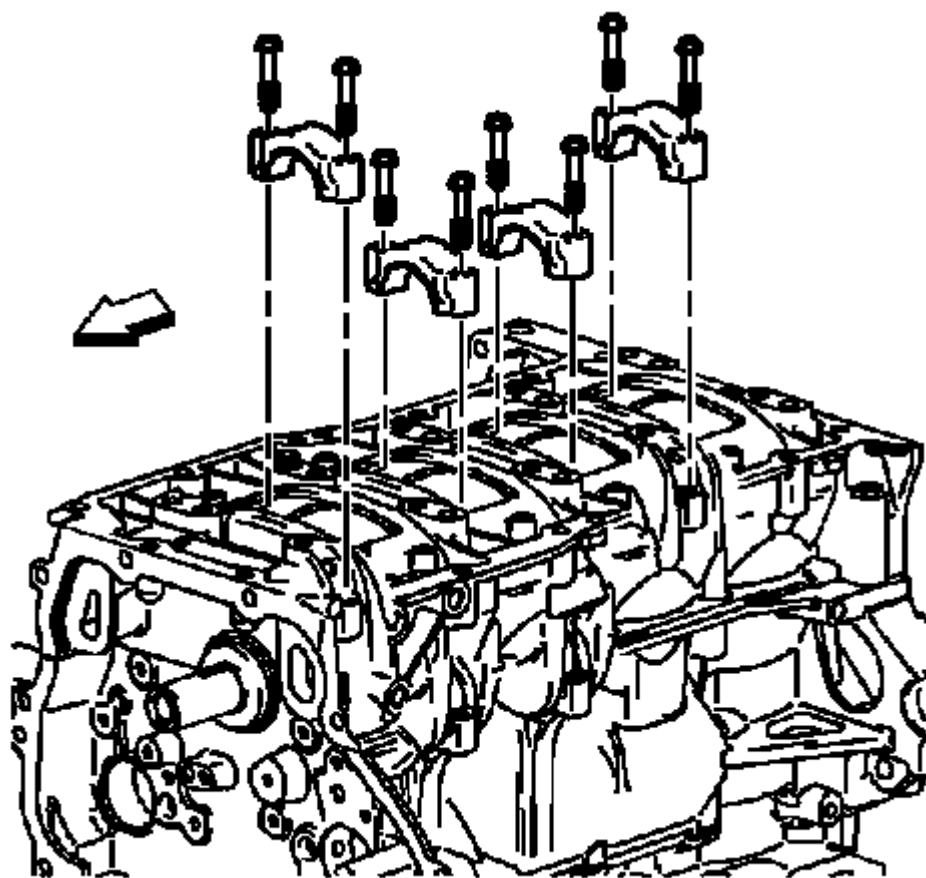
Fig. 176: Connecting Rod Bolts & Caps Courtesy of GENERAL MOTORS CORP.
