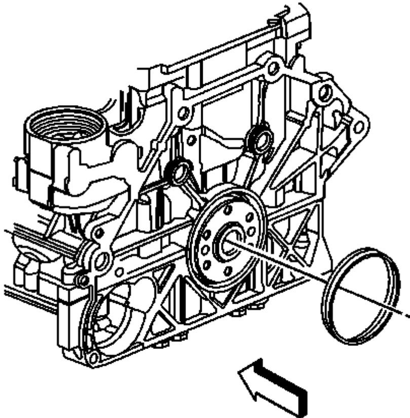
Fig. 183: Crankshaft Rear Oil Seal Courtesy of GENERAL MOTORS CORP.
