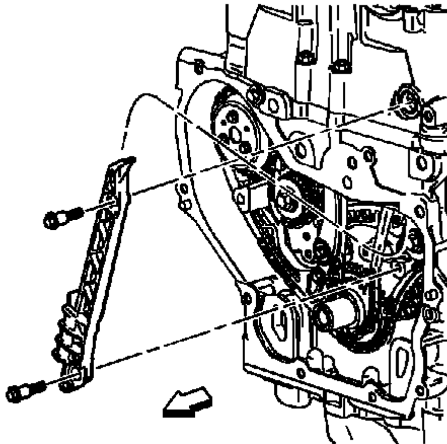
Fig. 82: Fixed Timing Chain Guide
