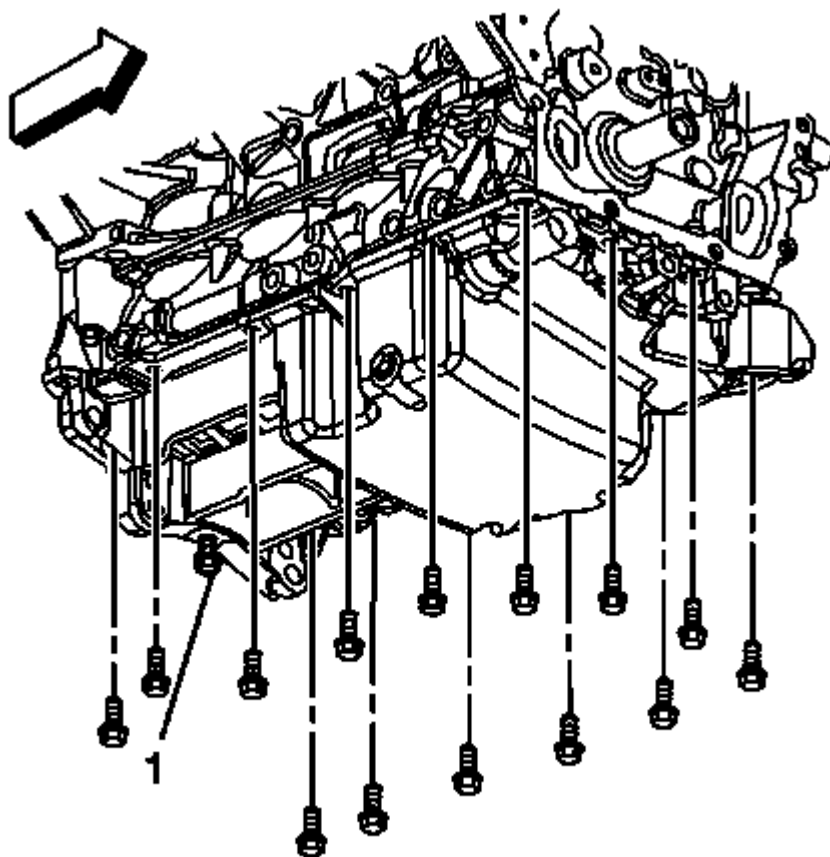
Fig. 170: Oil Pan Bolts
