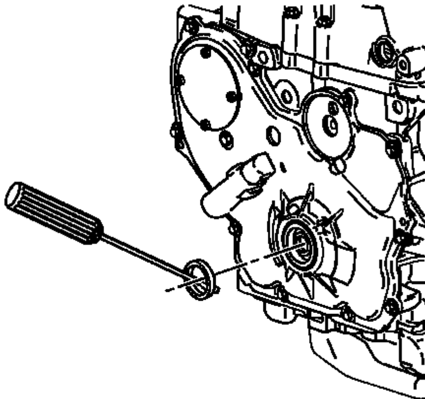
Fig. 45: Front Crankshaft Oil Seal Courtesy of GENERAL MOTORS CORP.
