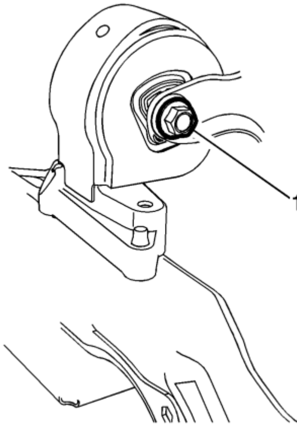
Fig. 11: Rear Transaxle Mount Through Bolt Courtesy of GENERAL MOTORS CORP.
