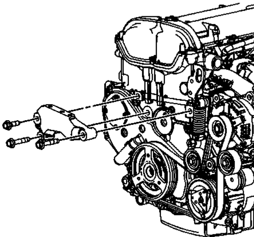
Fig. 53: Engine Mount Bracket And Engine Bolts Courtesy of GENERAL MOTORS CORP.
