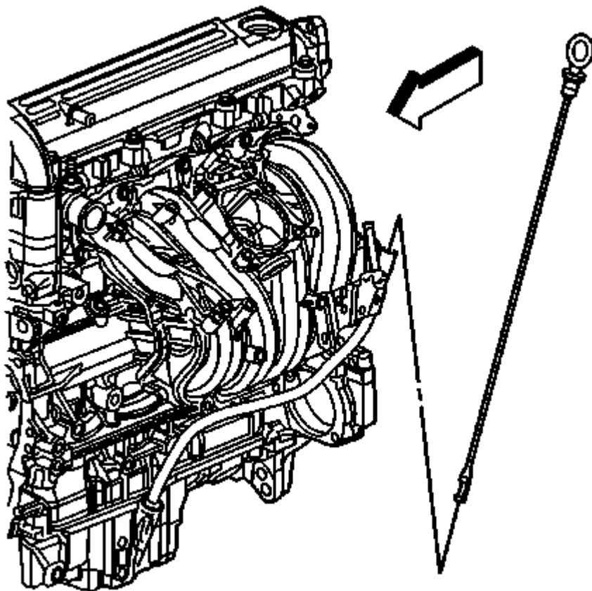
Fig. 35: Oil Level Indicator
