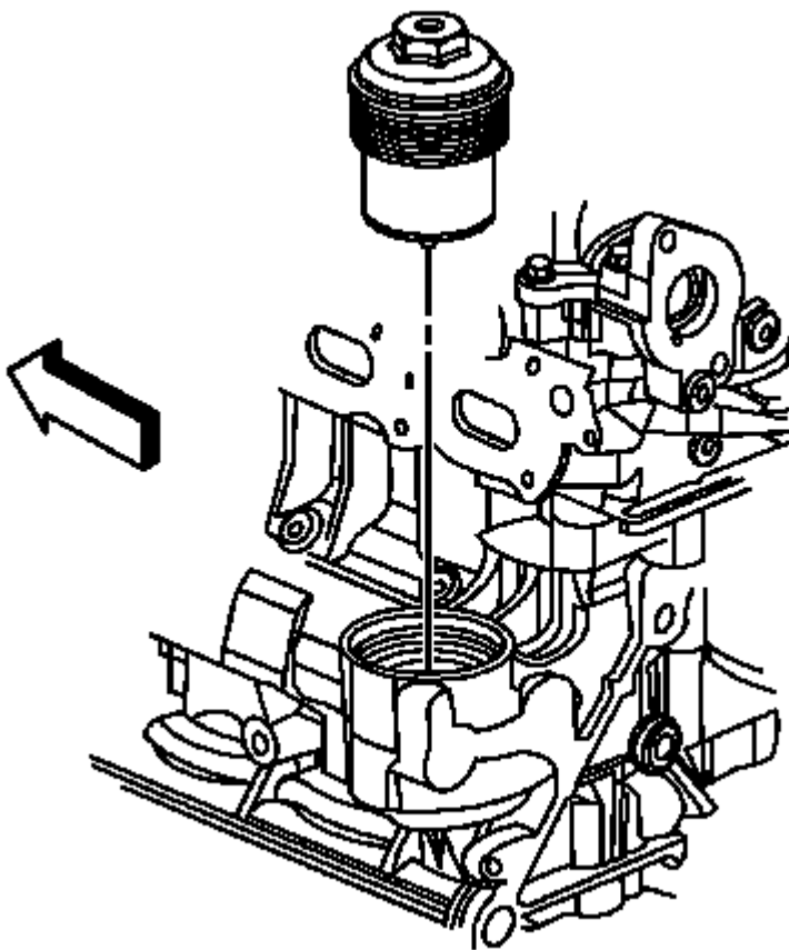
Fig. 208: Oil Filter Cap Courtesy of GENERAL MOTORS CORP.
