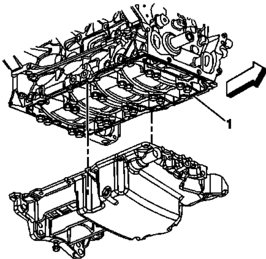
Fig. 172: Oil Pan
