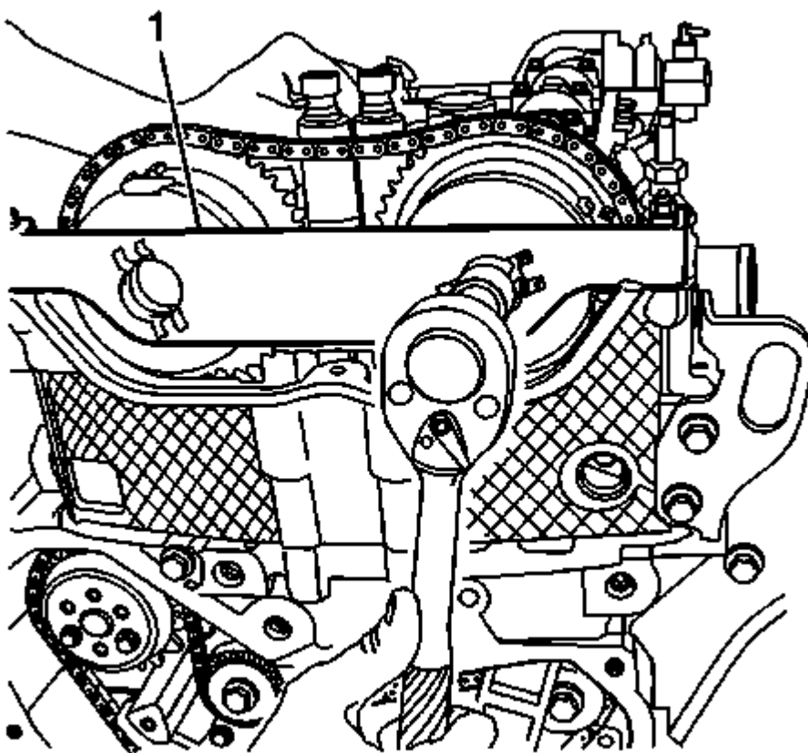
Fig. 113: Camshaft Actuator Retainer Courtesy of GENERAL MOTORS CORP.
