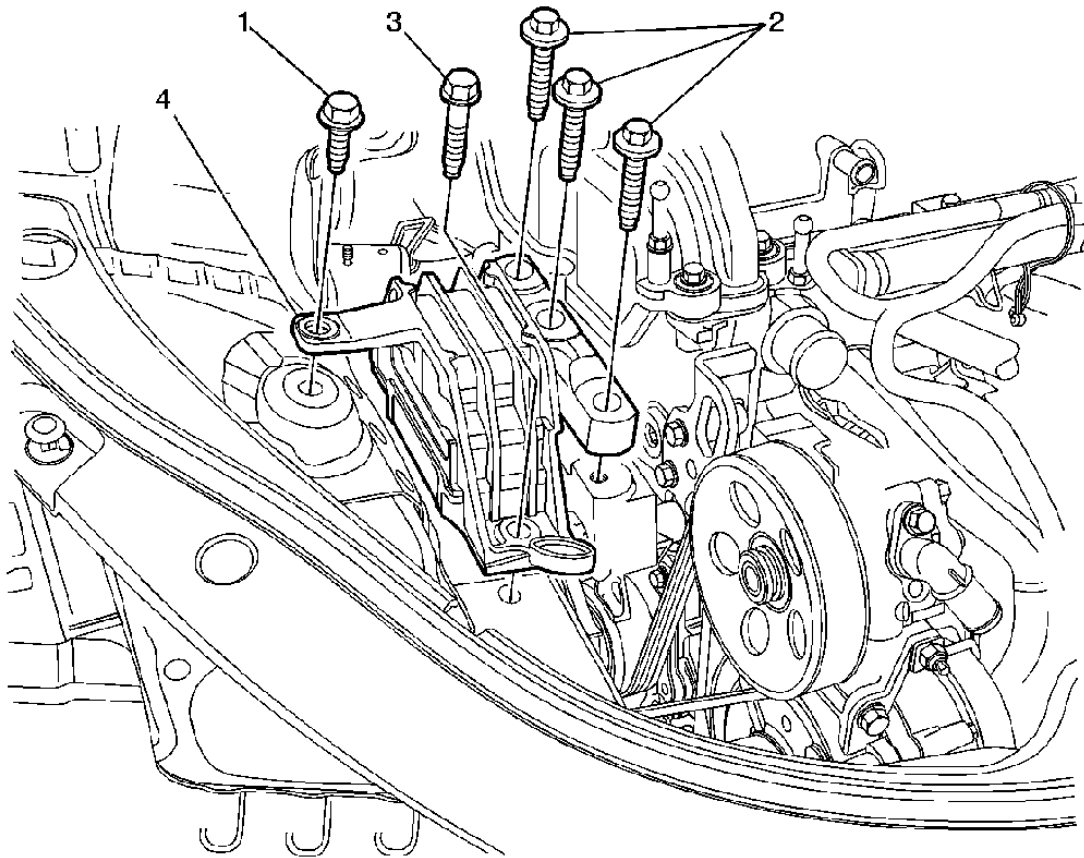
Fig. 22: Engine Mount
