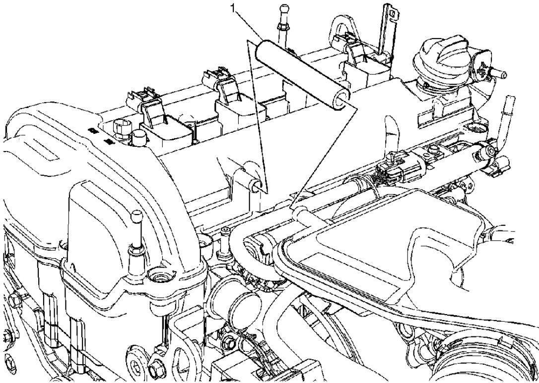
Fig. 36: Positive Crankcase Ventilation Hose/Pipe/Tube Courtesy of GENERAL MOTORS CORP.
