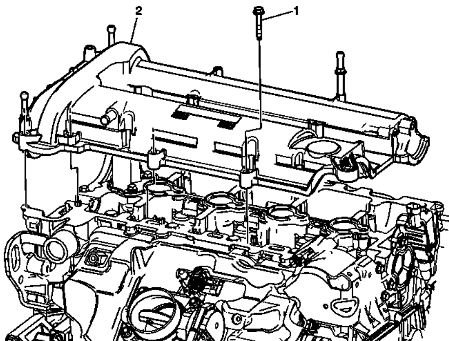
Fig. 89: Camshaft Cover
