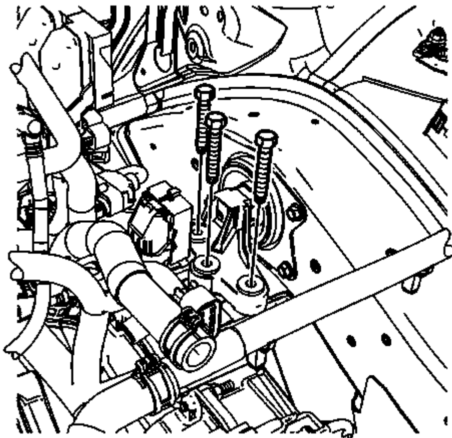
Fig. 200: Transaxle Mount To Transaxle Bolts Courtesy of GENERAL MOTORS CORP.
