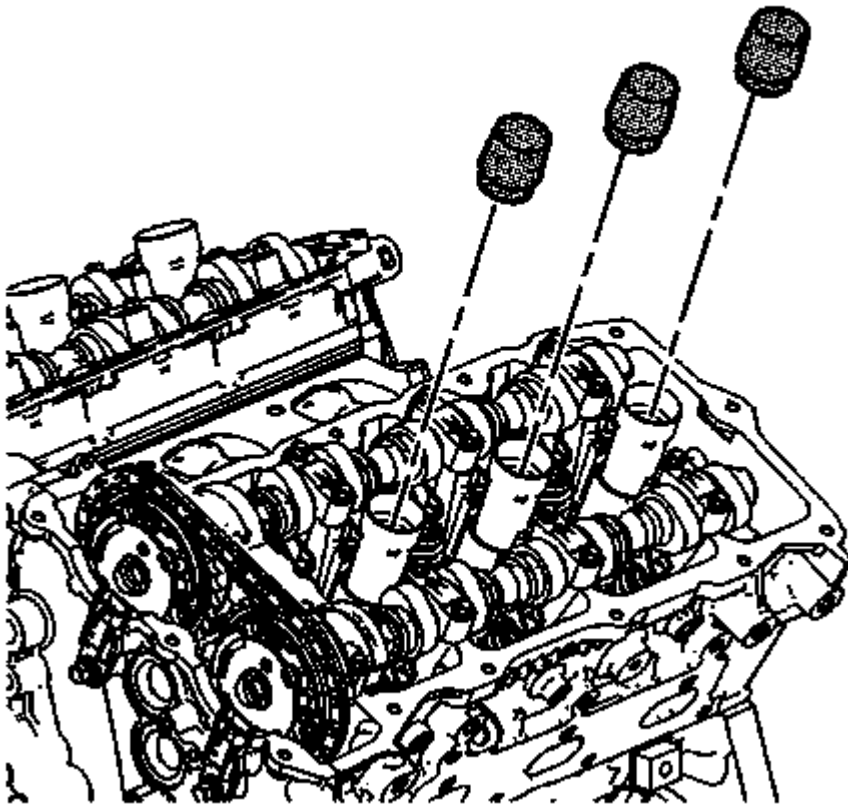
Fig. 50: Plugging Spark Plug Holes Courtesy of GENERAL MOTORS COMPANY
