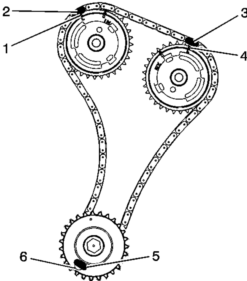
Fig. 115: Locating Left Secondary Camshaft Drive Chain Timing Marks Courtesy of GENERAL MOTORS COMPANY
