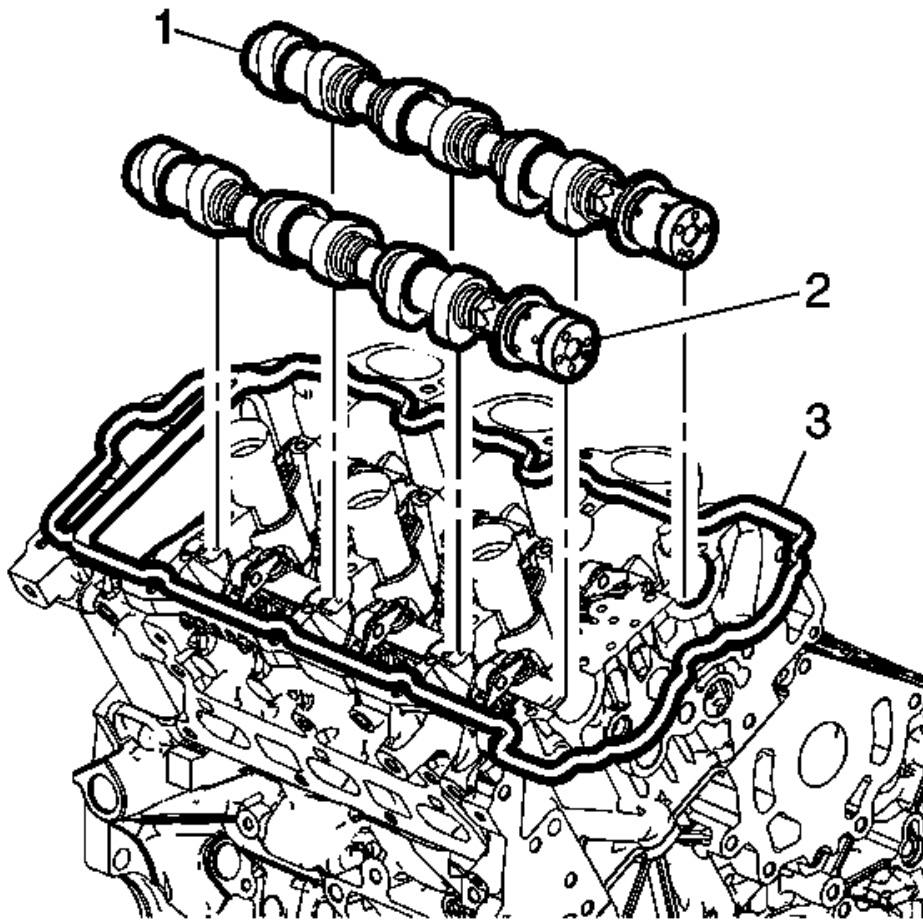
Fig. 140: Right Cylinder Head Camshaft Intake And Exhaust Positioning Points Courtesy of GENERAL MOTORS COMPANY
