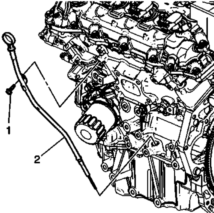
Fig. 29: View Of Oil Level Indicator Tube Components Courtesy of GENERAL MOTORS COMPANY
