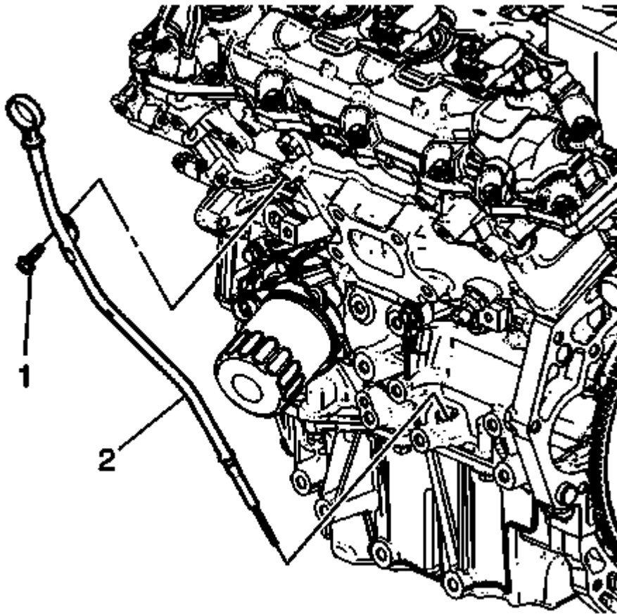
Fig. 26: View Of Oil Level Indicator Tube Components Courtesy of GENERAL MOTORS COMPANY
