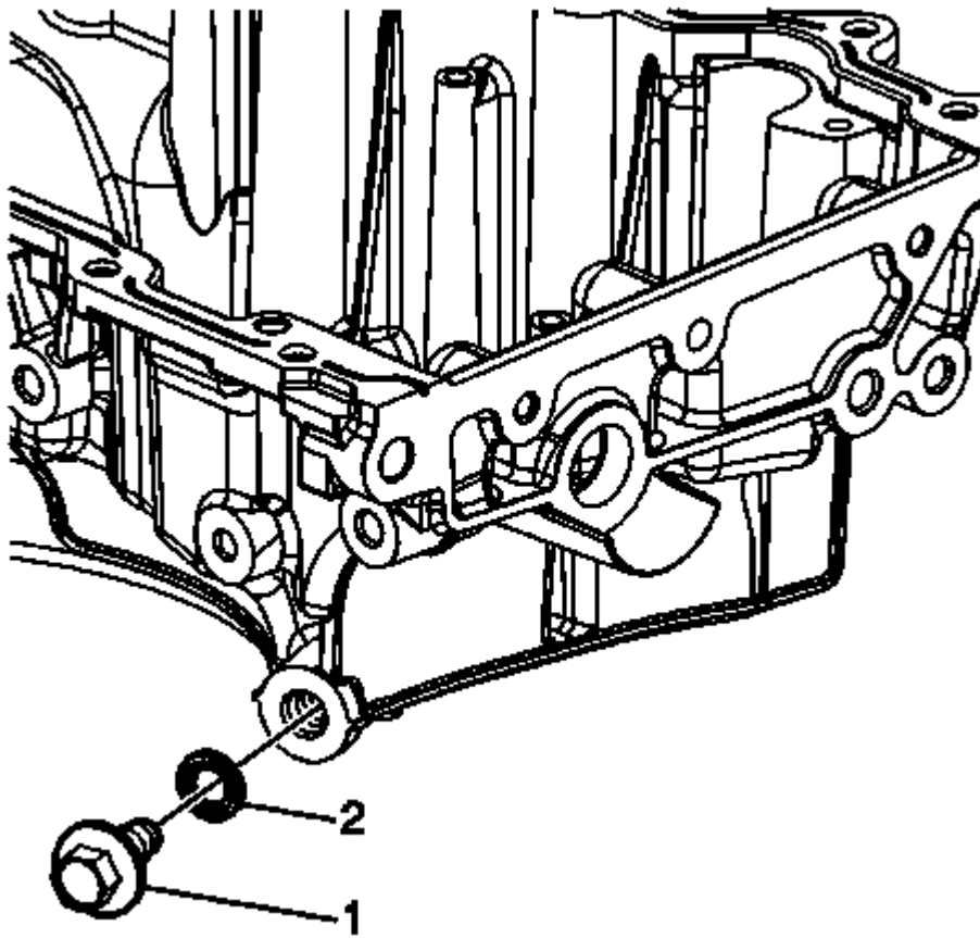
Fig. 201: Oil Pan Drain Plug And Seal Courtesy of GENERAL MOTORS COMPANY
