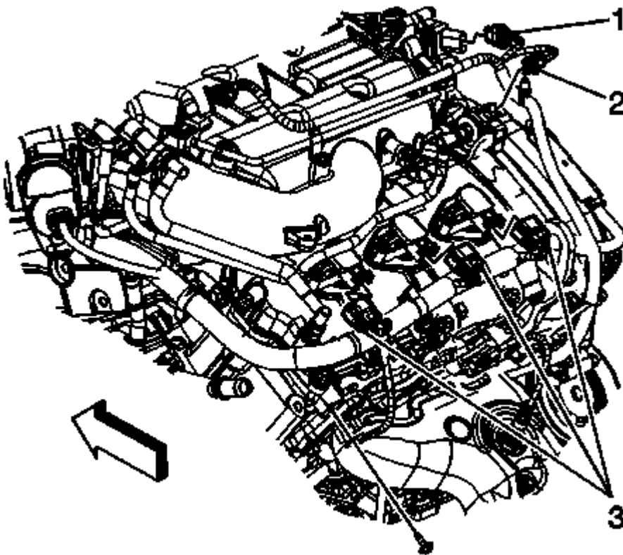
Fig. 229: Identifying EVAP Canister Purge Solenoid, Ignition Coils & Intake Manifold Tuning Valve
