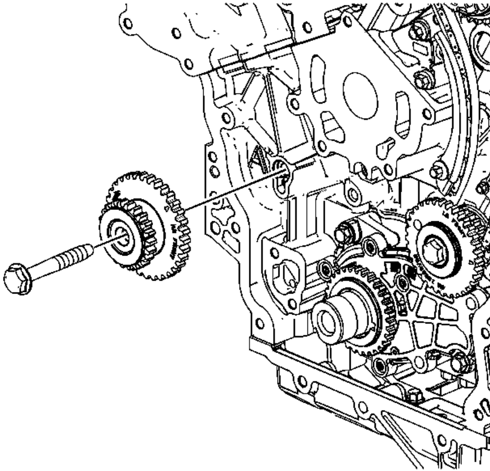
Fig. 79: Identifying Camshaft Intermediate Drive Chain Idler & Bolt Courtesy of GENERAL MOTORS COMPANY
