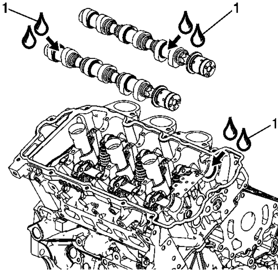
Fig. 139: Right Cylinder Head Camshaft Lubrication Points Courtesy of GENERAL MOTORS COMPANY
