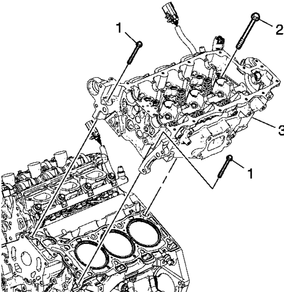
Fig. 172: View Of Left Cylinder Head & Bolts Courtesy of GENERAL MOTORS COMPANY
