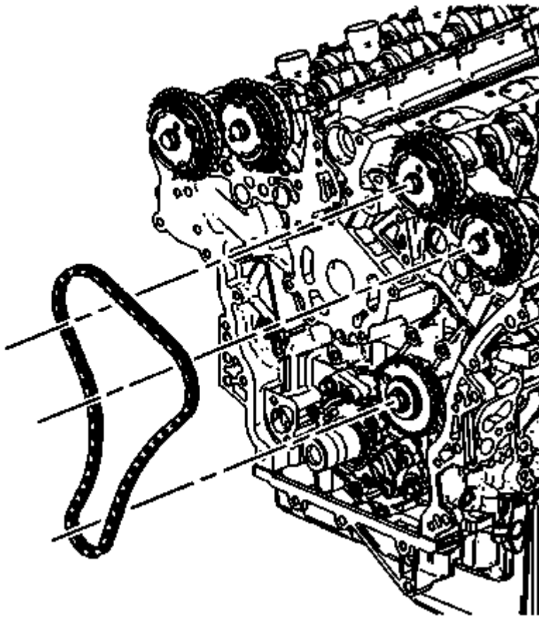
Fig. 60: View Of Left Bank Secondary Camshaft Drive Chain Courtesy of GENERAL MOTORS COMPANY
