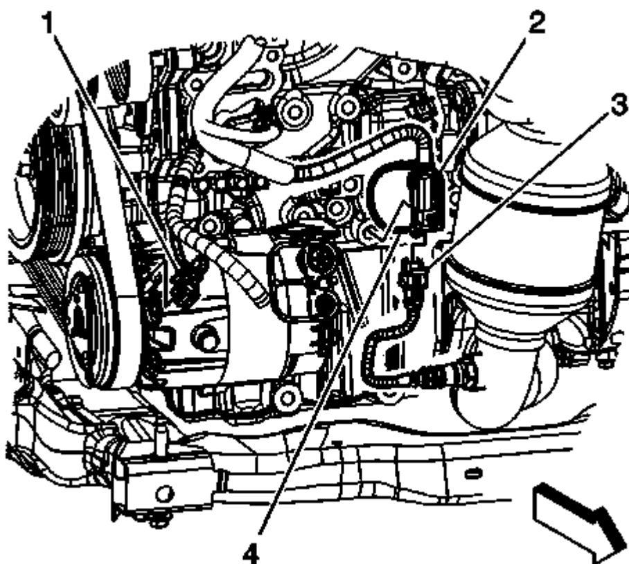
Fig. 217: Electrical Connectors - Left Side Courtesy of GENERAL MOTORS COMPANY
