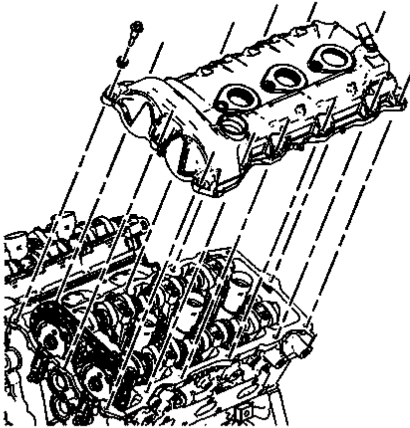
Fig. 41: View Of Left Camshaft Cover Courtesy of GENERAL MOTORS COMPANY
