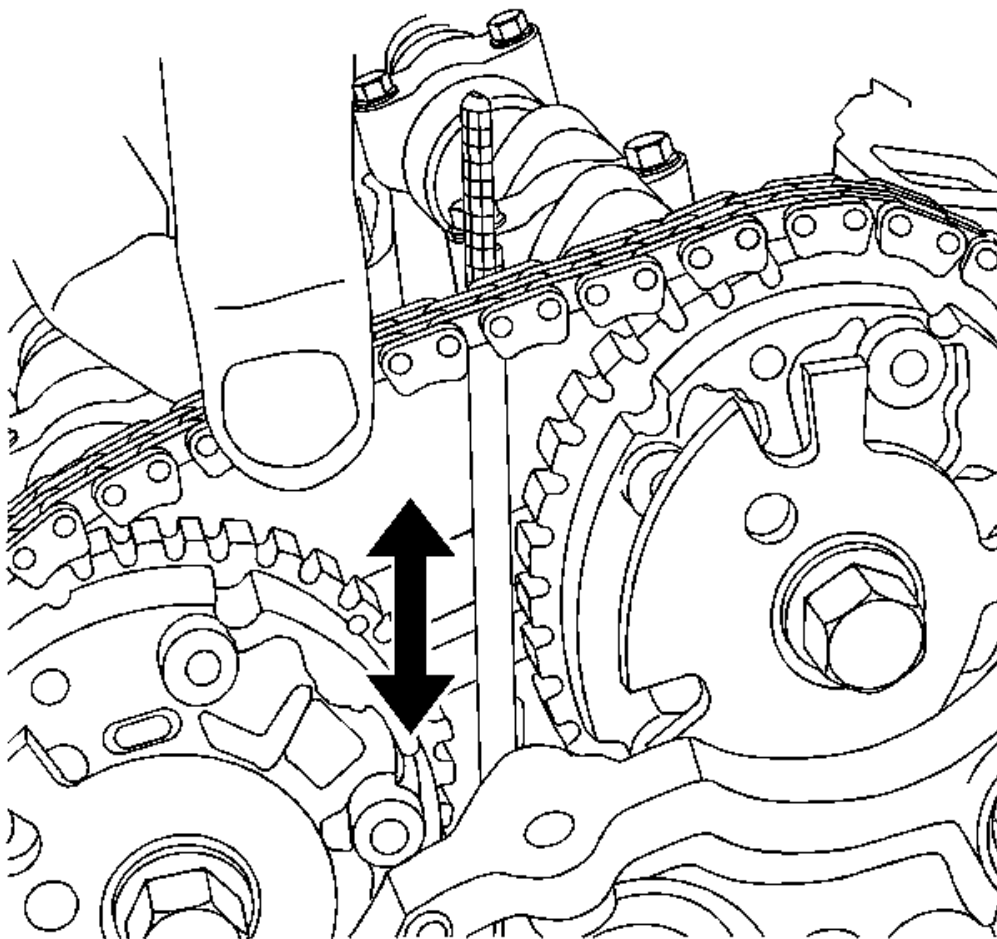
Fig. 101: Slack In Timing Drive Chain Courtesy of GENERAL MOTORS COMPANY
