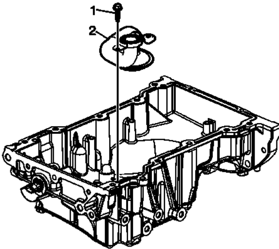
Fig. 204: Oil Suction Pipe Bolts
