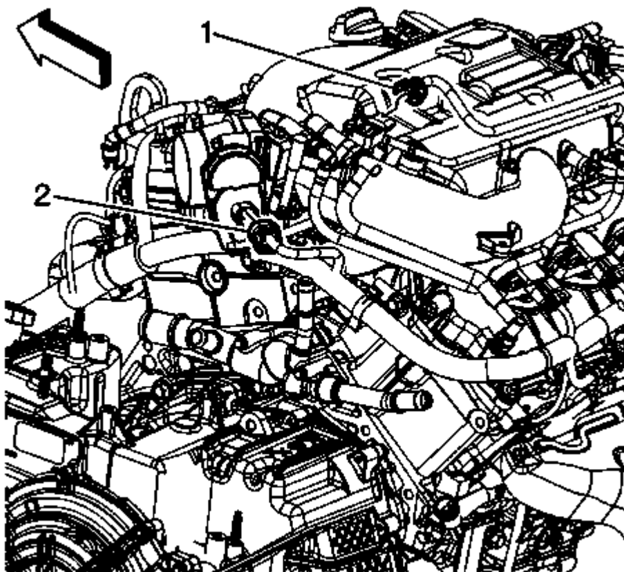
Fig. 230: Identifying MAP Sensor & ETC Electrical Connectors Courtesy of GENERAL MOTORS COMPANY
