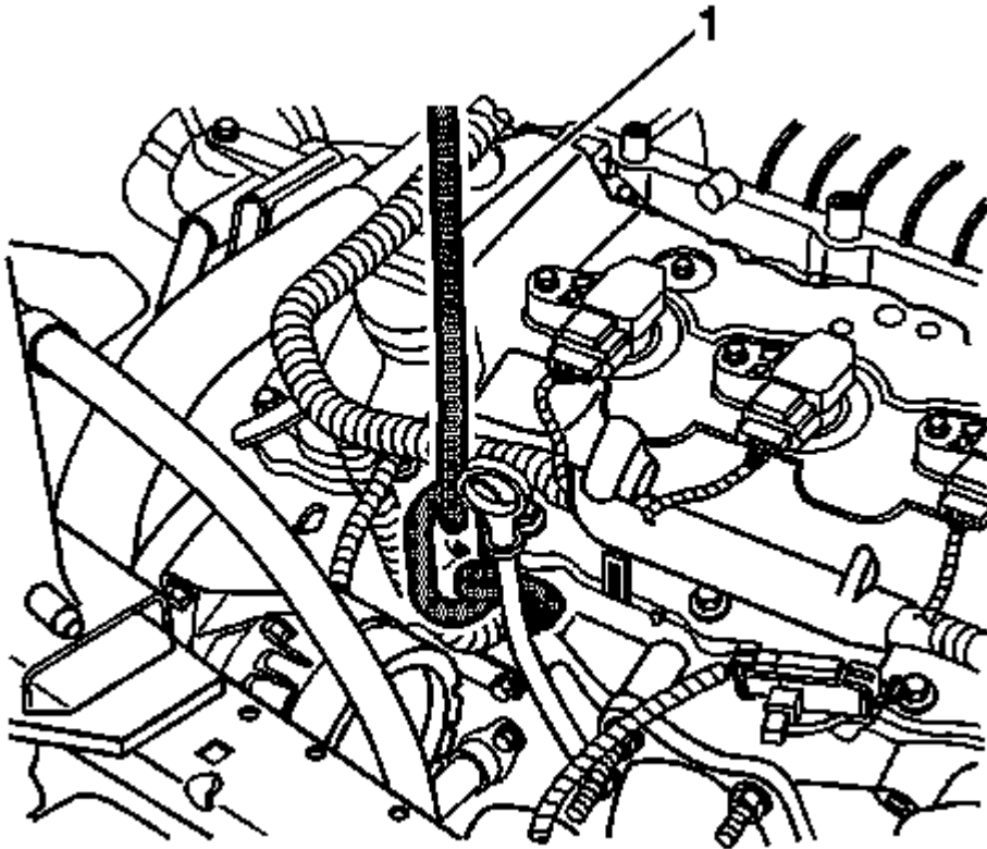
Fig. 5: View Of Engine Lift Bracket (Right Cylinder Head) Courtesy of GENERAL MOTORS COMPANY
