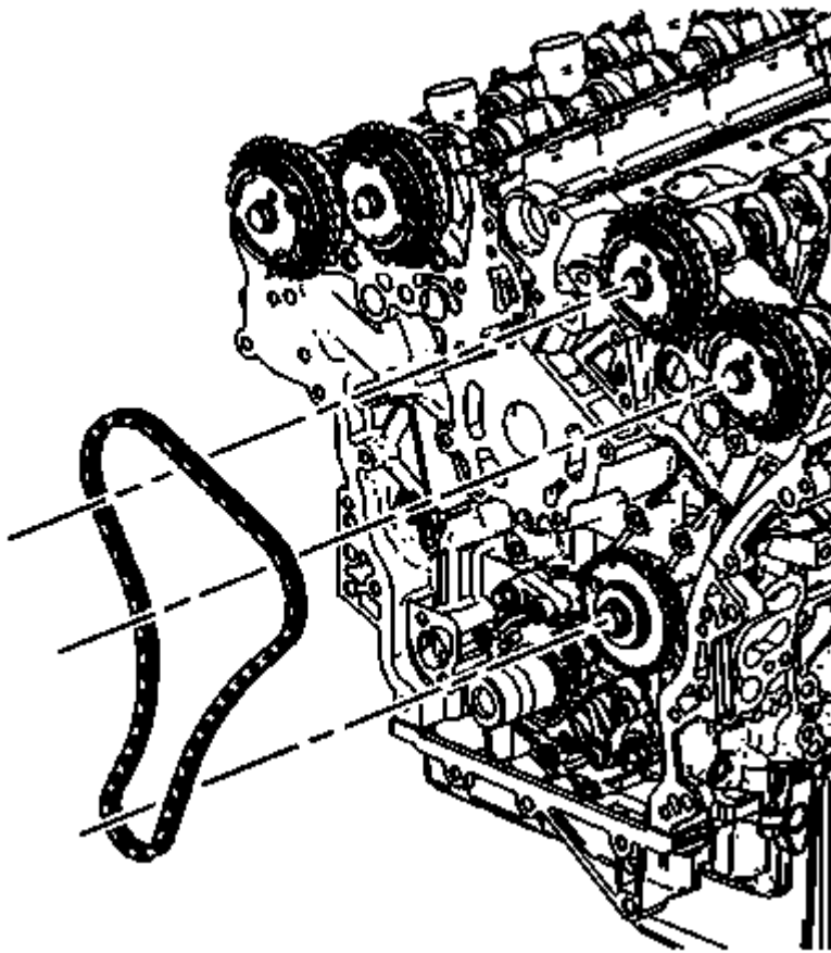
Fig. 59: View Of Left Bank Secondary Camshaft Drive Chain Courtesy of GENERAL MOTORS COMPANY
