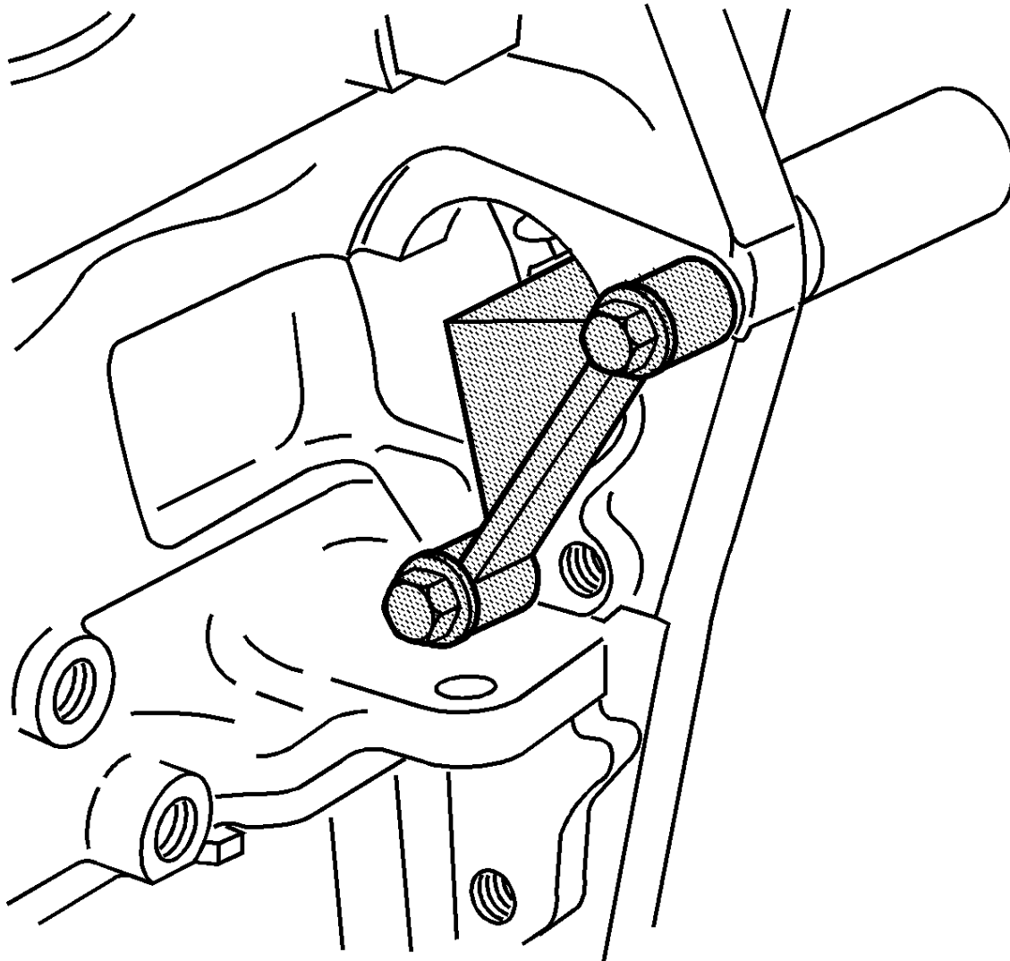
Fig. 154: Flywheel Holding Tool
