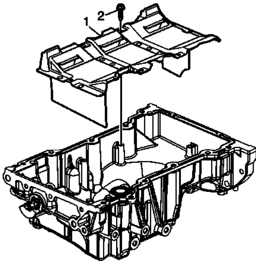
Fig. 197: Oil Pan Scraper
