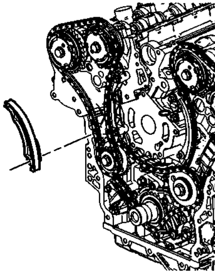
Fig. 70: View Of Right Secondary Camshaft Drive Chain Shoe Courtesy of GENERAL MOTORS COMPANY
