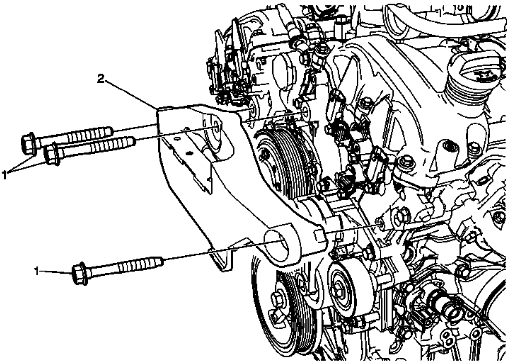
Fig. 10: Identifying Engine Mount Bracket - Right Side Courtesy of GENERAL MOTORS COMPANY
