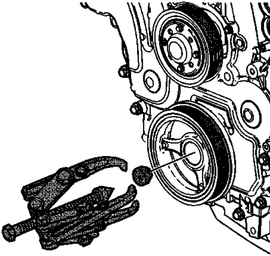
Fig. 33: Crankshaft Button & Remover Courtesy of GENERAL MOTORS COMPANY
