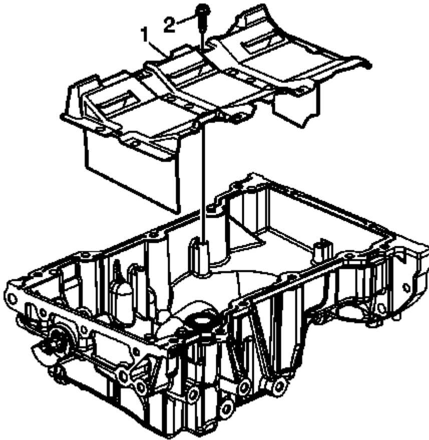
Fig. 205: Oil Pan Scraper
