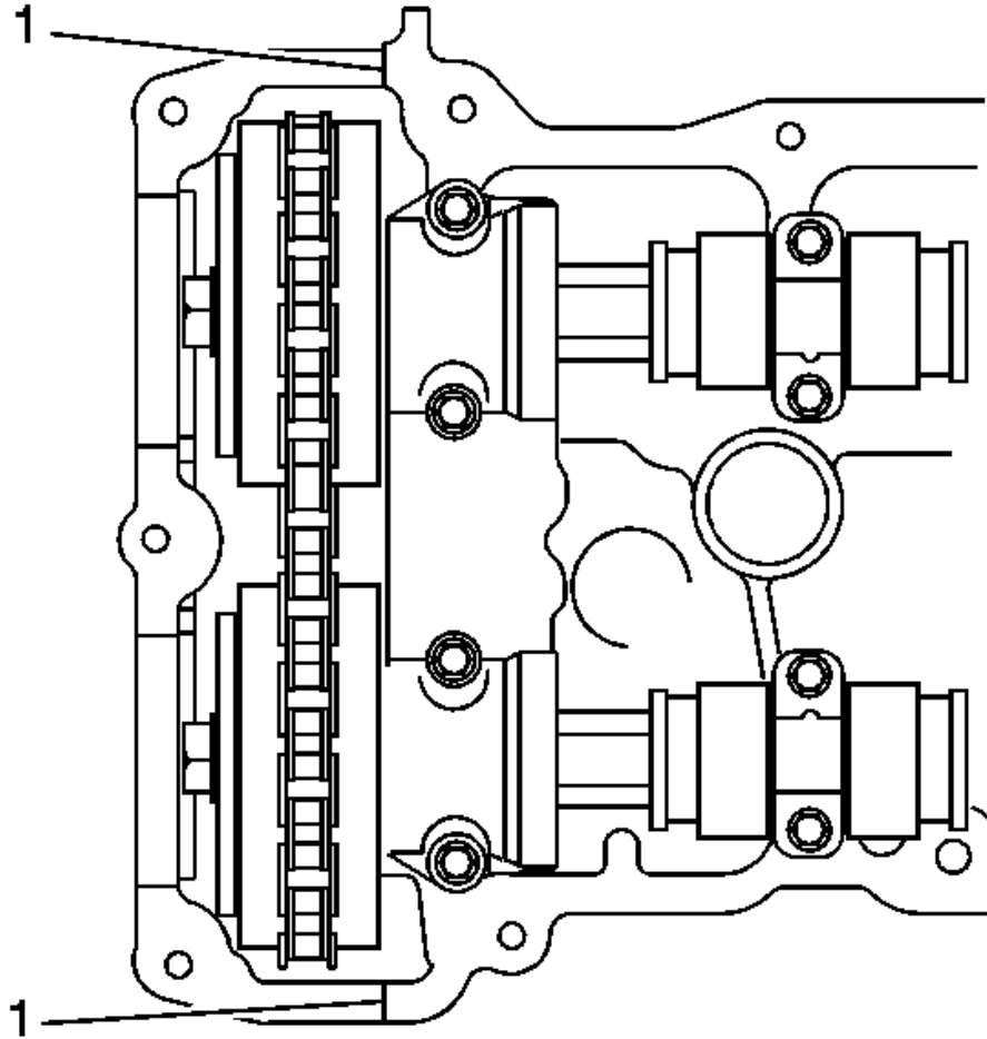
Fig. 52: Identifying Engine Front Cover Split Lines Courtesy of GENERAL MOTORS COMPANY
