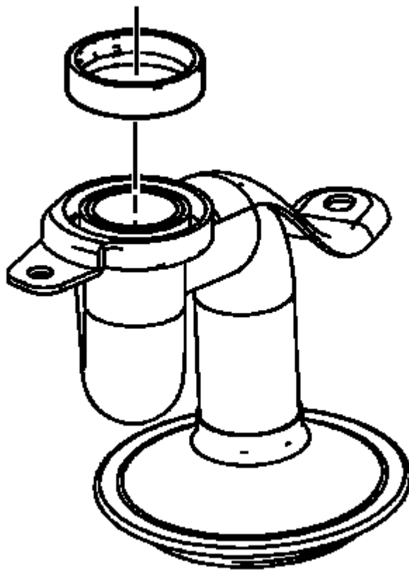
Fig. 209: View Of Oil Suction Tube Seal & Oil Suction Tube Courtesy of GENERAL MOTORS COMPANY
