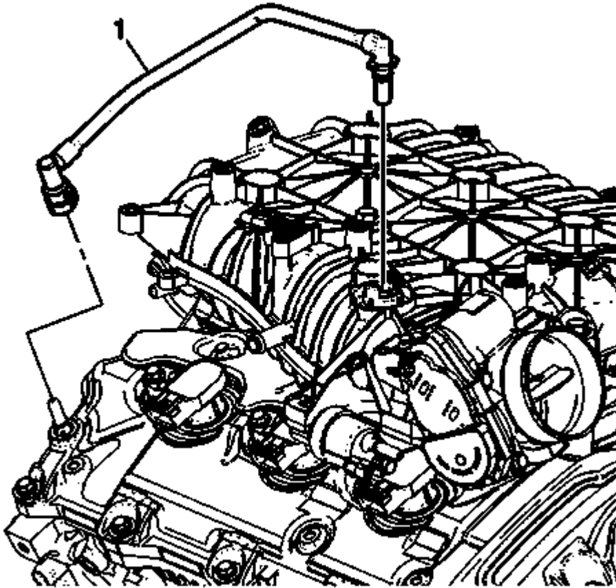
Fig. 25: View Of Positive Crankcase Ventilation Tube Courtesy of GENERAL MOTORS COMPANY
