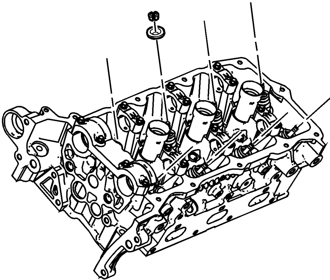
Fig. 165: View Of Valve Spring Keepers Courtesy of GENERAL MOTORS COMPANY
