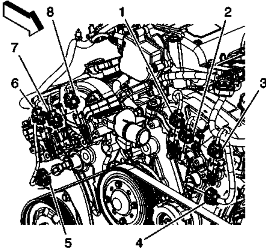
Fig. 213: Identifying Camshaft Position Sensors Courtesy of GENERAL MOTORS COMPANY
