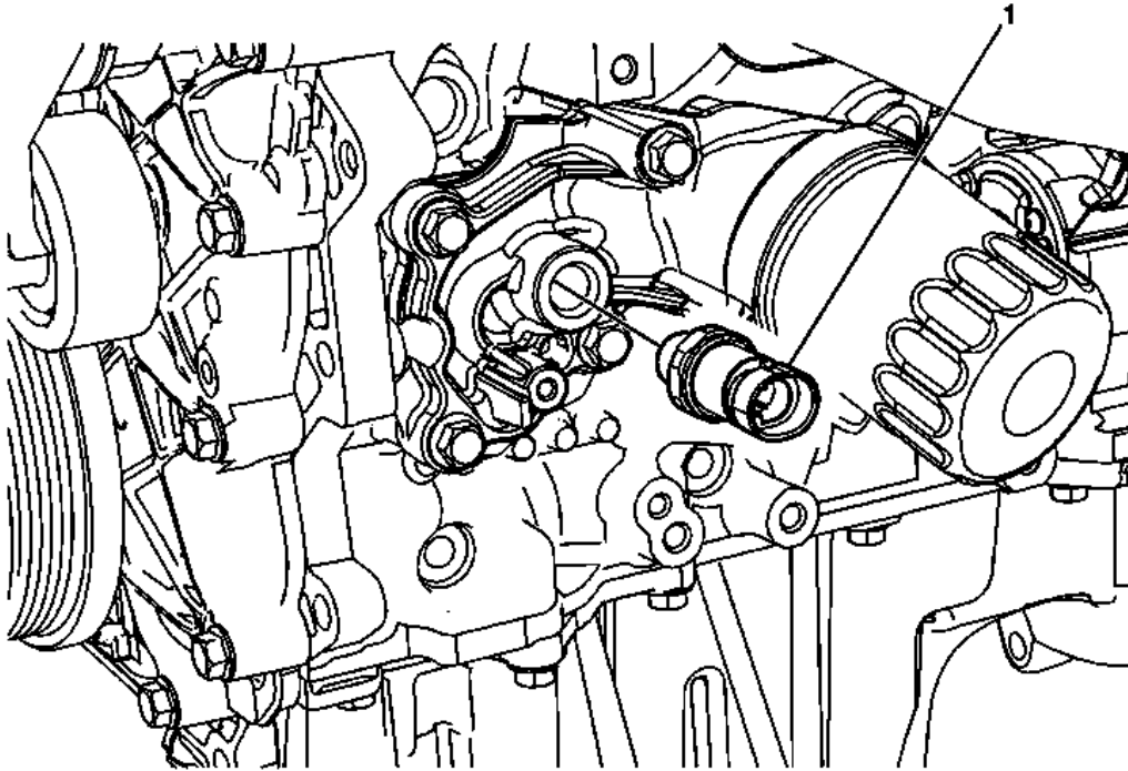
Fig. 195: Identifying Engine Oil Pressure Sensor And/Or Switch (LF1, LFW or LFX)
