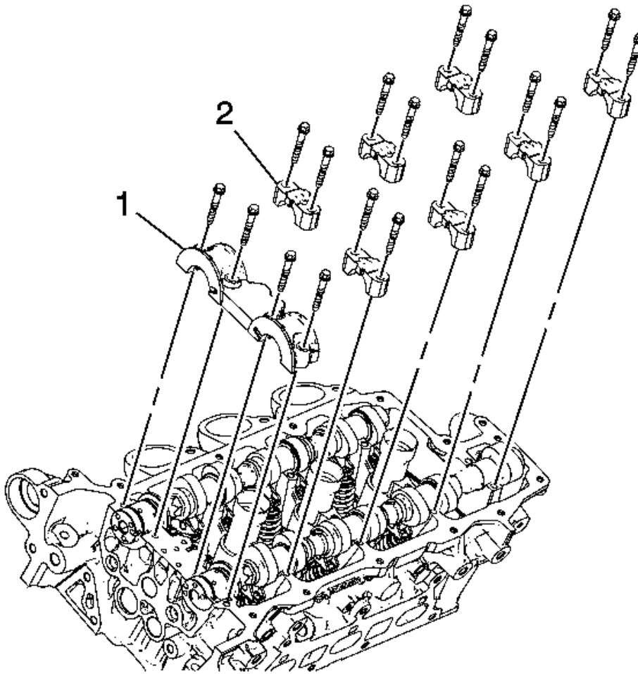
Fig. 133: Camshaft Bearing Caps And Bolts Courtesy of GENERAL MOTORS COMPANY
