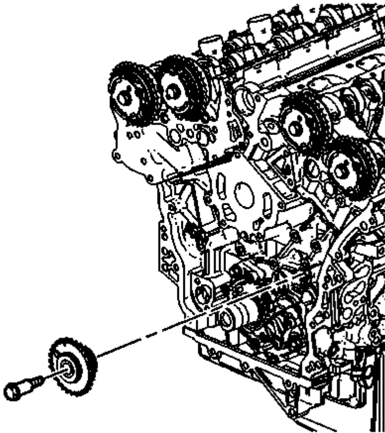
Fig. 77: View Of Left Camshaft Intermediate Drive Chain Idler Sprocket Courtesy of GENERAL MOTORS COMPANY
