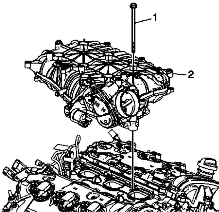
Fig. 18: View Of Intake Manifold Assembly Courtesy of GENERAL MOTORS COMPANY
