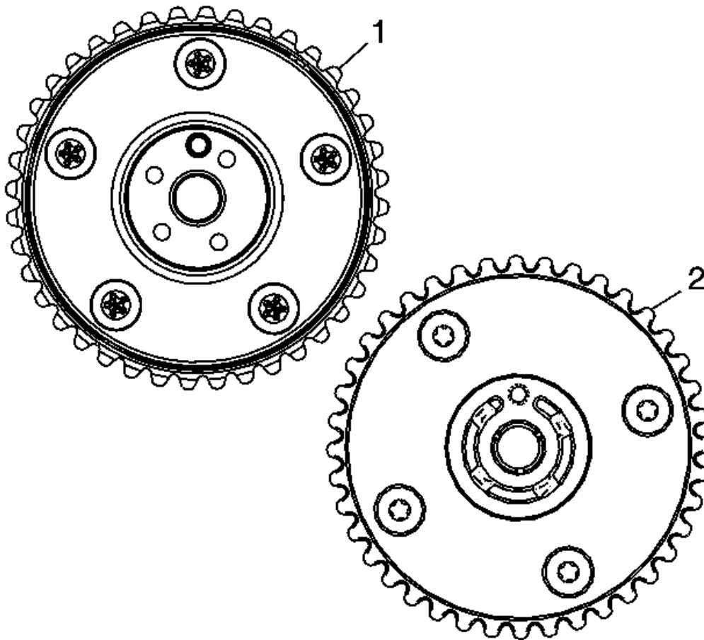
Fig. 122: Identifying Camshaft Position Actuators
