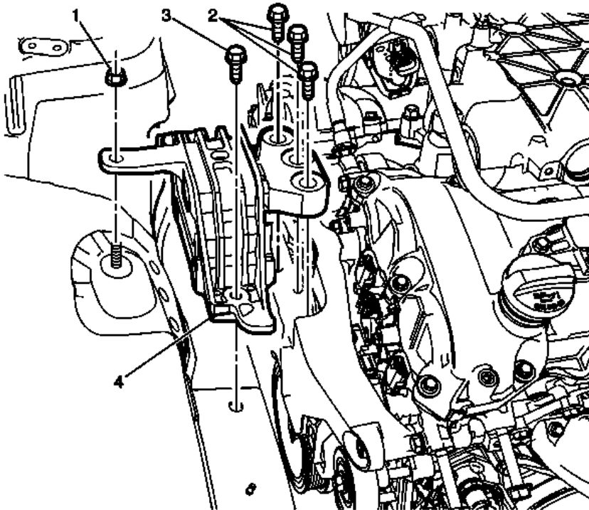
Fig. 9: View Of Engine Mount - Right Side
