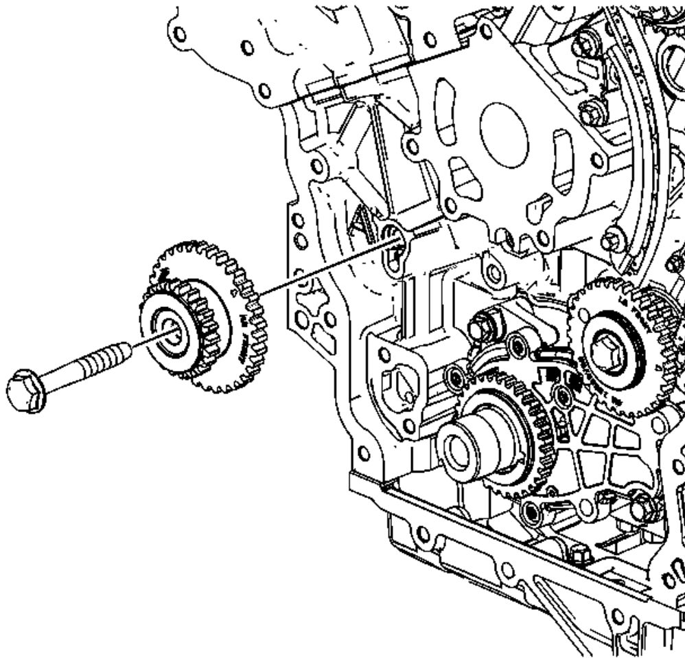
Fig. 78: Identifying Camshaft Intermediate Drive Chain Idler & Bolt Courtesy of GENERAL MOTORS COMPANY
