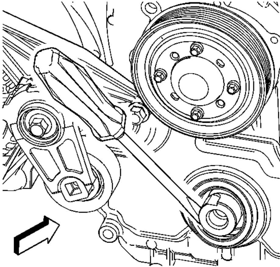
Fig. 39: Removing Crankshaft Front Oil Seal Courtesy of GENERAL MOTORS COMPANY
