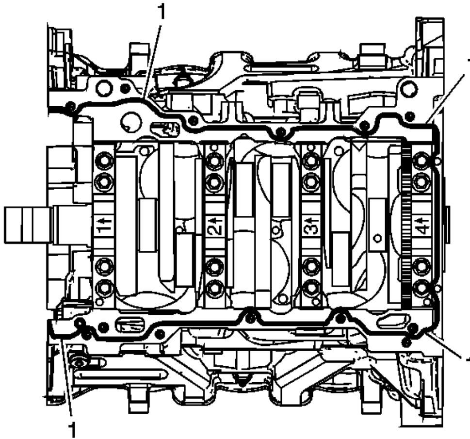
Fig. 190: Identifying Sealant Application Locations On Block Pan Rail & Crankshaft Rear Oil Seal Housing
