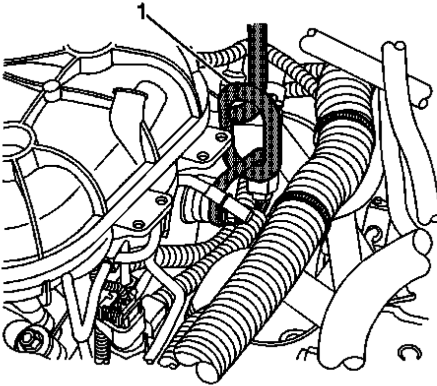
Fig. 6: Identifying Engine Lift Bracket (Left Cylinder Head) Courtesy of GENERAL MOTORS COMPANY
