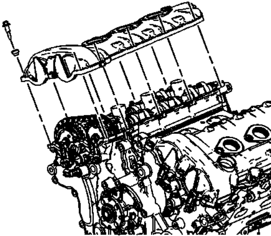
Fig. 49: Identifying Right Camshaft Cover & Bolts Courtesy of GENERAL MOTORS COMPANY
