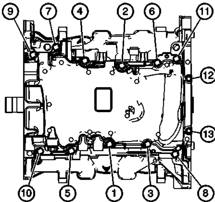
Fig. 194: Identifying Oil Pan Bolts - Tightening Sequence Courtesy of GENERAL MOTORS COMPANY
