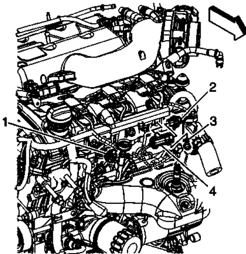
Fig. 226: Identifying ECT & HO2S Wiring Harness Connectors Courtesy of GENERAL MOTORS COMPANY
