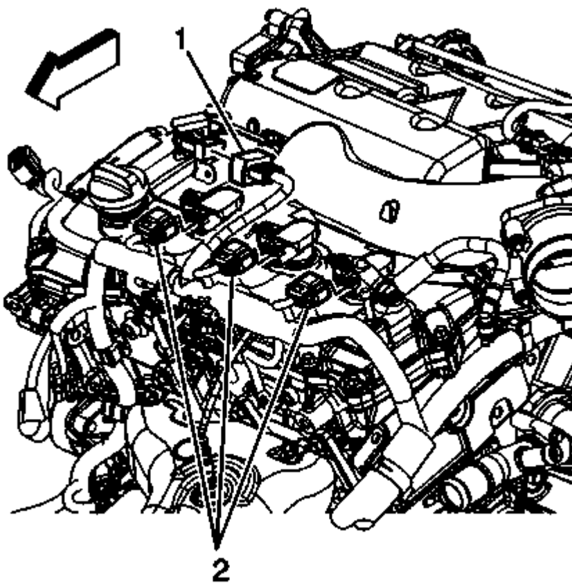
Fig. 216: Identifying Ignition Coils & Fuel Injector Wiring Harness Connector Courtesy of GENERAL MOTORS COMPANY
