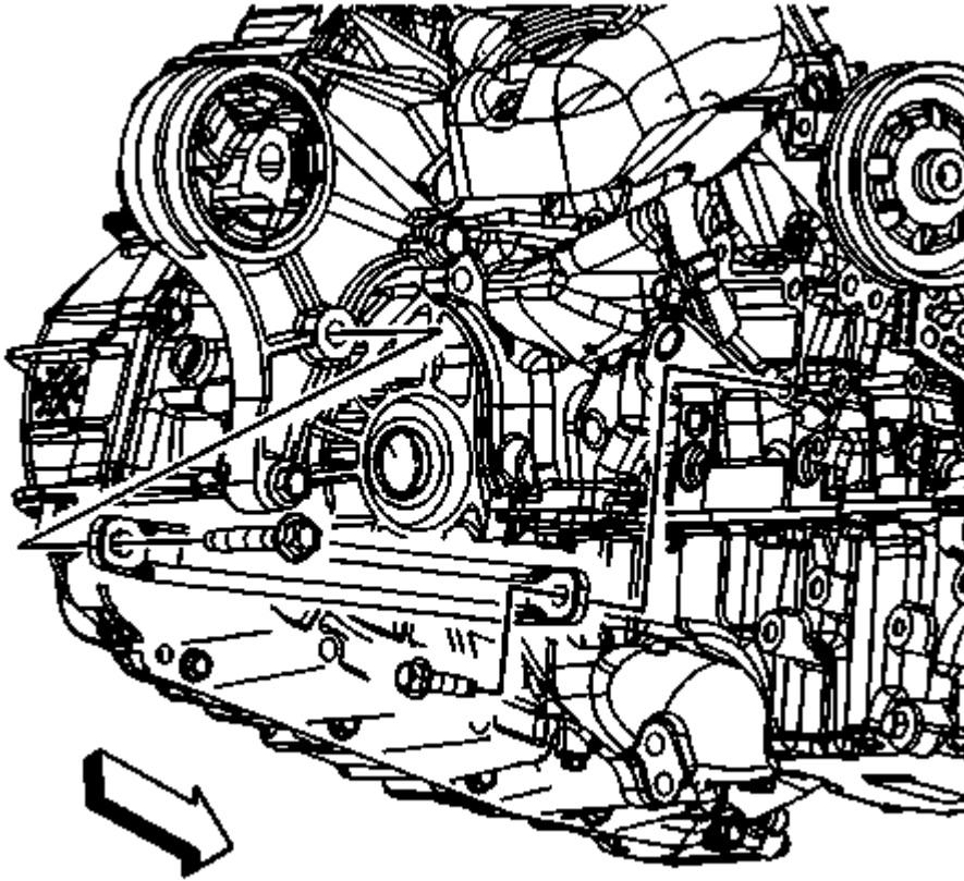
Fig. 223: Identifying Oil Pan Brace Bolt & Brace Courtesy of GENERAL MOTORS COMPANY
