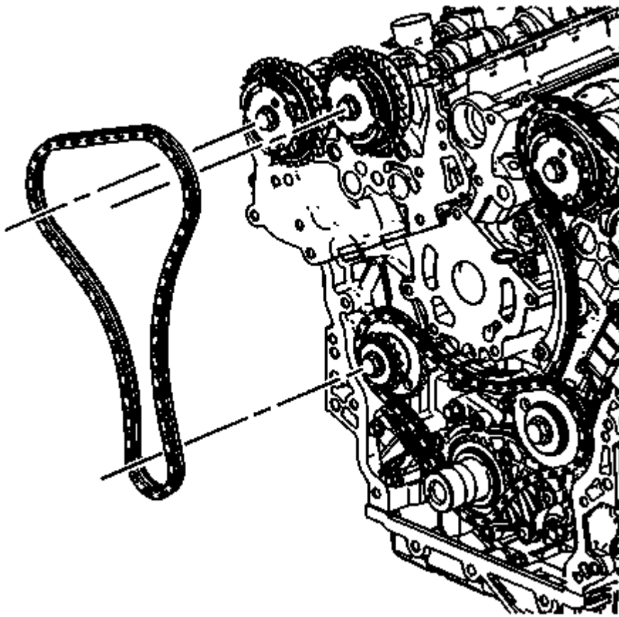
Fig. 62: View Of Right Bank Secondary Camshaft Drive Chain Courtesy of GENERAL MOTORS COMPANY
