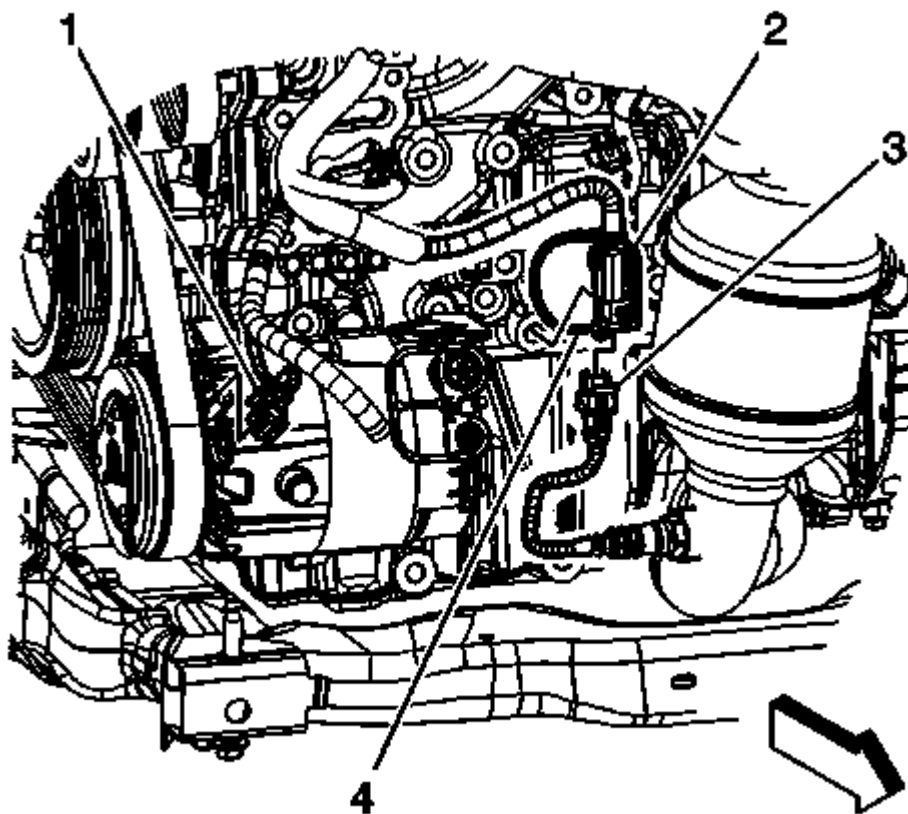
Fig. 227: Electrical Connectors - Left Side Courtesy of GENERAL MOTORS COMPANY
