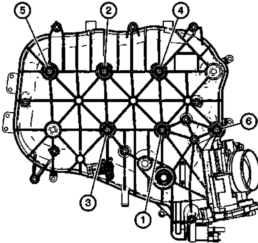
Fig. 22: Identifying Intake Manifold Bolt Tightening Sequence Courtesy of GENERAL MOTORS COMPANY
