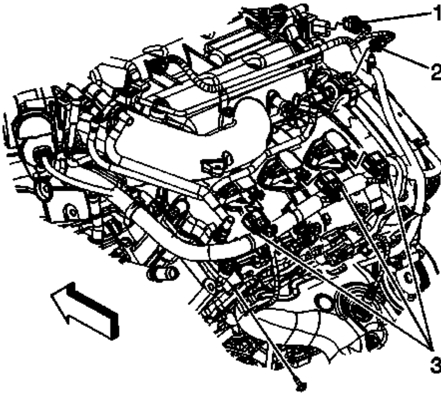
Fig. 215: Identifying EVAP Canister Purge Solenoid, Ignition Coils & Intake Manifold Tuning Valve
