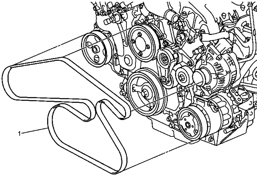
Fig. 1: Identifying Drive Belt Routing Courtesy of GENERAL MOTORS COMPANY
