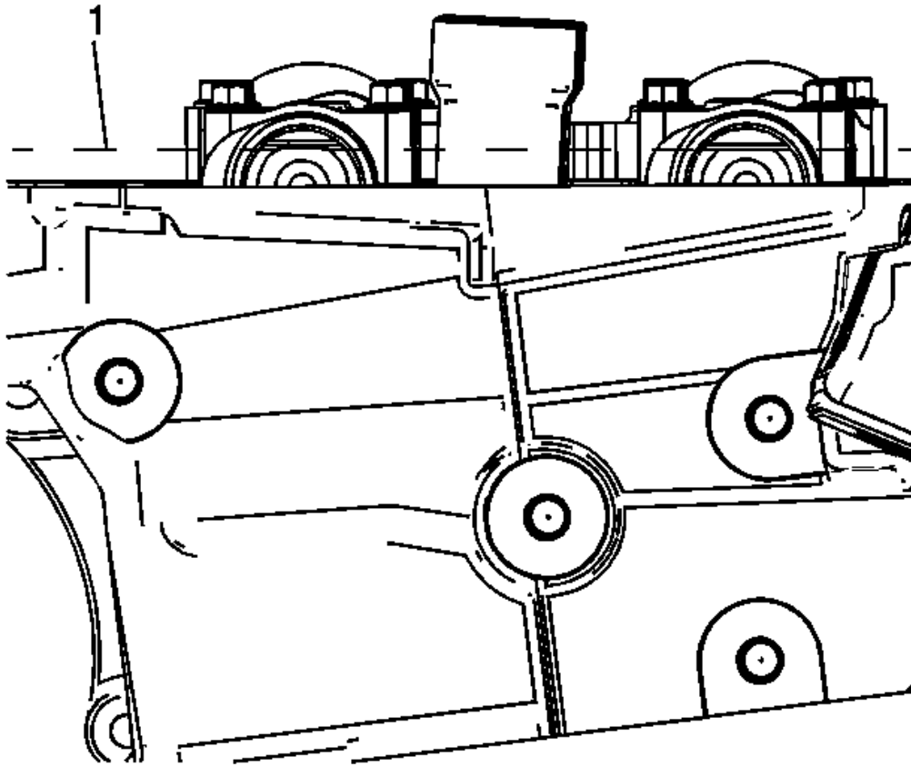
Fig. 130: View Of Camshaft Flats Parallel With Camshaft Cover Rail Courtesy of GENERAL MOTORS COMPANY
