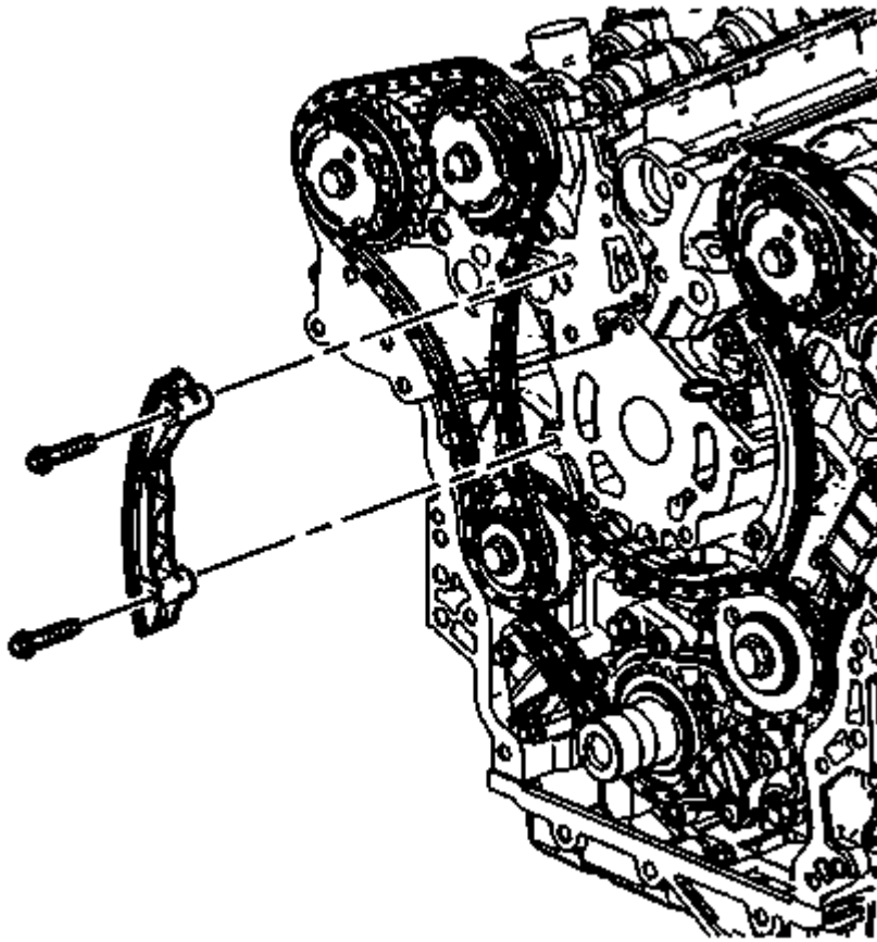
Fig. 73: View Of Right Secondary Camshaft Drive Chain Guide & Bolts Courtesy of GENERAL MOTORS COMPANY
