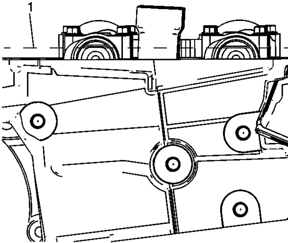
Fig. 114: View Of Camshaft Flats Parallel With Camshaft Cover Rail Courtesy of GENERAL MOTORS COMPANY
