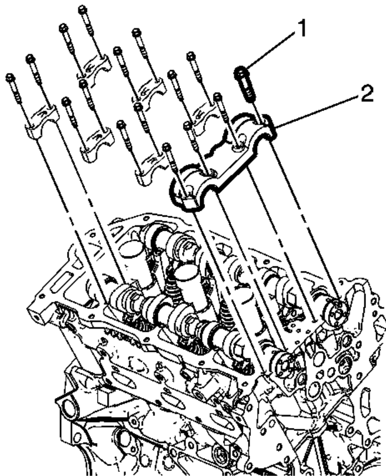
Fig. 136: Camshaft Bearing Caps And Bolts Courtesy of GENERAL MOTORS COMPANY
