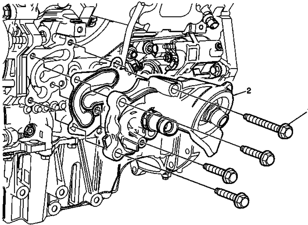
Fig. 30: Oil Filter Adapter & Fasteners Courtesy of GENERAL MOTORS COMPANY
