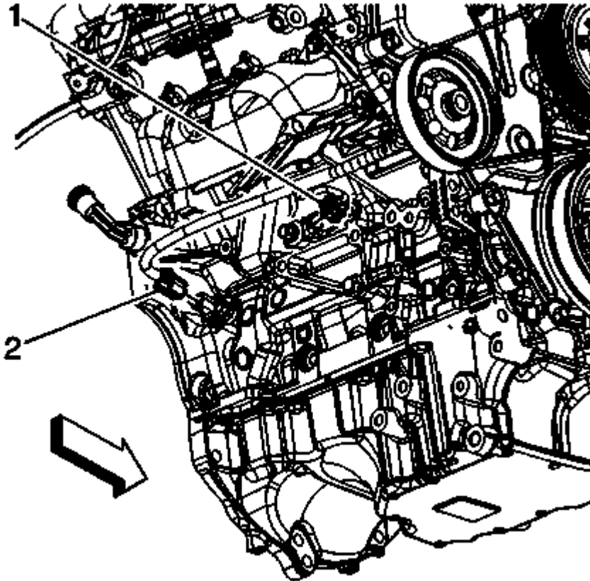
Fig. 212: Identifying CKP Sensor & Knock Sensor Courtesy of GENERAL MOTORS COMPANY
