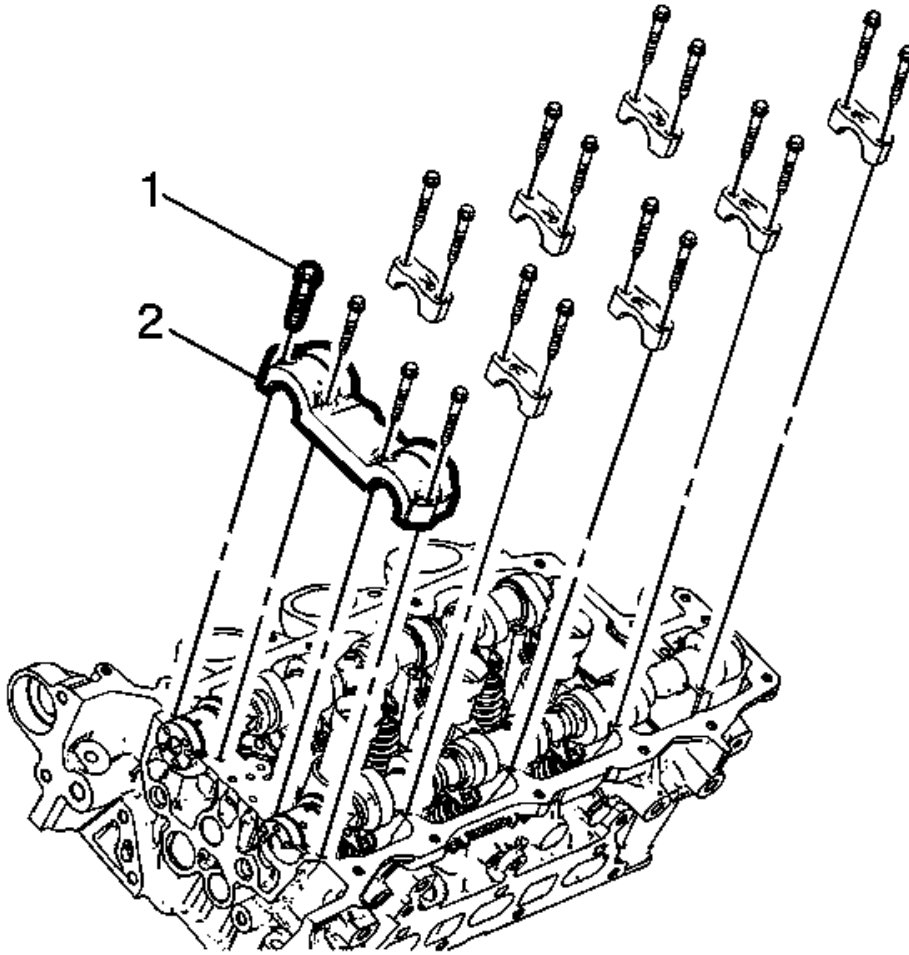
Fig. 125: Bearing Cap Bolts
