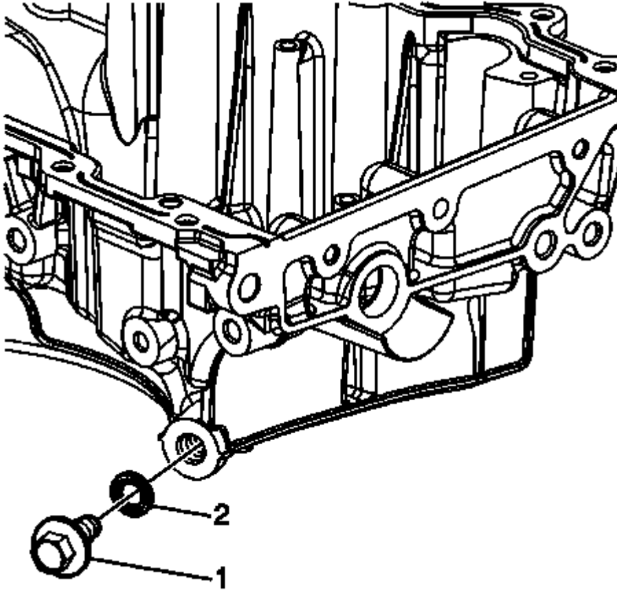
Fig. 196: Oil Pan Drain Plug And Seal Courtesy of GENERAL MOTORS COMPANY
