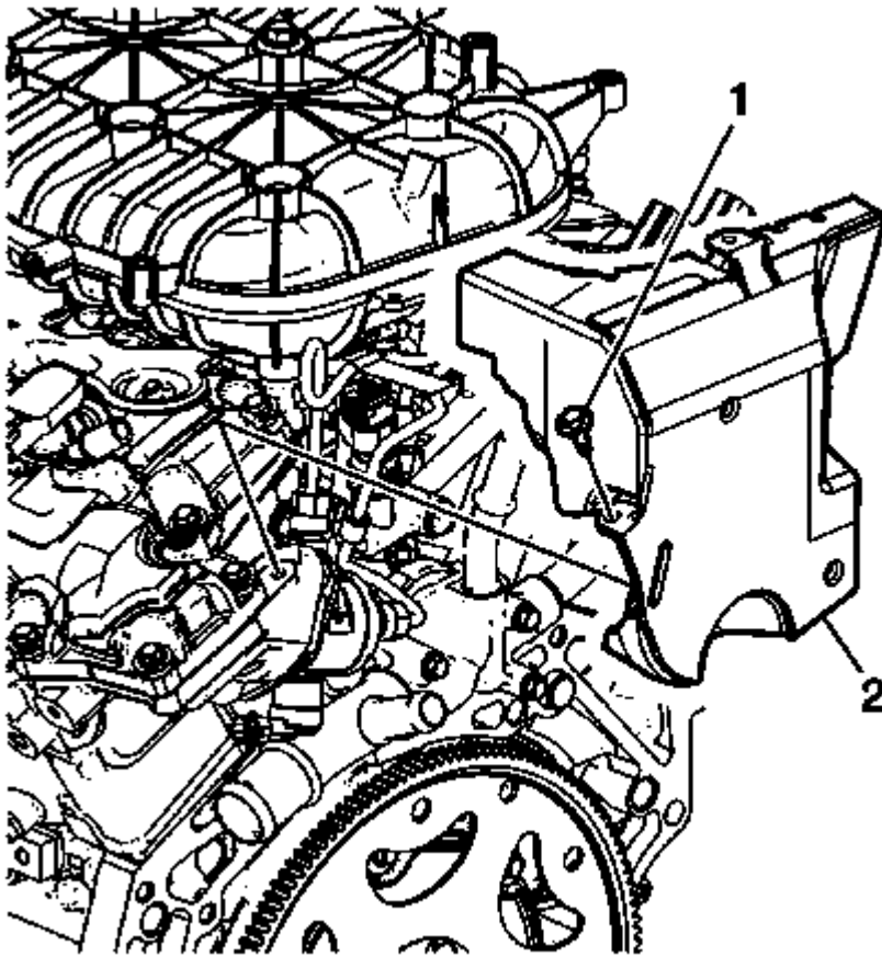
Fig. 17: View Of Fuel Pump Cover & Bolt Courtesy of GENERAL MOTORS COMPANY
