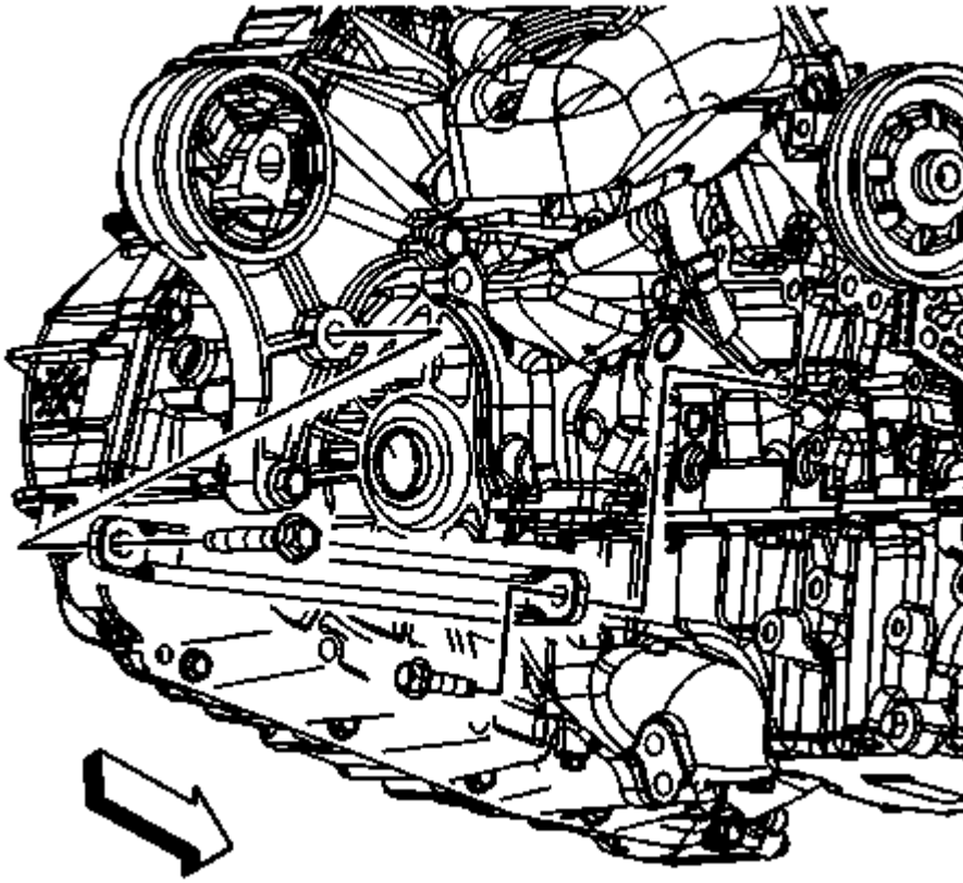
Fig. 220: Identifying Oil Pan Brace Bolt & Brace Courtesy of GENERAL MOTORS COMPANY
