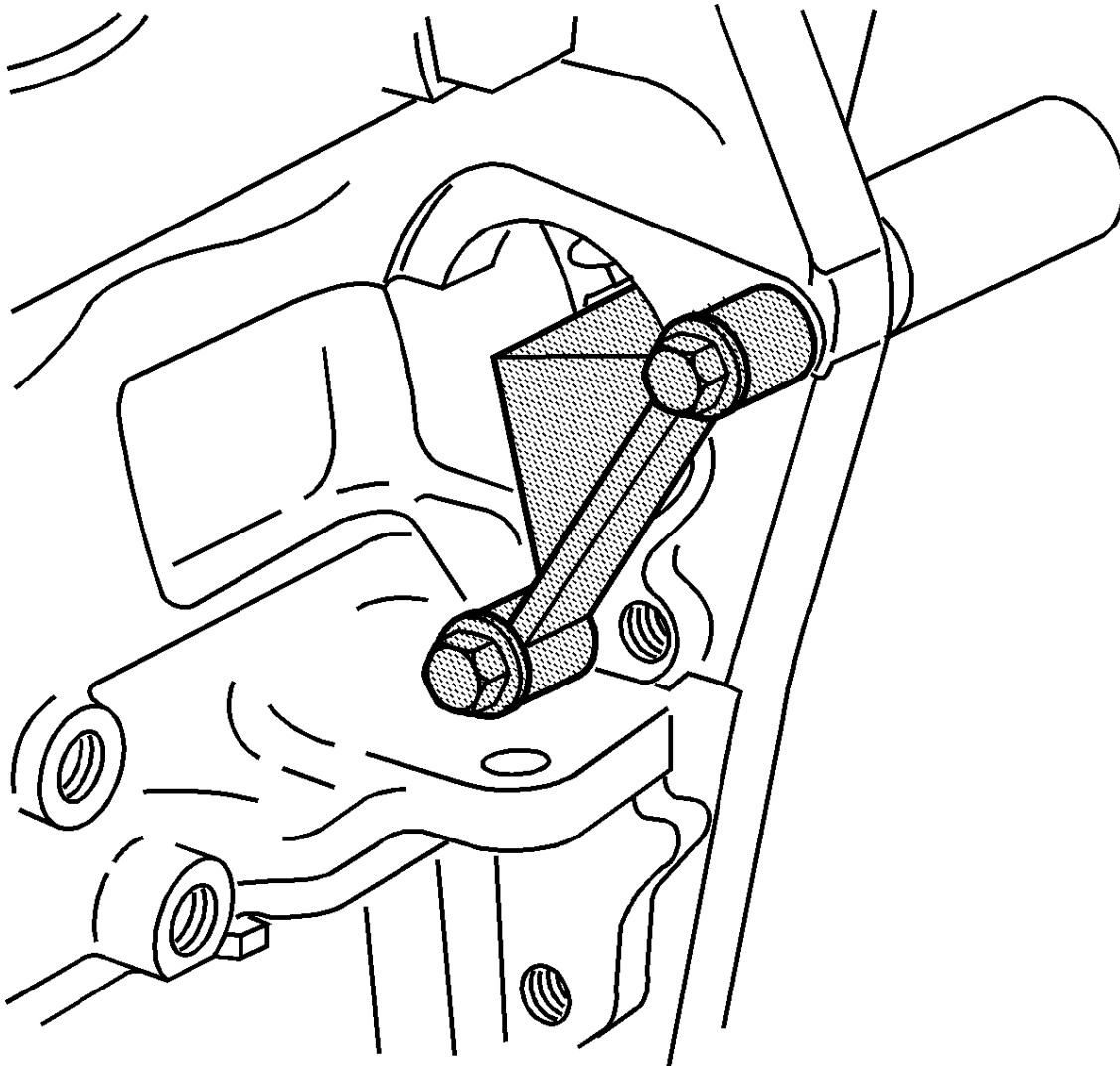
Fig. 163: Flywheel Holding Tool Courtesy of GENERAL MOTORS COMPANY
