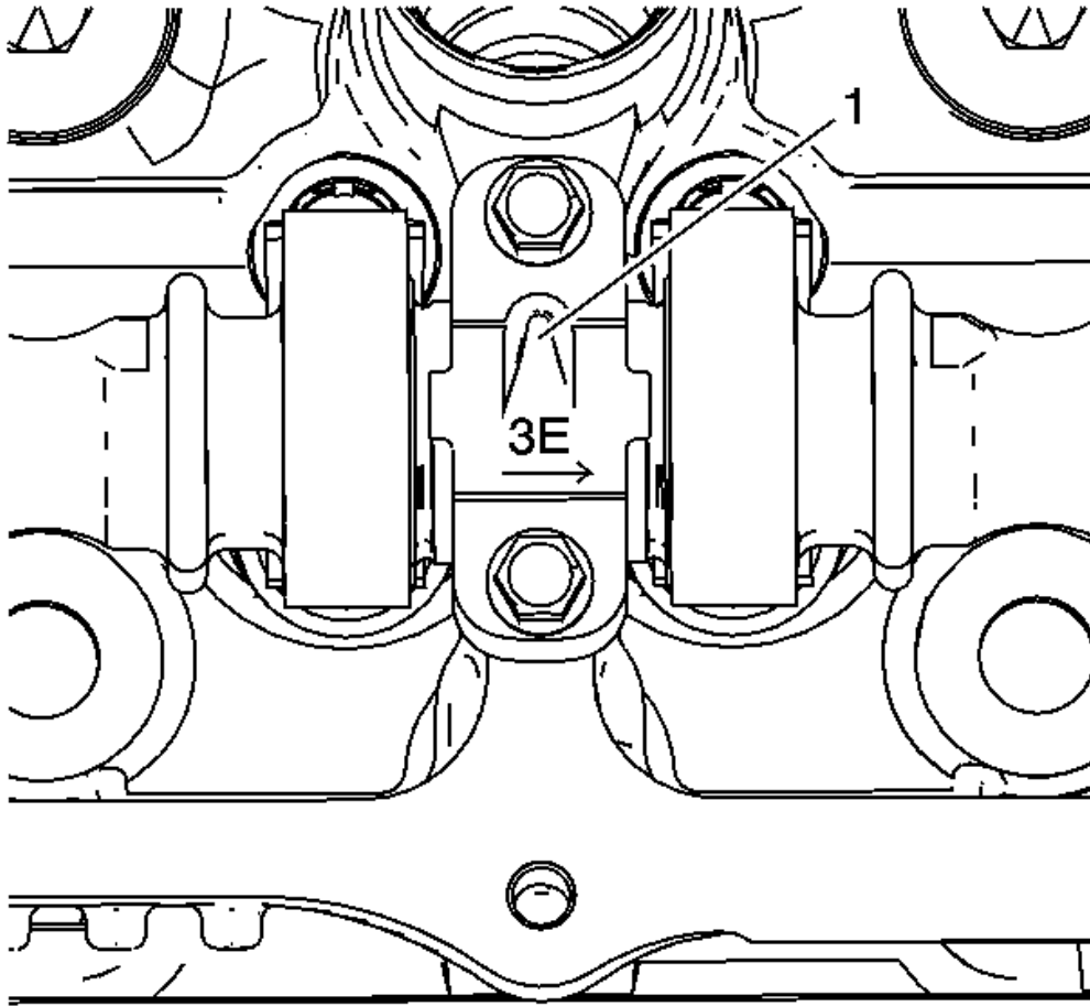
Fig. 142: Right Cylinder Head Camshaft Bearing Cap Markings Courtesy of GENERAL MOTORS COMPANY
