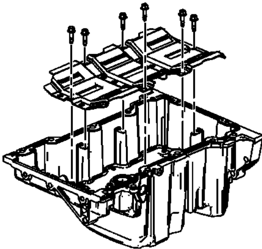
Fig. 206: View Of Oil Pan Scraper And Bolts Courtesy of GENERAL MOTORS COMPANY
