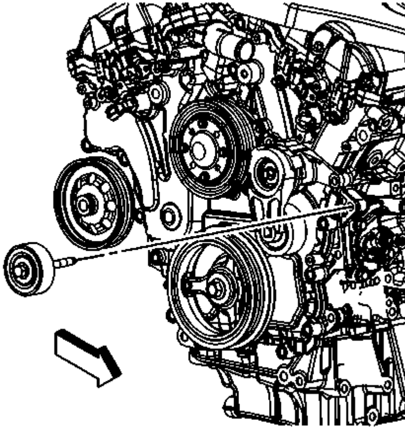
Fig. 3: Identifying Drive Belt Idler Pulley Courtesy of GENERAL MOTORS COMPANY
