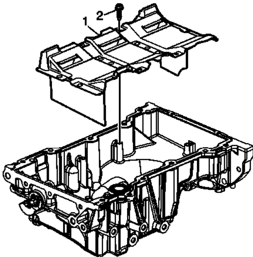
Fig. 197: Oil Pan Scraper
