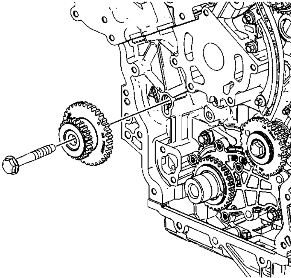
Fig. 79: Right Camshaft Intermediate Drive Chain Idler And Bolt Courtesy of GENERAL MOTORS COMPANY
