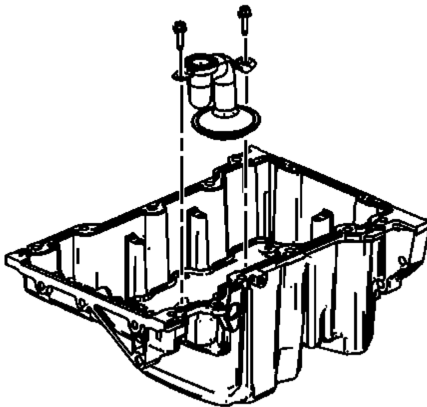
Fig. 207: Oil Suction Pipe
