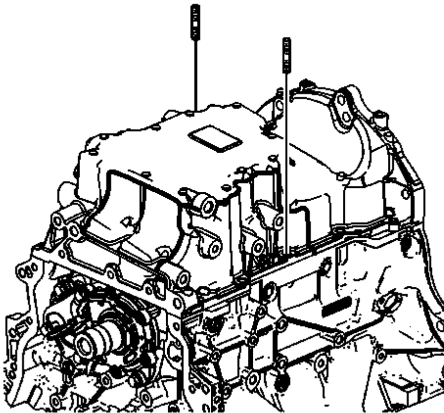
Fig. 192: Engine Block Guide Pins Courtesy of GENERAL MOTORS COMPANY
