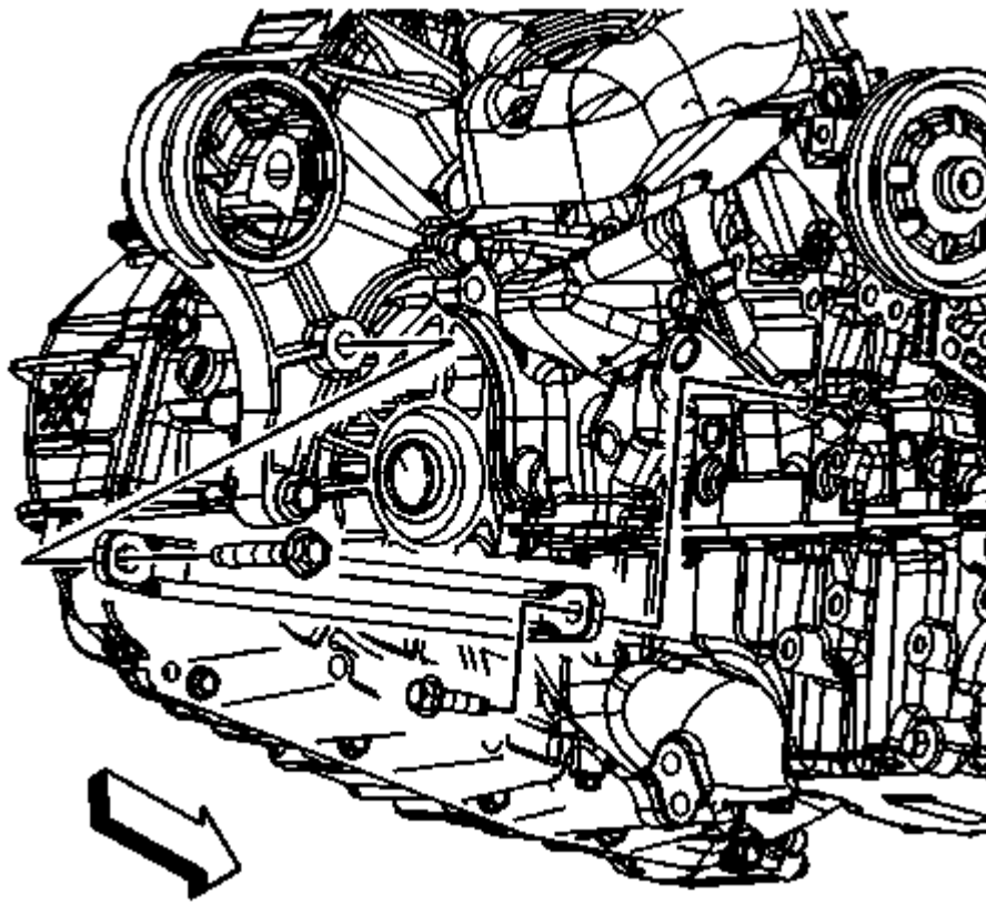
Fig. 220: Oil Pan Brace Bolt And Brace Courtesy of GENERAL MOTORS COMPANY
