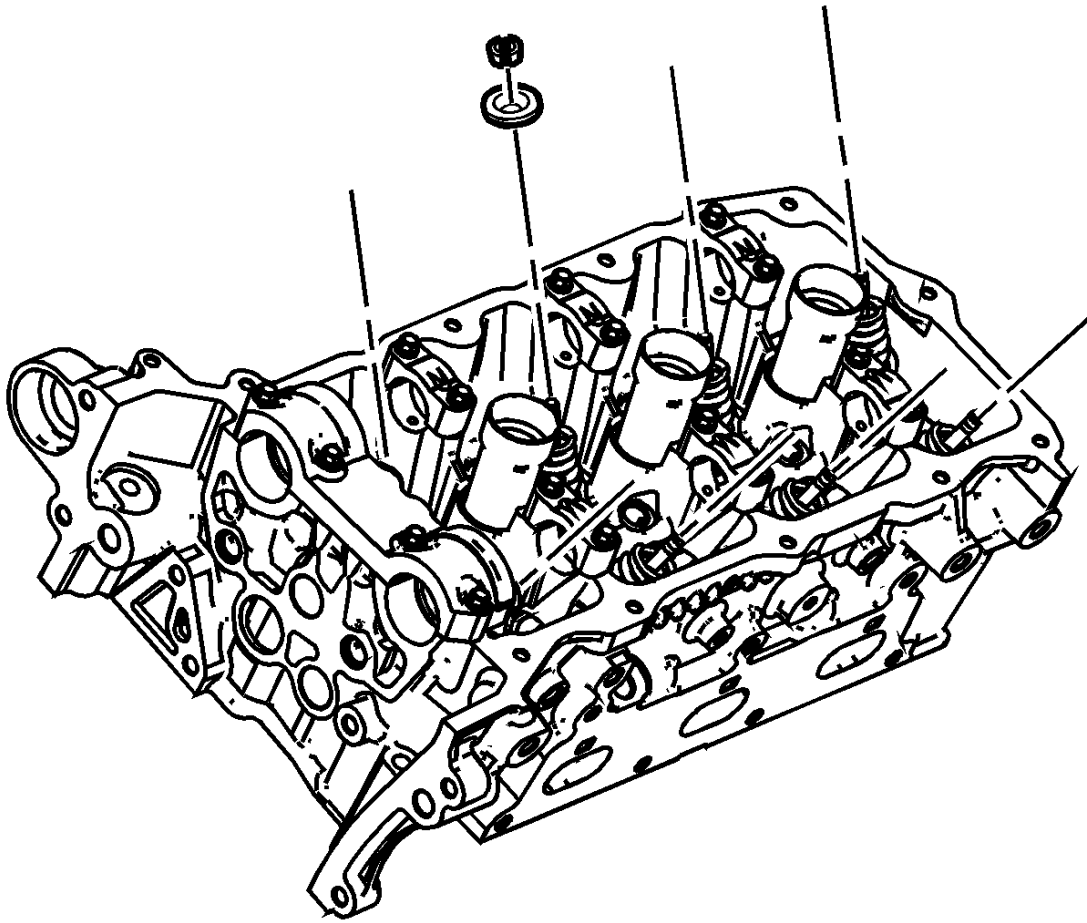
Fig. 162: Valve Spring Keepers And Valve Spring Retainers Courtesy of GENERAL MOTORS COMPANY
