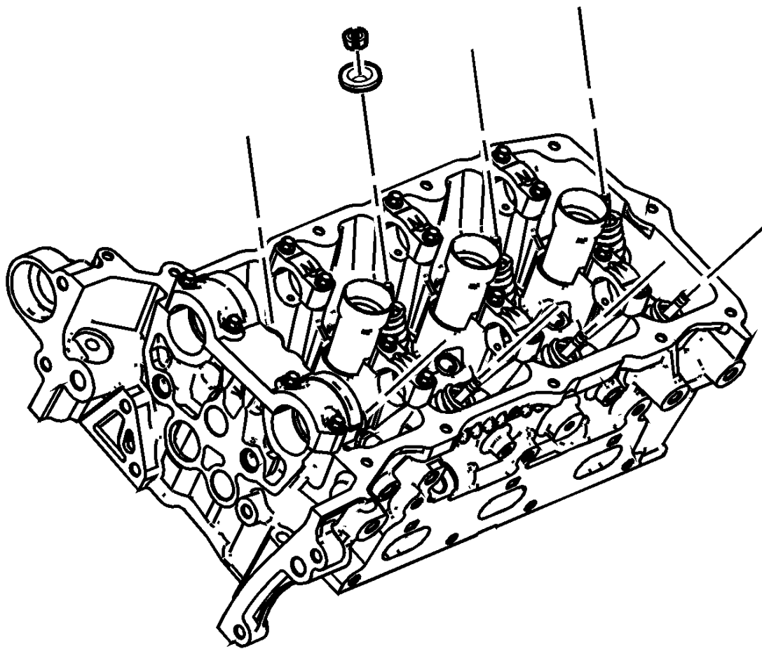
Fig. 165: Valve Spring Keepers And Valve Spring Retainers Courtesy of GENERAL MOTORS COMPANY
