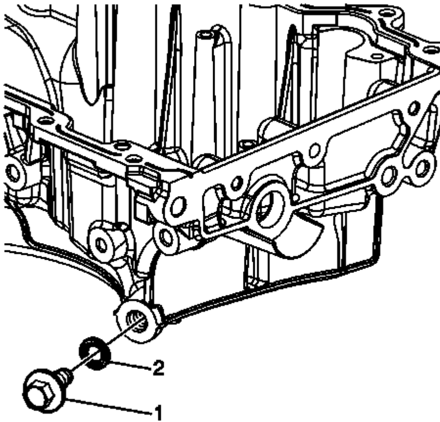
Fig. 201: Oil Pan Drain Plug And Seal
