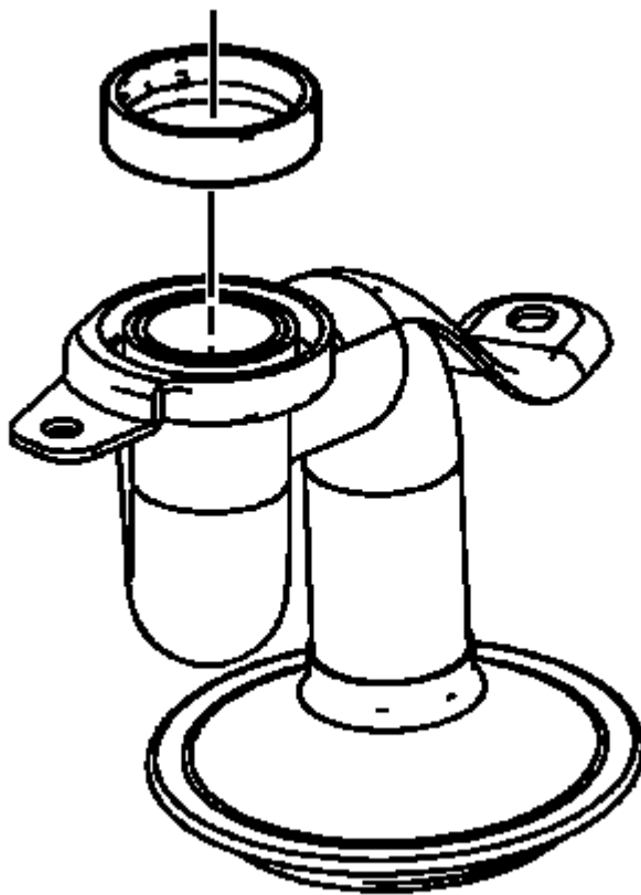
Fig. 208: Oil Suction Tube And Seal Courtesy of GENERAL MOTORS COMPANY
