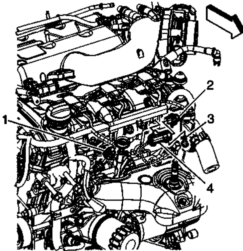
Fig. 218: ECT And HO2S Wiring Harness Connectors Courtesy of GENERAL MOTORS COMPANY
