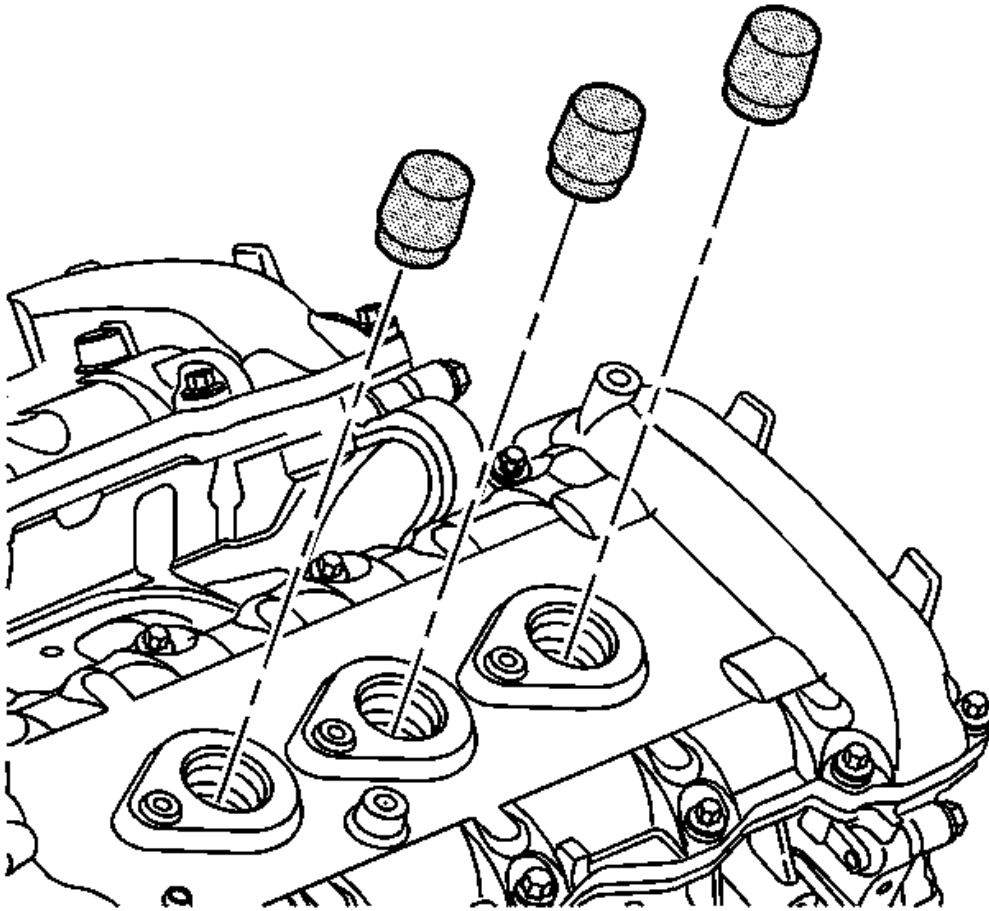
Fig. 56: Spark Plug Tube Plugs
