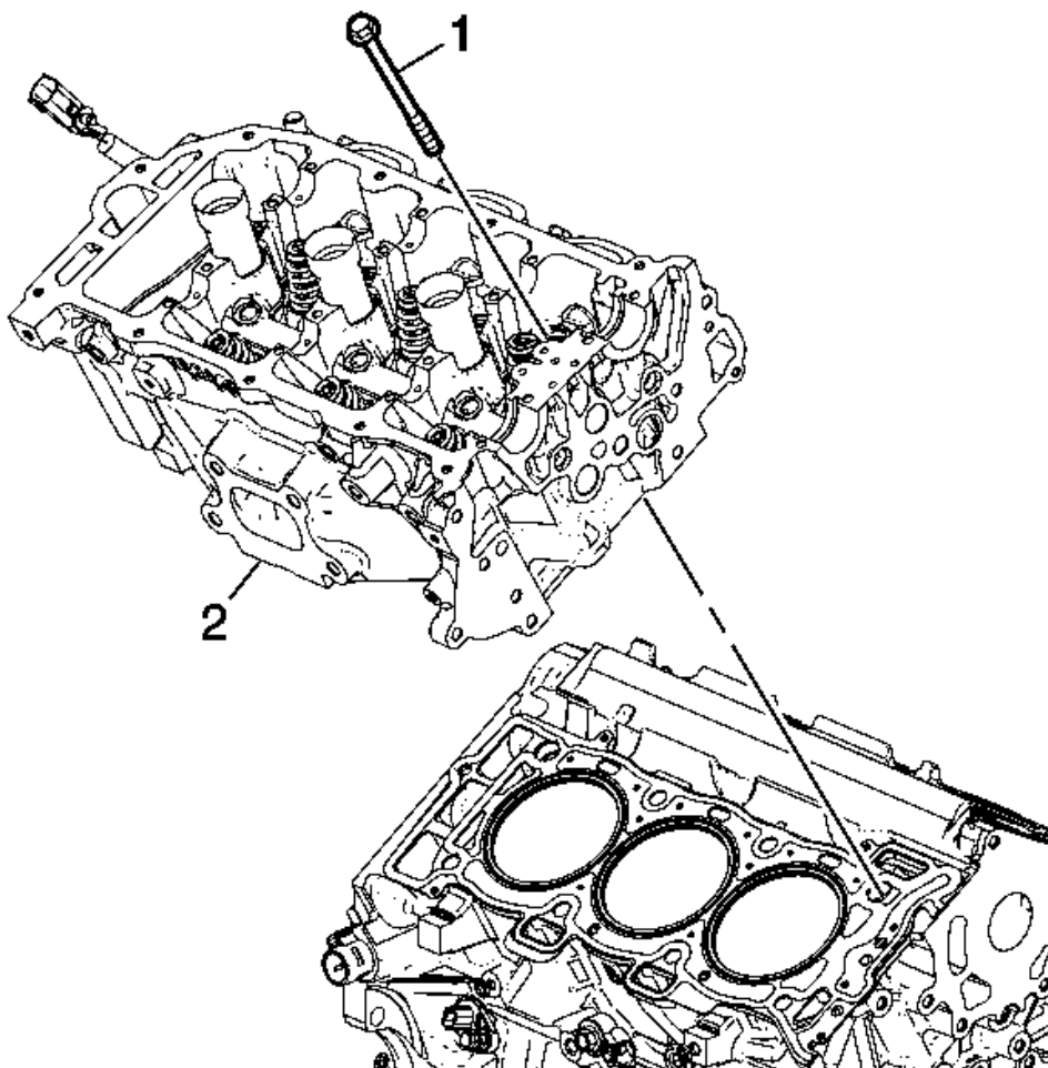
Fig. 177: Right Cylinder Head And Bolts Courtesy of GENERAL MOTORS COMPANY
