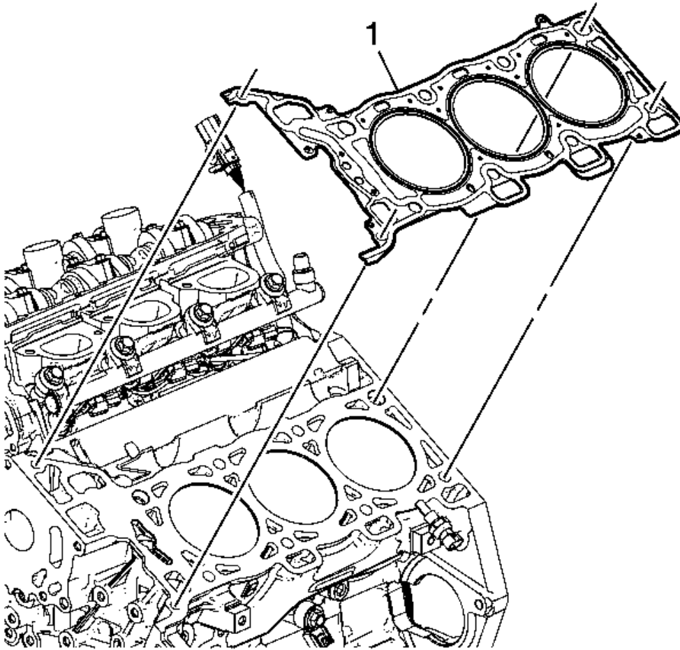
Fig. 174: Left Cylinder Head Gasket Courtesy of GENERAL MOTORS COMPANY
