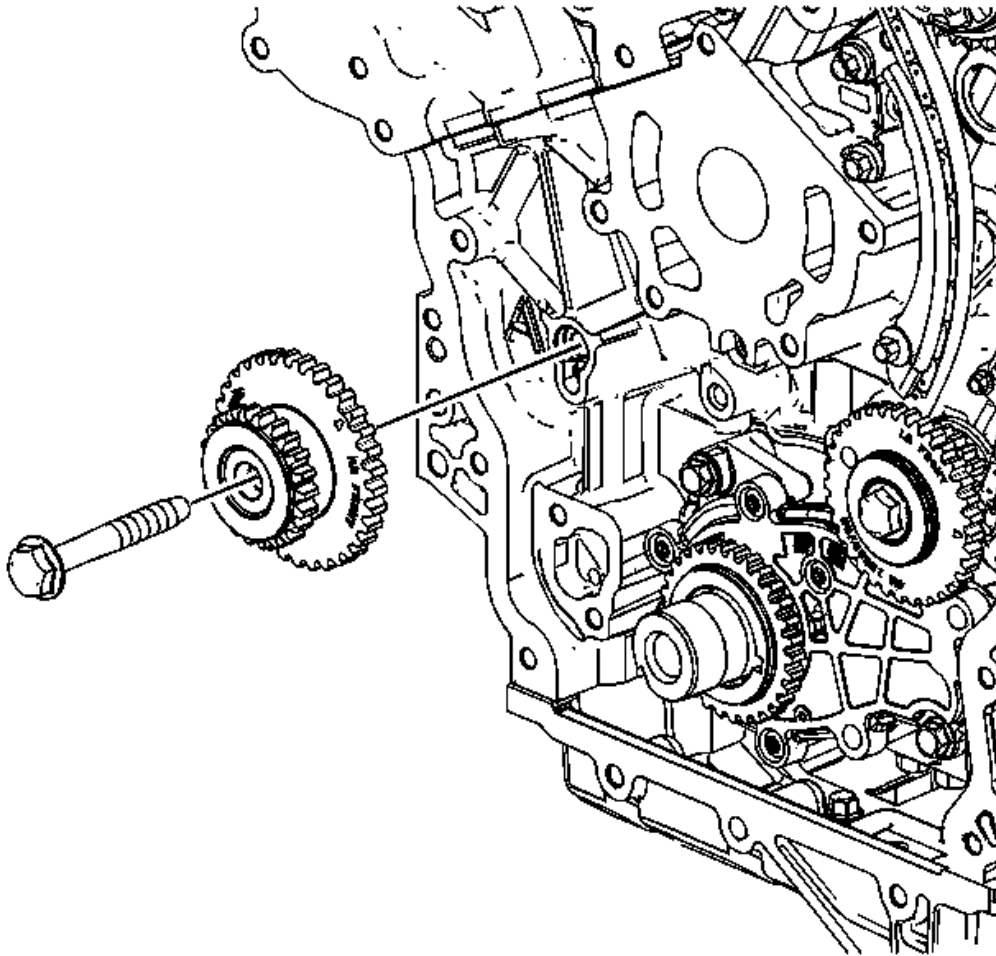
Fig. 78: Right Camshaft Intermediate Drive Chain Idler And Bolt Courtesy of GENERAL MOTORS COMPANY
