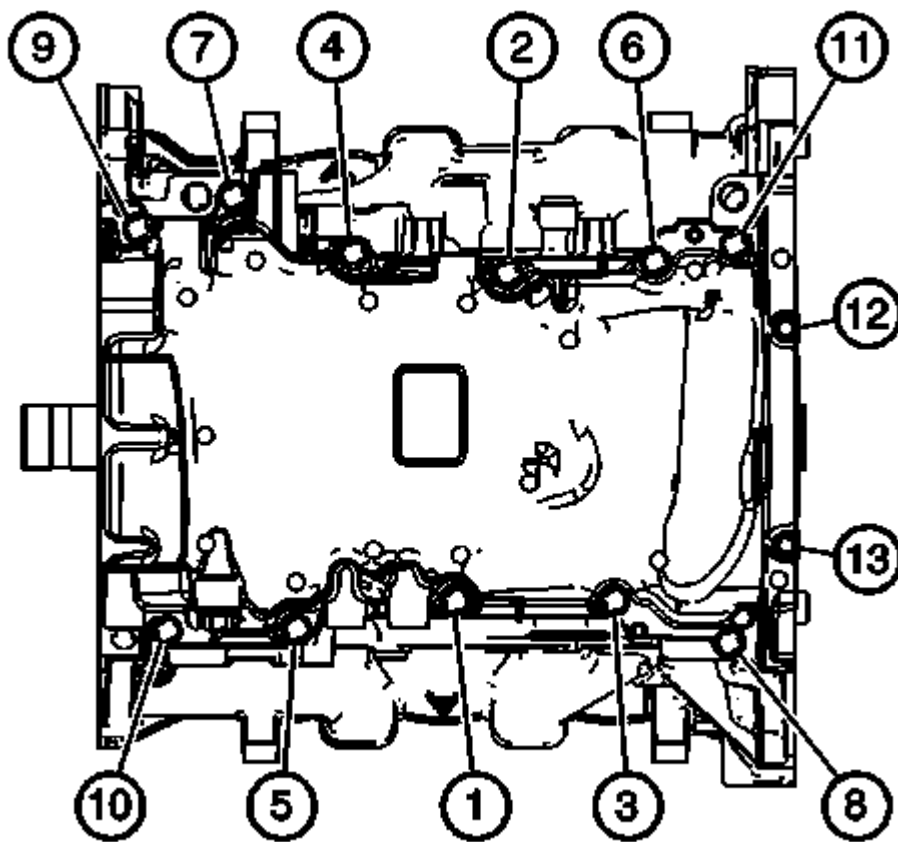
Fig. 194: Oil Pan Bolts Tightening Sequence Courtesy of GENERAL MOTORS COMPANY
