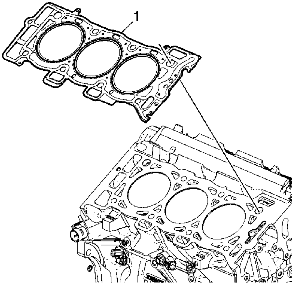
Fig. 178: Right Cylinder Head Gasket Courtesy of GENERAL MOTORS COMPANY
