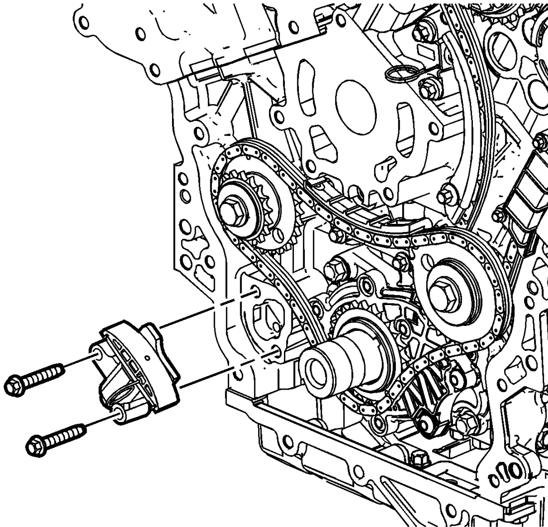
Fig. 80: Primary Camshaft Drive Chain Tensioner Courtesy of GENERAL MOTORS COMPANY
