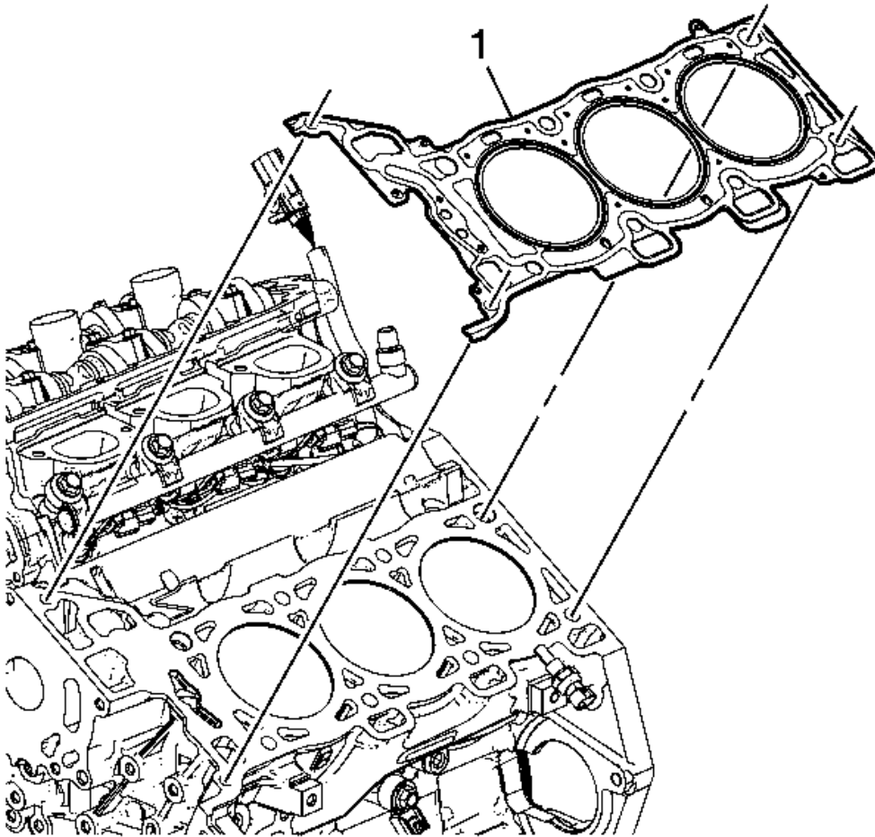
Fig. 173: Left Cylinder Head Gasket Courtesy of GENERAL MOTORS COMPANY
