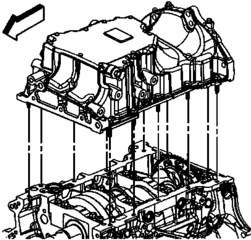
Fig. 188: Engine Oil Pan
