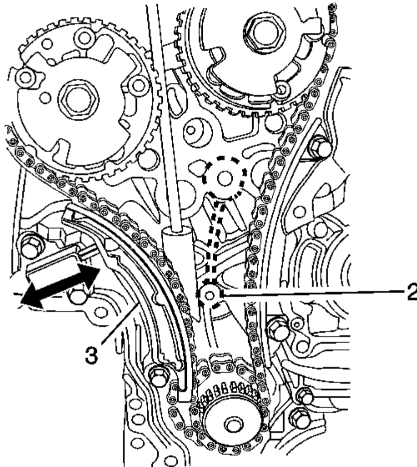
Fig. 99: Gap Between Chain And Internal Rib In Front Cover Courtesy of GENERAL MOTORS COMPANY
