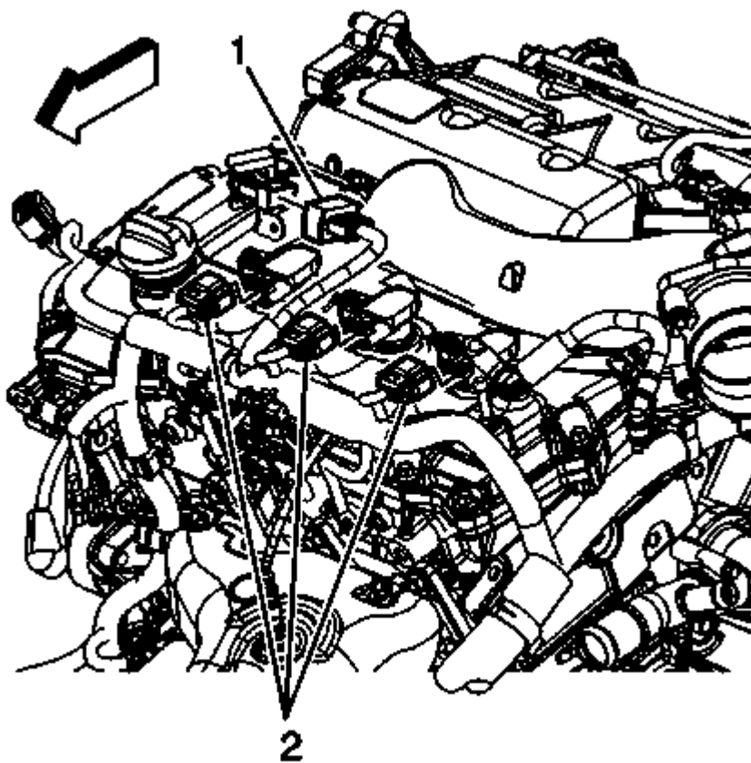
Fig. 216: Ignition Coil And Fuel Injector Wiring Harness Connectors Courtesy of GENERAL MOTORS COMPANY
