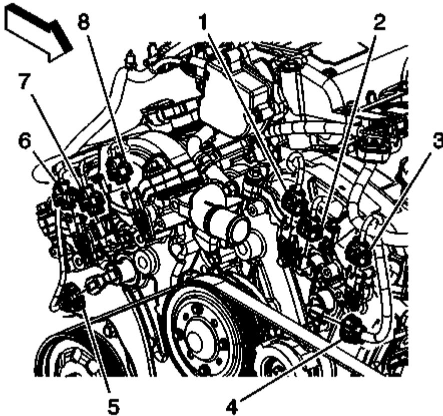
Fig. 231: Camshaft Position Sensor Electrical Connectors Courtesy of GENERAL MOTORS COMPANY
