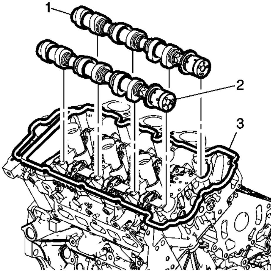
Fig. 140: Right Cylinder Head Camshaft Intake & Exhaust Positioning Points Courtesy of GENERAL MOTORS COMPANY
