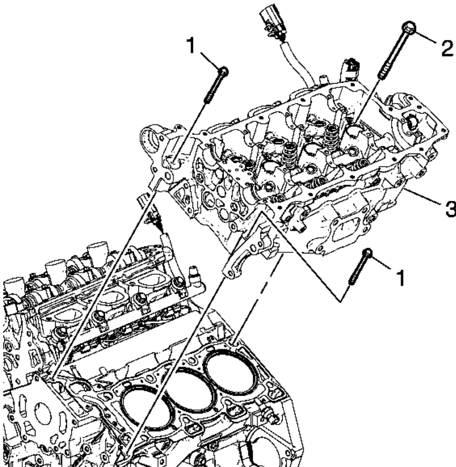
Fig. 172: Left Cylinder Head And Bolts Courtesy of GENERAL MOTORS COMPANY
