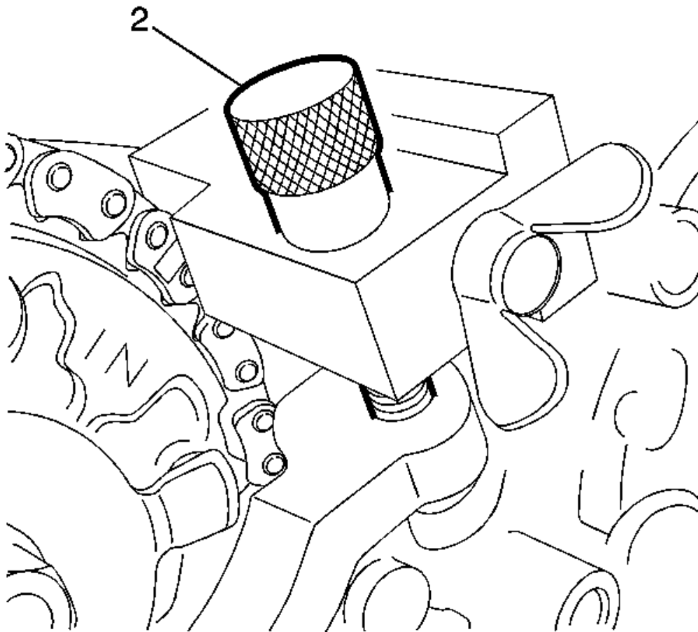
Fig. 112: Retainer Thumbscrew
