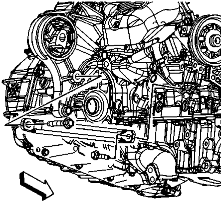
Fig. 223: Oil Pan Brace Bolt And Brace Courtesy of GENERAL MOTORS COMPANY
