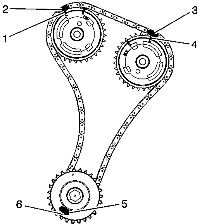
Fig. 121: Left Secondary Camshaft Drive Chain Timing Marks Courtesy of GENERAL MOTORS COMPANY
