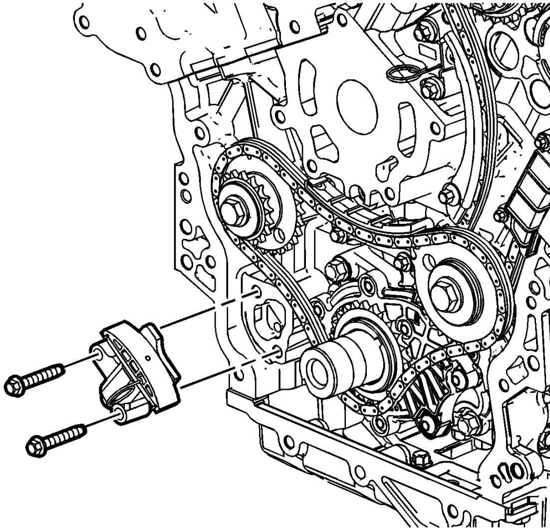
Fig. 81: Primary Camshaft Drive Chain Tensioner Courtesy of GENERAL MOTORS COMPANY
