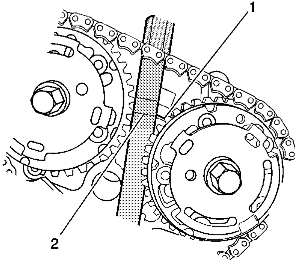
Fig. 116: Timing Chain Retention Tool Courtesy of GENERAL MOTORS COMPANY
