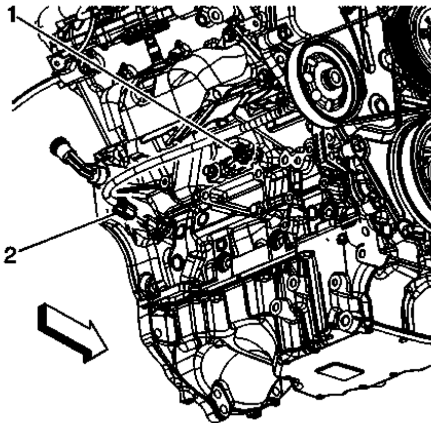
Fig. 232: CKP Sensor And Knock Sensor Courtesy of GENERAL MOTORS COMPANY
