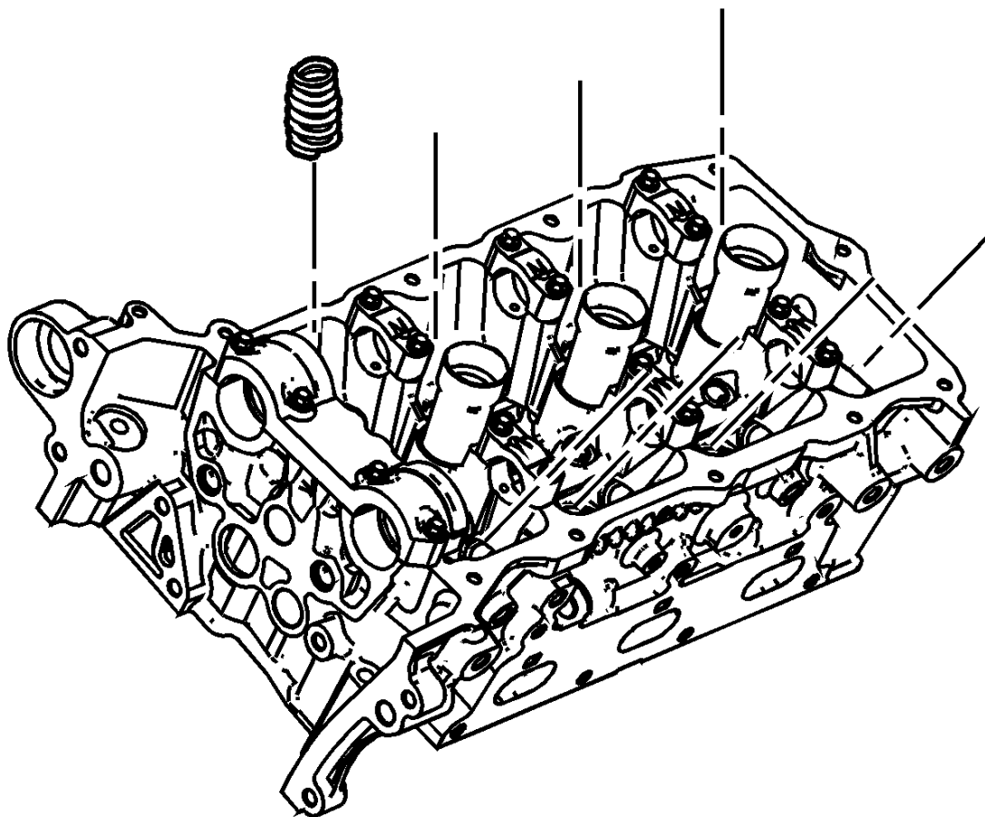
Fig. 160: Valve Spring Courtesy of GENERAL MOTORS COMPANY
