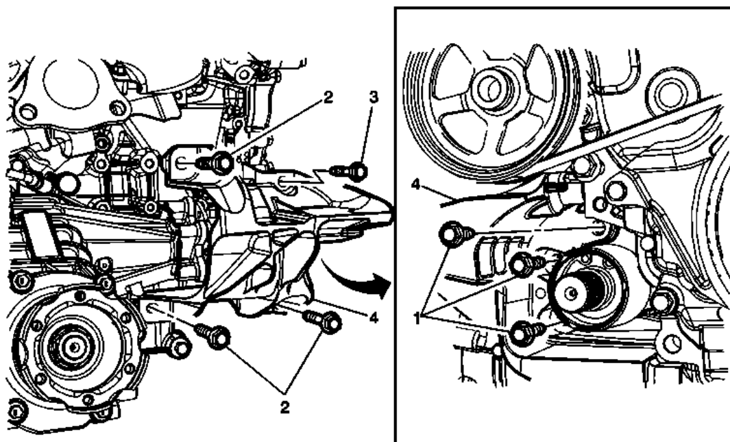
Fig. 9: Mount Bracket (All Wheel Drive)
