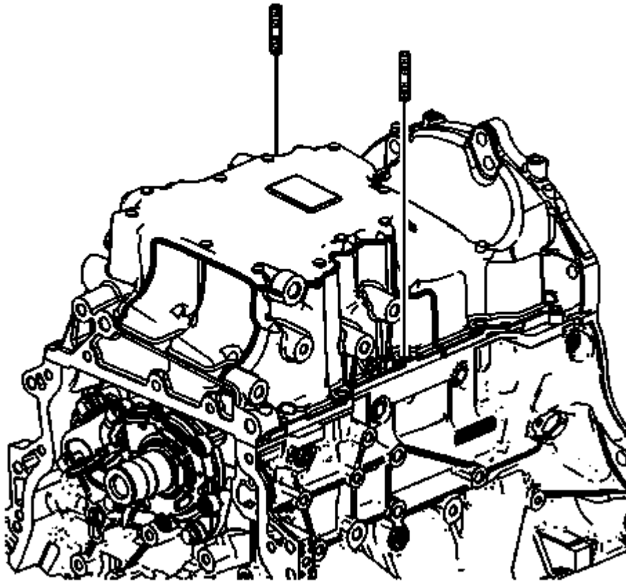
Fig. 223: Engine Block Guide Pins Courtesy of GENERAL MOTORS COMPANY
