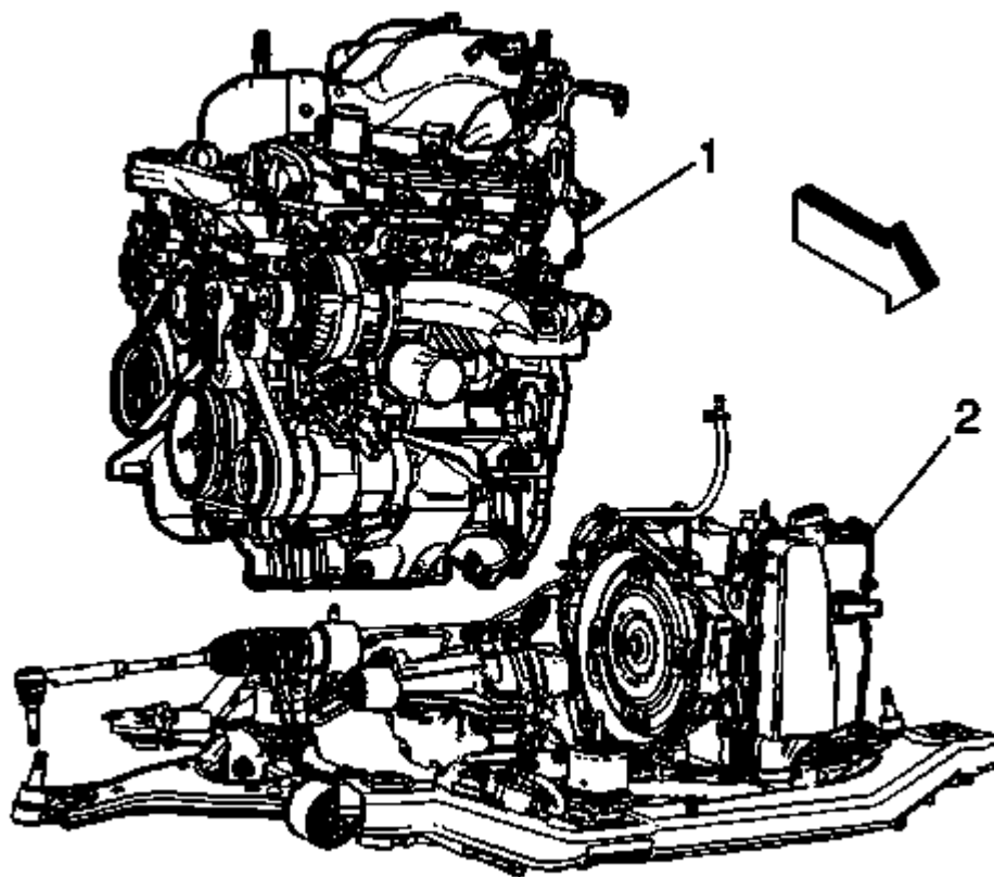
Fig. 255: Engine And Automatic Transaxle Courtesy of GENERAL MOTORS COMPANY
