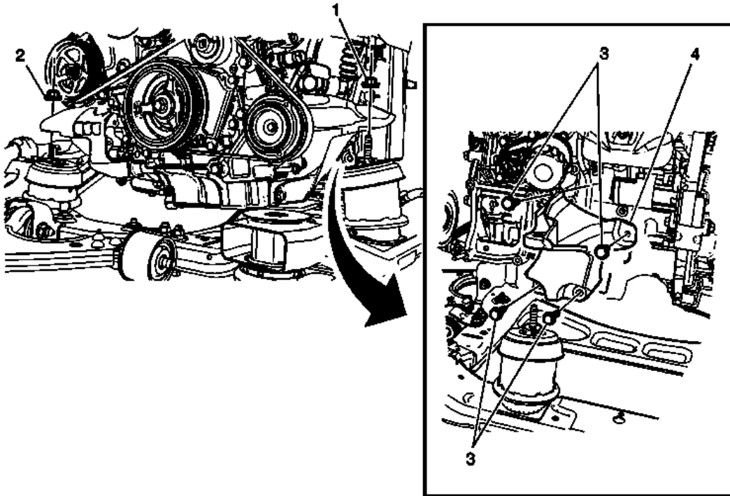
Fig. 7: Engine Font Mount Assembly Courtesy of GENERAL MOTORS COMPANY
