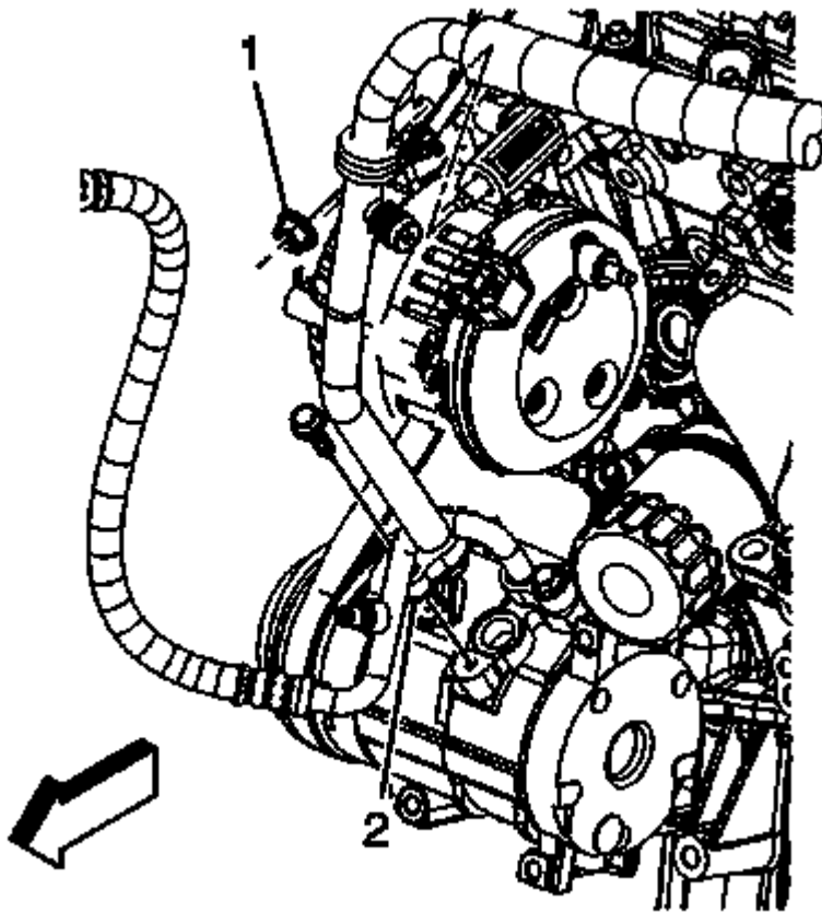
Fig. 274: Suction Hose Bracket Nut
