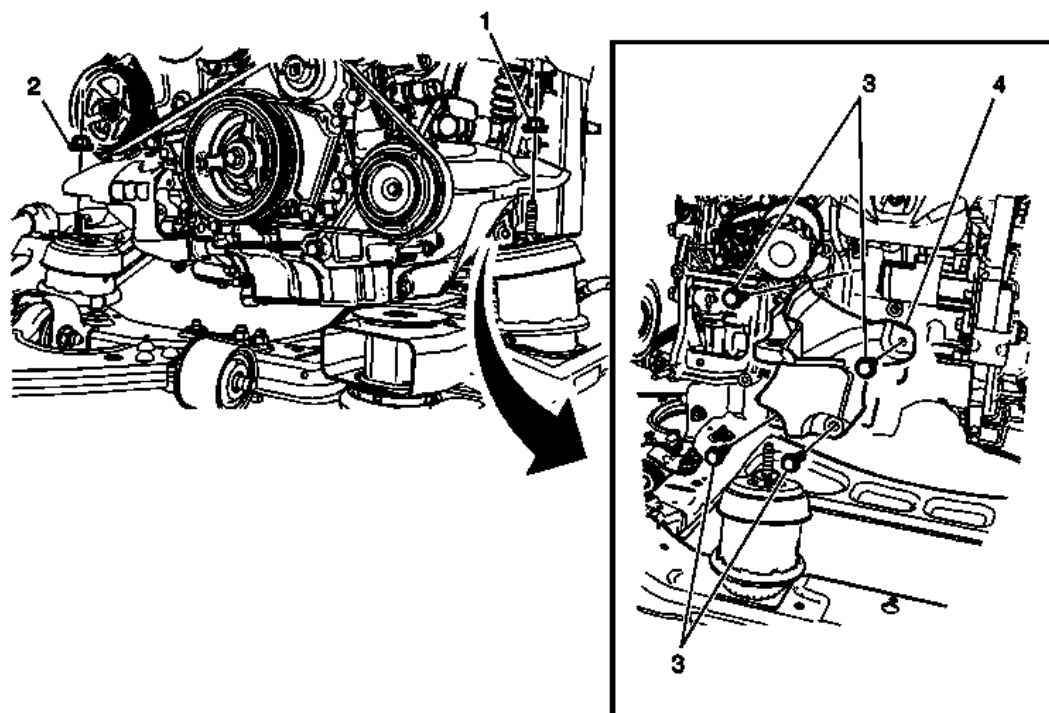
Fig. 7: Engine Front Mount Bracket
