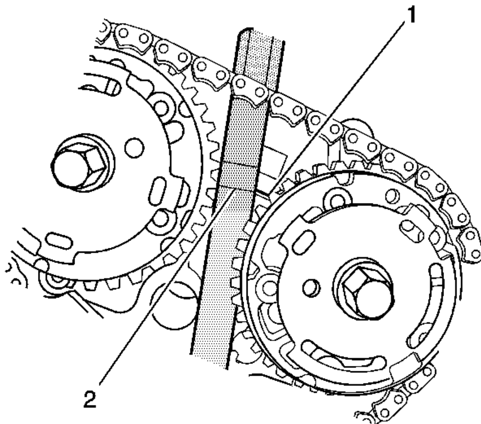
Fig. 149: Inserting Timing Chain Retention Tool Courtesy of GENERAL MOTORS COMPANY
