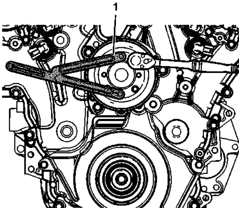
Fig. 65: Water Pump Pulley Holding Tool
