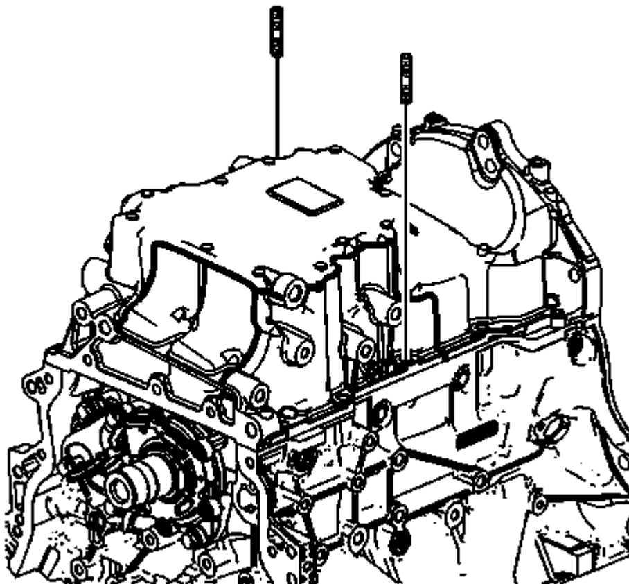
Fig. 217: View Of Engine Block Guides Courtesy of GENERAL MOTORS COMPANY
