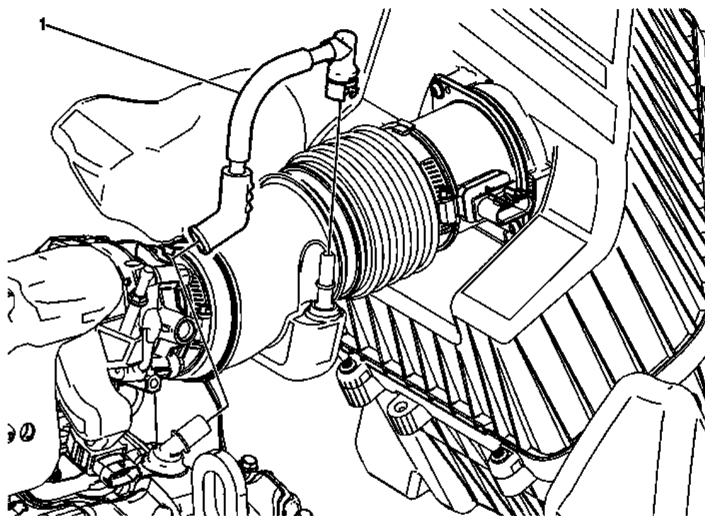
Fig. 13: Identifying Front Positive Crankcase Ventilation Tube
