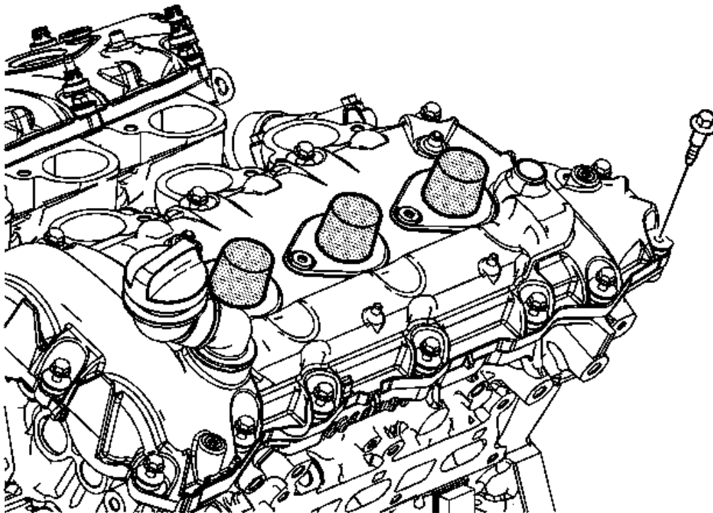
Fig. 49: View of Camshaft Cover & Bolts Courtesy of GENERAL MOTORS COMPANY
