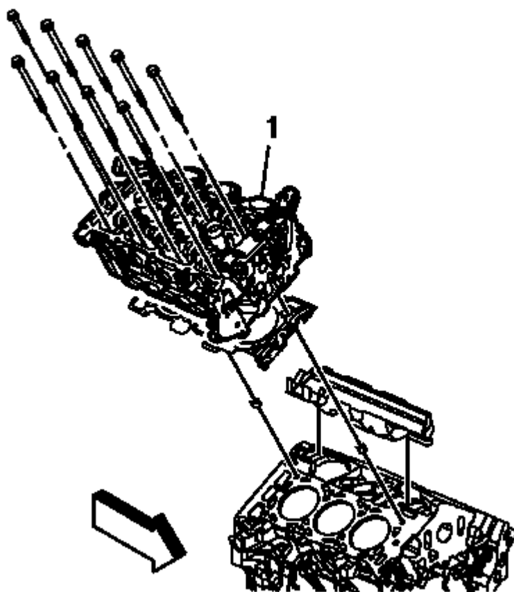
Fig. 204: Cylinder Head
