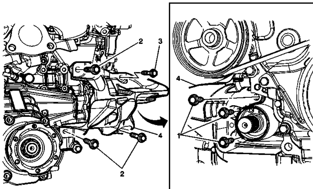
Fig. 9: Engine Mount Bracket & Components (All Wheel Drive)
