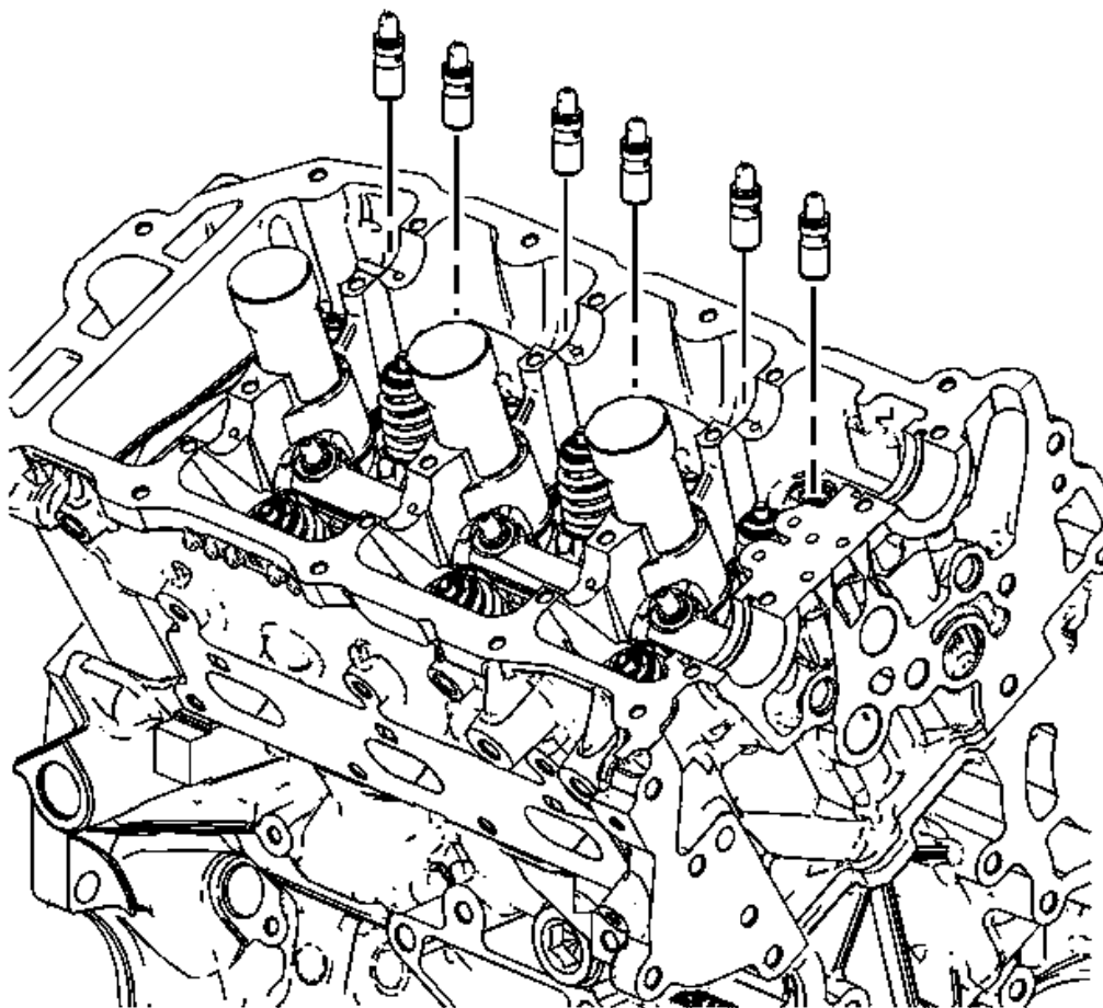
Fig. 176: Identifying Stationary Hydraulic Lash Adjuster (SHLA)
