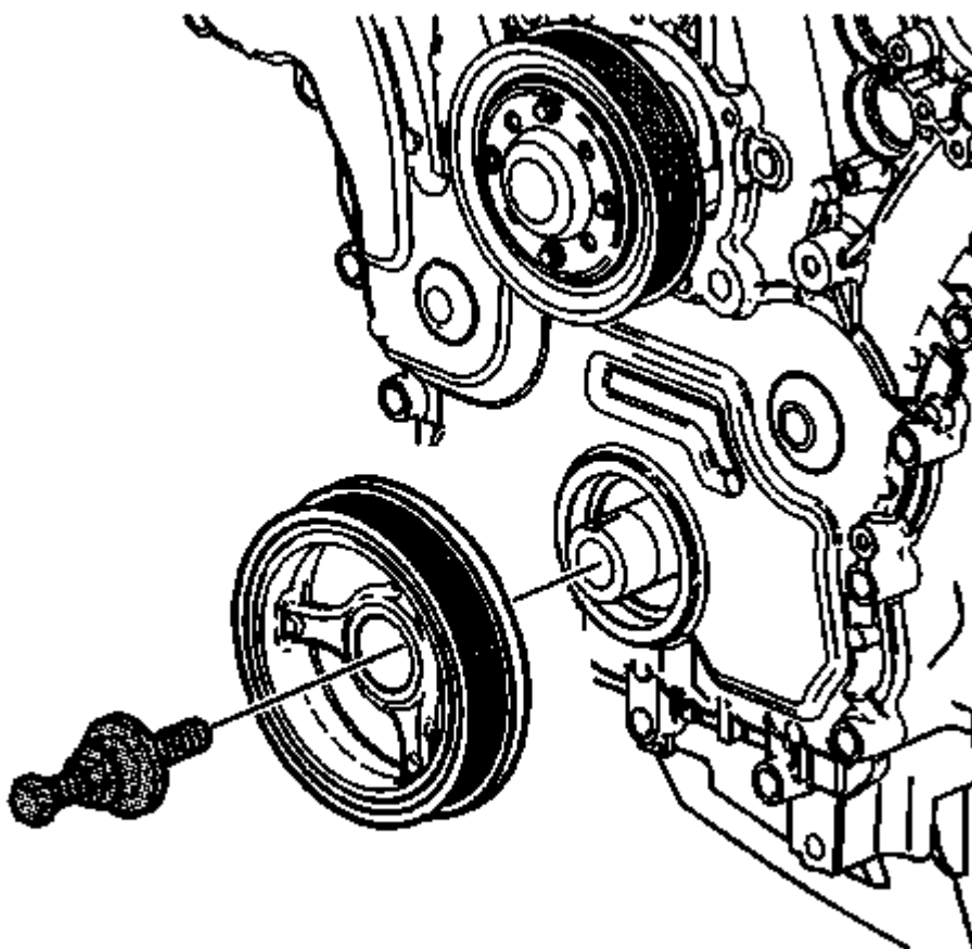
Fig. 39: View Of Crankshaft Balancer & Installation Tool Courtesy of GENERAL MOTORS COMPANY
