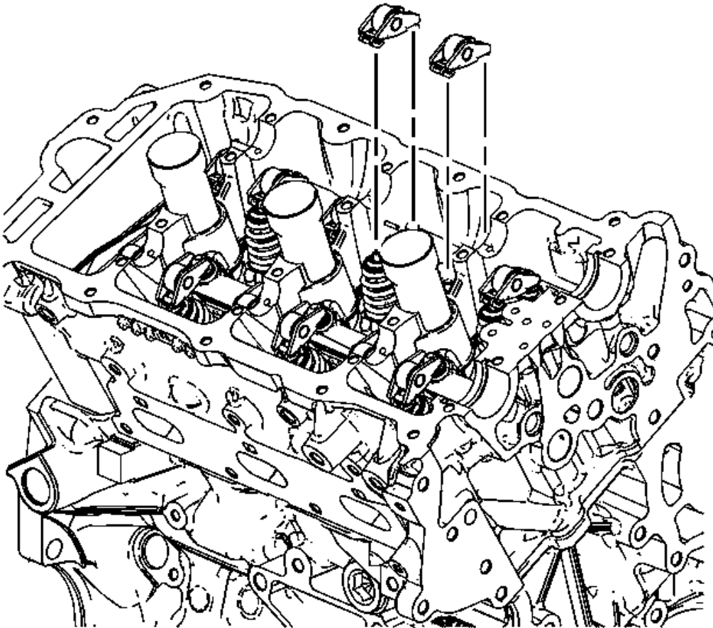
Fig. 153: Identifying Valve Rocker Arms Courtesy of GENERAL MOTORS CORP.
