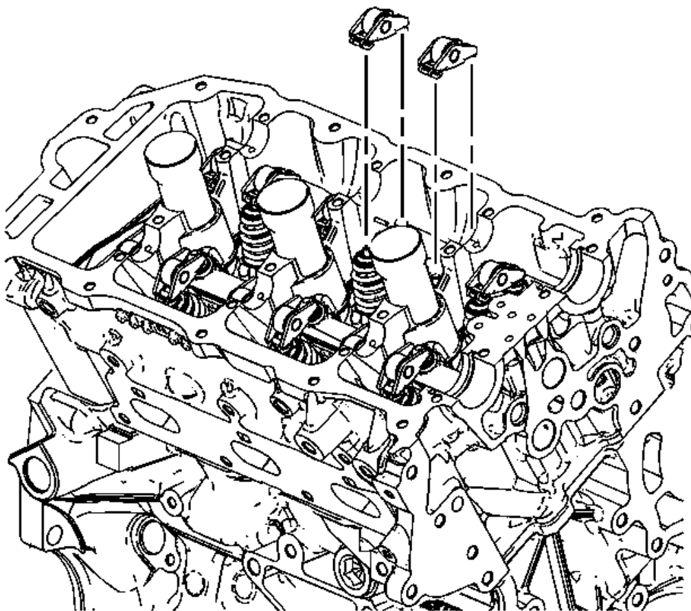
Fig. 154: Identifying Valve Rocker Arms Courtesy of GENERAL MOTORS CORP.
