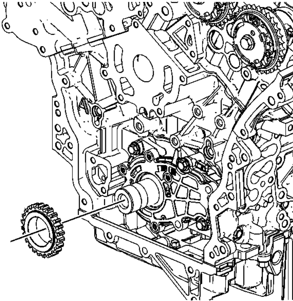
Fig. 82: View Of Crankshaft Sprocket Courtesy of GENERAL MOTORS CORP.
