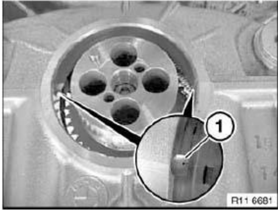
Fig. 90: Identifying Sealant Outlet Courtesy of BMW OF NORTH AMERICA, INC.
