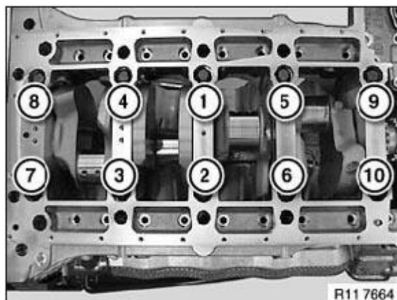
Fig. 121: Identifying Fitting Bolts Tightening Sequence Courtesy of BMW OF NORTH AMERICA, INC.
