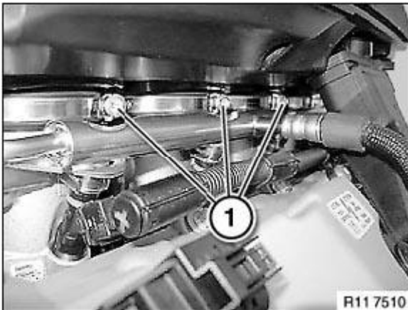
Fig. 454: Identifying Hose Clamp Courtesy of BMW OF NORTH AMERICA, INC.
