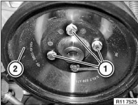
Fig. 194: Identifying Belt Pulley And Screws Courtesy of BMW OF NORTH AMERICA, INC.
