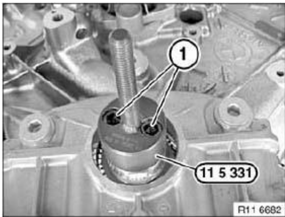
Fig. 127: Securing Special Tool (11 5 331) With Bolts Courtesy of BMW OF NORTH AMERICA, INC.
