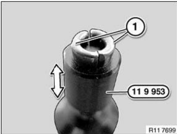
Fig. 299: Pressing Valve Key
