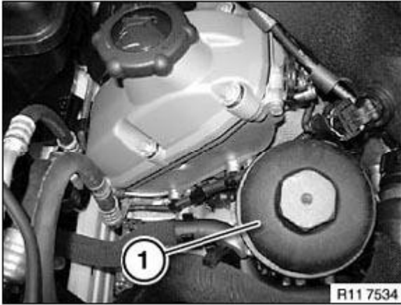
Fig. 430: Identifying Oil Filter Cover Courtesy of BMW OF NORTH AMERICA, INC.
