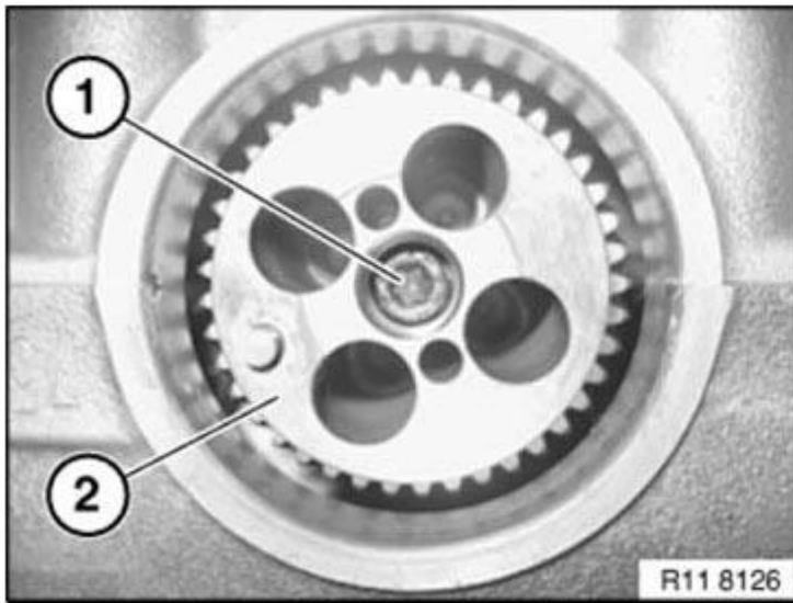
Fig. 126: Identifying Oil Pump Drive Gear And Bolt Courtesy of BMW OF NORTH AMERICA, INC.
