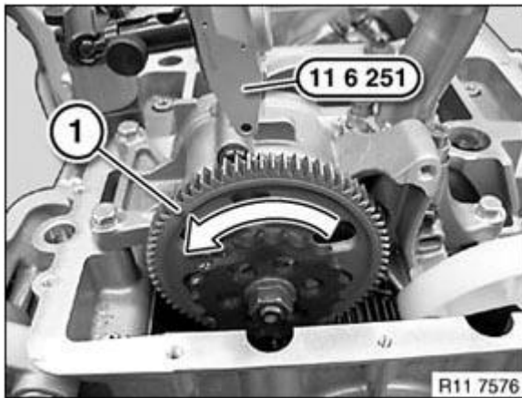
Fig. 427: Turning Oil Suction Pump Gearwheel Courtesy of BMW OF NORTH AMERICA, INC.
