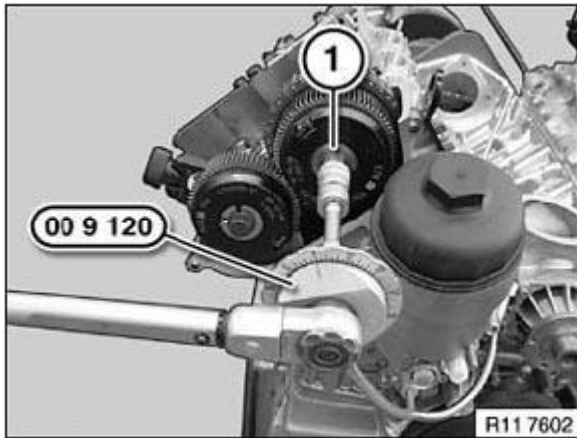
Fig. 205: Securing Central Bolt Using Special Tool (00 9 120) Courtesy of BMW OF NORTH AMERICA, INC.
