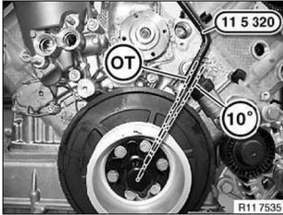
Fig. 312: Identifying Crankshaft Position Courtesy of BMW OF NORTH AMERICA, INC.
