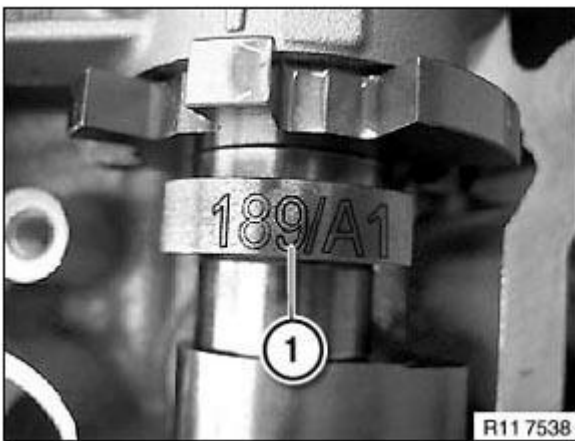
Fig. 200: Identifying Exhaust Camshaft Designation Courtesy of BMW OF NORTH AMERICA, INC.
