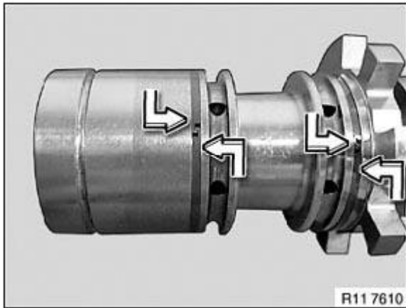
Fig. 236: Removing Plain Compression Rings Courtesy of BMW OF NORTH AMERICA, INC.
