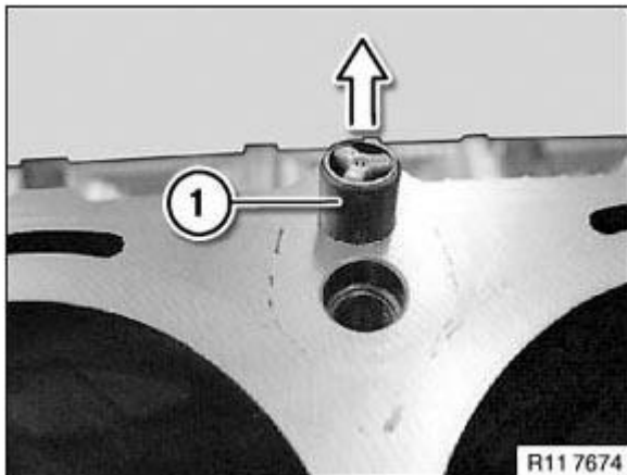
Fig. 74: Removing Non-Return Valves Courtesy of BMW OF NORTH AMERICA, INC.
