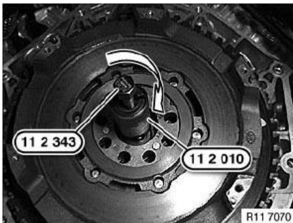
Fig. 143: Removing Roller Bearing Using Special Tool (11 2 343)
