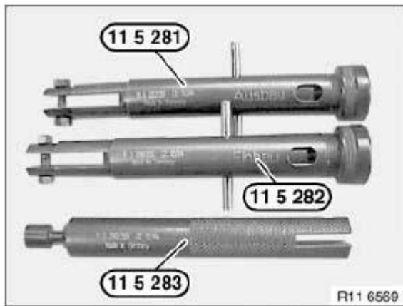
Fig. 267: Identifying Special Tool (11 5 281 And 11 5 282) Courtesy of BMW OF NORTH AMERICA, INC.
