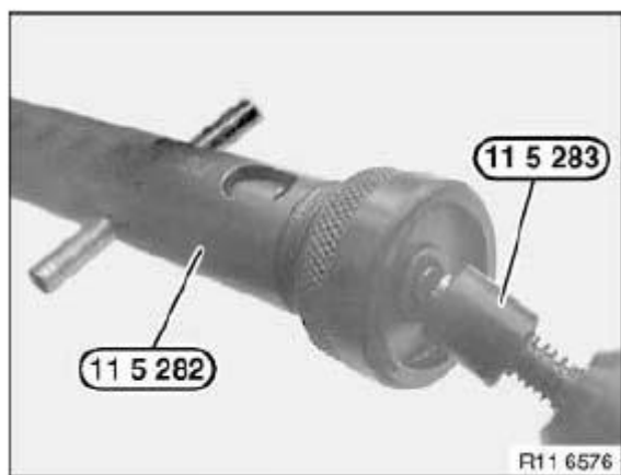
Fig. 281: Identifying Special Tool (11 5 283) Courtesy of BMW OF NORTH AMERICA, INC.
