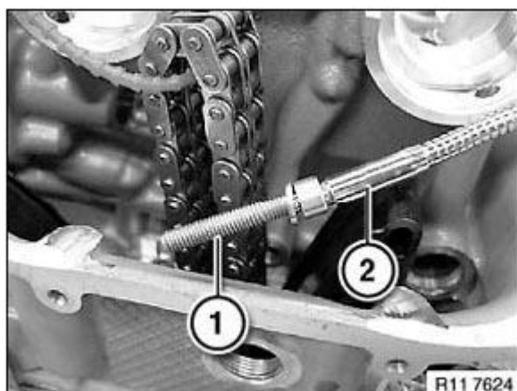
Fig. 55: Identifying Screw On Magnet Courtesy of BMW OF NORTH AMERICA, INC.
