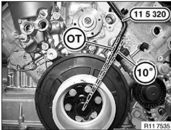
Fig. 224: Identifying Crankshaft Position Courtesy of BMW OF NORTH AMERICA, INC.
