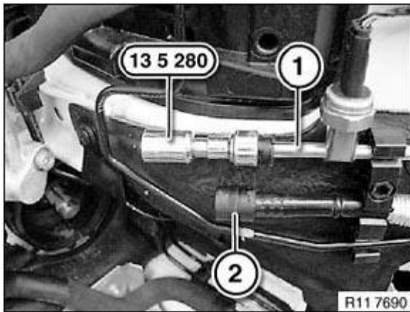
Fig. 27: Locking Fuel Line With Special Tool (13 5 280) Courtesy of BMW OF NORTH AMERICA, INC.
