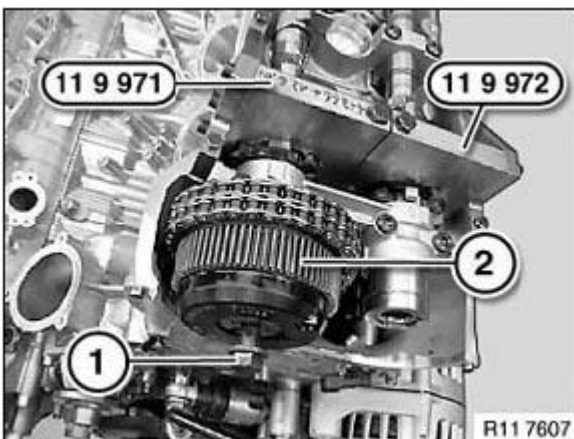
Fig. 341: Identifying Inlet Adjustment Unit And Central Bolt Courtesy of BMW OF NORTH AMERICA, INC.
