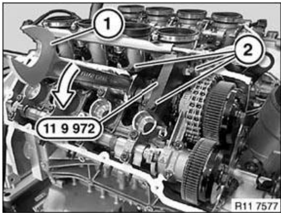
Fig. 388: Rotating Inlet Camshaft Courtesy of BMW OF NORTH AMERICA, INC.
