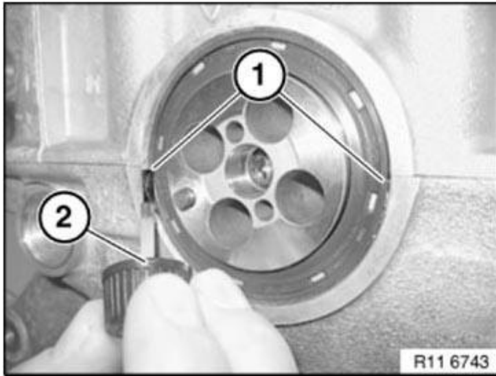
Fig. 138: Applying Liquid Sealing Compound At Outlet Bore Courtesy of BMW OF NORTH AMERICA, INC.
