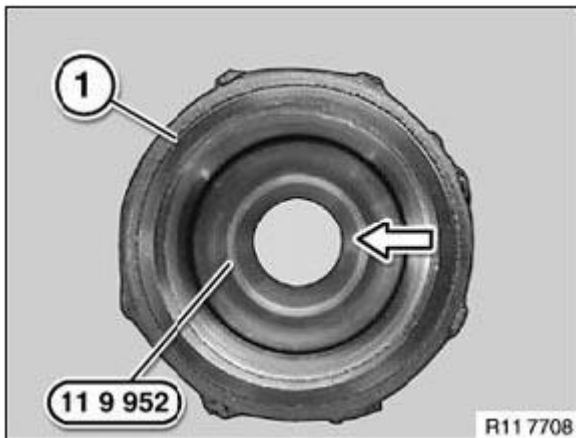
Fig. 280: Inserting Special Tool (11 9 952) Into Valve Cage
