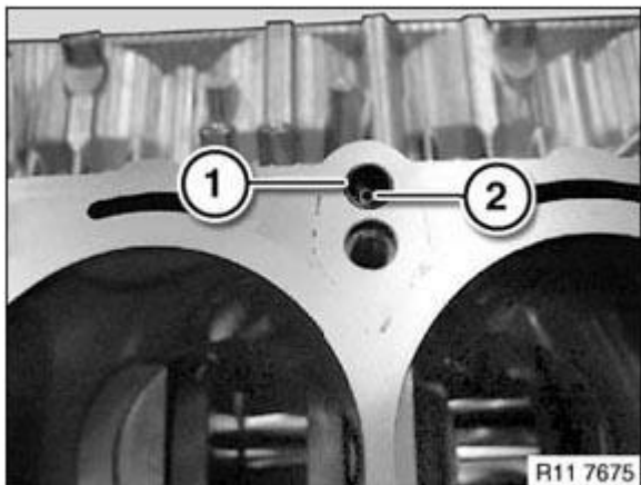
Fig. 75: Identifying Spacer Sleeves And Non-Return Valves Courtesy of BMW OF NORTH AMERICA, INC.
