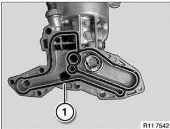
Fig. 433: Identifying Seal
