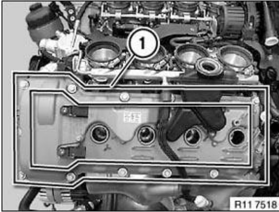
Fig. 64: Identifying Cylinder Head Cover Courtesy of BMW OF NORTH AMERICA, INC.
