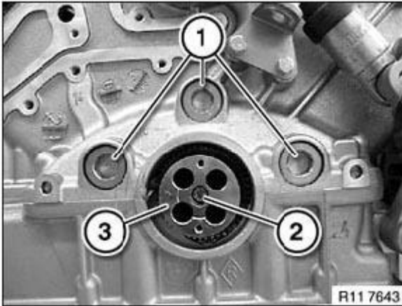
Fig. 255: Identifying Screw Plugs, Screw And Intermediate Piece Courtesy of BMW OF NORTH AMERICA, INC.
