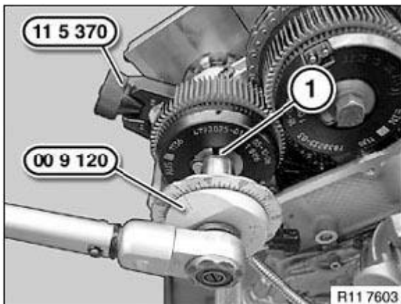
Fig. 378: Securing Central Bolt Using Special Tool (00 9 120) Courtesy of BMW OF NORTH AMERICA, INC.
