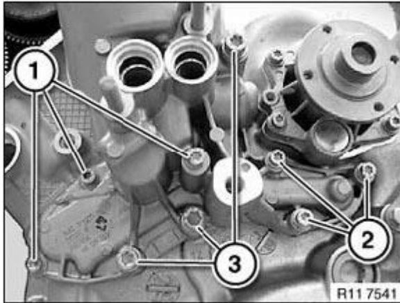
Fig. 432: Identifying Screws
