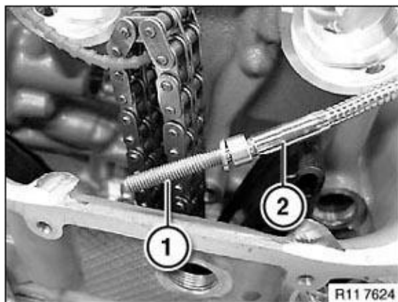
Fig. 46: Identifying Screw On Magnet
