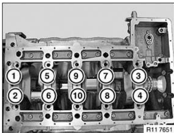
Fig. 105: Identifying M11 Bearing Seat Bolts Removal Sequence Courtesy of BMW OF NORTH AMERICA, INC.
