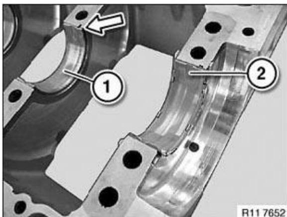
Fig. 98: Identifying Crankcase Lower Half Guide Lugs Position Courtesy of BMW OF NORTH AMERICA, INC.
