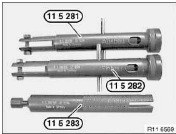
Fig. 288: Identifying Special Tool (11 5 281 And 11 5 282) Courtesy of BMW OF NORTH AMERICA, INC.
