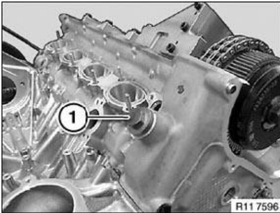
Fig. 340: Identifying Chain Tensioner Courtesy of BMW OF NORTH AMERICA, INC.
