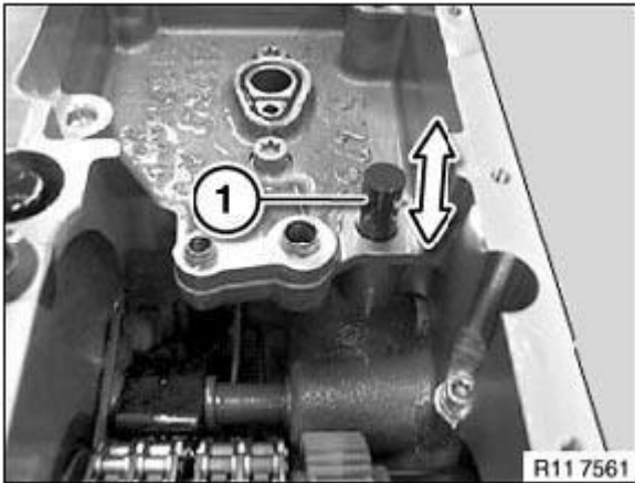
Fig. 420: Removing Piston
