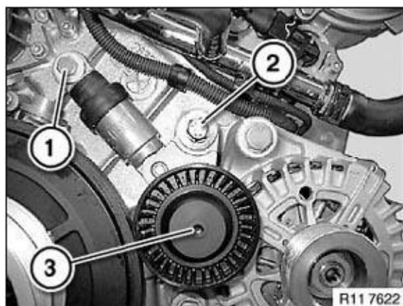
Fig. 195: Identifying Belt Tensioner And Screws Courtesy of BMW OF NORTH AMERICA, INC.
