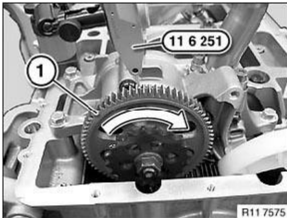
Fig. 359: Turning Oil Suction Pump Gearwheel Courtesy of BMW OF NORTH AMERICA, INC.
