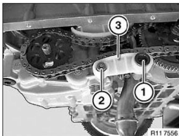
Fig. 418: Identifying Sliding Rail And Screw Courtesy of BMW OF NORTH AMERICA, INC.
