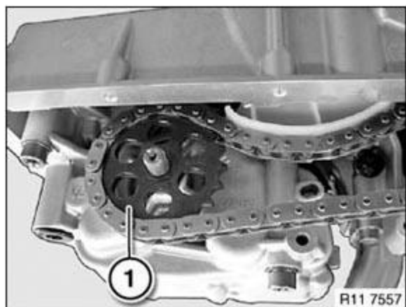
Fig. 419: Identifying Sprocket Wheel Courtesy of BMW OF NORTH AMERICA, INC.
