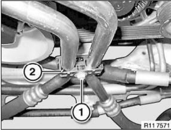
Fig. 435: Identifying Bracket And Nut Courtesy of BMW OF NORTH AMERICA, INC.
