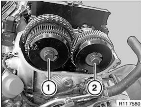
Fig. 336: Identifying Central Bolt Courtesy of BMW OF NORTH AMERICA, INC.
