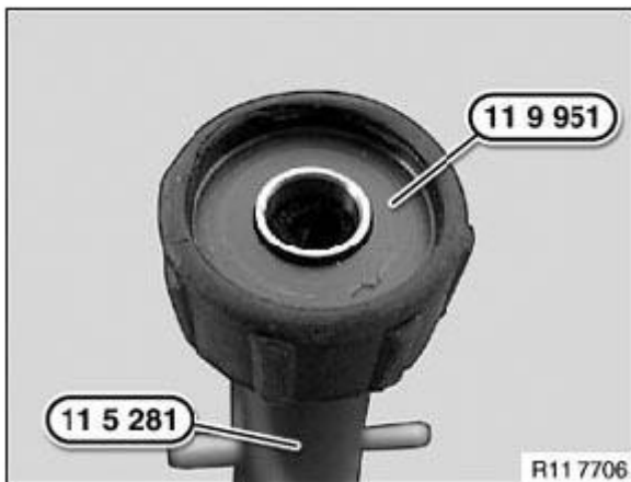
Fig. 272: Identifying Special Tool (11 5 281 And 11 9 951) Courtesy of BMW OF NORTH AMERICA, INC.
