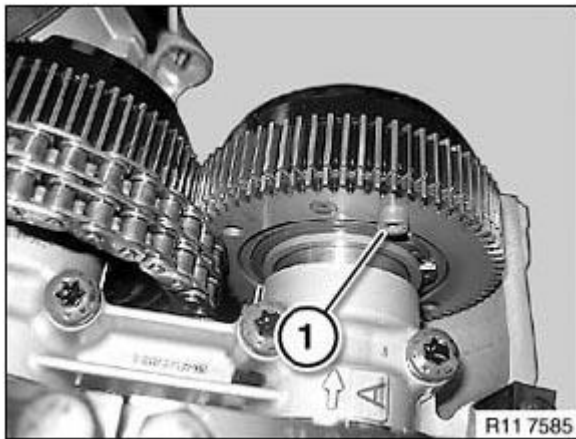
Fig. 317: Identifying Hexagon Socket Screw Courtesy of BMW OF NORTH AMERICA, INC.
