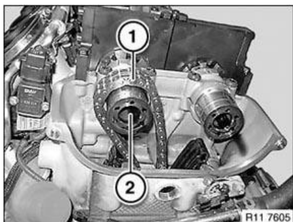
Fig. 344: Identifying Timing Chain
