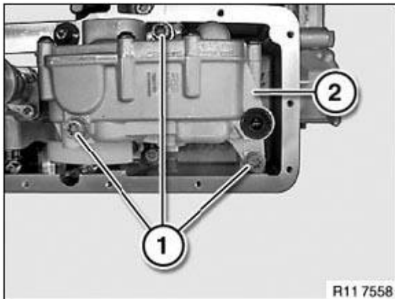
Fig. 422: Identifying Screws And Oil Pump Courtesy of BMW OF NORTH AMERICA, INC.
