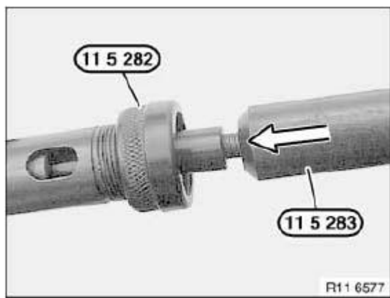
Fig. 282: Pressing Valve Keys Courtesy of BMW OF NORTH AMERICA, INC.
