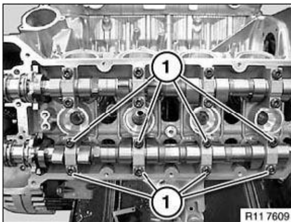
Fig. 239: Identifying Camshaft Screws Courtesy of BMW OF NORTH AMERICA, INC.
