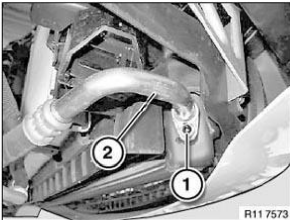
Fig. 436: Identifying Oil Line And Nut Courtesy of BMW OF NORTH AMERICA, INC.
