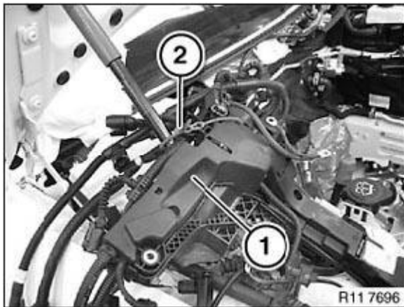
Fig. 28: Securing Engine Wiring Harness With Cable Tie Courtesy of BMW OF NORTH AMERICA, INC.
