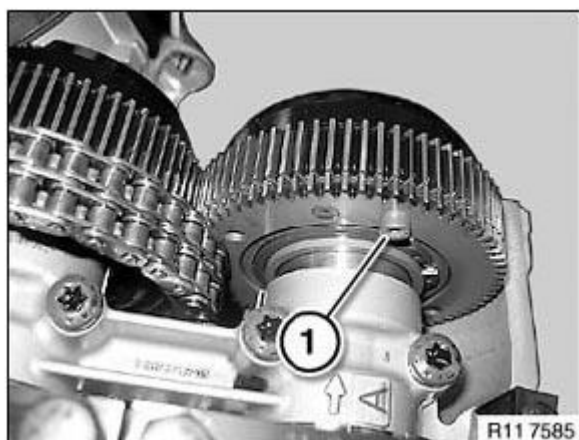
Fig. 320: Identifying Socket Screw
