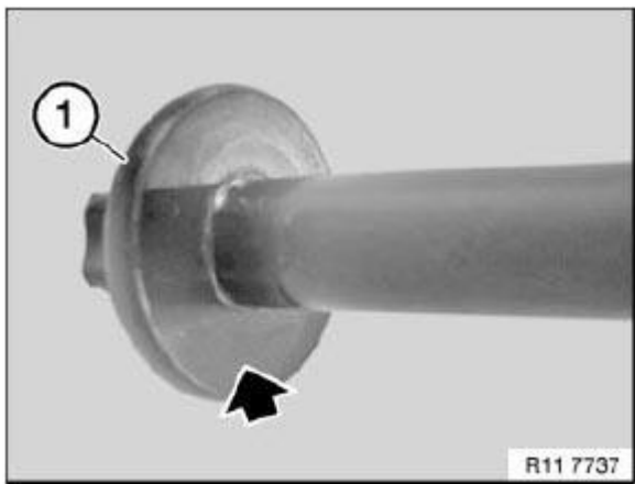
Fig. 363: Coat Contact Face Of New Central Bolt (1) With Copper Paste Courtesy of BMW OF NORTH AMERICA, INC.
