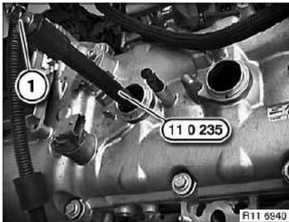
Fig. 5: Identifying Special Tool (11 0 235)
