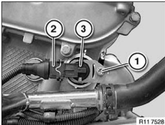
Fig. 392: Identifying Screw, Solenoid Valve And Plug Connections Courtesy of BMW OF NORTH AMERICA, INC.
