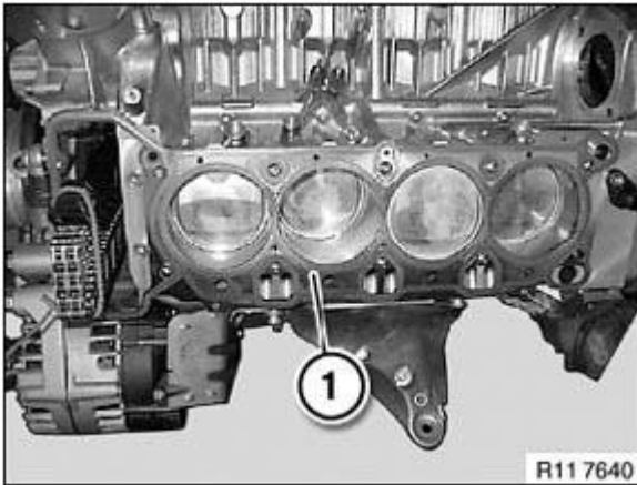
Fig. 72: Identifying Cylinders 5-8 Head Gasket Courtesy of BMW OF NORTH AMERICA, INC.
