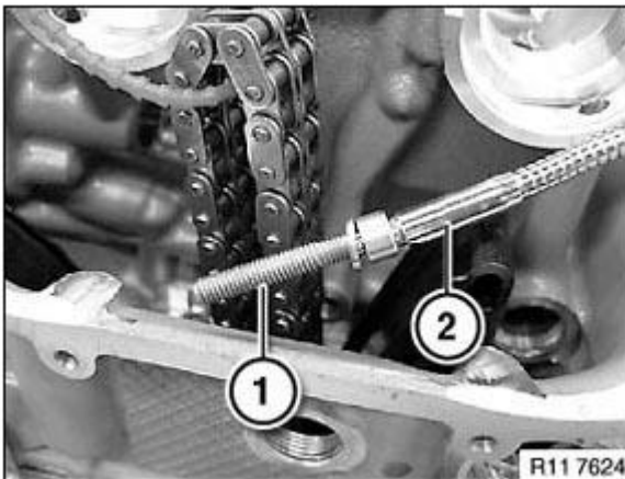
Fig. 60: Identifying Cylinder Head Bolt Courtesy of BMW OF NORTH AMERICA, INC.
