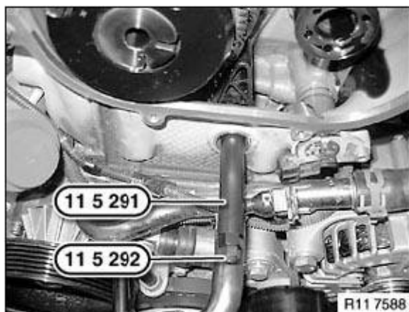
Fig. 321: Identifying Special Tools (11 5 291) And (11 5 292)
