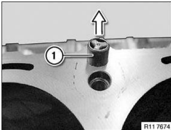
Fig. 69: Removing Non-Return Valves
