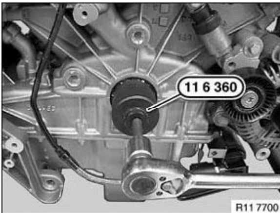
Fig. 80: Screwing Special Tool (11 6 360) Into Radial Seal Courtesy of BMW OF NORTH AMERICA, INC.
