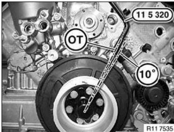
Fig. 374: Identifying Special Tool (11 5 320) On Vibration Damper Courtesy of BMW OF NORTH AMERICA, INC.
