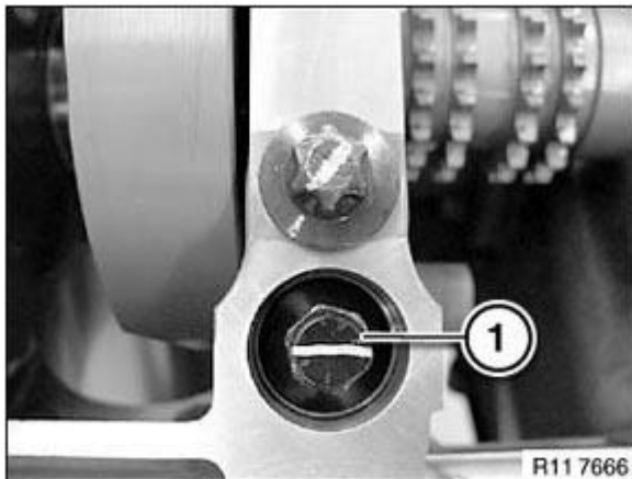
Fig. 108: Identifying Bolts With Colored Line Courtesy of BMW OF NORTH AMERICA, INC.
