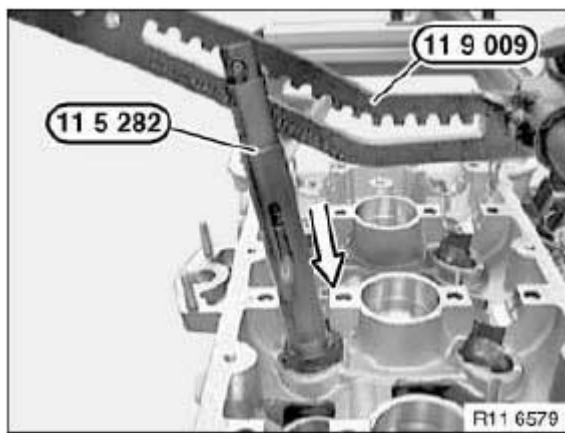
Fig. 273: Pressing Down Special Tool (11 5 282) With (11 9 009) Courtesy of BMW OF NORTH AMERICA, INC.
