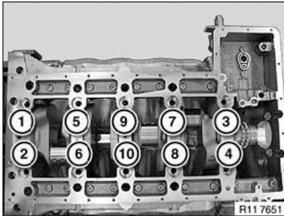
Fig. 95: Identifying M11 Bearing Seat Bolts Tightening Sequence Courtesy of BMW OF NORTH AMERICA, INC.
