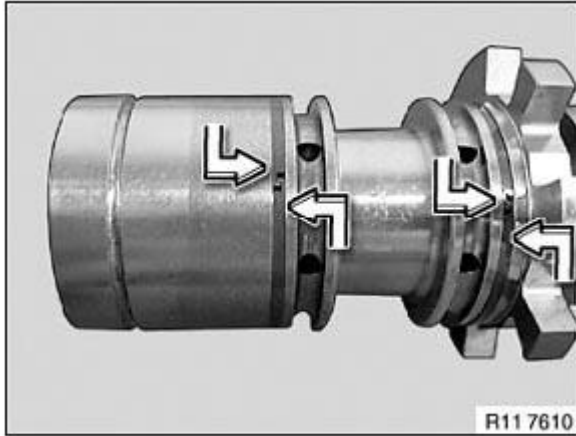
Fig. 194: Pressing Plain Compression Rings Upwards And Downwards Courtesy of BMW OF NORTH AMERICA, INC.
