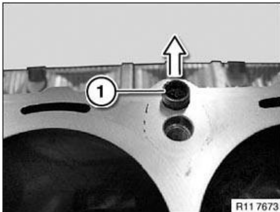
Fig. 68: Removing Spacer Sleeves
