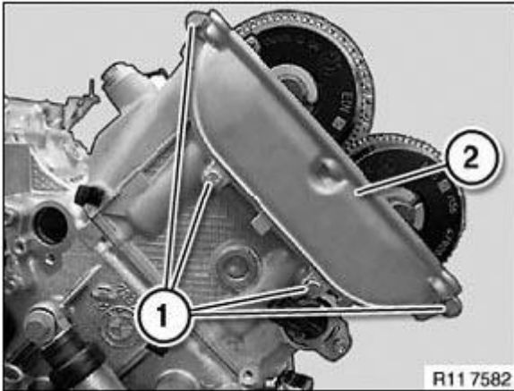
Fig. 328: Identifying Cylinder Bank 2 Bolts And Timing Case Cover
