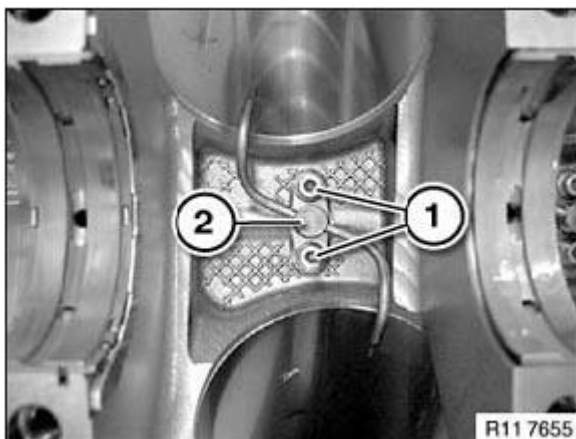
Fig. 144: Identifying Oil Nozzle And Screws Courtesy of BMW OF NORTH AMERICA, INC.
