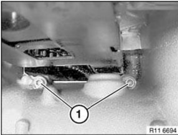
Fig. 59: Identifying Screw And Gearcase Courtesy of BMW OF NORTH AMERICA, INC.
