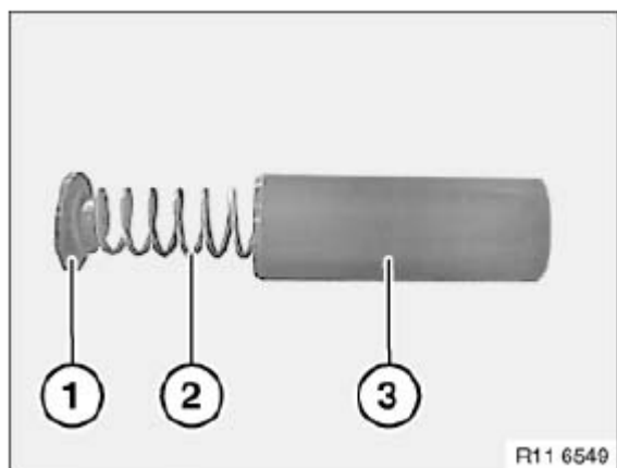
Fig. 404: Identifying Base Valve, Spring And Piston Courtesy of BMW OF NORTH AMERICA, INC.
