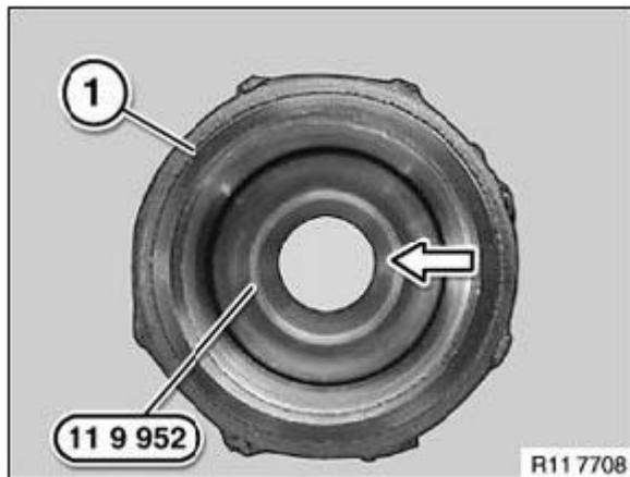
Fig. 269: Inserting Special Tool (11 9 952) In Valve Cage Courtesy of BMW OF NORTH AMERICA, INC.
