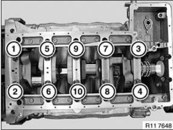
Fig. 94: Identifying Fit Bolts (M9) Tightening Sequence Courtesy of BMW OF NORTH AMERICA, INC.
