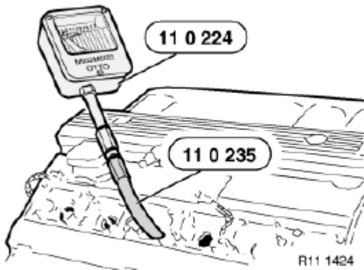
Fig. 6: Connecting Special Tool (11 0 224) And Bar Pressure Adapter To Diagnosis Tester
