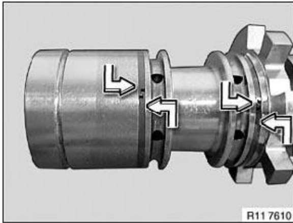
Fig. 206: Pressing Plain Compression Rings Upwards And Downwards Courtesy of BMW OF NORTH AMERICA, INC.
