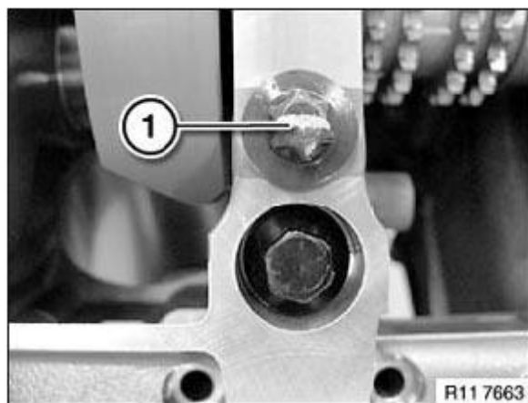
Fig. 105: Identifying M11 Bearing Seat Bolts With Colored Line Courtesy of BMW OF NORTH AMERICA, INC.
