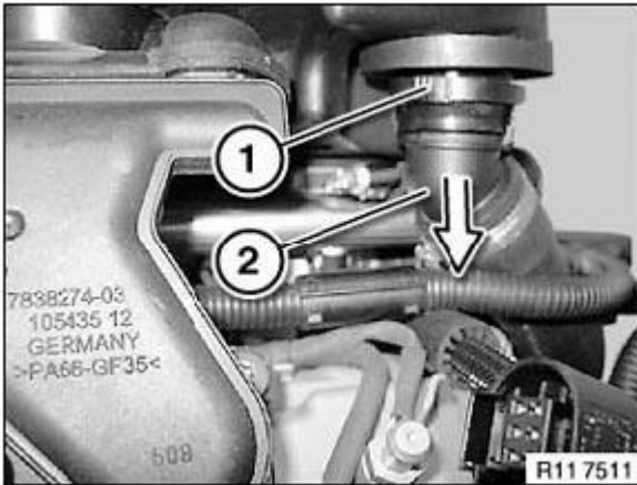
Fig. 433: Identifying Idle Actuator Incoming Air Fastener And Hose Courtesy of BMW OF NORTH AMERICA, INC.
