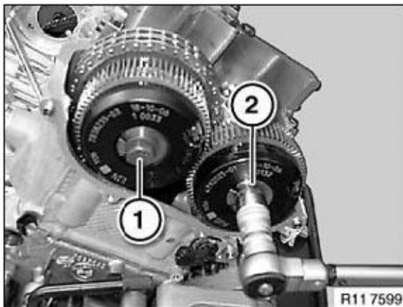
Fig. 319: Inserting Central Bolts
