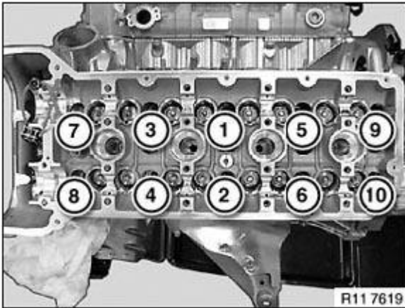
Fig. 54: Identifying Cylinder Head Bolts Tightening Sequence Courtesy of BMW OF NORTH AMERICA, INC.
