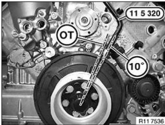
Fig. 384: Rotating Crankshaft At Central Bolt With Special Tool (11 5 320) Courtesy of BMW OF NORTH AMERICA, INC.
