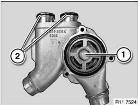
Fig. 431: Identifying Thermostat And Rubber Section Courtesy of BMW OF NORTH AMERICA, INC.
