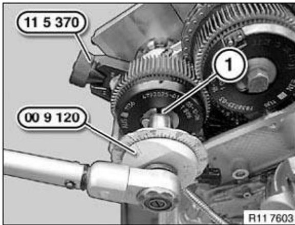
Fig. 237: Securing Central Bolt With Special Tool (00 9 120) Courtesy of BMW OF NORTH AMERICA, INC.
