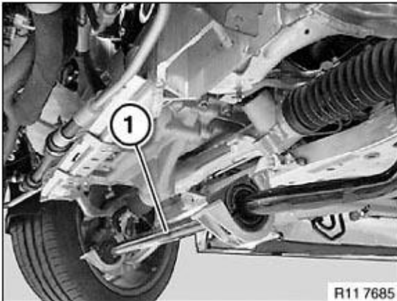
Fig. 7: Identifying Stabilizer On Front Axle Carrier Courtesy of BMW OF NORTH AMERICA, INC.
