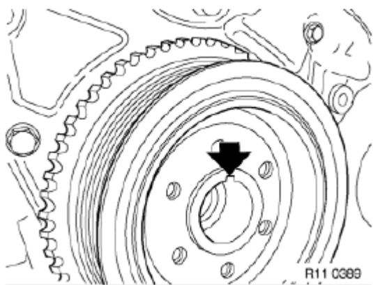
Fig. 160: Aligning Vibration Damper With Groove To Featherkey
