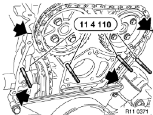
Fig. 103: Identifying Special Tool (11 4 110) Courtesy of BMW OF NORTH AMERICA, INC.
