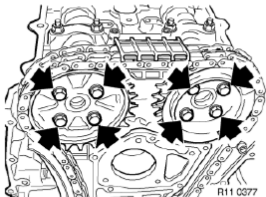
Fig. 232: Locating Chain Wheels Screws Courtesy of BMW OF NORTH AMERICA, INC.
