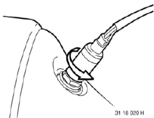
Fig. 301: Disconnecting Connector For Oxygen Sensor Courtesy of BMW OF NORTH AMERICA, INC.
