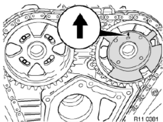
Fig. 61: Locating Arrow On Sensor Gear In Cylinder Axis Points
