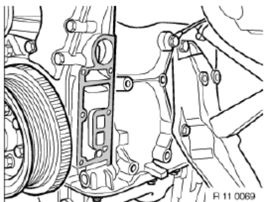
Fig. 280: Identifying Sealing Faces
