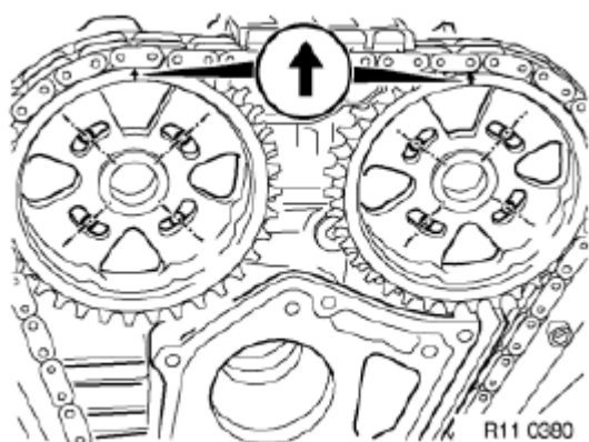
Fig. 60: Locating Arrow On Chain Wheel
