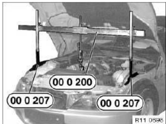
Fig. 89: Identifying Special Tools
