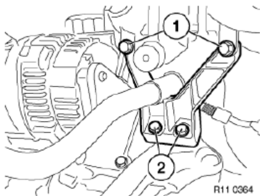
Fig. 294: Identifying Screws Courtesy of BMW OF NORTH AMERICA, INC.
