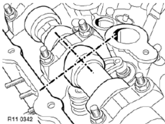
Fig. 250: Rotating Engine On Central Screw Engine-Wise Until Cams On Camshaft Point Vertically Upwards Courtesy of BMW OF NORTH AMERICA, INC.
