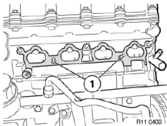
Fig. 299: Identifying Hollow Bushes (1)
