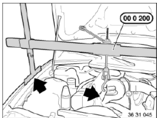
Fig. 90: Identifying Special Tool (00 0 200)
