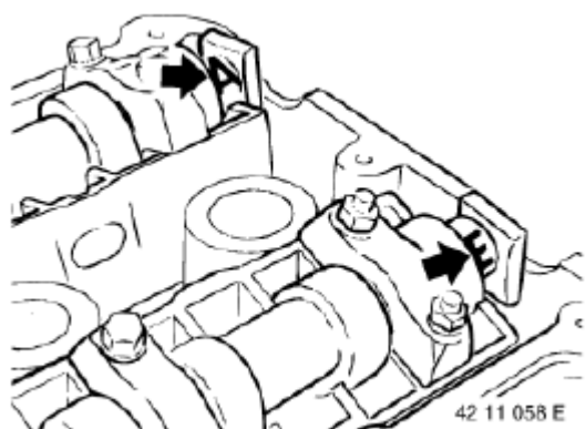
Fig. 202: Locating Exhaust And Intake Camshaft
