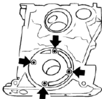
Fig. 275: Locating Oil-Pump Cover Bolts Courtesy of BMW OF NORTH AMERICA, INC.
