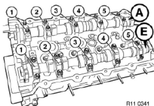
Fig. 201: Locating Camshaft Bolts
