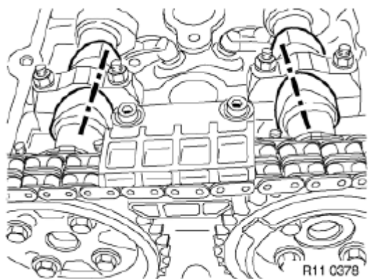
Fig. 211: Camshaft Alignment
