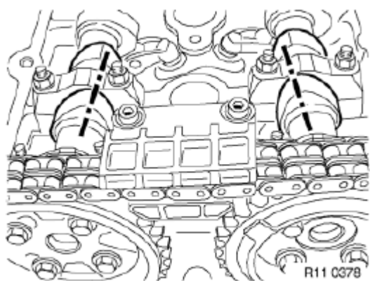
Fig. 195: Camshaft Alignment
