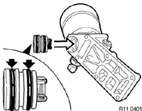
Fig. 281: Identifying Sealing Rings On Non-Return Valve
