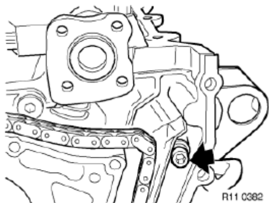
Fig. 48: Locating Slide Rail Adjusting Screw
