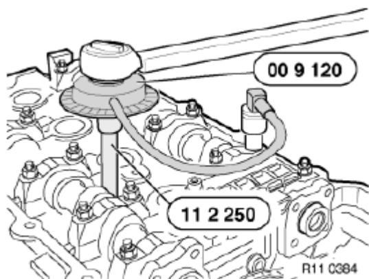
Fig. 52: Identifying Special Tools
