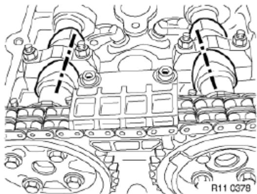
Fig. 242: Turning Central Screw To Rotate Crankshaft Courtesy of BMW OF NORTH AMERICA, INC.
