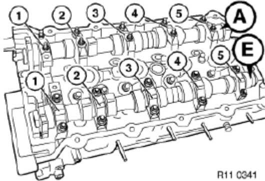
Fig. 203: Locating Camshaft Bolts
