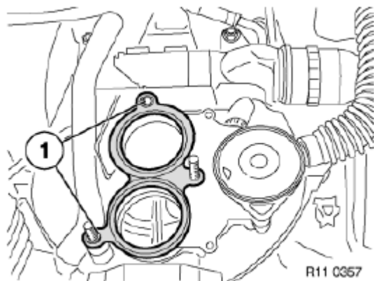
Fig. 296: Identifying Dowel Sleeves
