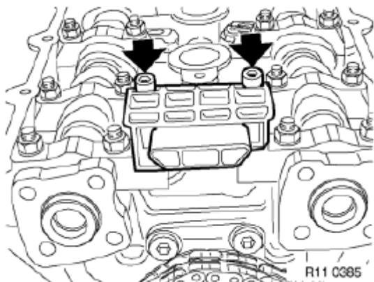
Fig. 237: Locating Chain Guide
