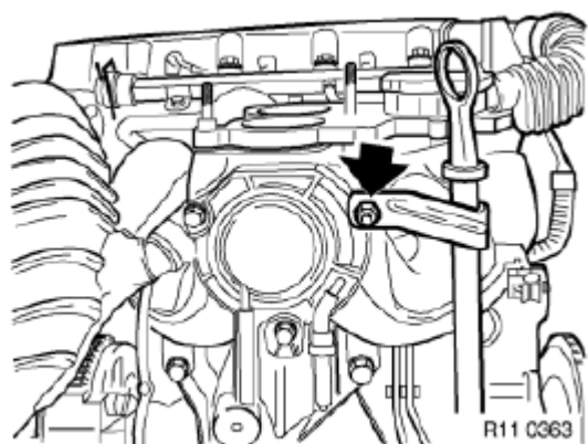
Fig. 293: Locating Guide Pipe For Dipstick Courtesy of BMW OF NORTH AMERICA, INC.
