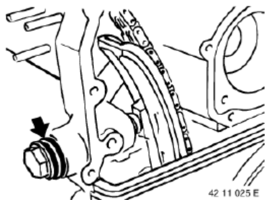
Fig. 233: Locating Screw Plug Courtesy of BMW OF NORTH AMERICA, INC.
