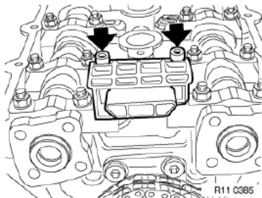
Fig. 200: Locating Chain Guide
