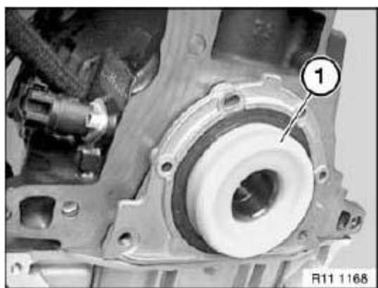
Fig. 130: Identifying Support Bushing
