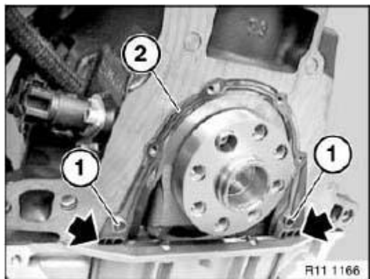
Fig. 128: Identifying Dowel Sleeves And Seal Courtesy of BMW OF NORTH AMERICA, INC.
