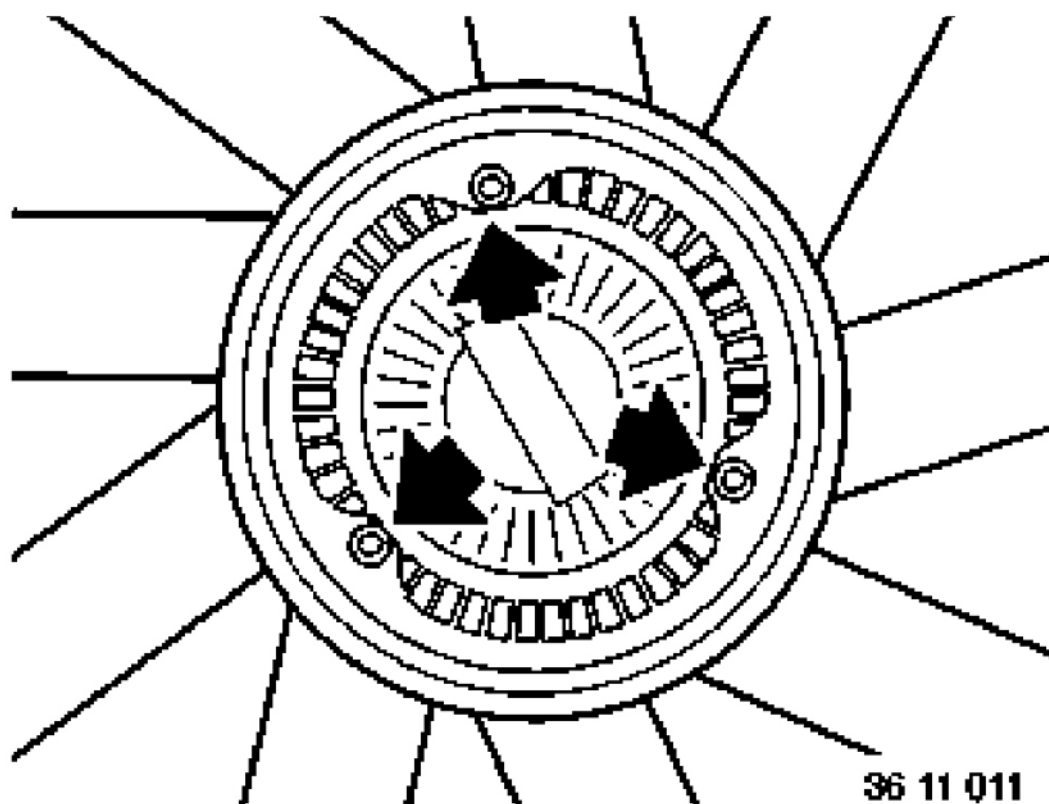
Fig. 287: Locating Fan Coupling Screws Courtesy of BMW OF NORTH AMERICA, INC.
