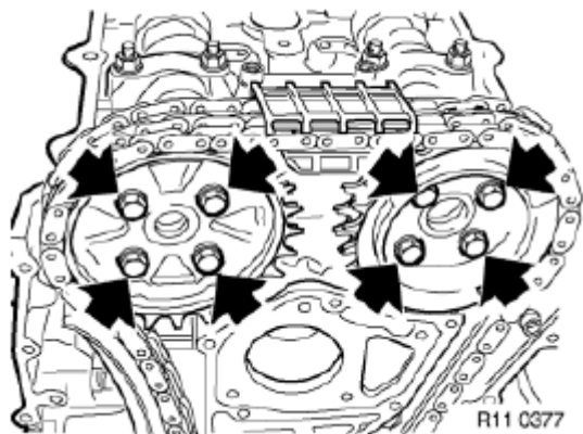
Fig. 199: Locating Chain Wheels Screws
