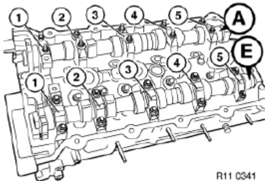
Fig. 240: Locating Exhaust And Intake Camshaft Courtesy of BMW OF NORTH AMERICA, INC.
