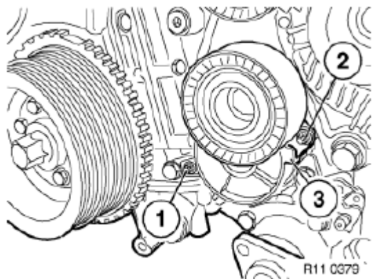
Fig. 192: Identifying Screws
