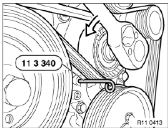
Fig. 189: Identifying Special Tool (11 3 340) Courtesy of BMW OF NORTH AMERICA, INC.
