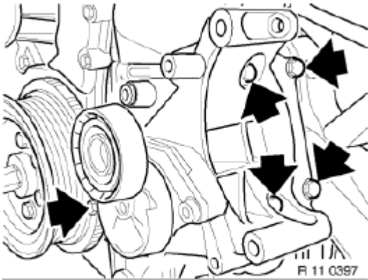
Fig. 278: Locating Alternator Carrier Bolts Courtesy of BMW OF NORTH AMERICA, INC.
