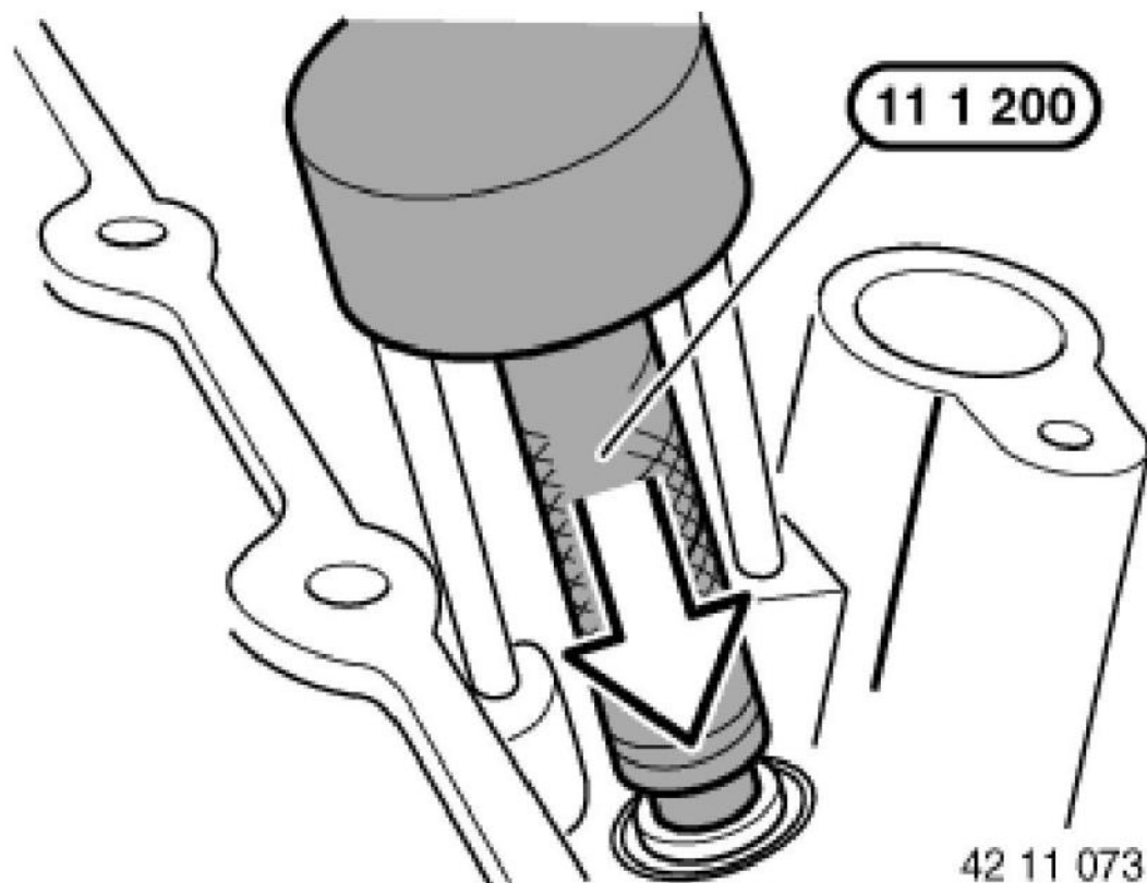
Fig. 79: Pressing Valve Stem Seal Courtesy of BMW OF NORTH AMERICA, INC.
