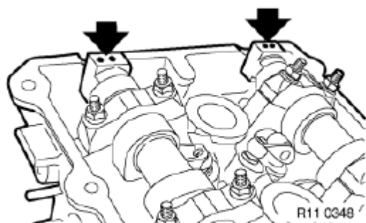
Fig. 57: Alignment Bores Point Upward
