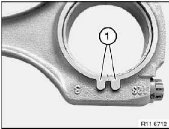
Fig. 154: Identifying Connecting Rod Elevation Courtesy of BMW OF NORTH AMERICA, INC.
