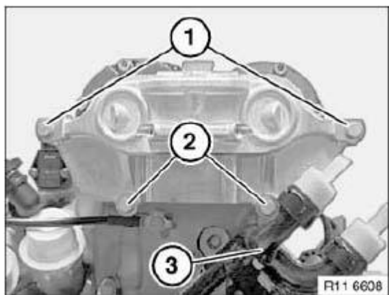
Fig. 366: Identifying VANOS Adjustment Unit With Screws Courtesy of BMW OF NORTH AMERICA, INC.
