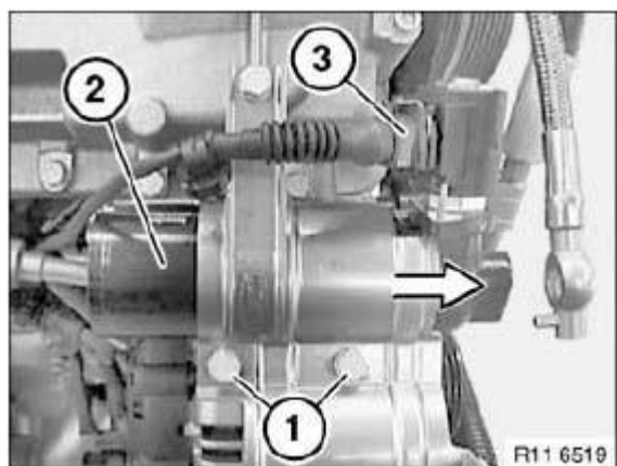
Fig. 77: Removing VANOS Pressure Accumulator Courtesy of BMW OF NORTH AMERICA, INC.
