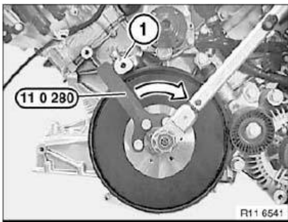
Fig. 139: Tightening Stress Bolts
