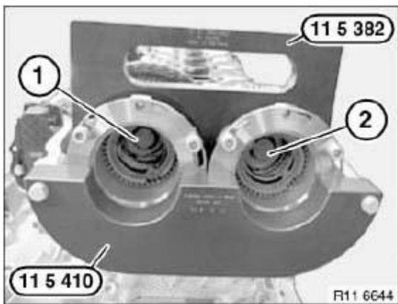
Fig. 339: Identifying Special Tool 11 5 382 And Central Bolts Courtesy of BMW OF NORTH AMERICA, INC.
