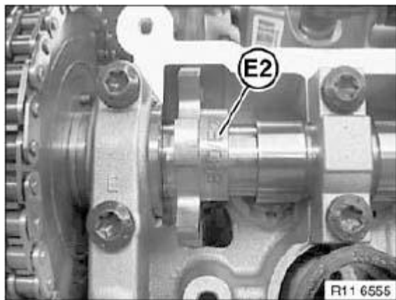
Fig. 323: Identifying Designation On Dihedron Points Upwards Courtesy of BMW OF NORTH AMERICA, INC.
