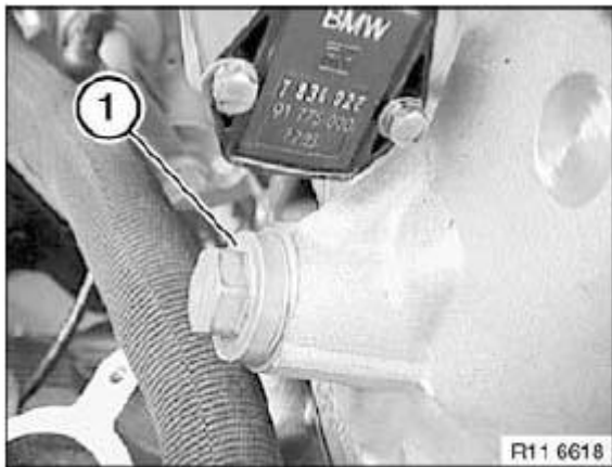
Fig. 338: Identifying Chain Tensioner Courtesy of BMW OF NORTH AMERICA, INC.
