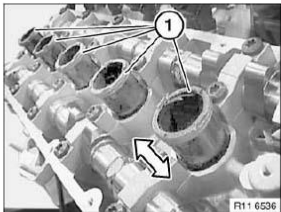
Fig. 38: Removing Spark Plug Tube Courtesy of BMW OF NORTH AMERICA, INC.
