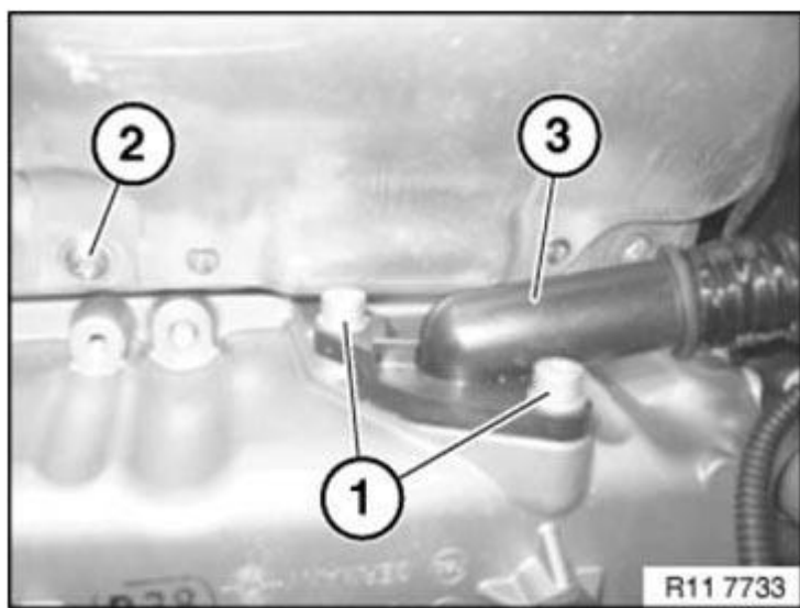
Fig. 470: Identifying Screws And Heat Shield Courtesy of BMW OF NORTH AMERICA, INC.
