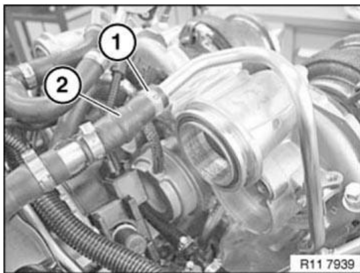
Fig. 479: Identifying Coolant Feed Line And Hose Clamp Courtesy of BMW OF NORTH AMERICA, INC.
