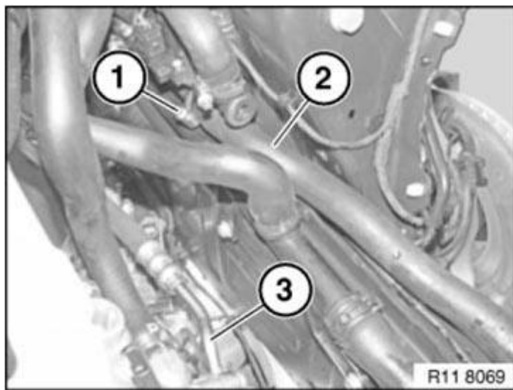
Fig. 27: Identifying Hose Clip And Coolant Hose Courtesy of BMW OF NORTH AMERICA, INC.
