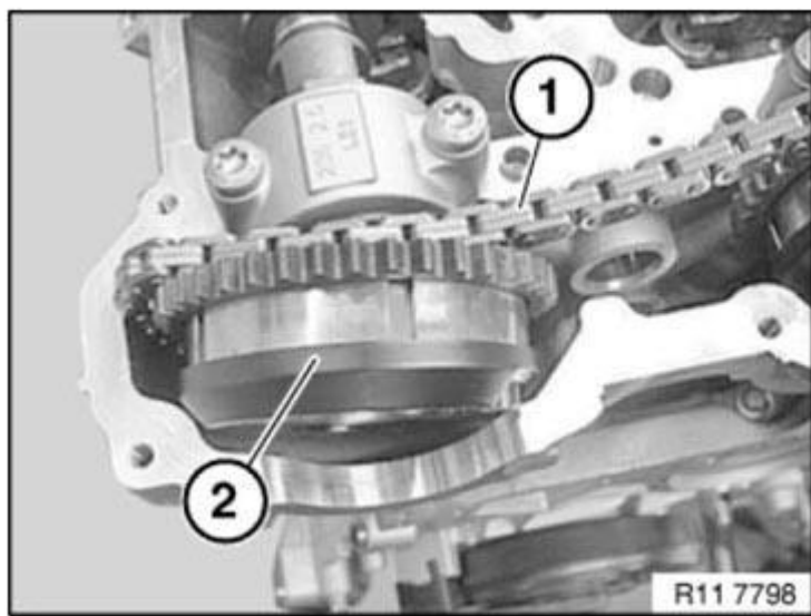
Fig. 383: Identifying Exhaust Adjustment Unit And Timing Chain Courtesy of BMW OF NORTH AMERICA, INC.
