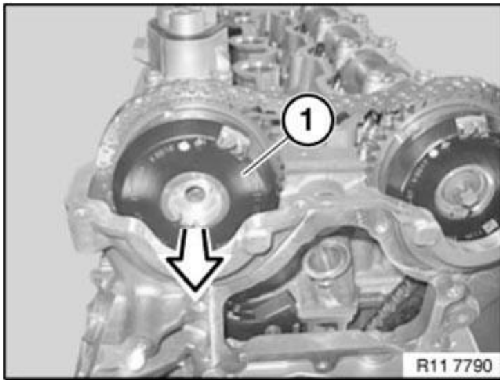
Fig. 352: Identifying Exhaust Adjustment Unit Courtesy of BMW OF NORTH AMERICA, INC.
