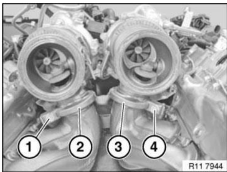
Fig. 501: Identifying V-Band Clamp With Mounting Screws Courtesy of BMW OF NORTH AMERICA, INC.
