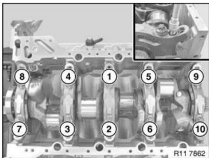
Fig. 122: Identifying Collar Bolts (M8) Releasing Sequence Courtesy of BMW OF NORTH AMERICA, INC.
