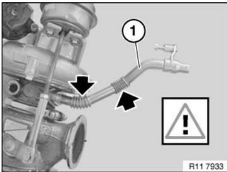
Fig. 485: Identifying Thermal Linear Compensators On Oil Return Pipe
