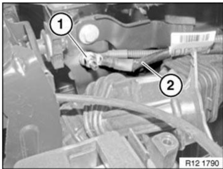
Fig. 21: Identifying Slacken Nut And Battery Earth Lead Courtesy of BMW OF NORTH AMERICA, INC.
