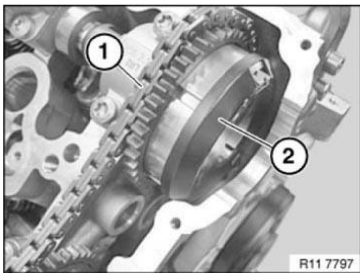
Fig. 380: Identifying Exhaust Adjustment Unit And Timing Chain Courtesy of BMW OF NORTH AMERICA, INC.
