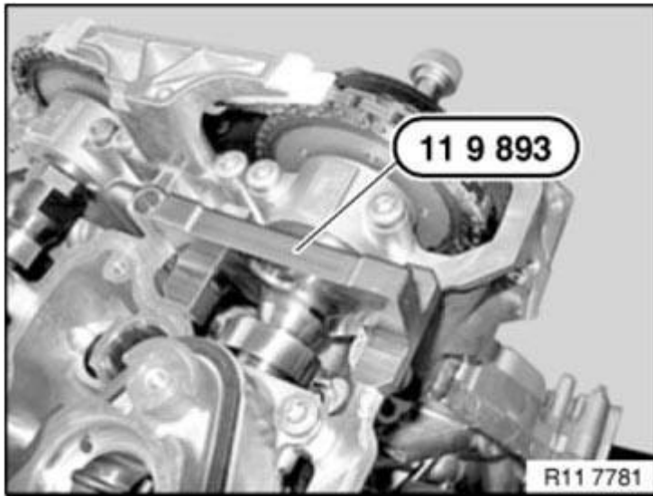
Fig. 201: Identifying Special Tool 11 9 893 On Exhaust Camshaft Courtesy of BMW OF NORTH AMERICA, INC.
