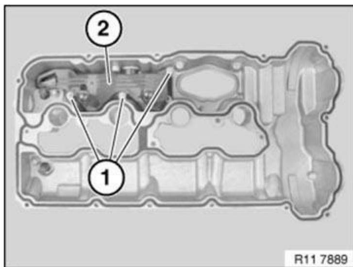
Fig. 75: Identifying Profile Seal Of Cylinder Head Cover Courtesy of BMW OF NORTH AMERICA, INC.
