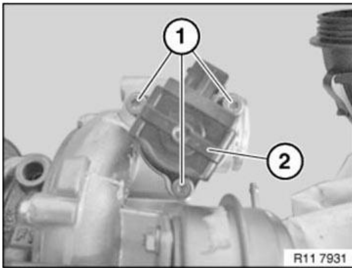
Fig. 463: Identifying Electric Changeover Valve And Screws Courtesy of BMW OF NORTH AMERICA, INC.
