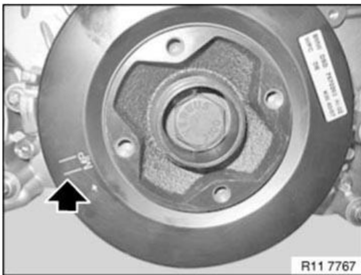
Fig. 221: Identifying Mounting Position Of Special Tool 11 8 570 Courtesy of BMW OF NORTH AMERICA, INC.
