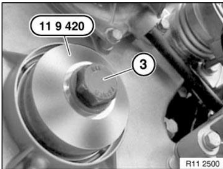
Fig. 104: Identifying Special Tool And Central Bolt Courtesy of BMW OF NORTH AMERICA, INC.
