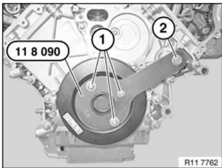
Fig. 146: Securing Special Tool 11 8 090 With Belt Tensioner Bolt To Timing Case Cover
