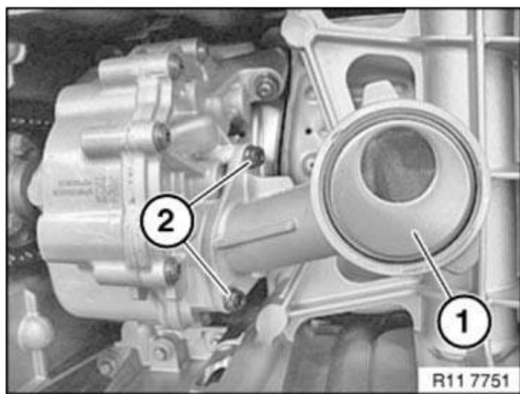
Fig. 400: Identifying Intake Pipe And Screws Courtesy of BMW OF NORTH AMERICA, INC.
