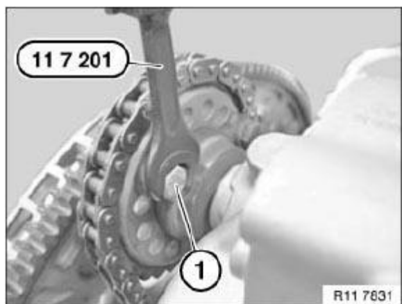
Fig. 421: Removing Oil Pump Sprocket Wheel Nuts Courtesy of BMW OF NORTH AMERICA, INC.
