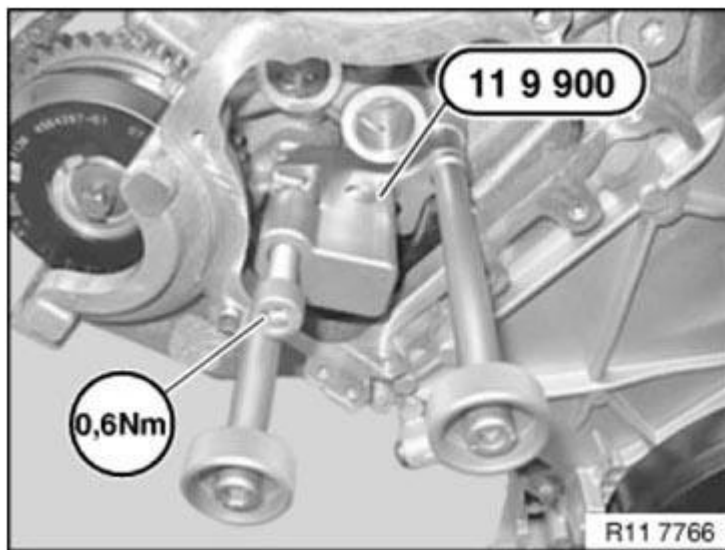
Fig. 321: Preloading Hexagon Socket Screw With Special Tool 00 9 250 To 0.6 Nm Courtesy of BMW OF NORTH AMERICA, INC.
