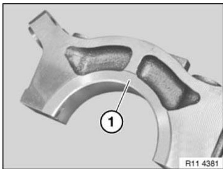
Fig. 110: Identifying Main Bearing Cap Thrust Washers Surfaces Courtesy of BMW OF NORTH AMERICA, INC.
