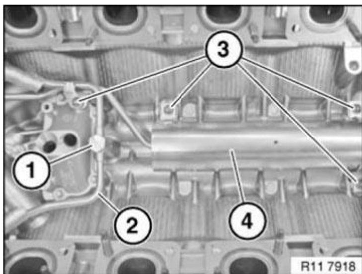
Fig. 436: Identifying Banjo Bolt, Screws And Vacuum Reservoir Courtesy of BMW OF NORTH AMERICA, INC.
