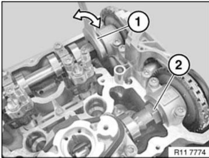
Fig. 258: Rotating Exhaust Camshaft At Dihedron With Fork Wrench Into Suitable Position Courtesy of BMW OF NORTH AMERICA, INC.
