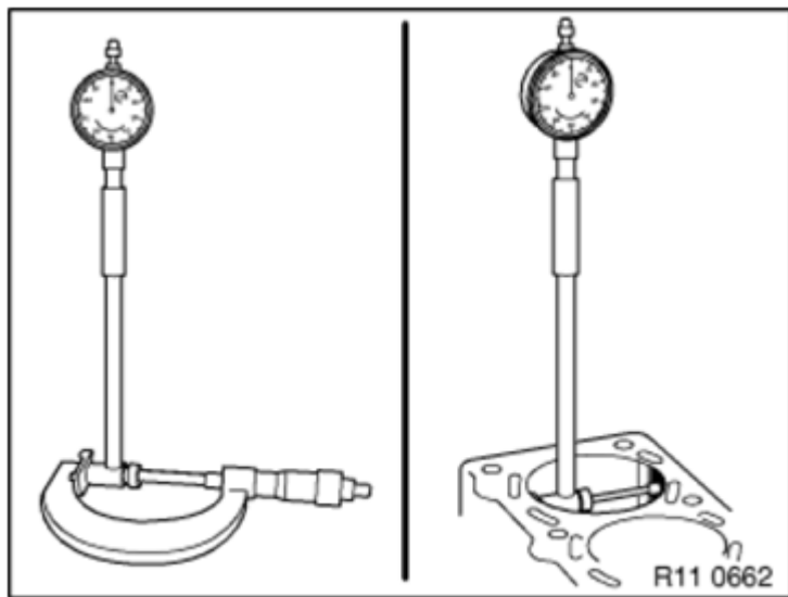
Fig. 179: Checking Diameter Of Cylinder Bore Courtesy of BMW OF NORTH AMERICA, INC.
