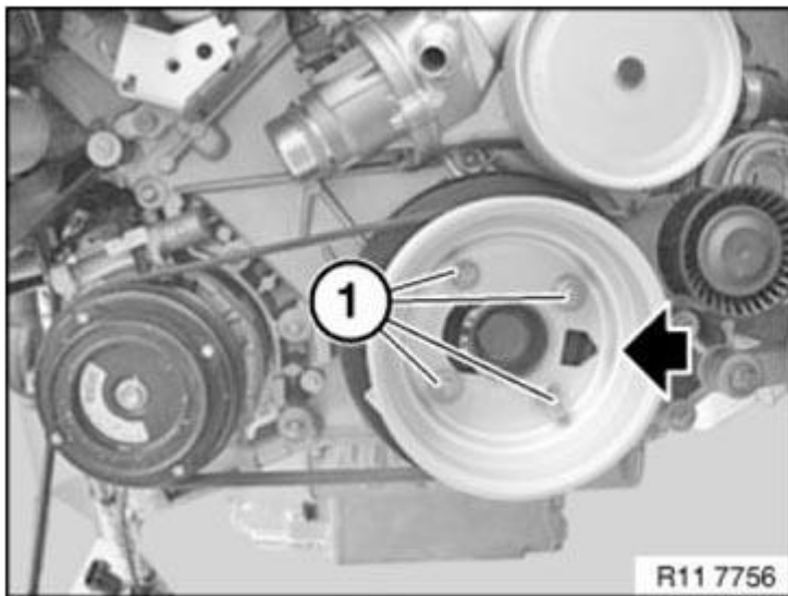
Fig. 189: Identifying Crank Pulley Screws And Marking Courtesy of BMW OF NORTH AMERICA, INC.
