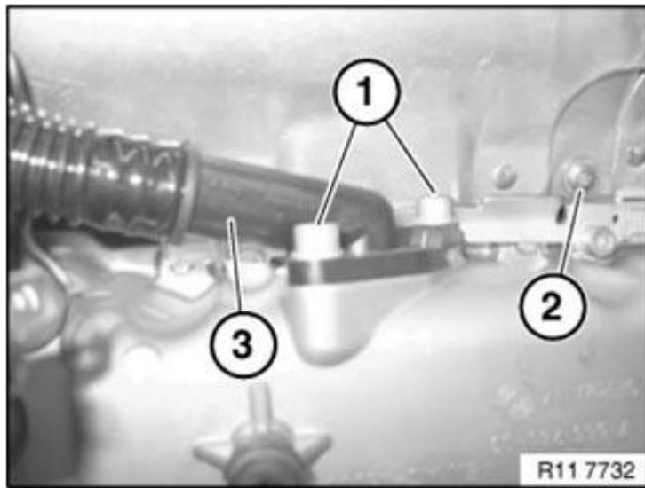
Fig. 469: Identifying Screws And Heat Shield Courtesy of BMW OF NORTH AMERICA, INC.
