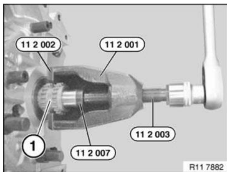
Fig. 280: Removing Sprocket Wheel With Special Tool 11 2 003 Courtesy of BMW OF NORTH AMERICA, INC.
