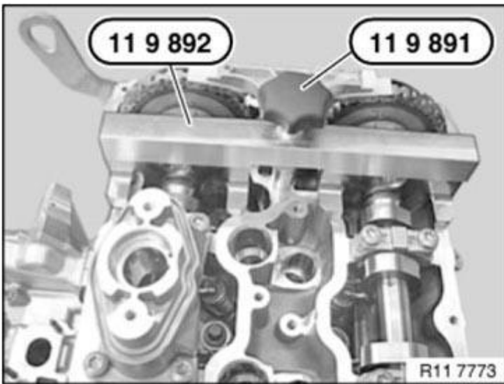
Fig. 392: Positioning Special Tool 11 9 892 On Special Tool 11 9 893 Courtesy of BMW OF NORTH AMERICA, INC.
