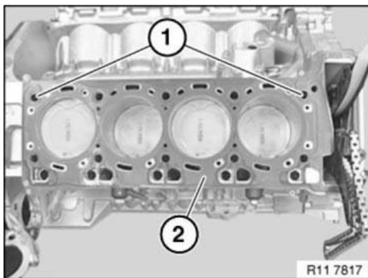
Fig. 78: Identifying Fitting Sleeves And Cylinder Head Gasket Courtesy of BMW OF NORTH AMERICA, INC.
