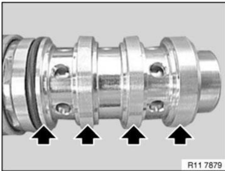
Fig. 341: Inspecting Notches Or Scratches For Solenoid Valve Housing Courtesy of BMW OF NORTH AMERICA, INC.
