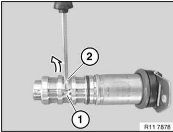
Fig. 370: Bending Open Welding Spots On Filter Element With Screwdriver Courtesy of BMW OF NORTH AMERICA, INC.
