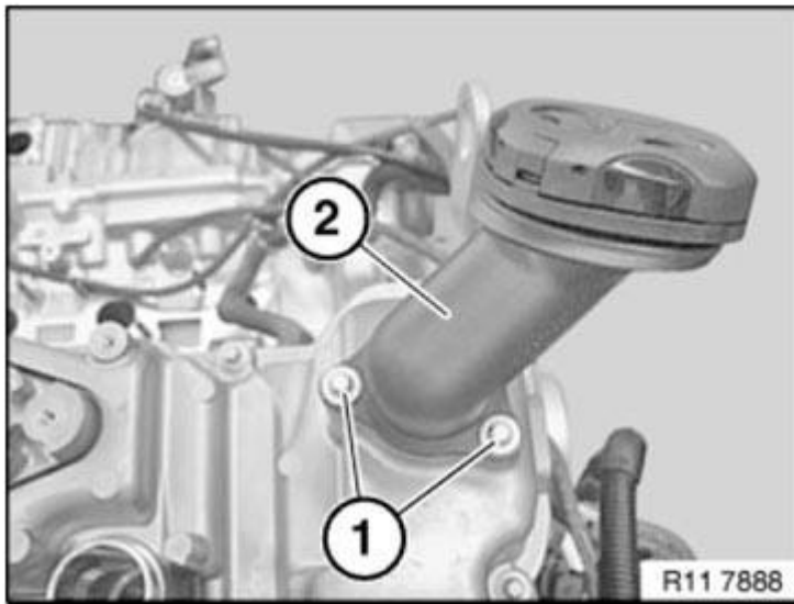
Fig. 72: Identifying Oil Filler Neck And Screws Courtesy of BMW OF NORTH AMERICA, INC.
