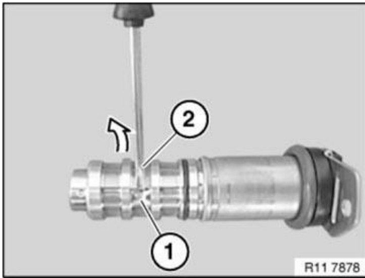
Fig. 340: Bending Open Welding Spots On Filter Element With Screwdriver Courtesy of BMW OF NORTH AMERICA, INC.
