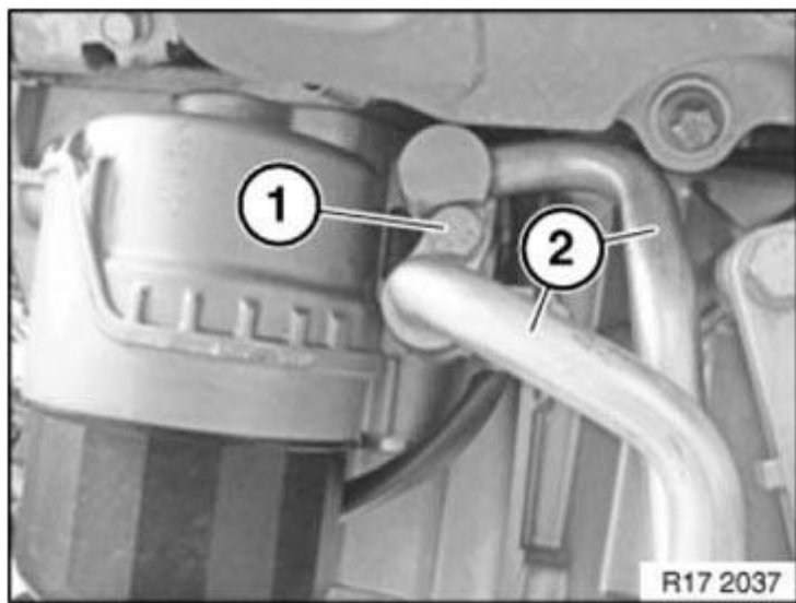
Fig. 29: Identifying Oil Pipes Screw Courtesy of BMW OF NORTH AMERICA, INC.
