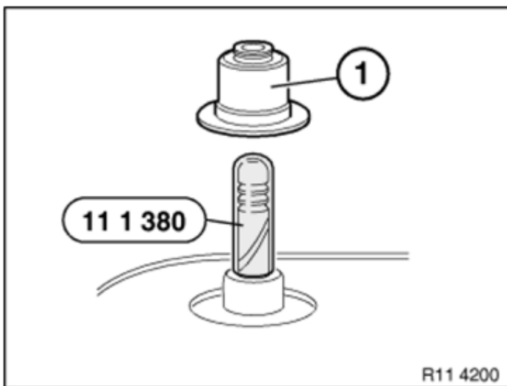
Fig. 300: Identifying Valve Stem Seal And Special Tool 11 6 380 Courtesy of BMW OF NORTH AMERICA, INC.
