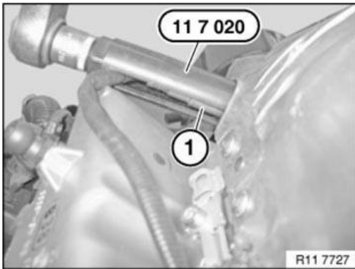
Fig. 535: Releasing Monitoring Sensor Using Special Tool 11 7 020 Courtesy of BMW OF NORTH AMERICA, INC.
