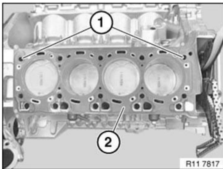
Fig. 63: Identifying Fitting Sleeves And Cylinder Head Gasket Courtesy of BMW OF NORTH AMERICA, INC.
