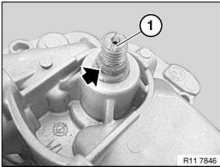
Fig. 411: Checking Mounting Flats On Pump Shaft For Damage Courtesy of BMW OF NORTH AMERICA, INC.
