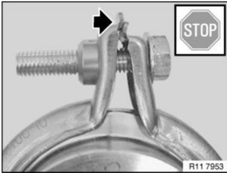
Fig. 514: Locating V-Band Clamp Position Courtesy of BMW OF NORTH AMERICA, INC.
